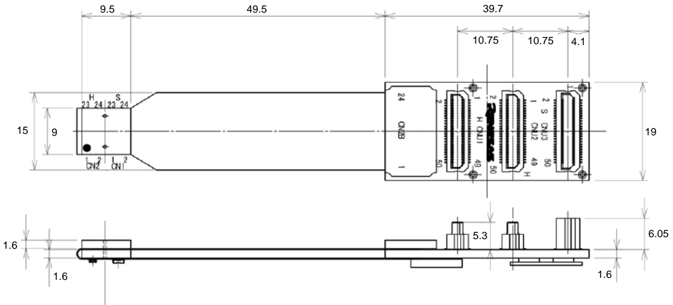
< Bottom view >
