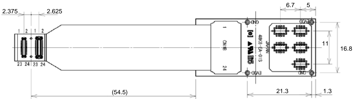
< Bottom view >
