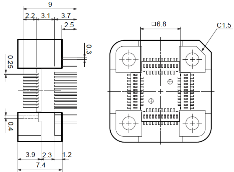
< Bottom view >
