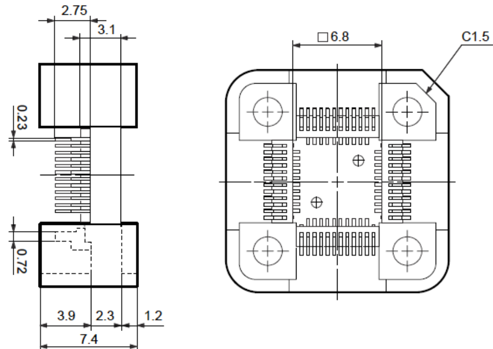
< Bottom view >
