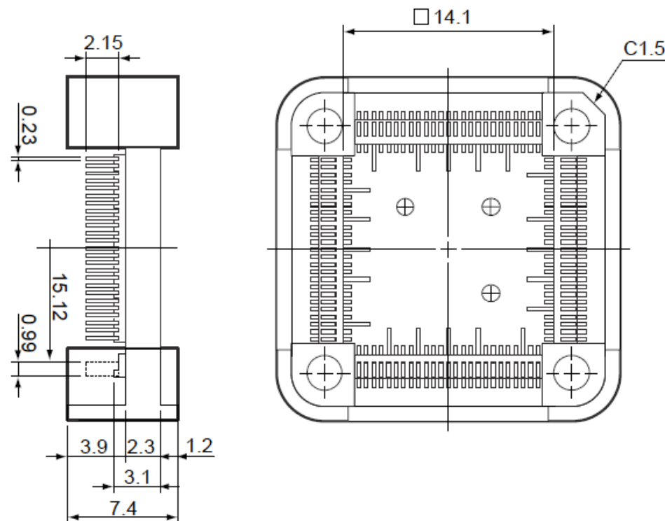
< Bottom view >
