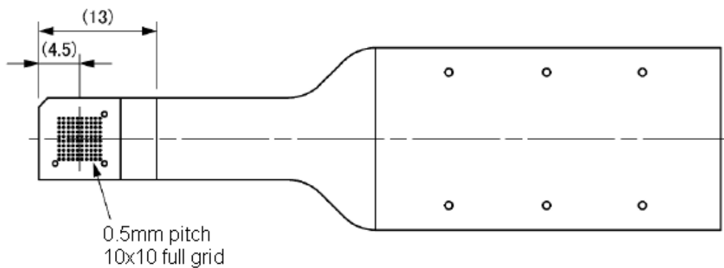
< Bottom view >
