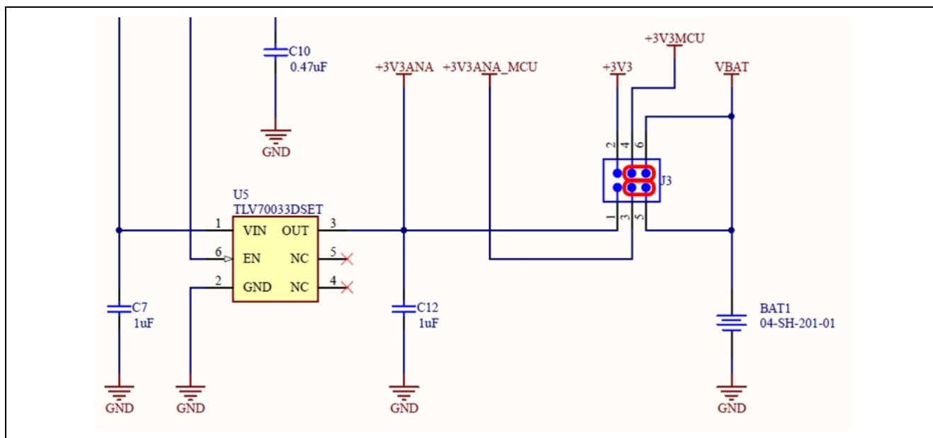
Figure 10. Battery Current Measurement
