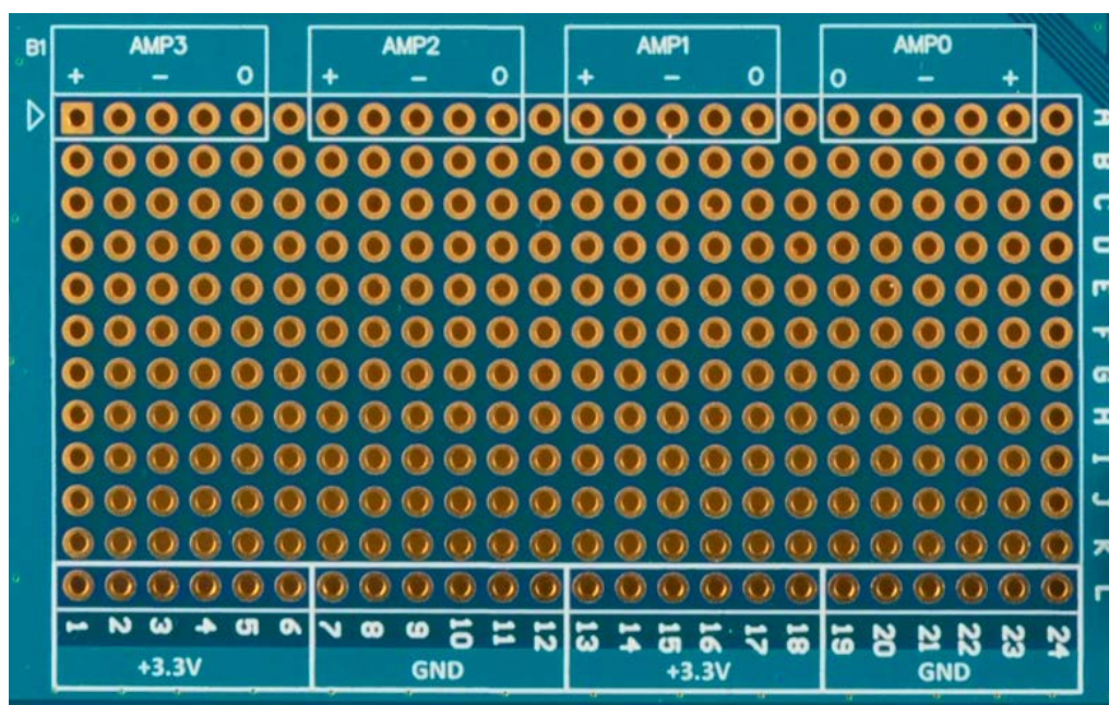
Figure 25. Breadboard Area
