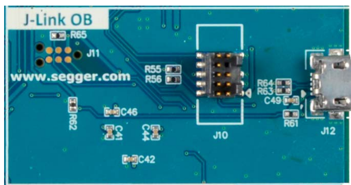
Figure 14. J-Link OB USB Programming and Debug
