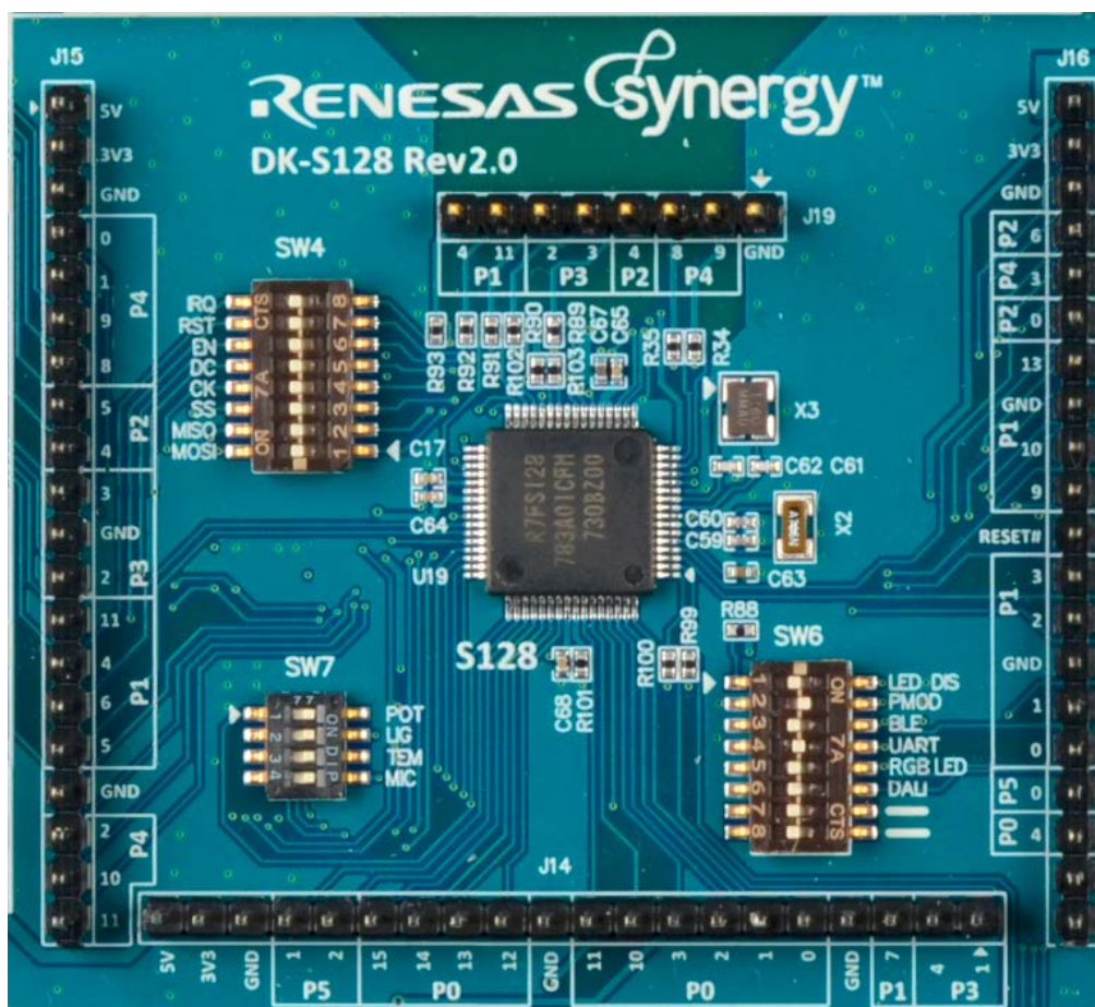
Figure 26. MCU Breakout Pin Headers
