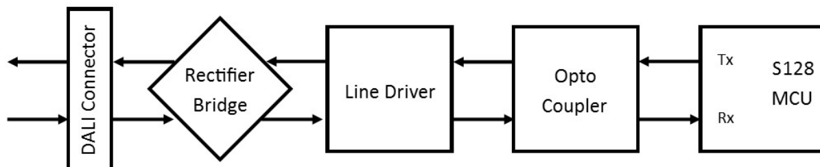
Figure 22. DALI Interface Circuit Block Diagram
