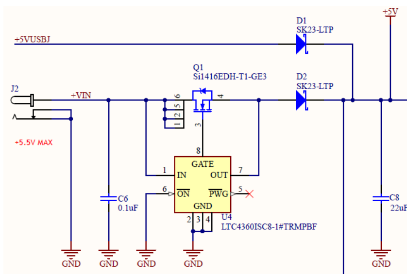
Figure 8. Main Input Power Schematic
