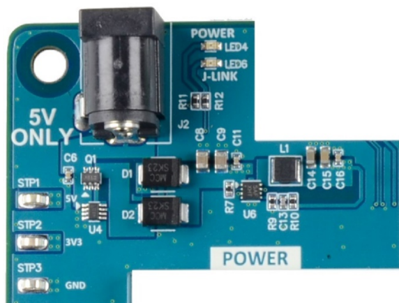
Figure 7. Input Power Section
