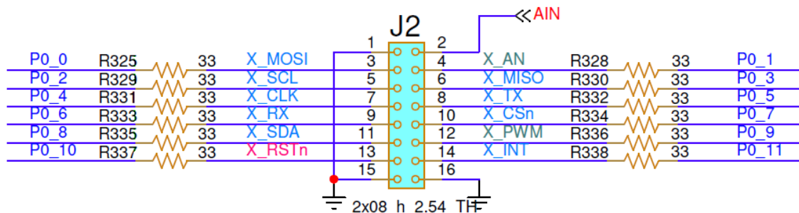
Figure 49. J2 schematic
