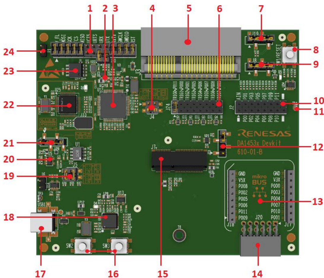
Figure 14. Pro-motherboard (610-01-A)
