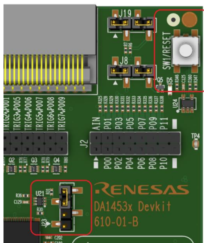
Figure 30. Position of the SW1 and J23 header on the DA1453x Pro-motherboard
