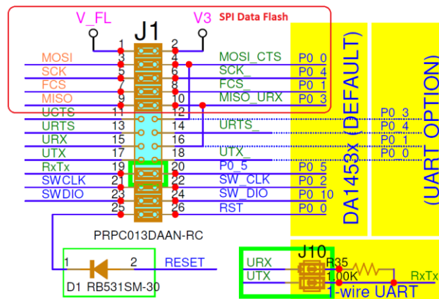
Figure 33. Jumper configuration at J1 header on Pro-motherboard
