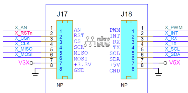
Figure 56. MikroBus slot
