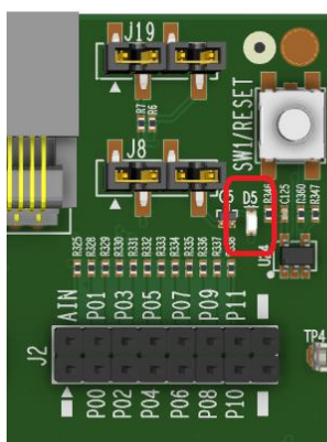
Figure 55. User LED position
