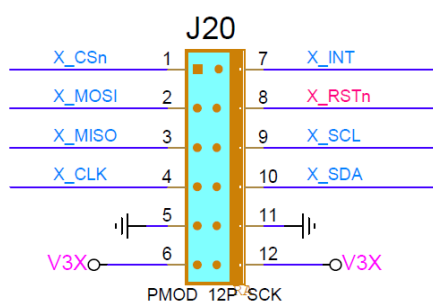
Figure 58. PMOD slot
