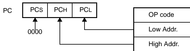
図4-18 CALL !addr16/BR !addr16 の例
