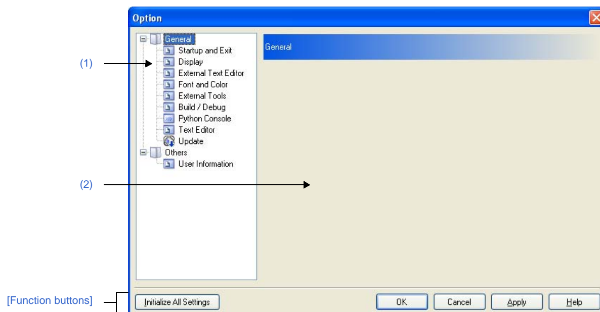
Figure A-44. Option Dialog Box
