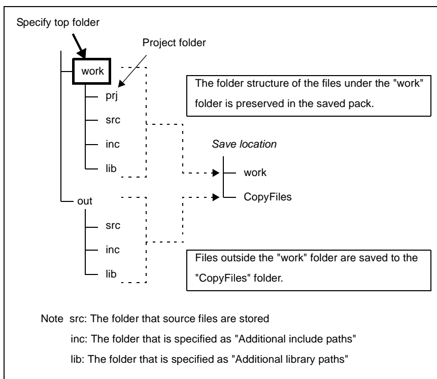
Figure 2-85. Sample of Project Pack
