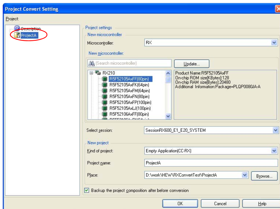
Figure 2-71. Project Convert Setting Dialog Box (When Project Is Selected)
