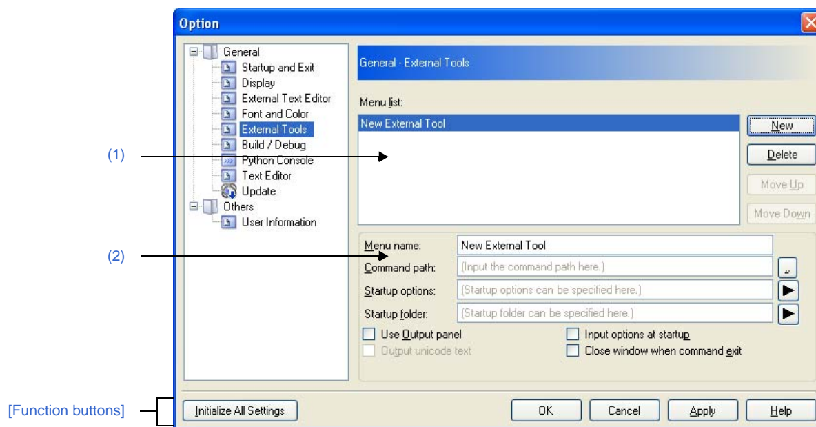
Figure A-51. Option Dialog Box ([General - External Tools] Category)
