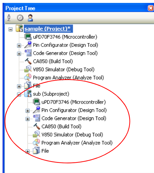
Figure 2-50. Project Tree Panel (After Adding a Subproject)
