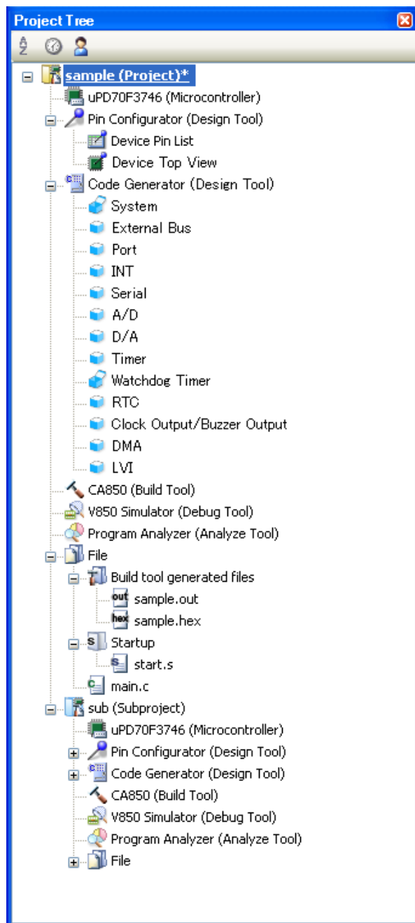
Figure 2-43. Project Tree Panel
