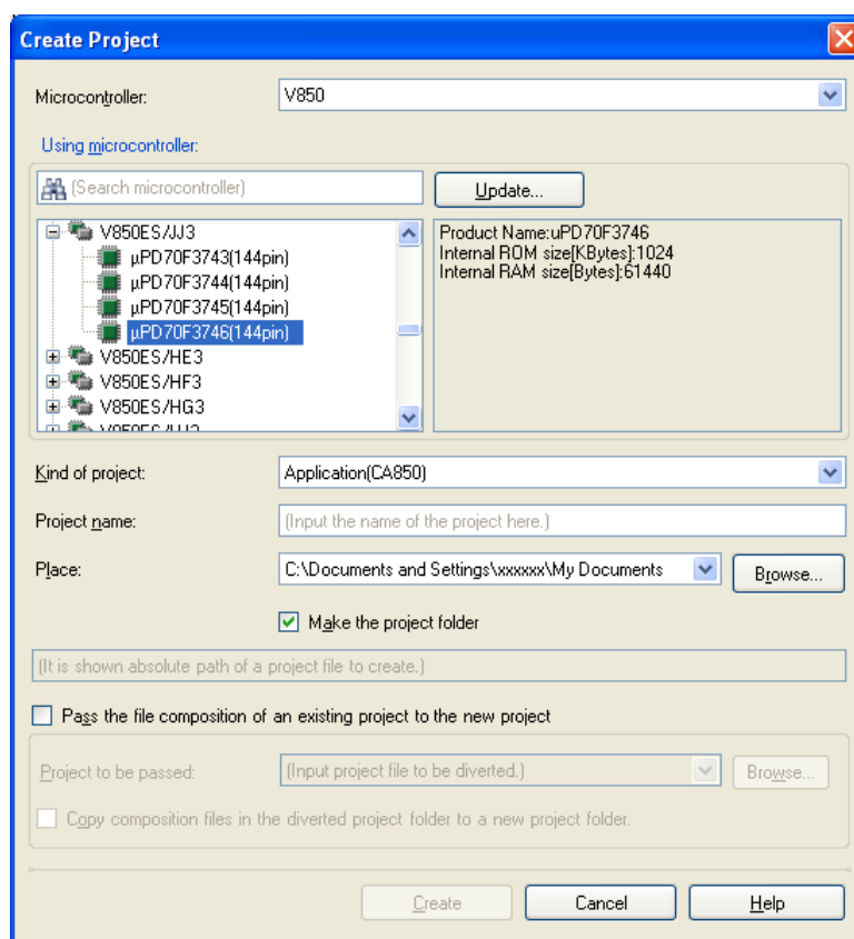
Figure 2-47. Create Project Dialog Box (After Setting Items)
