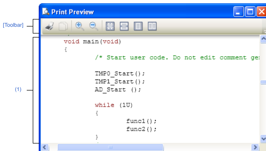
Figure A-38. Print Preview Window
