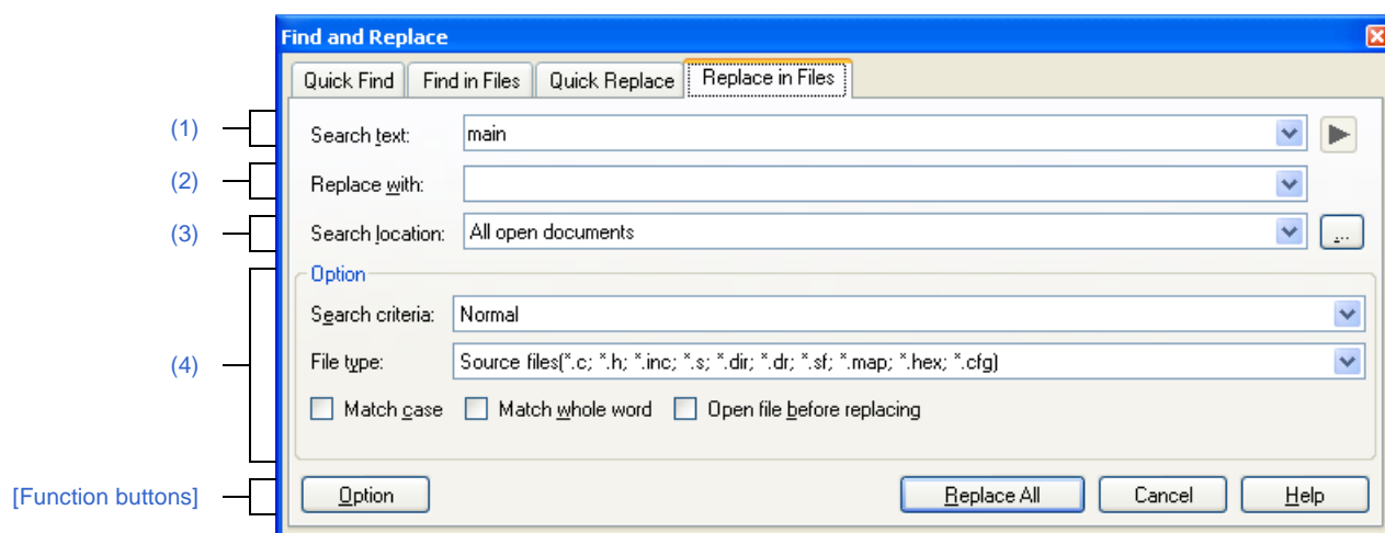
Figure A-36. Find and Replace Dialog Box: [Replace in Files] Tab
