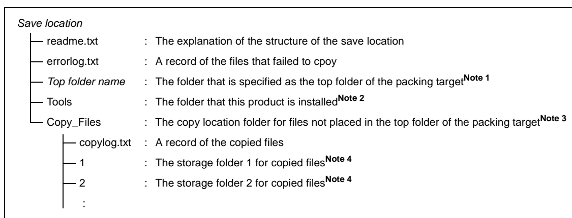
Figure 2-87. Save Location Folder Structure
