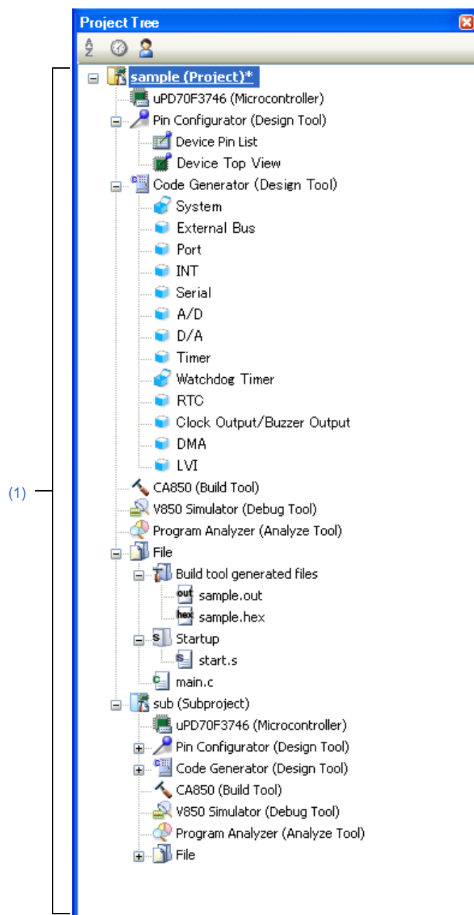
Figure A-19. Project Tree Panel
