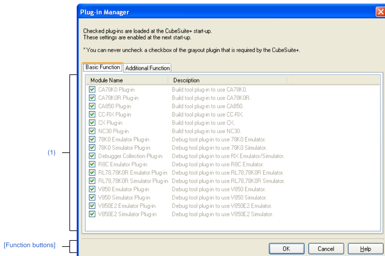
Figure A-58. Plug-in Manager Dialog Box: [Basic Function] Tab
