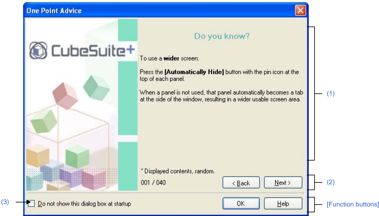
Figure A-70. One Point Advice Dialog Box
