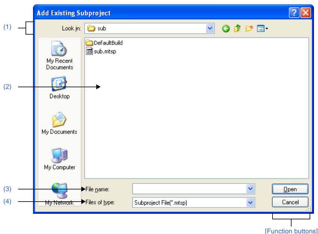
Figure A-74. Add Existing Subproject Dialog Box
