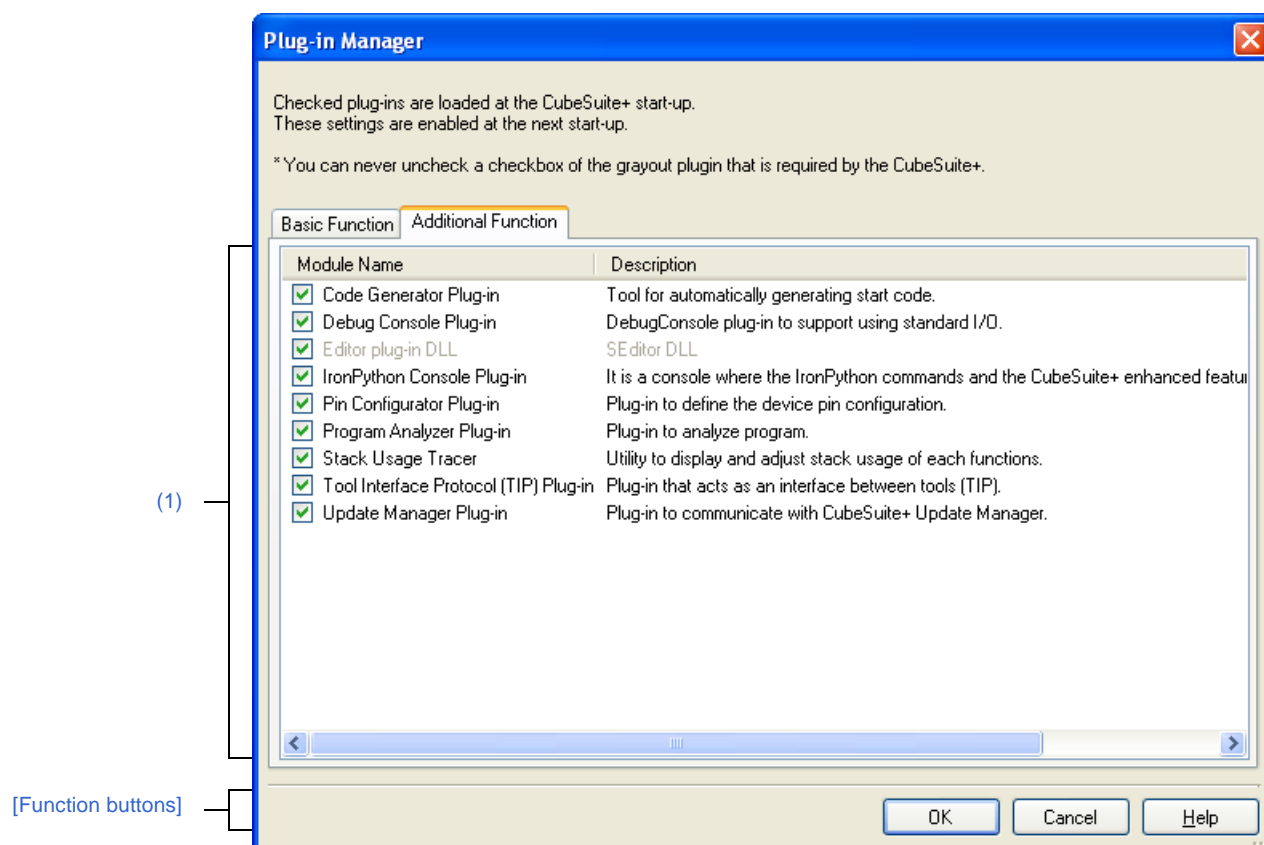
Figure A-59. Plug-in Manager Dialog Box: [Additional Function] Tab
