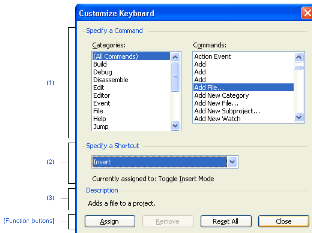
Figure A-65. Customize Keyboard Dialog Box
