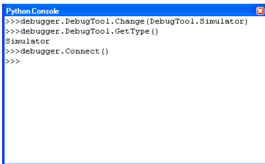
Figure 2-92. Python Console Panel
