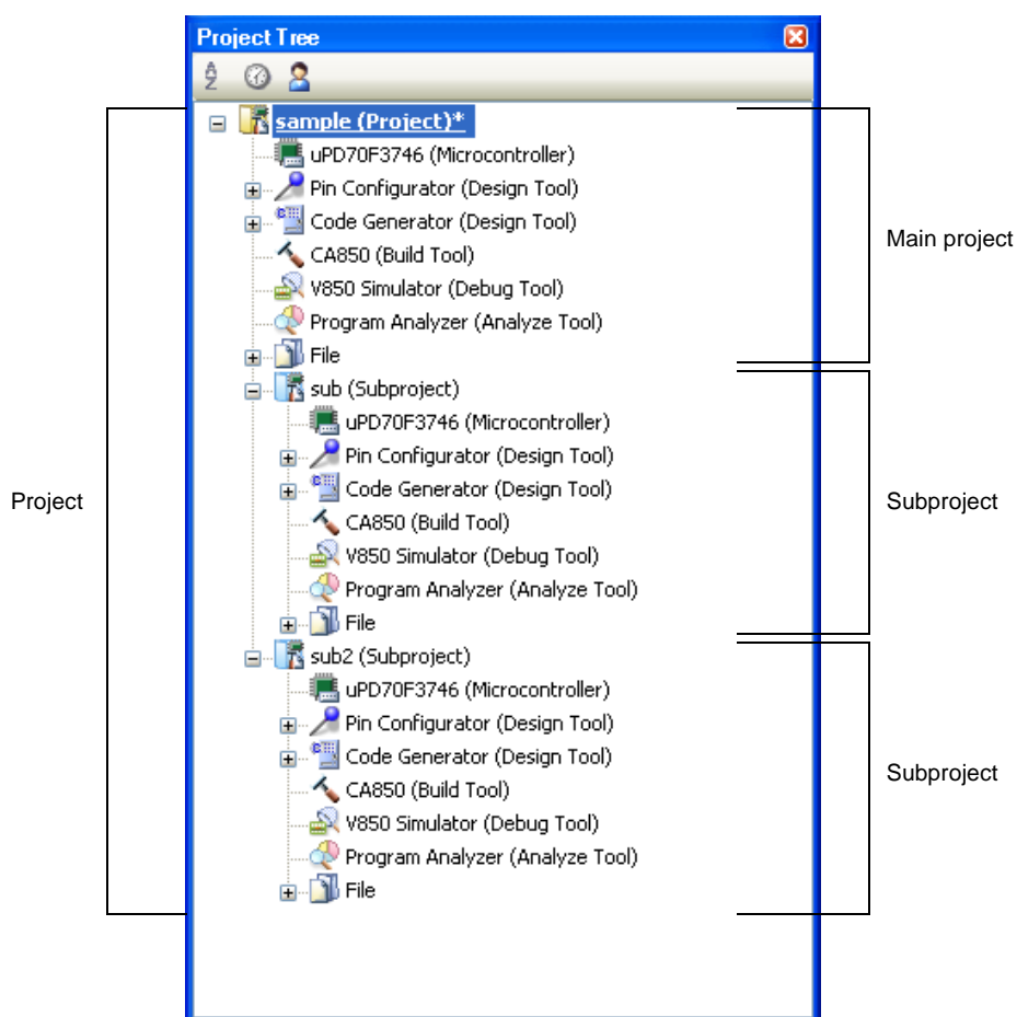
Figure 2-44. Project Tree Panel (When Subprojects Added)
