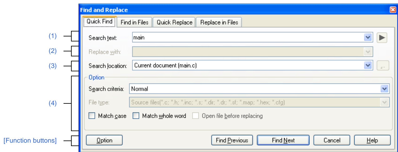
Figure A-33. Find and Replace Dialog Box: [Quick Find] Tab
