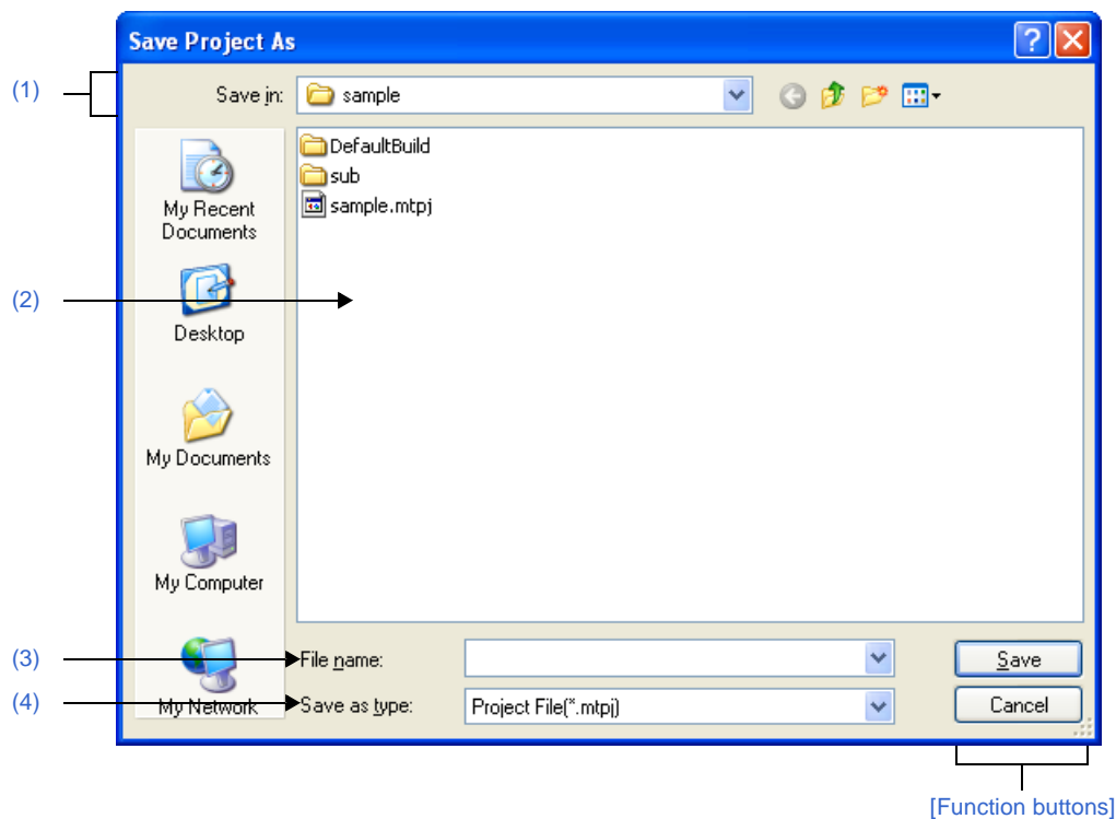
Figure A-76. Save Project As Dialog Box
