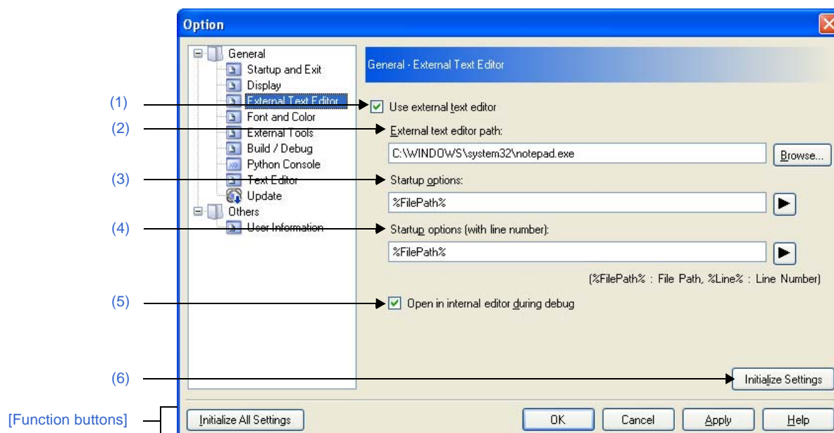
Figure A-47. Option Dialog Box ([General - External Text Editor] Category)
