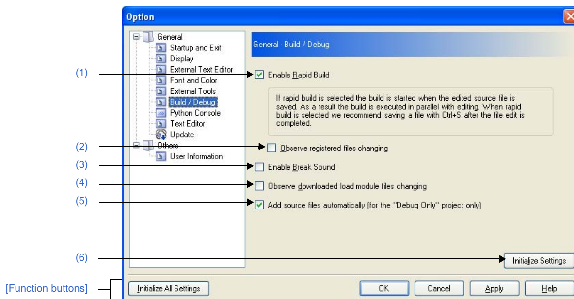
Figure A-52. Option Dialog Box ([General - Build/Debug] Category)
