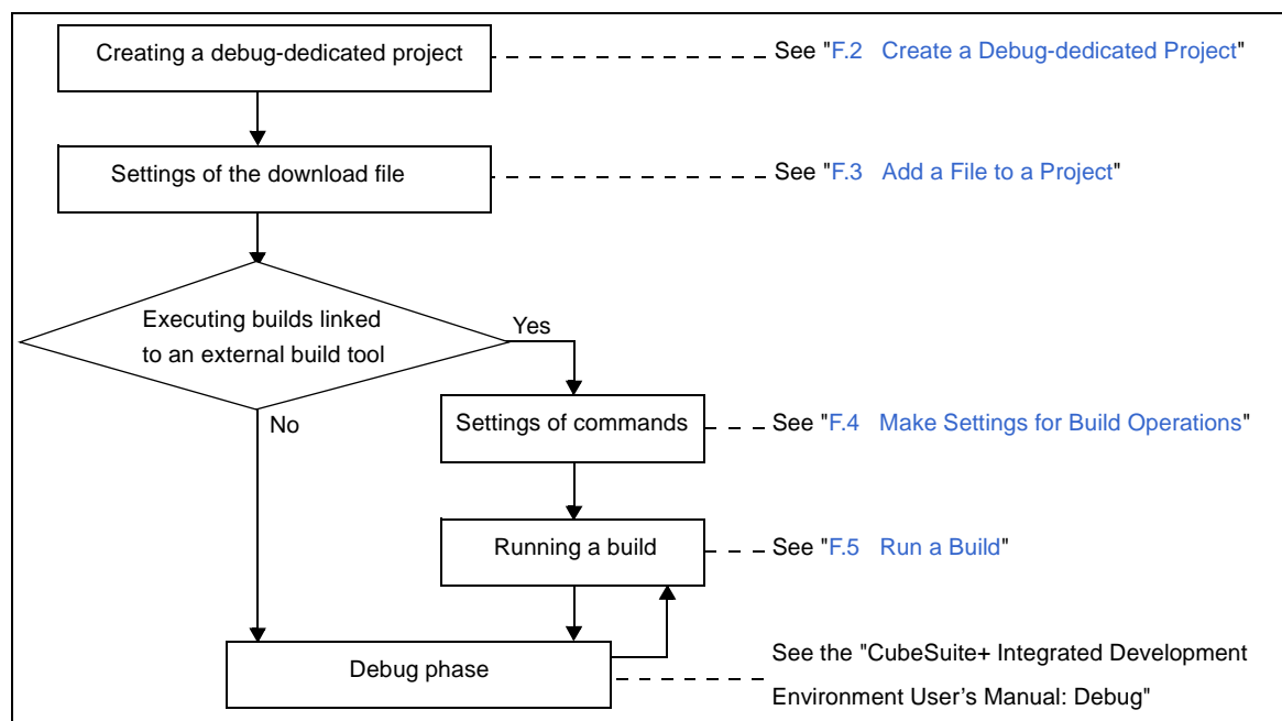
Figure F-1. Operational Sequence for Using a Debug-dedicated Project
