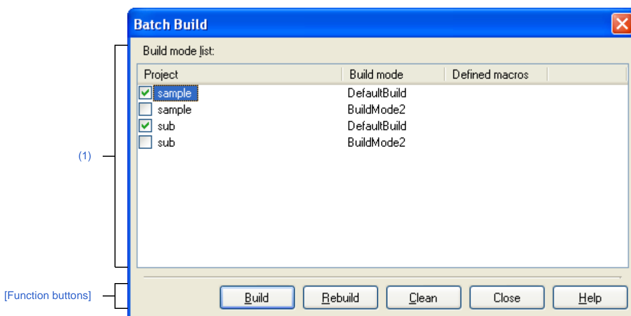
Figure A-41. Batch Build Dialog Box
