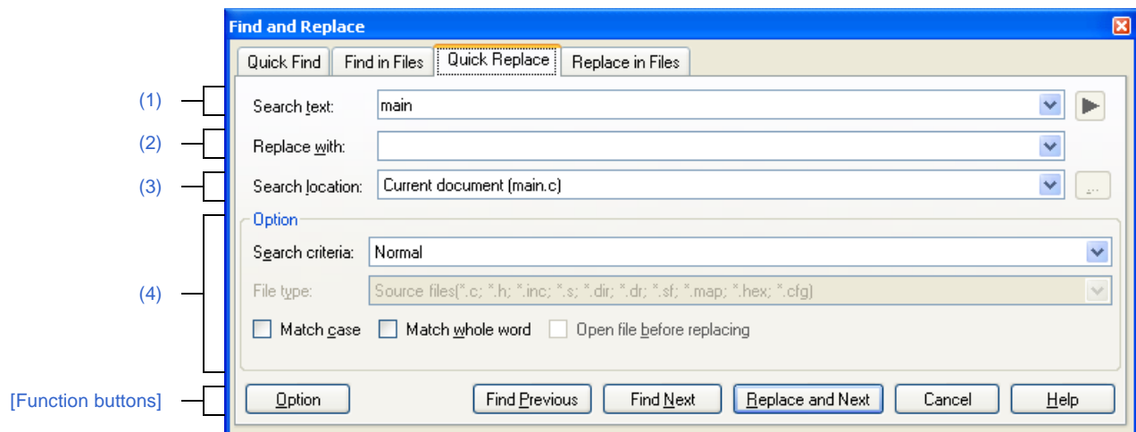
Figure A-35. Find and Replace Dialog Box: [Quick Replace] Tab
