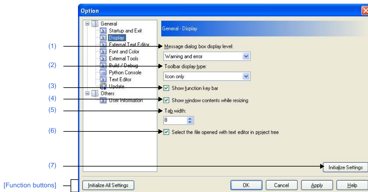
Figure A-46. Option Dialog Box ([General - Display] Category)
