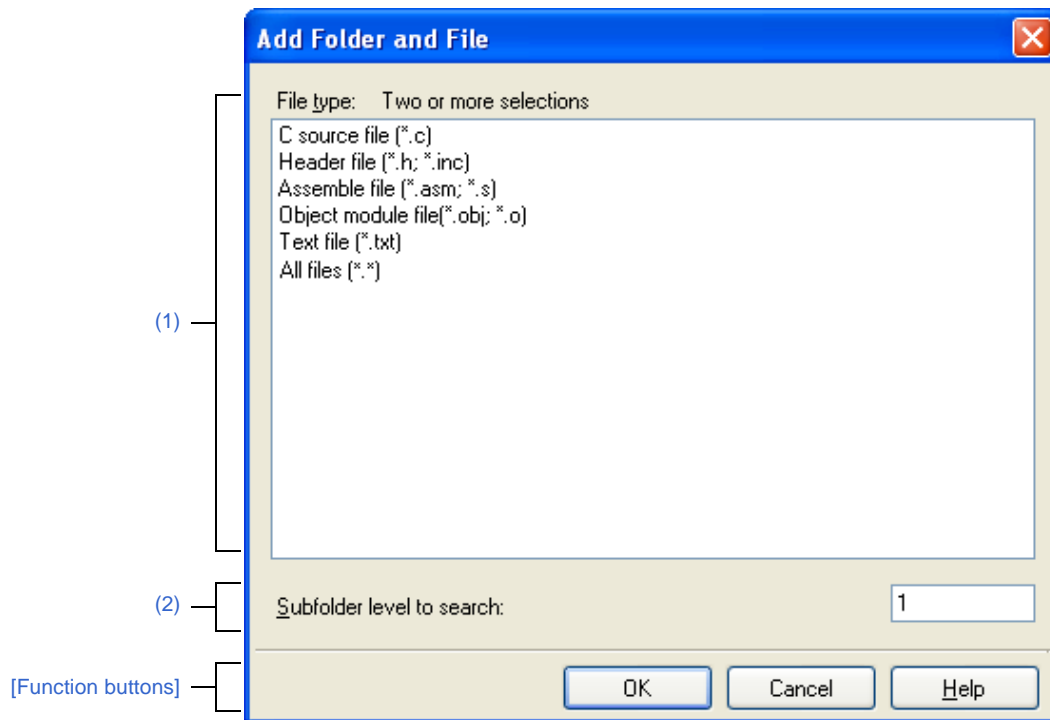
Figure A-28. Add Folder and File Dialog Box
