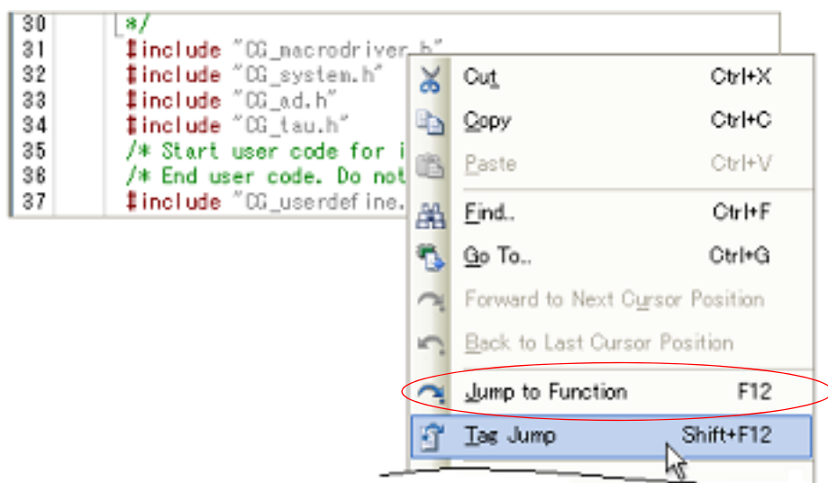
Figure 2.15 Tag Jump
