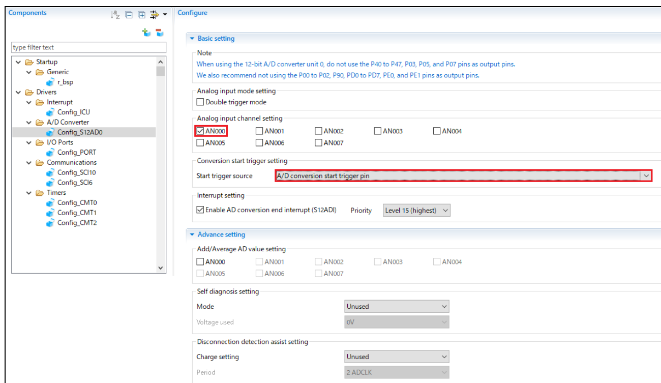
Figure 4-43 Config_S12AD0 setting (1)
