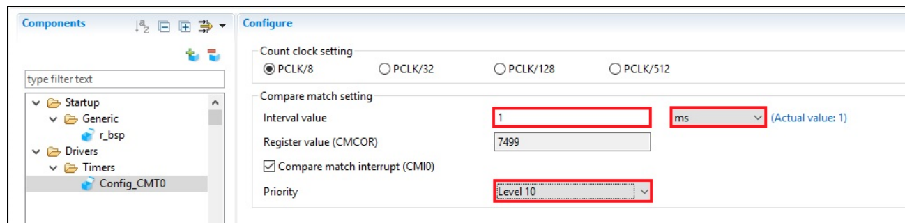
Figure 4-13 Config_CMT0 setting
