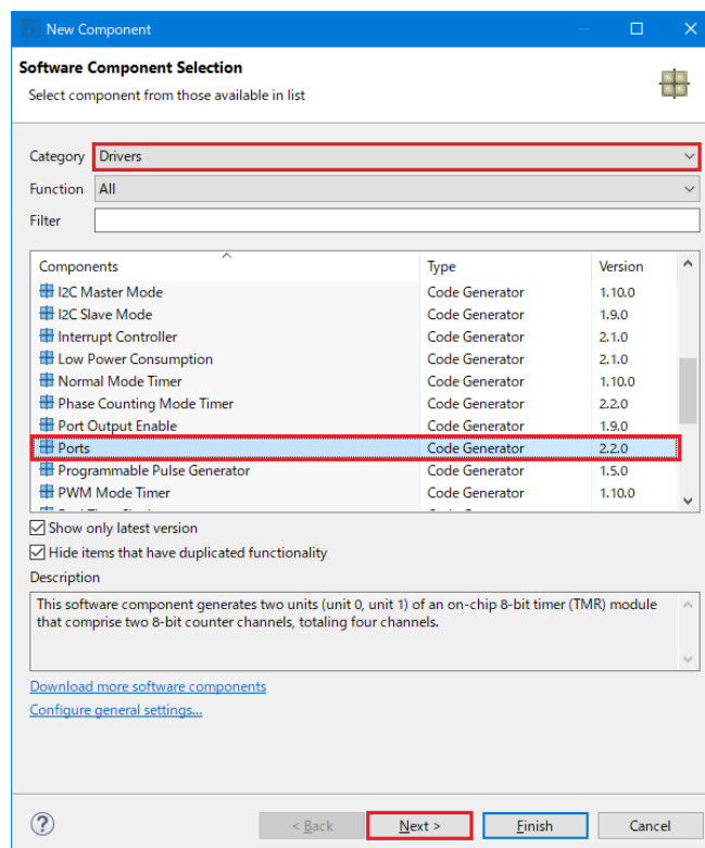
Figure 4-23 Select Ports
