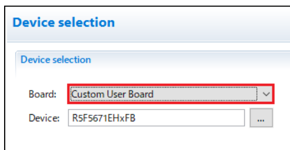
Figure 4-3 Select board
