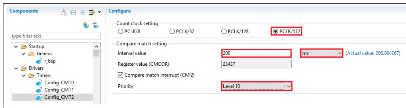
Figure 4-19 Config_CMT2 setting
