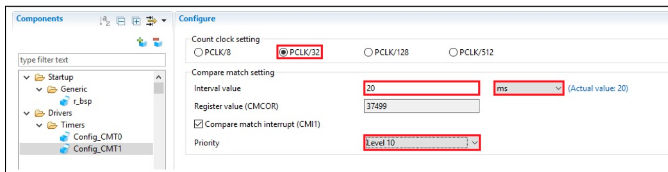
Figure 4-16 Config_CMT1 setting
