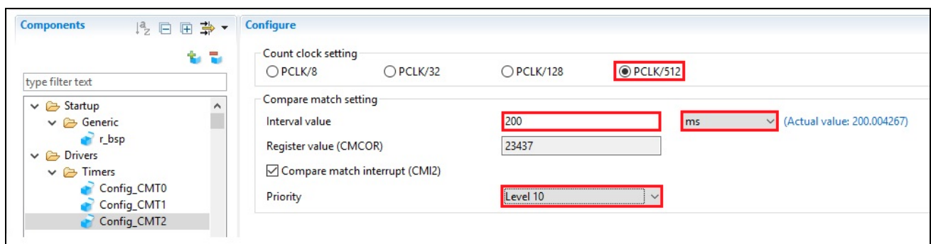
Figure 4-19 Config_CMT2 setting
