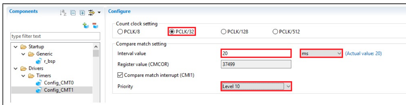
Figure 4-16 Config_CMT1 setting
