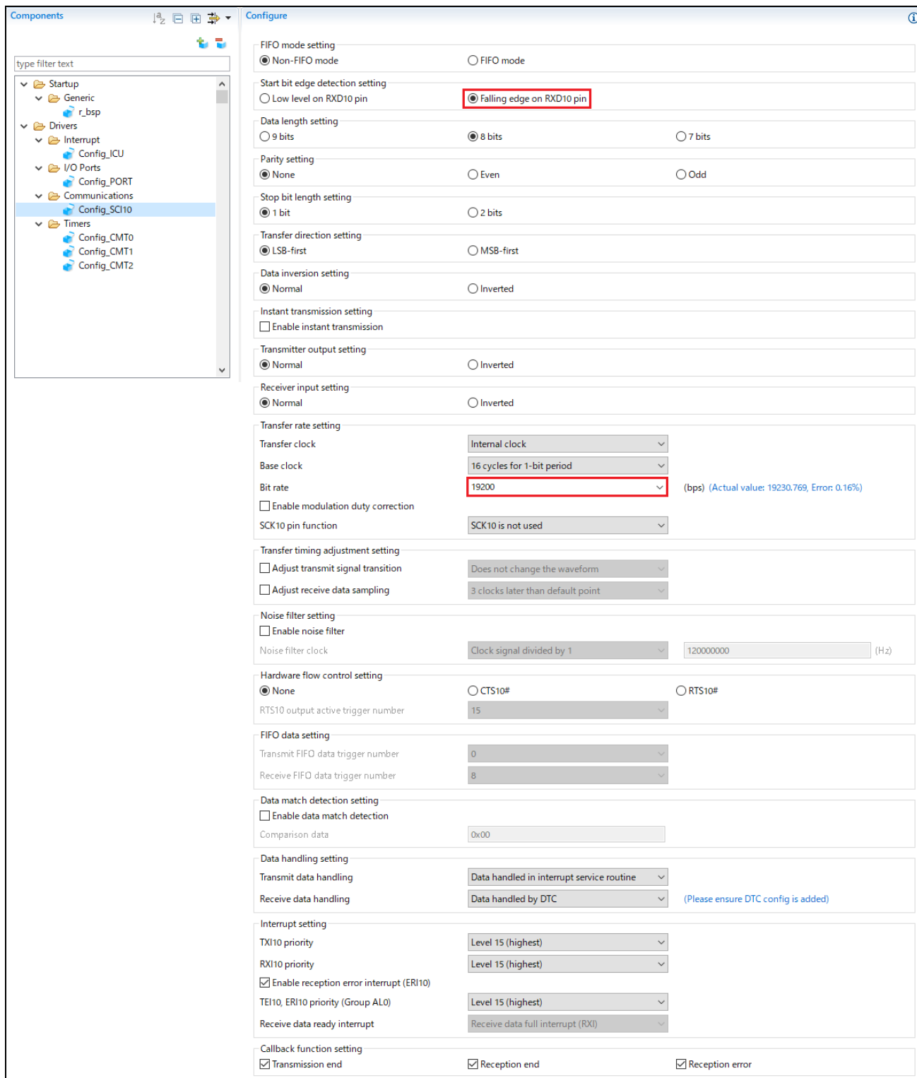
Figure 4-35 Config_SCI10 setting
