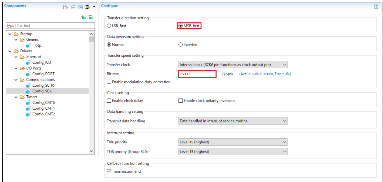
Figure 4-40 Config_SCI6 setting
