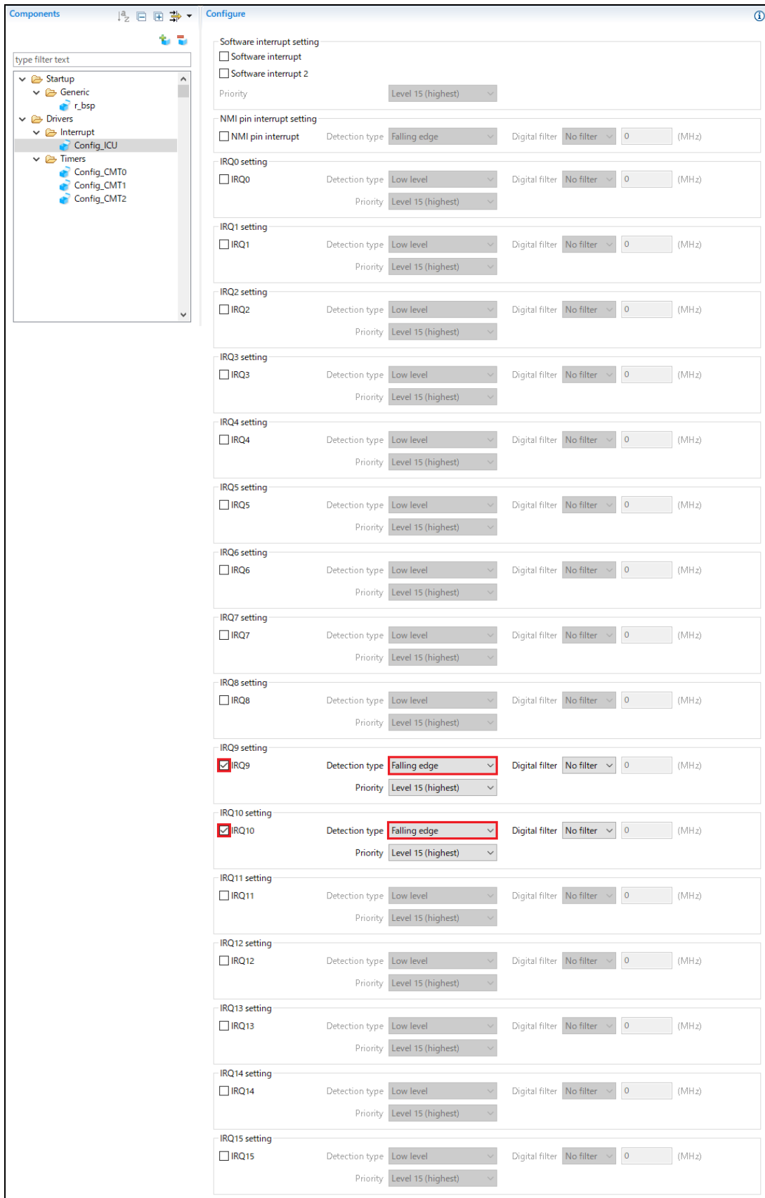
Figure 4-22 Config_ICU setting
