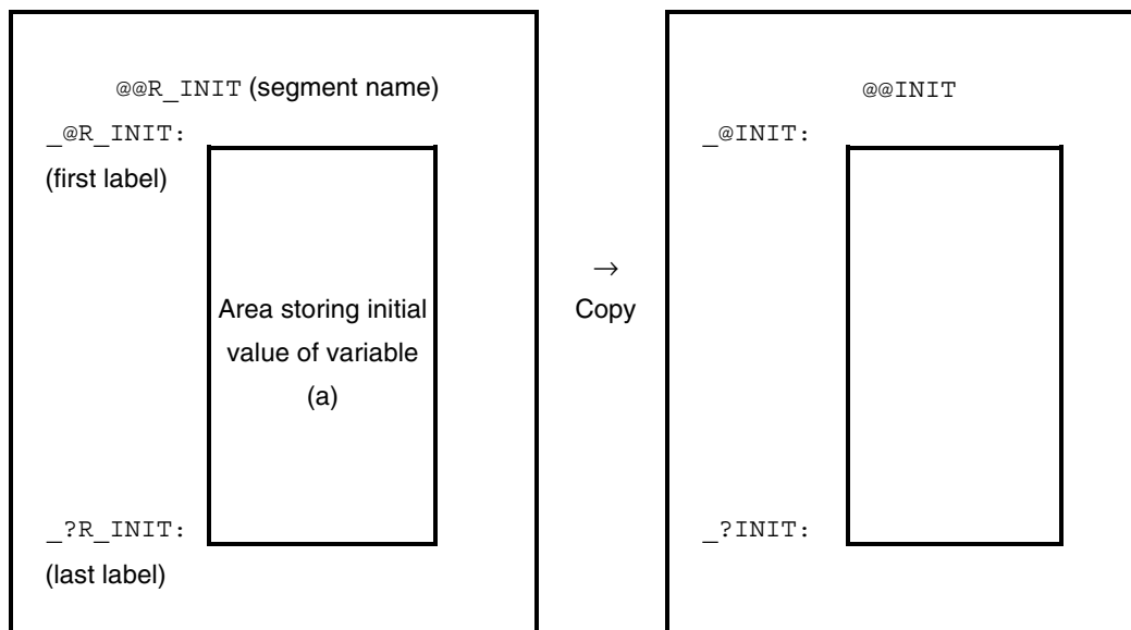
Figure 8-1. ROMization Processing
