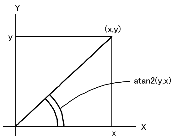
Figure 7.1 Meaning of atan2 Function
