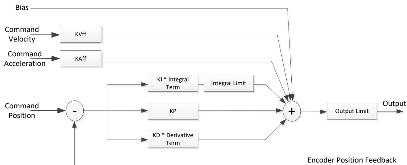
Figure 8 PID Regulator Structure
