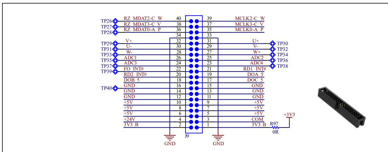
Figure 3-19 Inverter Board Interface
