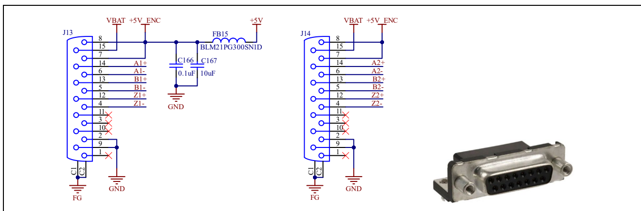
Figure 3-11 Encoder Interface
