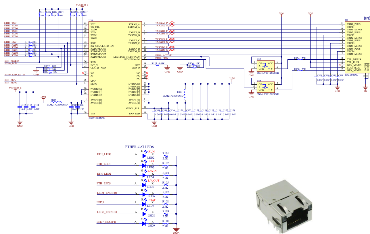
Figure 3-14 EtherCAT Interface
