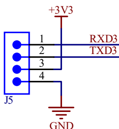
Figure 3-13 UART Interface
