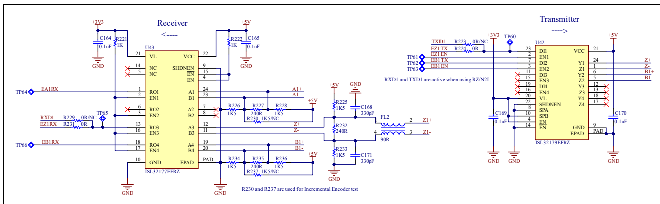
Figure 3-11 Encoder Interface
