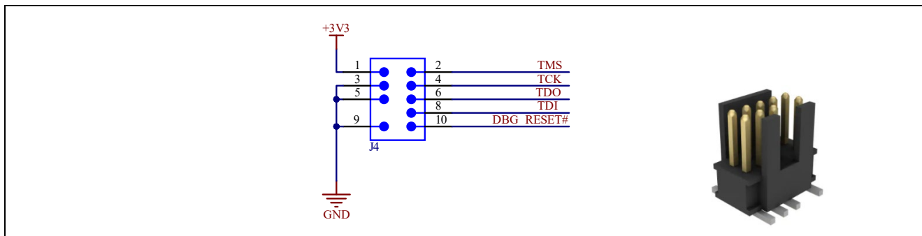
Figure 3-4 JTAG Interface
