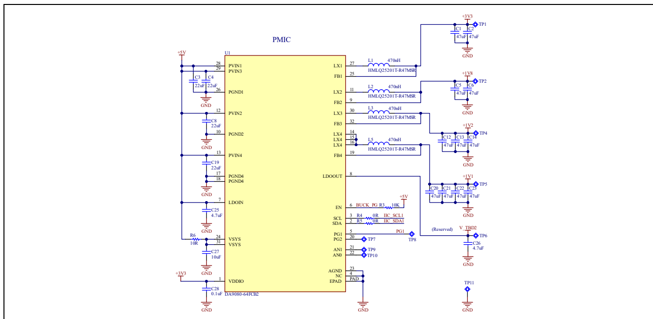
Figure 3-1 PMIC
