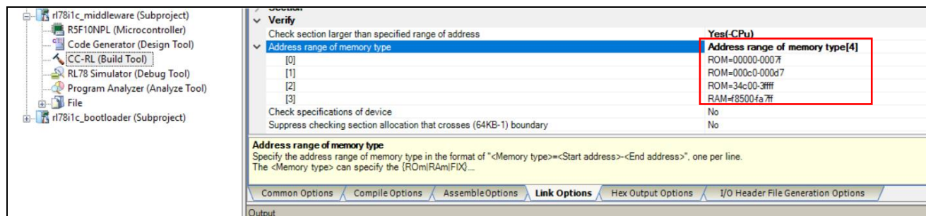
Figure 4-9 : Middleware - Address Range of Memory Type (CS+)
