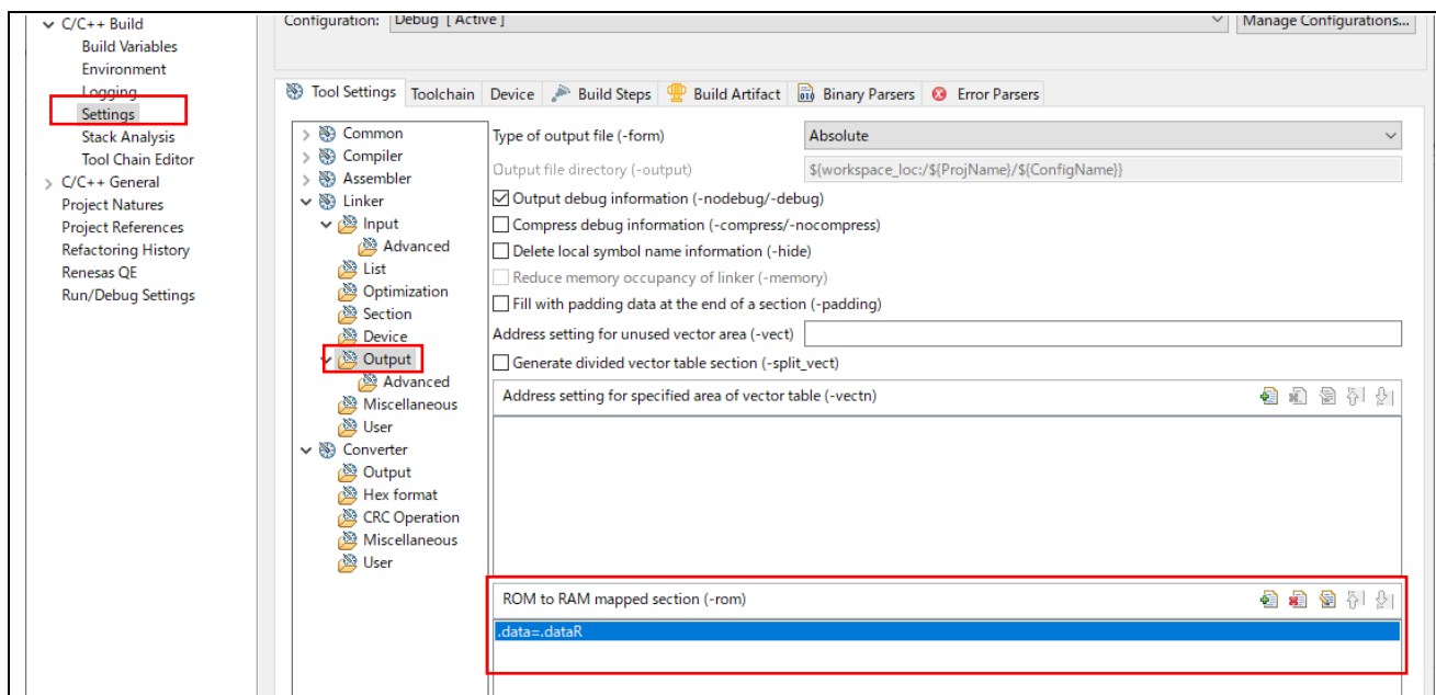
Figure 4-23 : User Application - ROM to RAM Mapped Section (e 2 studio)
