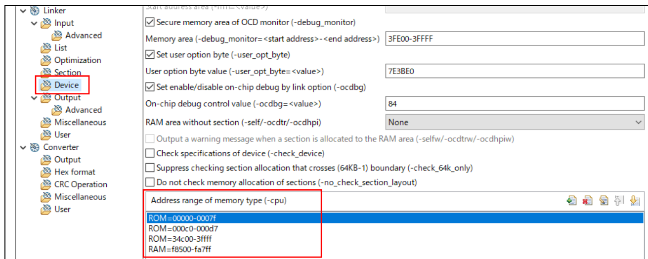
Figure 4-10 : Middleware - Address Range of Memory Type (e2studio)
