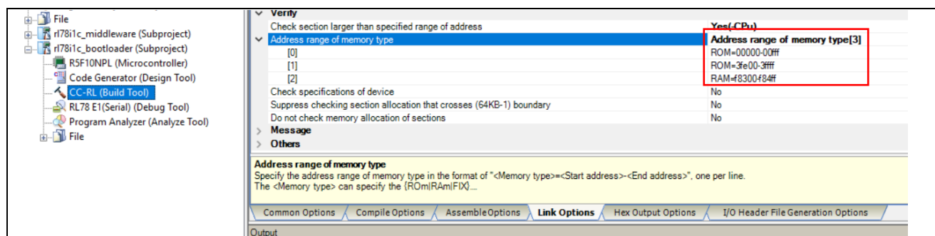
Figure 4-13 : Bootloader - Address Range of Memory Type (CS+)
