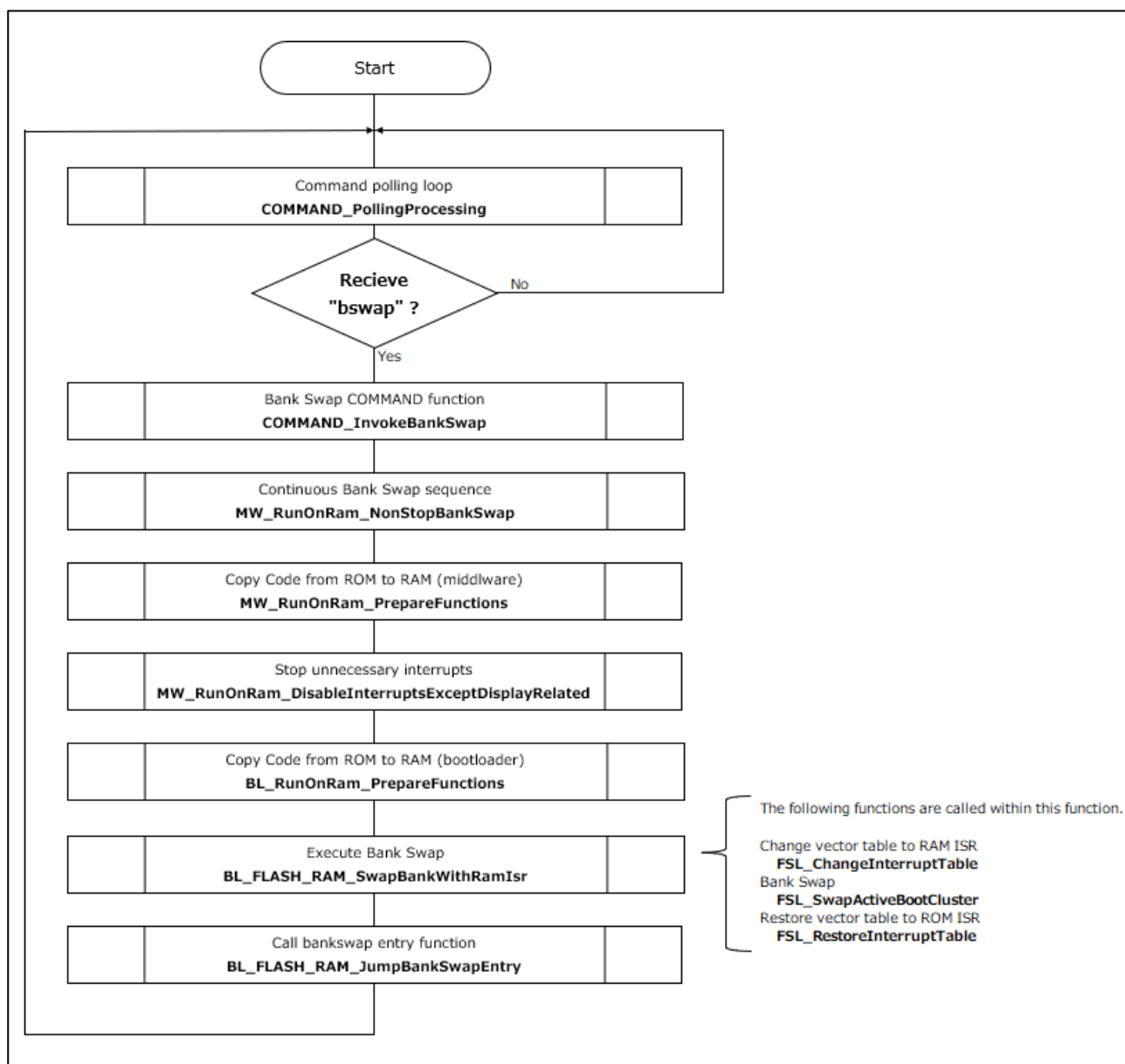
Figure 4-31 : Example of API Function Usage
