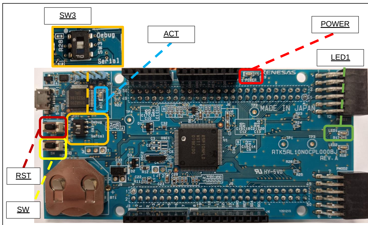
Figure 3-1 : Outline of Fast Prototyping Board
