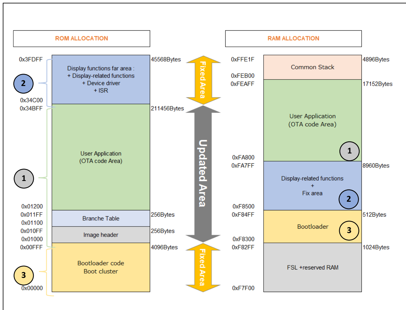
Figure 4-2 : Memory Mapping
