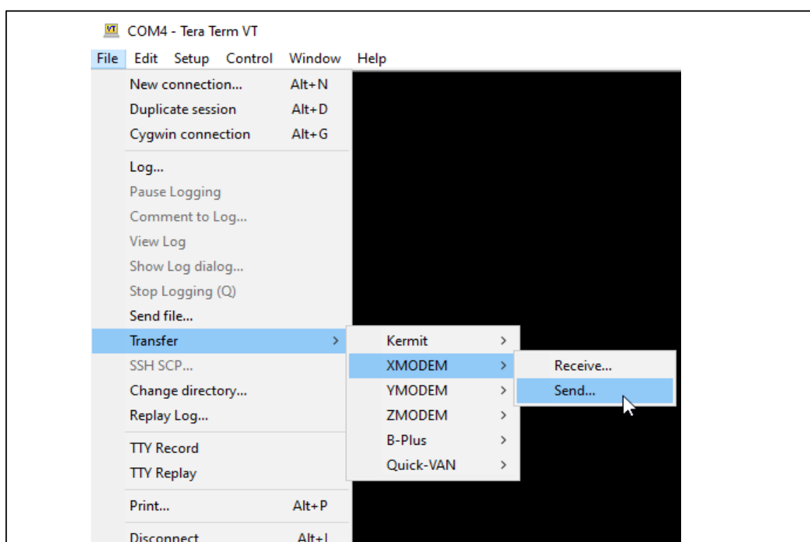
Figure 3-10 : Select XMODEM
