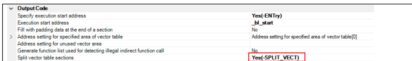
Figure 4-28 : Split Vector Table Sections (CS+)
