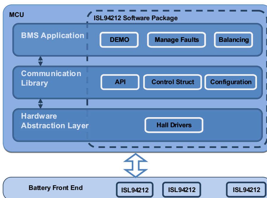
Figure 1. Software Package Structure
