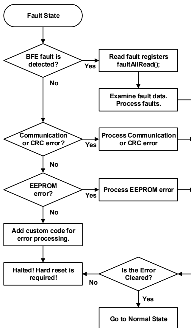
Figure 10. Fault Management Flowchart
