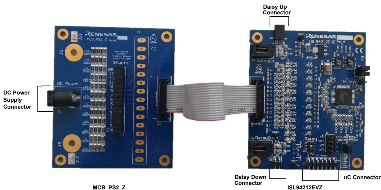
Figure 15. Resistor Ladder and ISL94212 Evaluation Board
