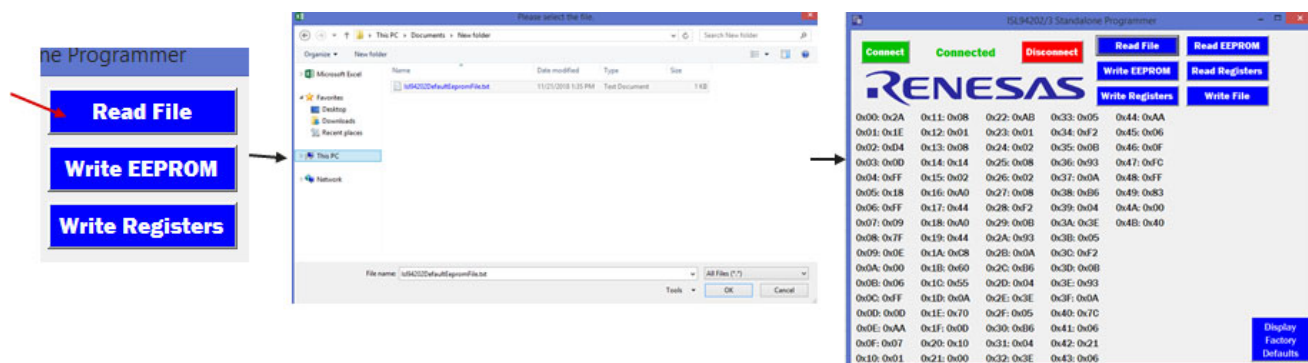
Figure 3. Read File
