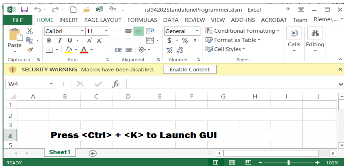
Figure 1. Workbook View
