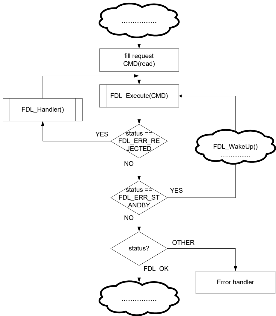
Figure 4-2: FDL read command execution
