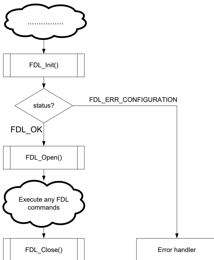
Figure 4-1: Initialization flow
