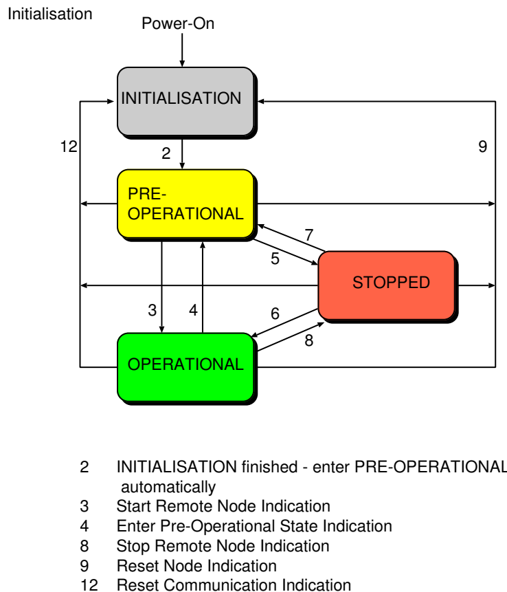
Figure 6, Minimal Boot-Up Procedure
