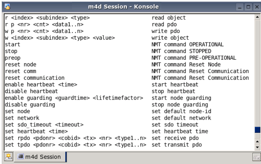
Figure 59, CANopen CiA-309-3 Gateway (m4d)
