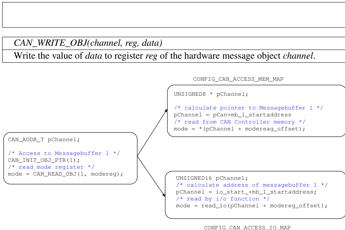
Figure 50, Driver Macros Full-CAN Controller
