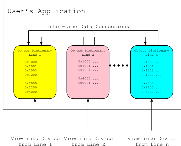
Figure 56, Multi-Line Object Dictionary
