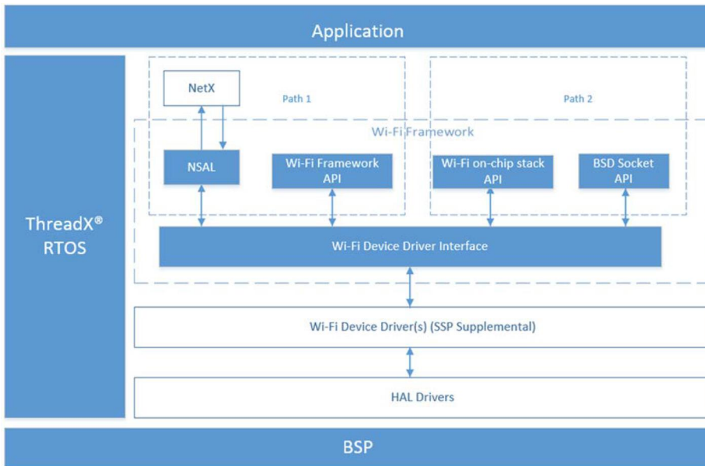
Figure 1: Synergy Wi-Fi Framework layered architecture.
