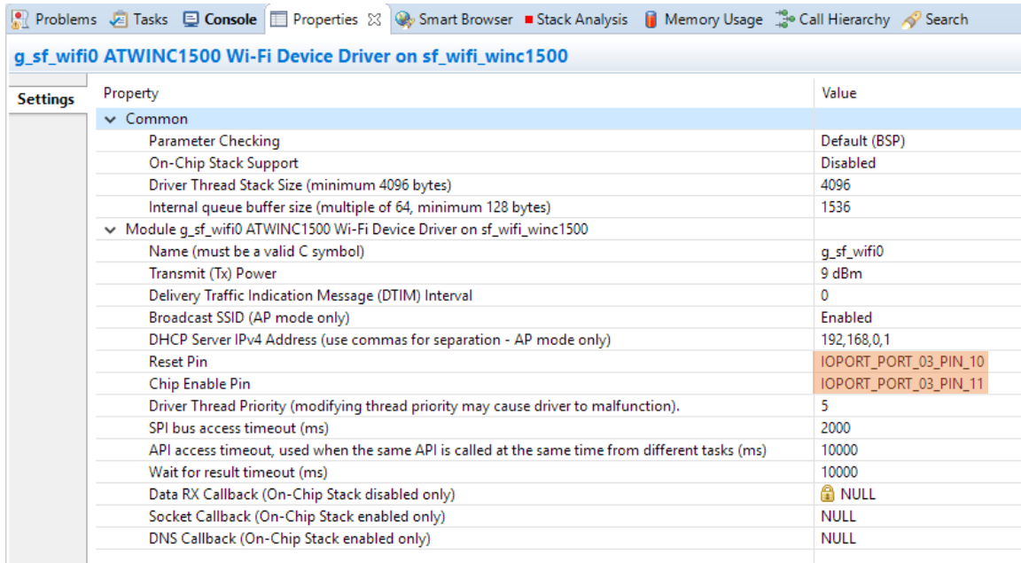
Figure 9: ATWINC1500 Wi-Fi Device Driver on sf_wifi_winc1500 configuration.
