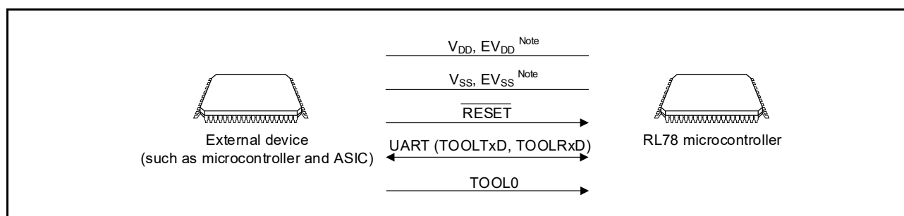
Figure 33 - 3 Environment for Writing Program to Flash Memory
