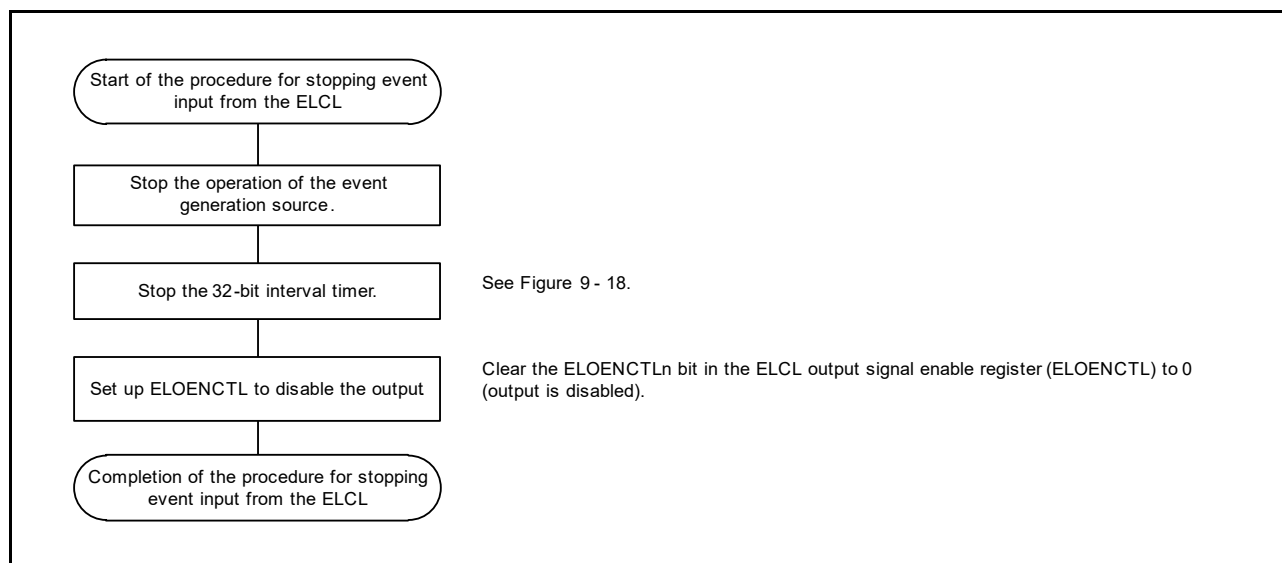
Figure 9 - 22 Procedure for Stopping Event Input from the ELCL
