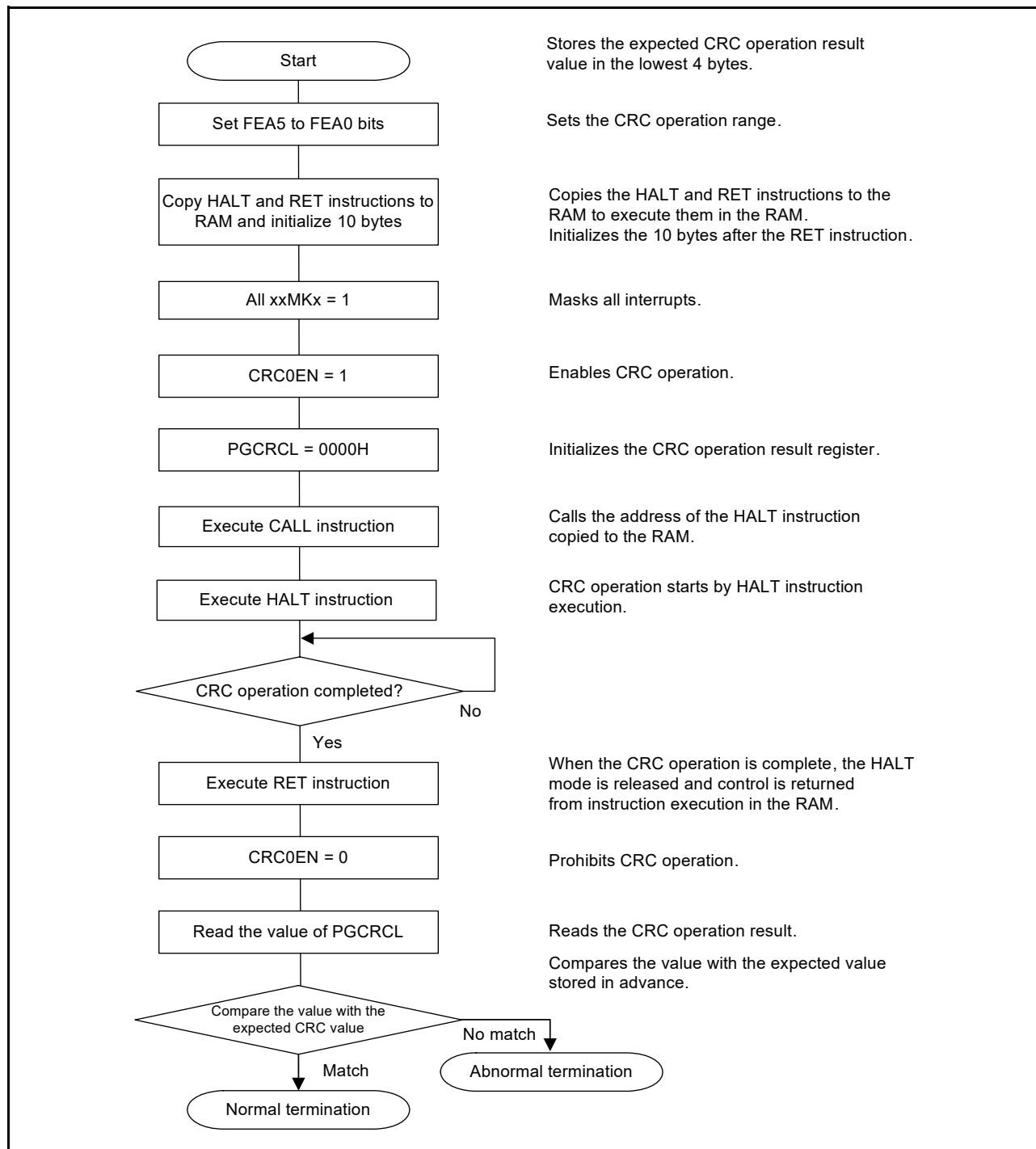
Figure 27 - 3 Flowchart of Flash Memory CRC Operation (High-speed CRC)
