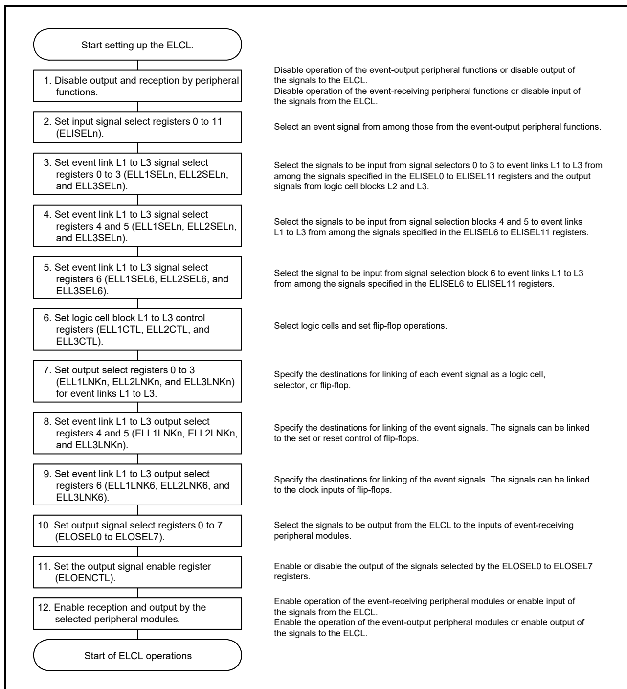
Figure 20 - 31 Procedure of Setting the ELCL
