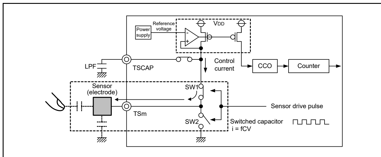
Figure 30 - 21 Charging
