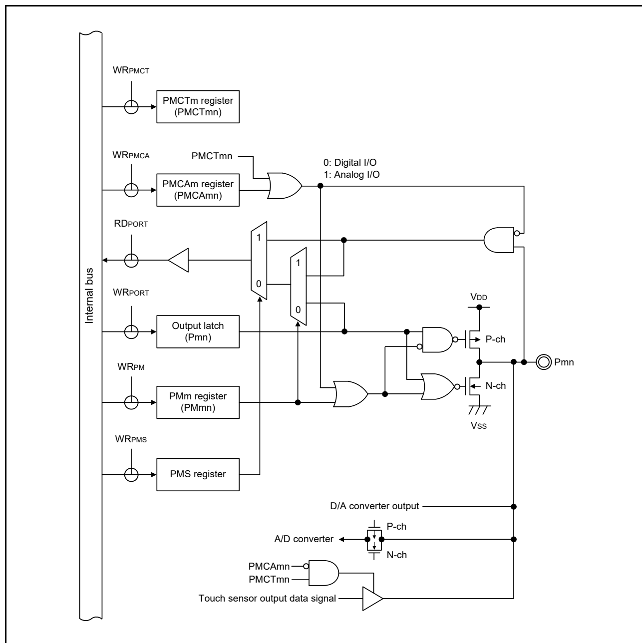
Figure 2 - 9 Pin Block Diagram for Pin Type 4-35-1
