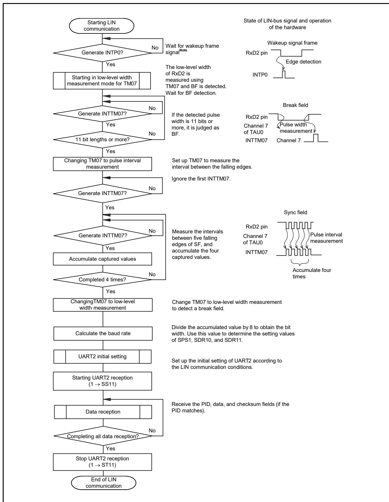
Figure 15 - 99 Flowchart of LIN Reception
