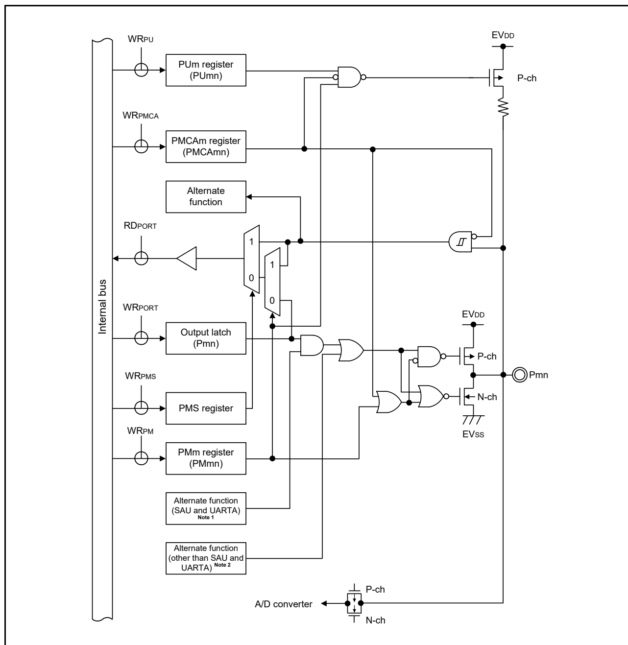
Figure 2 - 15 Pin Block Diagram for Pin Type 7-3-3
