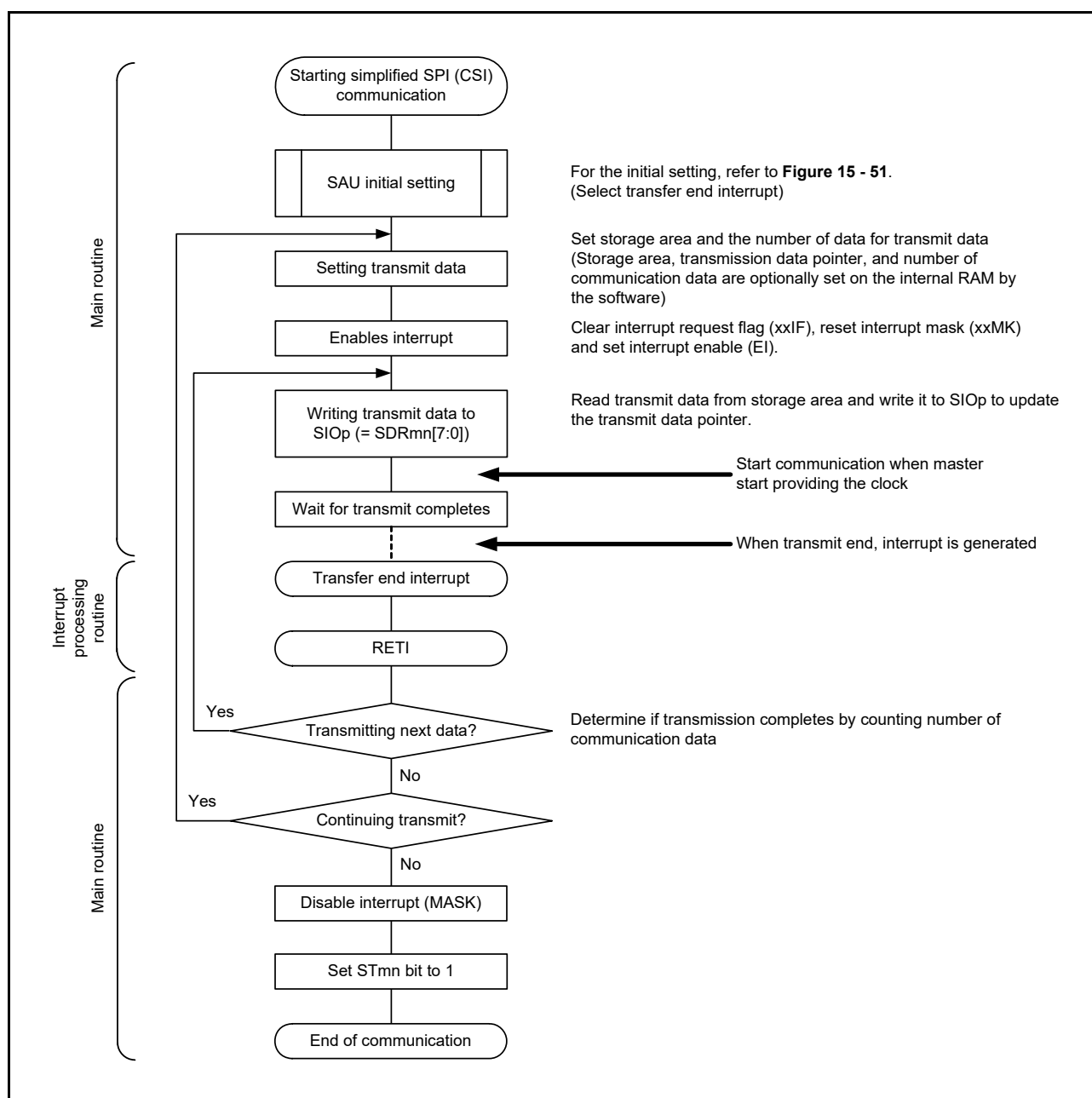
Figure 15 - 55 Flowchart of Slave Transmission (in Single-transmission Mode)
