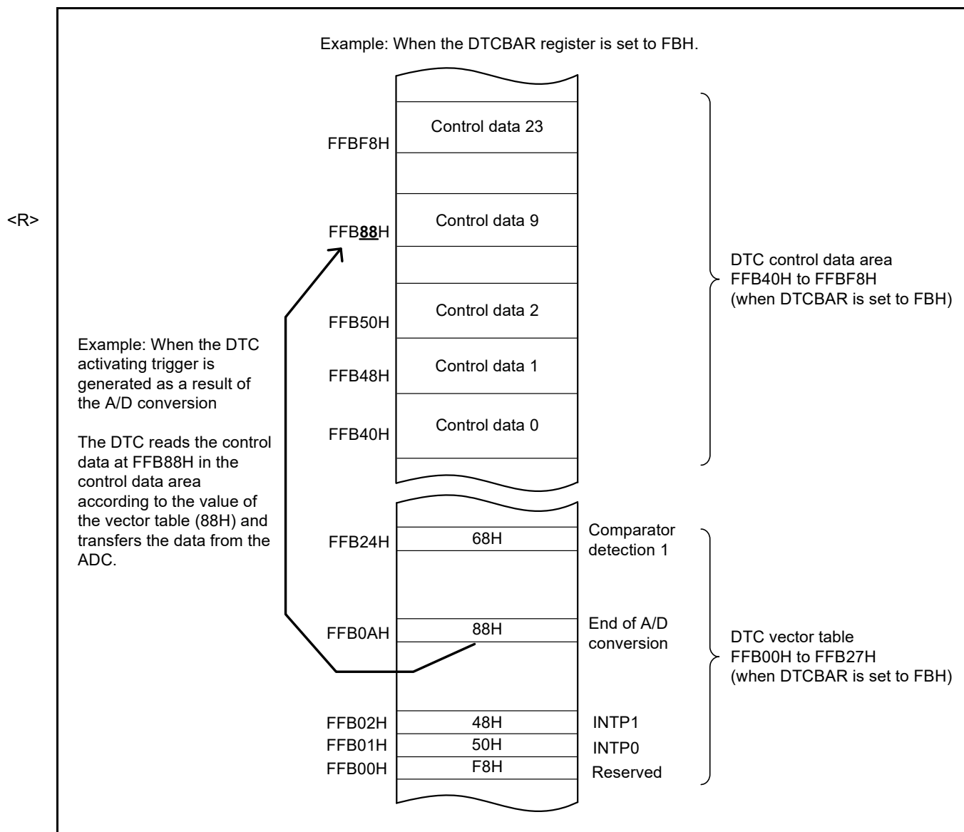
Figure 19 - 4 Start Addresses of Control Data and Vector Table
