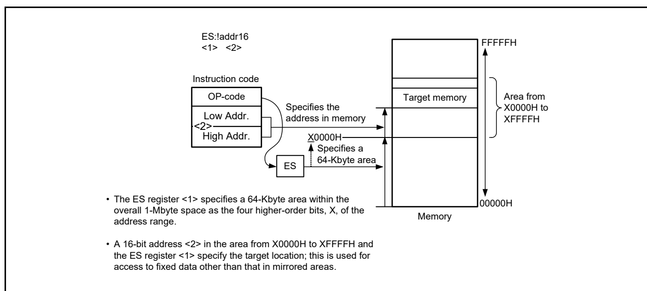
Figure 3 - 24 Example of ES:!addr16
