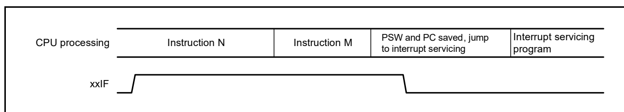
Figure 21 - 11 Holding Interrupt Requests Pending
