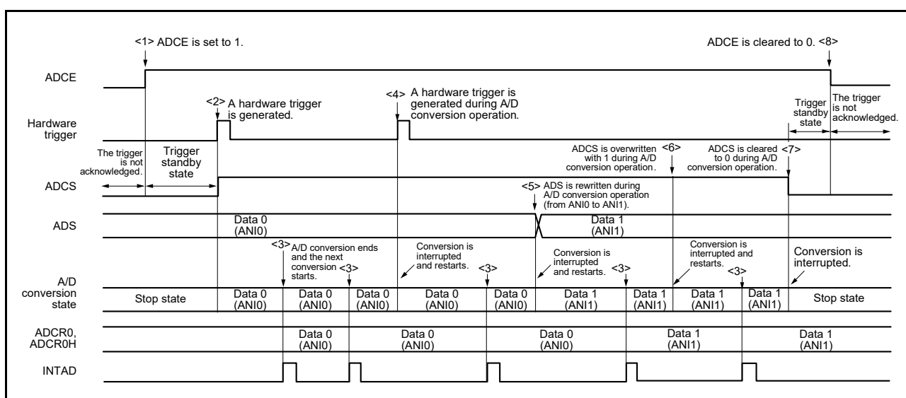
Figure 12 - 30 Example of Hardware Trigger Wait Mode (Select Mode, Sequential Conversion Mode) Operation Timing
