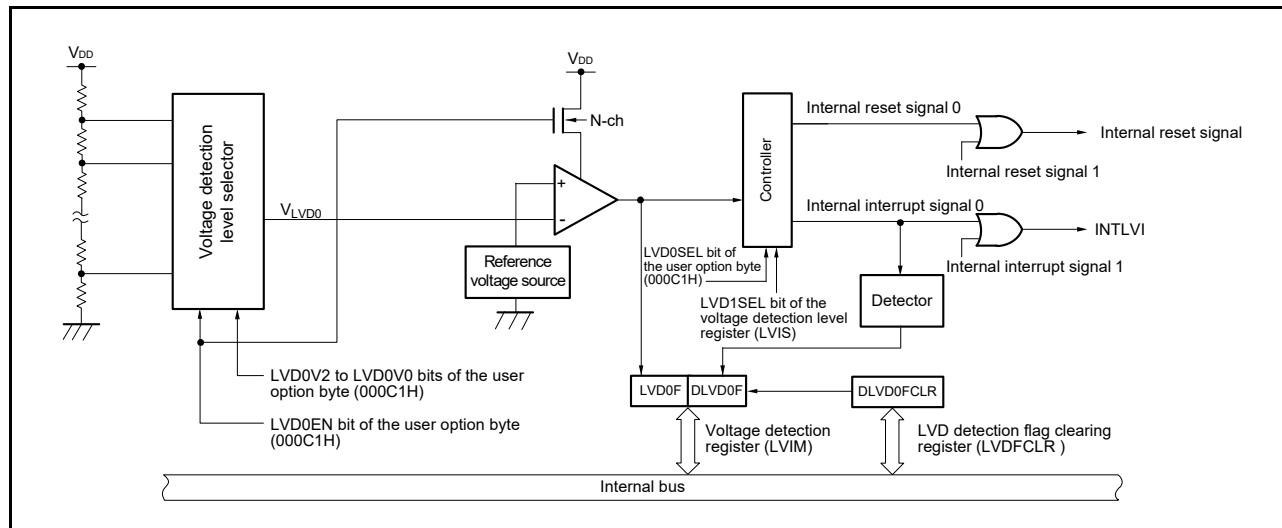
Figure 26 - 1 Block Diagram of LVD0
