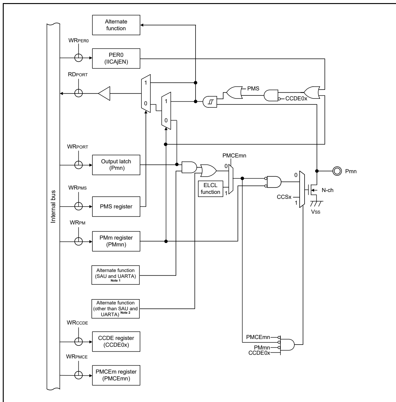
&lt;R&gt; Figure 2 - 35 Pin Block Diagram for Pin Type 12-38-3
