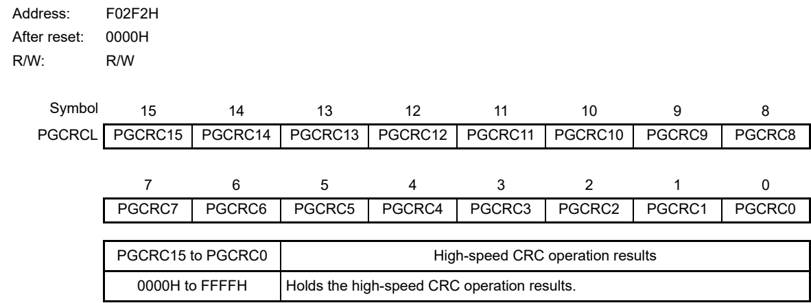
Figure 27 - 2 Format of Flash Memory CRC Operation Result Register (PGCRCL)
