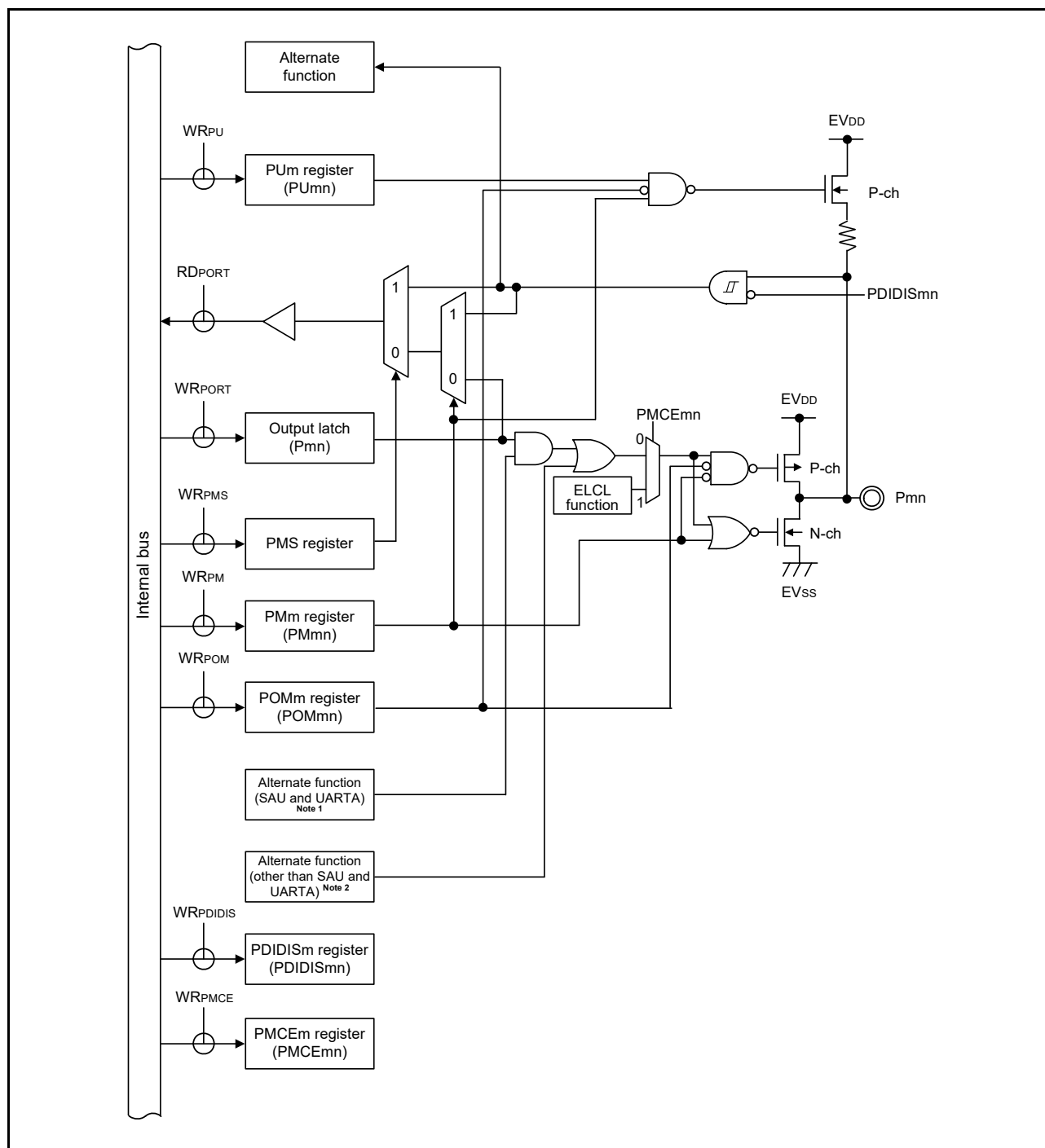
Figure 2 - 13 Pin Block Diagram for Pin Type 7-1-12
