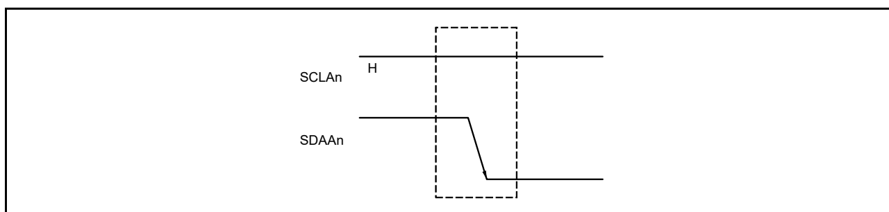
Figure 16 - 15 Start Conditions
