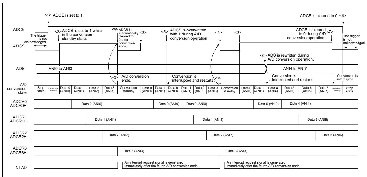
Figure 12 - 21 Example of Software Trigger No-wait Mode (Scan Mode, One-shot Conversion Mode) Operation Timing
