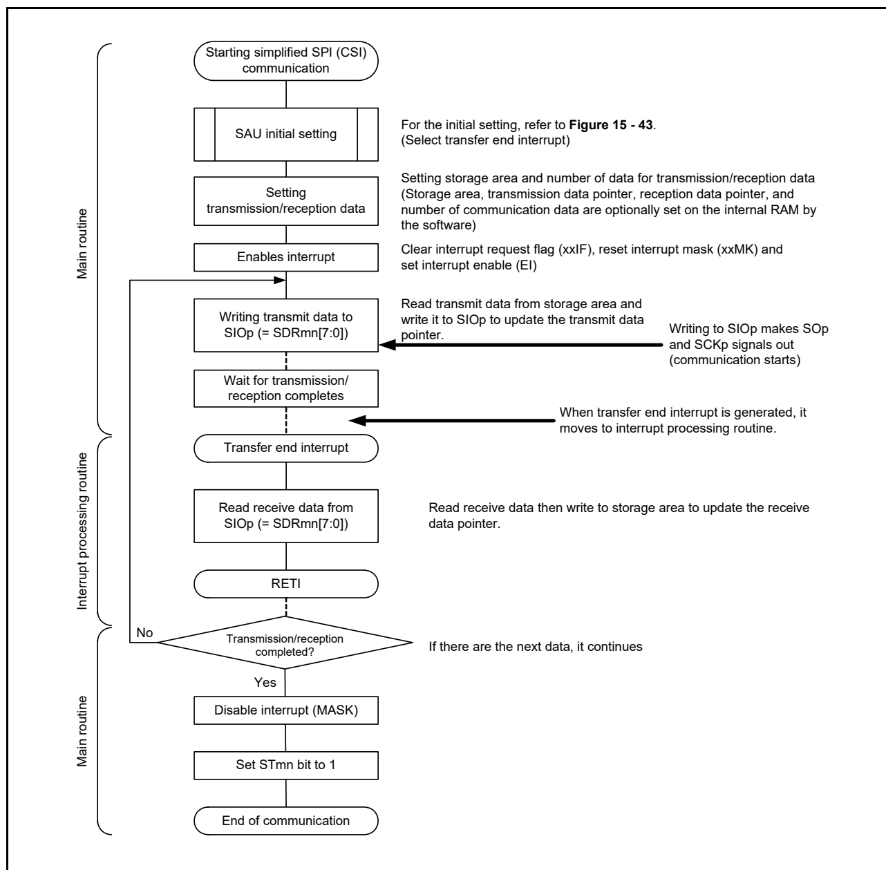
Figure 15 - 47 Flowchart of Master Transmission/Reception (in Single-transmission/reception Mode)
