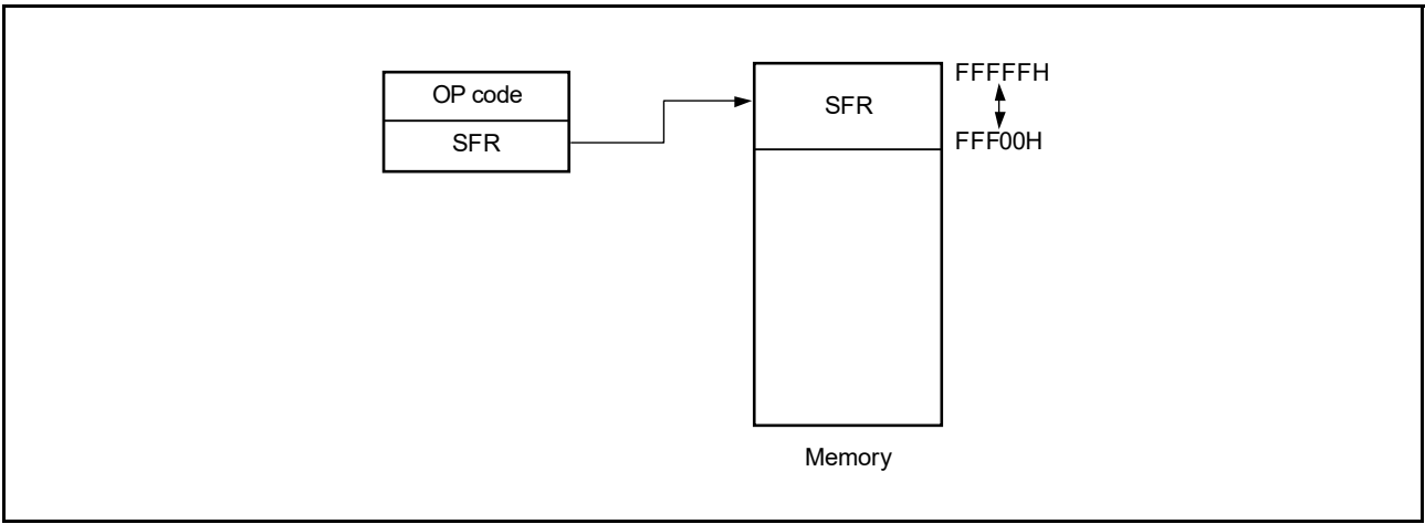
Figure 3 - 26 Outline of SFR Addressing
