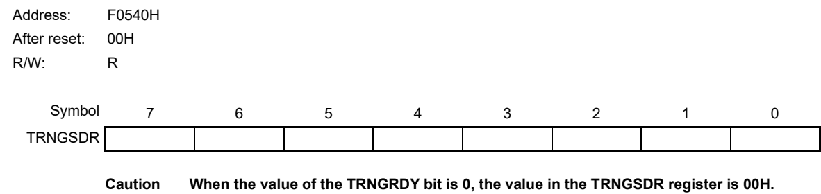
Figure 28 - 2 Format of Random Number Seed Data Register (TRNGSDR)
