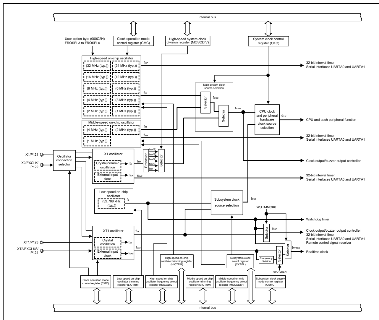
&lt;R&gt; Figure 6 - 1 Block Diagram of Clock Generator
