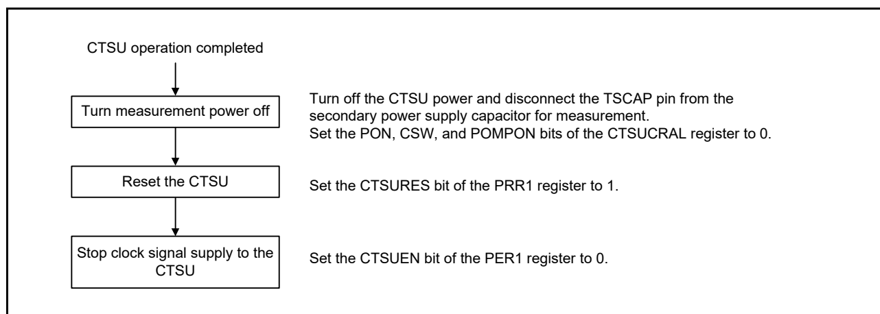
Figure 30 - 25 CTSU Stopping Flowchart
