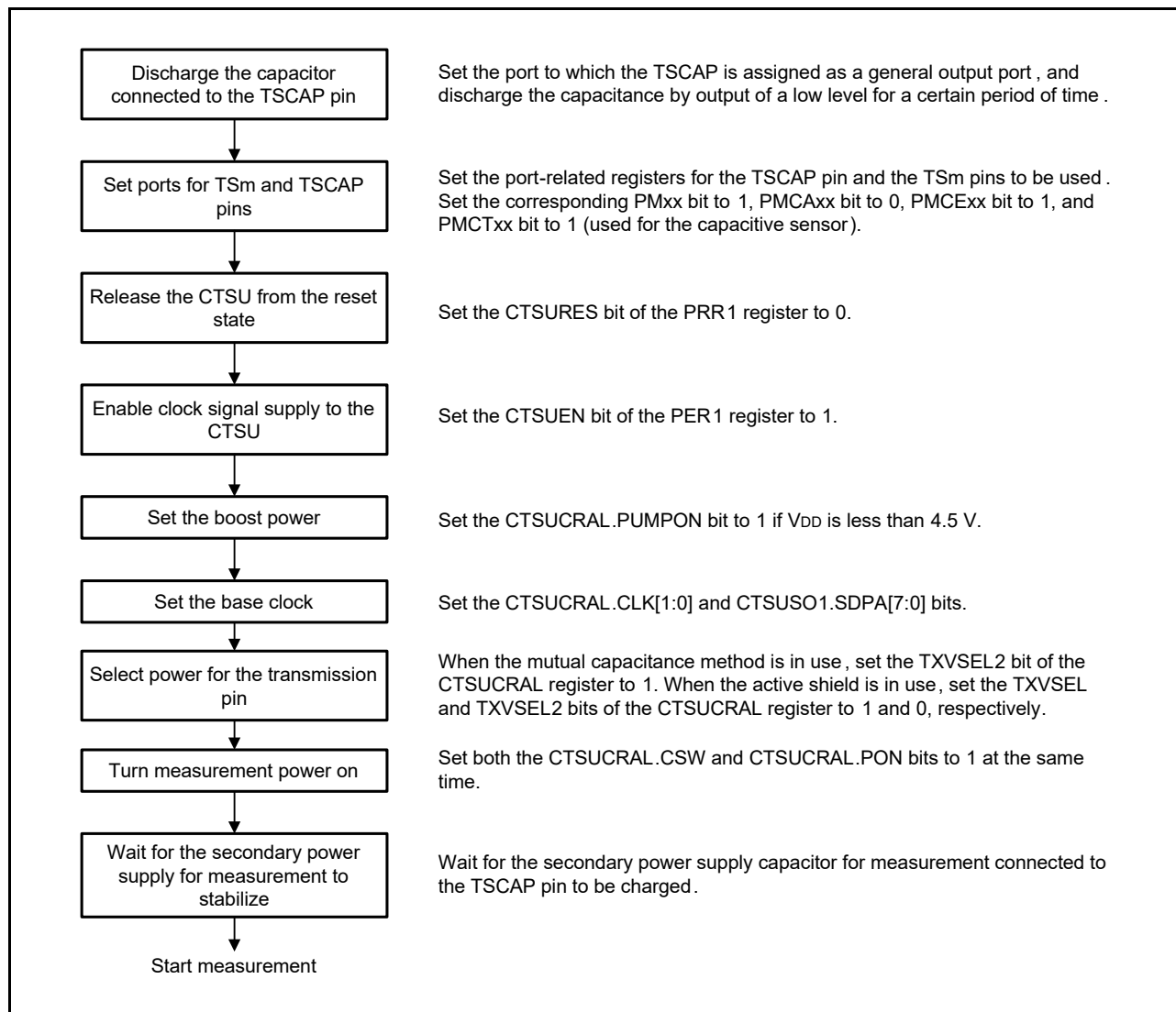
Figure 30 - 24 CTSU Initial Setting Procedure
