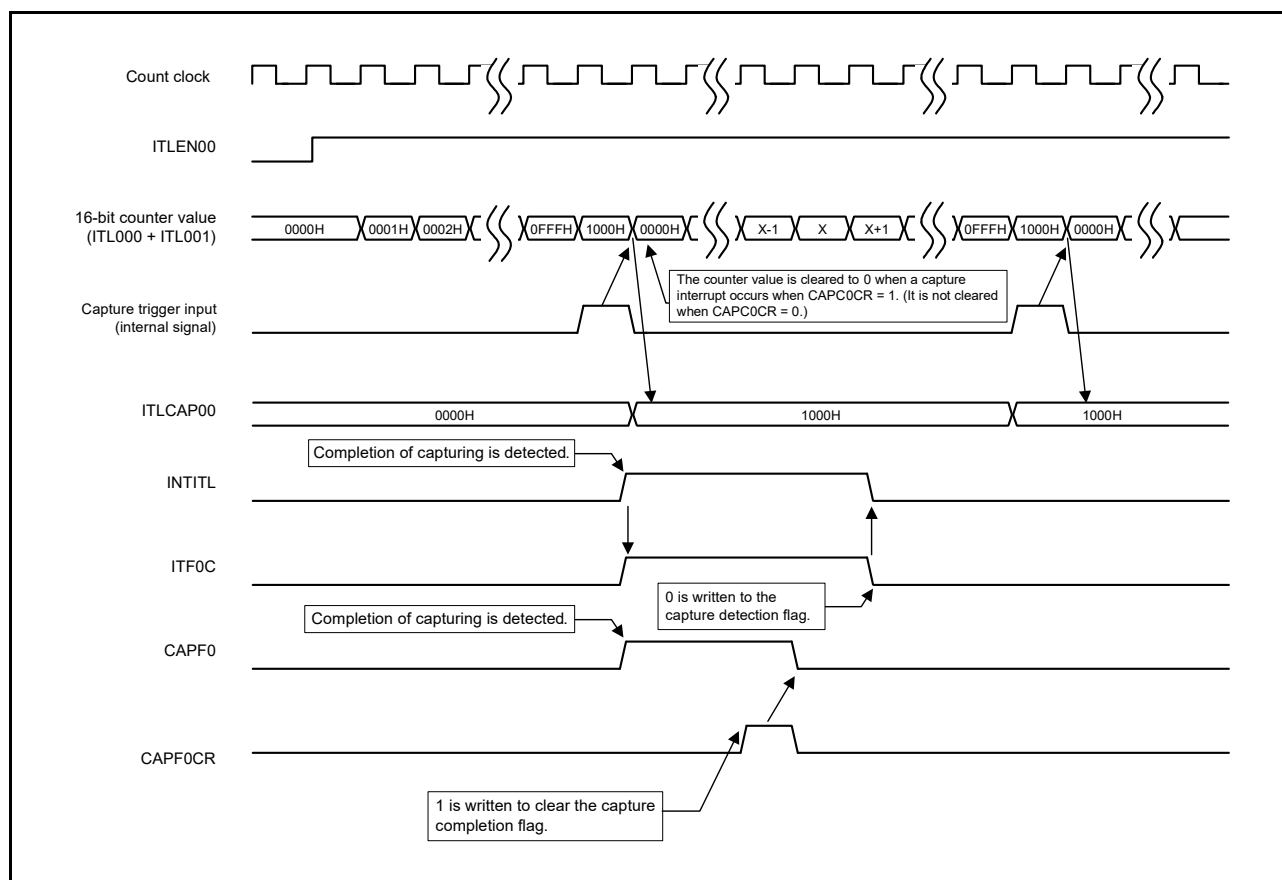
<R> Figure 9 - 15 Example of Capture Operation
