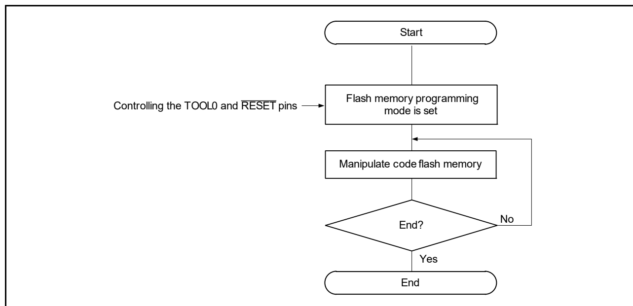
Figure 33 - 6 Code Flash Memory Manipulation Procedure
