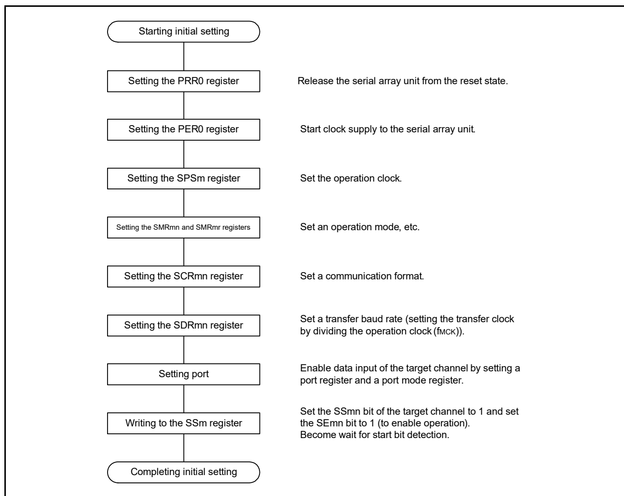
Figure 15 - 85 Initial Setting Procedure for UART Reception
