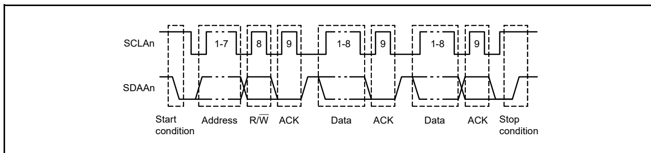
Figure 16 - 14 I 2 C Bus Serial Data Transfer Timing
