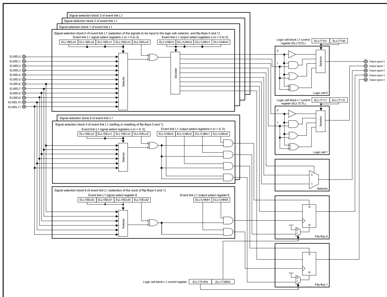
Figure 20 - 2 Block Diagram of Logic Cell Block L1
