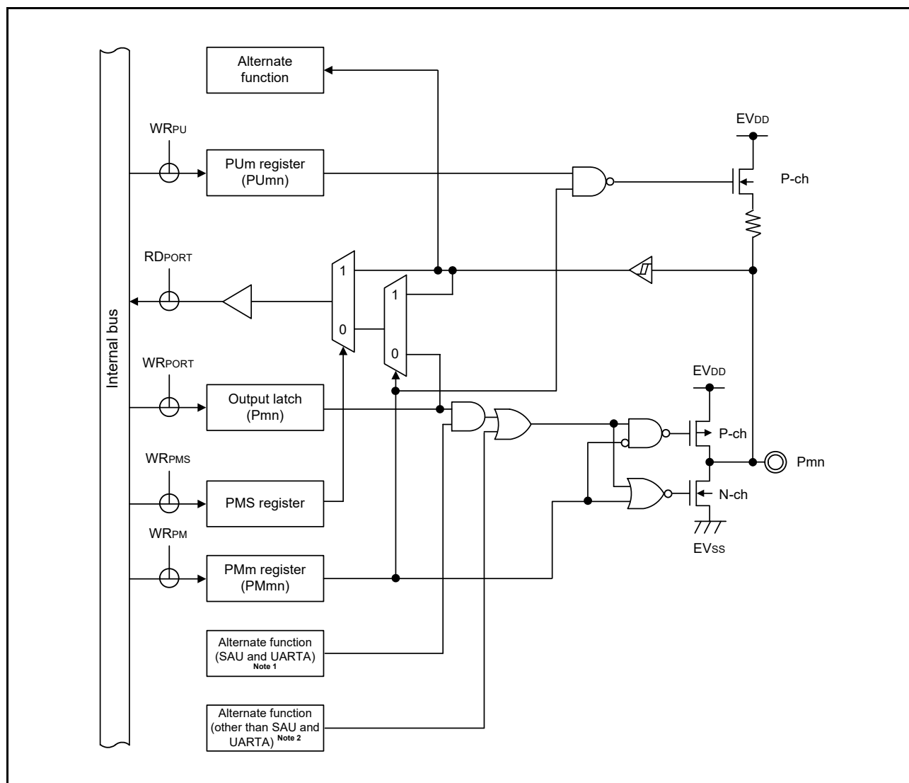
Figure 2 - 11 Pin Block Diagram for Pin Type 7-1-3
