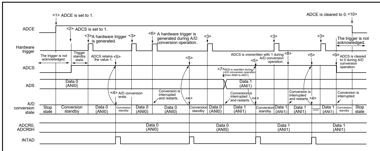
Figure 12 - 27 Example of Hardware Trigger No-wait Mode (Select Mode, One-shot Conversion Mode) Operation Timing
