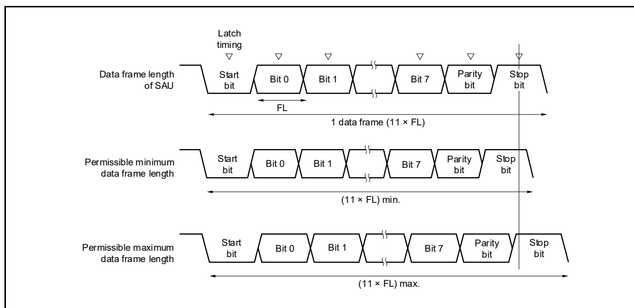
Figure 15 - 95 Permissible Baud Rate Range for Reception (1 Data Frame Length = 11 Bits)
