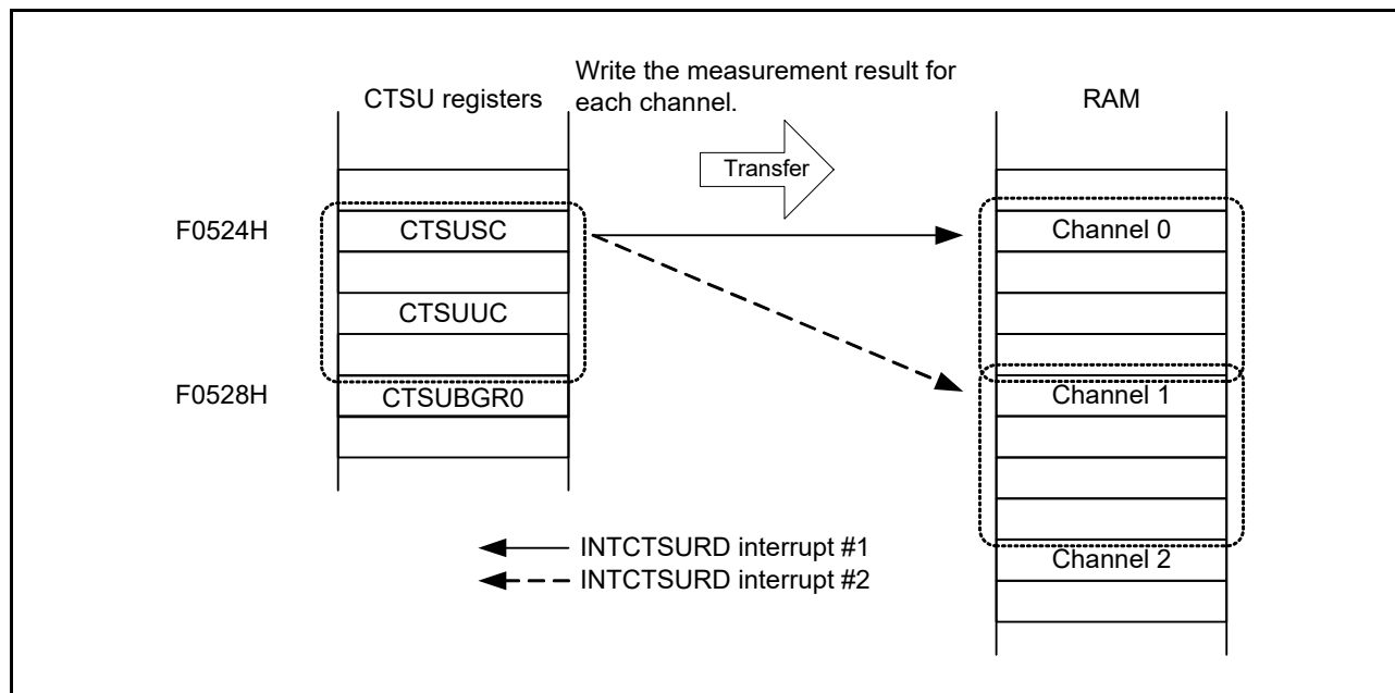
Figure 30 - 30 Data Transfer Operation on an INTCTSURD Interrupt
