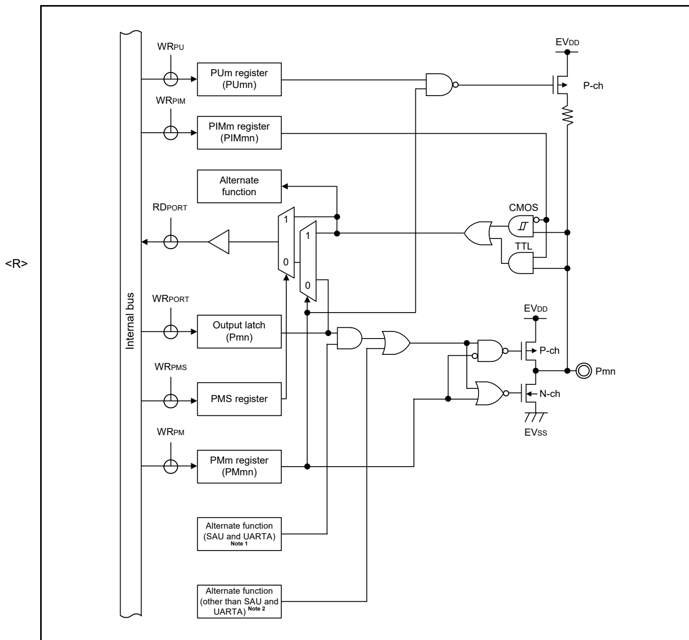
Figure 2 - 23 Pin Block Diagram for Pin Type 8-1-3
