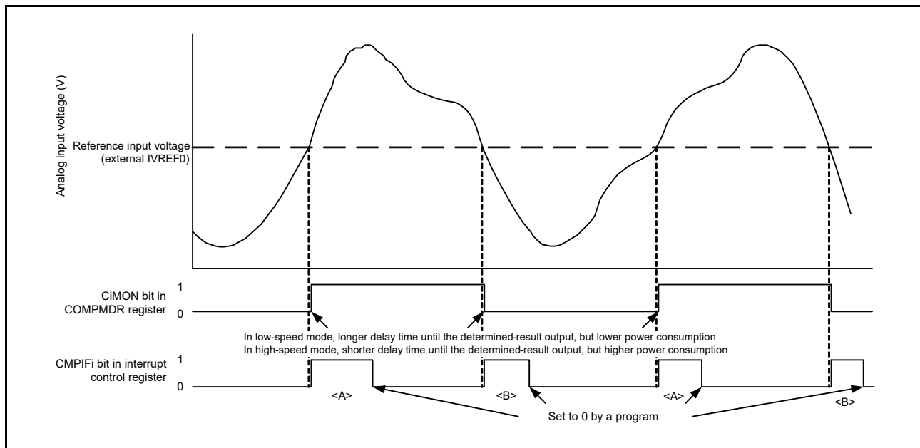
Figure 14 - 7 Example of the Comparator i ( i = 0, 1 ) Operation
