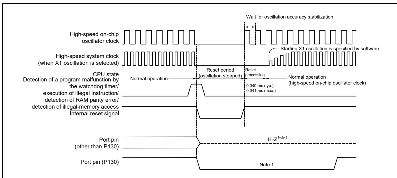
Figure 24 - 3 Timing of Reset Due to Detection of a Program Malfunction by the Watchdog Timer, Execution of Illegal Instruction, Detection of RAM Parity Error, or Detection of Illegal-memory Access
