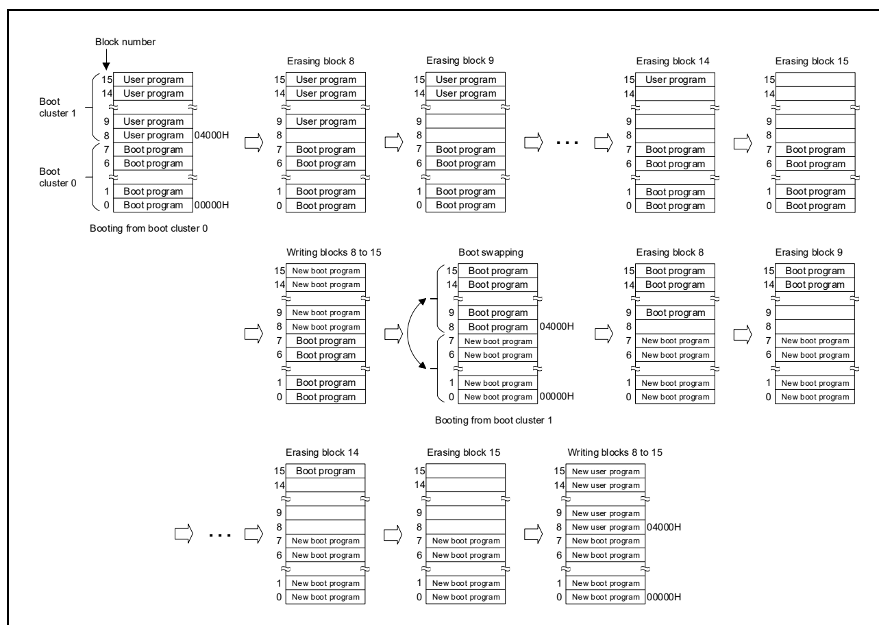
Figure 33 - 31 Example of Executing Boot Swapping
