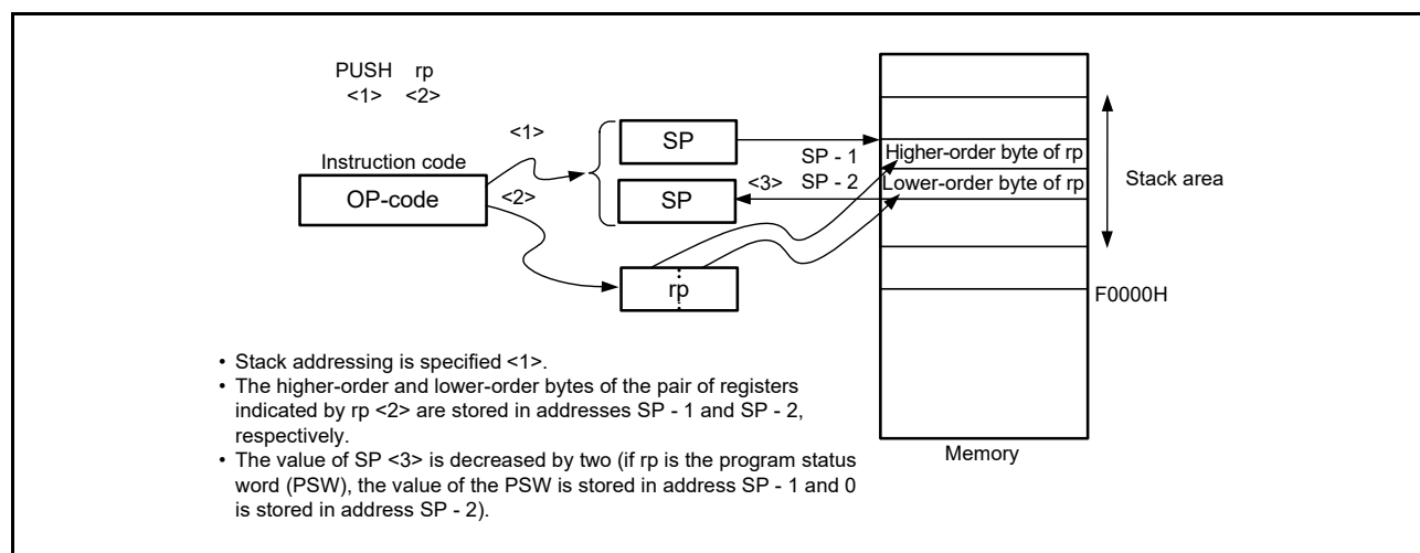
Figure 3 - 38 Example of PUSH rp
