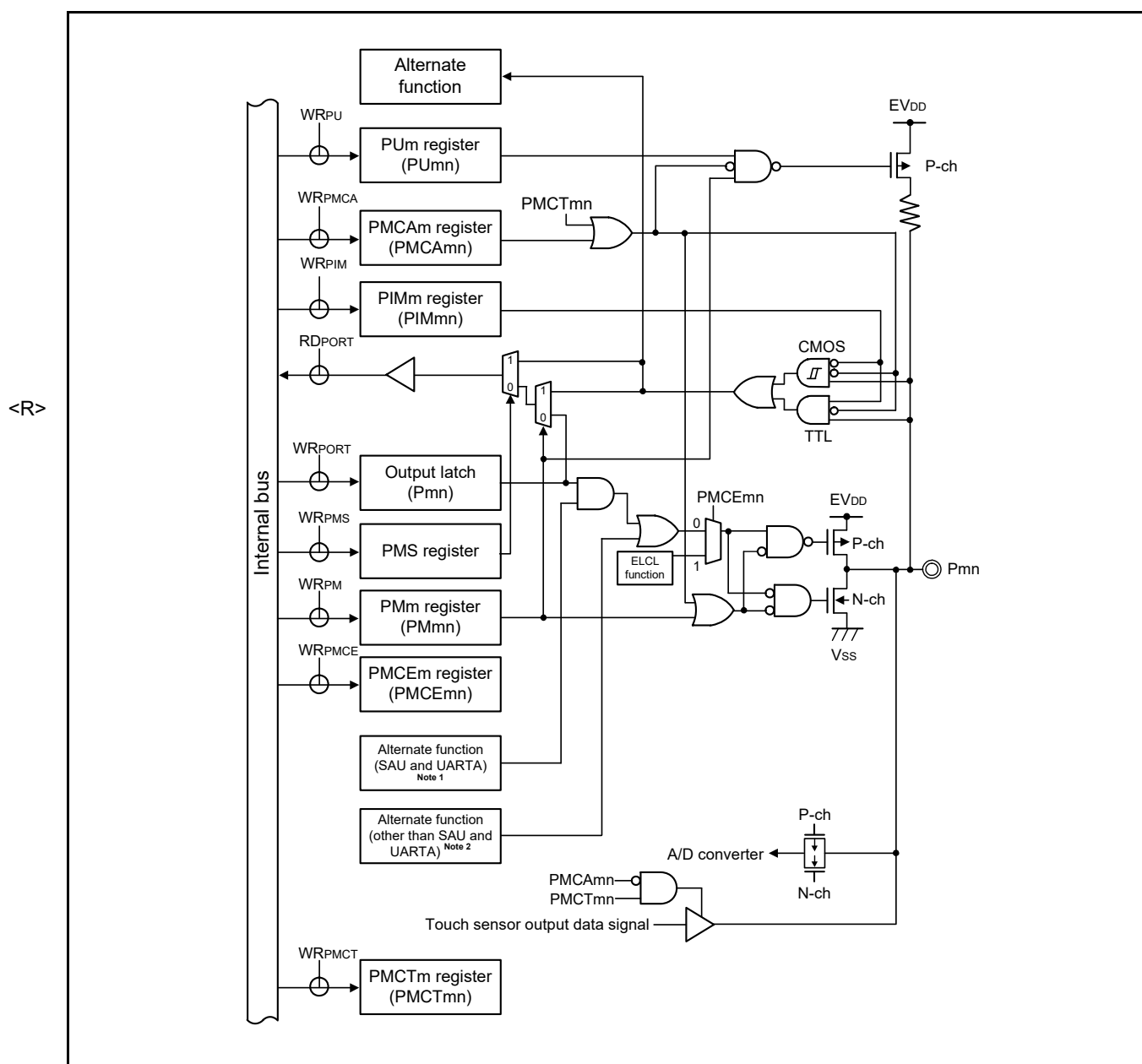
Figure 2 - 29 Pin Block Diagram for Pin Type 8-33-2
