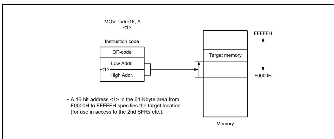
Figure 3 - 23 Example of !addr16
