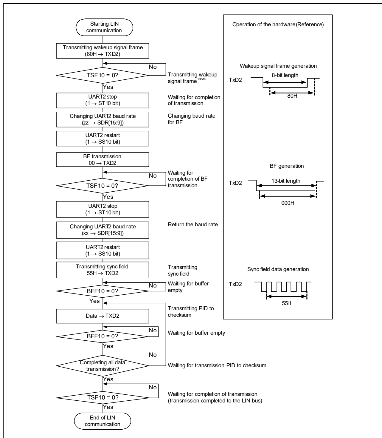
Figure 15 - 97 Flowchart for LIN Transmission
