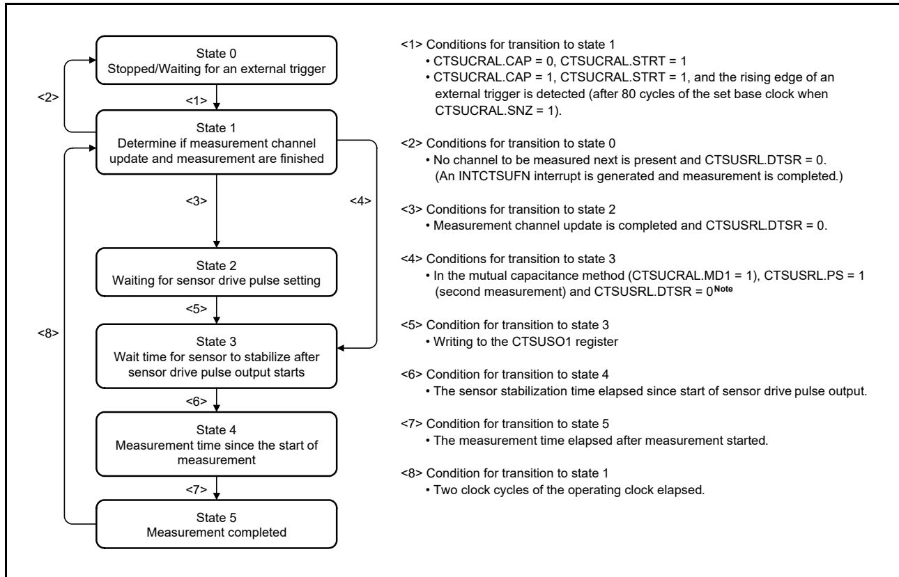
Figure 30 - 5 Transitions between the Measurement States
