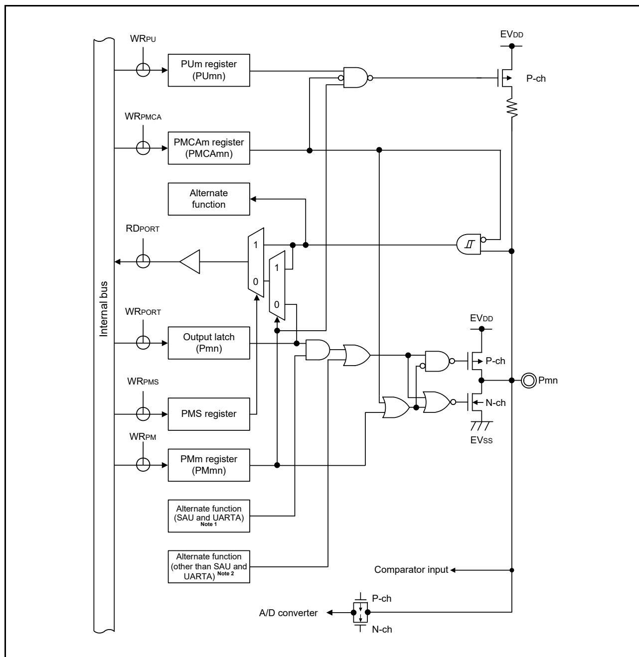
Figure 2 - 16 Pin Block Diagram for Pin Type 7-9-5
