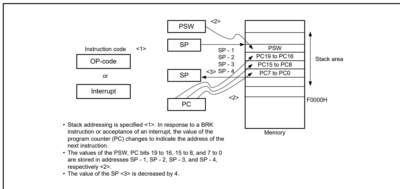
Figure 3 - 42 Example of Interrupt, BRK
