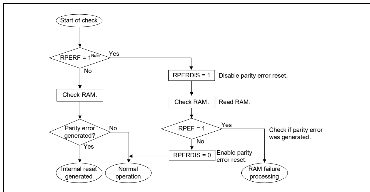
Figure 27 - 11 Flowchart of RAM Parity Check
