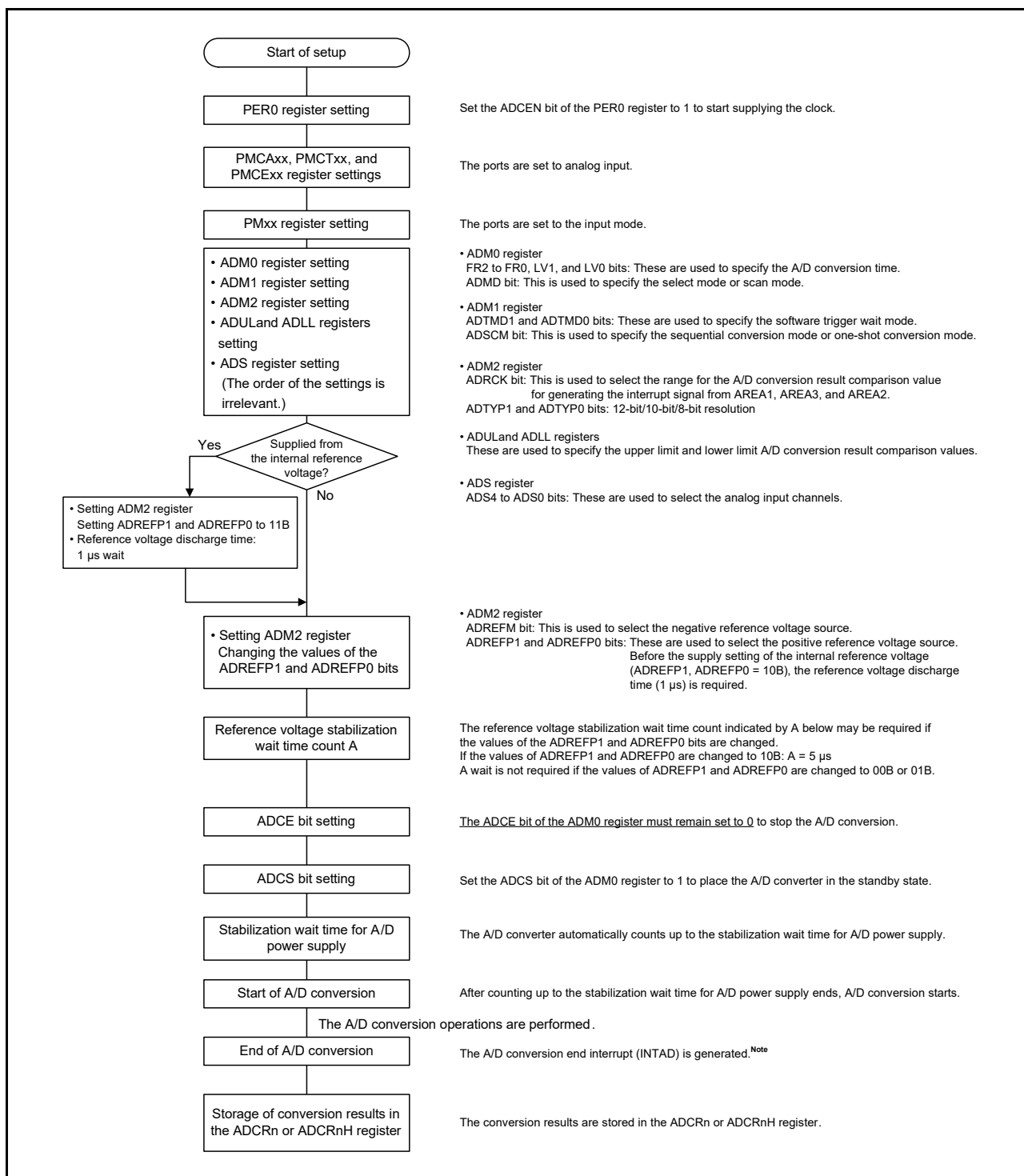
Figure 12 - 35 Settings in Software Trigger Wait Mode
