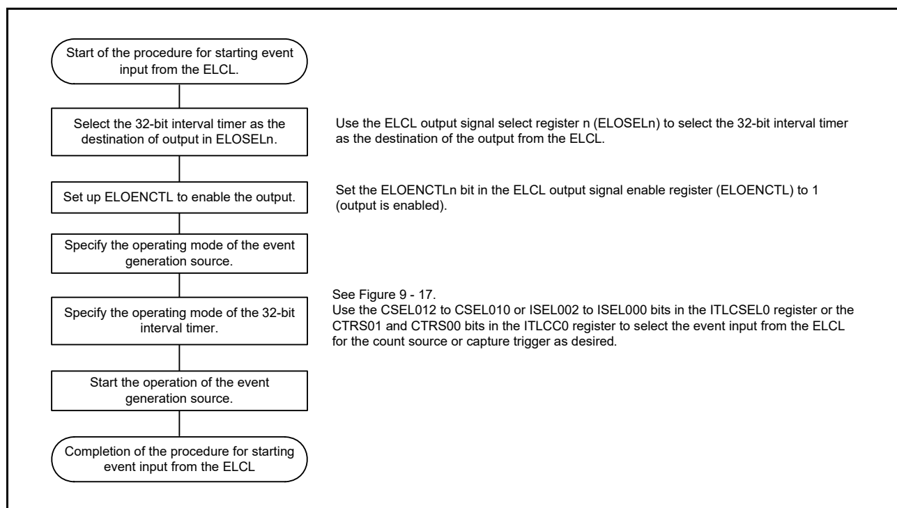
Figure 9 - 21 Procedure for Starting Event Input from the ELCL
