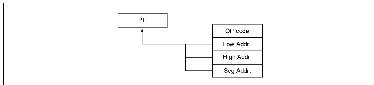
Figure 3 - 17 Example of CALL !!addr20/BR !!addr20
