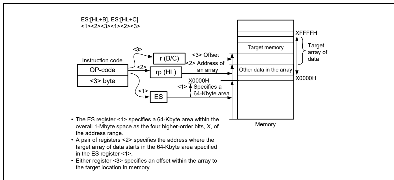
Figure 3 - 37 Example of ES:[HL+B], ES:[HL+C]
