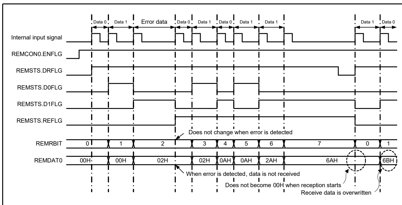
Figure 18 - 39 REMDAT0 and REMRBIT Registers Operation upon Error Detection when REMCON0.EC = 0
