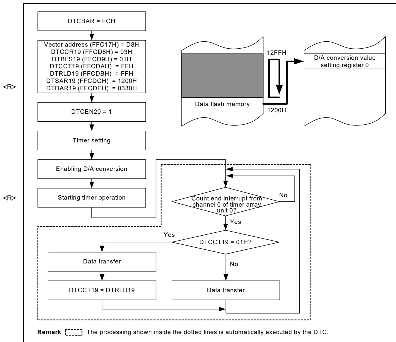
Figure 19 - 20 Example 2 of Using Repeat Mode: Outputting a Sine Wave Using the 8-bit D/A Converter
