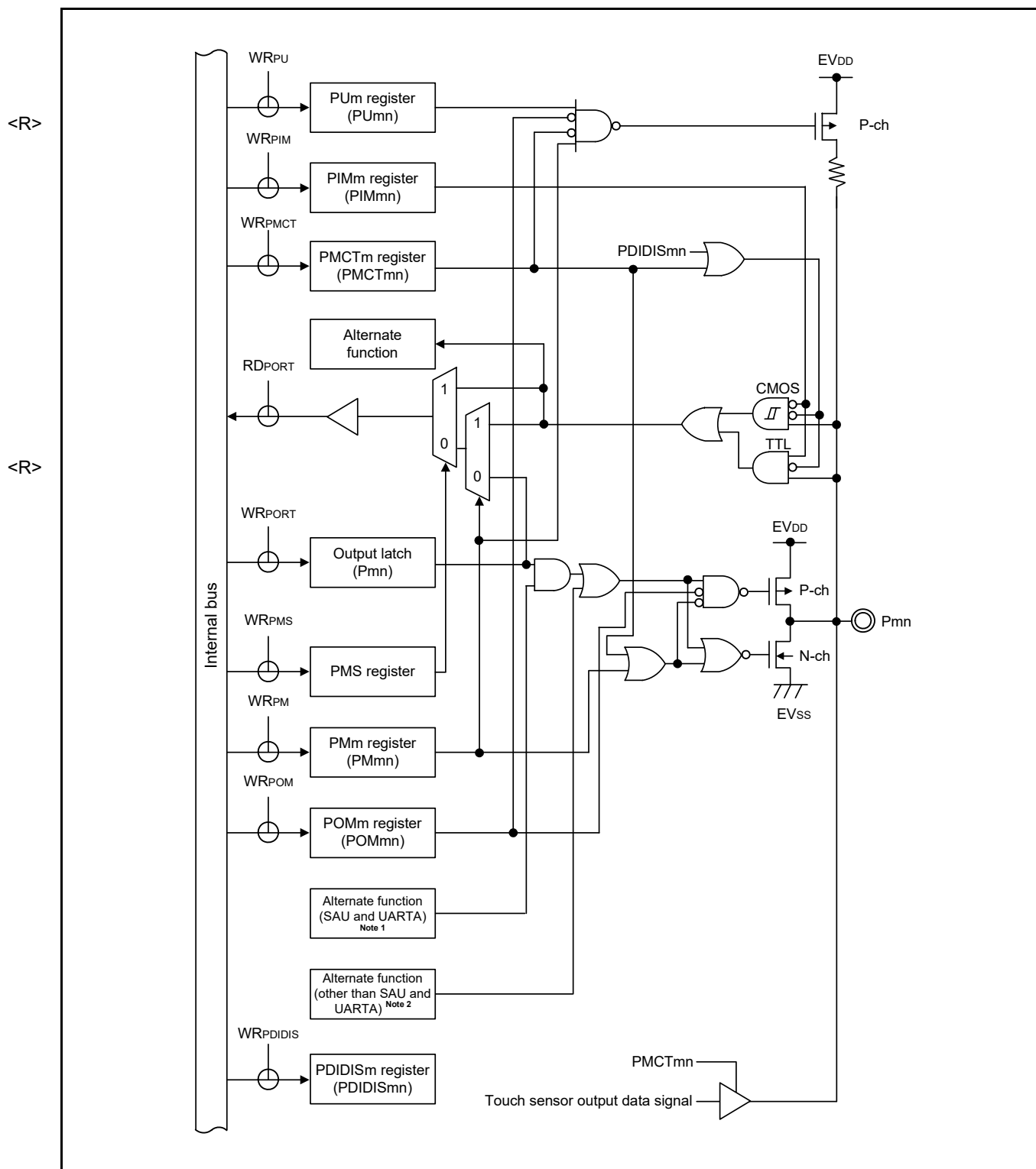
Figure 2 - 28 Pin Block Diagram for Pin Type 8-31-2
