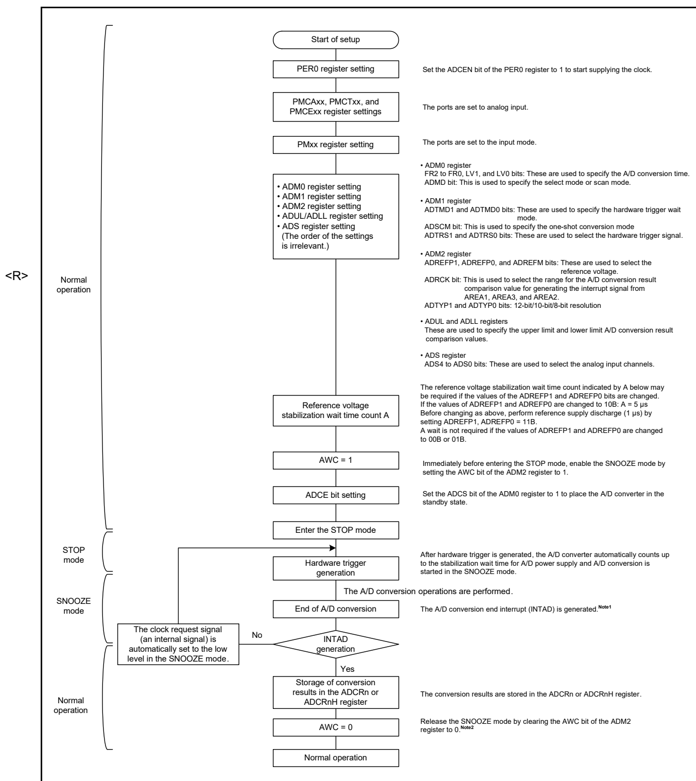
Figure 12 - 45 Flowchart for Setting up SNOOZE Mode (Hardware Trigger)
