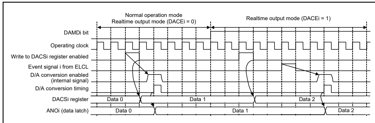
Figure 13 - 6 Timing for Outputting D/A Conversion Value
