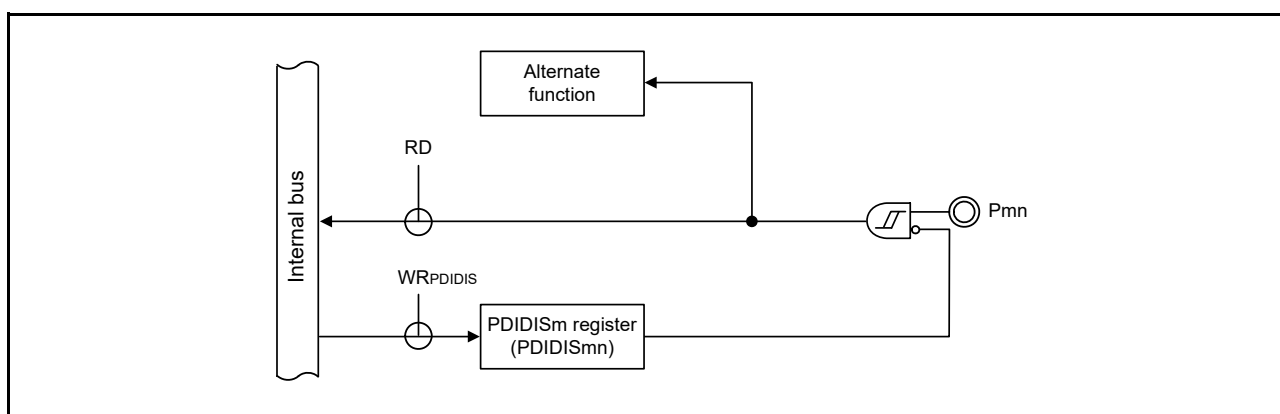
Figure 2 - 5 Pin Block Diagram for Pin Type 2-1-3
