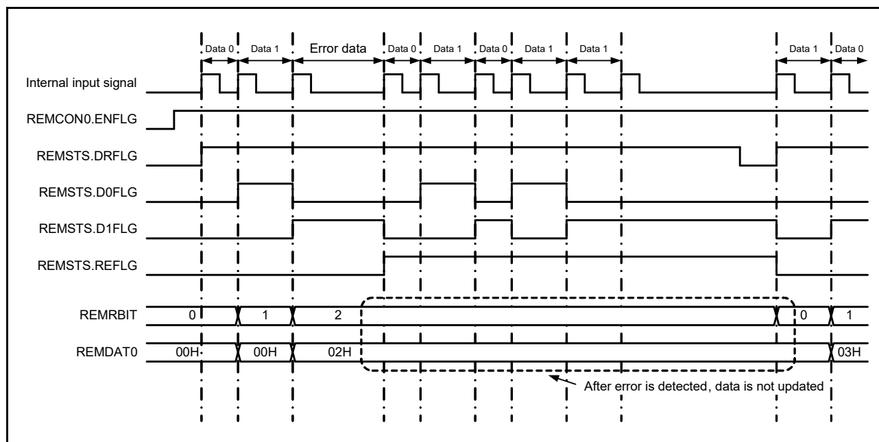
Figure 18 - 40 REMDAT0 and REMRBIT Registers Operation upon Error Detection when REMCON0.EC = 1
