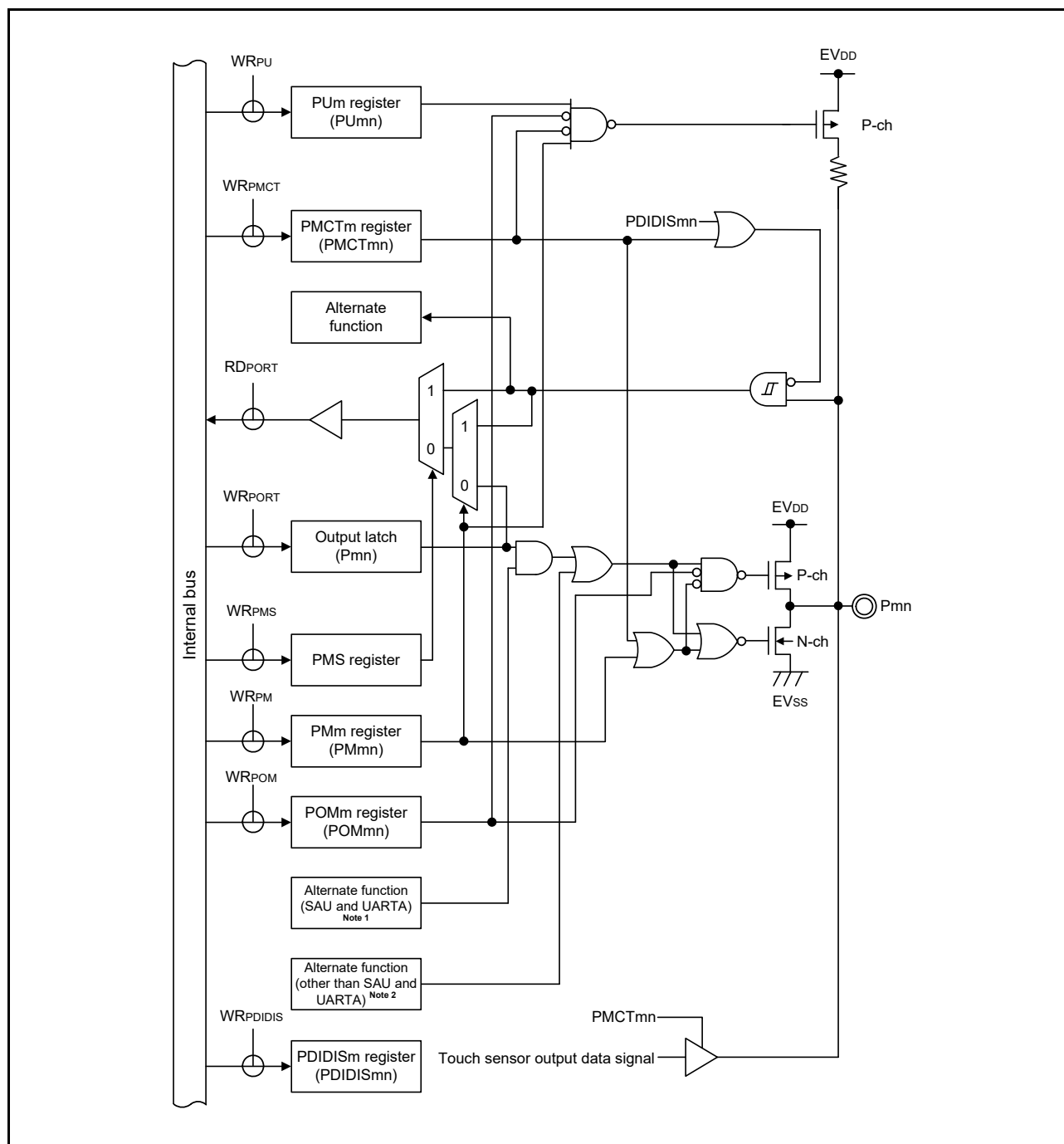
Figure 2 - 19 Pin Block Diagram for Pin Type 7-31-3
