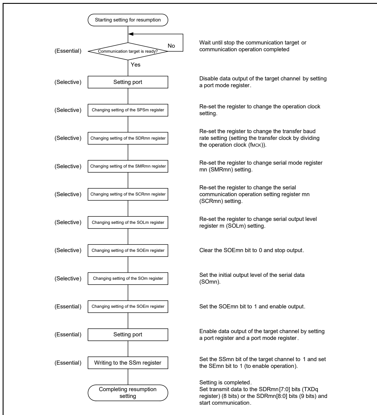
Figure 15 - 79 Procedure for Resuming UART Transmission
