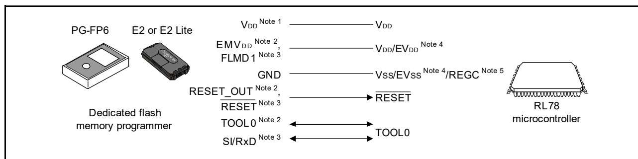
Figure 33 - 2 Communications with Dedicated Flash Memory Programmer
