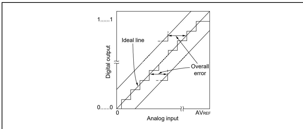
Figure 12 - 46 Overall Error
