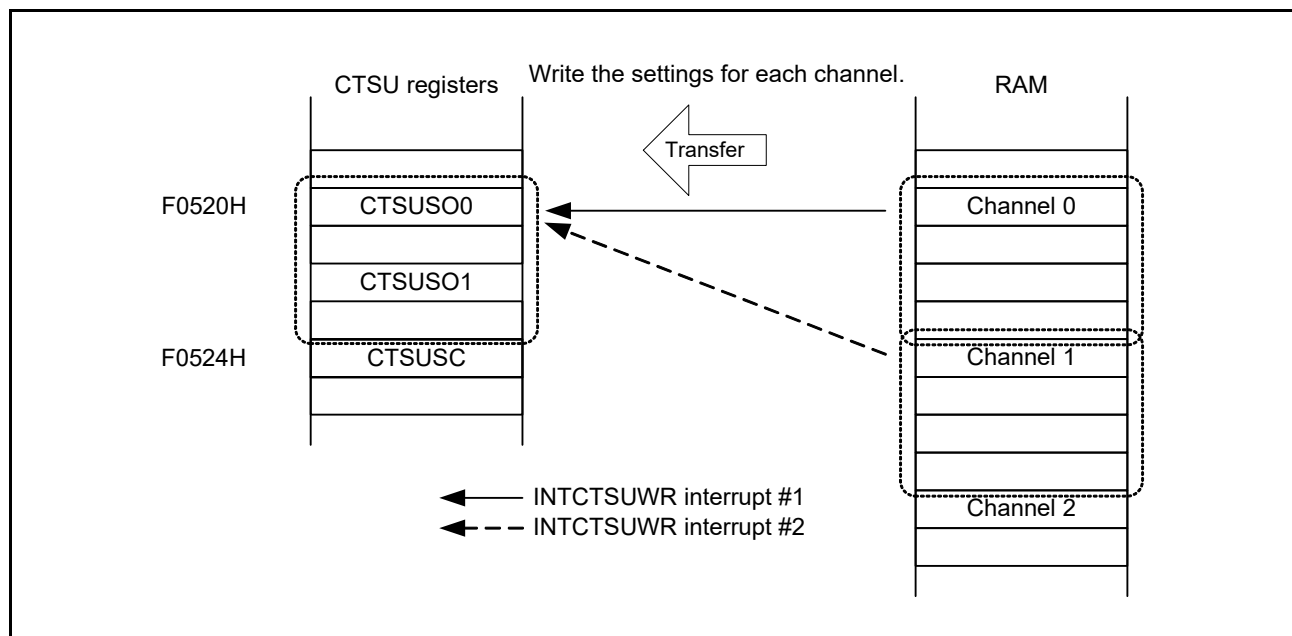
Figure 30 - 29 Data Transfer on an INTCTSUIWR Interrupt
