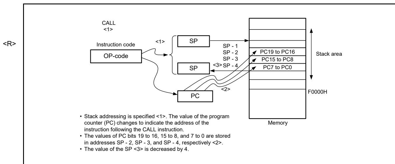
Figure 3 - 40 Example of CALL, CALLT
