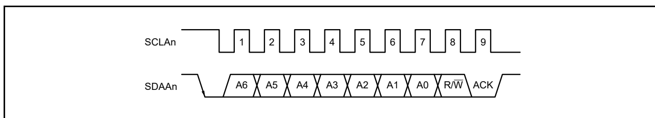
Figure 16 - 18 ACK
