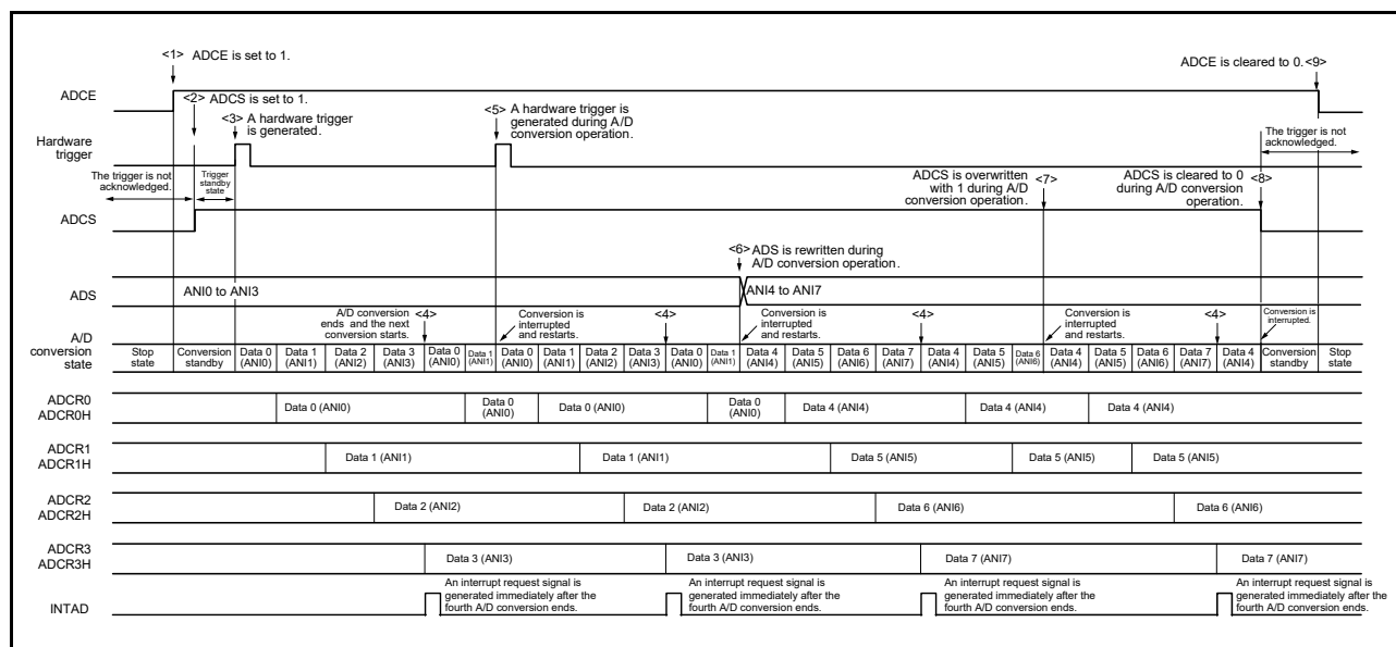
Figure 12 - 28 Example of Hardware Trigger No-wait Mode (Scan Mode, Sequential Conversion Mode) Operation Timing
