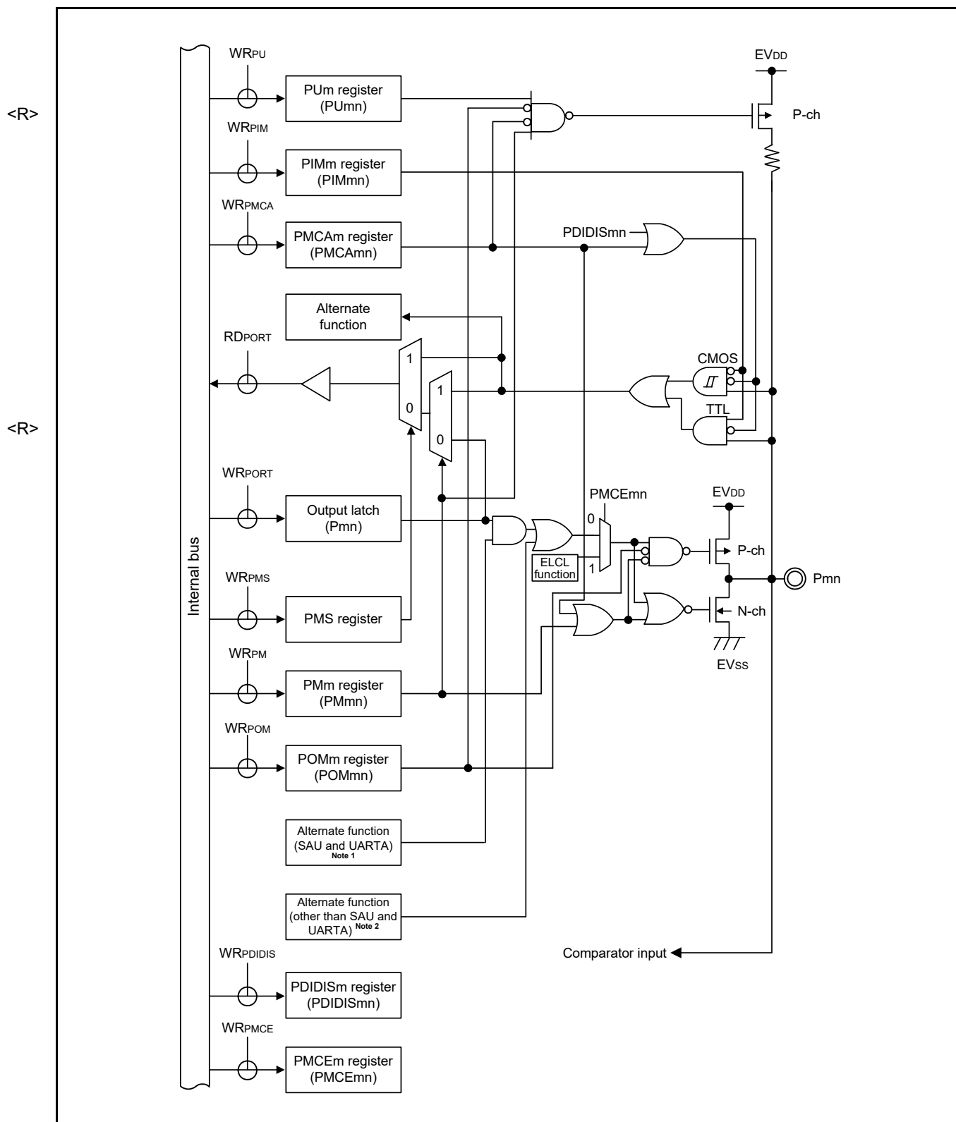
Figure 2 - 26 Pin Block Diagram for Pin Type 8-6-9
