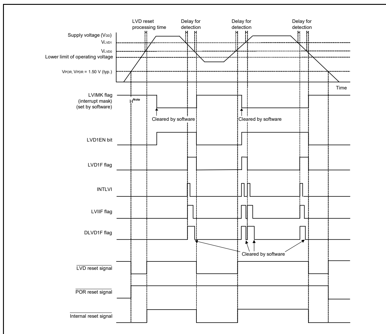
Figure 26 - 9 Timing of the Interrupt Request Signal Generated in LVD1
