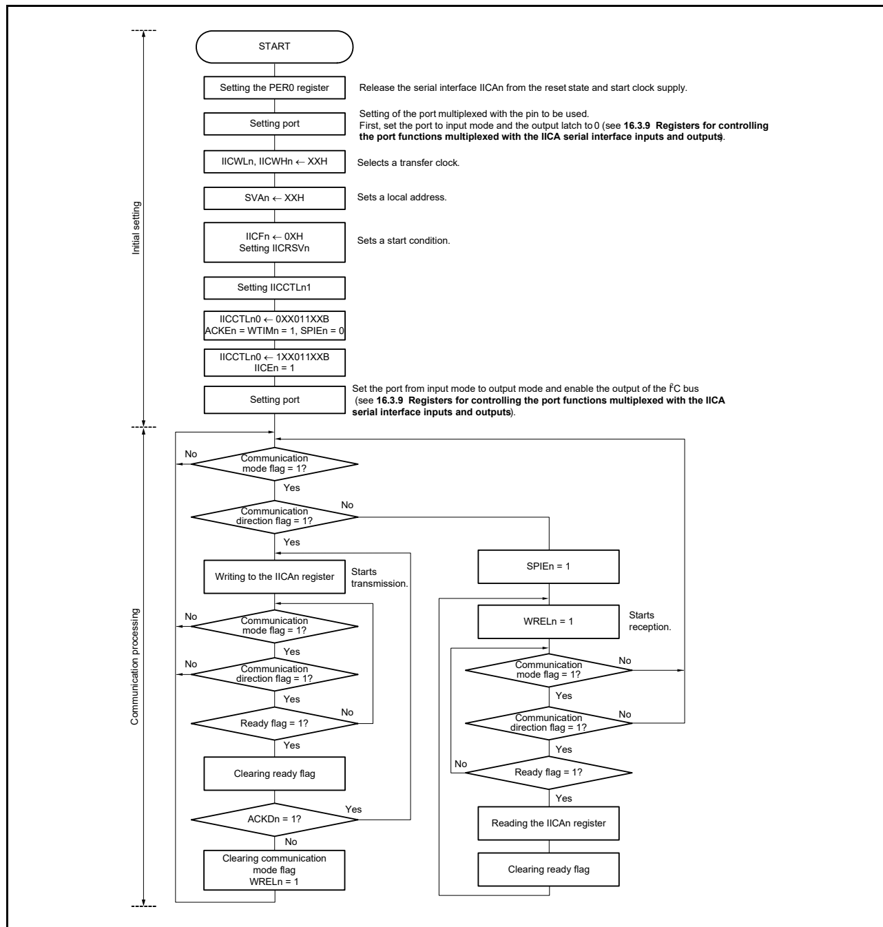
Figure 16 - 30 Slave Operation Flowchart (1)
