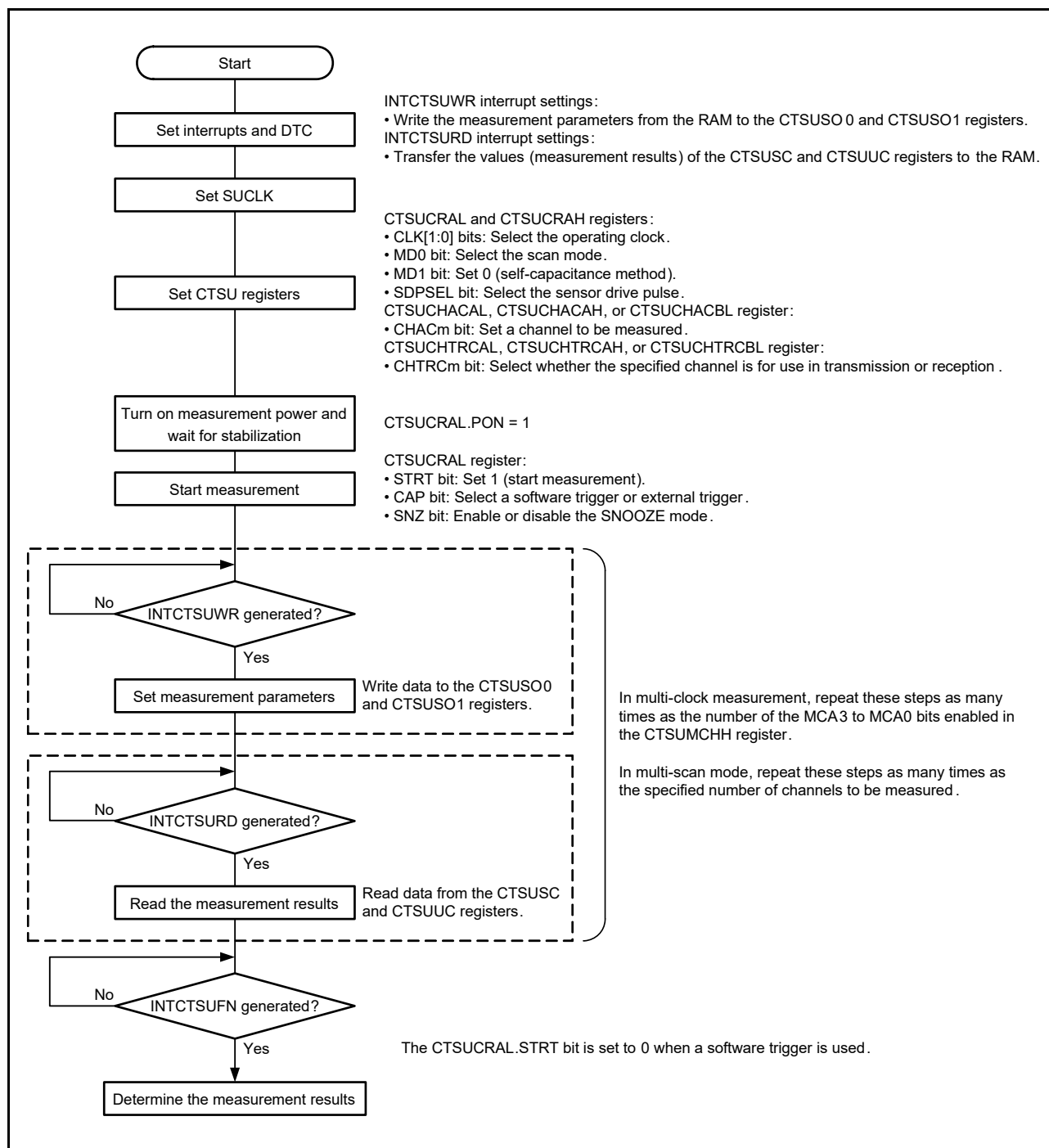
Figure 30 - 27 Control Procedure in the Self-capacitance Method
