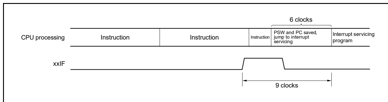
Figure 21 - 8 Interrupt Request Acknowledgment Timing (Minimum Time)
