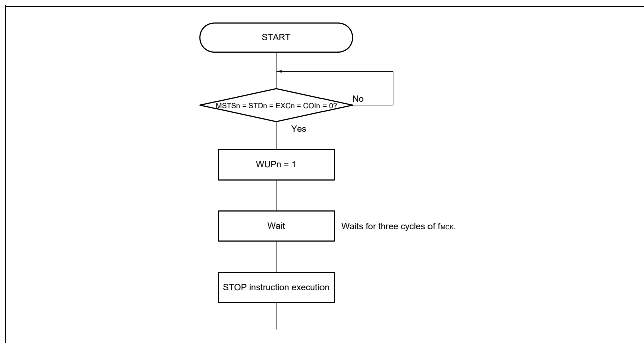
Figure 16 - 22 Flow for Setting WUPn = 1
