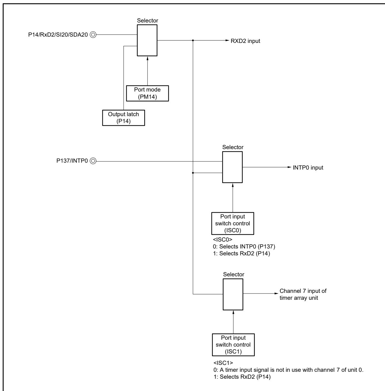
Figure 15 - 100 Port Configuration for Reception of LIN in 30- to 40-pin Products
