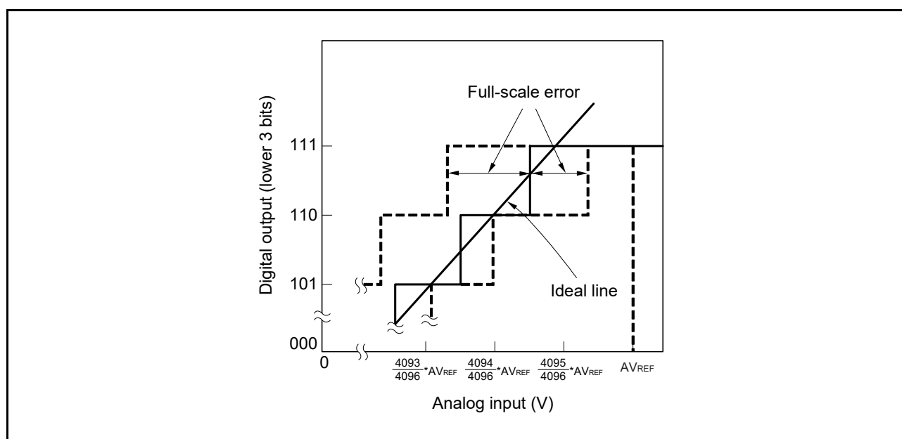
Figure 12 - 49 Full-scale Error
