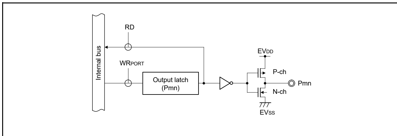
Figure 2 - 3 Pin Block Diagram for Pin Type 1-1-1
