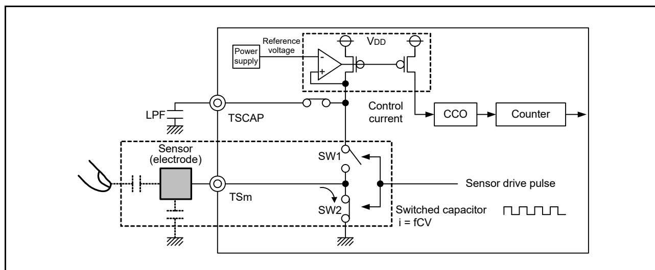
Figure 30 - 22 Discharging
