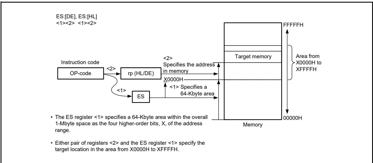
Figure 3 - 28 Example of ES:[DE], ES:[HL]
