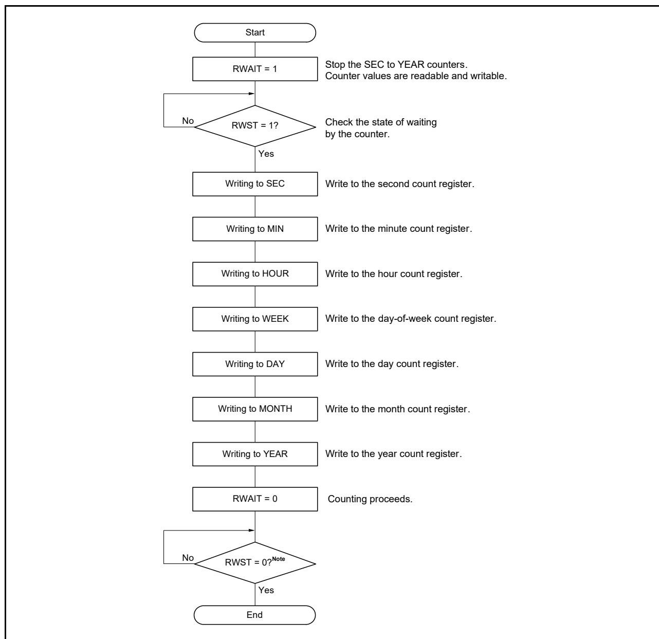
Figure 8 - 21 Procedure for Writing to the Realtime Clock
