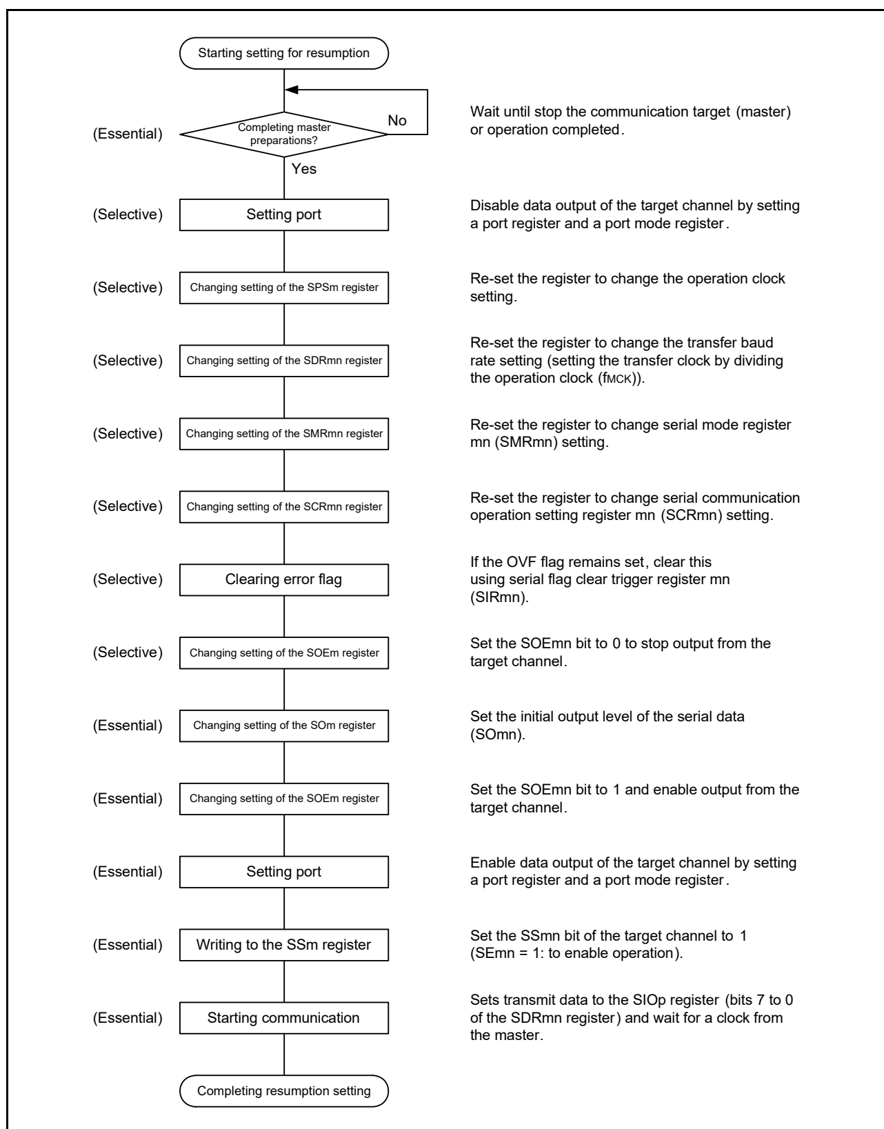
Figure 15 - 53 Procedure for Resuming Slave Transmission
