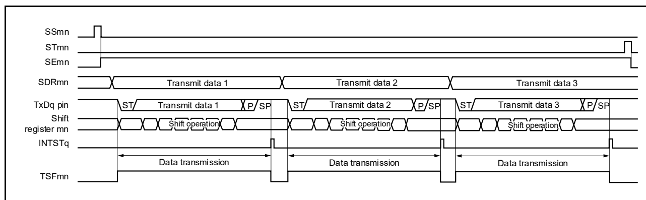
Figure 15 - 80 Timing Chart of UART Transmission (in Single-transmission Mode)
