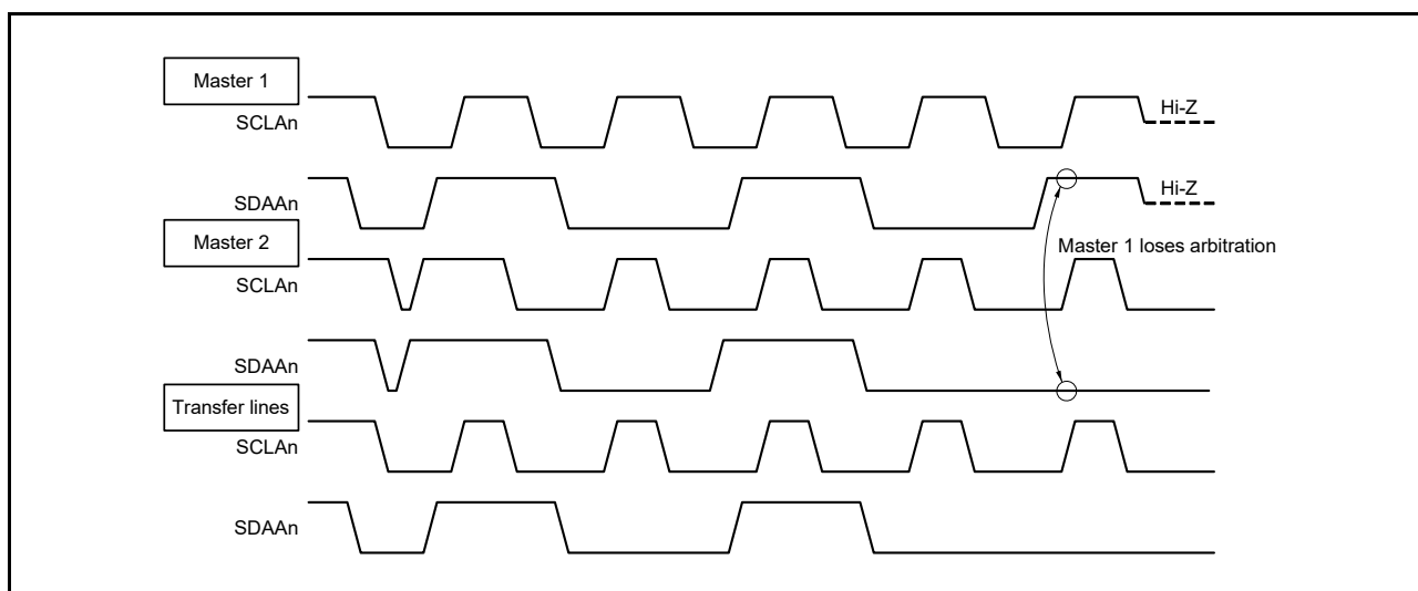
Figure 16 - 21 Arbitration Timing Example
