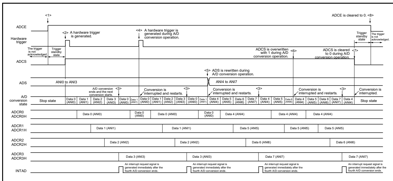
Figure 12 - 32 Example of Hardware Trigger Wait Mode (Scan Mode, Sequential Conversion Mode) Operation Timing
