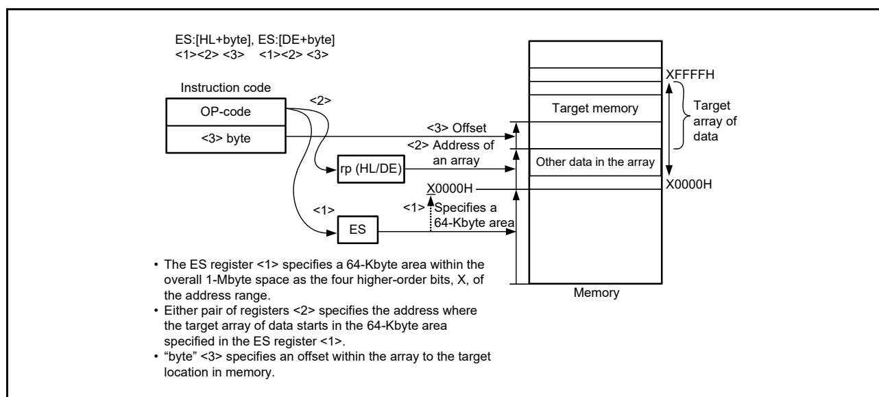
Figure 3 - 33 Example of ES:[HL+byte], ES:[DE+byte]
