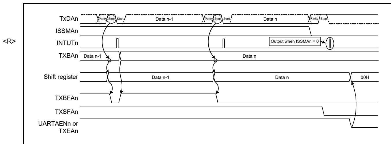
Figure 17 - 20 Timing Chart When Continuous Transmission Is Completed
