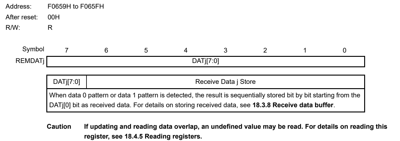
Figure 18 - 22 Format of Receive Data j Register (REMDATj)
