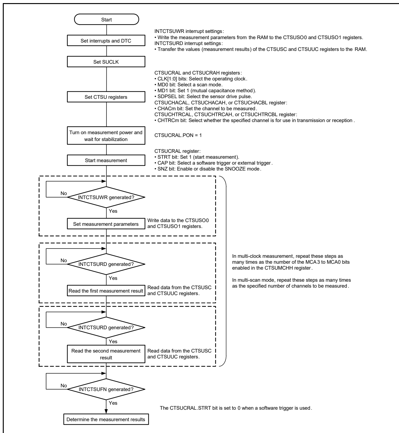
Figure 30 - 28 Control Procedure in the Mutual Capacitance Method
