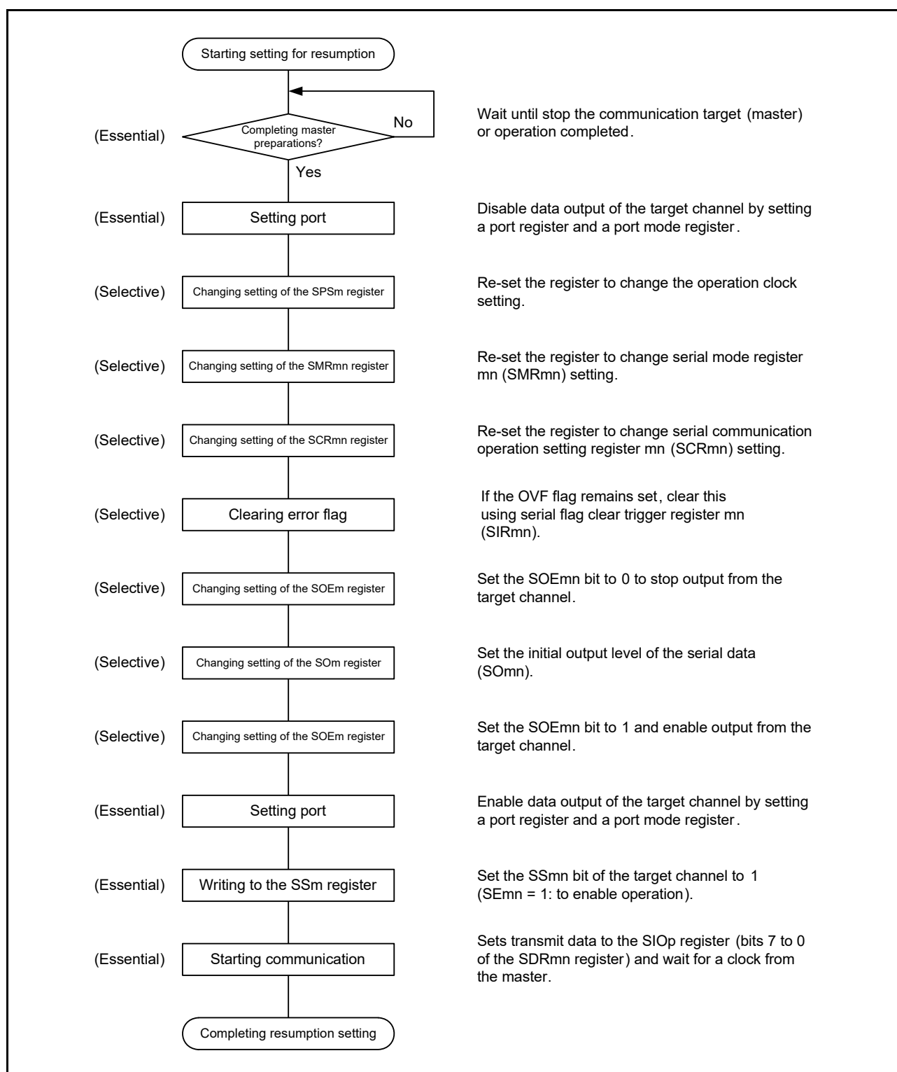
Figure 15 - 67 Procedure for Resuming Slave Transmission/Reception
