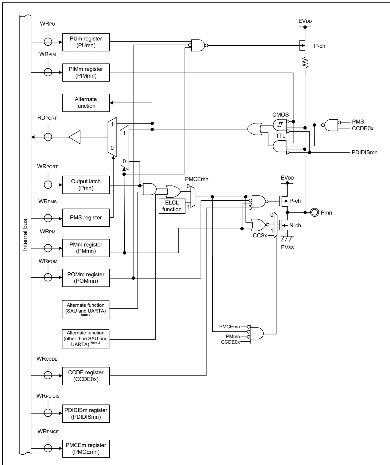
&lt;R&gt; Figure 2 - 32 Pin Block Diagram for Pin Type 8-38-2
