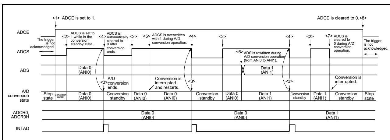
Figure 12 - 19 Example of Software Trigger No-wait Mode (Select Mode, One-shot Conversion Mode) Operation Timing
