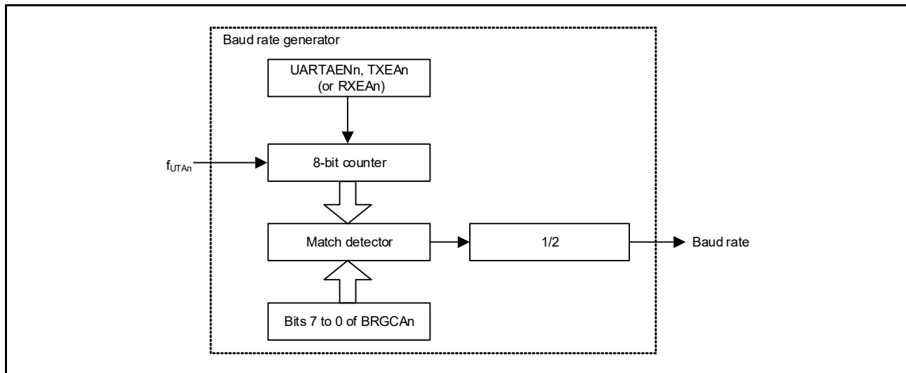
Figure 17 - 24 Configuration of Baud Rate Generator
