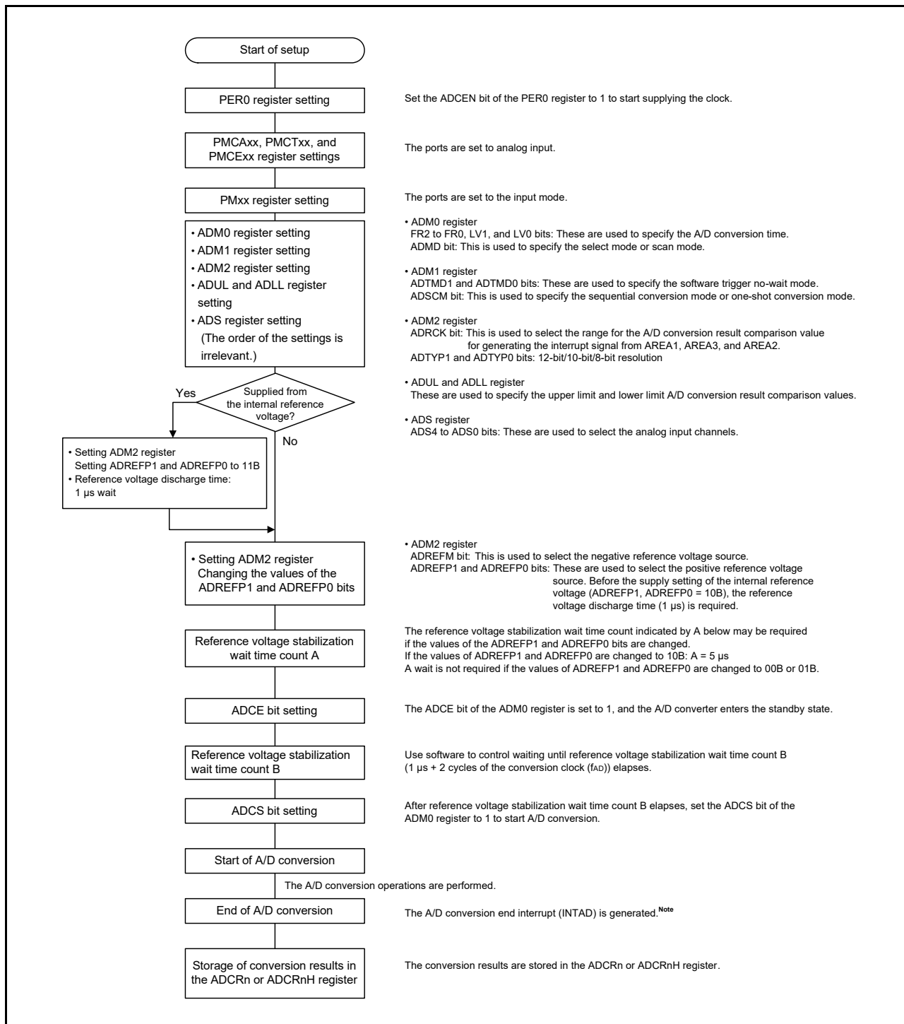
Figure 12 - 34 Settings in Software Trigger No-wait Mode
