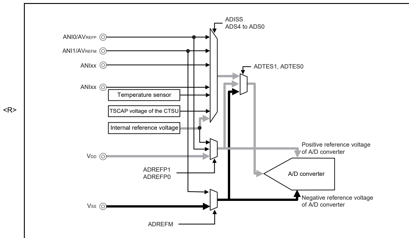
Figure 27 - 19 Configuration of Testing of the A/D Converter
