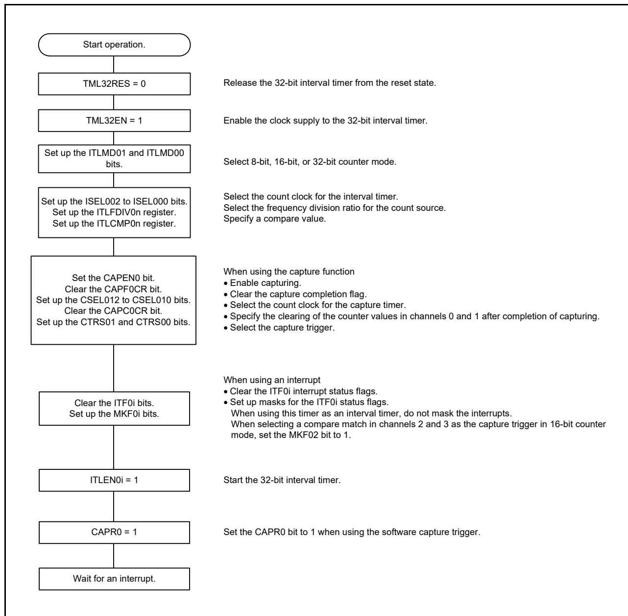
Figure 9 - 17 Procedure for Starting the 32-Bit Interval Timer
