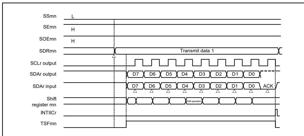
Figure 15 - 107 Timing Chart of Data Transmission
