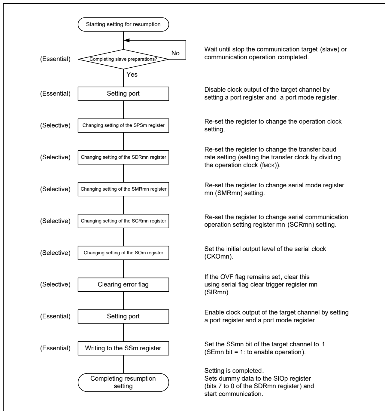
Figure 15 - 37 Procedure for Resuming Master Reception
