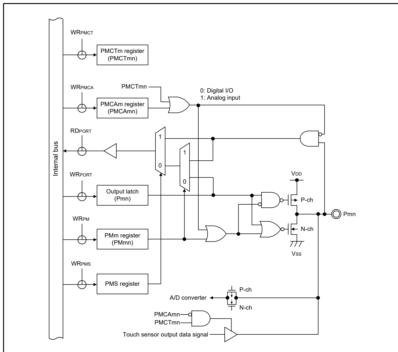
Figure 2 - 8 Pin Block Diagram for Pin Type 4-33-1
