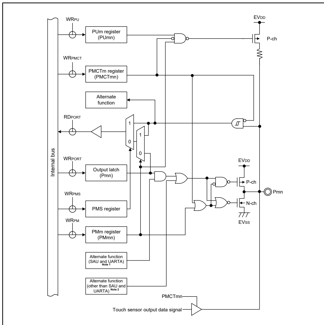
Figure 2 - 18 Pin Block Diagram for Pin Type 7-31-2
