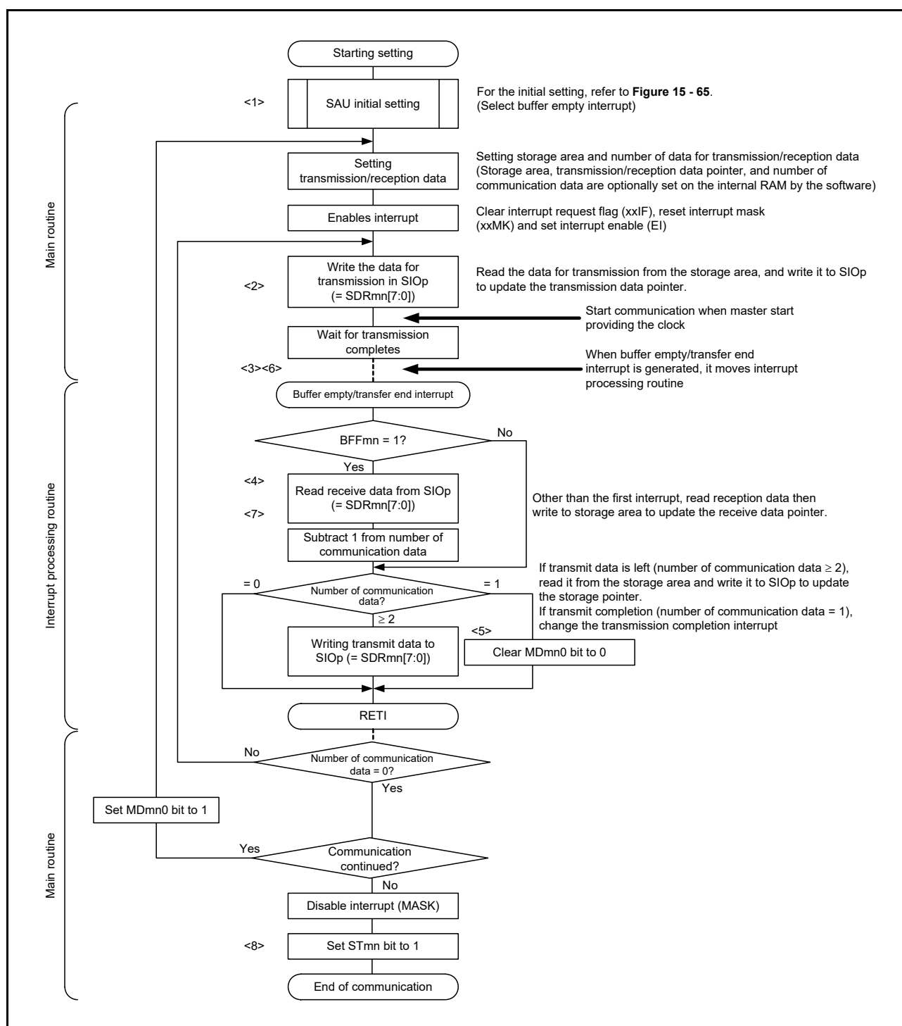
Figure 15 - 71 Flowchart of Slave Transmission/Reception (in Continuous Transmission/Reception Mode)
