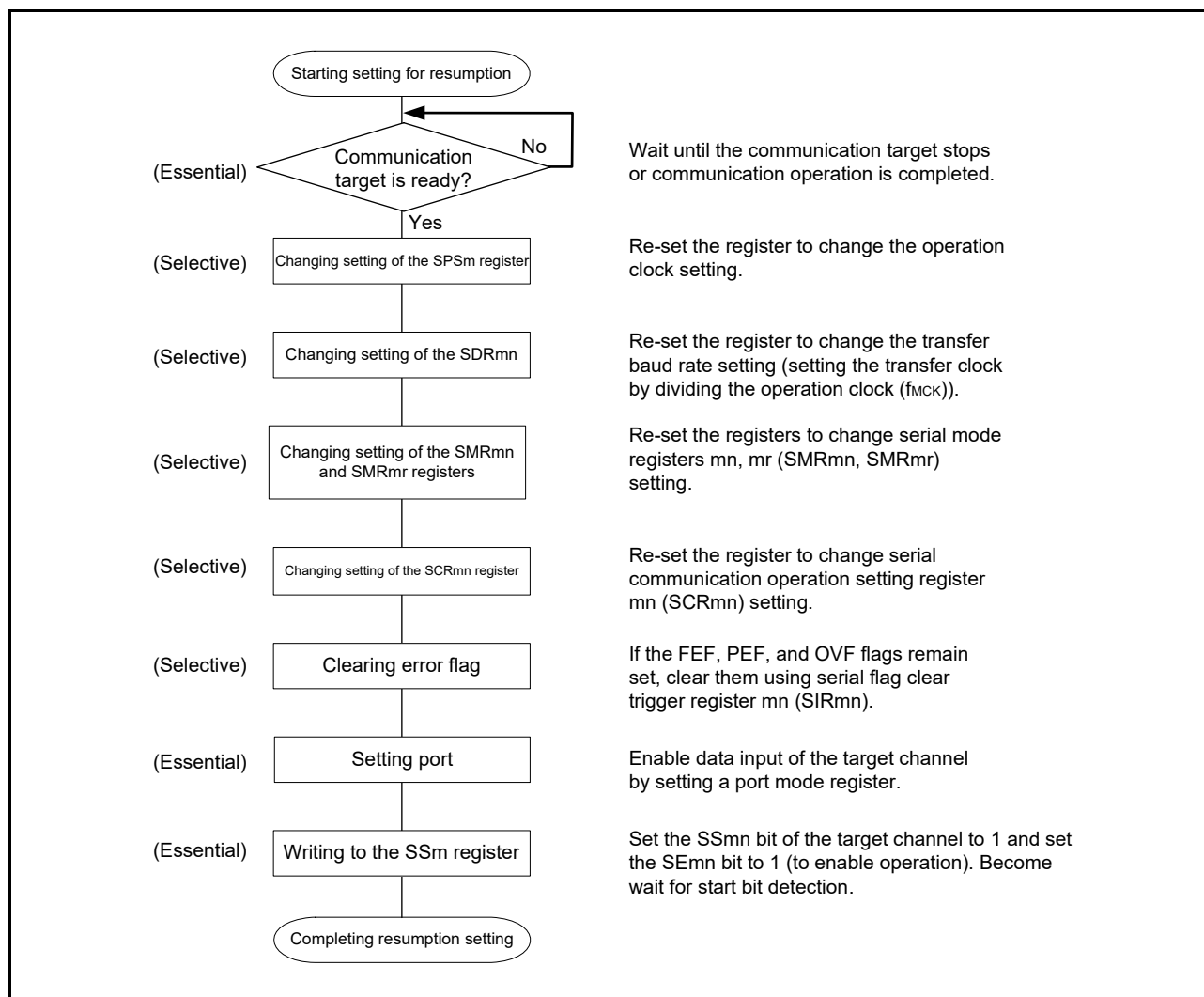
Figure 15 - 87 Procedure for Resuming UART Reception
