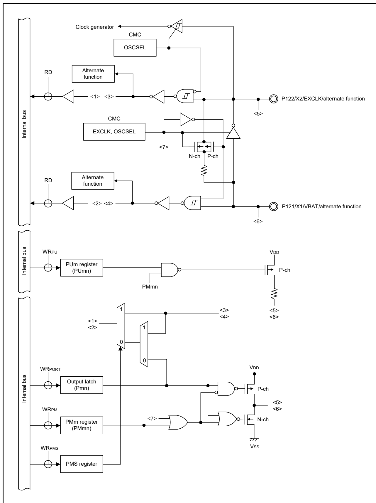
Figure 2 - 14 Pin Block Diagram for Pin Type 7-2-1
