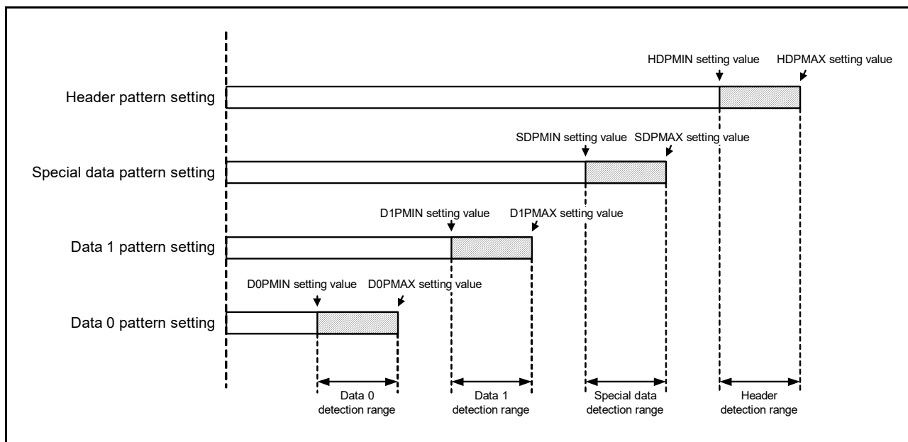
Figure 18 - 31 Examples of Setting Pattern Setting Registers
