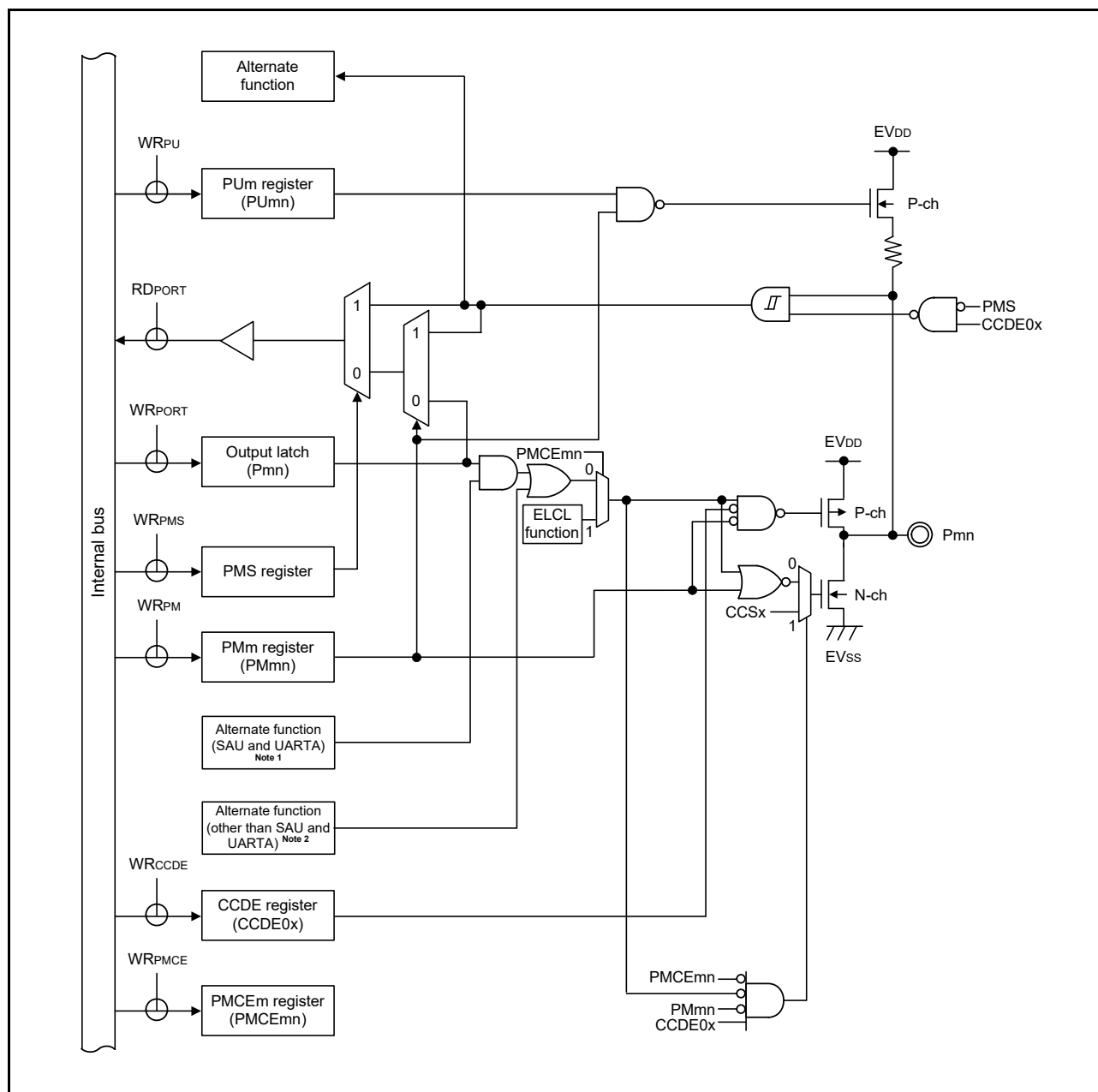
<R> Figure 2 - 21 Pin Block Diagram for Pin Type 7-38-1
