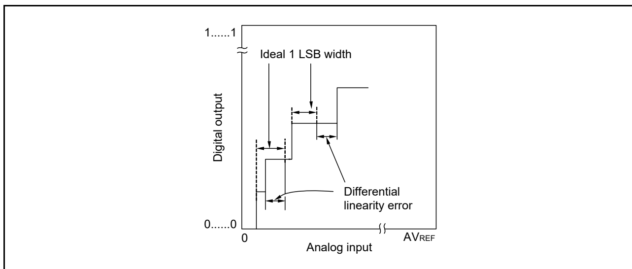
Figure 12 - 51 Differential Linearity Error
