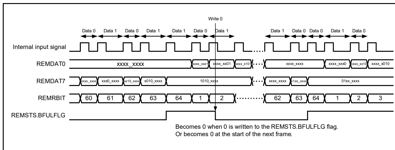
Figure 18 - 37 REMRBIT Register Operation (REMSTS.BFULFLG Flag = 1)
