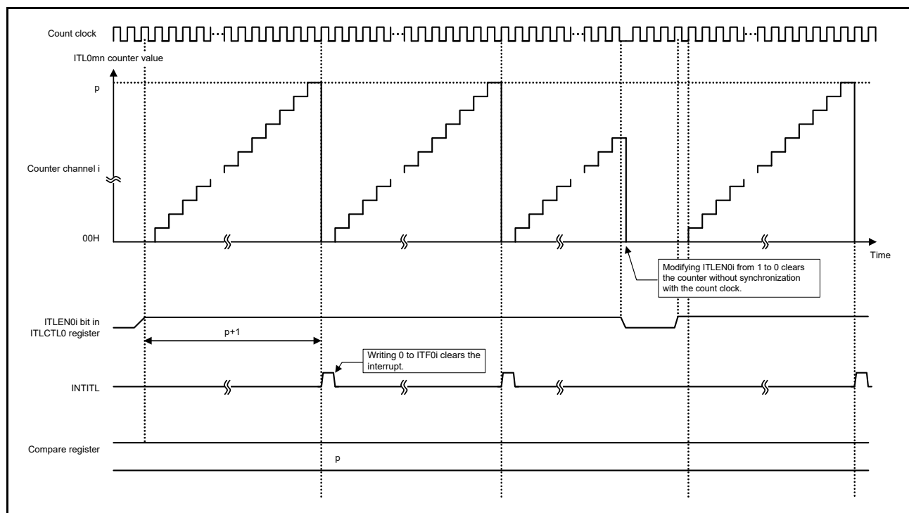
<R> Figure 9 - 14 Example of Timer Operation in 8-bit Counter Mode
