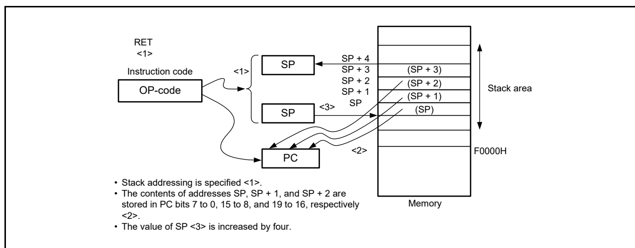
Figure 3 - 41 Example of RET
