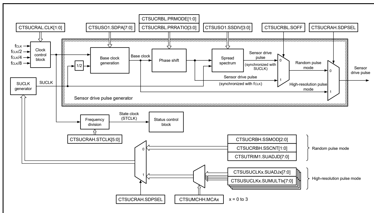
&lt;R&gt; Figure 30 - 4 Configuration of Clock Signals for Sensor Drive Pulse Output
