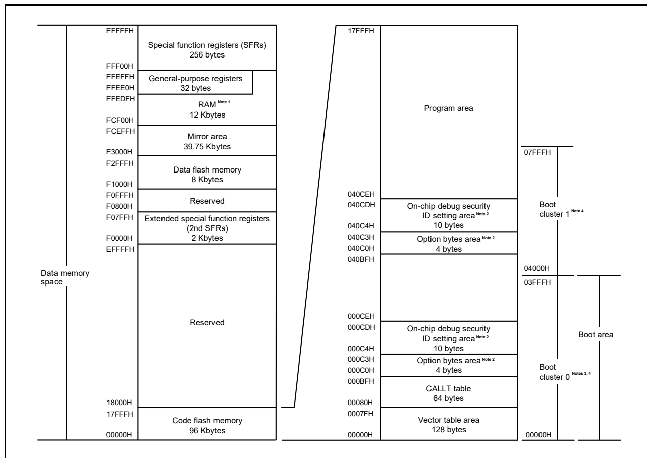
Figure 3 - 1 Memory Map (R7F100GxF (x = A, B, C, E, F, G, J, L))
