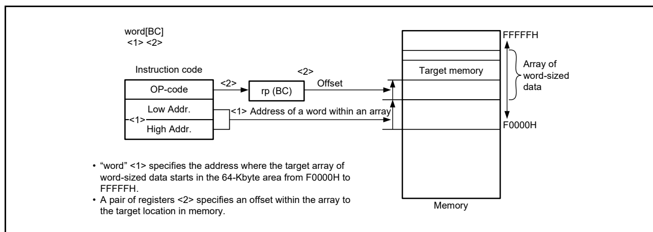
Figure 3 - 32 Example of word[BC]
