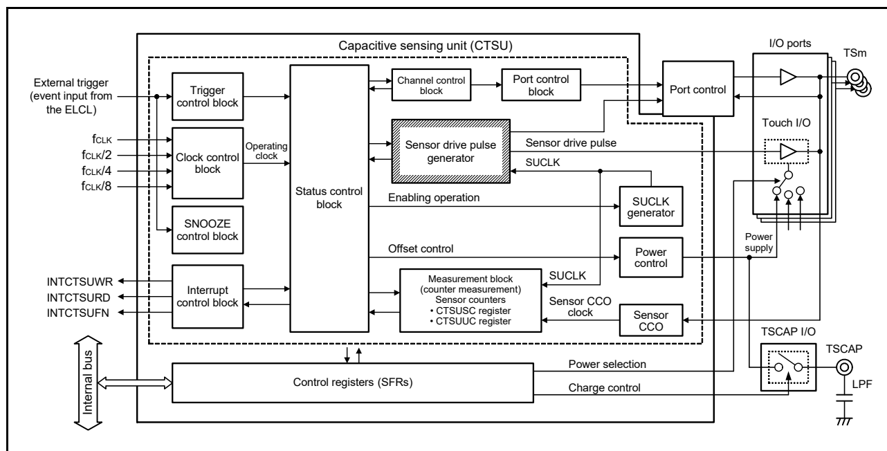
&lt;R&gt; Figure 30 - 3 Block Diagram of the CTSU
