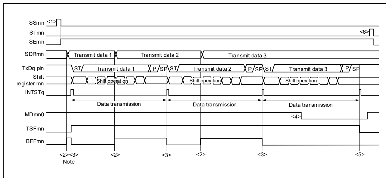
Figure 15 - 82 Timing Chart of UART Transmission (in Continuous Transmission Mode)
