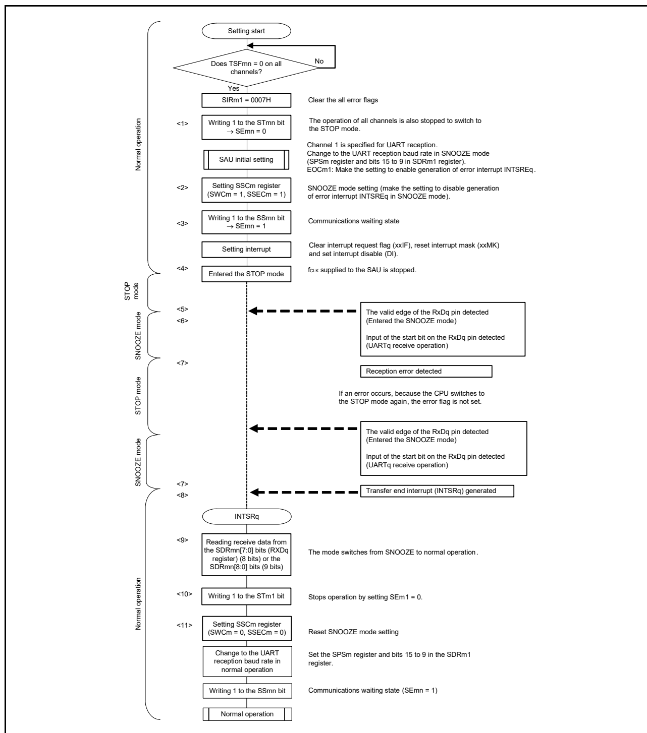
Figure 15 - 94 Flowchart of SNOOZE Mode Operation (EOCm1 = 1, SSECm = 1)
