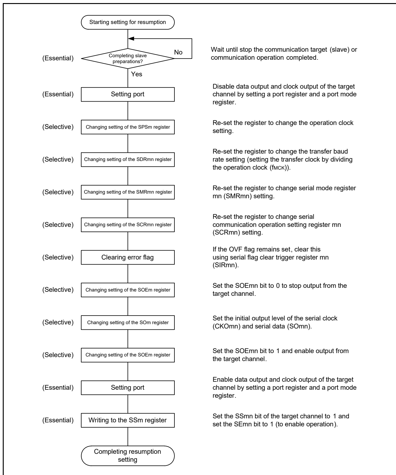
Figure 15 - 45 Procedure for Resuming Master Transmission/Reception
