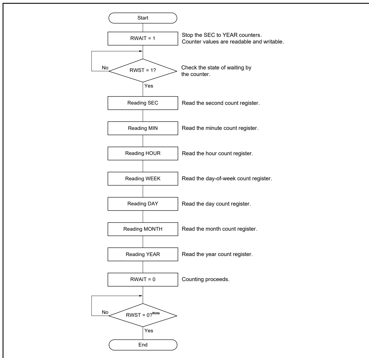
Figure 8 - 19 Procedure for Reading the Realtime Clock
