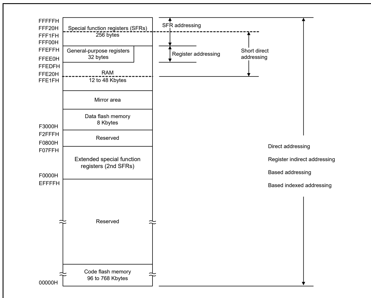
Figure 3 - 9 Correspondence Between Data Memory and Addressing
