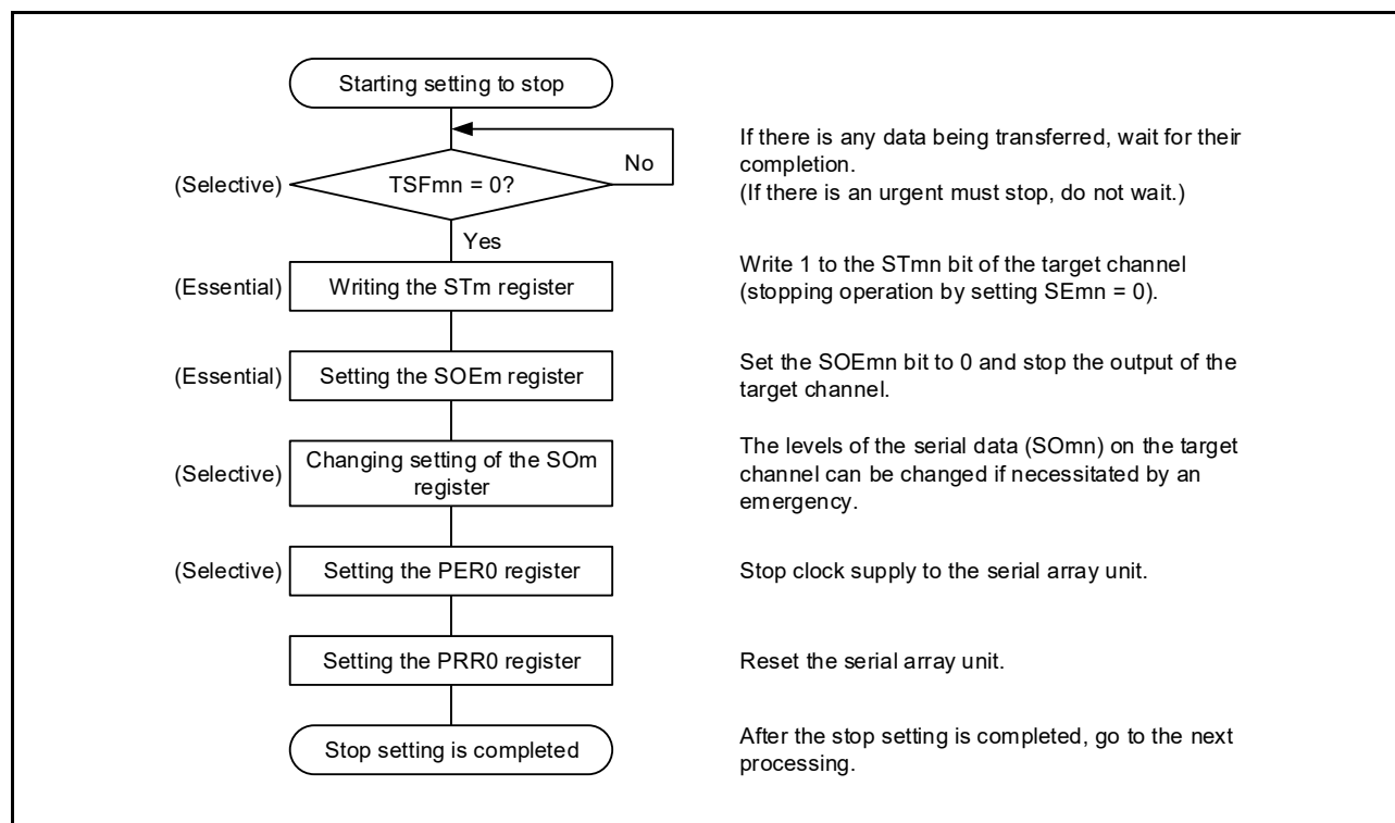
Figure 15 - 78 Procedure for Stopping UART Transmission
