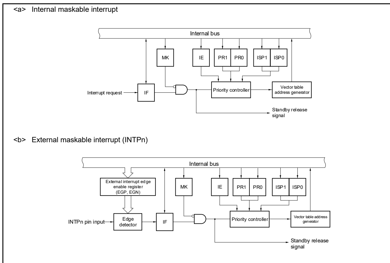
Figure 21 - 1 Basic Configuration of Interrupt Function (1/2)
