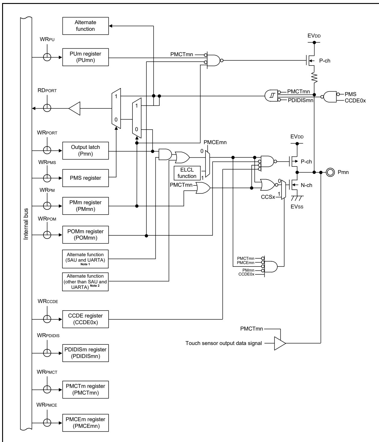
&lt;R&gt; Figure 2 - 22 Pin Block Diagram for Pin Type 7-39-1
