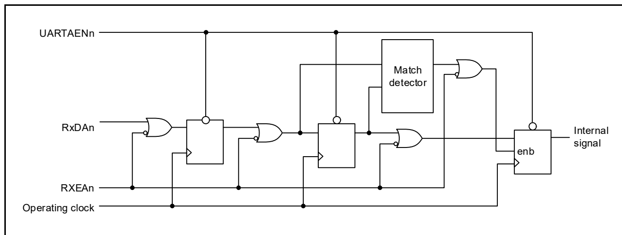
Figure 17 - 23 Noise Filter
