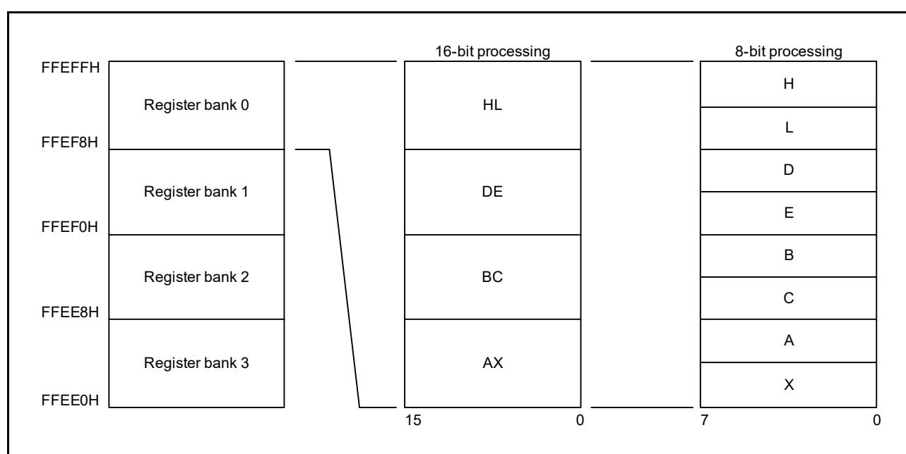
Figure 3 - 13 Configuration of General-Purpose Registers (Function Name)
