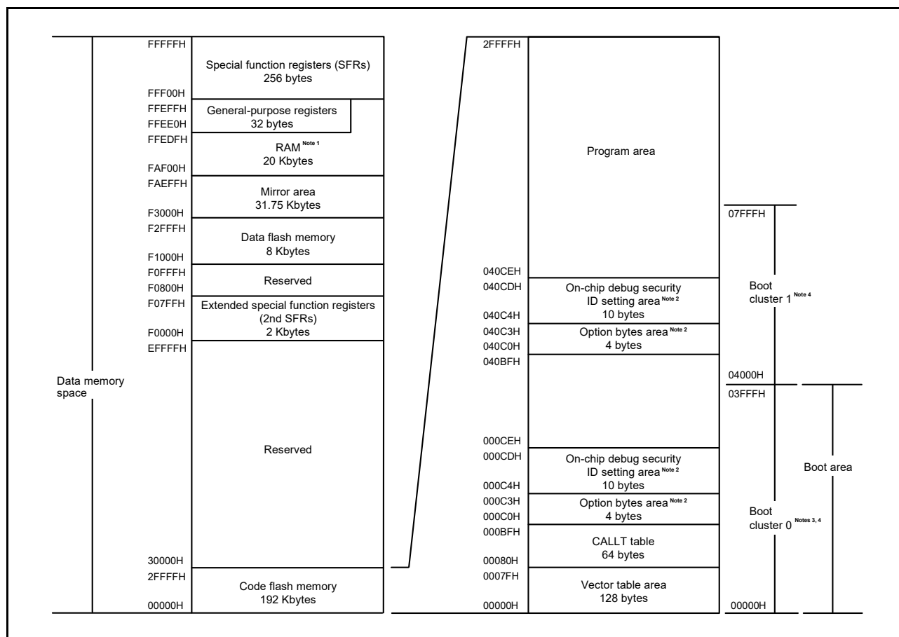
Figure 3 - 3 Memory Map (R7F100GxH (x = A, B, C, E, F, G, J, L, M, P))
