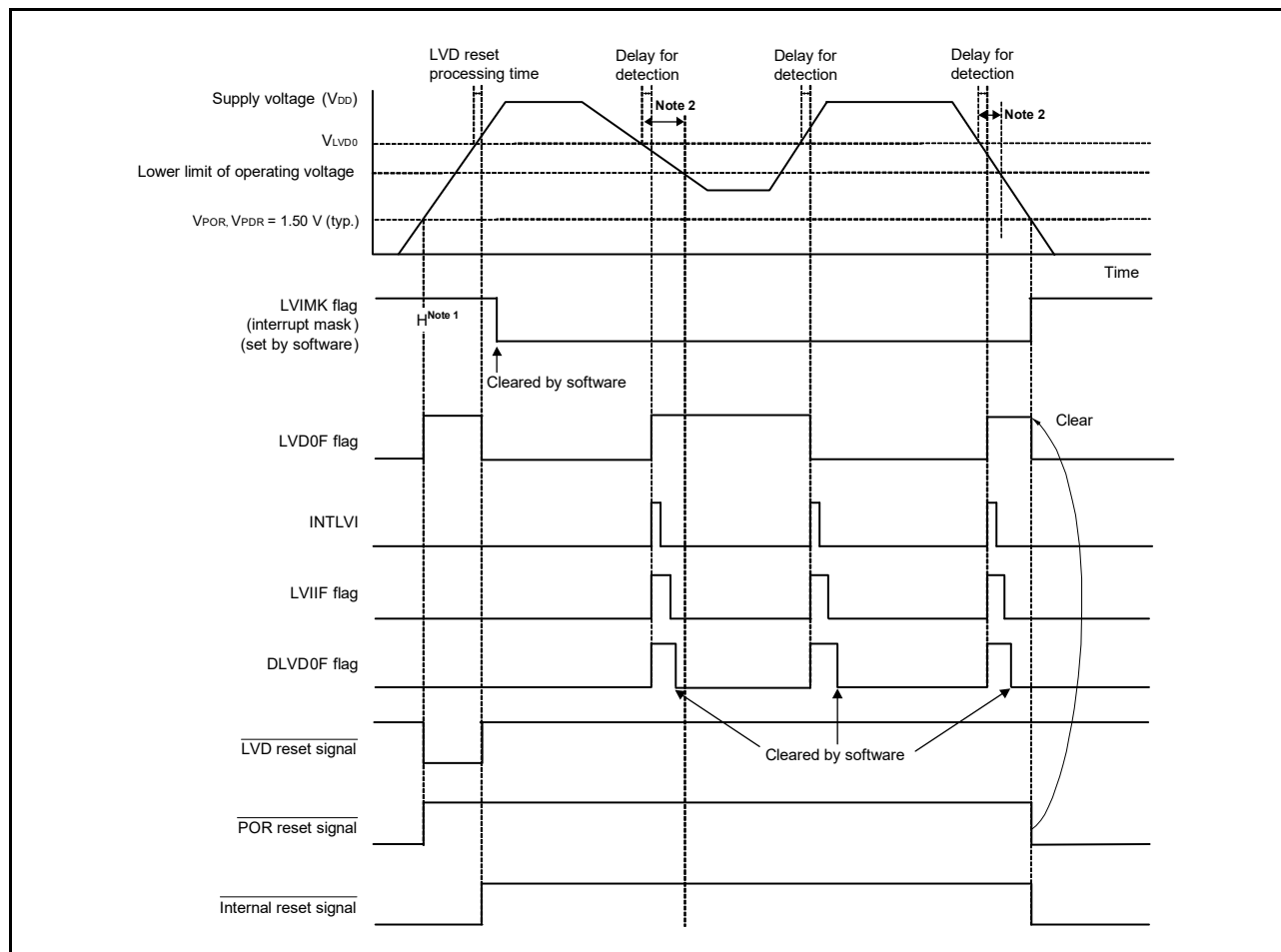
Figure 26 - 8 Timing of the Interrupt Request Signal Generated in LVD0
