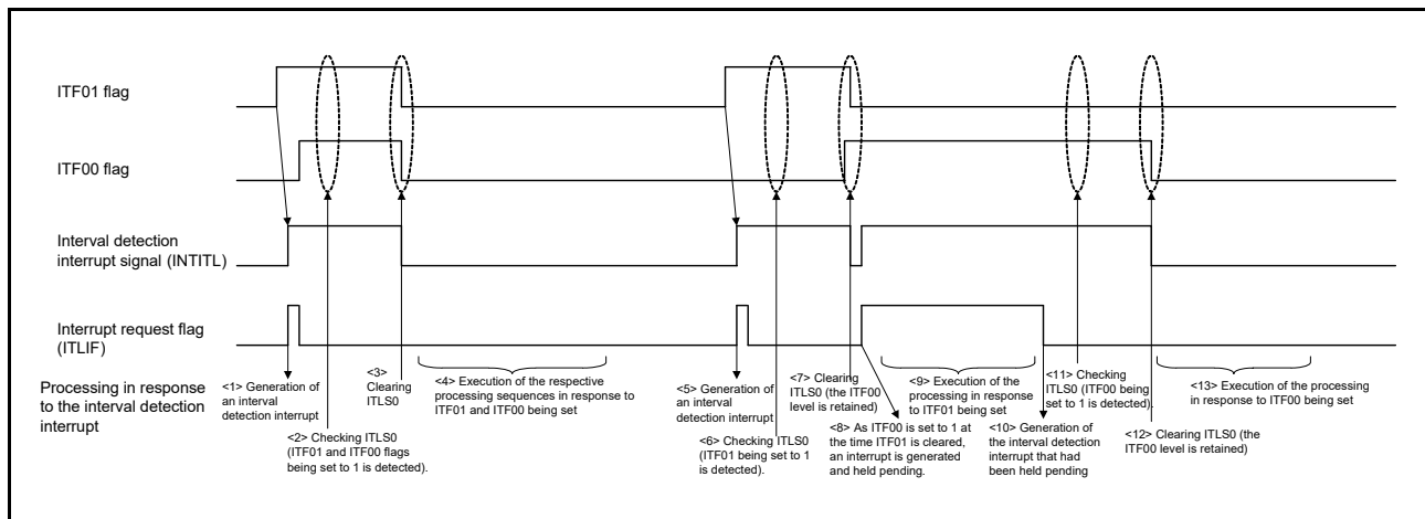
Figure 9 - 16 Example of Clearing the Detected Flags
