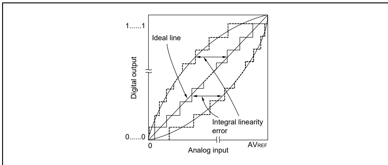
Figure 12 - 50 Integral Linearity Error
