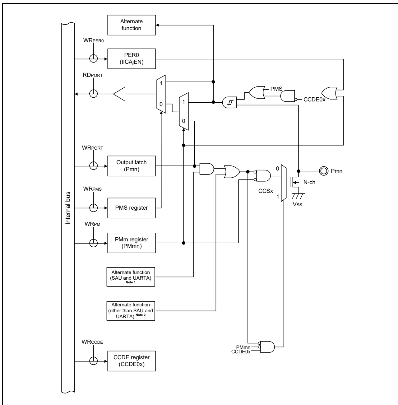
&lt;R&gt; Figure 2 - 34 Pin Block Diagram for Pin Type 12-38-2
