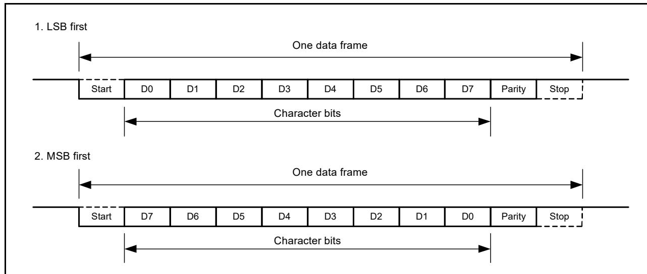
Figure 17 - 14 Transmit/Receive Data Format
