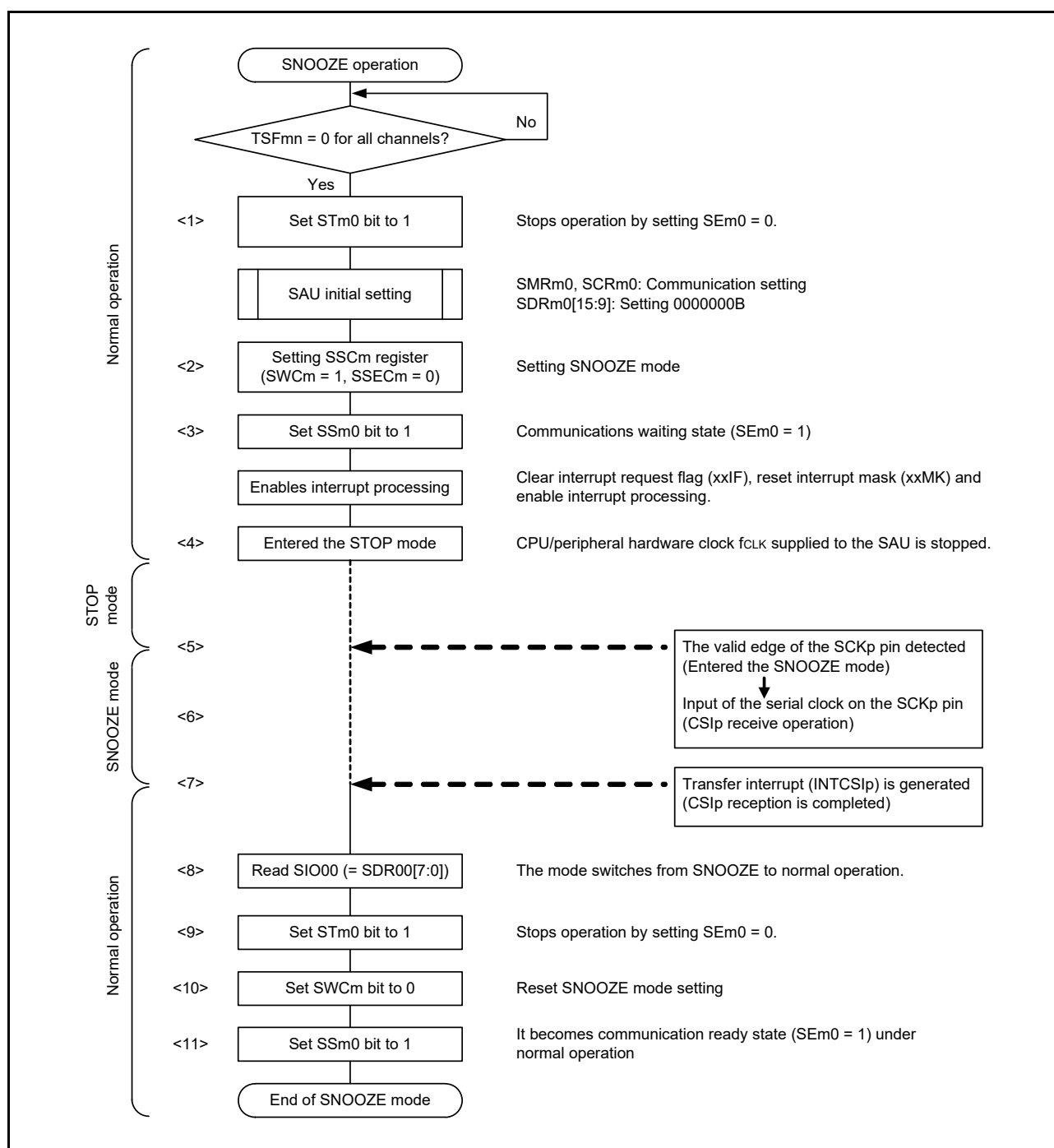
Figure 15 - 73 Flowchart of SNOOZE Mode Operation (once startup)
