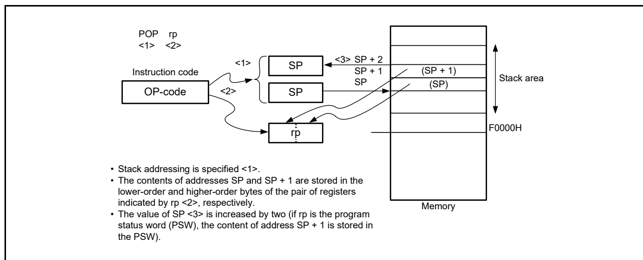
Figure 3 - 39 Example of POP
