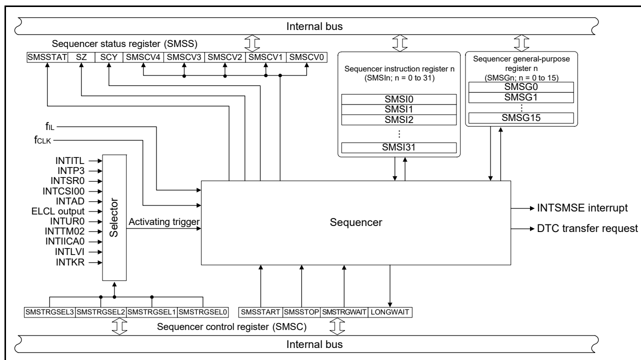
Figure 29 - 1 Block Diagram of the SNOOZE Mode Sequencer
