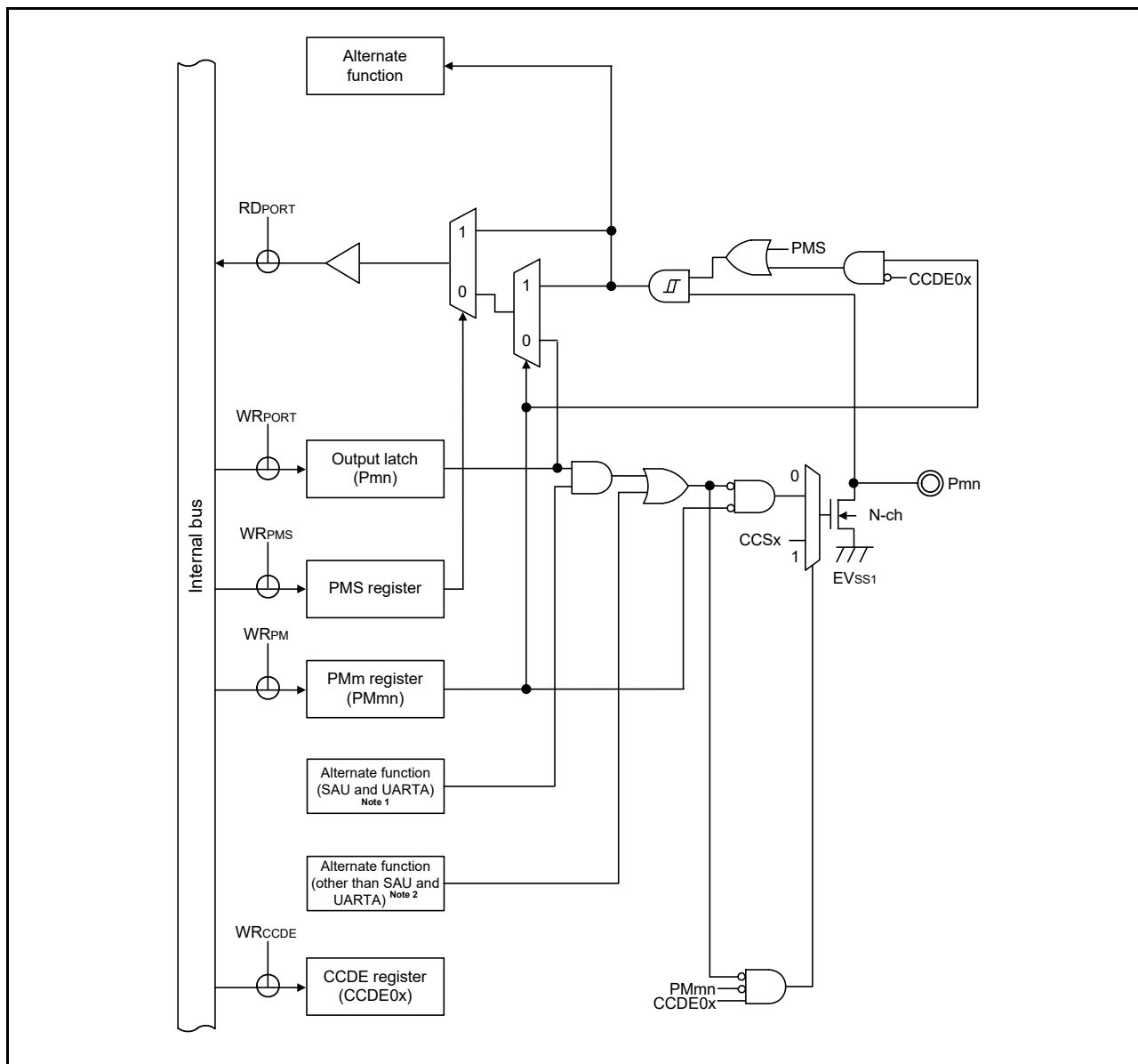
&lt;R&gt; Figure 2 - 33 Pin Block Diagram for Pin Type 12-38-1
