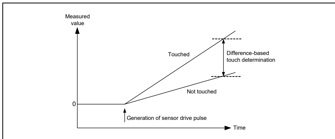
Figure 30 - 23 Change in Measured Value When the Electrode Is Touched or Not Touched
