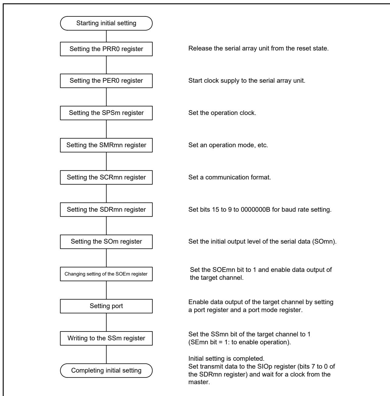
Figure 15 - 65 Initial Setting Procedure for Slave Transmission/Reception
