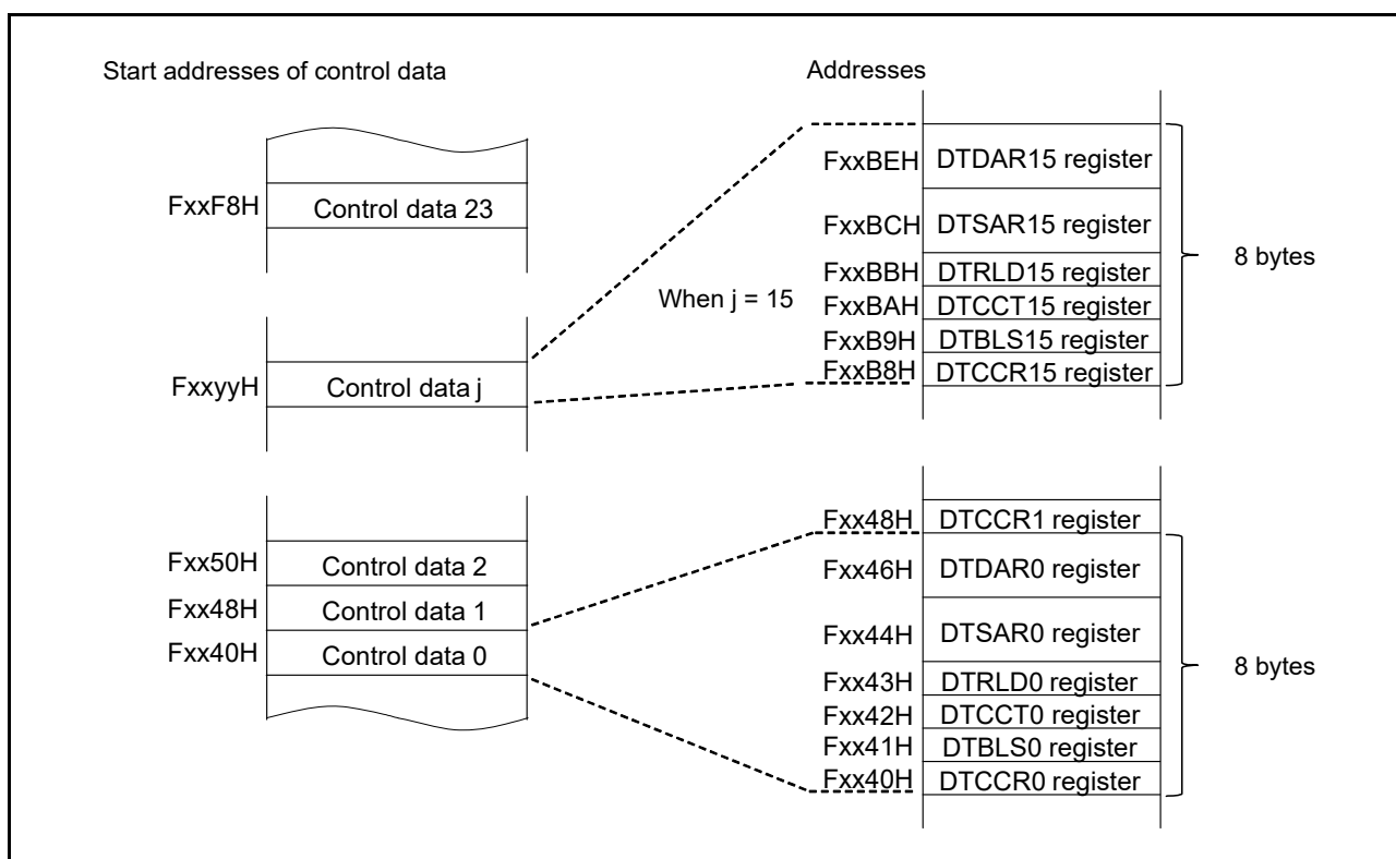
Figure 19 - 3 Control Data Allocation
