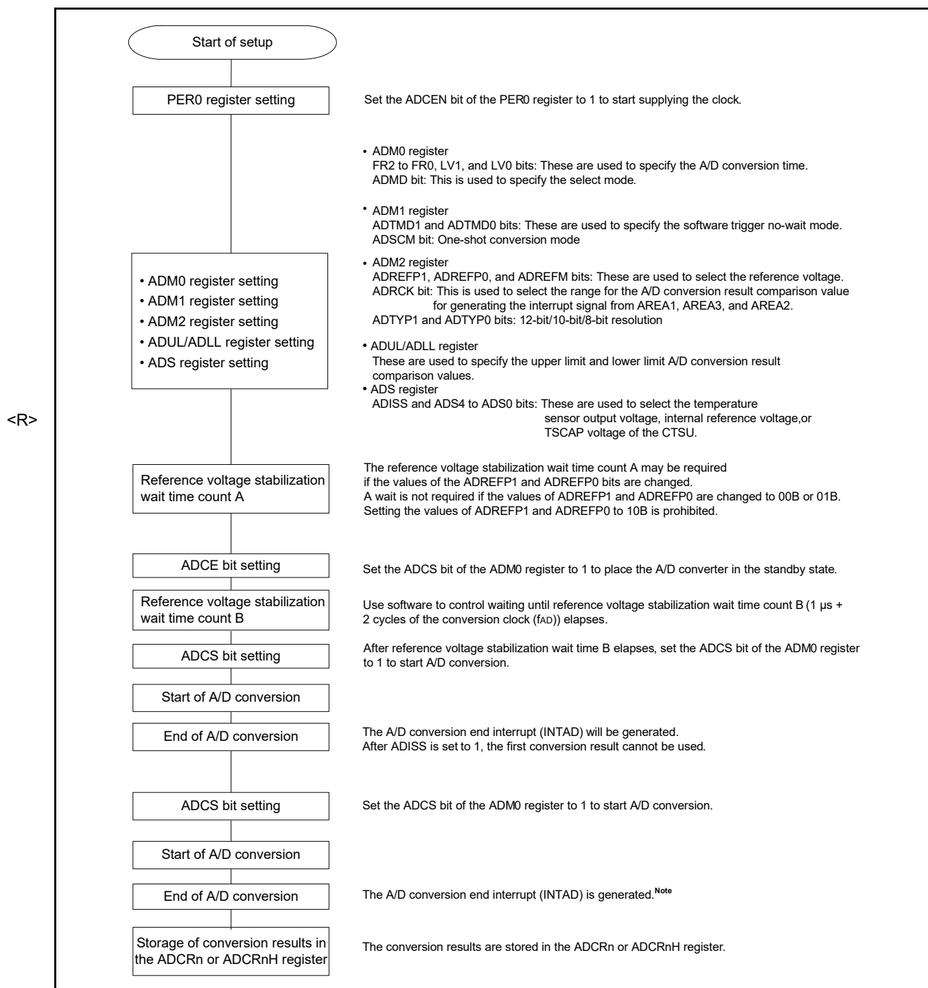
<R> Figure 12 - 38 Settings When Selecting the Temperature Sensor Output Voltage, Internal Reference Voltage, or TSCAP voltage of the CTSU
