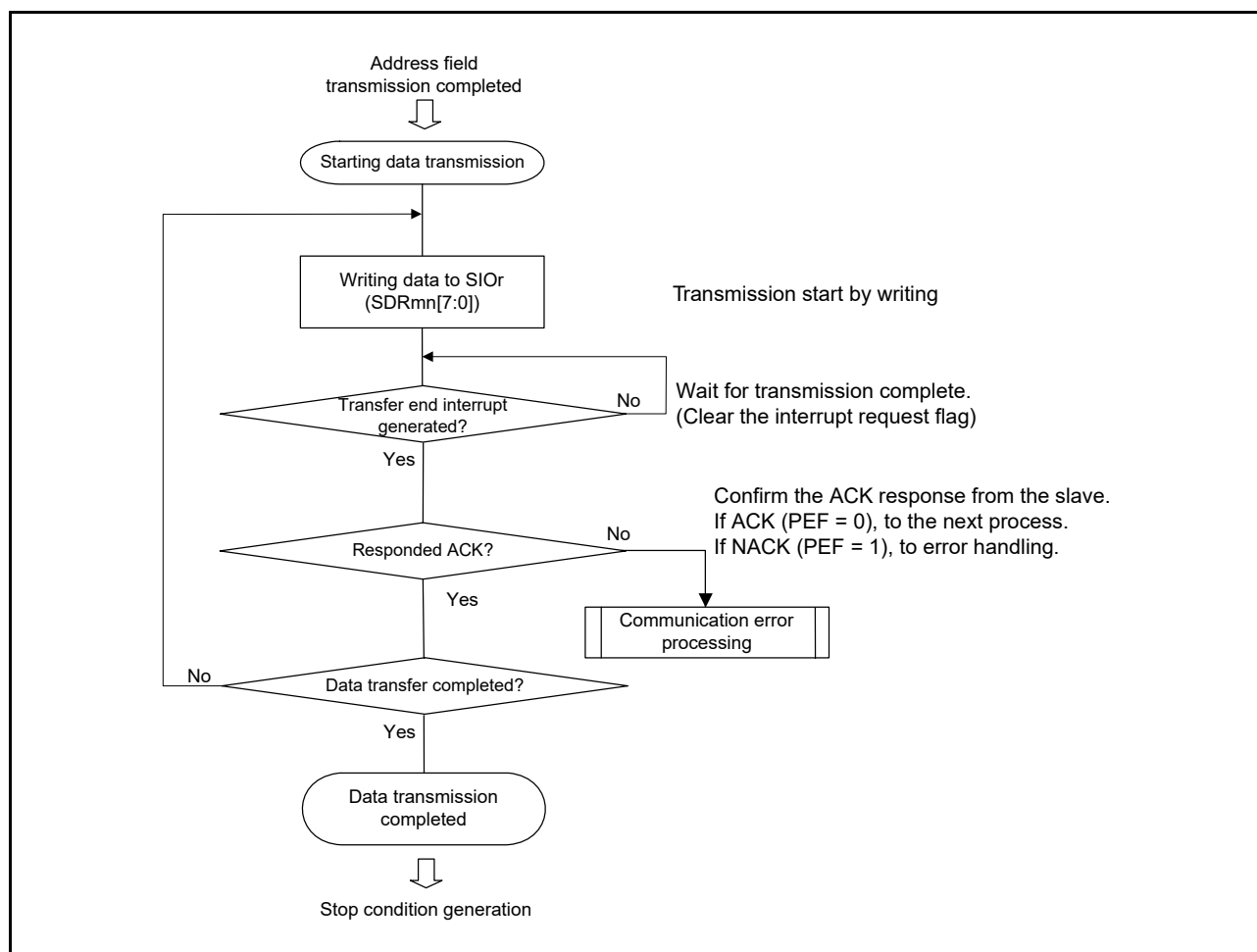
Figure 15 - 108 Flowchart of Simplified I 2 C Data Transmission
