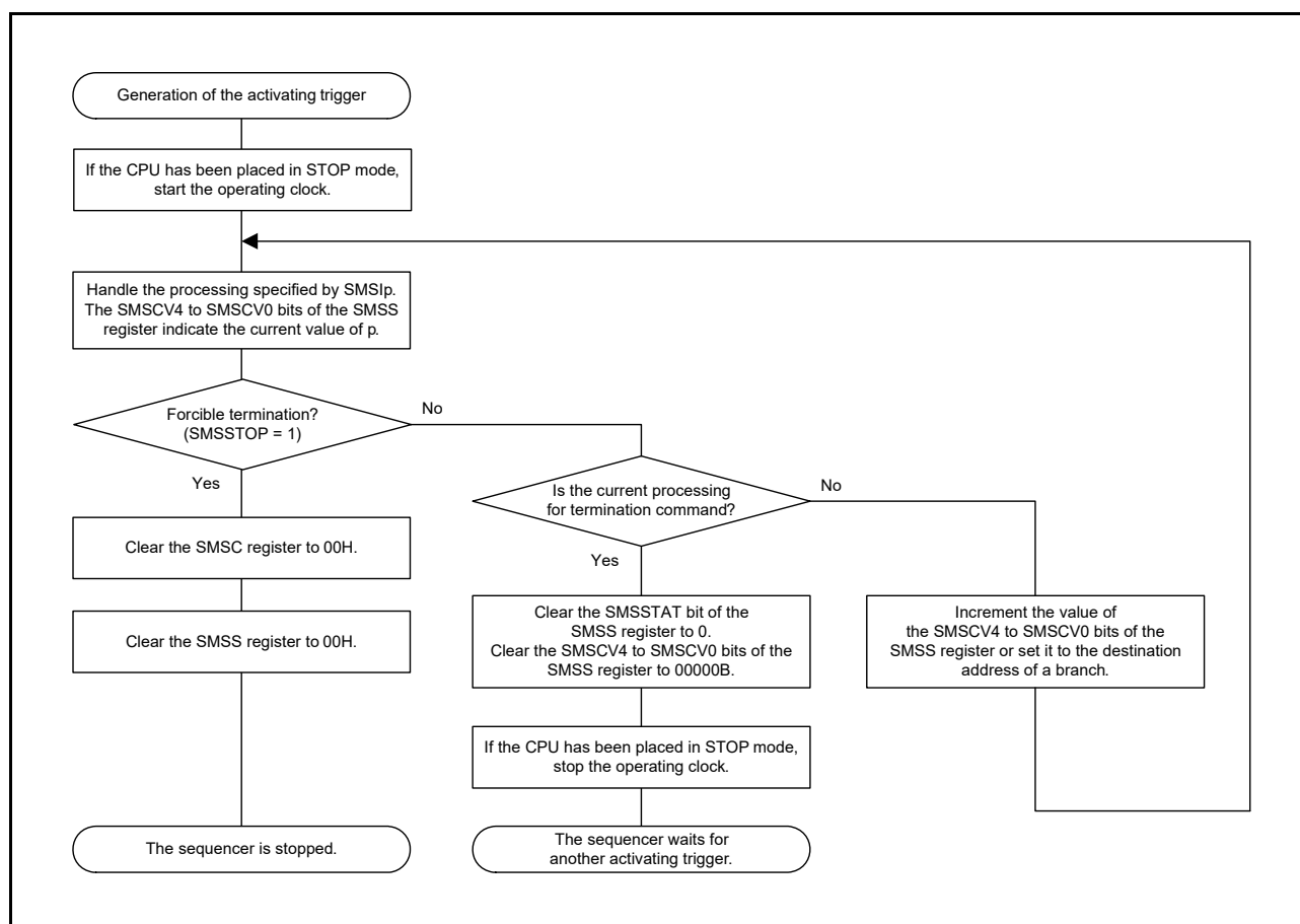
Figure 29 - 8 Flow of Internal Operations of the SNOOZE Mode Sequencer
