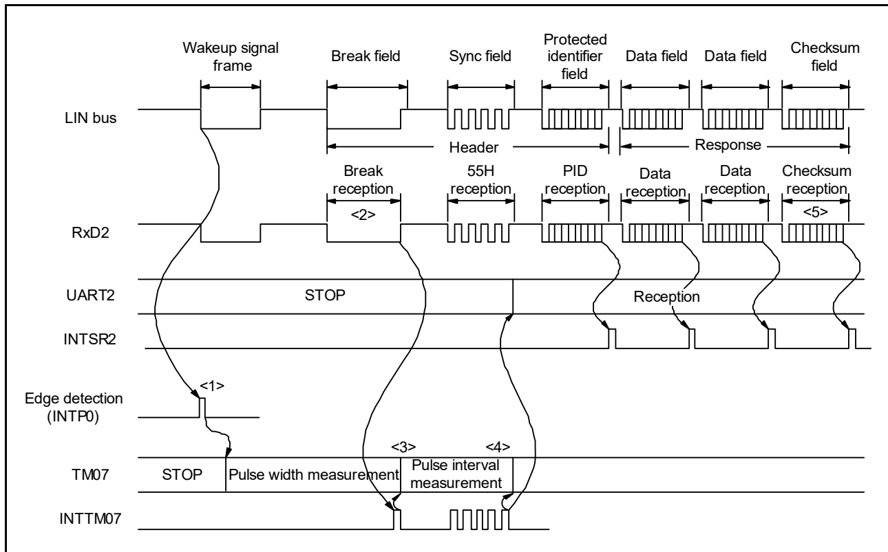
Figure 15 - 98 Reception Operation of LIN
