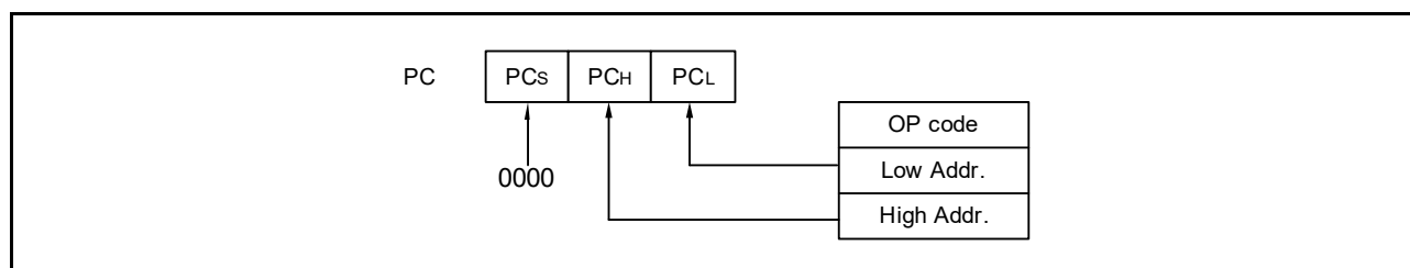
Figure 3 - 18 Example of CALL !addr16/BR !addr16
