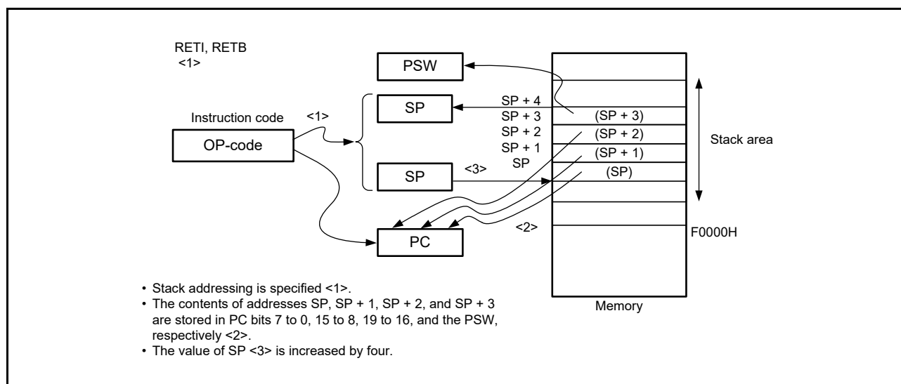
Figure 3 - 43 Example of RETI, RETB
