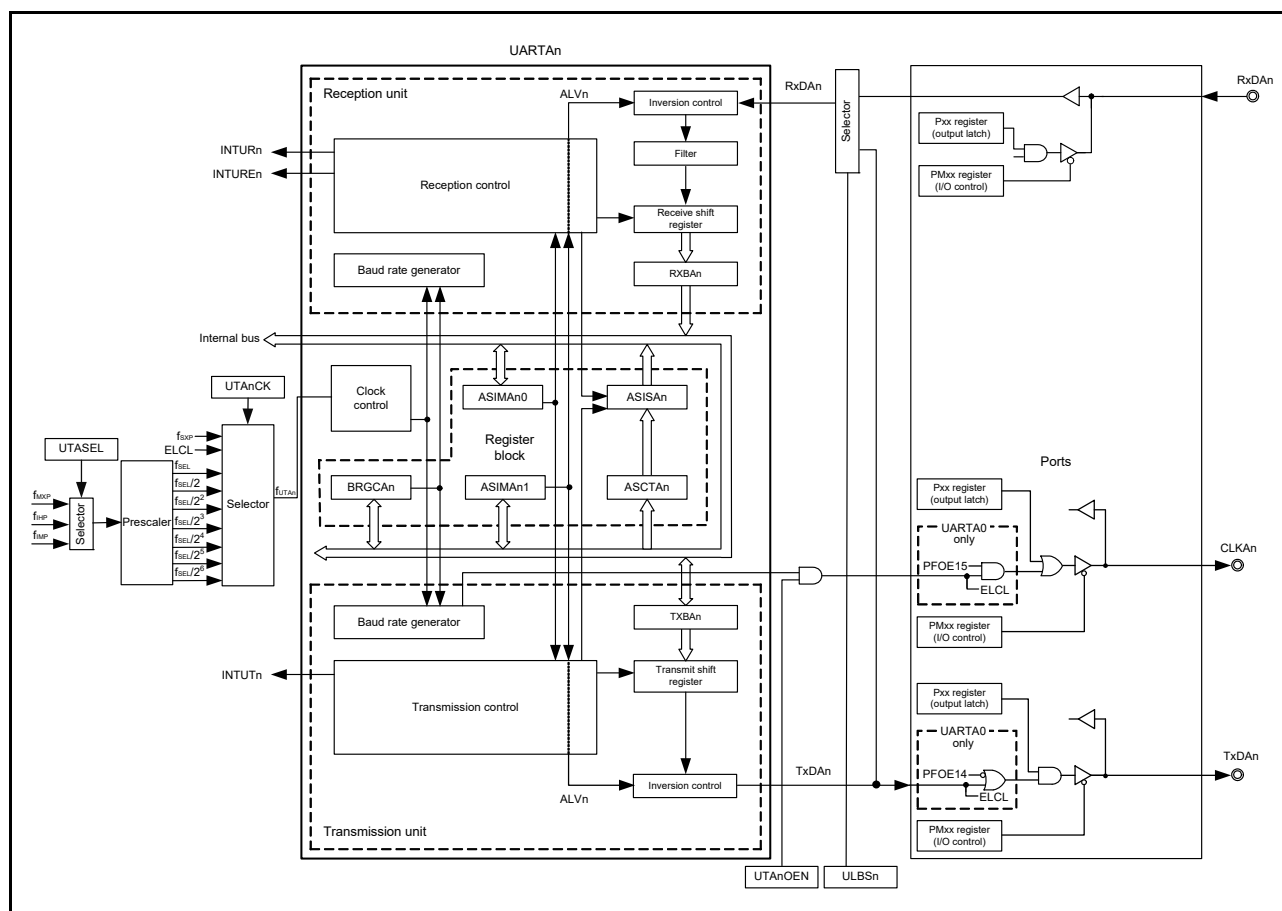
Figure 17 - 1 Block Diagram of UARTAn
