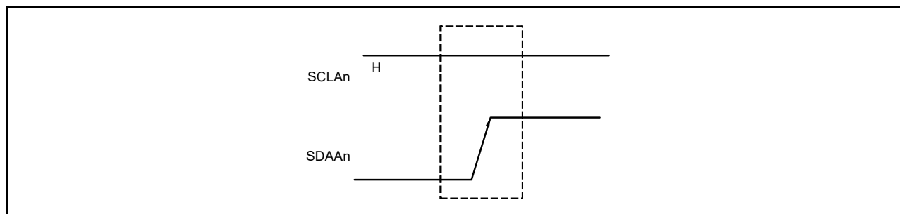
Figure 16 - 19 Stop Condition
