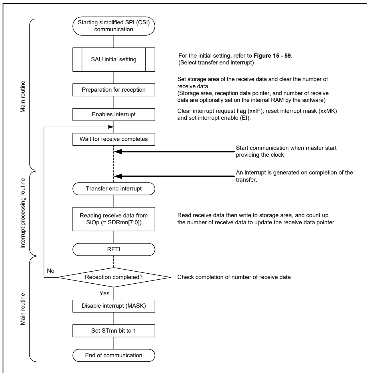
Figure 15 - 63 Flowchart of Slave Reception (in Single-reception Mode)
