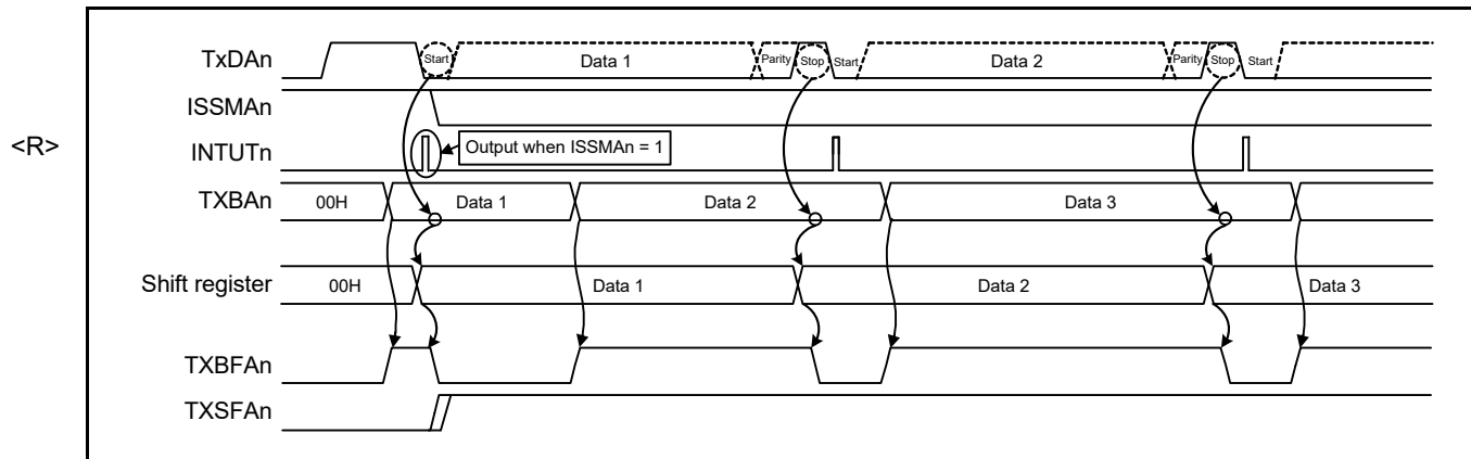
Figure 17 - 19 Timing Chart When Continuous Transmission Is Started
