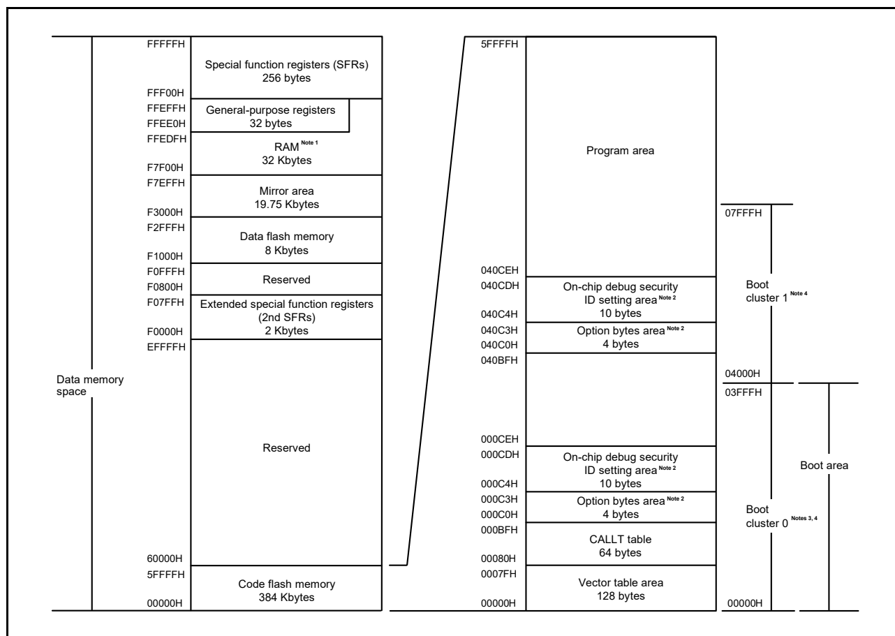
Figure 3 - 5 Memory Map (R7F100GxK (x = F, G, J, L, M, P, S))
