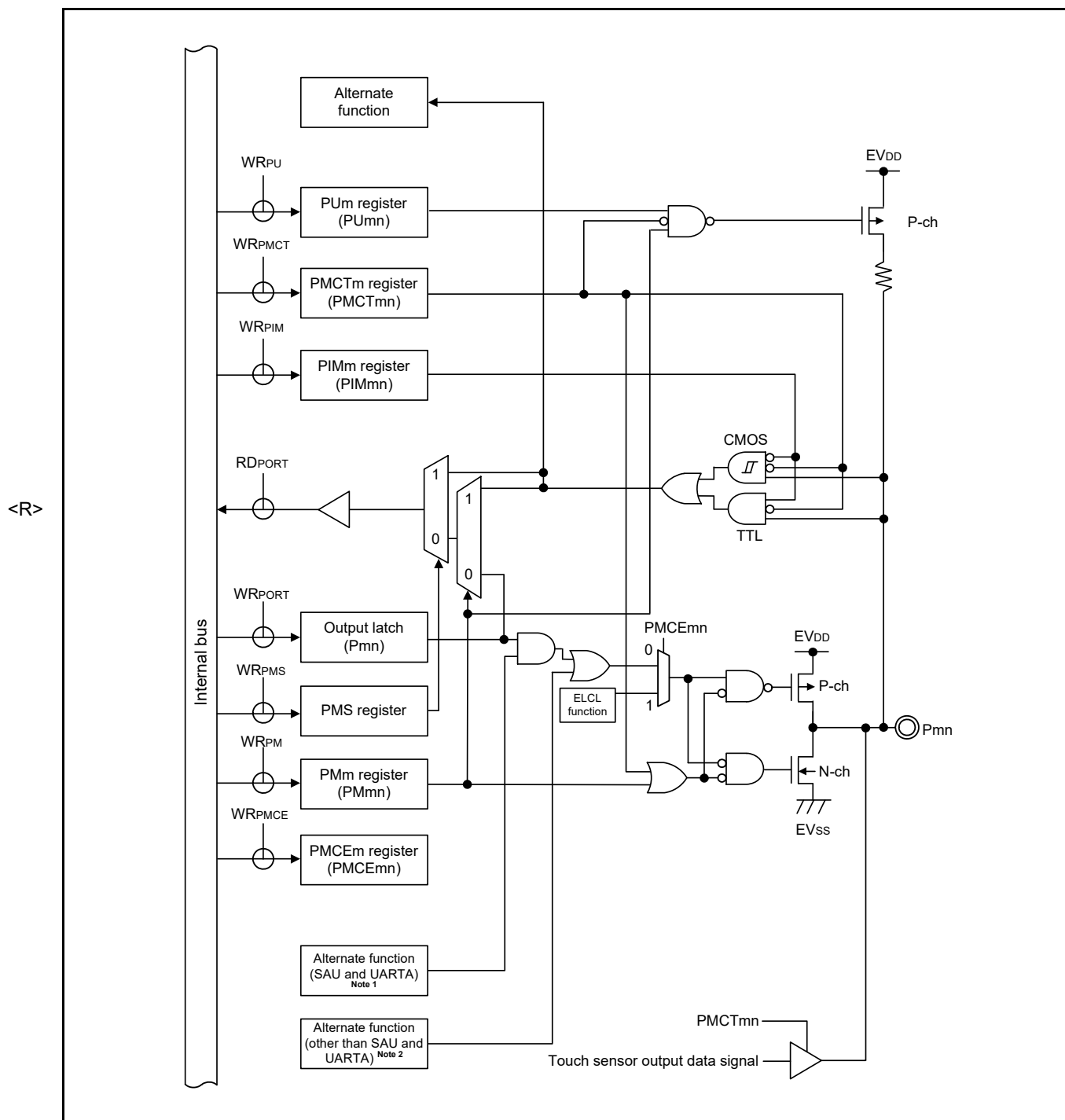
Figure 2 - 27 Pin Block Diagram for Pin Type 8-31-1
