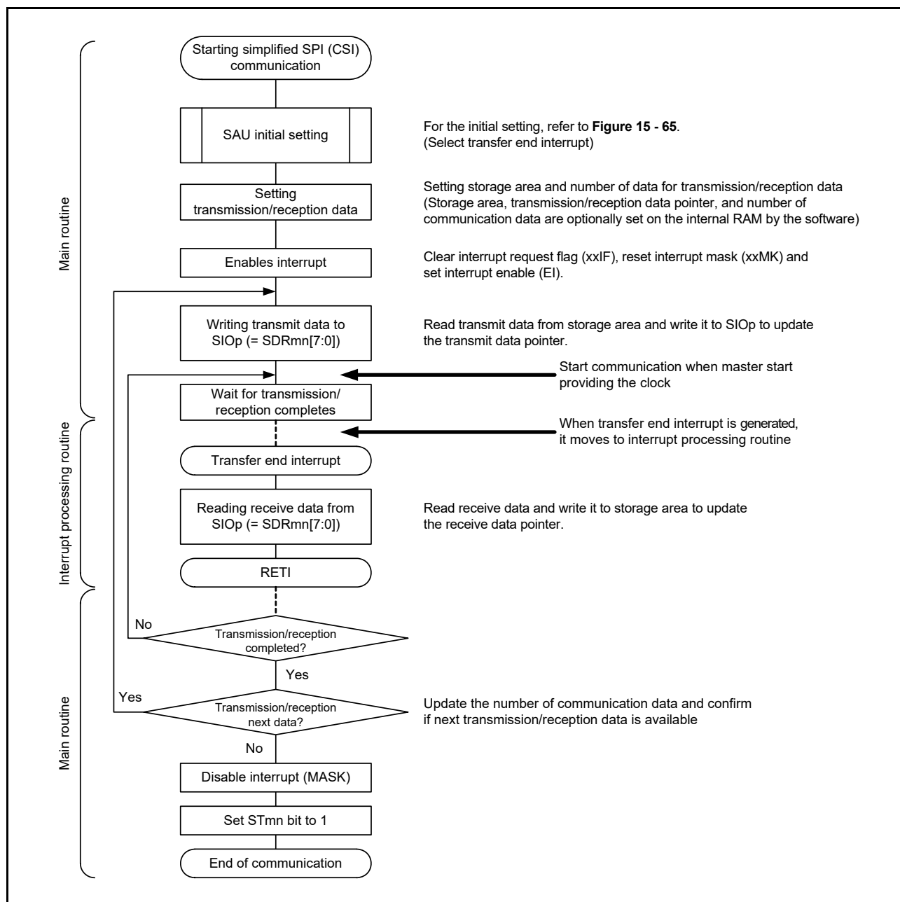
Figure 15 - 69 Flowchart of Slave Transmission/Reception (in Single-transmission/reception Mode)
