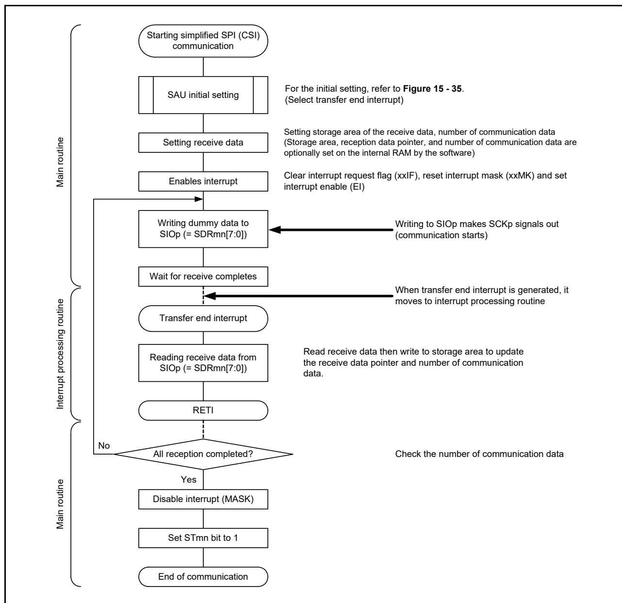
Figure 15 - 39 Flowchart of Master Reception (in Single-reception Mode)
