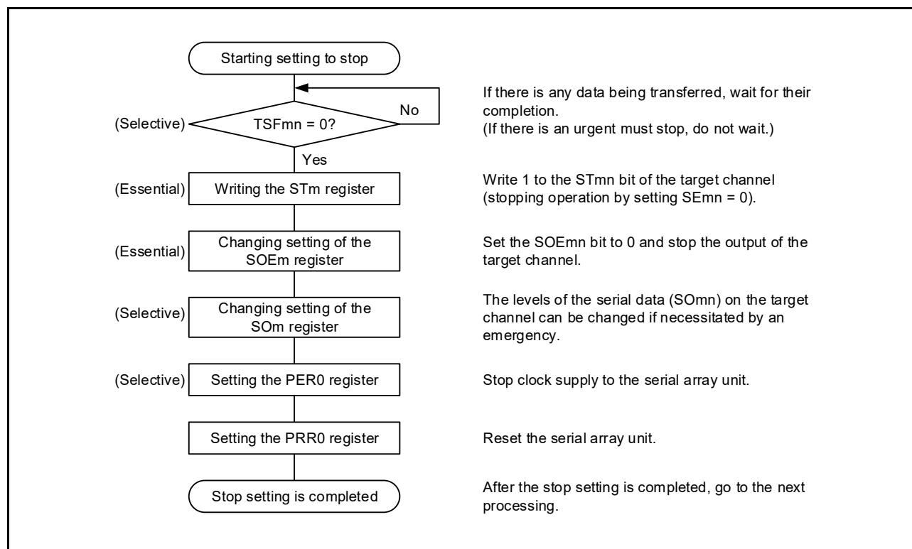
Figure 15 - 66 Procedure for Stopping Slave Transmission/Reception
