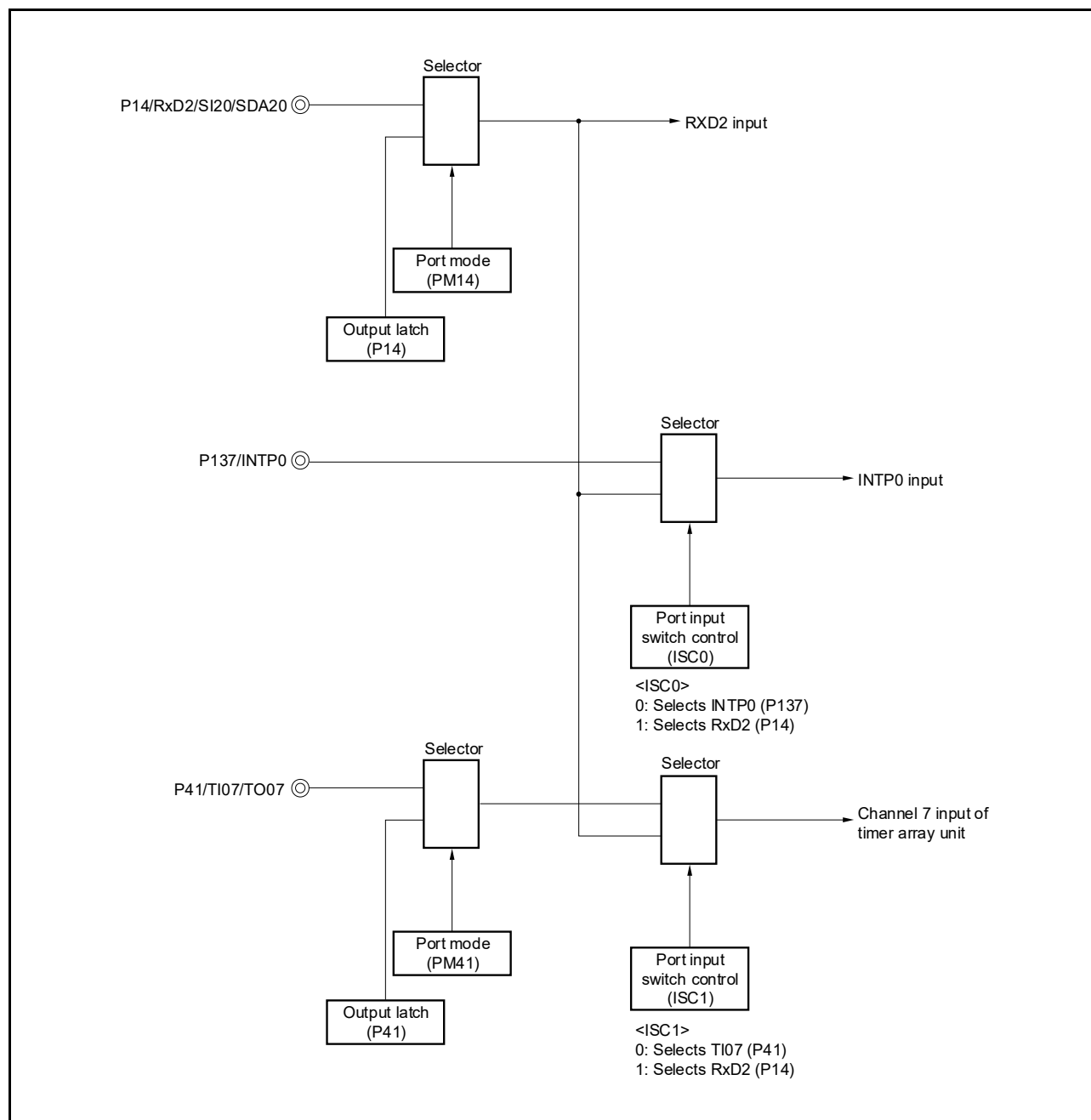
Figure 15 - 101 Port Configuration for Reception of LIN in 44- to 64-pin Products
