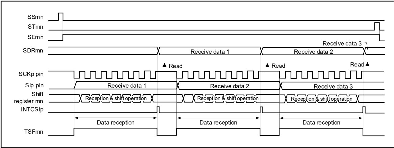
Figure 15 - 62 Timing Chart of Slave Reception (in Single-reception Mode) (Type 1: DAPmn = 0, CKPmn = 0)
