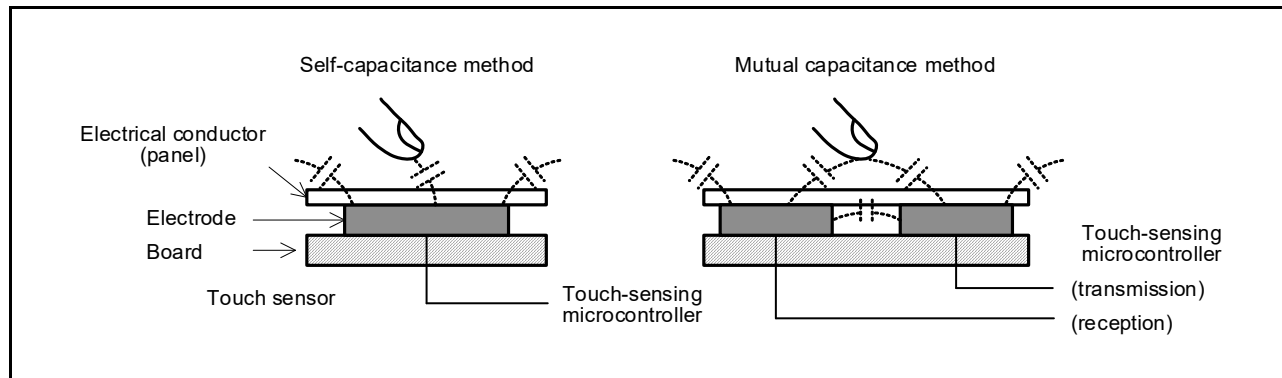
Figure 30 - 2 Self-capacitance Method and Mutual Capacitance Method
