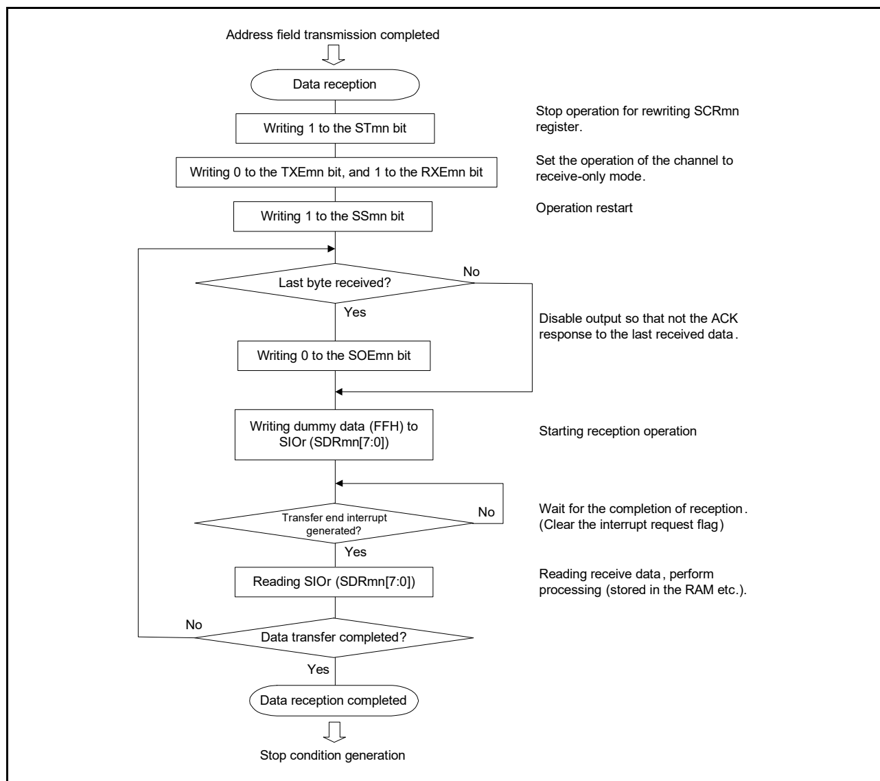
Figure 15 - 111 Flowchart of Data Reception
