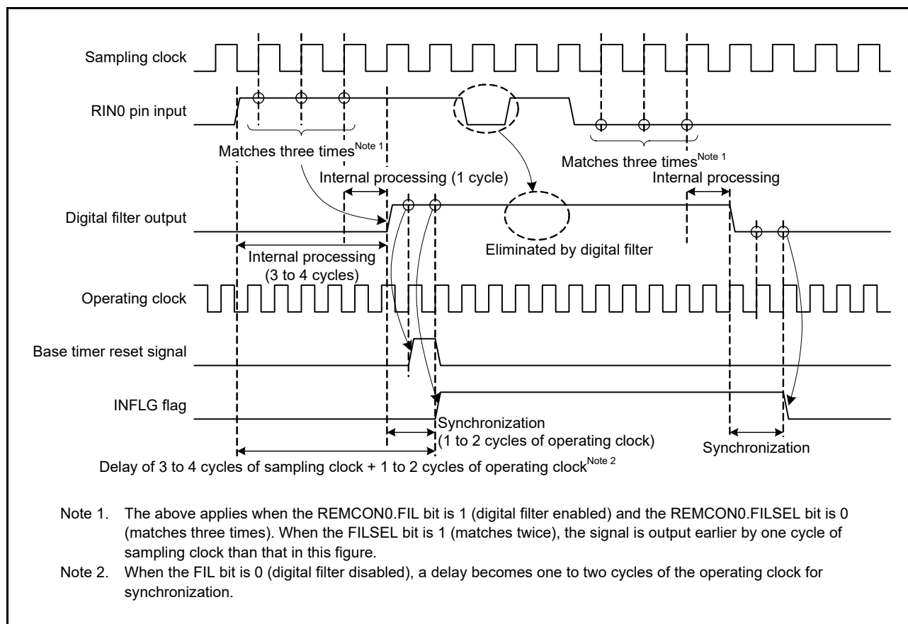
Figure 18 - 29 Digital Filtering for RIN0 Input
