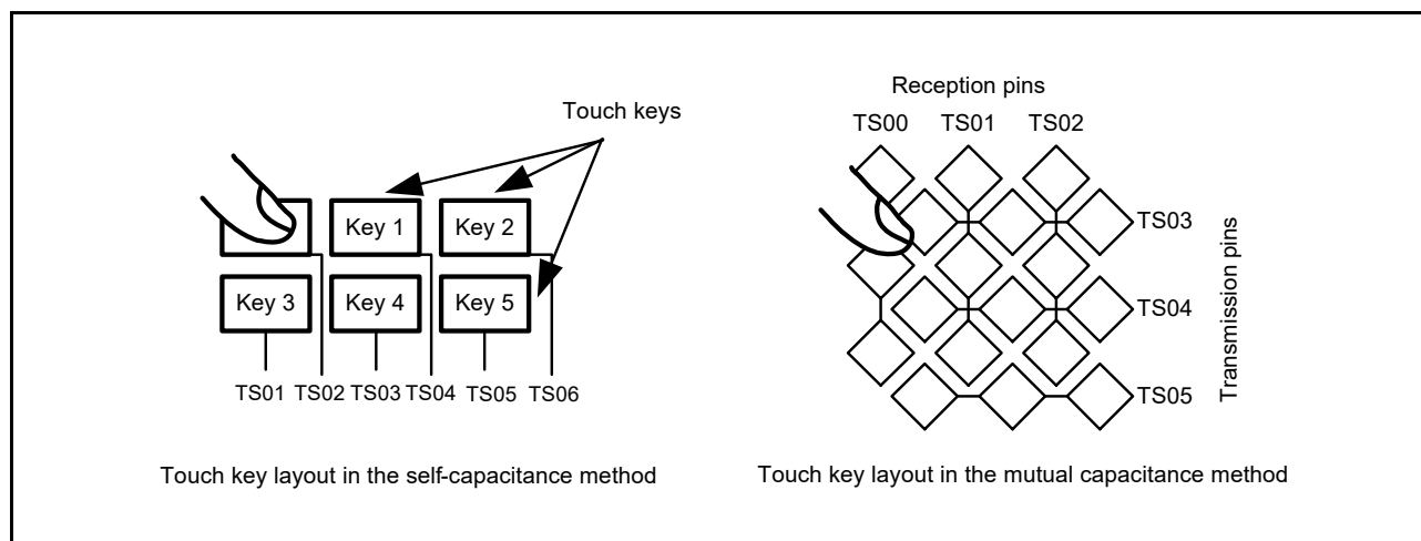
Figure 30 - 26 Overview of the Self-capacitance Method and the Mutual Capacitance Method
