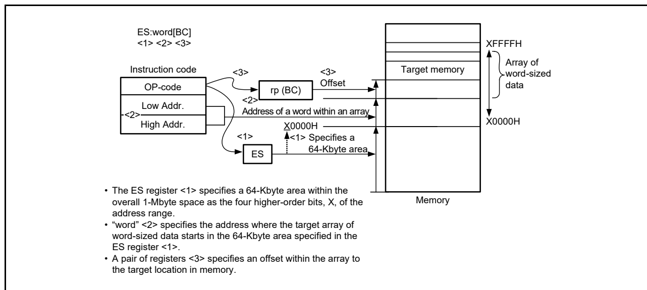
Figure 3 - 35 Example of ES:word[BC]
