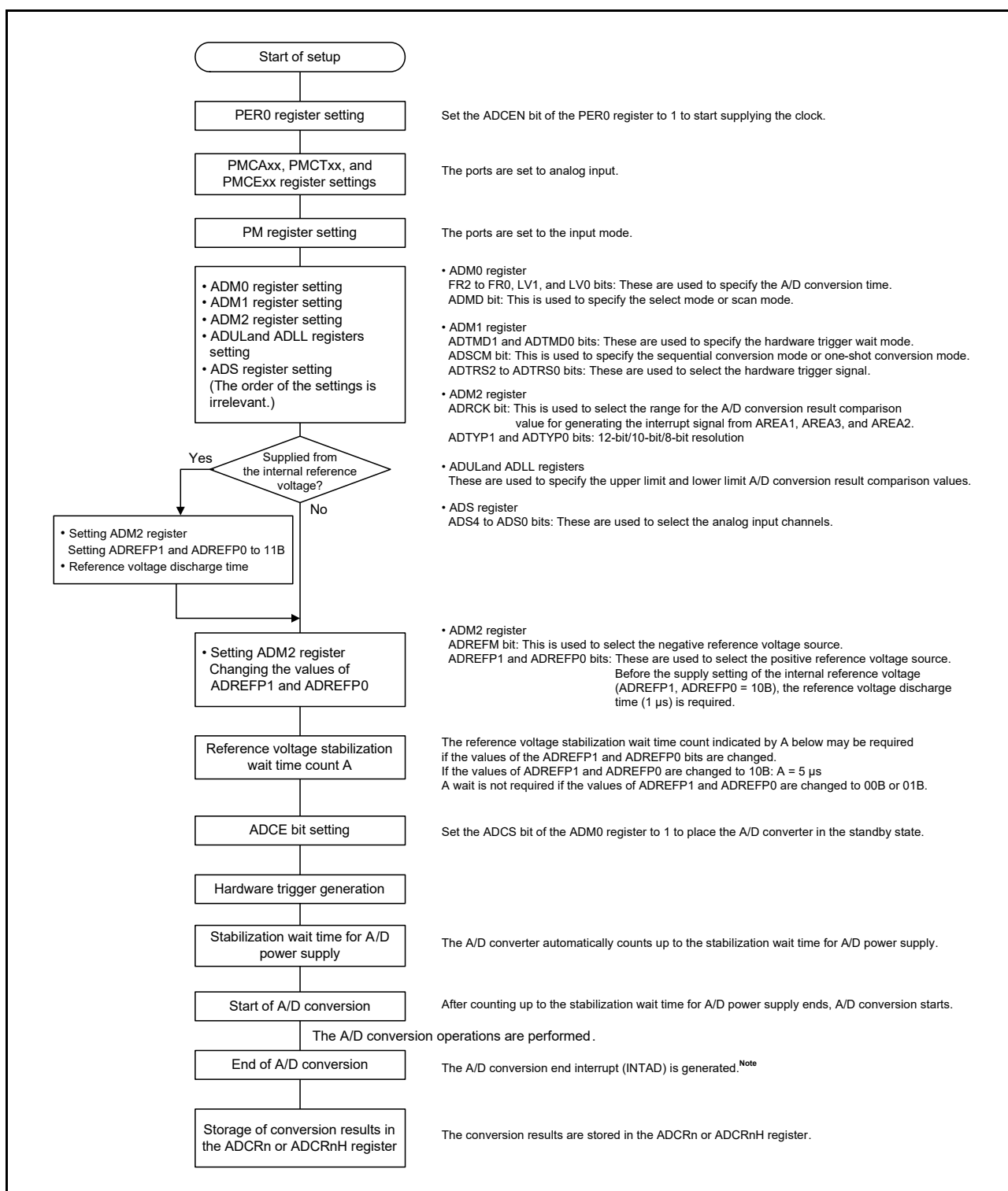
Figure 12 - 37 Settings in Hardware Trigger Wait Mode
