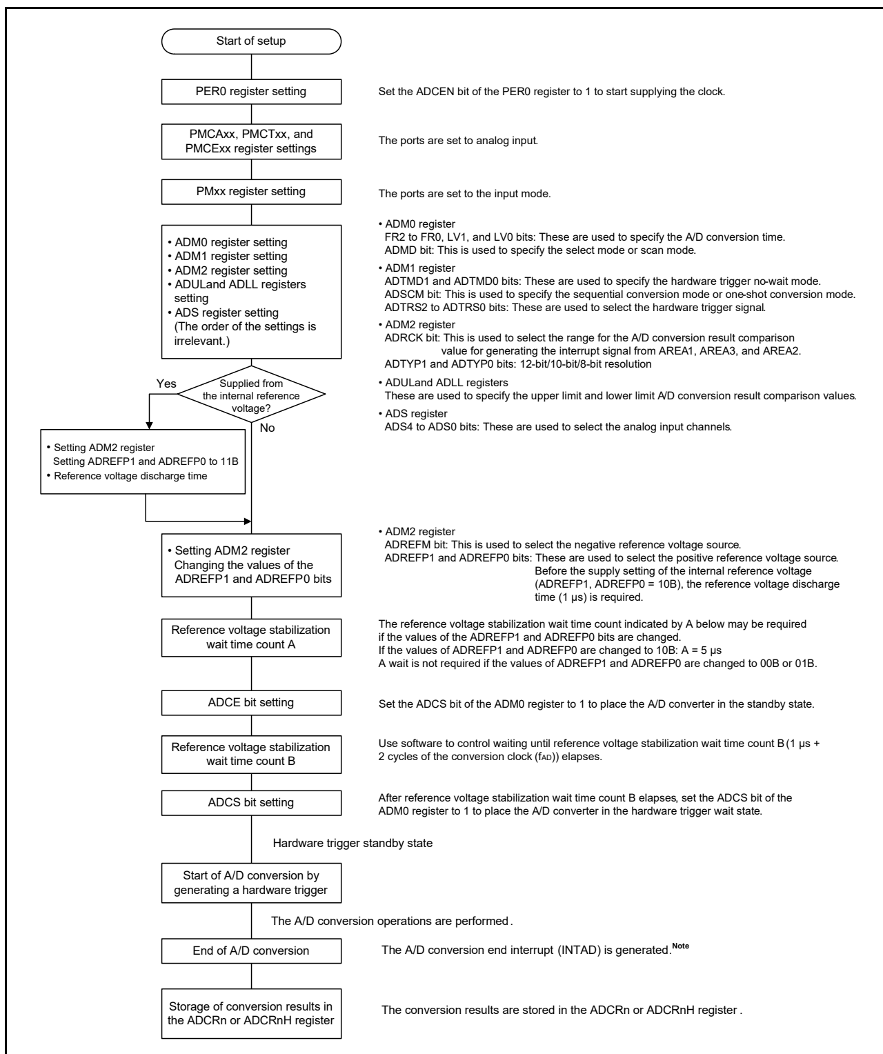
Figure 12 - 36 Settings in Hardware Trigger No-wait Mode
