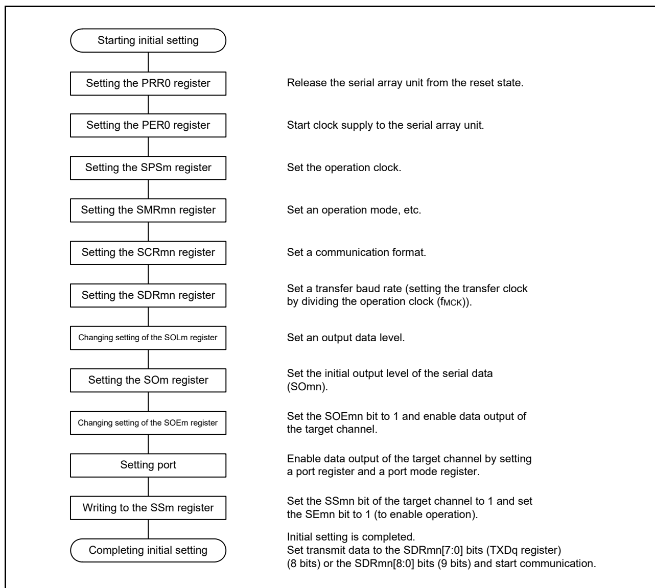
Figure 15 - 77 Initial Setting Procedure for UART Transmission
