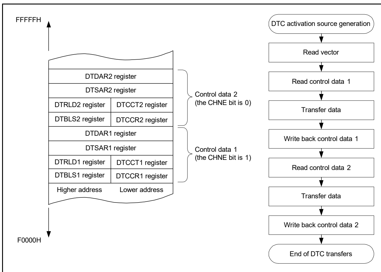
Figure 19 - 21 Data Transfers during Chain Transfers
