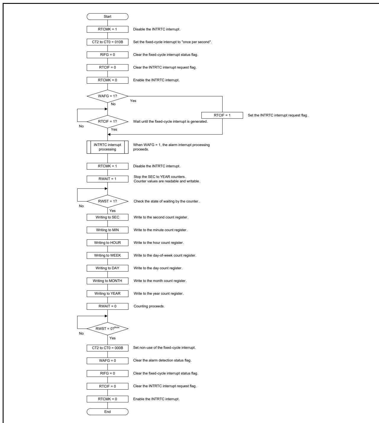
&lt;R&gt; Figure 8 - 22 Procedure for Writing to the Realtime Clock (When the Alarm Interrupt is in Use)
