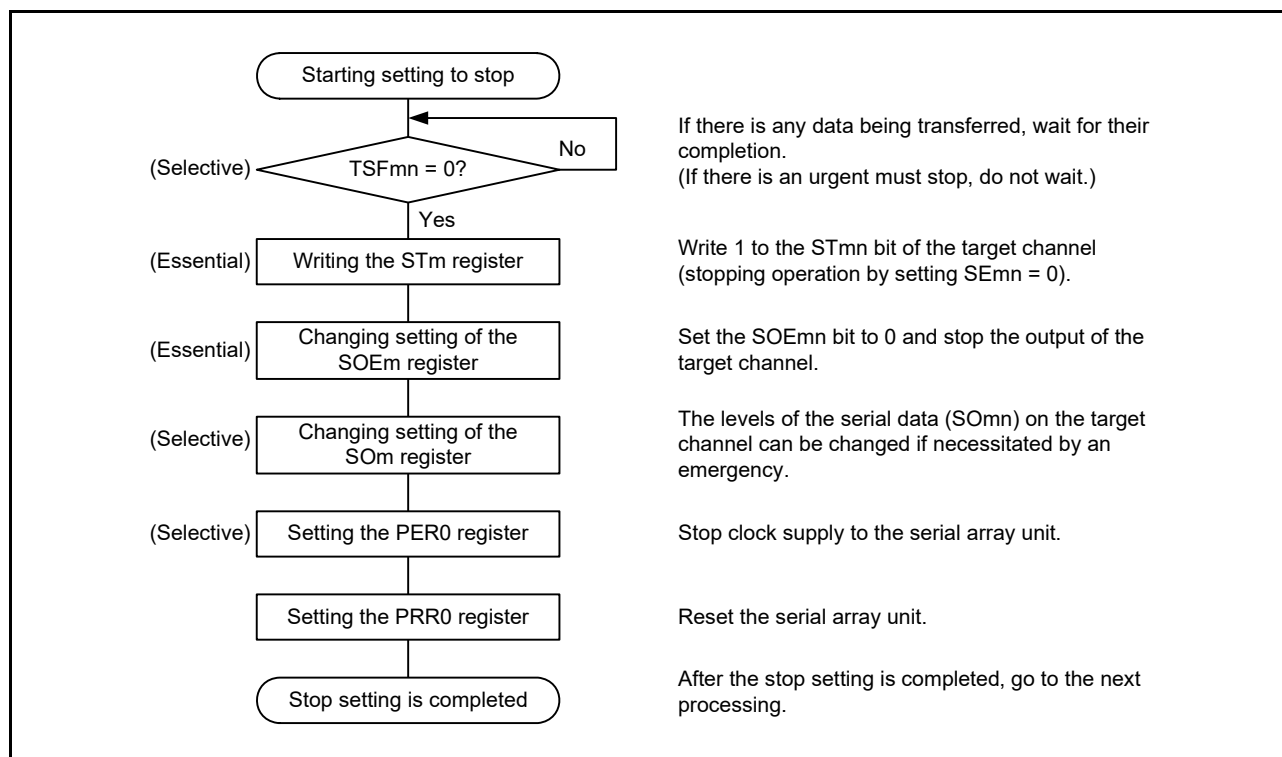
Figure 15 - 52 Procedure for Stopping Slave Transmission
