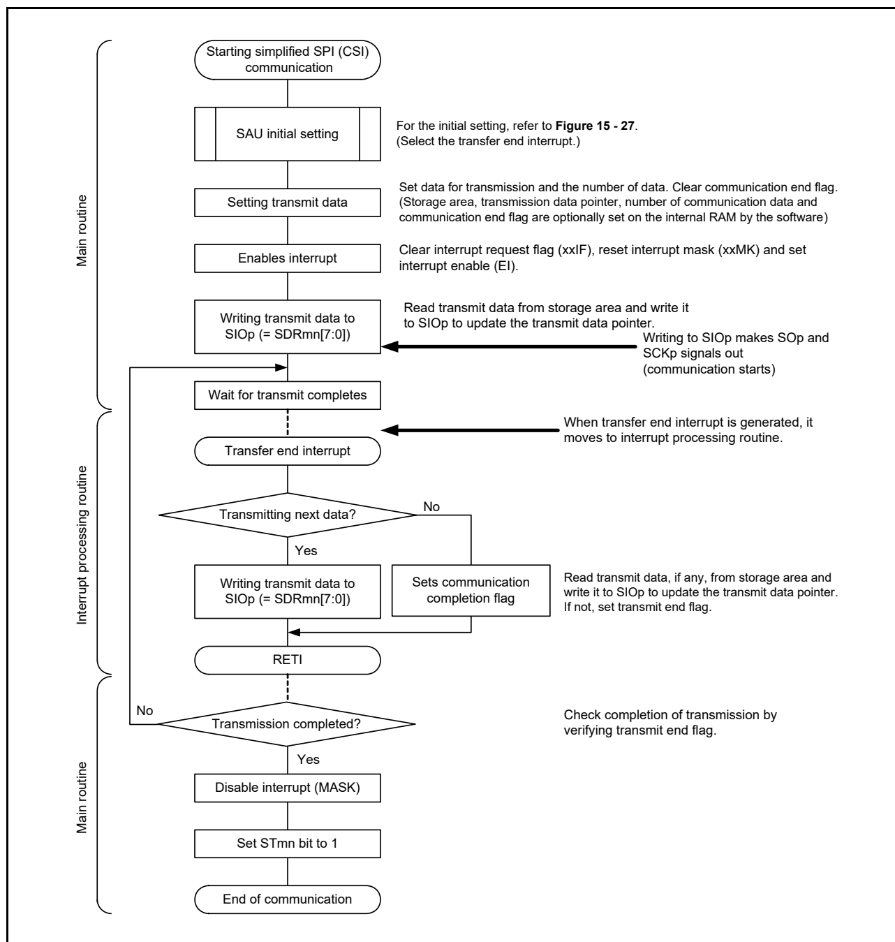
Figure 15 - 31 Flowchart of Master Transmission (in Single-transmission Mode)
