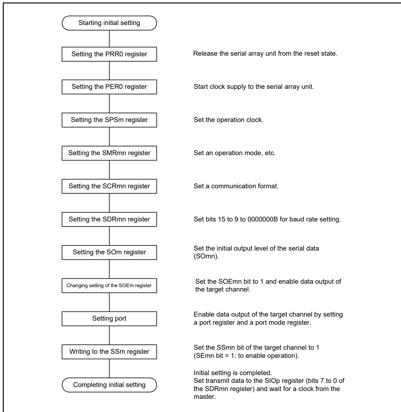
Figure 15 - 51 Initial Setting Procedure for Slave Transmission
