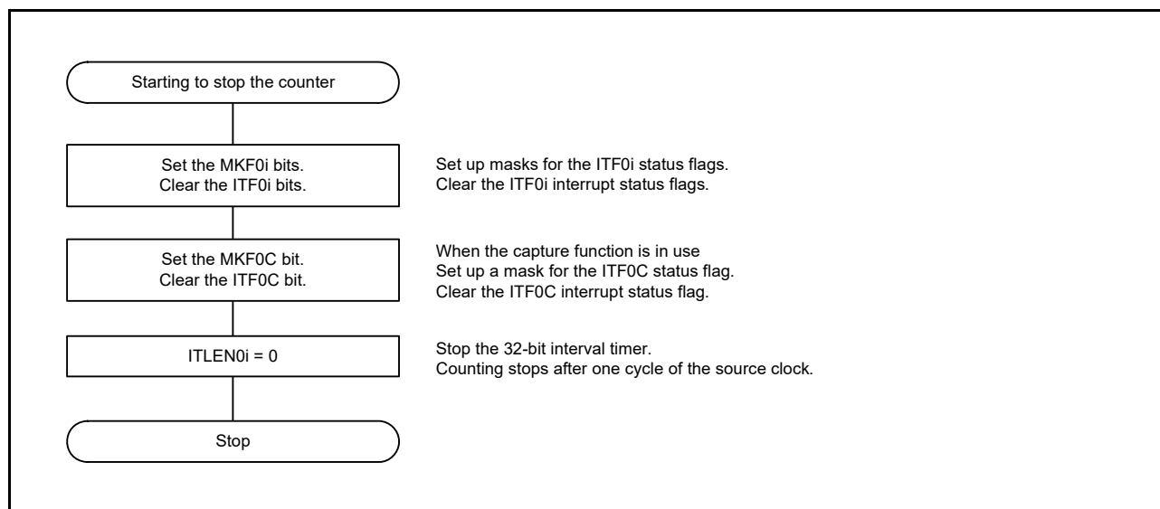
Figure 9 - 18 Procedure for Stopping the 32-Bit Interval Timer
