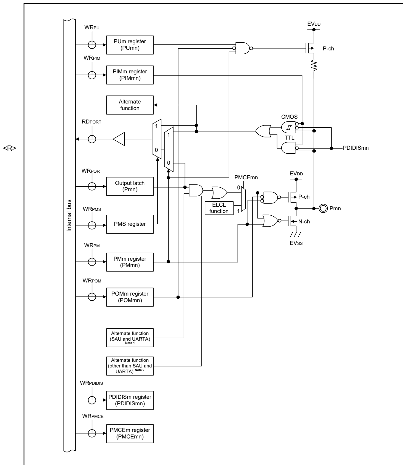
Figure 2 - 25 Pin Block Diagram for Pin Type 8-1-11
