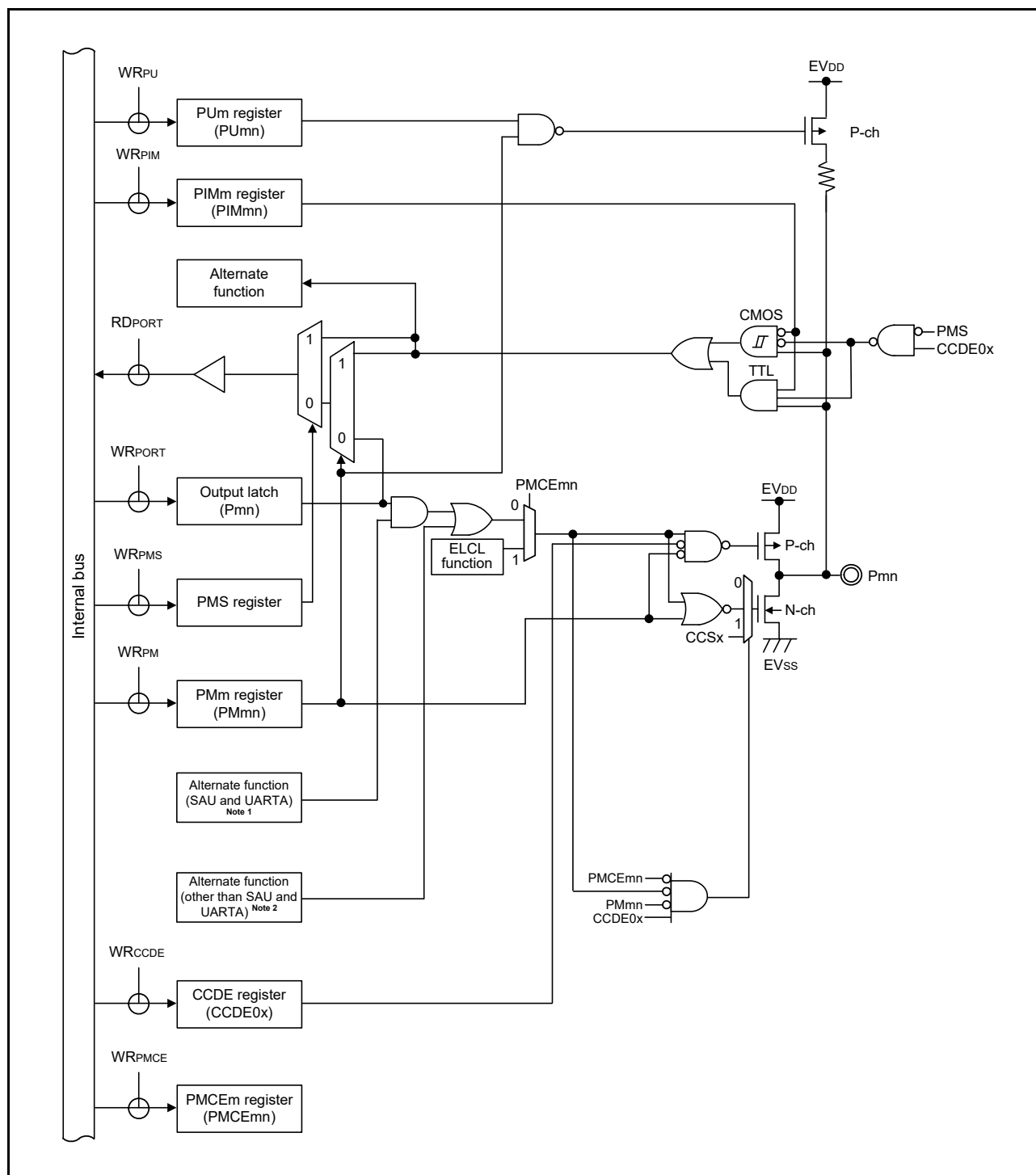
<R> Figure 2 - 31 Pin Block Diagram for Pin Type 8-38-1
