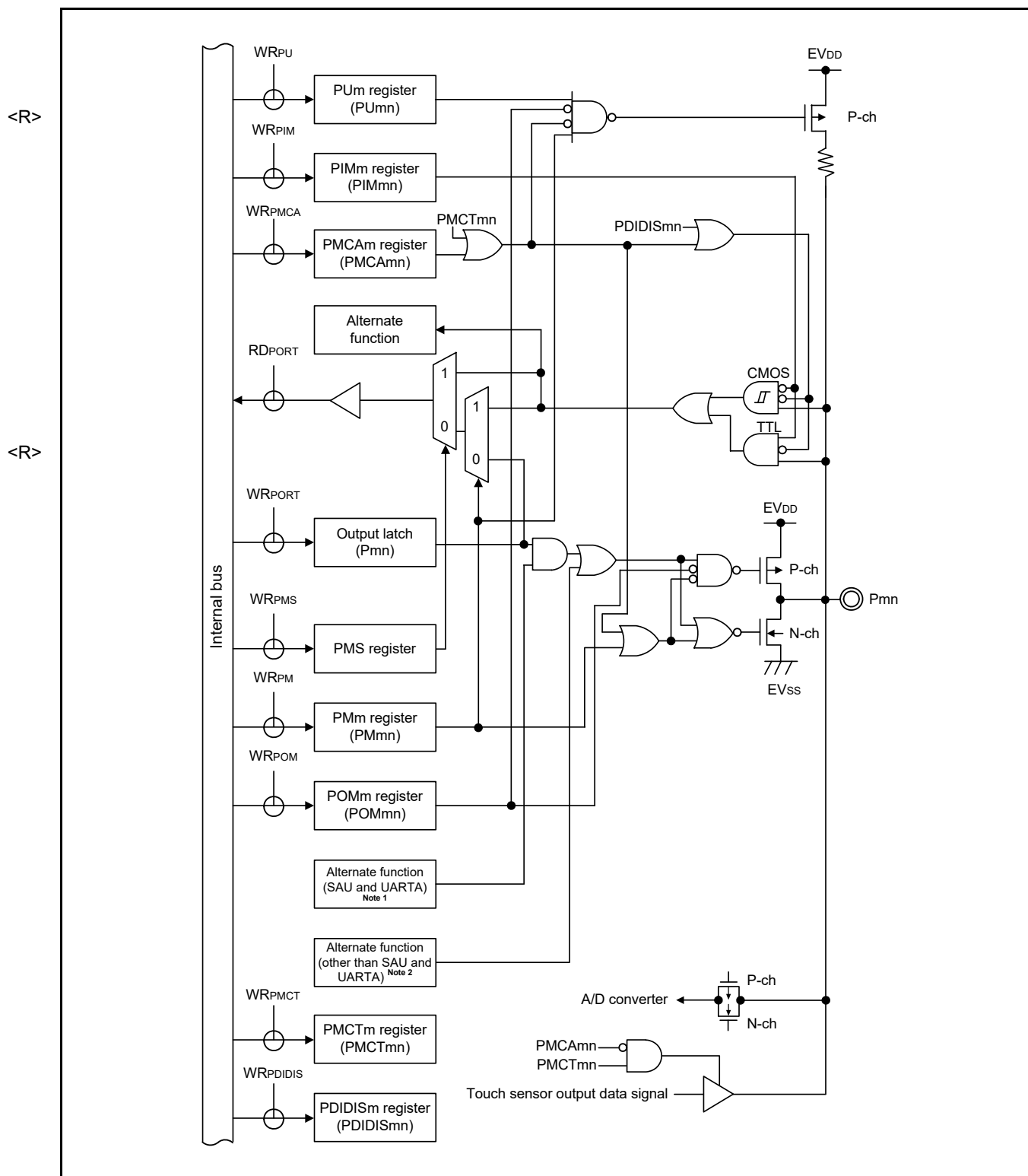
Figure 2 - 30 Pin Block Diagram for Pin Type 8-33-3
