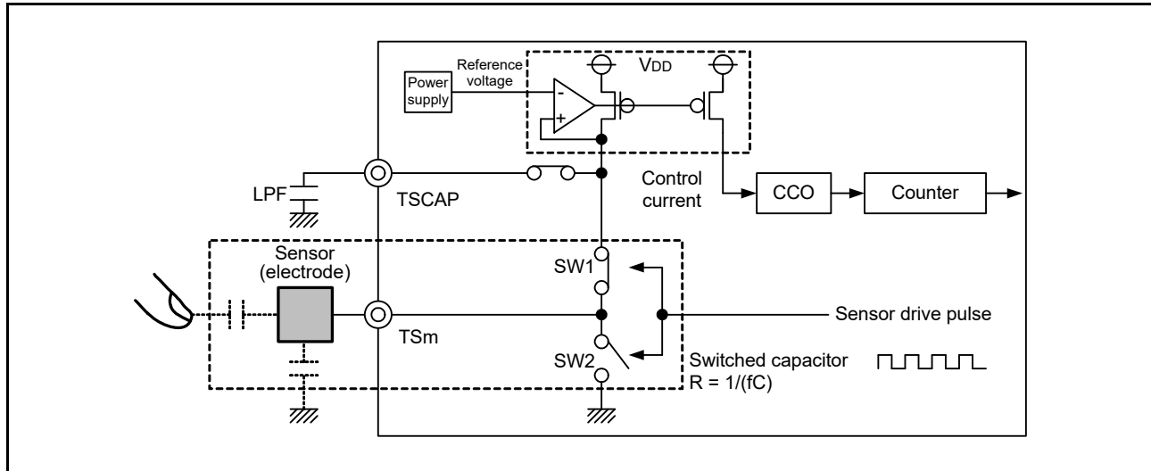
Figure 30 - 20 Measurement Circuit
