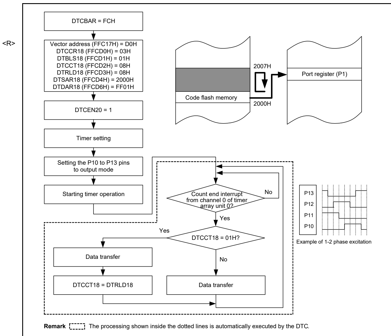
Figure 19 - 19 Example 1 of Using Repeat Mode: Outputting Stepping Motor Control Pulses Using Port Pins
