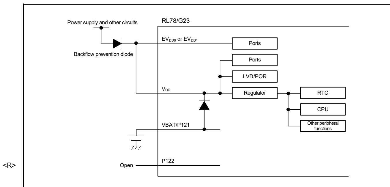
Figure 2 - 1 Example of the Connection of the VBAT Pin
