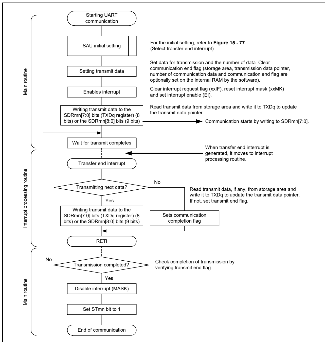
Figure 15 - 81 Flowchart of UART Transmission (in Single-transmission Mode)
