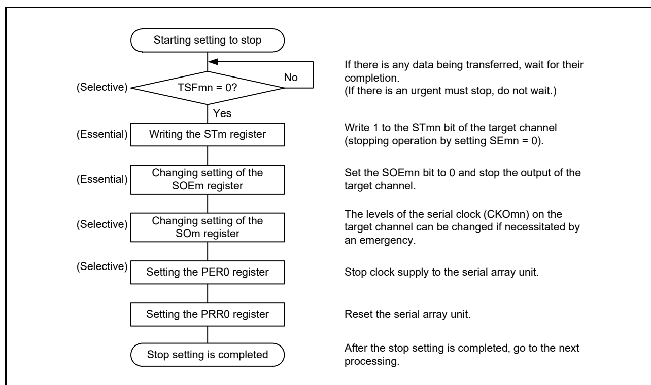
Figure 15 - 36 Procedure for Stopping Master Reception
