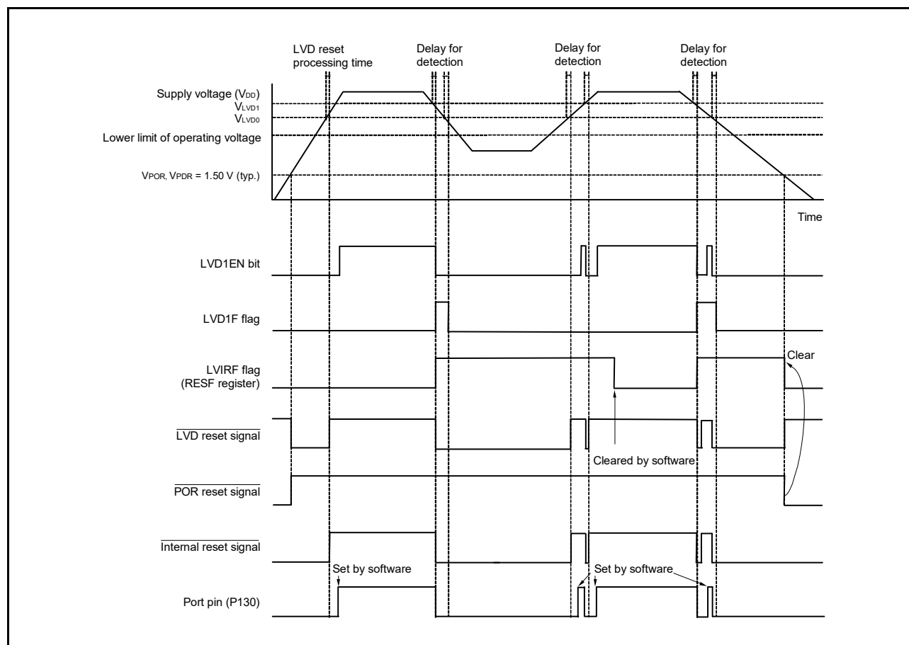
Figure 26 - 7 Timing of the Internal Reset Signal Generated in LVD1
