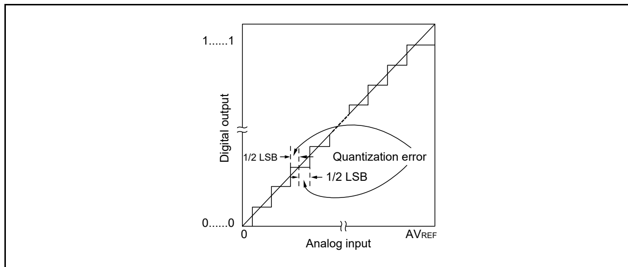
Figure 12 - 47 Quantization Error
