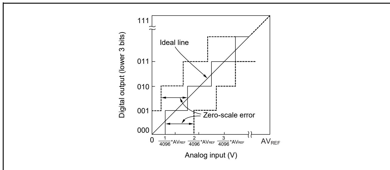
Figure 12 - 48 Zero-scale Error
