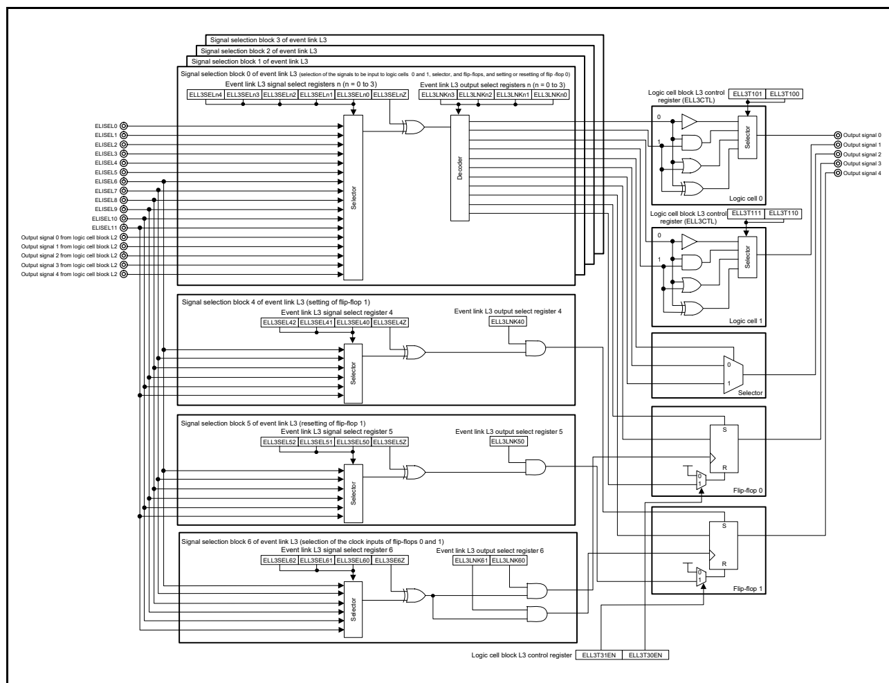
Figure 20 - 4 Block Diagram of Logic Cell Block L3
