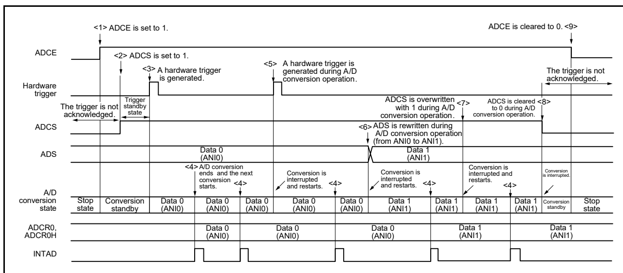
Figure 12 - 26 Example of Hardware Trigger No-wait Mode (Select Mode, Sequential Conversion Mode) Operation Timing
