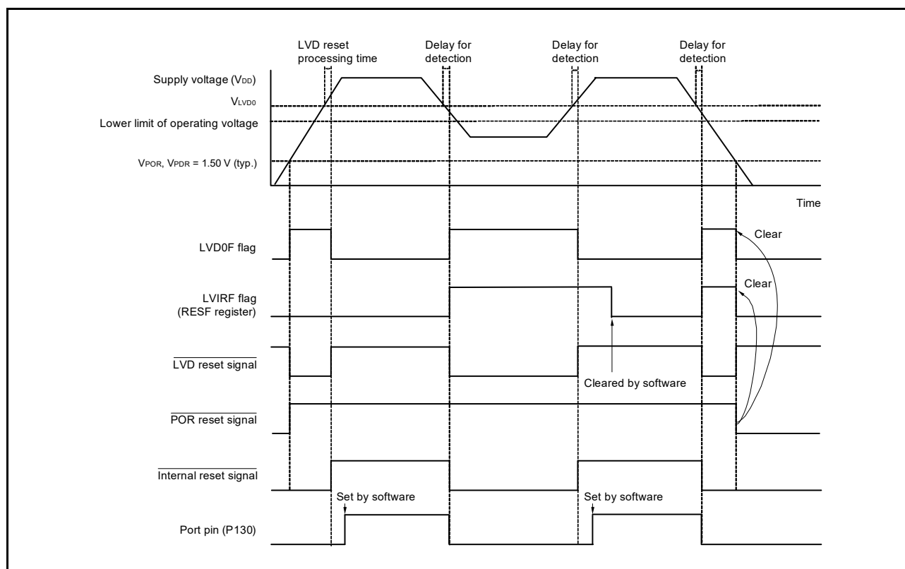
Figure 26 - 6 Timing of the Internal Reset Signal Generated in LVD0
