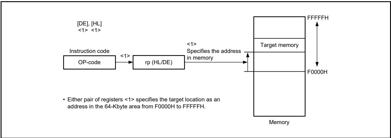
Figure 3 - 27 Example of [DE], [HL]
