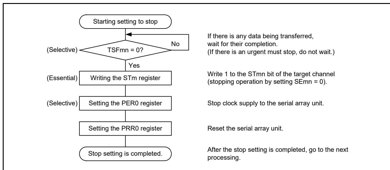
Figure 15 - 86 Procedure for Stopping UART Reception
