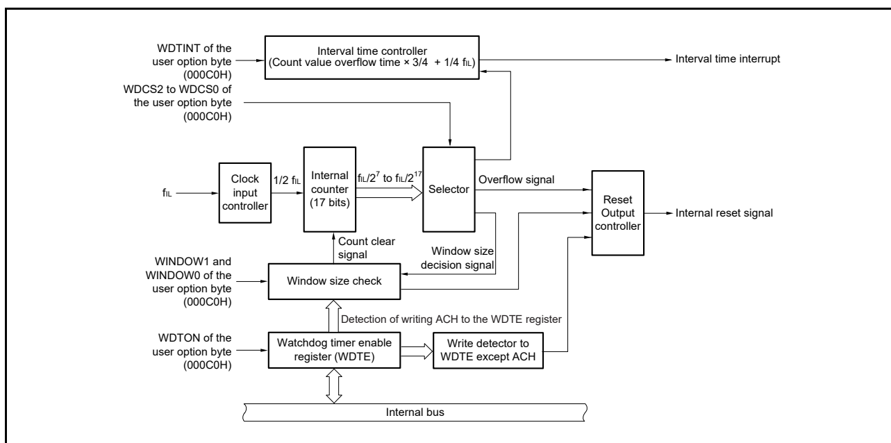
Figure 11 - 1 Block Diagram of Watchdog Timer
