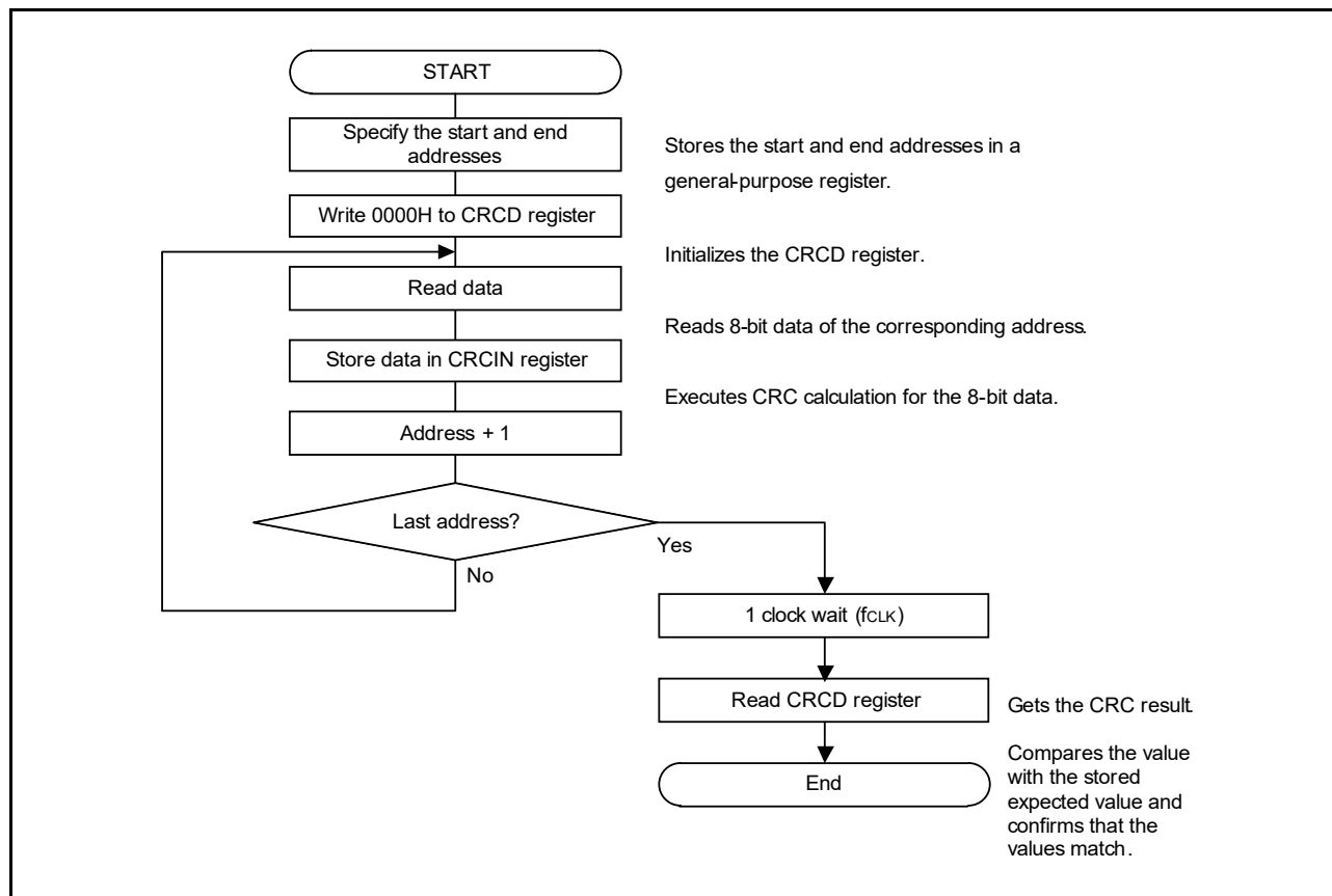
Figure 27 - 6 CRC Operation (General-purpose CRC)
