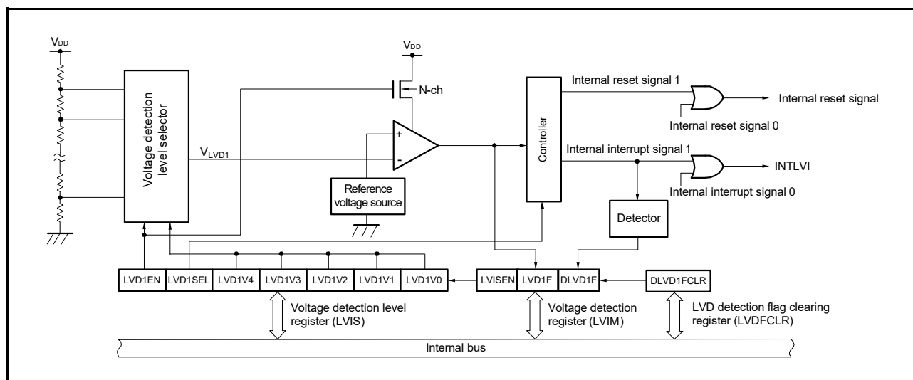
Figure 26 - 2 Block Diagram of LVD1
