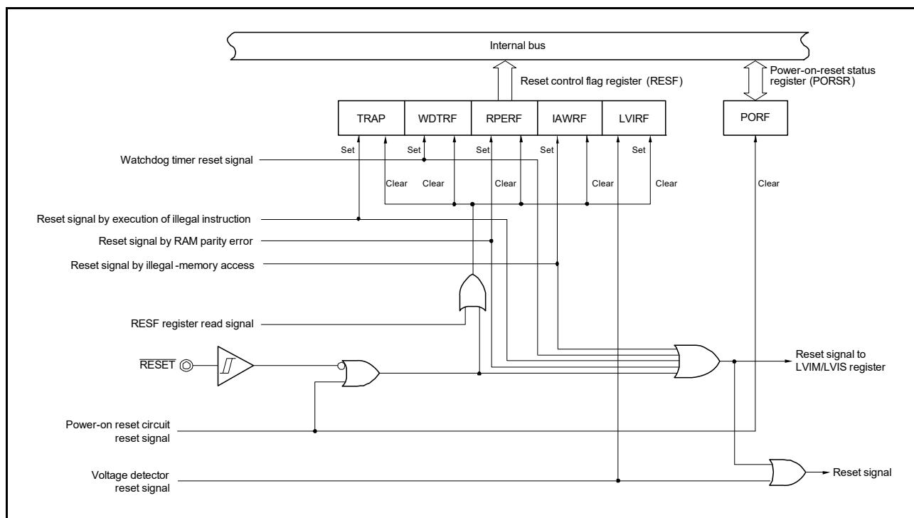
Figure 24 - 1 Block Diagram of Reset Function
