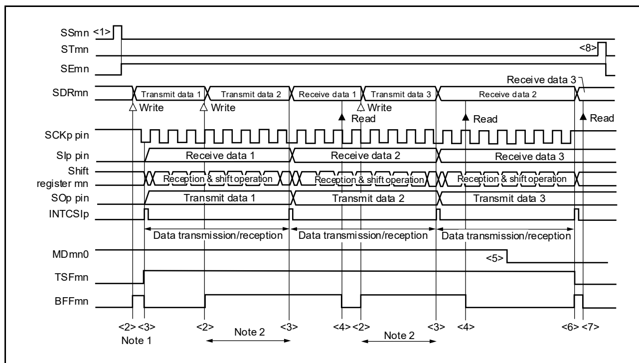
Figure 15 - 70 Timing Chart of Slave Transmission/Reception (in Continuous Transmission/Reception Mode) (Type 1: DAPmn = 0, CKPmn = 0)
