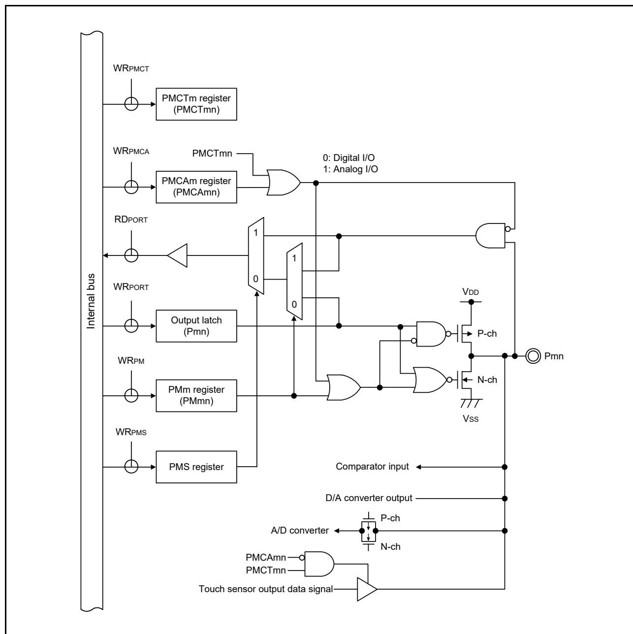
Figure 2 - 10 Pin Block Diagram for Pin Type 4-37-1
