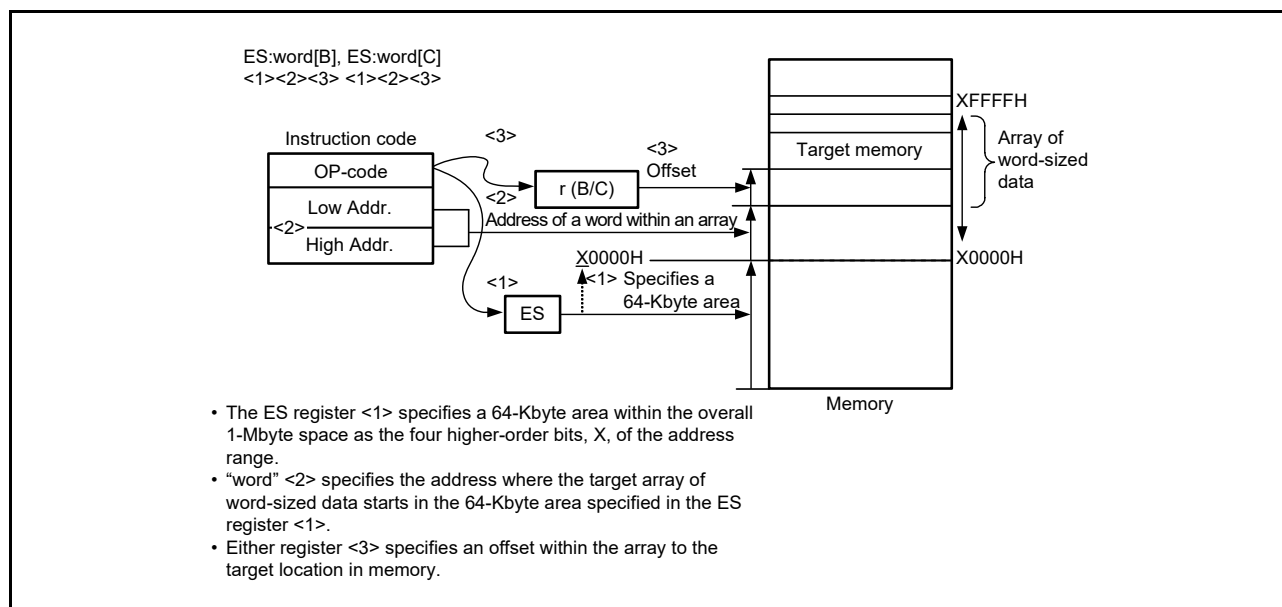
Figure 3 - 34 Example of ES:word[B], ES:word[C]
