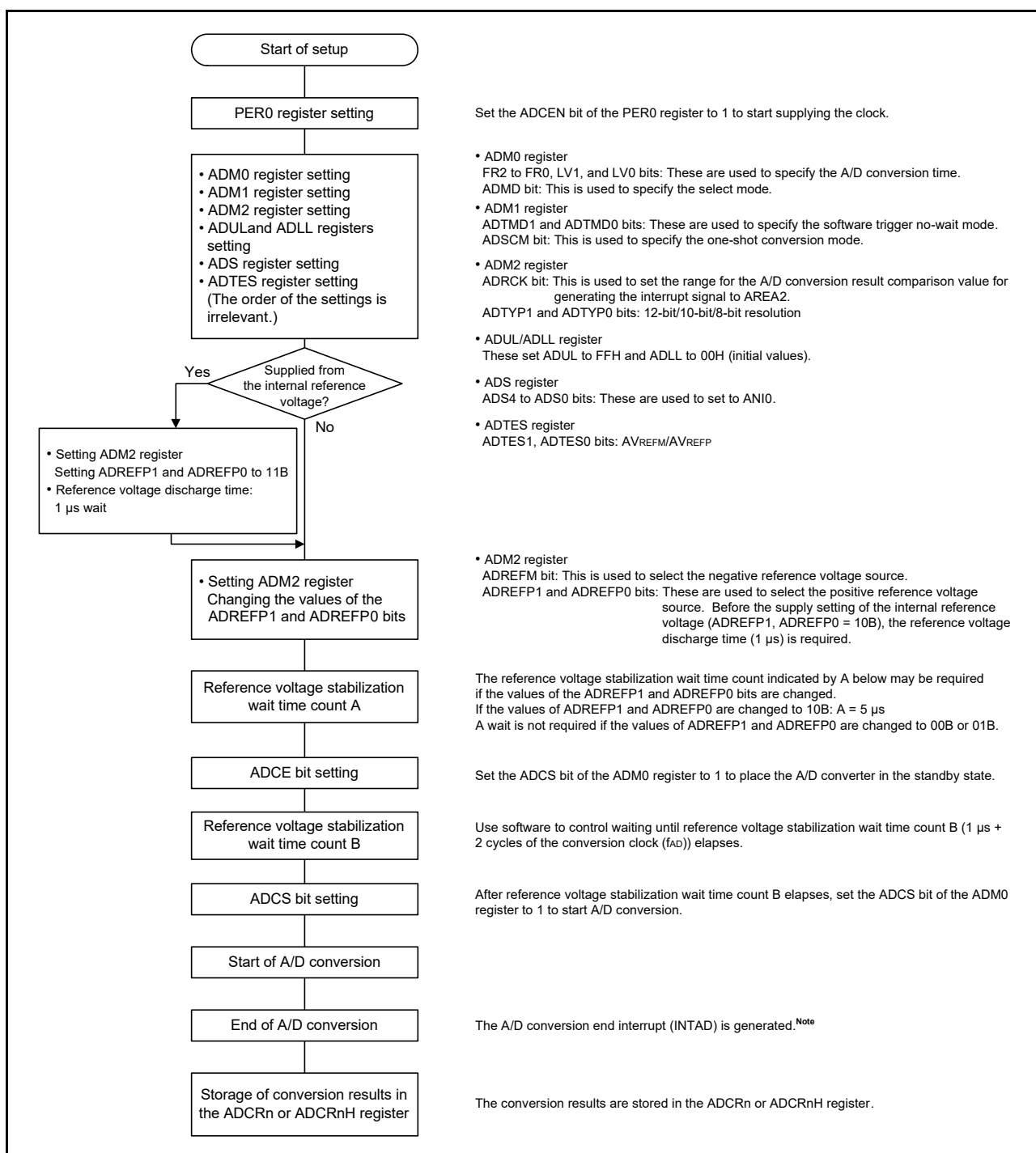
Figure 12 - 39 Settings in Test Mode
