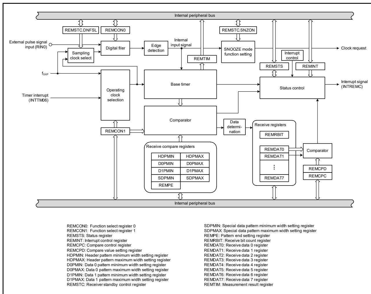
Figure 18 - 1 Block Diagram of Remote Control Signal Receiver
