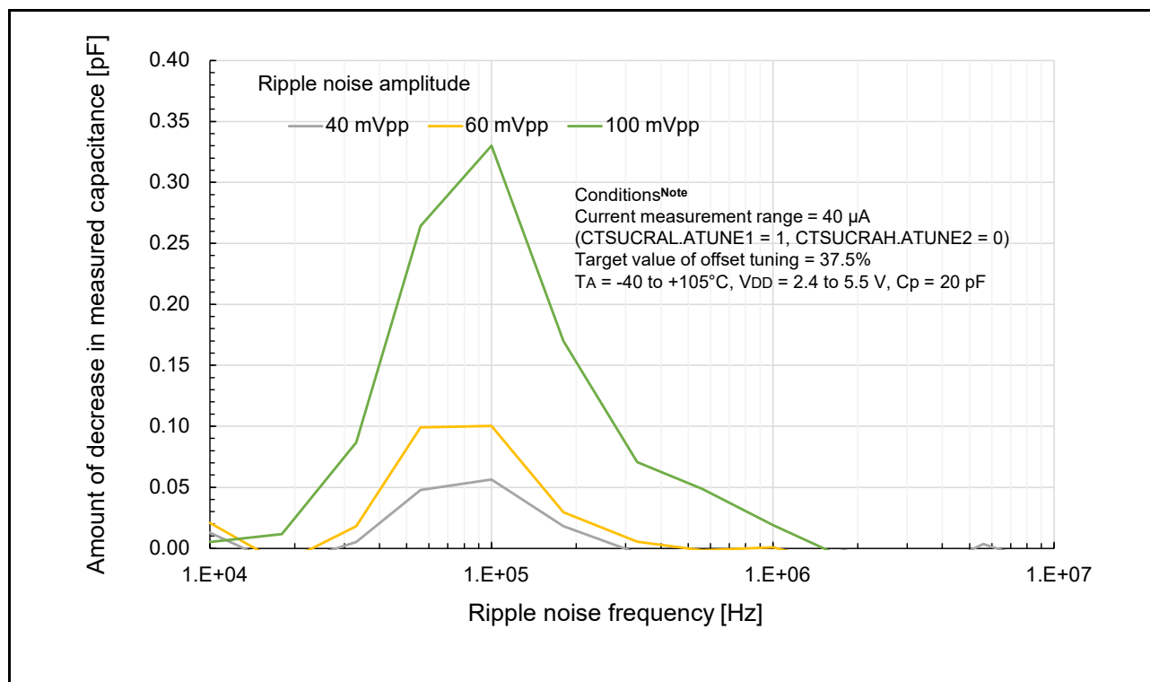
Figure 30 - 31 Amount of decrease in measured capacitance (reference value)
