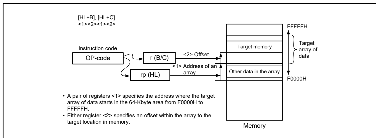
Figure 3 - 36 Example of [HL+B], [HL+C]
