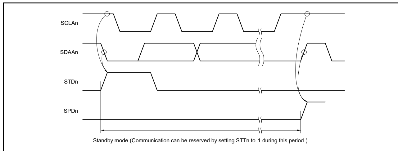
Figure 16 - 26 Timing for Accepting Communication Reservations
