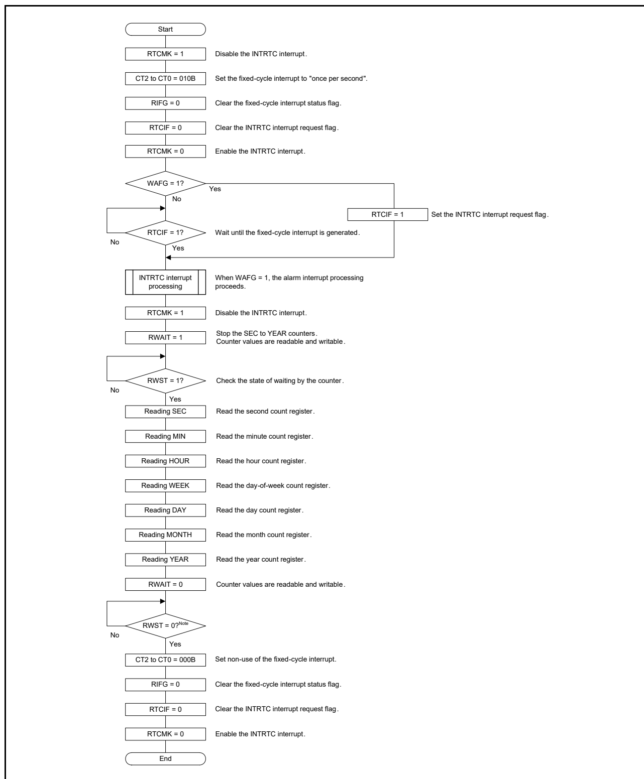
&lt;R&gt; Figure 8 - 20 Procedure for Reading the Realtime Clock (When the Alarm Interrupt is in Use)
