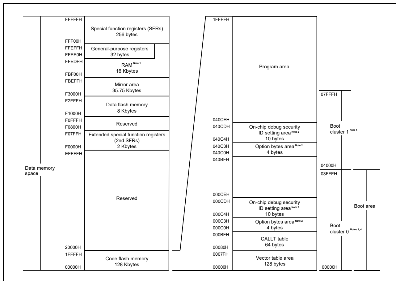
Figure 3 - 2 Memory Map (R7F100GxG (x = A, B, C, E, F, G, J, L, M, P))
