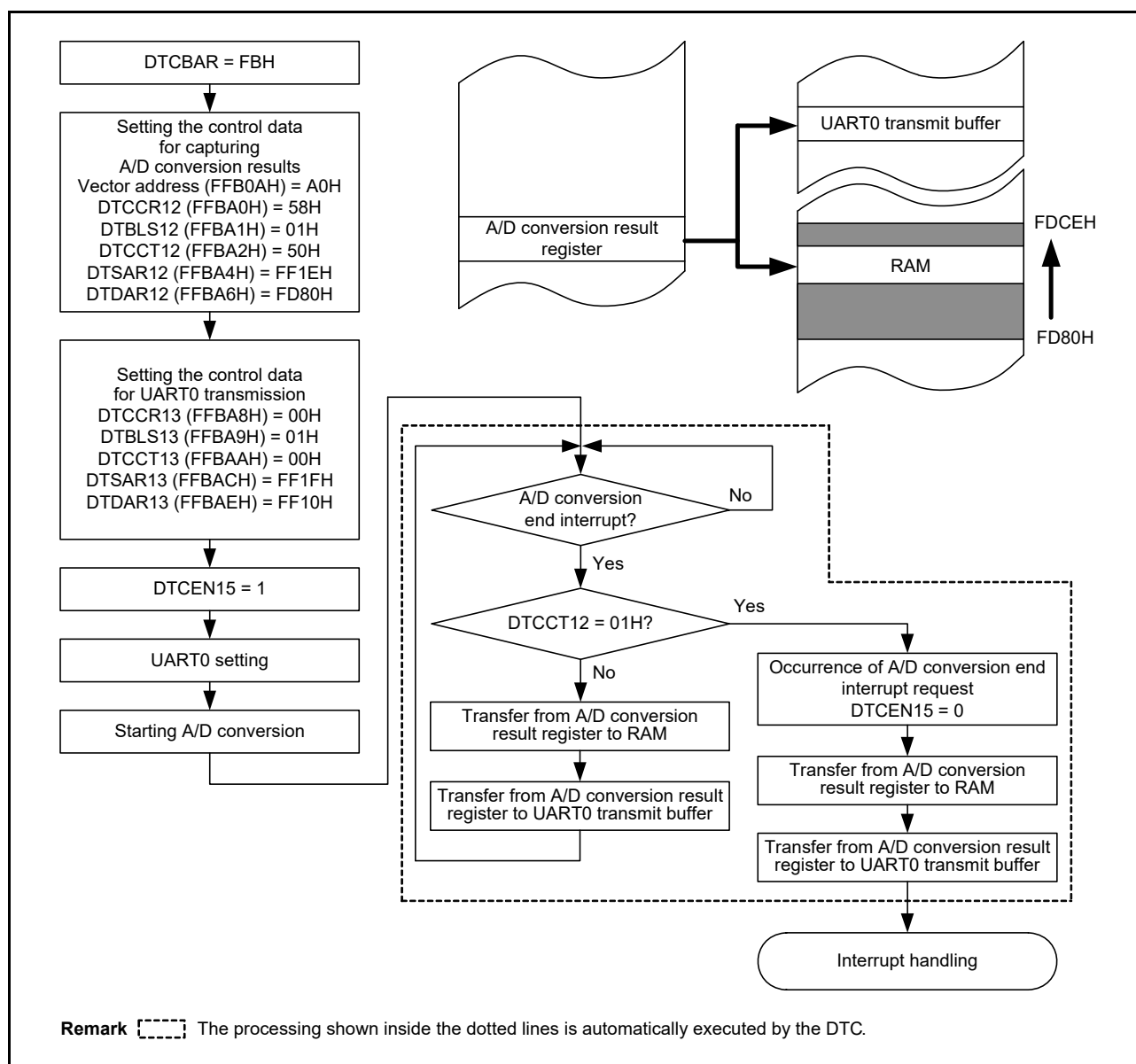
<R> Figure 19 - 22 Example of Using Chain Transfers: Consecutively Capturing A/D Conversion Results and UART0 Transmission
