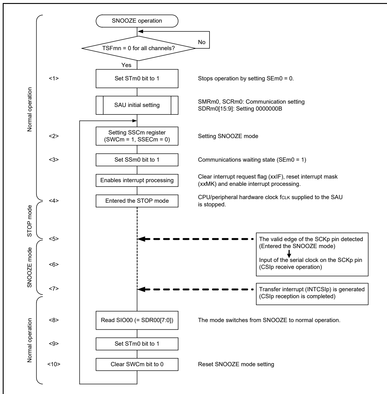
Figure 15 - 75 Flowchart of SNOOZE Mode Operation (continuous startup)
