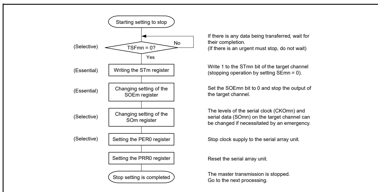
Figure 15 - 28 Procedure for Stopping Master Transmission
