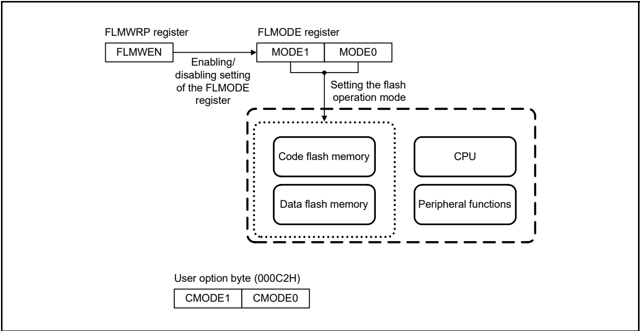
Figure 5 - 1 Block Diagram of Operation State Control
