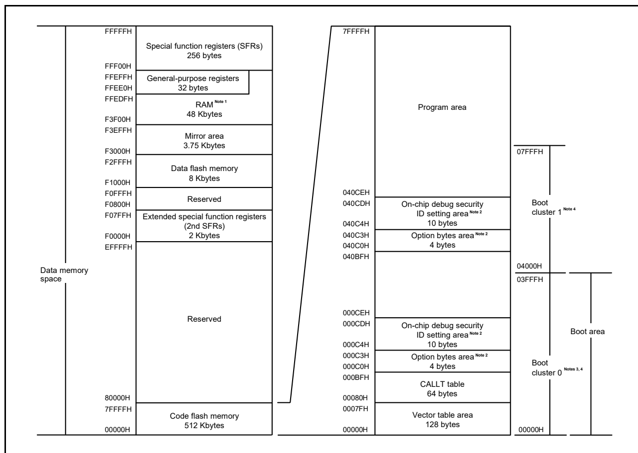
Figure 3 - 6 Memory Map (R7F100GxL (x = F, G, J, L, M, P, S))
