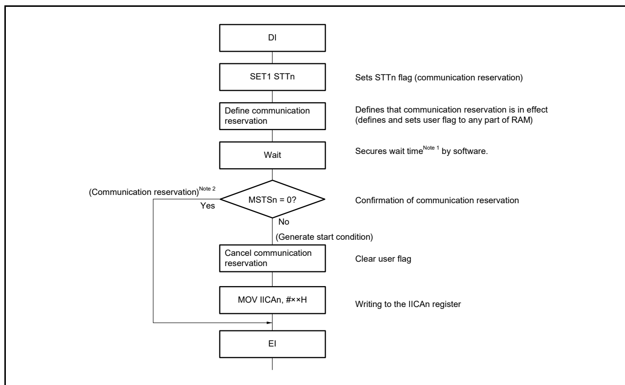
Figure 16 - 27 Communication Reservation Protocol
