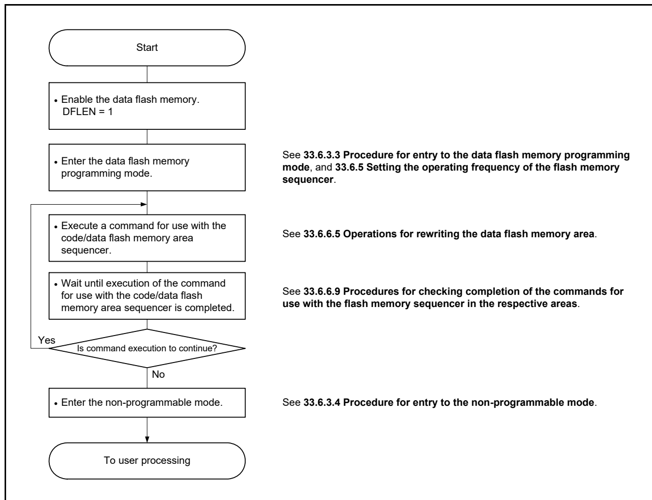
Figure 33 - 28 Flow of Executing the Commands to Rewrite the Data Flash Memory Area
