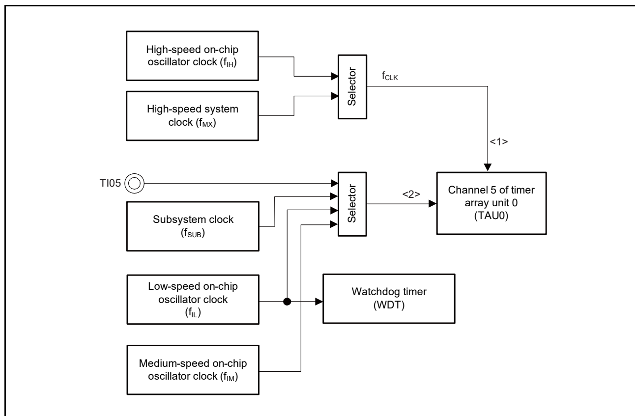
Figure 27 - 17 Configuration of Frequency Detection Function
