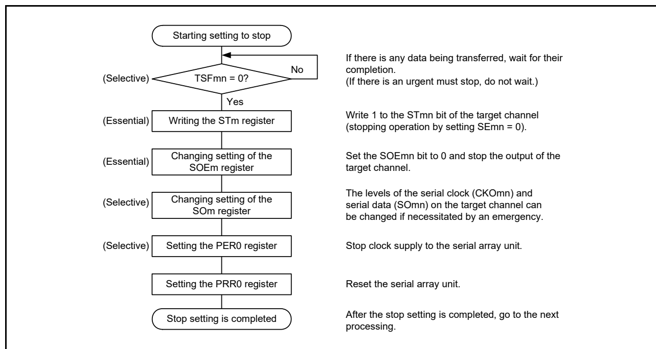
Figure 15 - 44 Procedure for Stopping Master Transmission/Reception
