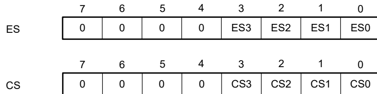
Figure 3-17. Configuration of ES and CS Registers
