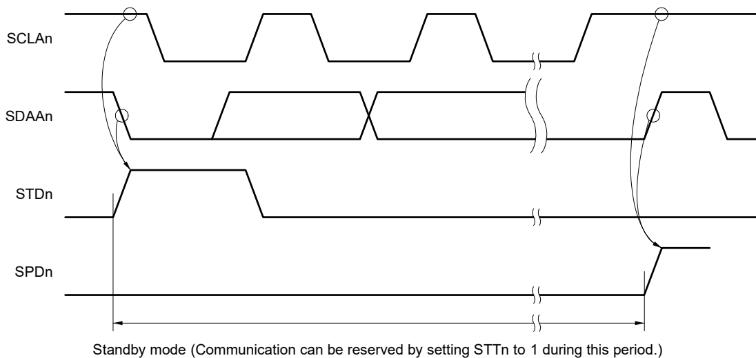
Figure 13-26. Timing for Accepting Communication Reservations
