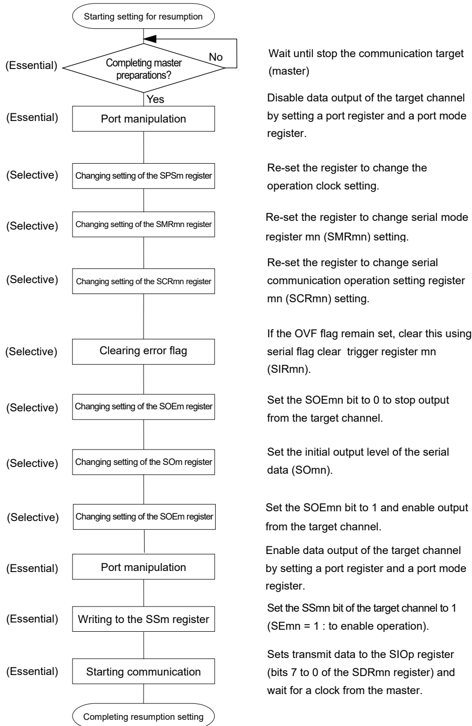
Figure 12-66. Procedure for Resuming Slave Transmission/Reception
