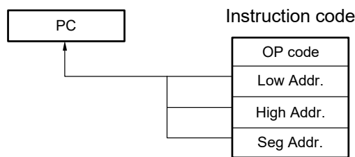
Figure 3-21. Example of CALL !addr16/BR !addr16
