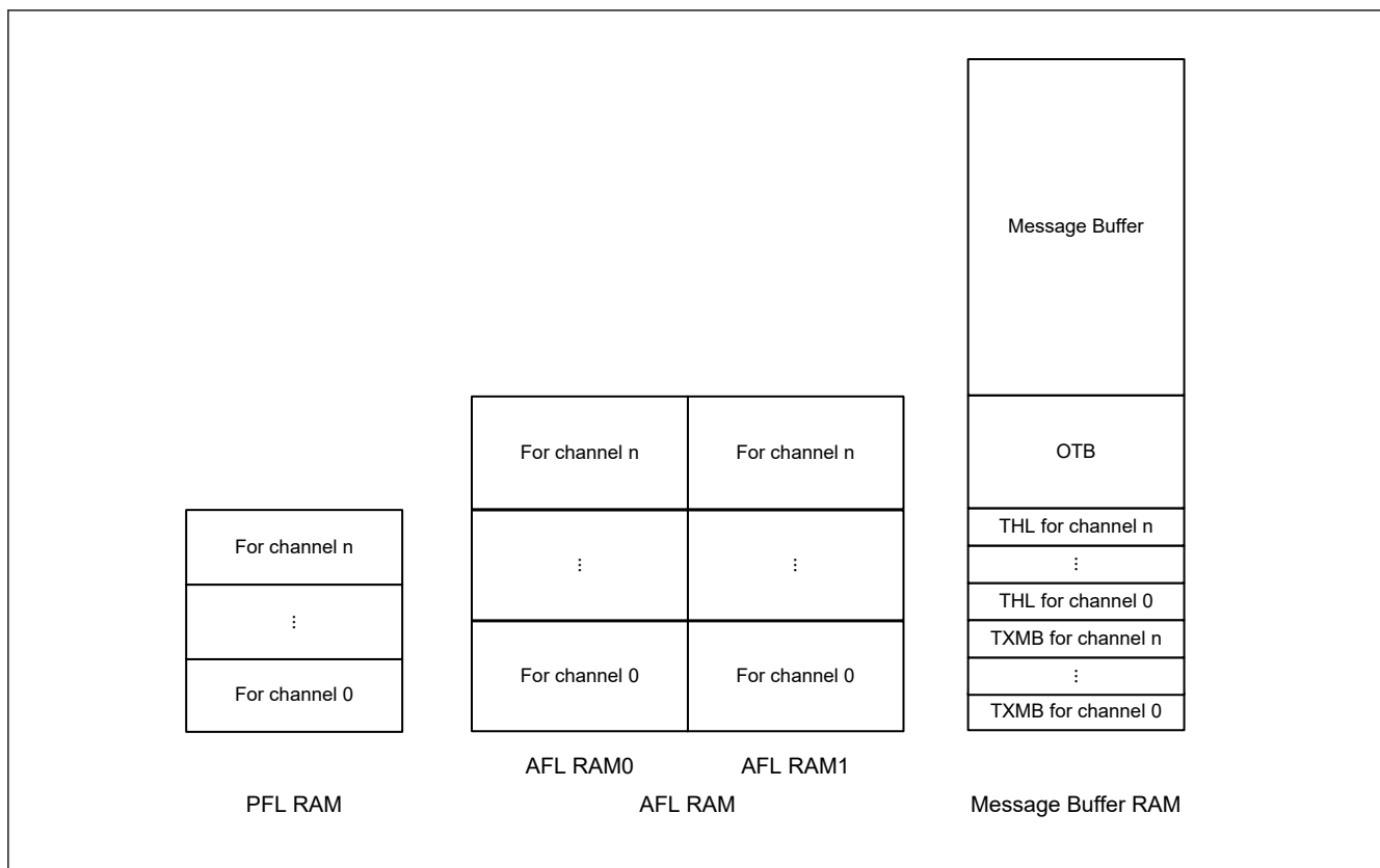
Figure 32.55 RAM area grouping
