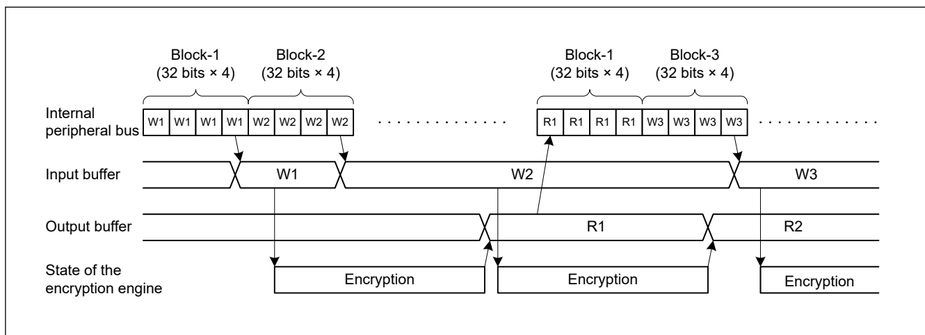
Figure 42.3 Encryption and decryption timing (AES)
