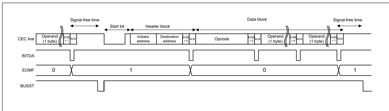
Figure 37.28 Timing of EOMF Flag
