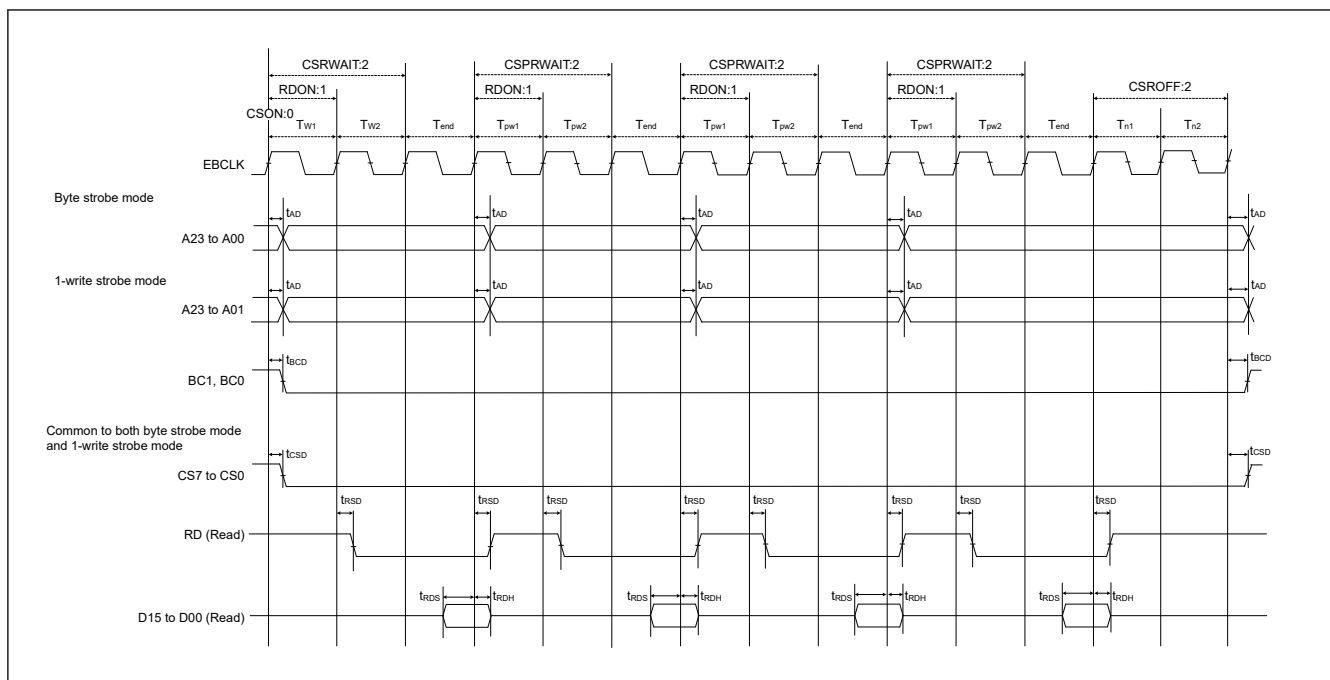
Figure 53.24 External bus timing for page read cycle with bus clock synchronized
