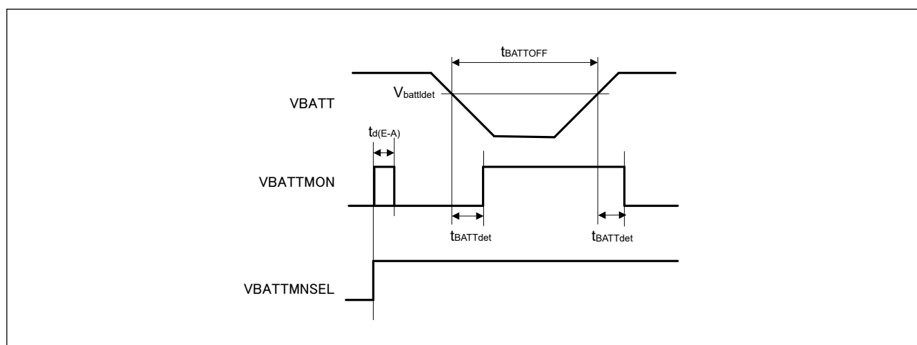
Figure 53.93 Battery backup function characteristics
