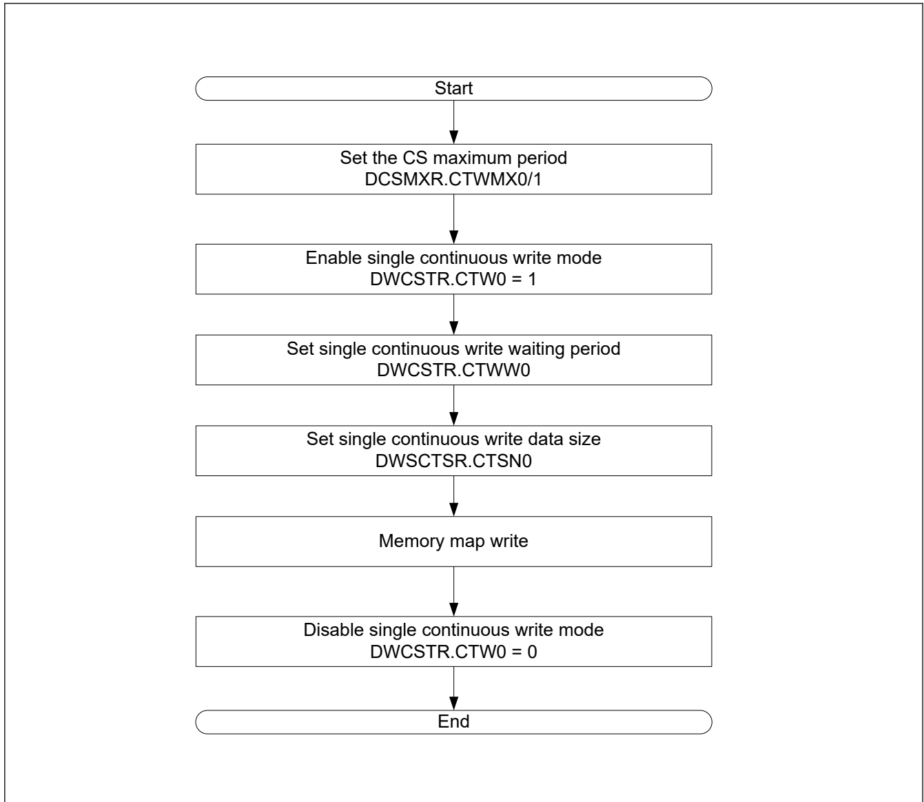
Figure 36.20 Procedure of single continuous write of OctaRAM
