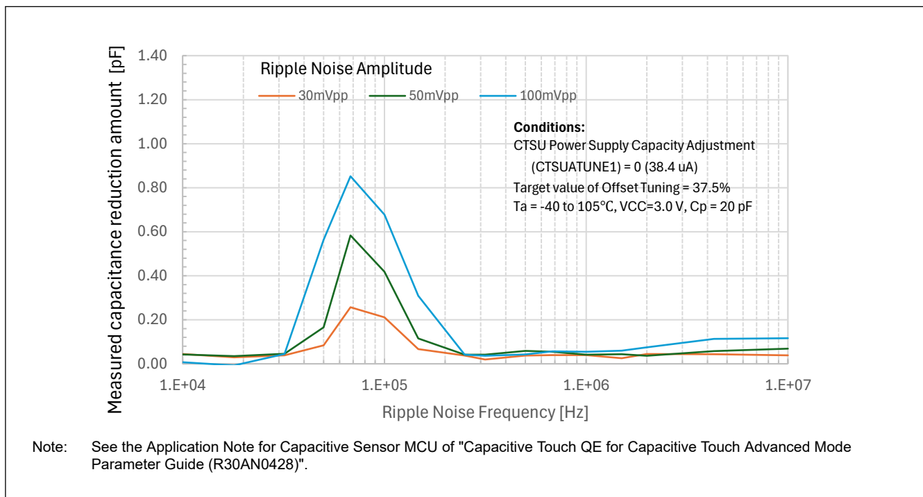
Figure 53.94 Measured capacitance reduction amount
