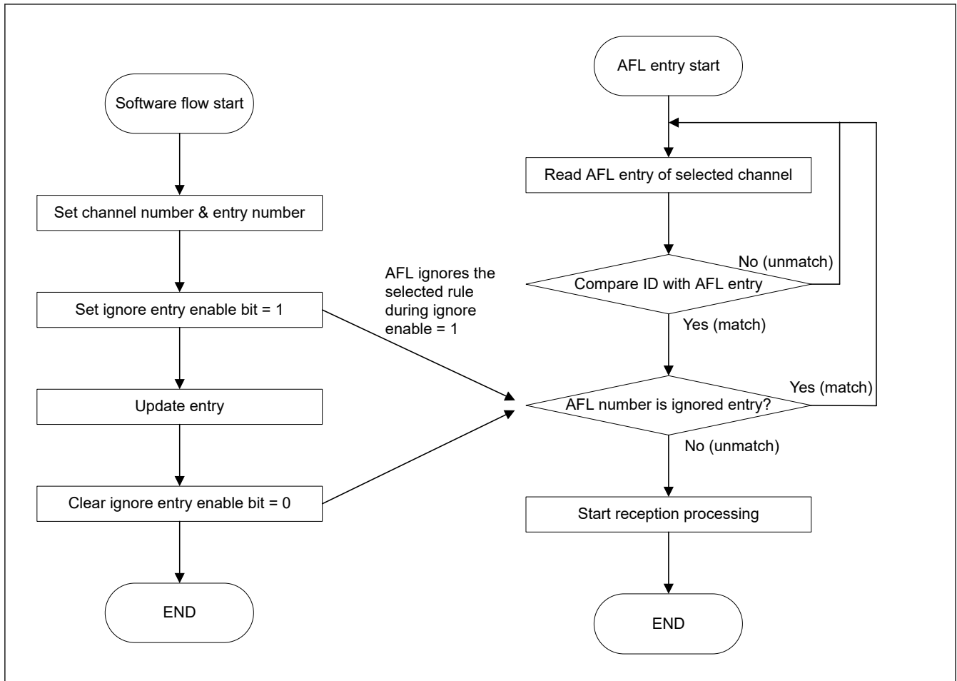
Figure 32.28 AFL entry update flow
