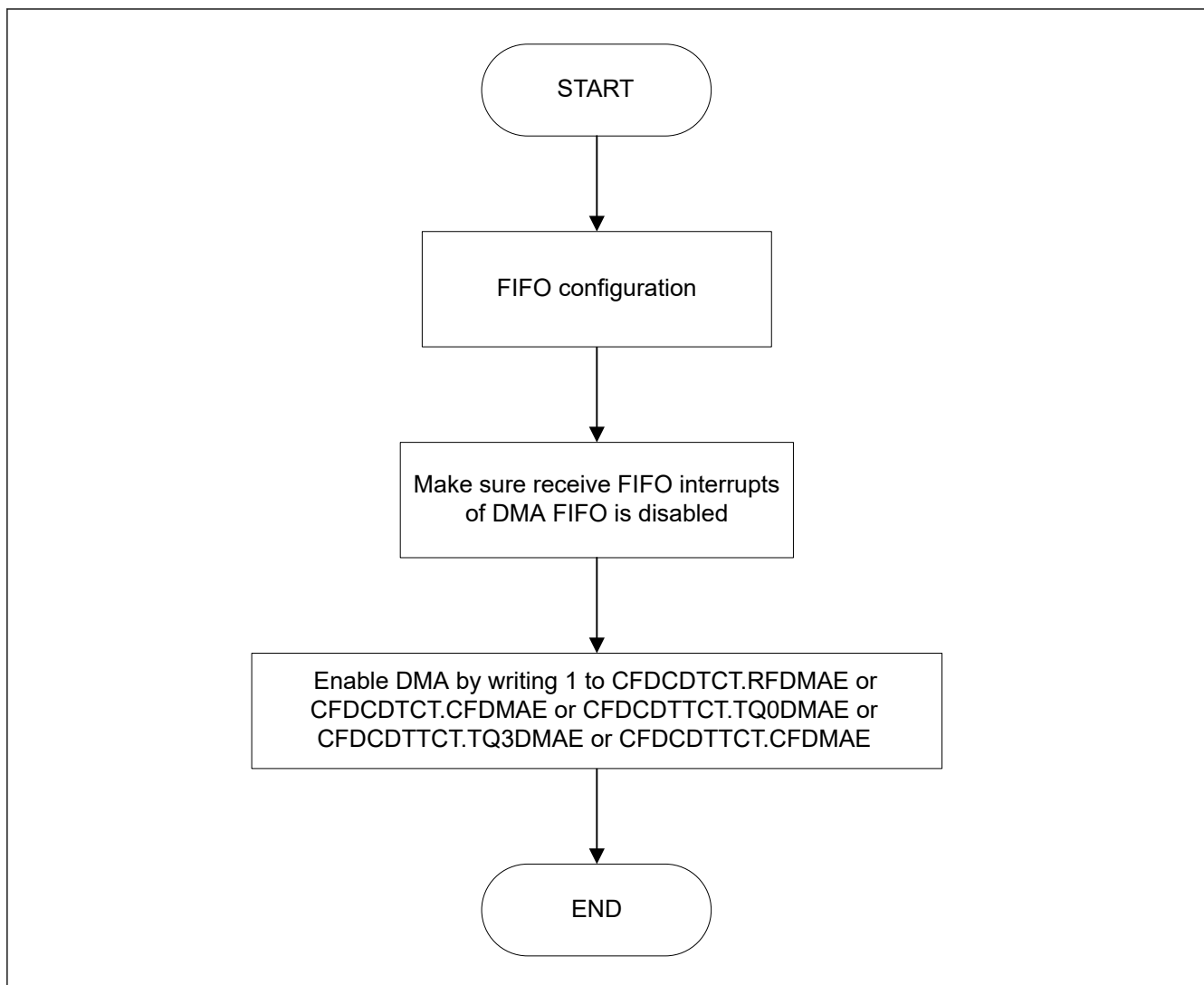
Figure 32.34 DMA enable flow
