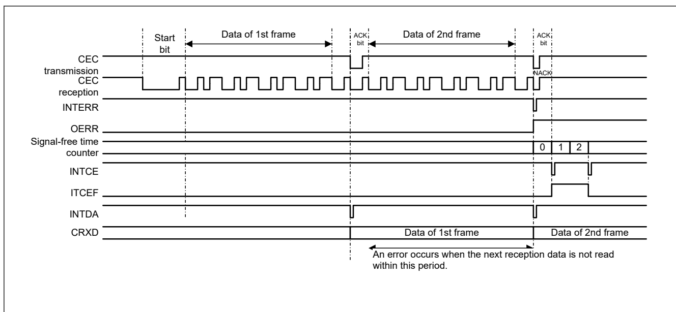
Figure 37.44 Timing of bus lock error during follower operation when 5 bits are set as signal-free time
