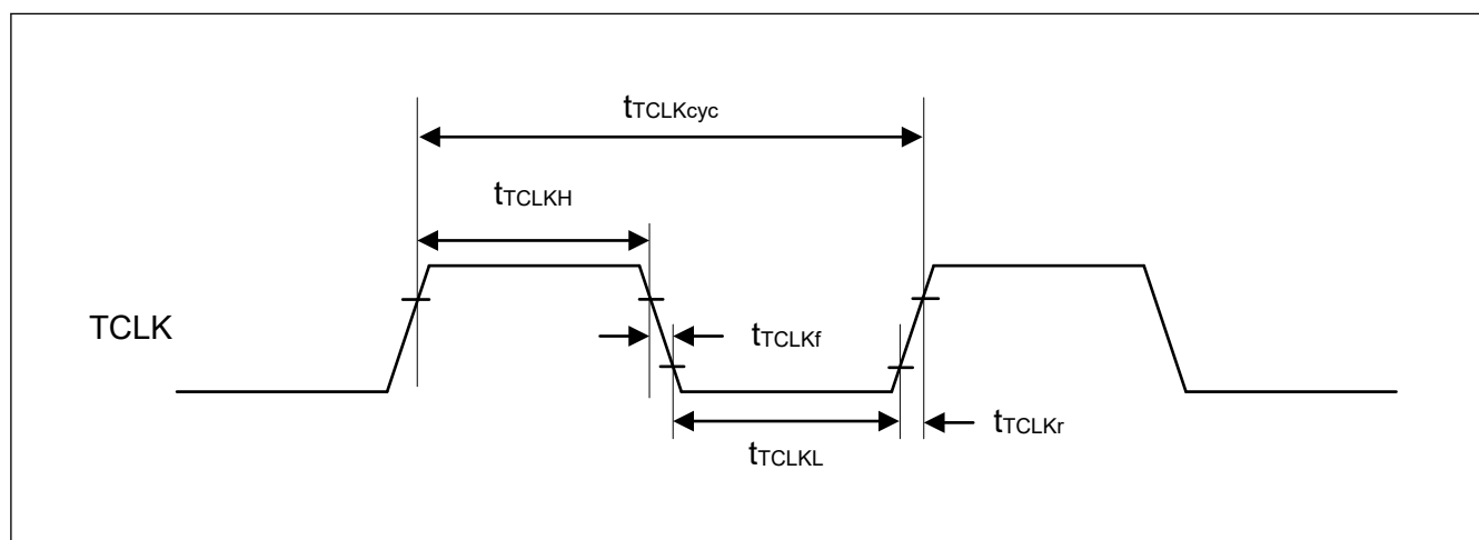
Figure 53.103 ETM TCLK timing
