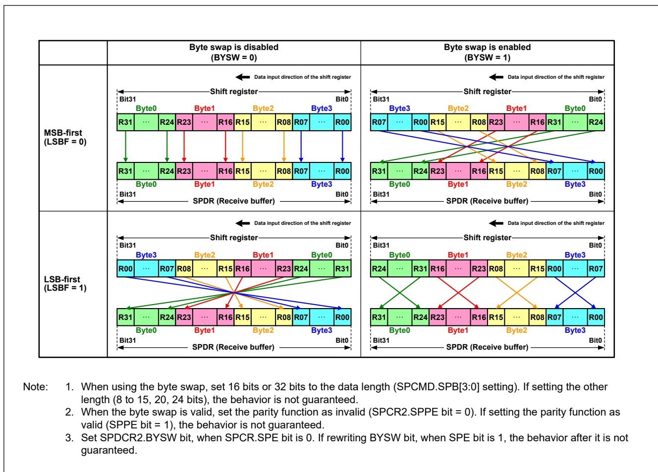
Figure 34.23 Byte swap with MSB/LSB transfer
