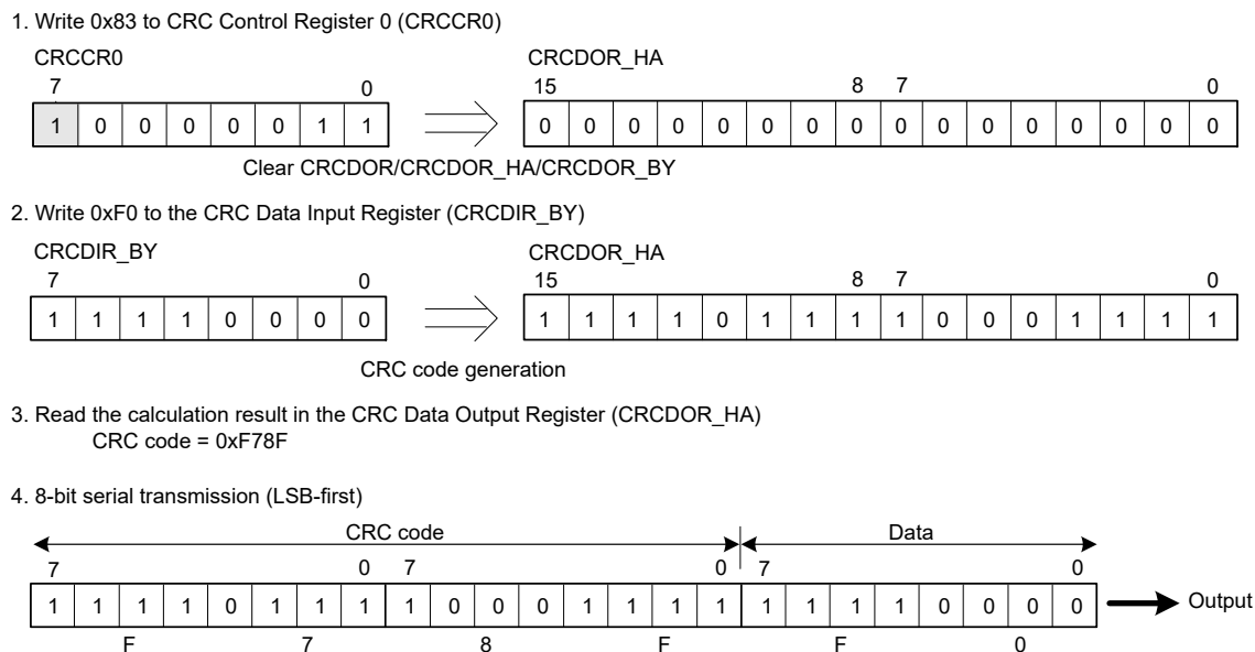
Figure 40.2 LSB-first data transmission
