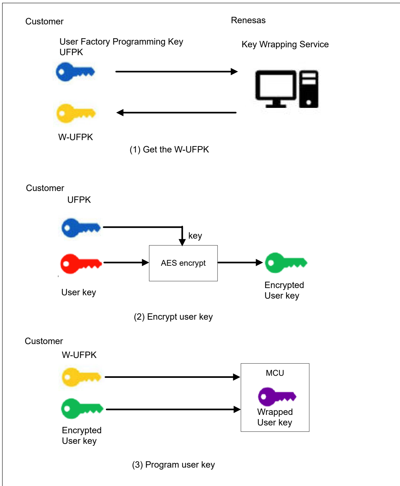
Figure 52.3 Key Injection
