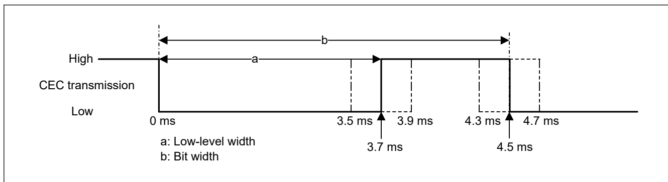
Figure 37.6 Example of start bit format
