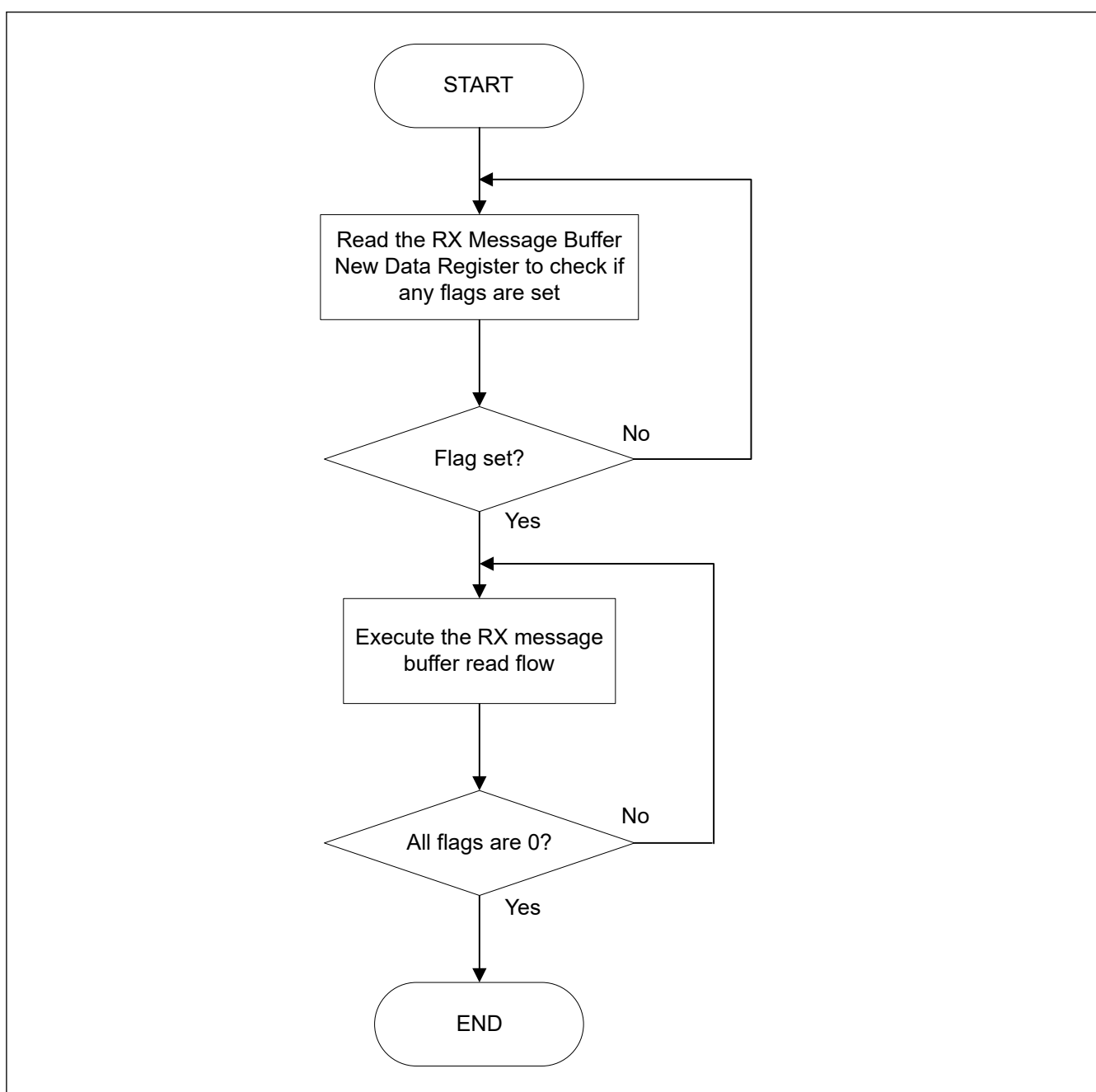
Figure 32.36 Access flow of RX message buffer
