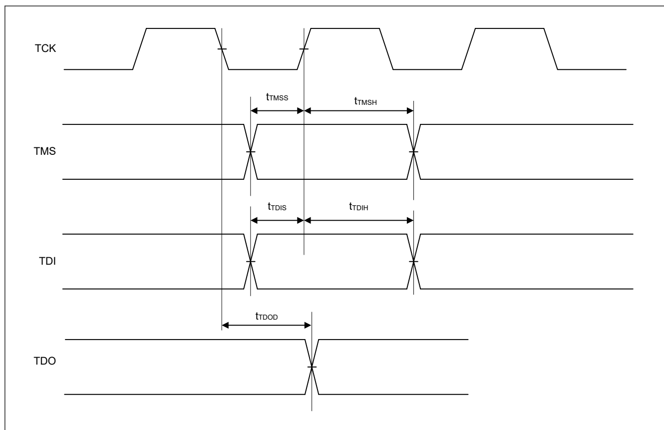
Figure 53.100 JTAG input/output timing
