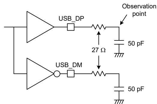
Figure 53.77 Test circuit in full-speed mode
