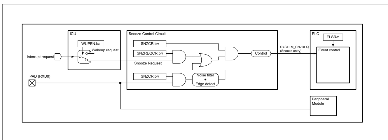
Figure 10.5 Snooze mode entry configuration
