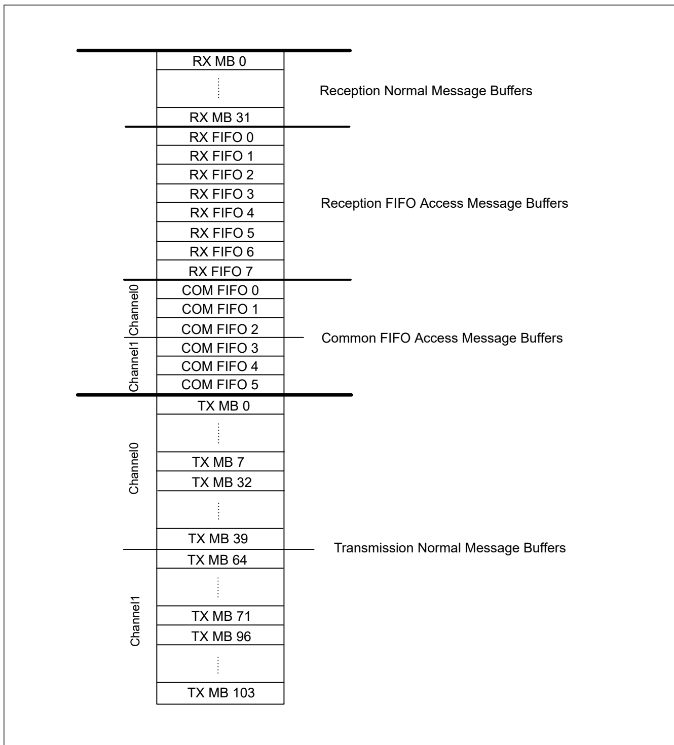
Figure 32.29 Message buffer configuration
