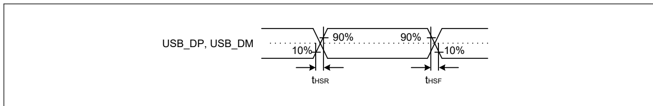
Figure 53.84 USB_DP and USB_DM output timing (high-speed)
