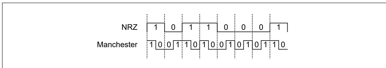
Figure 30.49 Example of Manchester Encoding
