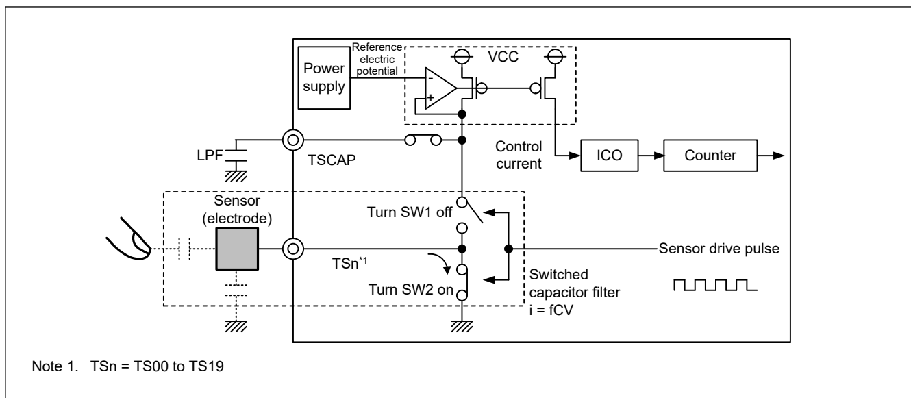
Figure 46.6 Discharging operation
