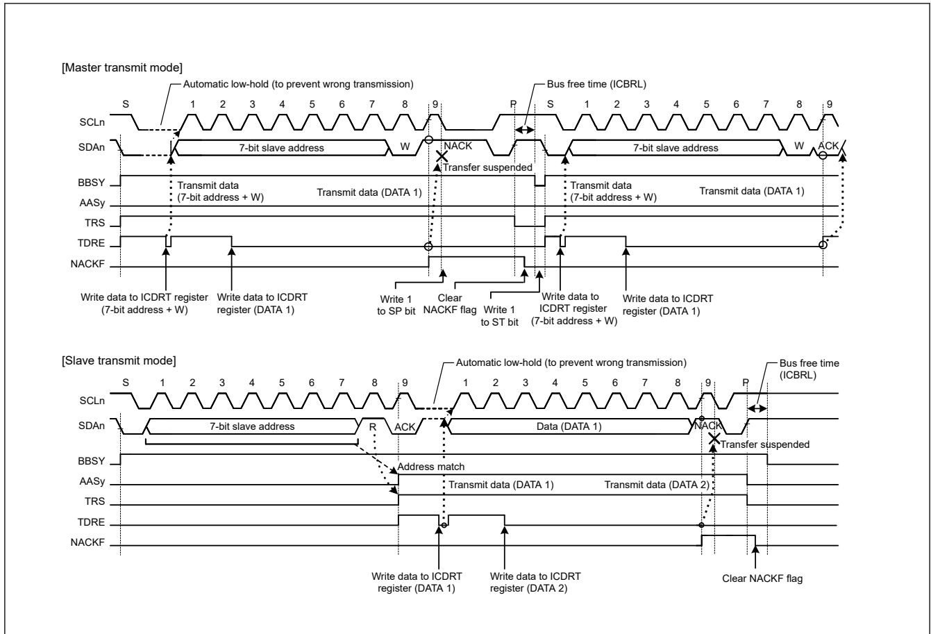
Figure 31.39 Suspension of data transfer when NACK is received, when NACKIE = 1
