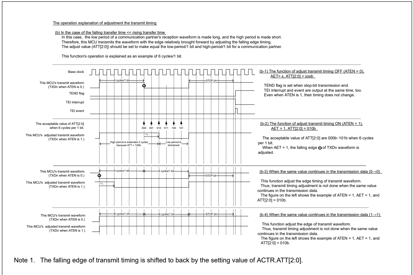
Figure 30.39 The adjustment operation explanation for the transmit timing when AET is 1
