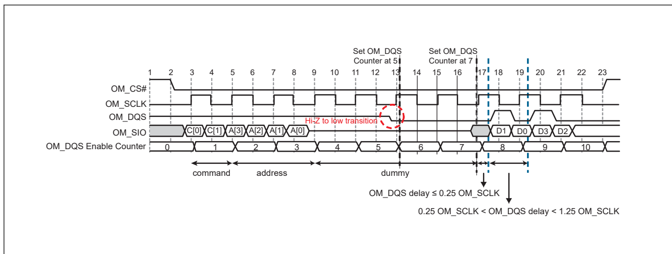
Figure 36.22 Timing example of OM_DQS clock input transitions from Hi-Z to Low (Flash DQPI mode, dummy cycle number = 4, OM_DQS pre-cycle on)
