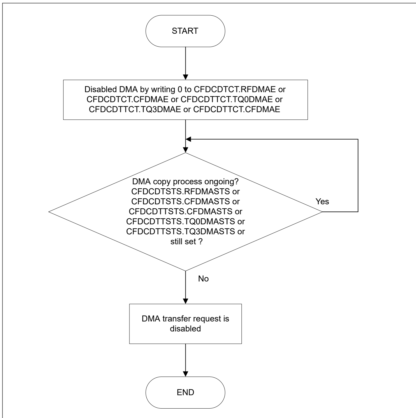
Figure 32.35 DMA disable flow
