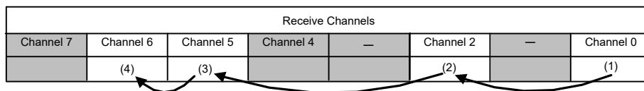
Figure 46.14 Software flow and example operation for self-capacitance multi-scan mode
