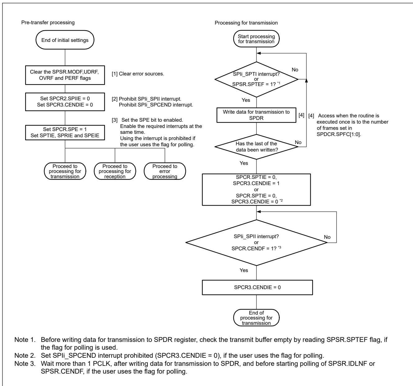
Figure 34.53 Transmission flow in slave mode
