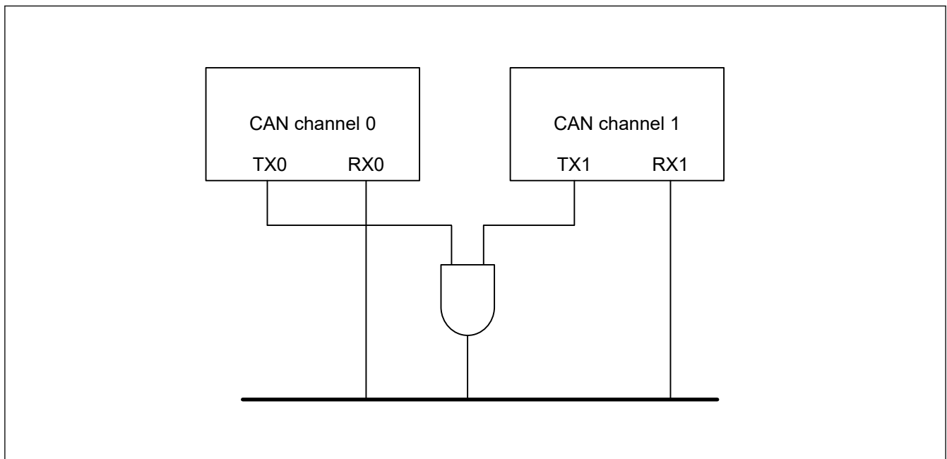
Figure 32.54 Internal CAN bus connections
