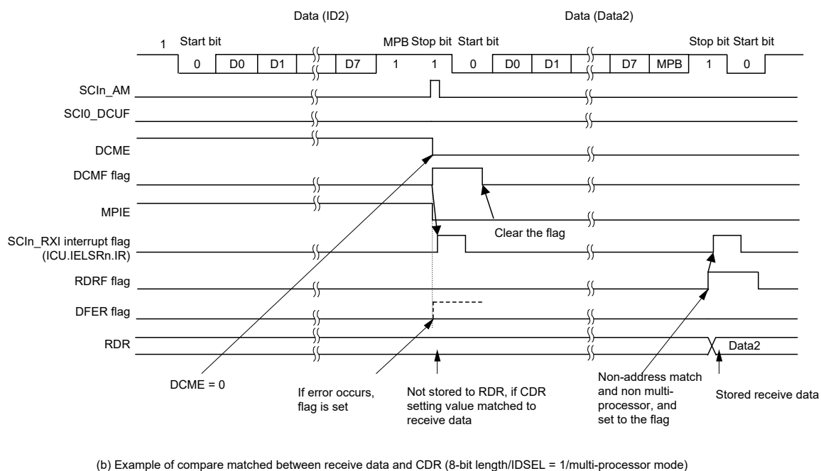
Figure 30.10 Example of address match (2) multi-processor mode
