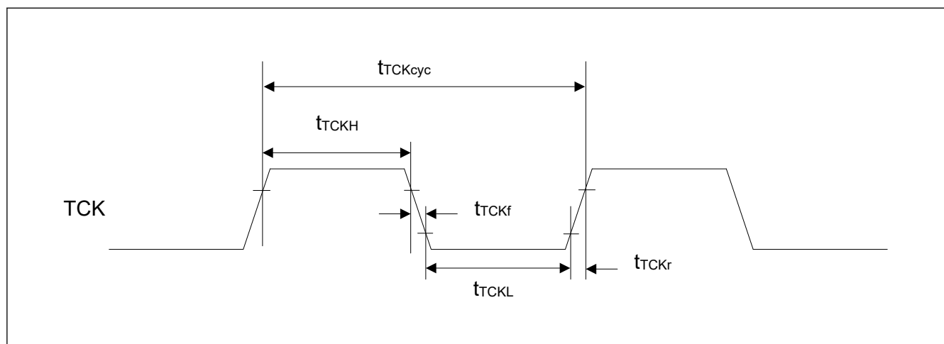
Figure 53.99 JTAG TCK timing
