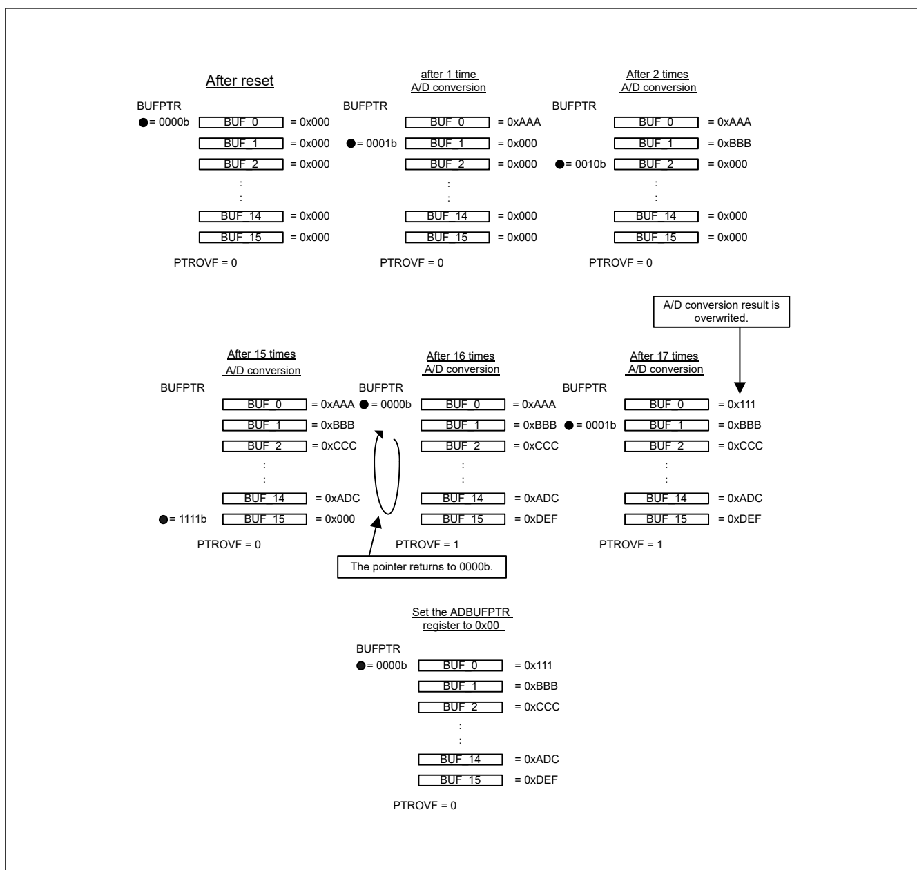
Figure 43.37 Data Buffers, Pointer, and Overflow Flag Operations
