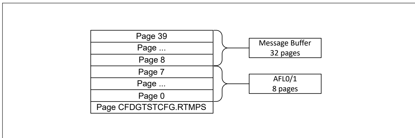
Figure 32.52 RAM page structure
