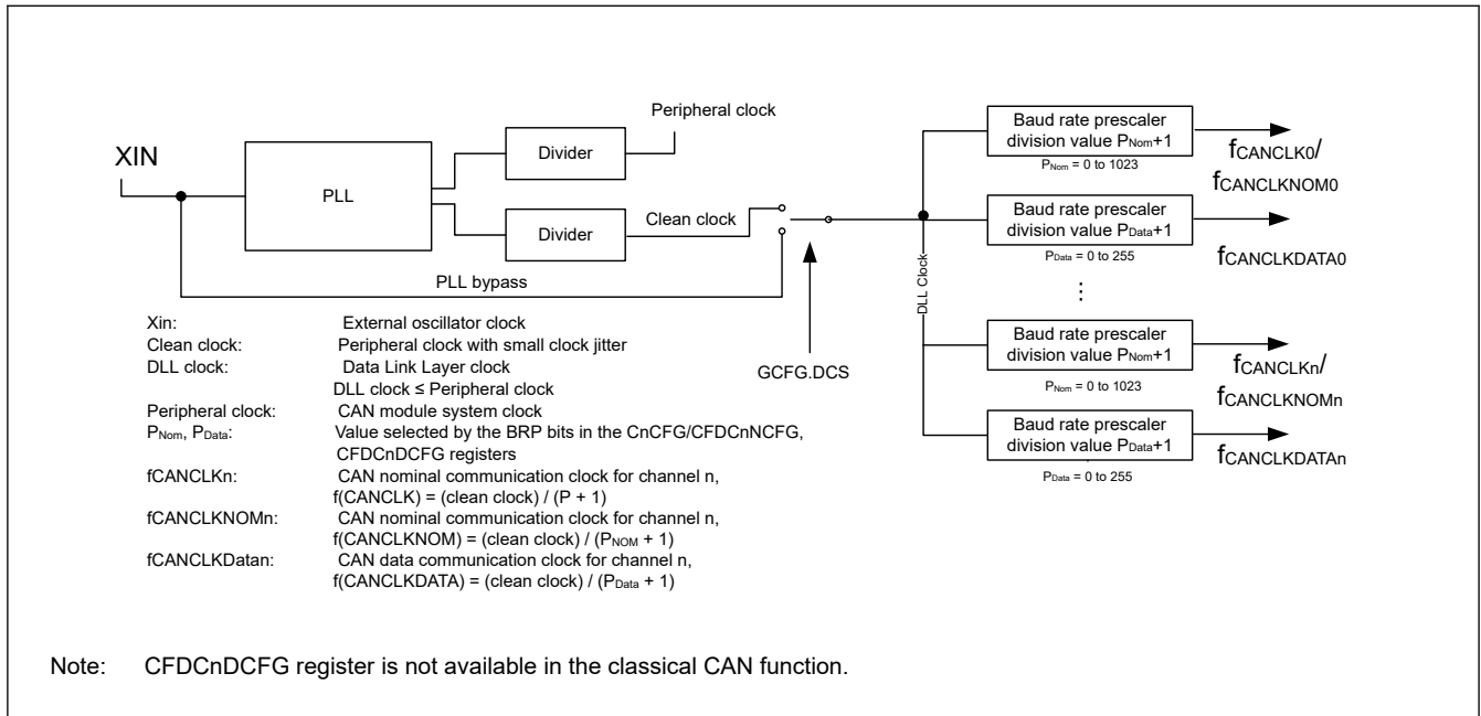
Figure 32.16 Block diagram of the circuit that generates the CAN channel communication clock
