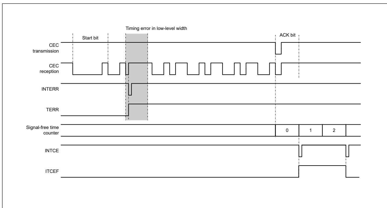
Figure 37.42 Timing error when bit width is not short during follower operation
