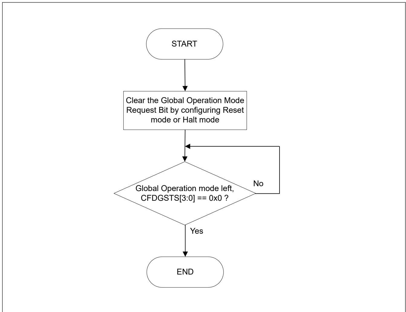
Figure 32.10 Procedure for exiting Global Operation mode
