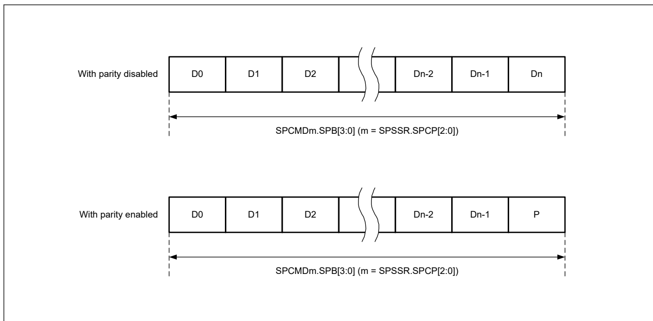
Figure 34.13 Data format with parity disabled and enabled
