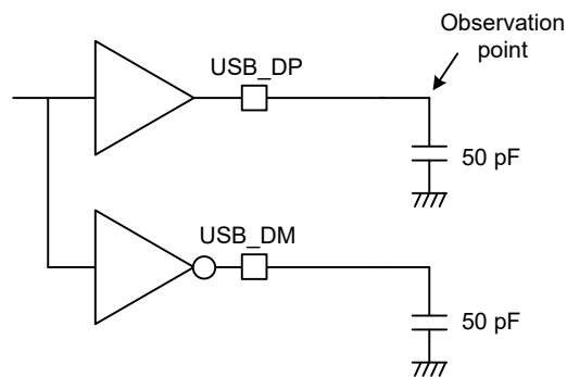
Figure 53.81 Test circuit in full-speed mode
