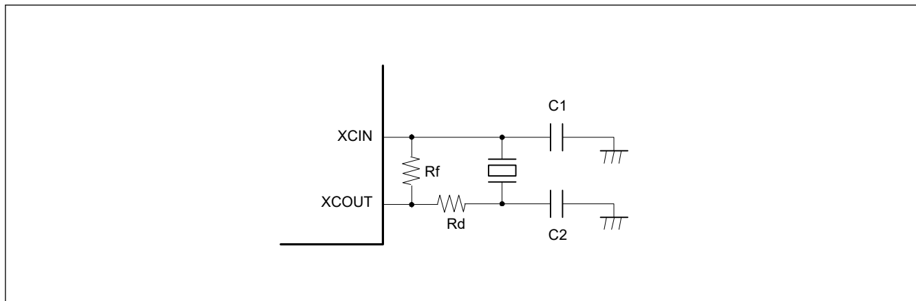
Figure 8.7 Connection example of a 32.768-kHz crystal resonator
