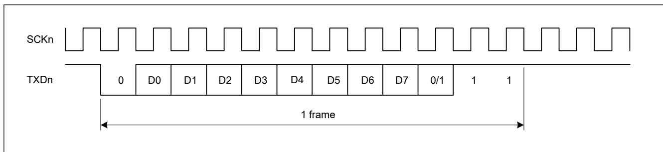
Figure 30.8 Phase relationship between output clock and transmit data in asynchronous mode when SMR.CHR = 0, PE = 1, MP = 0, and STOP = 1
