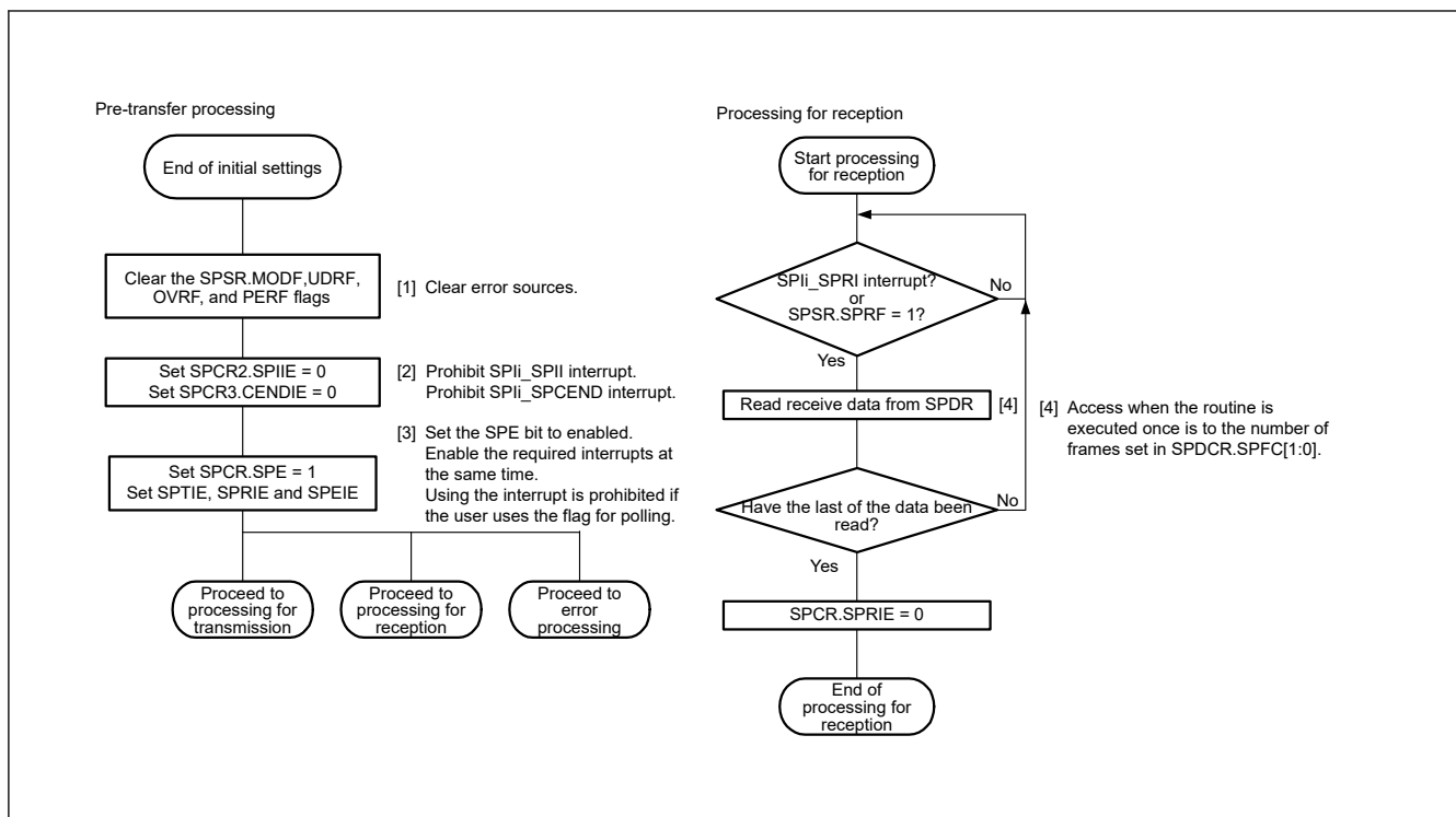
Figure 34.54 Reception flow in slave mode
