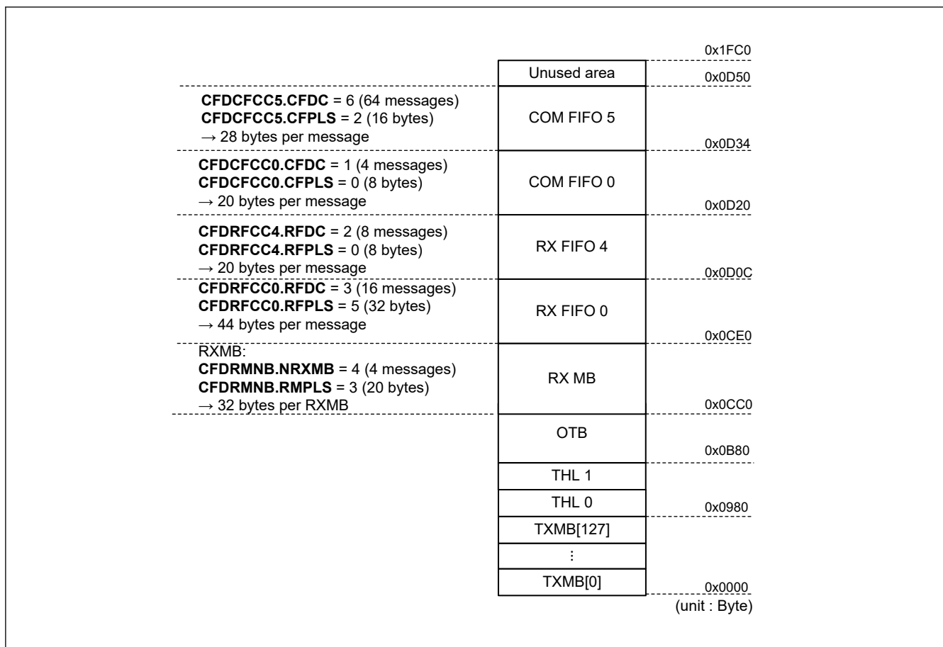
Figure 32.56 RX MB + FIFO buffers RAM area configuration examples of a CANFD 2 channel version
