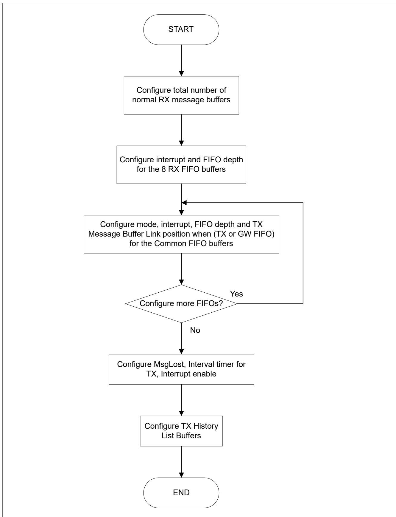
Figure 32.30 FIFO buffer configuration flow in CANFD module
