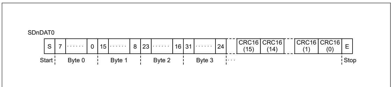
Figure 39.2 SDnDAT in 1-bit width mode
