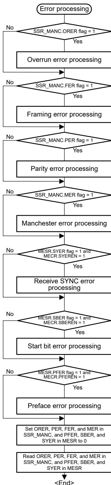
Figure 30.62 Example of Serial Reception Flowchart in Manchester Mode (Error Processing)
