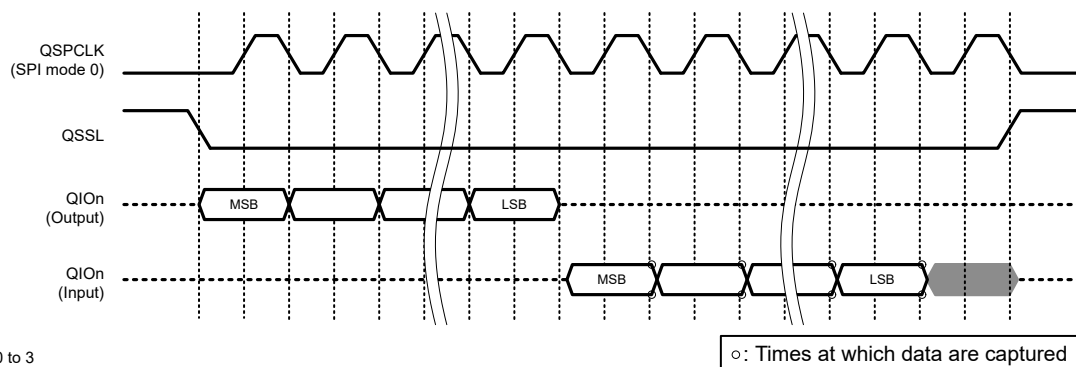
Figure 35.8 Basic serial interface timing (SPI mode 0)
