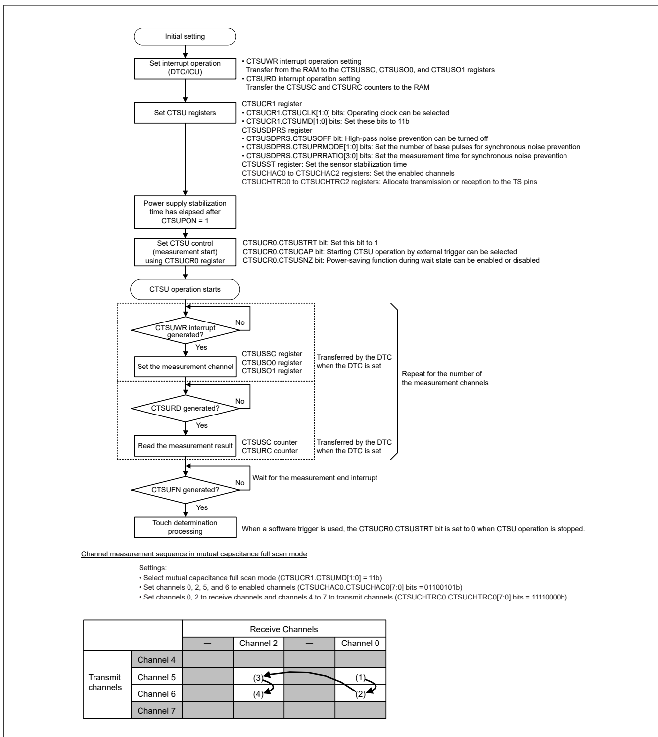
Figure 46.16 Software flow and example operation for mutual capacitance full scan mode
