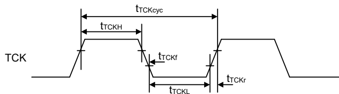
Figure 53.96 Boundary scan TCK timing
