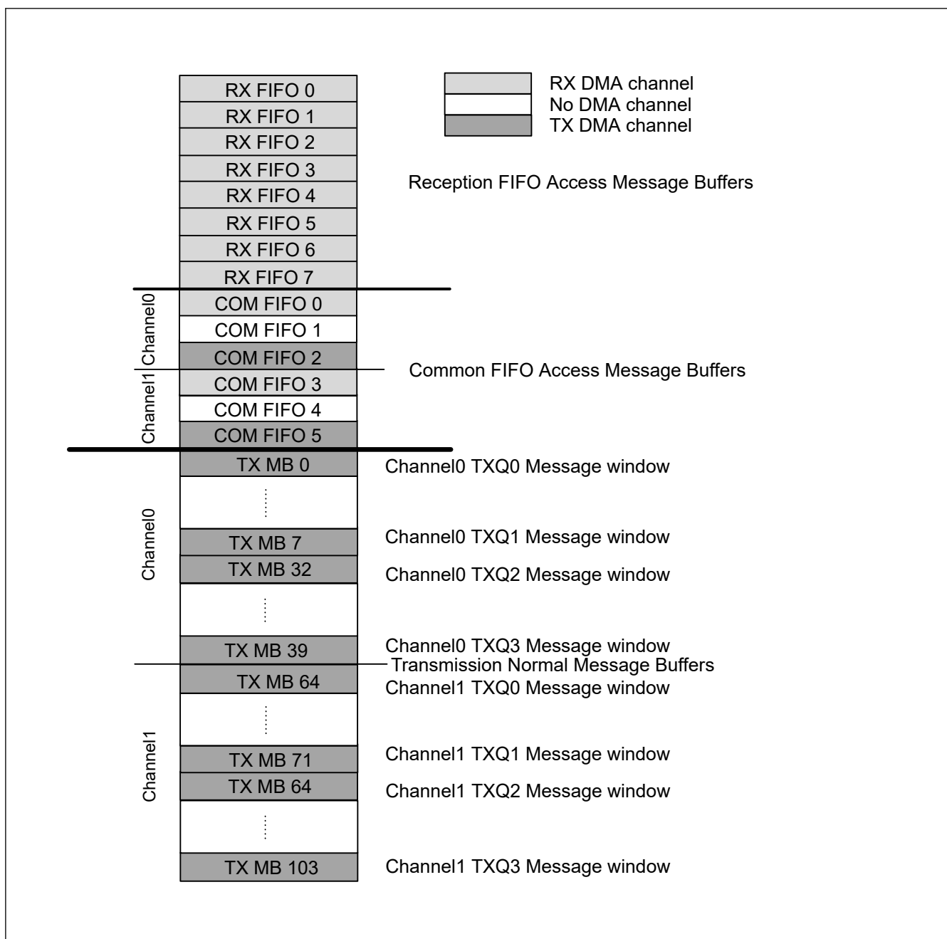
Figure 32.33 Message buffer connectable to a DMA channel
