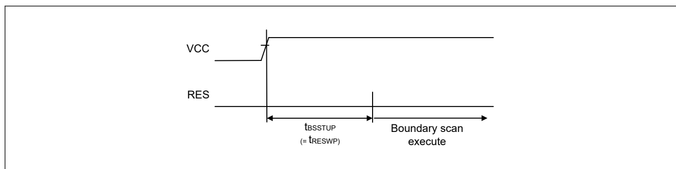
Figure 53.98 Boundary scan circuit startup timing
