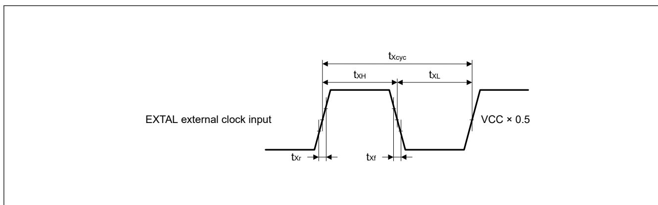
Figure 53.8 EXTERNAL external clock input timing
