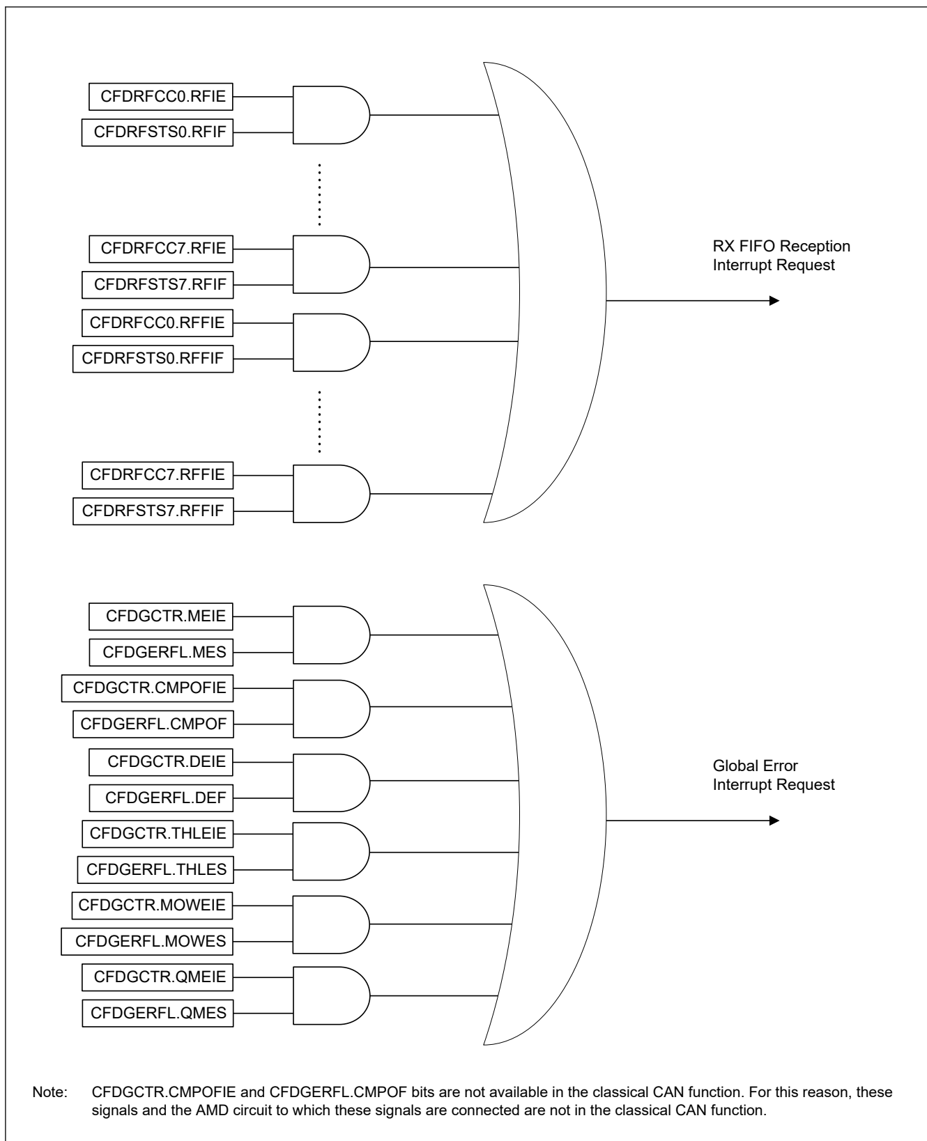
Figure 32.31 Global interrupt block diagram
