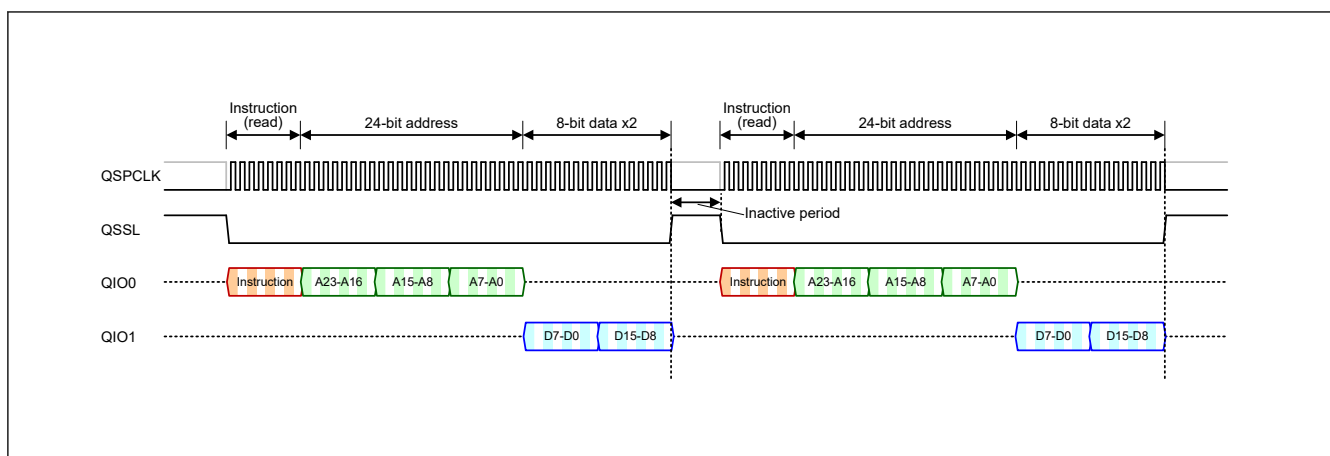
Figure 35.32 Successive data read operations based on individual conversion
