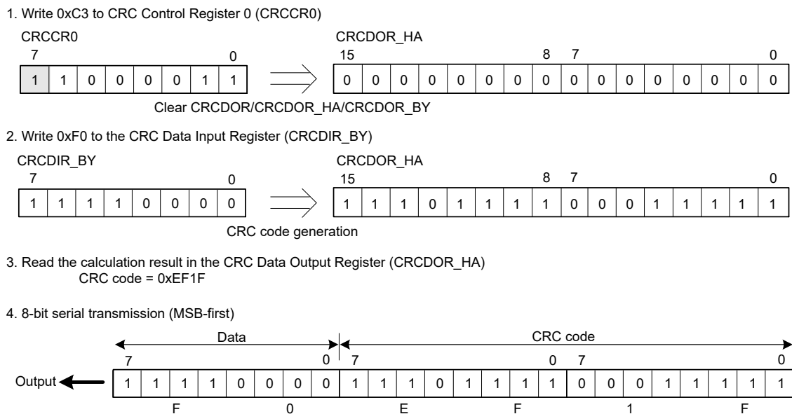
Figure 40.3 MSB-first data transmission
