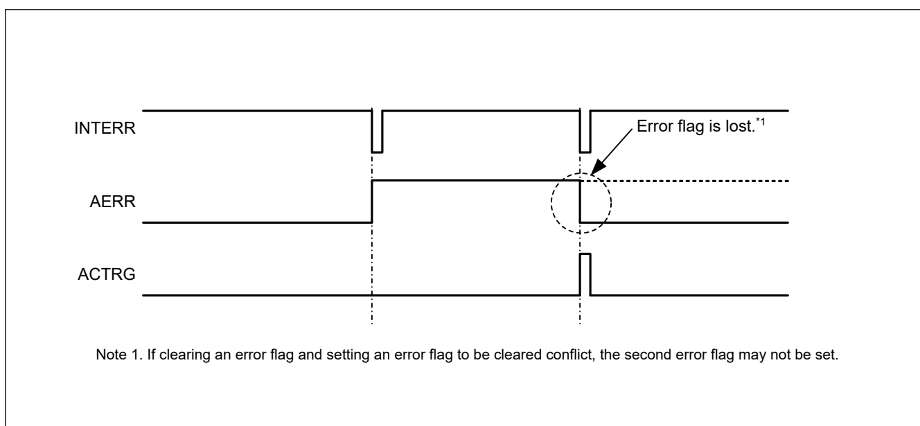
Figure 37.45 When two identical errors occurred and conflicted with the clear trigger
