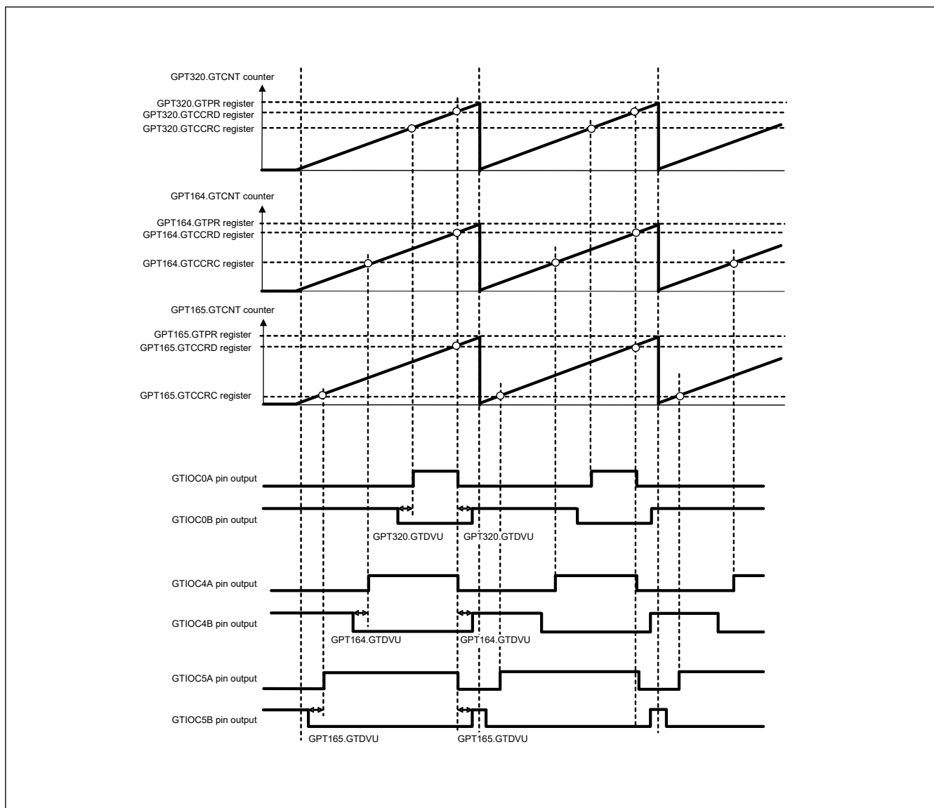
Figure 21.41 Example of a 3-phase saw-wave complementary PWM output with automatic dead time setting
