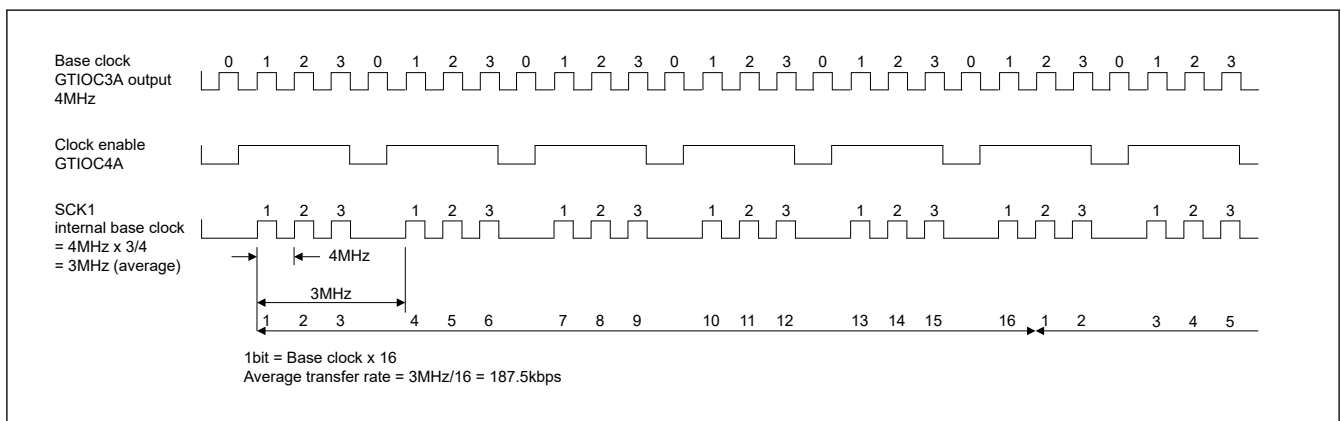
Figure 29.4 Example of average transfer rate setting when a GPT clock is input
