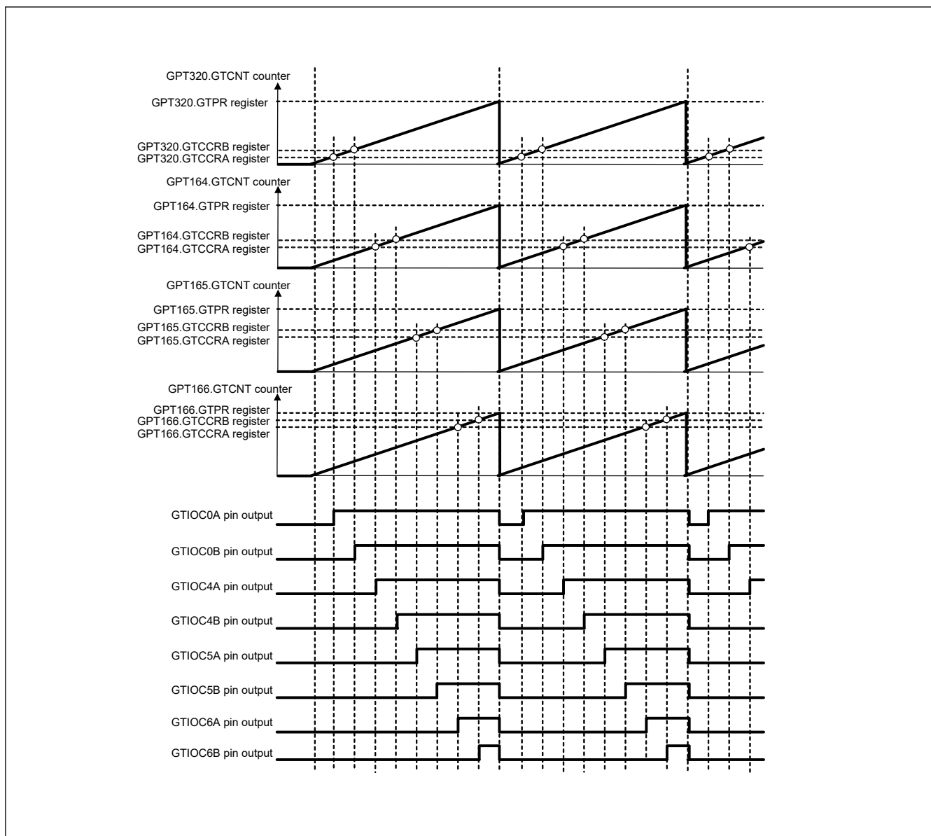
Figure 21.39 Example of a synchronized PWM output
