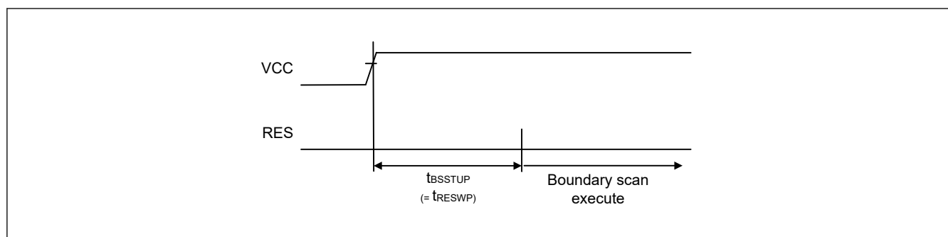
Figure 50.90 Boundary scan circuit startup timing
