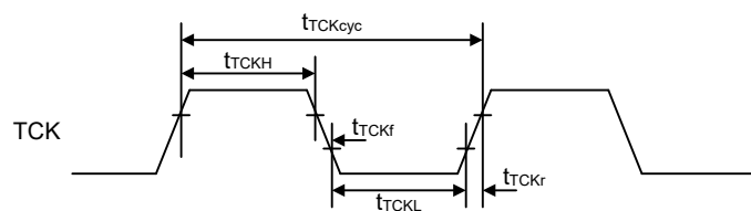
Figure 50.88 Boundary scan TCK timing
