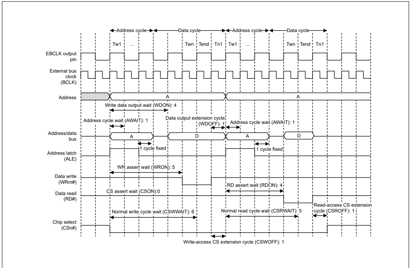
Figure 14.25 Example of bus timing with address/data multiplexed I/O interface (m = 0, 1)
