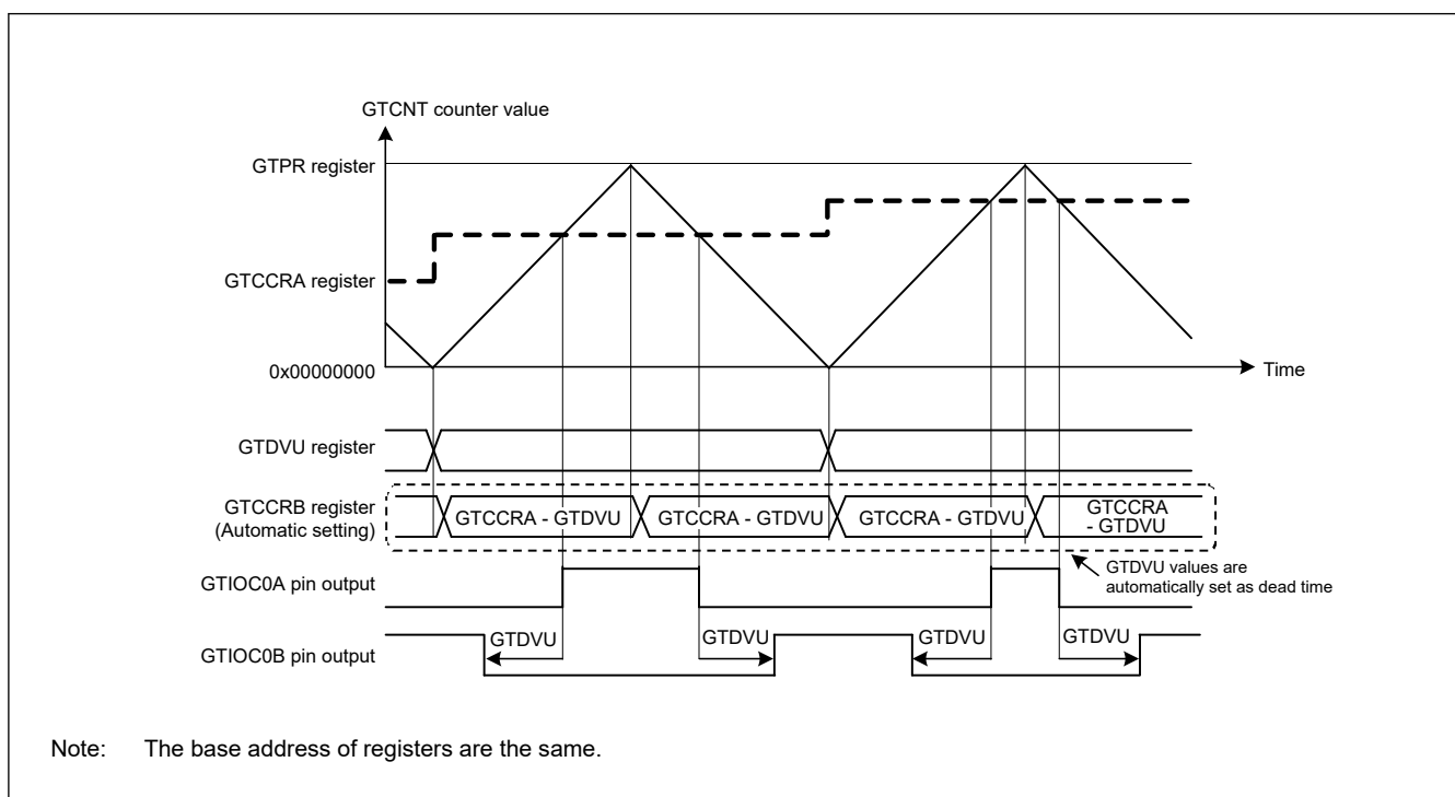
Figure 21.26 Example of an automatic compare-match value setting function with dead time in triangle-wave PWM mode 1, and active-high
