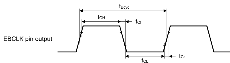
Figure 50.7 EBCLK output timing
