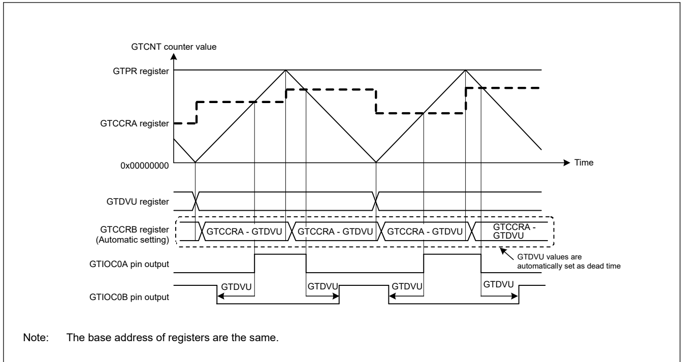
Figure 21.27 Example of an automatic compare-match value setting function with dead time in triangle-wave PWM mode 2 or 3, and active-high
