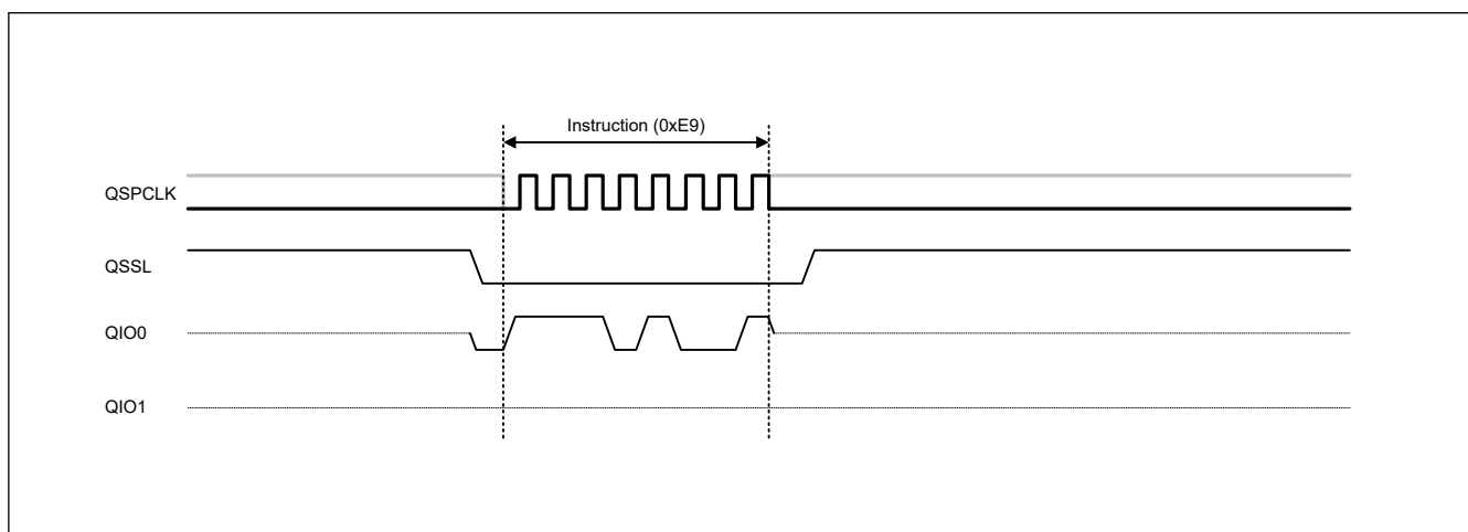
Figure 33.30 Exit 4-Byte Mode bus cycle
