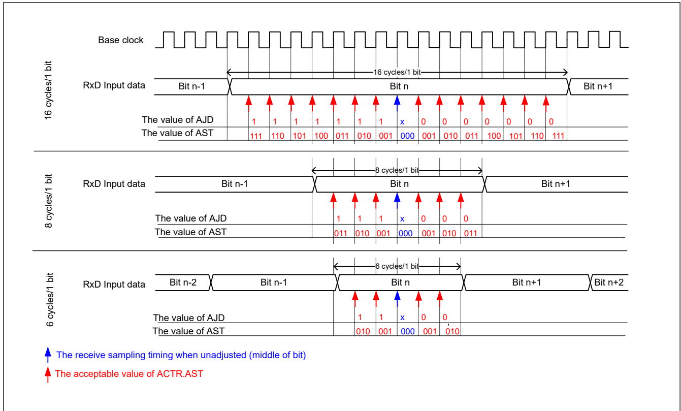
Figure 29.34 Overview of the adjustment operation for the reception sampling timing (asynchronous mode using an internal clock)
