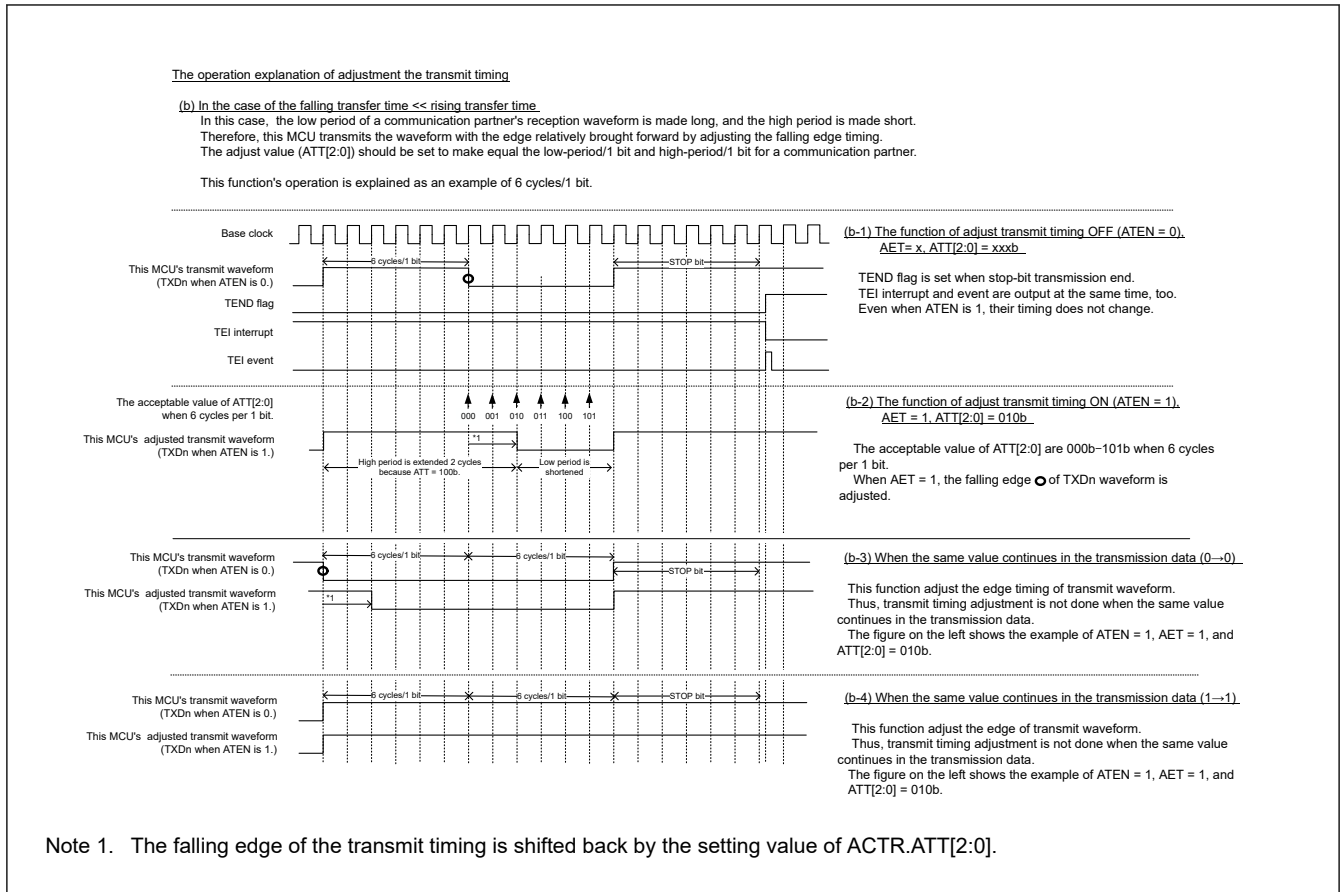
Figure 29.39 Adjustment operation explanation for a transmit timing when AET is 1
