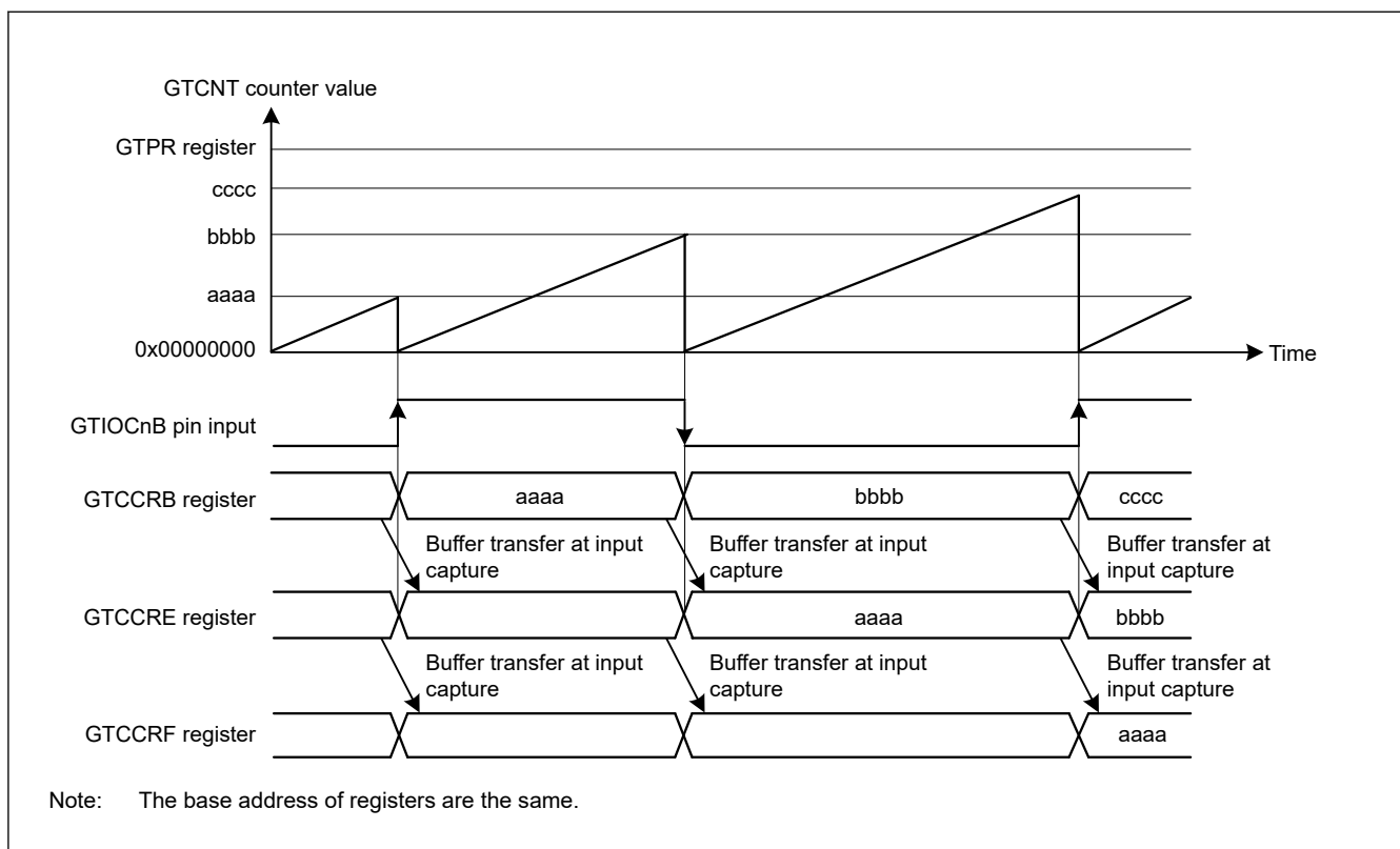
Figure 21.18 Example of GTCCRB double buffer operation with input capture at both edges of GTIOcNB input, saw waves in up-counting, and GTCNT counter cleared at both edges of GTIOcNB input
