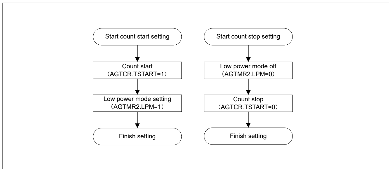
Figure 22.2 Flow chart for writing LPM bit
