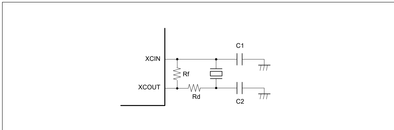
Figure 8.5 Connection example of a 32.768-kHz crystal resonator
