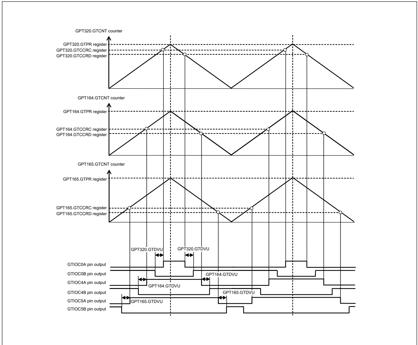
Figure 21.44 Example of a 3-phase asymmetric triangle-wave complementary PWM output with automatic dead time setting
