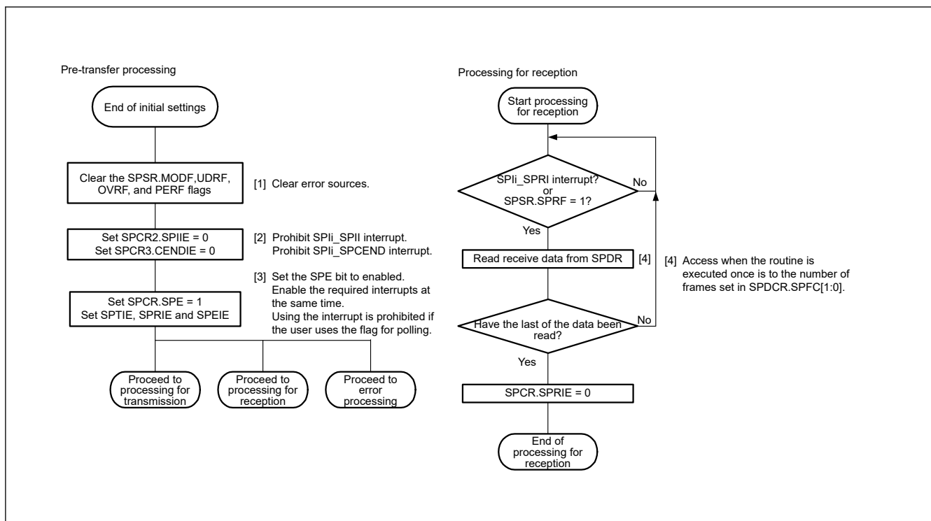
Figure 32.54 Reception flow in slave mode
