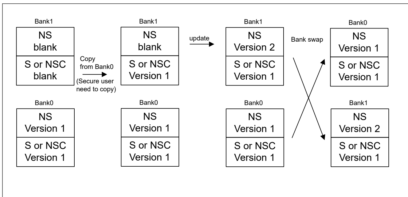
Figure 49.5 Field updating flow of non-secure region
