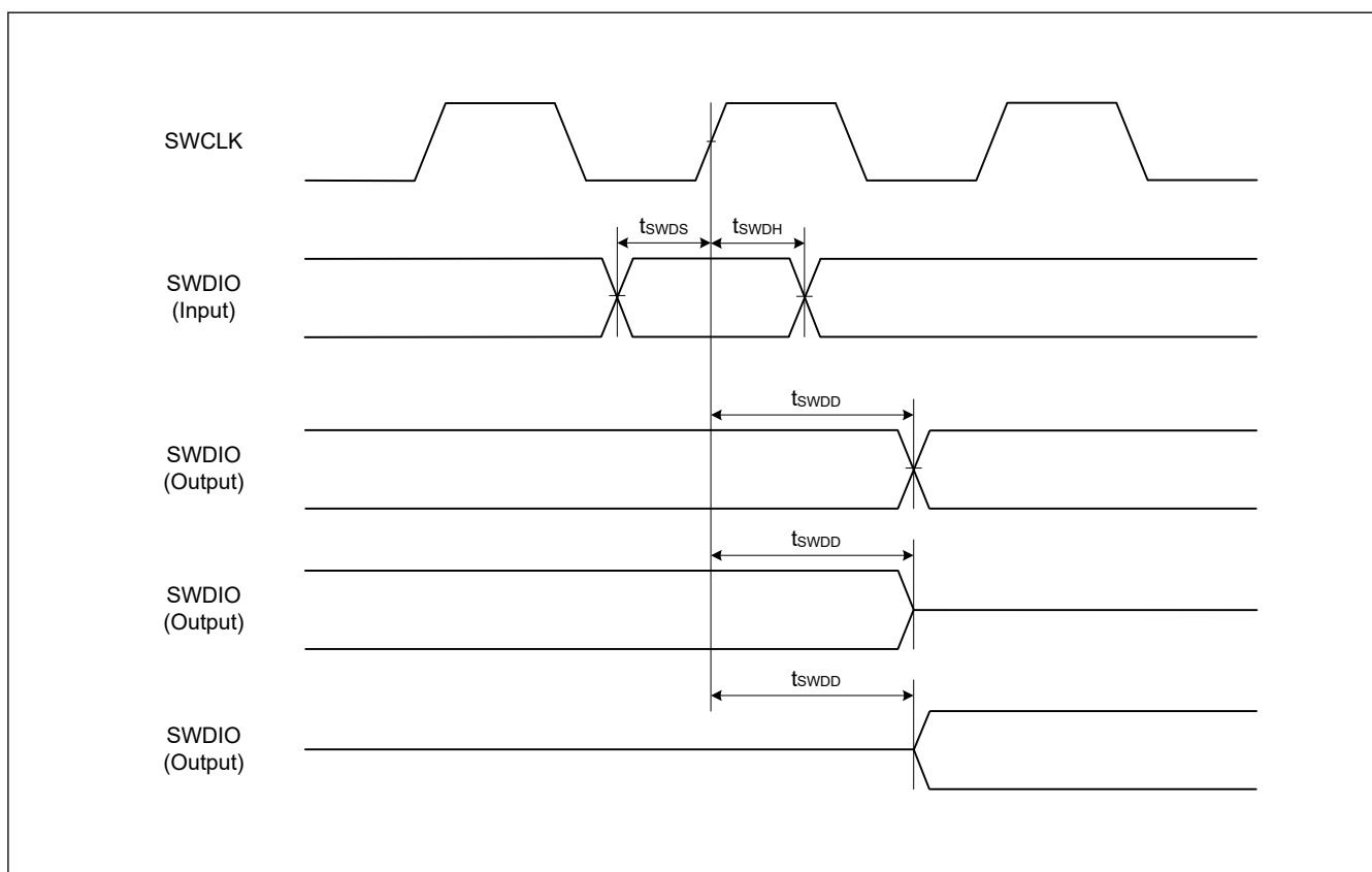
Figure 50.94 SWD input/output timing
