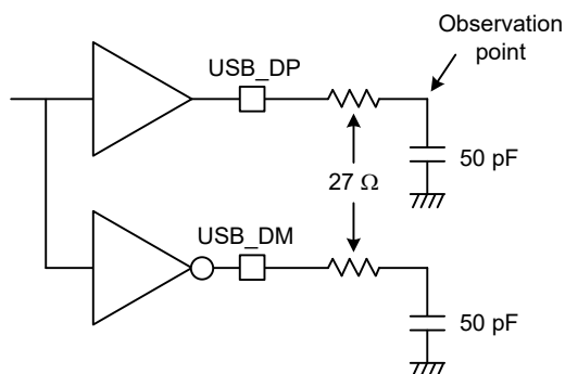
Figure 50.77 Test circuit in full-speed mode
