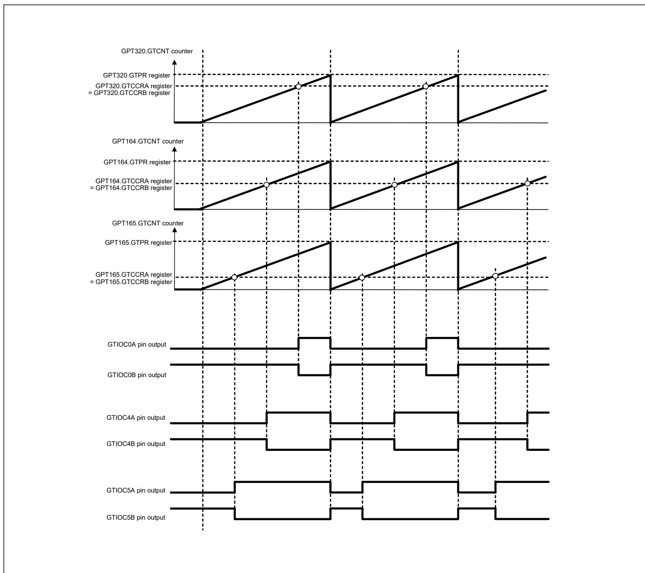
Figure 21.40 Example of a 3-phase saw-wave complementary PWM output
