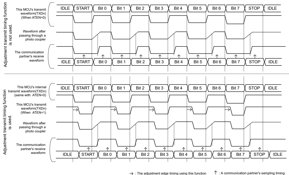
Figure 29.37 Explanation for a transmit waveform through a photo coupler
