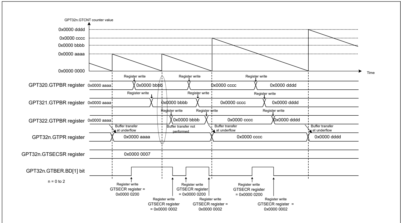
Figure 21.65 Example of multiple channel operations for disabling buffer operation (saw waves, single buffer operation)
