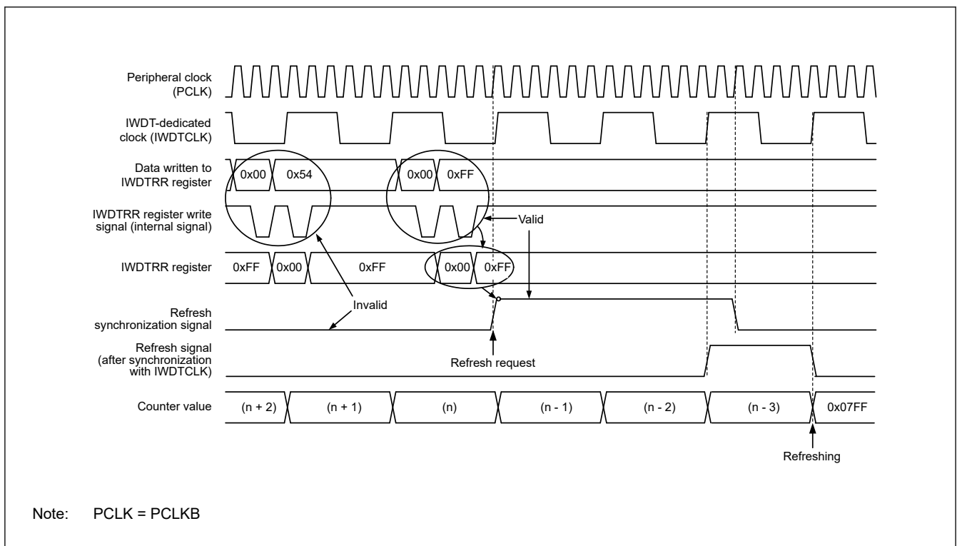
Figure 25.4 IWDT refresh operation waveforms when OFS0.IWDTCKS[3:0] = 0000b, OFS0.IWDTTOS[1:0] = 11b
