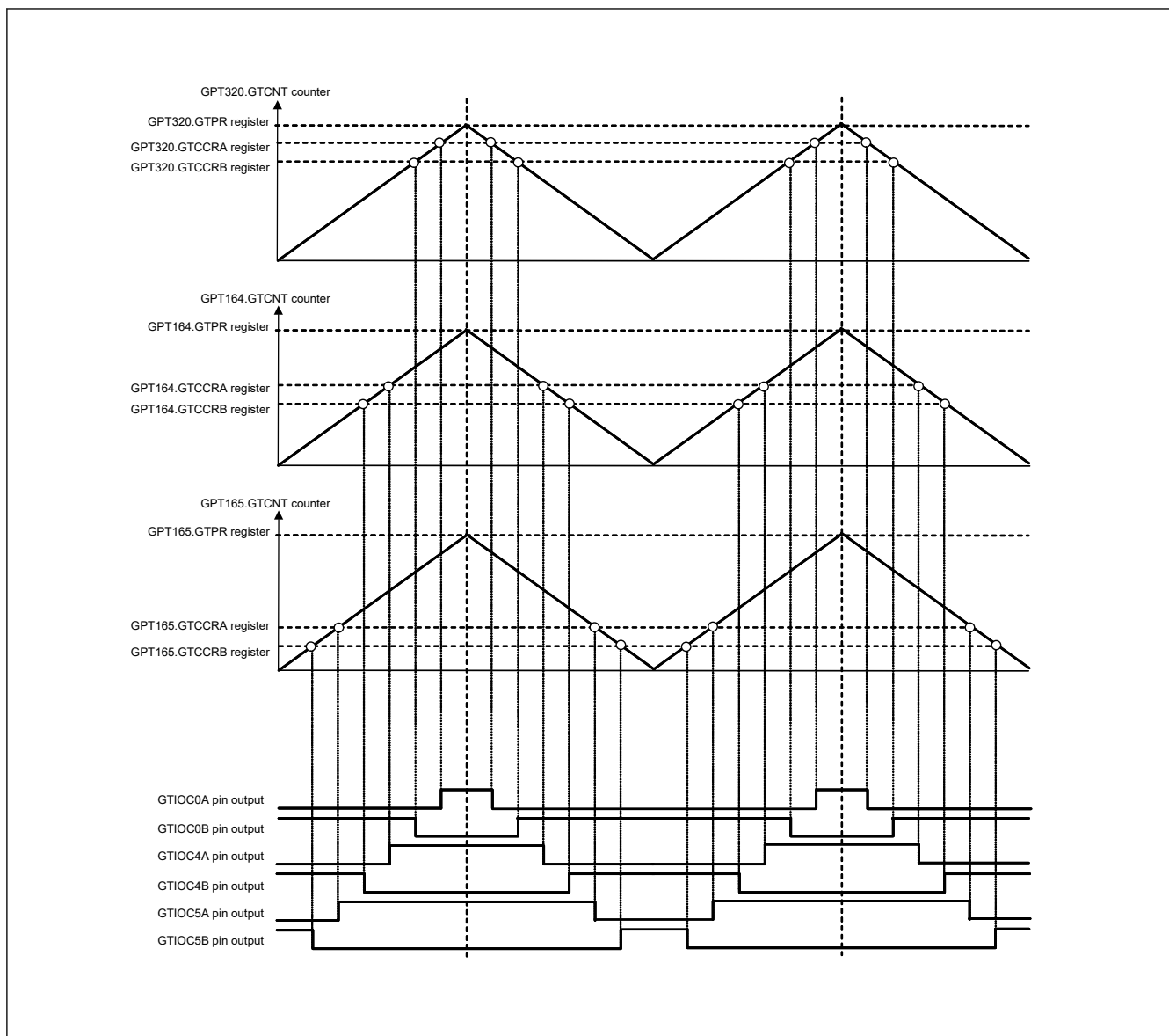
Figure 21.42 Example of a 3-phase triangle-wave complementary PWM output
