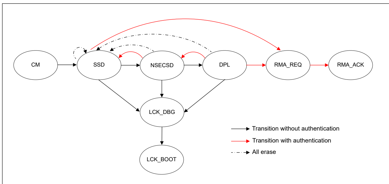
Figure 49.2 Illustration of the device lifecycle
