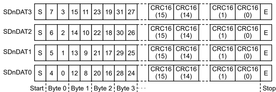
Figure 36.3 SDnDAT in 4-bit width mode
