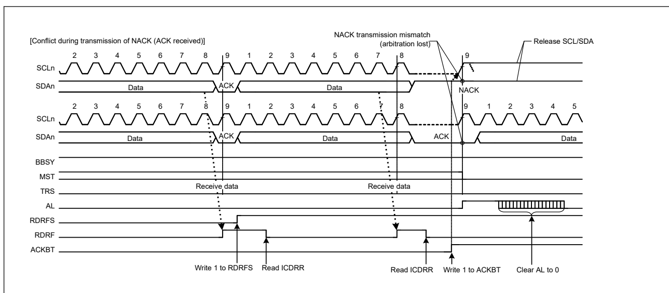
Figure 30.43 Example of arbitration-lost detection during transmission of NACK when NALE = 1
