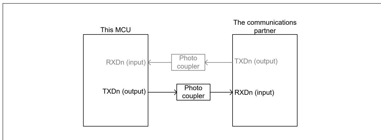
Figure 29.35 Block diagram image of a transmission through a photo coupler
