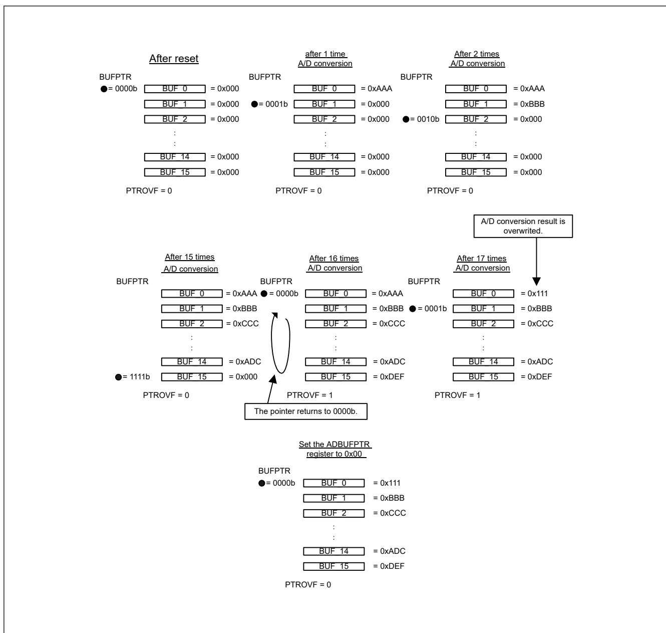
Figure 40.37 Data Buffers, Pointer, and Overflow Flag Operations
