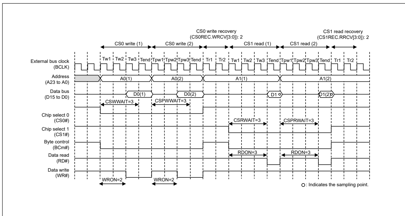
Figure 14.33 Example of recovery cycle insertion when a bus access is split with separate bus interface page access (m = 0 to 1)
