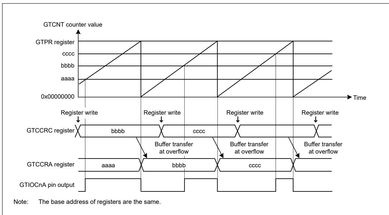
Figure 21.14 Example of GTCCRA buffer operation with output compare, saw waves in up-counting, high output at GTCCRA compare match, and low output at cycle end
