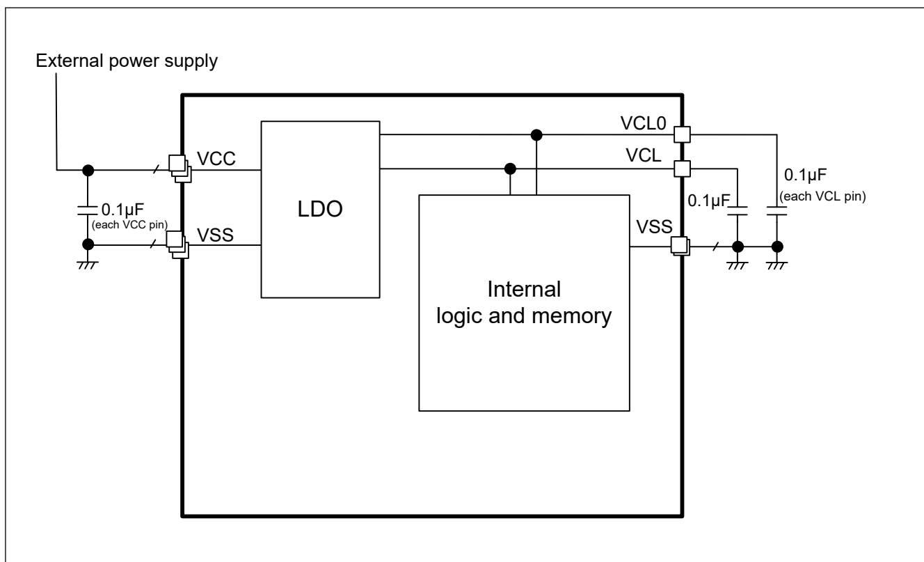
Figure 48.1 LDO mode settings
