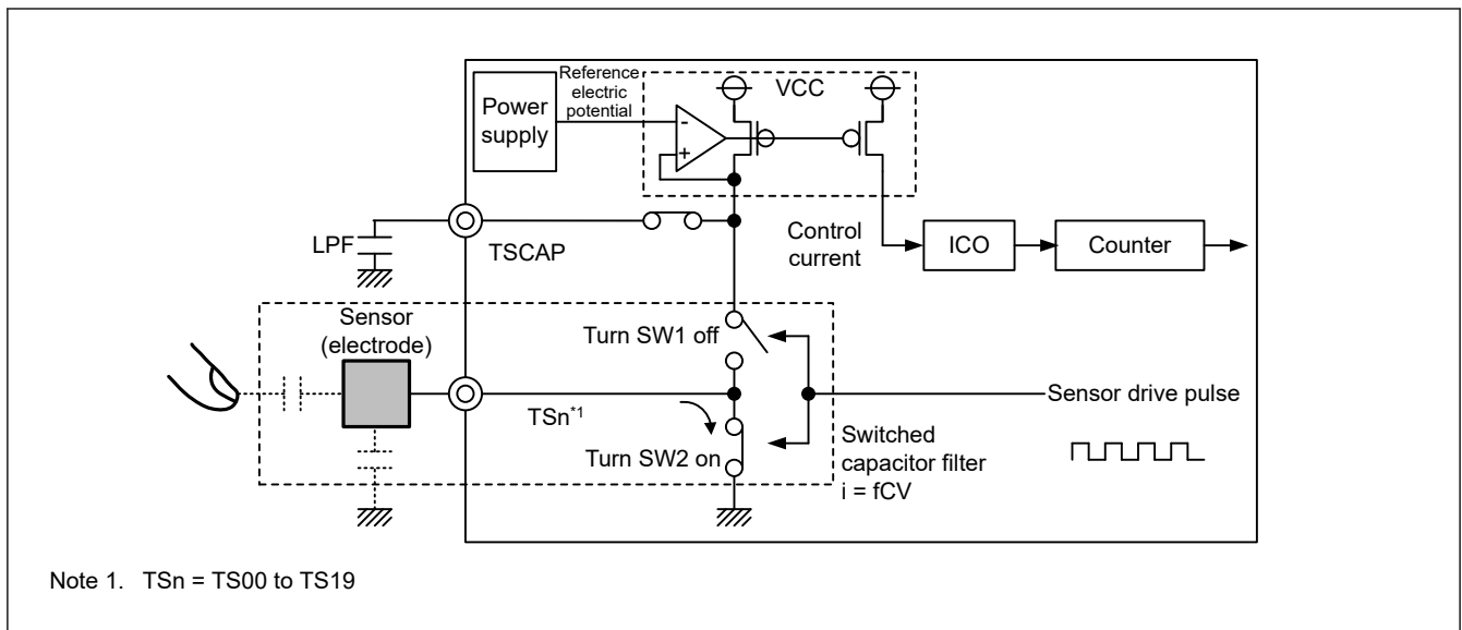
Figure 43.6 Discharging operation
