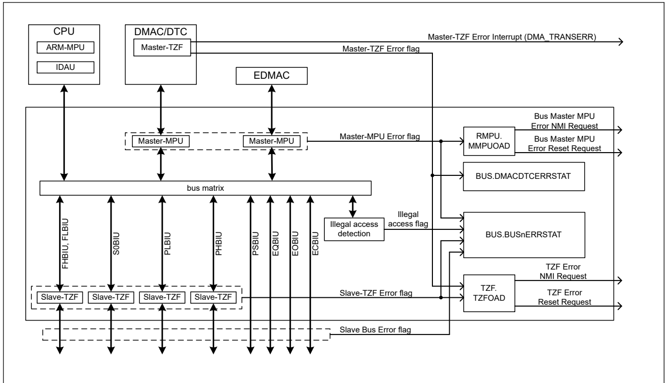
Figure 14.38 Operation from each error detection to user notification on the bus
