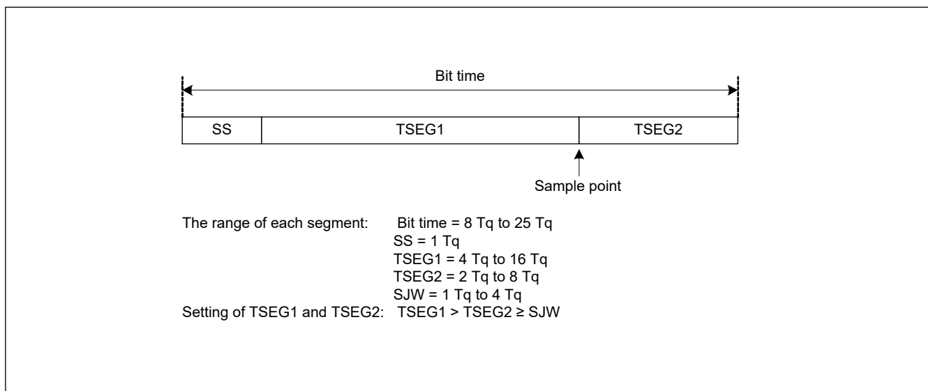
Figure 31.12 Bit timing
