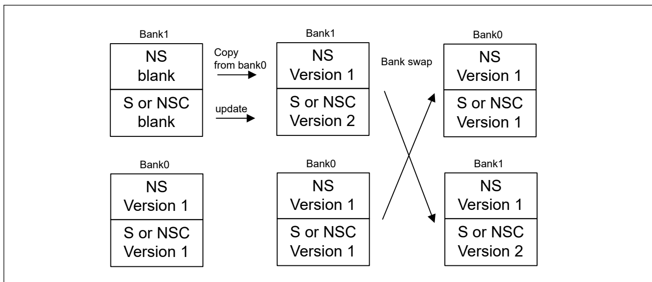
Figure 49.4 Field updating flow of secure or non-secure callable region
