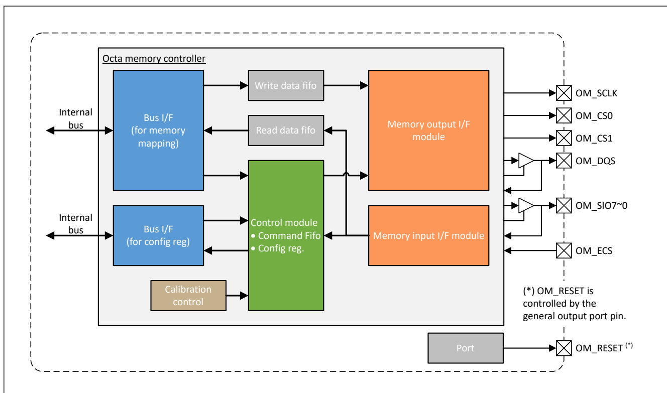
Figure 34.1 Block diagram
