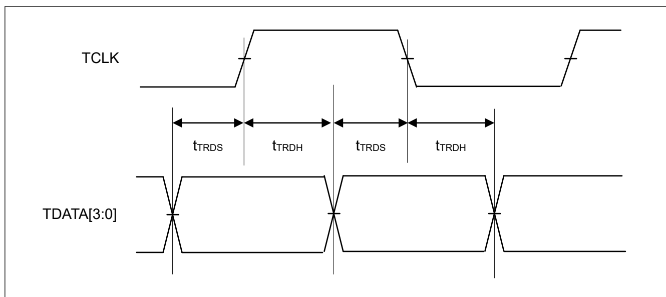
Figure 50.96 ETM output timing
