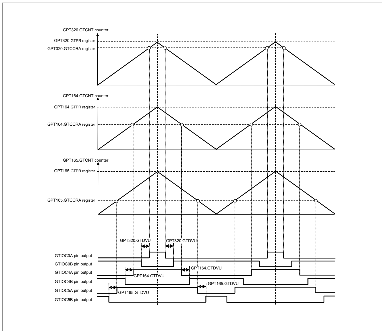
Figure 21.43 Example of a 3-phase triangle-wave complementary PWM output with automatic dead time setting
