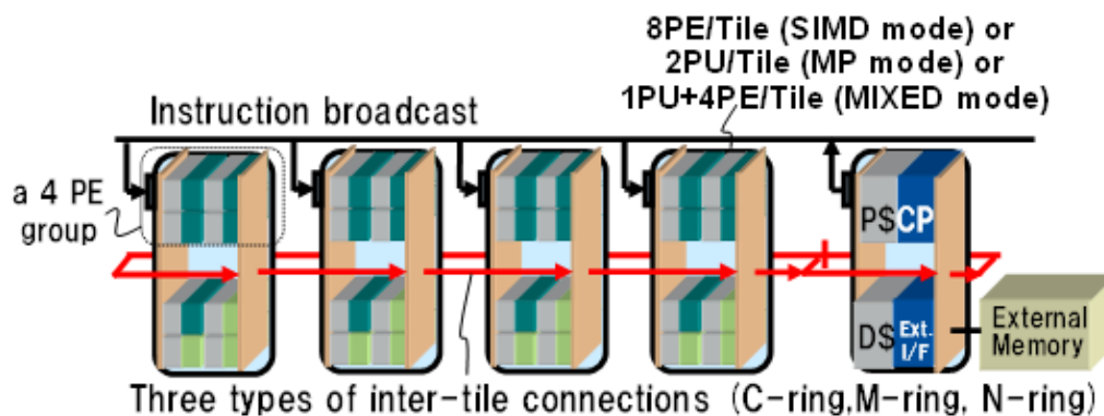
Figure 6 Example Physical Configuration of IMAP System (for XC Core)
