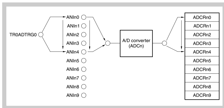
Figure 14-11 Example of Scan Mode Operation (Timer Trigger Scan) (ANIn0 to ANIn4)
