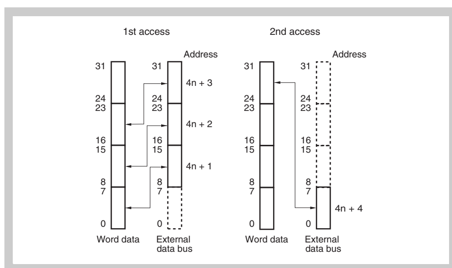
Figure 4-39 Word access to 32-bit data bus at address 4n+1 (little endian)
