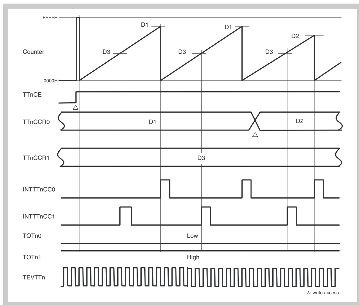
Figure 11-9 Basic operation timing in external event count mode (1/3) When D1 > D2 > D3 , only value of TnCCR0 register is rewritten, TOTn0 and TOTn1 are not output. The signal input from TEVTTn and internally synchronized is counted as the count clock (TnOE0, 1 = 0, TnOL0 = 0, TnOL1 = 1)
