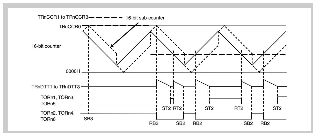
Figure 10-94 Timer output change after compare register updating by peak reload when “TRnCCR1 to TRnCCR3 = TRnCCR0” → “(TRnDTC0 + TRnDTC1) < TRnCCR1 to TRnCCR3 < (TRnCCR0 – TRnDTC1 × 2)”
