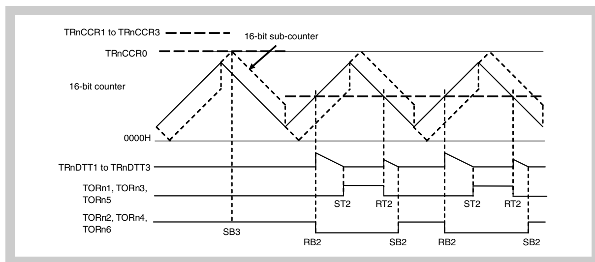
Figure 10-88 Timer output change after compare register updating by trough reload when “TRnCCR1 to TRnCCR3 = TRnCCR0” → “(TRnDTC0 + TRnDTC1) < TRnCCR1 to TRnCCR3 < (TRnCCR0 – TRnDTC1 – TRnDTC0)”
