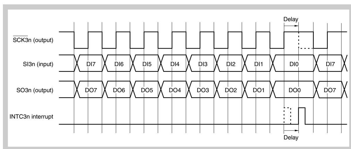
Figure 17-12 Delay Control of Transmission/Reception Completion Interrupt (INTC3n)
