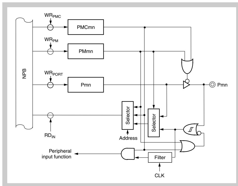
Figure 20-16 Port Type 10
