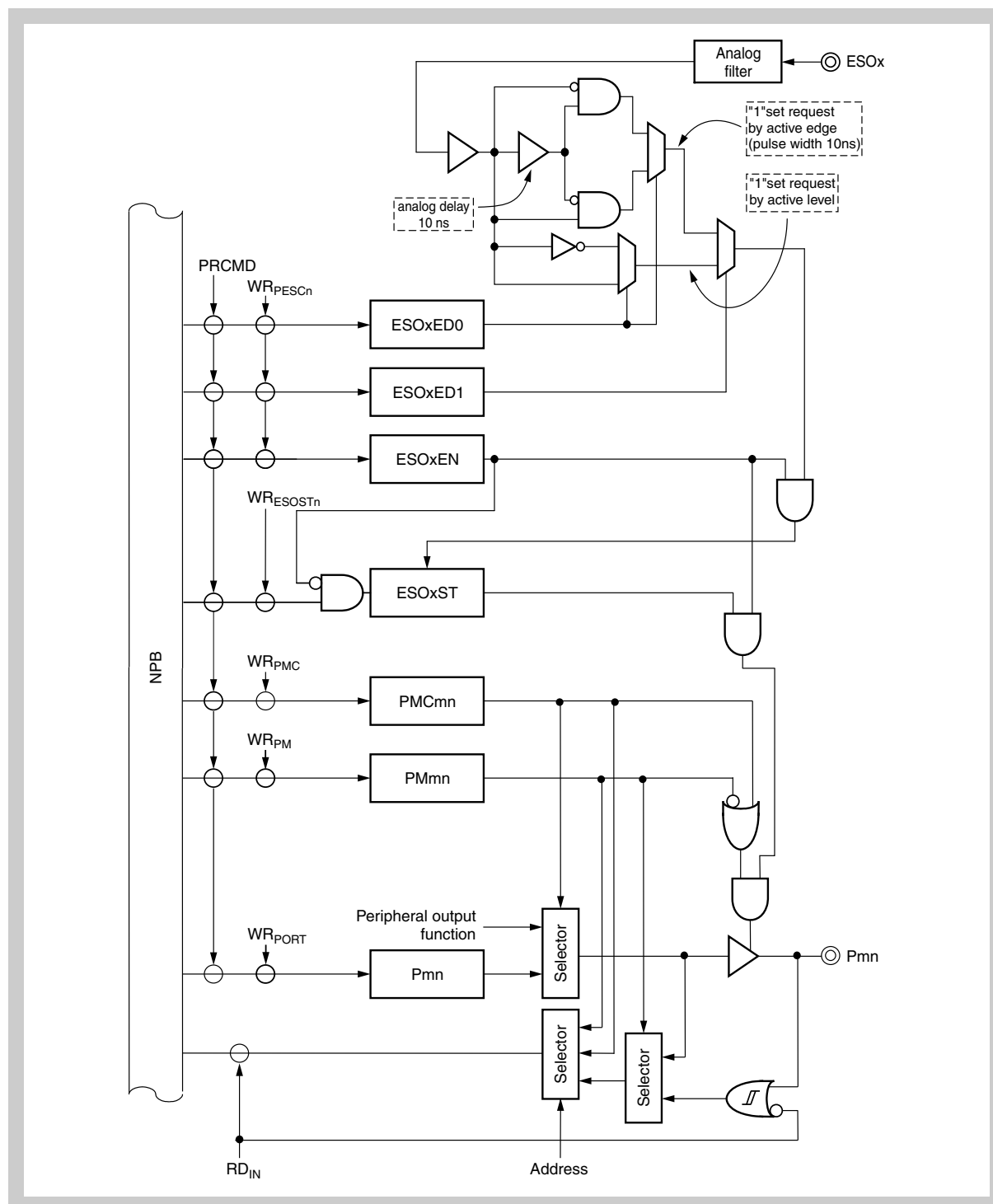
Figure 20-19 Port Type 13
