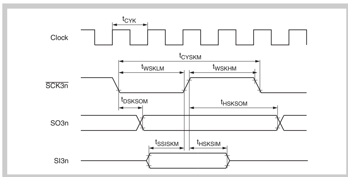
Figure 25-15 CSI3 timing in master mode (CKP, DAP bits = 00 B or 11 B )
