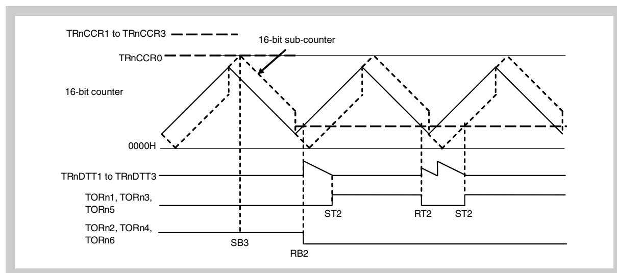
Figure 10-87 Timer output change after compare register updating by trough reload when “TRnCCR1 to TRnCCR3 = TRnCCR0” → “(TRnDTC0 + 1) < TRnCCR1 to TRnCCR3 ≤ (TRnDTC0 + TRnDTC1)”
