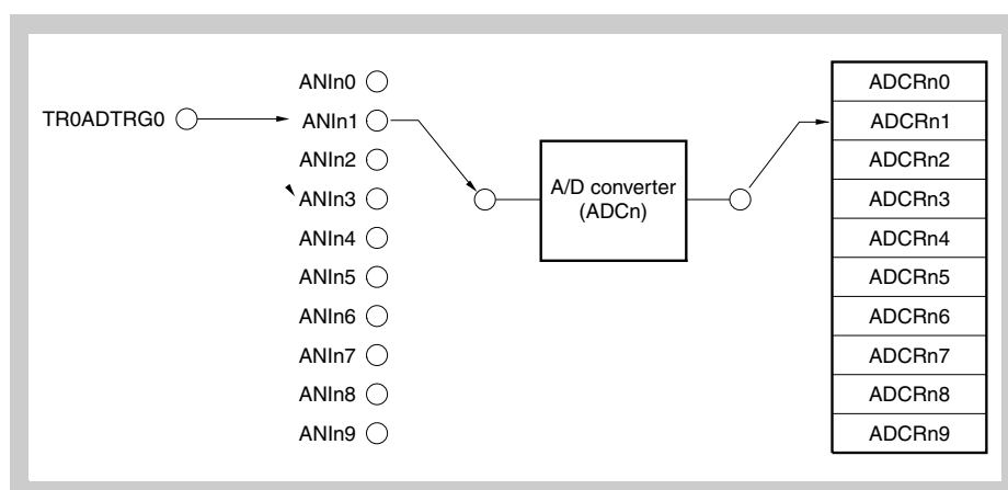
Figure 14-9 Example of 1-Buffer Mode Operation (Timer Trigger Select: 1 Buffer) (ANIn1)
