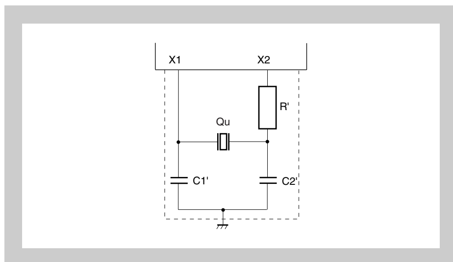
Figure 25-1 Oscillator recommendations
