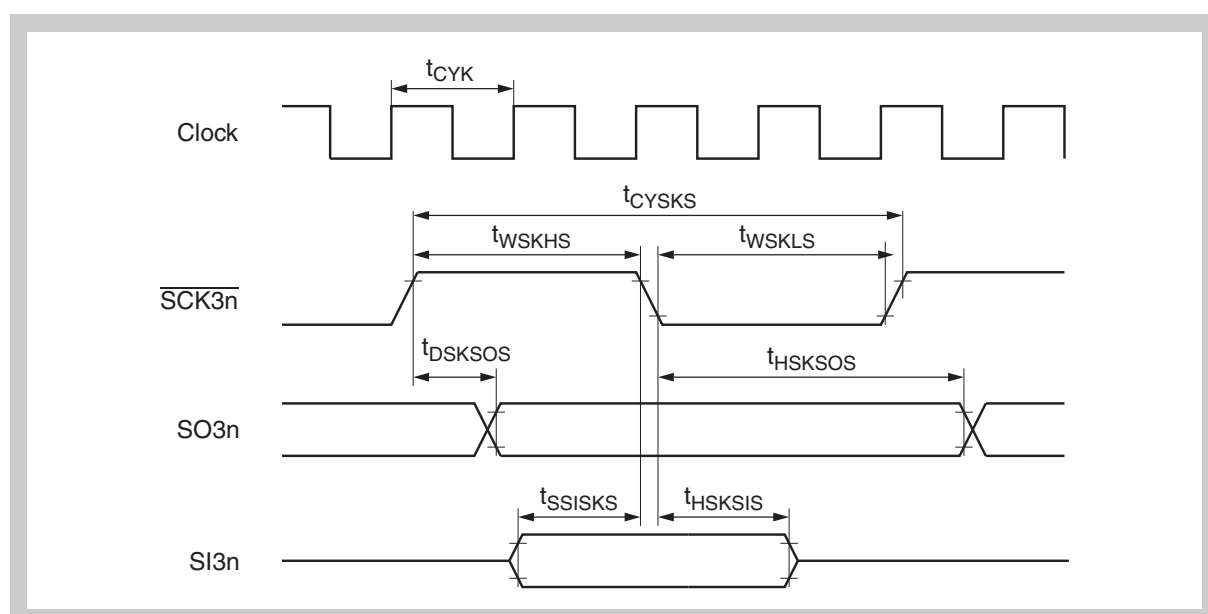
Figure 25-18 CSI3 timing in slave mode (CKP, DAP bits = 01 B or 10 B )
