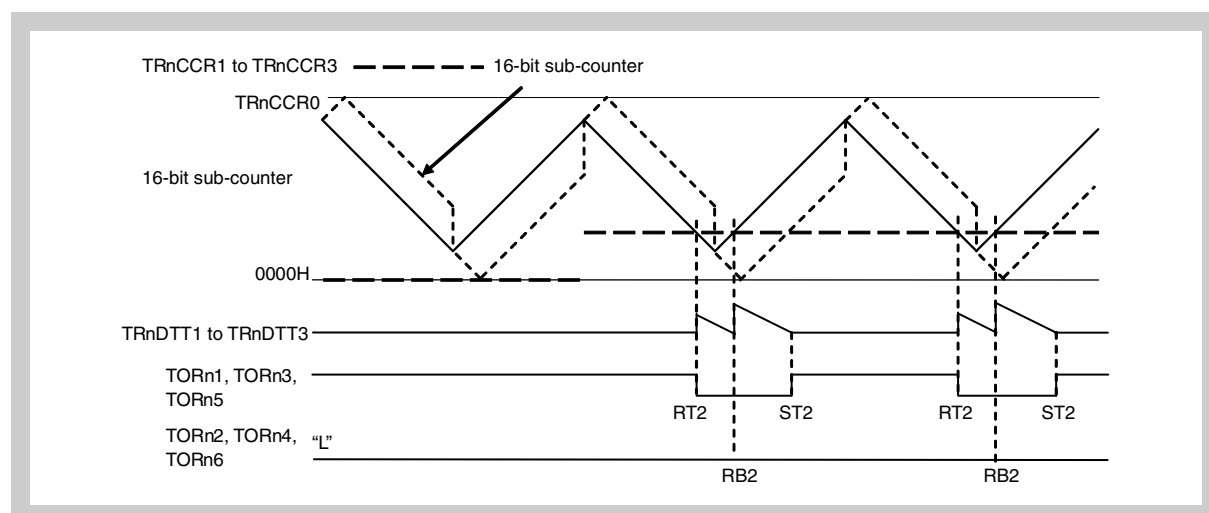
Figure 10-103 Timer output change after compare register updating by peak reload when “TRnCCR1 to TRnCCR3 = 0000 H ” → “(TRnDTC0 + 1) < TRnCCR1 to TRnCCR3 < (TRnDTC0 + TRnDTC1)”
