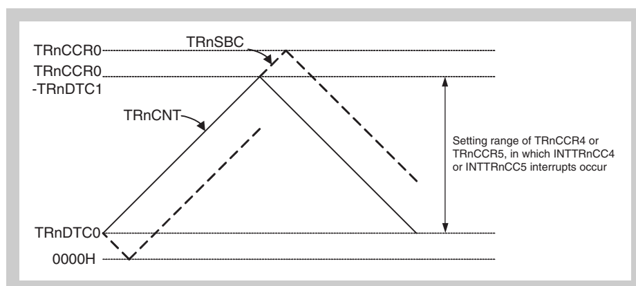
Figure 10-23 Compare match interrupt occurrence related to TRnCCR4 and TRnCCR5 in high-accuracy T-PWM mode
