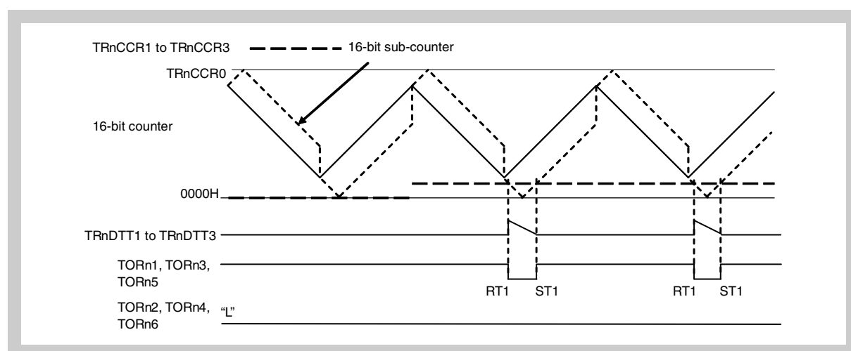
Figure 10-104 Timer output change after compare register updating by peak reload when “TRnCCR1 to TRnCCR3 = 0000 H ” → “0000 H < TRnCCR1 to TRnCCR3 ≤ (TRnDTC0 + 1)”
