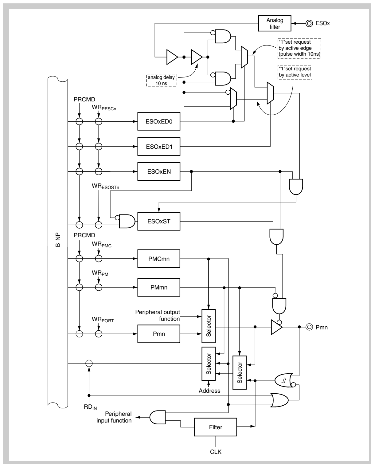
Figure 20-20 Port Type 14
