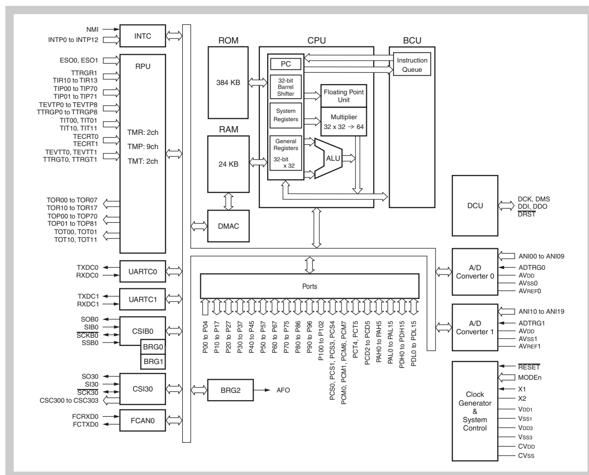
Figure 1-3 Internal Block Diagram of \mu PD70F3447
