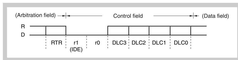
Figure 18-8 Control field
