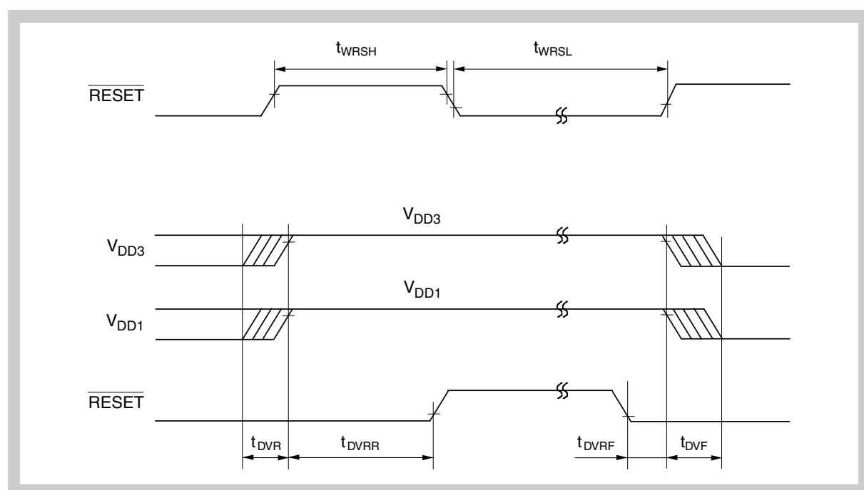
Figure 25-6 Reset Timing
