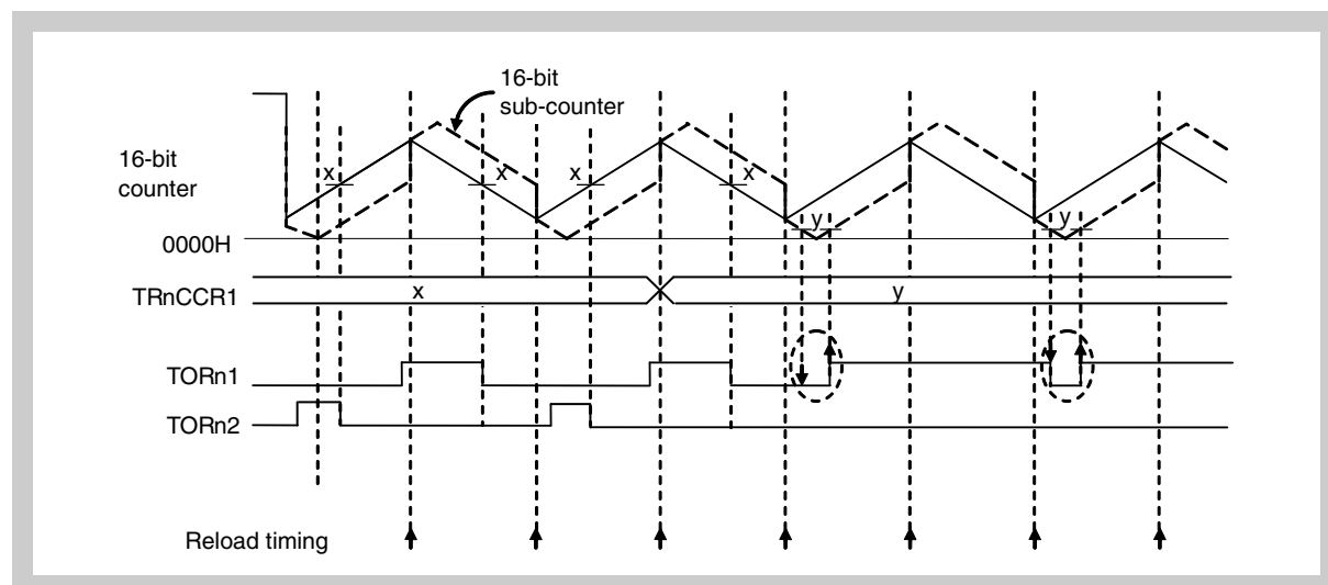
Figure 10-75 Timing of timer output in high-accuracy T-PWM mode when rewriting from “ (TRnDTC0 + TRnDTC1) < TRnCCR1 < (TRnCCR0 - TRnDTC0 - TRnDTC1) ” to “ TRnCCR1 < (TRnDTC0 + TRnDTC1) ”
