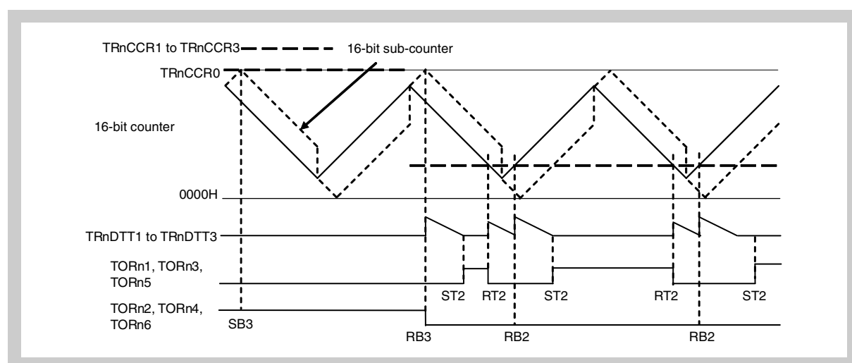
Figure 10-95 Timer output change after compare register updating by peak reload when “TRnCCR1 to TRnCCR3 = TRnCCR0” → “(TRnDTC0 + 1) < TRnCCR1 to TRnCCR3 ≤ (TRnDTC0 + TRnDTC1)”
