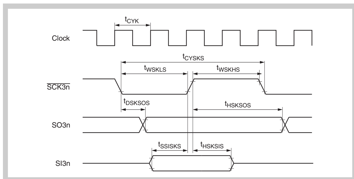
Figure 25-17 CSI3 timing in slave mode (CKP, DAP bits = 00 B or 11 B )
