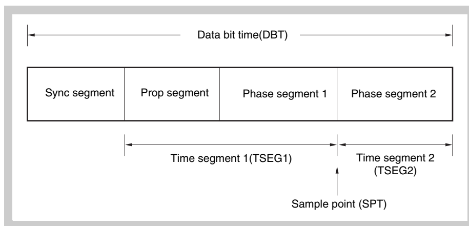
Figure 18-18 Segment setting
