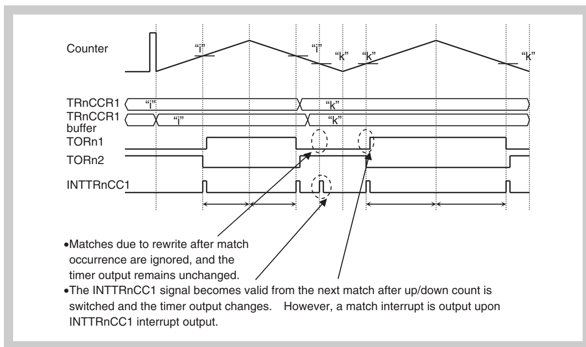
Figure 10-10 Anytime rewrite timing in <4> interval (rewrite after match occurrence)
