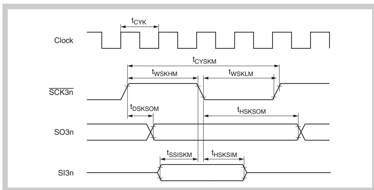
Figure 25-16 CSI3 timing in master mode (CKP, DAP bits = 01 B or 10 B )
