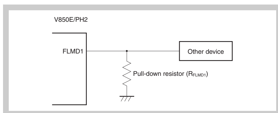
Figure 24-12 FLMD1 pin connection example
