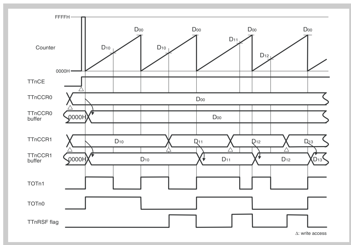
Figure 11-18 Basic operation timing in PWM mode (1/2) when only value of TTnCCR1 is rewritten, and TOTn0 and TOTn1 are output (TTnOE0, 1 = 1, TTnOL0, 1 = 0)
