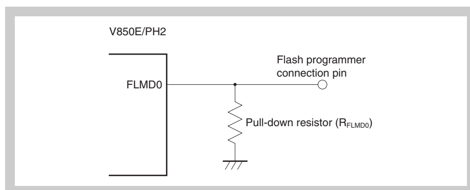
Figure 24-11 FLMD0 pin connection example
