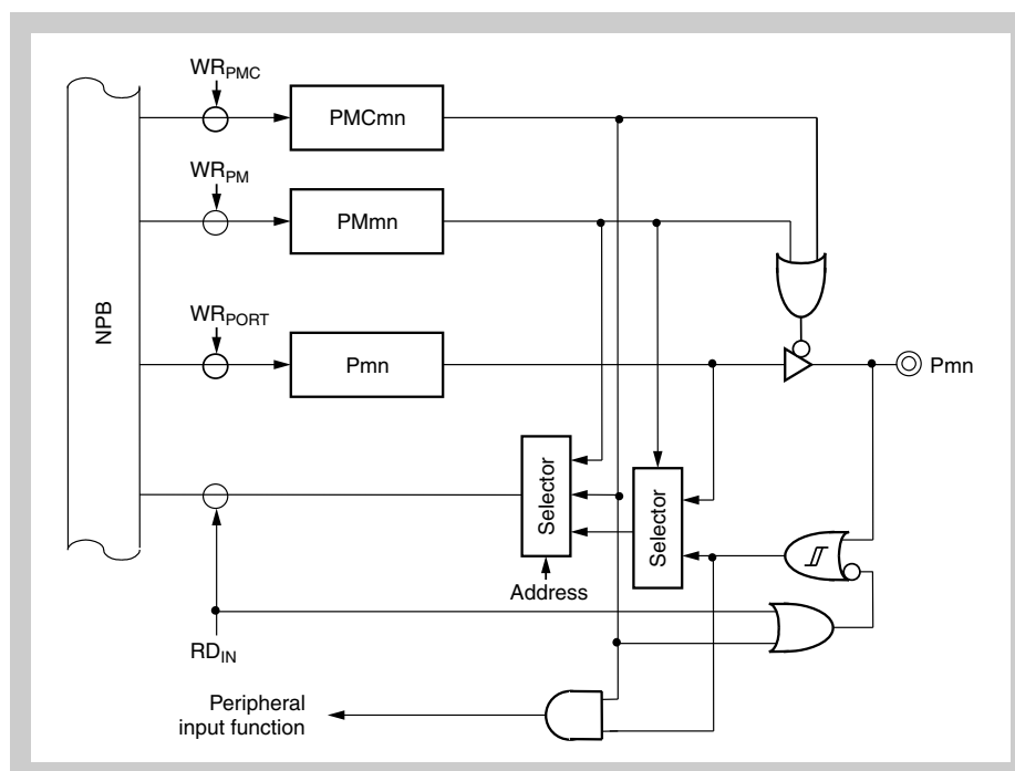
Figure 20-5 Port Type 2
