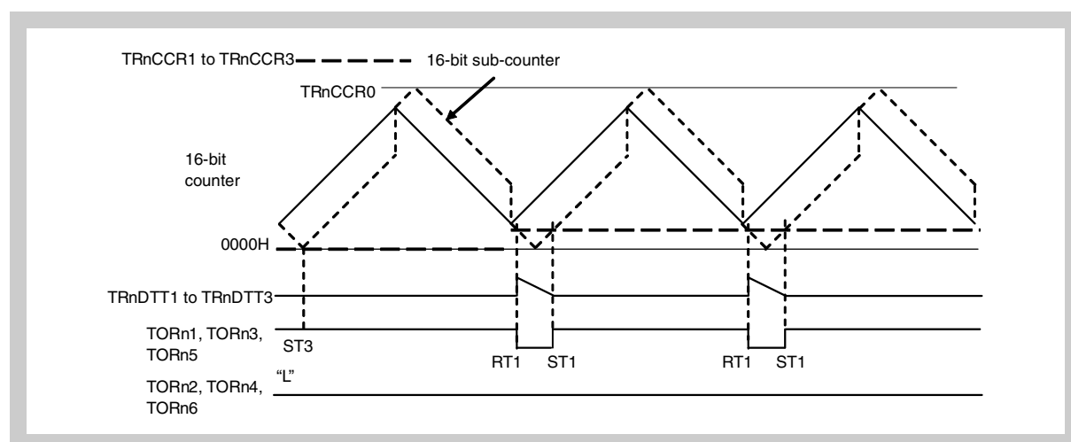
Figure 10-77 Timer output change after compare register updating by trough reload when “TRnCCR1 to TRnCCR3 = 0000 H ” → “0000 H < TRnCCR1 to TRnCCR3 < TRnDTC0”
