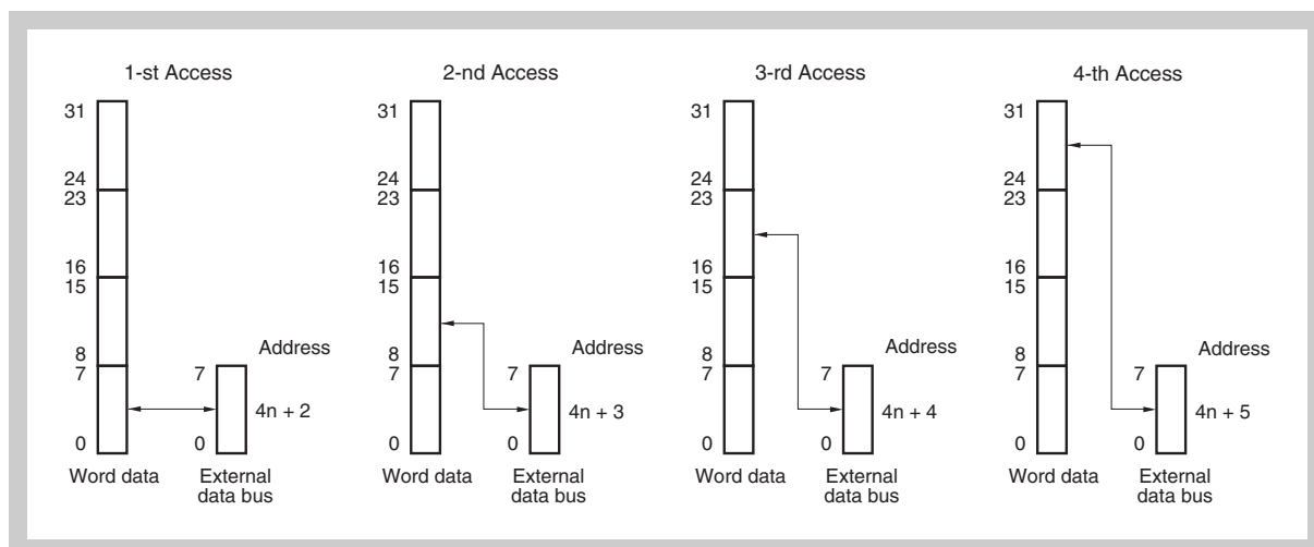
Figure 4-10 Word access to 8-bit data bus at address 4n+2 (little endian)
