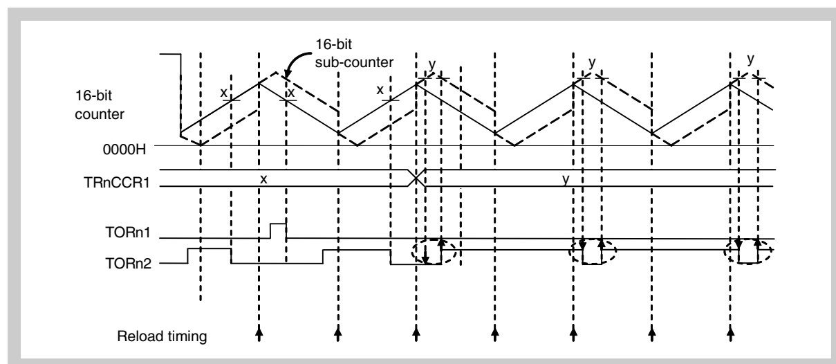
Figure 10-76 Timing of timer output in high-accuracy T-PWM mode when rewriting from “ (\text{TRnDTC0} + \text{TRnDTC1}) < \text{TRnCCR1} < (\text{TRnCCR0} - \text{TRnDTC0} - \text{TRnDTC1}) ” to “ (\text{TRnCCR0} - \text{TRnDTC1} + 1) < \text{TRnCCR1} < \text{TRnCCR0} ”
