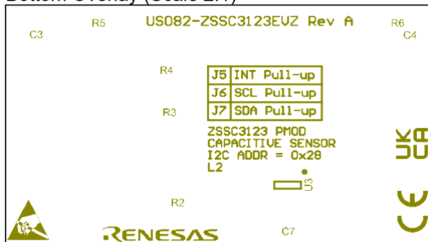
Figure 12. Bottom Overlay
