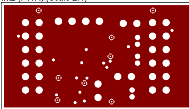
Figure 10. Layer 3 (Signal)
