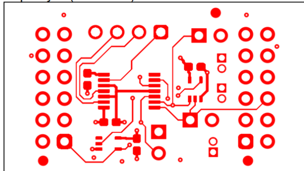
Figure 8. Top Layer
