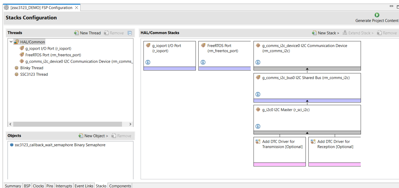
Figure 14. FSP Stacks
