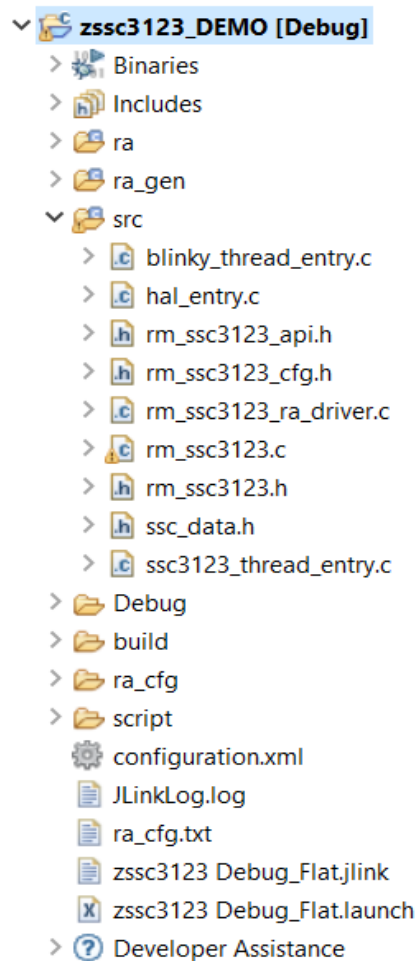
Figure 13. Project Structure
