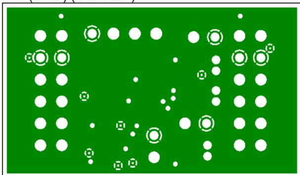
Figure 9. Layer 2 (GND)
