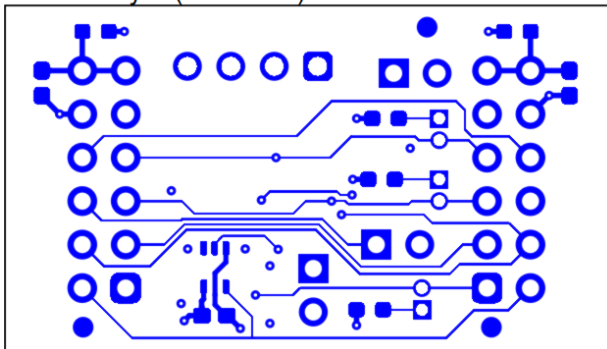
Figure 11. Bottom Layer
