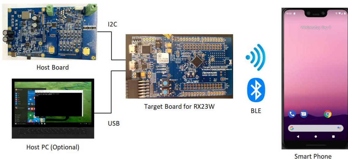
Figure 12-1: Bluetooth System makeup
