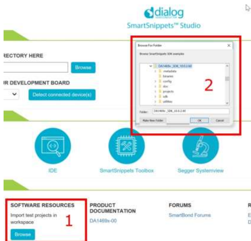
Figure 37: Project import
