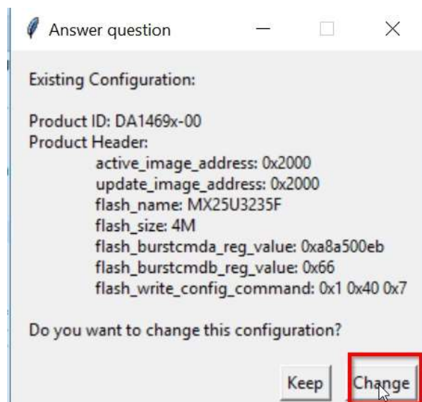
Figure 43: Configuration Summary
