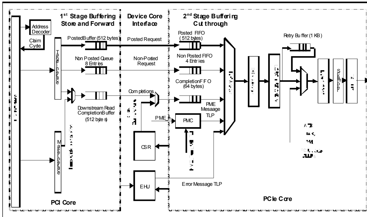
Figure 5: Upstream Data Path
