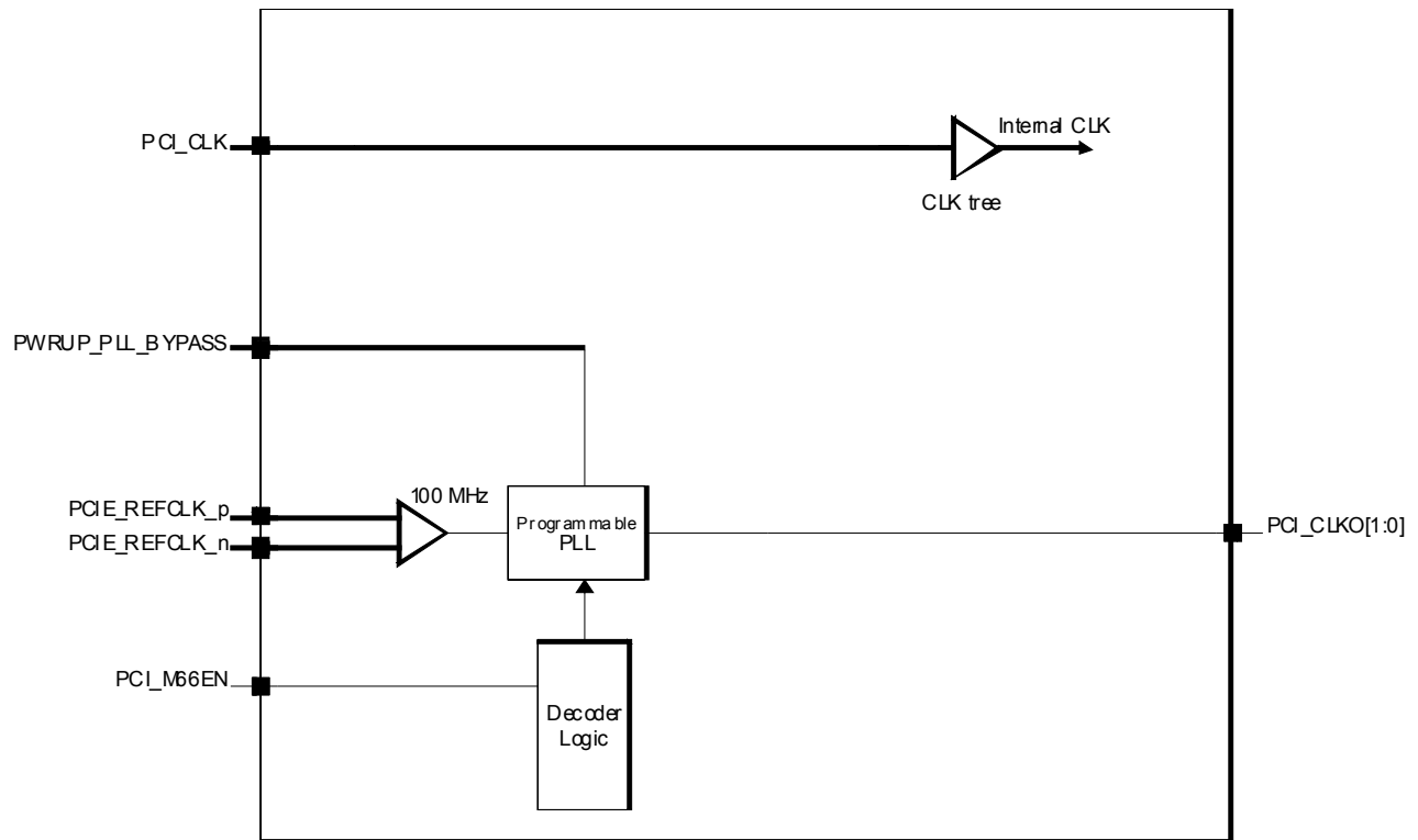
Figure 25: PCI Clocking
