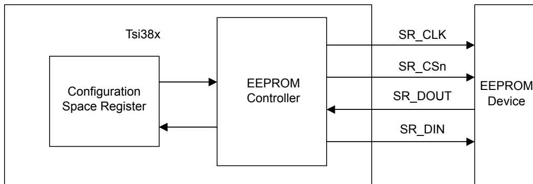
Figure 28: EEPROM Interface
