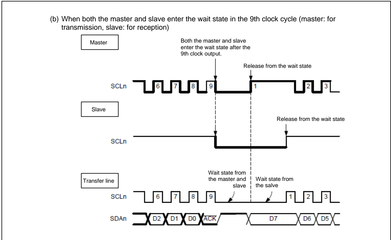
Figure 37.6-7 Wait (2/2)
