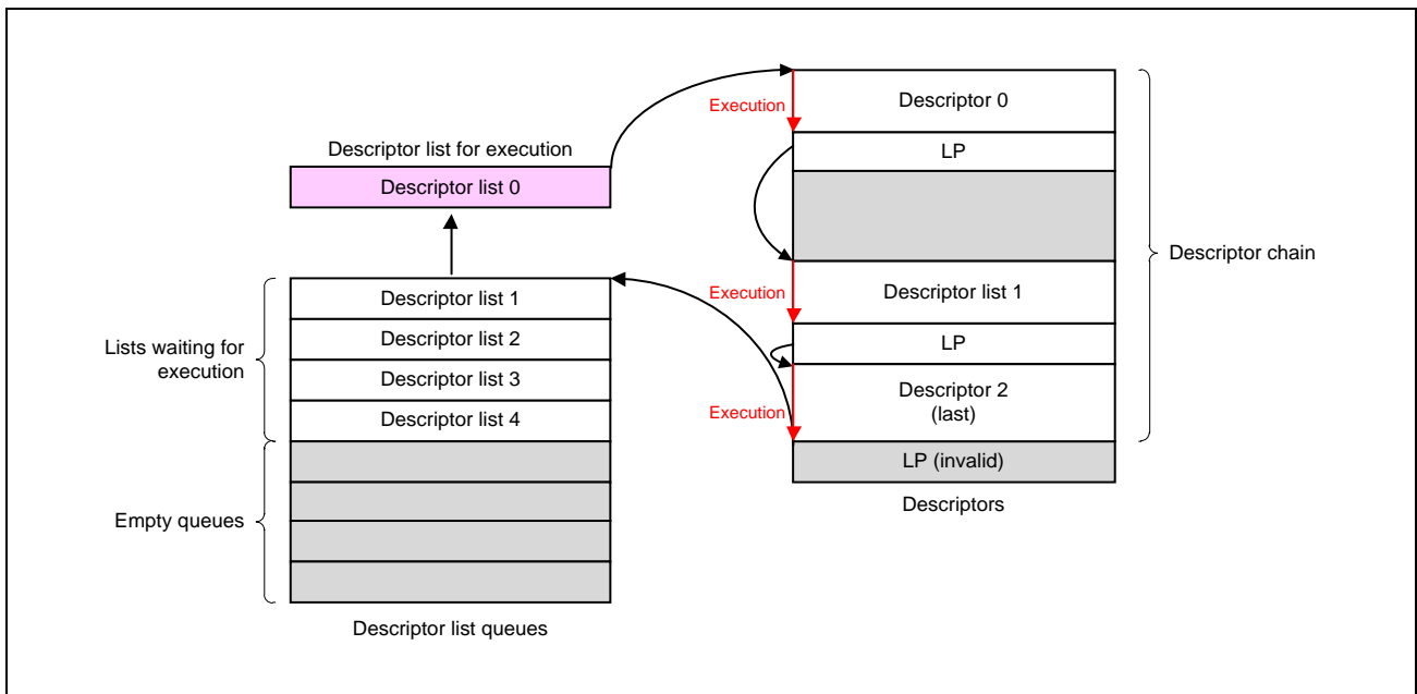
Figure 35.7-1 Descriptor Chain
