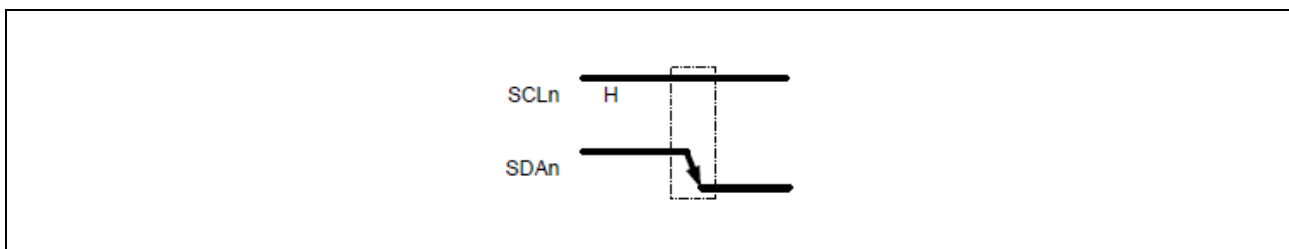
Figure 37.6-2 Start Condition
