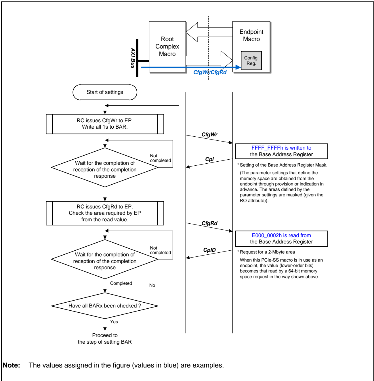
Figure 35.8-3 Example Settings for the PCIe Address Space
