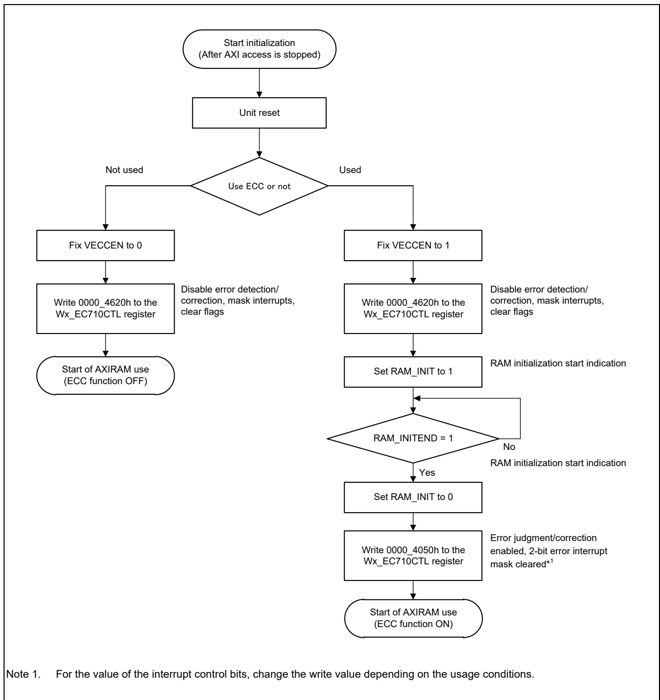
Figure 12.5-5 Initialization Flow by H/W
