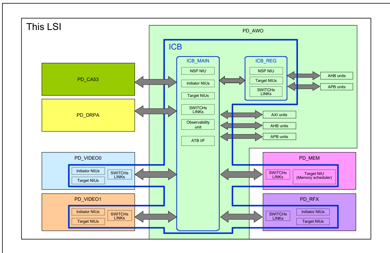
Figure 46.2-1 Internal Configuration
