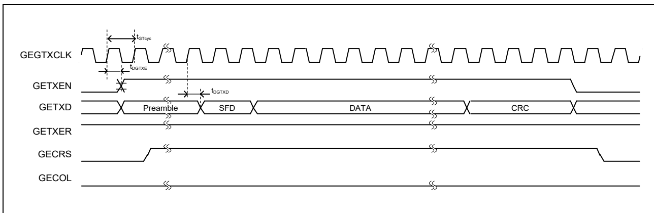
Figure 51.5-7 Transmission Timing
