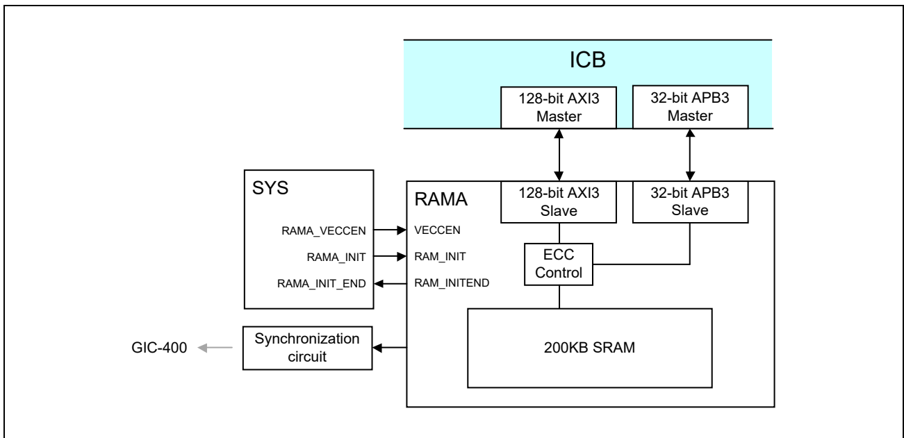
Figure 12.1-1 Connection Diagram
