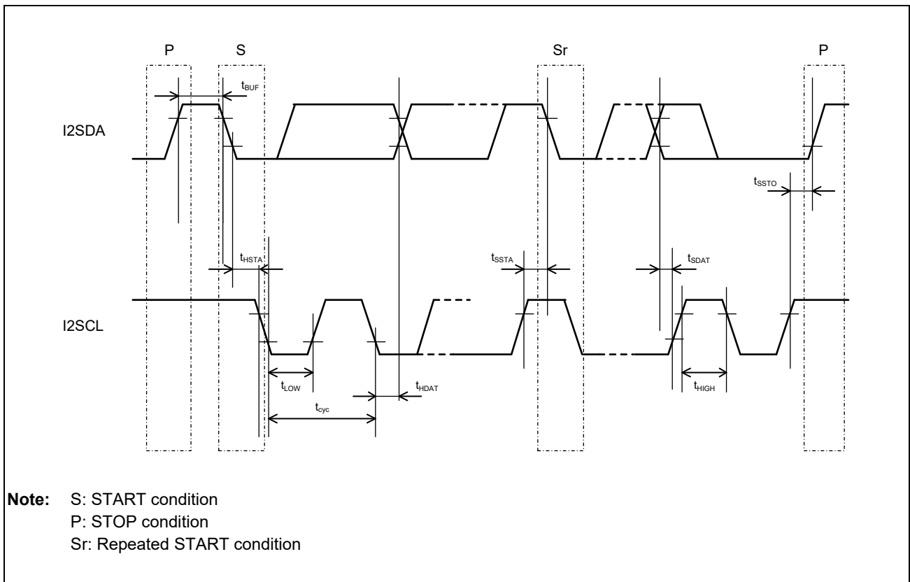
Figure 51.5-1 IIC Timing
