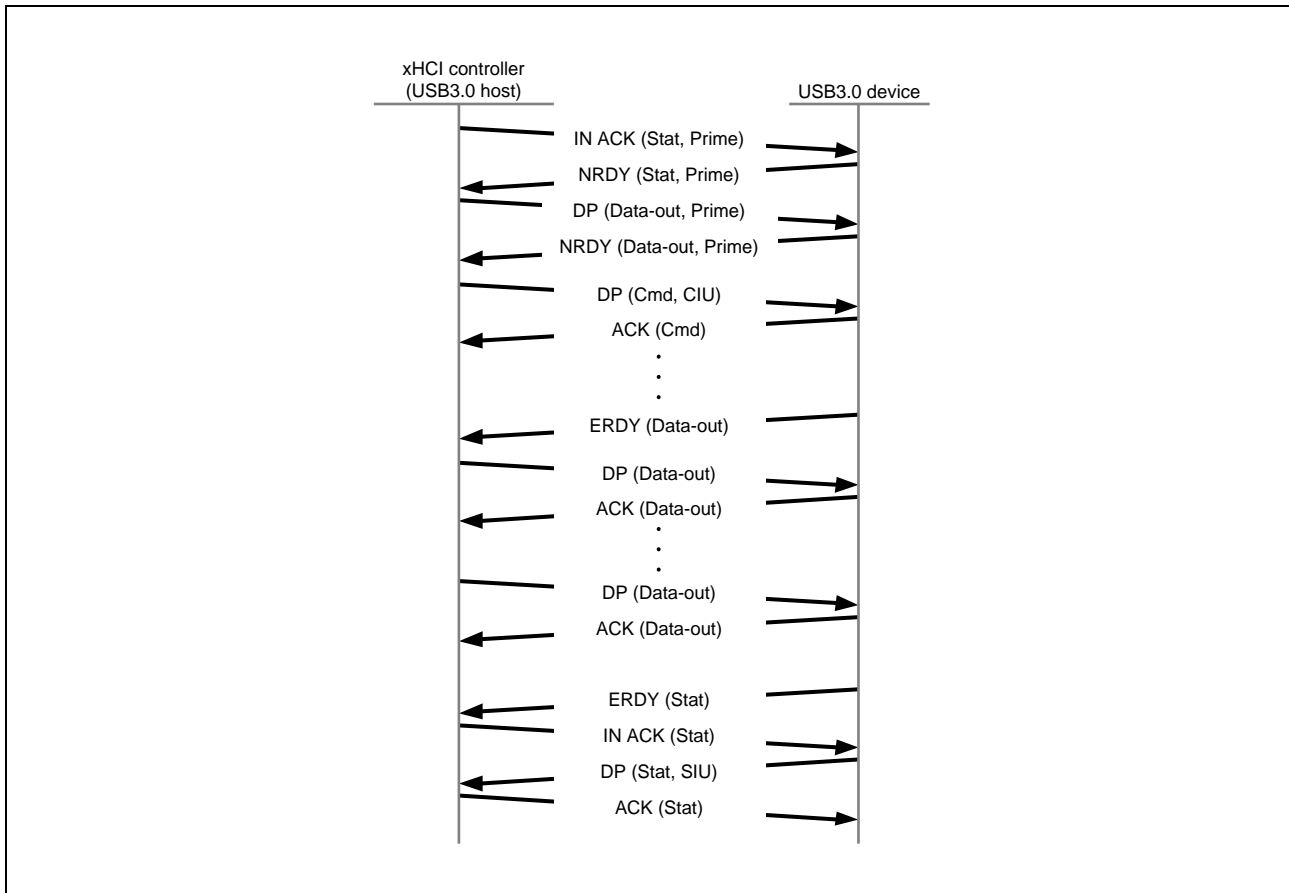
Figure 34.6-36 Example SuperSpeed UASP Data-OUT Transfer
