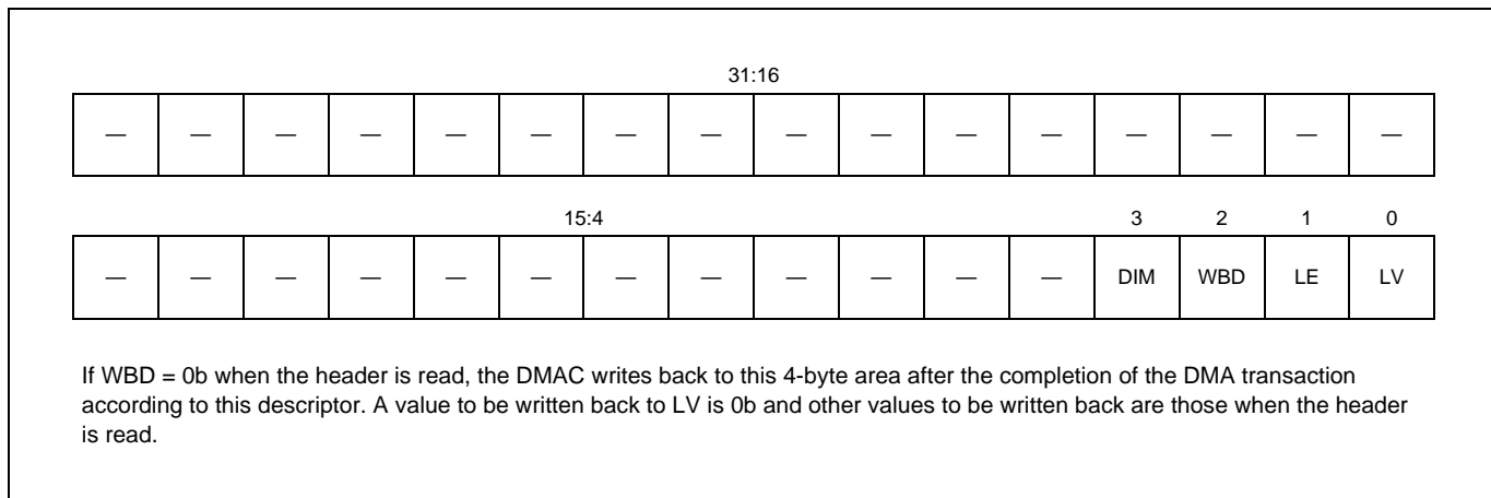
Figure 19.6-7 Header Area
