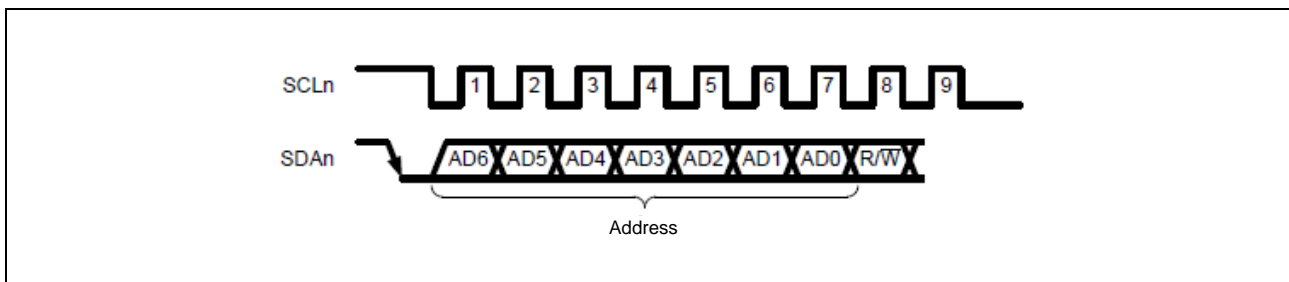
Figure 37.6-3 Address
