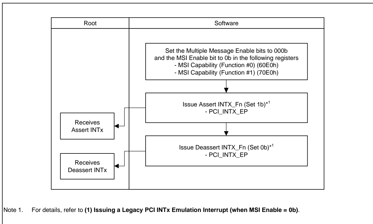
Figure 35.7-3 Legacy Interrupt Issuing Flow
