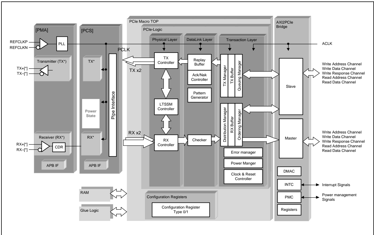
Figure 35.3-1 Block Diagram
