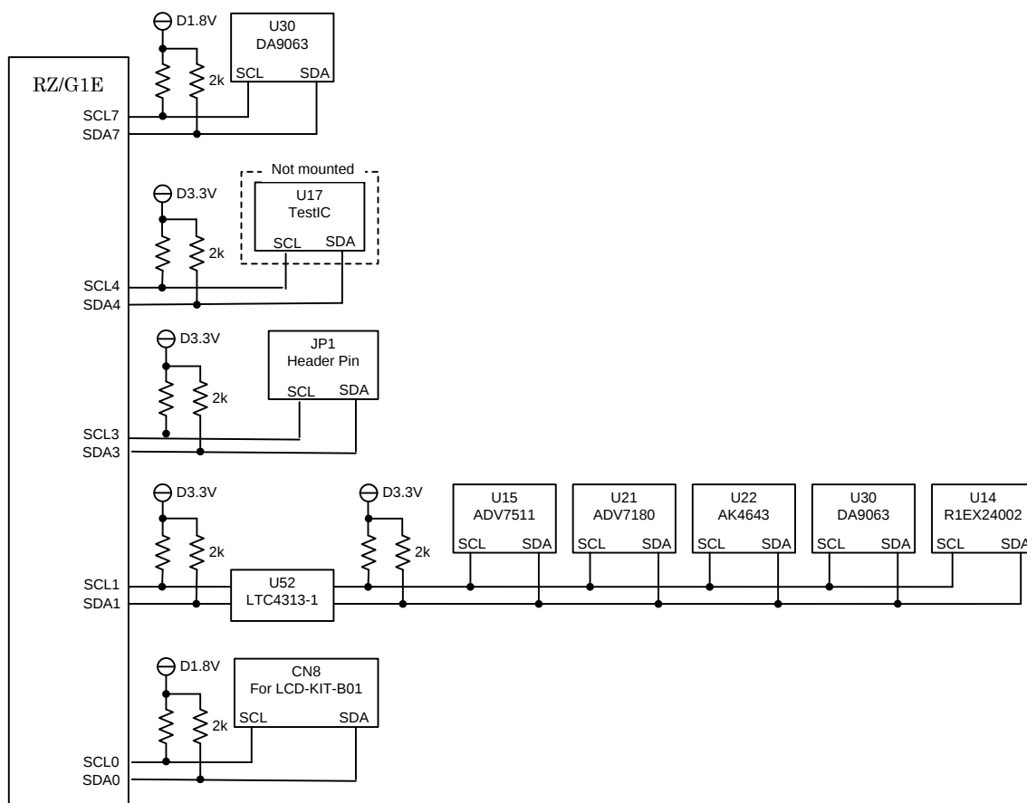
Figure 2.14.1 Block Diagram of I²C Interface
