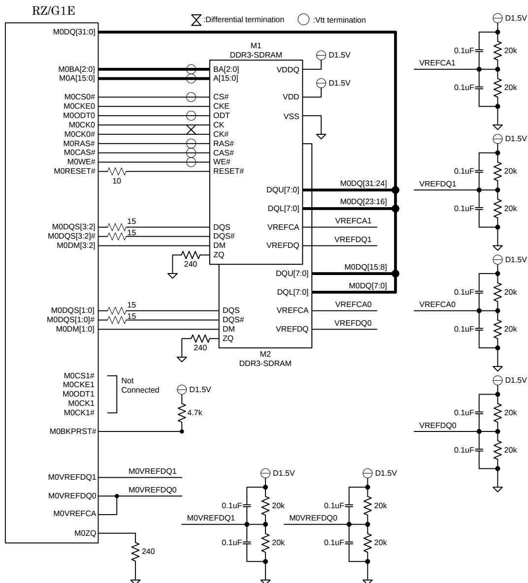
Figure 2.2.1 Block Diagram of DDR3-SDRAM Interface
