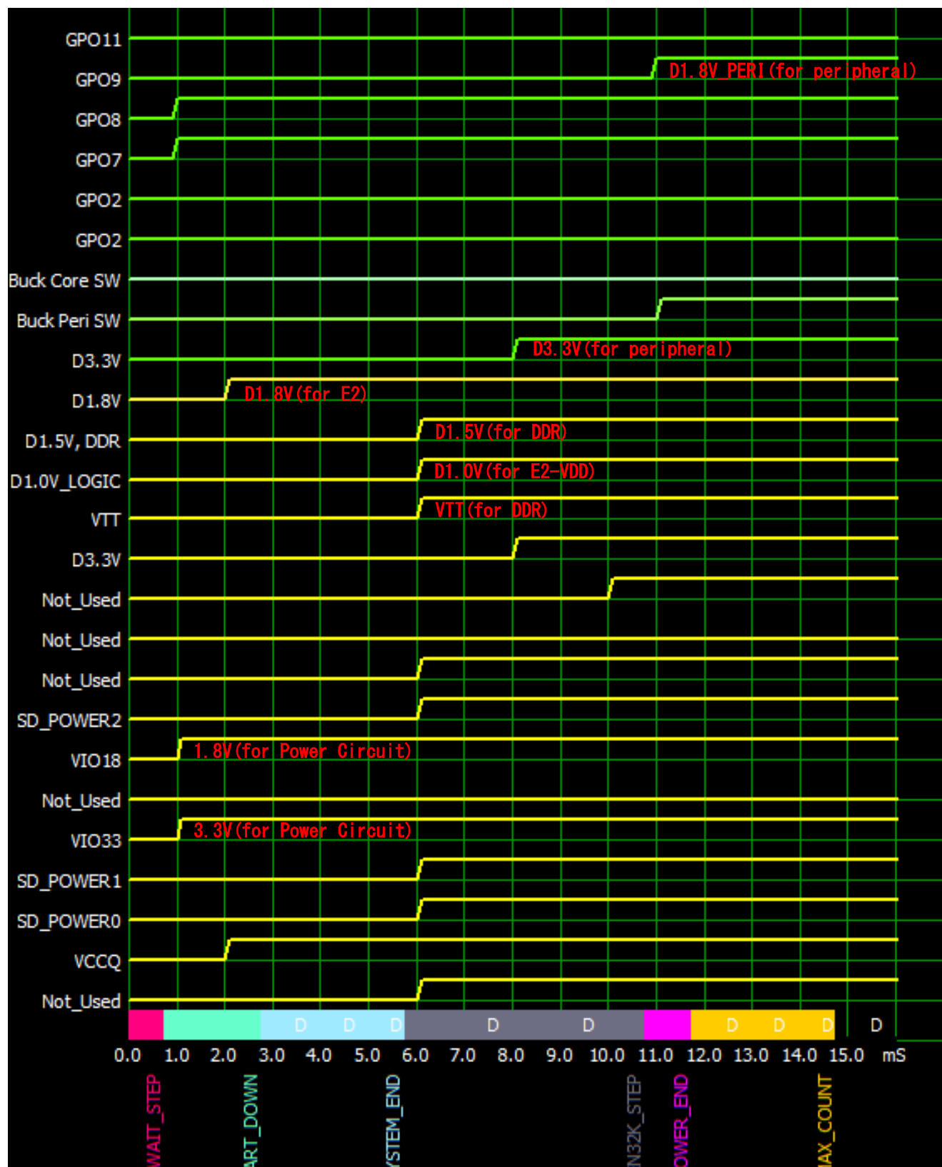
Figure 2.18.2 Power-On Sequence
