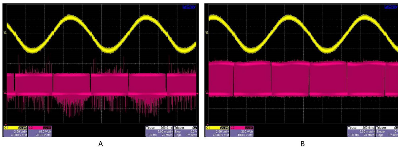
Figure 10. Waveform of Active Switch Version of the Bridgeless Totem-Pole PFC at High-Line, 3.5kW at High-Line CH1: input current Iin (2A/div); CH2: (A) Vgs of Q2 (10V/div), (B) Vds of Q2 (200V/div)
