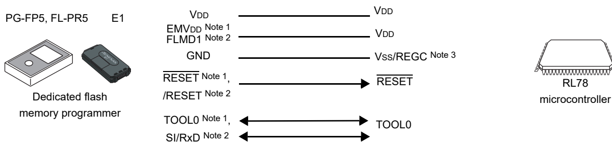
Figure 30 - 2 Communication with Dedicated Flash Memory Programmer
