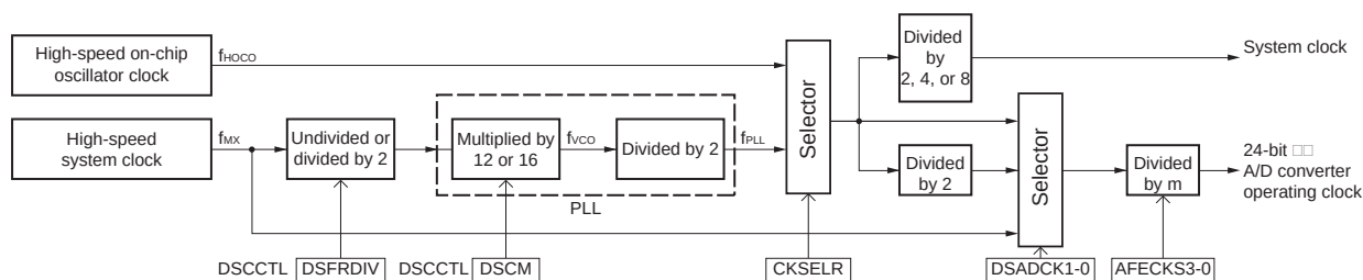
Figure 5 - 13 Relationship Between PLL and \Delta\Sigma A/D Converter
