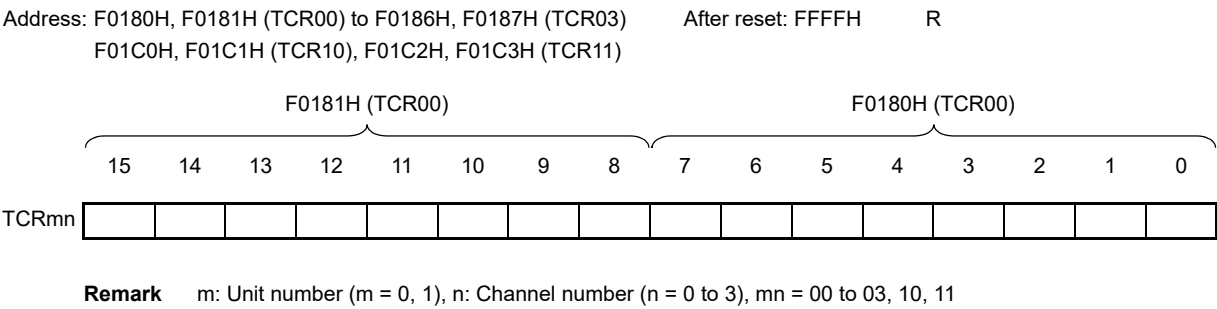
Figure 6 - 9 Format of Timer counter register mn (TCRmn)
