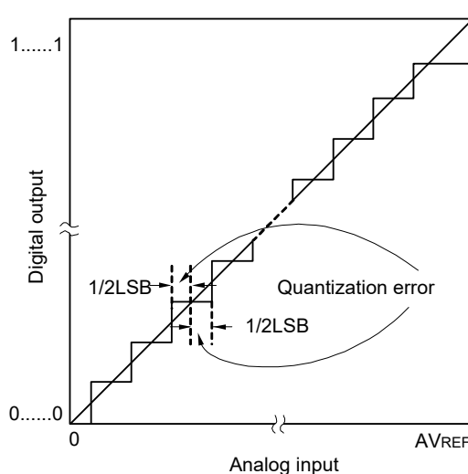
Figure 16 - 41 Quantization Error
