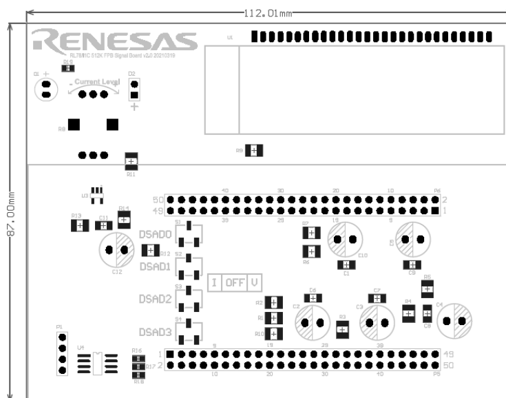
Figure 4: Part Layout
