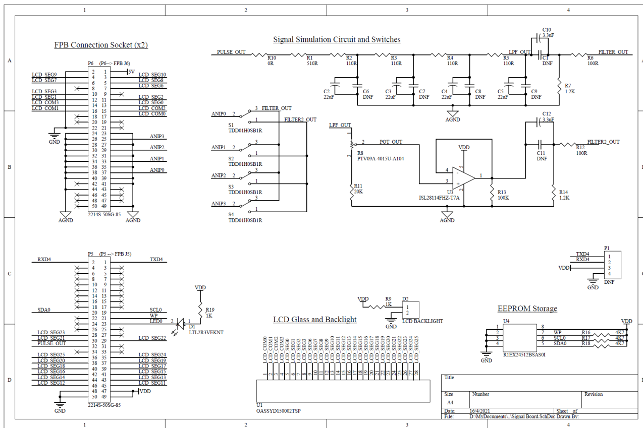
Figure 3: Schematic
