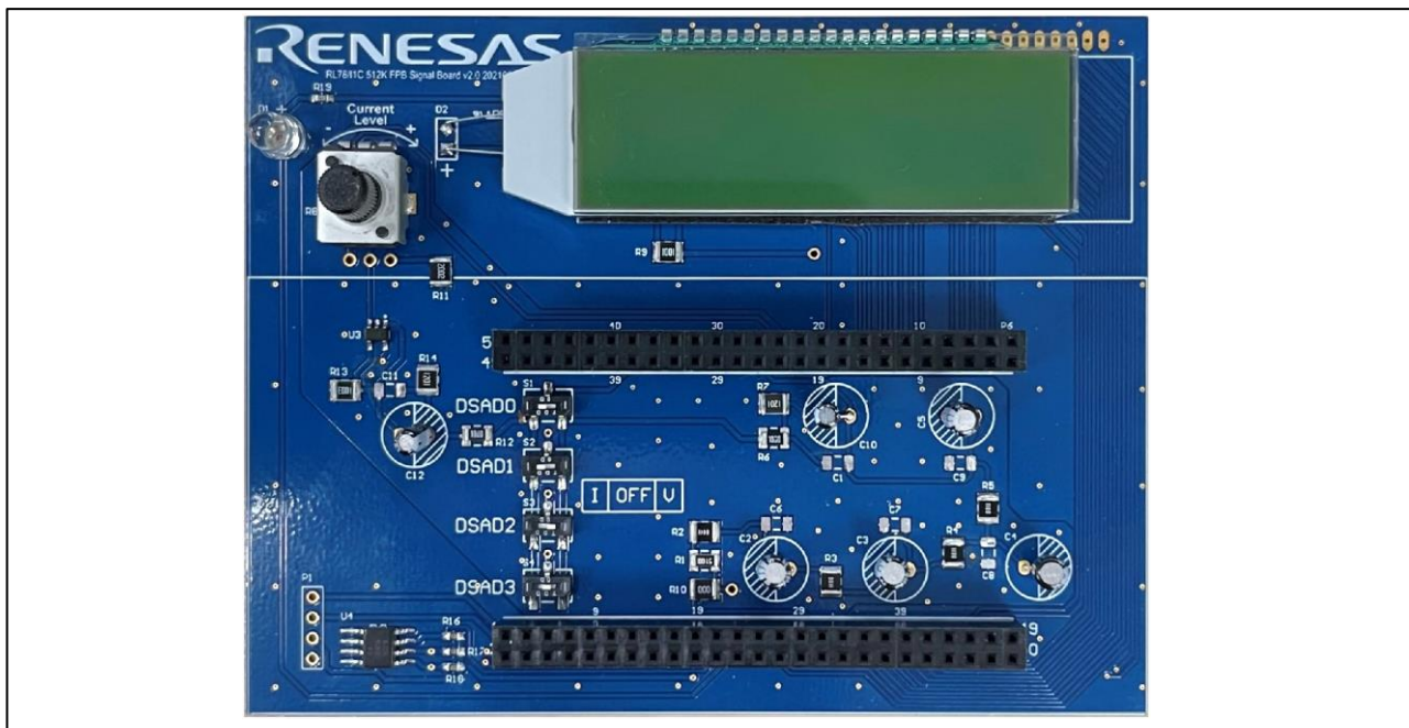
Figure 1: RL78/I1C(512KB) FPB Signal Board
