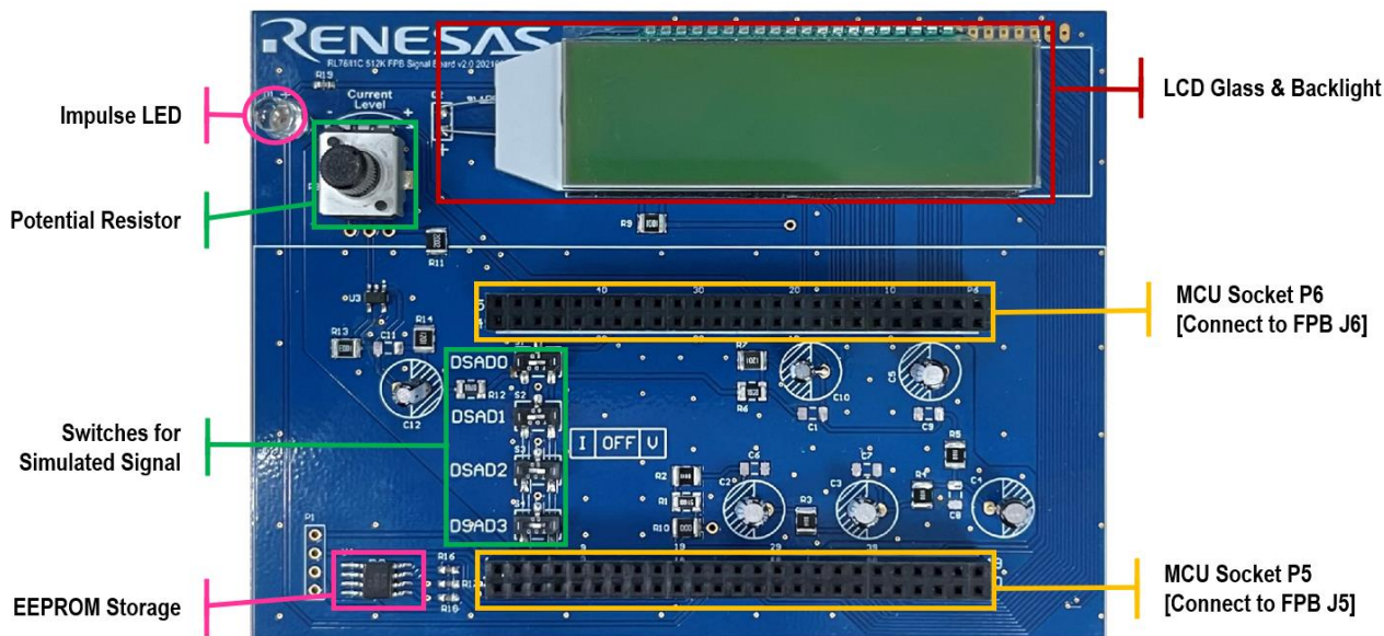
Figure 5: Board Layout
