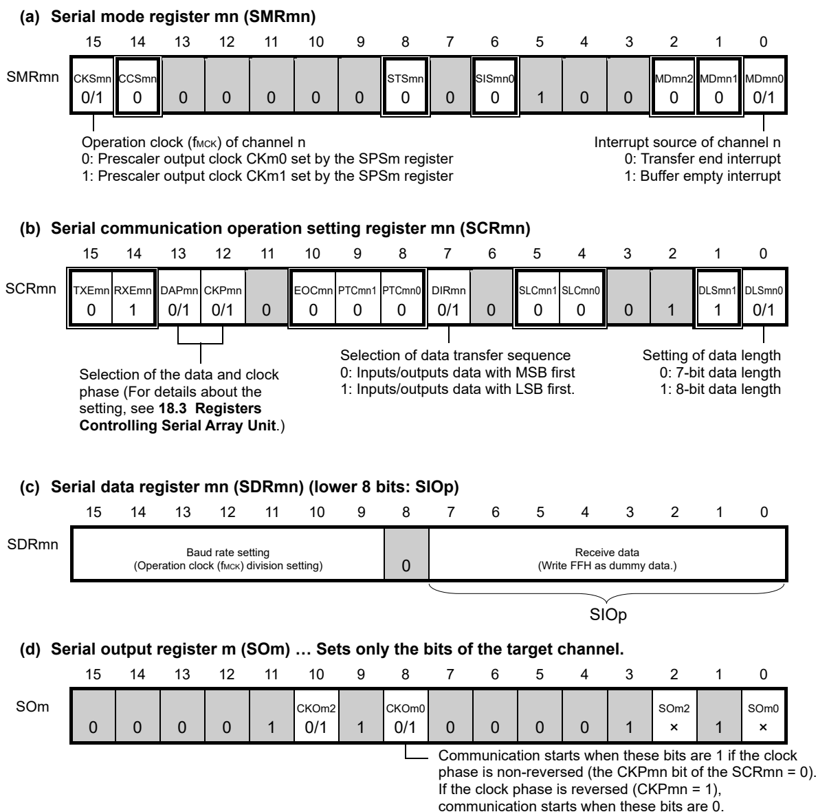
Figure 18-34. Example of Contents of Registers for Master Reception of simplified SPI (CSI00, CSI10, CSI30) (1/2)
