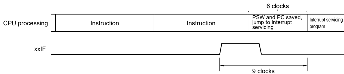
Figure 24-8. Interrupt Request Acknowledgment Timing (Minimum Time)
