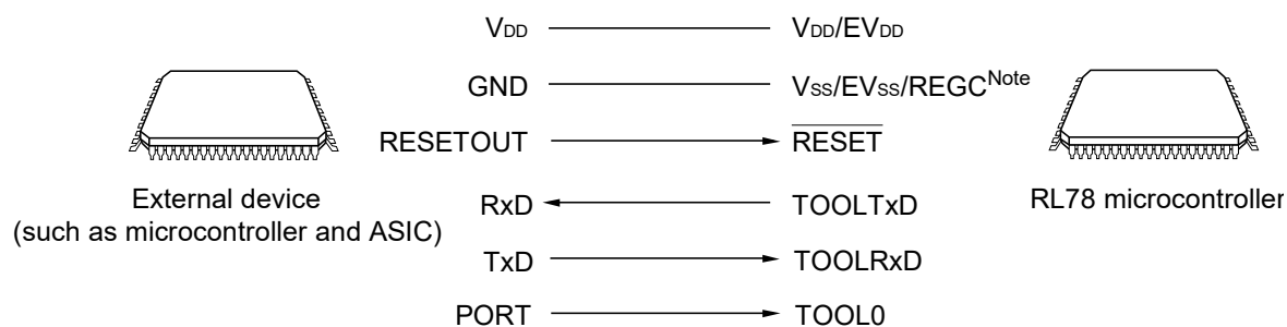
Figure 36-4. Communication with External Device
