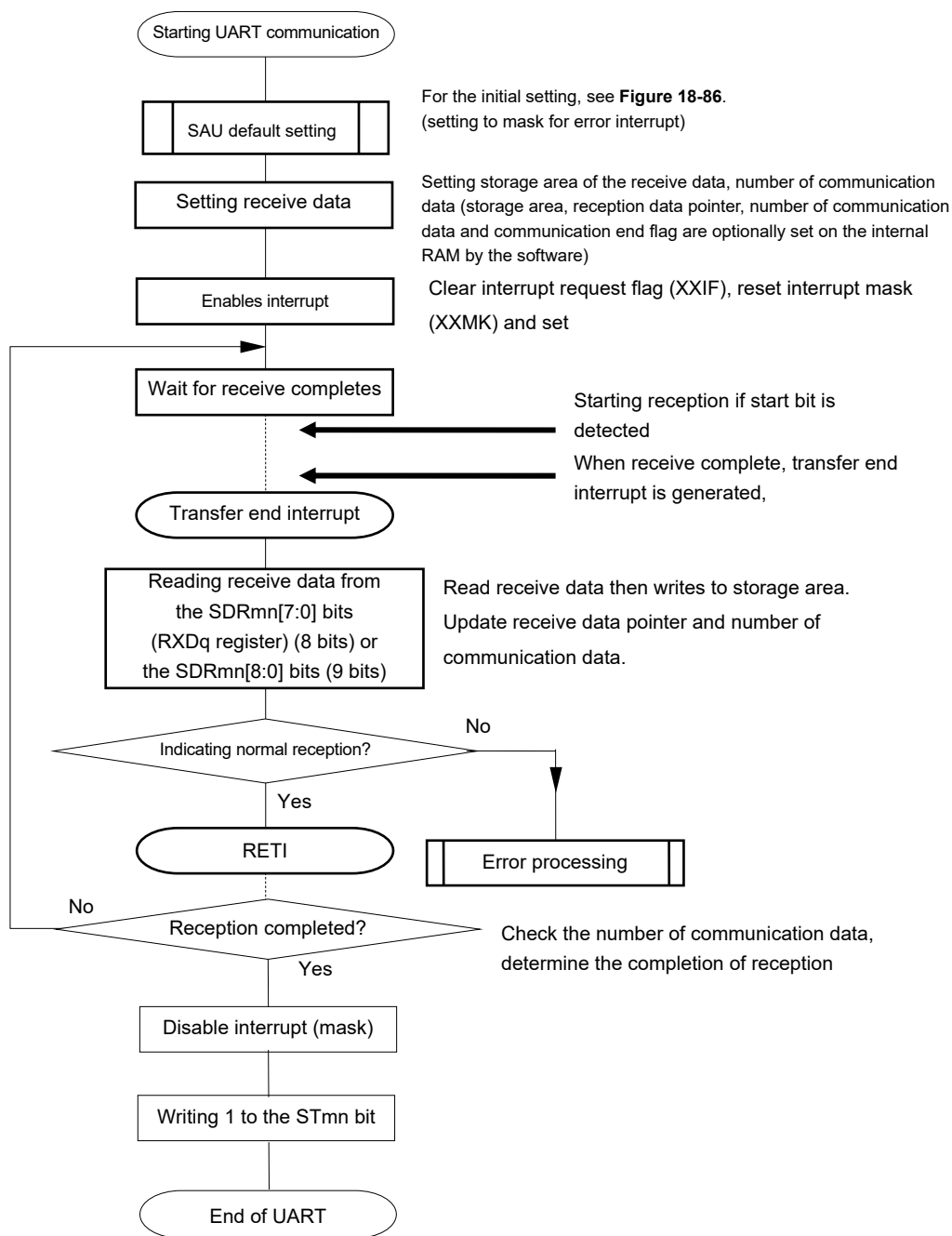
Figure 18-90. Flowchart of UART Reception
