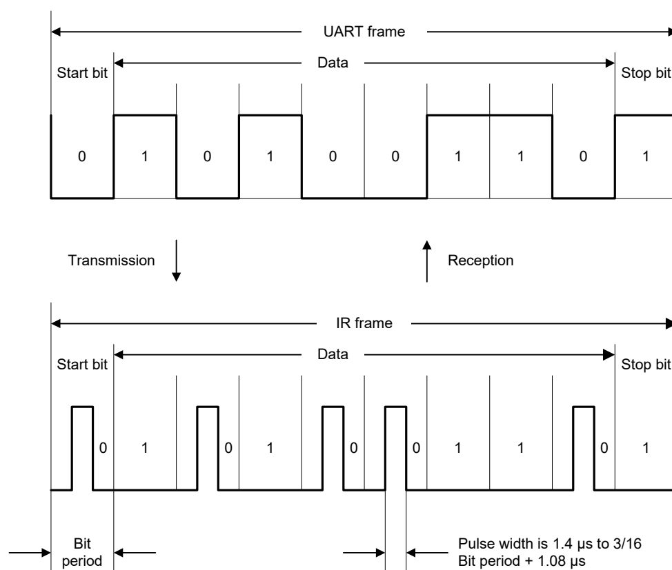
Figure 20-5. IrDA Transmission/Reception
