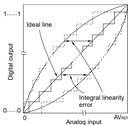
Figure 15-43. Integral Linearity Error
