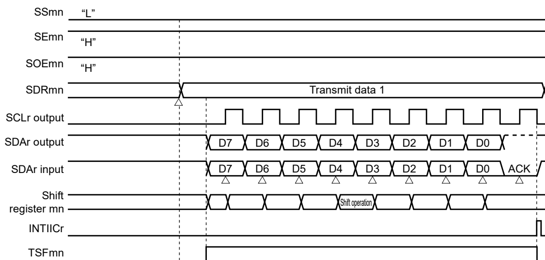
Figure 18-109. Timing Chart of Data Transmission
