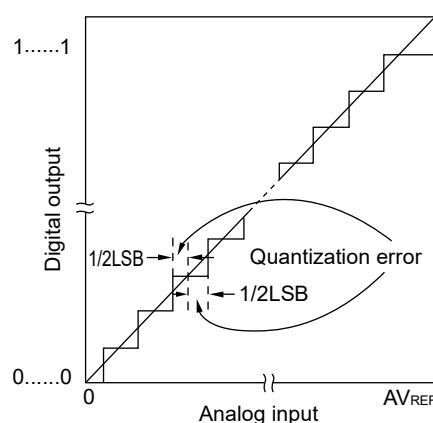
Figure 15-40. Quantization Error
