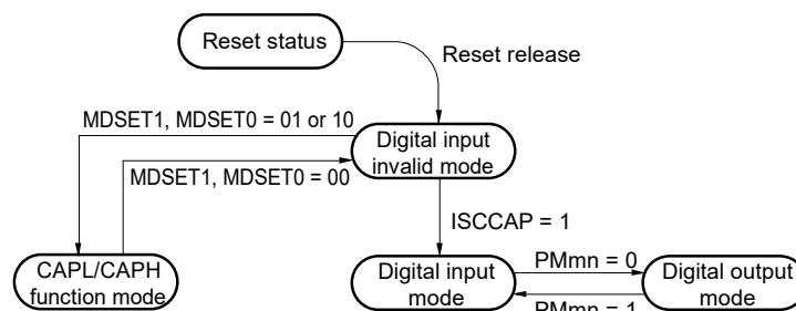
Figure 21-9. CAPL/P126 and CAPH/P127 Pin Function Status Transitions
