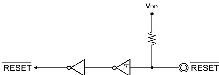
Figure 2-2. Pin Block Diagram for Pin Type 3-1-1
