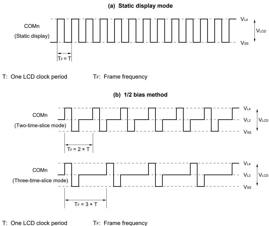
Figure 21-23. Common Signal Waveforms (1/3)
