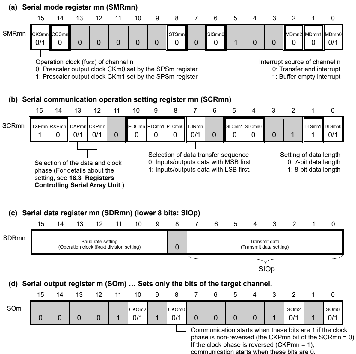
Figure 18-26. Example of Contents of Registers for Master Transmission of simplified SPI (CSI00, CSI10, CSI30) (1/2)
