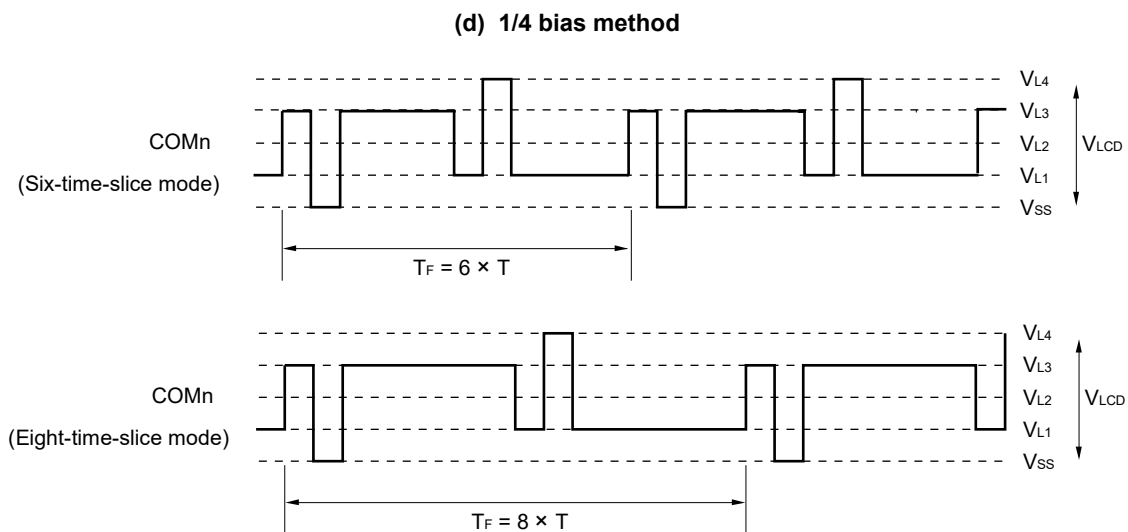
Figure 21-23. Common Signal Waveforms (3/3)
