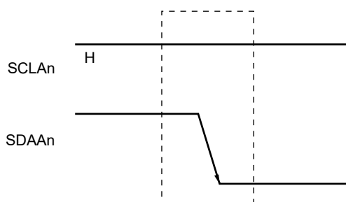
Figure 19-16. Start Conditions
