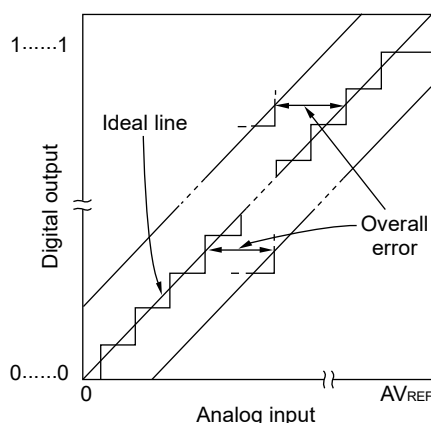
Figure 15-39. Overall Error
