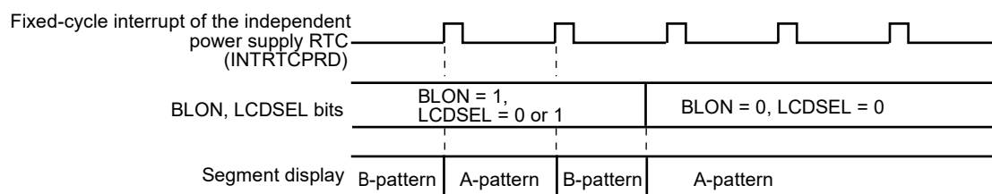
Figure 21-15. Switching Operation from Blinking Display to A-Pattern Display
