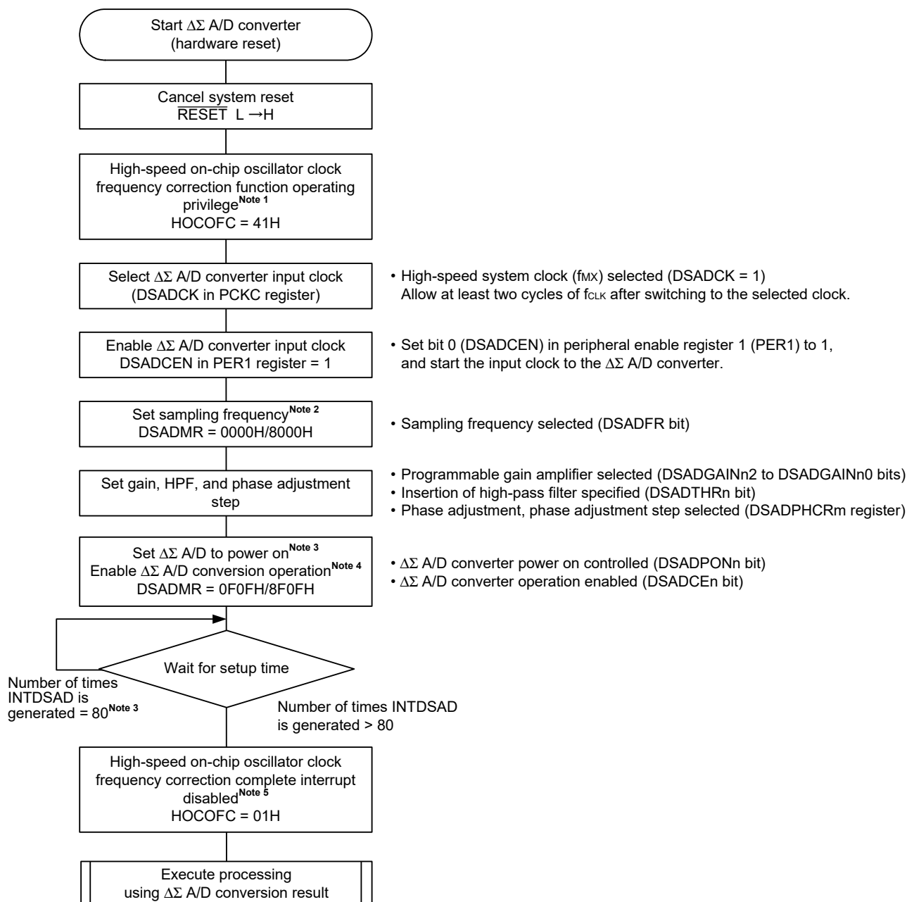
Figure 17-21. Initialization Flowchart
