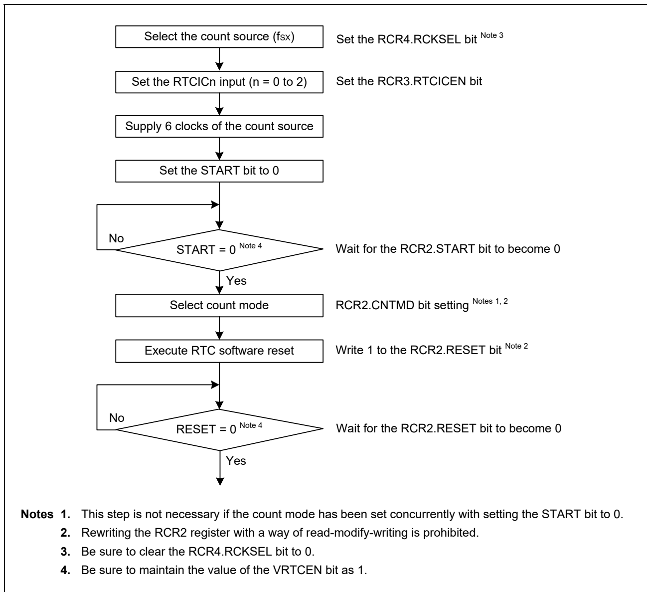
Figure 9-56. Clock and Count Mode Setting Procedure
