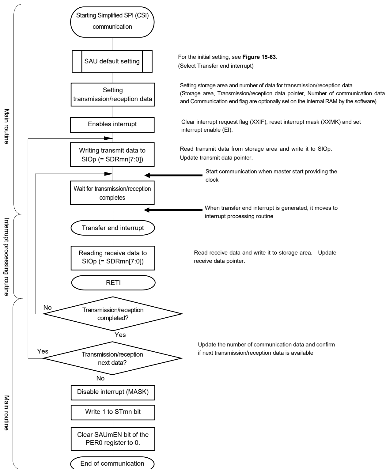
Figure 15-67. Flowchart of Slave Transmission/Reception (in Single-Transmission/Reception Mode)
