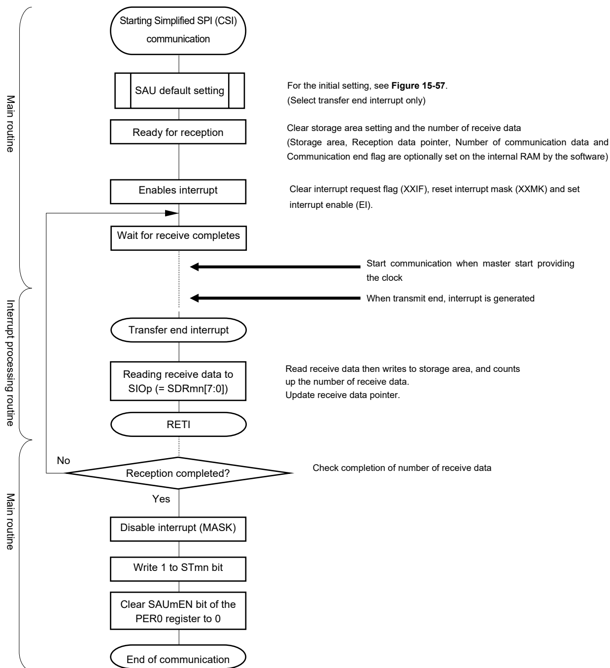
Figure 15-61. Flowchart of Slave Reception (in Single-Reception Mode)
