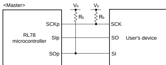
Simplified SPI (CSI) mode connection diagram (during communication at different potential)
