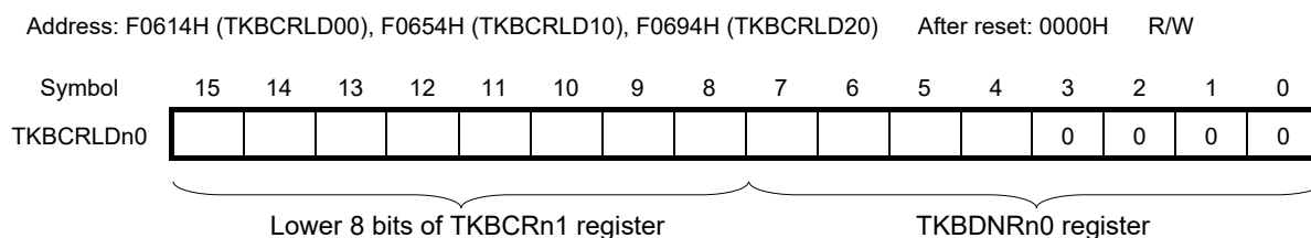
Figure 7-14. Format of 16-bit Timer KB Compare 1L & Dithering Count Register n0 (TKBCRLDn0)
