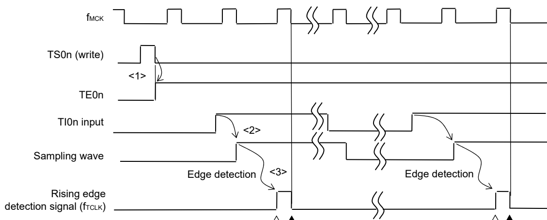
Figure 6-24. Timing of f_{CLK} and Count Clock ( f_{TCLK} ) (When CCS0n = 1, Noise Filter Unused)
