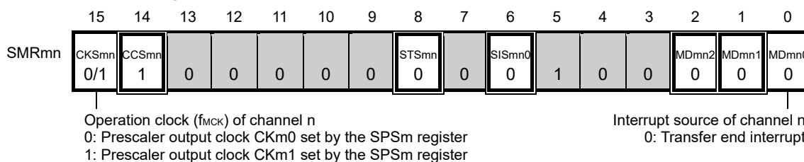
Figure 15-56. Example of Contents of Registers for Slave Reception of Simplified SPI (CSI00) (1/2)
