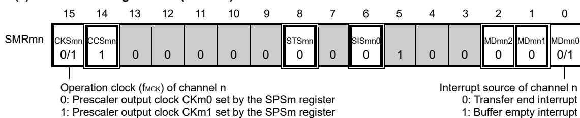
Figure 15-48. Example of Contents of Registers for Slave Transmission of Simplified SPI (CSI00) (1/2)
