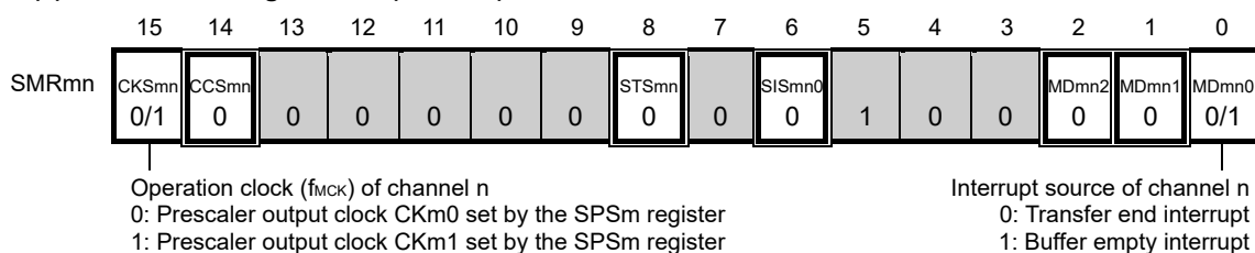
Figure 15-24. Example of Contents of Registers for Master Transmission of Simplified SPI (CSI00)
