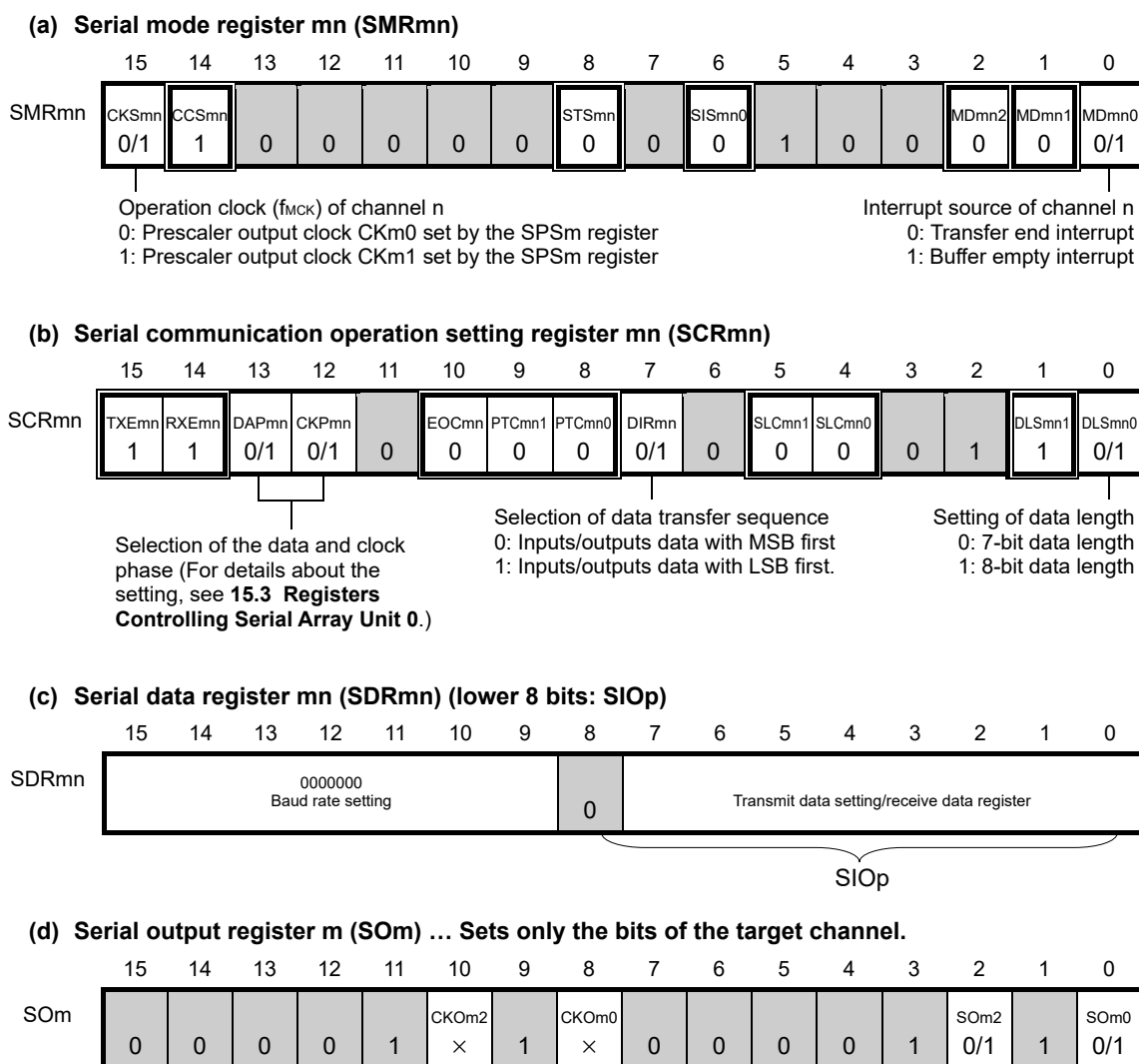
Figure 15-62. Example of Contents of Registers for Slave Transmission/Reception of Simplified SPI (CSI00) (1/2)
