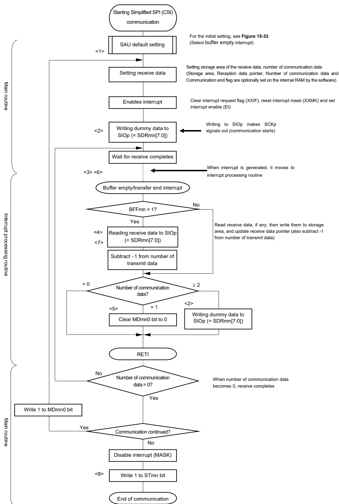
Figure 15-39. Flowchart of Master Reception (in Continuous Reception Mode)
