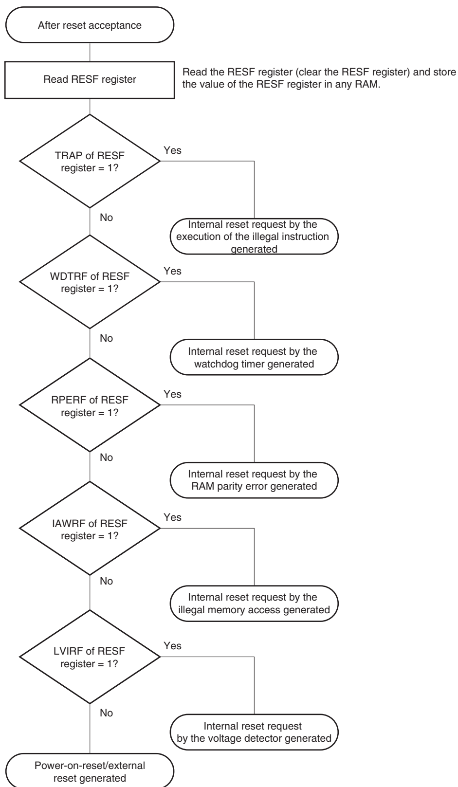
Figure 22-5. Procedure for Checking Reset Source
