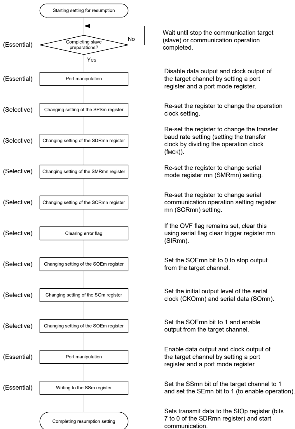
Figure 15-43. Procedure for Resuming Master Transmission/Reception
