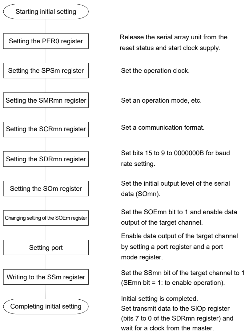
Figure 15-63. Initial Setting Procedure for Slave Transmission/Reception
