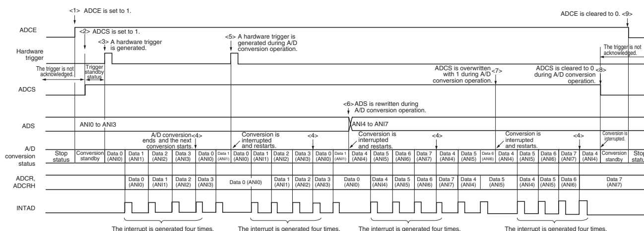
Figure 12-23. Example of Hardware Trigger No-wait Mode (Scan Mode, Sequential Conversion Mode) Operation Timing
