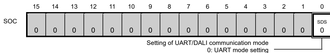
Figure 16-27. Example of Contents of Registers for UART Transmission (1/2)
