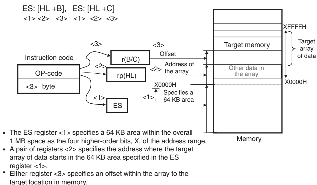
Figure 3-33. Example of ES:[HL+B], ES:[HL+C]
