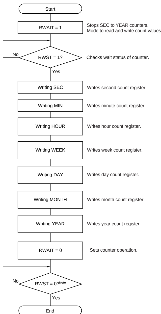
Figure 9-22. Procedure for Writing Real-time Clock
