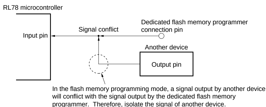
Figure 28-3. Signal Conflict ( \overline{\text{RESET}} Pin)
