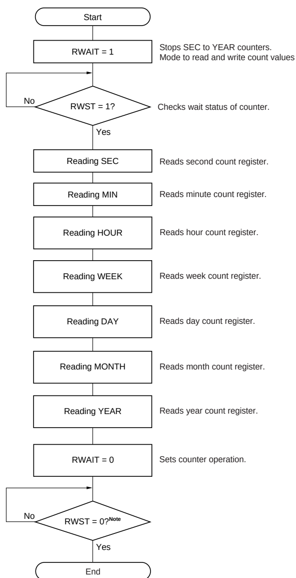
Figure 9-21. Procedure for Reading Real-time Clock
