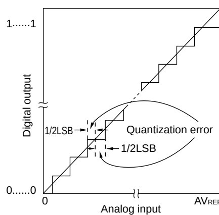
Figure 12-39. Quantization Error
