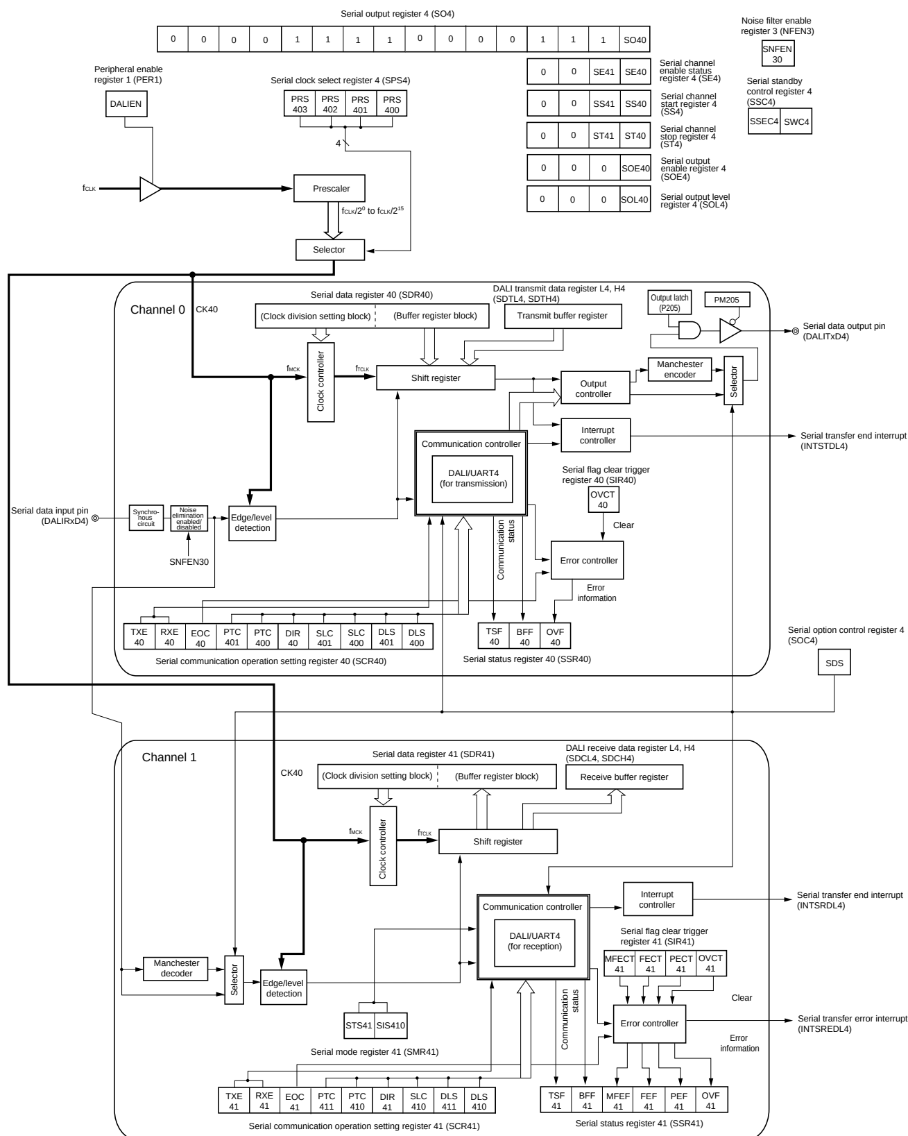
Figure 16-1. Block Diagram of Serial Array Unit 4 (DALI/UART4)
