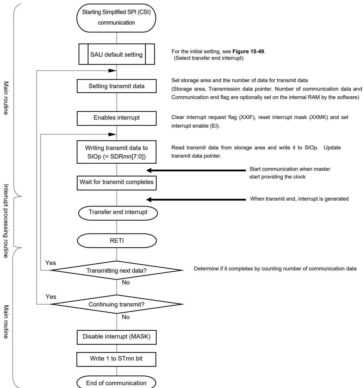
Figure 15-53. Flowchart of Slave Transmission (in Single-Transmission Mode)
