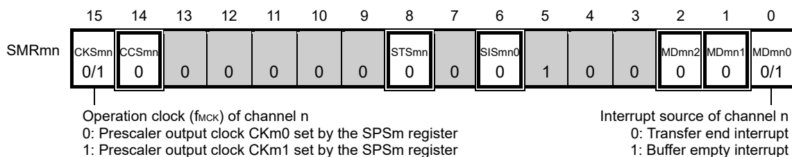
Figure 15-40. Example of Contents of Registers for Master Transmission/Reception of Simplified SPI (CSI00) (1/2)
