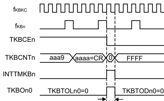
Figure 7-35. Figure of Timing of Stop Operation (Operation of TKBCEn Is Simultaneous with the Generation of Timer Count Clock.)
