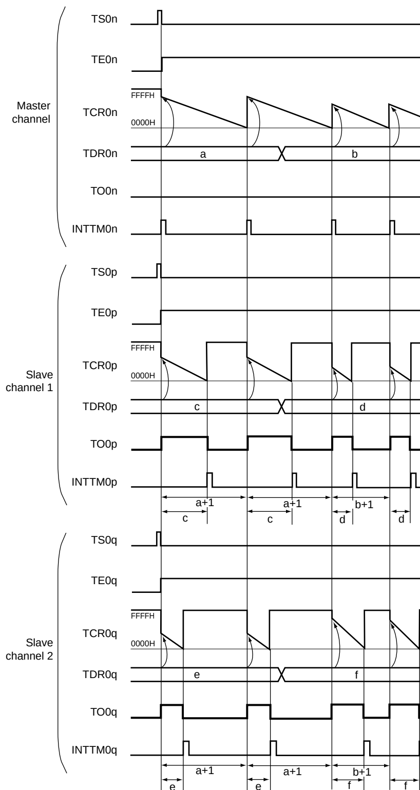
Figure 6-71. Example of Basic Timing of Operation as Multiple PWM Output Function (Output Two Types of PWMs)
