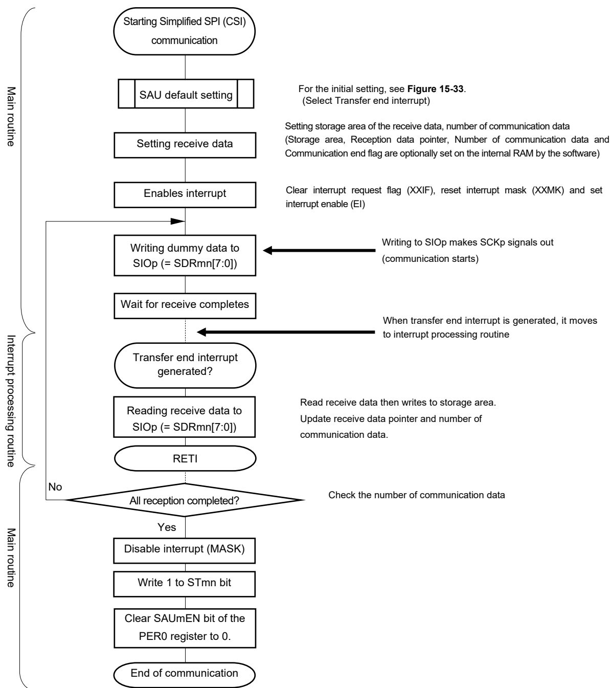
Figure 15-37. Flowchart of Master Reception (in Single-Reception Mode)
