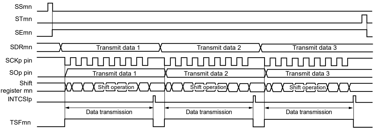
Figure 15-28. Timing Chart of Master Transmission (in Single-Transmission Mode) (Type 1: DAPmn = 0, CKPmn = 0)
