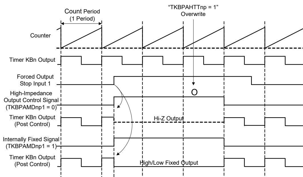
Figure 7-82. Forced Output Stop Function 1 at TKBPAHCMnp1, TKBPAHCMnp0 = 1, 0
