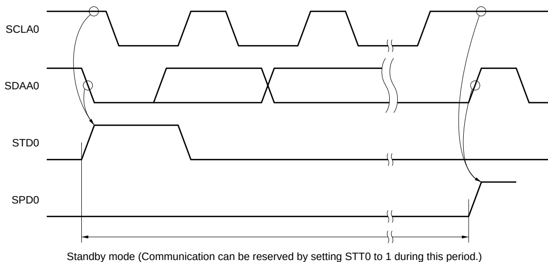
Figure 17-27. Timing for Accepting Communication Reservations
