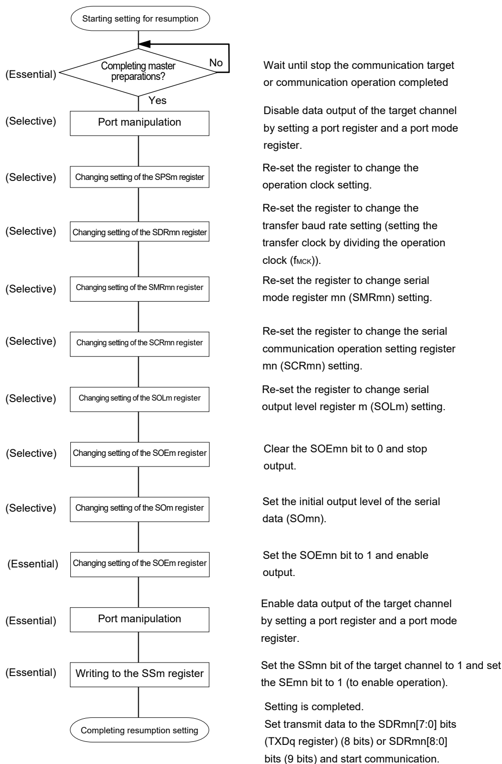
Figure 15-78. Procedure for Resuming UART Transmission
