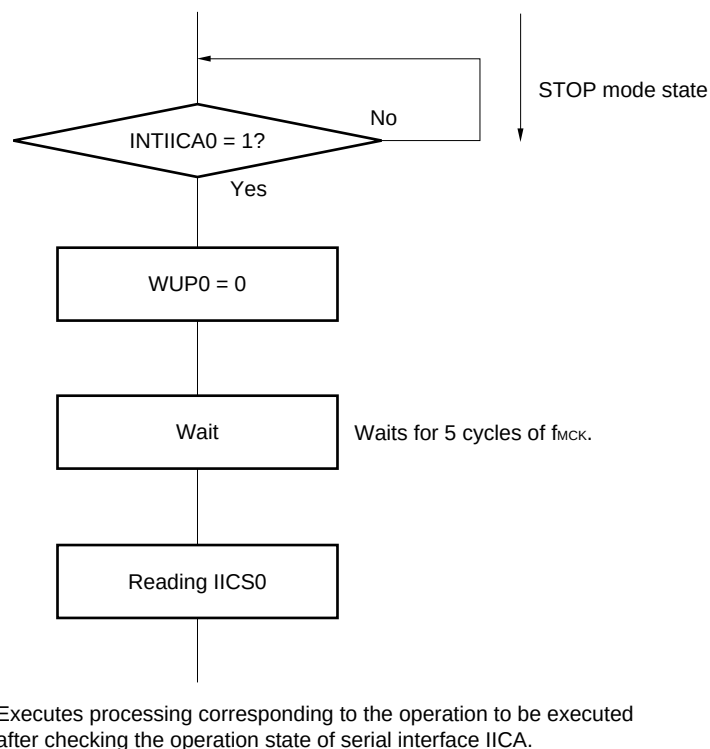
Figure 17-24. Flow When Setting WUP0 = 0 upon Address Match (Including Extension Code Reception)
