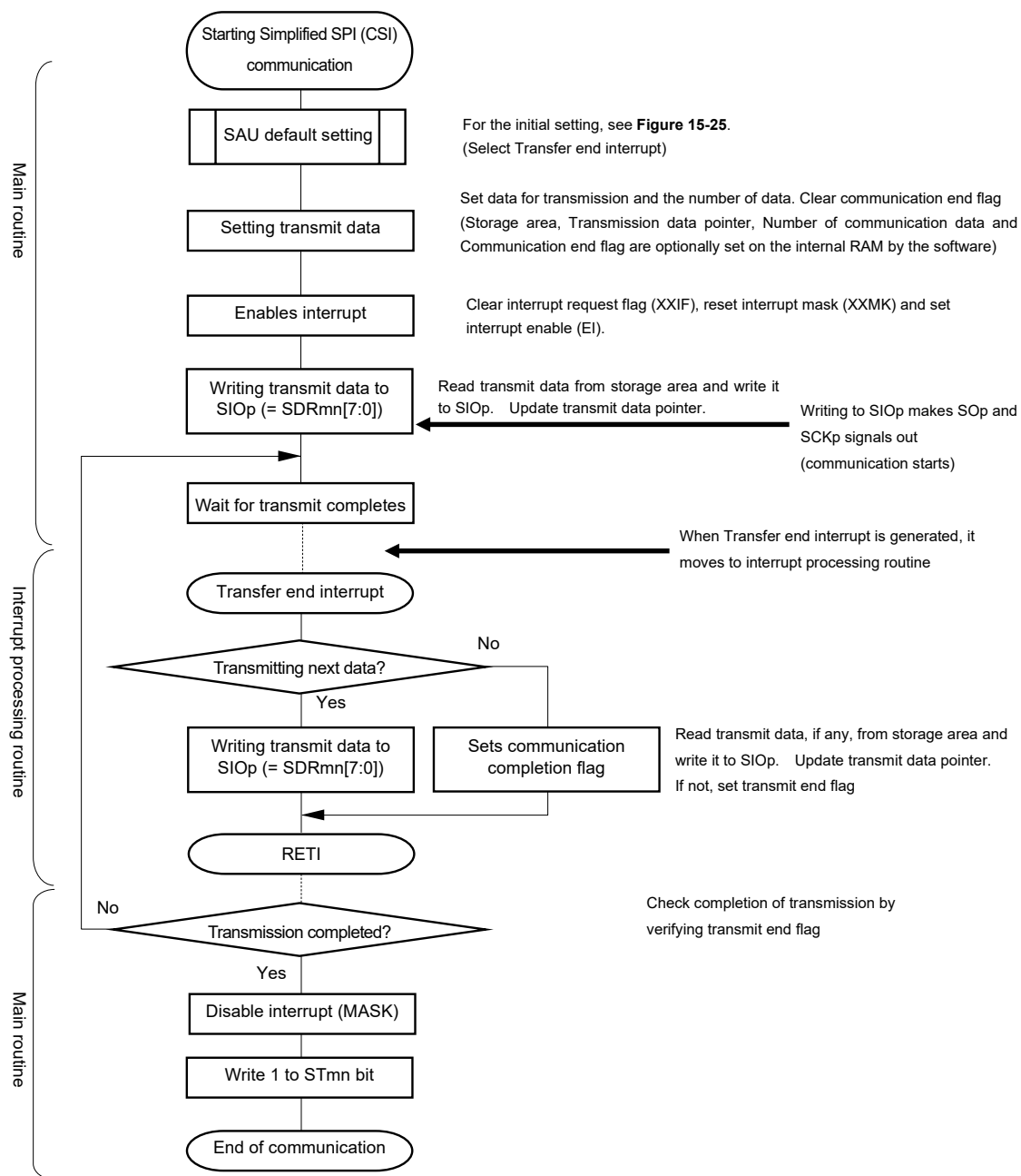
Figure 15-29. Flowchart of Master Transmission (in Single-Transmission Mode)
