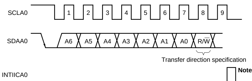
Figure 17-18. Transfer Direction Specification
