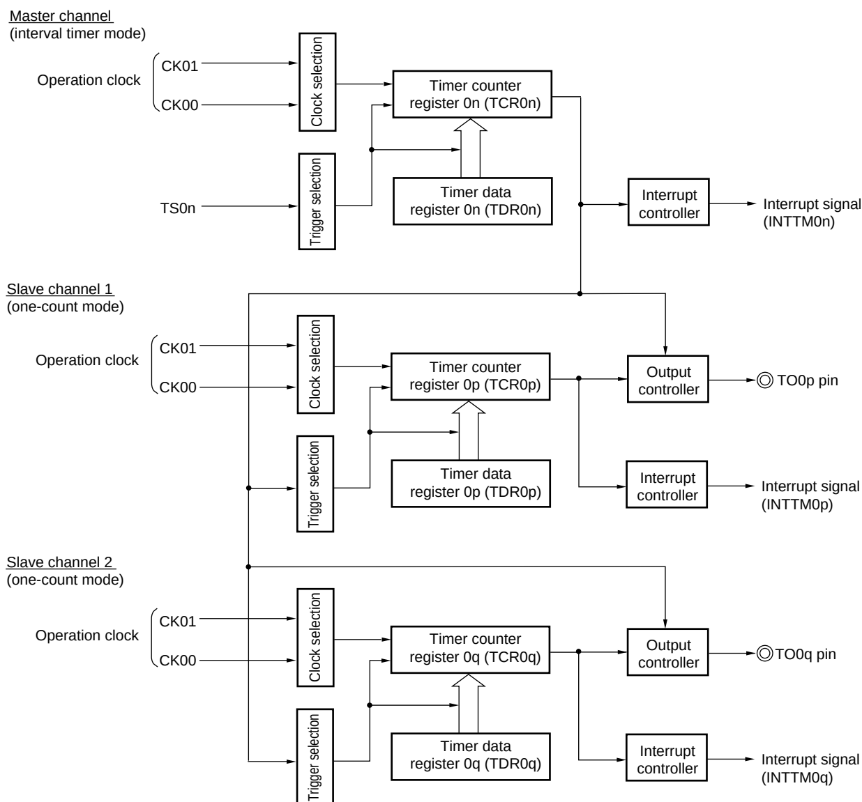
Figure 6-70. Block Diagram of Operation as Multiple PWM Output Function (Output Two Types of PWMs)
