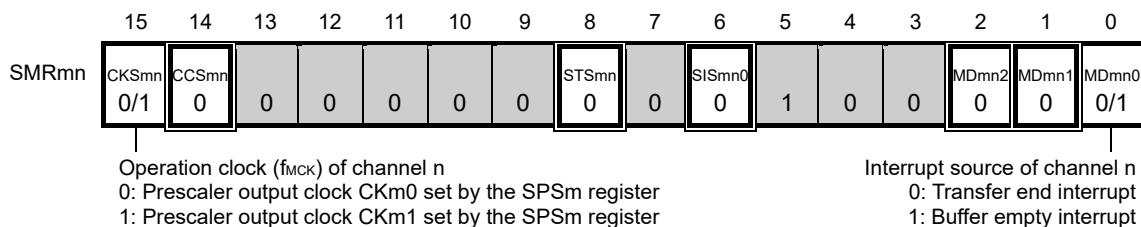
Figure 15-32. Example of Contents of Registers for Master Reception of Simplified SPI (CSI00) (1/2)
