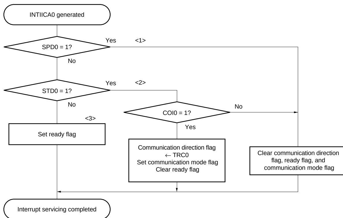
Figure 17-32. Slave Operation Flowchart (2)
