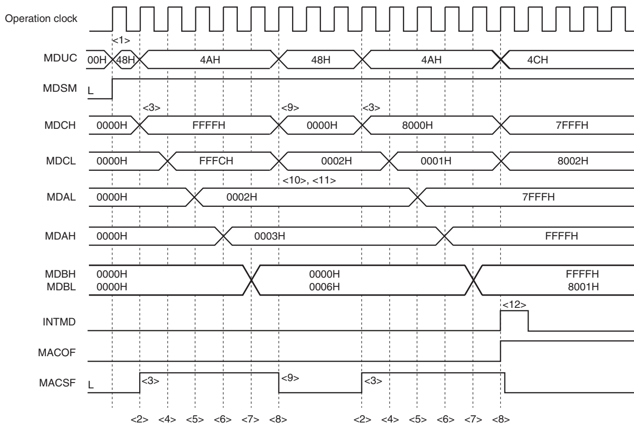
Figure 18-9. Timing Diagram of Multiply-Accumulation (signed) Operation (2 \times 3 + (-4) = 2 \rightarrow 32767 \times (-1) + (-2147483647) = -2147450882 \text{ (Overflow Occurs.)})
