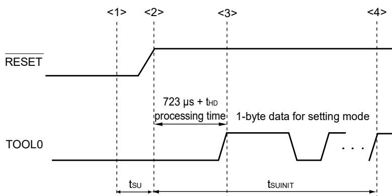
Figure 28-5. Setting of Flash Memory Programming Mode
