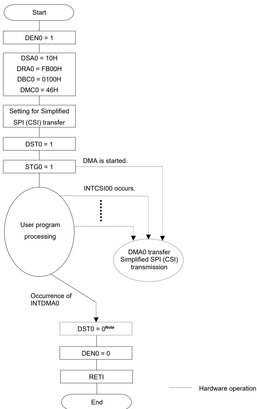
Figure 19-7. Example of Setting for Simplified SPI (CSI) Consecutive Transmission
