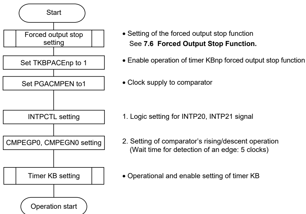
Figure 14-16. Operation Setting Flow Chart 2 of Comparator (CMP) (Using Timer Forced Output Stop Request Signal by INTP2m (Using Edge Circuit only))
