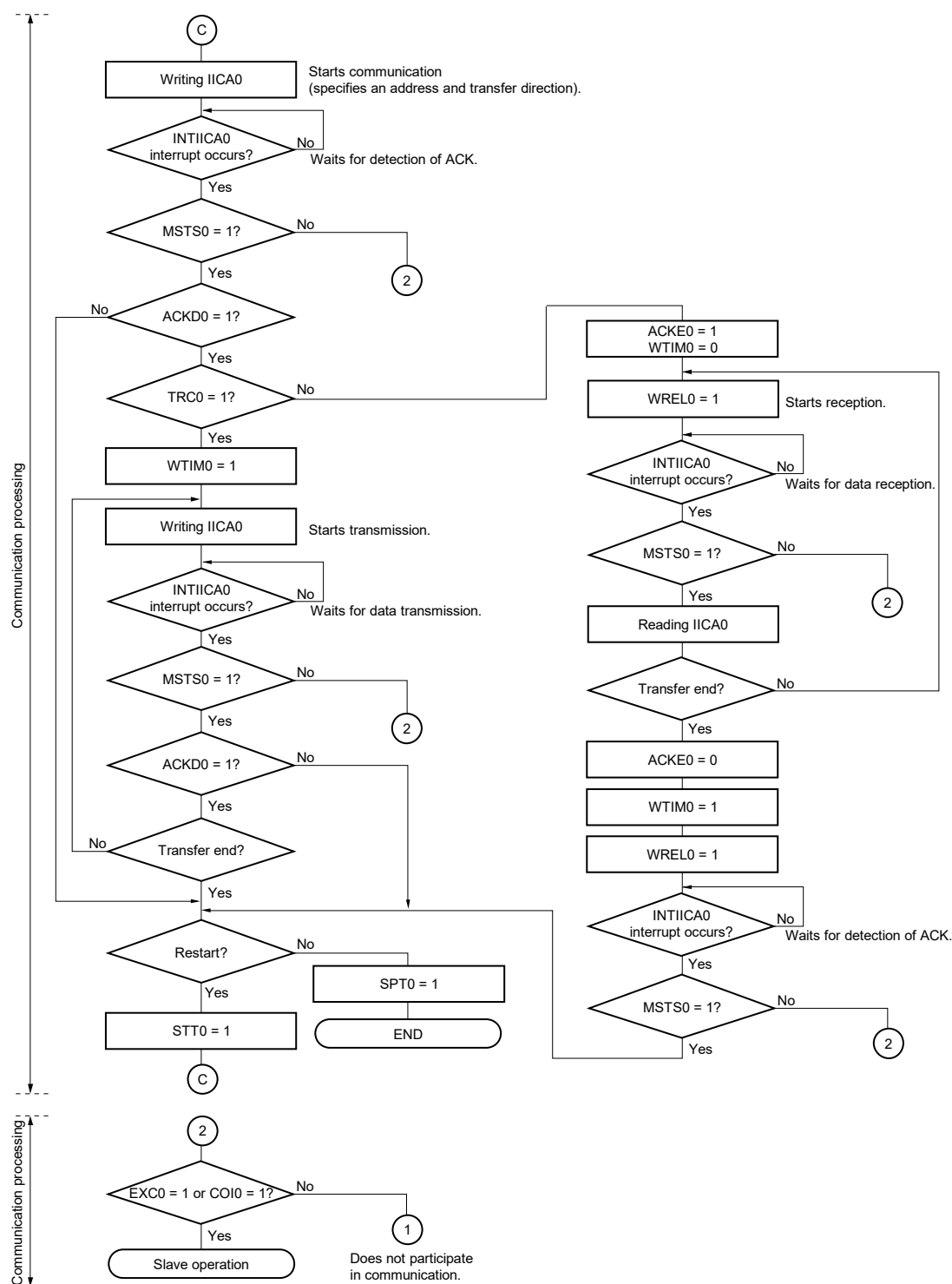
Figure 17-30. Master Operation in Multi-master System (3/3)
