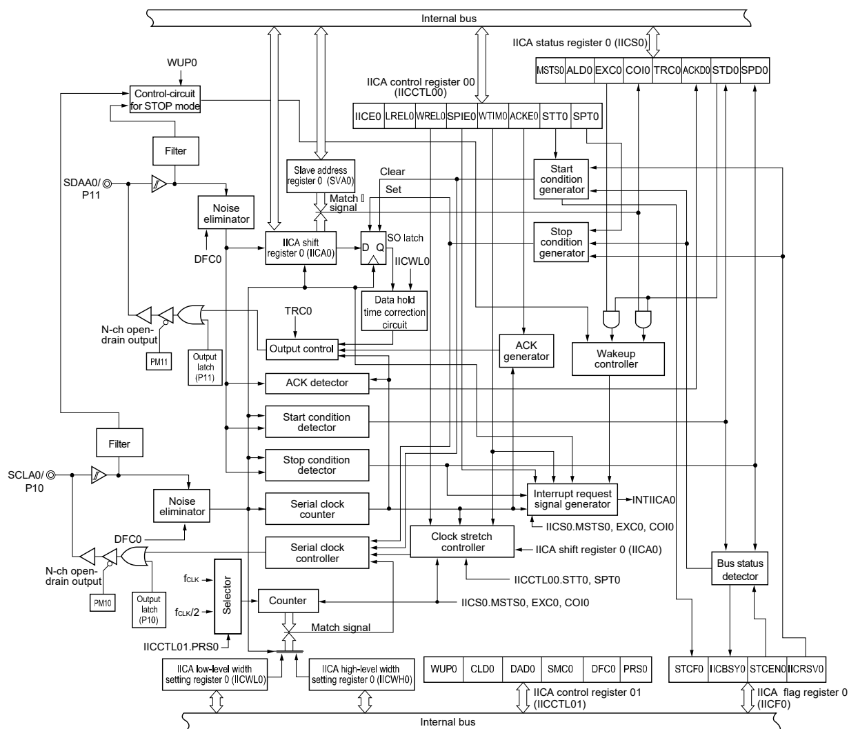
Figure 17-1. Block Diagram of Serial Interface IICA
