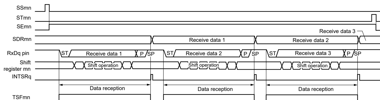
Figure 15-87. Timing Chart of UART Reception
