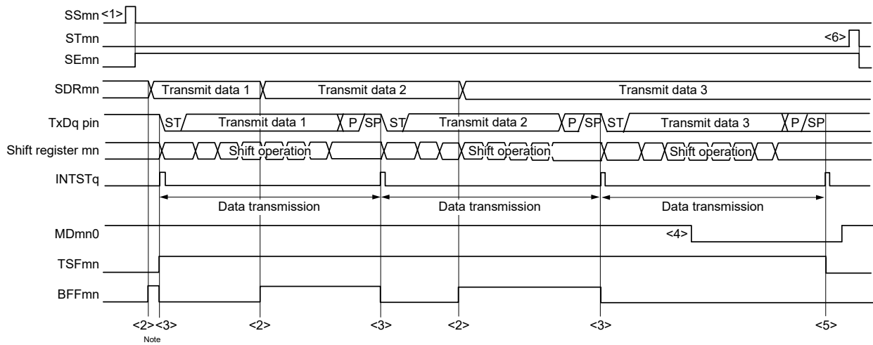
Figure 14 - 113 Timing Chart of UART Transmission (in Continuous Transmission Mode)
