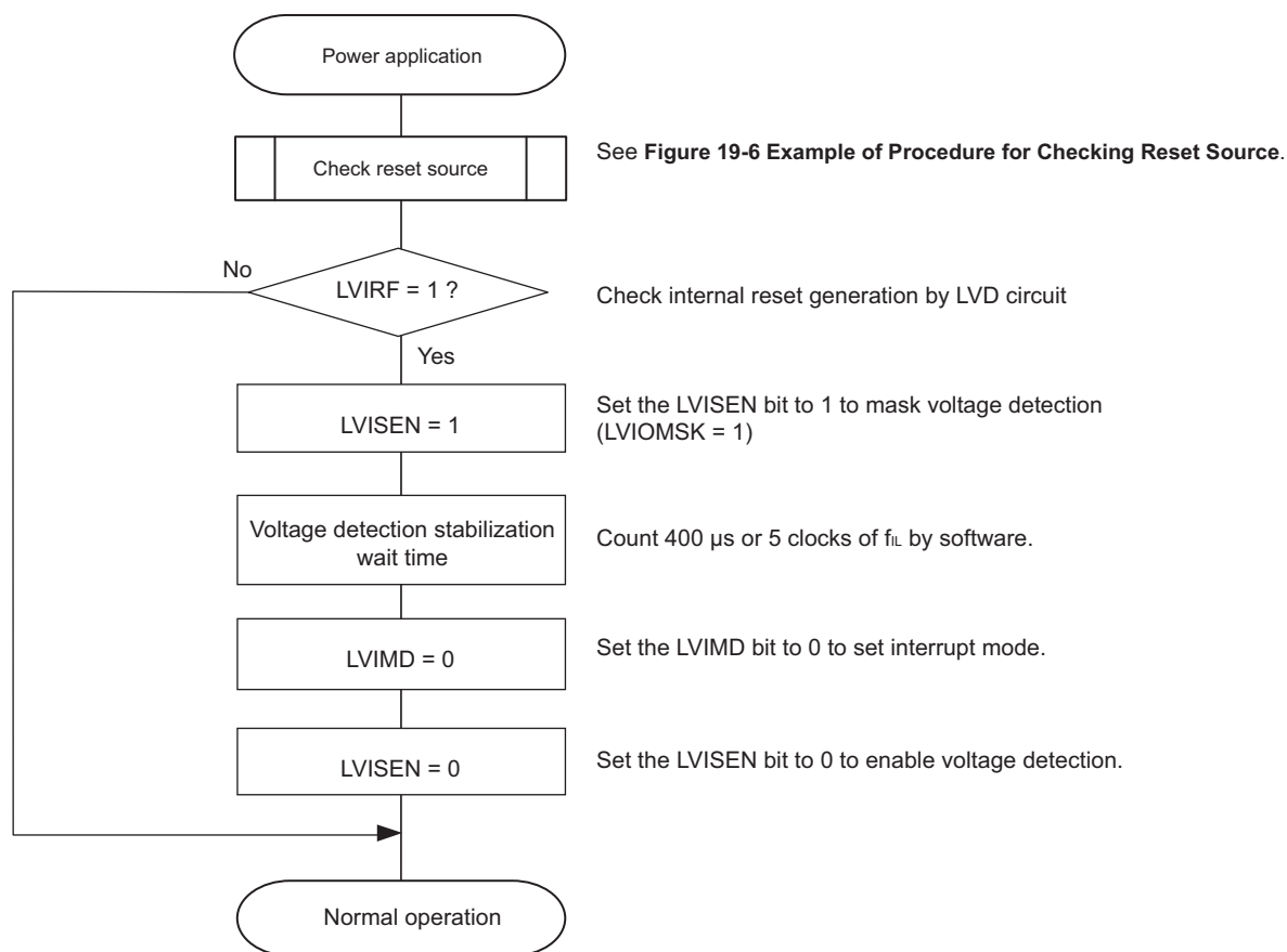
Figure 21 - 9 Initial Setting of Interrupt and Reset Mode
