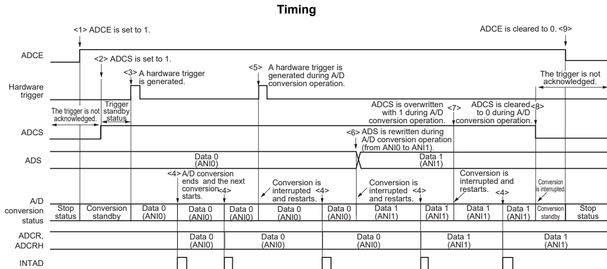
Figure 12 - 23 Example of Hardware Trigger No-Wait Mode (Select Mode, Sequential Conversion Mode) Operation
