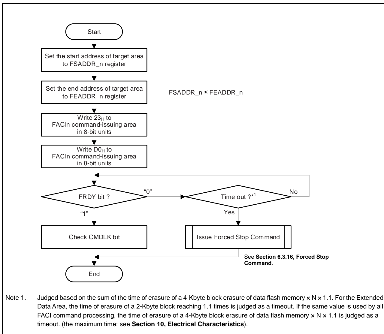
Figure 6.12 Area Erasure Command Usage
