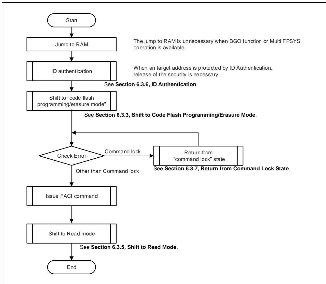
Figure 6.1 Overview of Command Usage in Code Flash Programming/Erasure Mode
