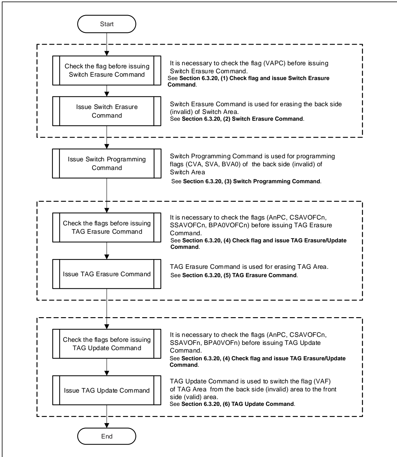
Figure 6.22 Switching Usage of Hardware Property Area
