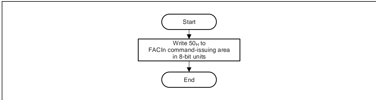
Figure 6.17 Status Clearing Command Usage
