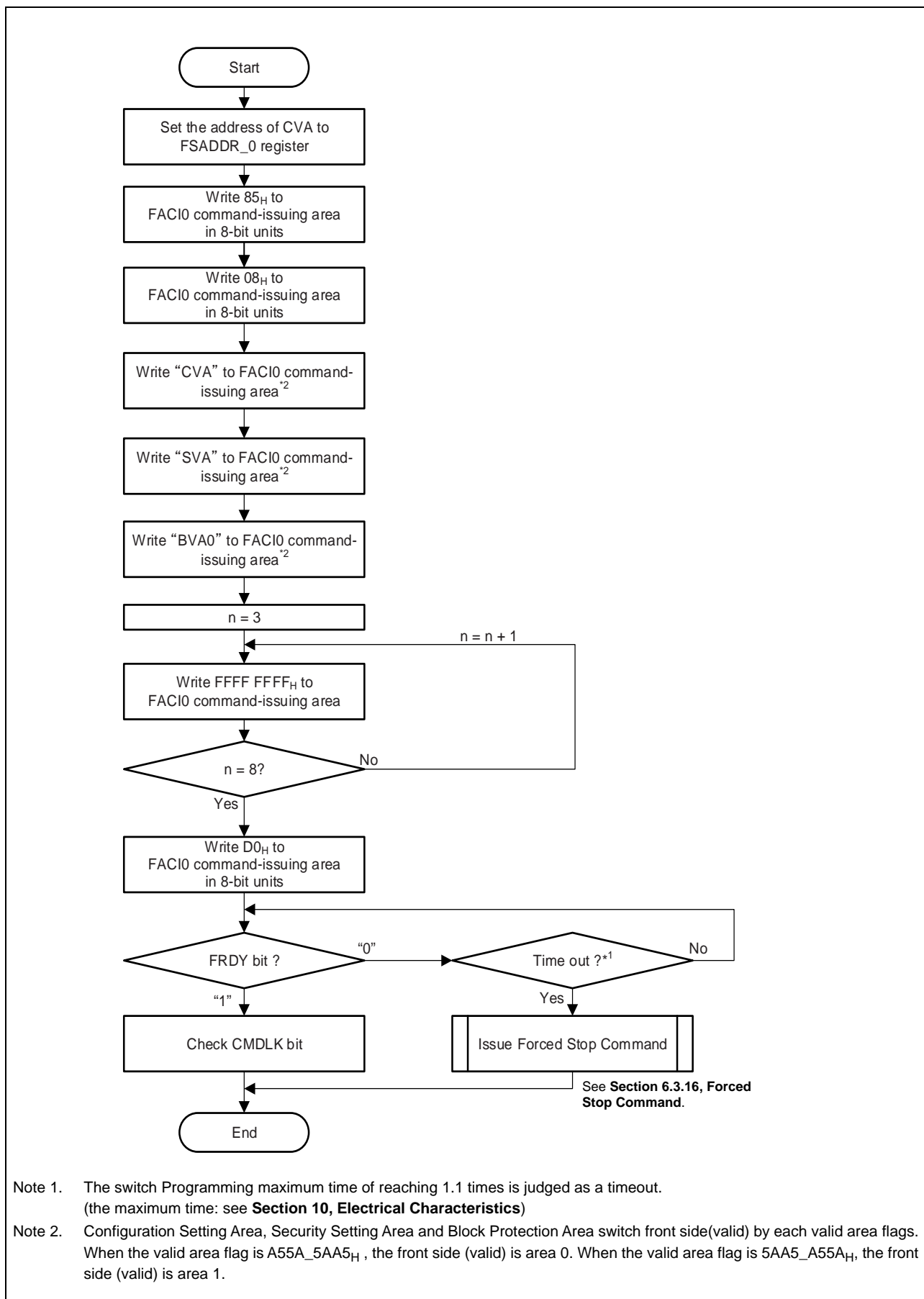
Figure 6.25 Switch Programming Command Usage
