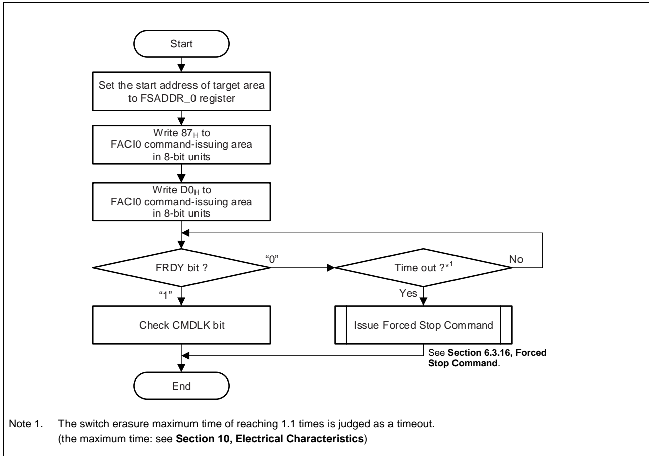
Figure 6.24 Switch Erasure Command Usage
