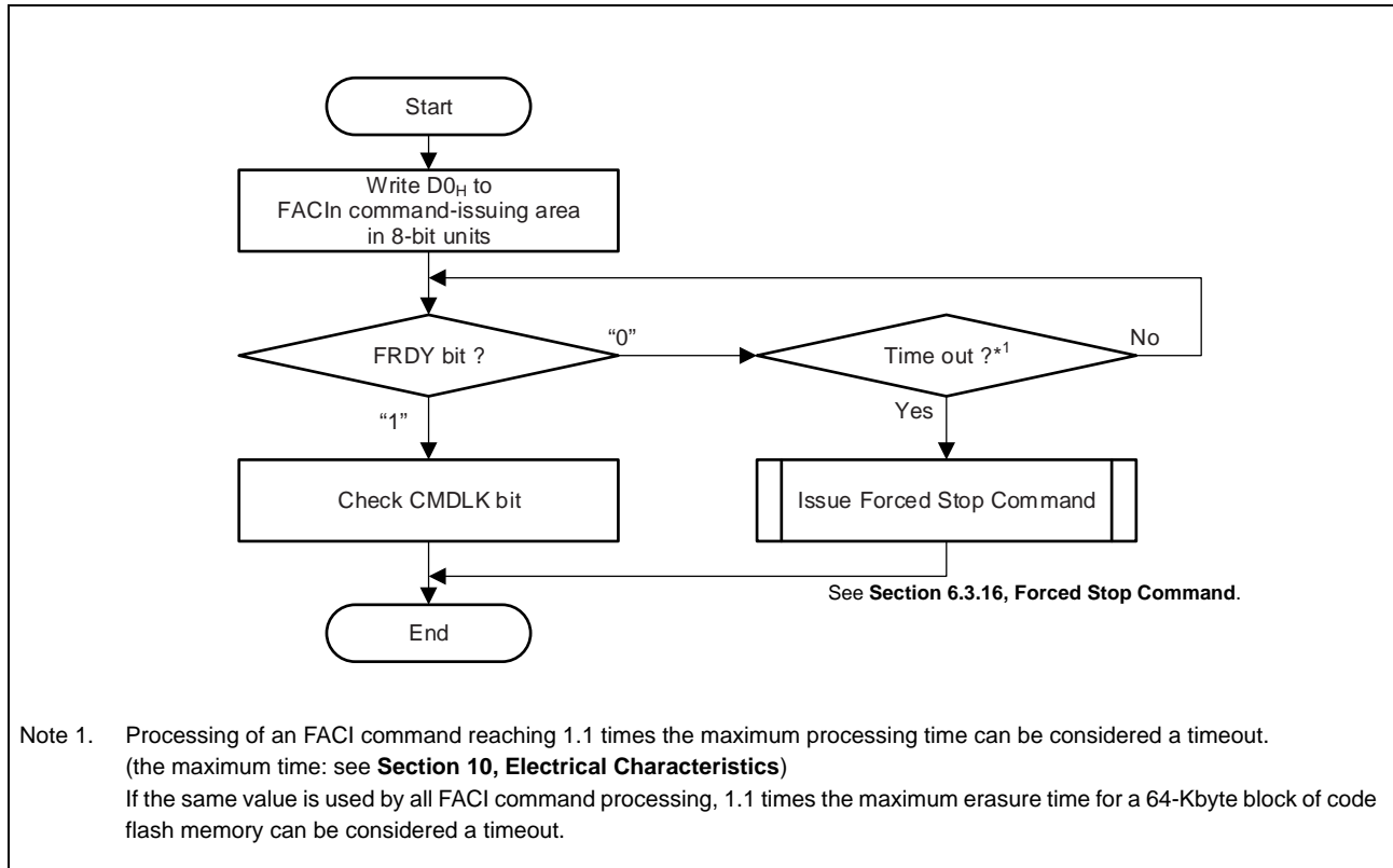
Figure 6.16 Programming/Erasure Resumption Command Usage
