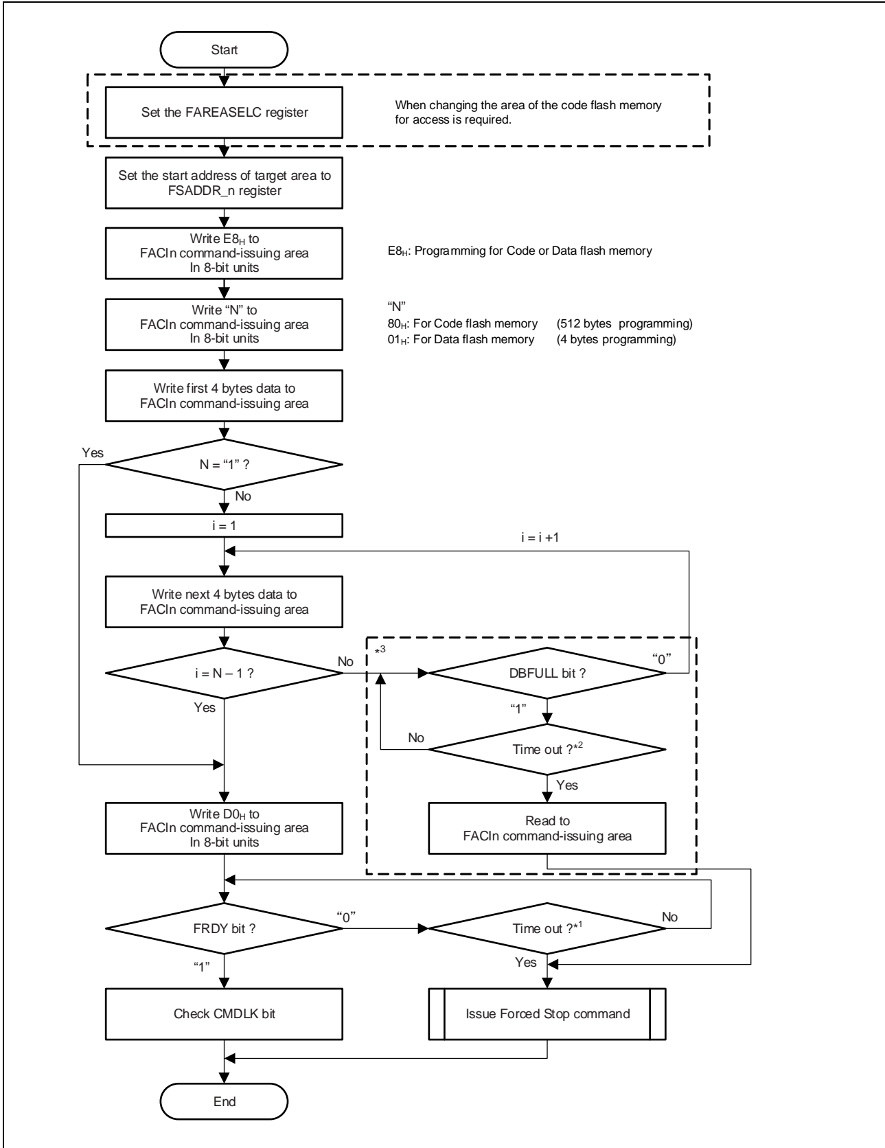
Figure 6.8 Programming Command Usage (1/2)
