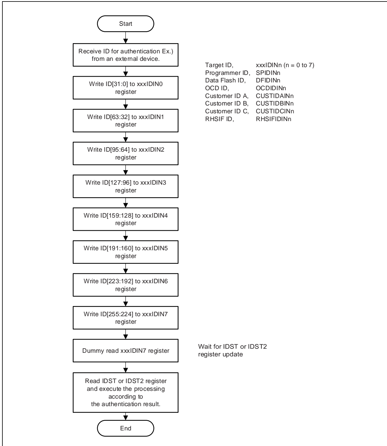
Figure 6.6 Flow of ID Authentication
