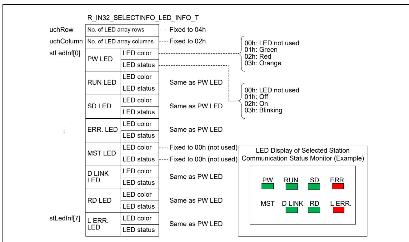
Figure 4.19Creating LED information
