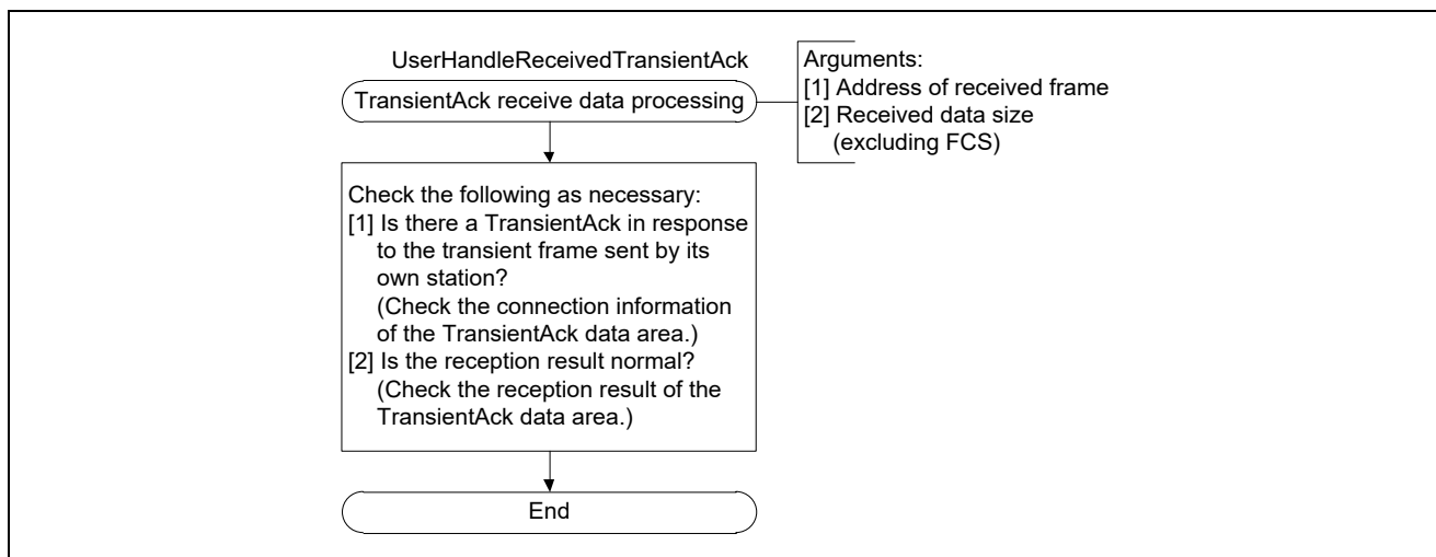
Figure 4.28 Flowchart for TransientAck Receive Data Processing
