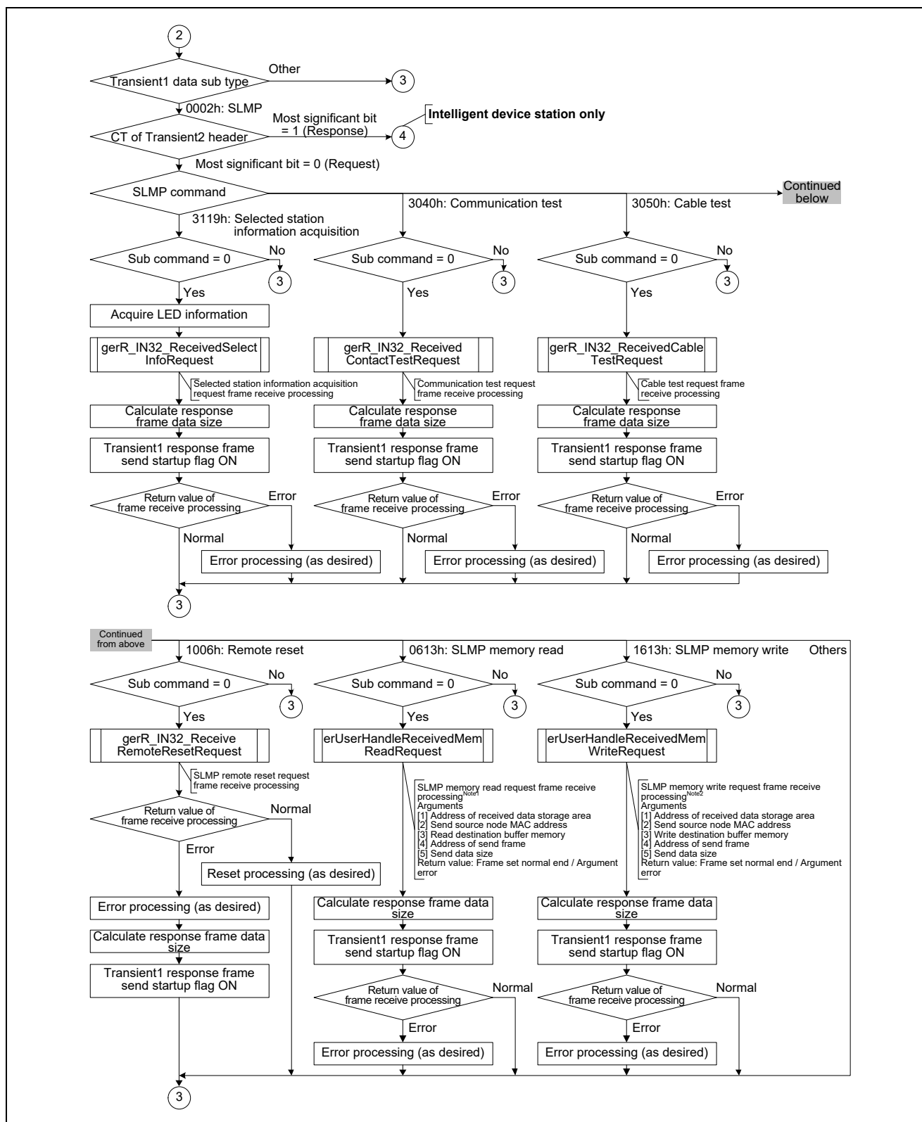
Figure 4.17 Flowchart for Transient1 Receive Data Processing (3/4)
