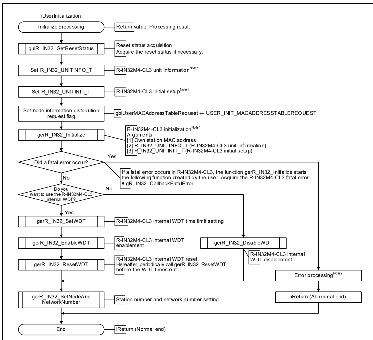
Figure 4.2 Flowchart for Initialization Processing
