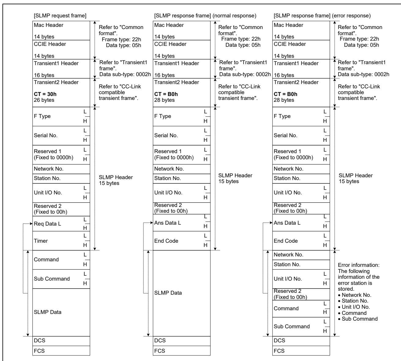
Figure 7.14 Overview of SLMP Frame Basic Format
