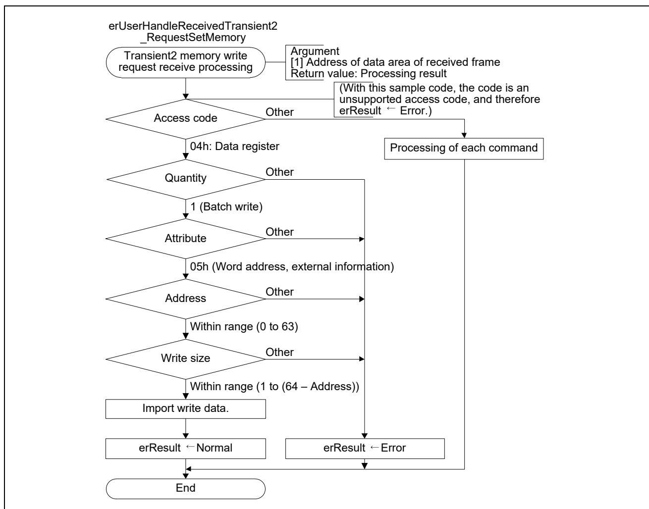
Figure 4.26 Flowchart for Transient2 Memory Write Request Receive Processing
