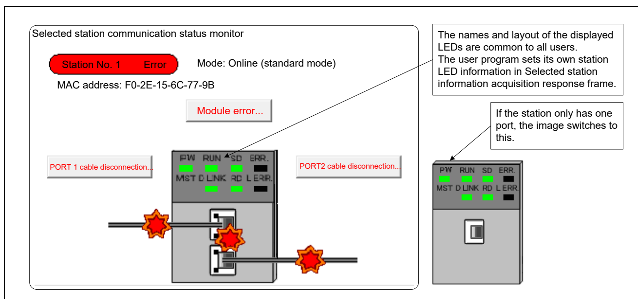
Figure 3.7 Display Example of Selected Station Communication Status Monitor
