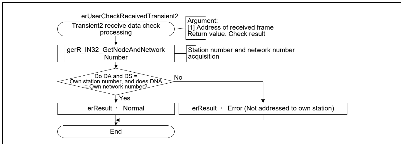
Figure 4.25 Flowchart for Transient2 Receive Data Check Processing
