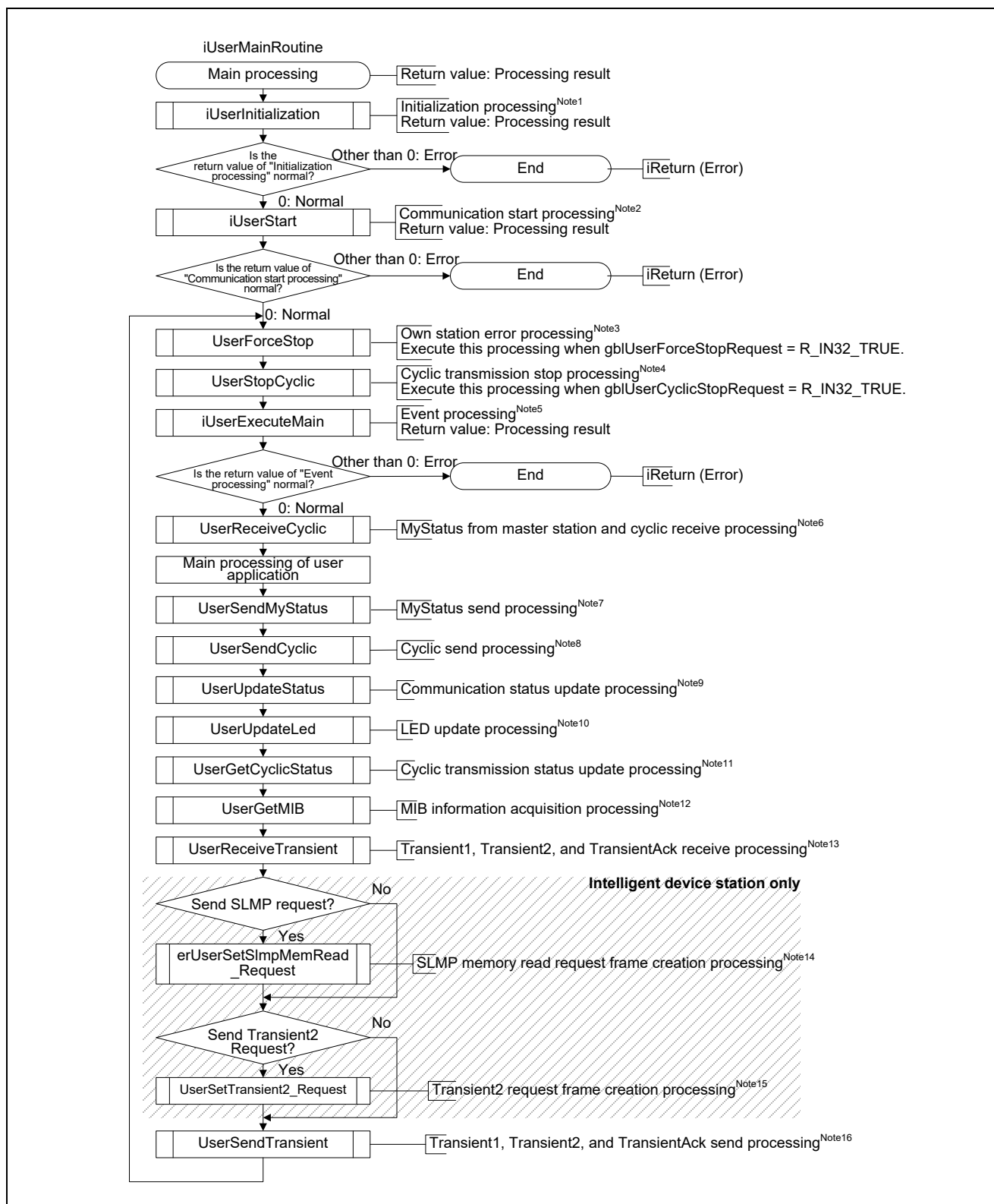
Figure 4.1 Flowchart for Main Processing
