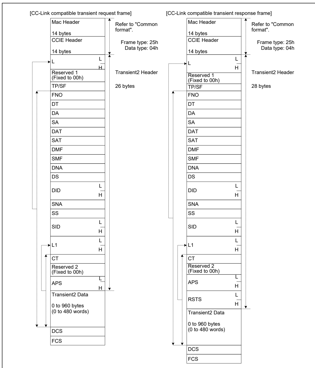
Figure 7.4 Overview of CC-Link Compatible Transient Frame Basic Format
