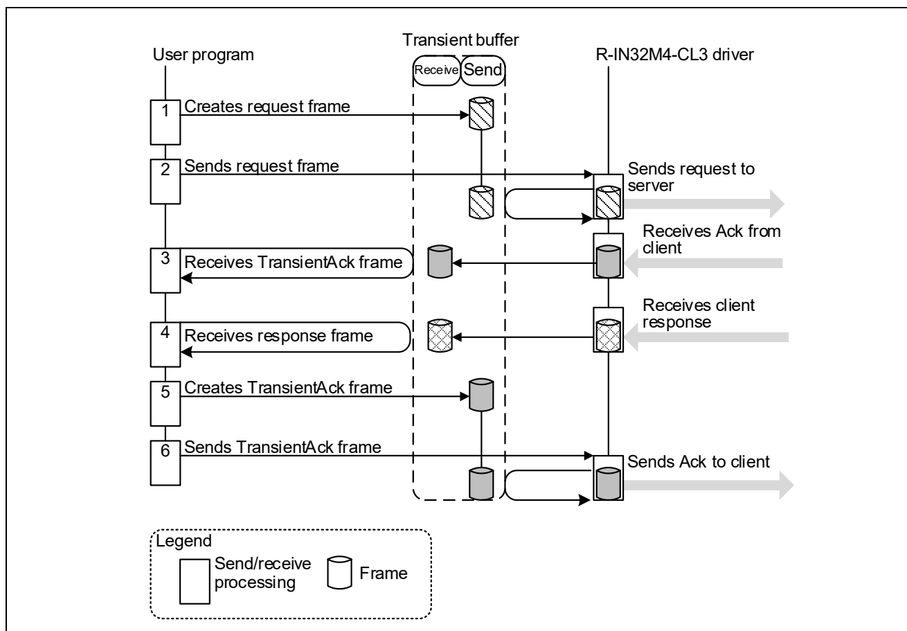
Figure 4.15 Client Processing Procedure
