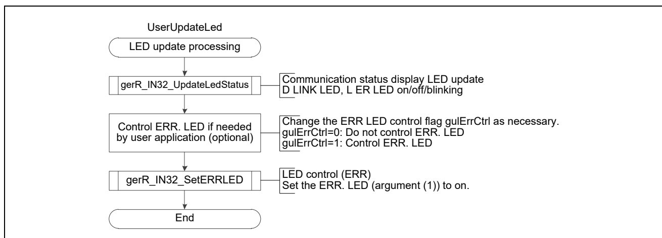
Figure 4.11 Flowchart for LED Update Processing
