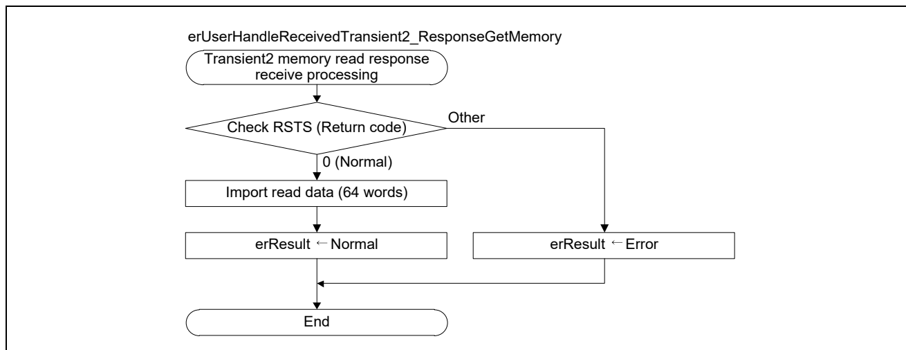
Figure 4.39 Flowchart for Transient2 Memory Read Response Receive Processing
