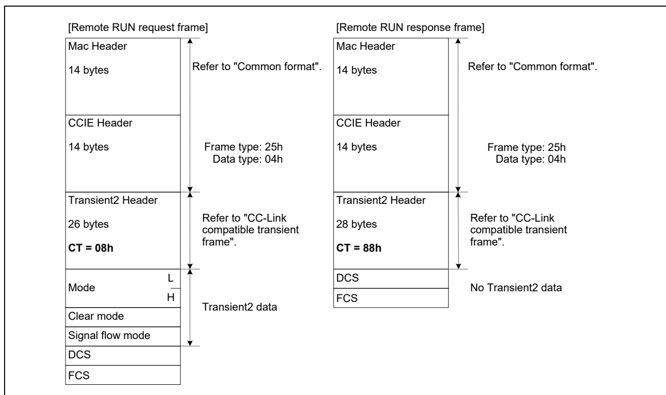
Figure 7.8 Overview of Remote RUN Frame Format
