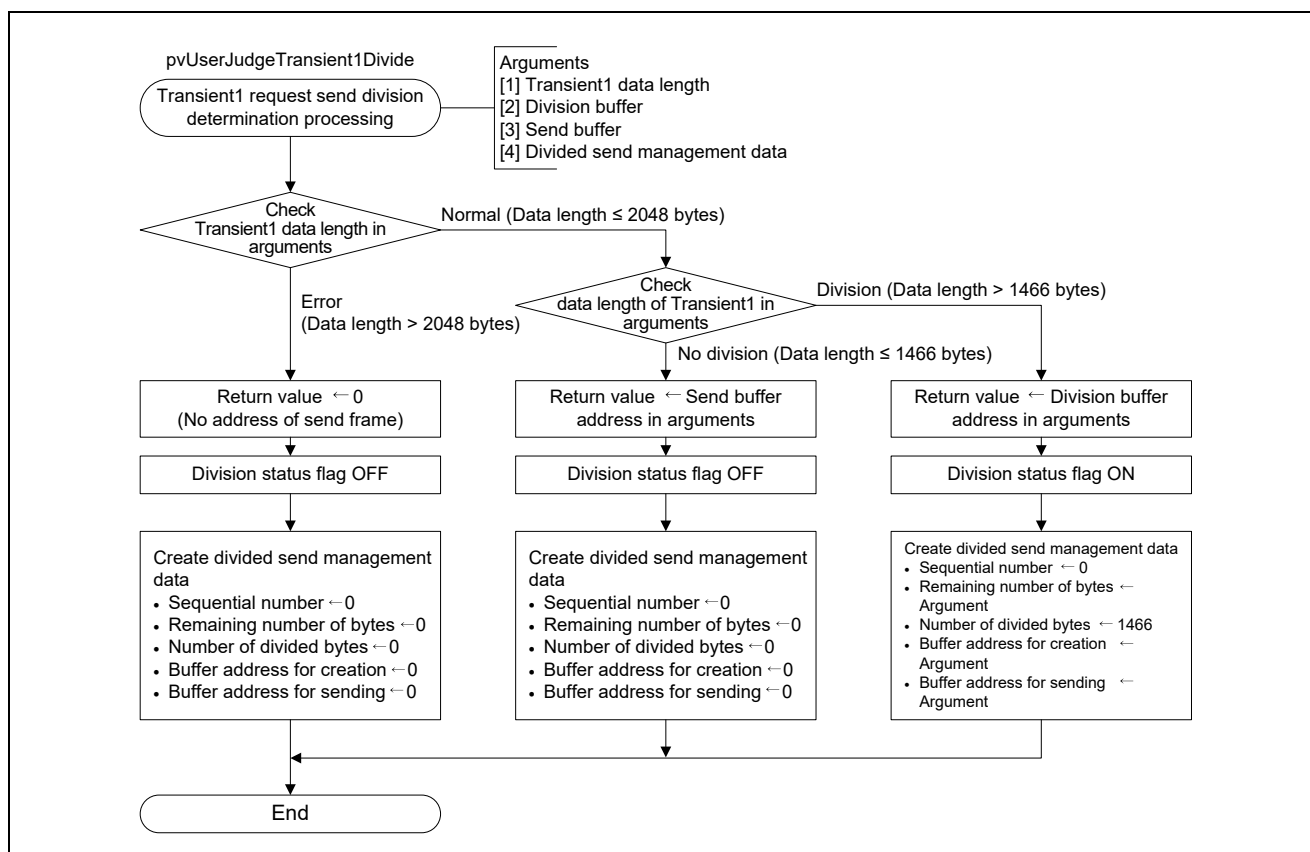
Figure 4.34 Flowchart for Transient1 Request Send Division Determination Processing
