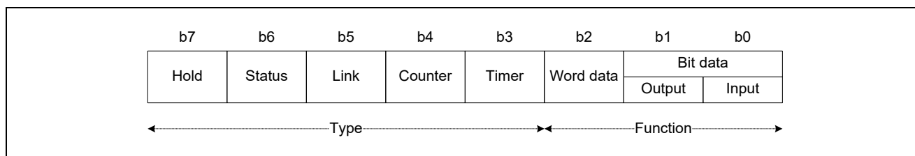
Figure 7.7 Access Code Definition
