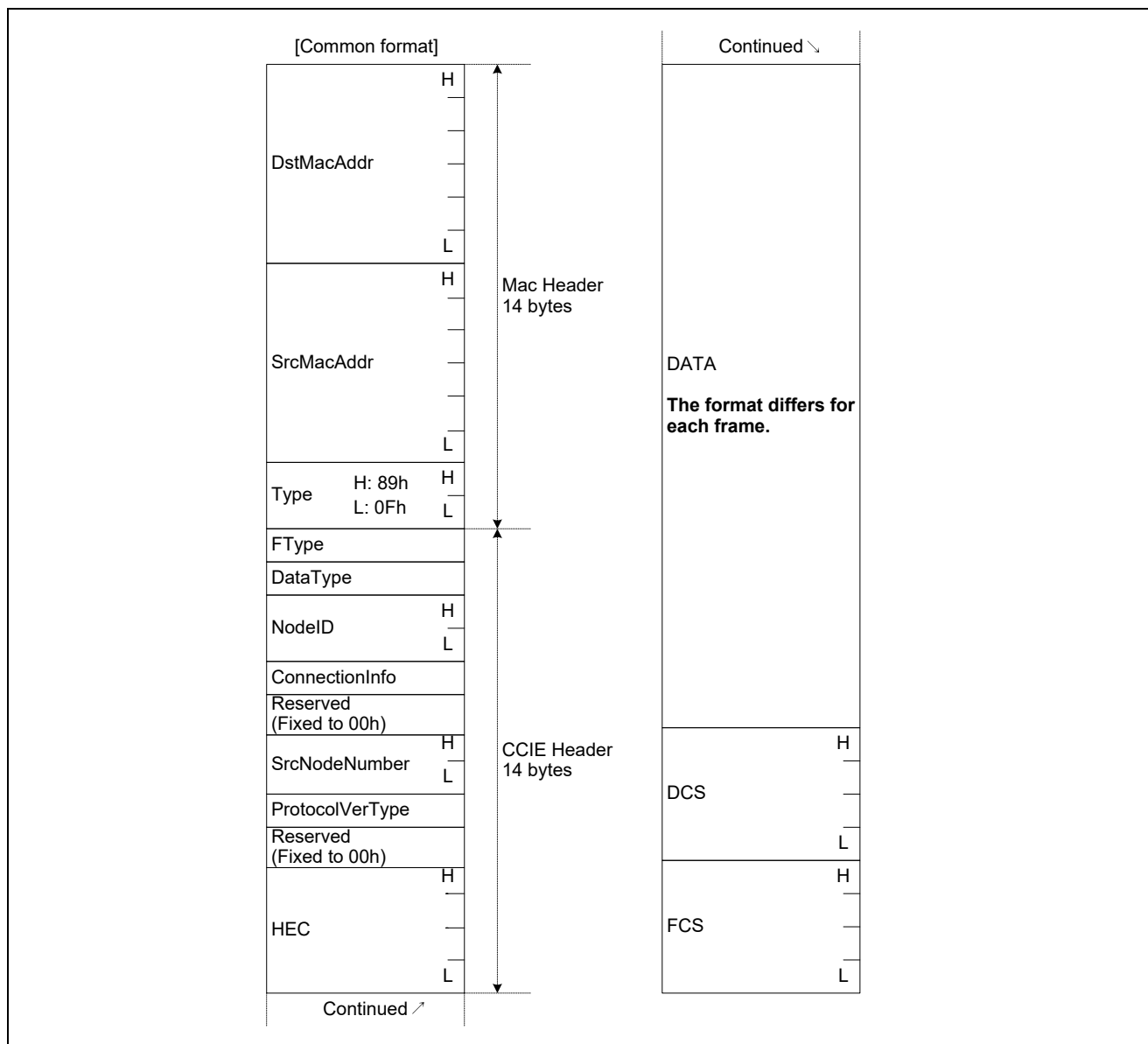
Figure 7.1 Overview of Frame Common Format
