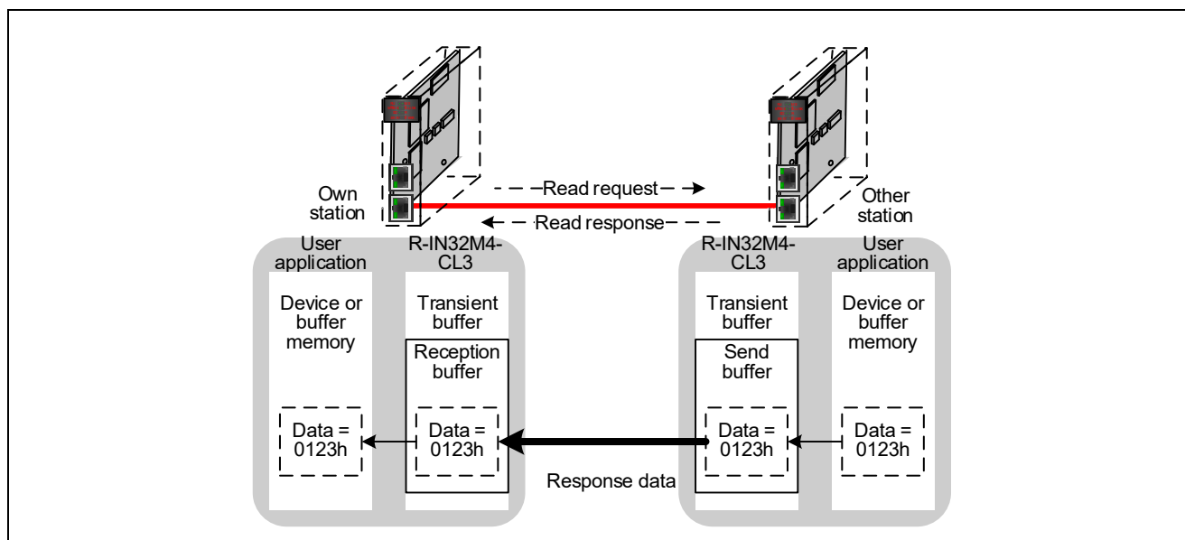
Figure 3.4 Flow of Transient Data
