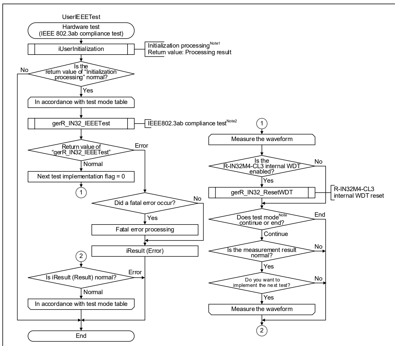
Figure 4.40 Flowchart for Hardware Test (IEEE802.3ab Compliance Test)
