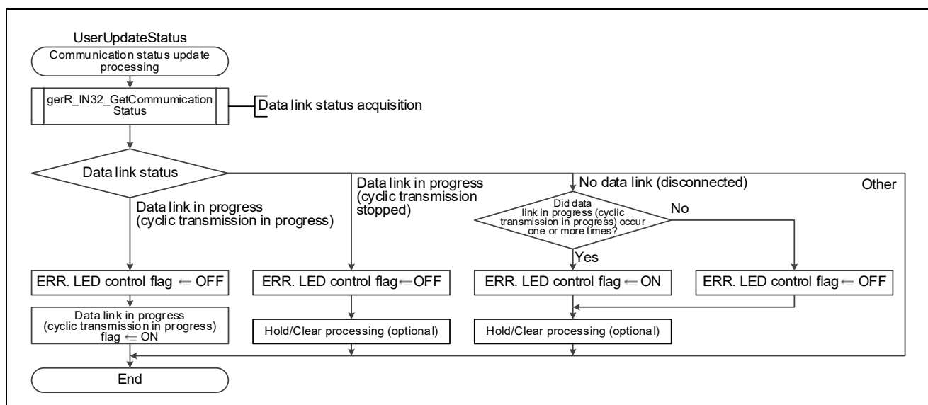
Figure 4.10 Flowchart for Communication Status Update Processing
