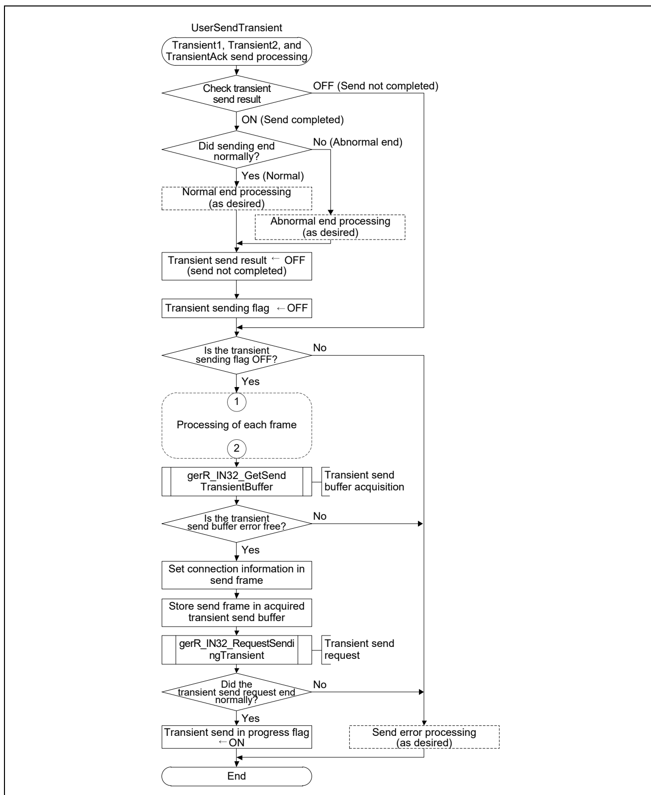
Figure 4.30 Flowchart for Transient1, Transient2, and TransientAck Send Processing (1/2)
