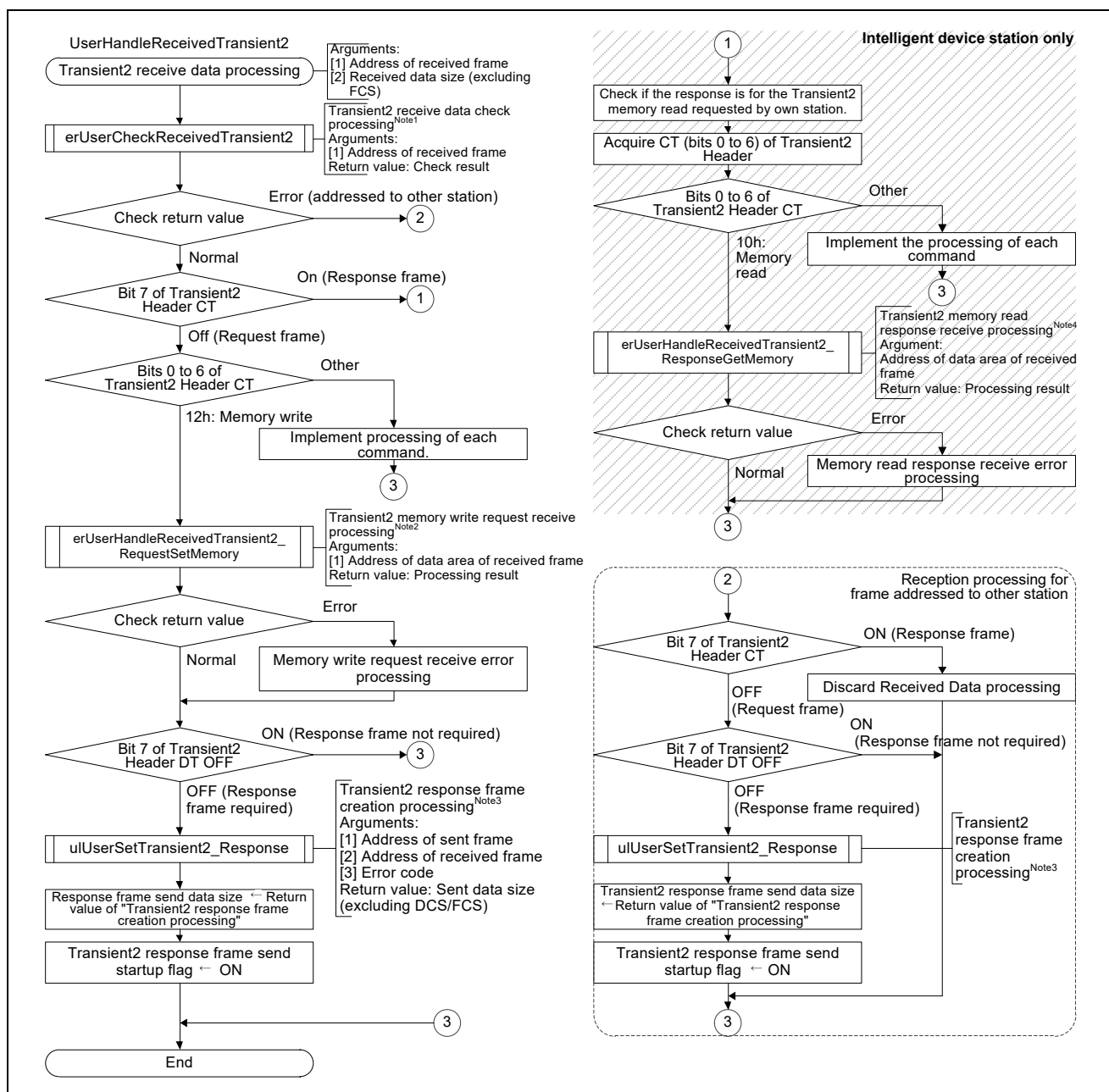
Figure 4.24 Flowchart for Transient2 Receive Data Processing
