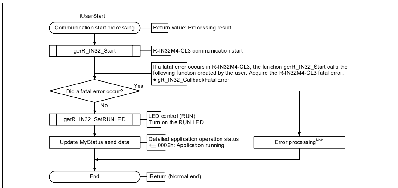
Figure 4.3 Flowchart for Communication Start Processing
