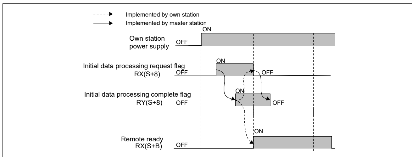
Figure 6.2 Timing Chart: Initial Data Processing Request/Complete Flag
