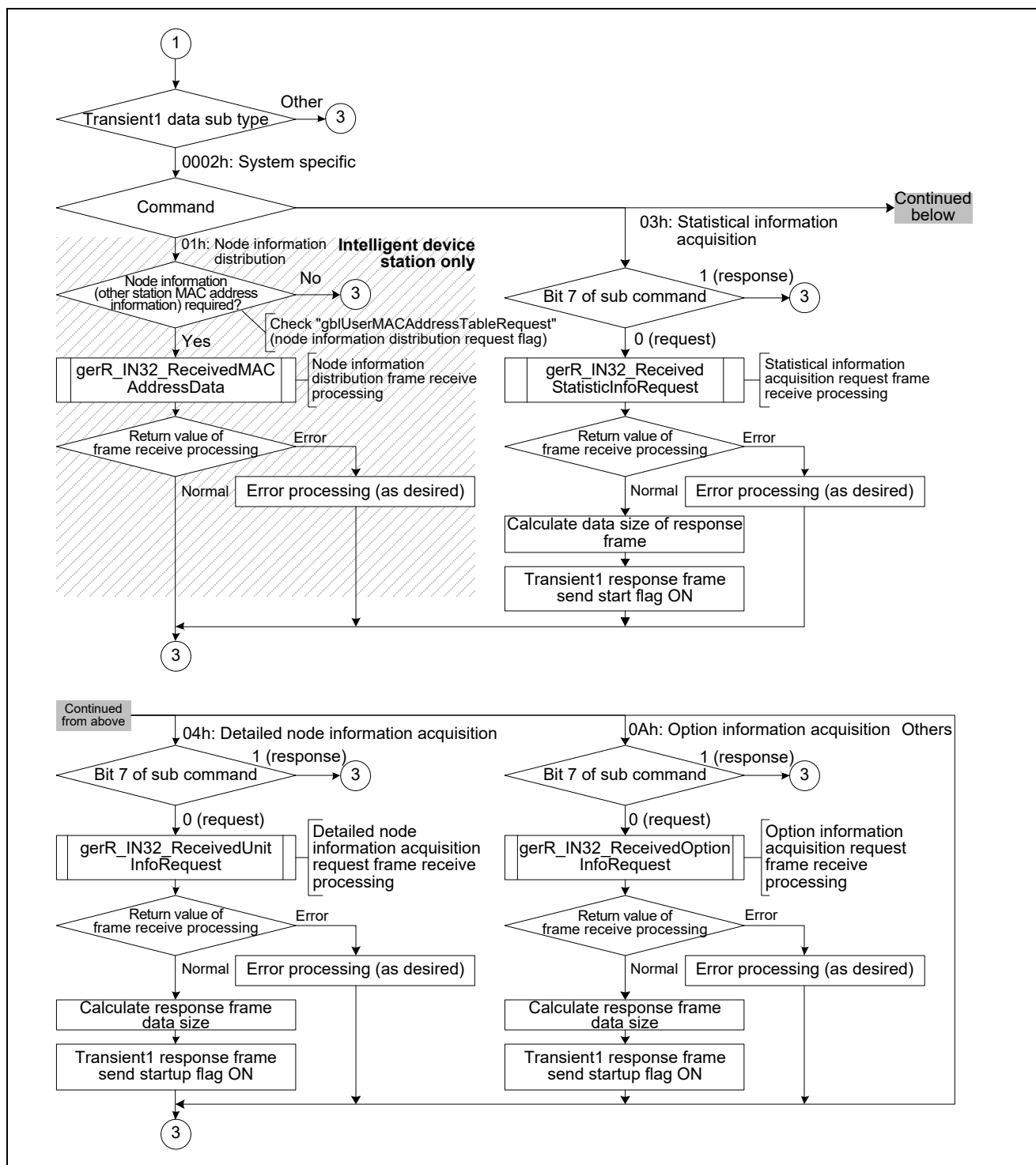
Figure 4.17 Flowchart for Transient1 Receive Data Processing (2/4)
