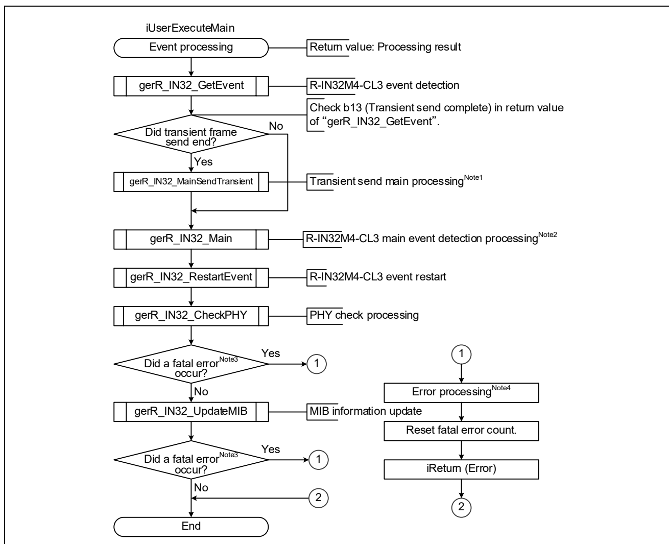
Figure 4.6 Flowchart for Event Processing
