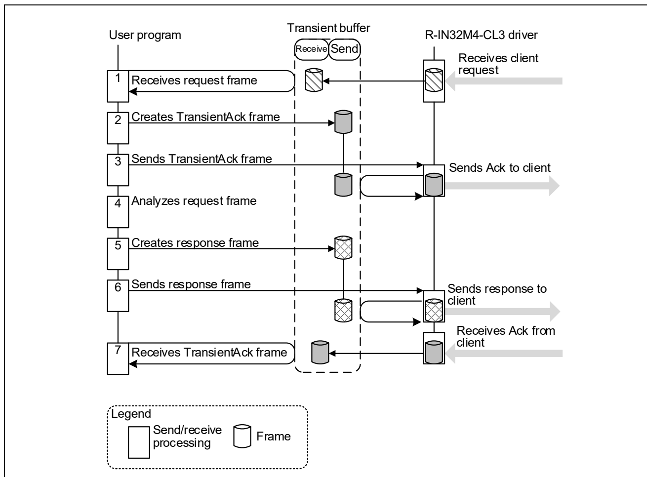
Figure 4.14 Server Processing Procedure
