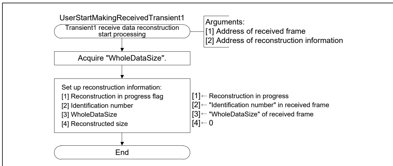
Figure 4.20 Flowchart for Transient1 Receive Data Reconstruction Start Processing
