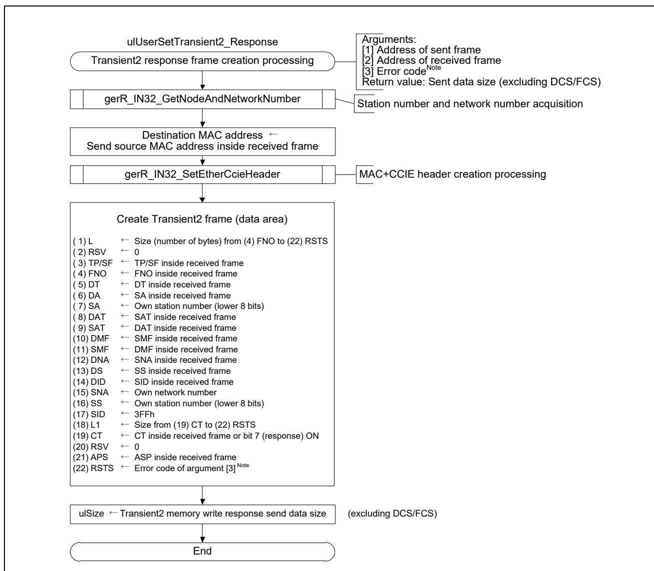
Figure 4.27 Flowchart for Transient2 Response Frame Creation Processing
