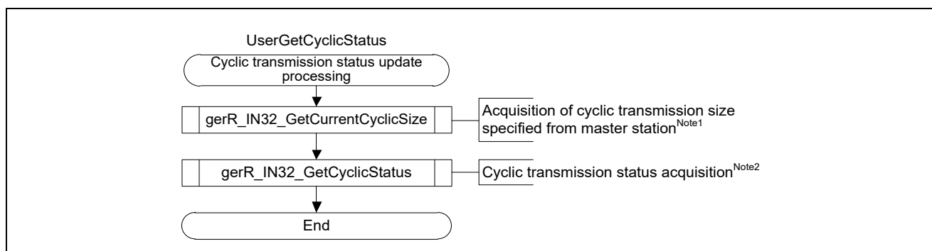
Figure 4.12 Flowchart for Cyclic Transmission Status Update Processing
