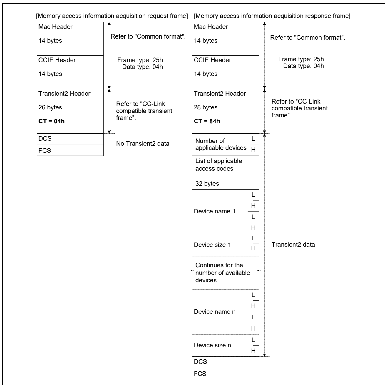
Figure 7.6 Overview of Memory Access Information Acquisition Frame Format
