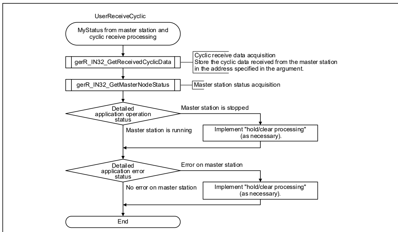
Figure 4.7 Flowchart for MyStatus from Master Station and Cyclic Receive Processing
