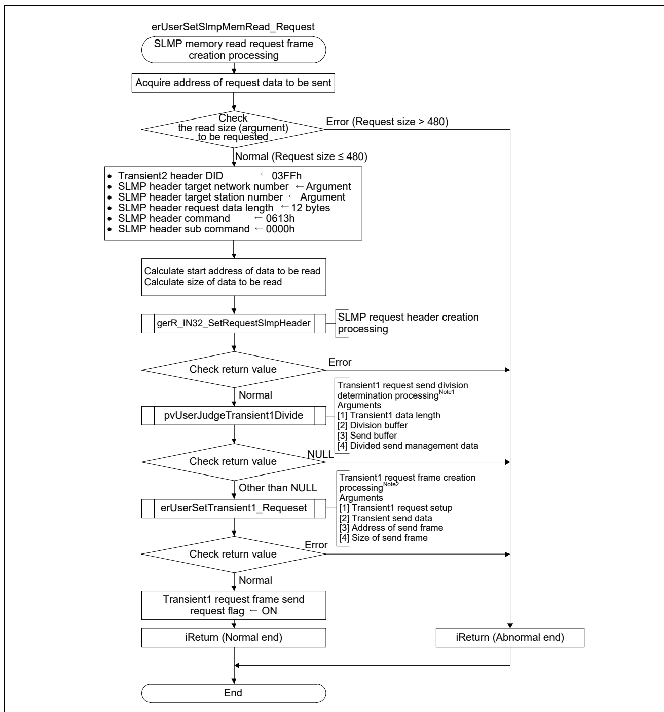
Figure 4.33 Flowchart for SLMP Memory Read Request Frame Creation Processing
