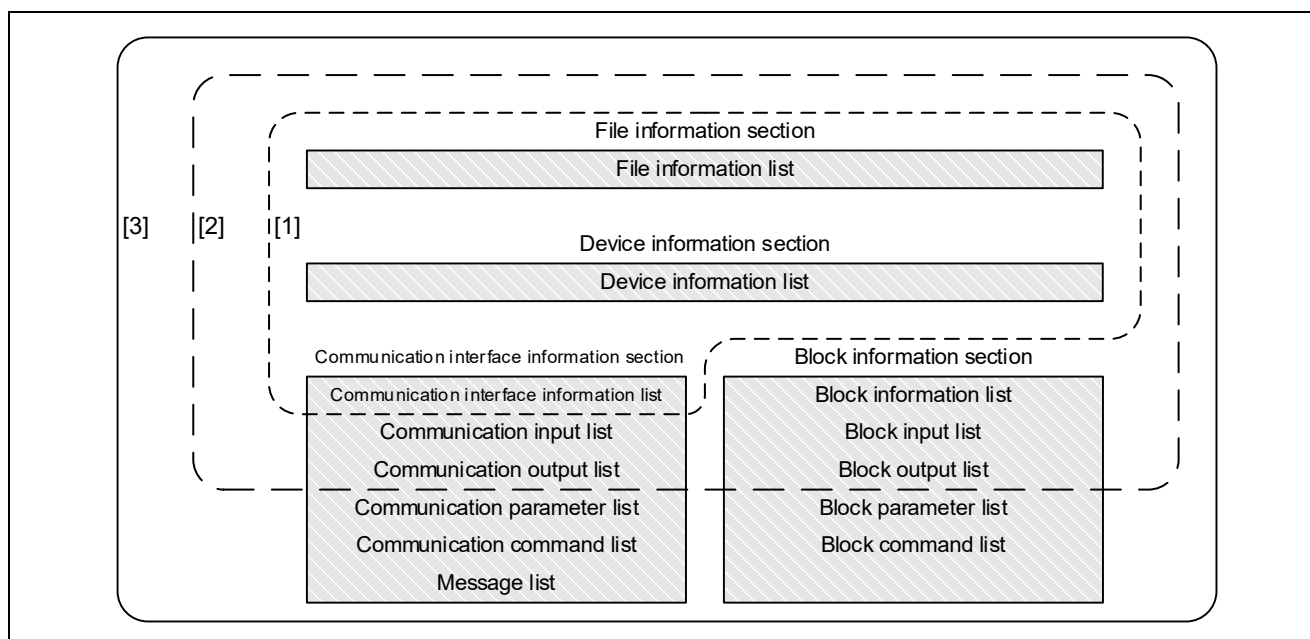
Figure 2.3 CSP+ File Section Configuration
