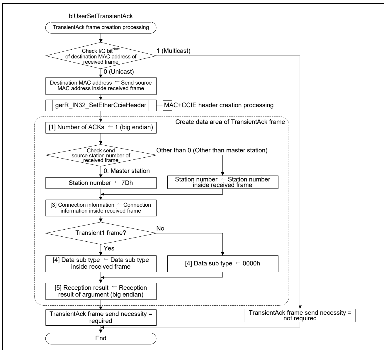
Figure 4.29 Flowchart for TransientAck Frame Creation Processing
