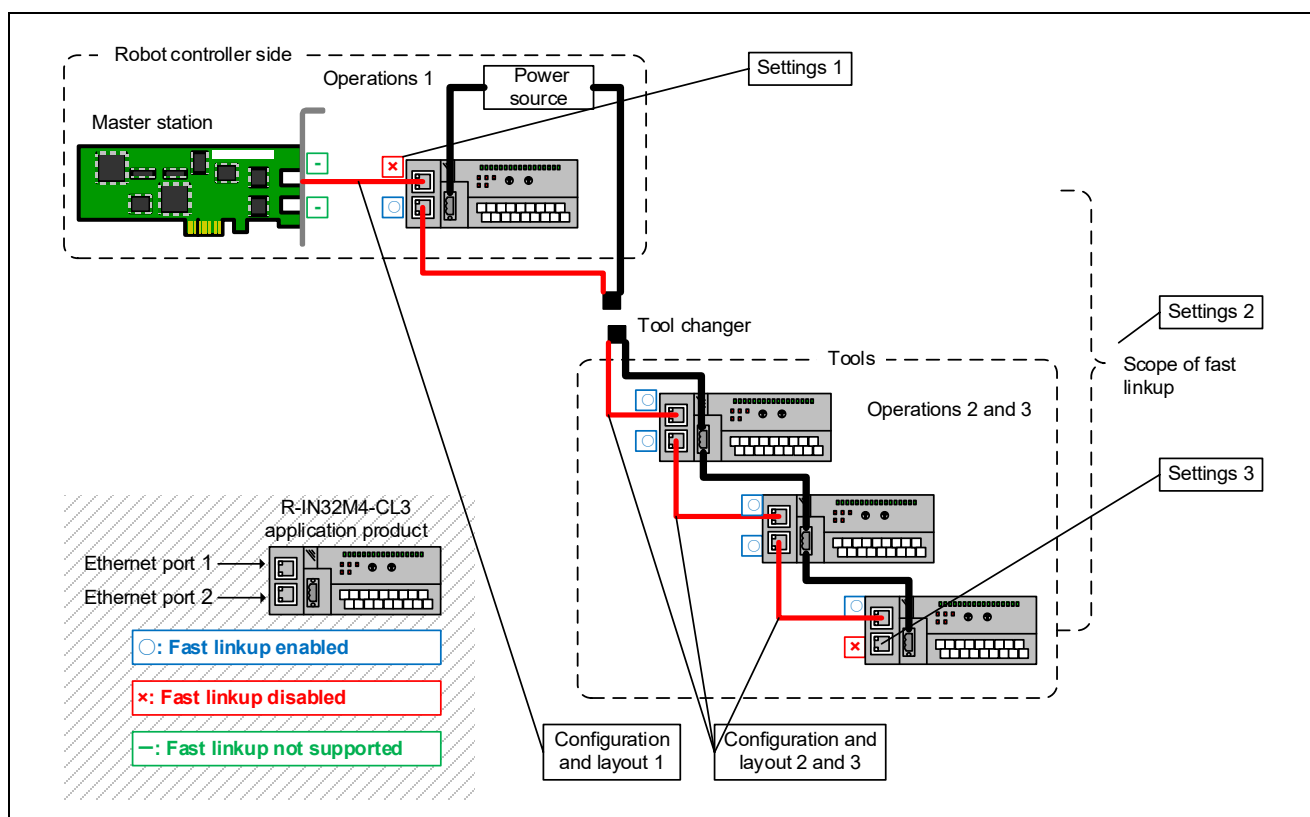
Figure 3.2 System Configuration with Fast Linkup (for an Industrial Robot Arm)
