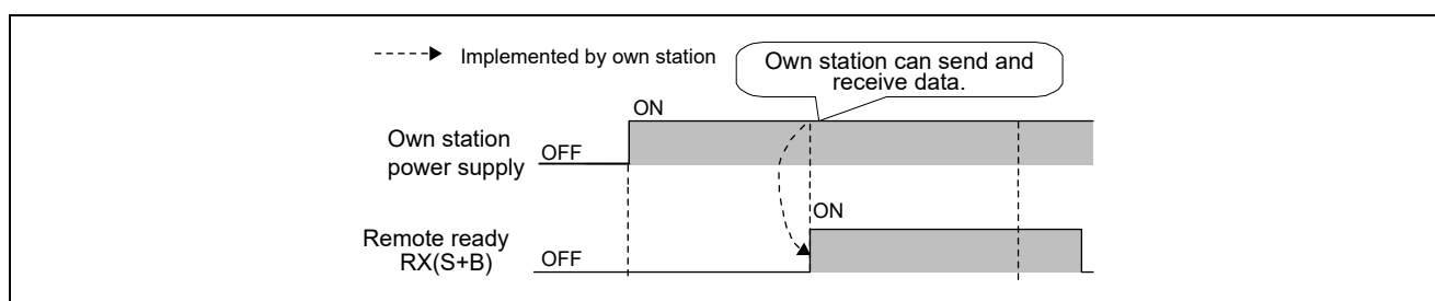
Figure 6.1 Timing Chart: Remote Ready
