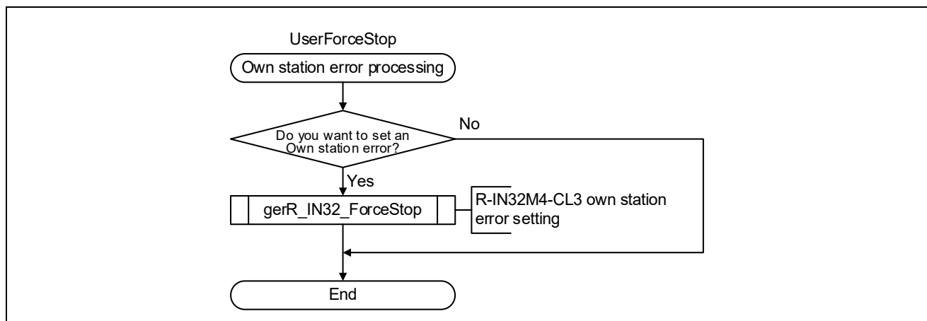
Figure 4.4 Flowchart for Own Station Error Processing
