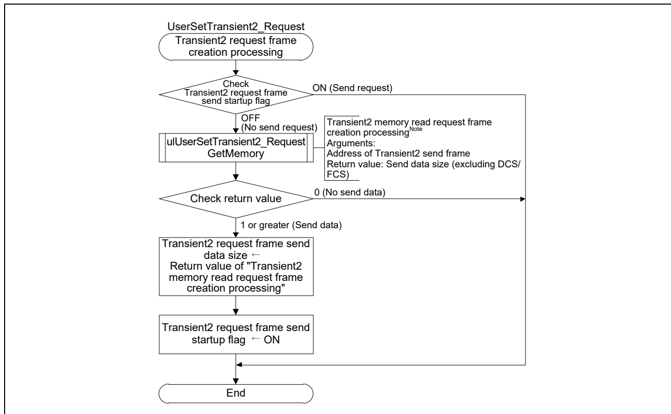
Figure 4.37 Flowchart for Transient2 Request Frame Creation Processing
