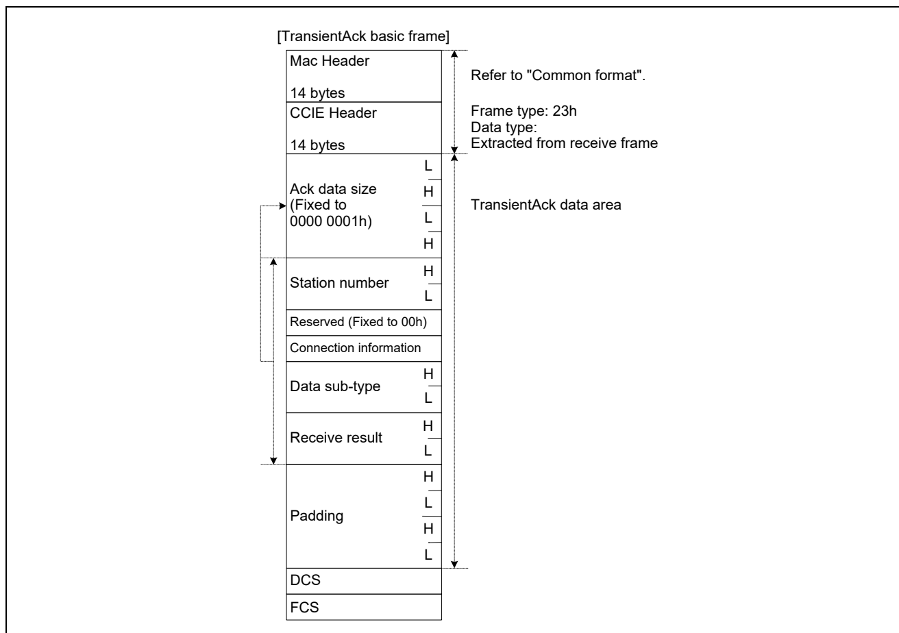
Figure 7.17 Overview of TransientAck Frame Format
