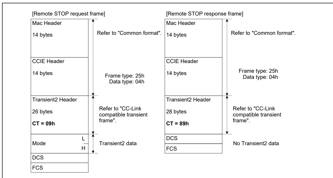
Figure 7.9 Overview of Remote STOP Frame Format
