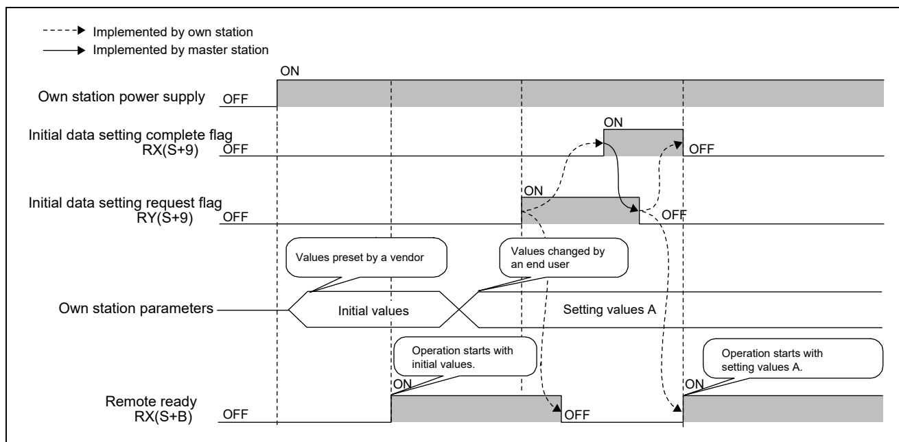
Figure 6.3 Timing Chart: Initial Data Setting Complete/Request Flag
