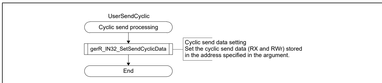
Figure 4.9 Flowchart for Cyclic Send Processing
