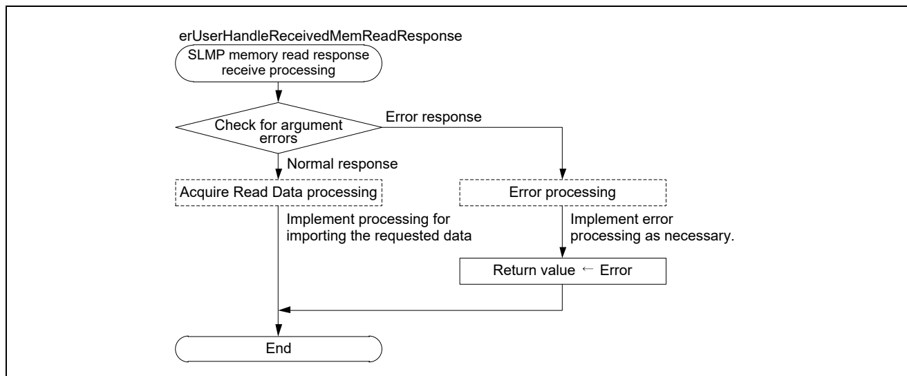
Figure 4.36 Flowchart for SLMP Memory Read Response Receive Processing
