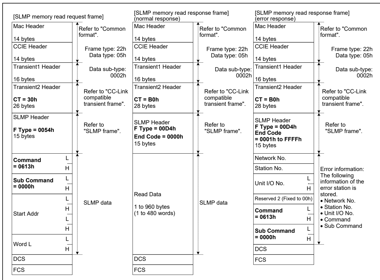
Figure 7.15 Overview of SLMP Memory Read Frame Format
