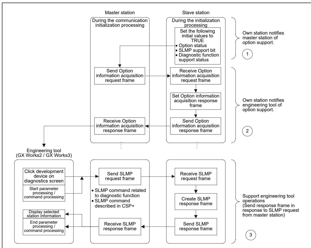
Figure 4.18 SLMP Request Reception Procedure
