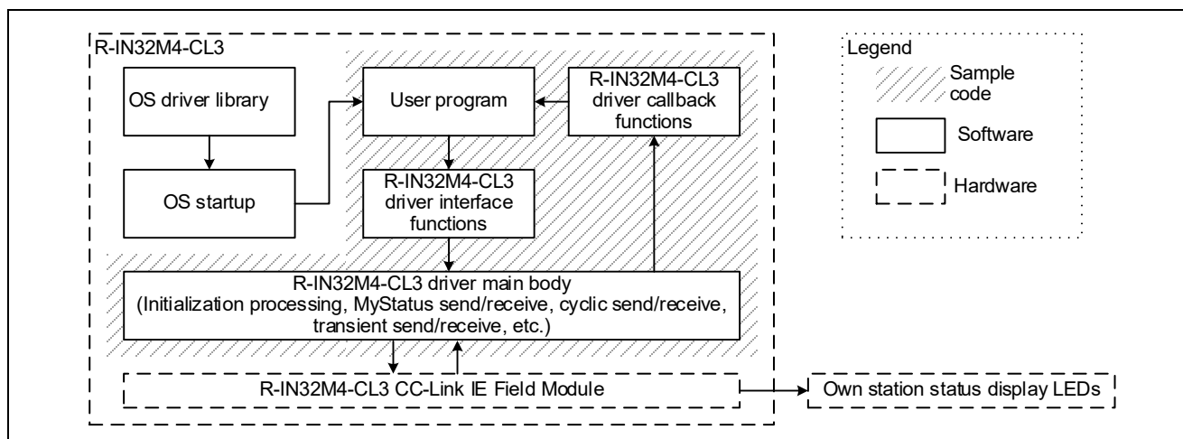
Figure 1.1 Software Configuration Overview
