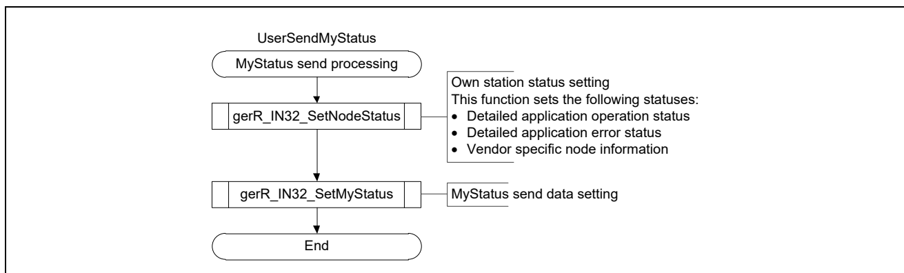
Figure 4.8 Flowchart for MyStatus Send Processing
