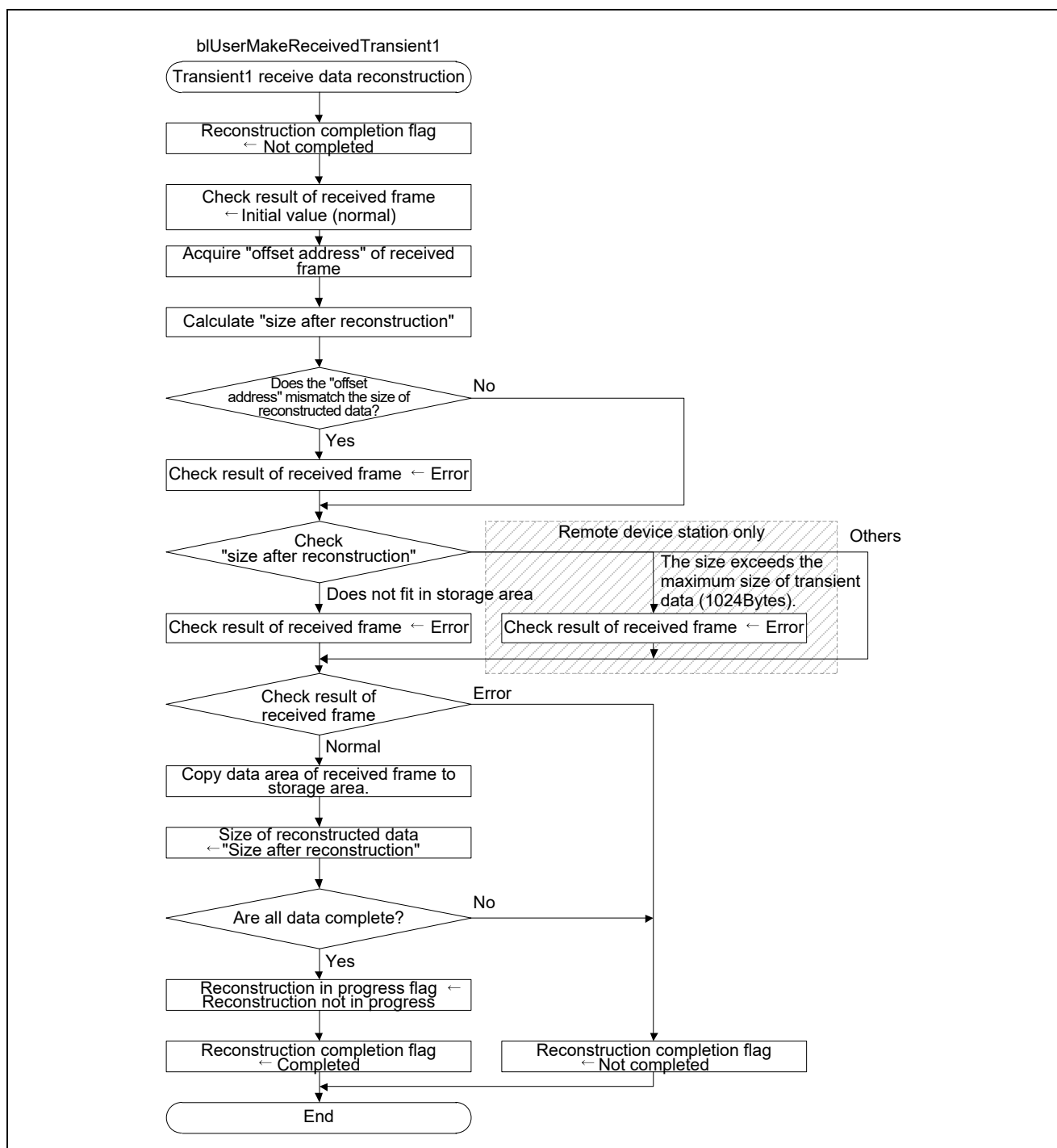
Figure 4.21 Flowchart for Transient1 Receive Data Reconstruction Processing
