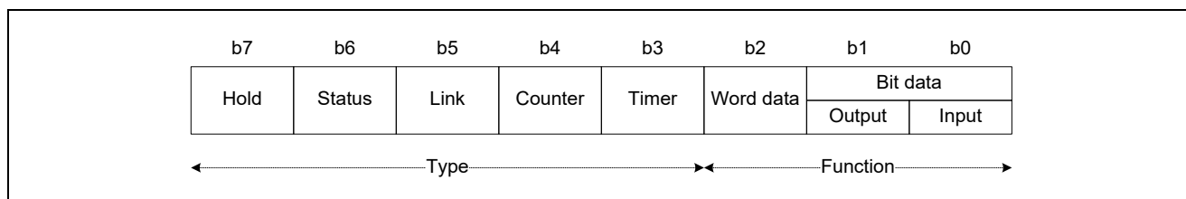
Figure 7.12 Access Code Definition
