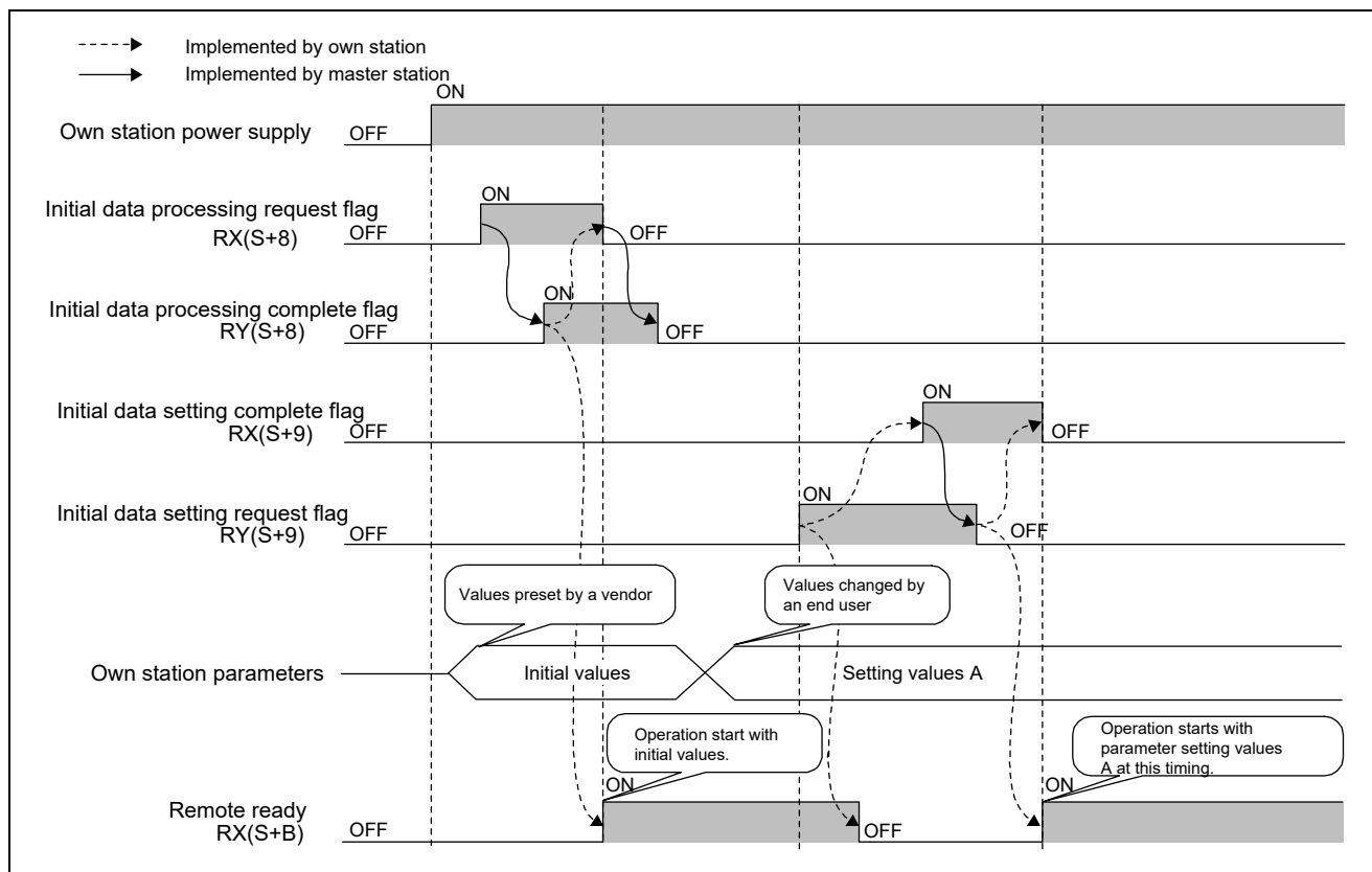
Figure 6.4 Timing Chart: Initial Data Processing and Setting
