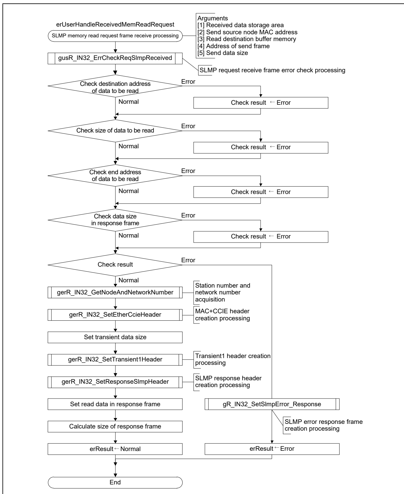
Figure 4.22 Flowchart for SLMP Memory Read Request Frame Receive Processing
