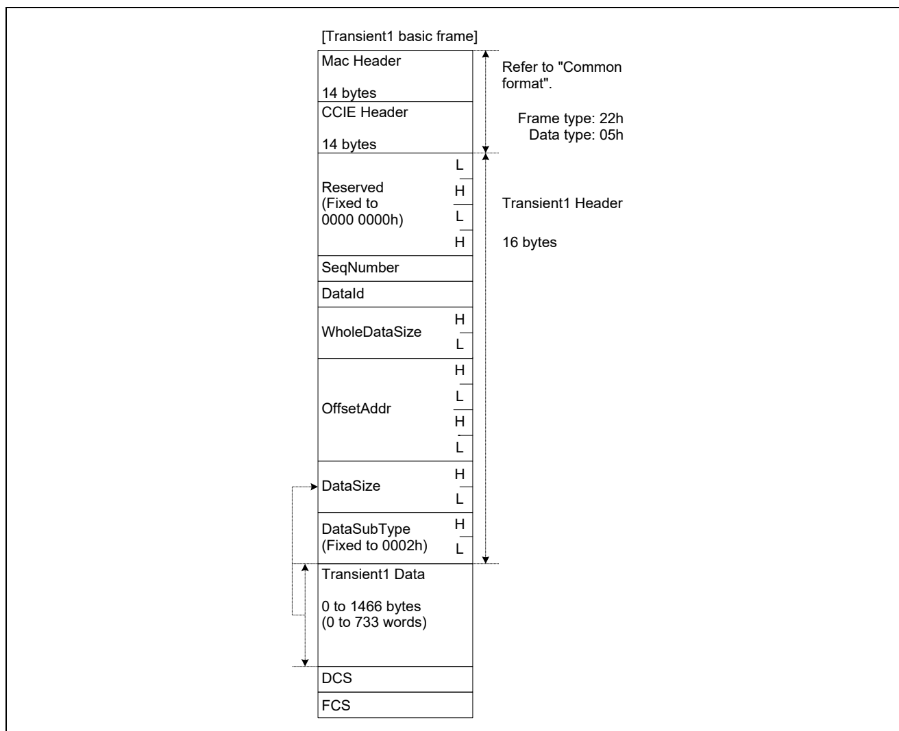
Figure 7.2 Overview of Transient1 Frame Basic Format
