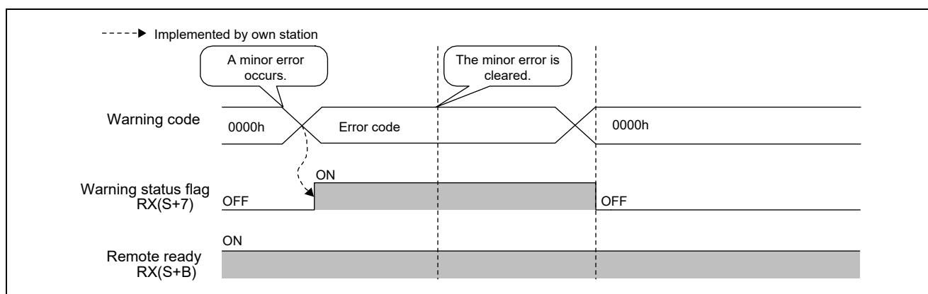
Figure 6.6 Timing Chart: Warning Status Flag
