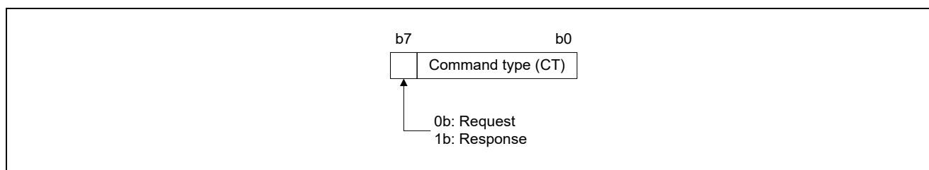
Figure 7.5 Data Structure of CC-Link Compatible Transient Command Type
