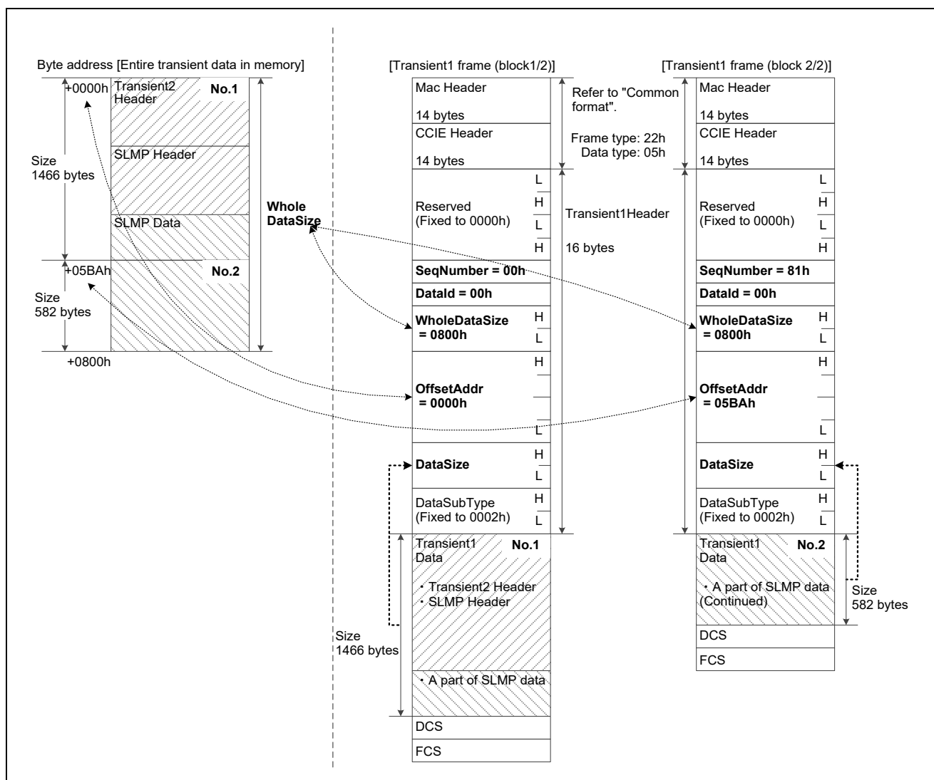
Figure 7.3 Example of Transient1 Frame Division
