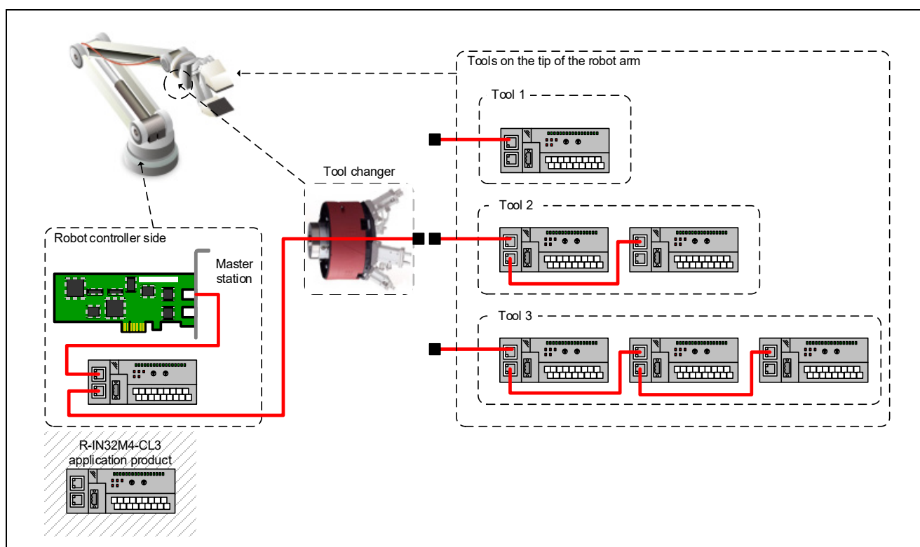
Figure 3.1 Example of Fast Linkup Usage (for an Industrial Robot Arm)
