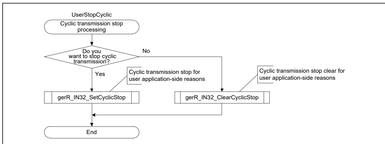
Figure 4.5 Flowchart for Cyclic Transmission Stop Processing
