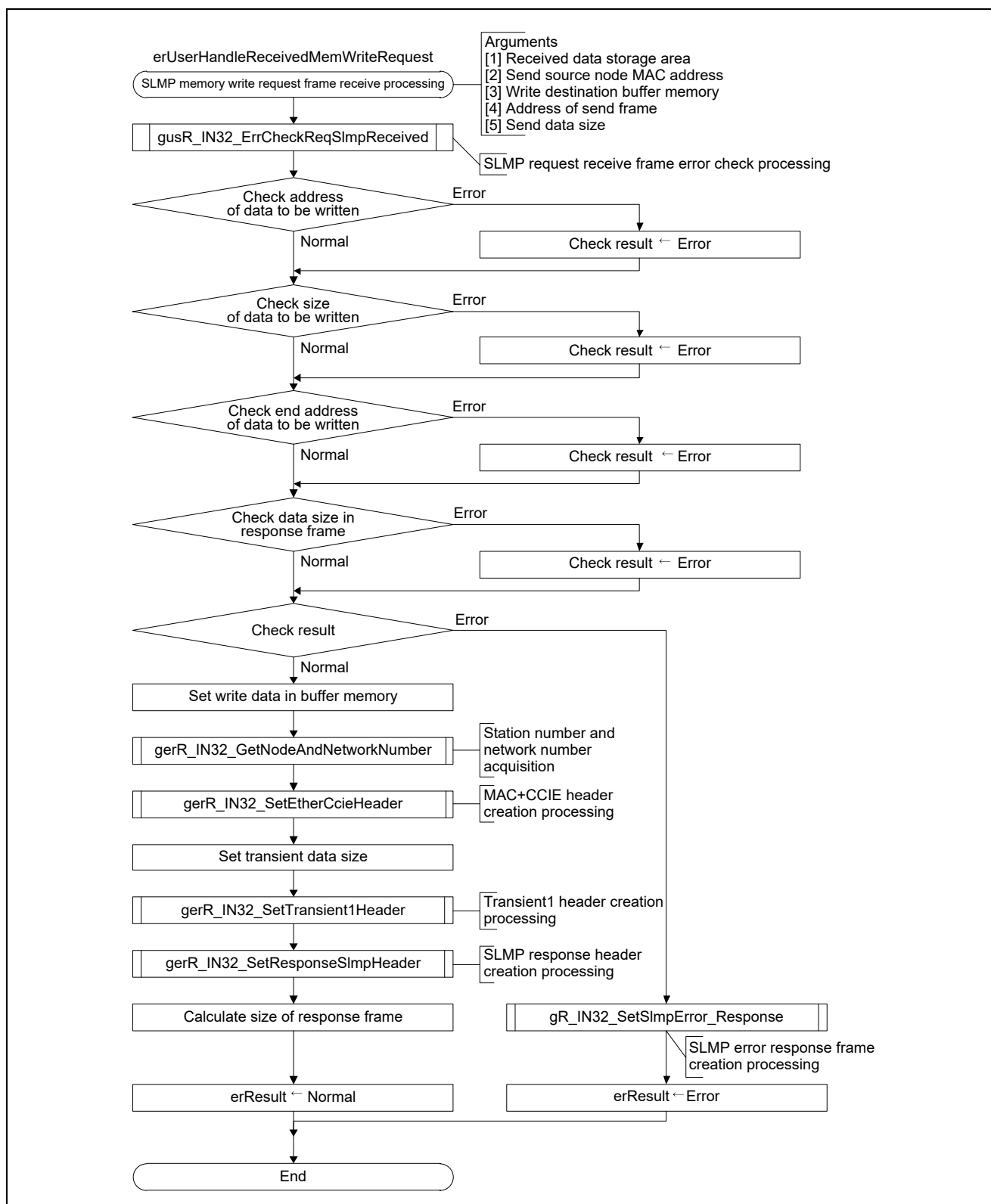
Figure 4.23 Flowchart for SLMP Memory Write Request Frame Receive Processing
