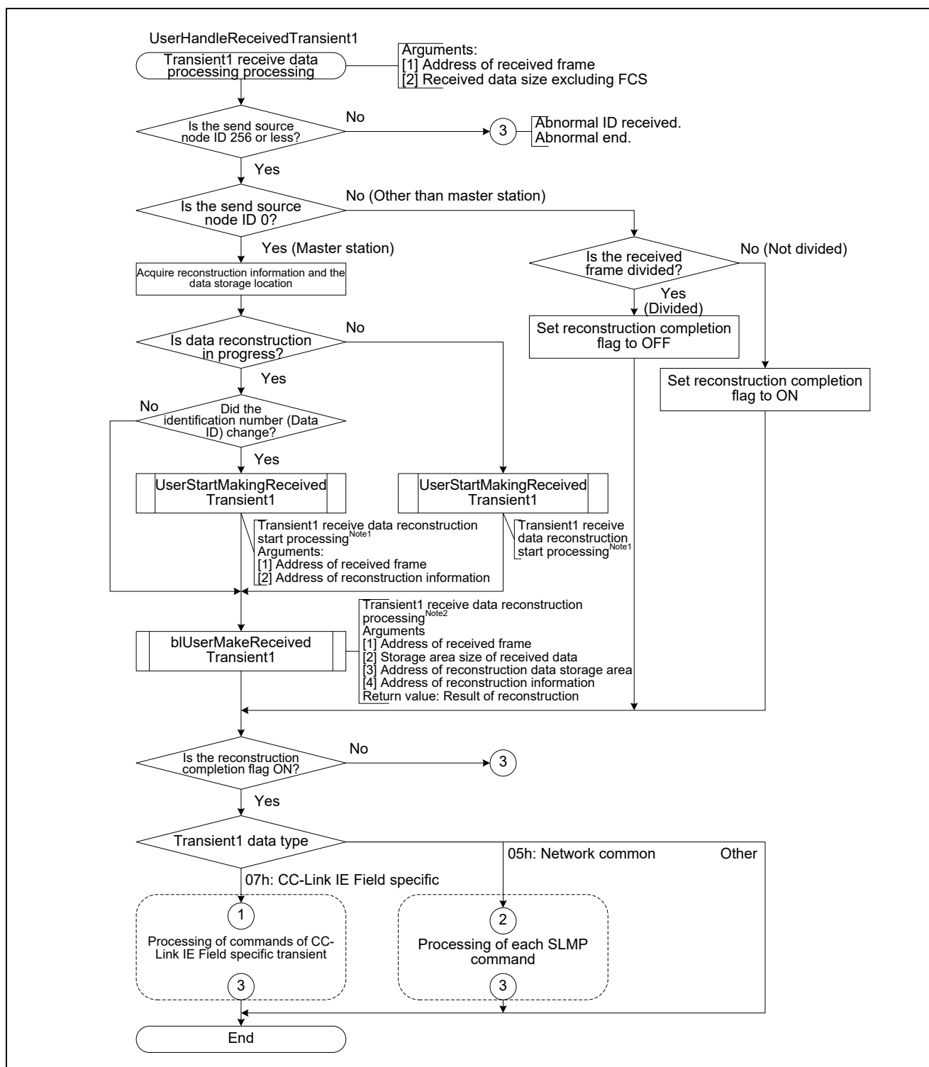
Figure 4.17 Flowchart for Transient1 Receive Data Processing (1/4)
