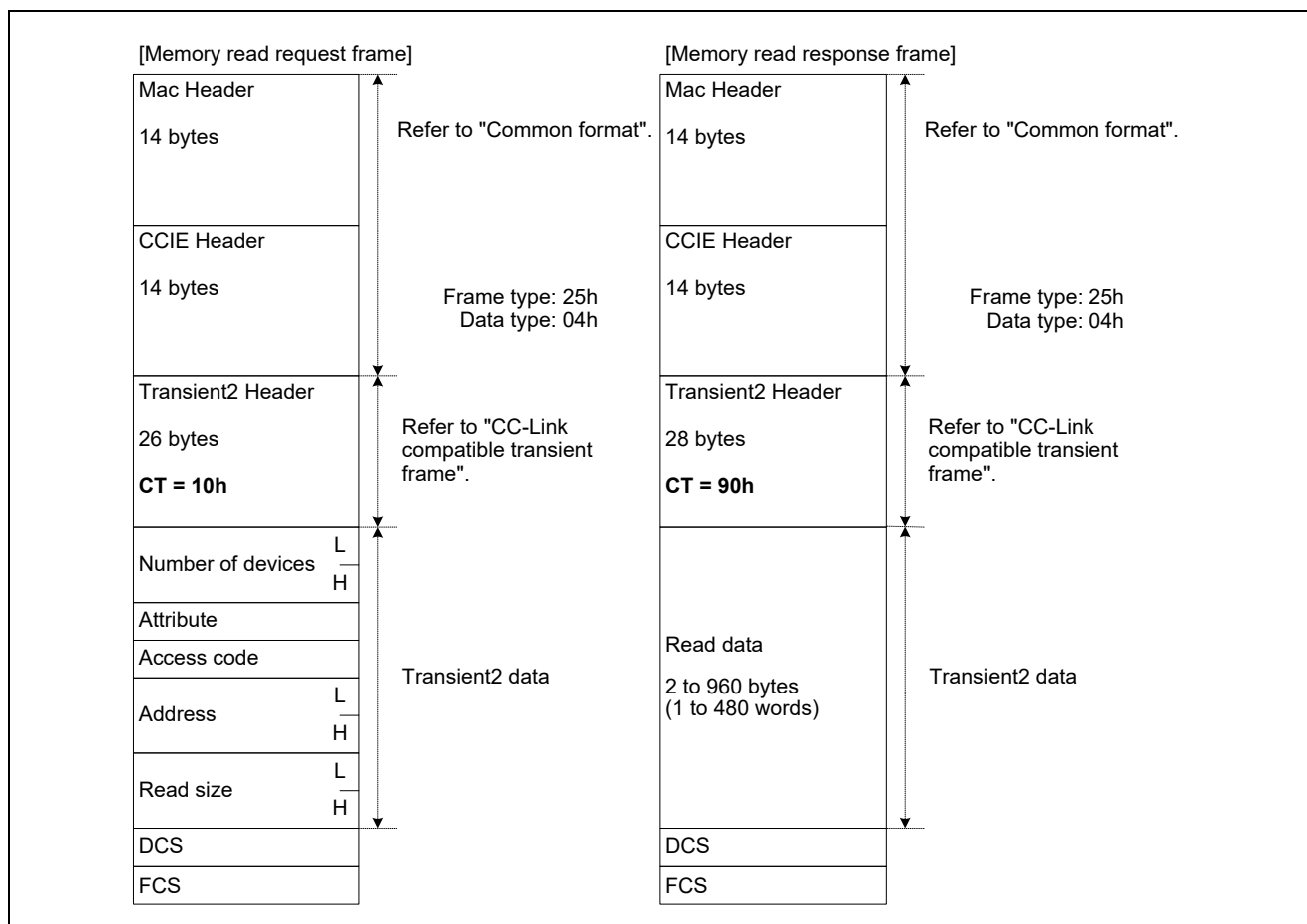
Figure 7.10 Overview of Memory Read Frame Format
