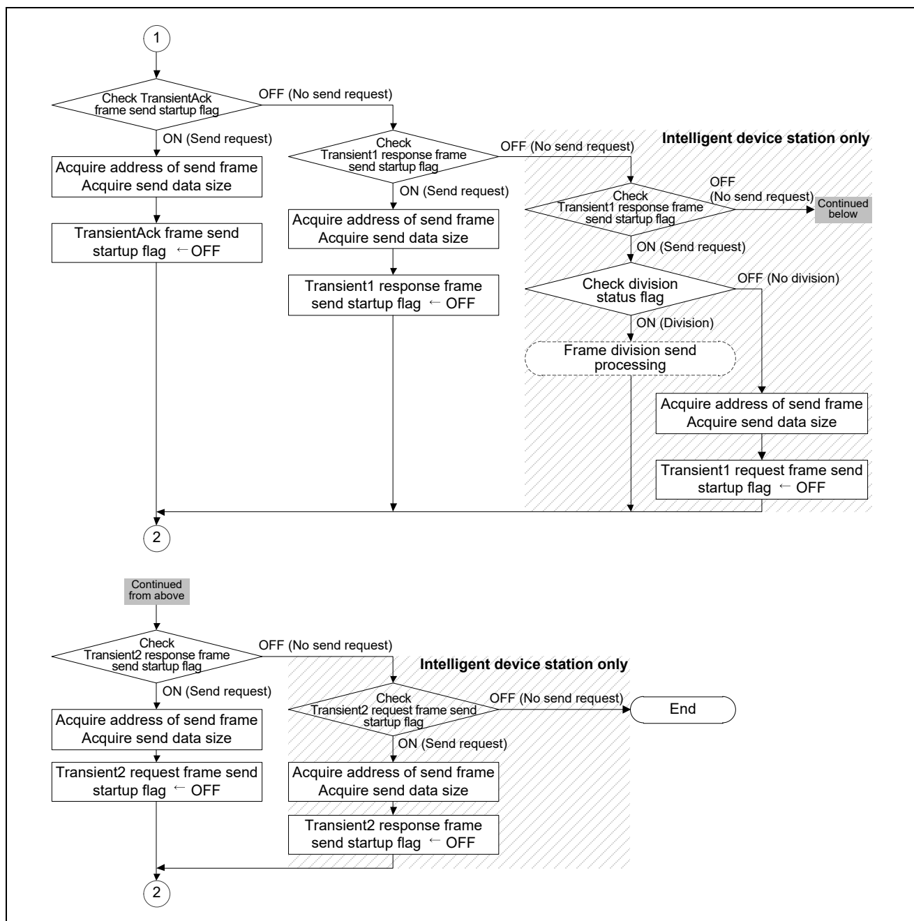
Figure 4.30 Flowchart for Transient1, Transient2, and TransientAck Send Processing (2/2)
