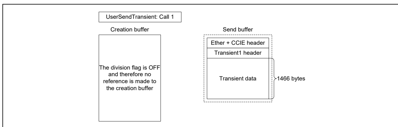
Figure 4.32 When Dividing and Transferring Transient Data Having a Size of 1466 Bytes or Less (When the Division Flag is OFF)
