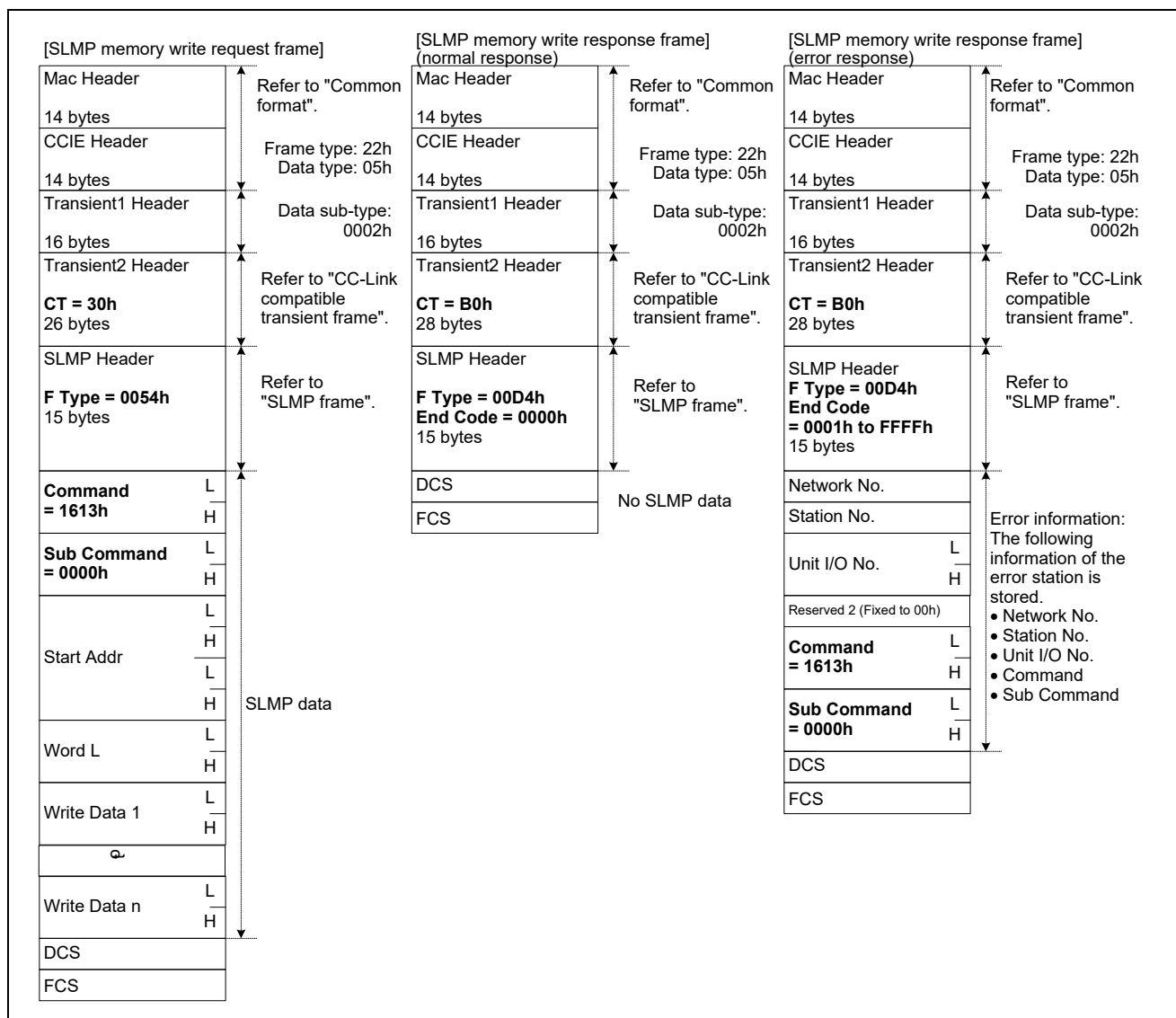
Figure 7.16 Overview of SLMP Memory Write Frame Format
