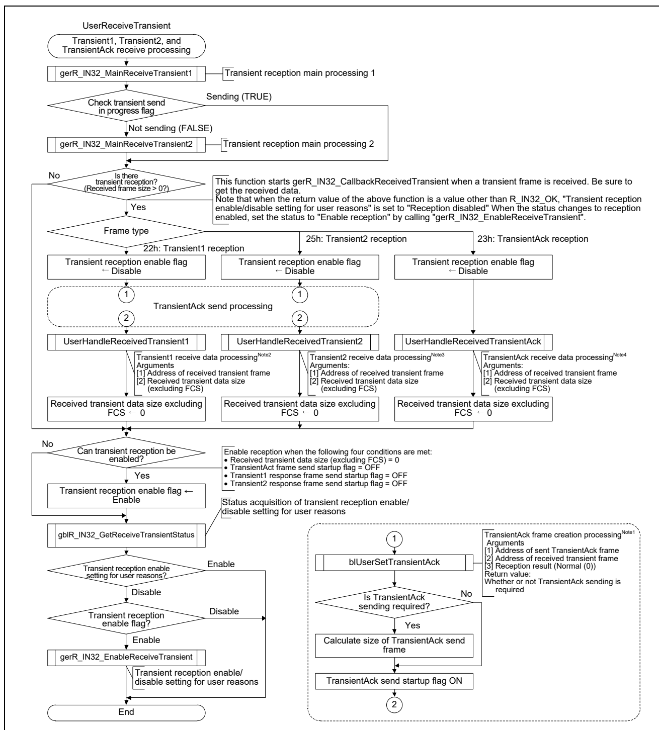
Figure 4.16 Flowchart for Transient1, Transient2, and TransientAck Receive Processing
