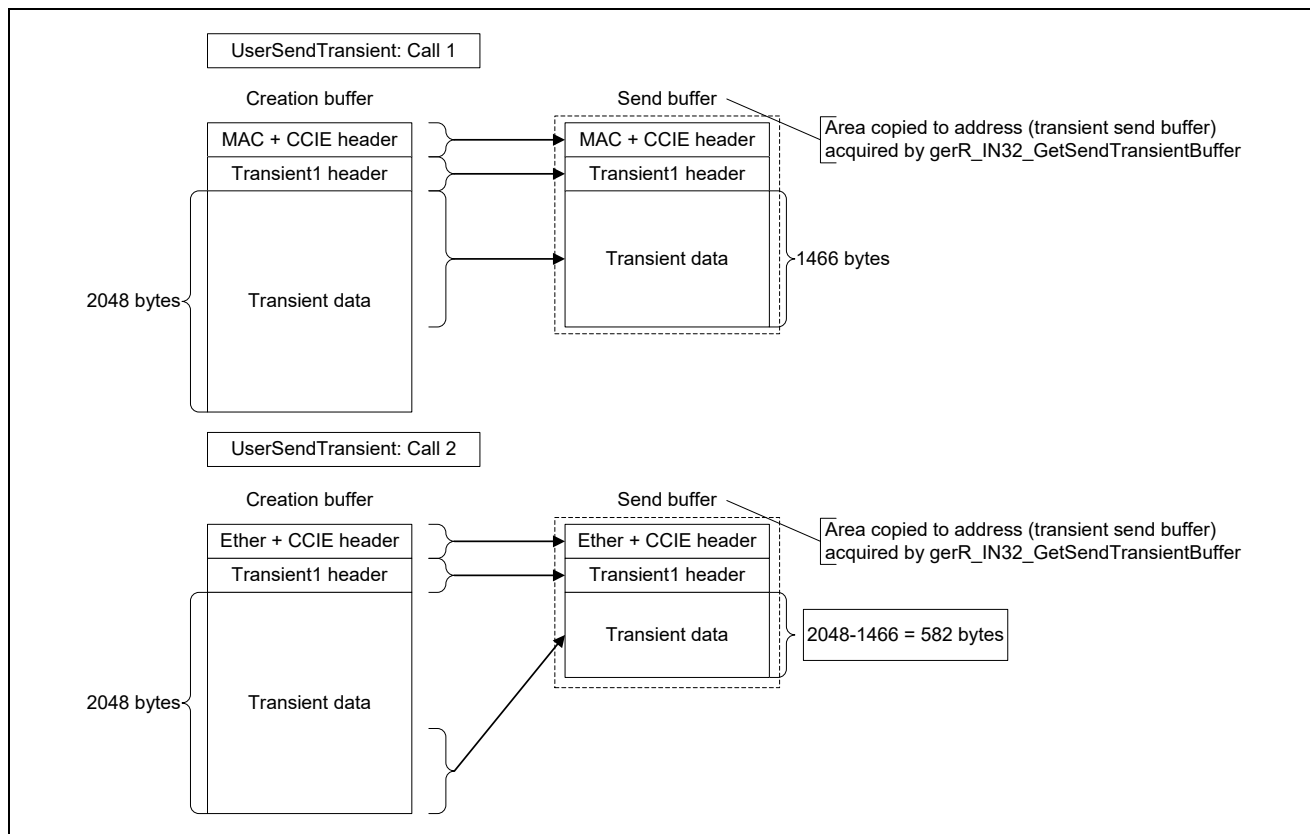
Figure 4.31 When Dividing and Transferring Transient Data Having a Size of 2048 Bytes (When the Division Flag is ON)
