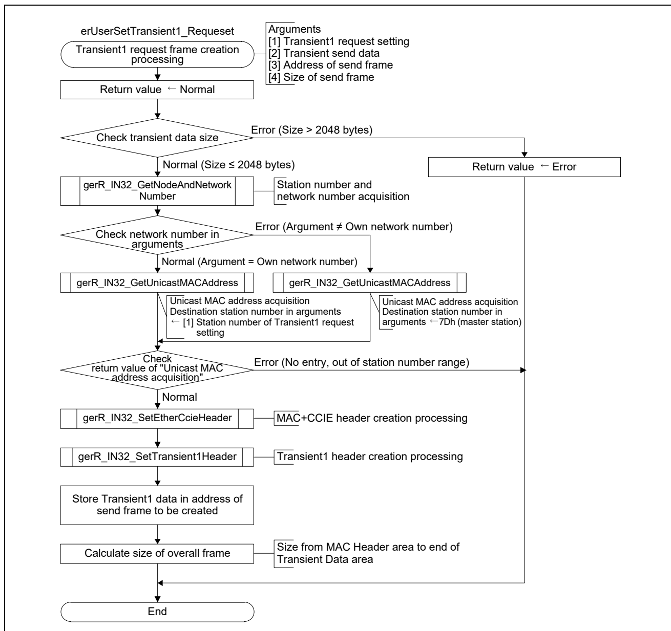
Figure 4.35 Flowchart for Transient1 Request Frame Creation Processing
