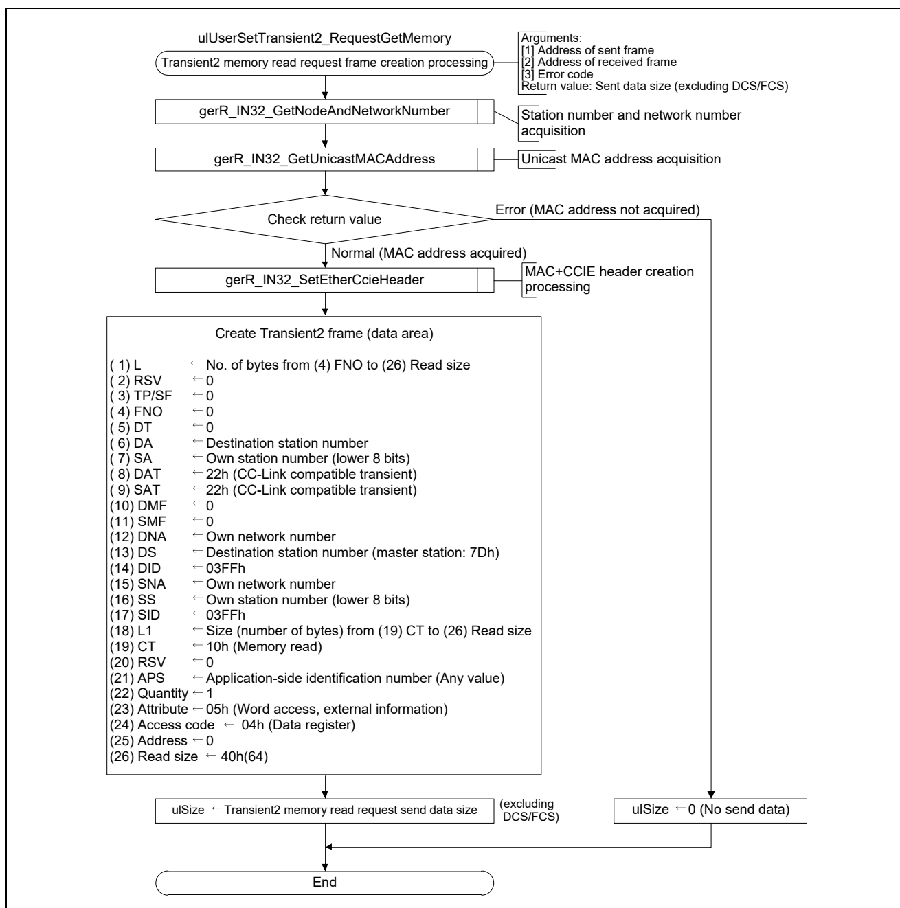
Figure 4.38 Flowchart for Transient2 Memory Read Request Frame Creation Processing
