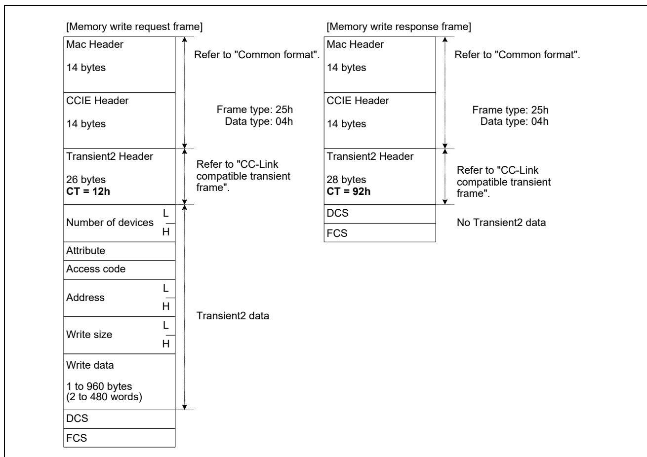
Figure 7.11 Overview of Memory Write Frame Format
