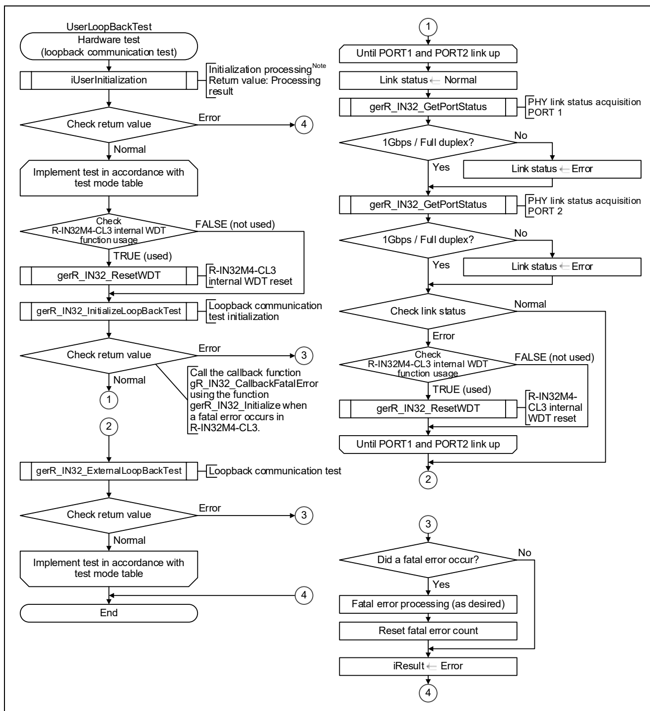
Figure 4.41 Flowchart for Hardware Test (Loopback Communication Test)
