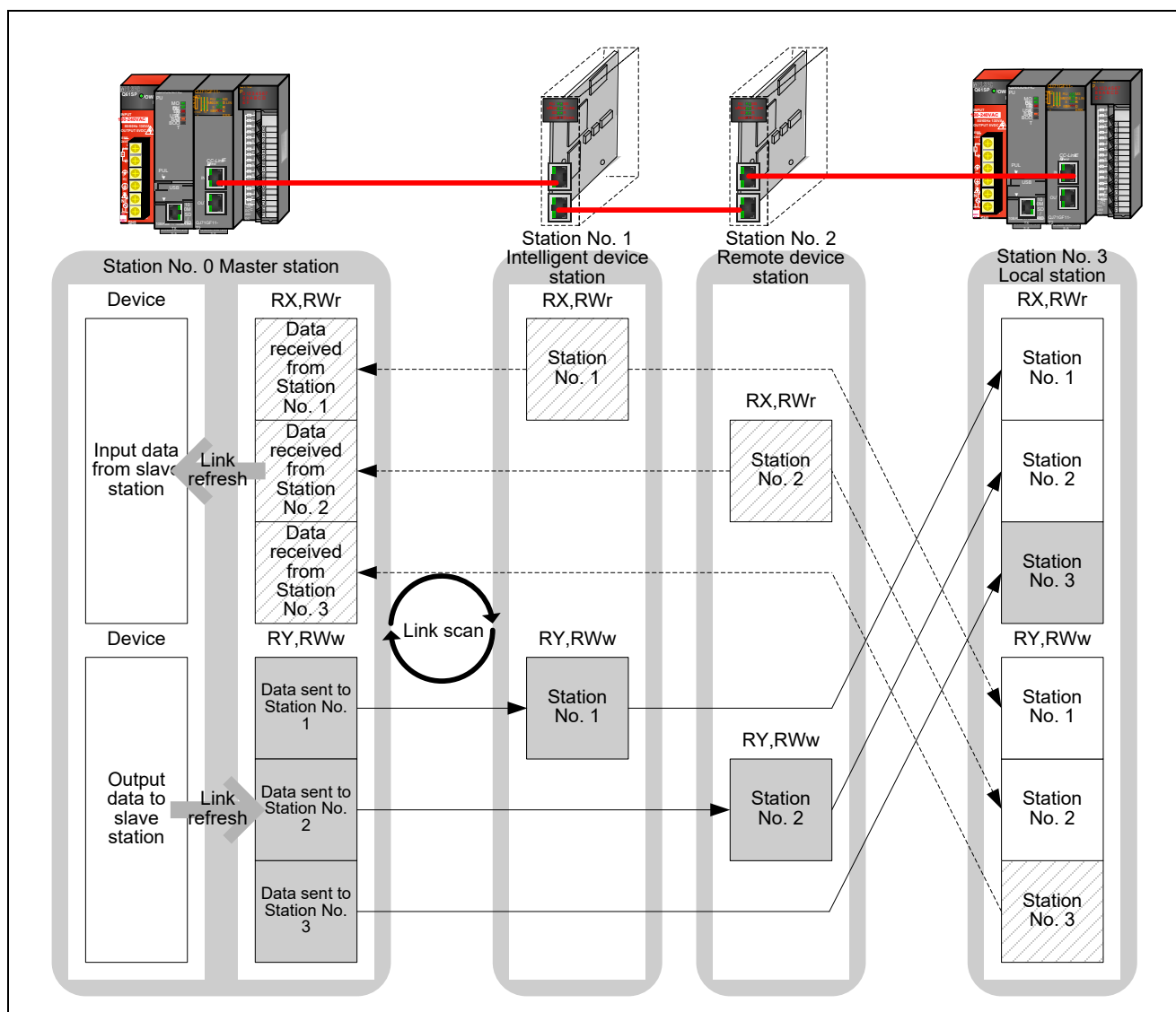
Figure 3.3 Flow of Cyclic Data
