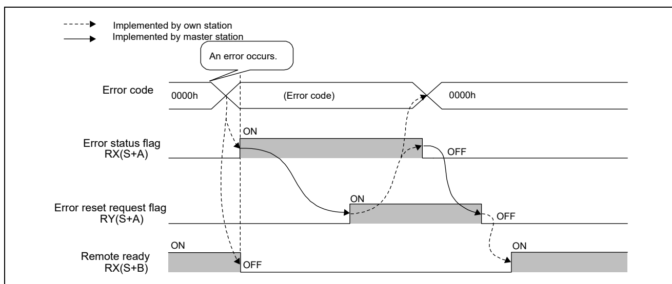
Figure 6.5 Timing Chart: Error Status Flag, Error Reset Request Flag
