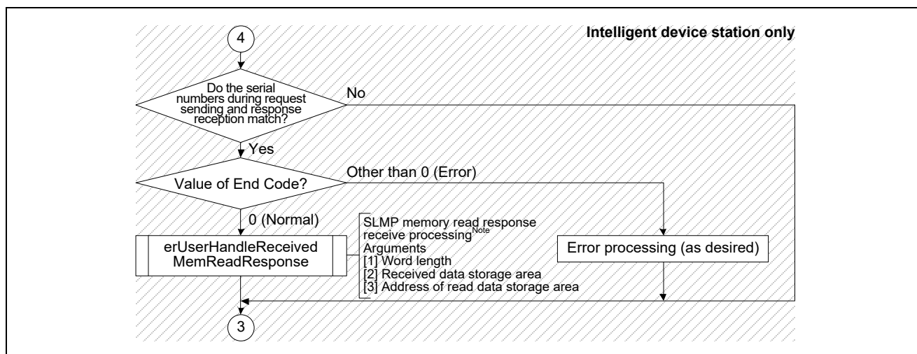
Figure 4.17 Flowchart for Transient1 Receive Data Processing (4/4)
