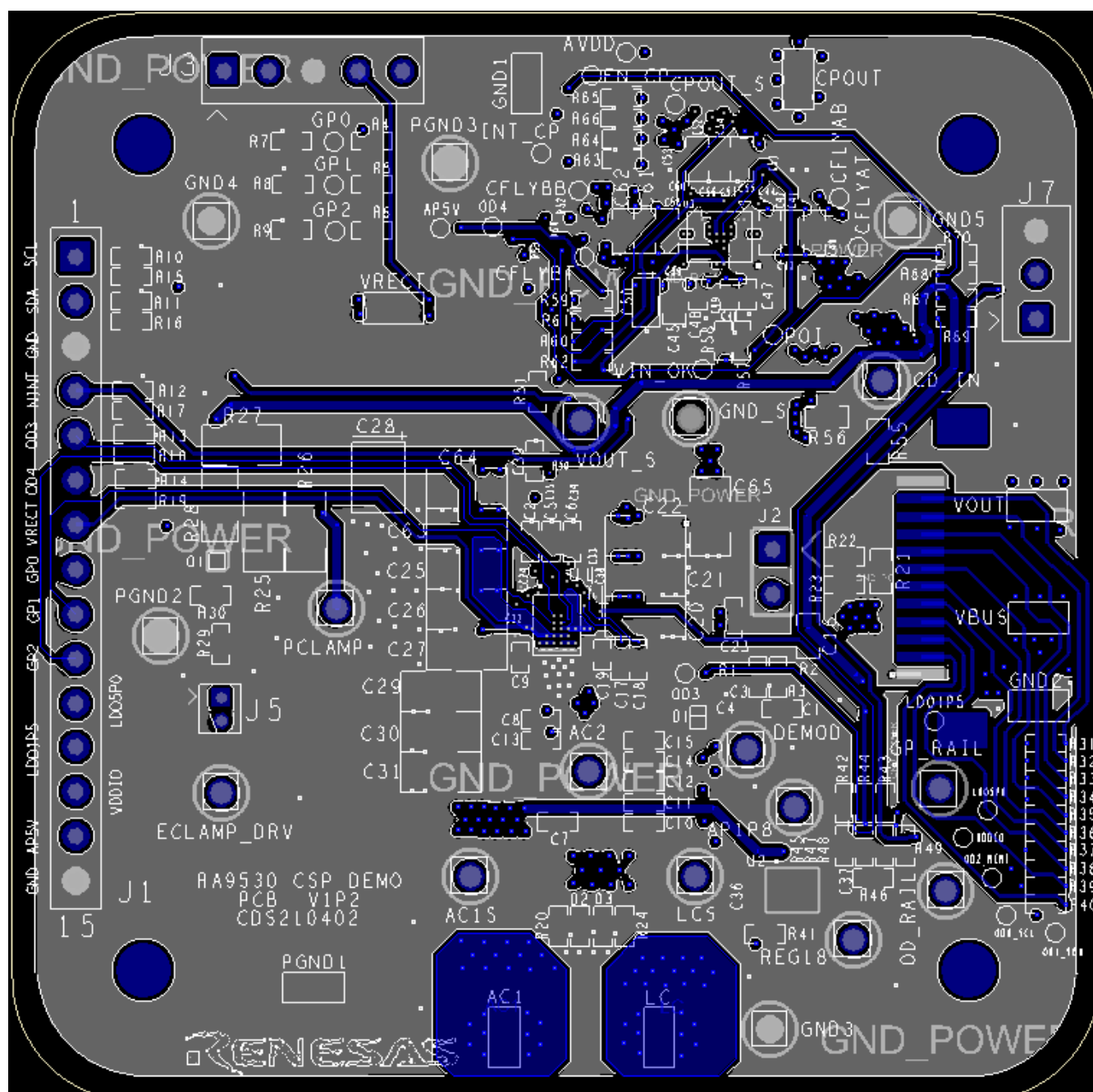
Figure 42. Bottom Layer
