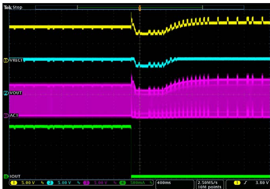
Figure 6. Load Dump
