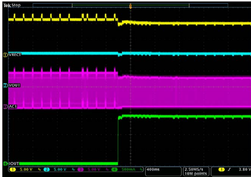
Figure 5. Load Step
