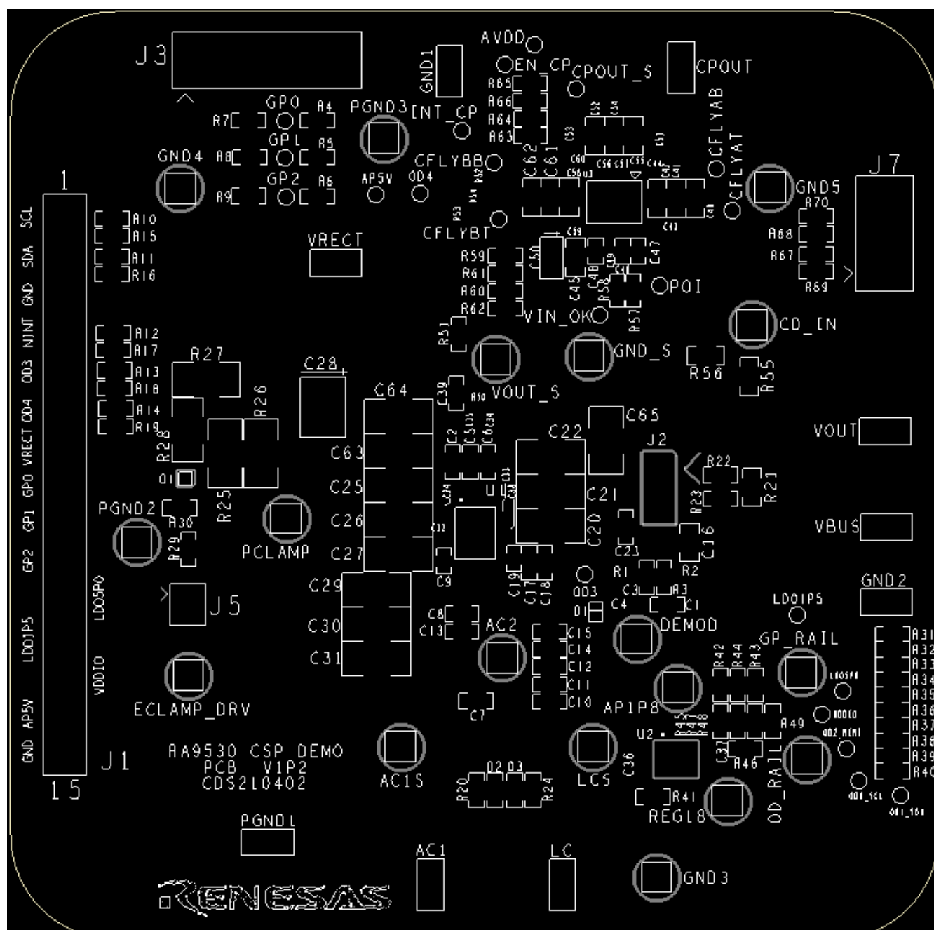
Figure 43. Assembly Drawing
