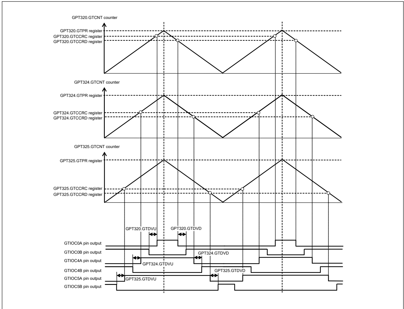
Figure 23.106 Example of 3-phase asymmetric triangle-wave complementary PWM output with automatic dead time setting
