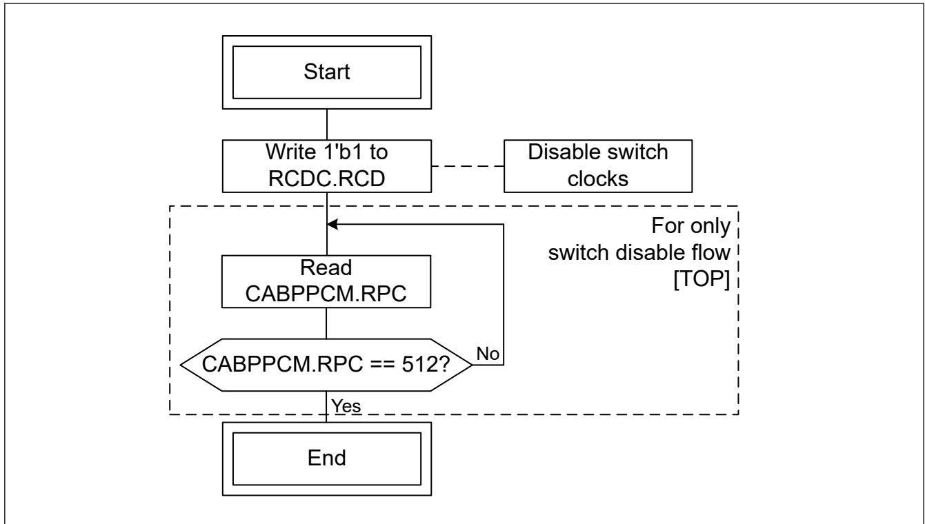
Figure 32.10 Switch clock disable flow
