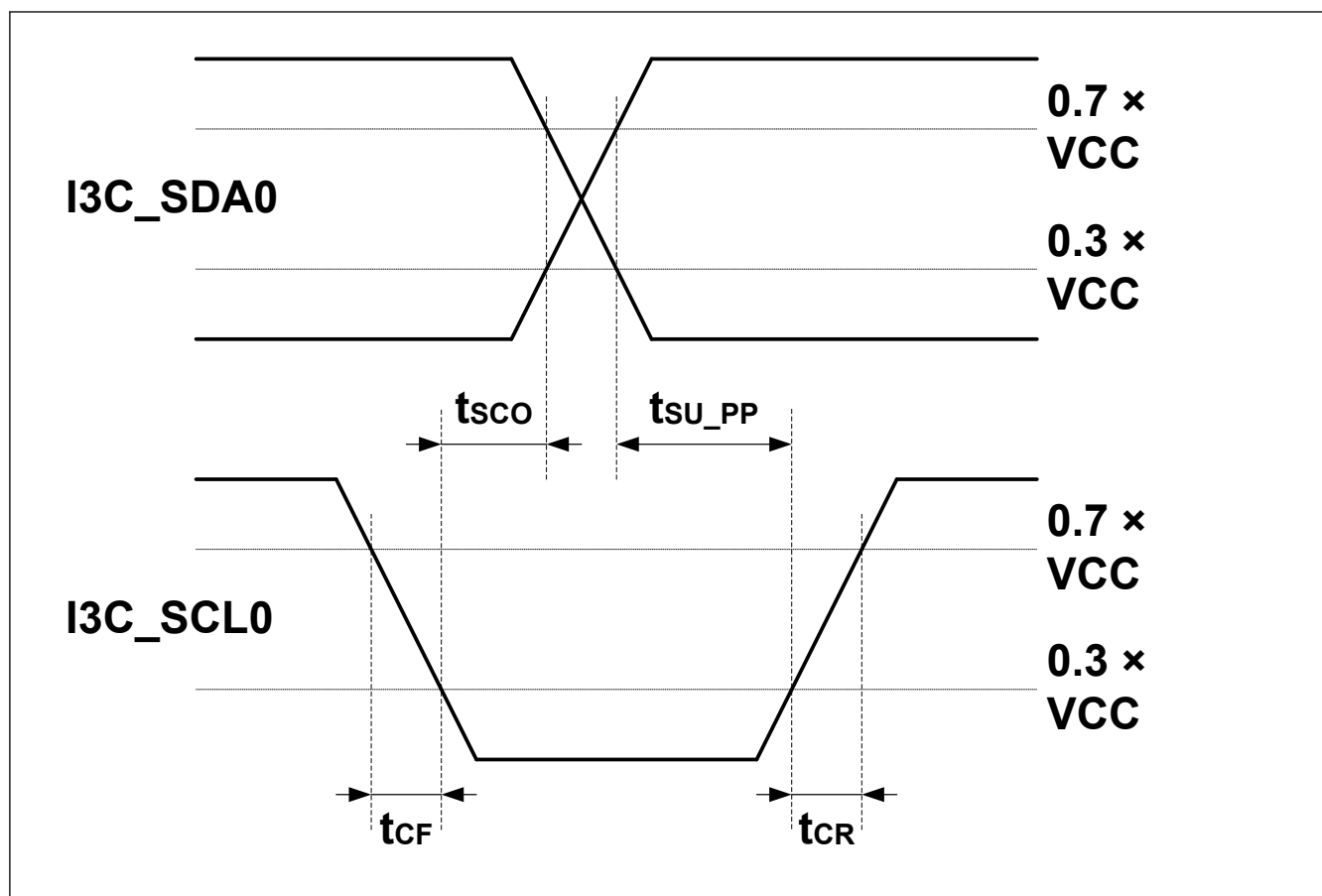
Figure 70.96 I3C Slave Out Timing
