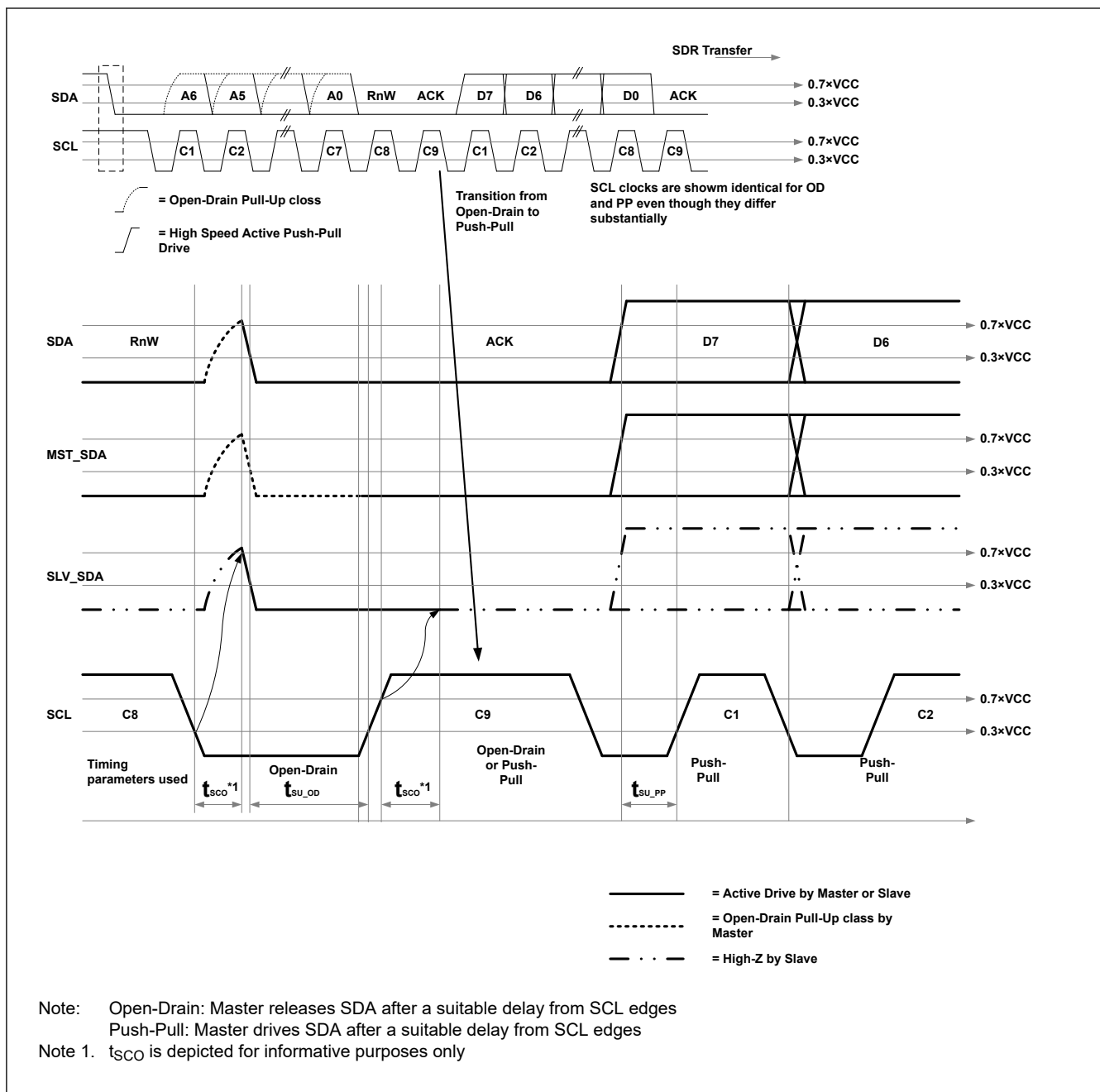
Figure 70.92 I3C Data Transfer – ACK by Slave
