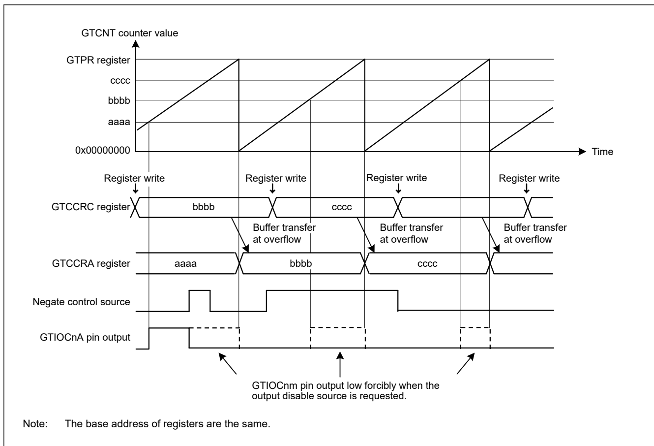
Figure 23.160 Example of GTIOCnm pin output disable control operation in saw-wave up-counting, buffer operation, active level 1, high output at GTCCRA compare match, low output at cycle end, and low output at output disable (n = 0 to 13, m = A, B)
