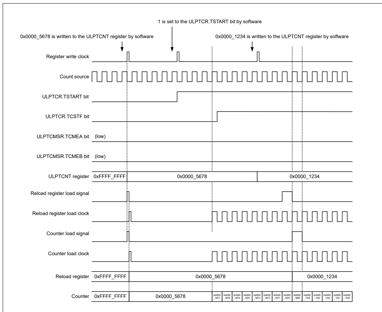
Figure 26.13 Counter and reload rewrite timing (under condition A or B)
