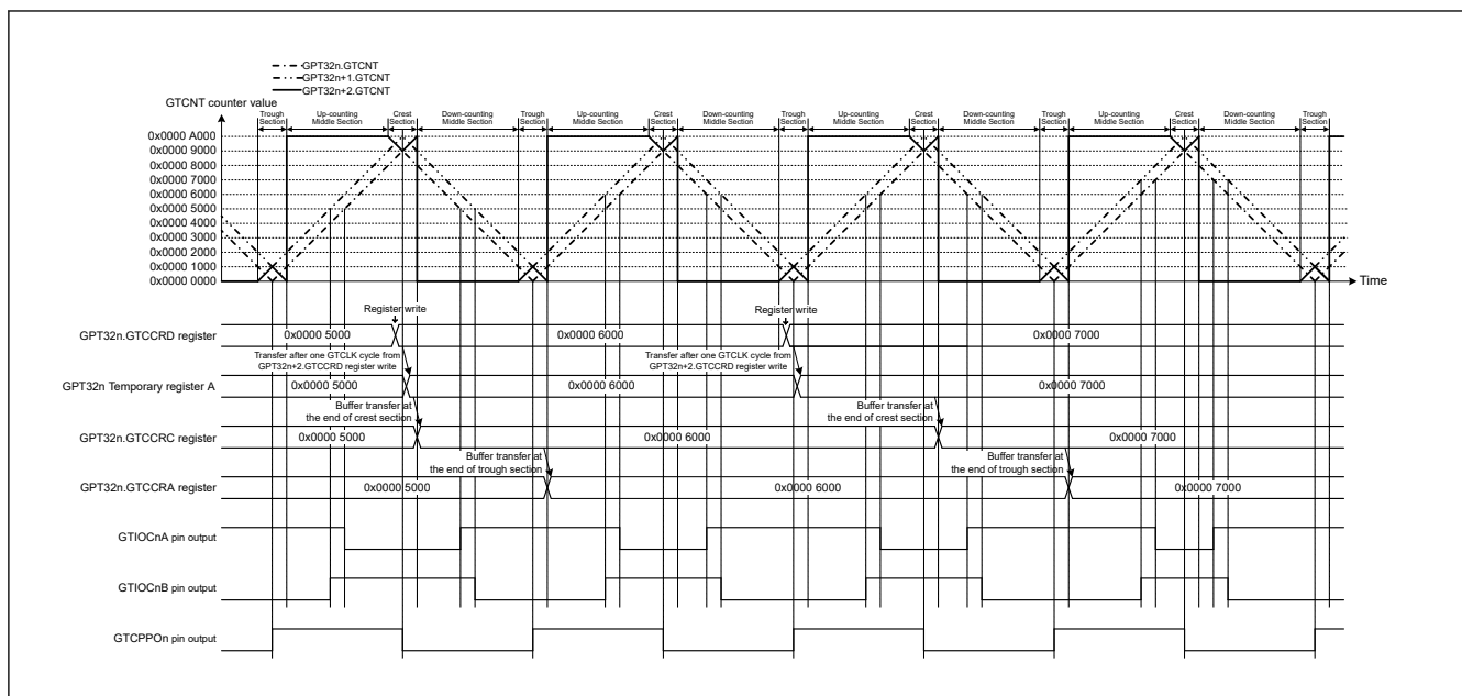
Figure 23.48 Example of Complementary PWM Mode 2 Operation (GTIOCnA pin = Low / GTIOCnB pin = High at GTCCRA register compare match during up-counting, GTIOCnA pin = High / GTIOCnB pin = Low at GTCCRA register compare match during down-counting, the dead time value is 0x0000 1000 and updating GTCCRD register in crest and trough sections) (n = 4, 7)
