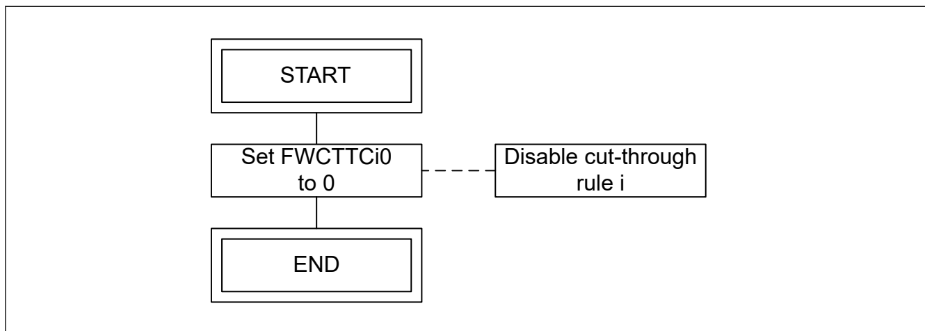
Figure 31.6 Cut-through rule i disable flow
