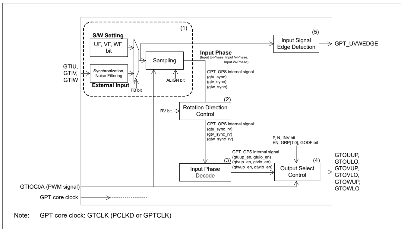
Figure 23.121 GPT_OPS Block Diagram
