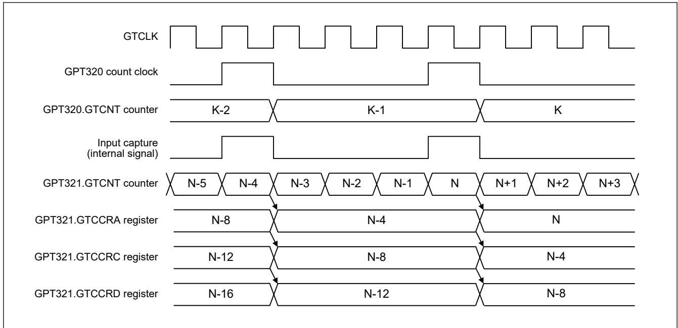
Figure 23.15 Example of the Timing of Input Capture Operation in Response to Count Clock from Other Channel
