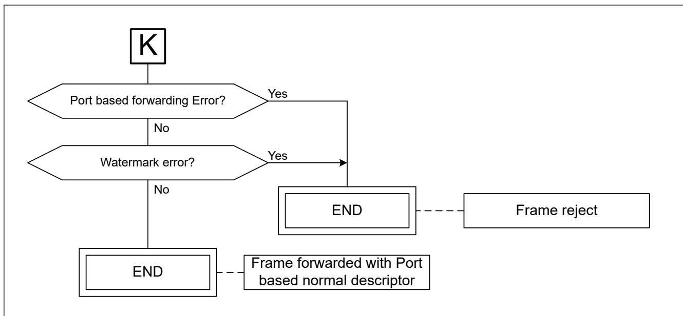
Figure 31.100 Port based forwarding unsecure flow
