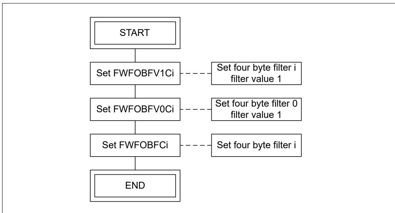
Figure 31.38 Setting flow of four-byte filter i
