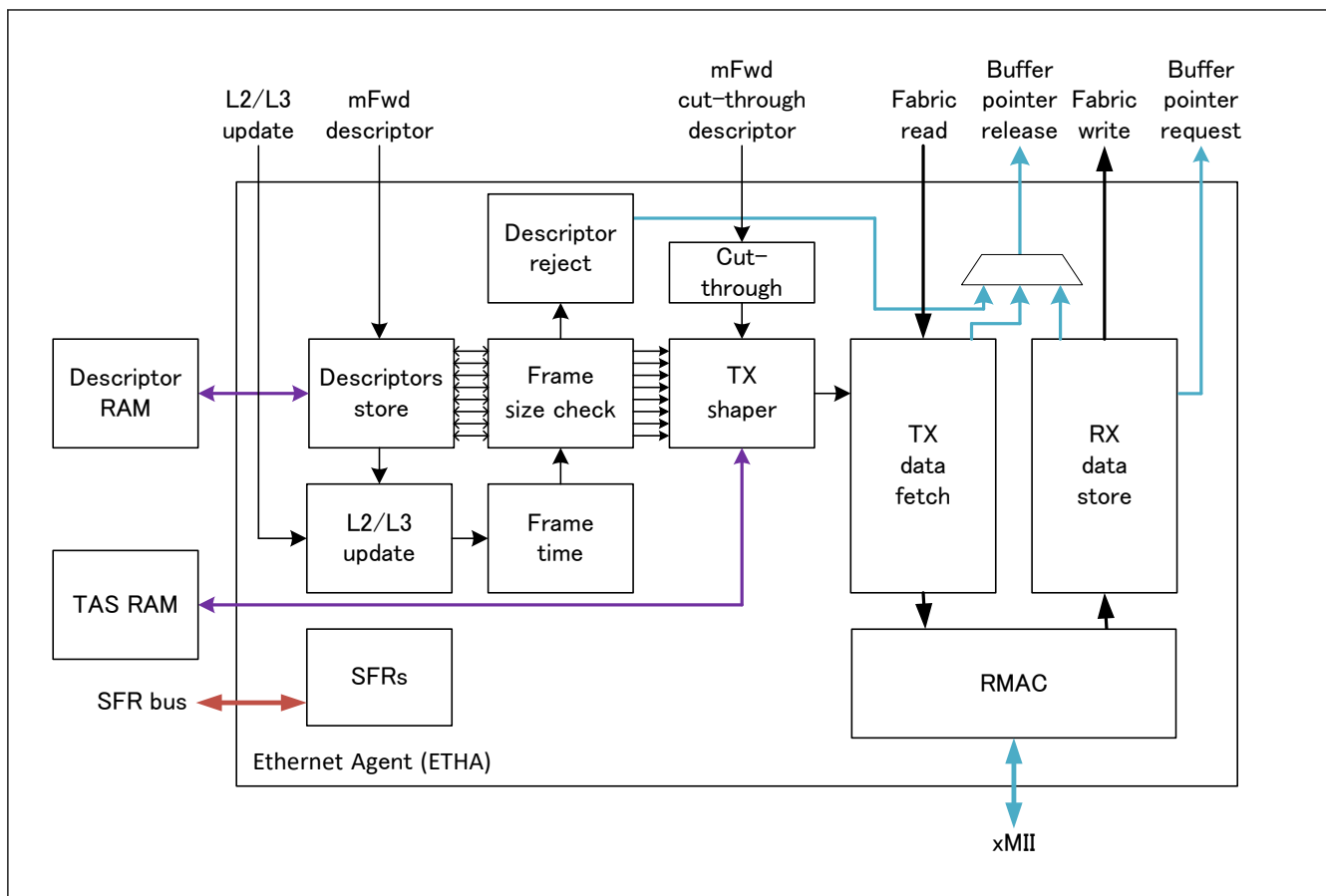
Figure 33.1 ETHA block diagram
