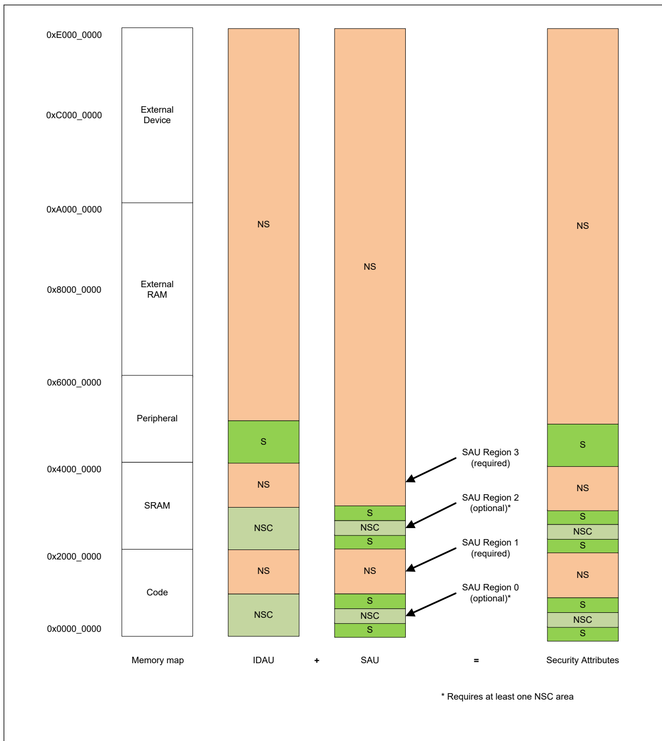
Figure 52.4 SAU settings and resulting security attributes
