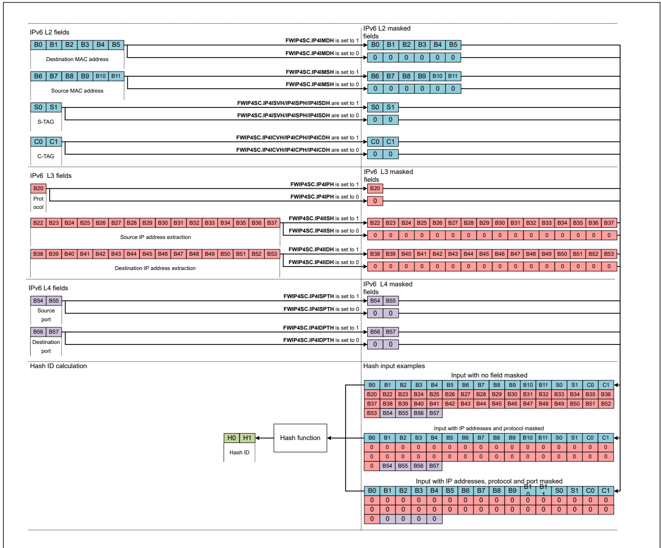
Figure 31.80 IPv6 Hash ID calculation
