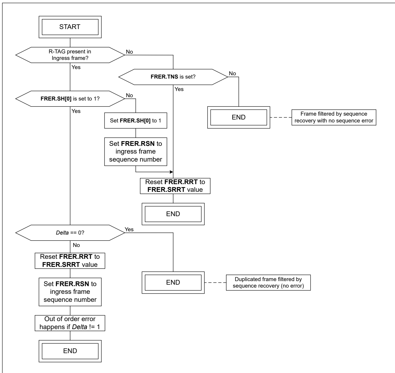
Figure 31.109 Sequence recovery match algorithm
