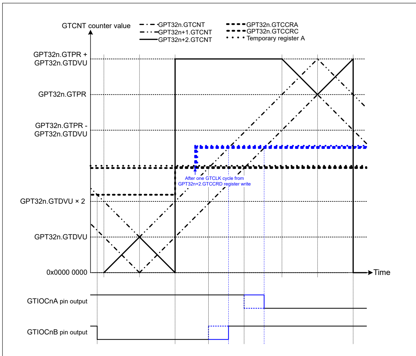
Figure 23.68 Example of Complementary PWM Mode 4 Single Buffer Operation (Up-Counting Middle Section) (Complementary PWM mode 4 single buffer operation, GTIOcNA pin = Low / GTIOcNB pin = High at GTCCRA register compare match during up-counting, GTIOcNA pin = High / GTIOcNB pin = Low at GTCCRA register compare match during down-counting, when a value larger than the GPT32n+1.GTCNT value is written to GTCCRD register before up-counting compare match) (n = 4, 7)
