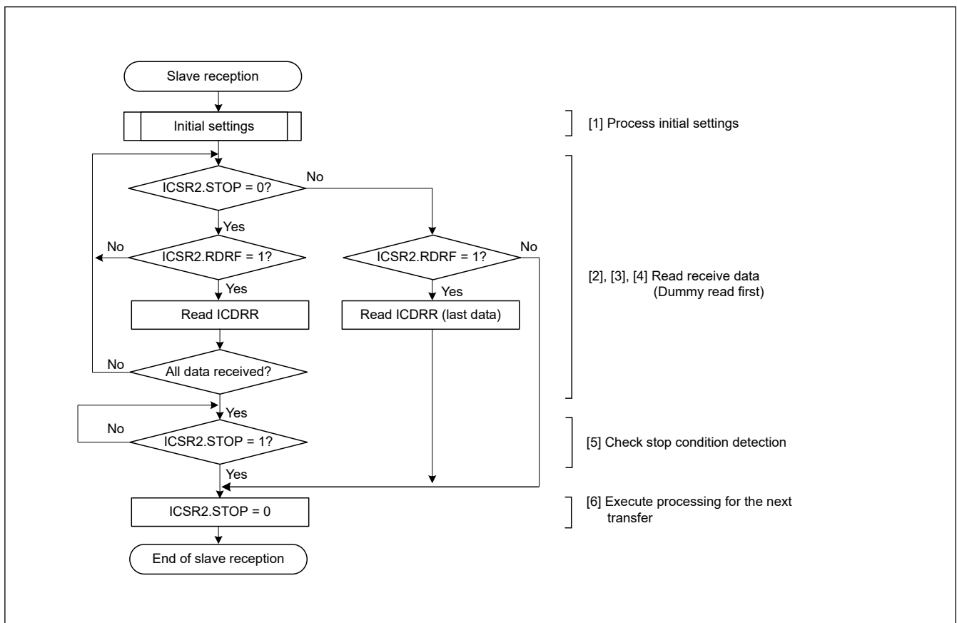
Figure 40.18 Example slave reception flow
