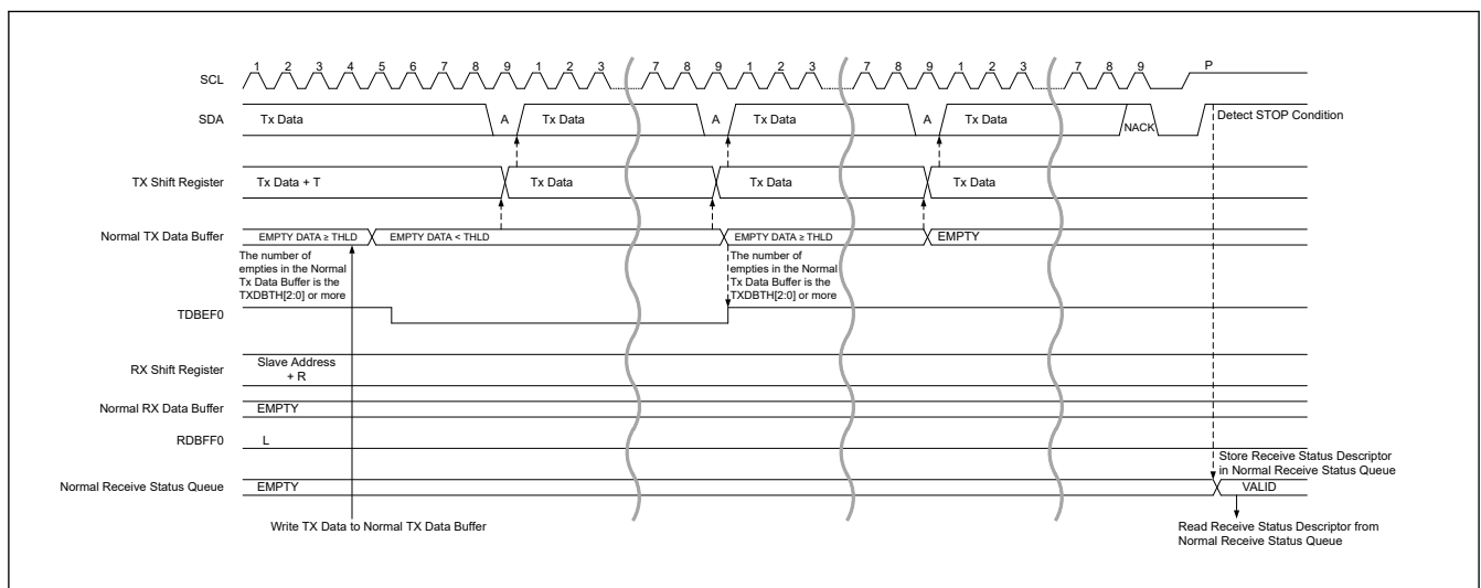
Figure 41.52 Legacy I 2 C message data read transfer timing (2/2)
