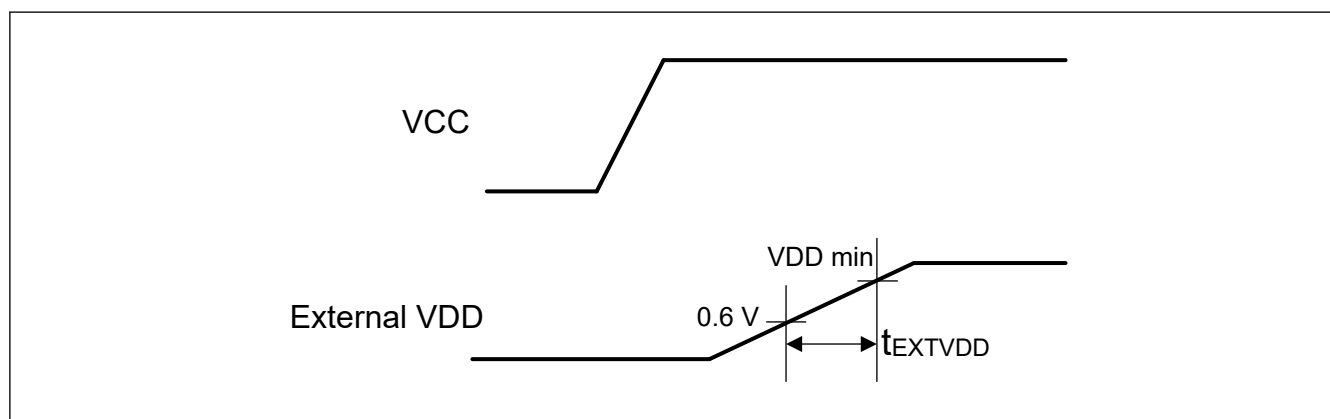
Figure 70.145 Power-up sequence of external VDD mode without using RES pin
