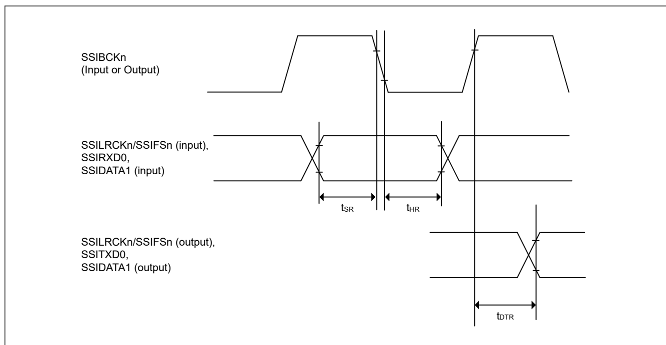
Figure 70.105 SSIE data transmit and receive timing when SSICR.BCKP = 1
