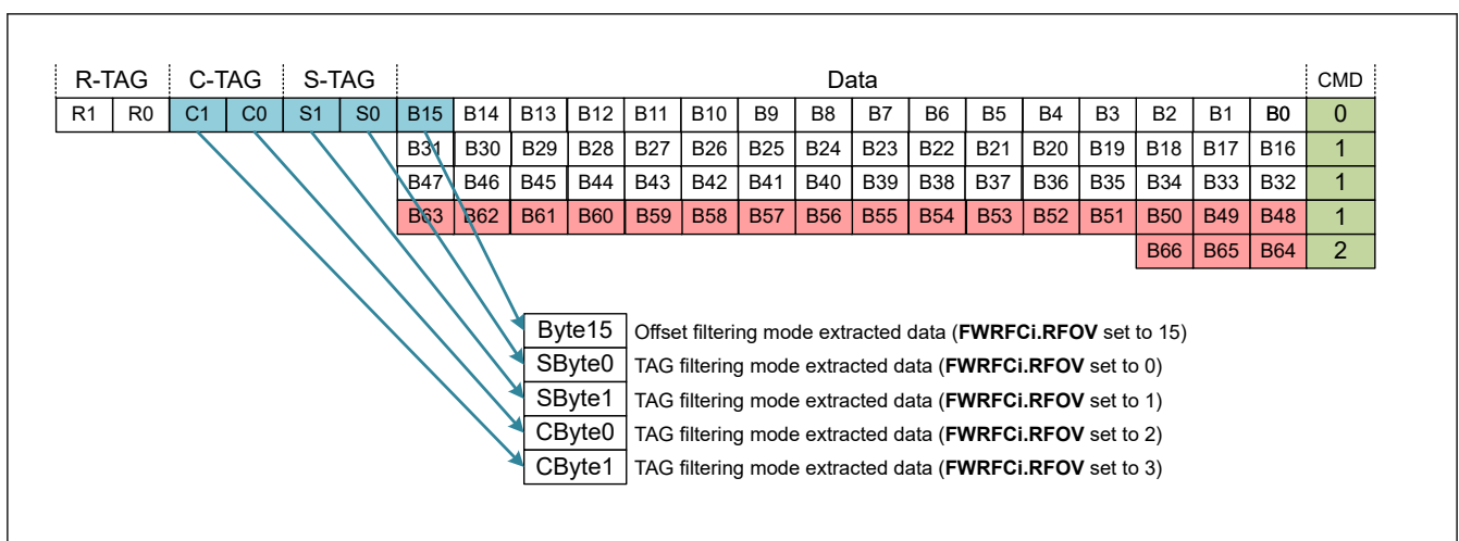
Figure 31.69 Range filter data extraction for filtering
