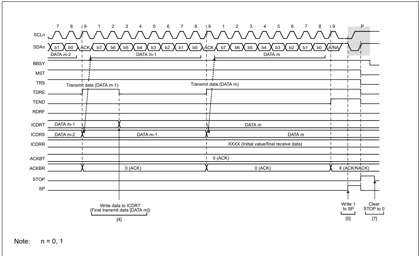
Figure 40.9 Master transmit operation timing (3)
