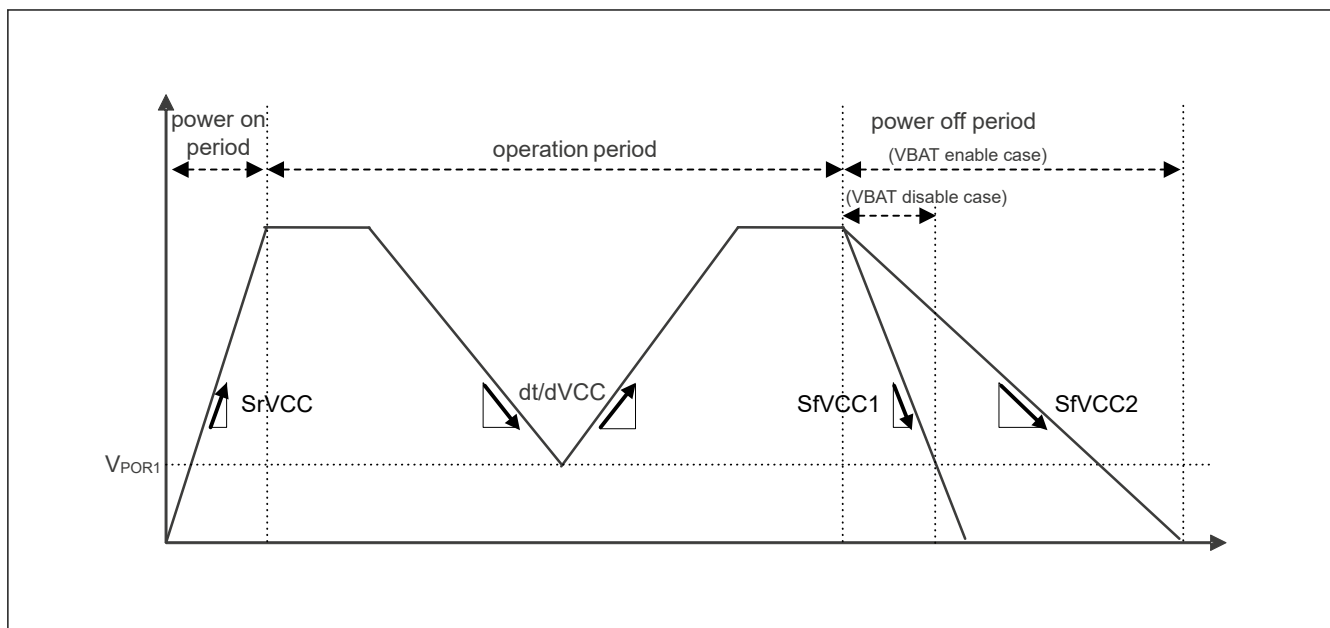
Figure 70.24 VCC rising and falling waveform
