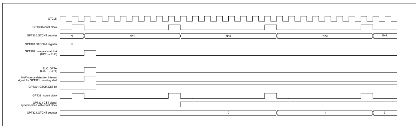
Figure 23.84 Example of Timing of Operations to Start Counting in Response to Event Input from ELC_GPTA
