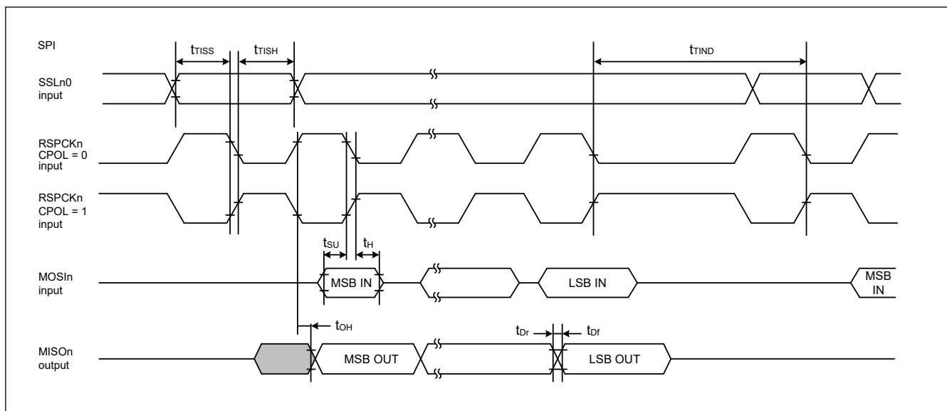
Figure 70.81 SPI timing for TI SSP slave when transmit with delay between frames
