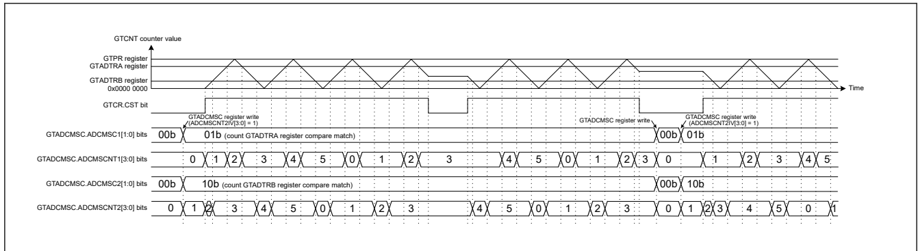
Figure 23.146 Example of A/D Conversion Start Request Compare Match Skipping Function Operation
