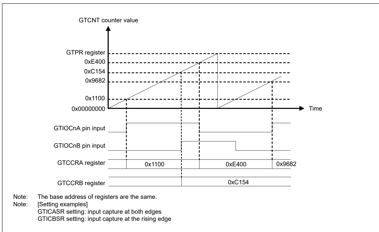
Figure 23.13 Example of input capture operation
