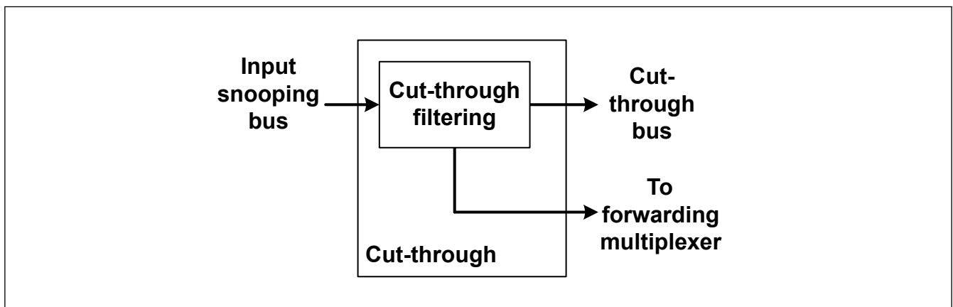
Figure 31.51 Cut-through forwarding block diagram
