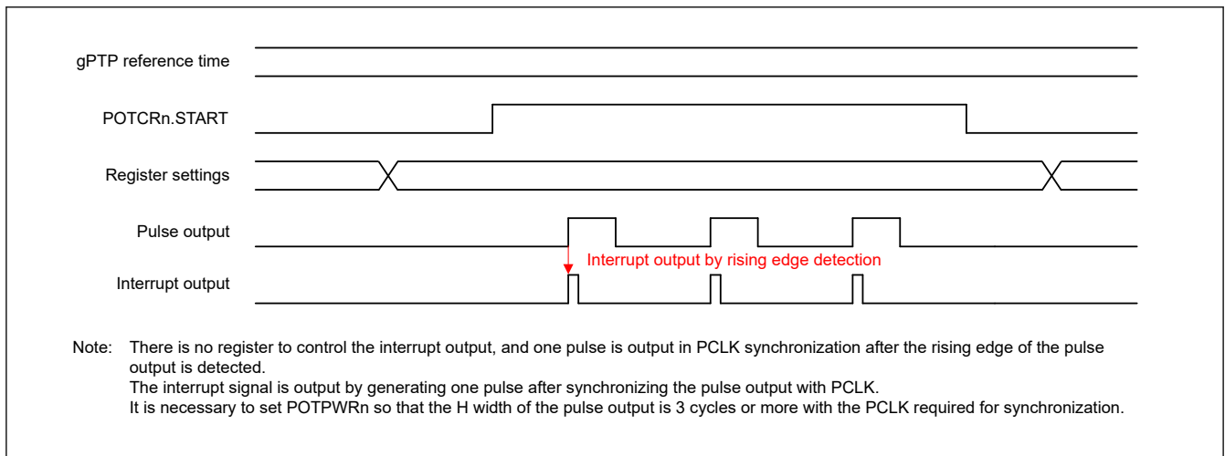
Figure 36.21 Detects the rising edge of the pulse output and outputs one pulse synchronized with PCLK
