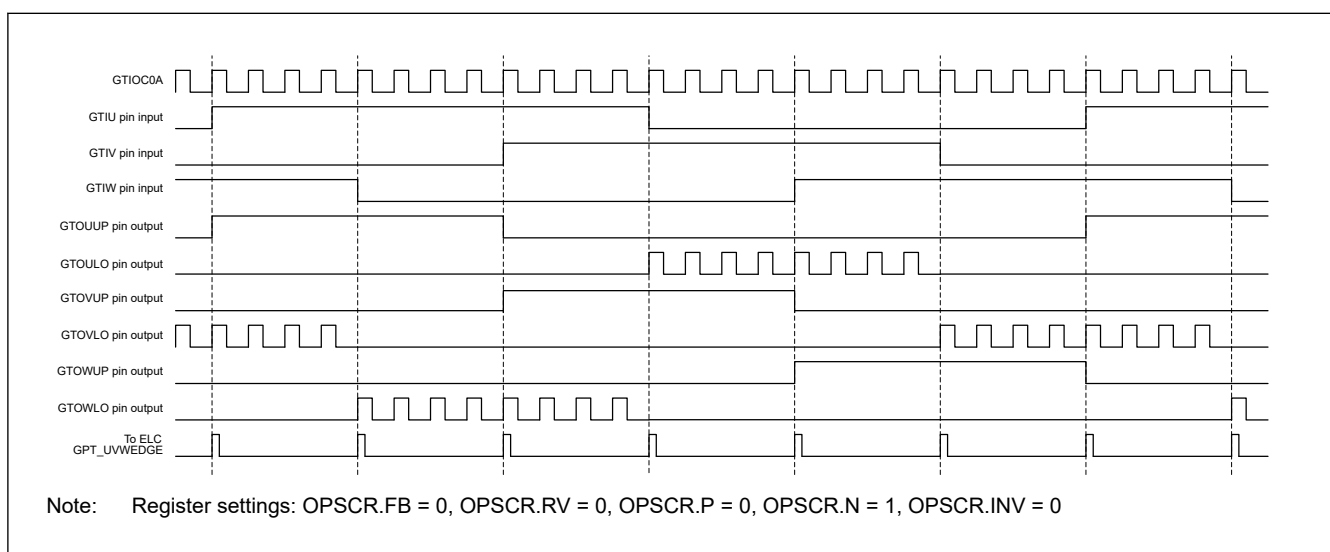
Figure 23.125 Example of GPT_OPS Chopped Output Operation (Negative Phase 120-degree)
