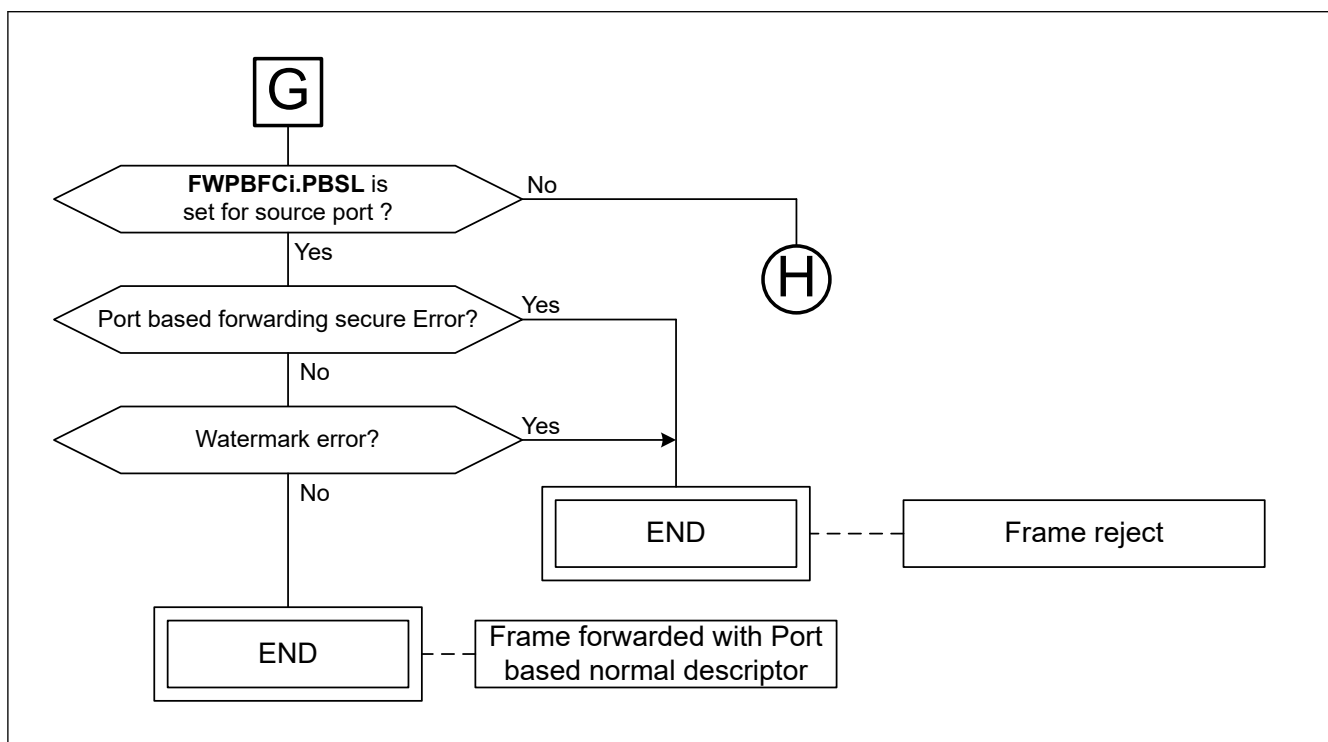
Figure 31.99 Port based forwarding secure flow
