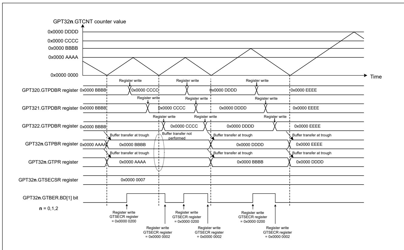
Figure 23.154 Example of Multiple Channel Operation for Disabling Buffer Operation (Triangle Waves, Double Buffer Operation)
