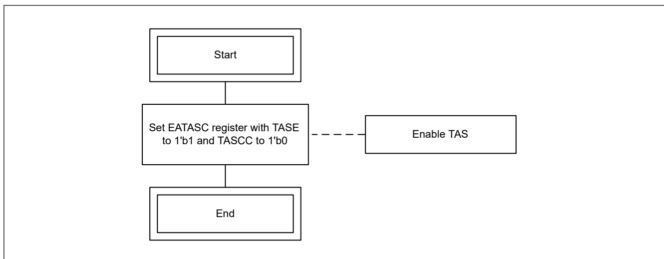
Figure 33.13 TAS enabling flow
