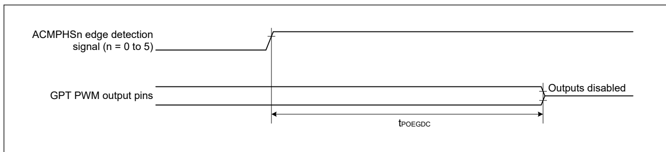
Figure 70.57 Output Disable Time for POEG in Response to Edge Detection Signal from a Comparator
