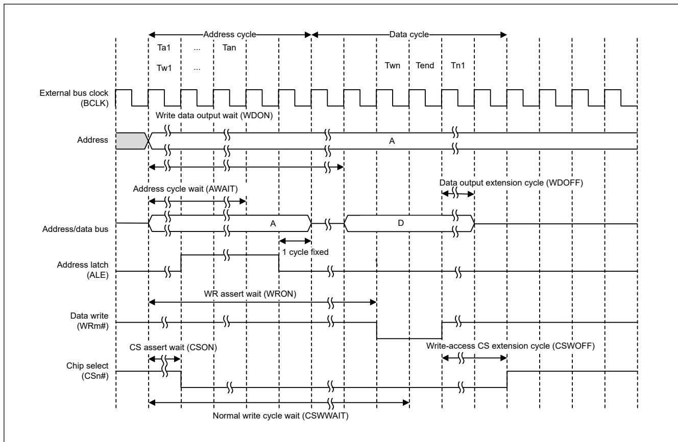
Figure 15.23 Example of write access operation with address/data multiplexed I/O interface (n = 0 to 7, m = 0, 1)
