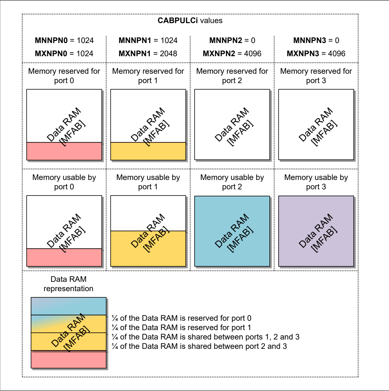
Figure 32.19 Hybrid memory setting example
