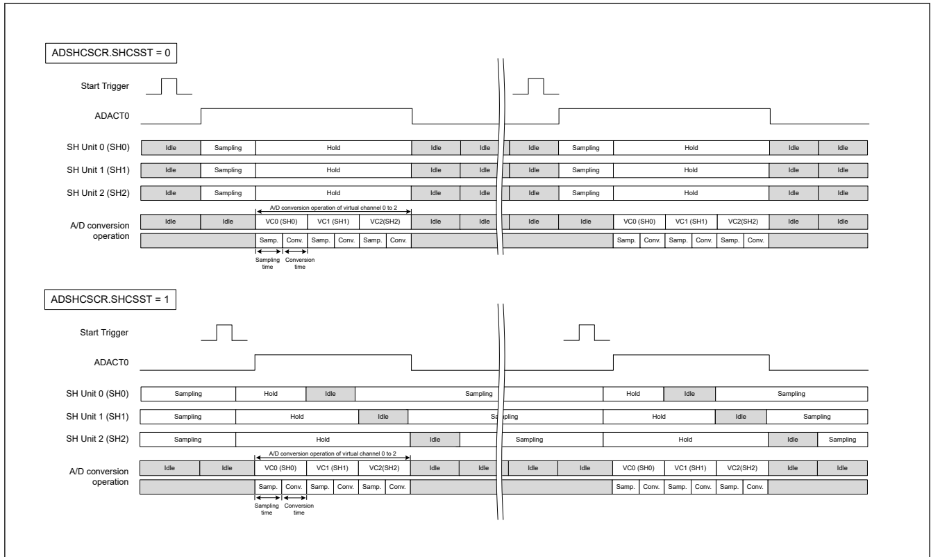
Figure 54.23 Difference between the function of channel-dedicated sample-and-hold circuit when using or not using constant sampling
