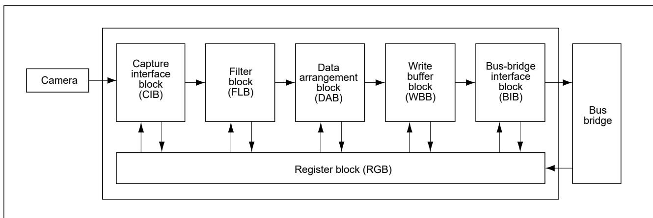
Figure 61.1 Block diagram of CEU
