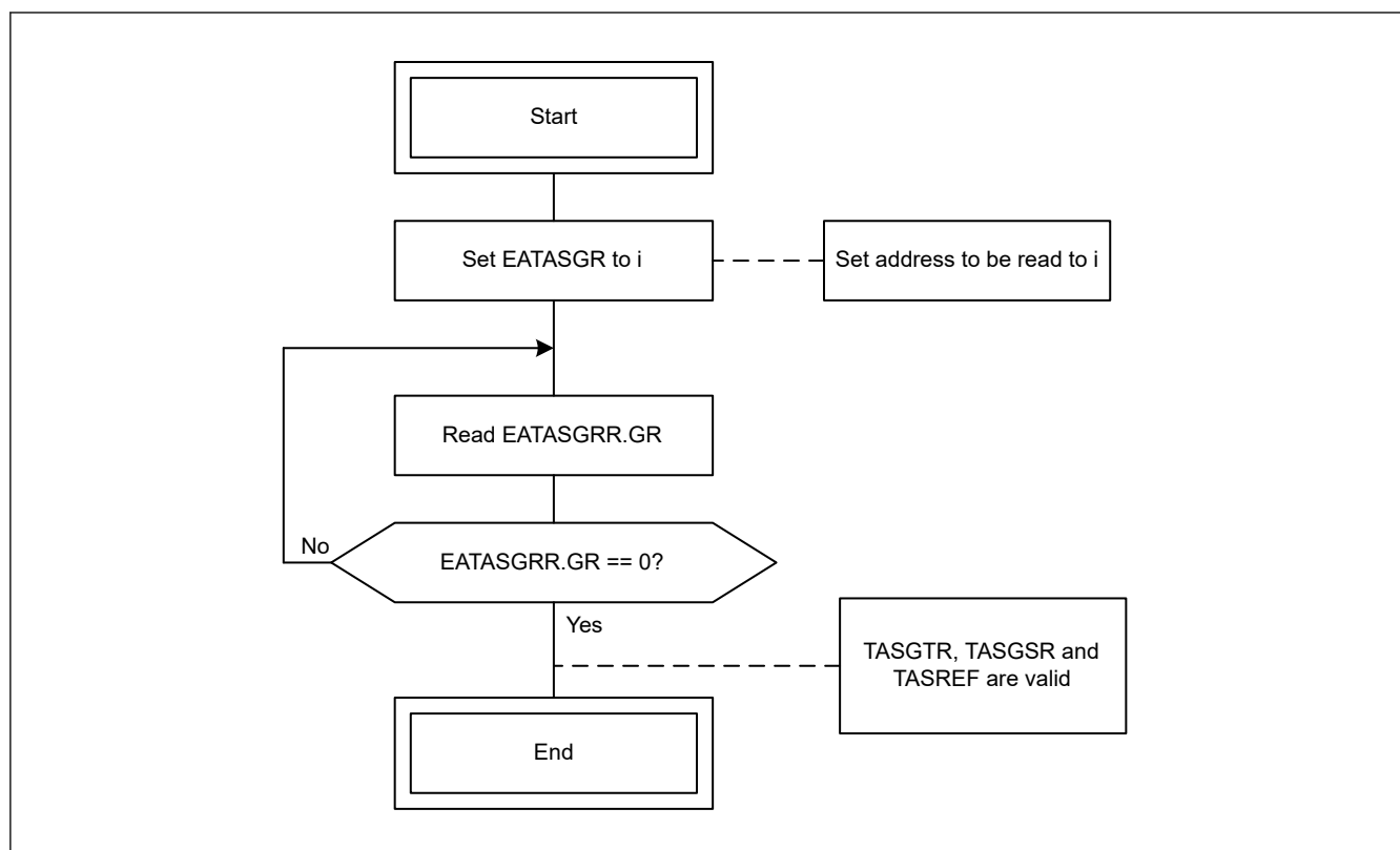
Figure 33.15 TAS entry i read flow
