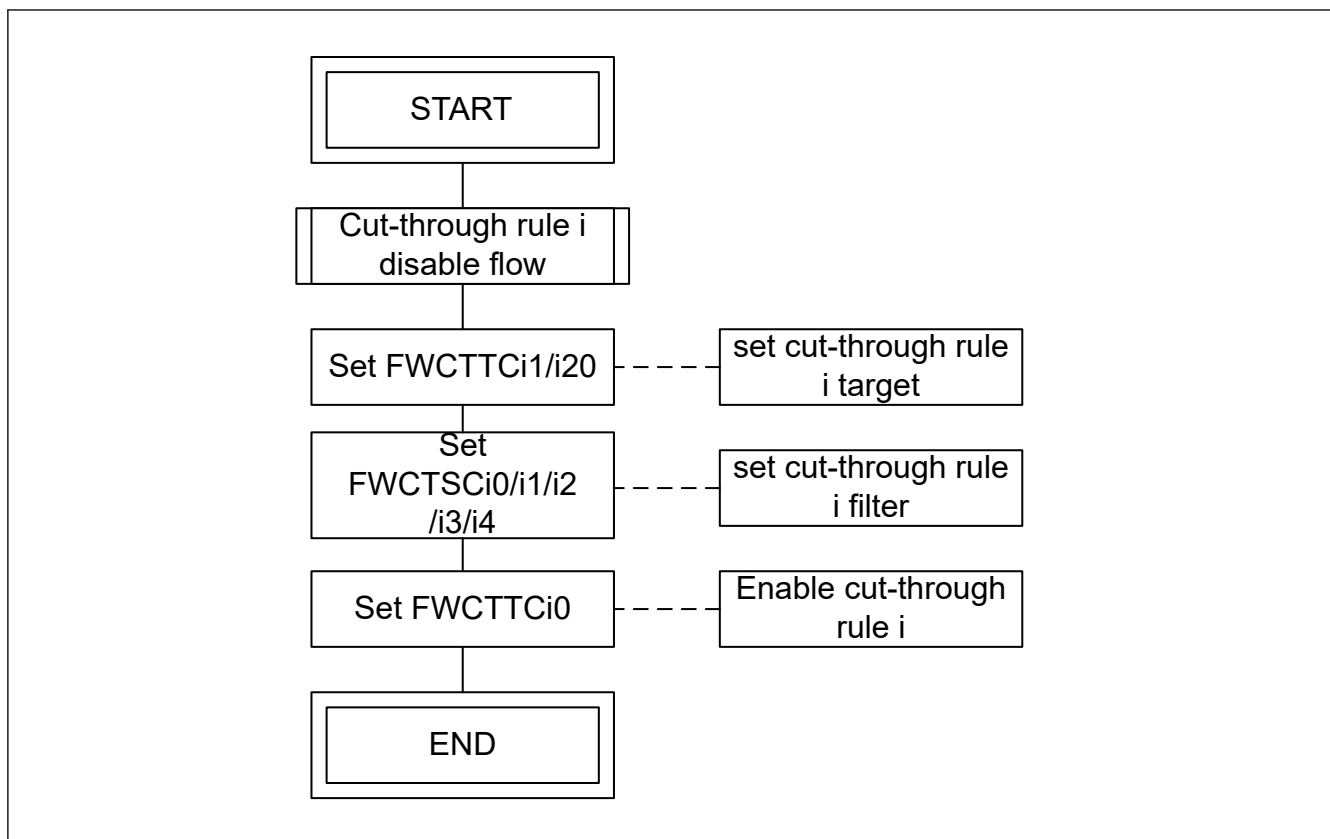
Figure 31.5 Cut-through rule i setting flow
