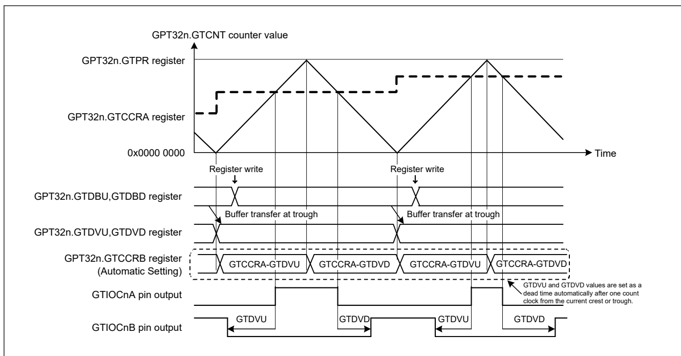
Figure 23.79 Example of automatic compare-match value setting function with dead time in triangle-wave PWM mode 1, GTDVU and GTDVD set to buffer operation, and active-high
