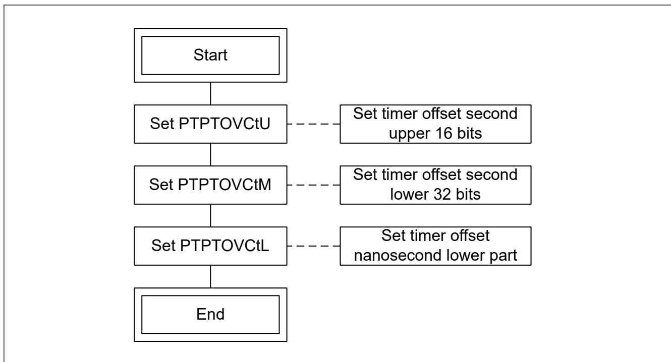
Figure 36.4 Timer t offset setting flow
