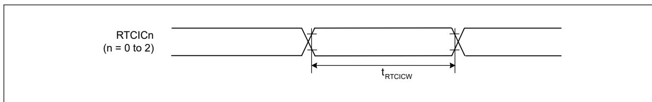
Figure 70.53 RTCICn input timing
