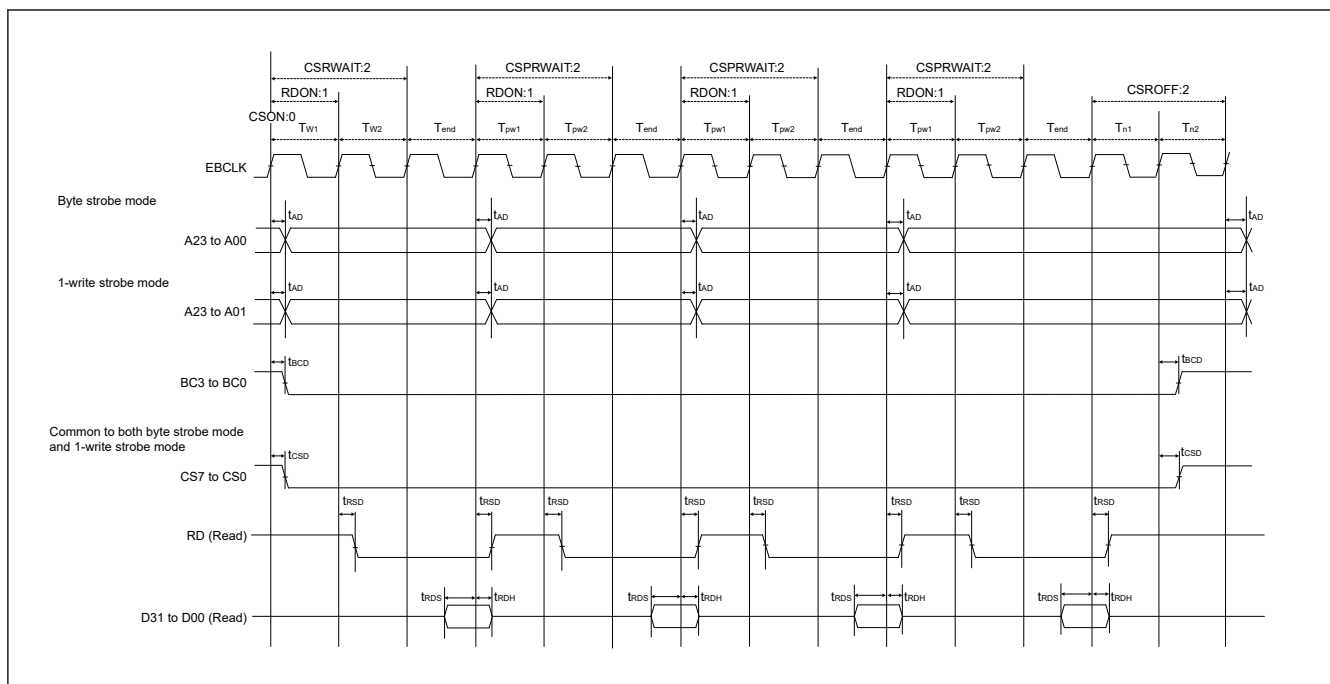
Figure 70.42 External bus timing for page read cycle with bus clock synchronized
