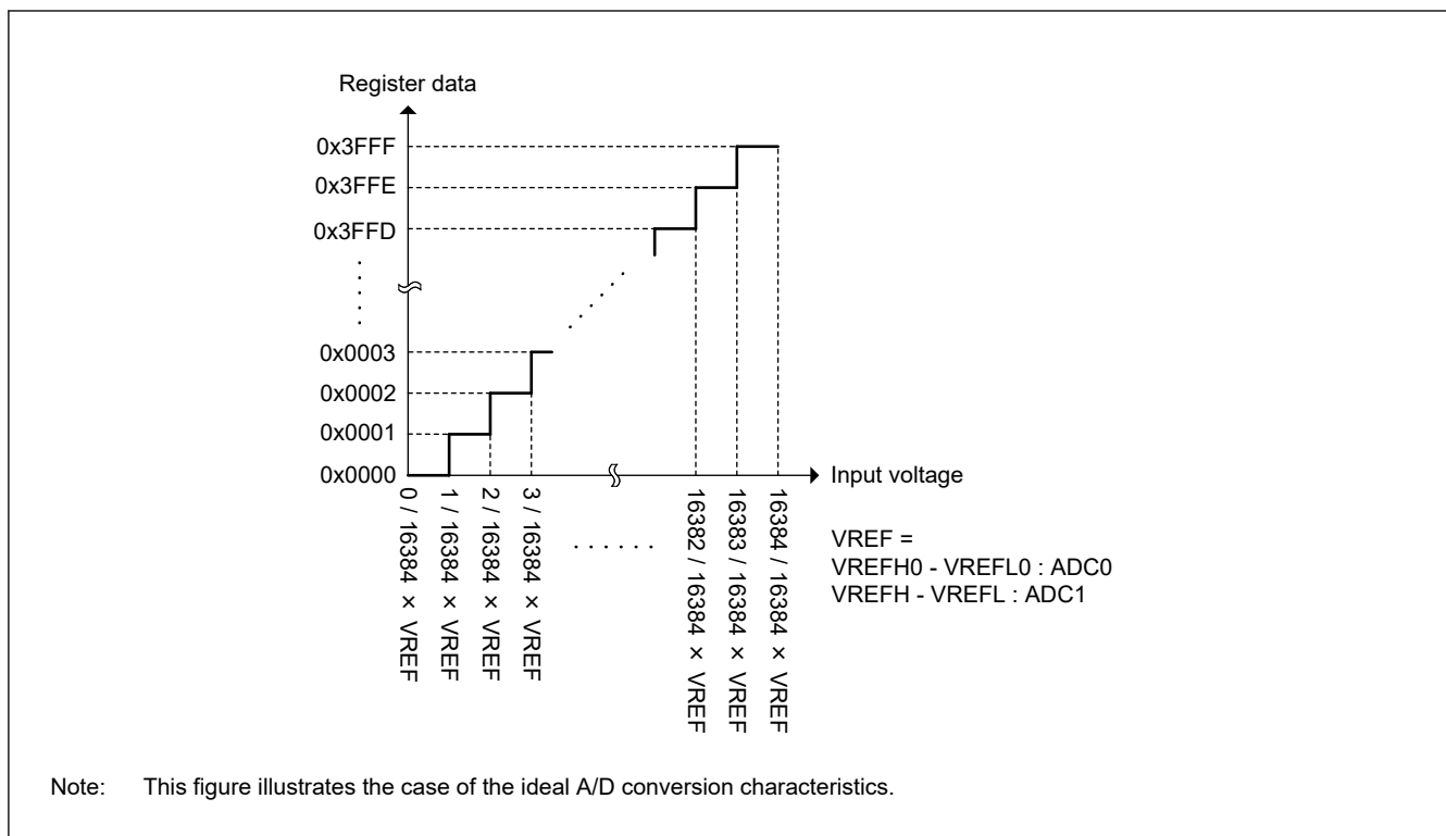
Figure 54.46 Data range of A/D conversion result (14-bit data length, Unsigned data, Single-ended input)
