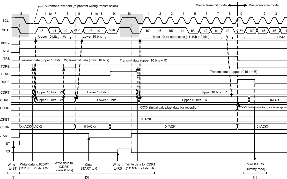
Figure 40.13 Master receive operation timing (2) with 10-bit address format when RDRFS = 0
