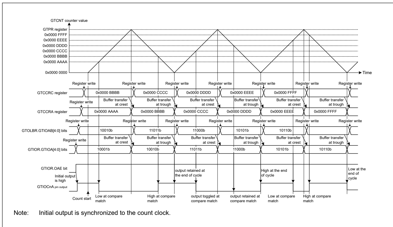
Figure 23.34 Example of Buffer Operation of the GTIOA and GTIOB Bits (Triangle-Wave PWM Mode 2, Buffer Transfer at Crests and Troughs)
