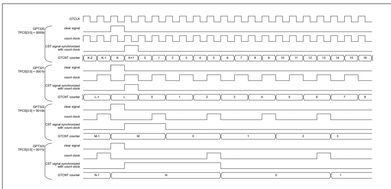
Figure 23.97 Example of Simultaneous Clearing Operation by Software (with Different Count Period)
