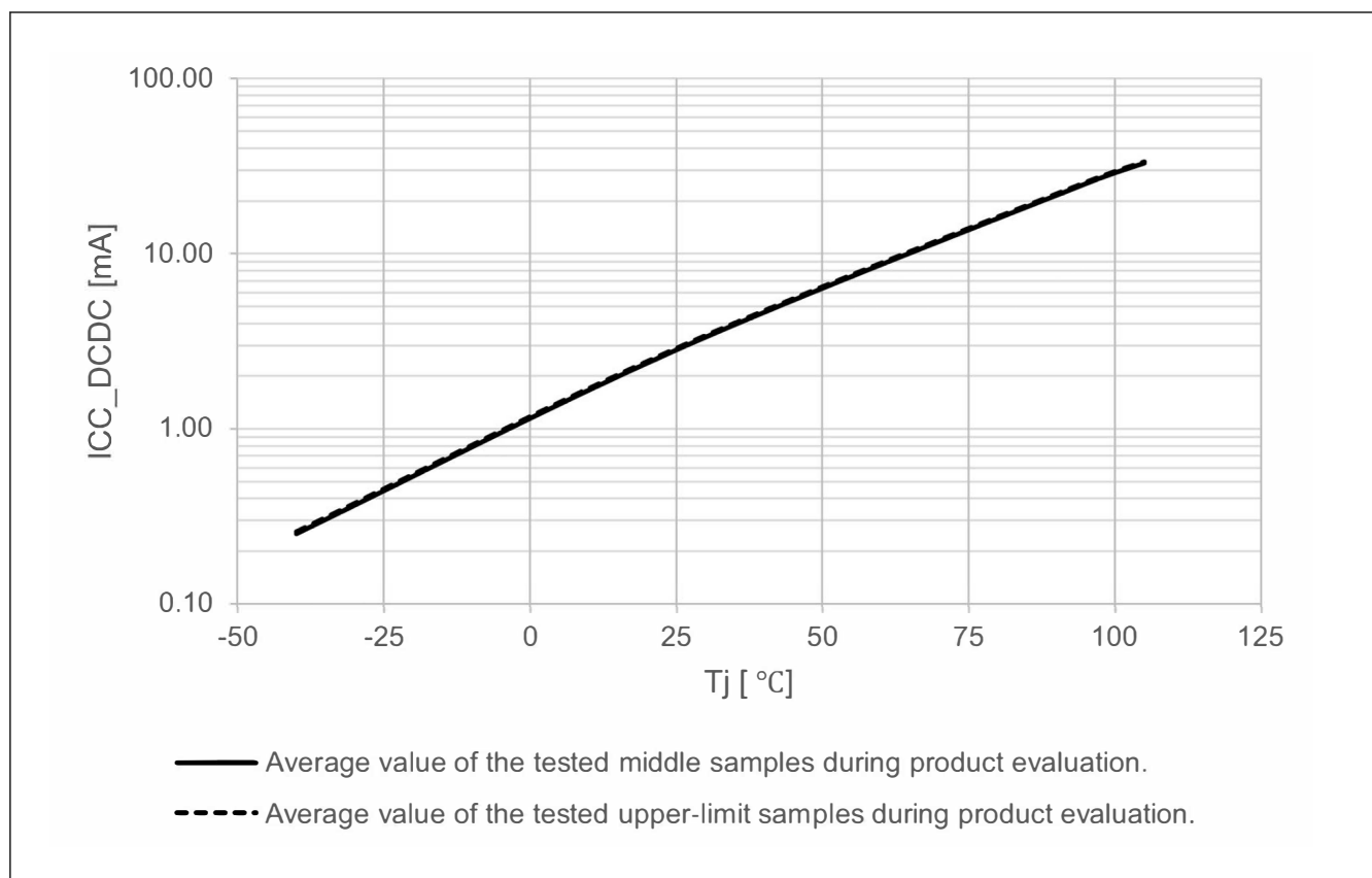
Figure 70.4 Temperature dependency in Software Standby mode ( ICC\_DCDC , SS2LP\_0 , SVSCR\_5 ) (reference data)
