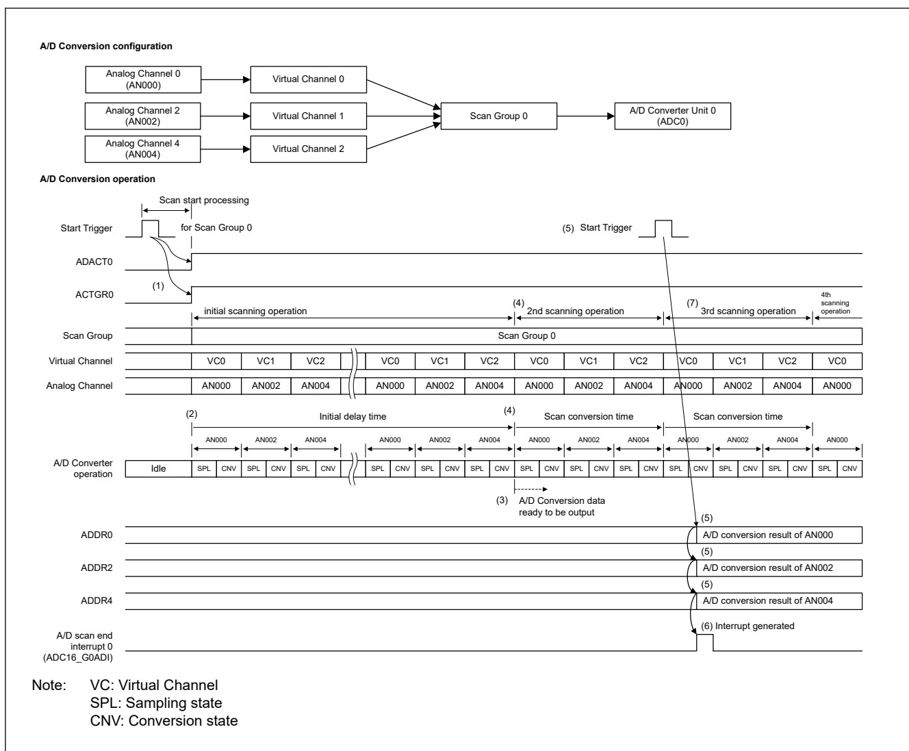
Figure 54.14 Example of scanning operation in Hybrid mode – Background continuous scan mode
