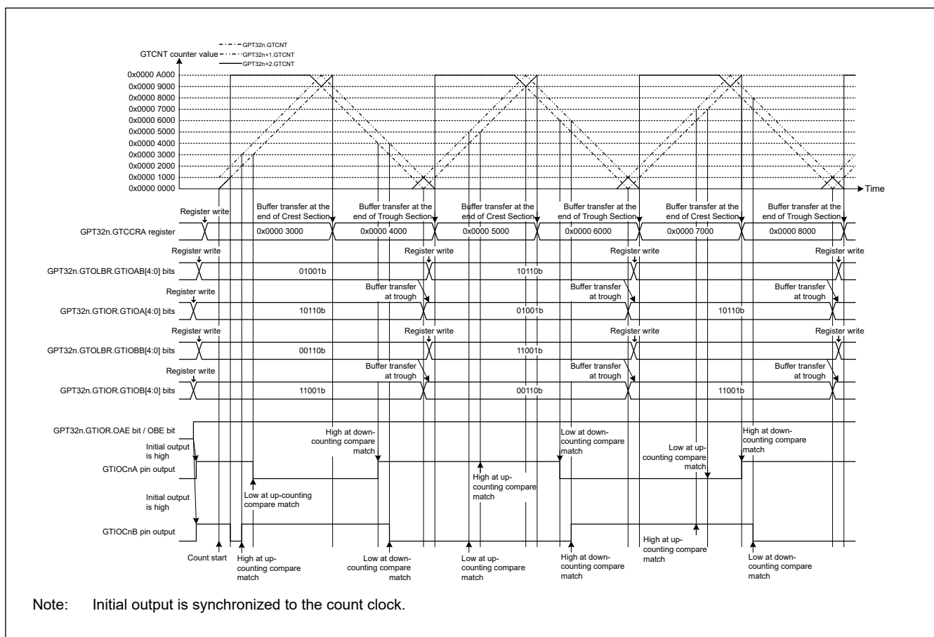
Figure 23.35 Example of Buffer Operation of the GTIOA and GTIOB Bits (Complementary PWM Mode 3, Buffer Transfer at Troughs)
