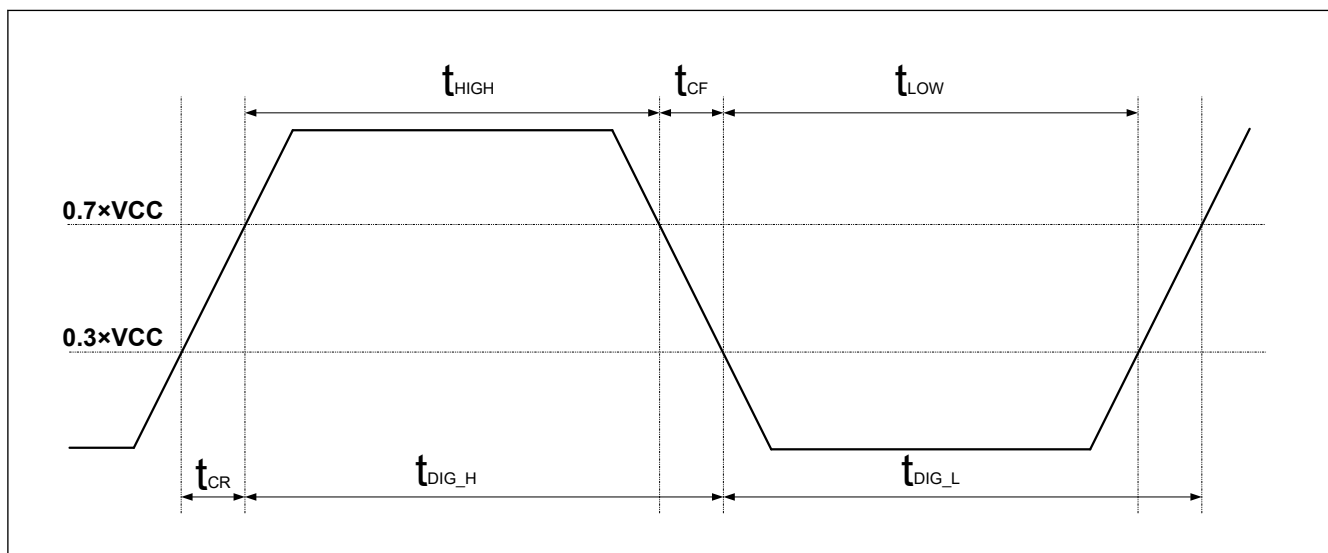
Figure 70.91 t_{DIG\_H} and t_{DIG\_L}
