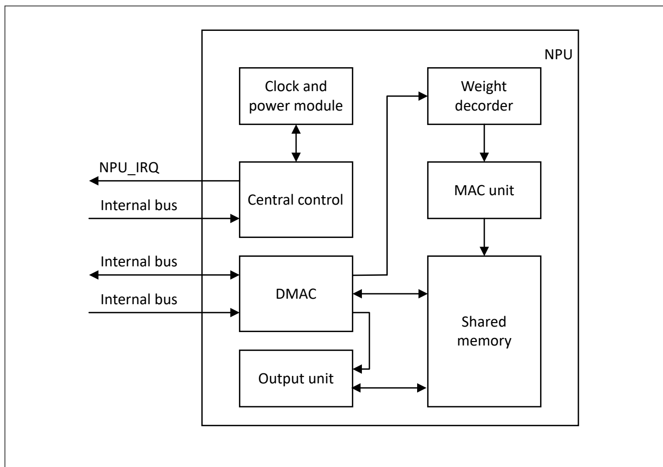
Figure 19.1 NPU block diagram
