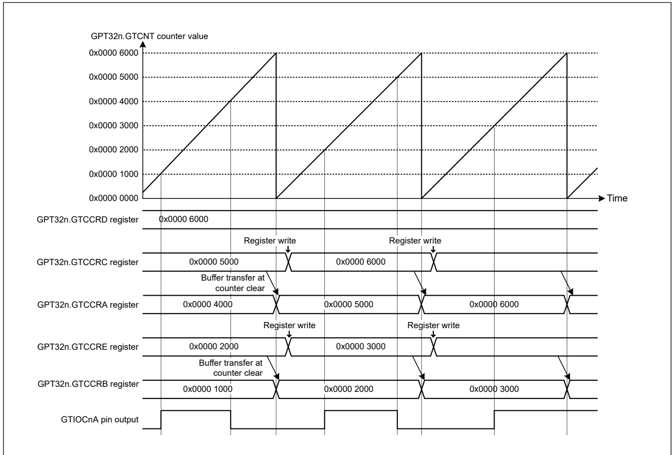
Figure 23.39 Example of Saw-Wave PWM Mode 2 Operation (Low Output at GTCCRA Register Compare Match, High Output at GTCCRB Register Compare Match, Low Output at the End of Cycle, Single Buffer Operation, Cleared at GTCCRD Register Compare Match, GTIOR.OAEOCD Bit =1) (n = 4 to 9)
