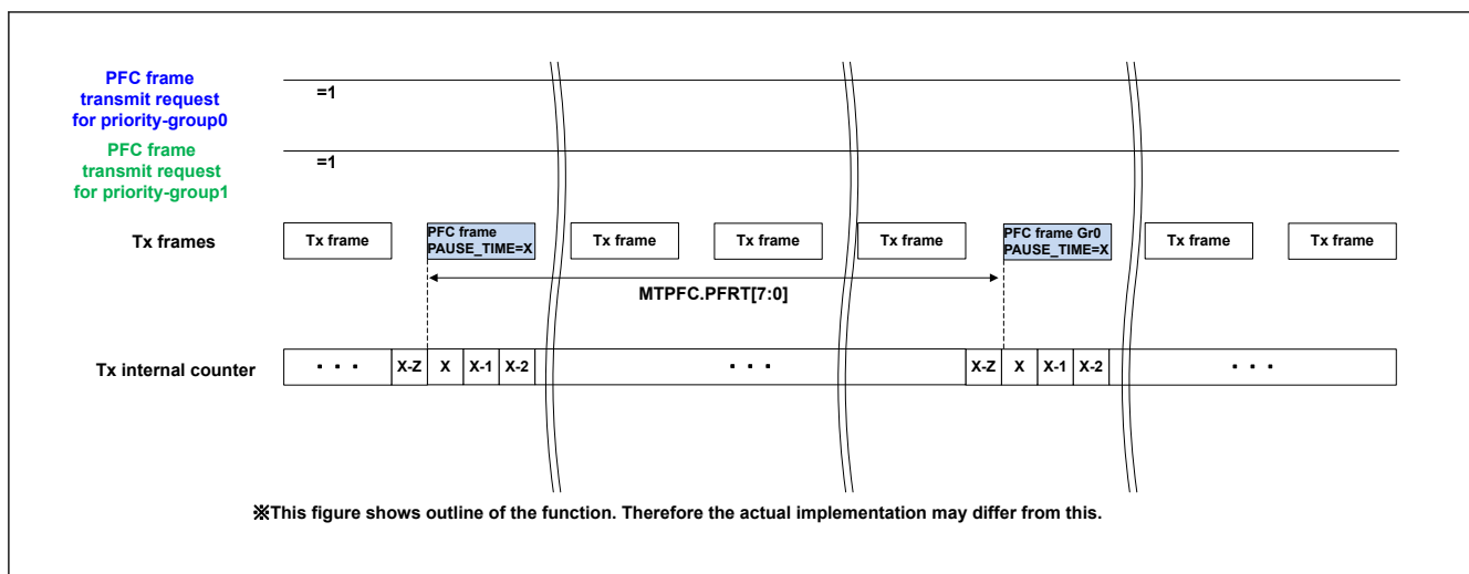
Figure 34.20 Transmitting PFC frame (part 2)
