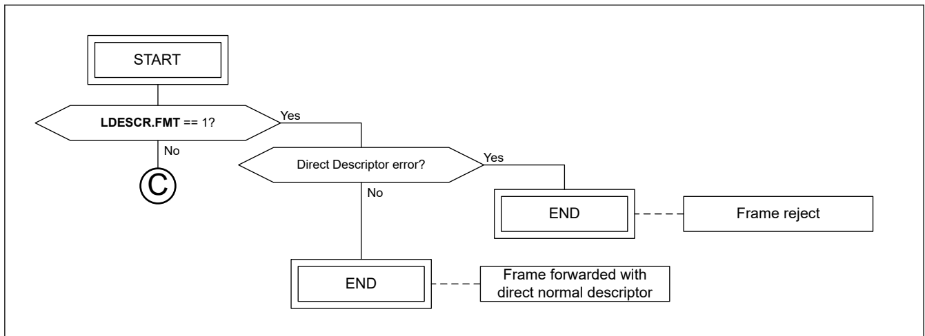
Figure 31.58 Direct descriptor forwarding flow
