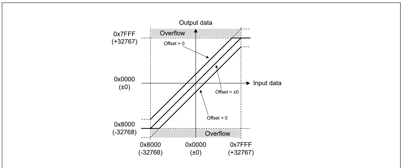
Figure 54.39 User's Offset Adjustment (16-bit data length format and Signed data format)
