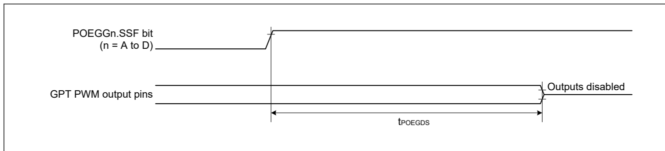
Figure 70.58 Output Disable Time for POEG in Response to the Register Setting
