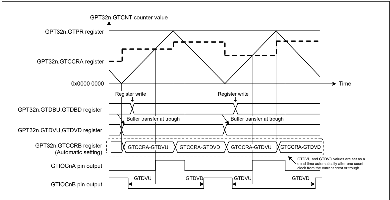
Figure 23.80 Example of automatic compare-match value setting function with dead time in triangle-wave PWM mode 2 or 3, GTDVU and GTDVD set to buffer operation, and active-high
