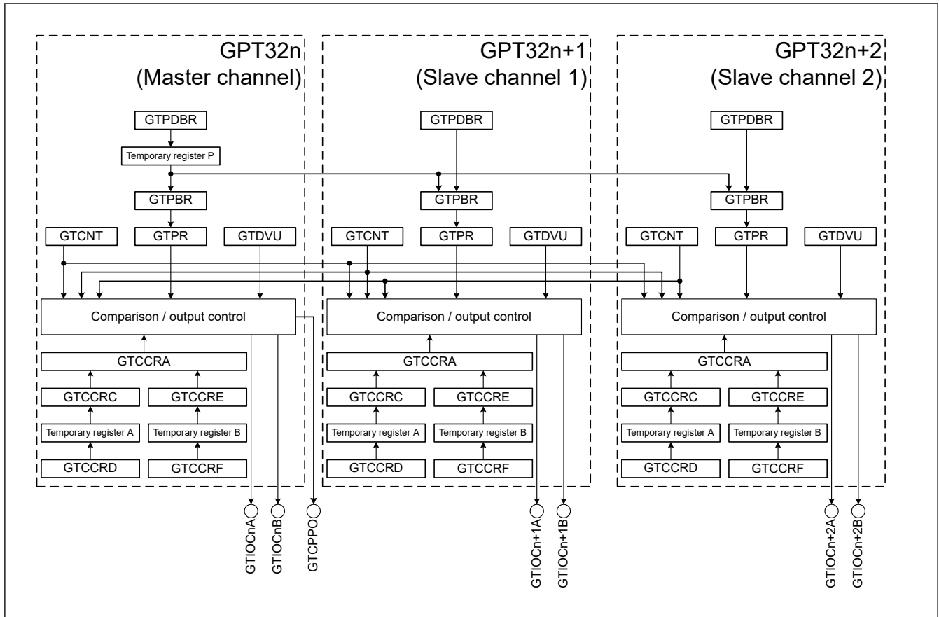
Figure 23.44 Block Diagram in Complementary PWM Mode 1, 2, 3 (n = 4, 7)
