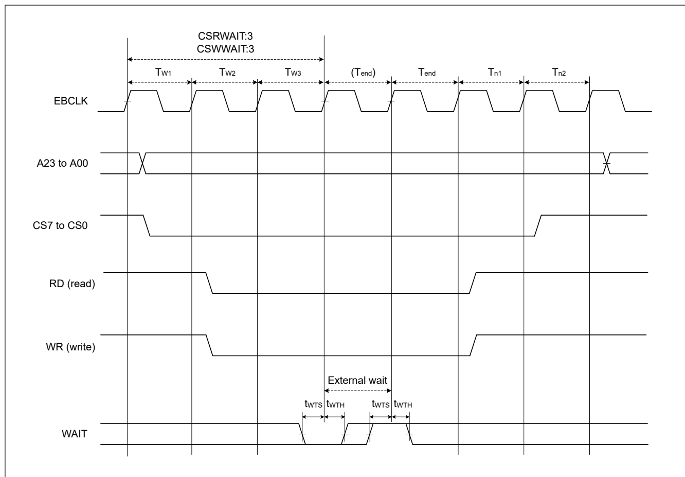
Figure 70.44 External bus timing for external wait control
