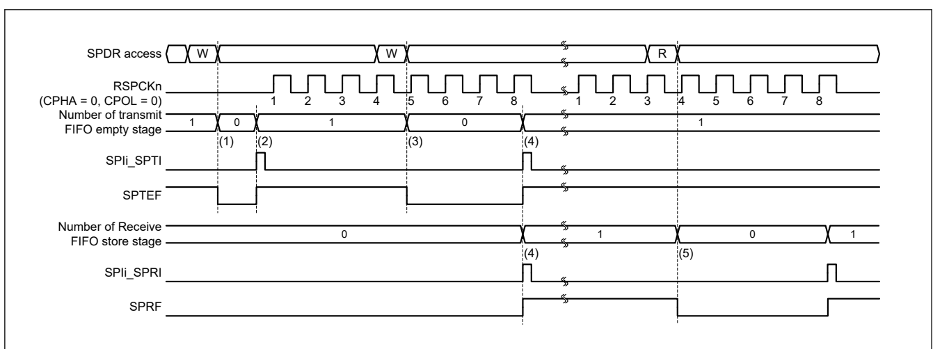
Figure 44.33 Operation example of the SPli_SPTI and SPli_SPRI interrupts when CPHA = 0 and CPOL = 0 in master mode
