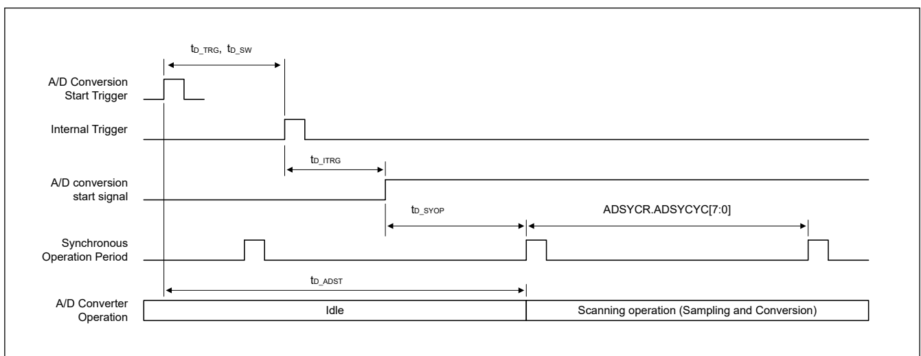
Figure 54.56 Scan start processing time
