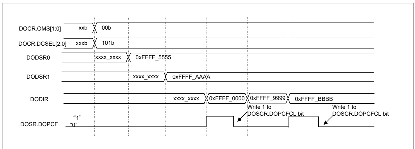
Figure 58.7 Example of Operation in Data Comparison Mode (Detection condition: Outside window)
