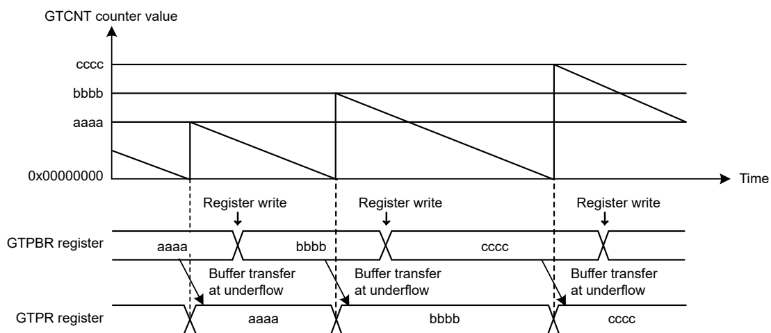
Figure 23.17 Example of GTPR buffer operation with saw waves in down-counting
