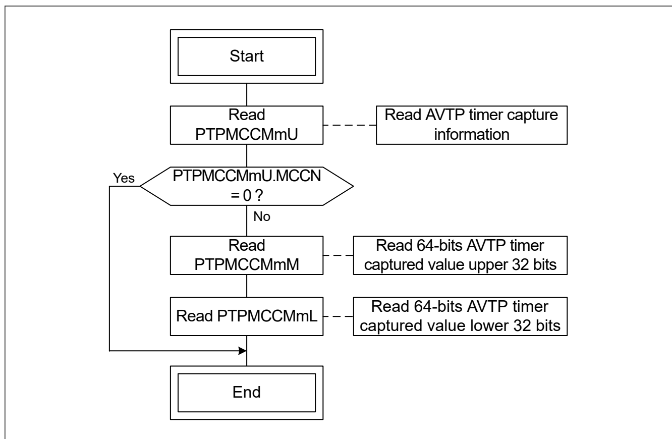
Figure 36.9 64-bit AVTP timer captured value reading flow
