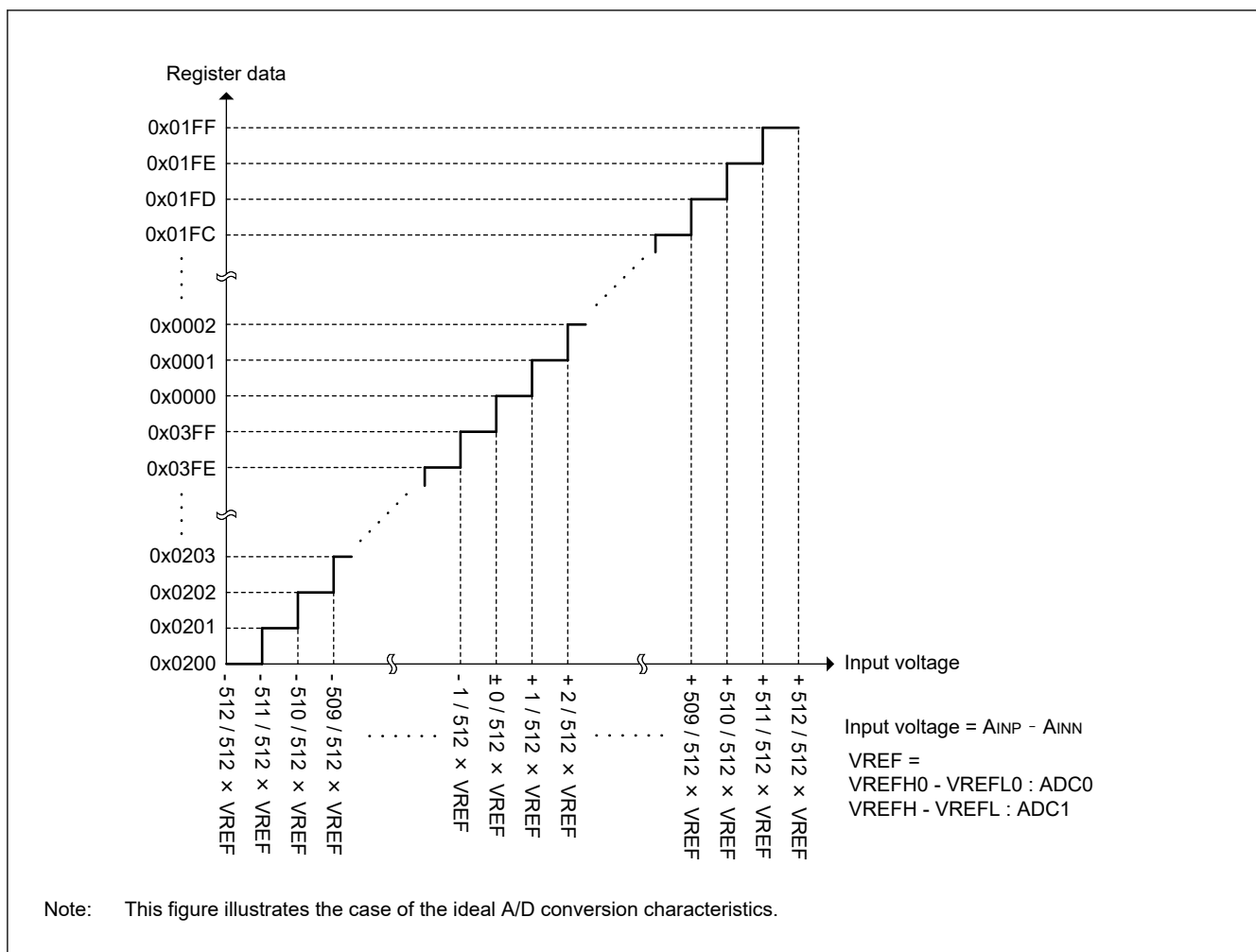
Figure 54.49 Data range of A/D conversion result (10-bit data length, Signed data, Differential input)
