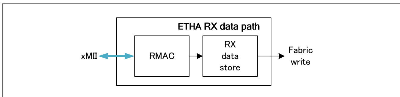
Figure 33.34 ETHA RX data path block diagram
