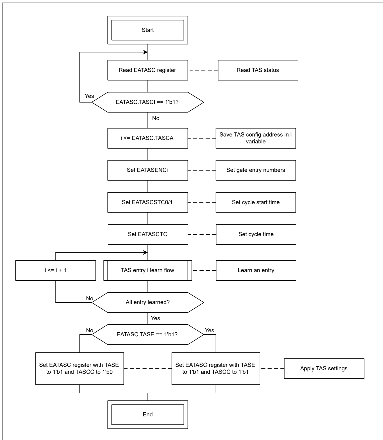
Figure 33.11 TAS setting flow
