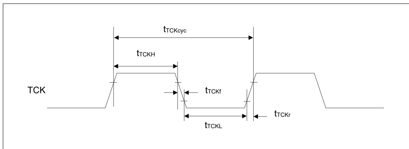
Figure 70.155 JTAG TCK timing
