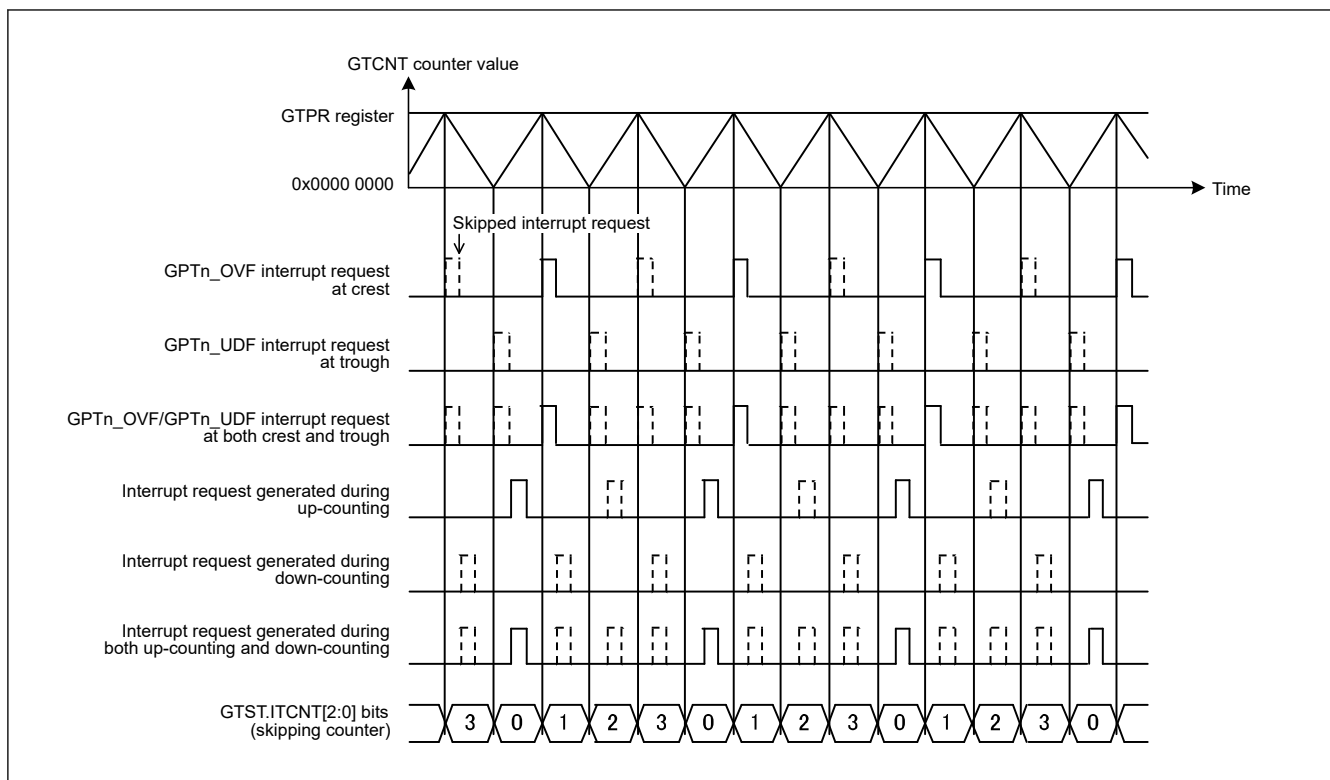
Figure 23.133 Example of Interrupt Skipping Function Operation (Triangle Waves, Counting and Skipping Both Troughs and Crests, Skipping Count: 3, Skipping Started at Down-Counting)
