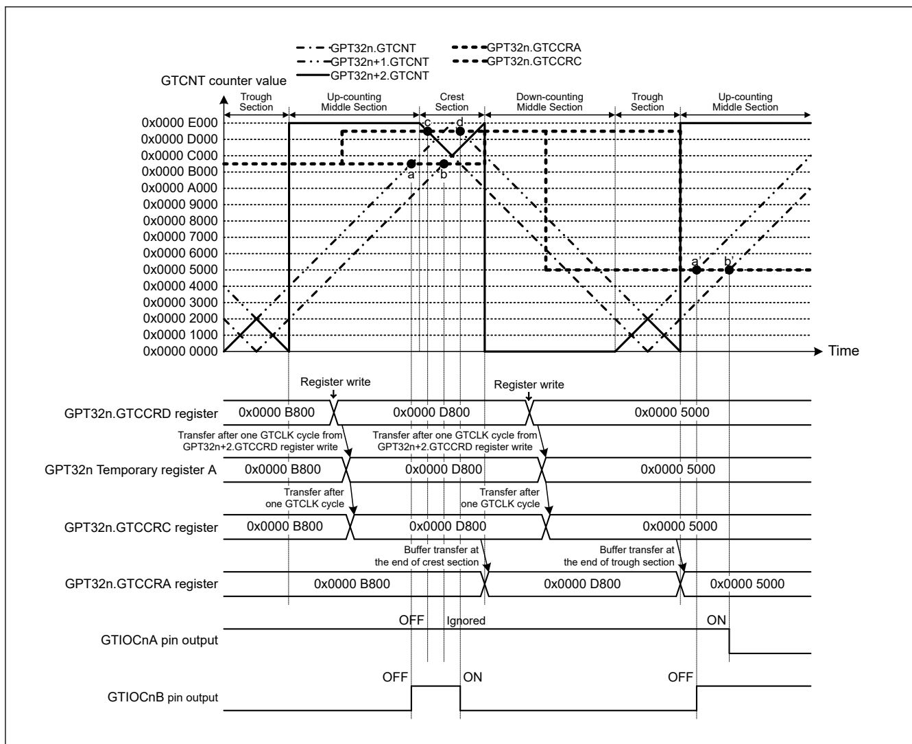
Figure 23.55 Example of Compare Match Generation Sequence Operation in Complementary PWM Mode (Complementary PWM mode 3 single buffer operation, GTIOcNA pin = Low / GTIOcNB pin = High at GTCCRA register compare match during up-counting, GTIOcNA pin = High / GTIOcNB pin = Low at GTCCRA register compare match during down-counting, the dead time value is 0x0000 2000, compare match generation order: a → c → b → d) (n = 4, 7)
