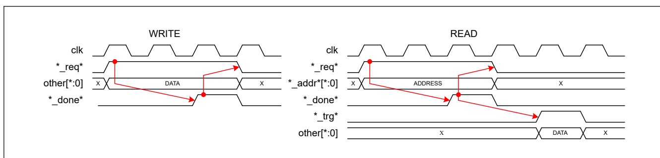
Figure 31.112 Fabric interface protocol
