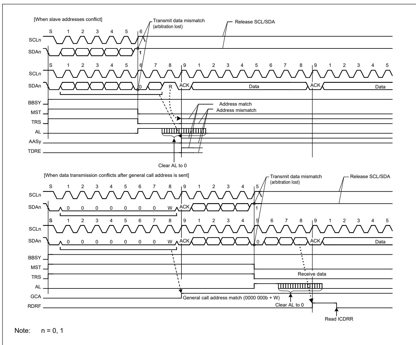
Figure 40.41 Examples of master arbitration-lost detection when MALE = 1
