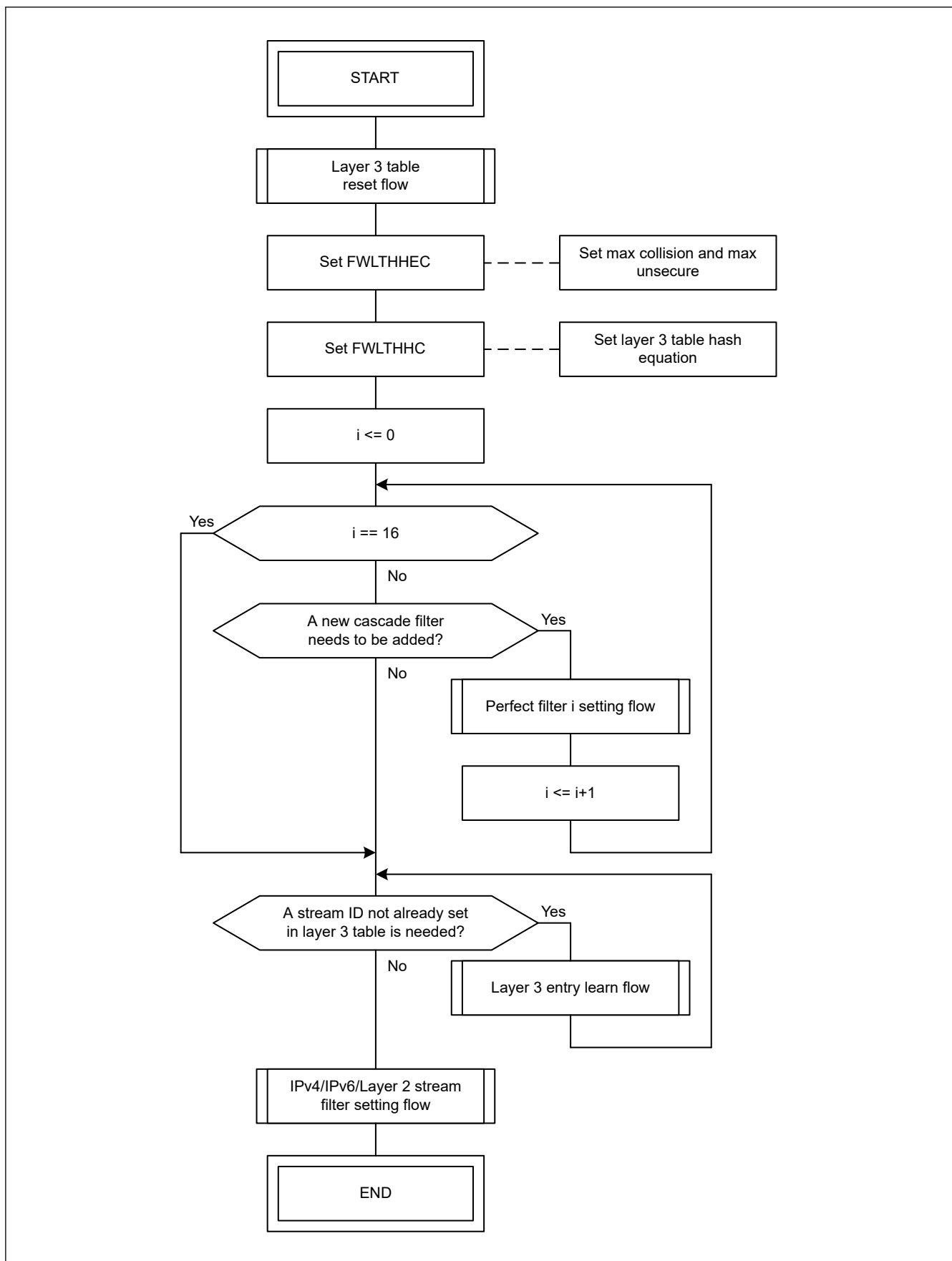
Figure 31.41 Setting flow of Layer 3 forwarding/routing/filtering
