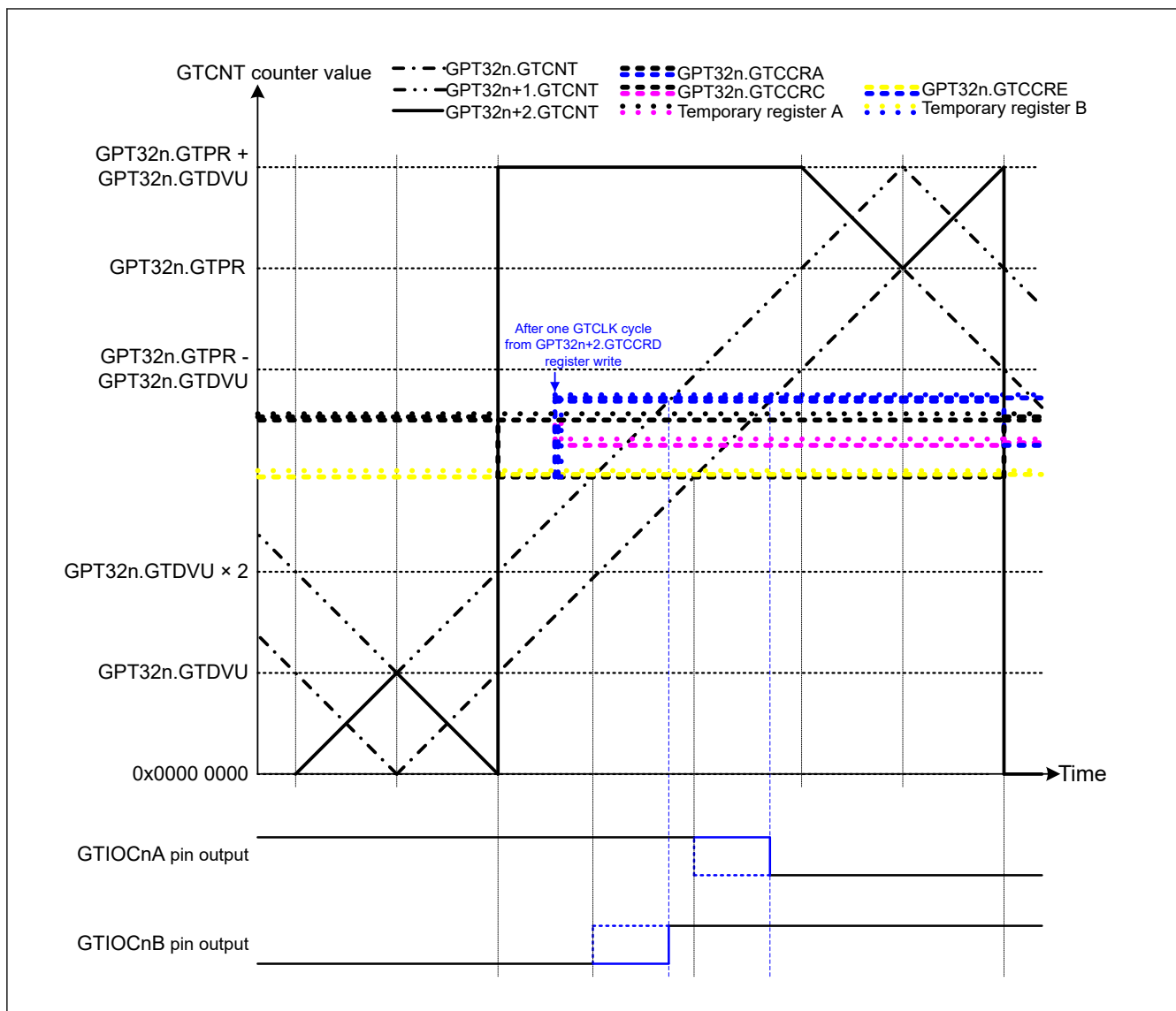
Figure 23.73 Example of Complementary PWM Mode 4 Double Buffer Operation (Up-Counting Middle Section) (Complementary PWM mode 4 double buffer operation, GTIOCnA pin = Low / GTIOCnB pin = High at GTCCRA register compare match during up-counting, GTIOCnA pin = High / GTIOCnB pin = Low at GTCCRA register compare match during down-counting, when a value larger than the GPT32n+1.GTCNT value is written to GTCCRF register before up-counting compare match) (n = 4, 7)
