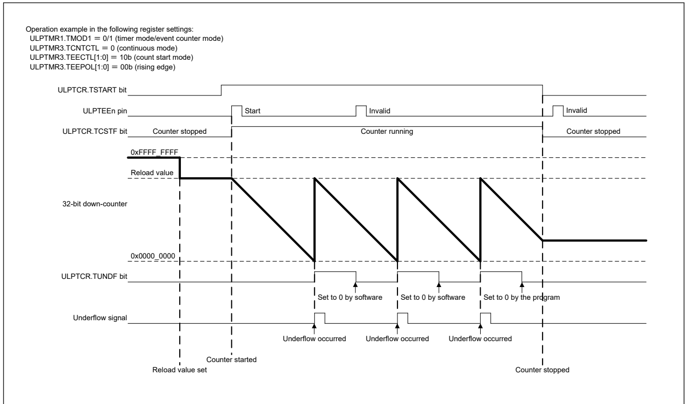
Figure 26.9 Operation example in common, continuous, and count start modes
