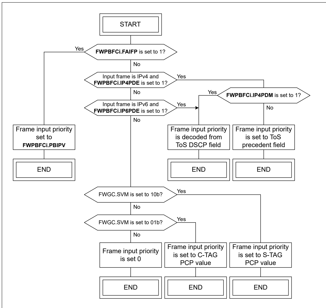
Figure 31.47 Priority assignment of frame input for port i
