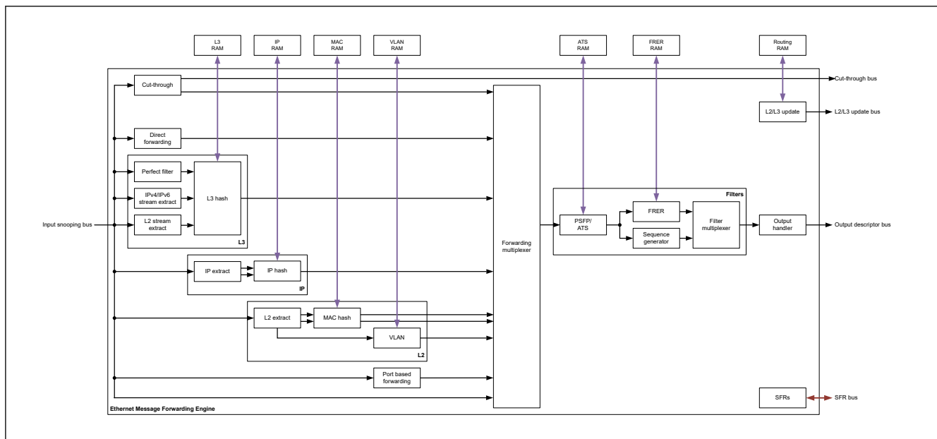
Figure 31.1 MFWD block diagram
