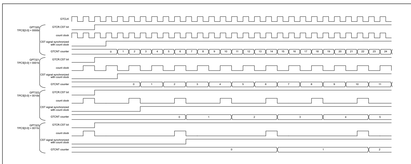
Figure 23.95 Example of Simultaneous Start Operation by Software (with Different Count Period)
