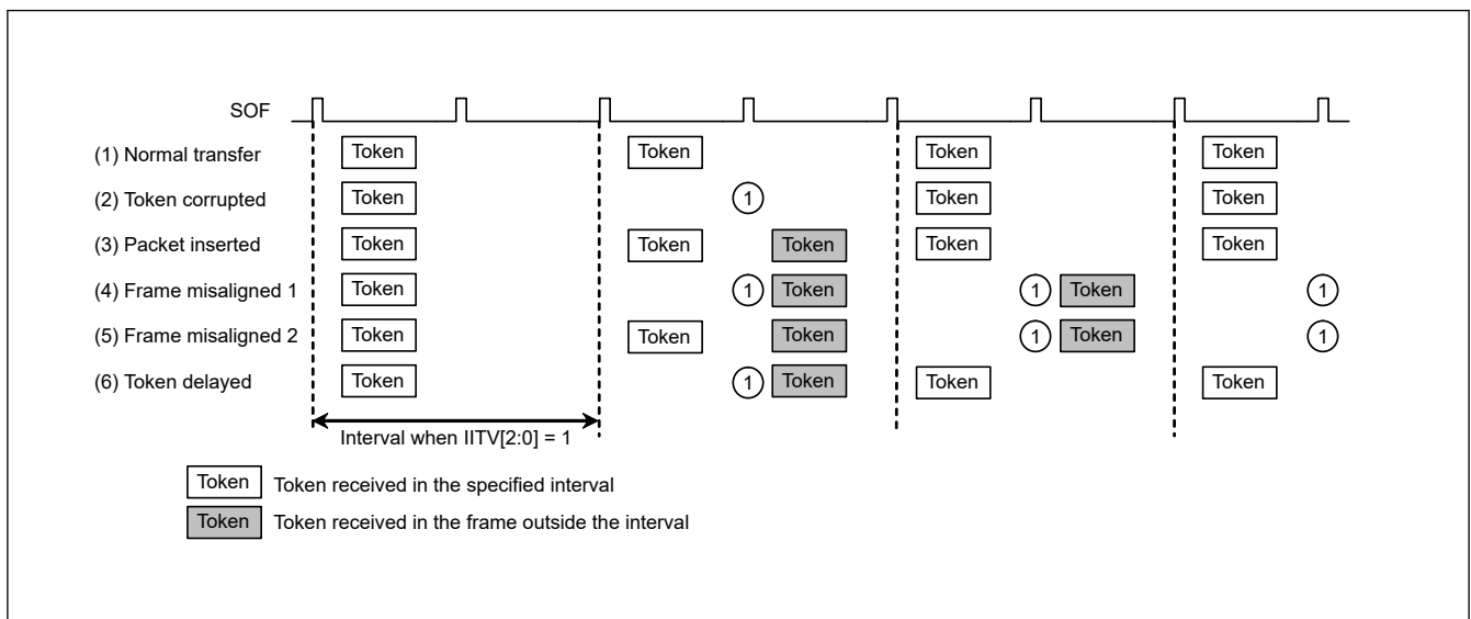
Figure 38.18 Example interval error occurrence when PIPEPERI.IITV[2:0] = 1
