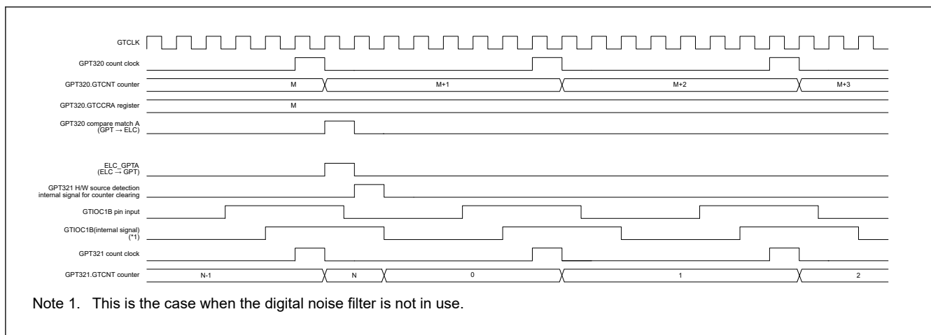
Figure 23.92 Examples of the Timing of Operations for Counter Clearing in Response to Event Input from the ELC_GPTA (During Counting Triggered by Hardware Source)
