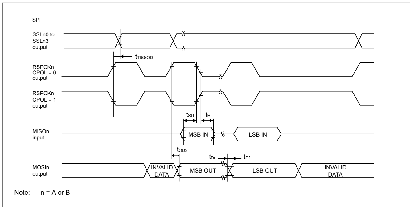
Figure 70.78 SPI timing for TI SSP master
