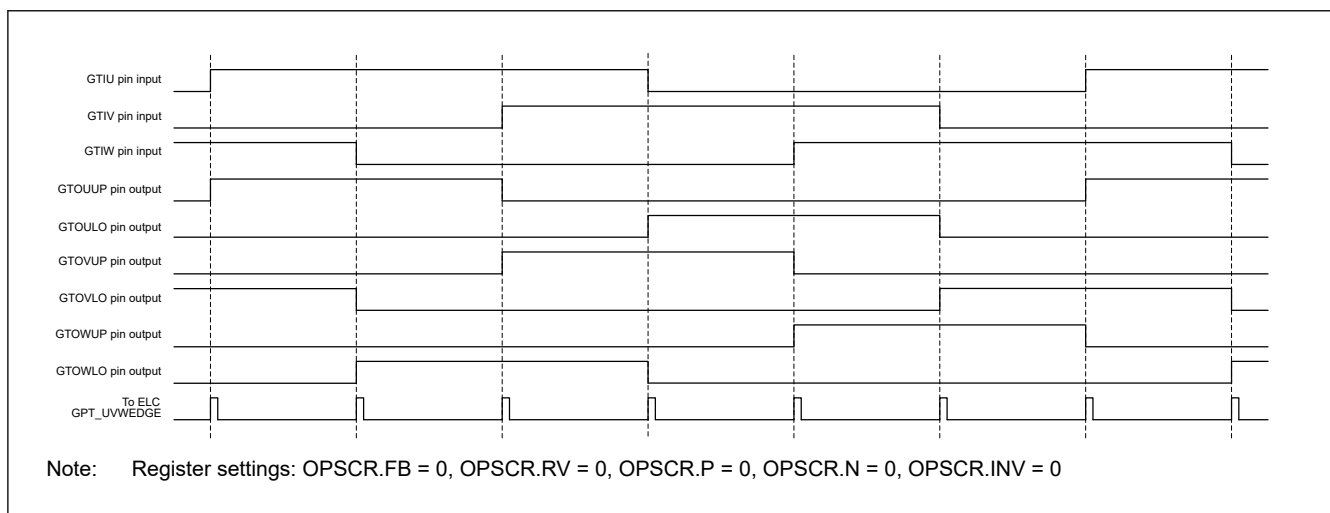
Figure 23.122 Example of GPT OPS Level Output Operation (Forward Rotation)
