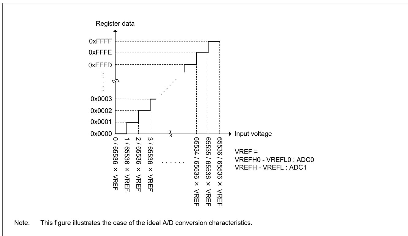
Figure 54.44 Data range of A/D conversion result (16-bit data length, Unsigned data, Single-ended input)
