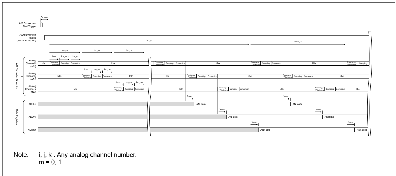
Figure 54.60 A/D conversion processing time (Hybrid mode)
