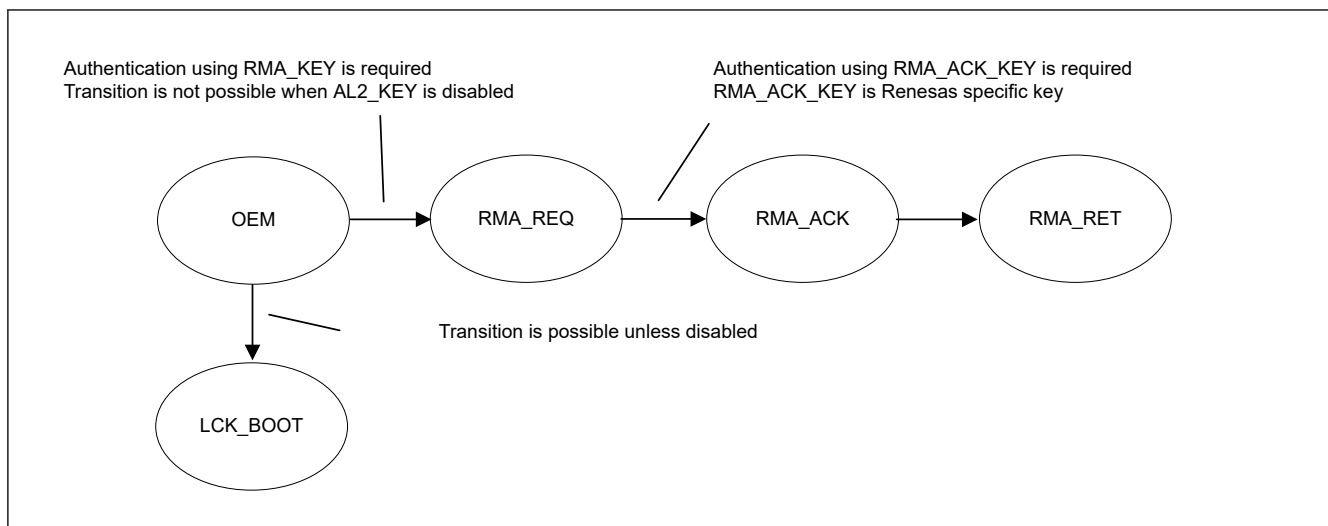
Figure 52.7 Device lifecycle states
