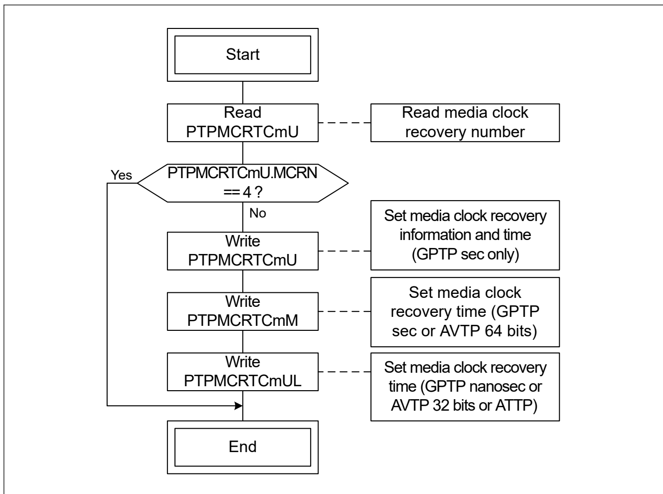
Figure 36.11 Media clock recovery time value setting flow
