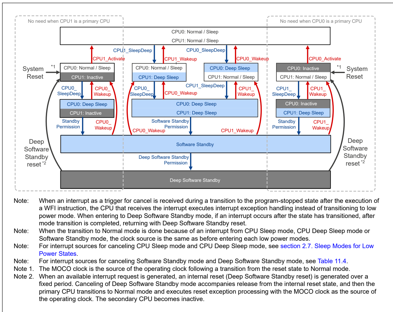
Figure 11.1 Low power mode transitions
