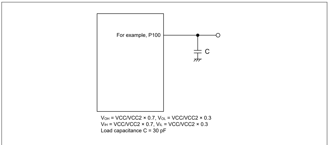
Figure 70.1 Input or output timing measurement conditions
