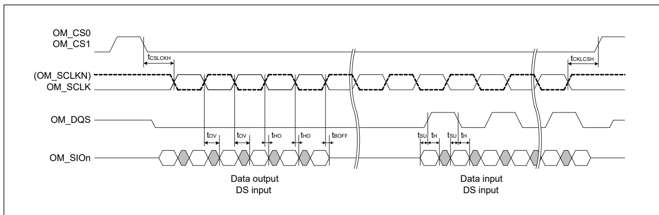
Figure 70.85 DDR transmit/receive timing (4S-4D-4D, 8D-8D-8D)
