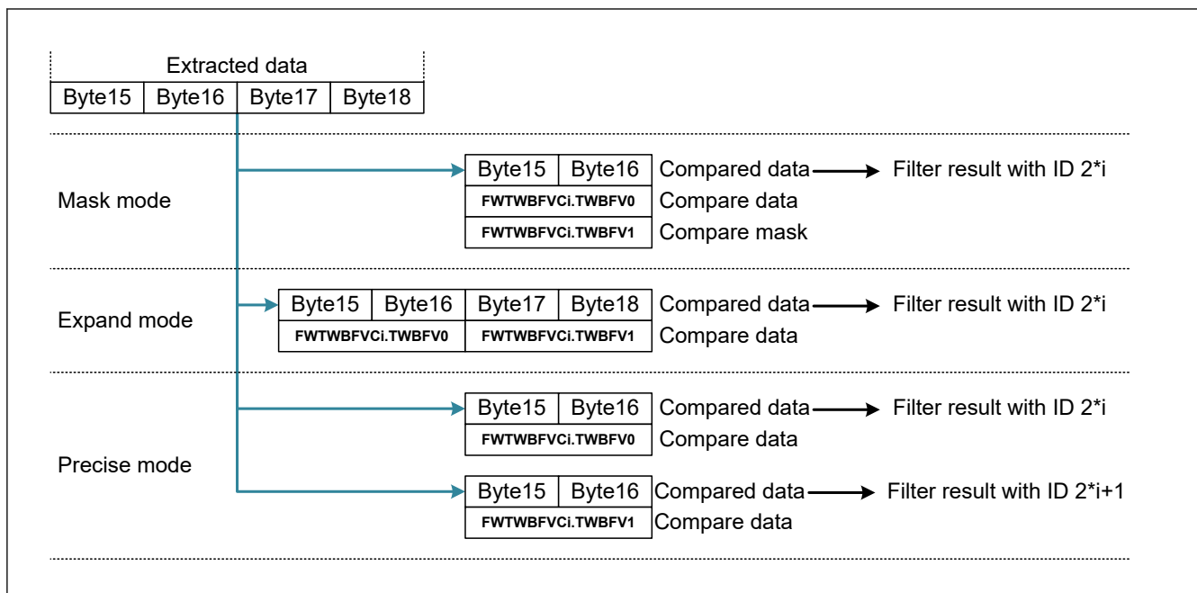
Figure 31.64 2-byte filter data extraction for filtering
