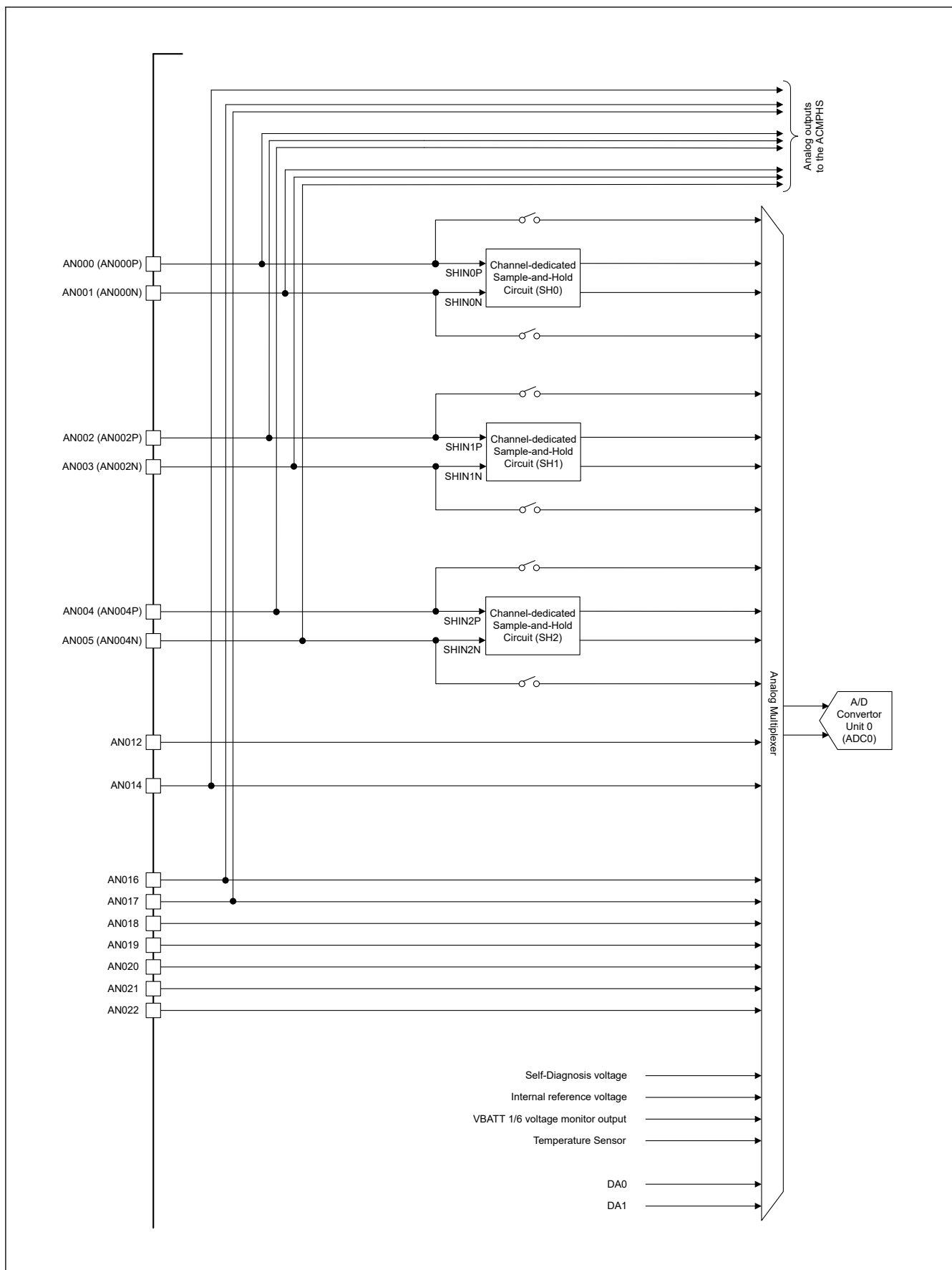
Figure 54.2 Analog channel structure for A/D converter unit 0
