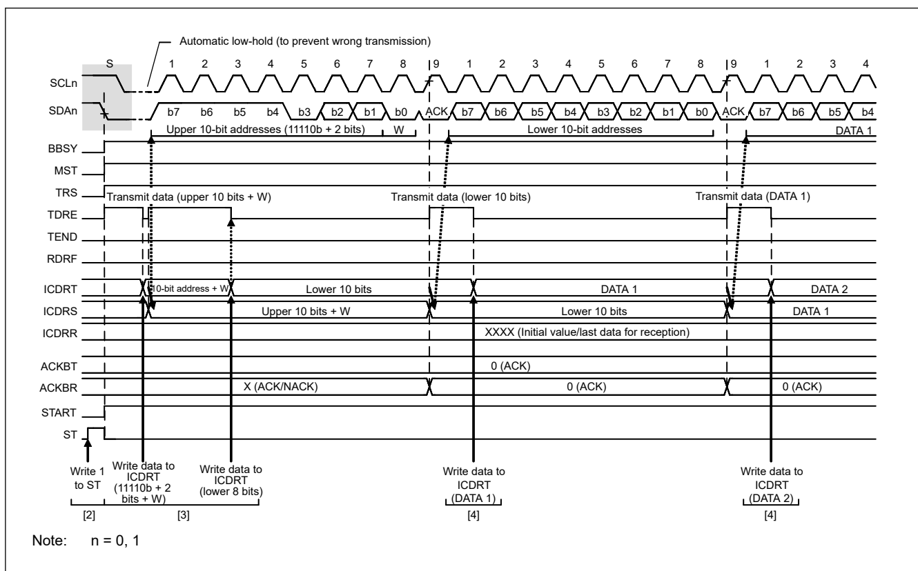
Figure 40.8 Master transmit operation timing (2) with 10-bit address format
