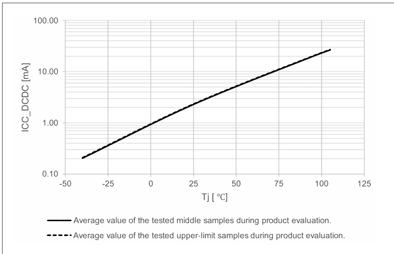
Figure 70.6 Temperature dependency in Software Standby mode ( ICC\_DCDC , SS2LP\_1 , SVSCR\_5 ) (reference data)
