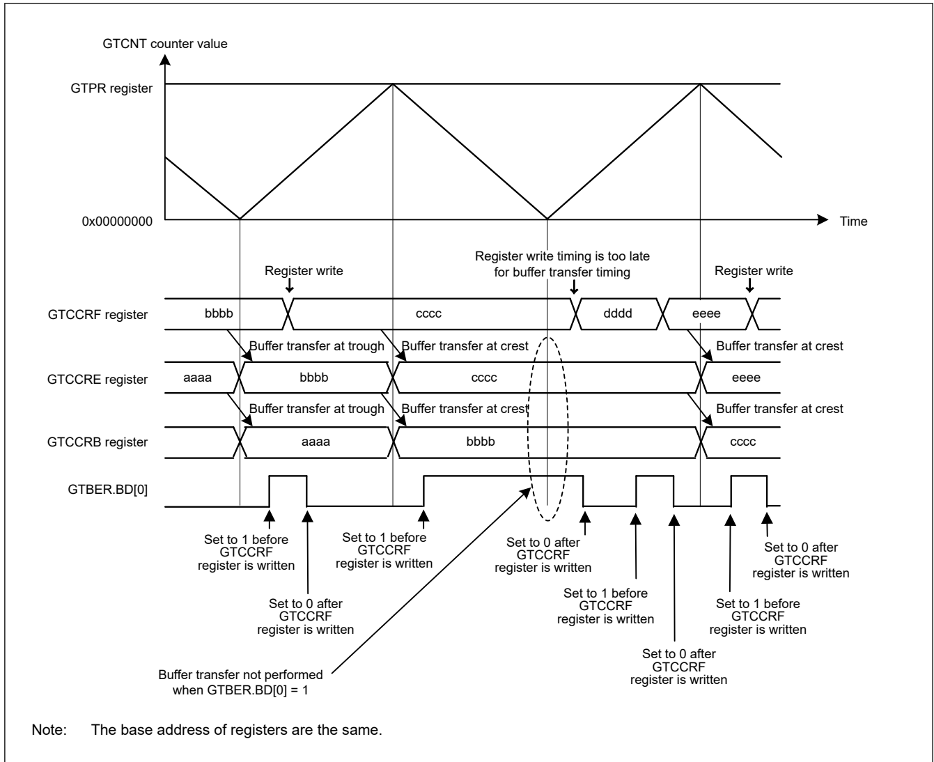
Figure 23.153 Example of operation for disabling buffer operation with triangle waves, double buffer operation, and buffer transfer at both troughs and crests
