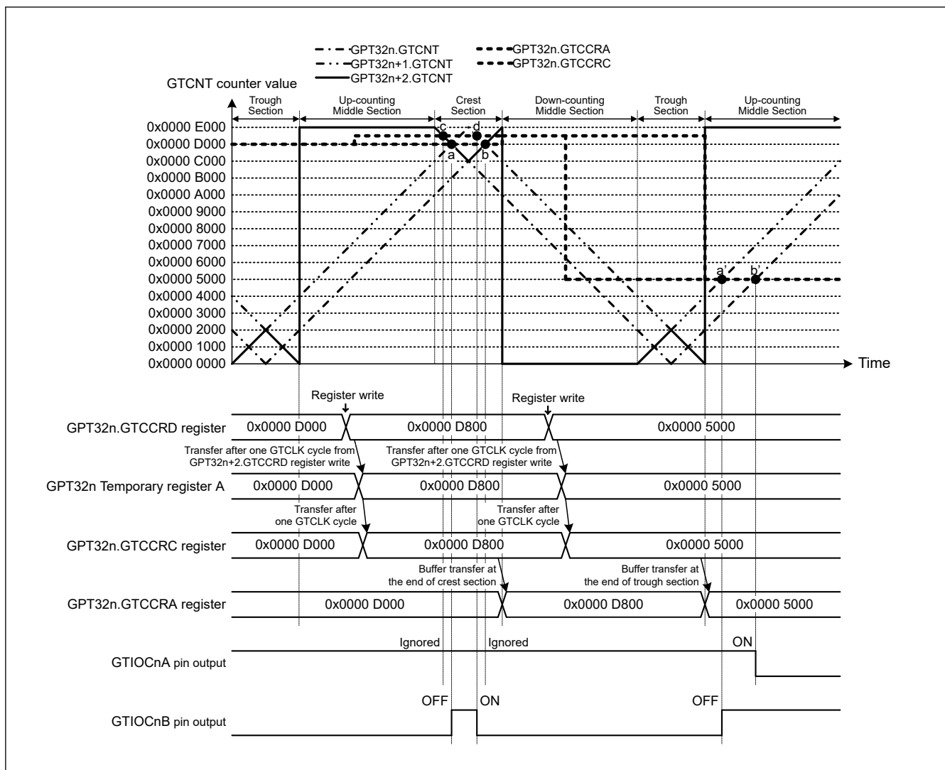
Figure 23.57 Example of Compare Match Generation Sequence Operation in Complementary PWM Mode (Complementary PWM mode 3 single buffer operation, GTIOCnA pin = Low / GTIOCnB pin = High at GTCCRA register compare match during up-counting, GTIOCnA pin = High / GTIOCnB pin = Low at GTCCRA register compare match during down-counting, the dead time value is 0x0000 2000, compare match generation order: c → a → d → b) (n = 4, 7)
