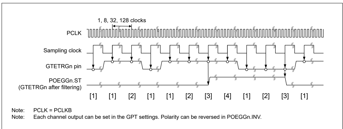
Figure 22.4 Output timing of external trigger to the GPT
