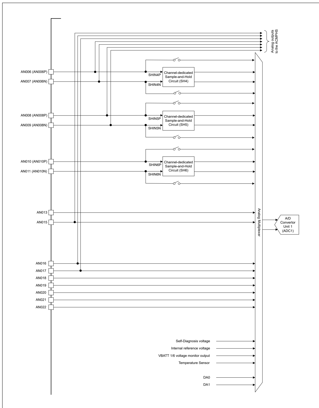
Figure 54.3 Analog channel structure for A/D converter unit 1
