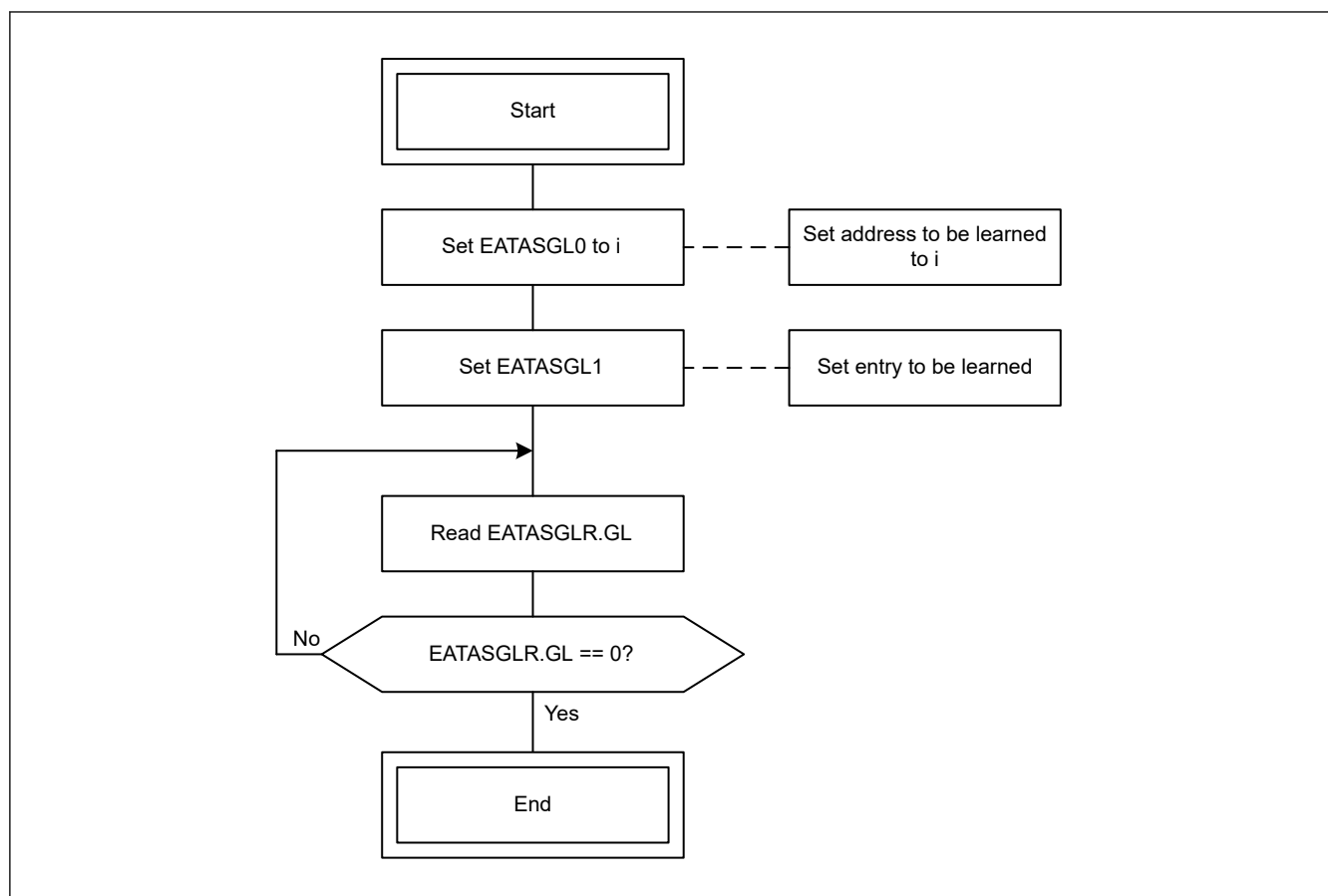
Figure 33.14 TAS entry i learn flow
