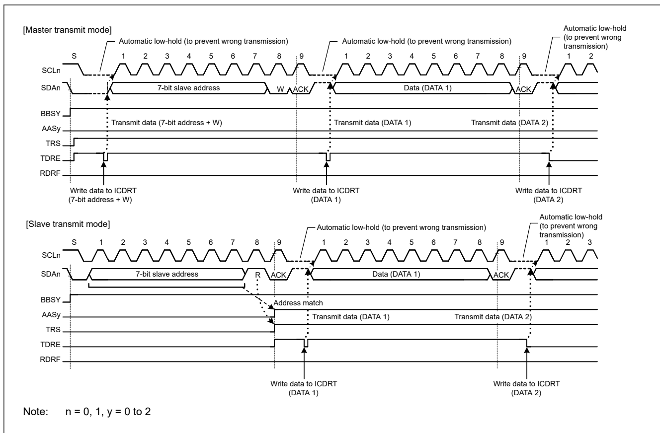
Figure 40.38 Automatic low-hold operation in transmit mode
