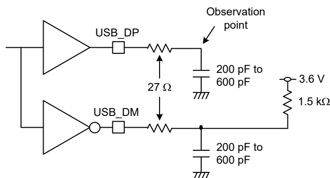
Figure 70.127 Test circuit in low-speed mode
