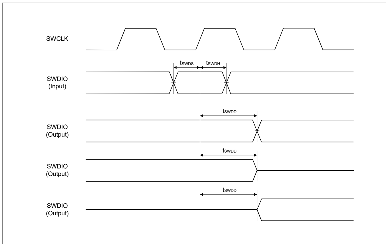
Figure 70.158 SWD input/output timing
