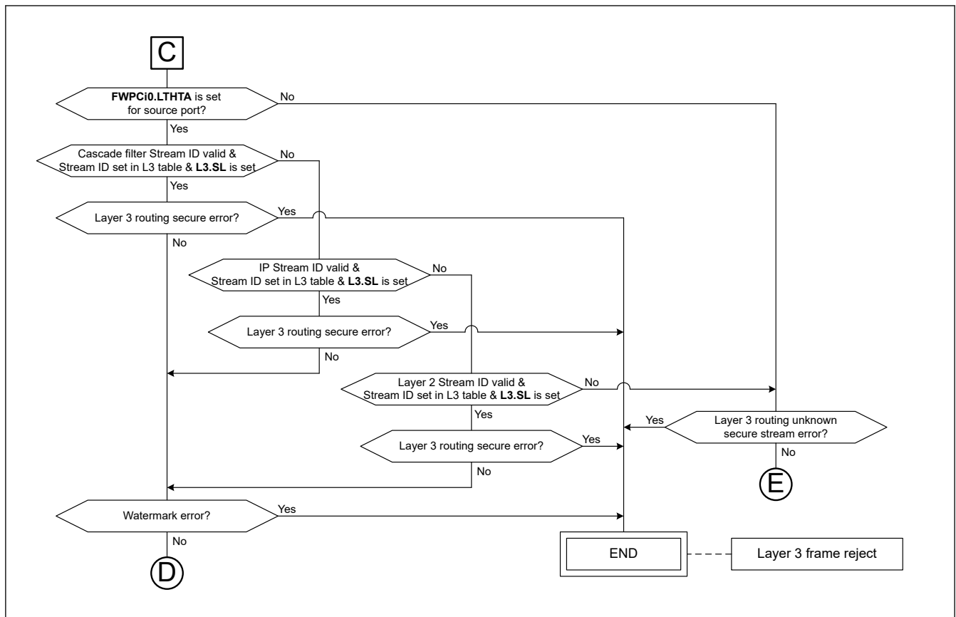
Figure 31.85 Layer 3 forwarding/routing secure flow
