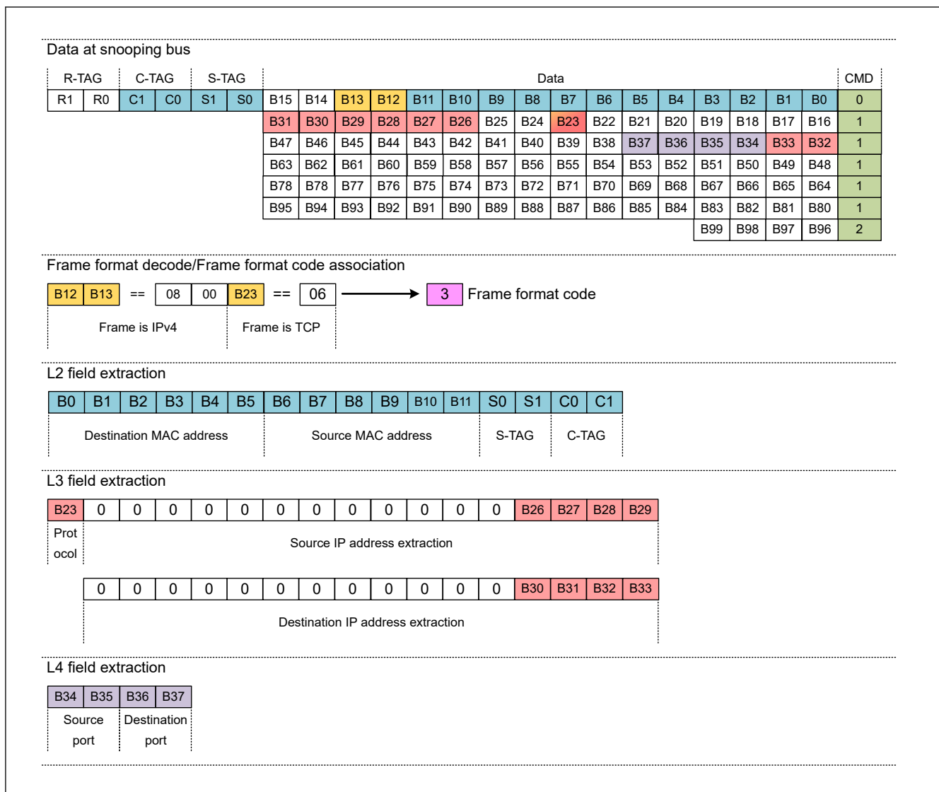
Figure 31.75 IPv4/TCP detection and data extraction
