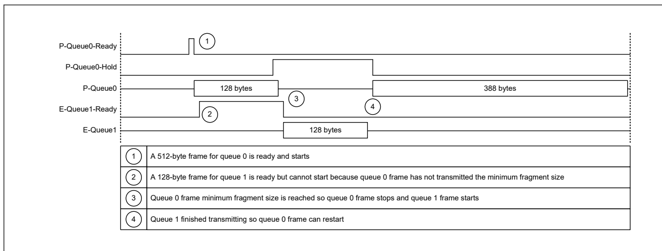
Figure 33.32 E-frame and p-frame transmission (EATPEC.AFS == 01)
