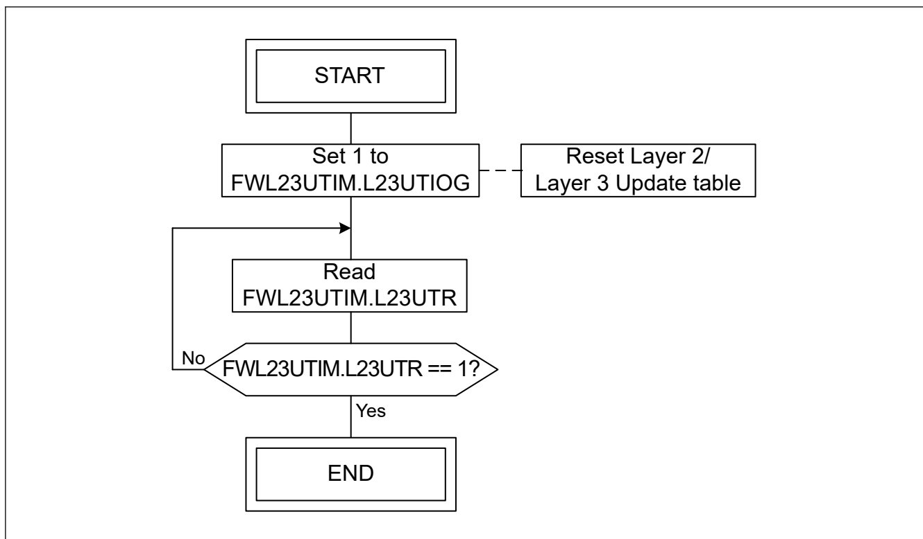
Figure 31.24 Reset flow of Layer 2/Layer 3 Update table
