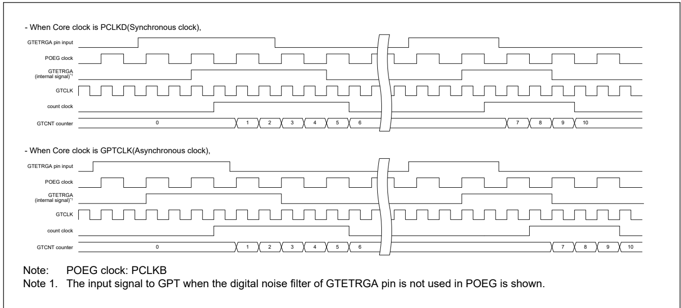
Figure 23.119 Example of External pulse width measuring function(Up-counting)
