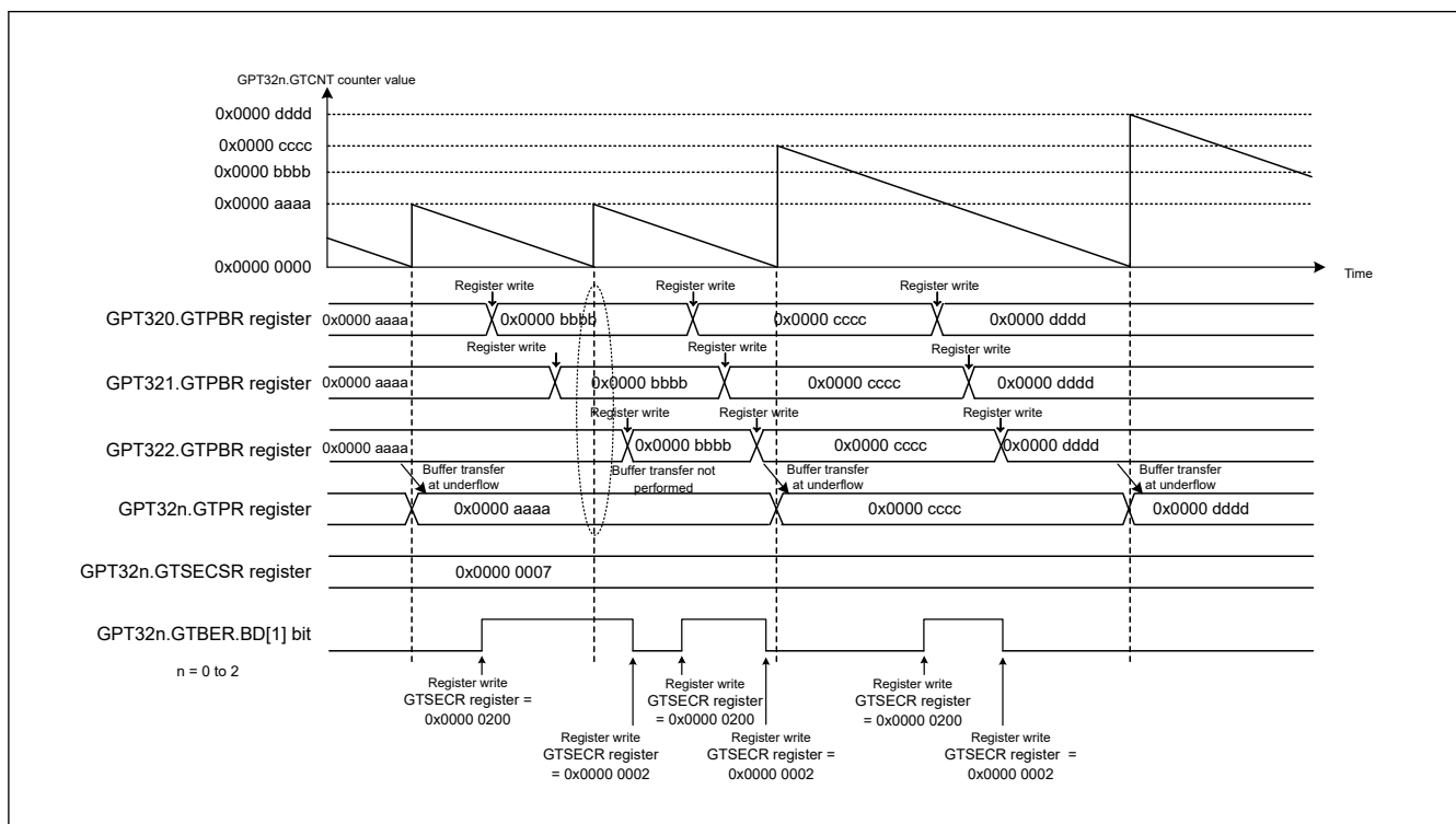
Figure 23.155 Example of Multiple Channel Operation for Disabling Buffer Operation (Saw Waves, Single Buffer Operation)
