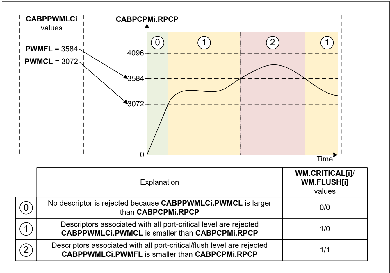
Figure 32.13 Example for per-port level-based watermark setting for port i
