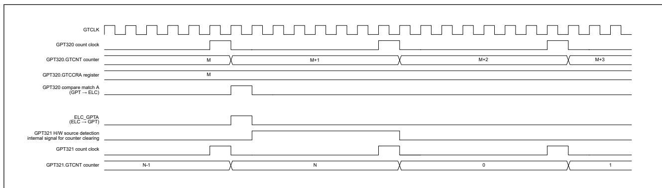
Figure 23.91 Examples of Timing of Operations for Counter Clearing in Response to Event Input from the ELC_GPTA (During the Counting of Cycles of Clock Signal Produced by Dividing the GTCLK Frequency)
