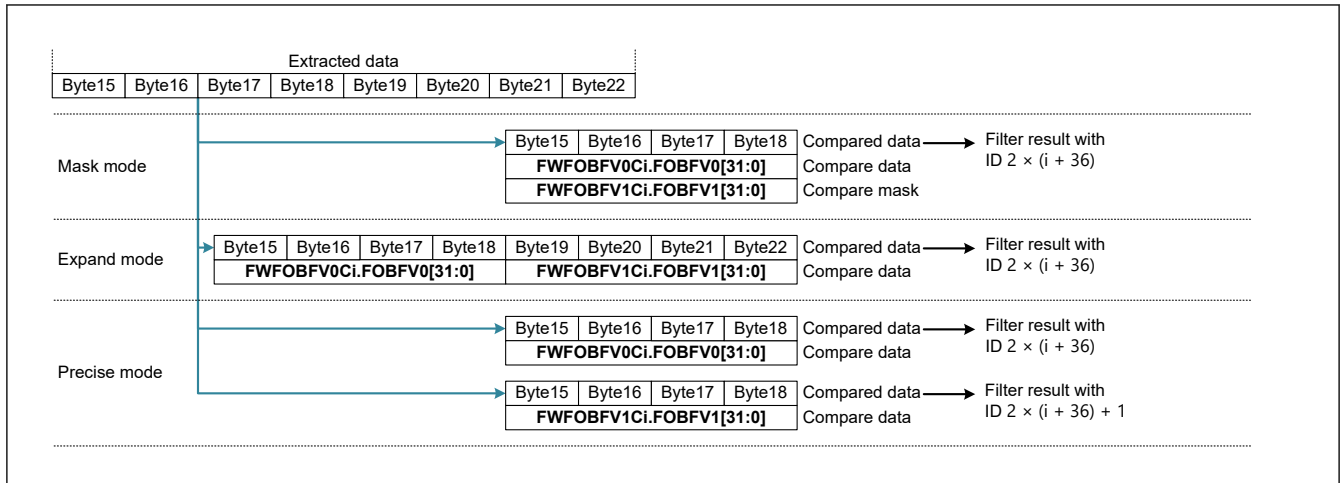
Figure 31.68 4-byte filter data extraction for filtering
