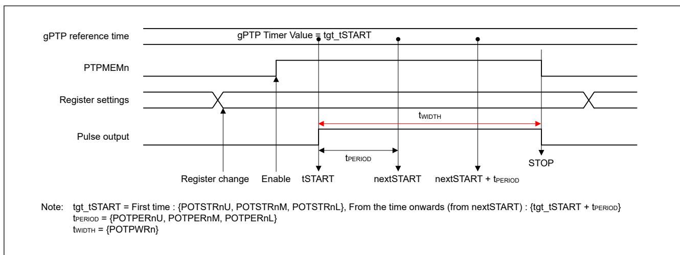
Figure 36.17 Pulse output H width register \geq when the POTCRn.START bit is changed from 0 to 1 by setting the pulse output cycle
