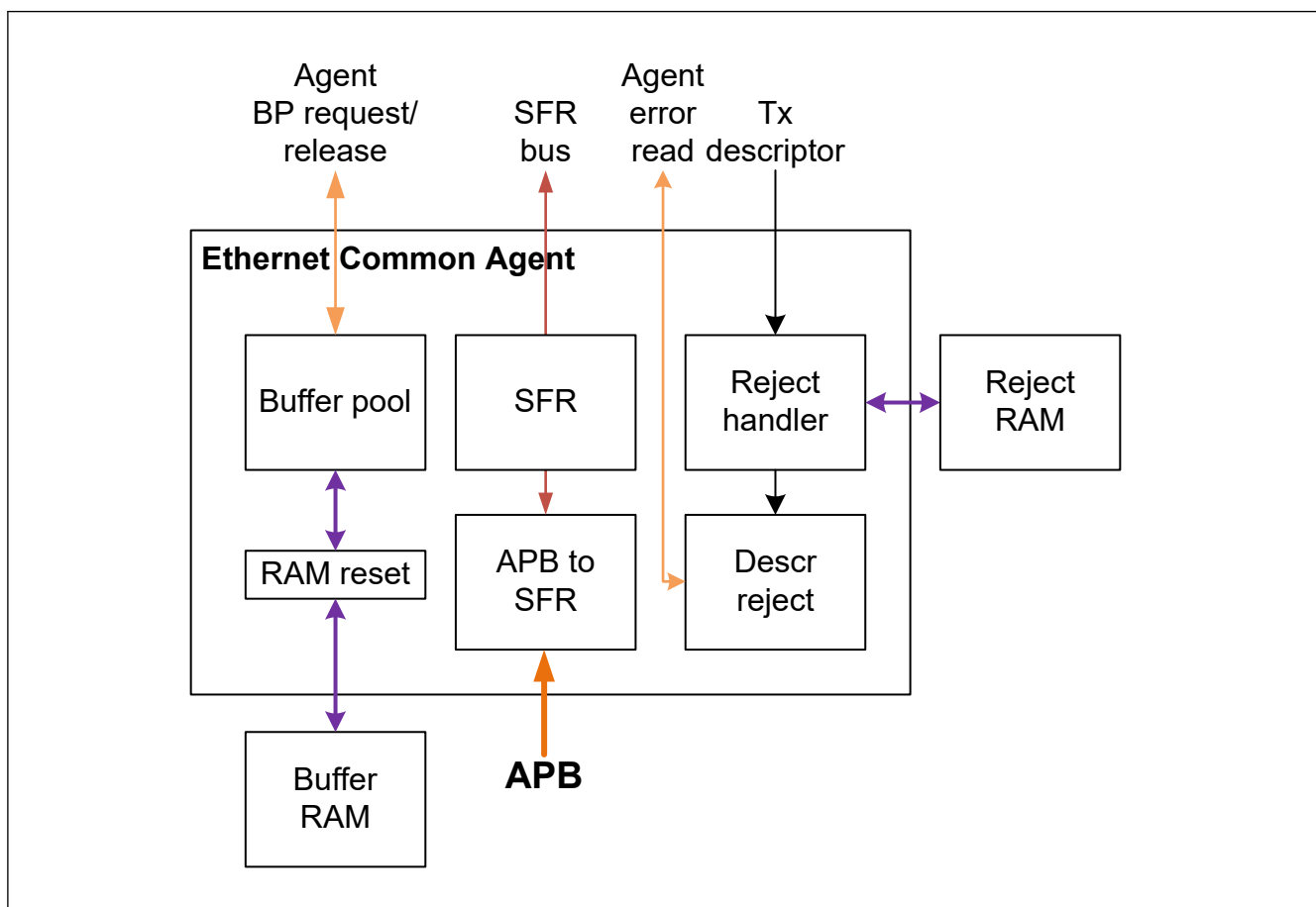
Figure 32.1 COMA block diagram
