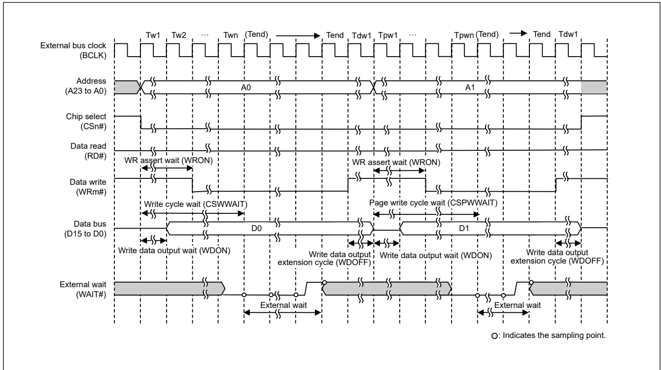
Figure 15.27 Example external wait timing for page write access to 16-bit bus space in byte strobe mode (when 1/1 BCLK is selected with the BCLK Pin Output Select bit ( n = 0 to 7 , m = 0, 1 ))
