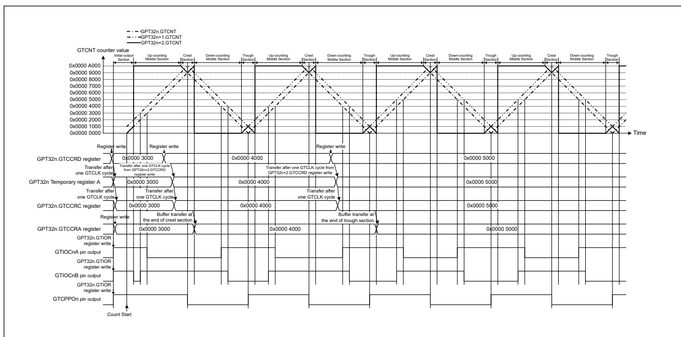
Figure 23.49 Example of Complementary PWM Mode 3 Operation (Single buffer operation, GTIOCnA pin = High / GTIOCnB pin = High as initial output, GTIOCnA pin = Low / GTIOCnB pin = High at GTCCRA register compare match during up-counting, GTIOCnA pin = High / GTIOCnB pin = Low at GTCCRA register compare match during down-counting, the dead time value is 0x0000 1000 and updating GTCCRD register in middle section) (n = 4, 7)
