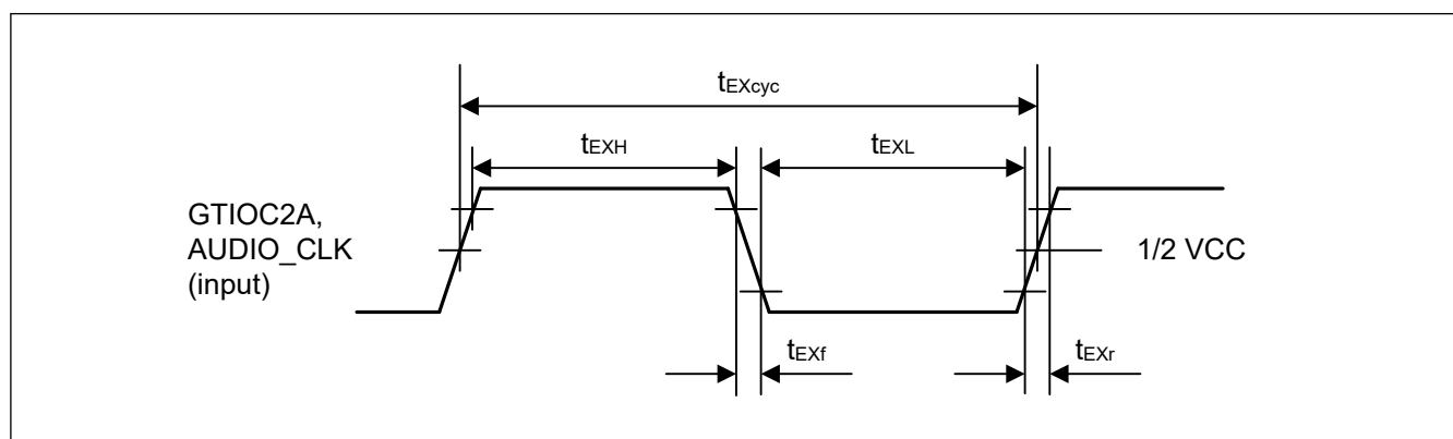
Figure 70.103 Clock input timing
