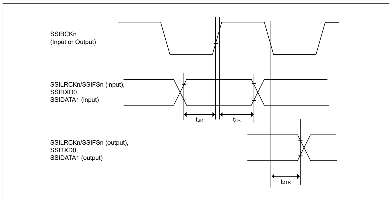
Figure 70.104 SSIE data transmit and receive timing when SSICR.BCKP = 0
