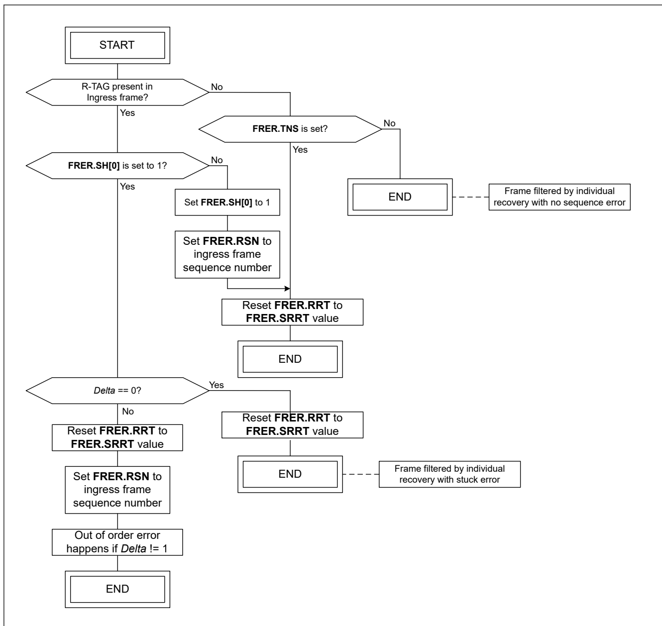
Figure 31.107 Individual recovery match algorithm
