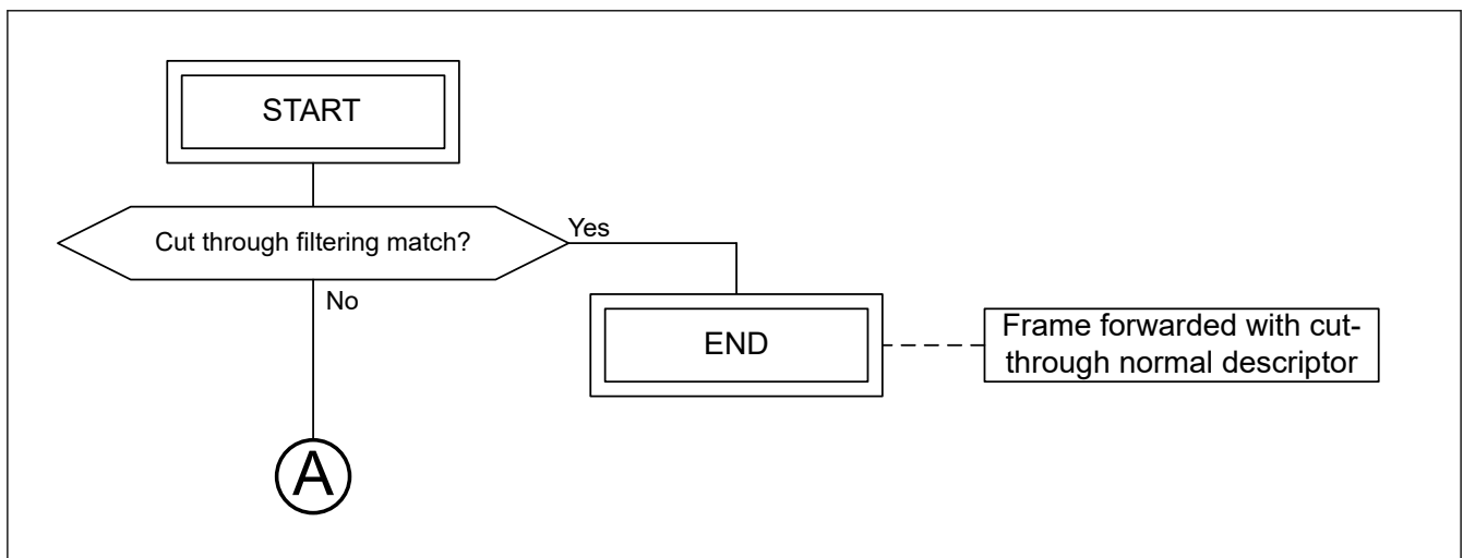
Figure 31.53 Cut-through forwarding flow
