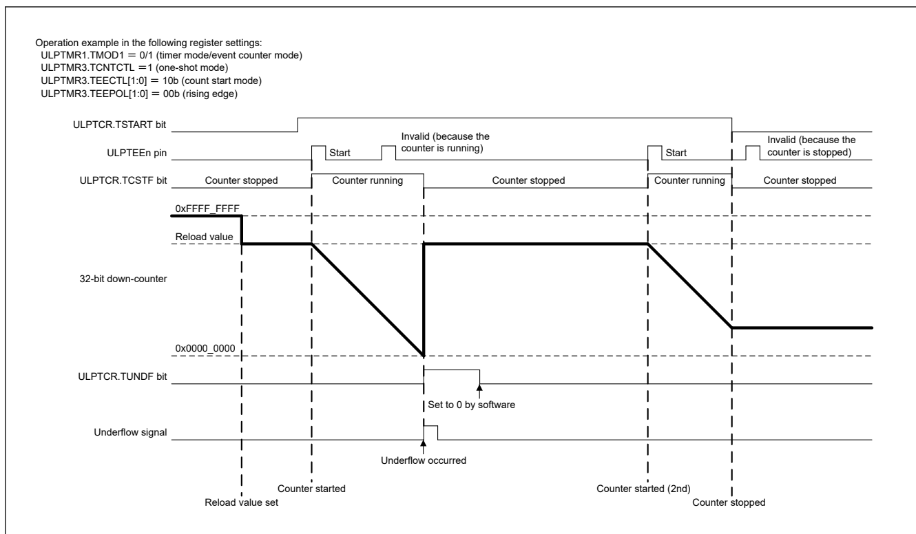
Figure 26.11 Operation example in common, one-shot, and count start modes
