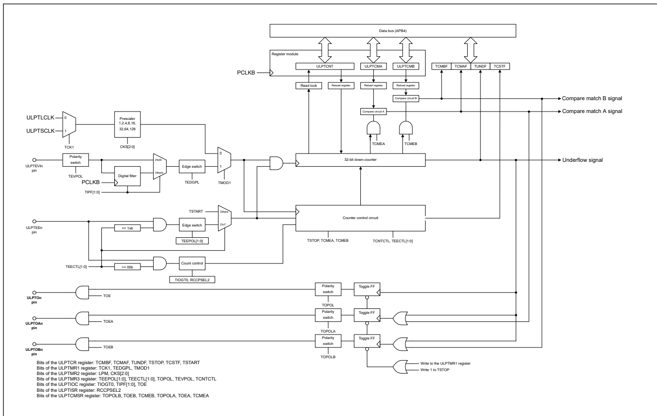
Figure 26.1 ULPT block diagram
