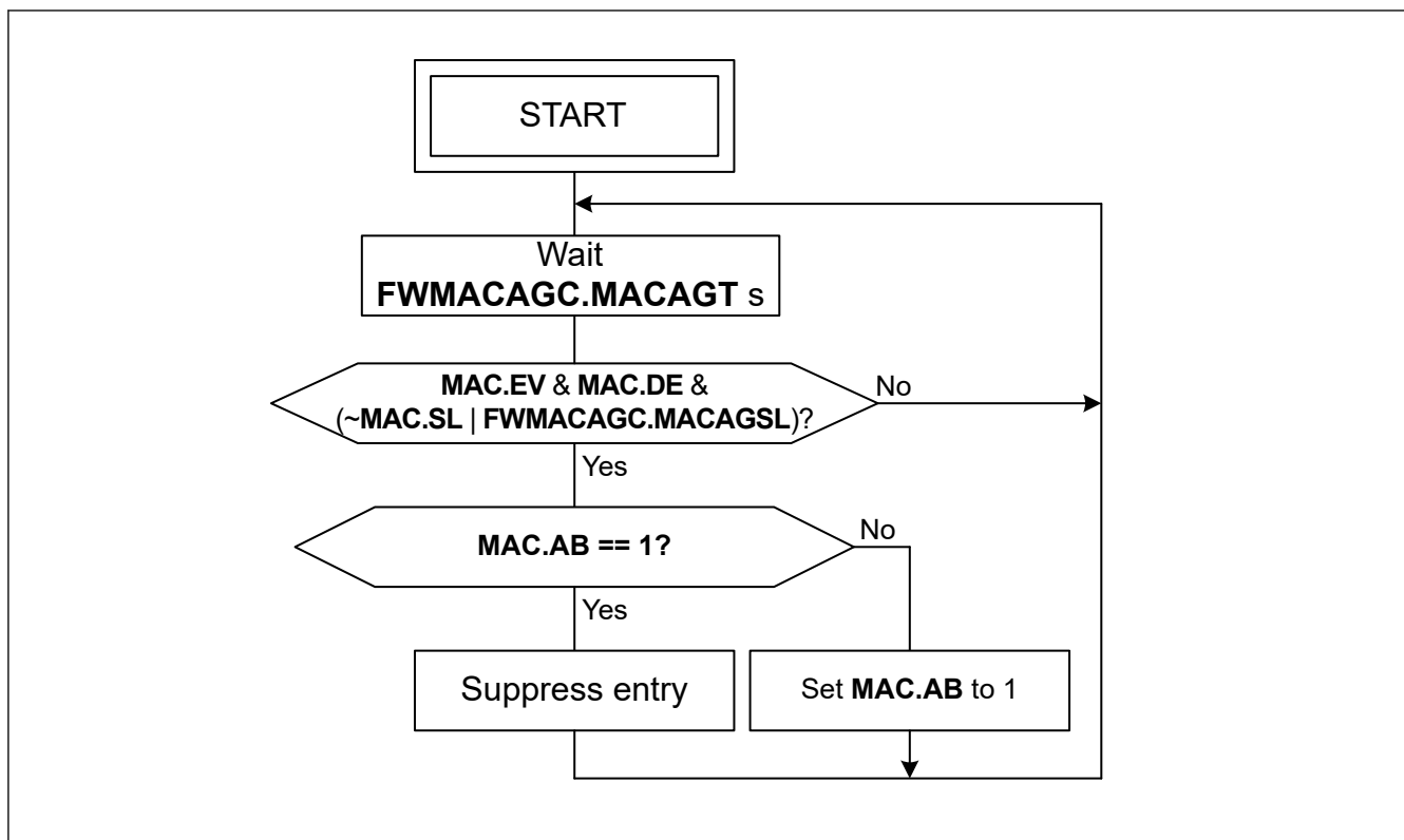
Figure 31.93 MAC aging algorithm
