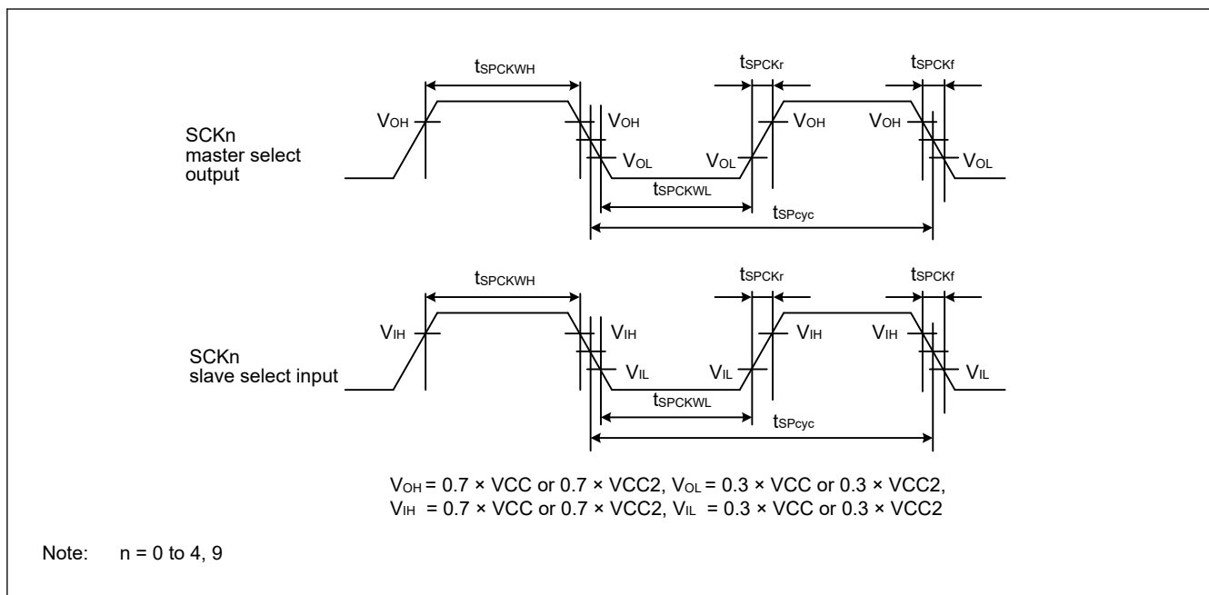
Figure 70.69 SCKn simple SPI mode clock timing
