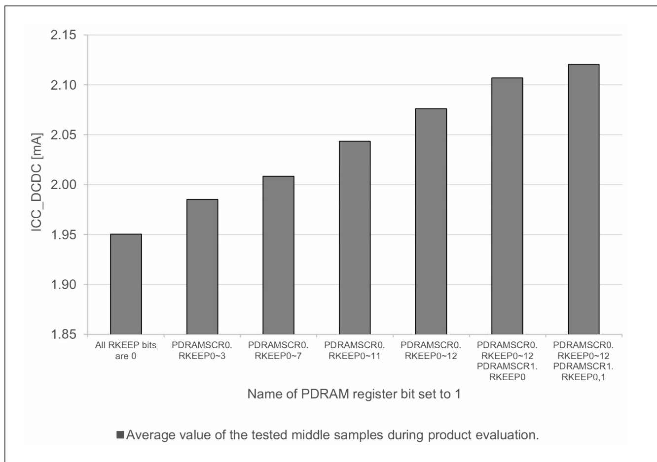
Figure 70.15 Software Standby current per SRAM state (ICC_DCDC, SS2LP_1, SVSCR_2) (reference data)
