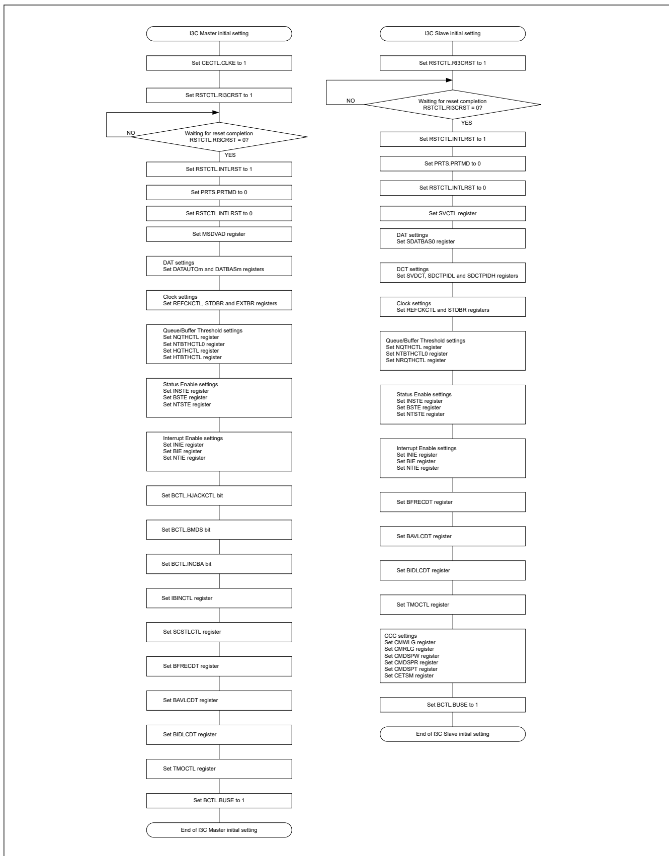
Figure 41.141 Example of each initialization flowchart for I3C master mode and slave mode
