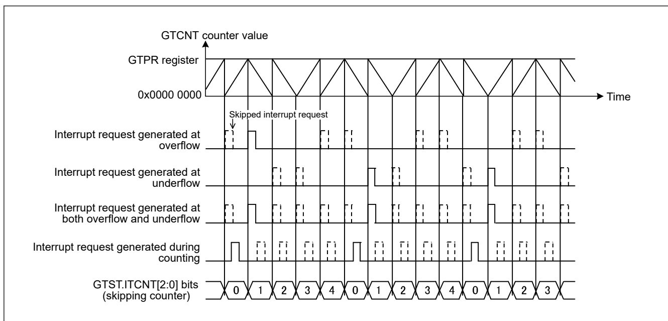
Figure 23.134 Example of Interrupt Skipping Function Operation (Saw Waves, Operation with Count Direction Changed, Counting and Skipping Both Overflows and Underflows, Skipping Count: 4)
