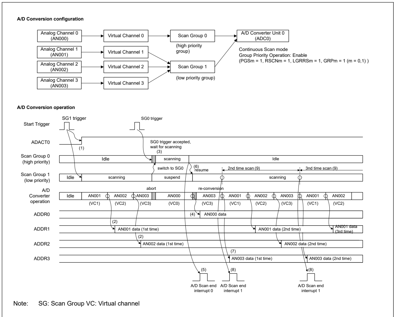
Figure 54.29 Example of group priority operation in SAR mode – Continuous scan mode (2 groups)
