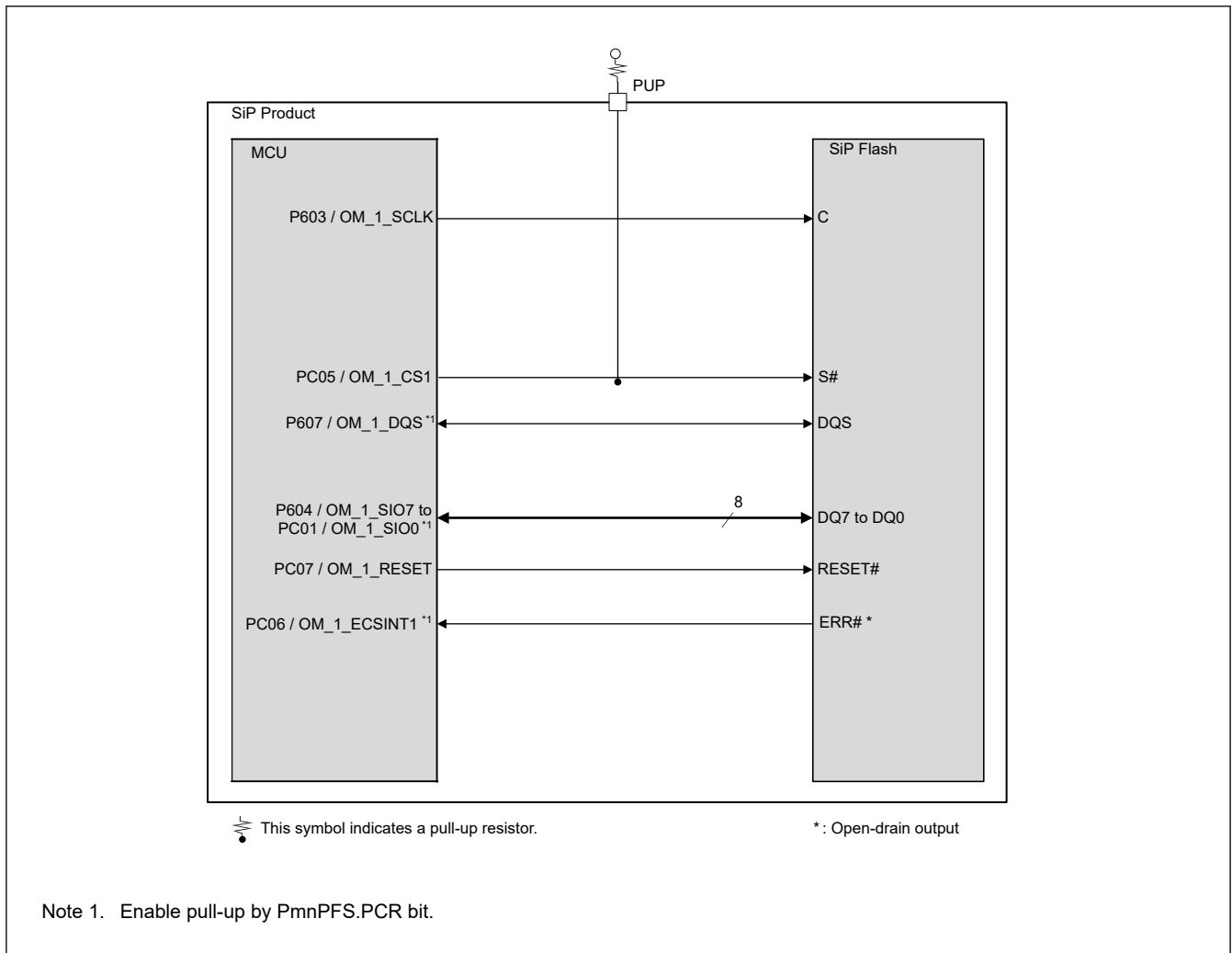
Figure 45.32 Connection between the MCU and the SiP Flash memory
