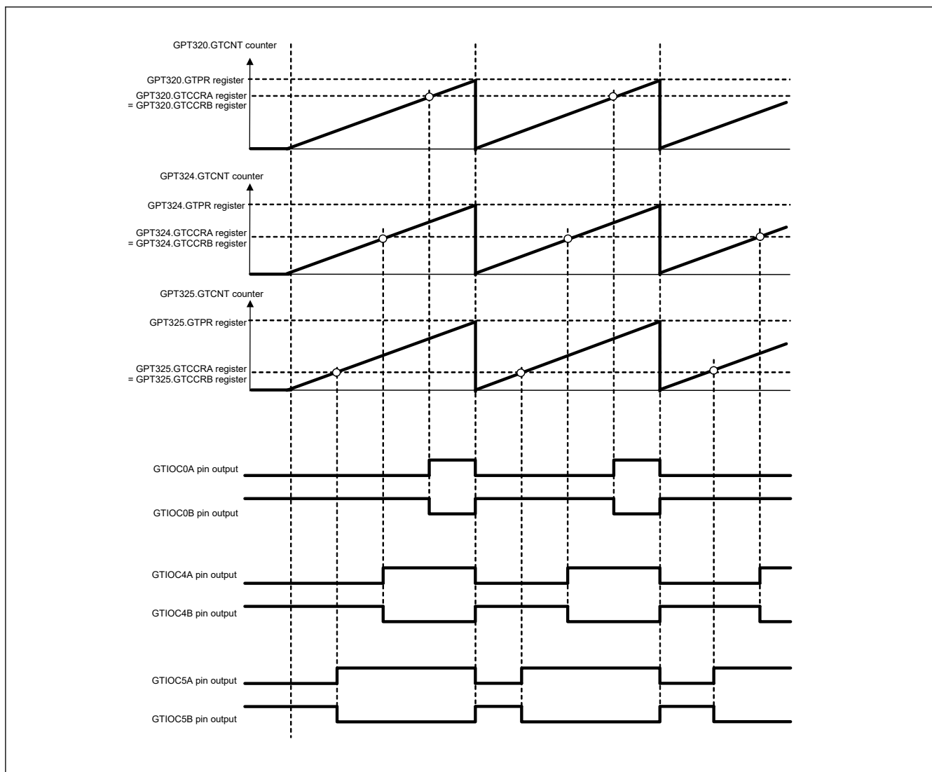
Figure 23.102 Example of 3-phase saw-wave complementary PWM output
