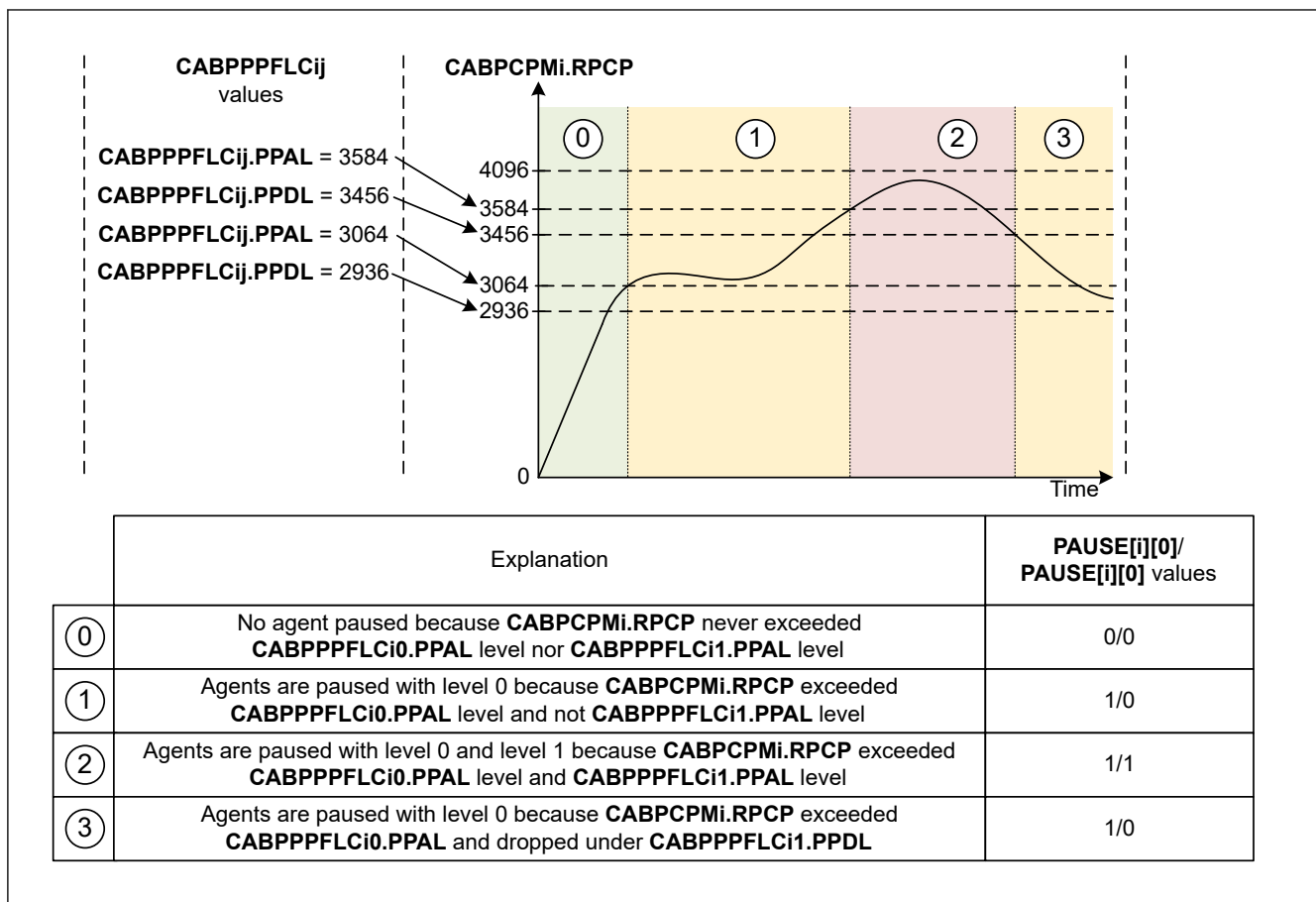
Figure 32.15 Example for per-port pause function setting for port i
