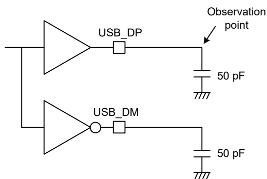
Figure 70.133 Test circuit in full-speed mode
