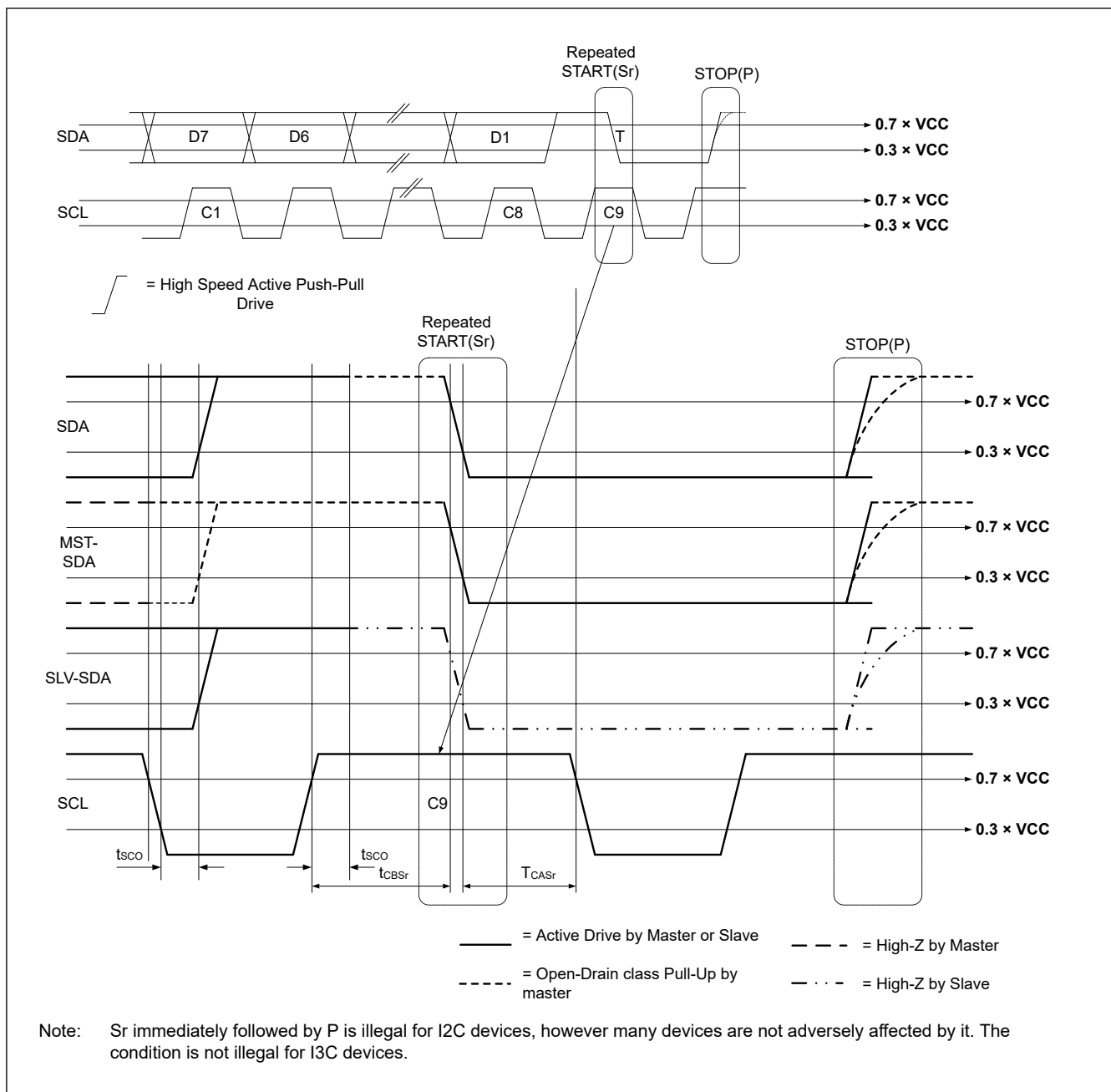
Figure 70.99 T-Bit When Master Ends Read with Repeated START and STOP
