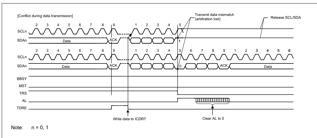
Figure 40.44 Example of slave arbitration-lost detection when SALE = 1
