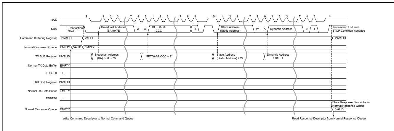
Figure 41.15 Dynamic address assign procedure (SETDASA CCC) timing
