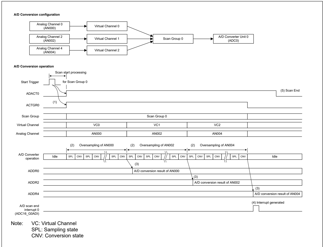
Figure 54.9 Example of scanning operation in Oversampling mode – Single scan mode
