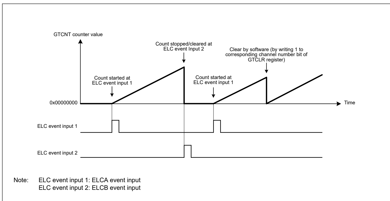
Figure 23.88 Examples of count clearing operation by hardware source in saw wave up-counting, started at ELCA input, and stopped/cleared at ELCB input
