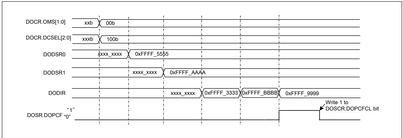
Figure 58.6 Example of Operation in Data Comparison Mode (Detection condition: Inside window)
