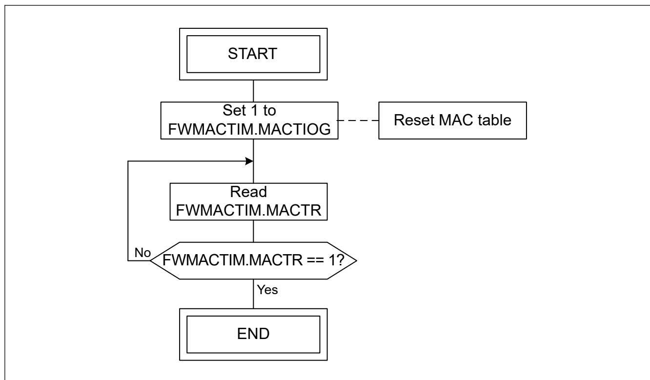
Figure 31.15 Reset flow of MAC table
