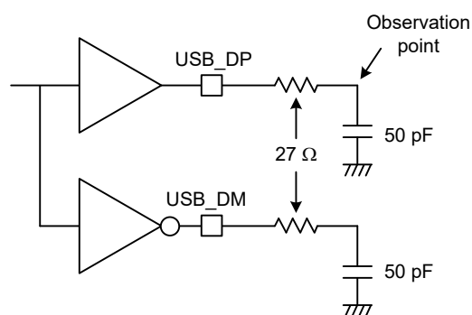
Figure 70.129 Test circuit in full-speed mode
