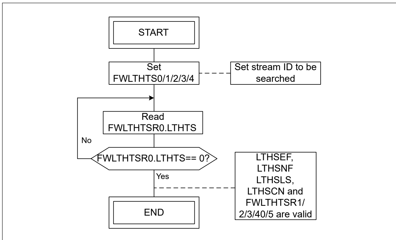
Figure 31.13 Layer 3 entry search flow
