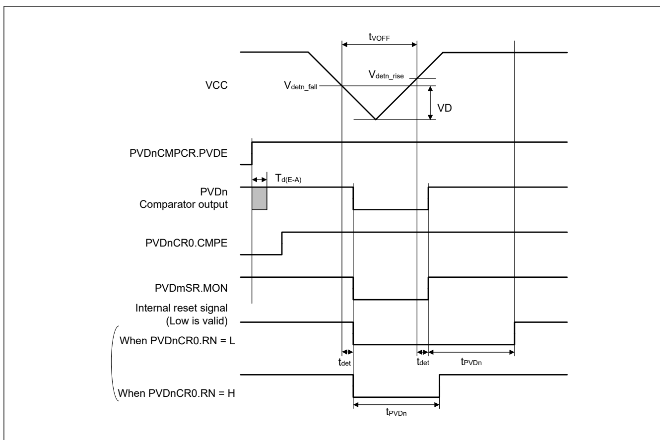
Figure 70.143 Voltage detection circuit timing ( V_{detn} ) ( n = 1, 2, 4, 5 )
