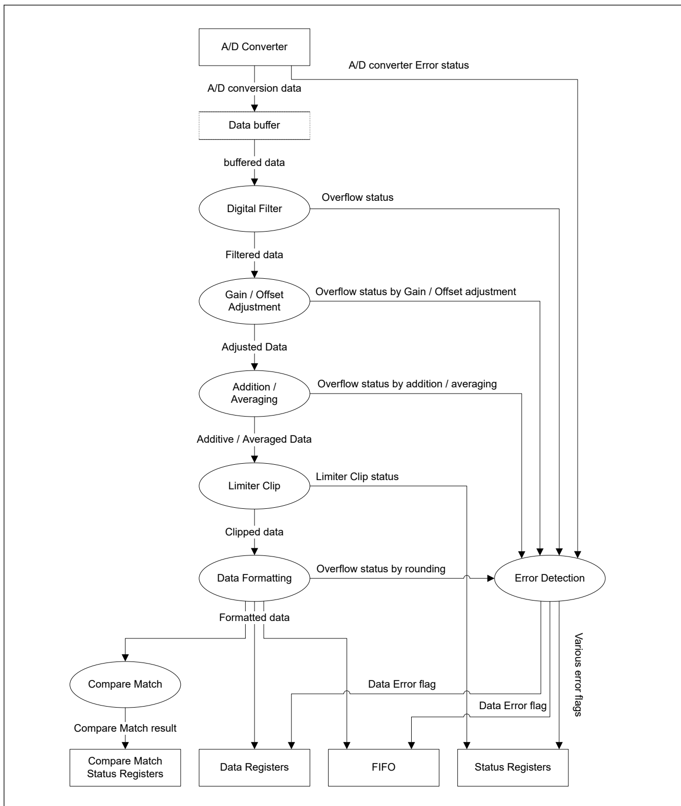
Figure 54.34 Internal data flow diagram of A/D conversion data
