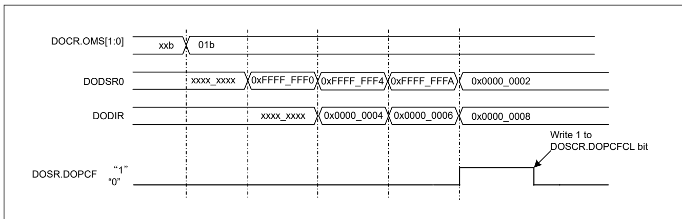
Figure 58.8 Example of Operation in Data Addition Mode
