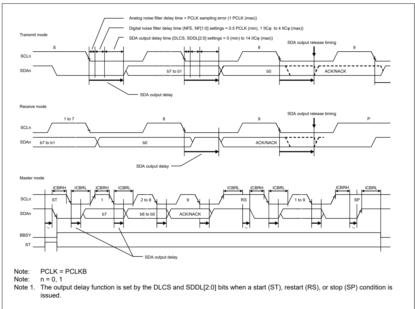
Figure 40.22 SDA output delay function
