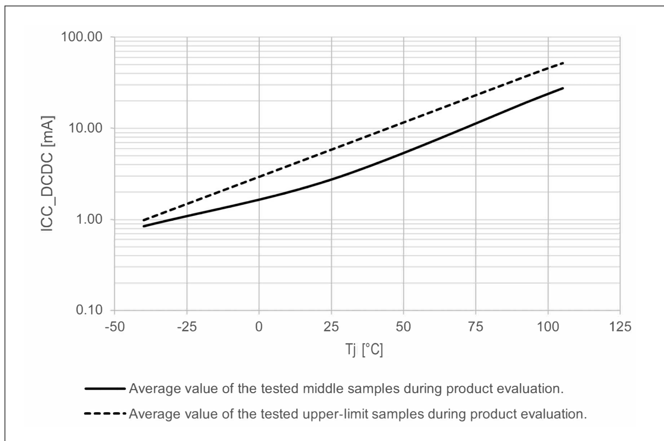
Figure 70.3 Temperature dependency in Software Standby mode ( ICC\_DCDC , SS2LP\_0 , SVSCR\_1 ) (reference data)
