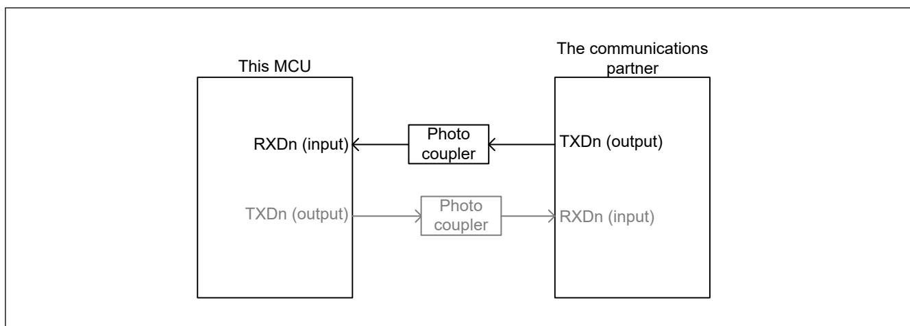
Figure 39.26 block diagram image of the reception through a photo coupler
