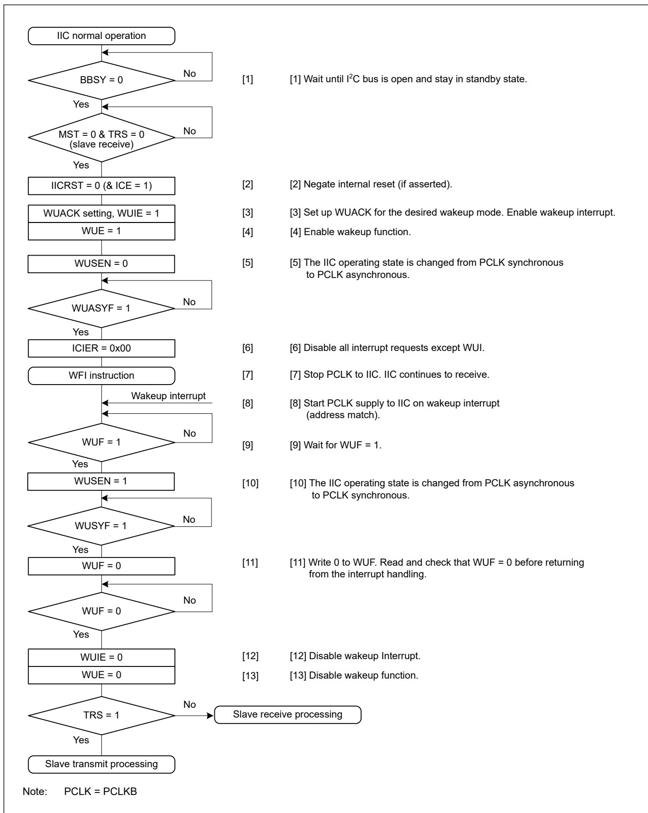
Figure 40.30 Example operation of normal wakeup mode 1 when wakeup is triggered by a wakeup interrupt on match of the slave address
