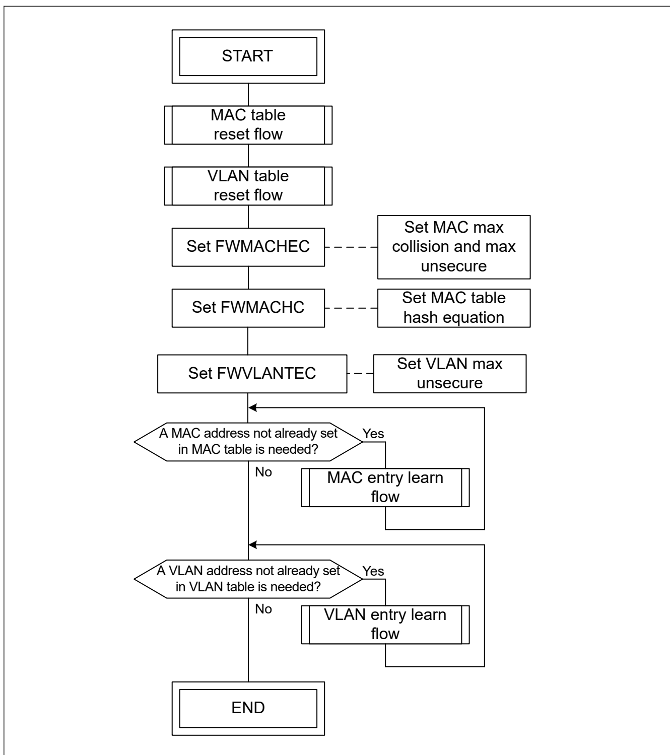
Figure 31.42 Setting flow of Layer 2 forwarding
