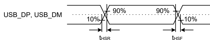
Figure 70.136 USB_DP and USB_DM output timing (high-speed)
