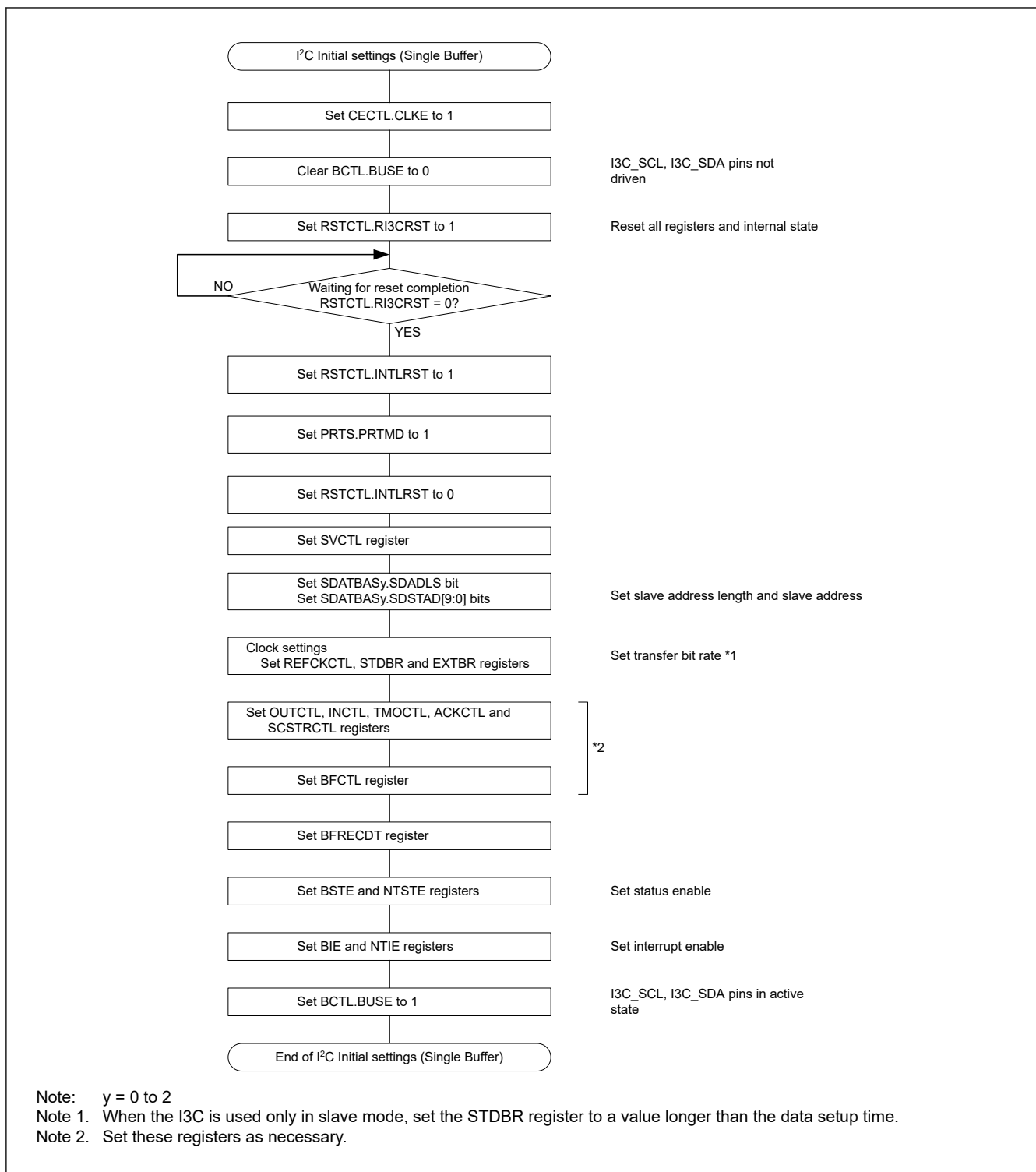
Figure 41.140 Example of I 2 C initialization flowchart (single buffer transfer)
