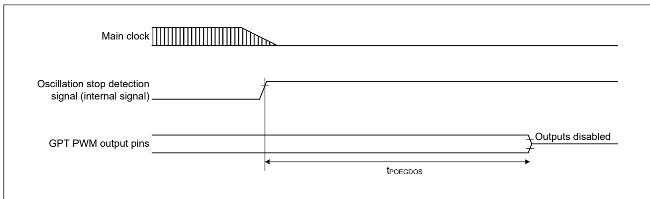
Figure 70.59 Output Disable Time of POEG in Response to the Oscillation Stop Detection
