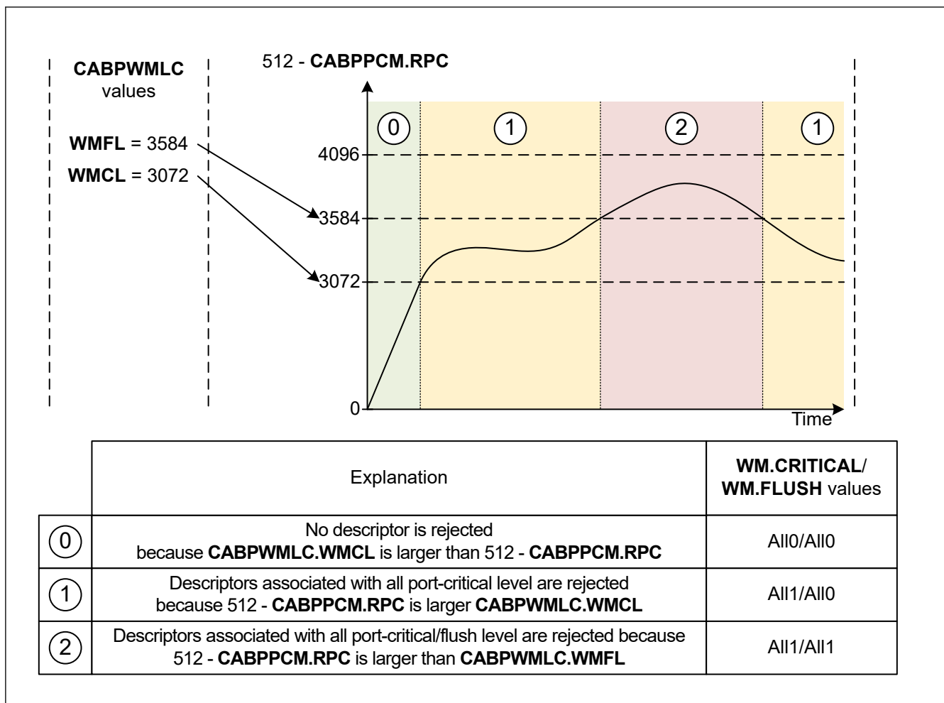
Figure 32.12 Example for global level-based watermark setting
