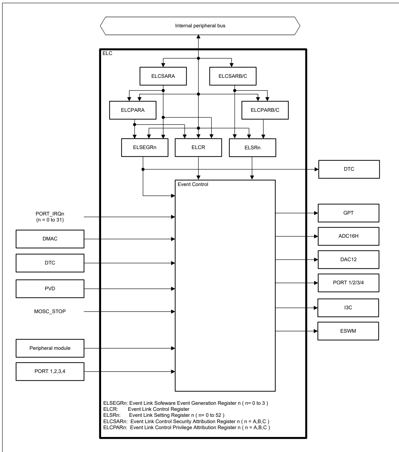
Figure 20.1 ELC block diagram
