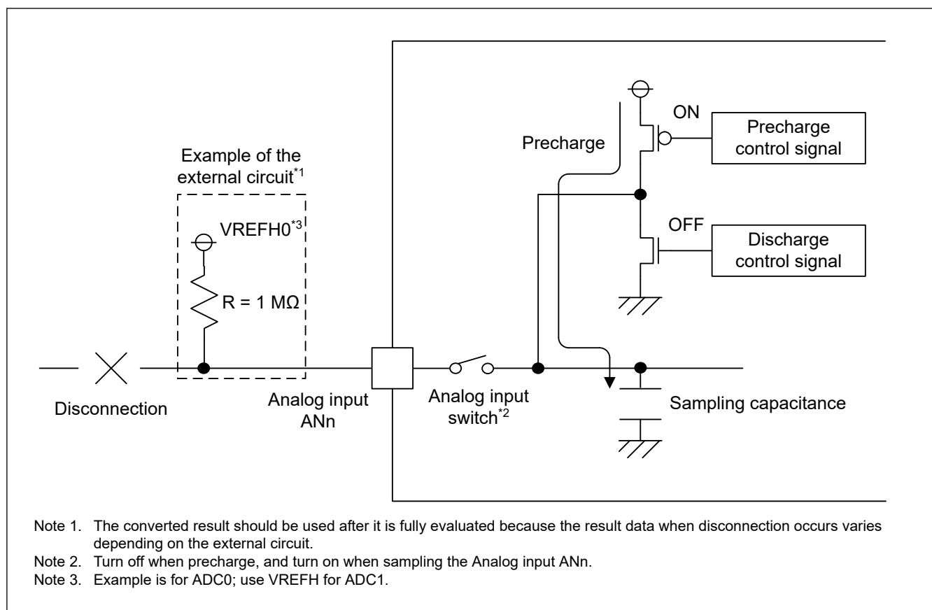
Figure 54.26 Example of disconnection detection when precharge is selected
