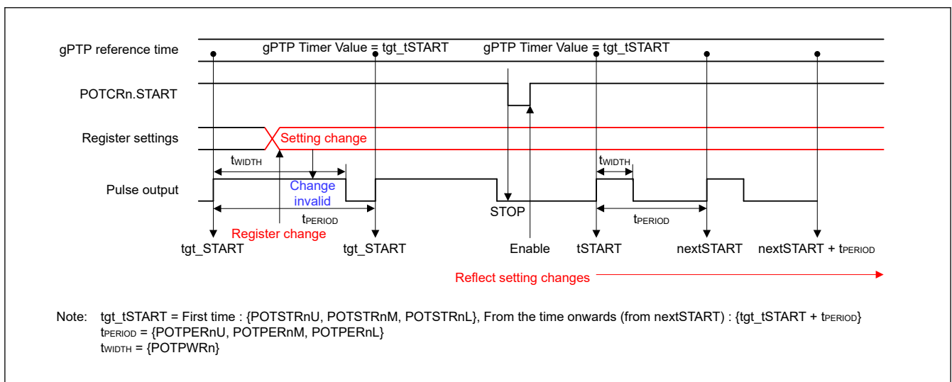
Figure 36.20 When the register setting is changed with the POTCRn.START bit set to 1
