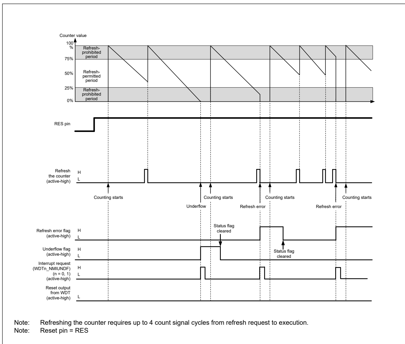
Figure 28.4 Operation example in auto start mode
