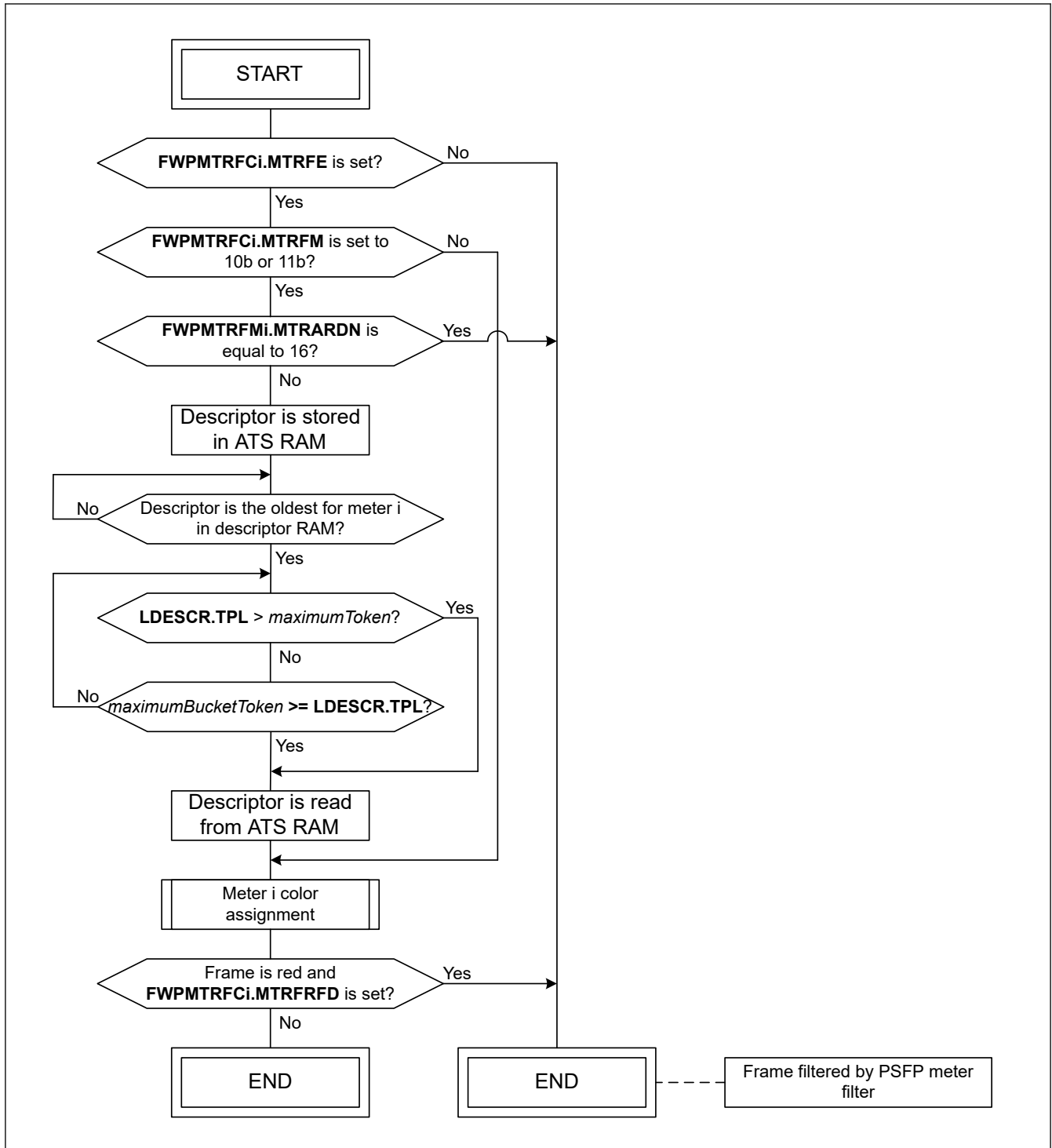
Figure 31.104 Meter filtering flow for meter i
