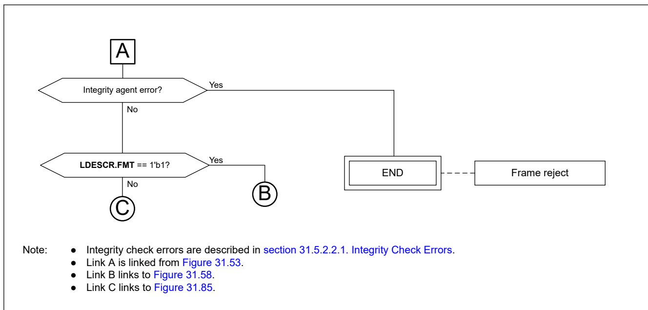
Figure 31.56 Integrity check flow
