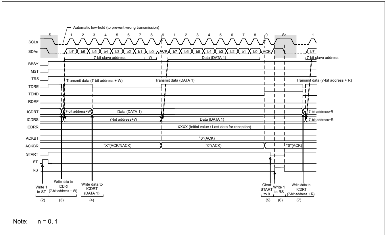
Figure 40.46 Restart condition issue timing after master transmission.
