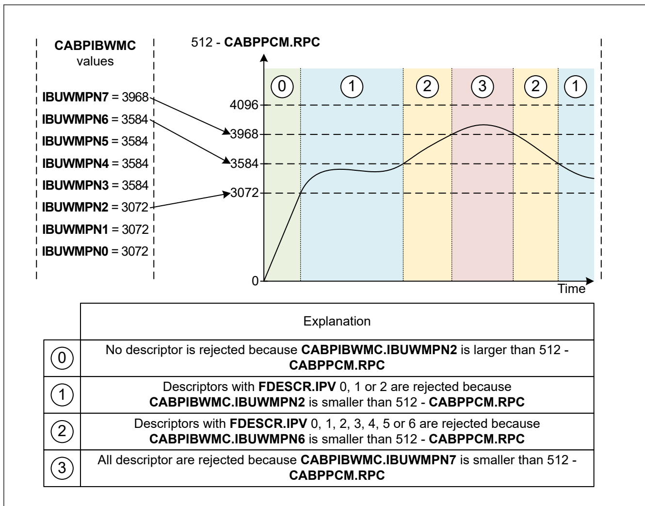
Figure 32.11 Example for IPV-based watermark setting
