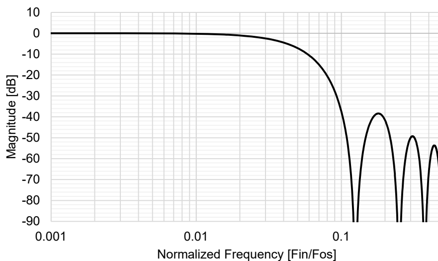
Figure 70.138 Digital filter characteristics (Sinc filter)
