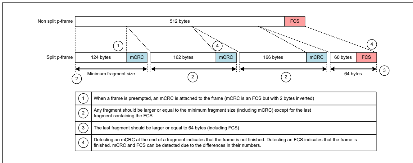
Figure 33.33 P-frame preemption (EATPEC.AFS == 01)
