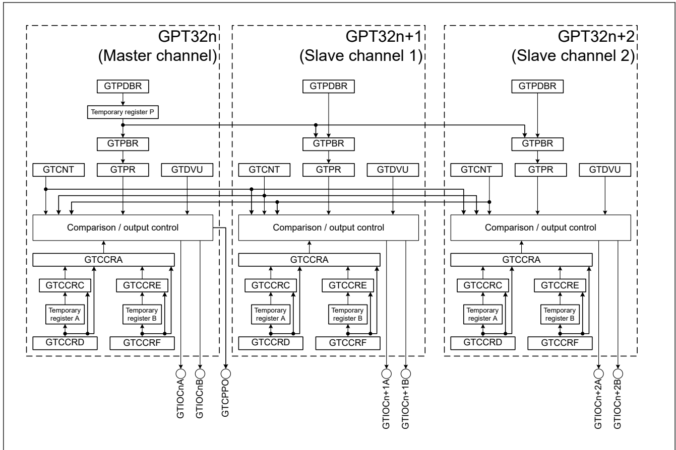
Figure 23.67 Block Diagram in Complementary PWM Mode 4 (n = 4, 7)
