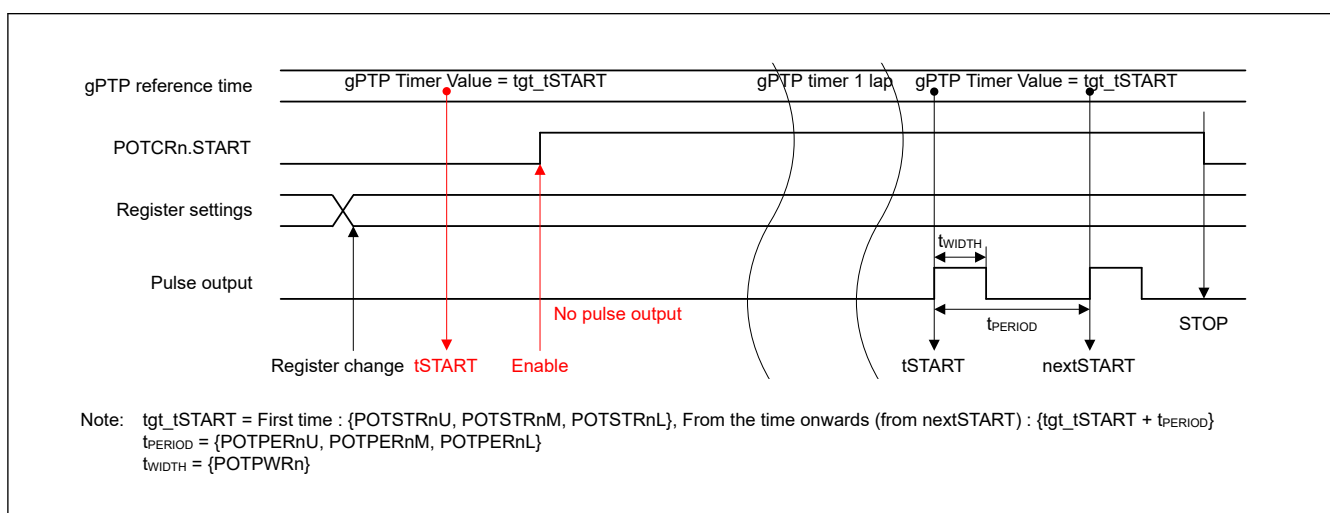
Figure 36.16 When changing the POTCRn.START bit from 0 to 1 after setting the register and after the start time
