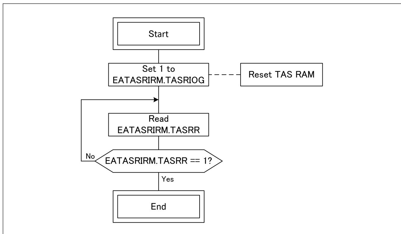
Figure 33.8 TAS RAM reset flow
