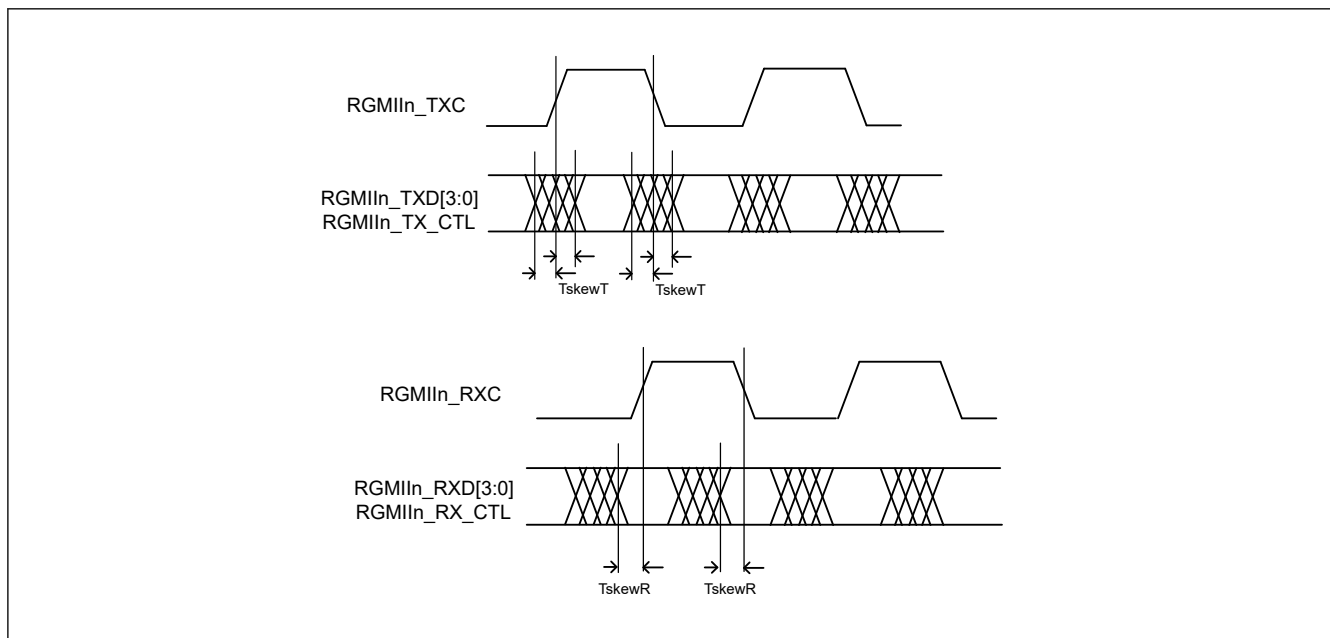
Figure 70.120 RGMII timing
