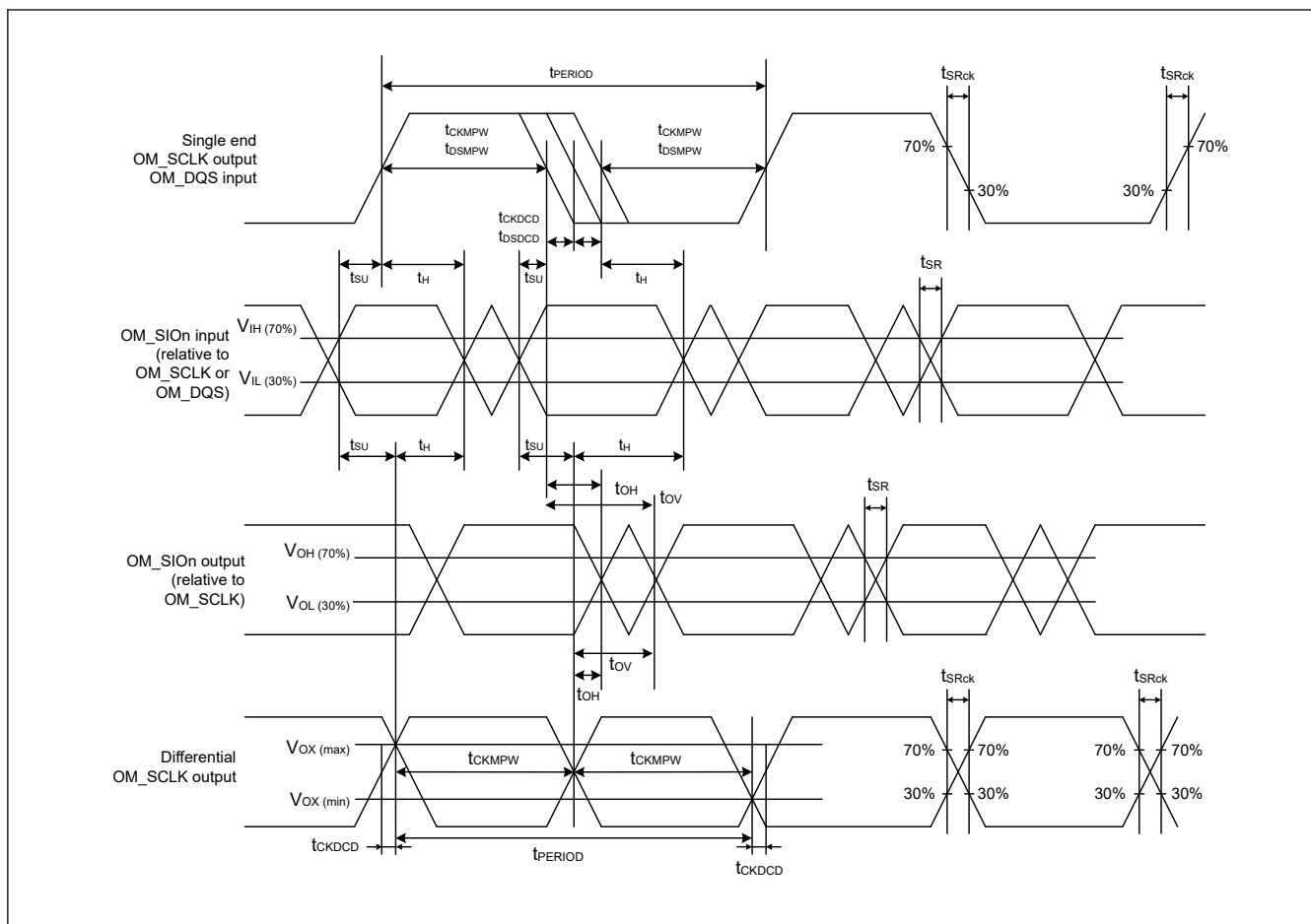
Figure 70.83 OSPI clock / DS timing
