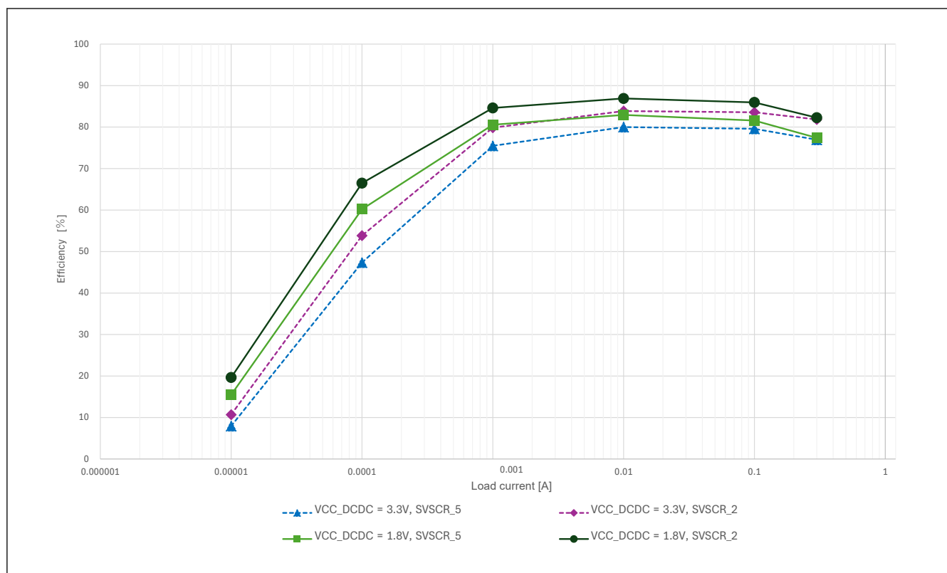
Figure 70.21 Typical DCDC efficiency (%) vs load current (A) in Software Standby mode (SSCR1.SS2LP = SS2LP_1), Tj = 25 °C
