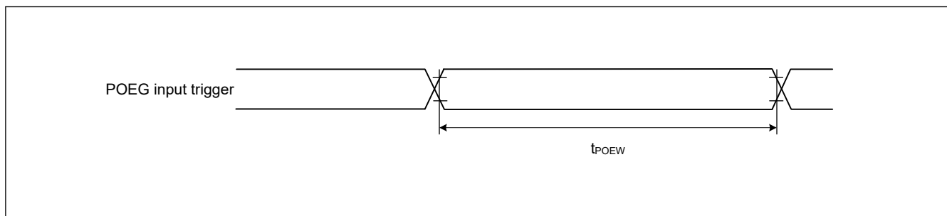
Figure 70.54 POEG input trigger timing
