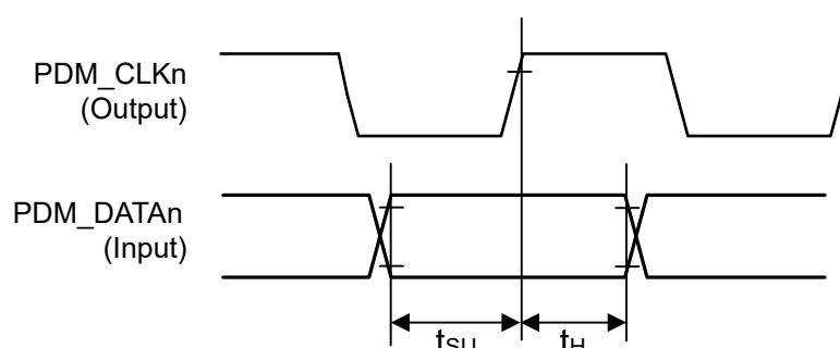
Figure 70.124 Receive Timing (Synchronized with the rise of PDM_CLKn)
