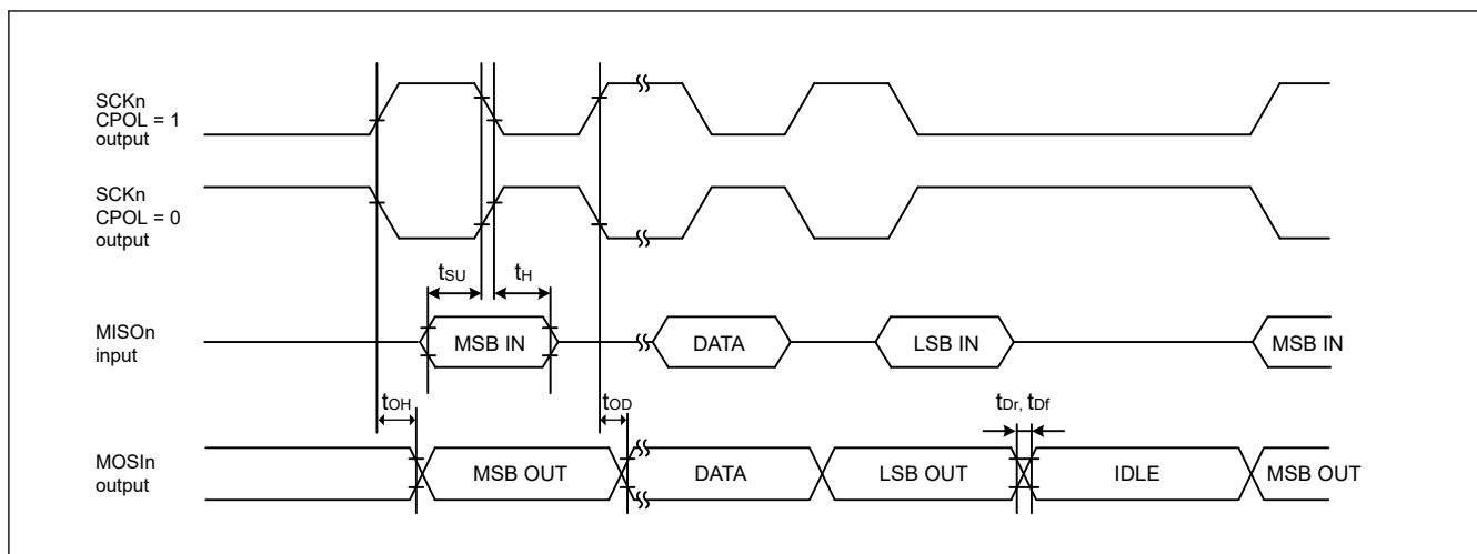
Figure 70.71 SCI simple SPI mode timing for master when CPHA = 1
