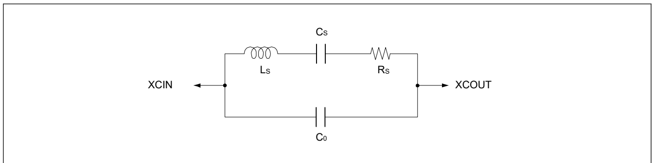
Figure 9.6 Equivalent circuit for the 32.768-kHz crystal resonator
