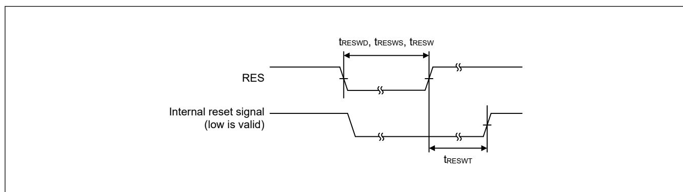
Figure 70.33 Reset input timing
