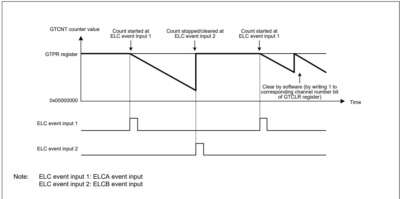
Figure 23.89 Examples of count clearing operation by hardware source in saw wave down-counting, started at ELCA input, and stopped/cleared at ELCB input
