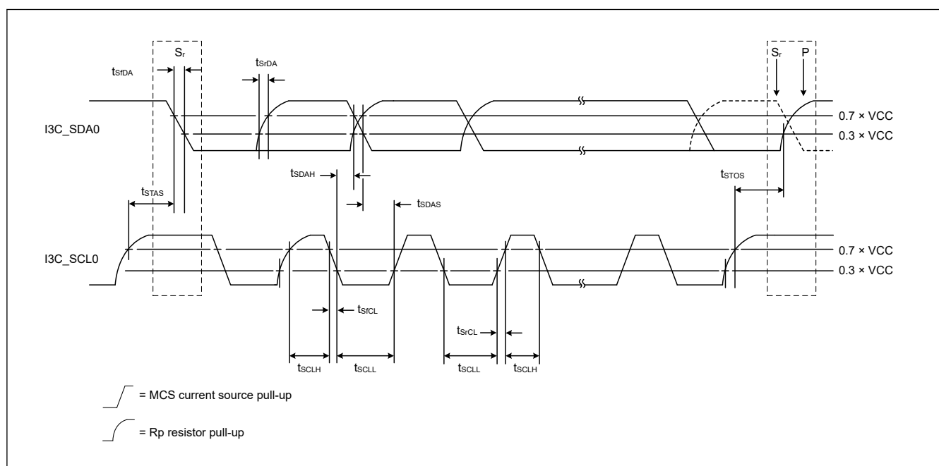
Figure 70.90 I 2 C bus interface input/output timing (Hs-mode)
