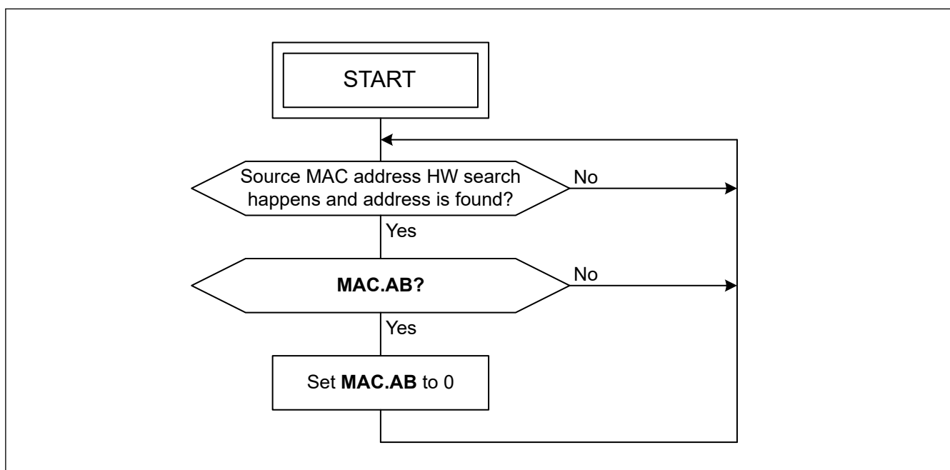
Figure 31.94 MAC source address search algorithm
