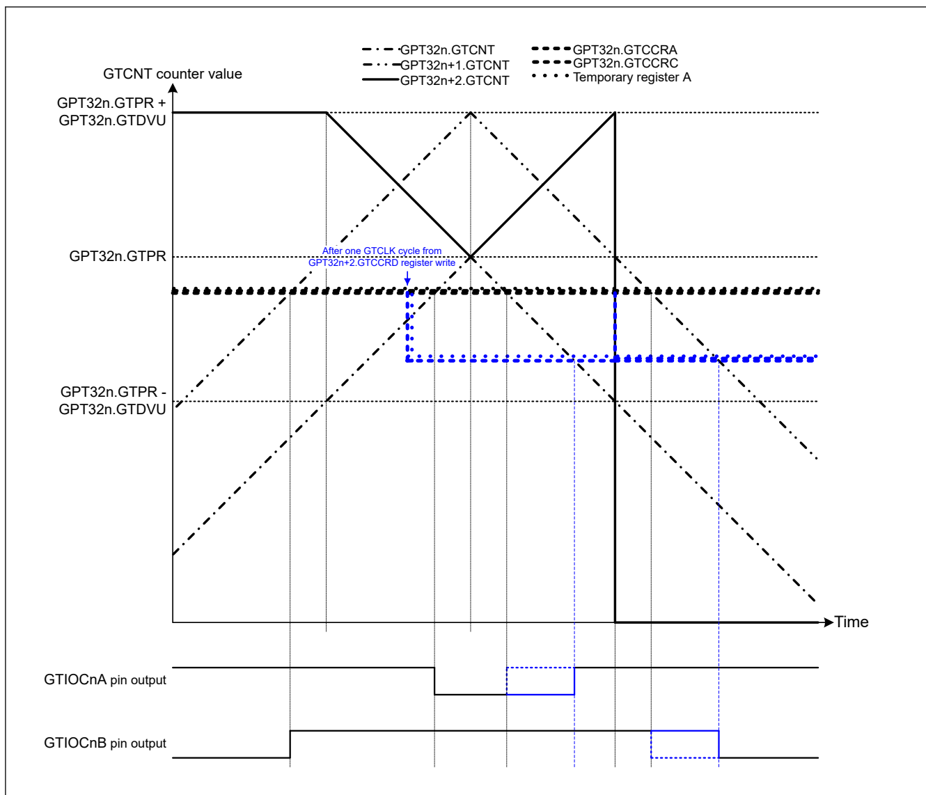
Figure 23.69 Example of Complementary PWM Mode 4 Single Buffer Operation (Up-Counting Crest Section) (Complementary PWM mode 4 single buffer operation, GTIOCnA pin = Low / GTIOCnB pin = High at GTCCR register compare match during up-counting, GTIOCnA pin = High / GTIOCnB pin = Low at GTCCR register compare match during down-counting, when a value is written to GTCCR register during the up-counting dead time) (n = 4, 7)
