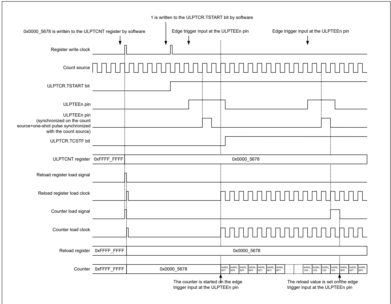
Figure 26.15 Counter and reload rewrite timing (under condition D)
