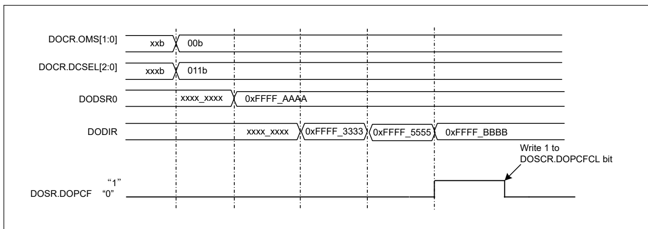
Figure 58.5 Example of Operation in Data Comparison Mode (Detection condition: Upper)
