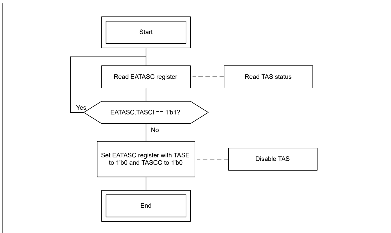
Figure 33.12 TAS disabling flow
