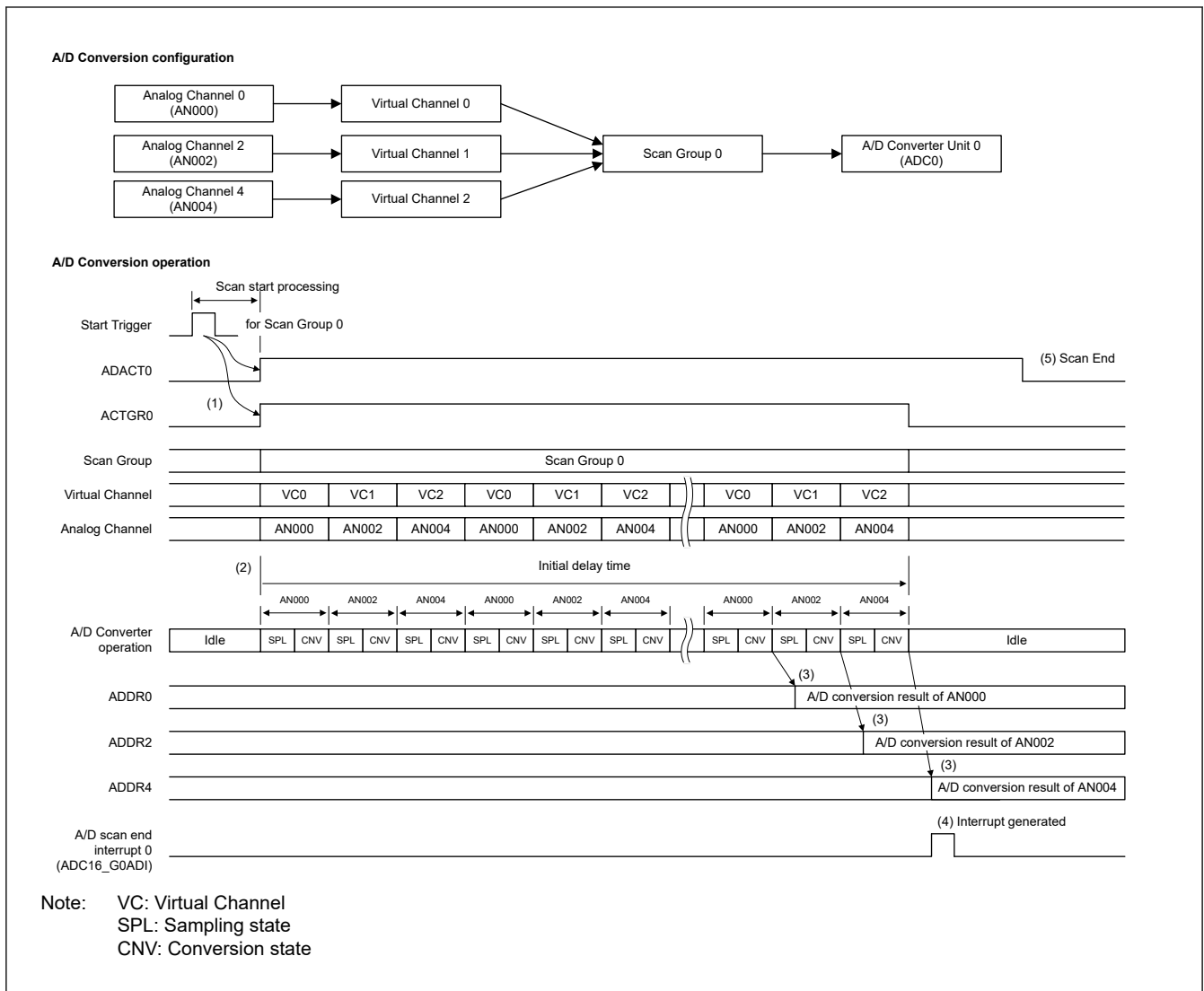
Figure 54.12 Example of scanning operation in Hybrid mode – Single scan mode
