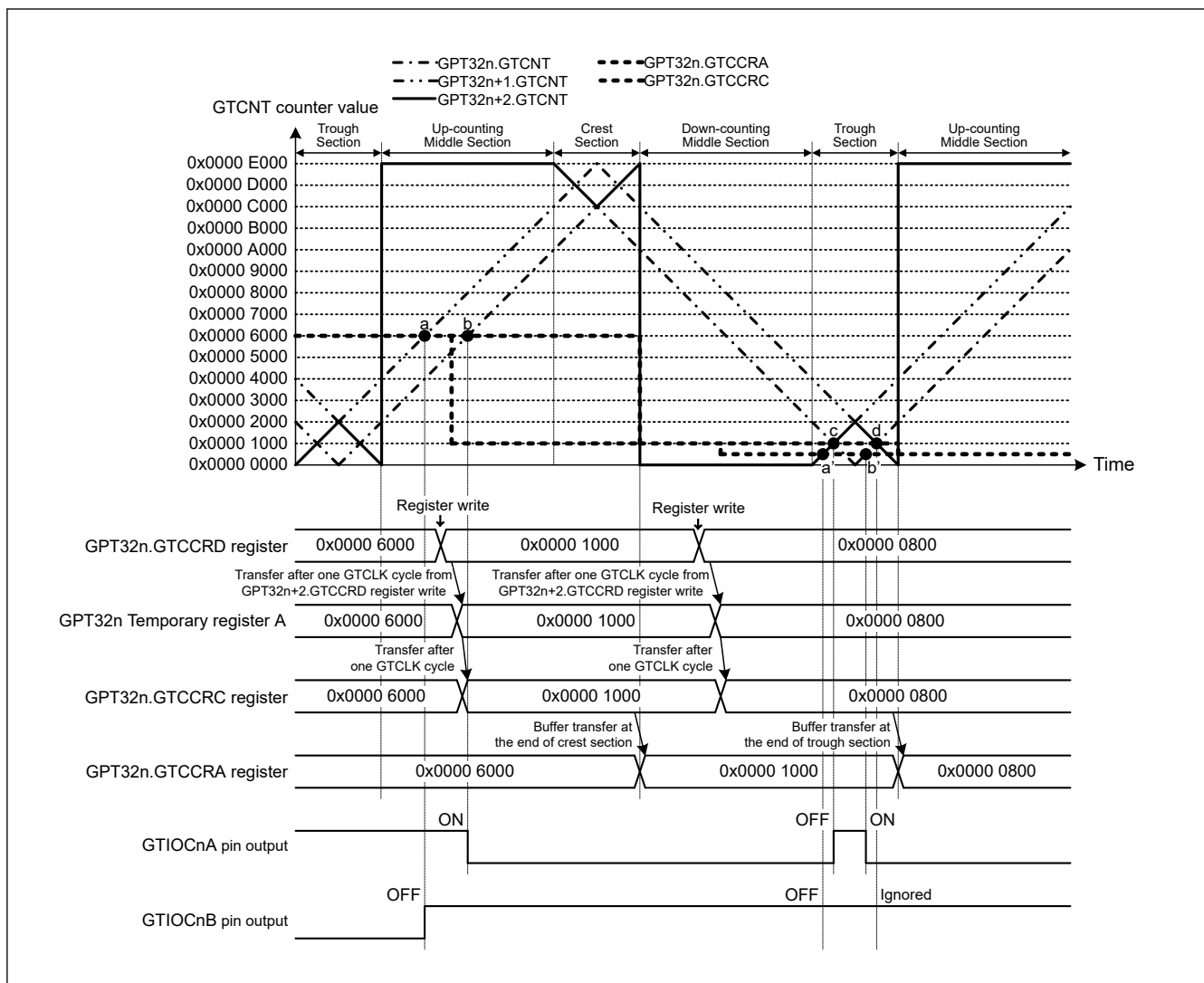
Figure 23.63 Example of Compare Match Generation Sequence Operation in Complementary PWM Mode (Complementary PWM mode 3 single buffer operation, GTIOCnA pin = Low / GTIOCnB pin = High at GTCCRA register compare match during up-counting, GTIOCnA pin = High / GTIOCnB pin = Low at GTCCRA register compare match during down-counting, the dead time value is 0x0000 2000, compare match generation order: a' → c → b' → d) (n = 4, 7)
