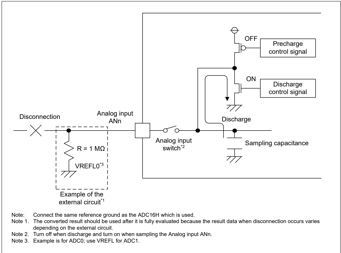
Figure 54.27 Example of disconnection detection when discharge is selected
