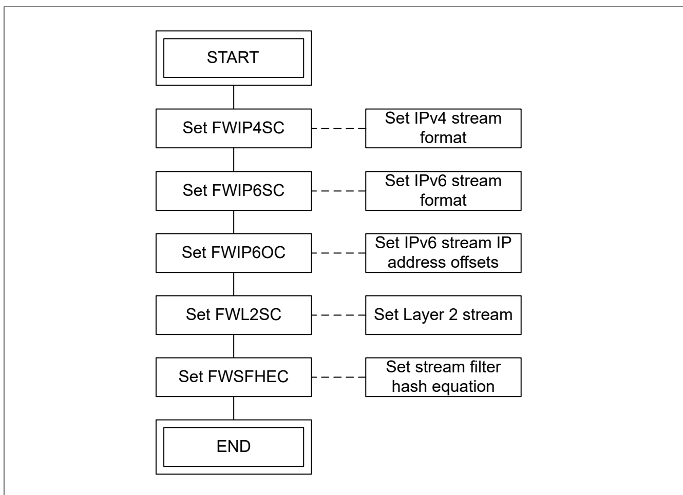
Figure 31.40 Setting flow of IPv4/IPv6/Layer 2 stream filter
