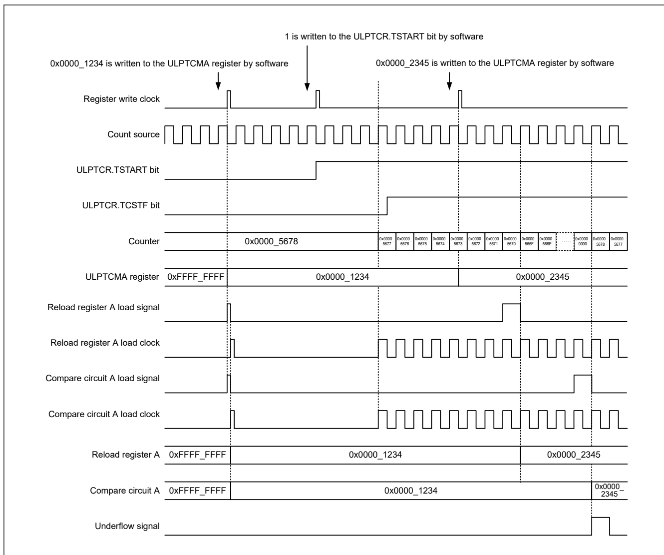
Figure 26.16 Rewrite timing for the compare circuit and reload register for compare match A
