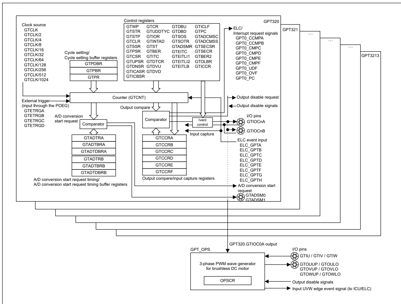
Figure 23.1 GPT block diagram (Saw-wave PWM mode 1, Saw-wave one-shot pulse mode, Triangle-wave PWM mode1,2,3)
