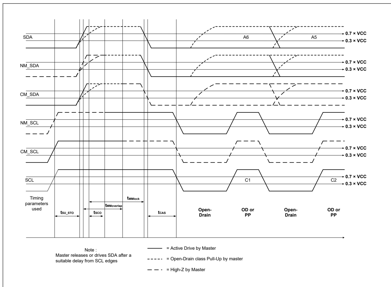
Figure 70.100 Master to Master Bus Handoff
