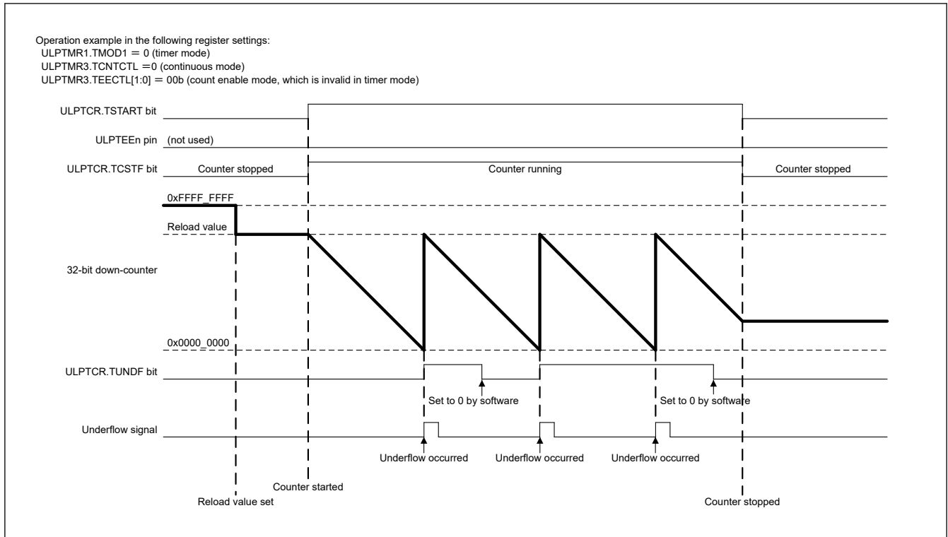
Figure 26.2 Operation example in timer and continuous modes
