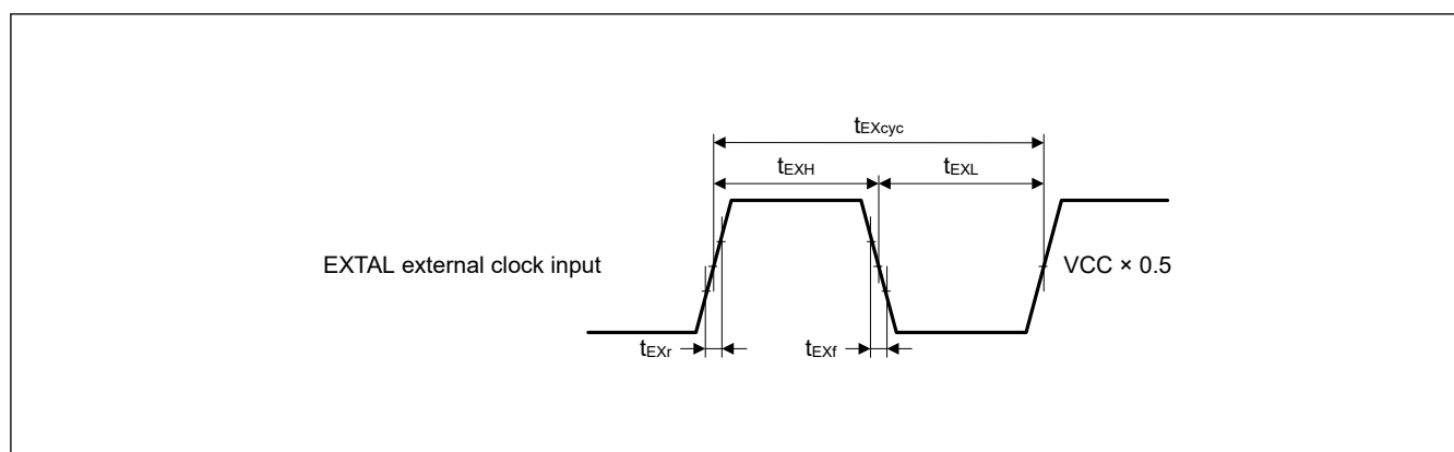
Figure 70.26 EXTAL external clock input timing
