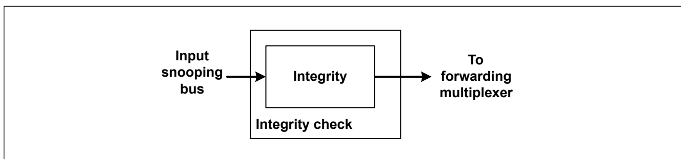
Figure 31.55 Integrity check block diagram
