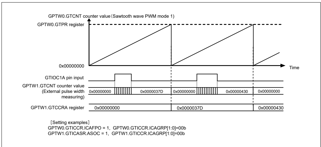
Figure 23.99 Example of input capture operation by inter channel cooperation (channel 1 is captured by the overflow of channel 0)
