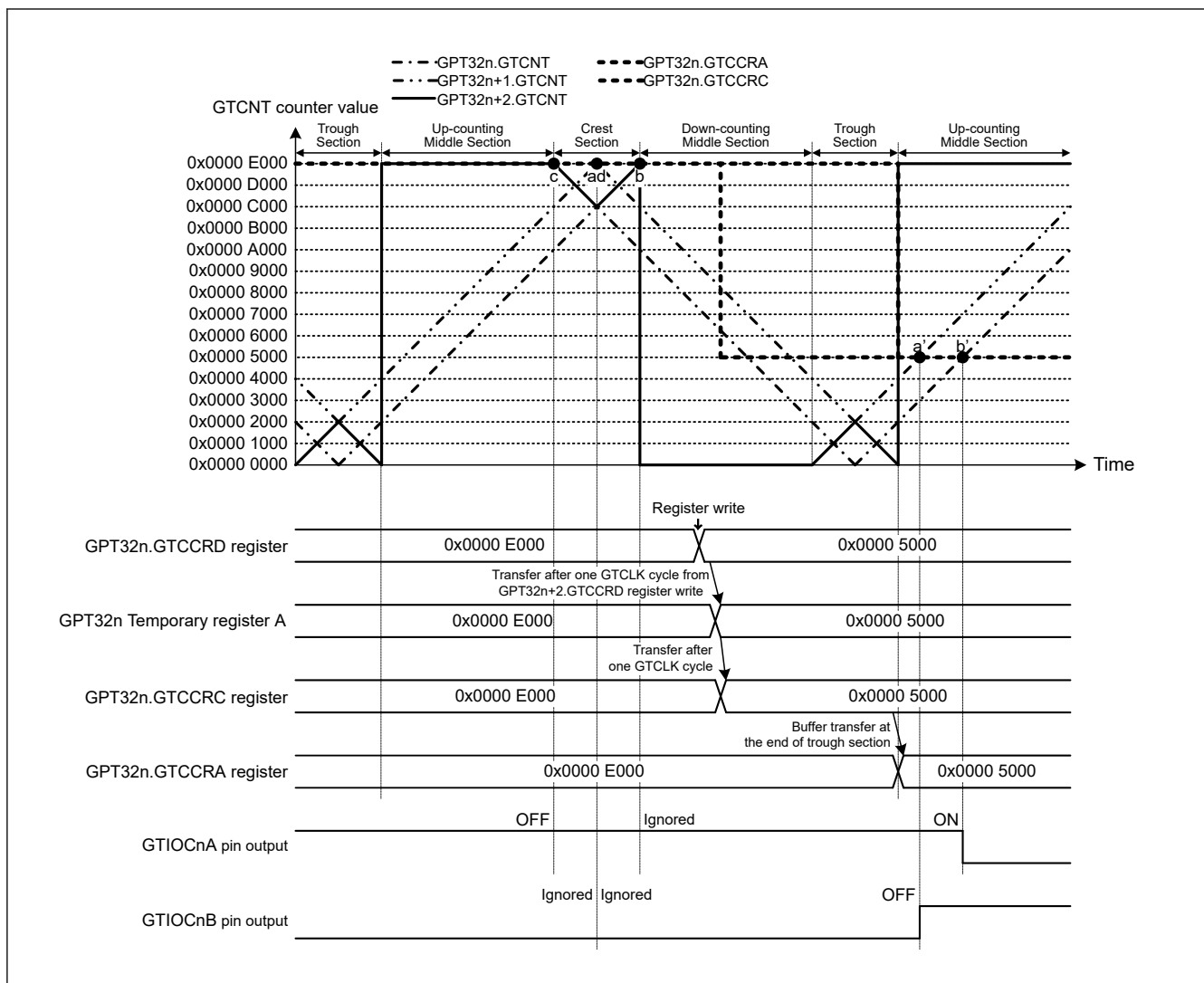
Figure 23.58 Example of Compare Match Generation Sequence Operation in Complementary PWM Mode (Complementary PWM mode 3 single buffer operation, GTIOCnA pin = Low / GTIOCnB pin = High at GTCCRA register compare match during up-counting, GTIOCnA pin = High / GTIOCnB pin = Low at GTCCRA register compare match during down-counting, the dead time value is 0x0000 2000, compare match generation order: c → (a, d) → b) (n = 4, 7)
