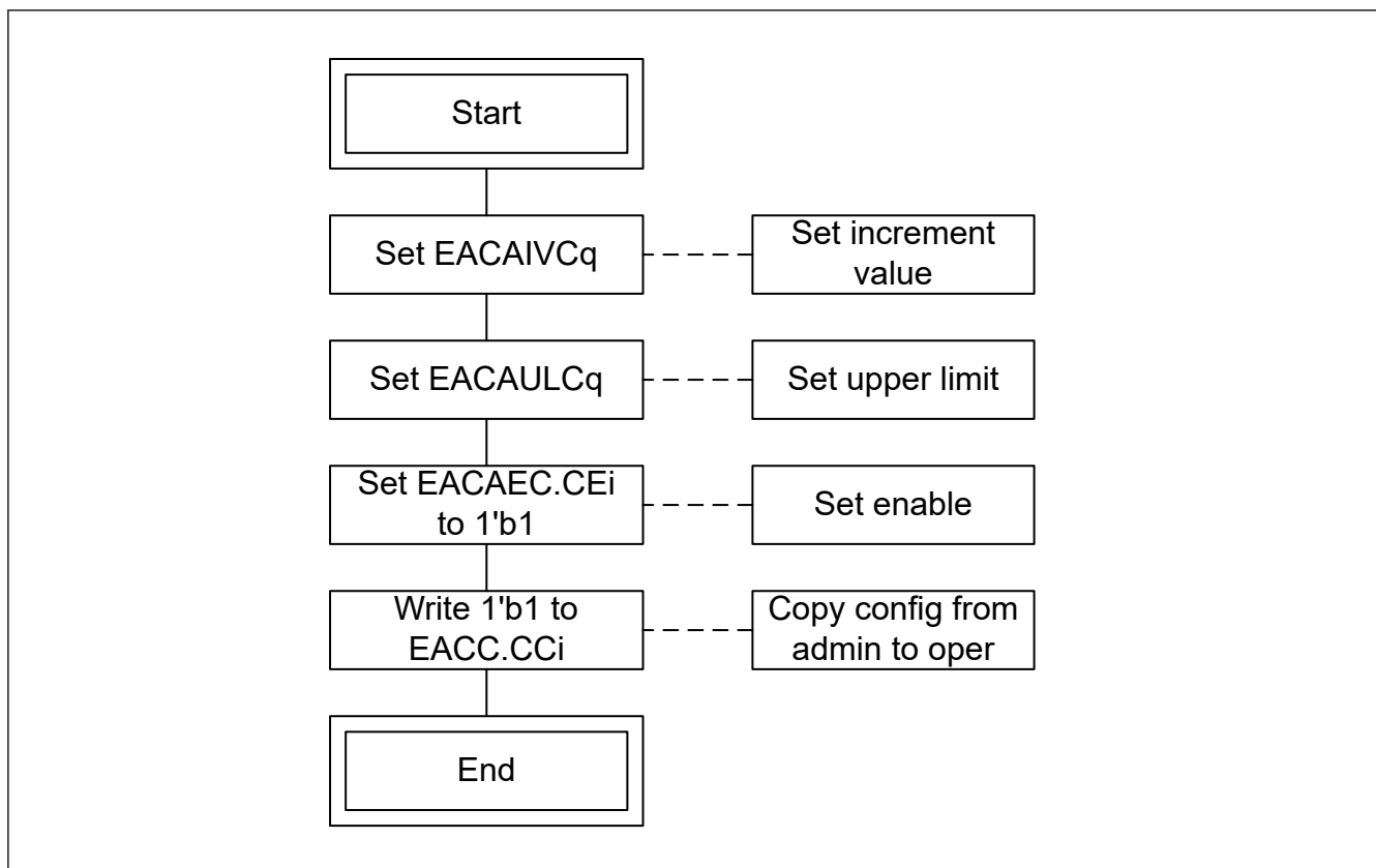
Figure 33.9 CBS q setting flow
