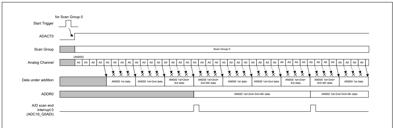
Figure 54.55 Example of data output decimation function (output every 4 times) when addition function is enabled (addition count is 4 times)
