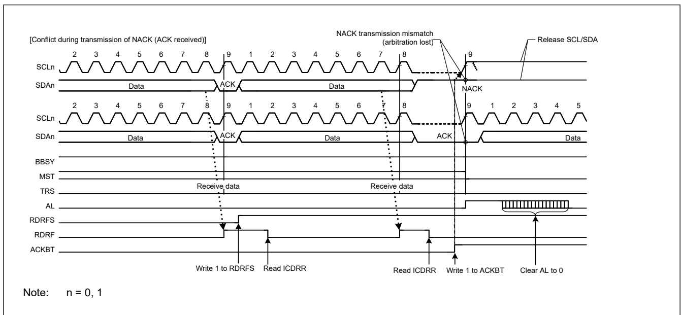
Figure 40.43 Example of arbitration-lost detection during transmission of NACK when NALE = 1
