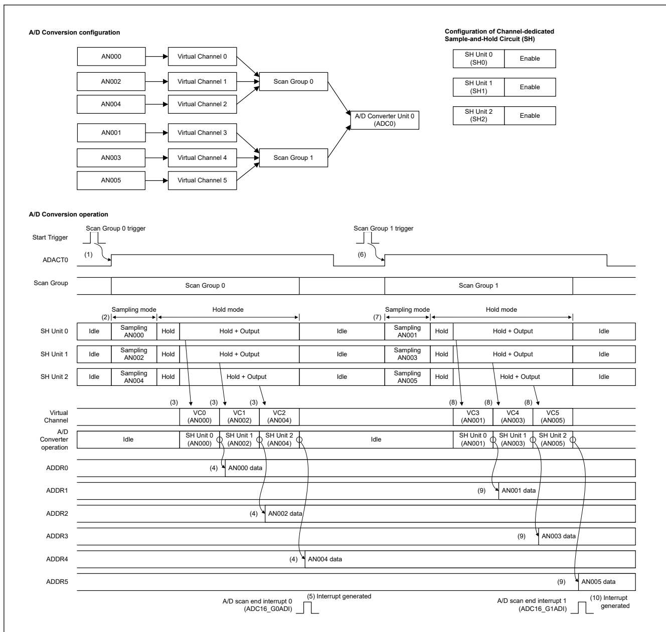
Figure 54.19 Example operation when channel-dedicated sample-and-hold circuit is shared with two analog channels in SAR mode
