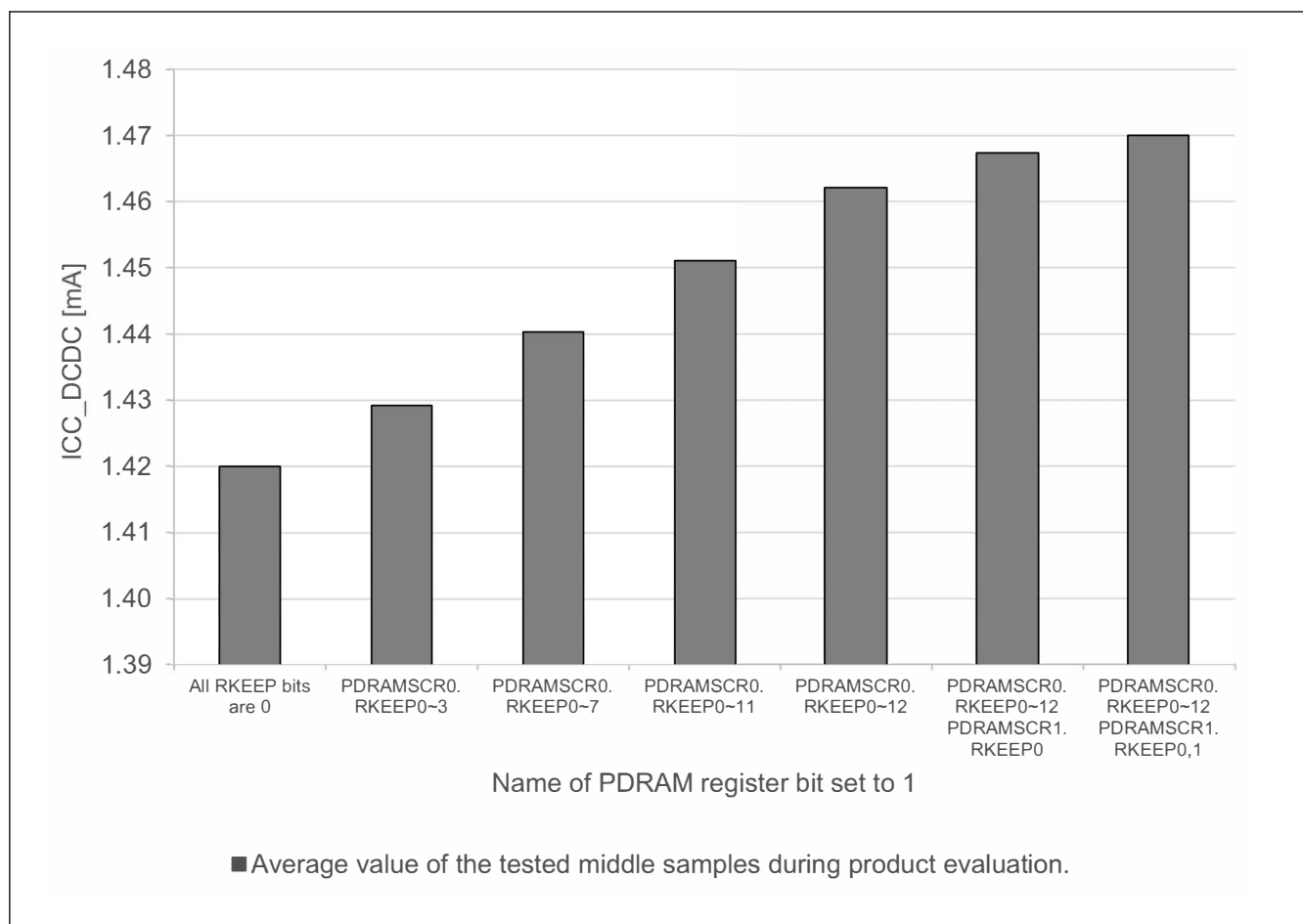
Figure 70.13 Software Standby current per SRAM state (ICC_DCDC, SS2LP_0, SVSCR_4) (reference data)
