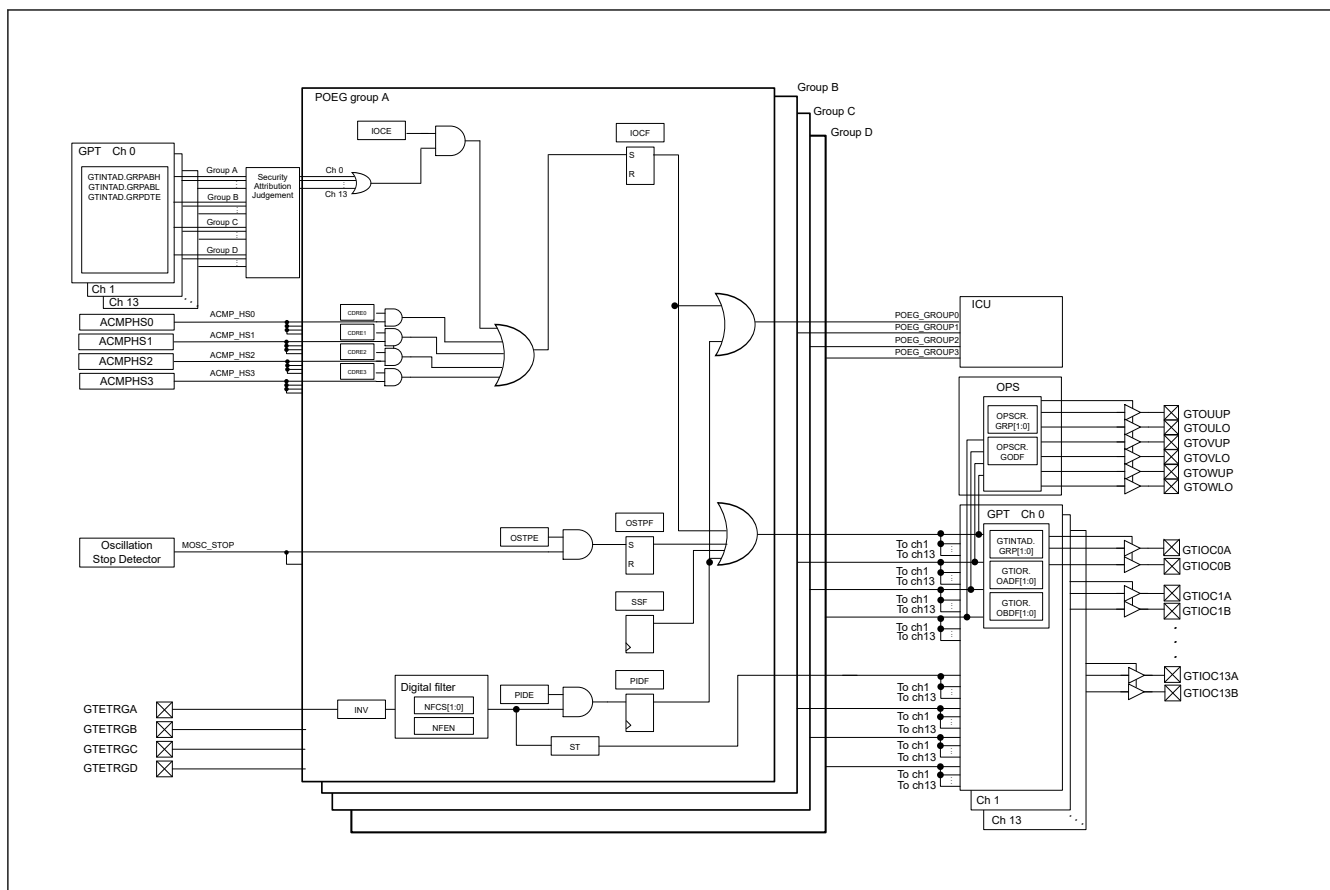
Figure 22.1 POEG block diagram
