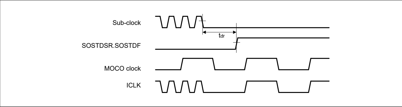
Figure 70.140 Sub-clock oscillation stop detection timing
