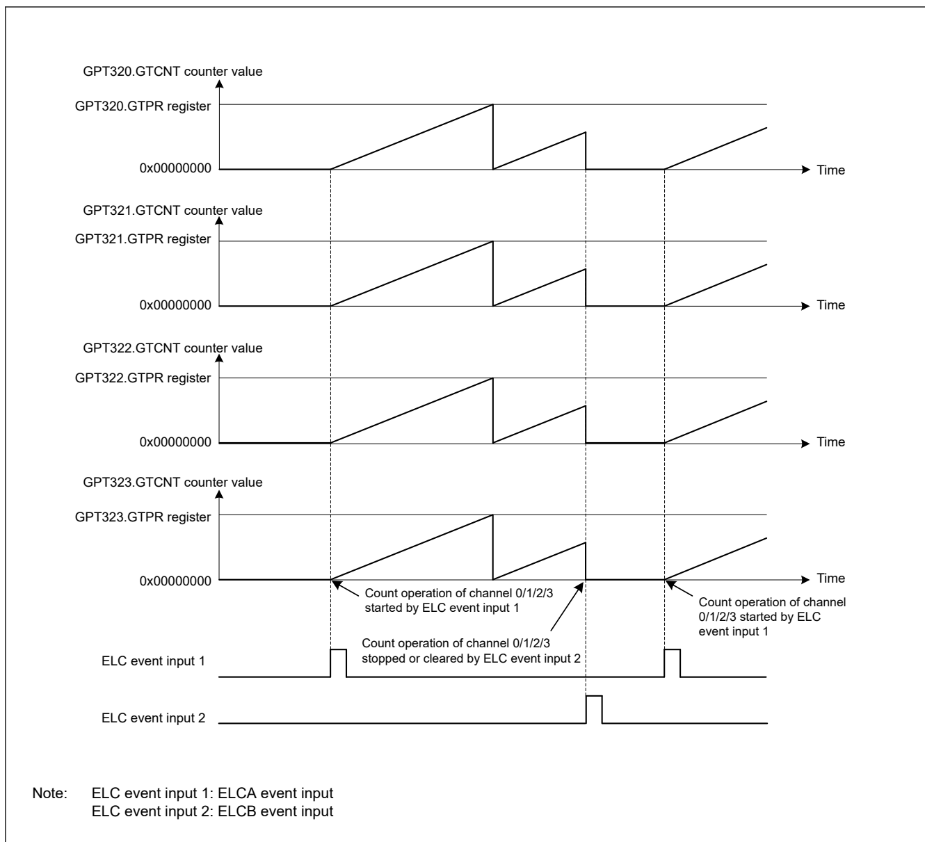
Figure 23.98 Example of a simultaneous start, stop, and clear by a hardware source with the same count cycle (GTPR register value)
