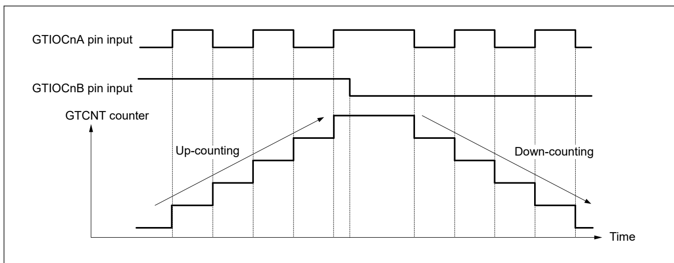
Figure 23.112 Example of phase counting mode 2 (C)
