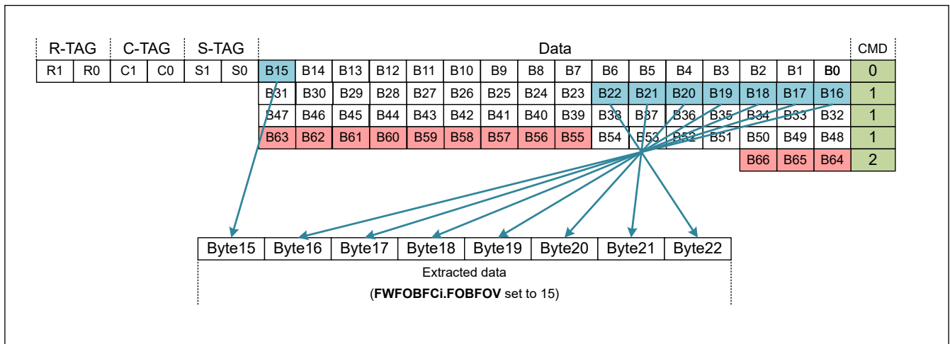
Figure 31.67 4-byte filter data extraction for filtering
