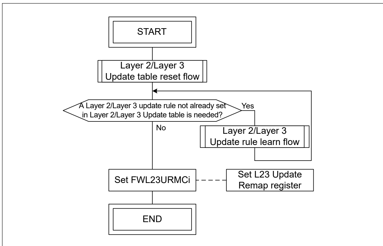
Figure 31.44 Setting flow of Layer 2/Layer 3 update
