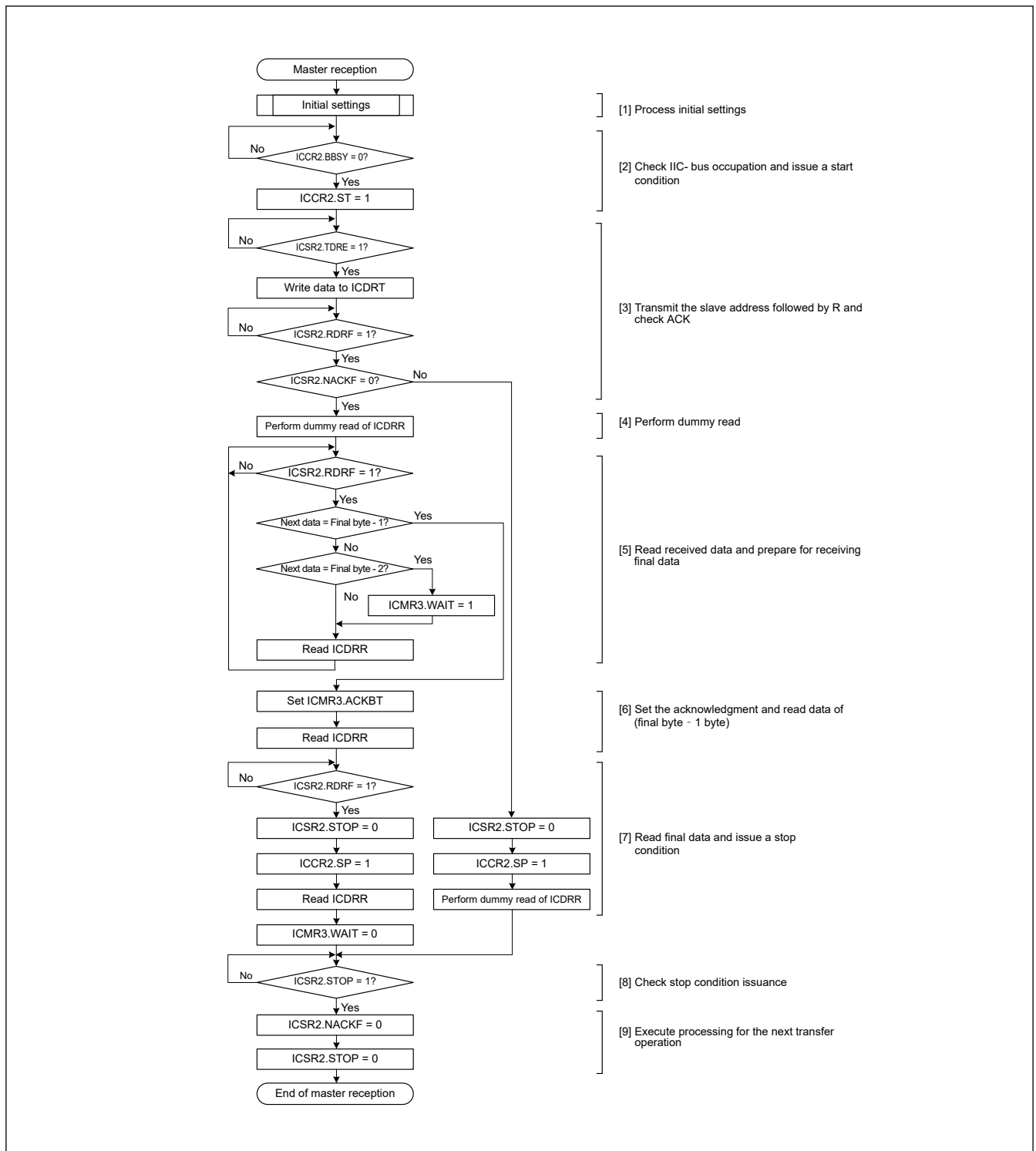
Figure 40.11 Example master reception flow with 7-bit address format of 3 or more bytes
