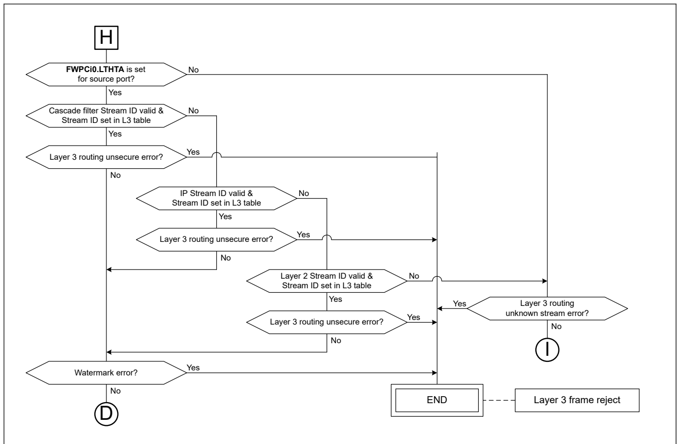
Figure 31.86 Layer 3 forwarding/routing unsecure flow
