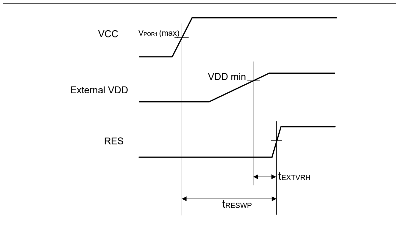
Figure 70.144 Power-up sequence of external VDD mode with using RES pin
