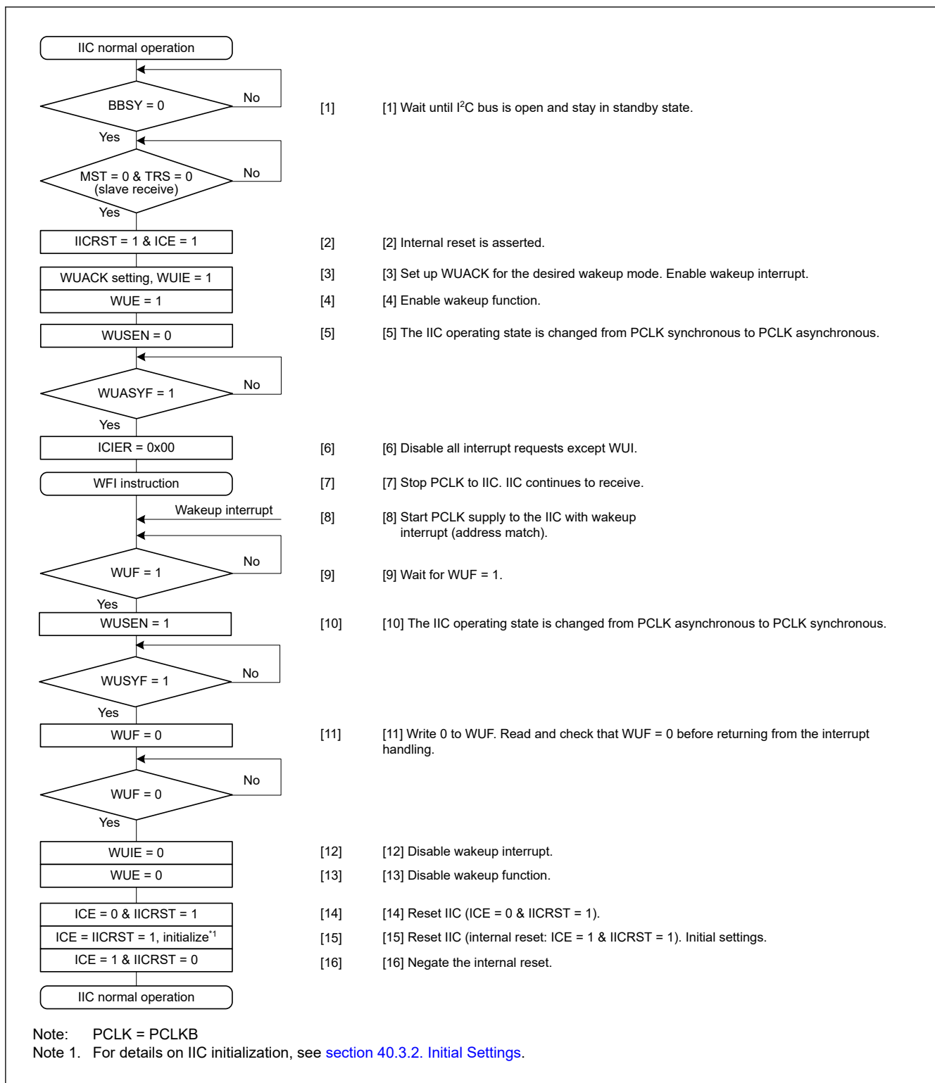
Figure 40.35 Example operation of command recovery mode and EEP response mode when wakeup is triggered by a wakeup interrupt on match of the slave address
