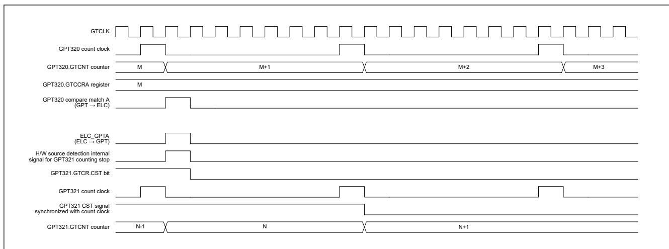
Figure 23.87 Example of Timing of Operations to Stop Counting in Response to Event Input from ELC_GPTA
