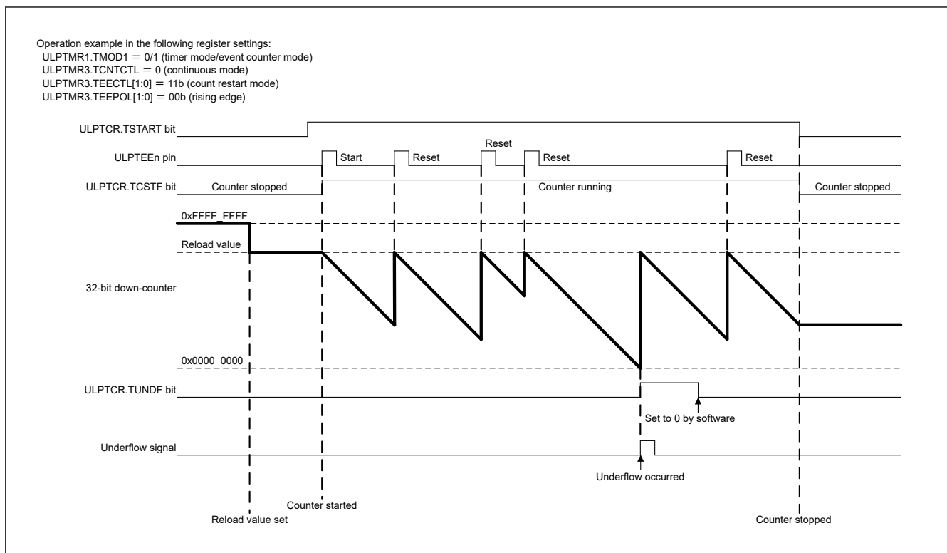
Figure 26.10 Operation example in common, continuous, and count restart modes
