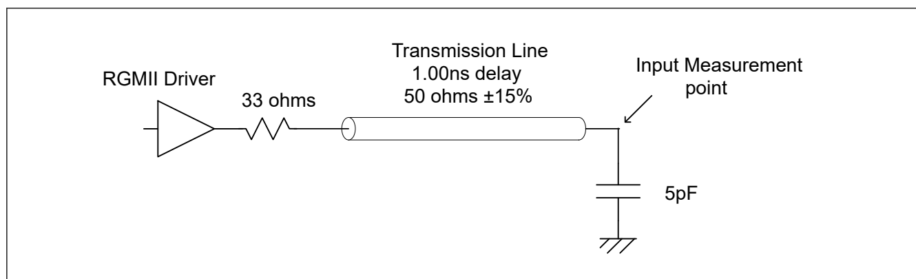
Figure 70.122 RGMII output timing measurement conditions
