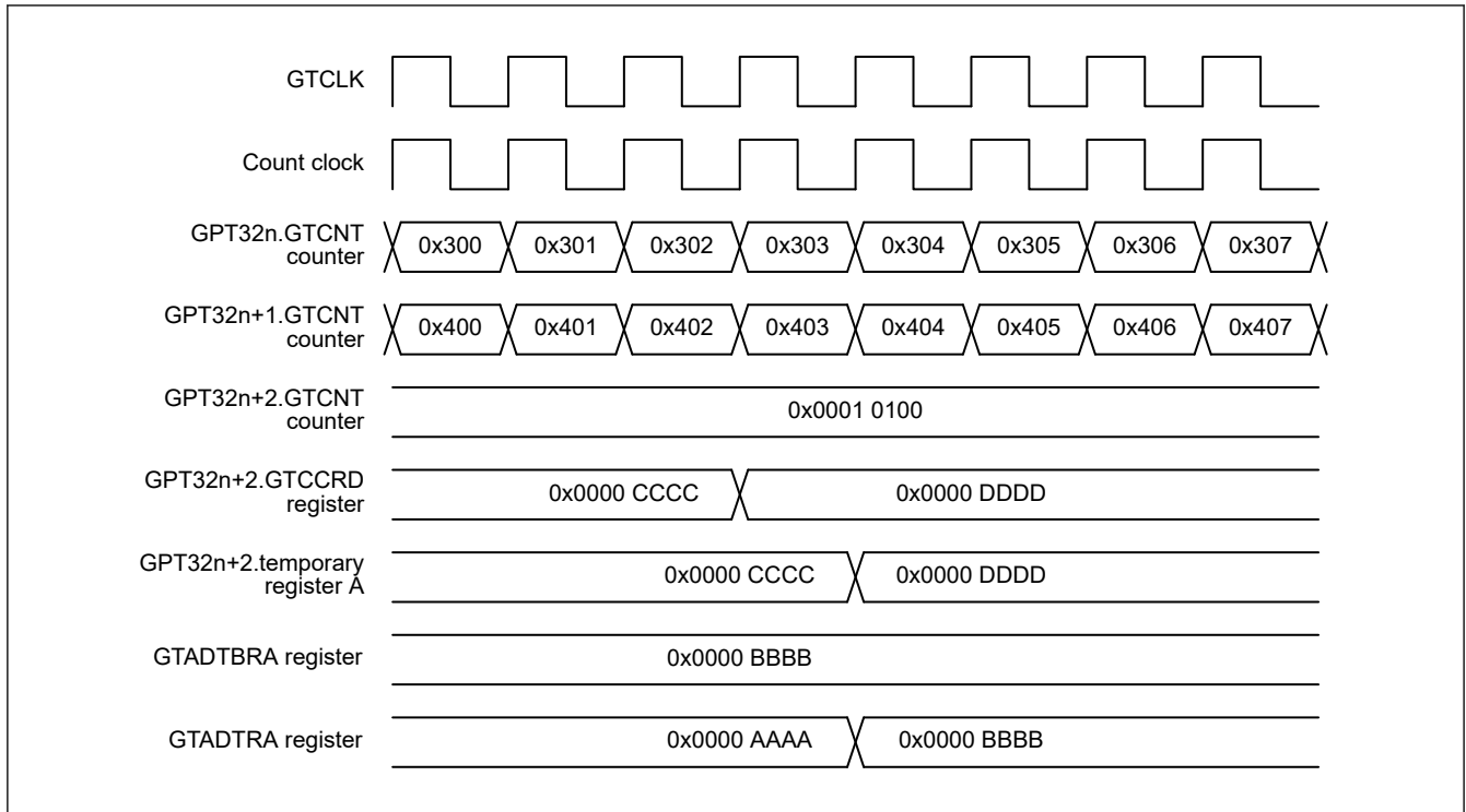
Figure 23.32 Example of Buffer Operation of the GTADTRA and GTADTRB Registers at the GTCCRD Register of Slave Channel 2 Updating in Complementary PWM Mode
