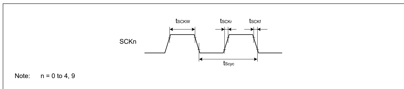
Figure 70.68 SCK clock input/output timing
