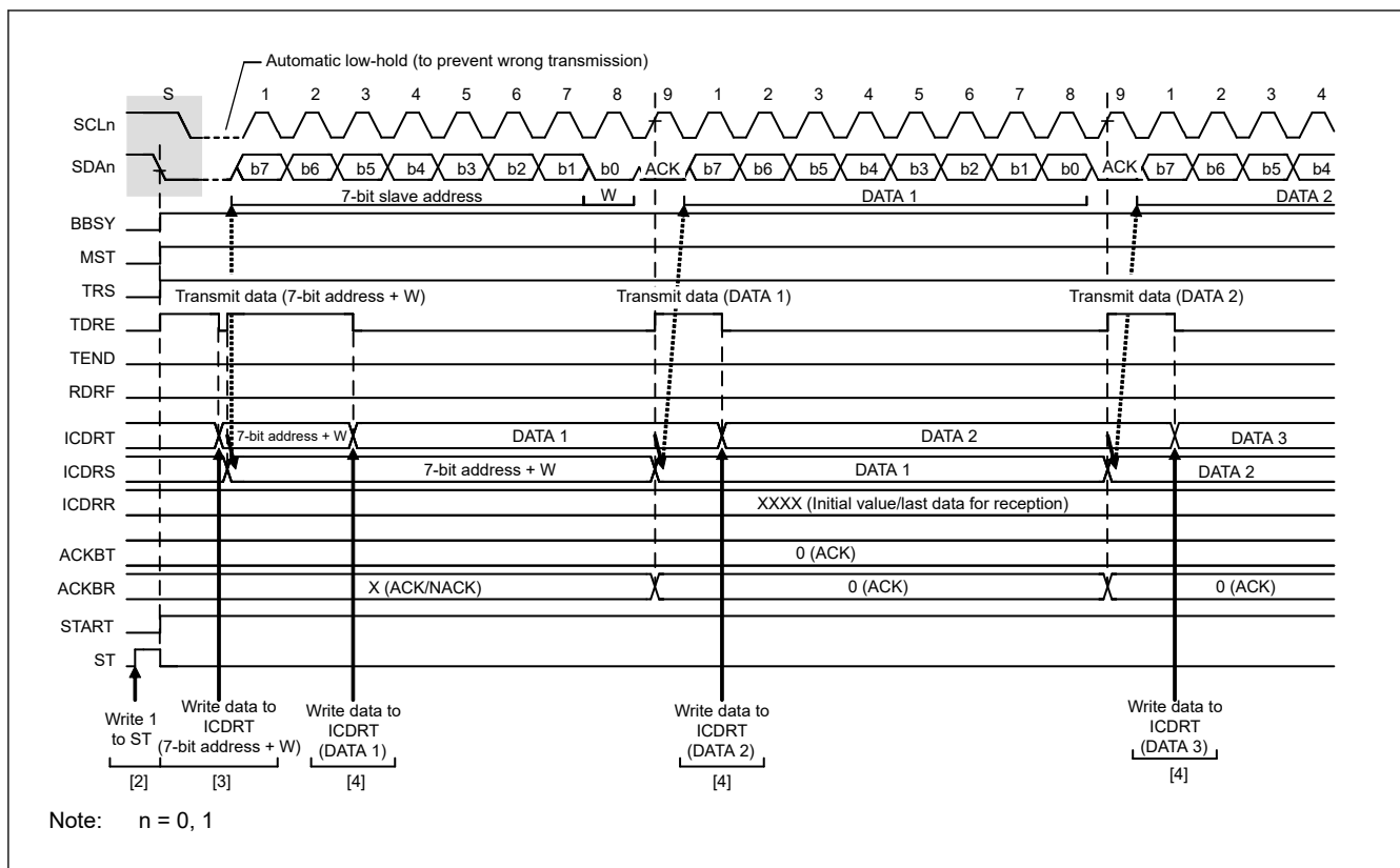
Figure 40.7 Master transmit operation timing (1) with 7-bit address format
