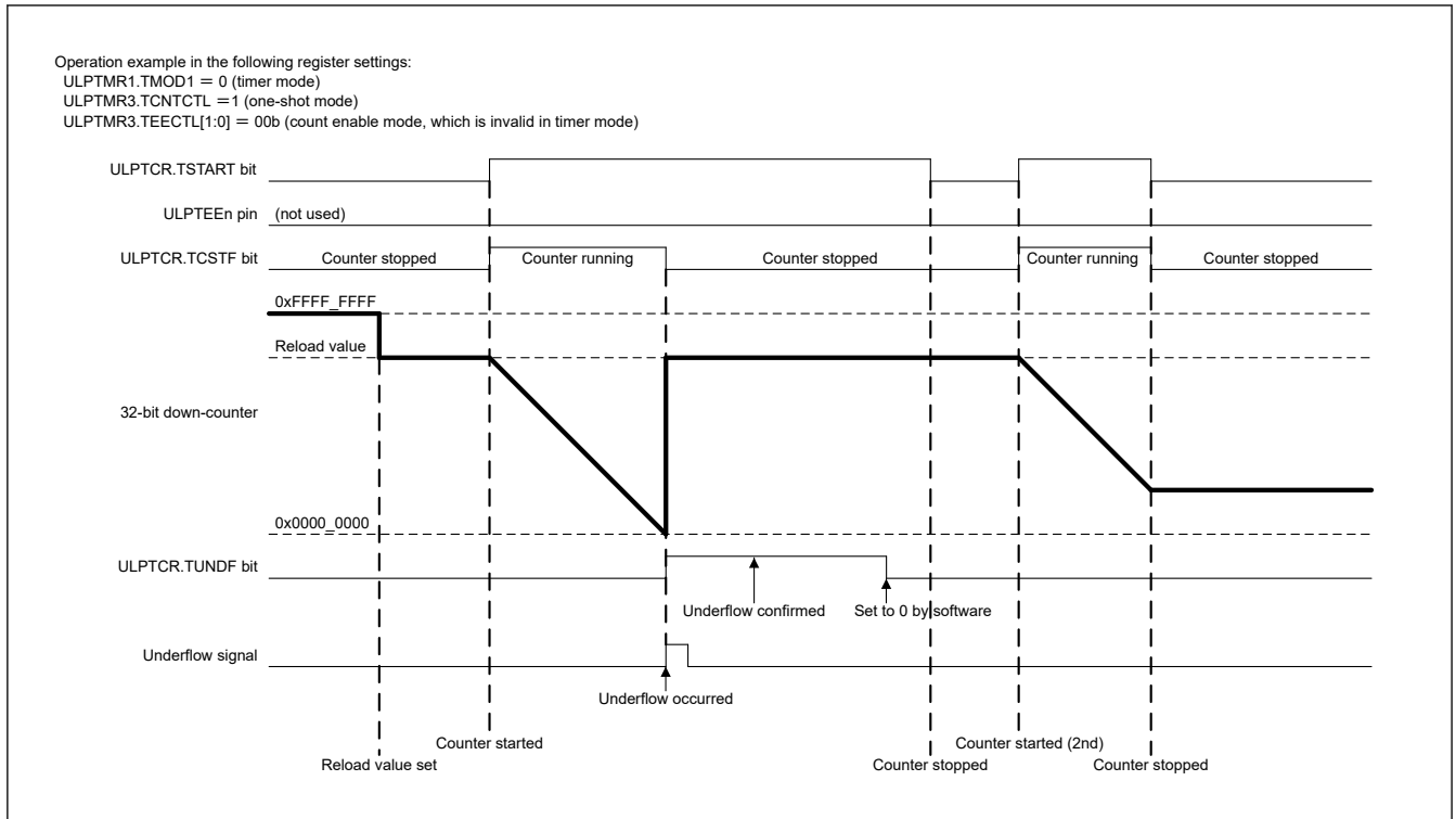
Figure 26.3 Operation example in timer and one-shot modes
