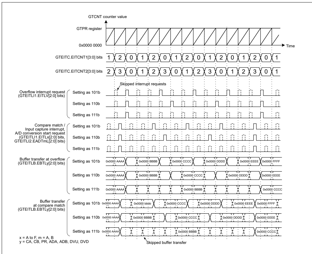
Figure 23.144 Example of Extended Interrupt Skipping Function Operation (Up-Counting Saw Waves, Counting Overflow, Extended Interrupt Skipping 1 Skipping Count: 2, Counting Overflow, Extended Interrupt Skipping 2 Skipping Count: 3, Extended Interrupt Skipping Counter 2 Initial Value: 0, Skipped in the Period other than GTEITC.EITCNTk bits (k = 1, 2) as GTEITC.EIVTTk bits.)
