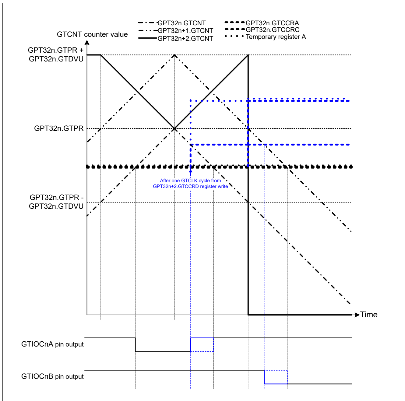
Figure 23.70 Example of Complementary PWM Mode 4 Single Buffer Operation (Down-Counting Crest Section) (Complementary PWM mode 4 single buffer operation, GTIOcNA pin = Low / GTIOcNB pin = High at GTCCRA register compare match during up-counting, GTIOcNA pin = High / GTIOcNB pin = Low at GTCCRA register compare match during down-counting, when a value not less than the GPT32n.GTCNT value is written to GTCCRD register after up-counting compare match before down-counting compare match) ( n = 4, 7 )
