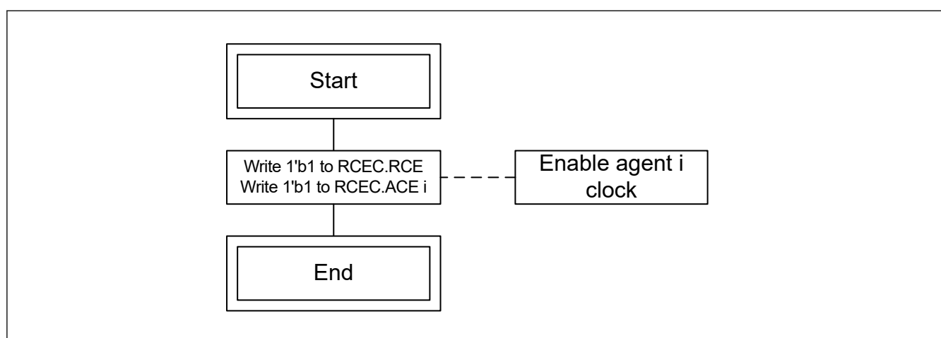
Figure 32.6 Agent i clock enable flow
