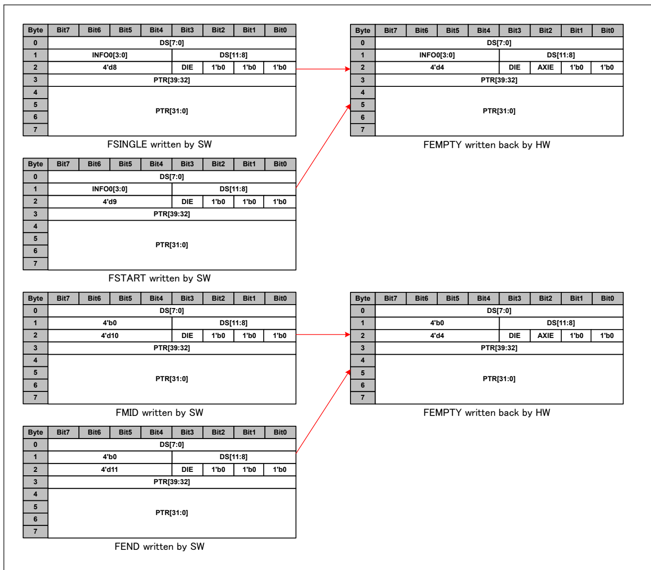
Figure 35.35 Data transmission process descriptor utilization format
