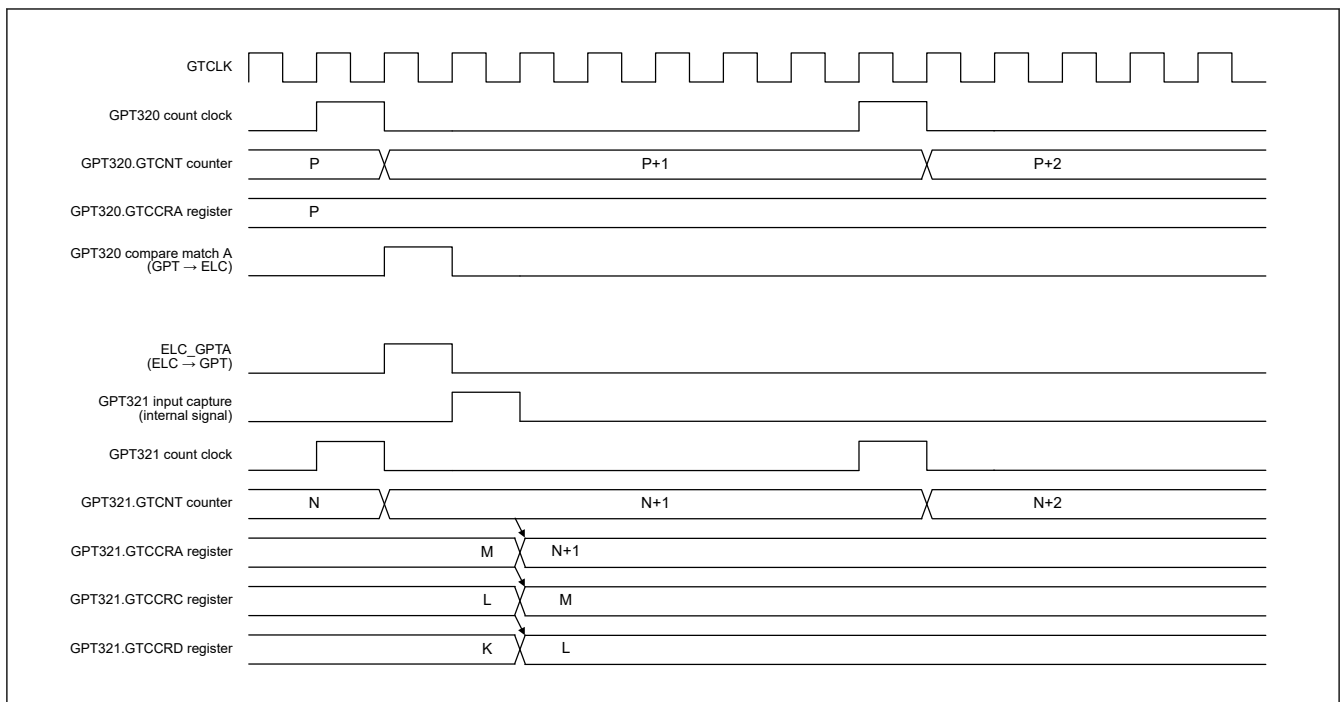
Figure 23.14 Example of the Timing of Input Capture Operation in Response to ELC_GPTA Event Input
