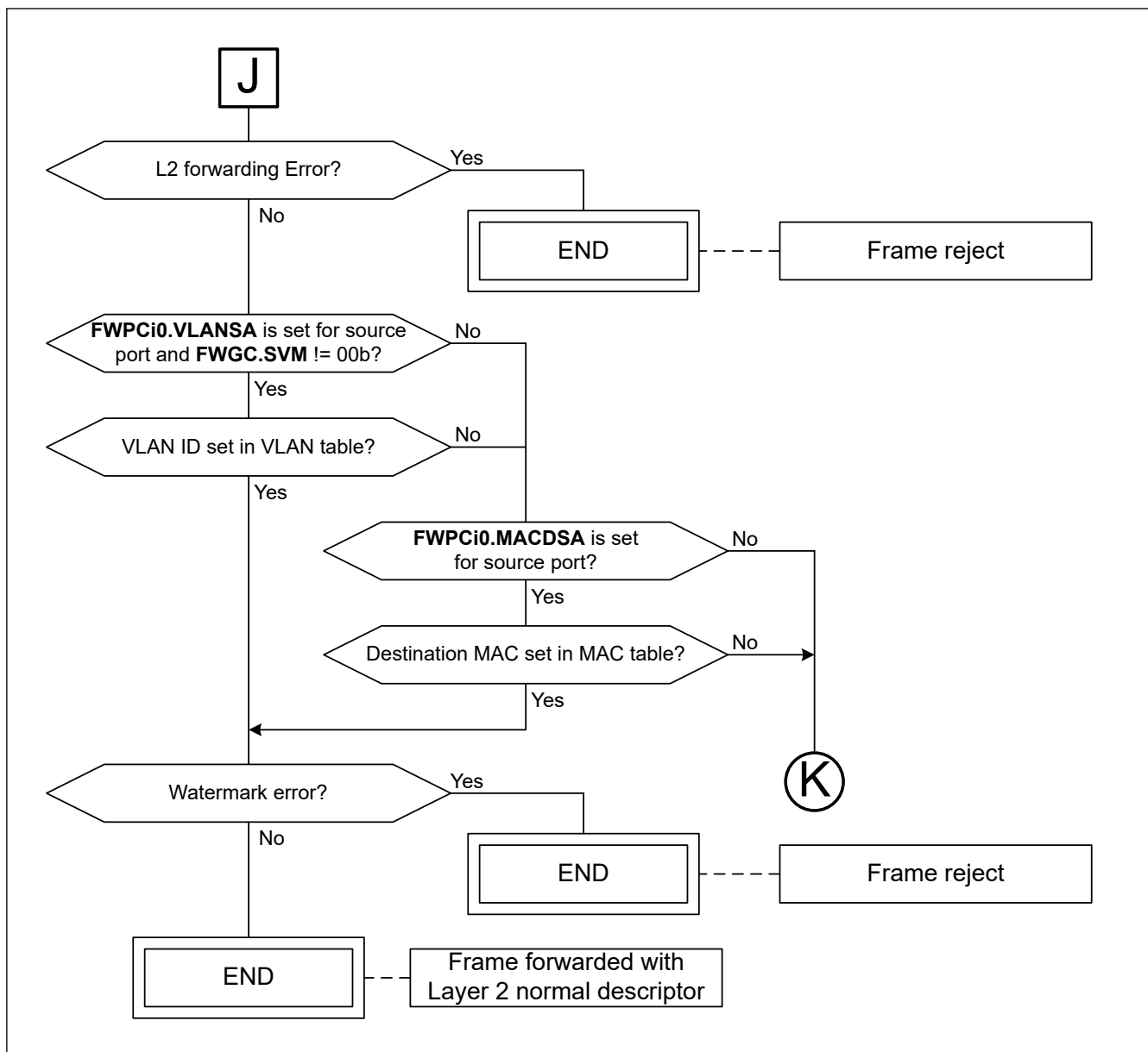
Figure 31.96 L2 forwarding unsecure flow
