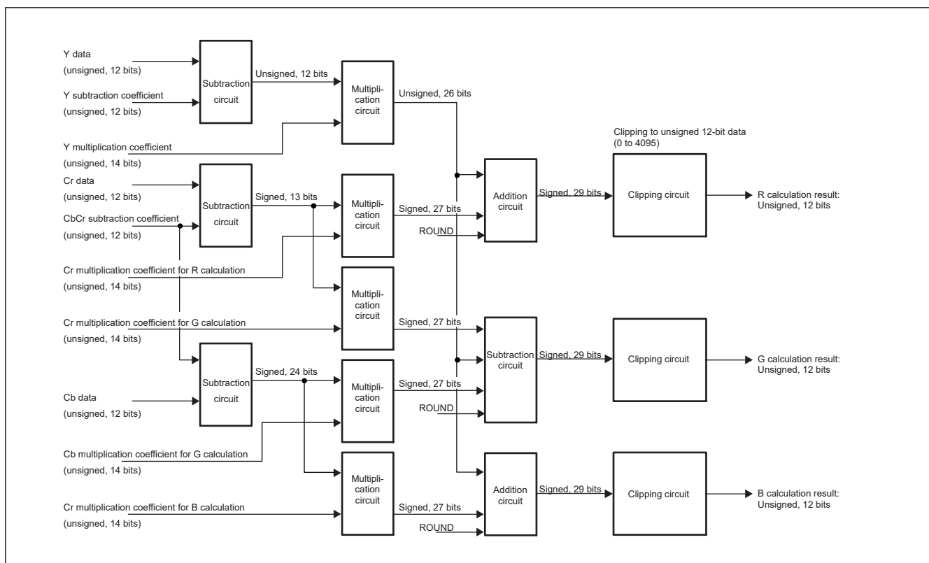
Figure 68.9 YCbCr to RGB calculation circuit configuration
