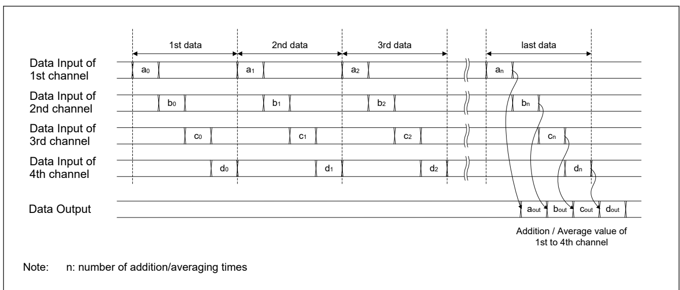
Figure 54.41 Example operation of A/D-converted value addition/averaging function (Hybrid mode)
