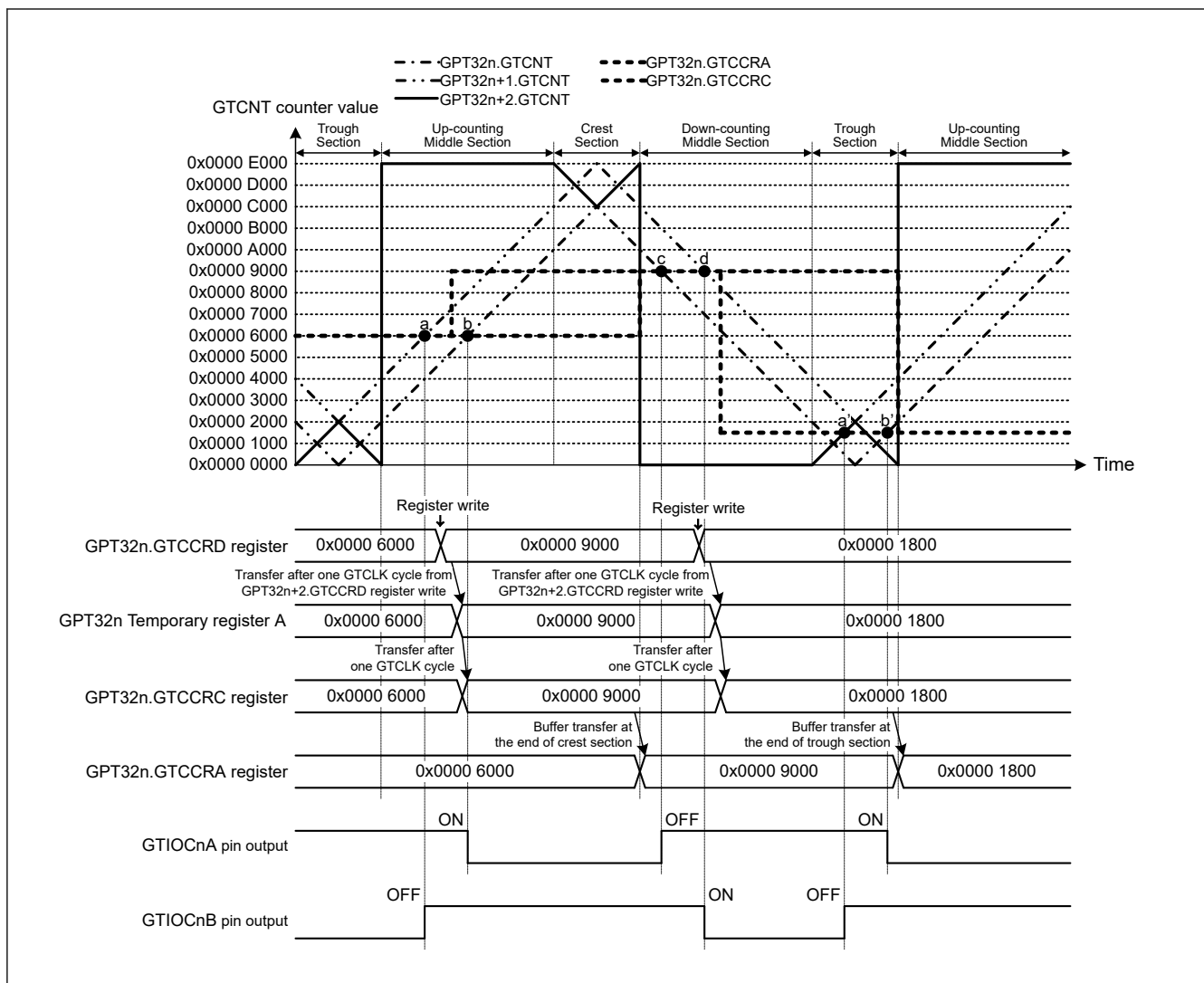
Figure 23.59 Example of Compare Match Generation Sequence Operation in Complementary PWM Mode (Complementary PWM mode 3 single buffer operation, GTIOCnA pin = Low / GTIOCnB pin = High at GTCCRA register compare match during up-counting, GTIOCnA pin = High / GTIOCnB pin = Low at GTCCRA register compare match during down-counting, the dead time value is 0x0000 2000, compare match generation order: c → d → a' → b' (n = 4, 7))
