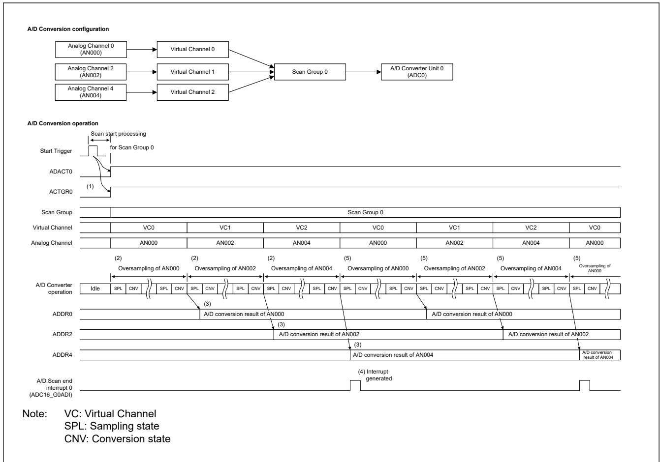
Figure 54.10 Example of scanning operation in Oversampling mode – Continuous scan mode
