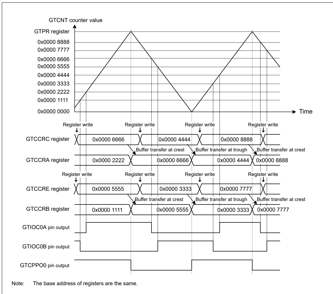
Figure 23.42 Example of triangle-wave PWM mode 2 operation with buffer operation, low output from the GTIOCnA pin and high output from the GTIOCnB pin at count start, output toggled at GTCCRA/ GTCCRB compare match, output retained at cycle end, and GTIOR.PSYE = 1
