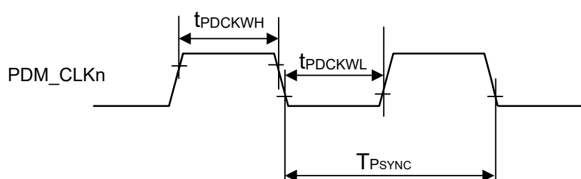
Figure 70.123 Timing of clock output (PDM_CLKn)
