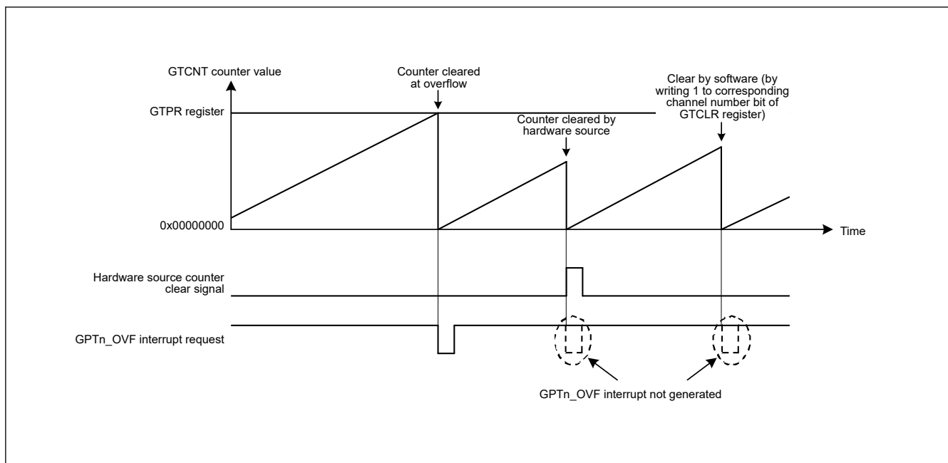
Figure 23.90 Relationship between counter clearing by hardware source and GPTn_OVF (n = 0 to 13) interrupt
