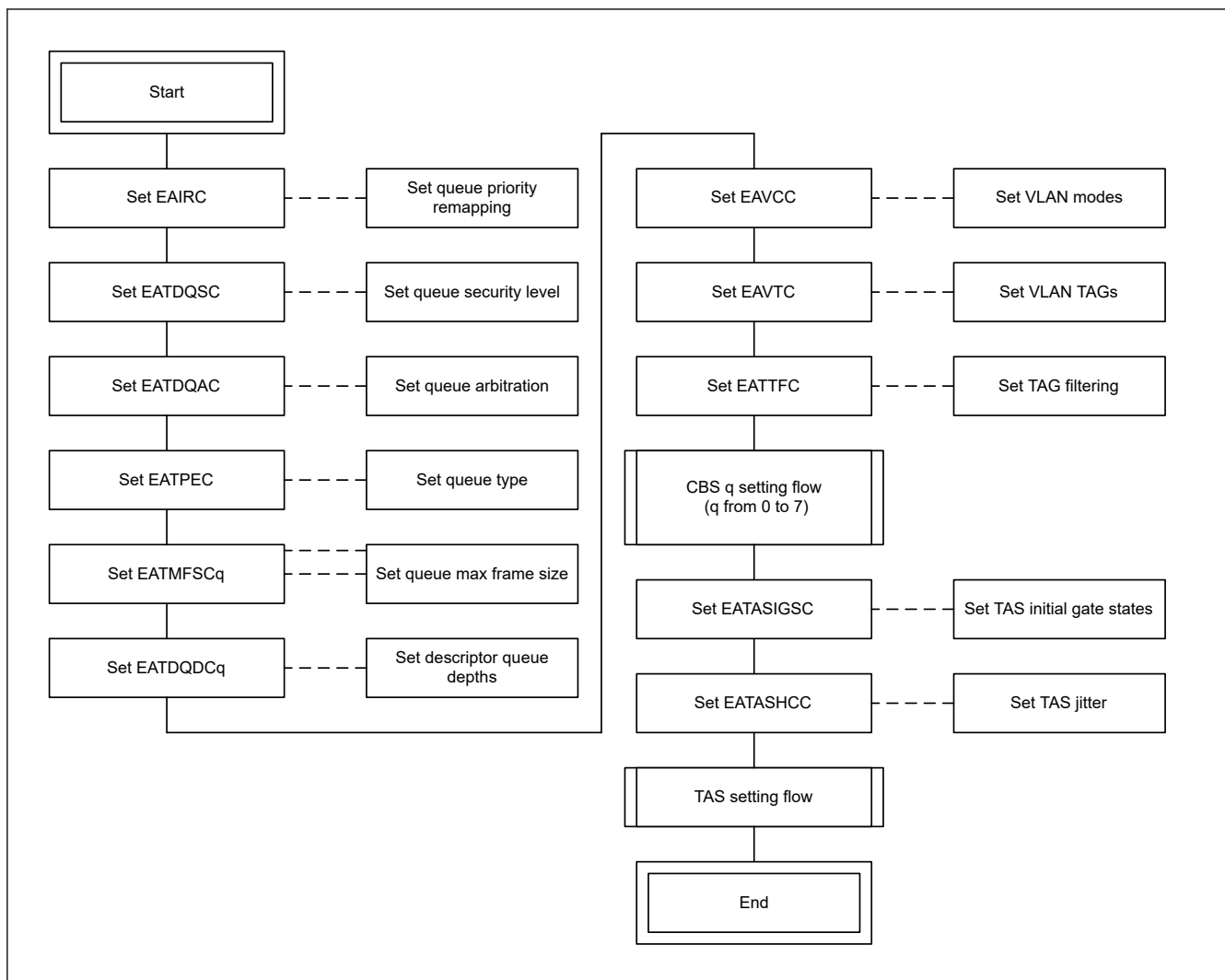
Figure 33.17 Full setting flow
