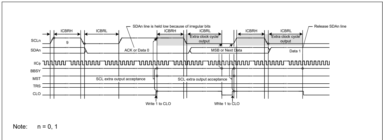
Figure 40.49 Extra SCL clock cycle output function using the CLO bit
