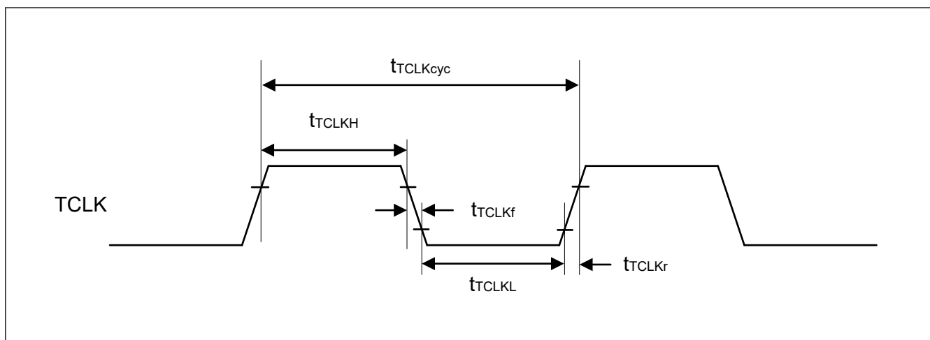
Figure 70.159 ETM TCLK timing
