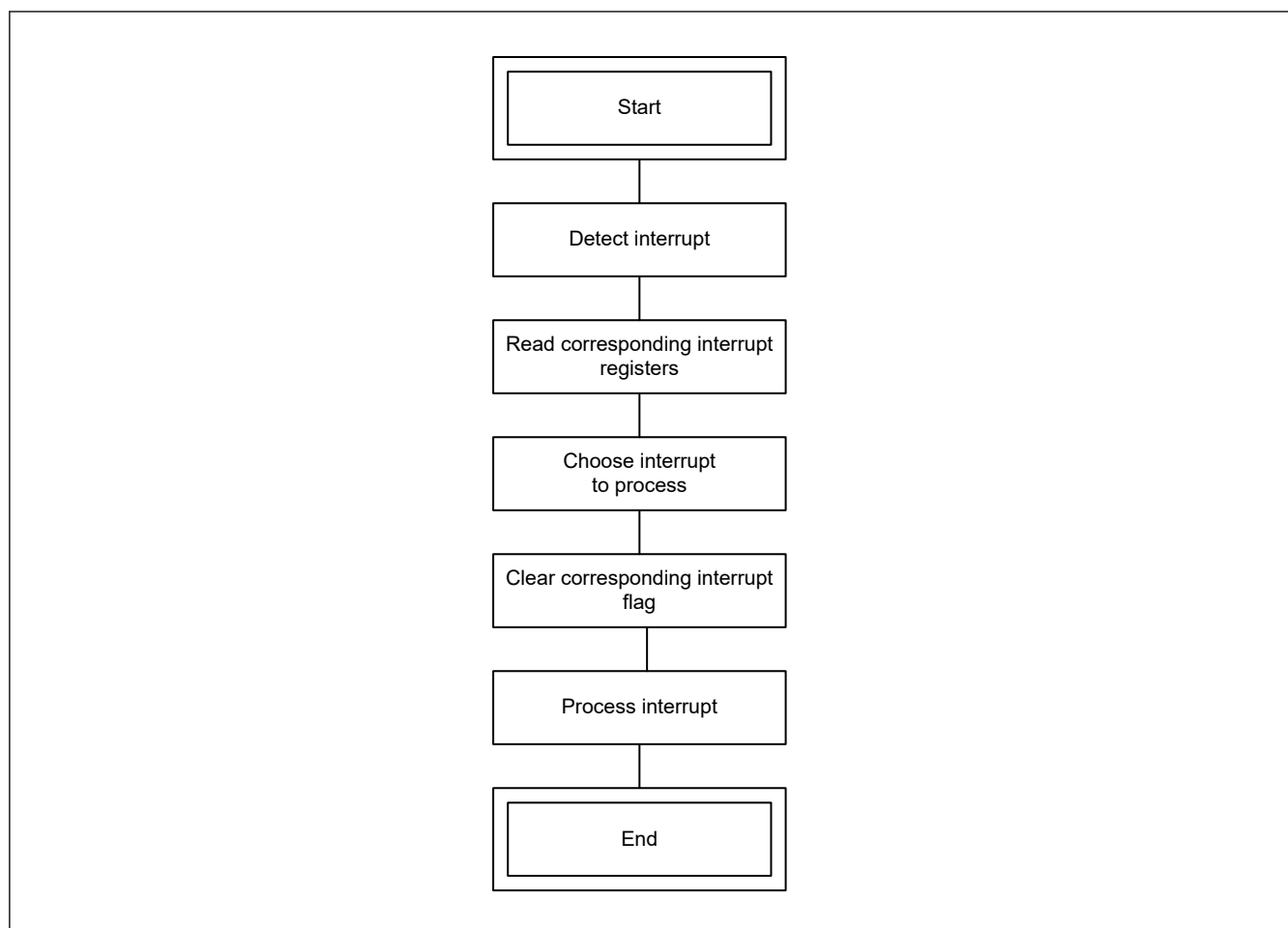
Figure 33.16 Interrupt handling flow
