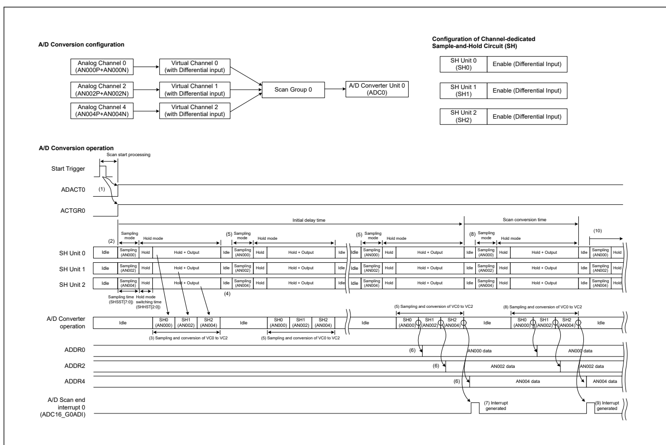
Figure 54.21 Basic operation of channel-dedicated sample-and-hold circuit in Hybrid mode – Continuous scan mode
