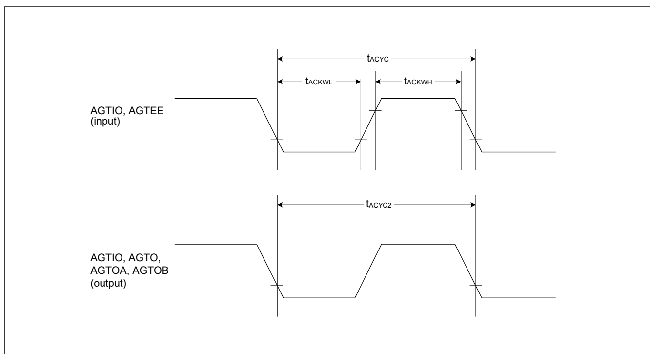
Figure 70.65 AGT input/output timing
