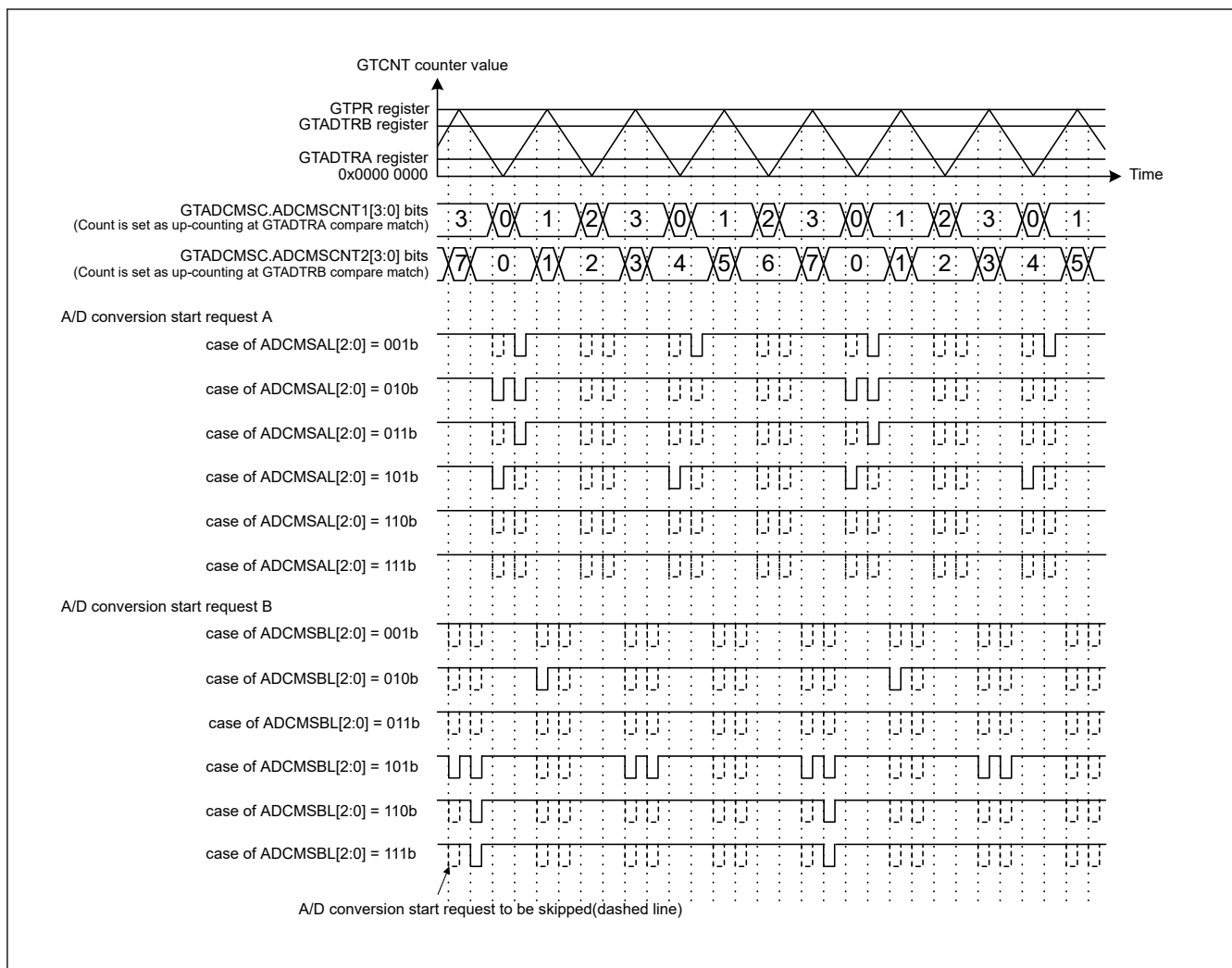
Figure 23.148 Example of A/D Conversion Start Request Compare Match Skipping Function Operation (Triangle wave, A/D Conversion Start Request Compare Match Skipping 1 Skipping Count: 3 Counting GTADTRA compare match, A/D Conversion Start Request Compare Match Skipping 2 Skipping Count: 7 Counting GTADTRB compare match)
