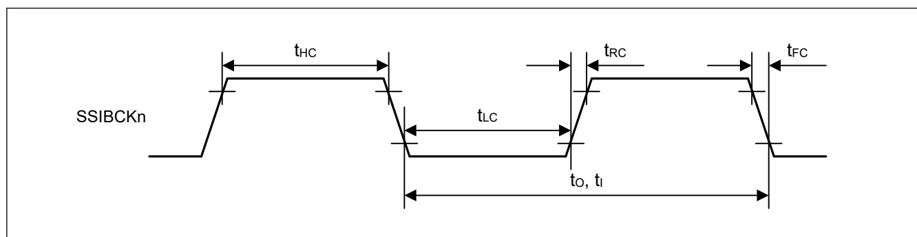
Figure 70.102 SSIE clock input/output timing
