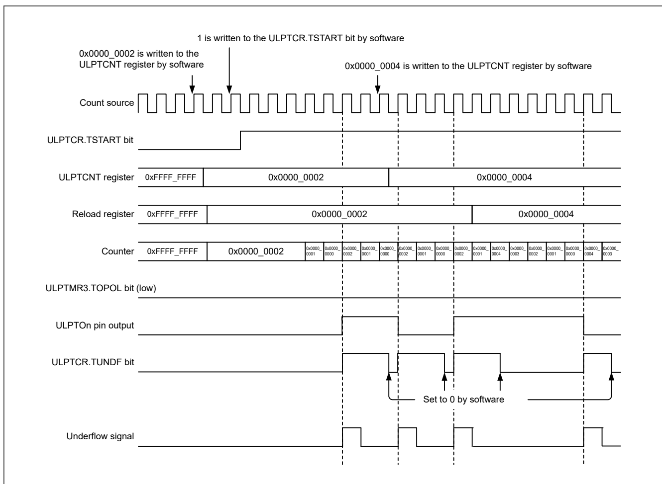
Figure 26.17 Operation example of pulse output
