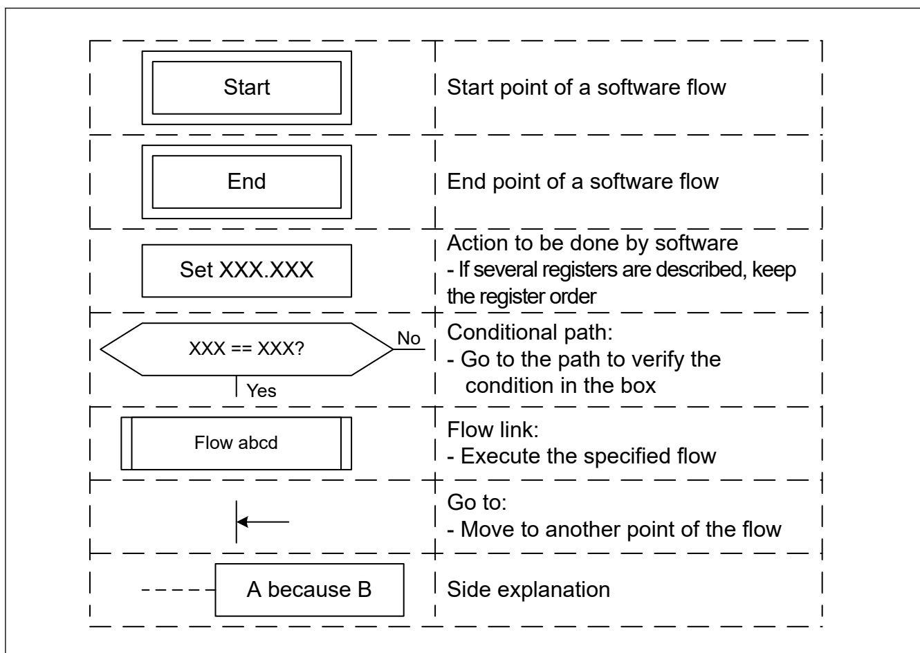
Figure 32.2 Software flow legend
