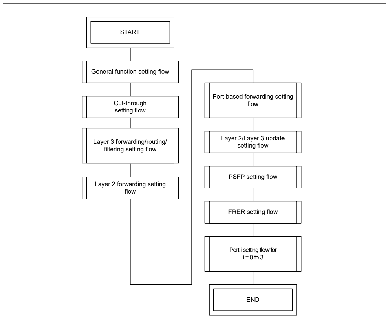
Figure 31.33 Full setting flow
