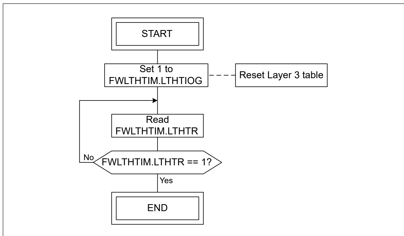
Figure 31.11 Reset flow of Layer 3 table
