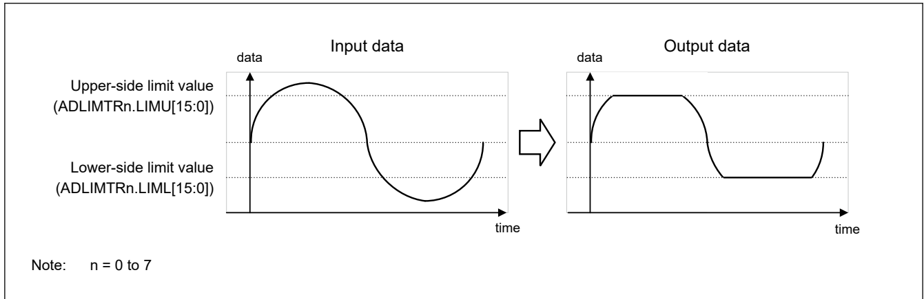
Figure 54.42 Example of limiter clip function operation
