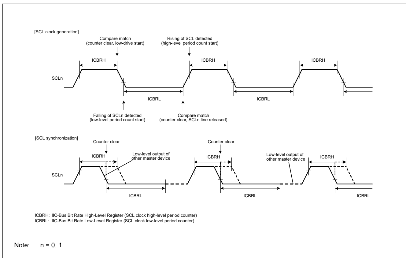
Figure 40.21 Generation and synchronization of SCL signal from IIC
