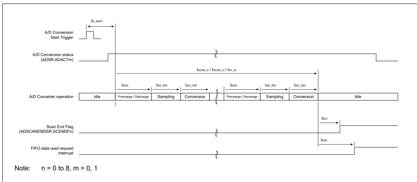
Figure 54.62 Scan end processing time (SAR/Oversampling/Hybrid mode – Single scan mode)
