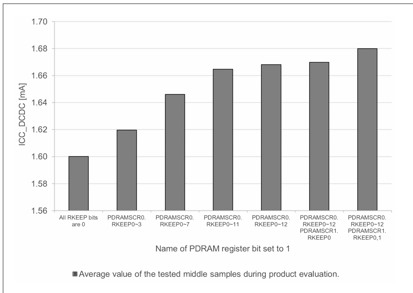
Figure 70.12 Software Standby current per SRAM state (ICC_DCDC, SS2LP_0, SVSCR_3) (reference data)
