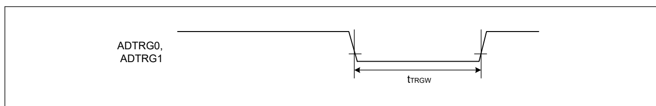
Figure 70.67 ADC trigger input timing
