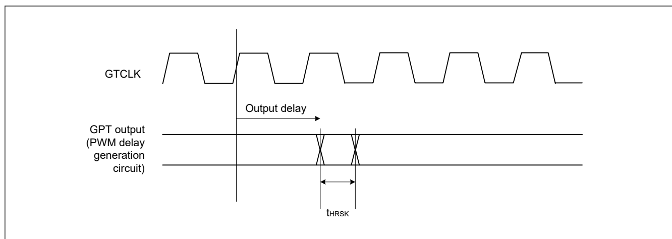
Figure 70.64 GPT (PDG) output delay skew
