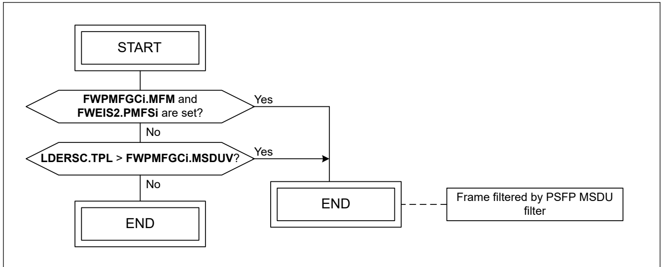
Figure 31.103 MSDU filtering flow for MSDU filter i
