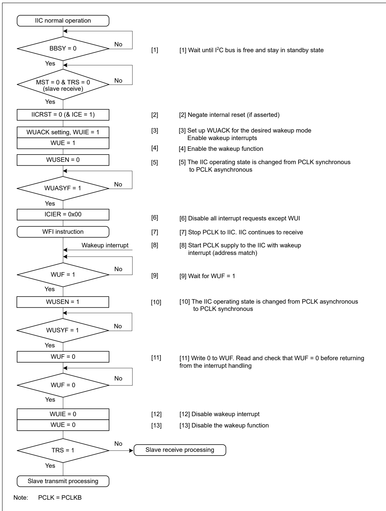
Figure 40.33 Example operation of normal wakeup mode 2 when wakeup is triggered by a wakeup interrupt on match of the slave address
