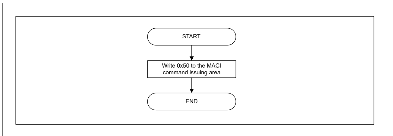
Figure 60.14 Usage of the Status Clear command
