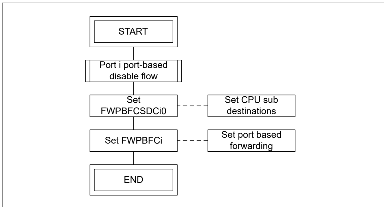
Figure 31.22 Port i port-based setting flow
