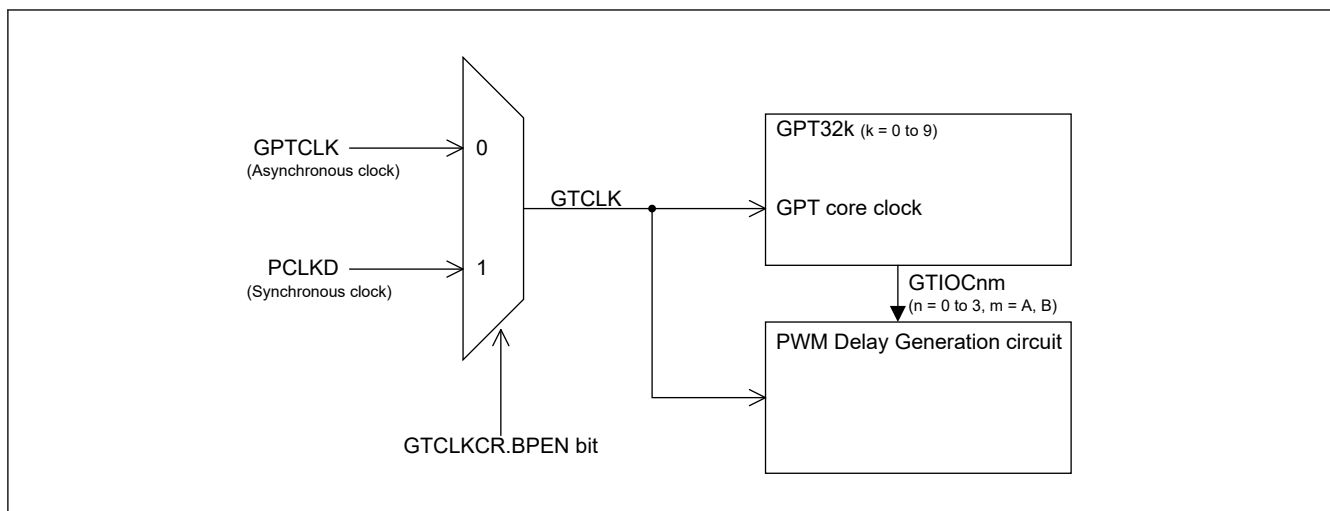
Figure 23.3 GPT core clock selection diagram
