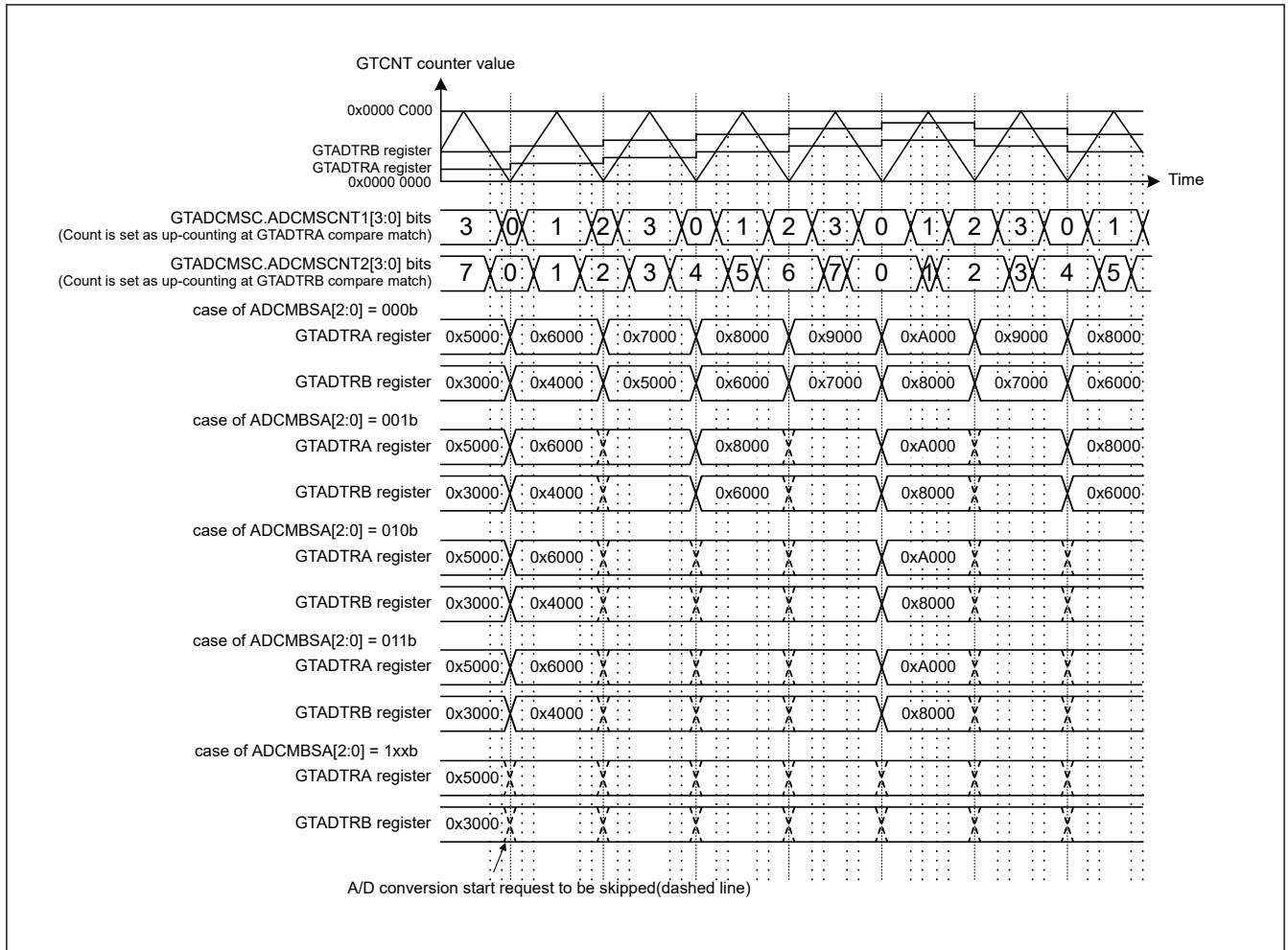
Figure 23.149 Example of A/D Conversion Start Request Compare Match Skipping Function Operation (Triangle wave, A/D Conversion Start Request Compare Match Skipping 1 Skipping Count: 3 Counting GTADTRA compare match, A/D Conversion Start Request Compare Match Skipping 2 Skipping Count: 7 Counting GTADTRB compare match, Buffer transfer of GTADTRA and GTADTRB at trough)
