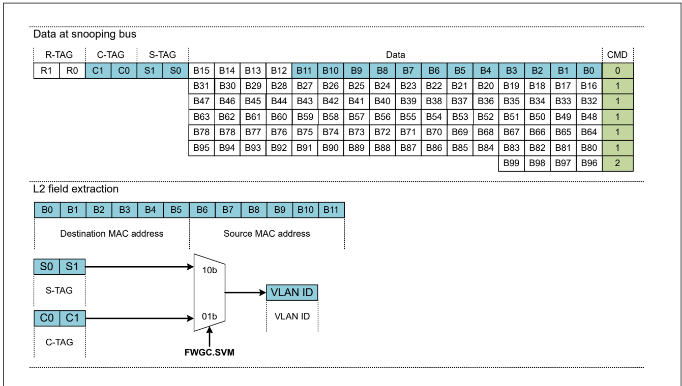
Figure 31.92 MAC address and VLAN ID extraction
