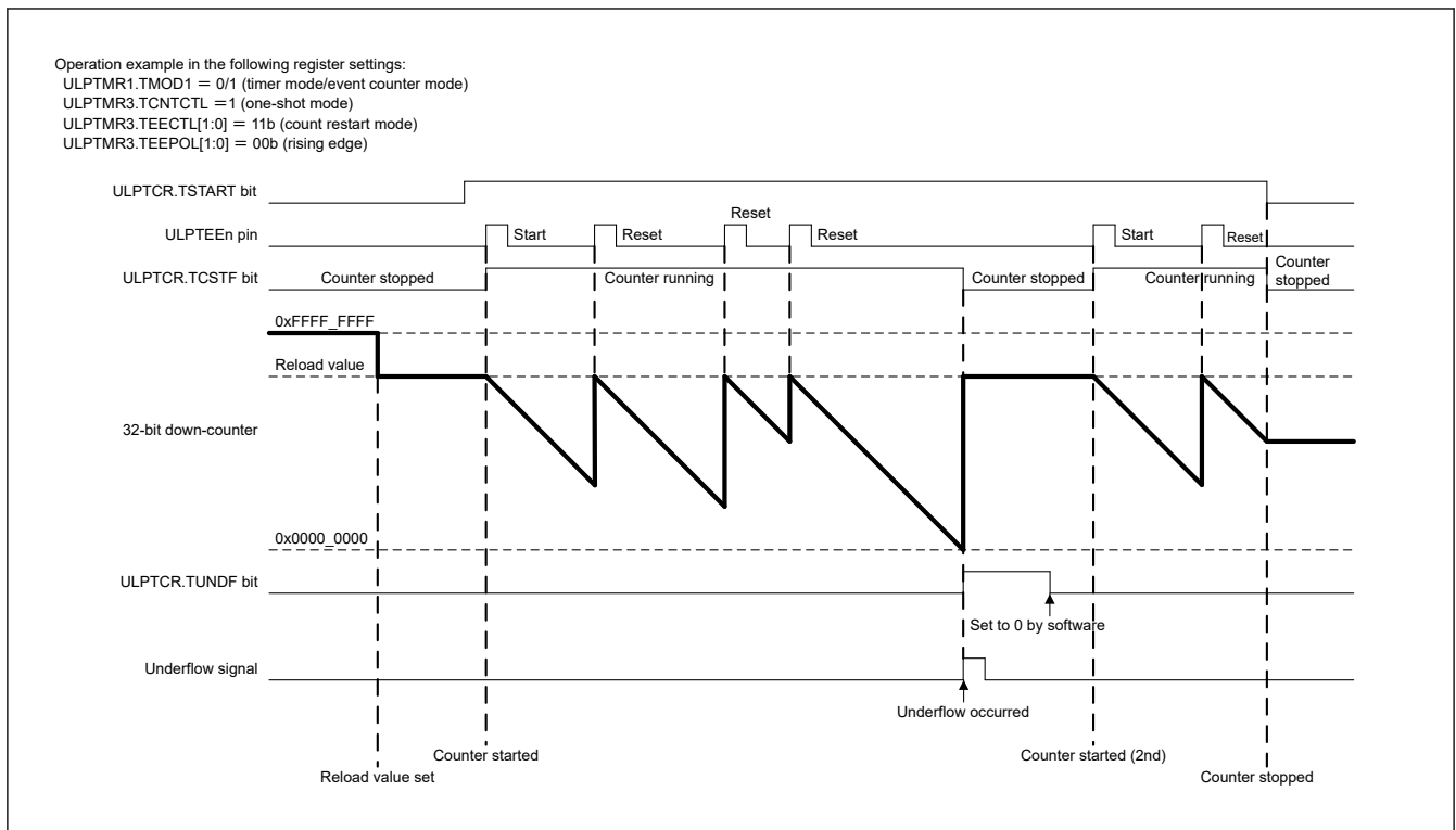
Figure 26.12 Operation example in common, one-shot, and count restart modes
