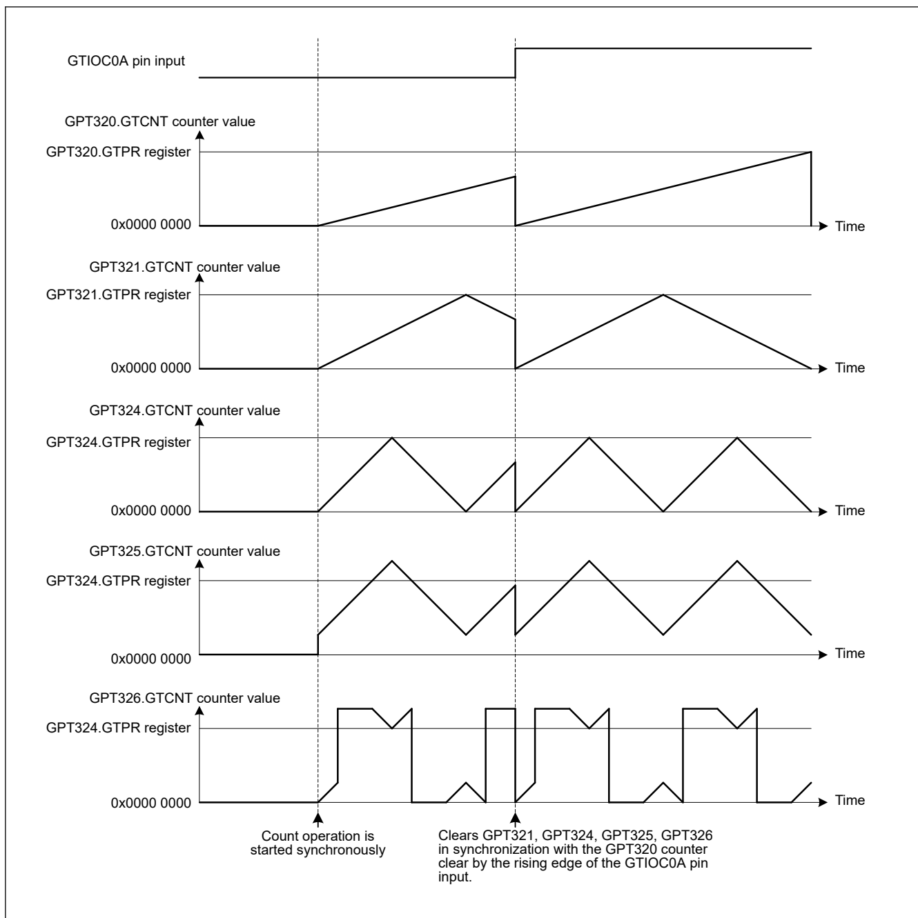
Figure 23.100 Example of Synchronous Clear Operation by Inter Channel Cooperation (GPT320 is saw-wave and counter is cleared by the rising edge of the GTIOC0A, GPT321 is triangle wave, GPT324,5,6 are complementary PWM mode. GPT320,1,4,5,6 are the same synchronous set/clear group)
