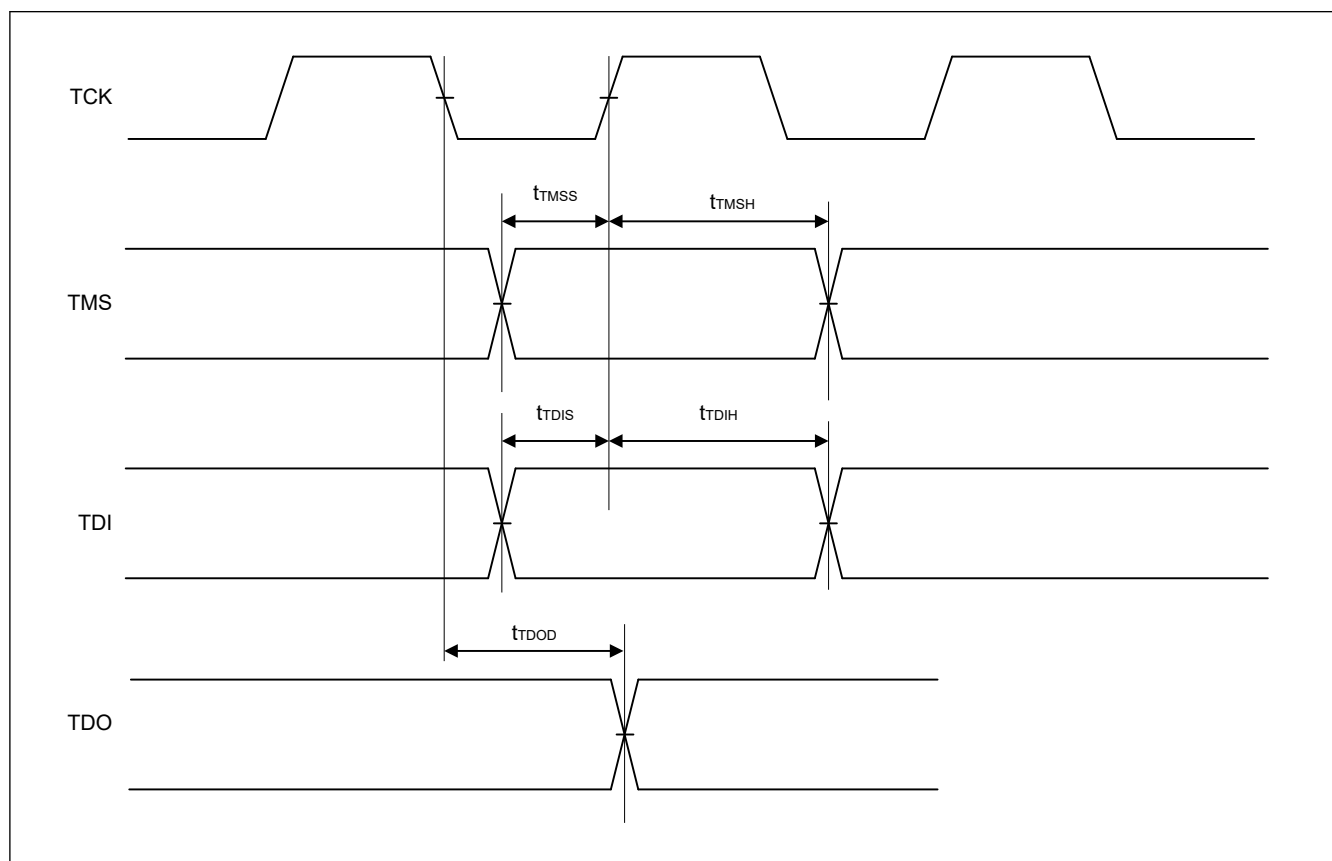
Figure 70.156 JTAG input/output timing
