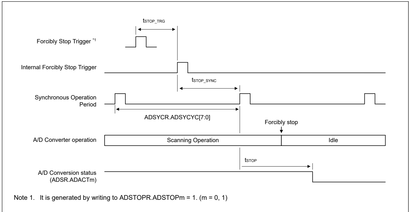
Figure 54.63 Forcibly stop processing time (SAR/Oversampling/Hybrid mode – Single scan mode)
