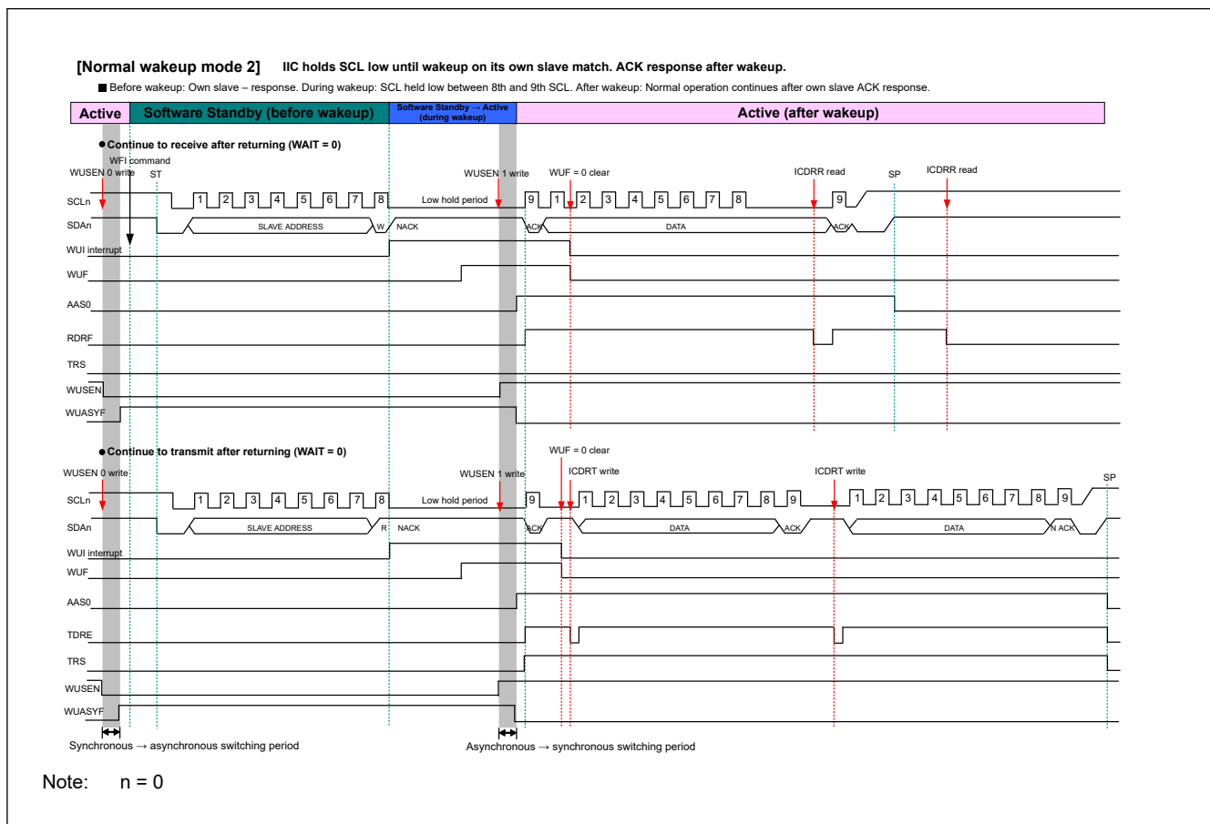
Figure 40.34 Timing of normal wakeup mode 2
