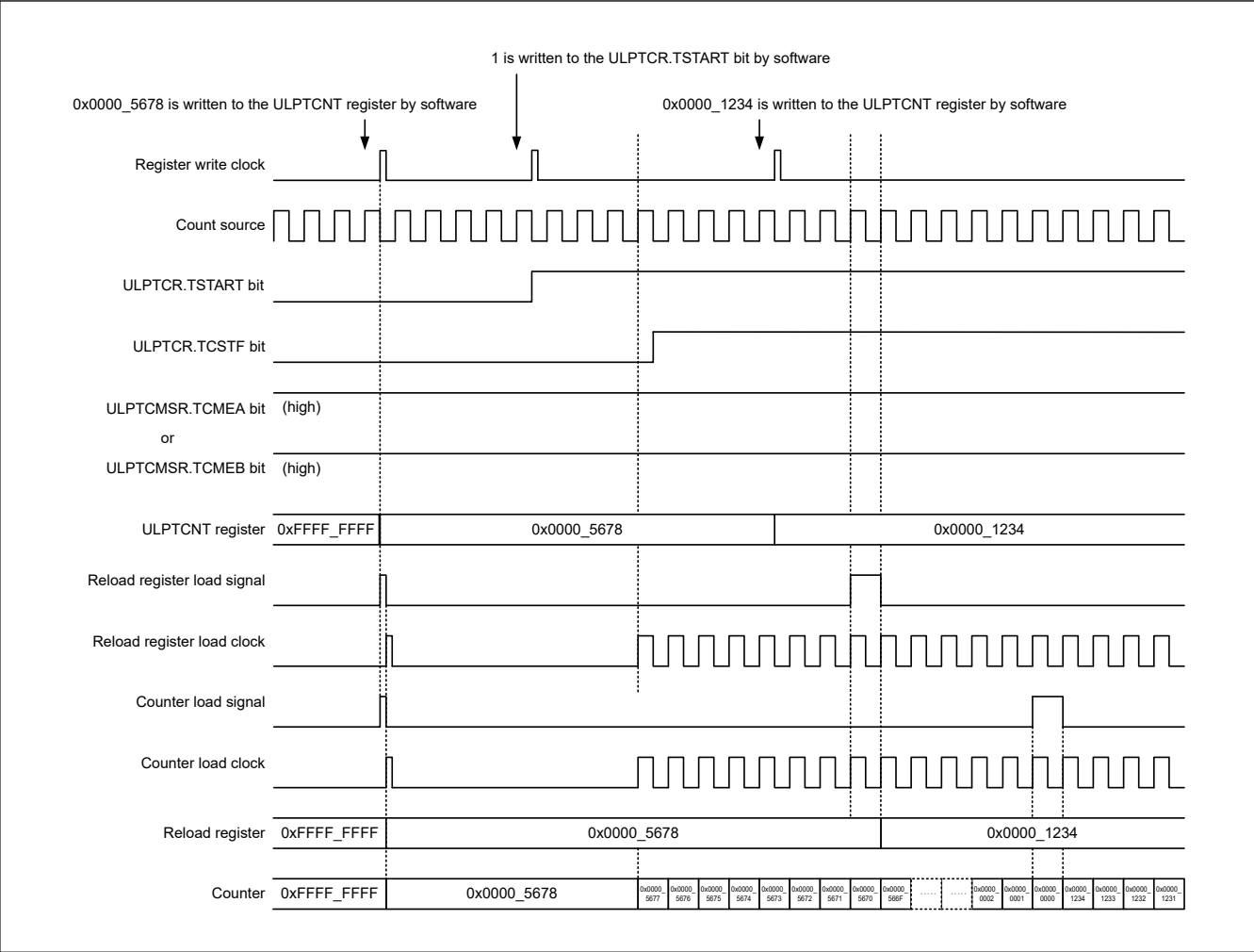
Figure 26.14 Counter and reload rewrite timing (under condition A or C)
