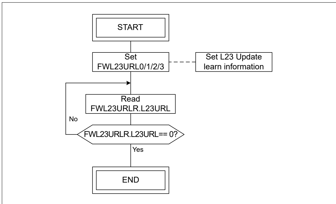
Figure 31.25 Learn flow of Layer 2/Layer 3 update rule
