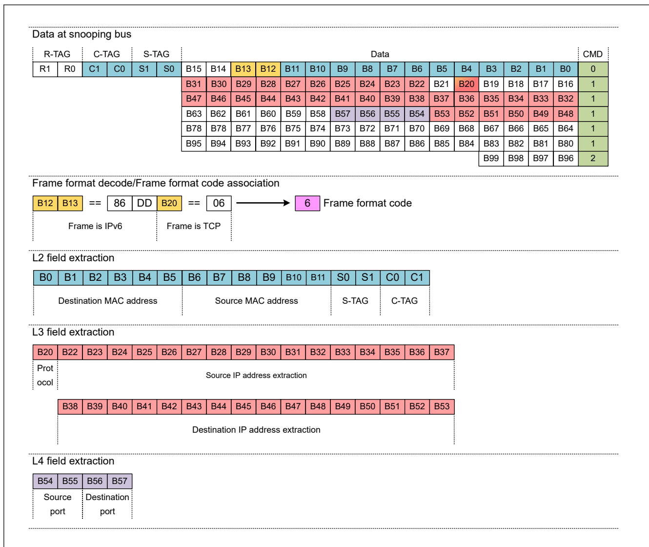
Figure 31.78 IPv6/TCP detection and data extraction
