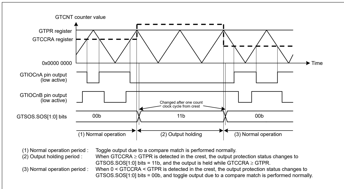
Figure 23.168 Example of Output Protection Function Operation When GTCCRA \geq GTPR is Set during Buffer Transfer at Crests (Restored to 0 < GTCCRA < GTPR during Buffer Transfer at Crests, Active Level: Low) (n = 0 to 13)
