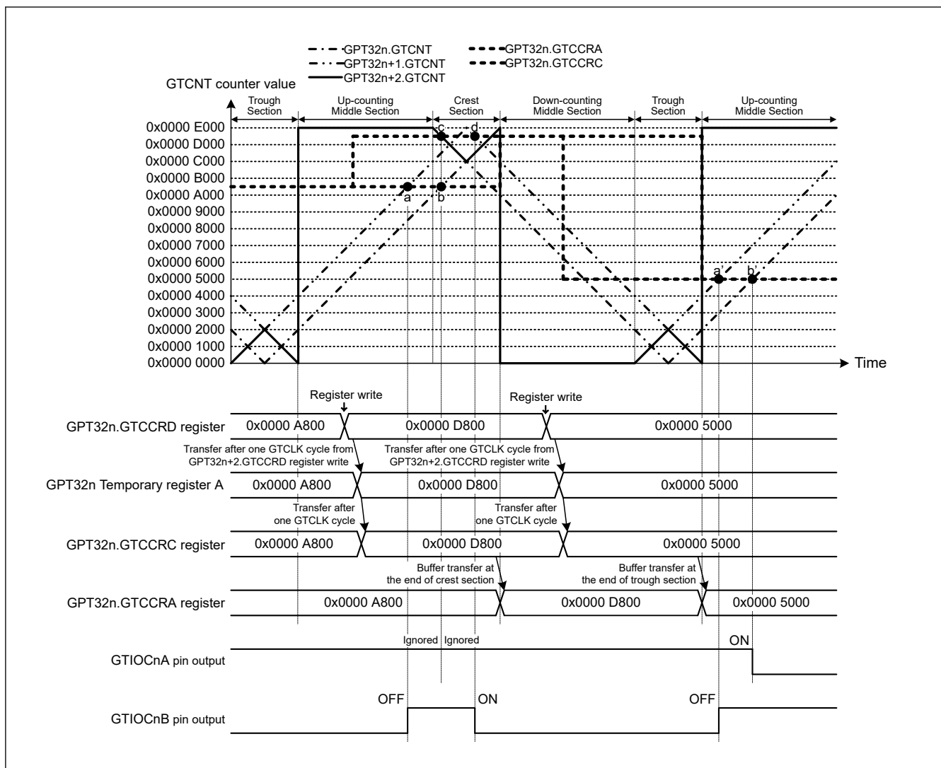
Figure 23.54 Example of Compare Match Generation Sequence Operation in Complementary PWM Mode (Complementary PWM mode 3 single buffer operation, GTIOCnA pin = Low / GTIOCnB pin = High at GTCCRA register compare match during up-counting, GTIOCnA pin = High / GTIOCnB pin = Low at GTCCRA register compare match during down-counting, the dead time value is 0x0000 2000, compare match generation order: a → (b, c) → d) (n = 4, 7)
