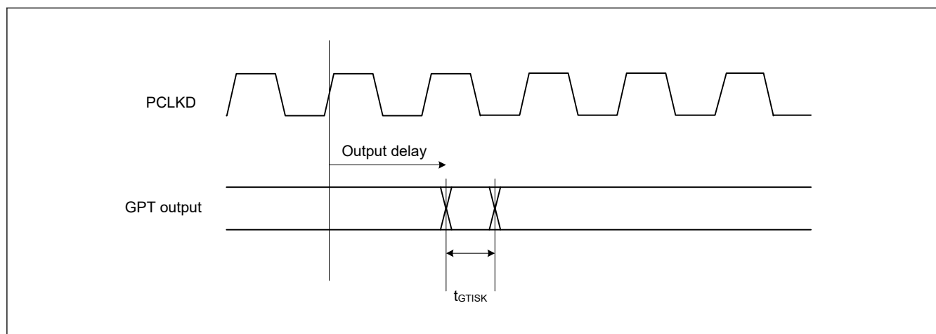
Figure 70.62 GPT output delay skew
