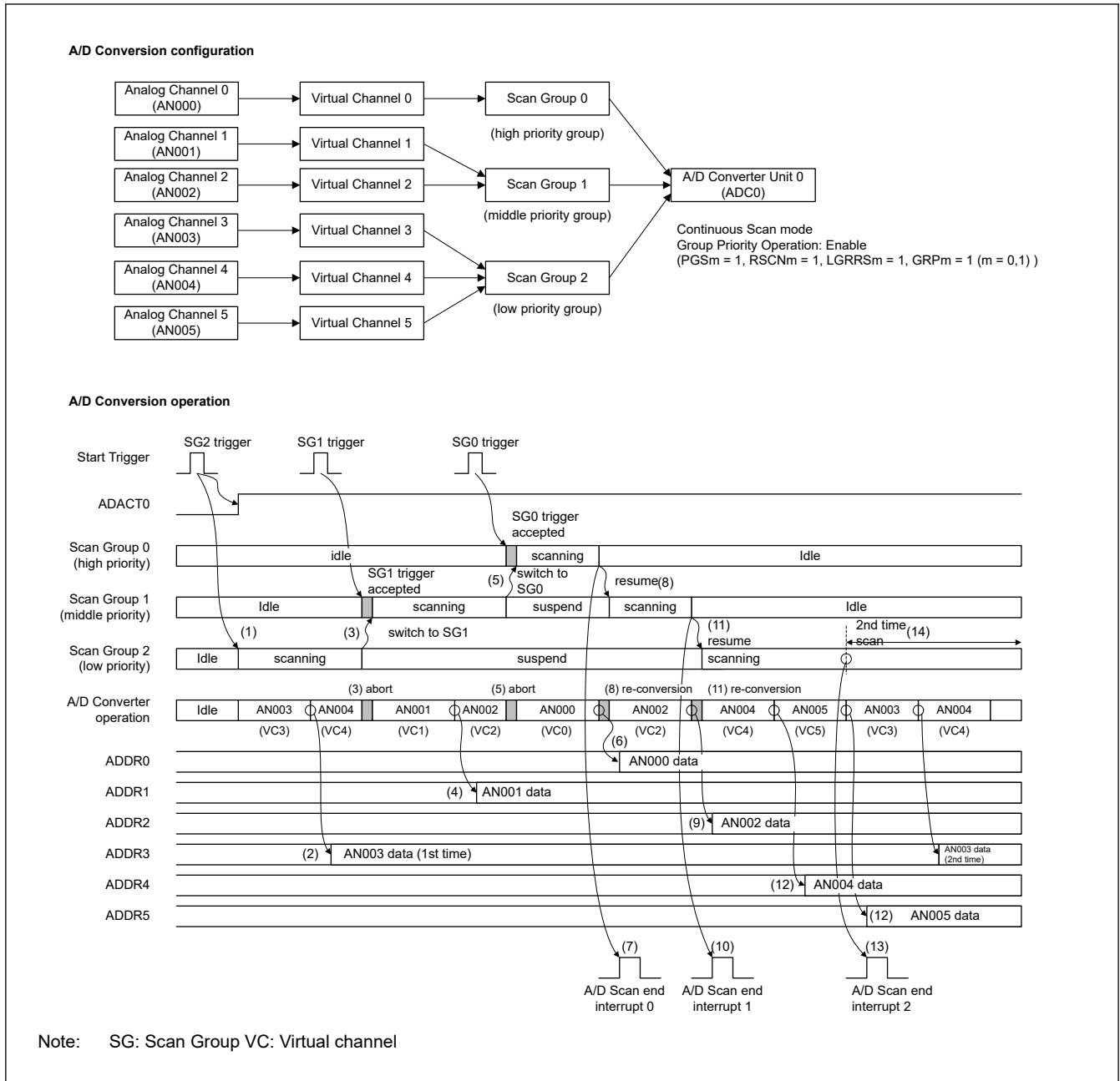
Figure 54.30 Example of group priority operation in SAR mode – Continuous scan mode (3 groups)
