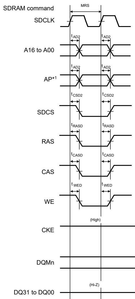
Figure 70.50 SDRAM mode register set timing
