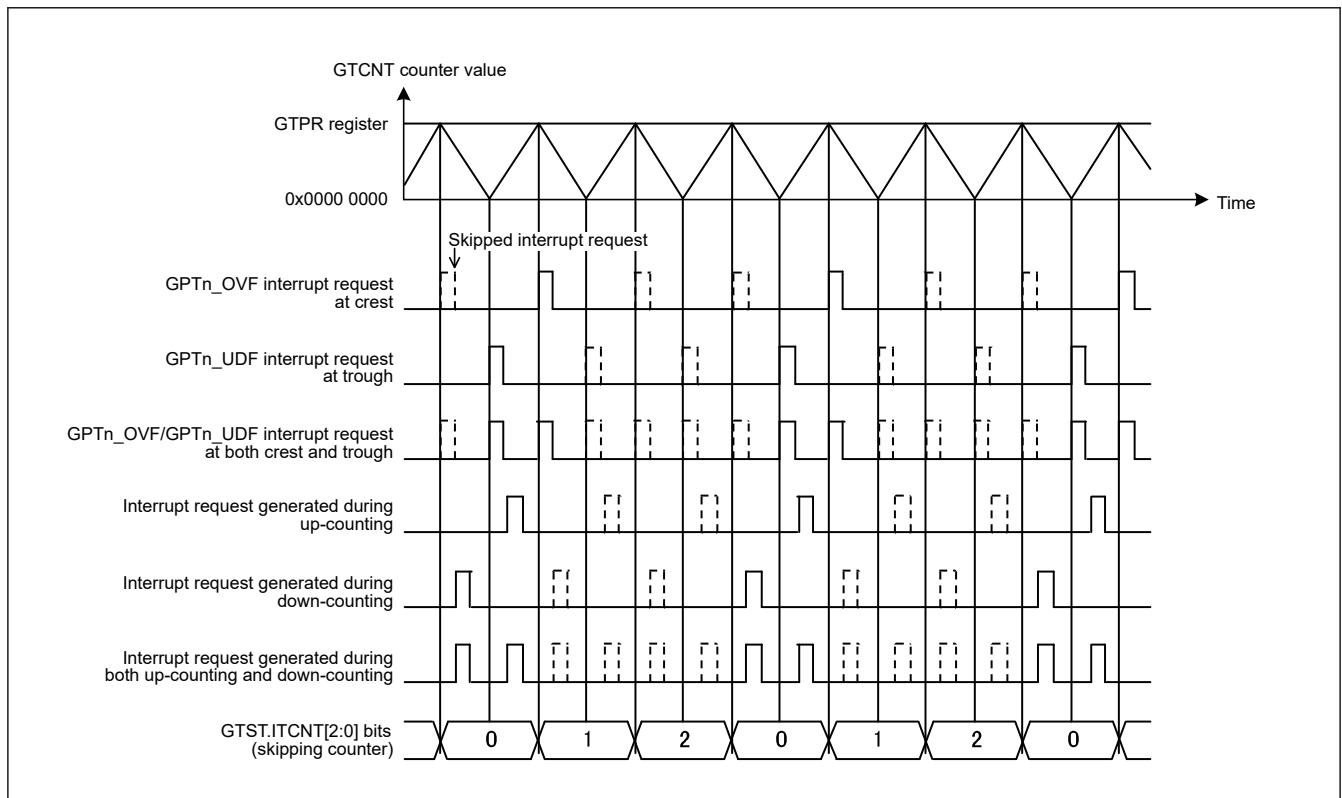
Figure 23.129 Example of Interrupt Skipping Function Operation (Triangle Waves, Counting and Skipping Crests, Skipping Count: 2)
