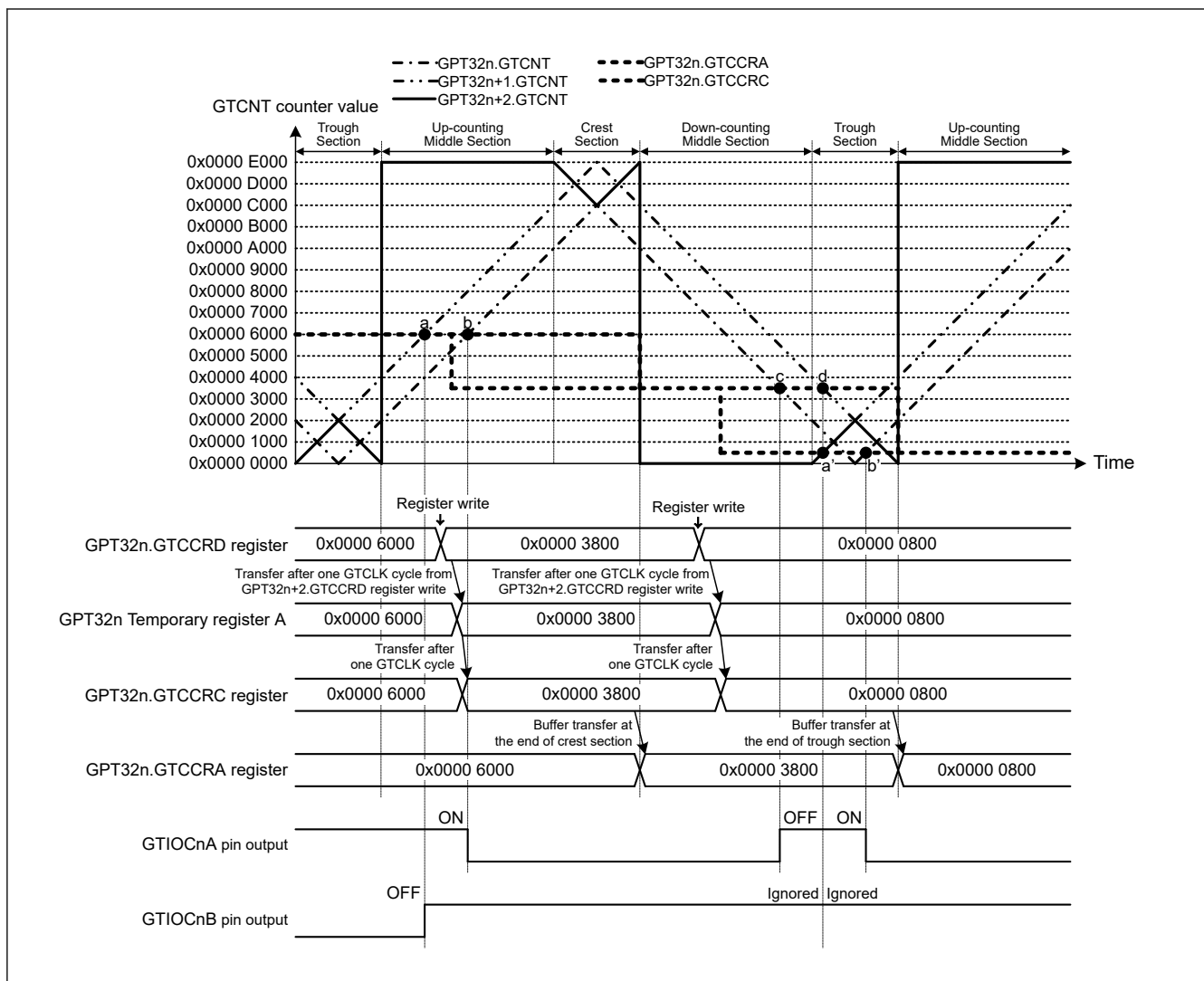
Figure 23.60 Example of Compare Match Generation Sequence Operation in Complementary PWM Mode (Complementary PWM mode 3 single buffer operation, GTIOCnA pin = Low / GTIOCnB pin = High at GTCCRA register compare match during up-counting, GTIOCnA pin = High / GTIOCnB pin = Low at GTCCRA register compare match during down-counting, the dead time value is 0x0000 2000, compare match generation order: c → (d, a') → b') (n = 4, 7)
