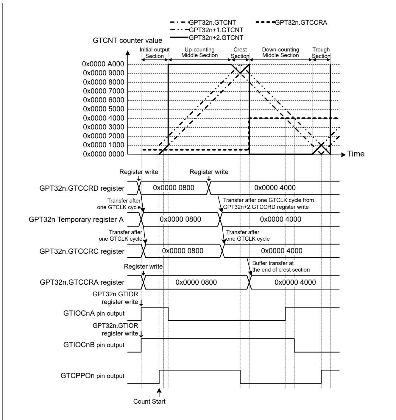
Figure 23.66 Example of Complementary PWM Mode Initial Output Operation (Complementary PWM mode 1 operation, GTIOcNA pin = Low / GTIOcNB pin = High at GTCCRA register compare match during up-counting, GTIOcNA pin = High / GTIOcNB pin = Low at GTCCRA register compare match during down-counting, the dead time value is 0x0000 1000, in the case that the initial GTCCRA register value is equal to or less than the dead time value) (n = 4, 7)
