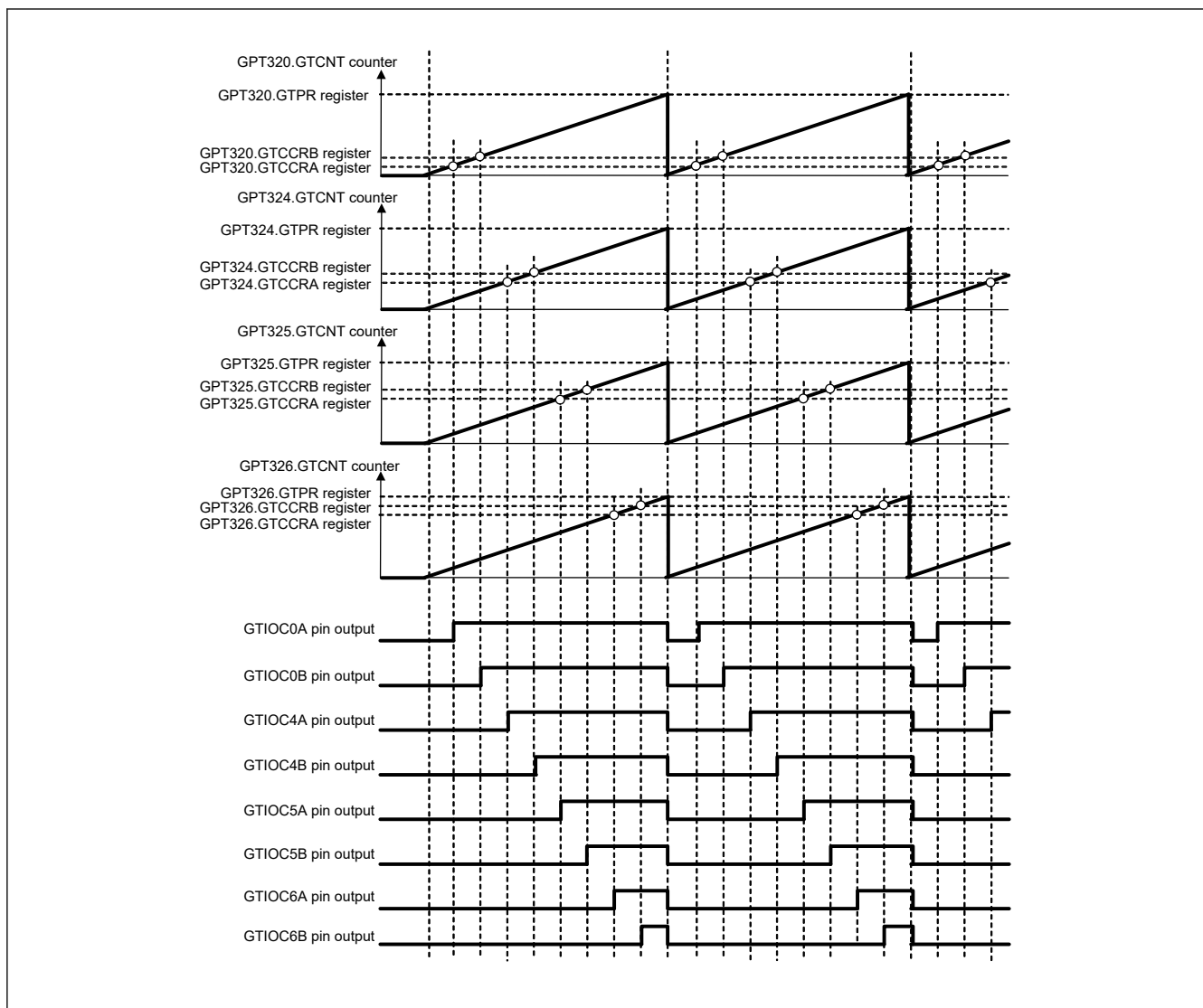
Figure 23.101 Example of synchronized PWM output
