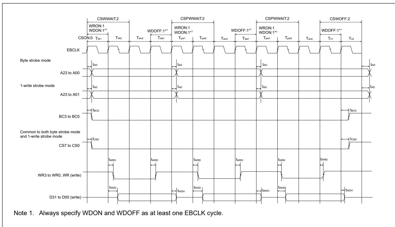
Figure 70.43 External bus timing for page write cycle with bus clock synchronized
