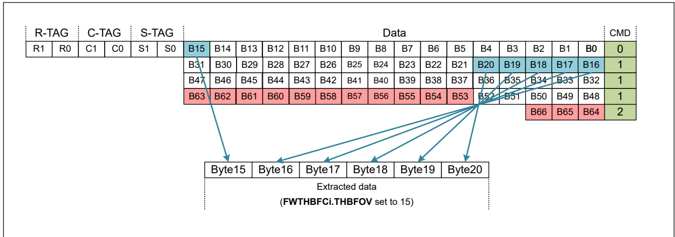
Figure 31.65 3-byte filter data extraction for filtering
