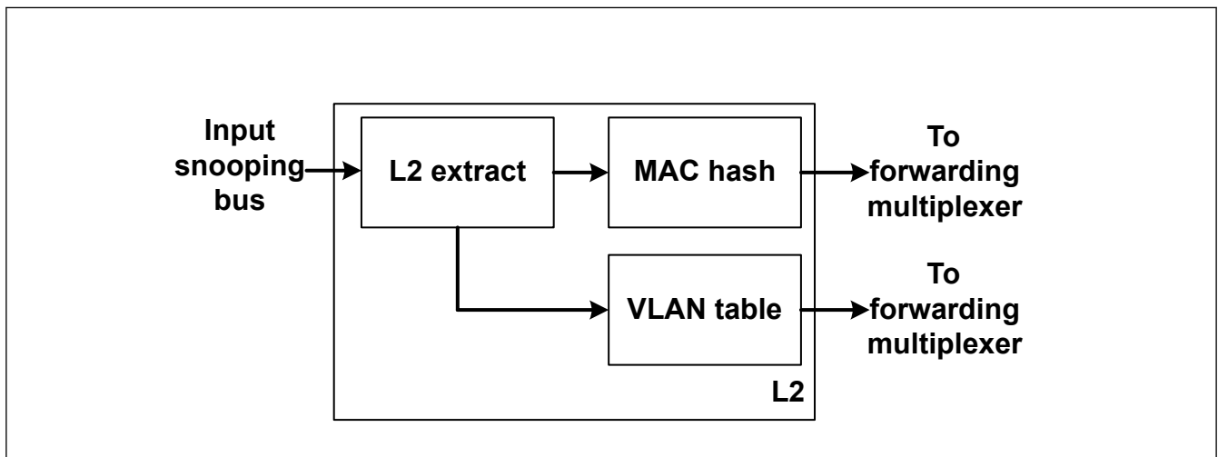
Figure 31.91 Block diagram of Layer 2 forwarding
