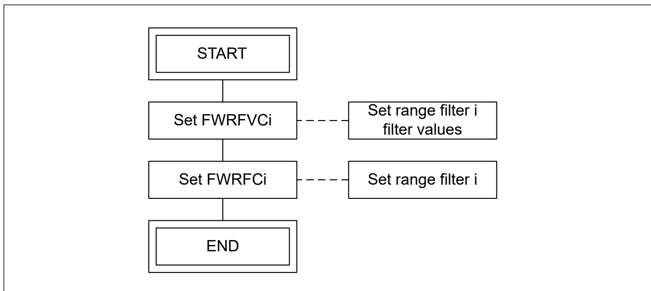
Figure 31.39 Setting flow of range filter i
