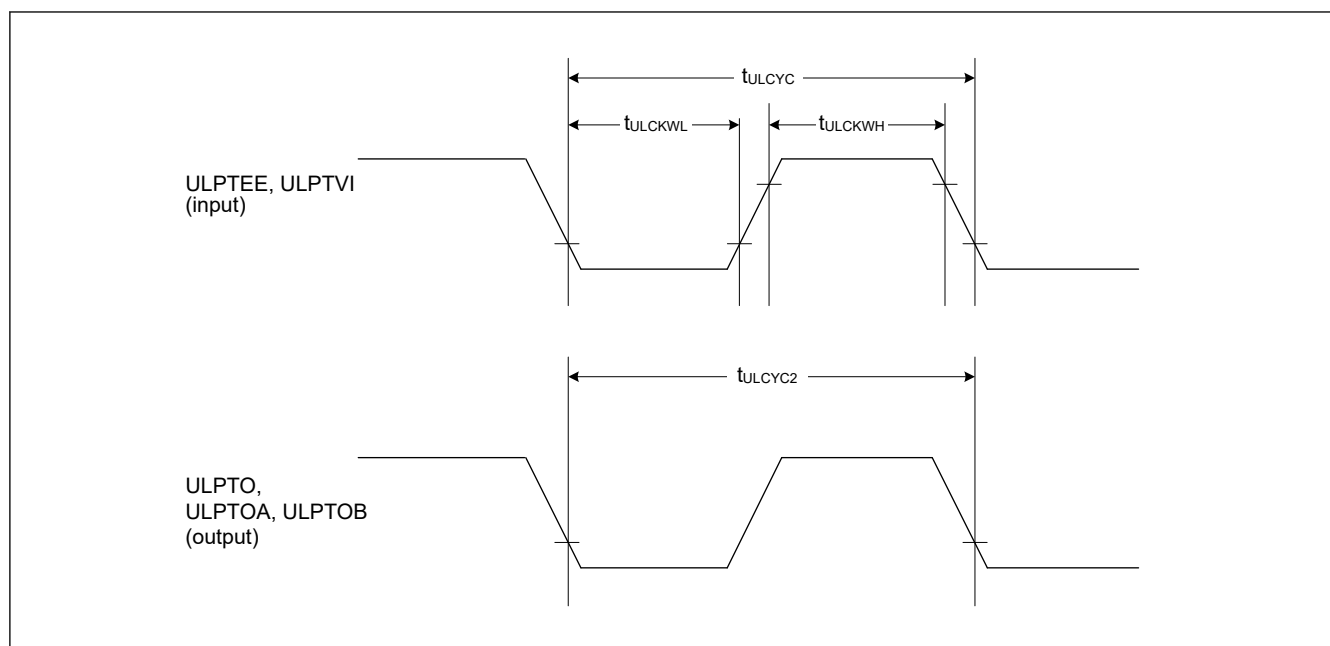
Figure 70.66 ULPT input/output timing
