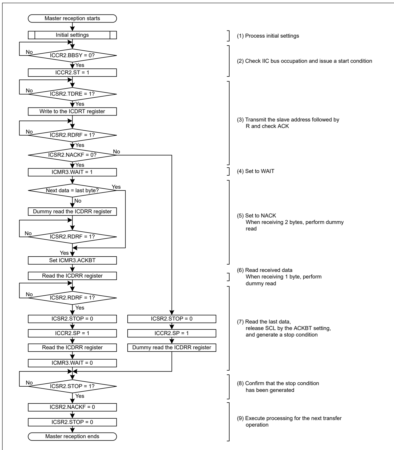
Figure 40.10 Example master reception flow with 7-bit address format of 1 byte or 2 bytes
