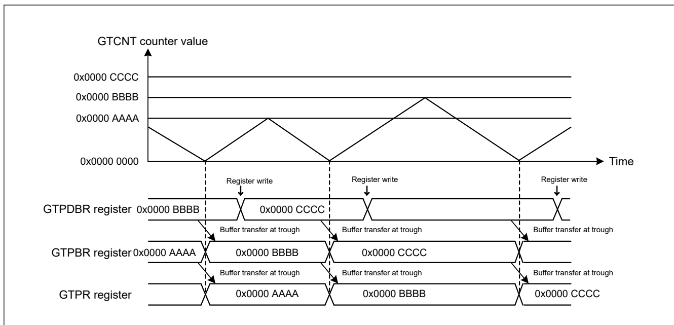
Figure 23.18 Example of GTPR double buffer operation with triangle waves
