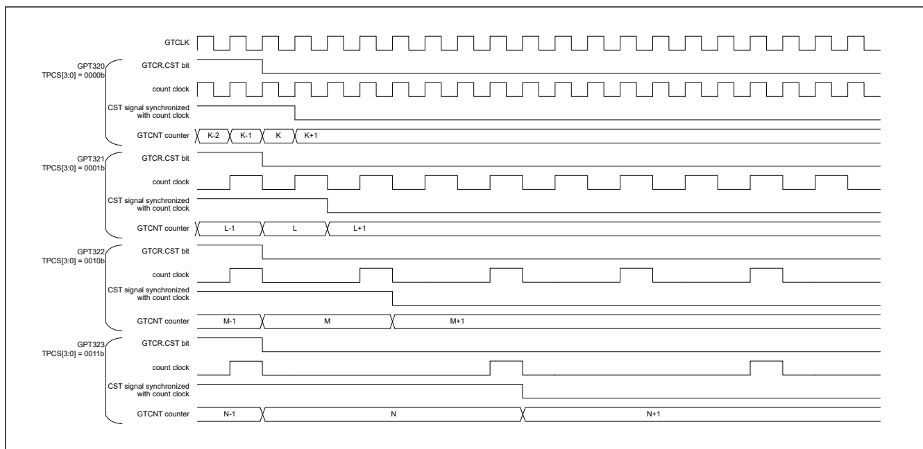
Figure 23.96 Example of Simultaneous Stop Operation by Software (with Different Count Period)
