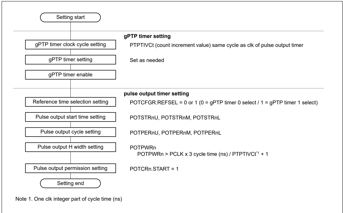
Figure 36.14 Operation setting flow of the pulse output timer
