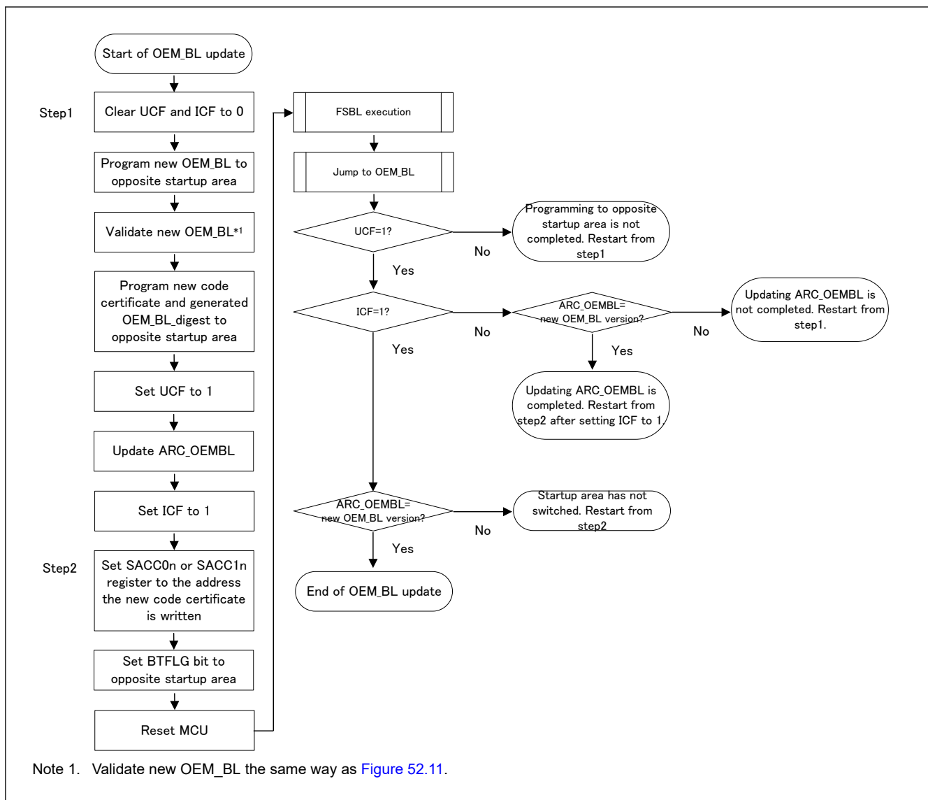
Figure 52.15 OEM_BL update flow
