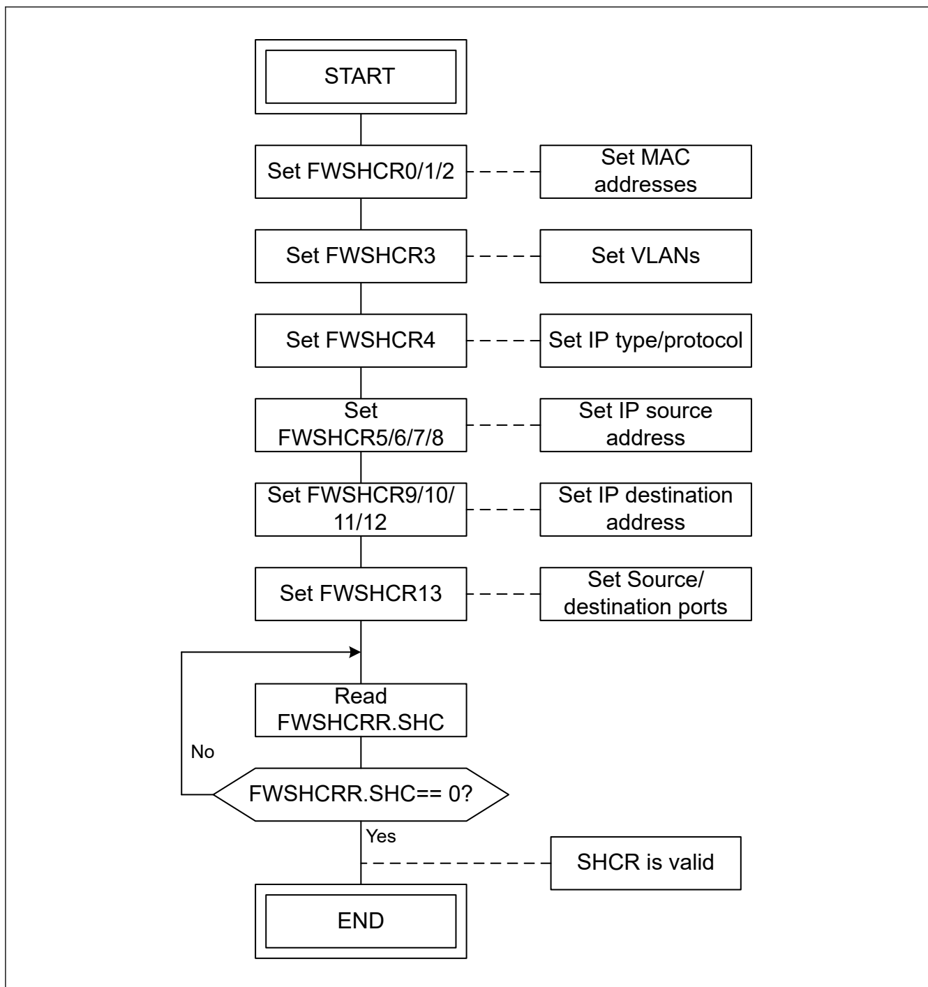
Figure 31.10 Hash hardware calculation flow
