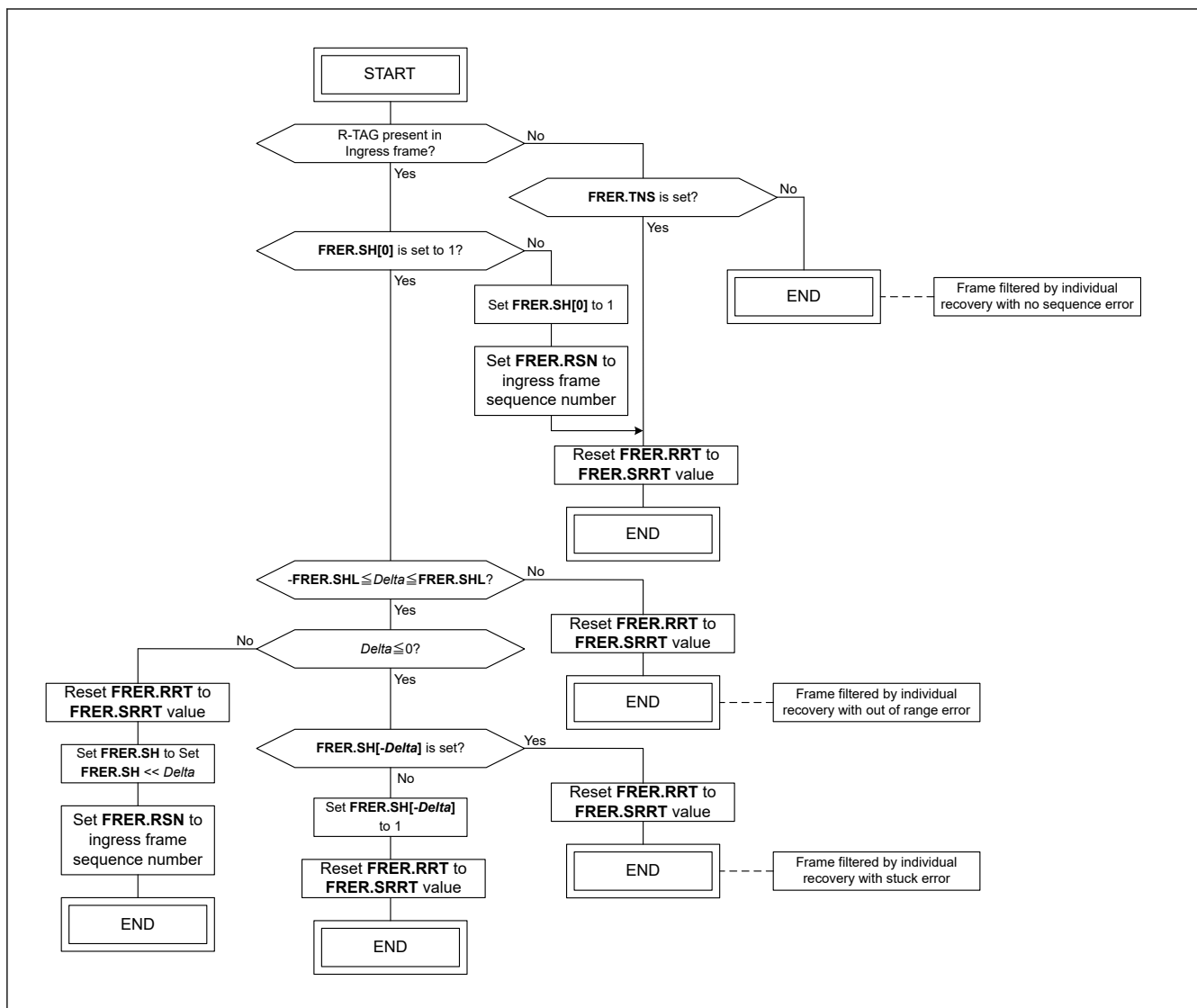
Figure 31.108 Individual recovery vector algorithm
