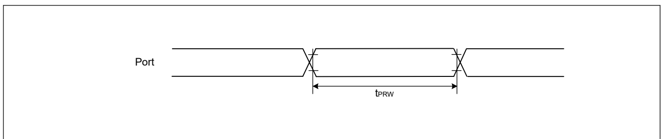
Figure 70.52 I/O ports input timing
