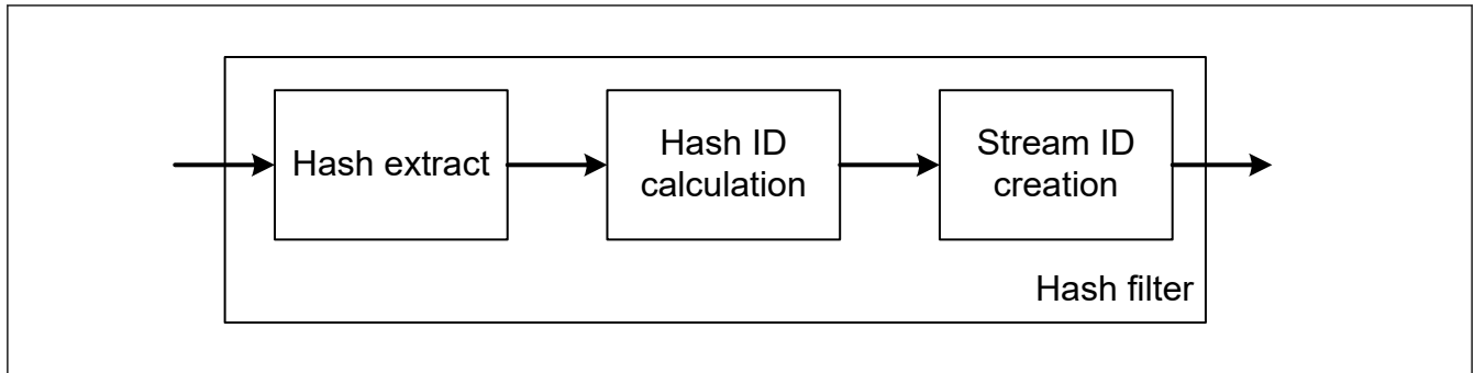
Figure 31.72 Hash filter block diagram
