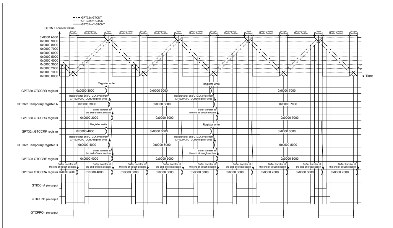
Figure 23.52 Example of Complementary PWM Mode 3 Operation (Double buffer operation, GTIOCnA pin = Low / GTIOCnB pin = High at GTCCRA register compare match during up-counting, GTIOCnA pin = High / GTIOCnB pin = Low at GTCCRA register compare match during down-counting, the dead time value is 0x0000 1000 and updating GTCCRD register in crest and trough sections) (n = 4, 7)
