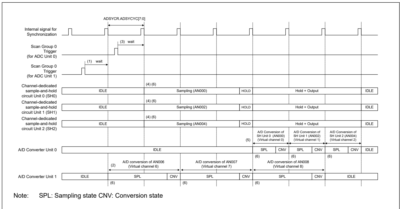
Figure 54.32 Example of synchronous operation using with channel-dedicated sample-and-hold circuit
