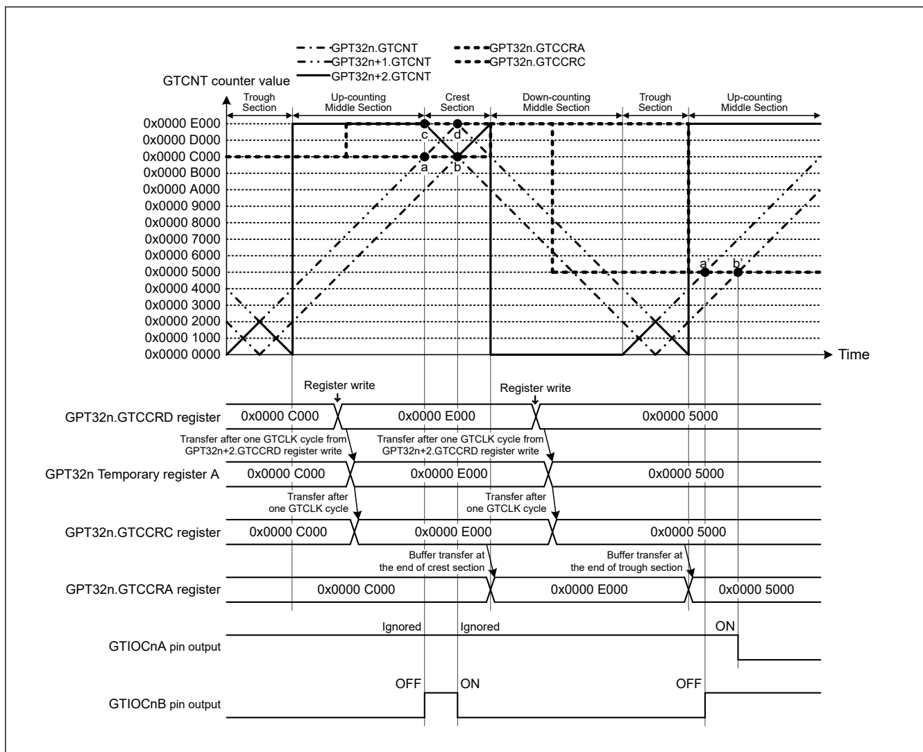
Figure 23.56 Example of Compare Match Generation Sequence Operation in Complementary PWM Mode (Complementary PWM mode 3 single buffer operation, GTIOCnA pin = Low / GTIOCnB pin = High at GTCCRA register compare match during up-counting, GTIOCnA pin = High / GTIOCnB pin = Low at GTCCRA register compare match during down-counting, the dead time value is 0x0000 2000, compare match generation order: (a, c) → (b, d)) (n = 4, 7)
