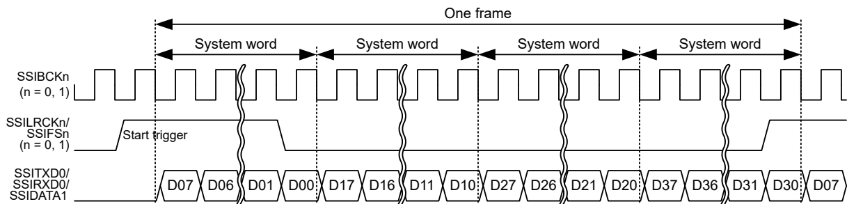
Figure 47.41 TDM format (without padding: system word length = data word length)
