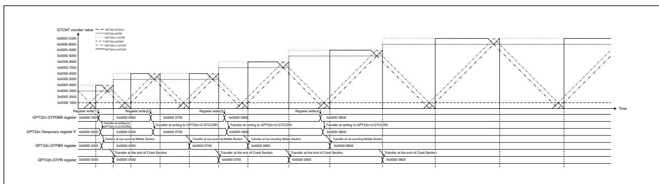
Figure 23.19 Example of GTPR double buffer operation with complementary PWM mode 1
