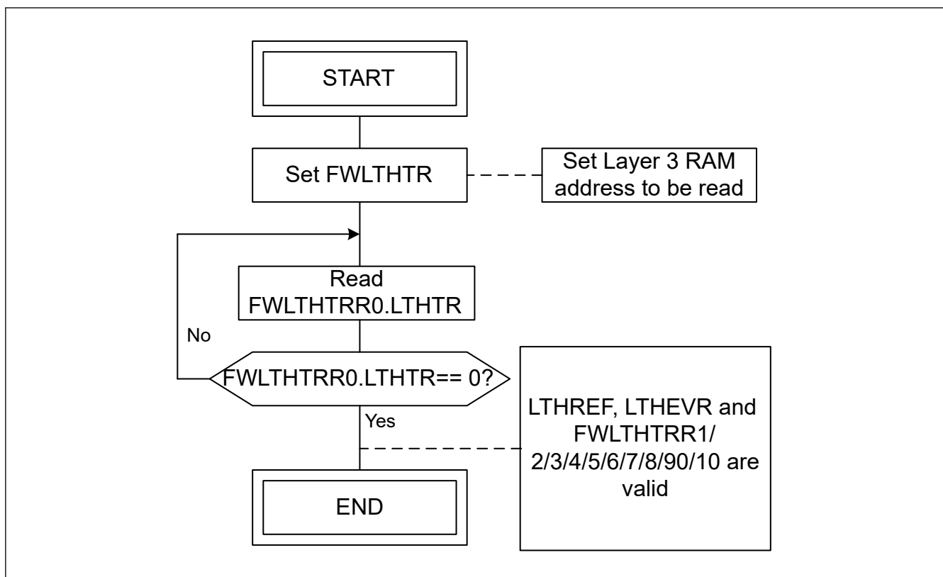
Figure 31.14 Layer 3 entry read flow
