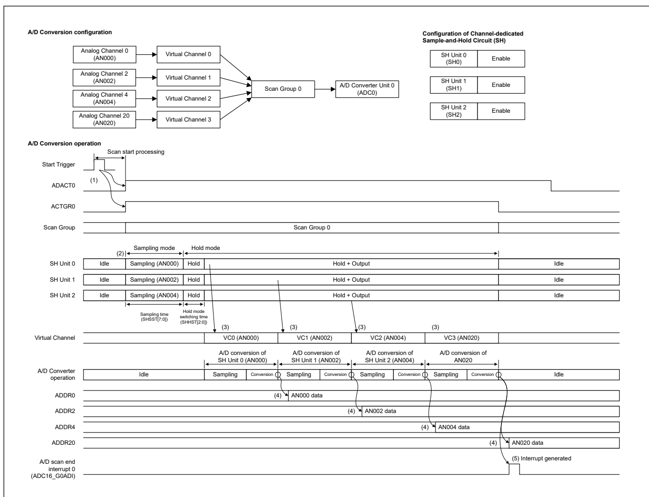
Figure 54.18 Basic operation of channel-dedicated sample-and-hold circuit in SAR mode
