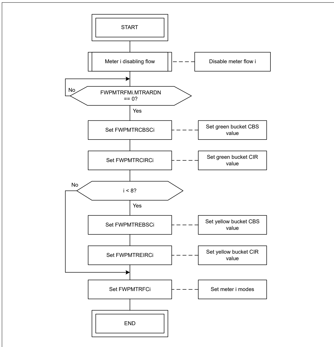
Figure 31.28 Meter i setting flow
