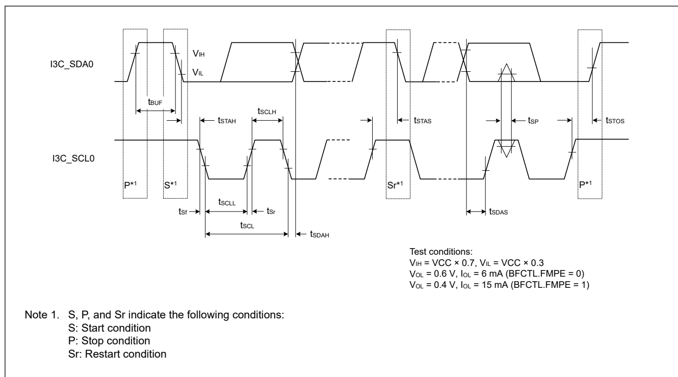
Figure 70.89 I 2 C bus interface input/output timing
