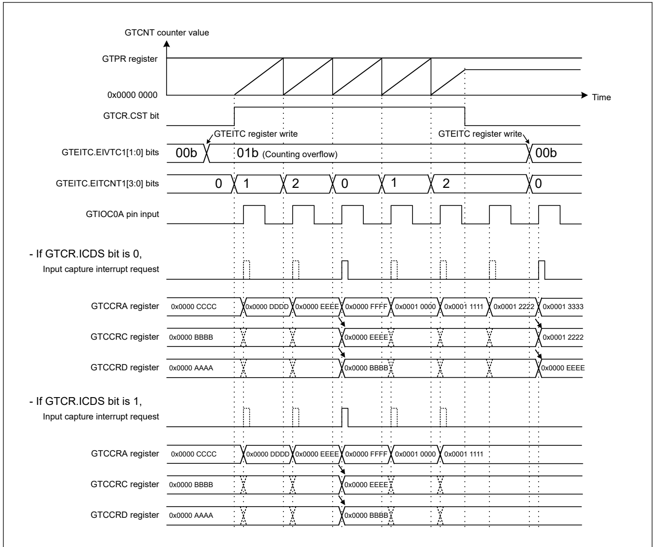
Figure 23.145 Example of Input Capture Operation in the Extended Interrupt Skipping Function Operation (Up-Counting Saw Waves, Counting Overflow, Extended Interrupt Skipping 1 Skipping Count: 2, Skipped in the Period other than the EITCNT1 as 0, Input Capture at the Input Rising)
