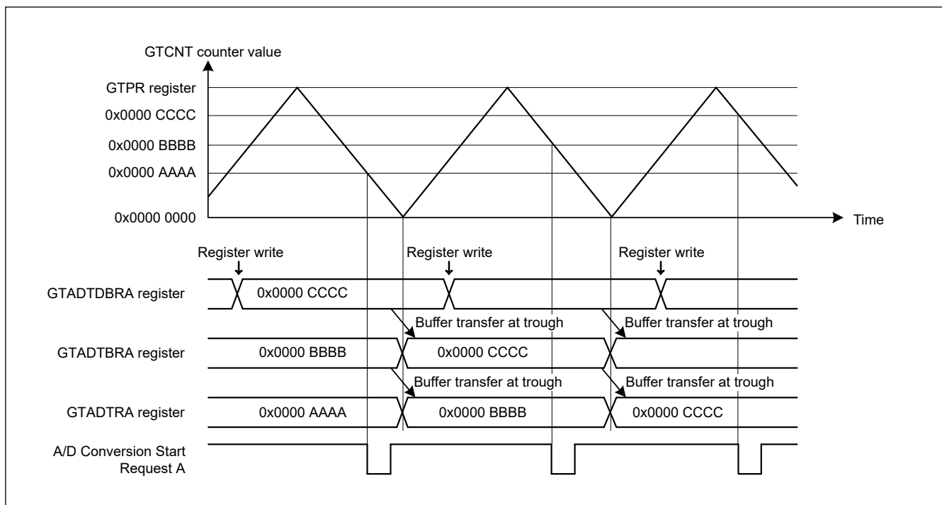
Figure 23.30 Example of Double Buffer Operation of the GTADTRA and GTADTRB Registers (Triangle Waves, Buffer Transfer at Troughs, A/D Conversion Start Request Generated by Down-Counting)
