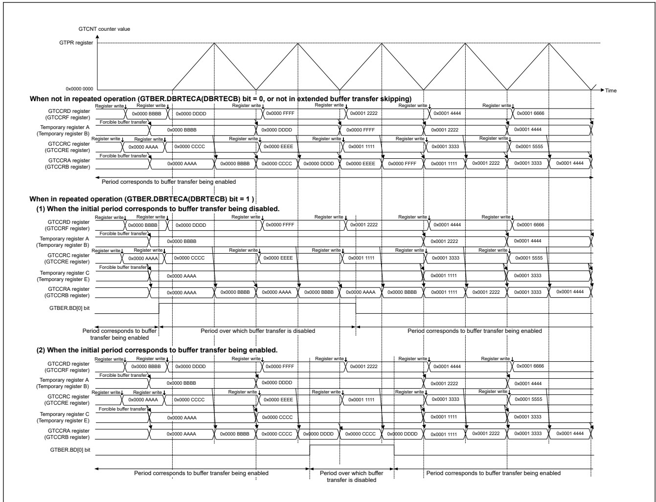
Figure 23.159 Example of Repeated Double-Buffer Operation When GTCCR Buffer Transfer is Disabled (Triangle-Wave PWM Mode 3, Updating the GTBER.BD[0] Bit)
