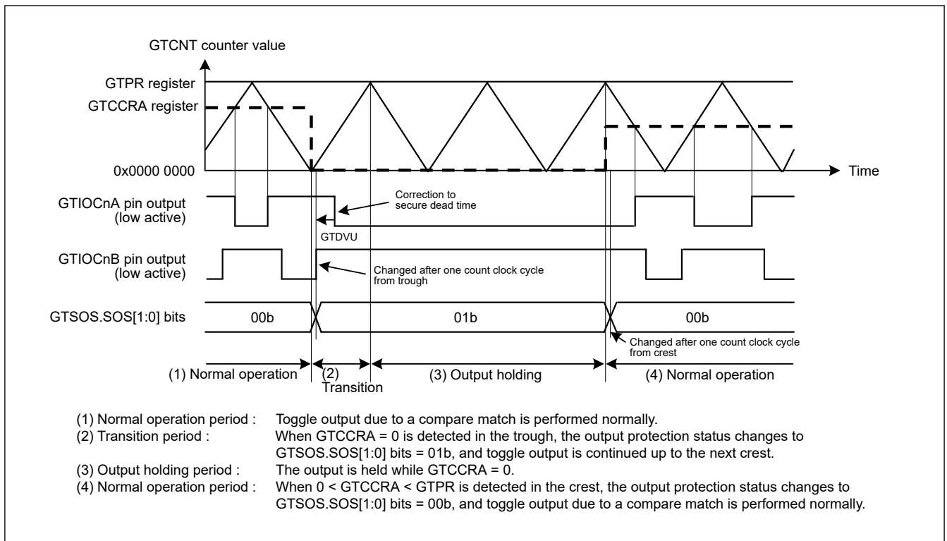
Figure 23.163 Example of Output Protection Function Operation When GTCCRA is Set to 0x0000 0000 during Buffer Transfer at Troughs (Restored to 0 < GTCCRA < GTPR during Buffer Transfer at Crests, Active Level: Low) (n = 0 to 13)
