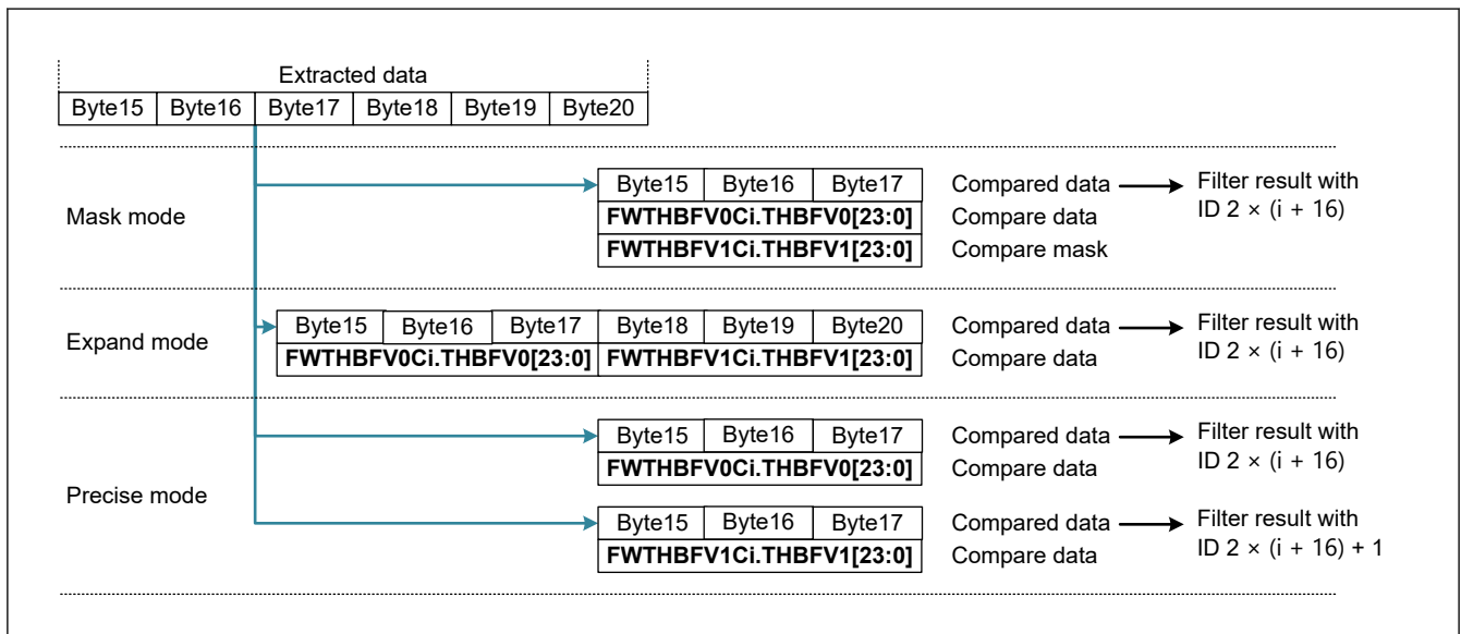
Figure 31.66 3-byte filter data extraction for filtering
