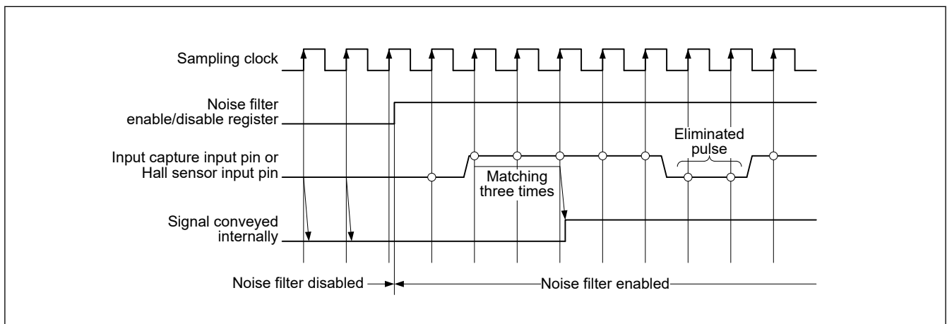
Figure 23.152 Timing of noise filtering
