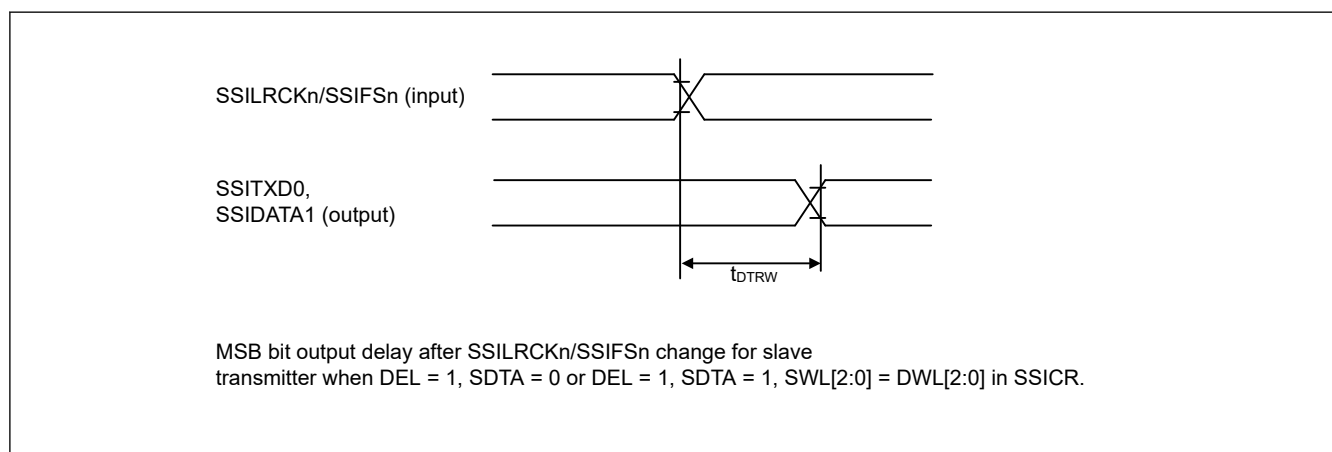
Figure 70.106 SSIE data output delay after SSILRCK0/SSIFS0 change
