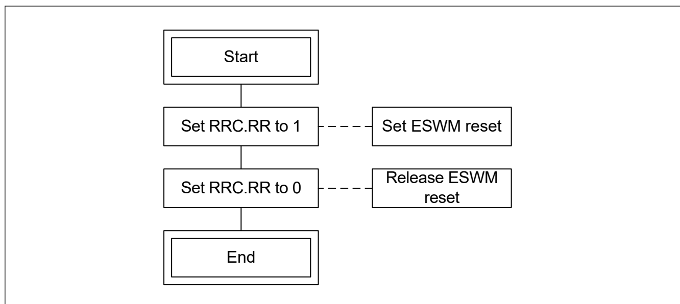
Figure 32.5 ESWM reset flow
