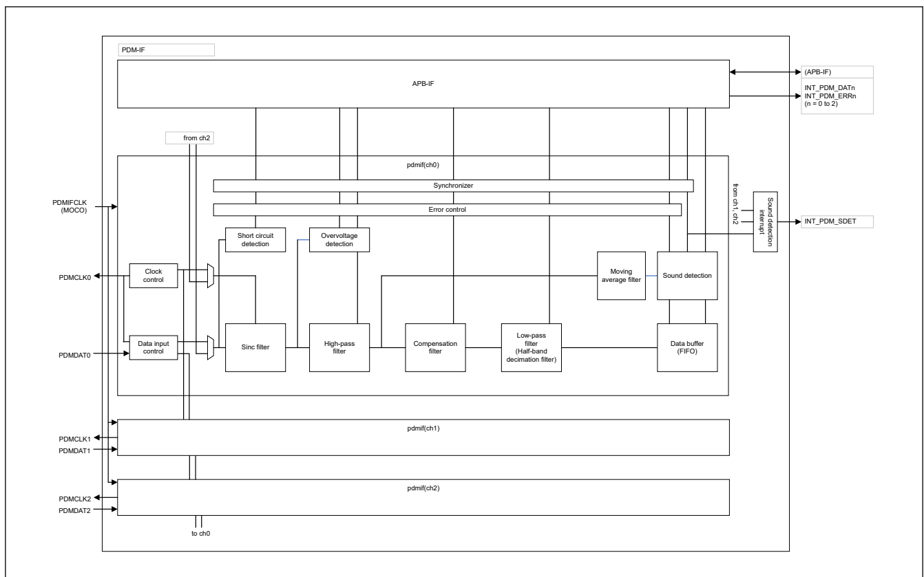
Figure 50.1 PDM-IF block diagram
