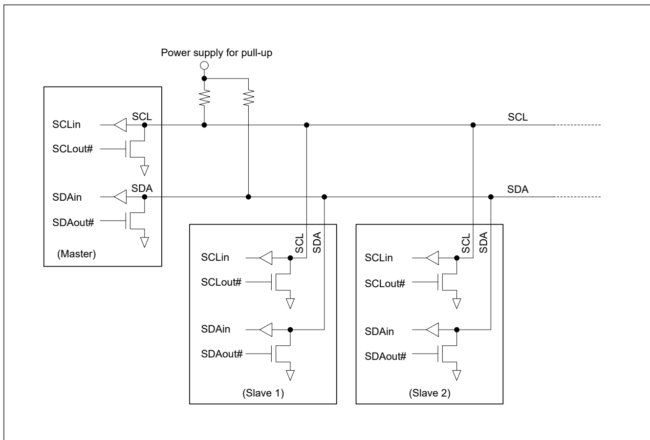
Figure 40.2 I/O pin connection to an external circuit (I 2 C bus configuration example)
