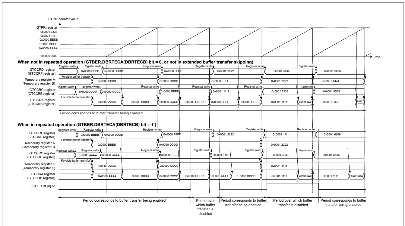
Figure 23.157 Example of Repeated Double-Buffer Operation When GTCCR Buffer Transfer is Disabled (Saw-Wave One-Shot Pulse Mode, Updating the GTBER.BD[0] Bit)
