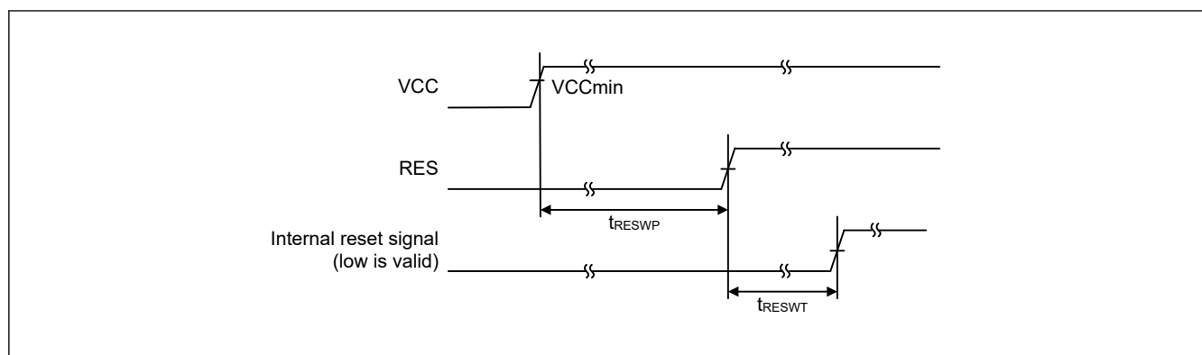
Figure 70.32 RES pin input timing under the condition that VCC exceeds V_{POR} voltage threshold
