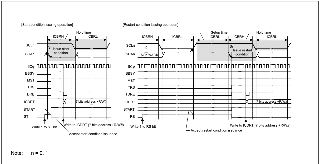
Figure 40.45 Start and restart condition issue timing using the ST and RS bits
