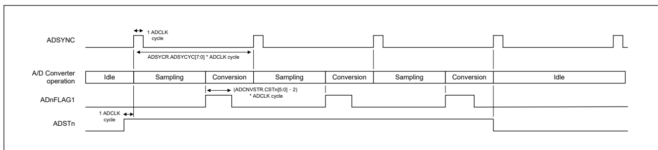
Figure 54.33 A/D conversion monitor signals
