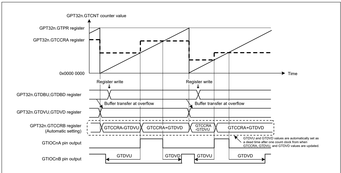
Figure 23.77 Example of automatic dead time setting function operation in saw-wave one-shot pulse mode, up-counting, GTDVU and GTDVD set to buffer operation, and active-high
