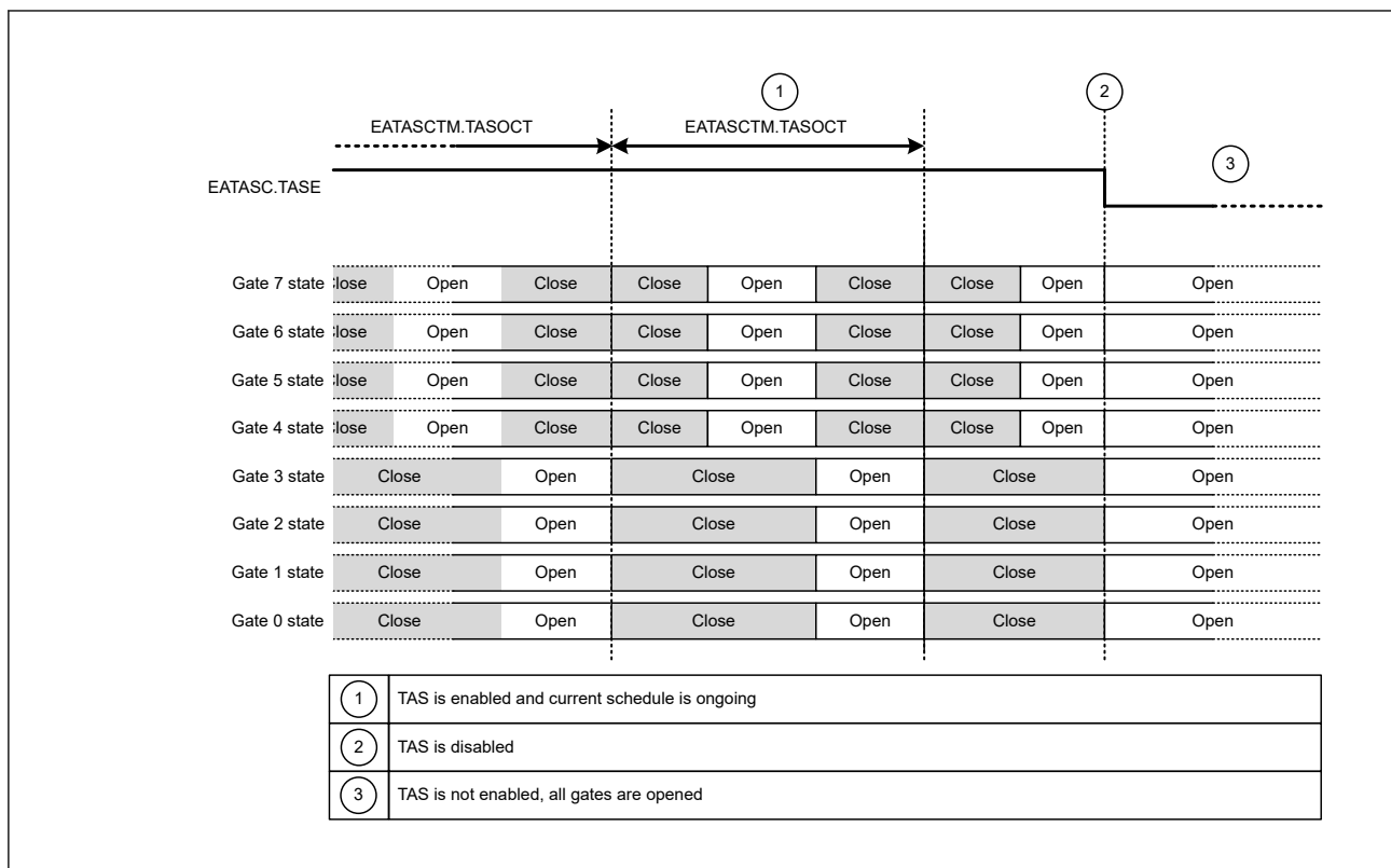
Figure 33.23 TAS behavior when its schedule is disabled
