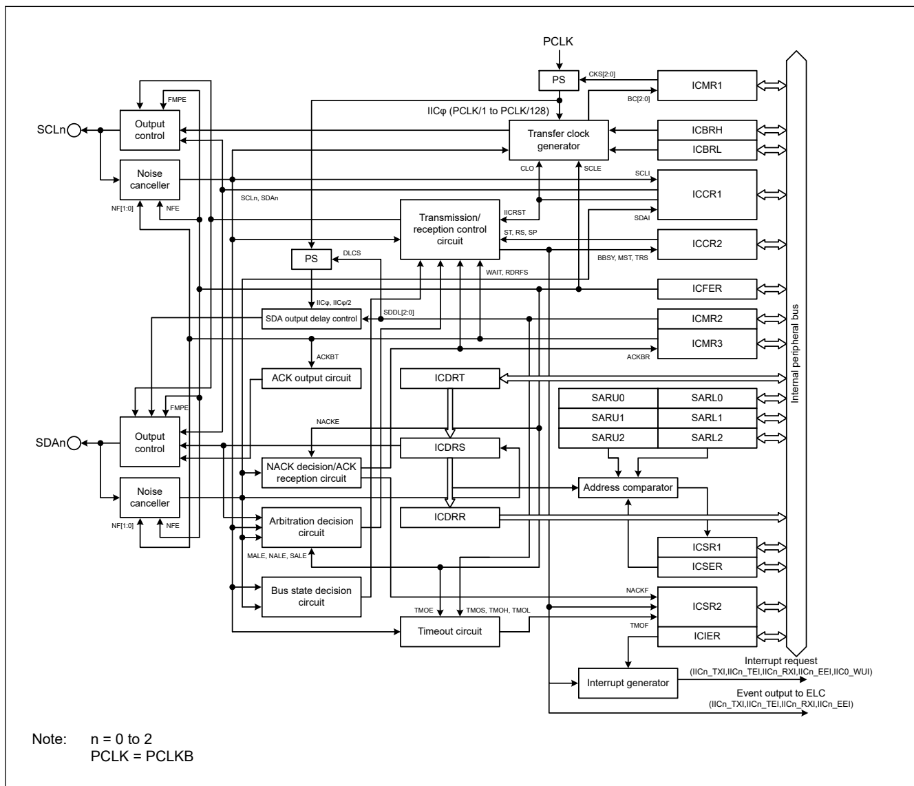
Figure 40.1 IIC block diagram
