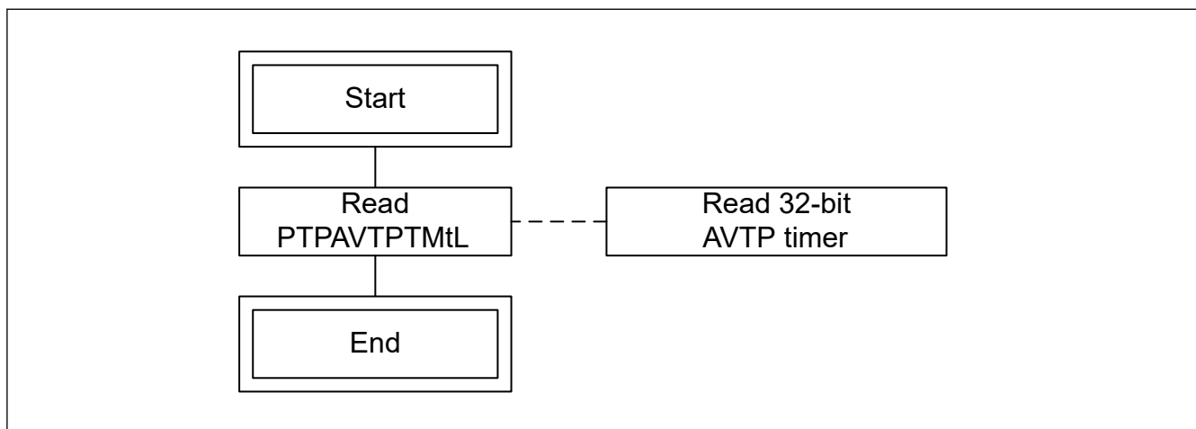
Figure 36.5 32-bit AVTP timer t reading flow
