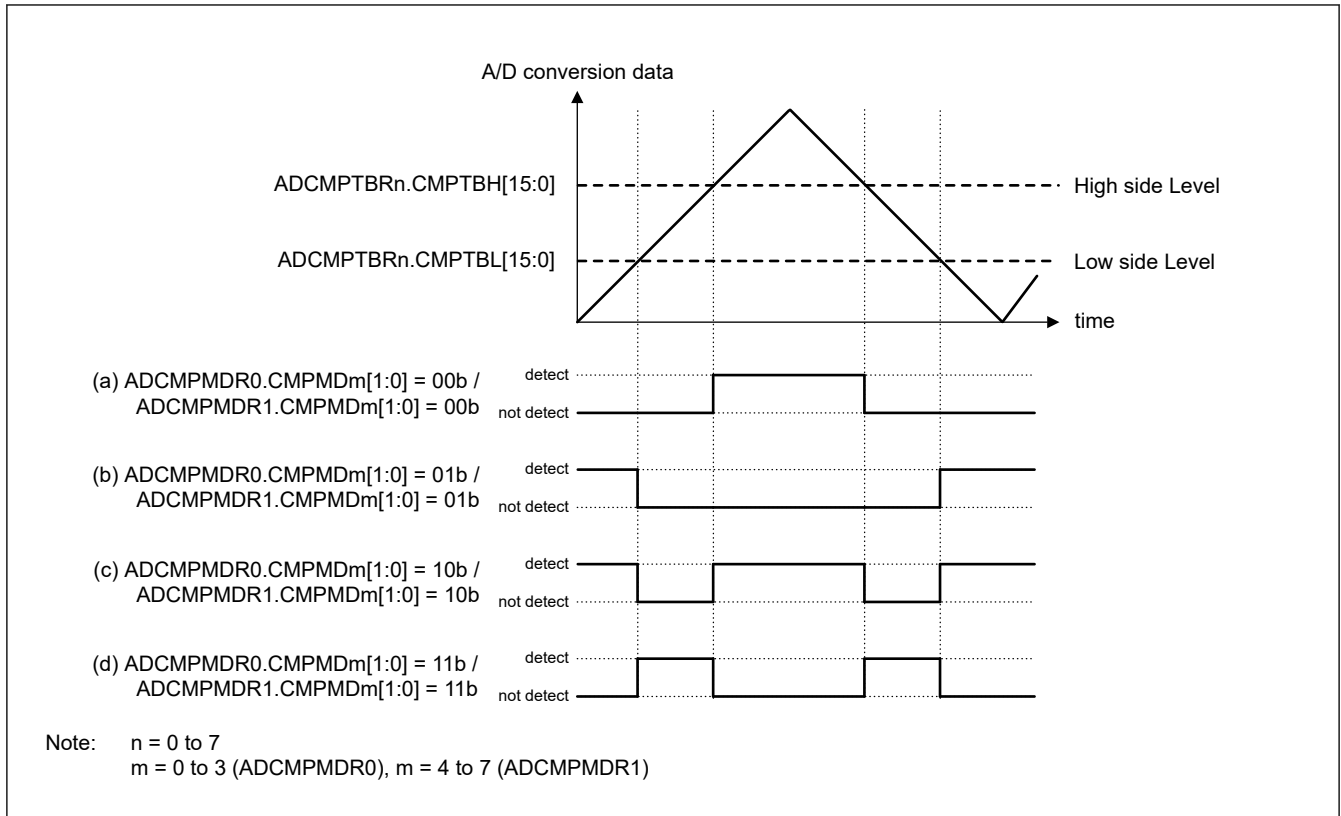
Figure 54.51 Compare match detection
