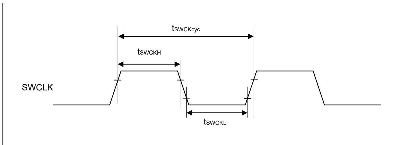
Figure 70.157 SWD SWCLK timing
