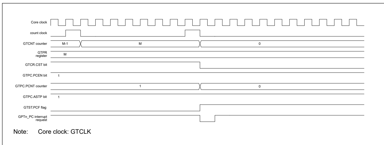
Figure 23.108 Example of the timing of operations for PWM cycle count function (saw-wave one-shot pulse mode, up-counting)
