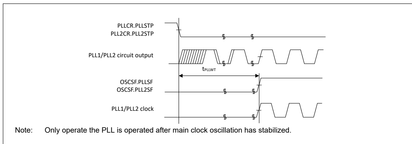
Figure 70.29 PLL1/PLL2 clock oscillation start timing
