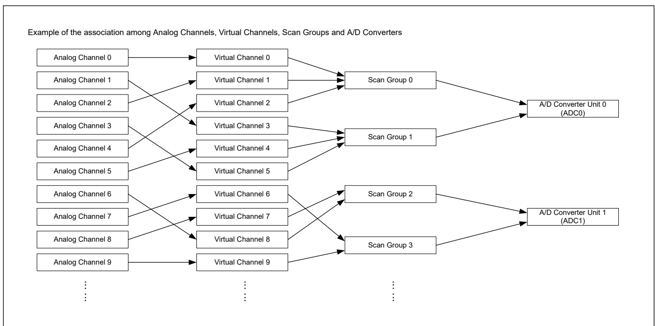
Figure 54.5 The concept of virtual channel
