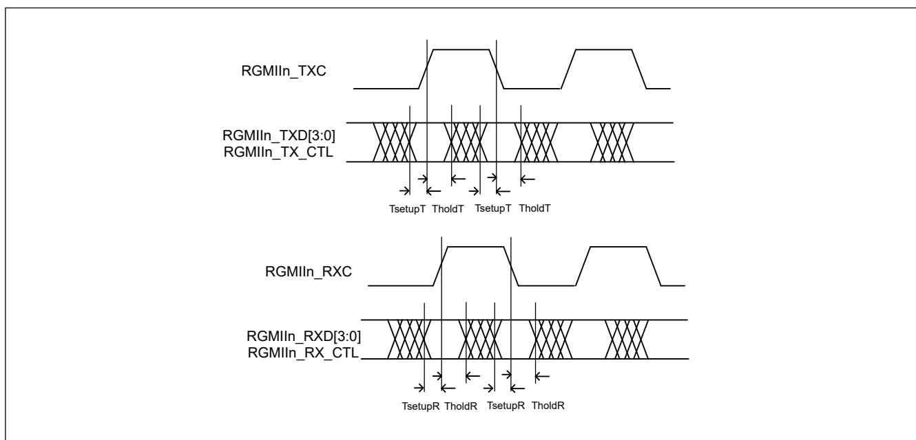
Figure 70.121 RGMII timing (RGMII-ID)
