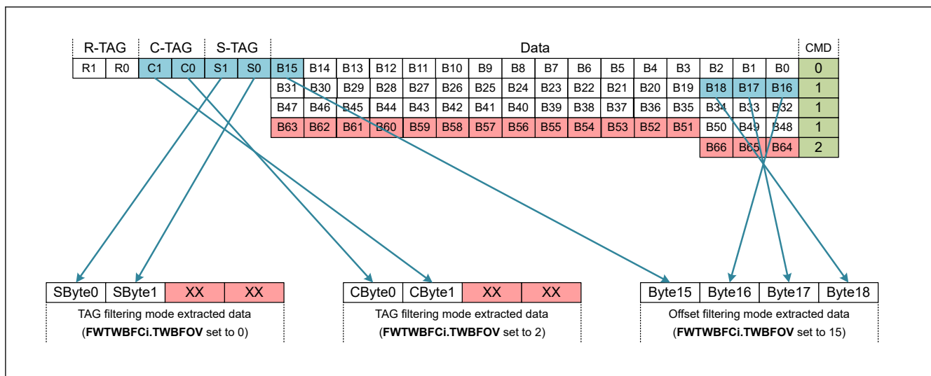
Figure 31.63 2-byte filter data extraction for filtering
