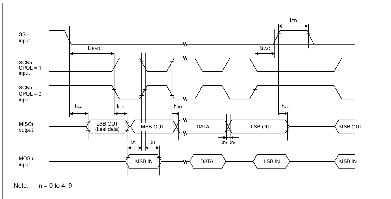
Figure 70.73 SCI simple SPI mode timing for slave when CPHA = 1
