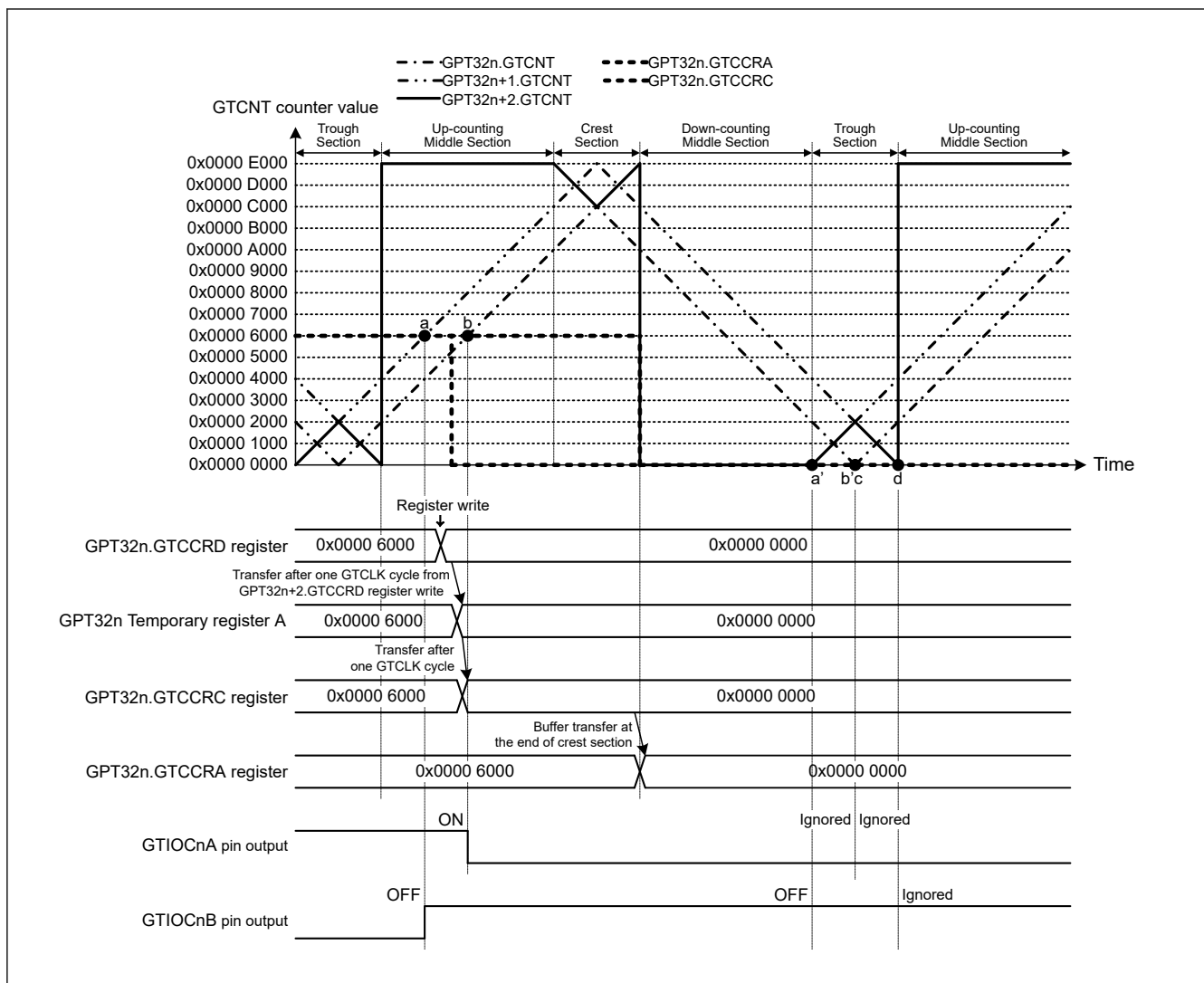
Figure 23.64 Example of Compare Match Generation Sequence Operation in Complementary PWM Mode (Complementary PWM mode 3 single buffer operation, GTIOCnA pin = Low / GTIOCnB pin = High at GTCCRA register compare match during up-counting, GTIOCnA pin = High / GTIOCnB pin = Low at GTCCRA register compare match during down-counting, the dead time value is 0x0000 2000, compare match generation order: a' → (b', c) → d) (n = 4, 7)
