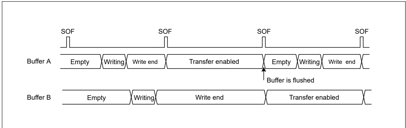
Figure 38.17 Example buffer flush operation
