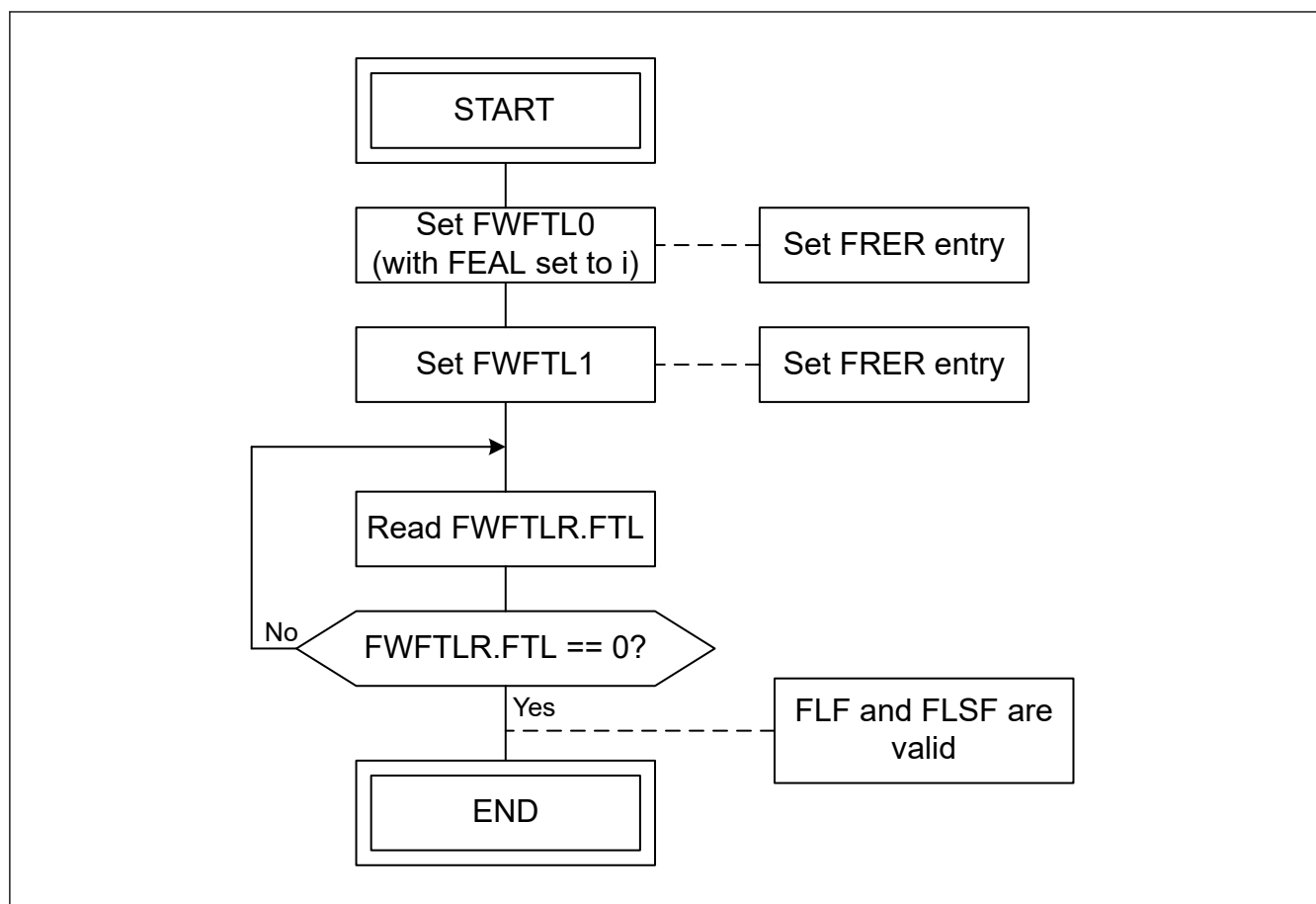
Figure 31.31 Learn flow of FRER entry i
