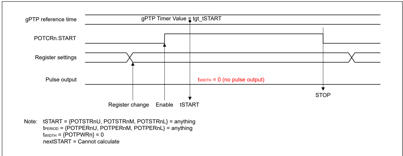
Figure 36.18 When changing the POTCRn.START bit from 0 to 1 with pulse output H width register = 0
