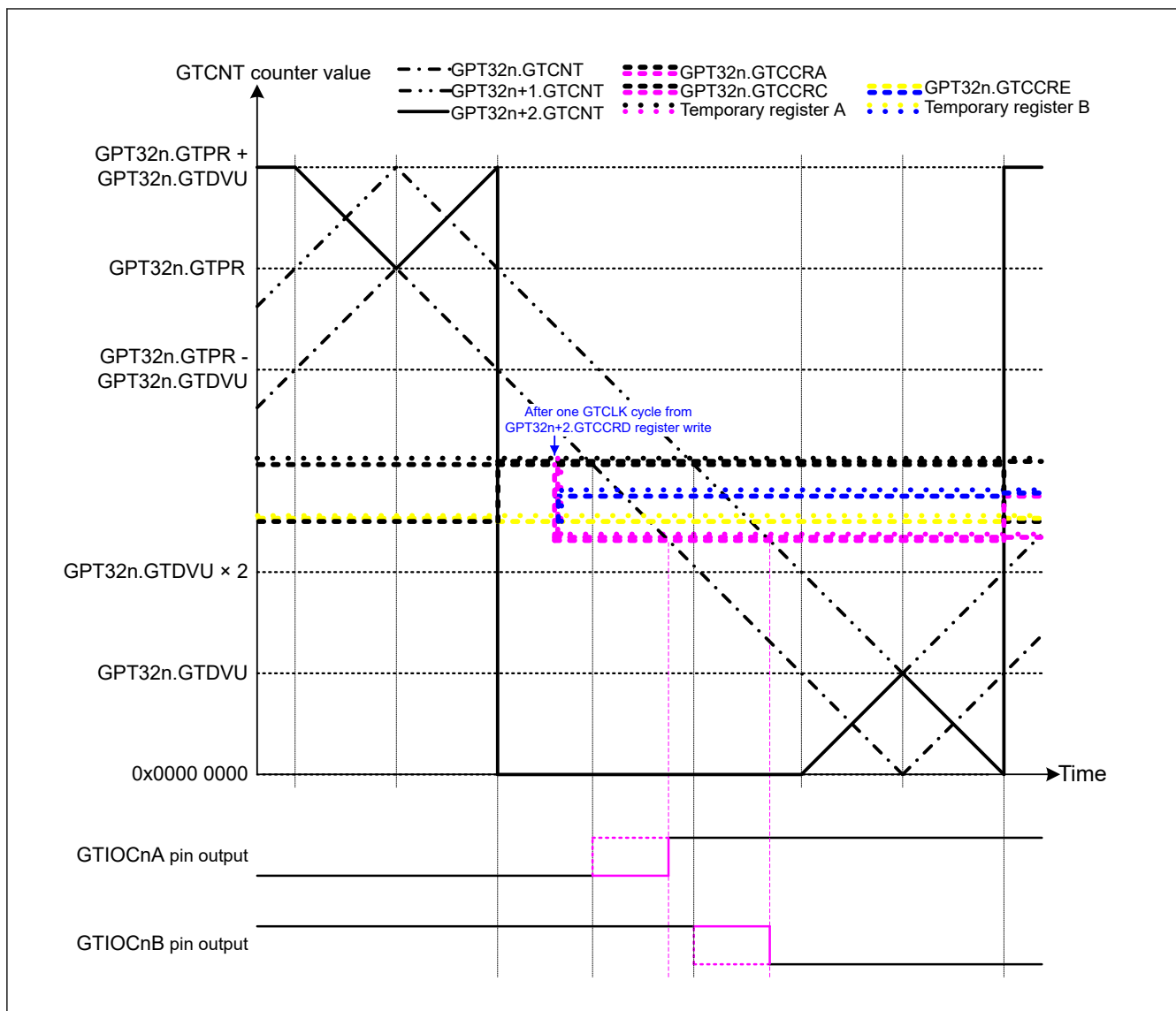
Figure 23.75 Example of Complementary PWM Mode 4 Double Buffer Operation (Down-Counting Middle Section) (Complementary PWM mode 4 double buffer operation, GTIOcNA pin = Low / GTIOcNB pin = High at GTCCRA register compare match during up-counting, GTIOcNA pin = High / GTIOcNB pin = Low at GTCCRA register compare match during down-counting, when a value smaller than the GPT32n.GTCNT value is written to GTCCRD register before down-counting compare match) (n = 4, 7)
