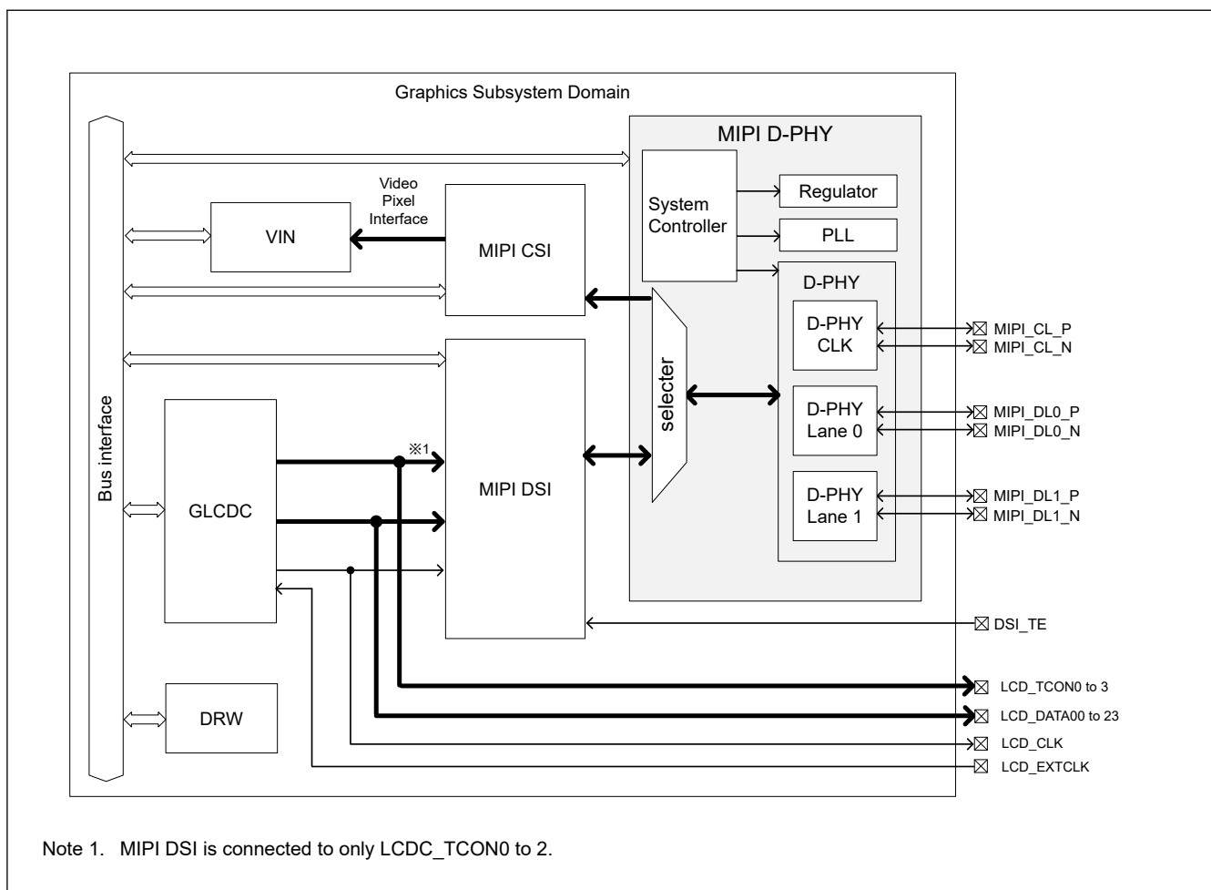
Figure 62.1 Graphics domain block diagram
