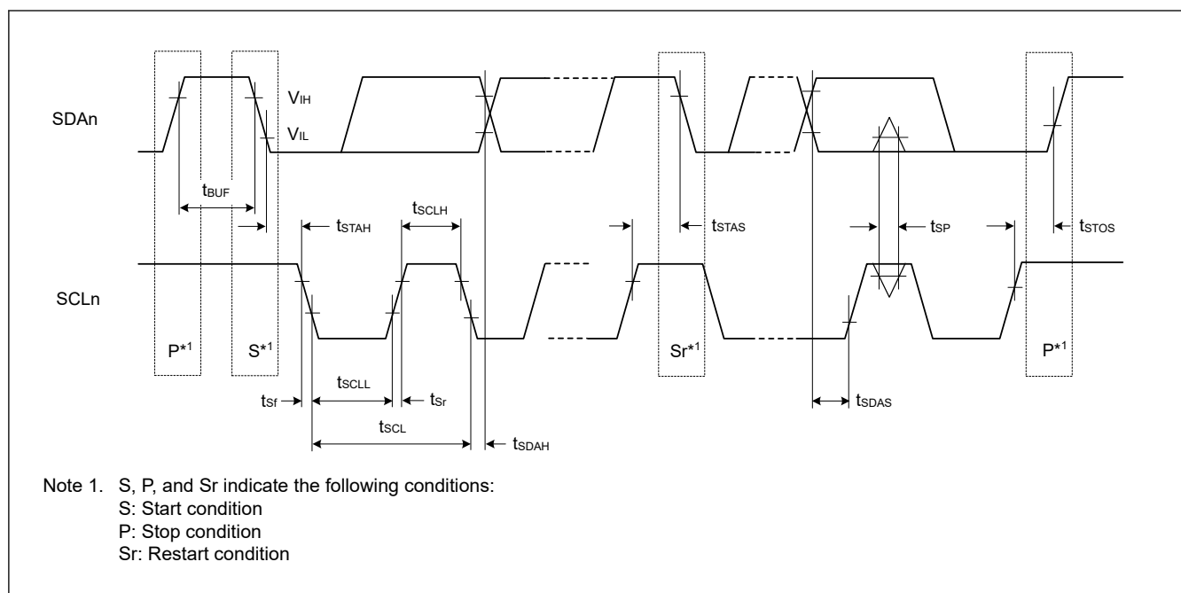
Figure 70.88 I 2 C bus interface input/output timing
