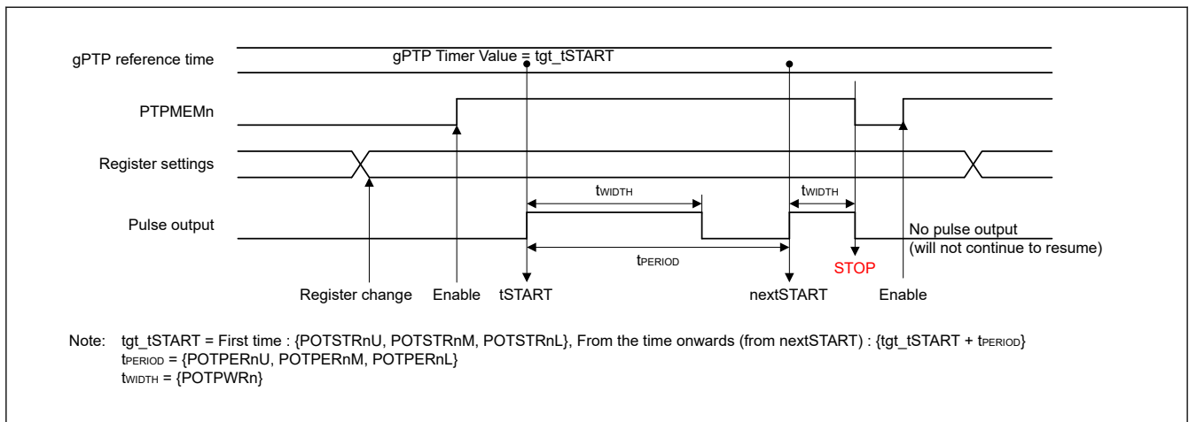
Figure 36.19 When the pulse output is stopped with the POTCRn.START bit set to 0
