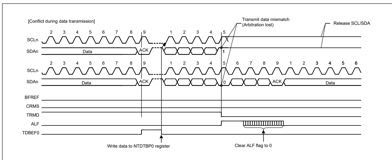
Figure 41.92 Example of slave arbitration-lost detection (SALE = 1)
