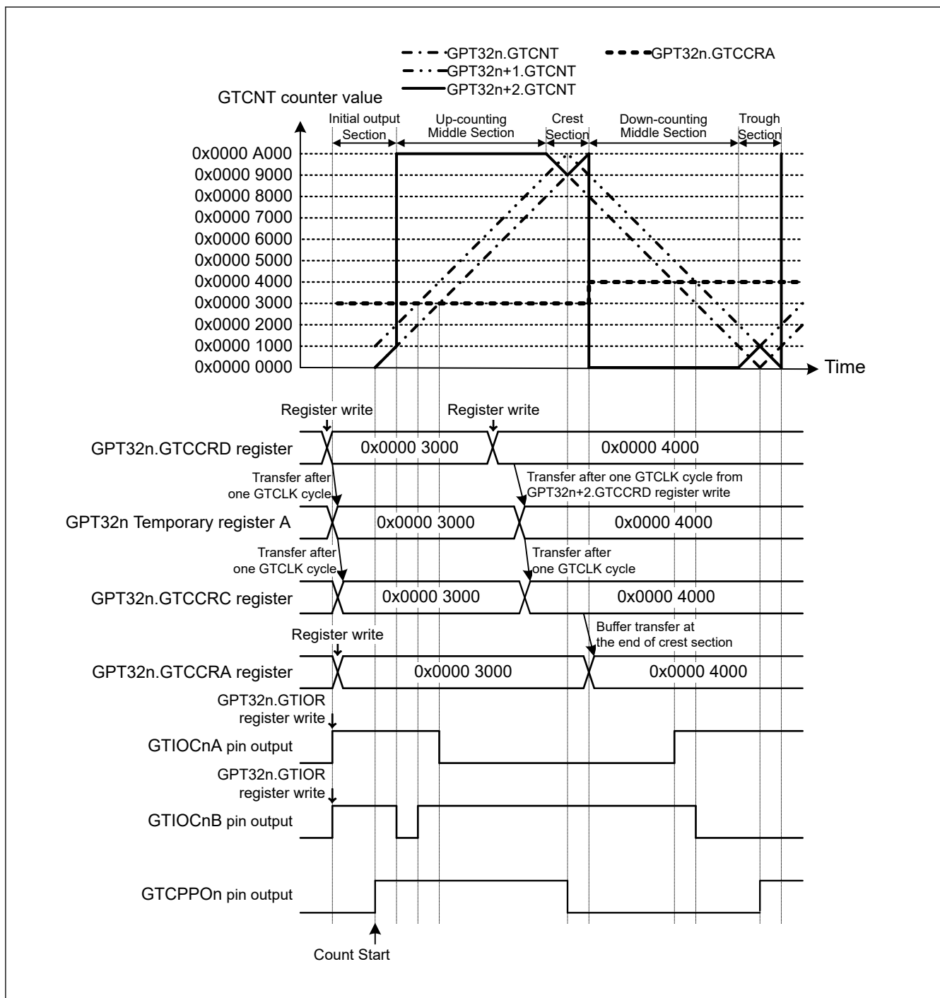
Figure 23.65 Example of Complementary PWM Mode Initial Output Operation (Complementary PWM mode 1 operation, GTIOCA pin = Low / GTIOCB pin = High at GTCCRA register compare match during up-counting, GTIOCA pin = High / GTIOCB pin = Low at GTCCRA register compare match during down-counting, the dead time value is 0x0000 1000, in the case that the initial GTCCRA register value is larger than the dead time value) (n = 4, 7)
