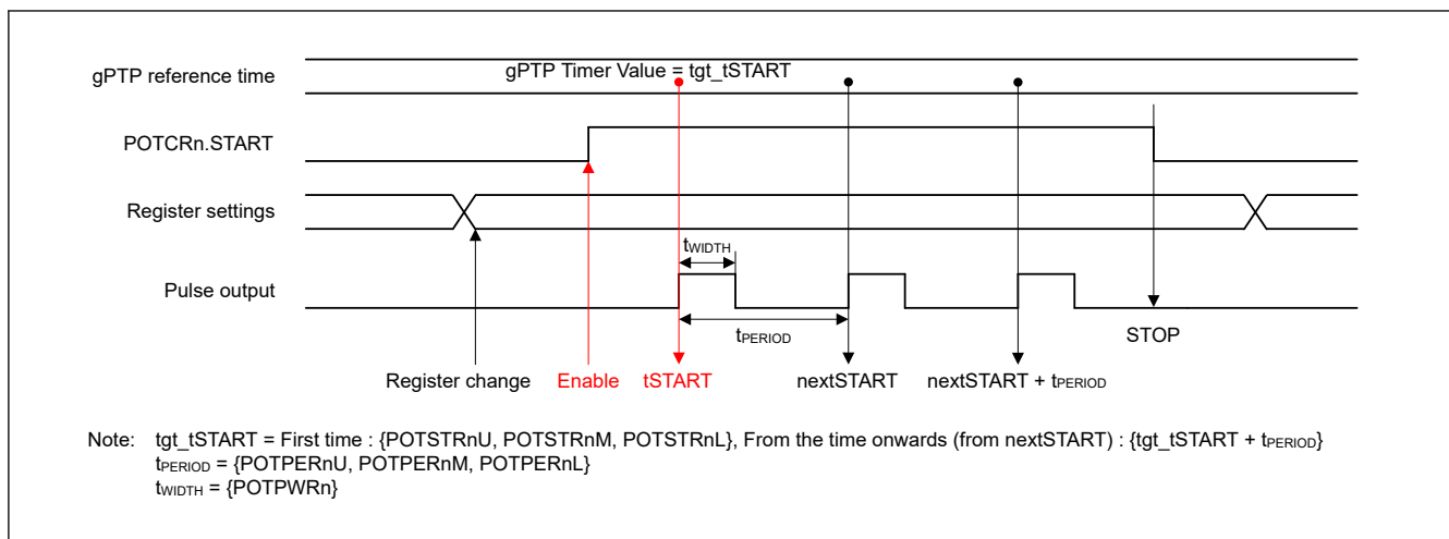
Figure 36.15 When changing the POTCRn.START bit from 0 to 1 after setting the register and before the start time
