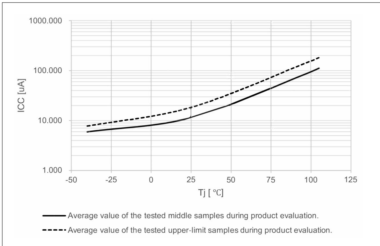
Figure 70.7 Temperature dependency in Deep Software Standby mode 1 (reference data)
