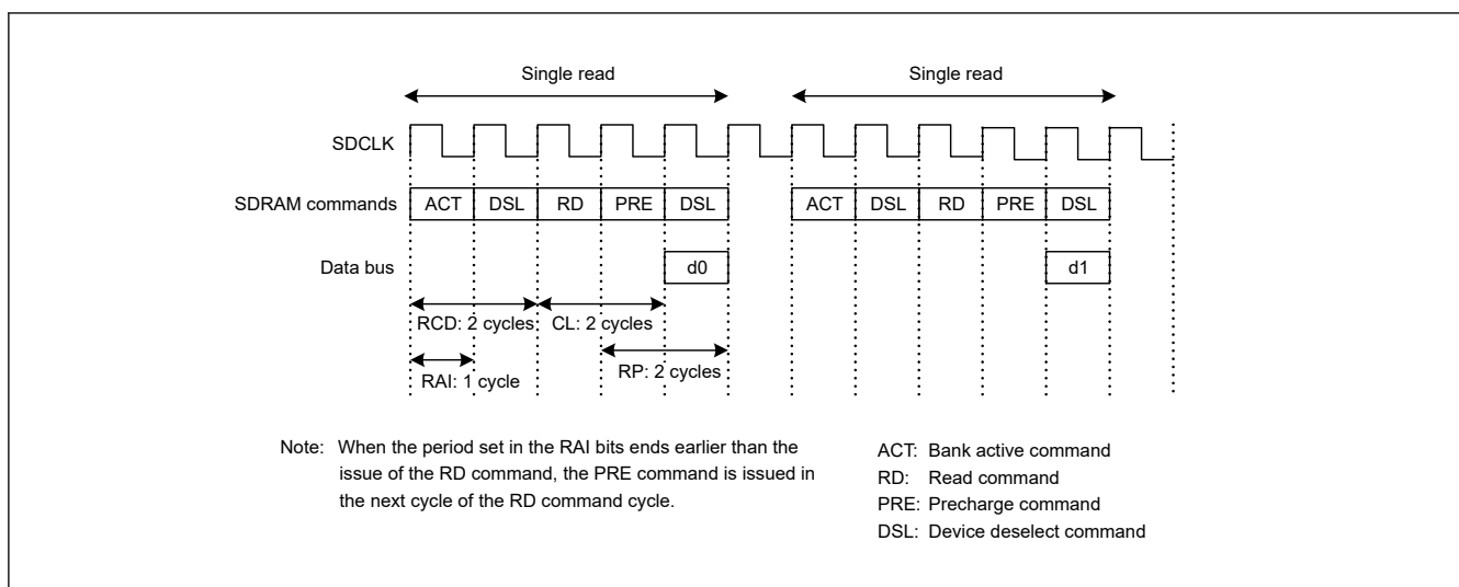
Figure 15.52 Example timing for single read (2)
