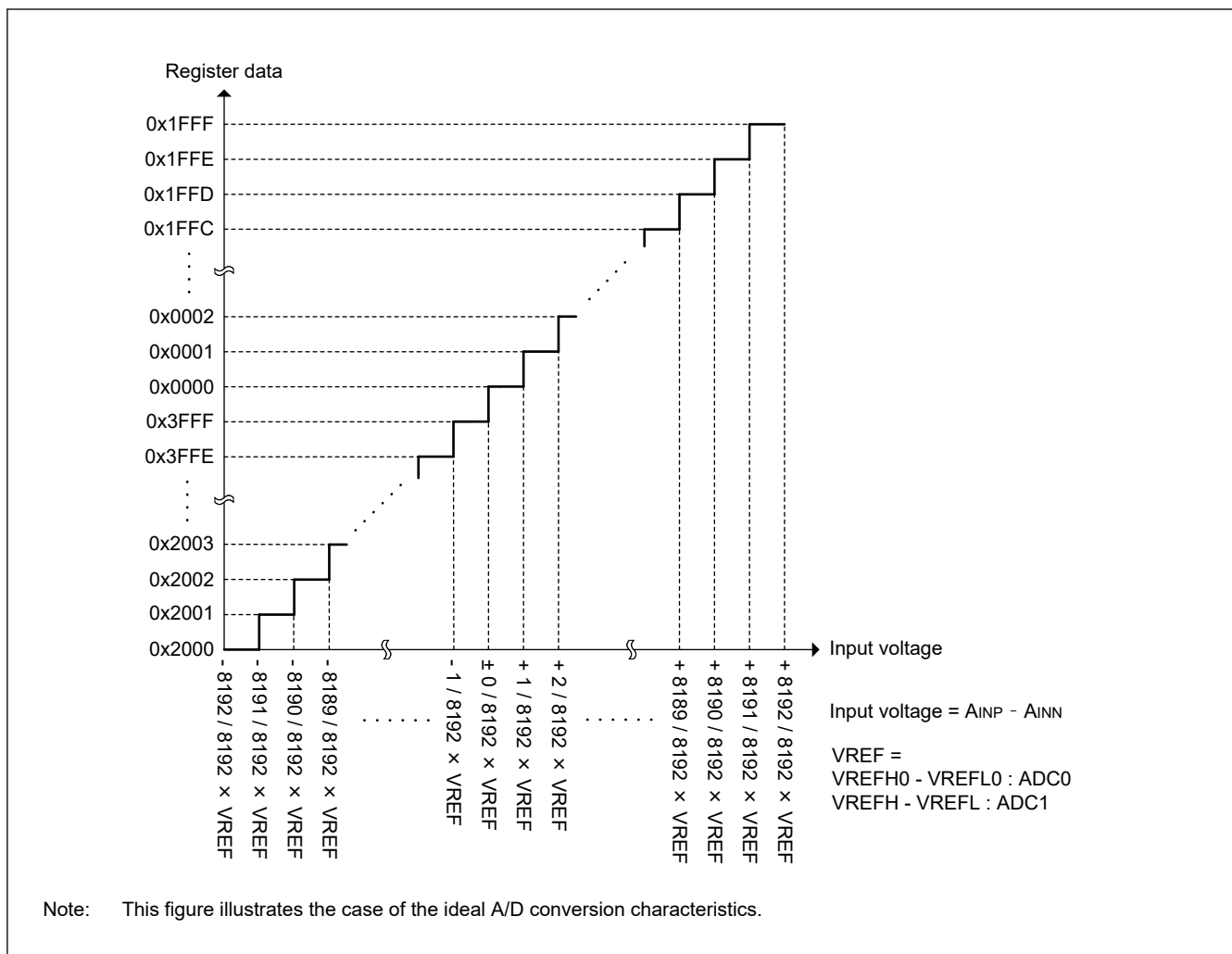
Figure 54.45 Data range of A/D conversion result (14-bit data length, Signed data, Differential input)
