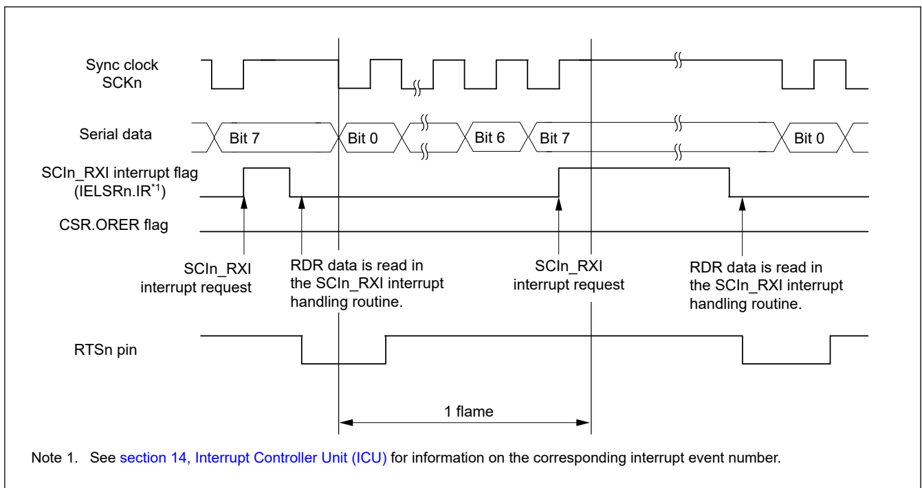
Figure 39.68 Example operation for serial reception in clock synchronous mode (2) when RTS function is used
