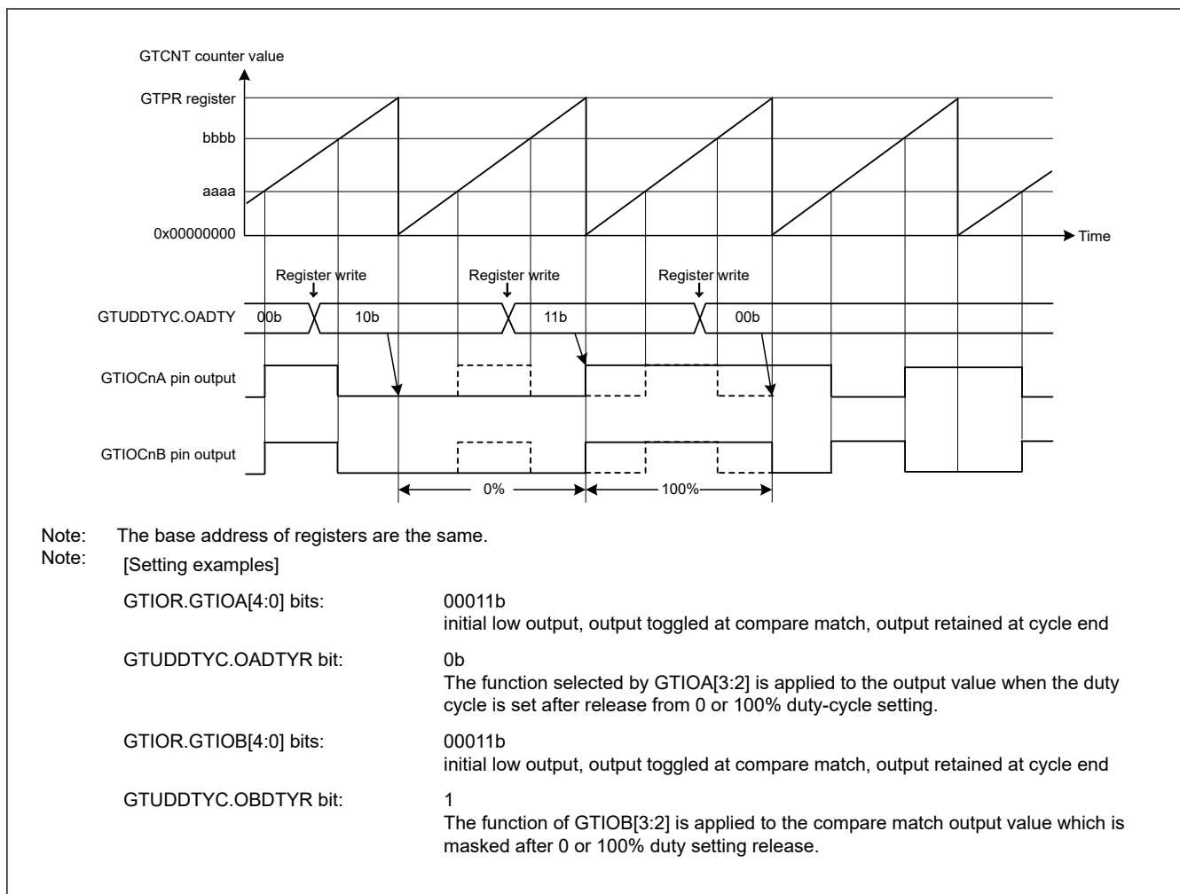
Figure 23.82 Example of output duty 0% and 100% function
