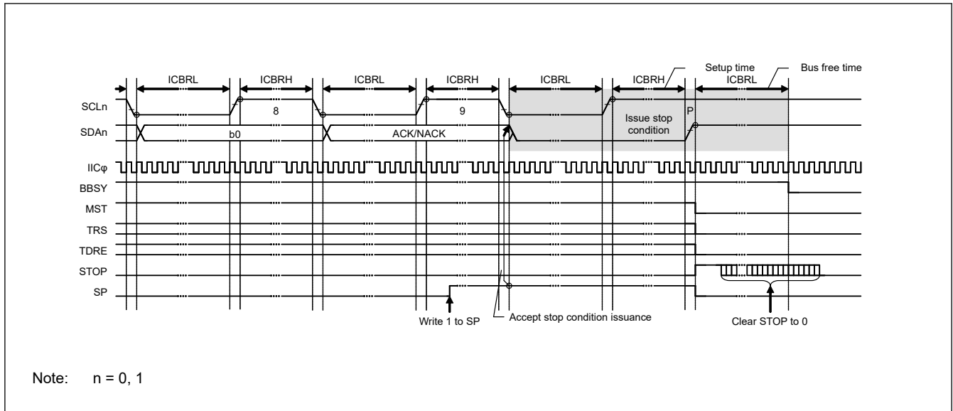
Figure 40.47 Stop condition issue timing using the SP bit
