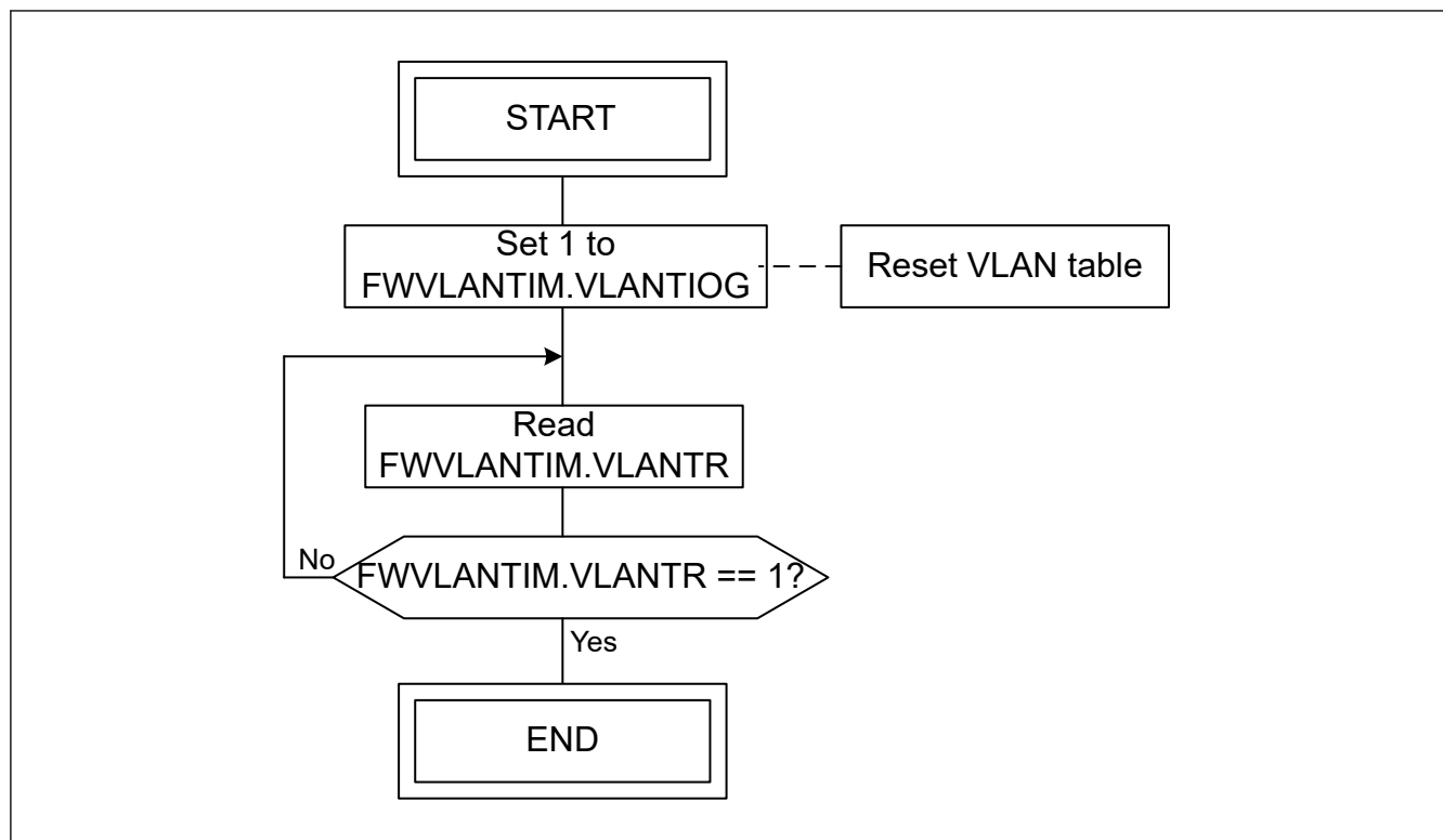
Figure 31.16 Reset flow of VLAN table
