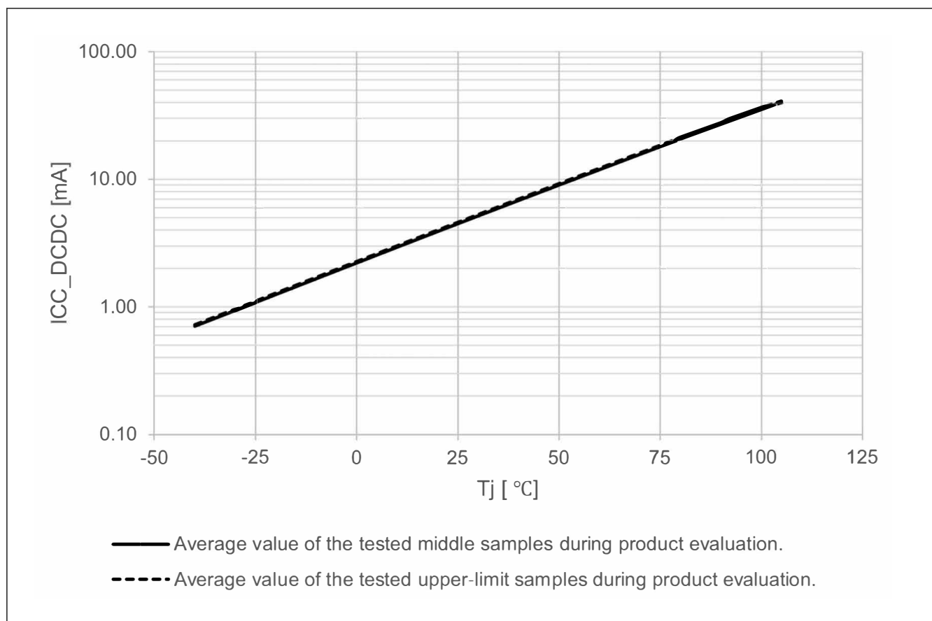
Figure 70.5 Temperature dependency in Software Standby mode ( ICC\_DCDC , SS2LP\_1 , SVSCR\_2 ) (reference data)
