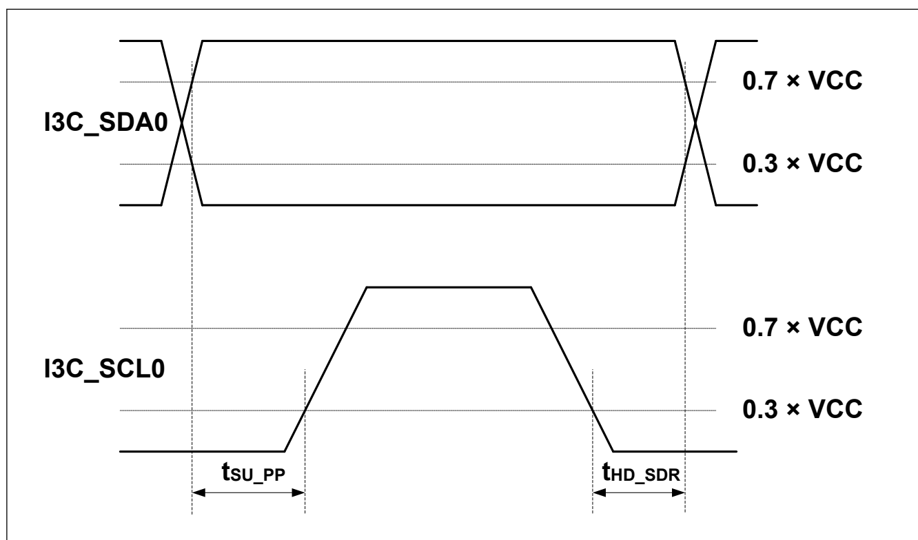
Figure 70.97 Master SDR Timing
