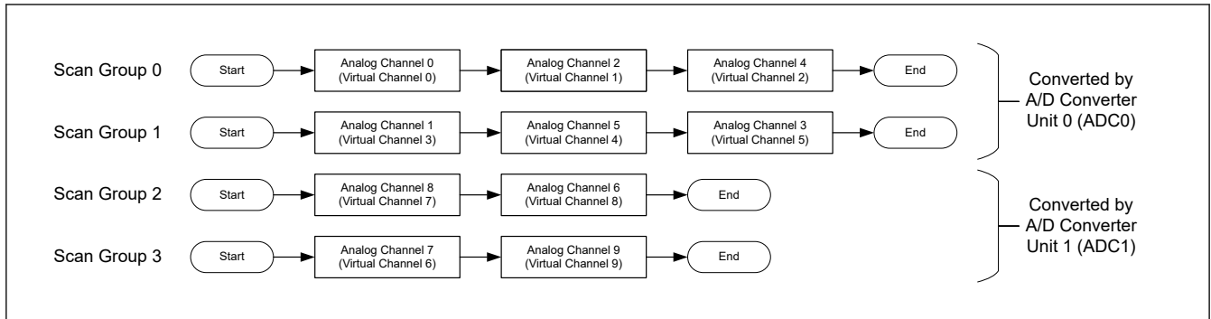
Figure 54.6 Example of A/D conversion order at the scanning operation
