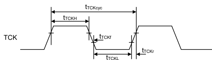
Figure 70.151 Boundary scan TCK timing
