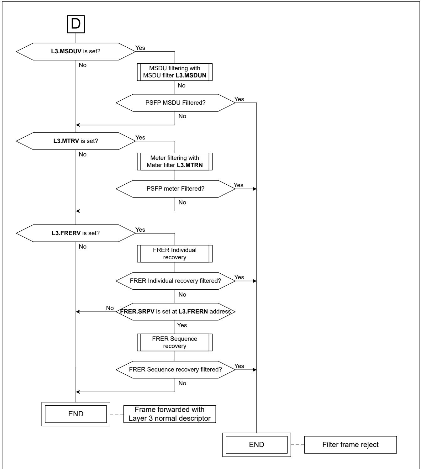
Figure 31.87 Layer 3 filtering flow
