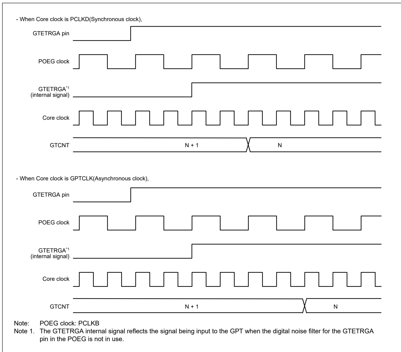
Figure 23.9 Example of event count operation in down-counting using hardware sources
