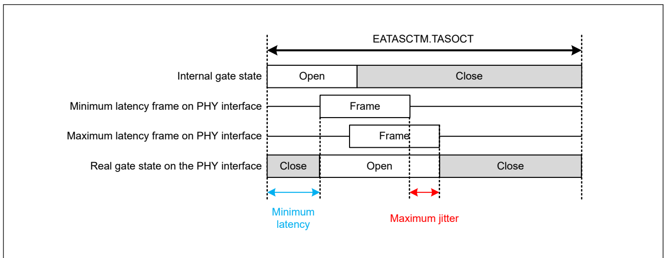
Figure 33.28 Minimum latency and maximum jitter
