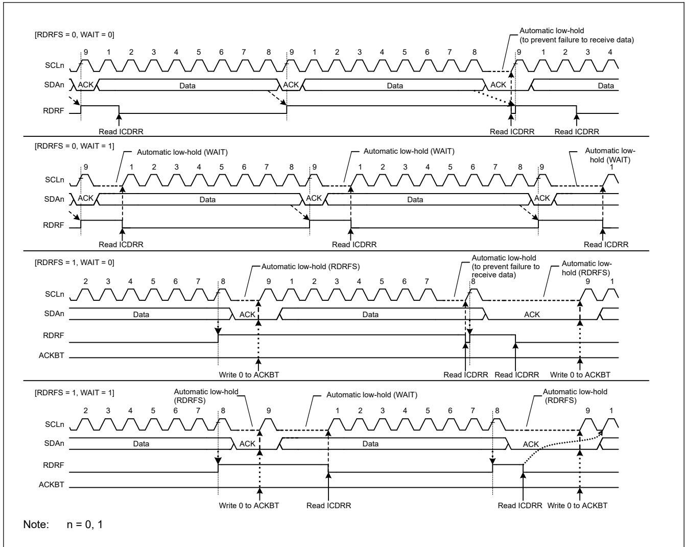
Figure 40.40 Automatic low-hold operation in receive mode using the RDRFS and WAIT bits
