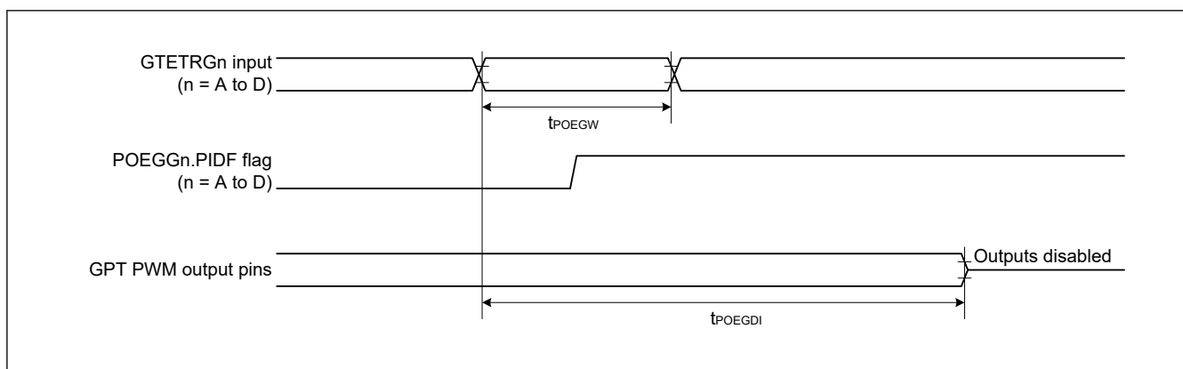
Figure 70.55 Output Disable Time for POEG via Detection Flag in Response to the Input Level Detection of the GTETRn pin
