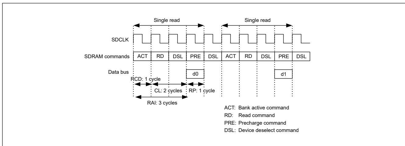
Figure 15.54 Example timing for single read (4)
