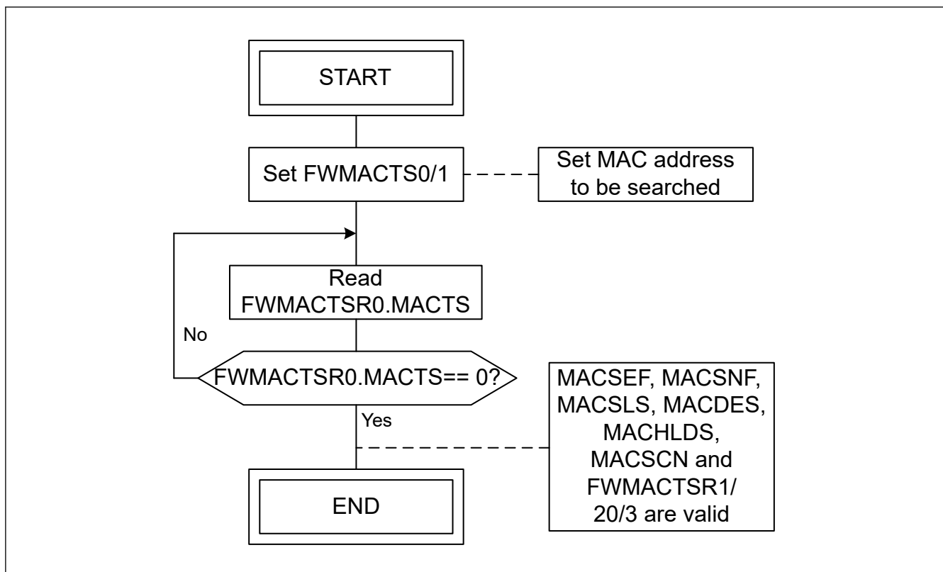
Figure 31.19 MAC entry search flow
