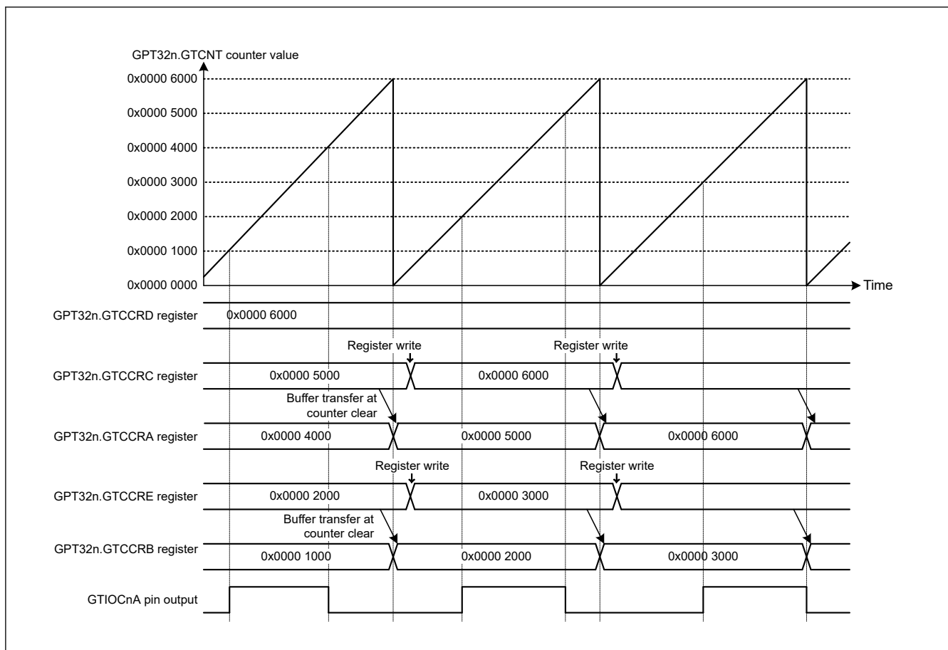
Figure 23.38 Example of Saw-Wave PWM Mode 2 Operation (Low Output at GTCCRA Register Compare Match, High Output at GTCCRB Register Compare Match, Low Output at the End of Cycle, Single Buffer Operation, Cleared at GTCCRD Register Compare Match, GTIOR.OAEOCD Bit = 0) (n = 4 to 9)
