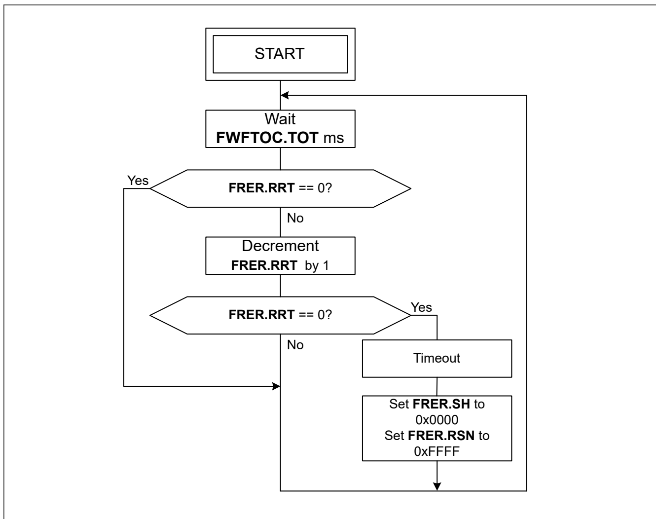
Figure 31.111 Timeout functional flow
