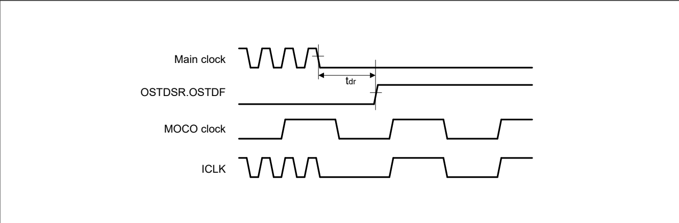
Figure 70.139 Oscillation stop detection timing
