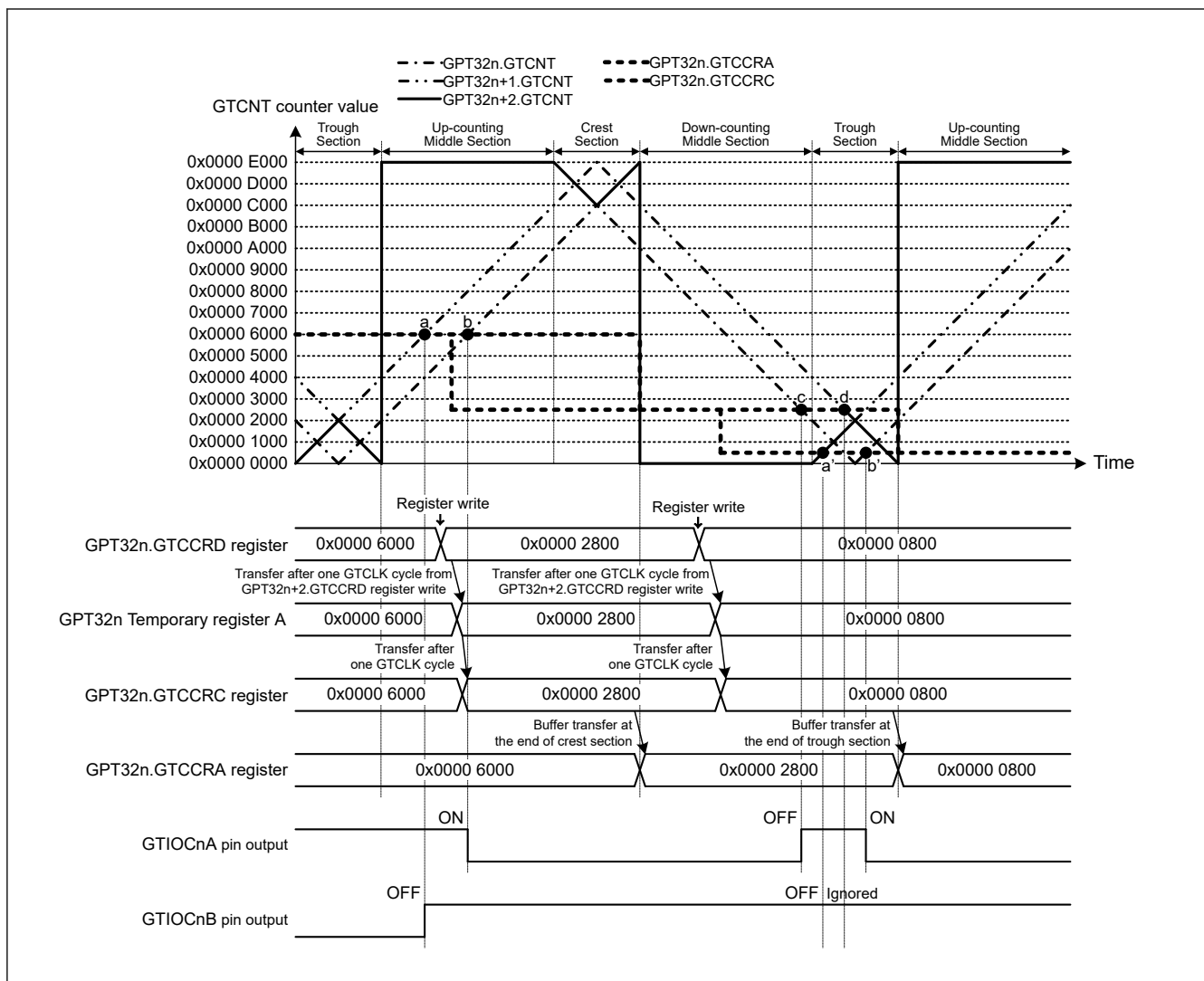
Figure 23.61 Example of Compare Match Generation Sequence Operation in Complementary PWM Mode (Complementary PWM mode 3 single buffer operation, GTIOCnA pin = Low / GTIOCnB pin = High at GTCCRA register compare match during up-counting, GTIOCnA pin = High / GTIOCnB pin = Low at GTCCRA register compare match during down-counting, the dead time value is 0x0000 2000, compare match generation order: c → a' → d → b') (n = 4, 7)
