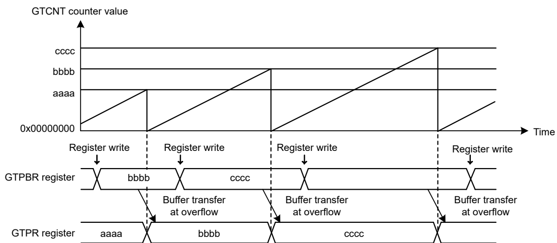
Figure 23.16 Example of GTPR buffer operation with saw waves in up-counting
