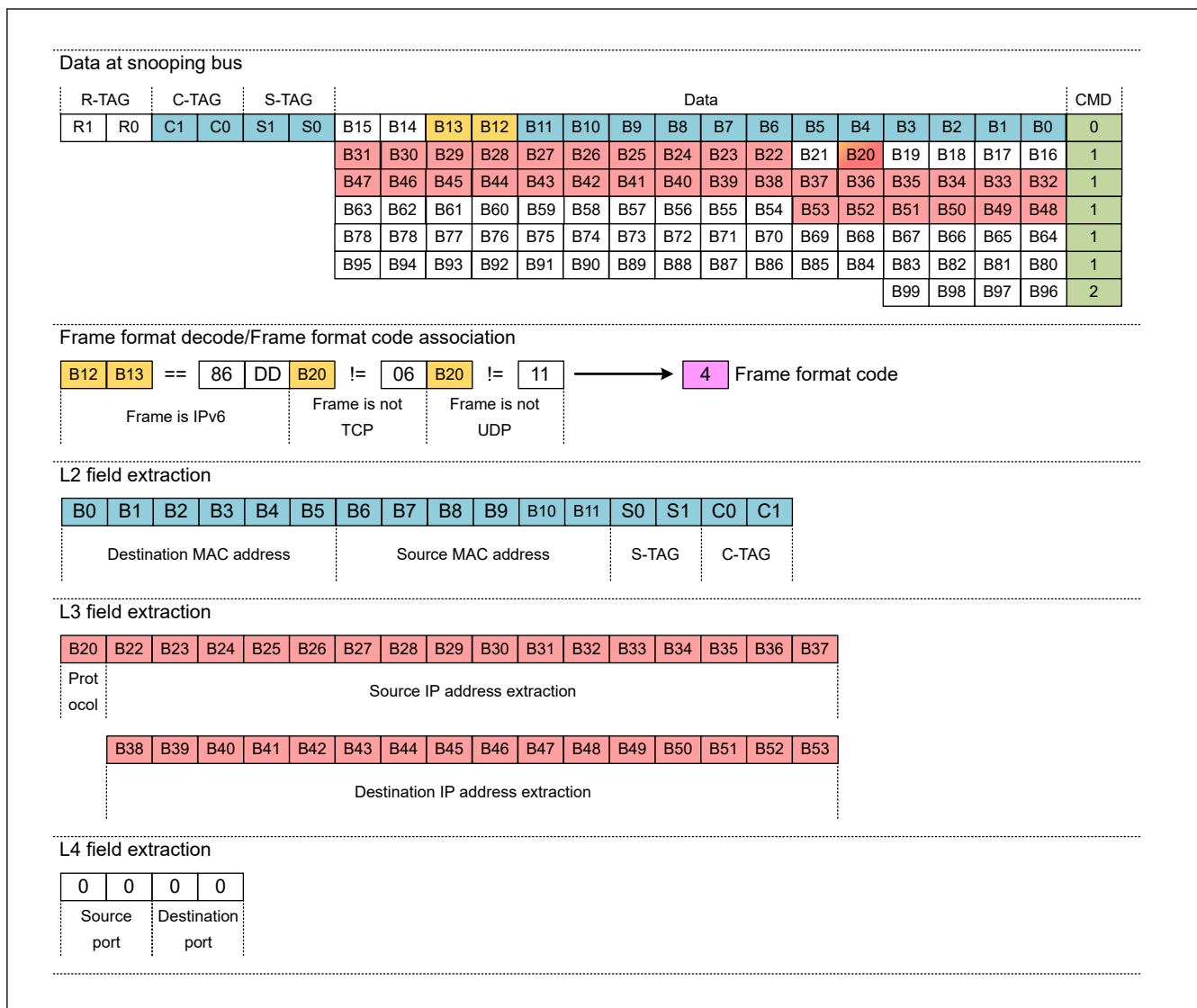
Figure 31.76 IPv6 detection and data extraction
