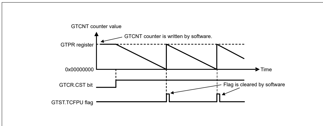
Figure 23.6 Example of periodic count operation in down-counting by the count clock
