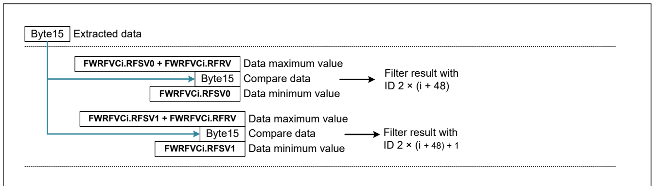
Figure 31.70 Range filter data extraction for filtering
