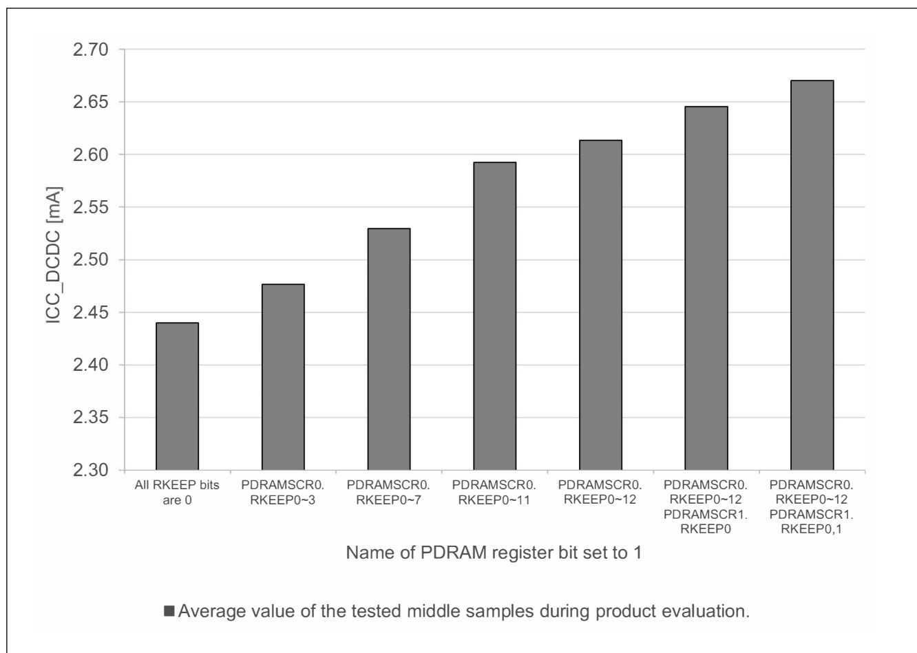
Figure 70.10 Software Standby current per SRAM state (ICC_DCDC, SS2LP_0, SVSCR_1) (reference data)
