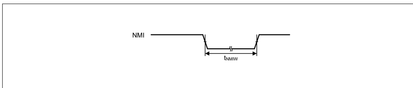
Figure 70.36 NMI interrupt input timing
