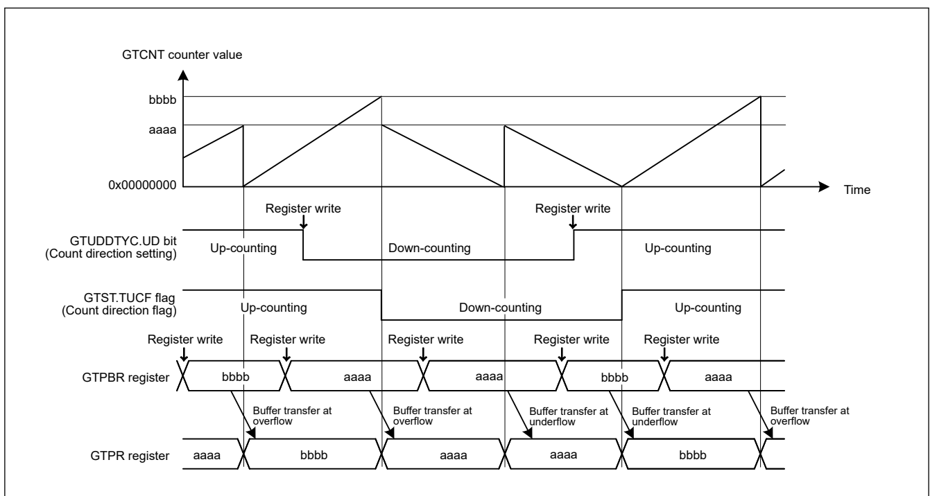
Figure 23.81 Example of a count direction changing function operation during buffer operation
