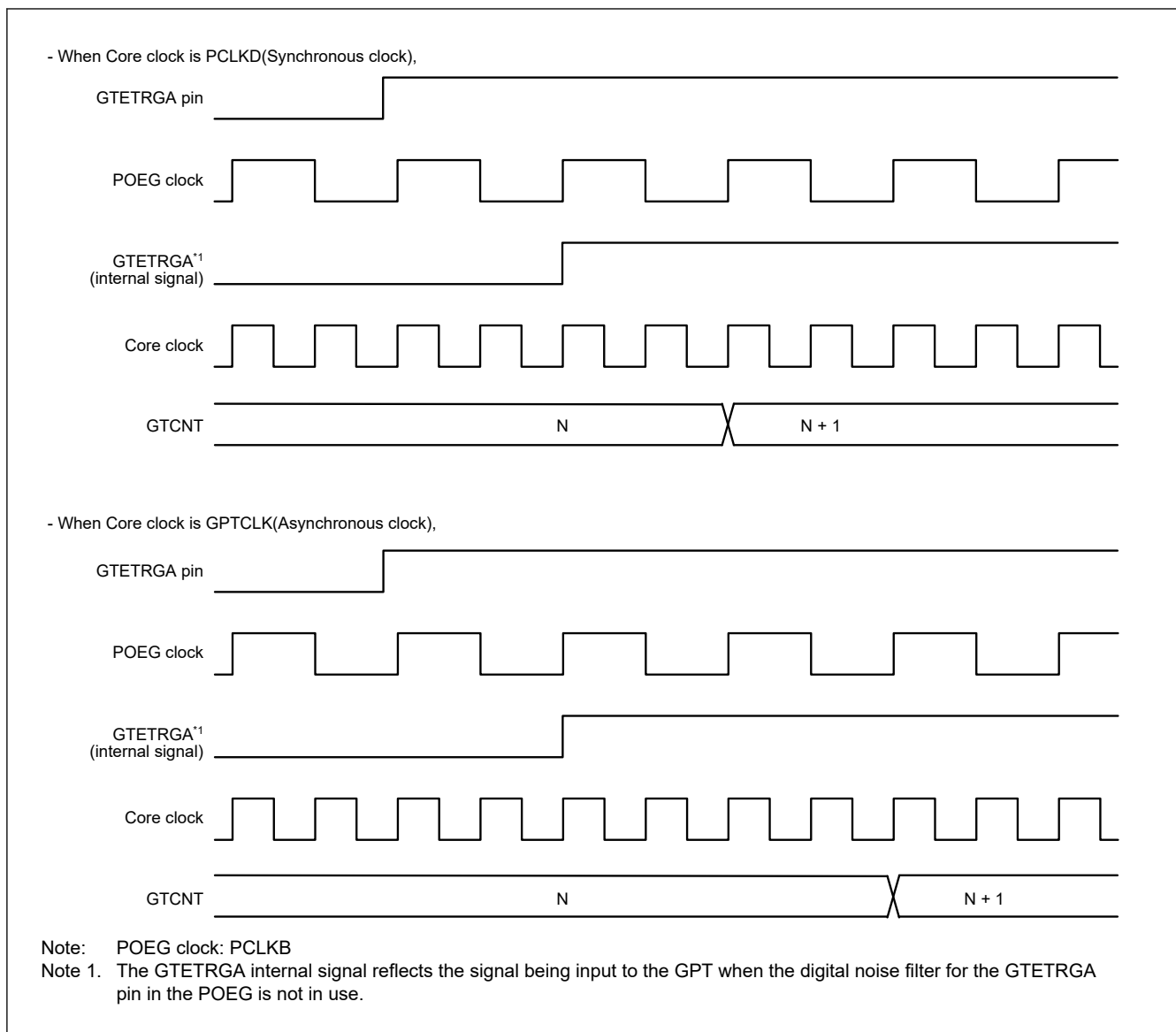
Figure 23.7 Example of event count operation in up-counting using hardware sources
