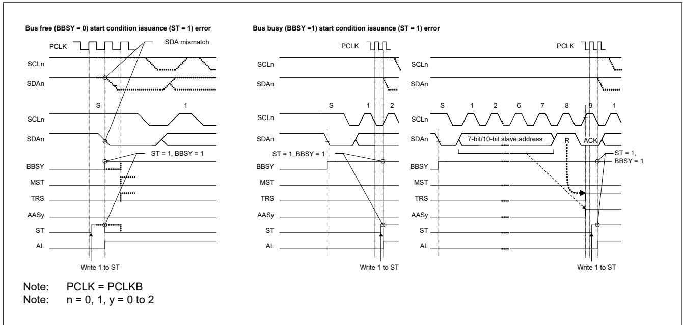
Figure 40.42 Arbitration-lost when start condition is issued when MALE = 1
