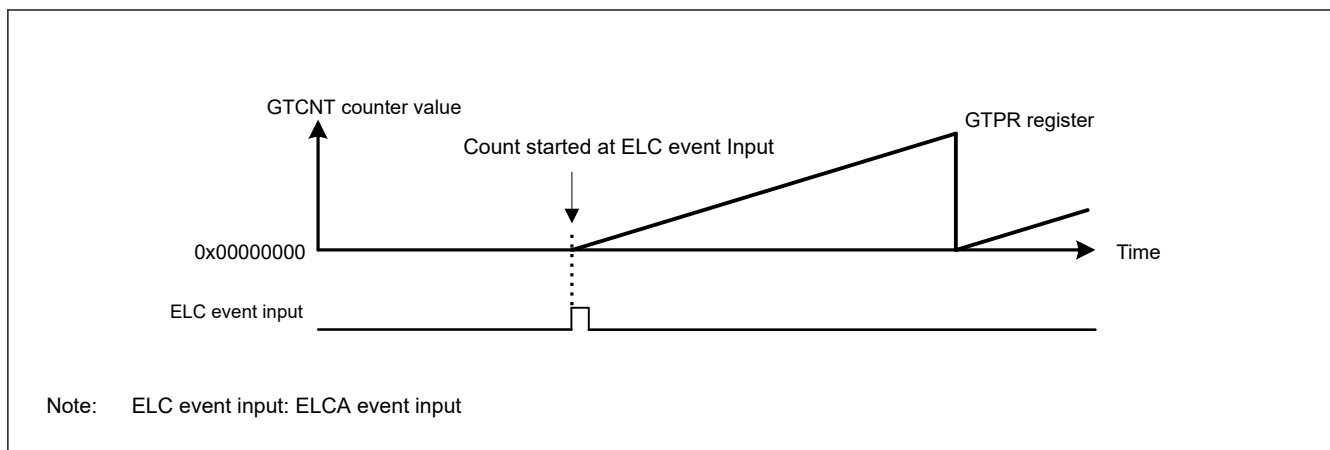
Figure 23.83 Example of count start operation by a hardware source started at the input of the signal from the ELCA event
