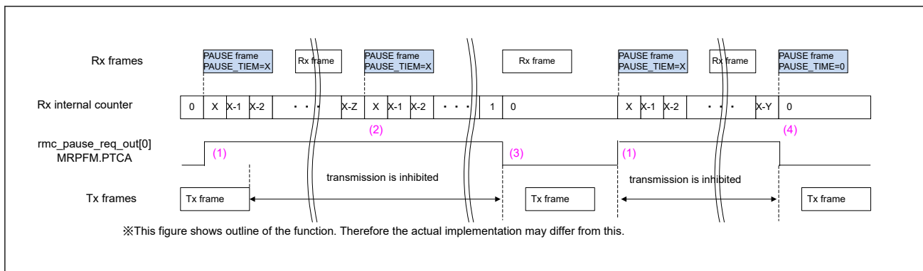
Figure 34.17 Reception of PAUSE frame
