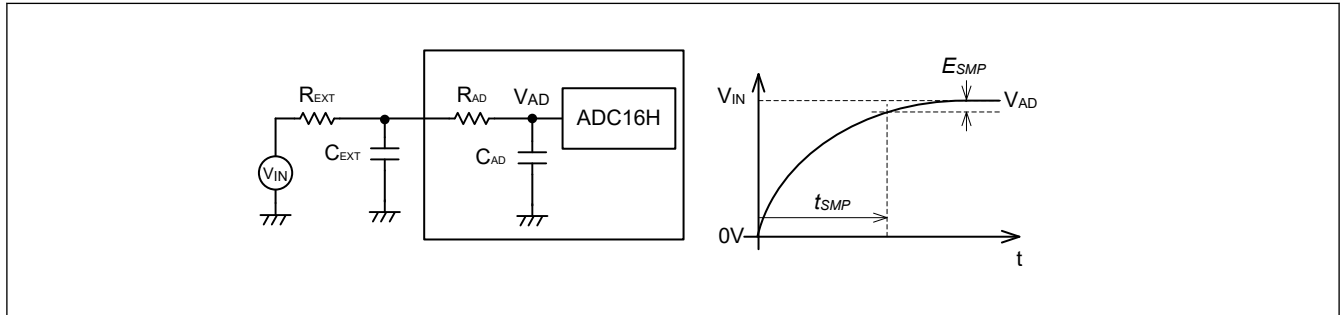
Figure 54.67 Simplified model of sample-and-hold circuit for A/D converter
