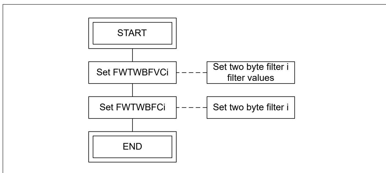
Figure 31.36 Setting flow of two-byte filter i
