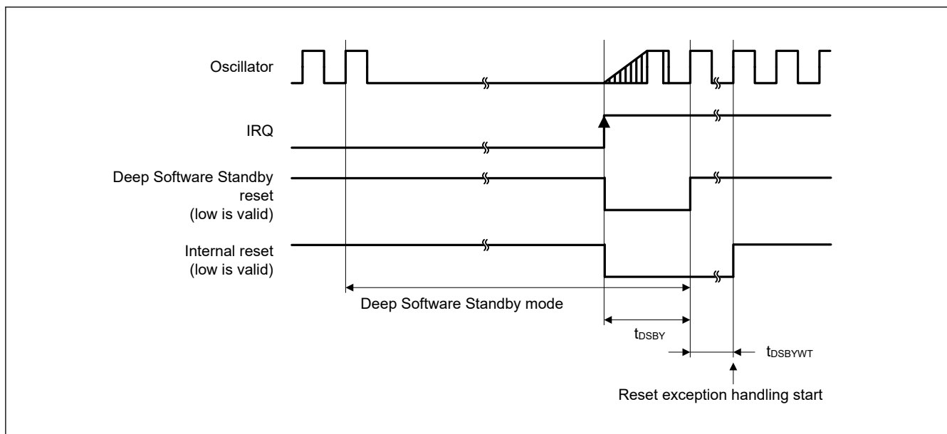
Figure 70.35 Deep Software Standby mode cancellation timing
