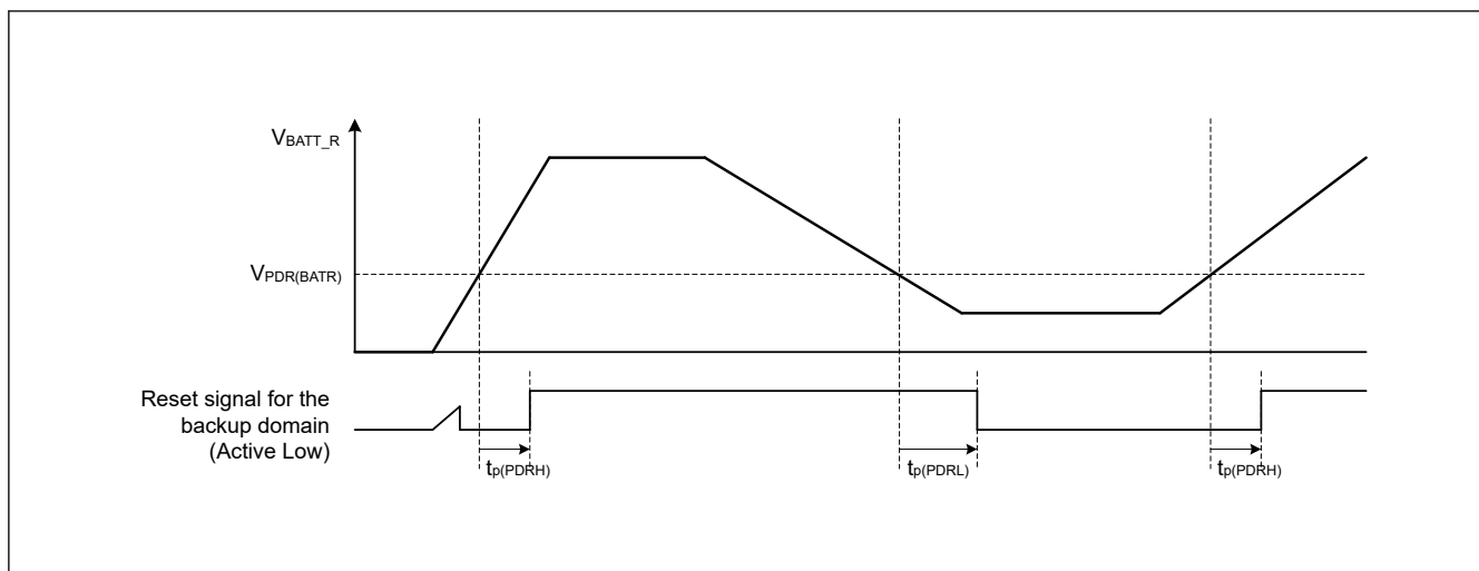
Figure 70.150 Backup domain reset characteristics
