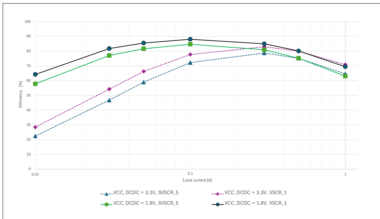
Figure 70.19 Typical DCDC efficiency (%) vs load current (A) in High-speed mode and Software Standby mode (SSCR1.SS2LP = SS2LP_1), Tj = 25 °C
