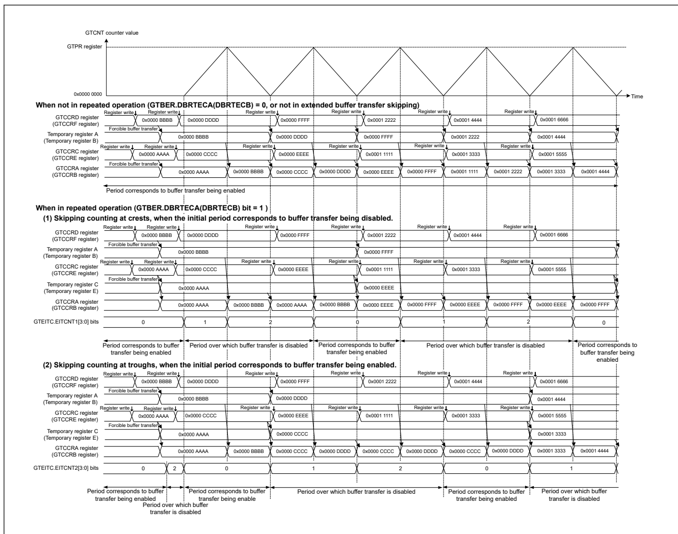
Figure 23.158 Example of Repeated Double-Buffer Operation When GTCCR Buffer Transfer is Disabled (Triangle-Wave PWM Mode 3, Using Extended Buffer Transfer Skipping, GTBER.BD[0] is Constantly 0)
