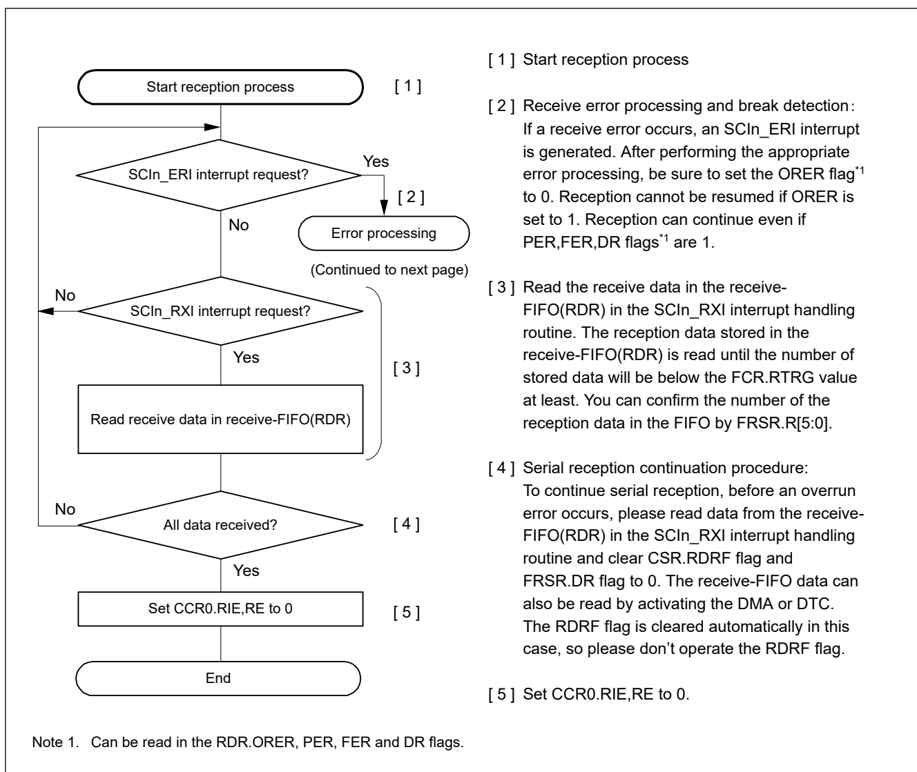
Figure 39.24 Example flow of serial reception in Asynchronous mode with FIFO selected and Address Matching Enabled (1)
