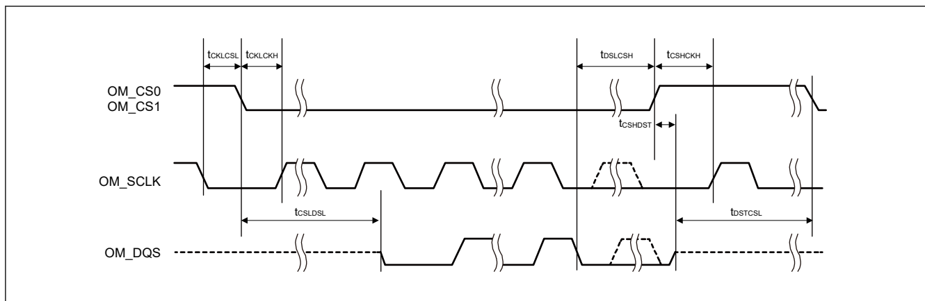
Figure 70.87 DS to CS signal timing
