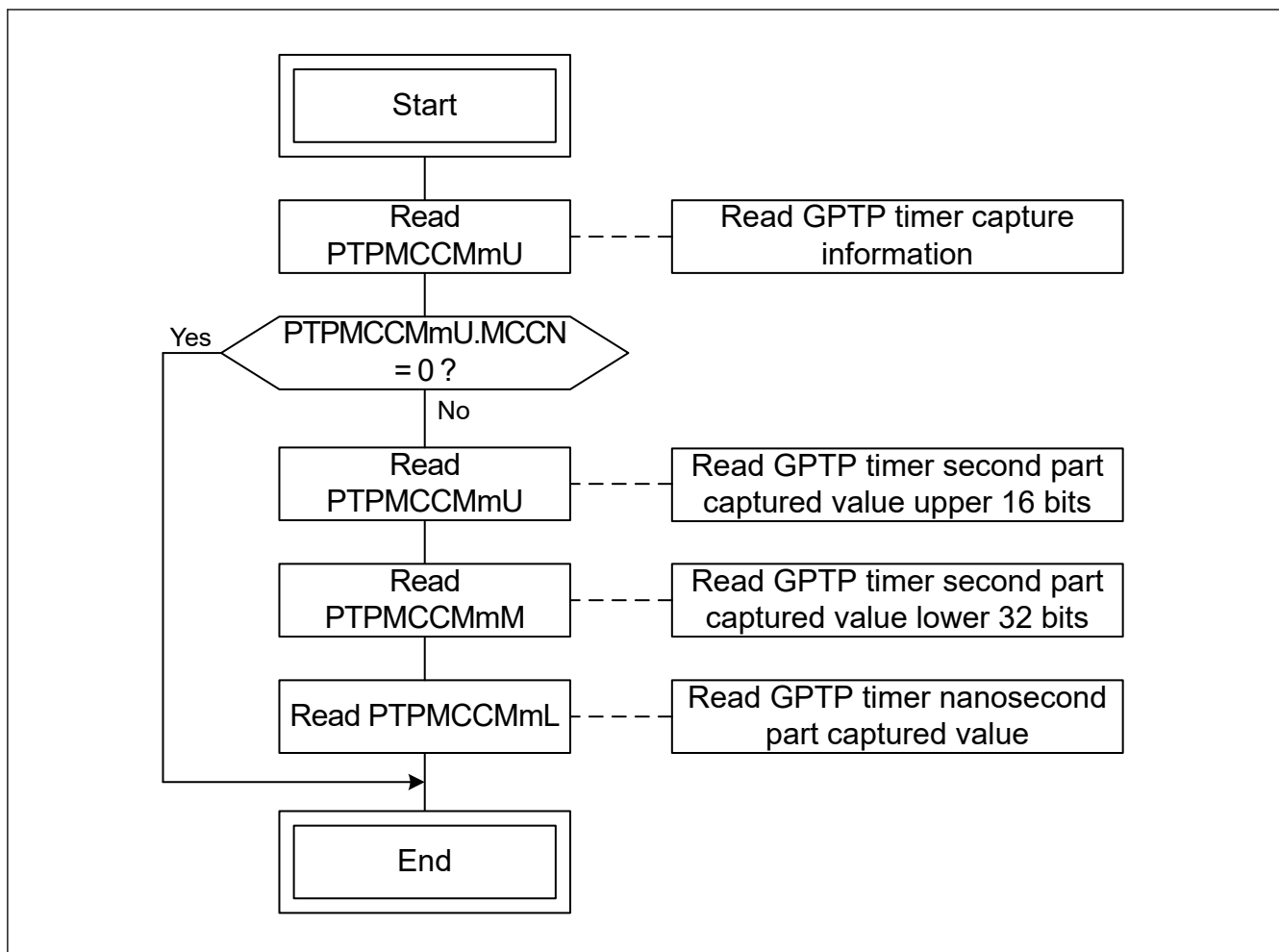
Figure 36.10 GPTP timer captured value reading flow
