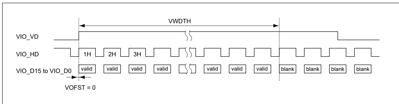
Figure 61.21 Vertical capture timing
