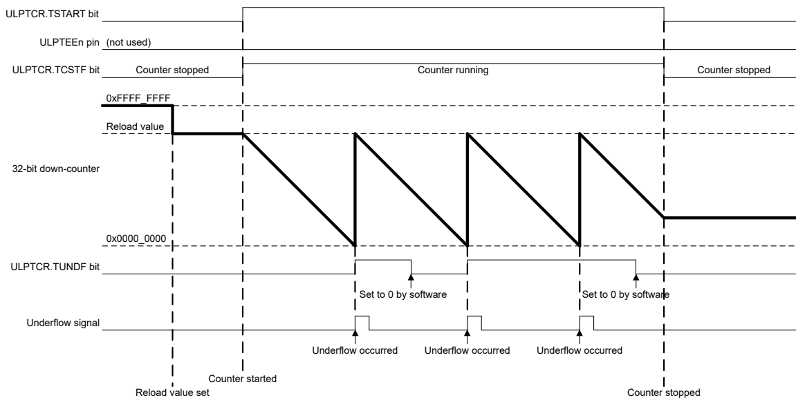
Figure 26.4 Operation example in event counter, continuous, and count enable modes (with the ULPTIOC.TIOGT0 bit set to 0)
