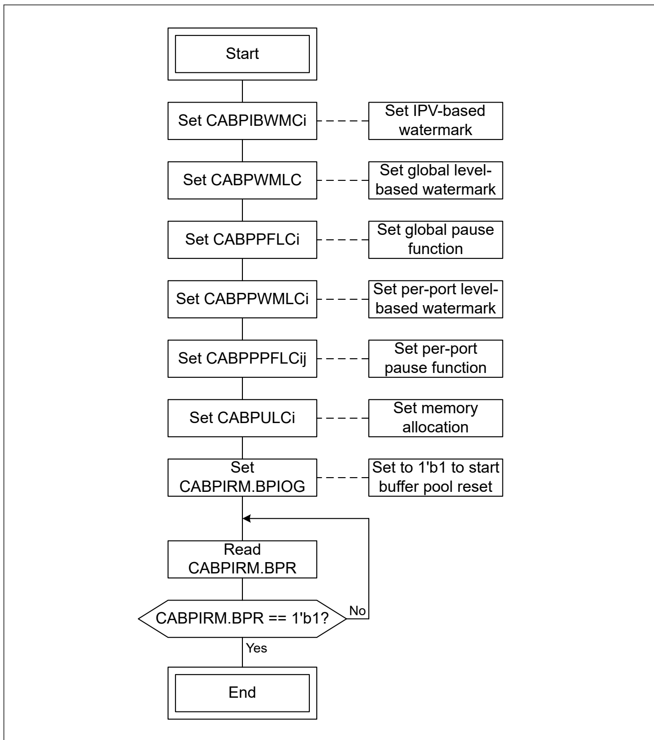
Figure 32.4 Buffer pool initialization flow
