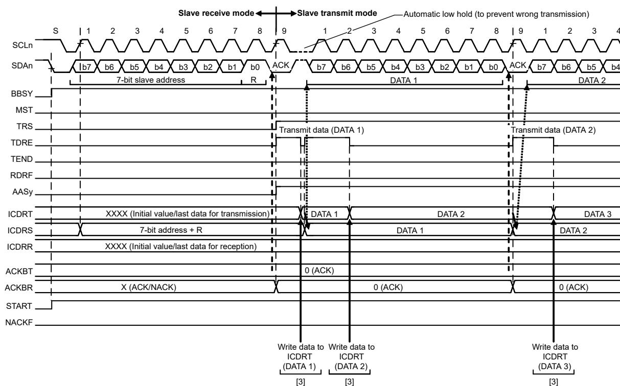
Figure 40.16 Slave transmit operation timing (1) with 7-bit address format
