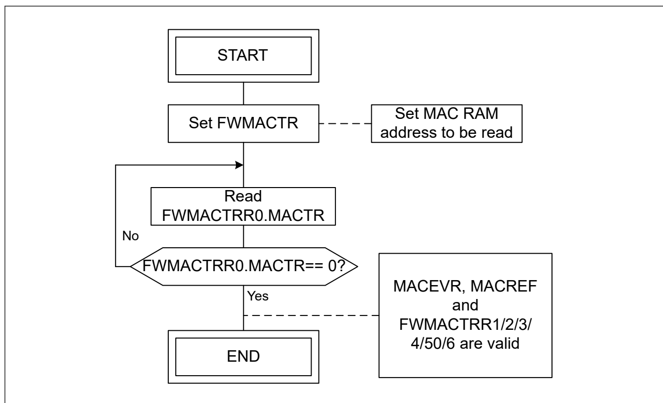
Figure 31.21 MAC entry read flow
