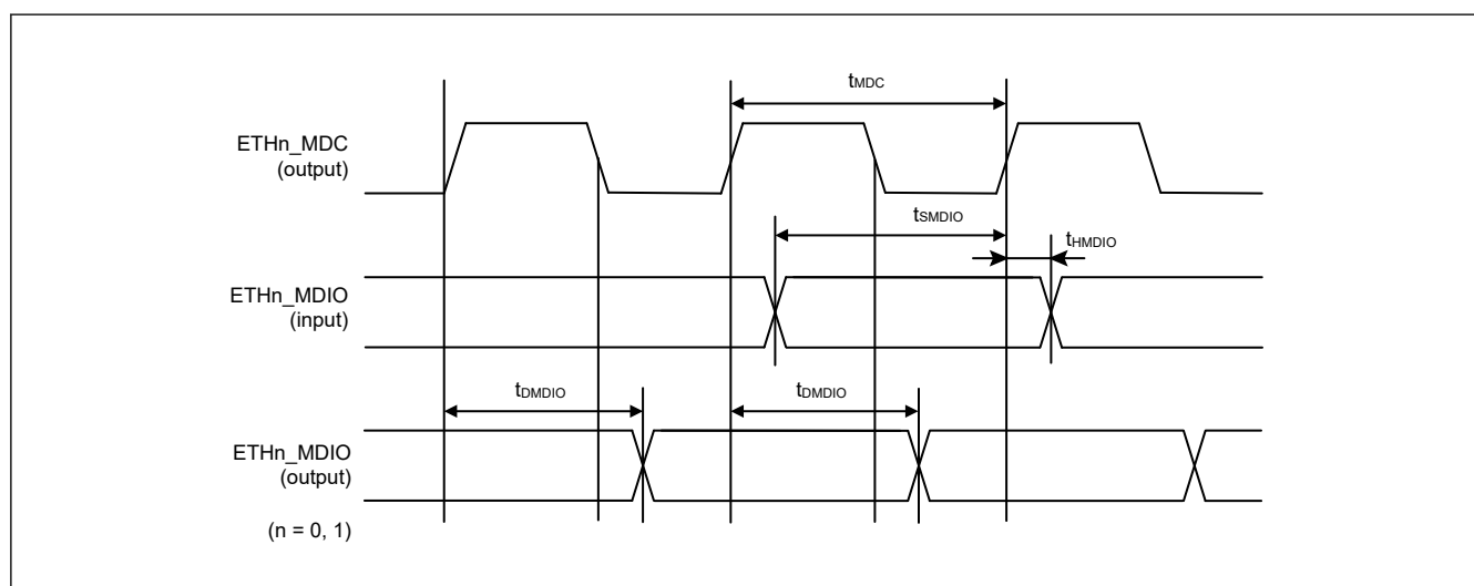
Figure 70.123 ETn_MDIO, ETn_MDC timing
