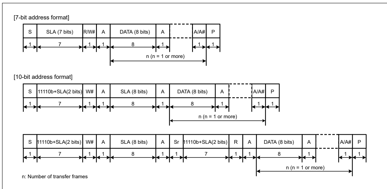
Figure 40.3 I 2 C bus format
