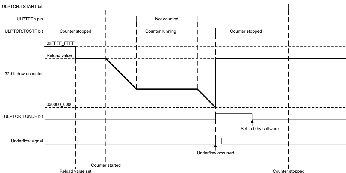
Figure 26.8 Operation example in event counter, one-shot, and count enable modes (with the ULPTIOC.TIOGT0 bit set to 1)
