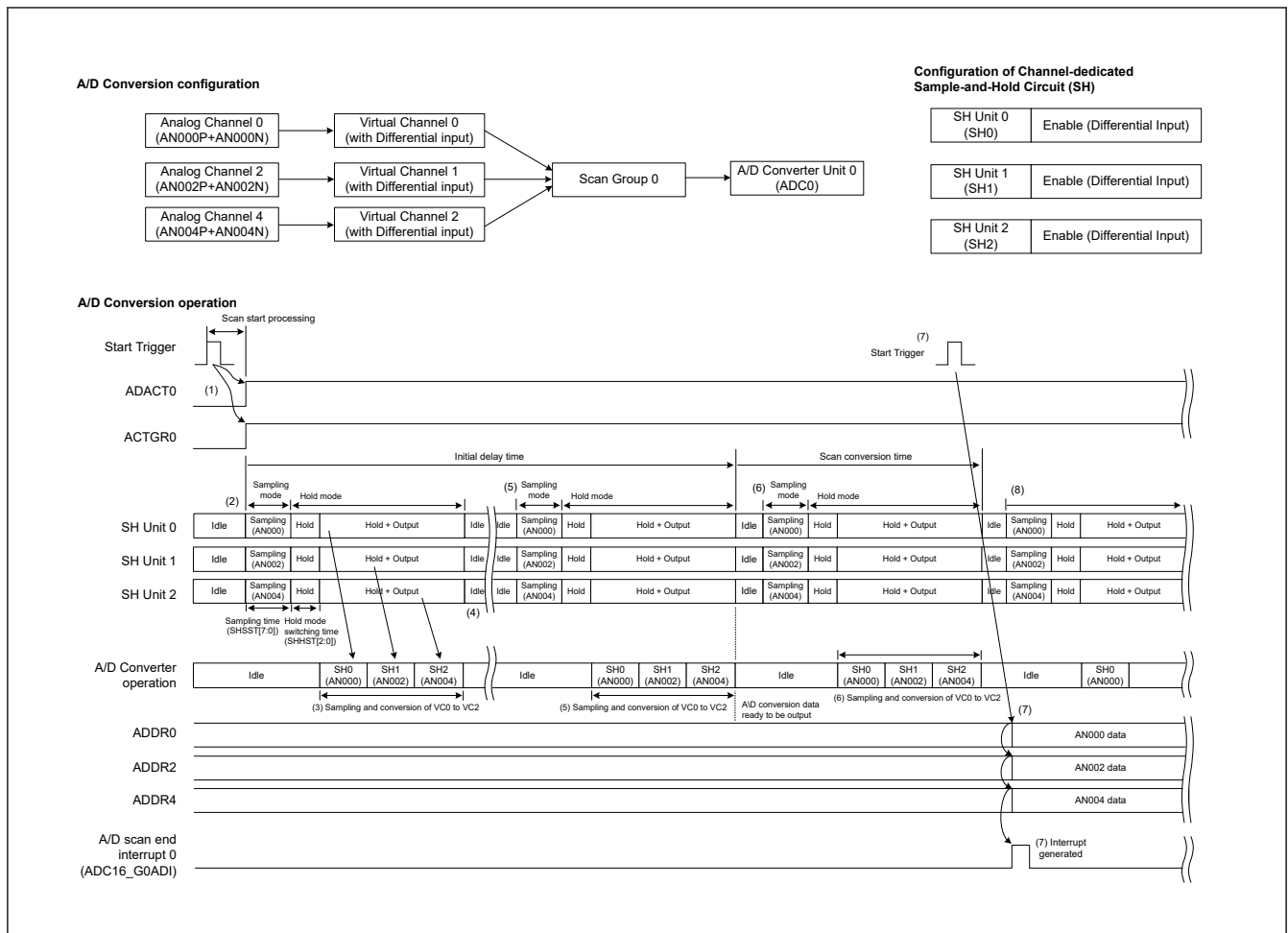
Figure 54.22 Basic operation of channel-dedicated sample-and-hold circuit in Hybrid mode – Background continuous scan mode
