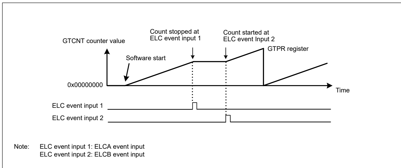
Figure 23.85 Example of count stop operation by hardware source started by software, stopped at ELCA input, and restarted at ELCB input
