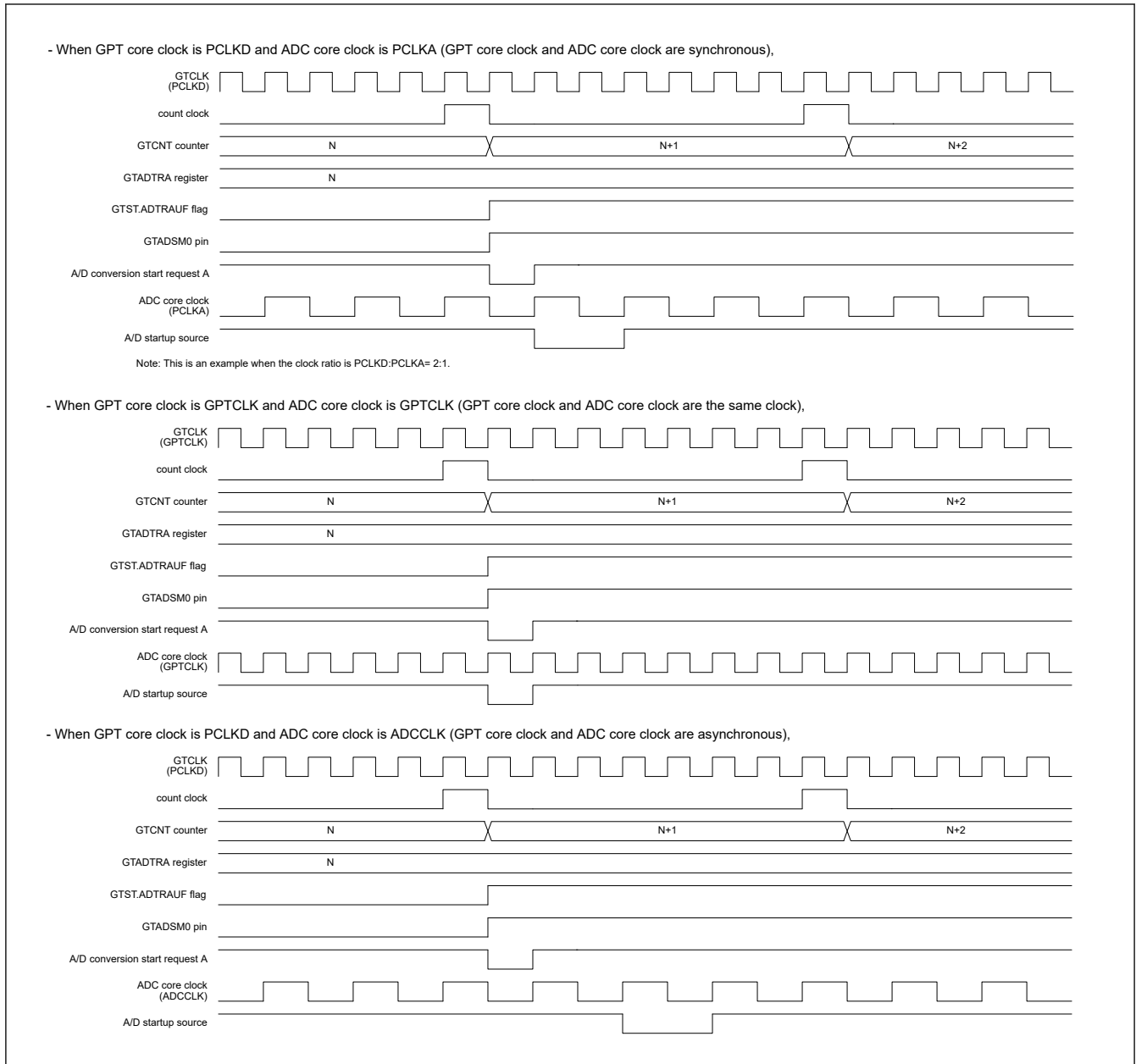
Figure 23.151 Example of A/D Conversion Start Request Timing Operation
