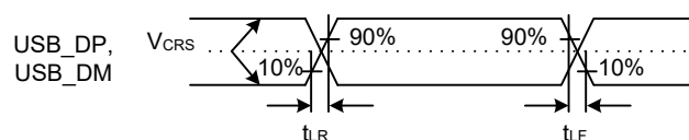
Figure 70.130 USB_DP and USB_DM output timing in low-speed mode
