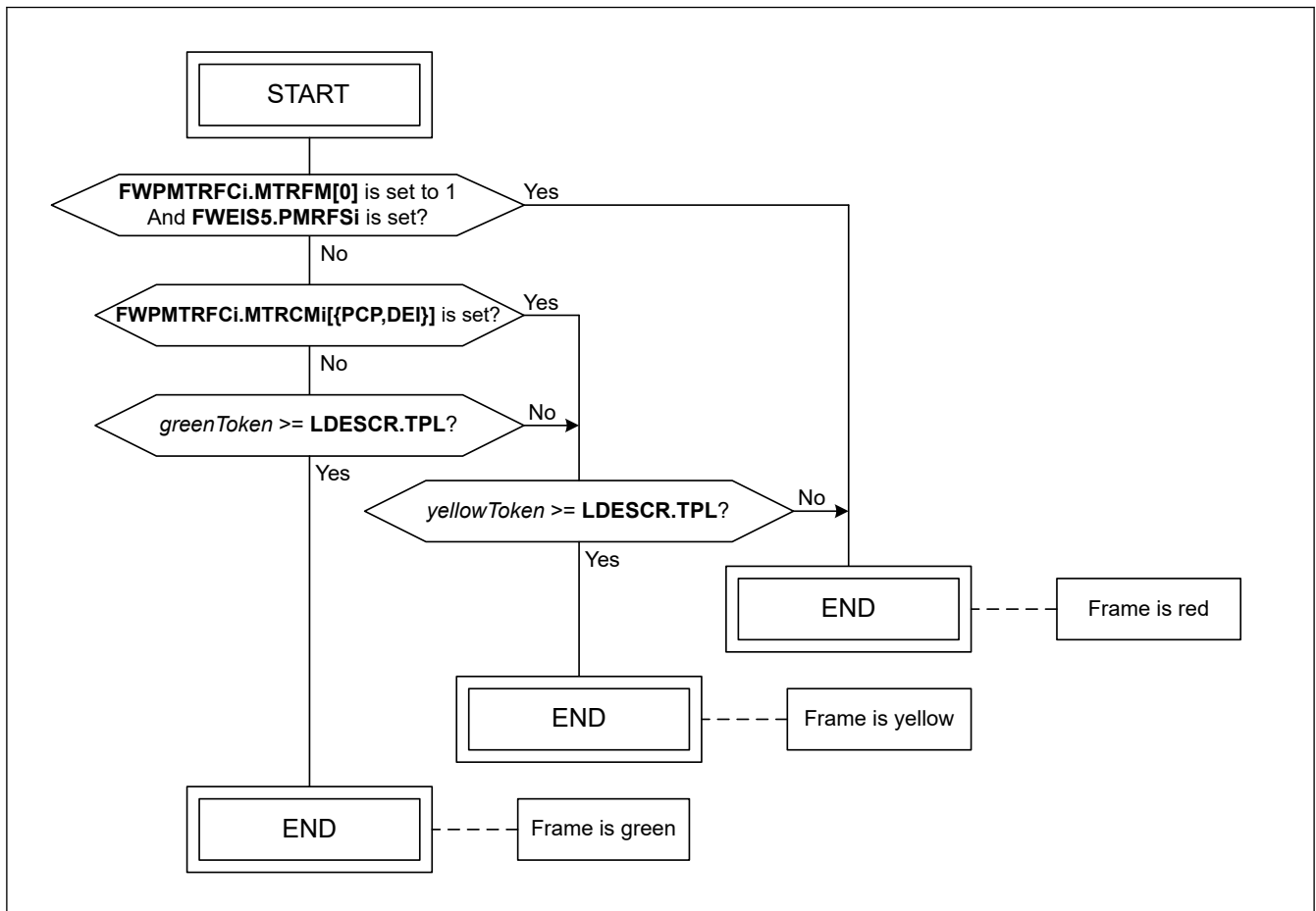
Figure 31.105 Double bucket meter i color assignment flow
