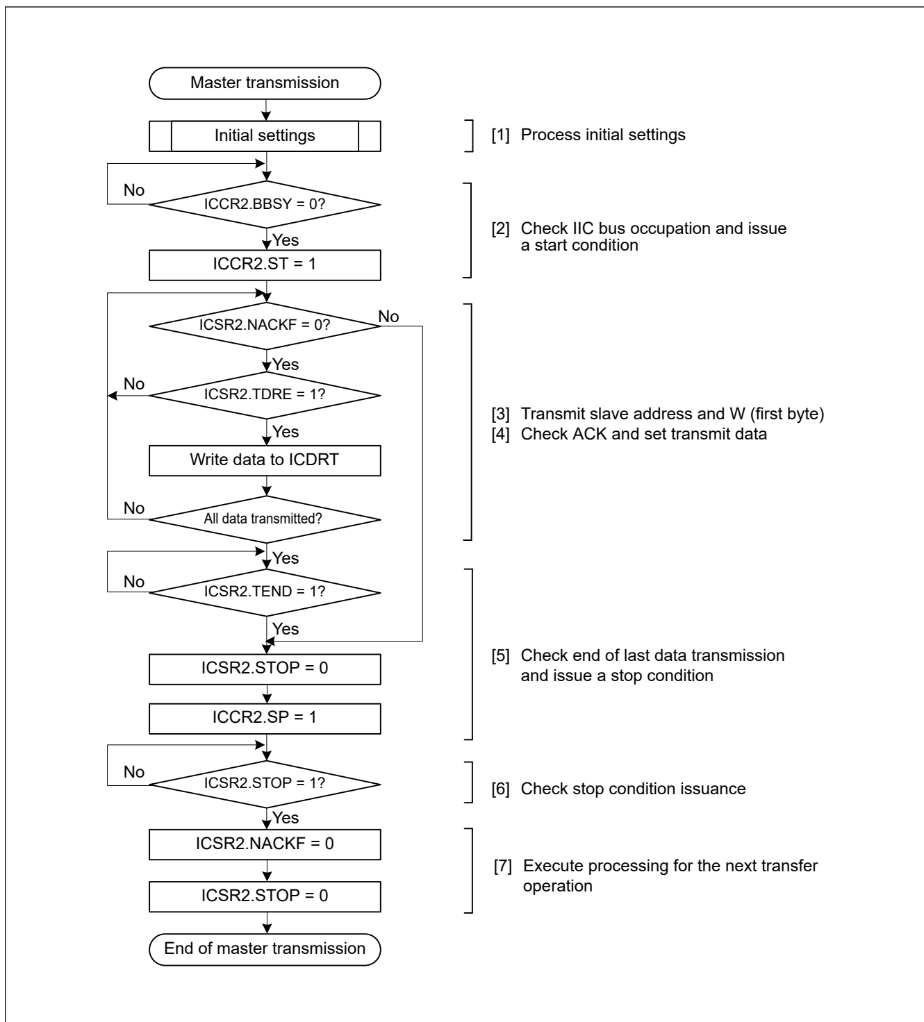
Figure 40.6 Example master transmission flow
