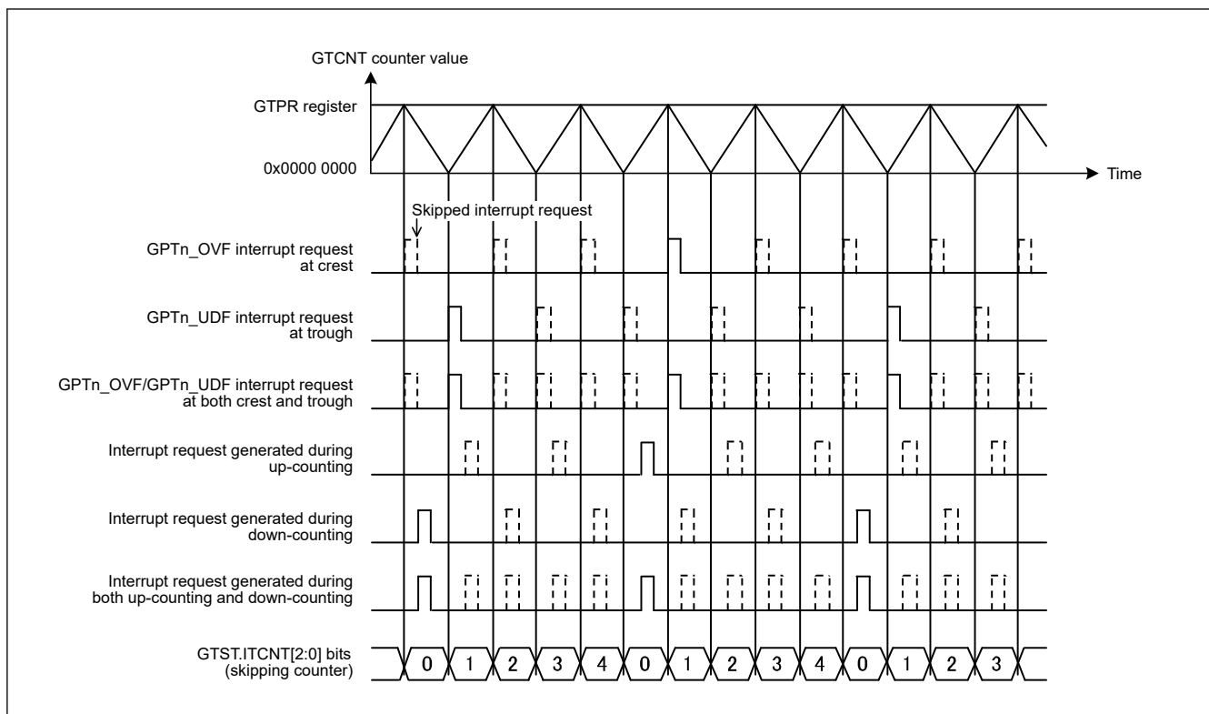
Figure 23.131 Example of Interrupt Skipping Function Operation (Triangle Waves, Counting and Skipping Both Troughs and Crests, Skipping Count: 4)
