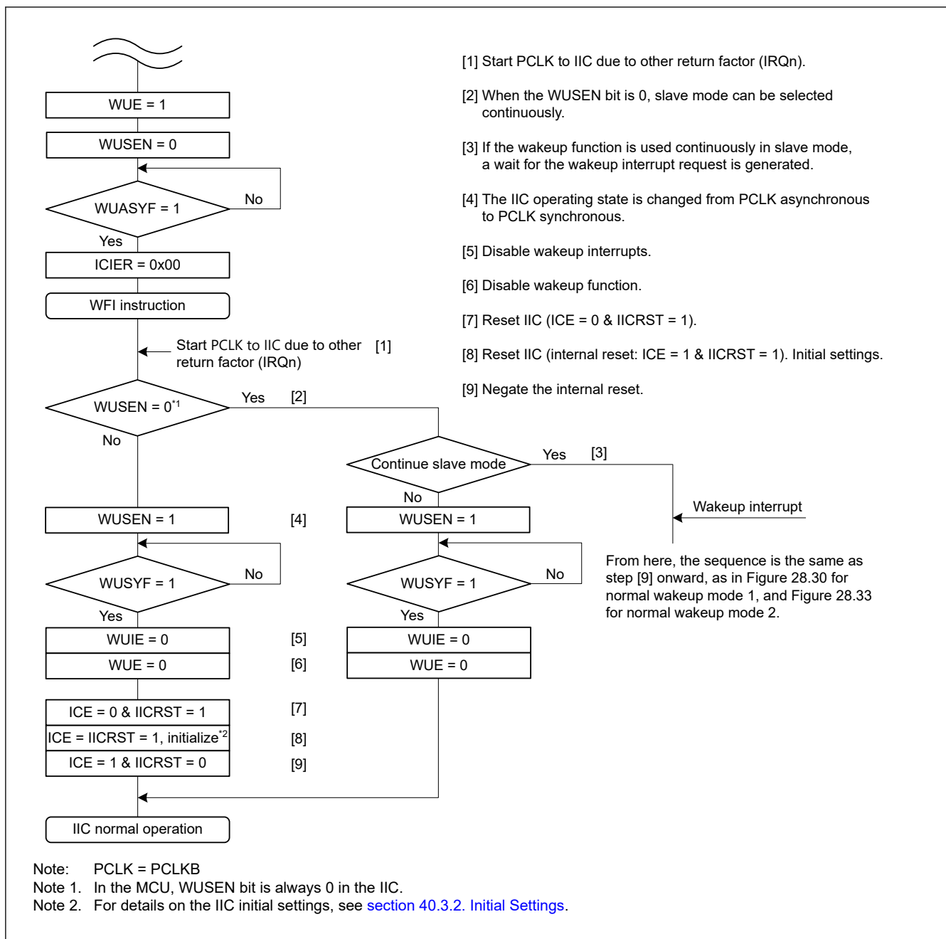
Figure 40.31 Example operation of normal wakeup modes 1 and 2 when wakeup is triggered by an interrupt other than IIC wakeup interrupt, for example, the IRQn
