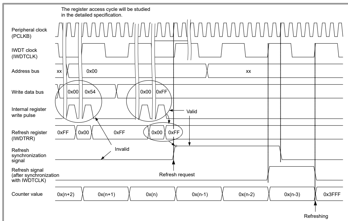
Figure 29.6 IWDT refresh operation waveforms (IWDTCR.CKS[3:0] = 0000b, IWDTCR.TOPS[1:0] = 11b)
