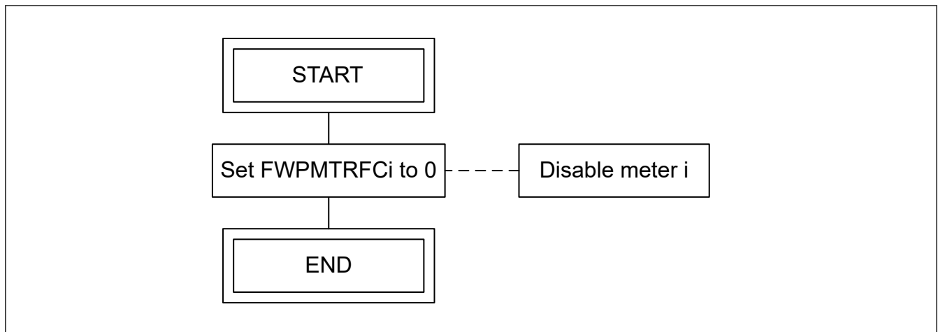
Figure 31.29 Disabling flow of meter i
