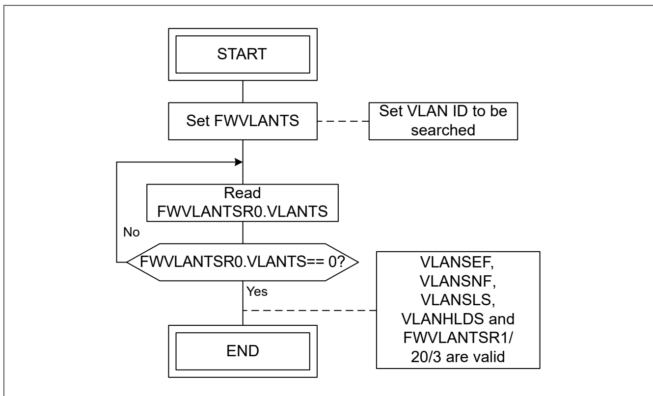
Figure 31.20 VLAN entry search flow
