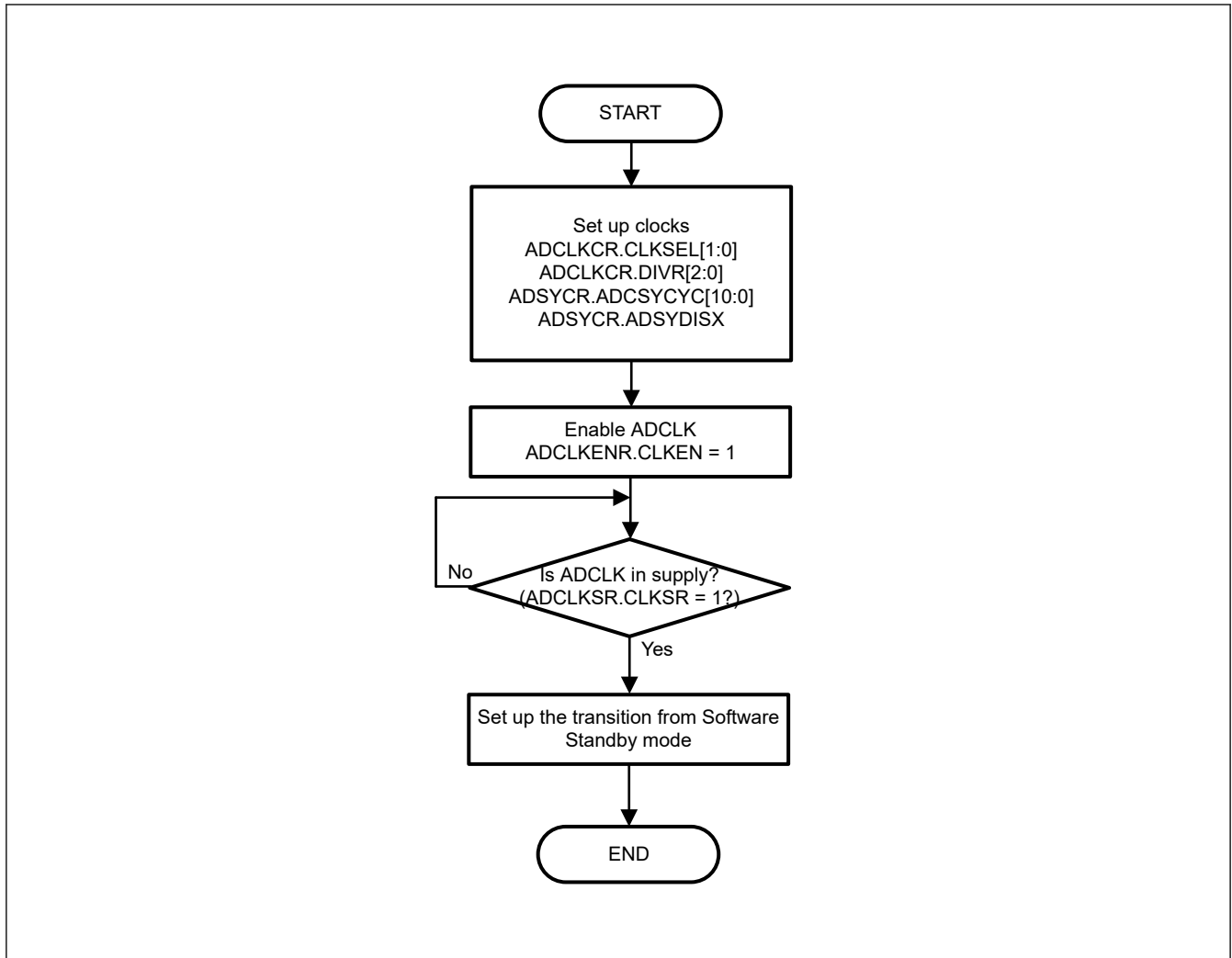
Figure 54.65 Example procedure for resuming Software Standby mode
