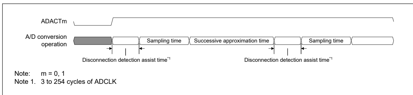
Figure 54.24 Operation of A/D conversion when disconnection detection assist function is used
