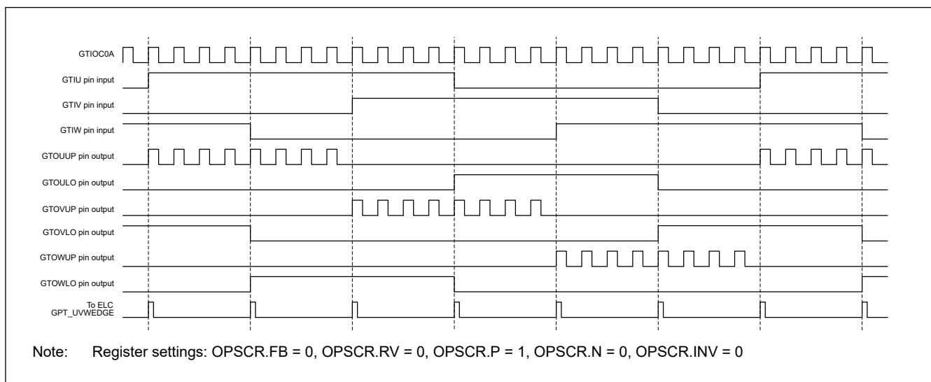
Figure 23.124 Example of GPT_OPS Chopped Output Operation (Positive Phase 120-degree)
