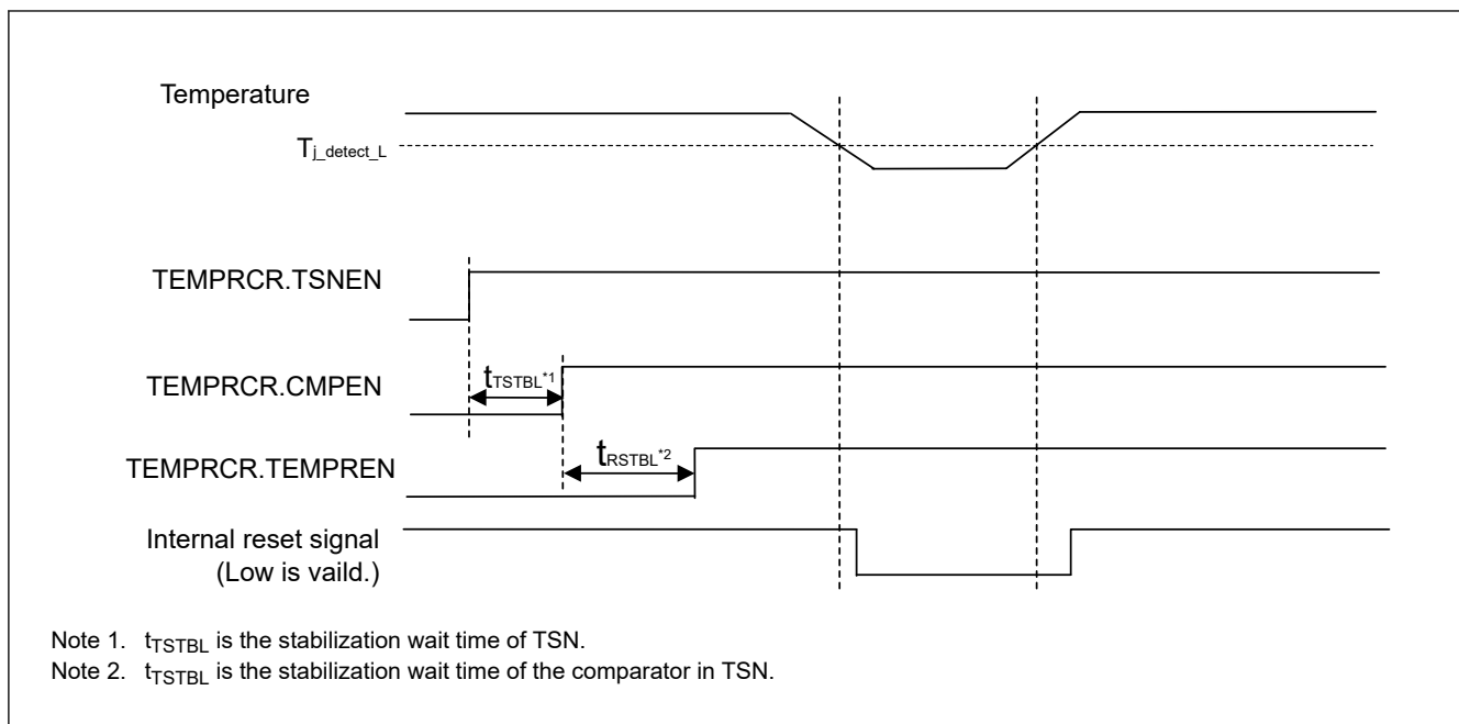
Figure 70.148 Timing of temperature monitor reset (Low-temperature detection)
