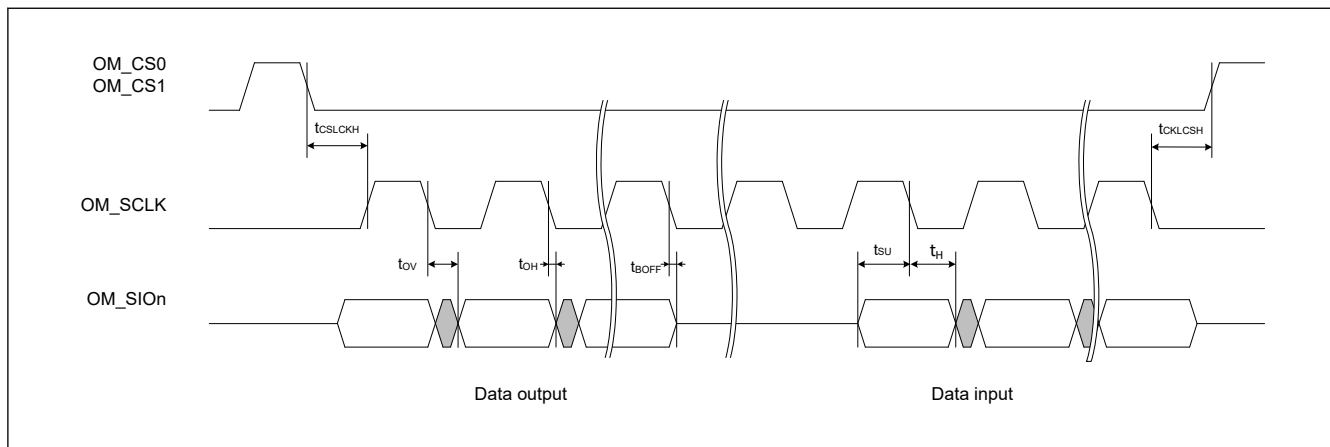
Figure 70.84 SDR transmit/receive timing (1S-1S-1S, 1S-2S-2S, 2S-2S-2S, 1S-4S-4S, 4S-4S-4S)
