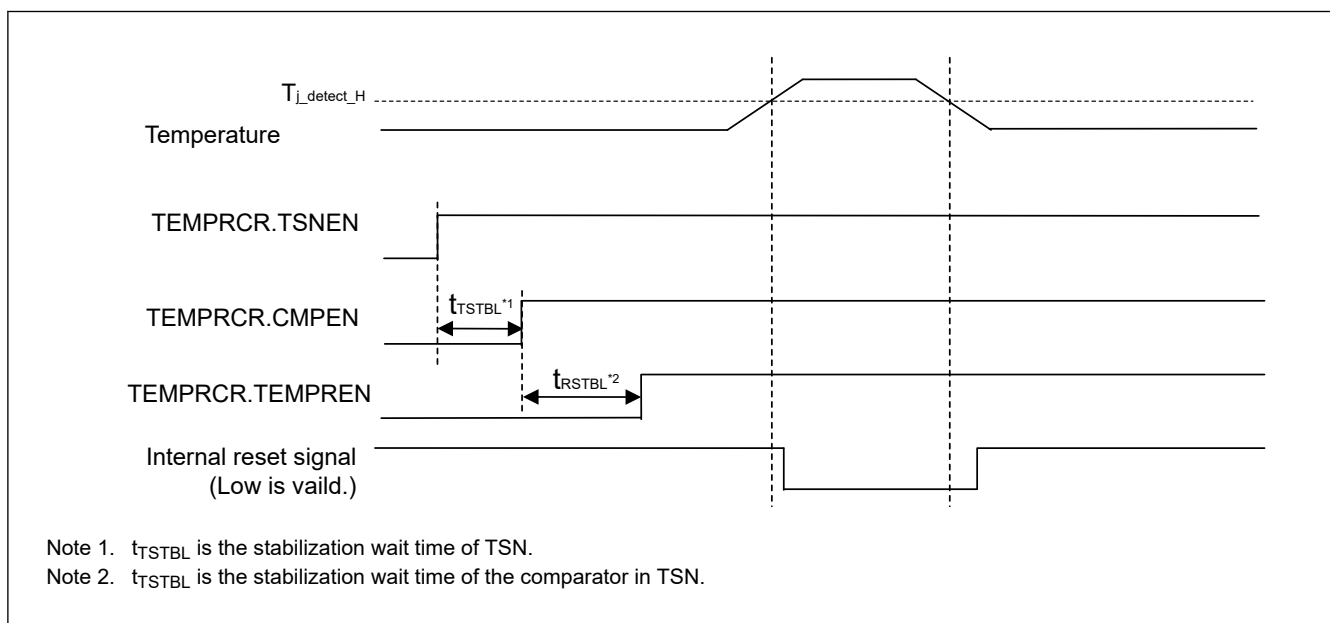
Figure 70.147 Timing of temperature monitor reset (High-temperature detection)
