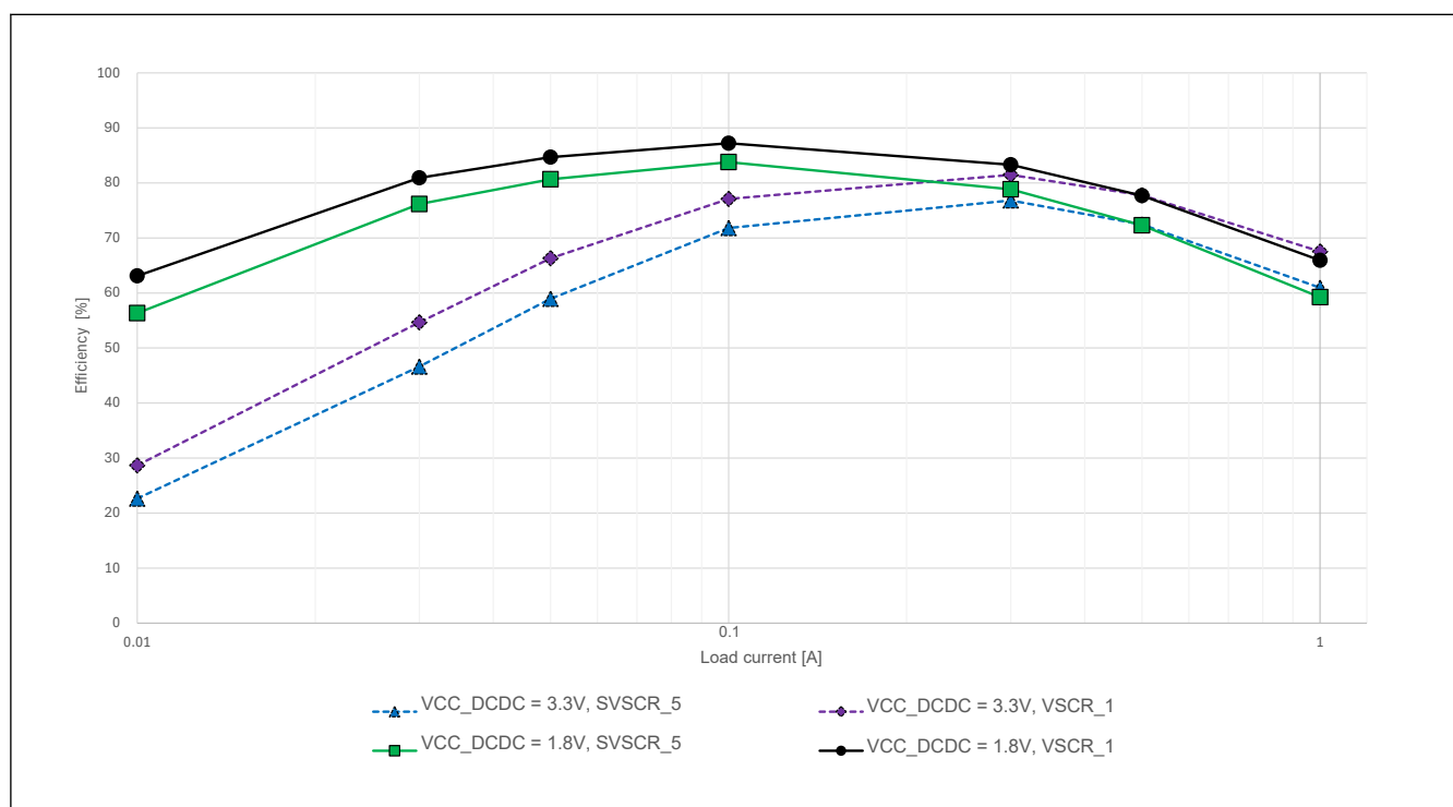
Figure 70.20 Typical DCDC efficiency (%) vs load current (A) in High-speed mode and Software Standby mode (SSCR1.SS2LP = SS2LP_0), Tj = 105 °C
