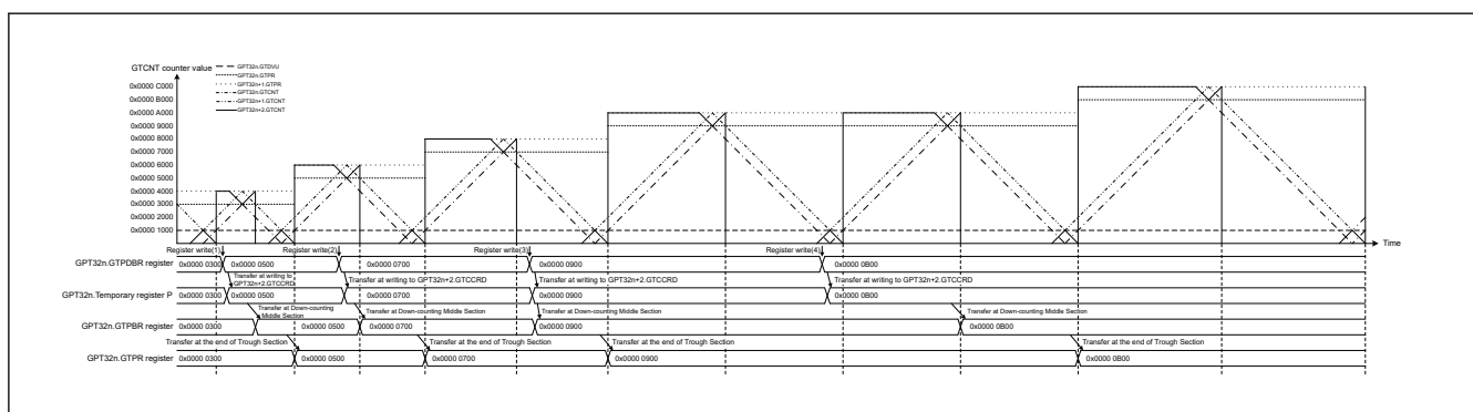
Figure 23.20 Example of GTPR double buffer operation with complementary PWM mode 2
