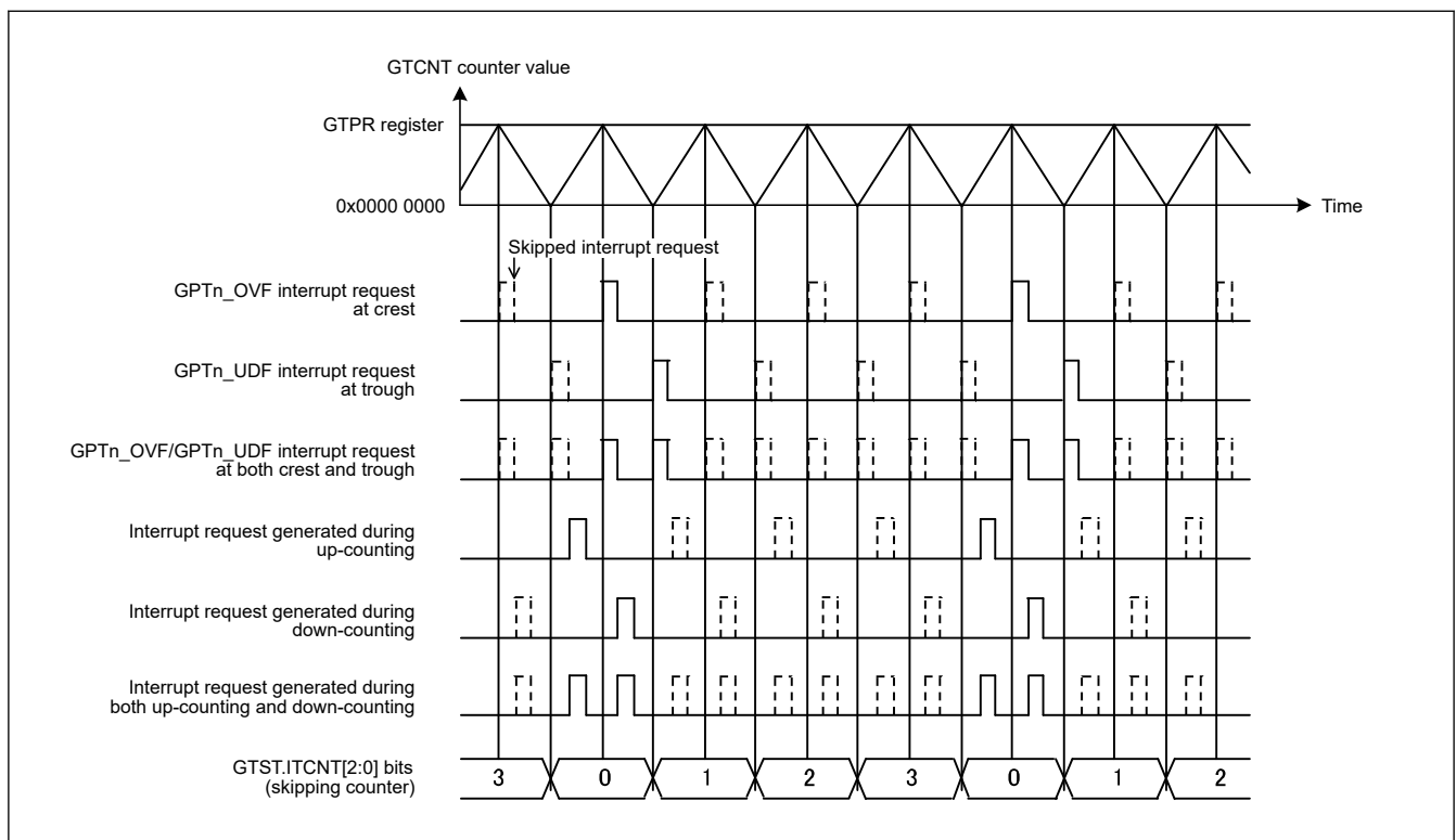
Figure 23.130 Example of Interrupt Skipping Function Operation (Triangle Waves, Counting and Skipping Troughs, Skipping Count: 3)
