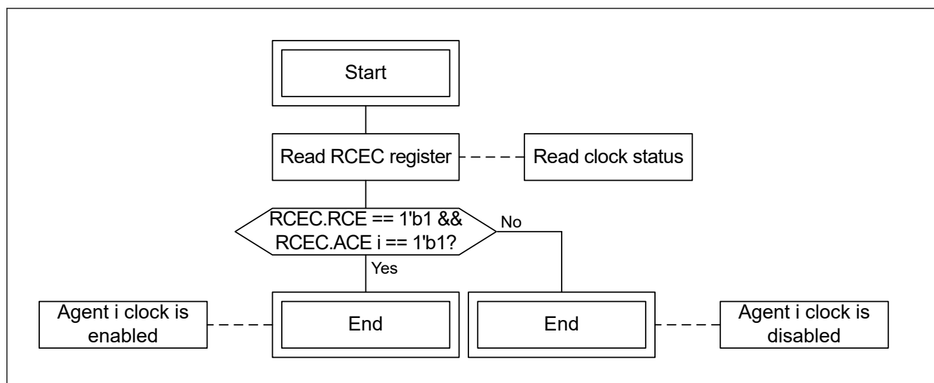
Figure 32.8 Agent i clock status check flow
