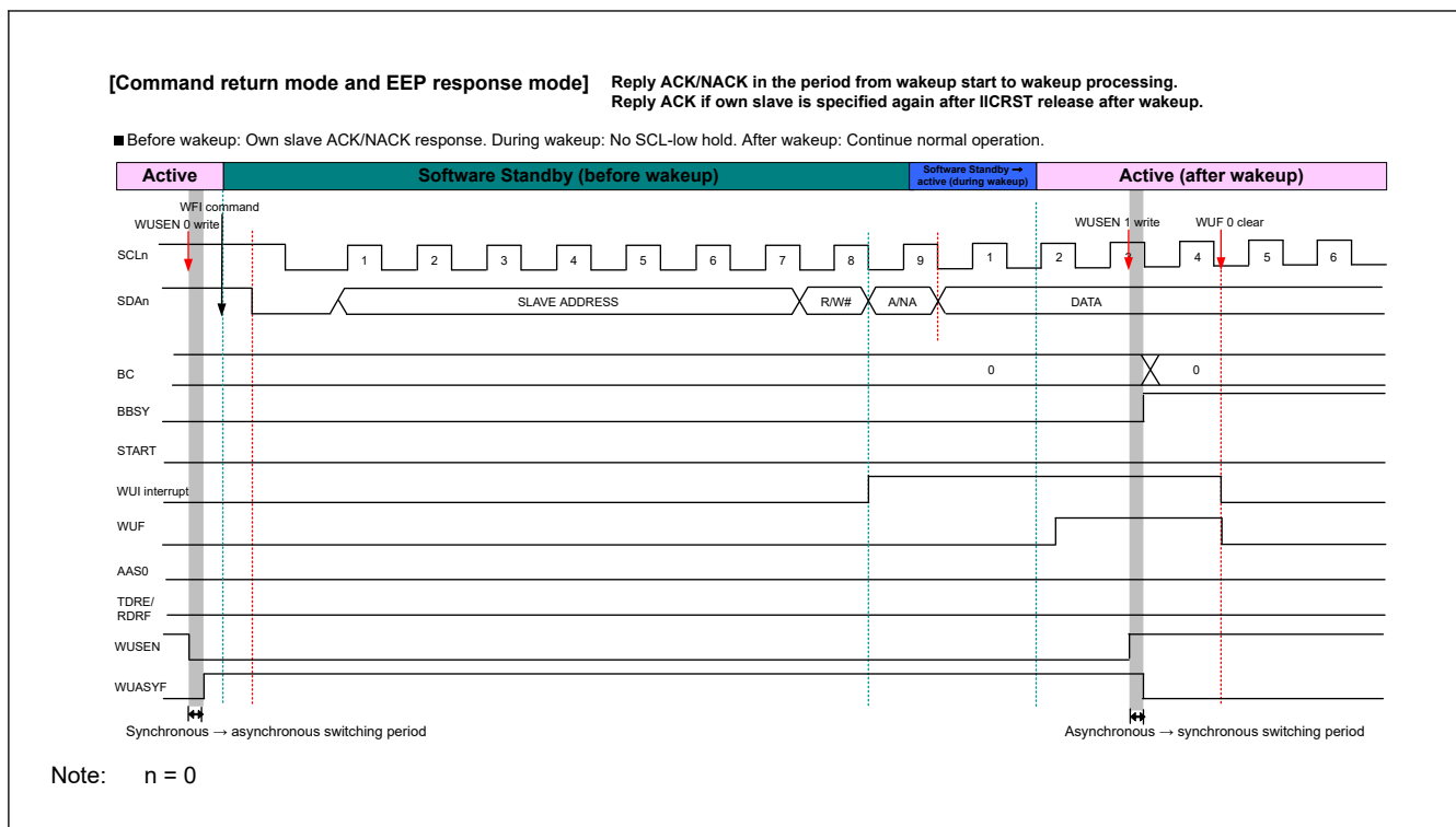
Figure 40.37 Timing of command recovery and EEP response modes
