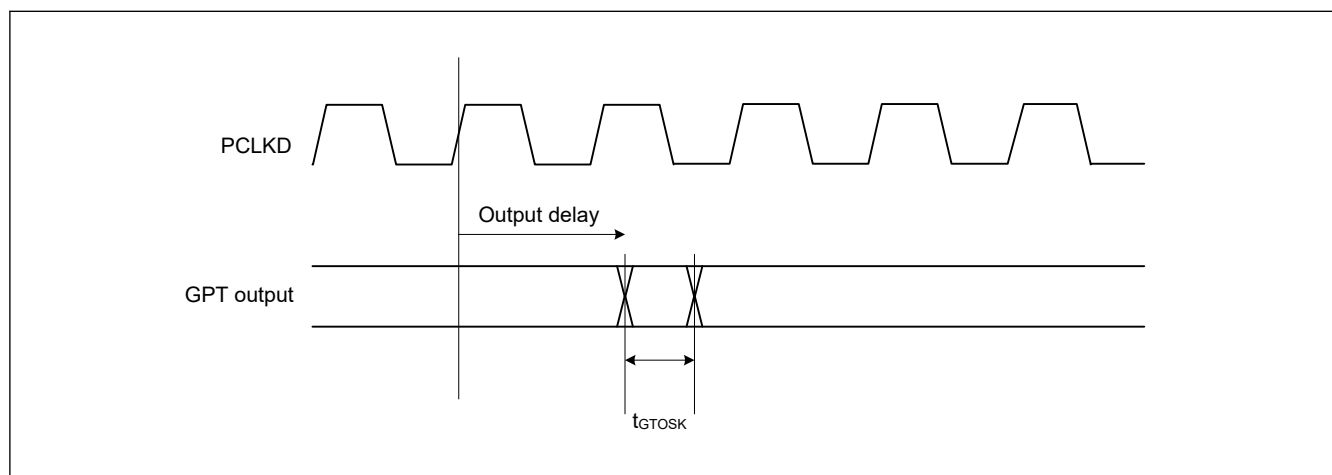
Figure 70.63 GPT output delay skew for OPS
