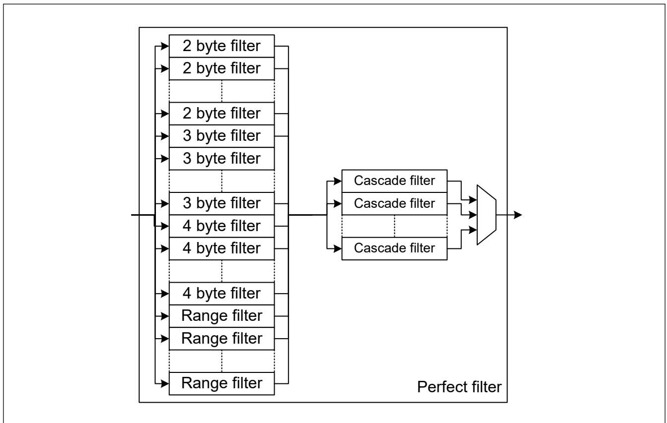
Figure 31.62 Perfect filter block diagram
