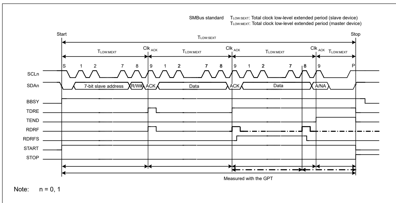
Figure 40.50 SMBus timeout measurement
