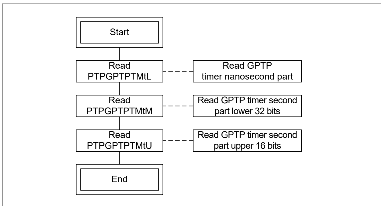
Figure 36.7 GPTP timer t reading flow
