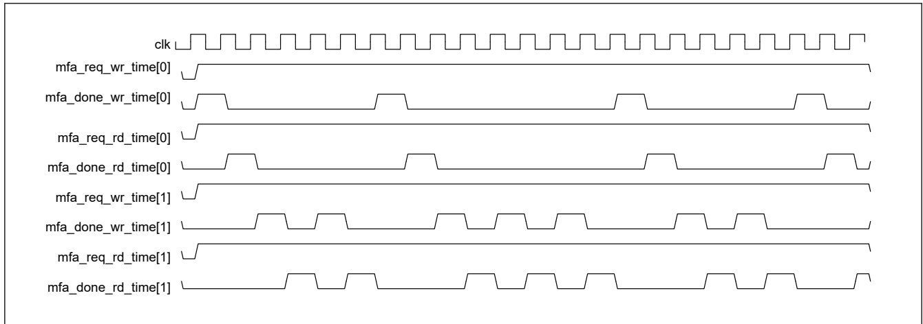
Figure 31.113 Done signal pattern example
