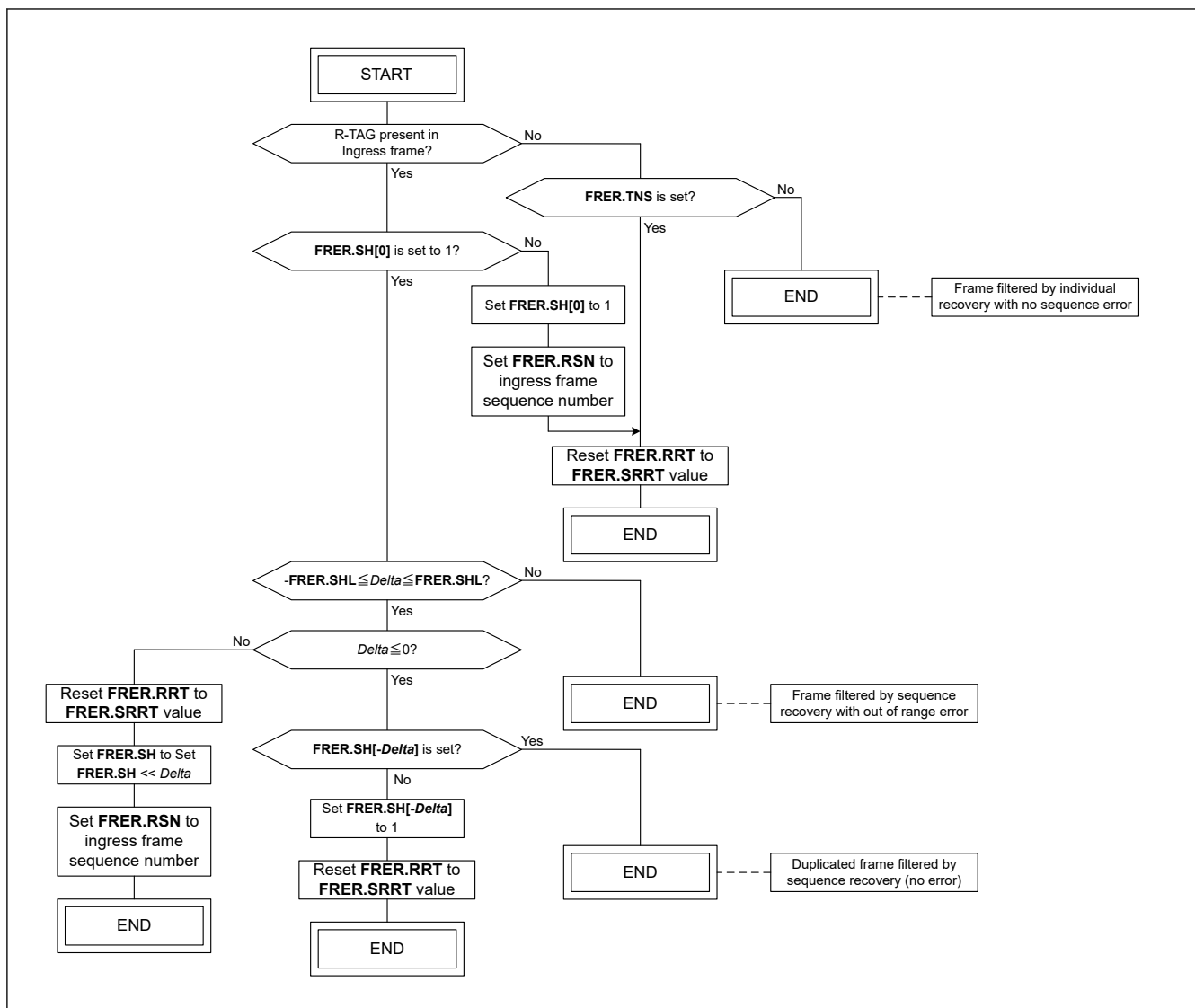
Figure 31.110 Sequence recovery vector algorithm
