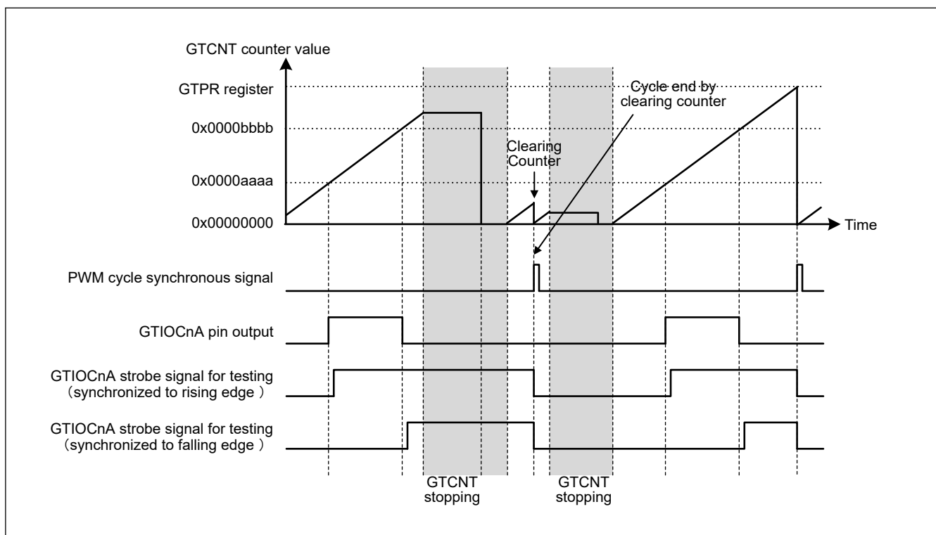
Figure 23.175 Example of output operation to PDG (2)
