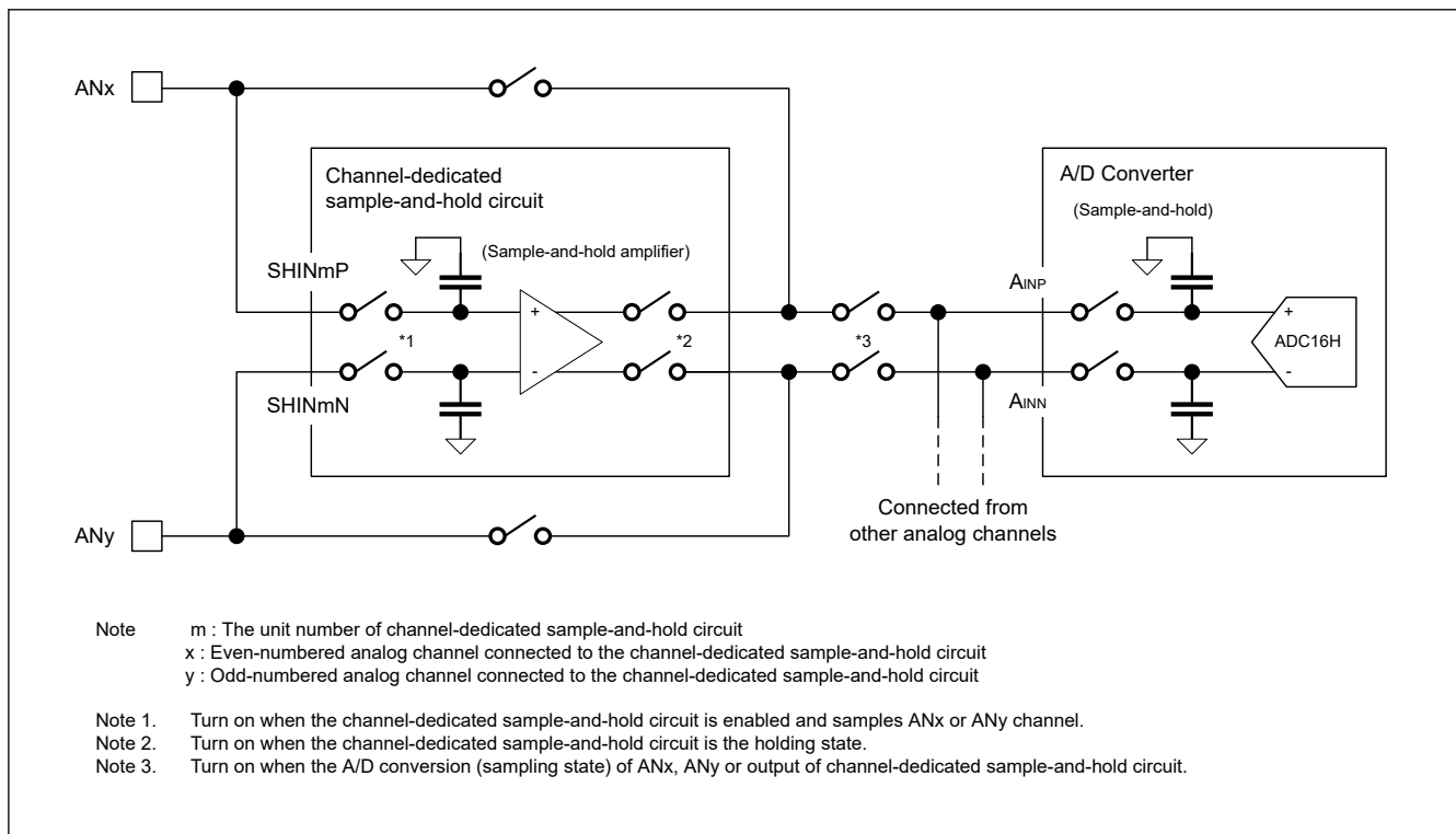
Figure 54.17 Internal configuration of channel-dedicated sample-and-hold circuit in Differential input mode
