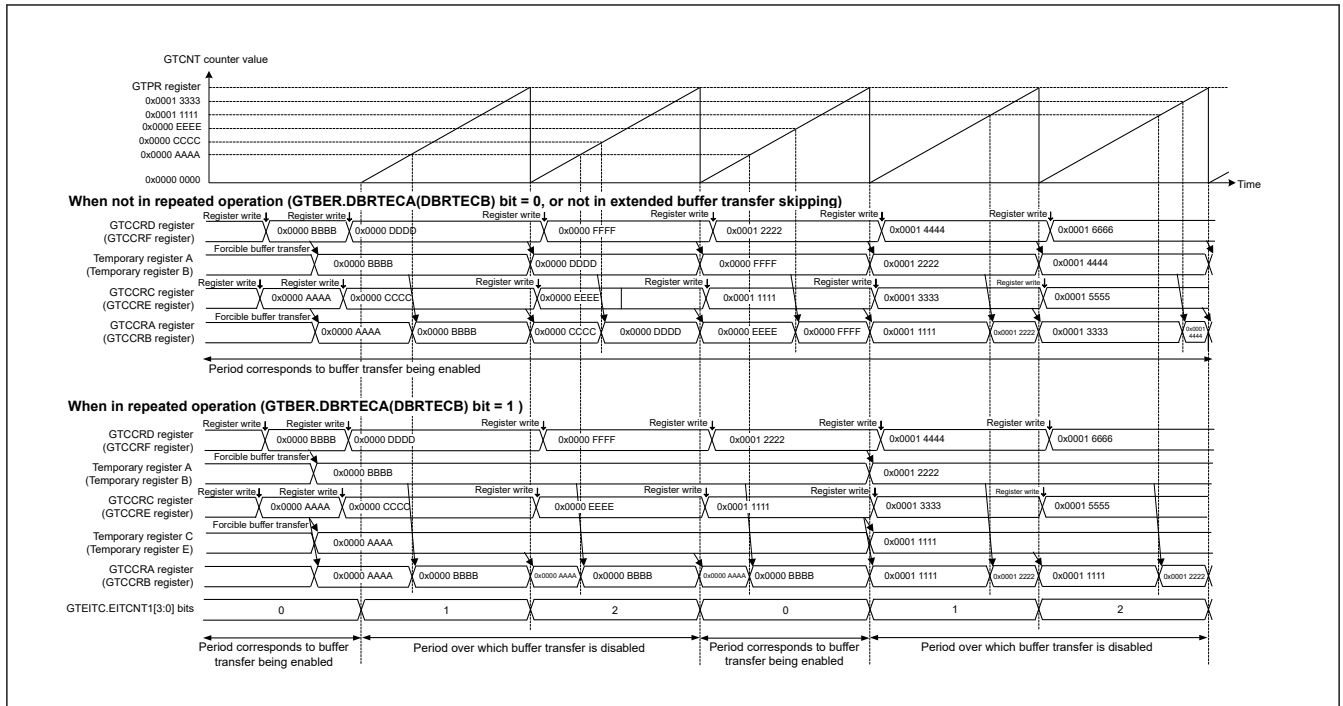
Figure 23.156 Example of Repeated Double-Buffer Operation When GTCCR Buffer Transfer is Disabled (Saw-Wave One-Shot Pulse Mode, Using Extended Buffer Transfer Skipping, GTBER.BD[0] is Constantly 0)
