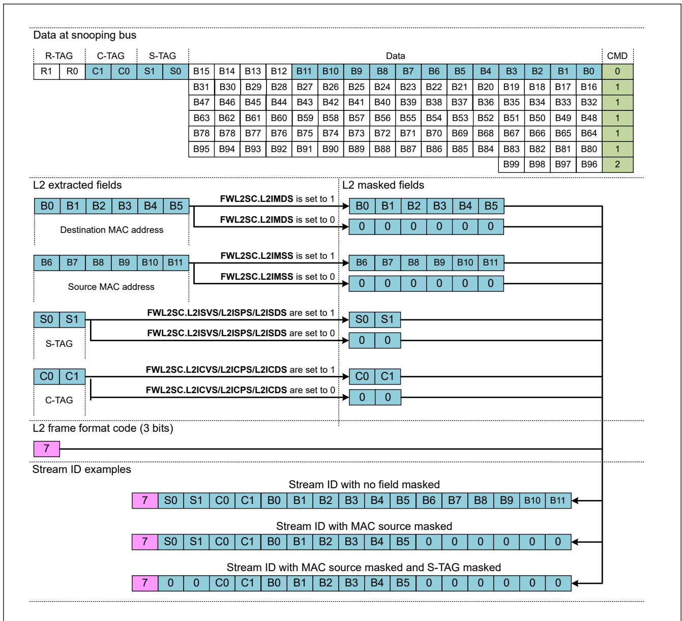
Figure 31.84 L2 stream ID creation
