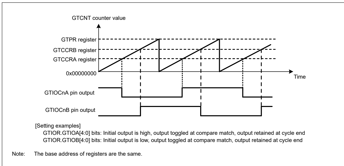
Figure 23.11 Example of toggled output operation (1)
