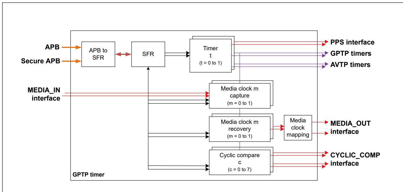
Figure 36.1 GPTP block diagram
