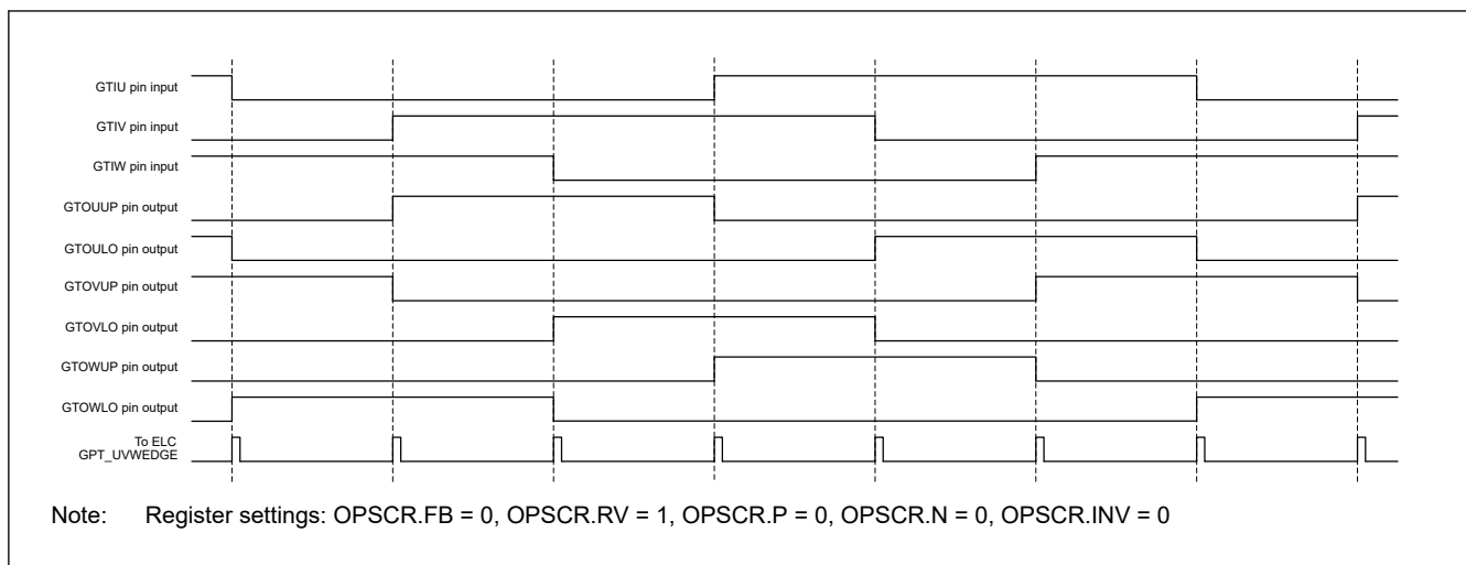
Figure 23.123 Example of GPT_OPS Level Output Operation (Reverse Rotation)
