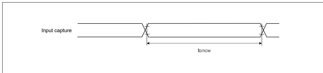
Figure 70.61 GPT input capture timing
