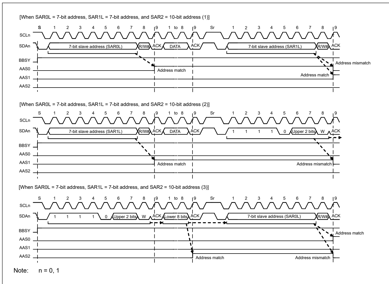
Figure 40.26 AASy flag set and clear timing with mixed 7-bit and 10-bit address formats
