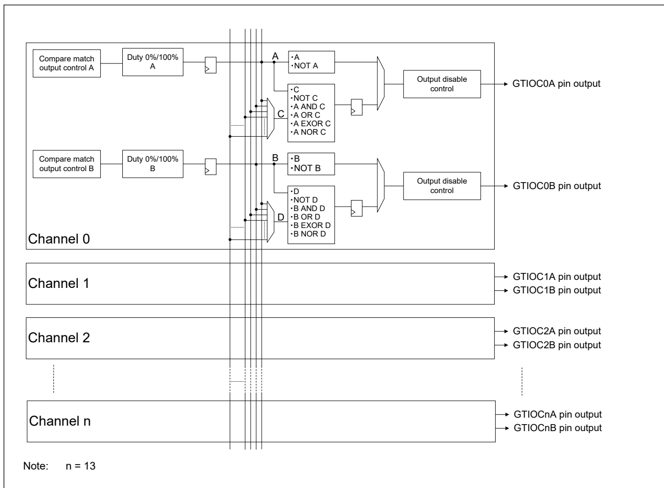
Figure 23.127 Block Diagram of Inter Channel Logical Operation
