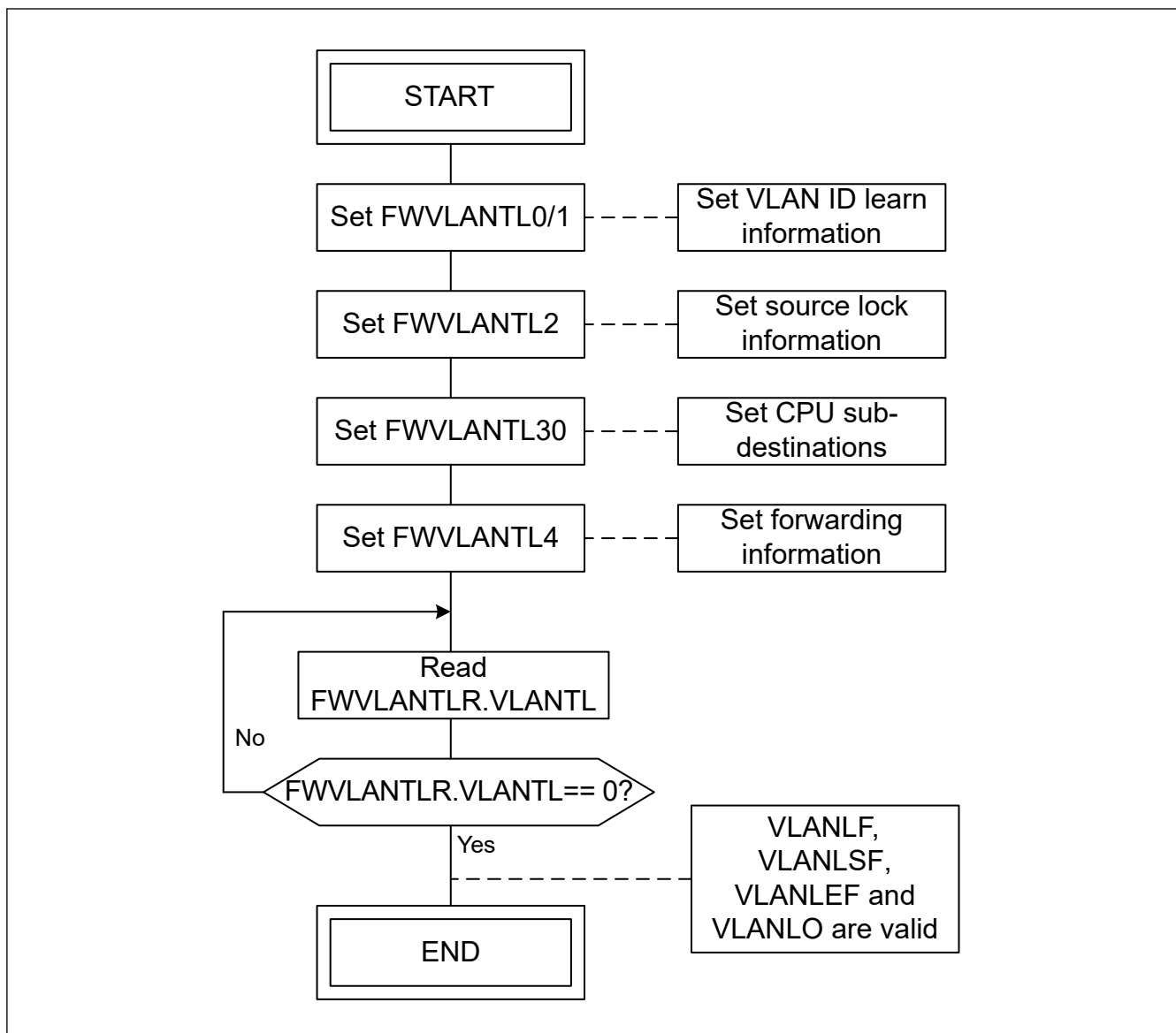
Figure 31.18 VLAN entry learn flow
