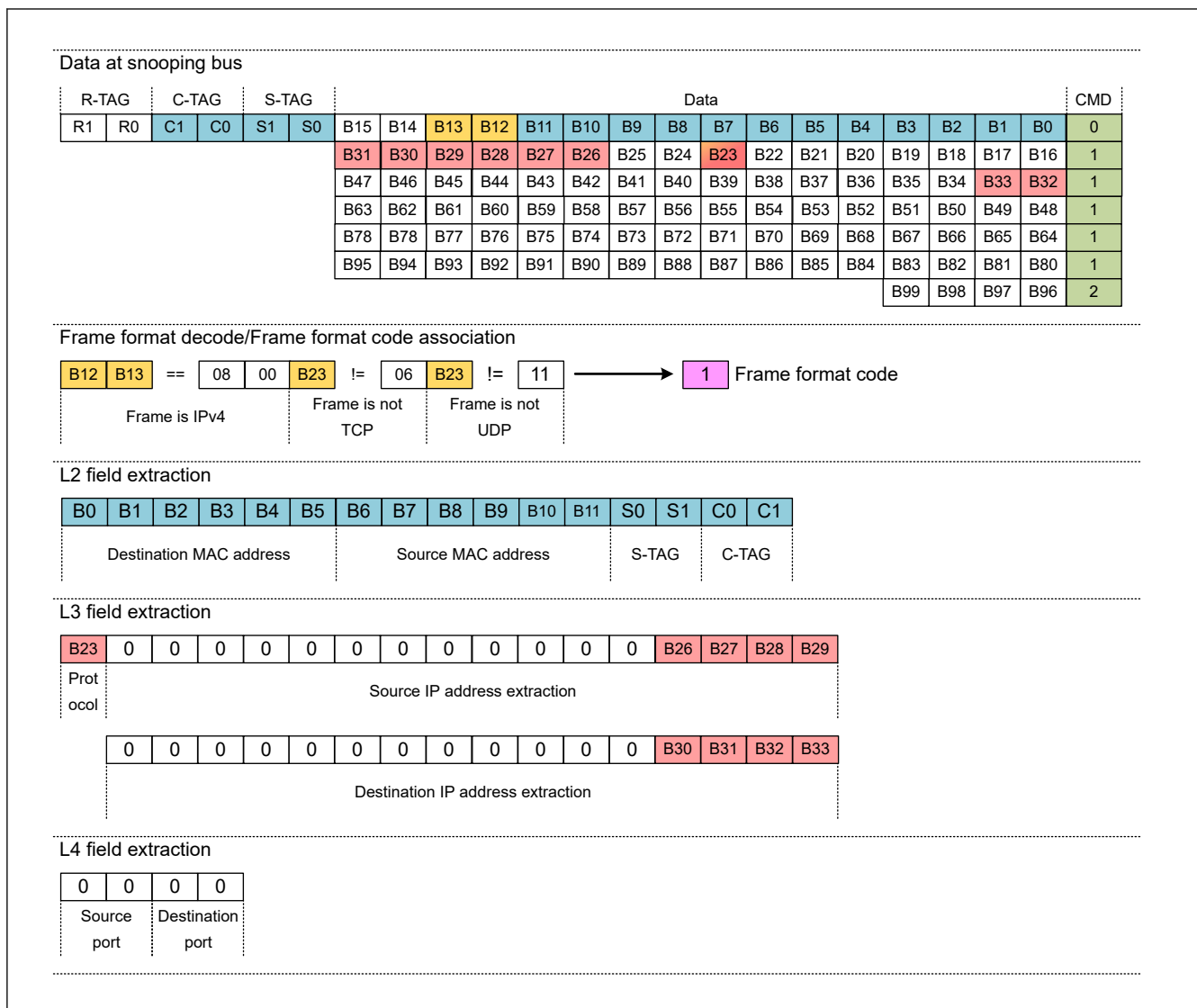
Figure 31.73 IPv4 detection and data extraction
