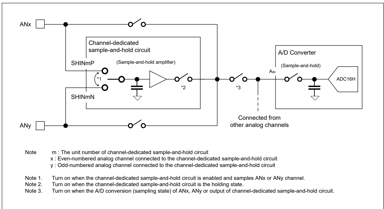
Figure 54.16 Internal configuration of channel-dedicated sample-and-hold circuit in Single-ended input mode
