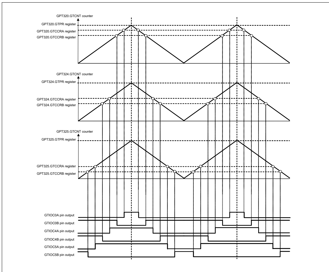
Figure 23.104 Example of 3-phase triangle-wave complementary PWM output
