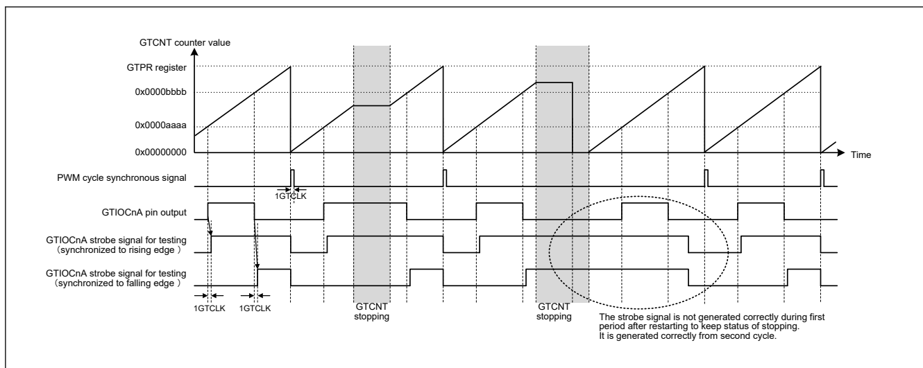
Figure 23.174 Example of output operation to PDG (1)
