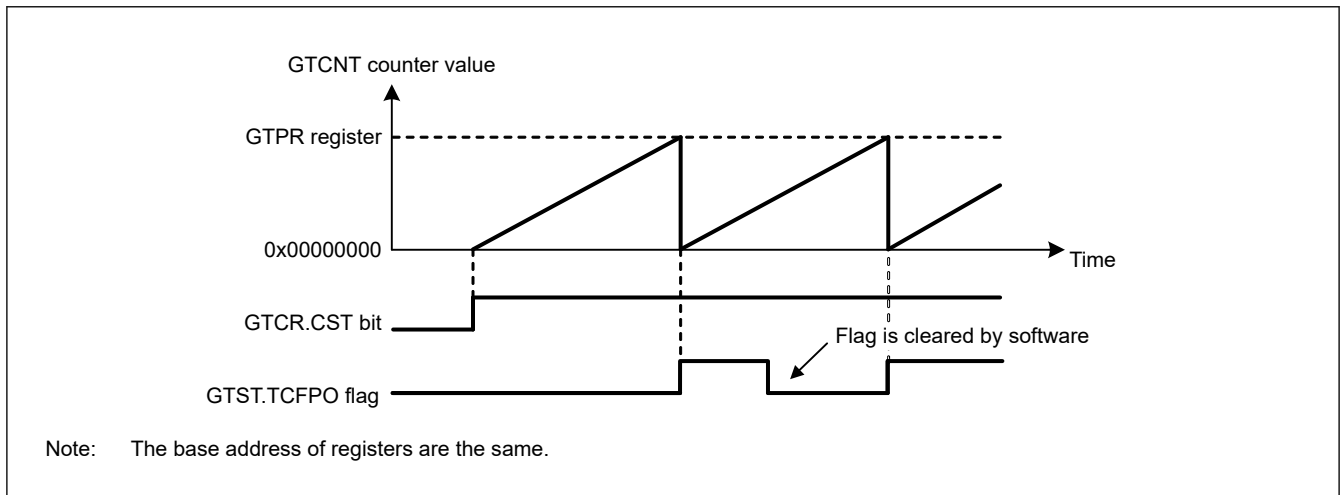
Figure 23.5 Example of periodic count operation in up-counting by the count clock
