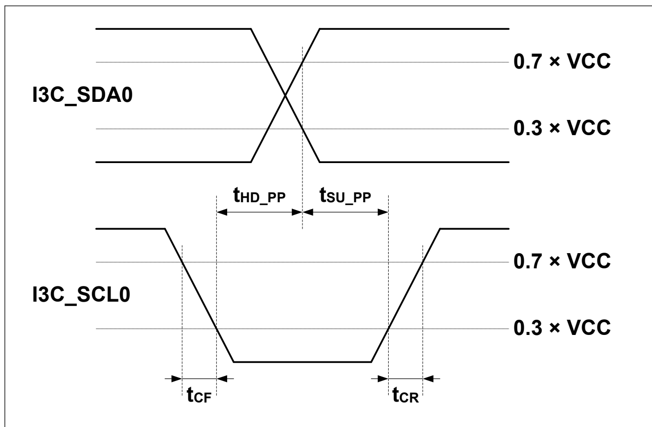
Figure 70.95 I3C Master Out Timing
