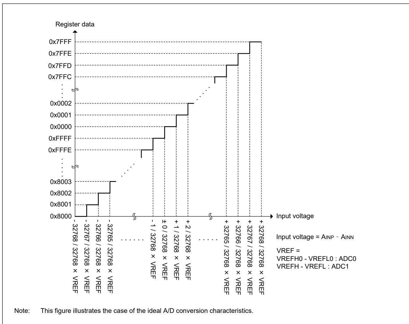
Figure 54.43 Data range of A/D conversion result (16-bit data length, Signed data, Differential input)
