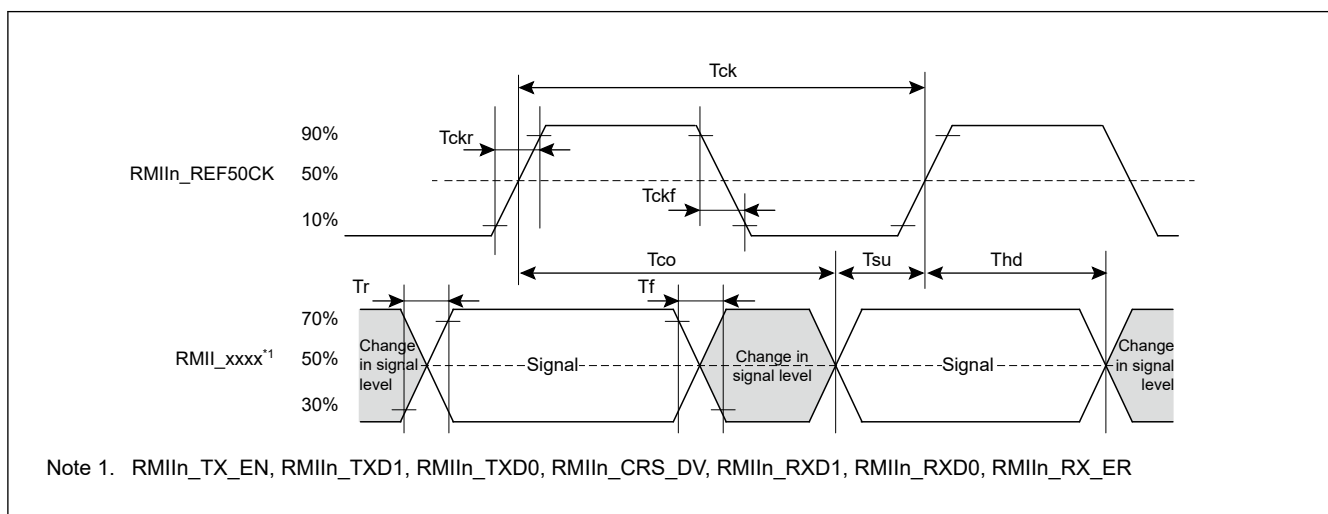
Figure 70.115 RMIIIn_REF50CK and RMII signal timing
