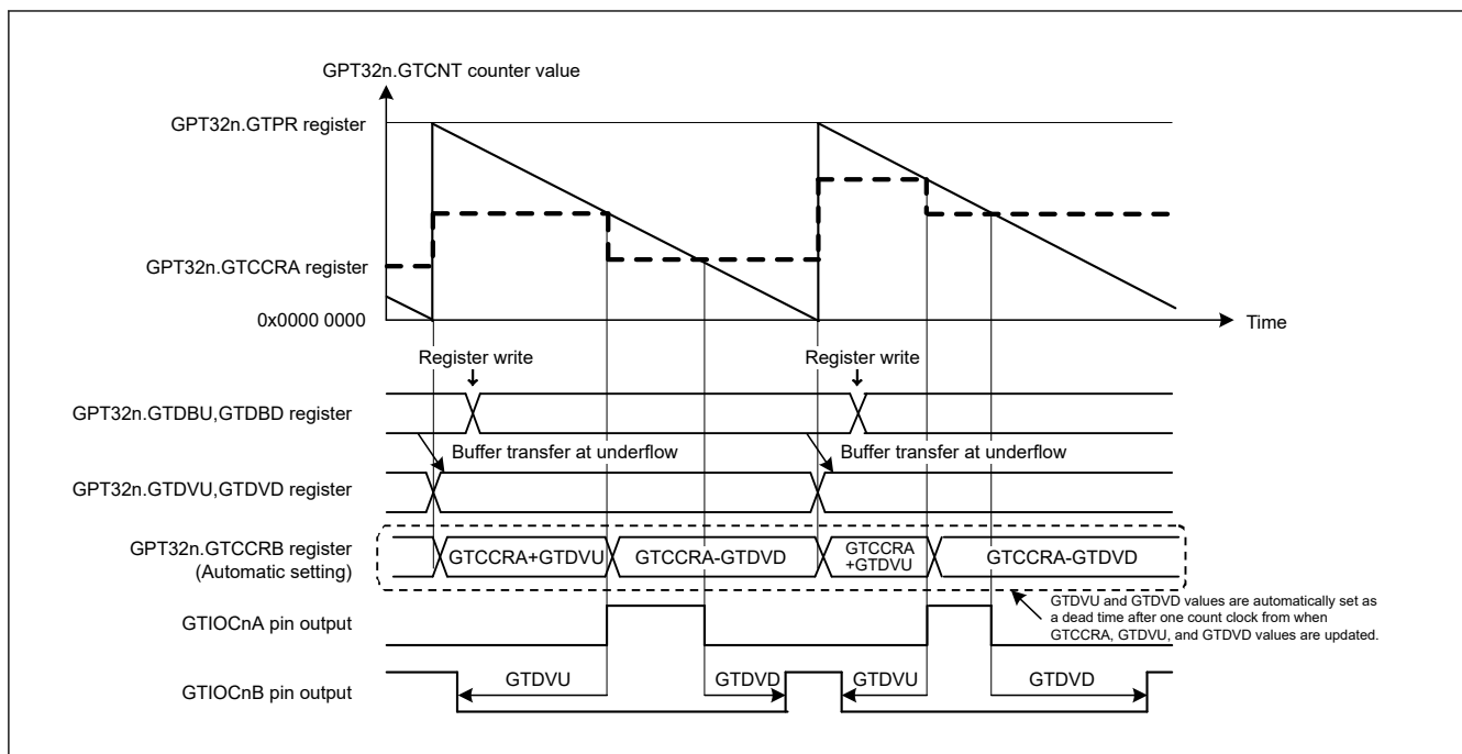
Figure 23.78 Example of automatic dead time setting function operation in saw-wave one-shot pulse mode, down-counting, GTDVU and GTDVD set to buffer operation, and active-high
