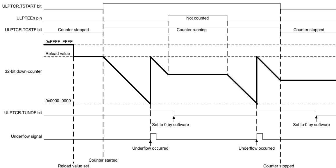
Figure 26.5 Operation example 1 in event counter, continuous, and count enable modes (with the ULPTIOC.TIOGT0 bit set to 1)
