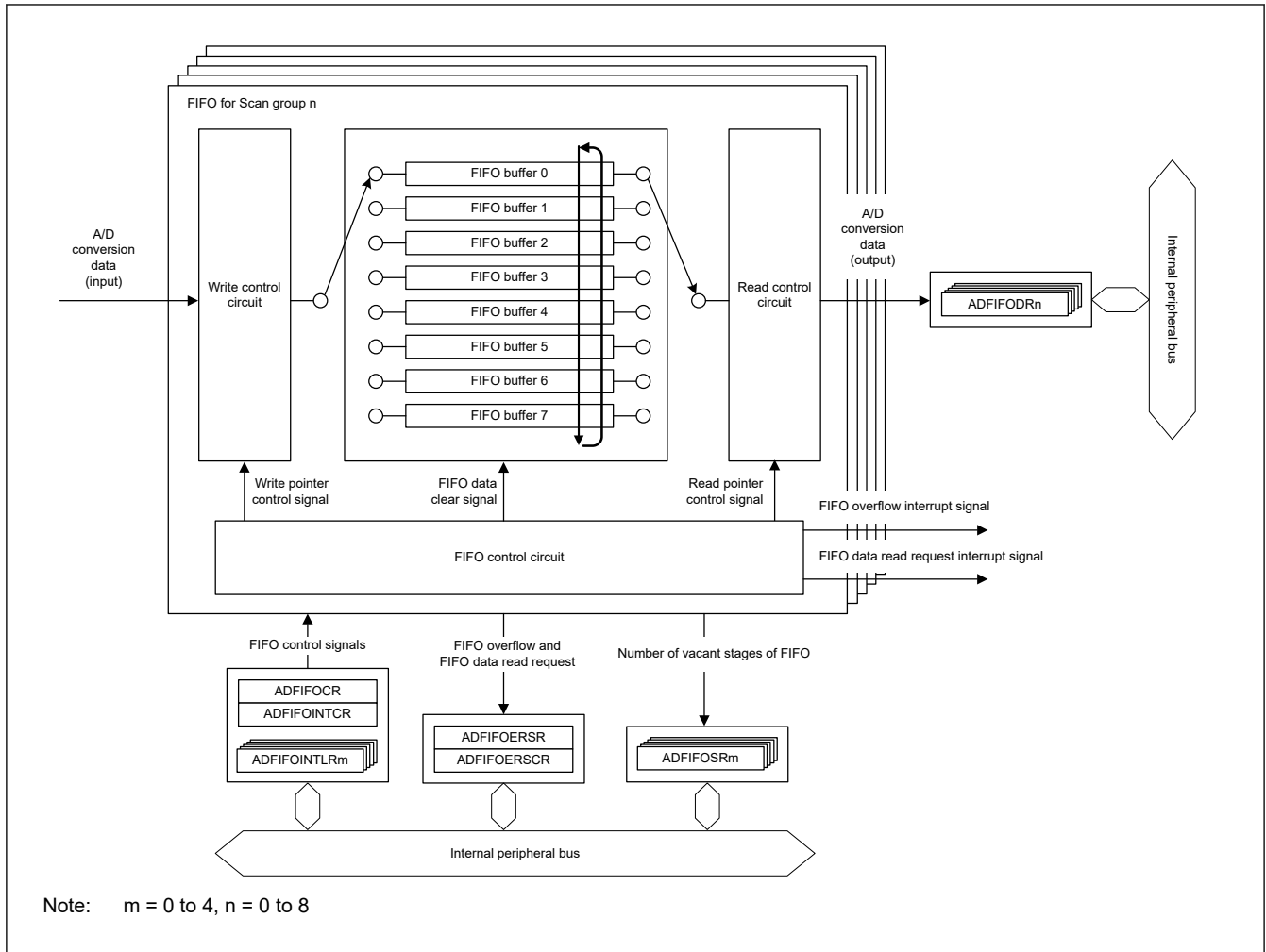
Figure 54.53 The block diagram of FIFO
