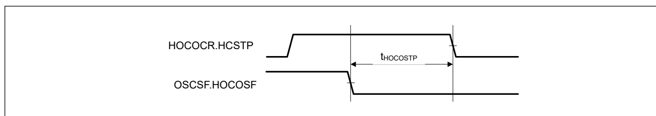
Figure 70.31 HOCO stop width time
