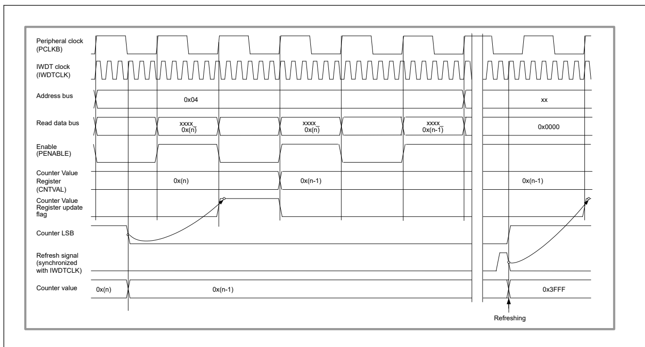
Figure 29.9 Processing for reading IWDT counter value when IWDTCR.CKS[3:0] = 0010b and IWDTCR.TOPS[1:0] = 11b
