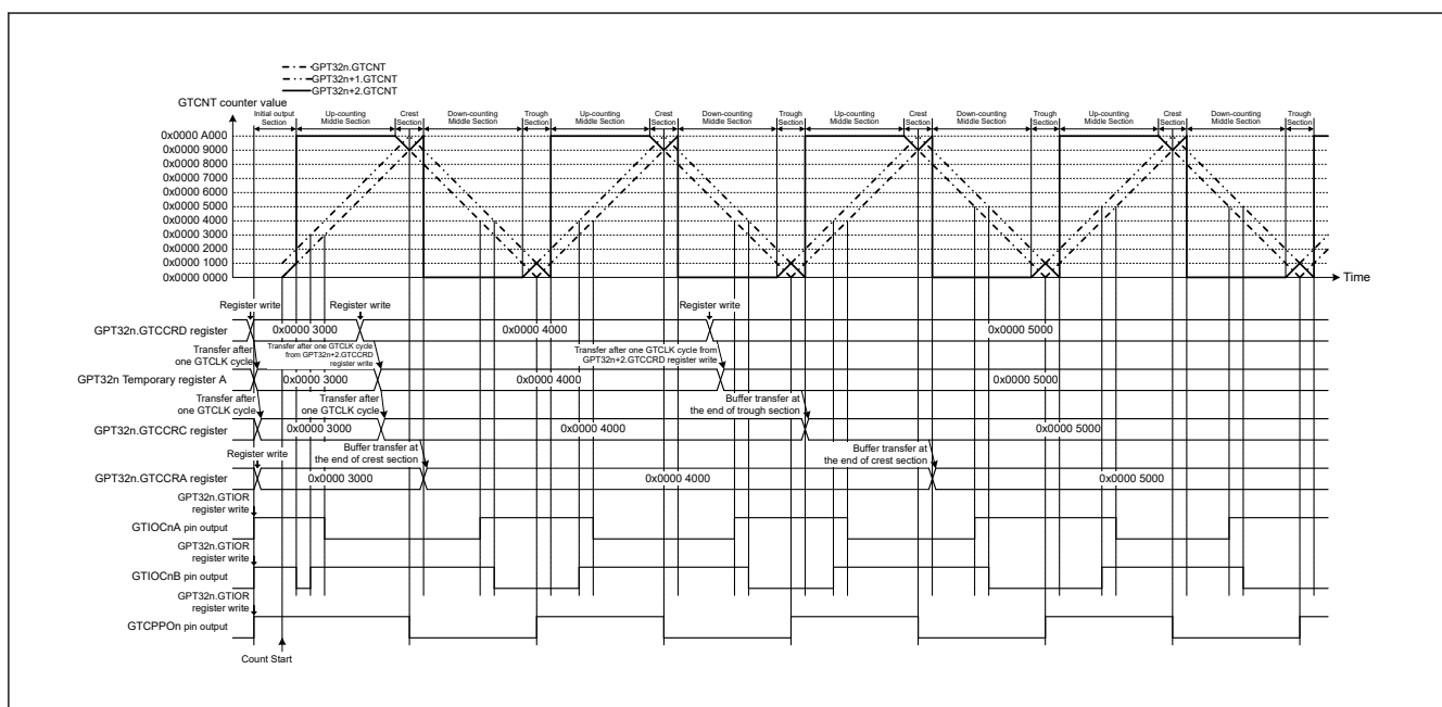
Figure 23.45 Example of Complementary PWM Mode 1 Operation (GTIOChA pin = High / GTIOChB pin = High as initial output, GTIOChA pin = Low / GTIOChB pin = High at GTCCRA register compare match during up-counting, GTIOChA pin = High / GTIOChB pin = Low at GTCCRA register compare match during down-counting, the dead time value is 0x0000 1000 and updating GTCCRD register in middle section) (n = 4, 7)
