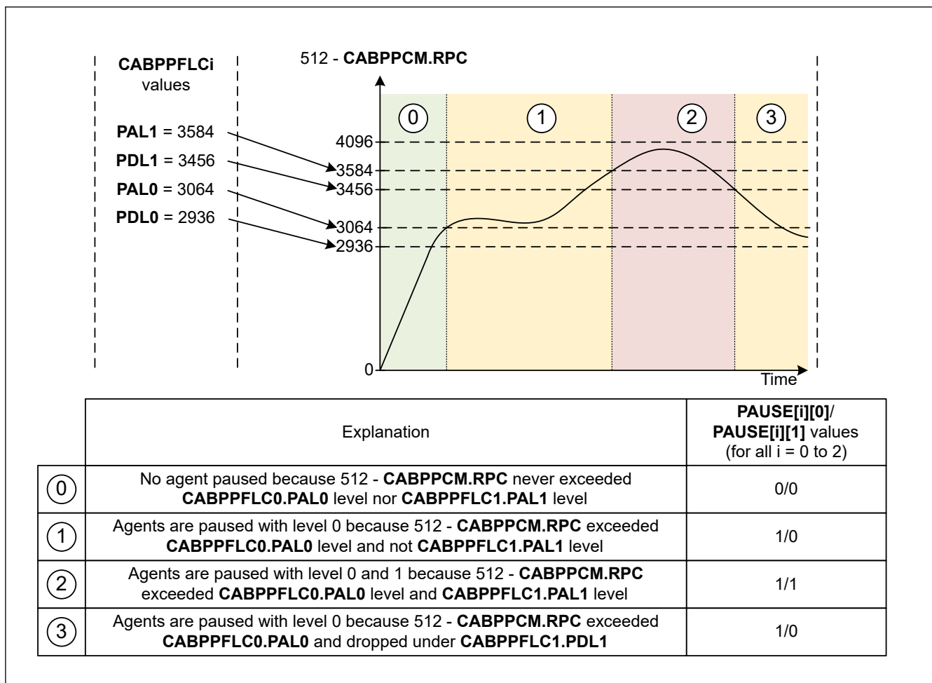
Figure 32.14 Example for global pause function setting
