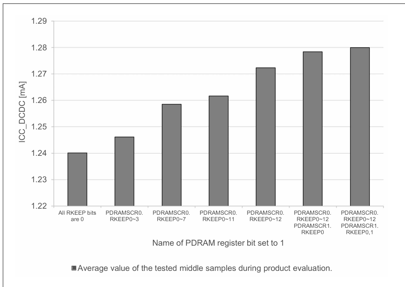
Figure 70.14 Software Standby current per SRAM state (ICC_DCDC, SS2LP_0, SVSCR_5) (reference data)
