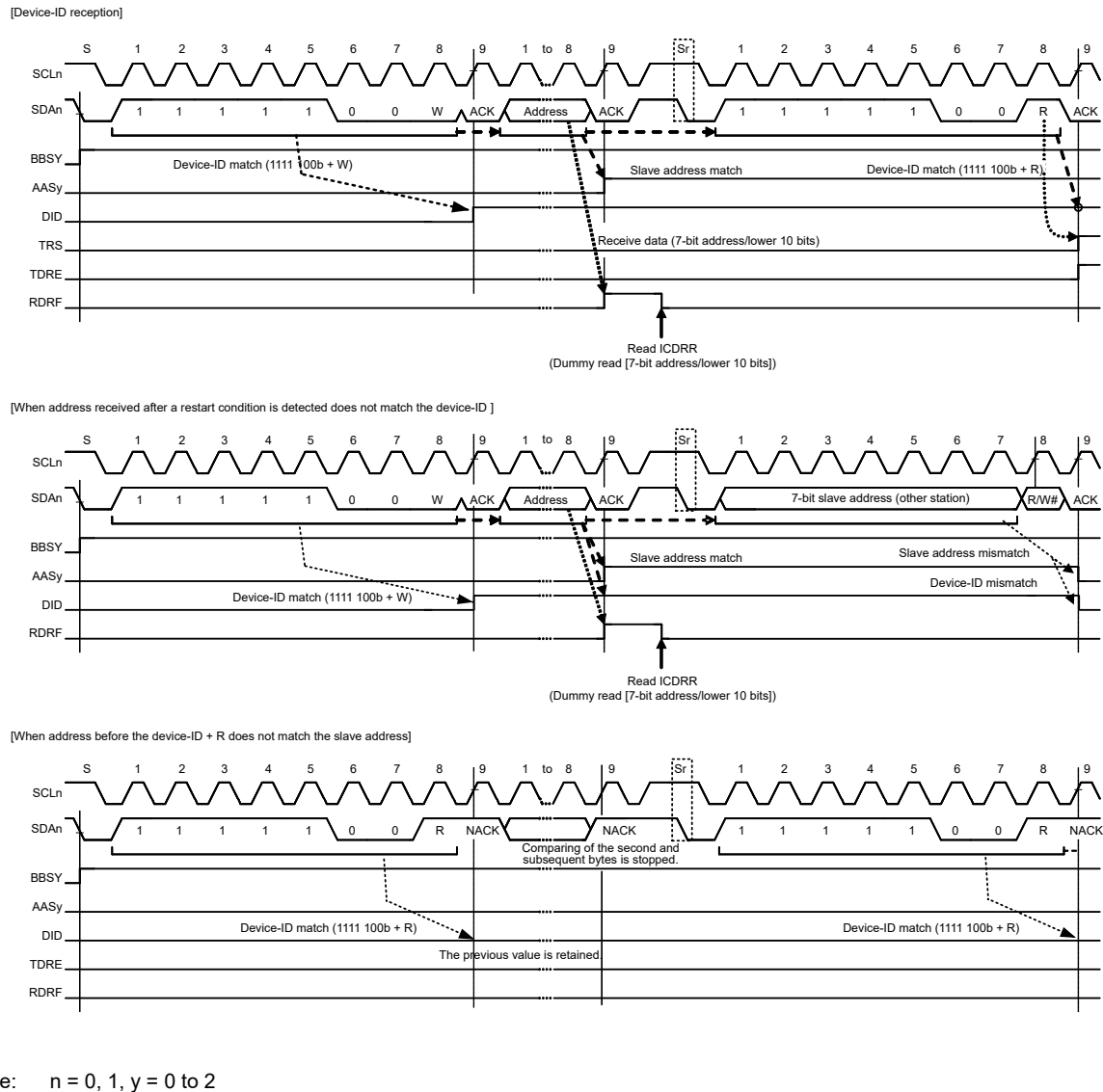
Figure 40.28 AASy and DID flag set and clear timing during reception of device ID
