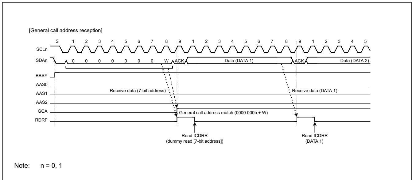
Figure 40.27 Timing of GCA flag setting during reception of general call address
