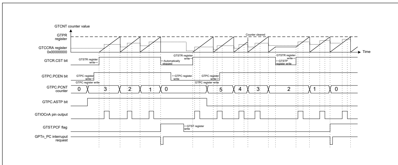
Figure 23.107 Example of PWM cycle count function (saw-wave one-shot pulse mode)
