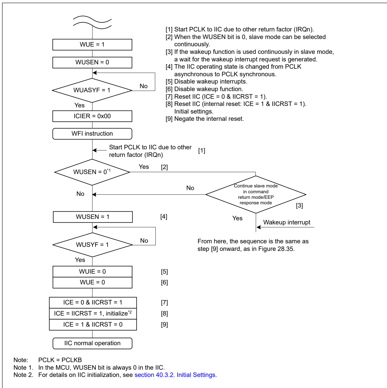
Figure 40.36 Example operation of command recovery and EEP response modes when wakeup is triggered by an interrupt other than IIC wakeup interrupt, for example, the IRQn
