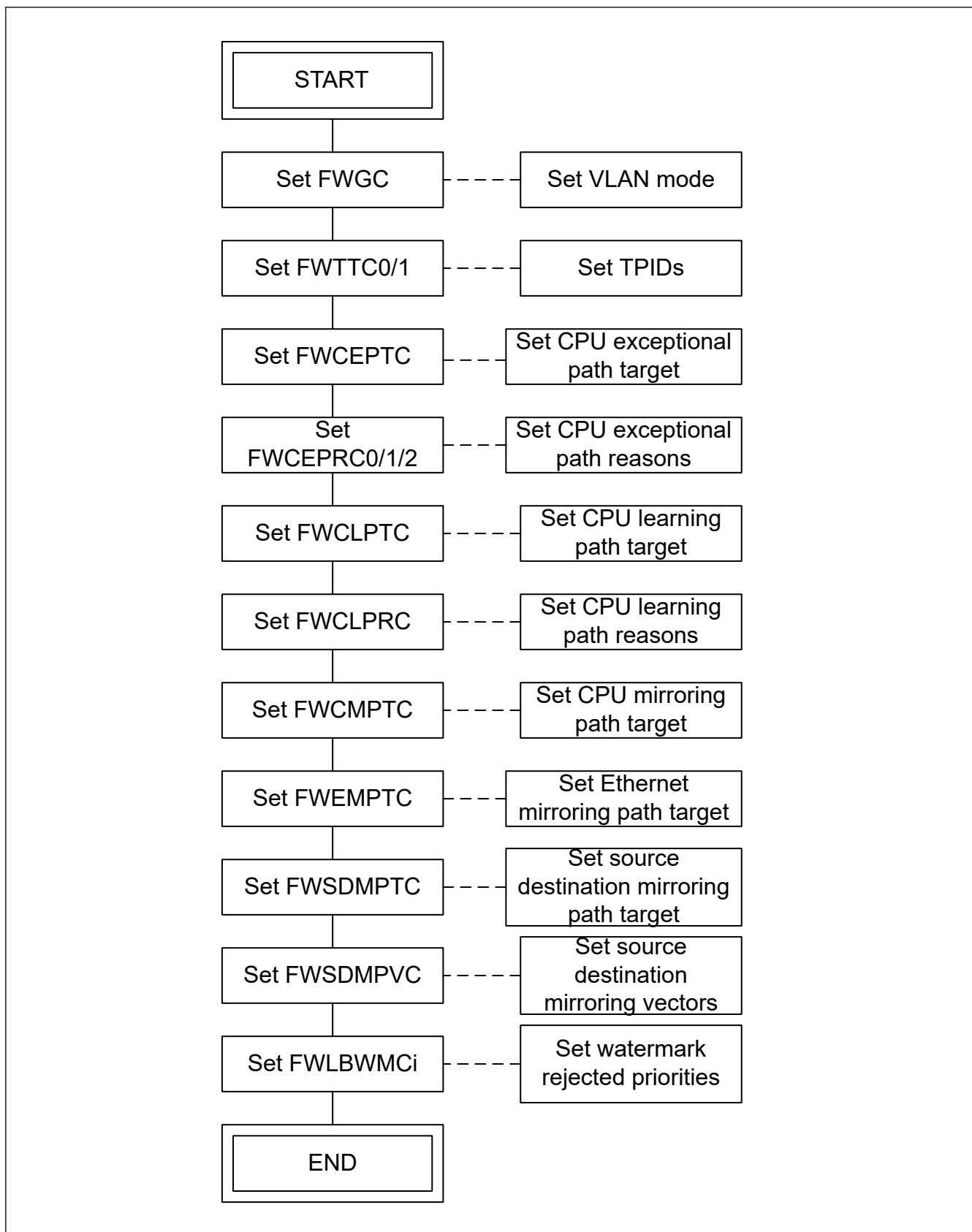
Figure 31.34 Setting flow of general function
