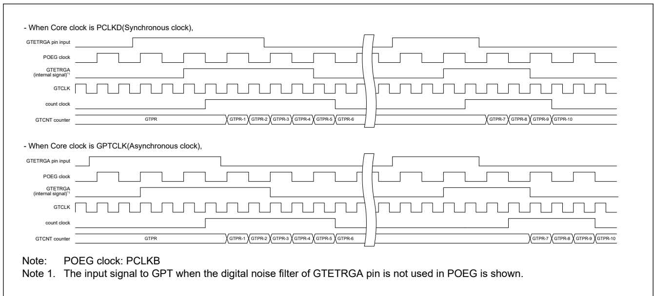
Figure 23.120 Example of External pulse width measuring function(Down-counting)
