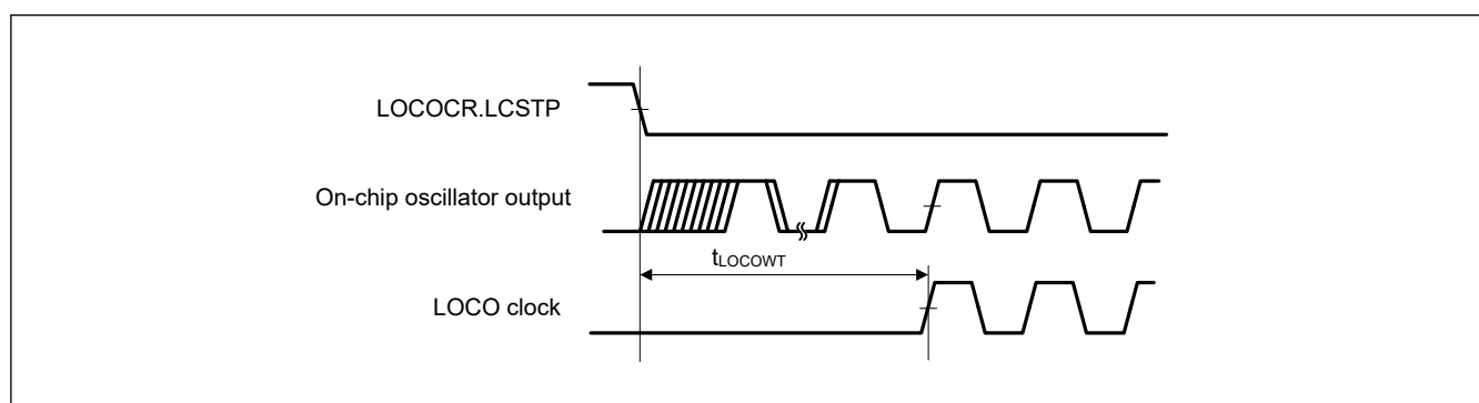
Figure 70.28 LOCO clock oscillation start timing
