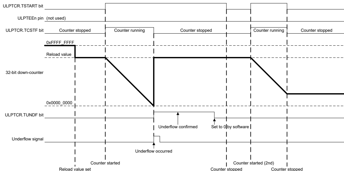
Figure 26.7 Operation example in event counter, one-shot, and count enable modes (with the ULPTIOC.TIOGT0 bit set to 0)
