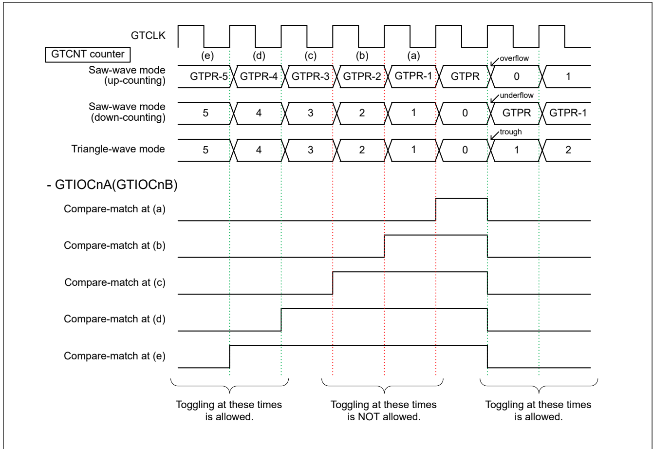
Figure 23.173 Example of unacceptable GTIOCnm signal timing (n = 0 to 3, m = A, B)
