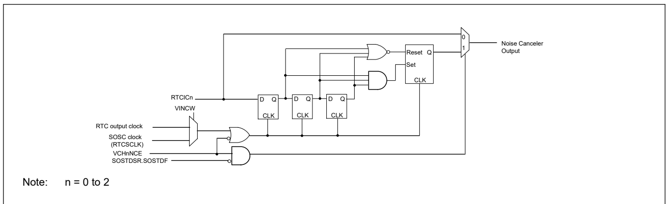
Figure 12.5 Noise canceler circuit block diagram
