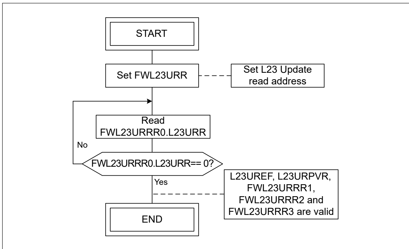
Figure 31.26 Read flow of Layer 2/Layer 3 Update rule
