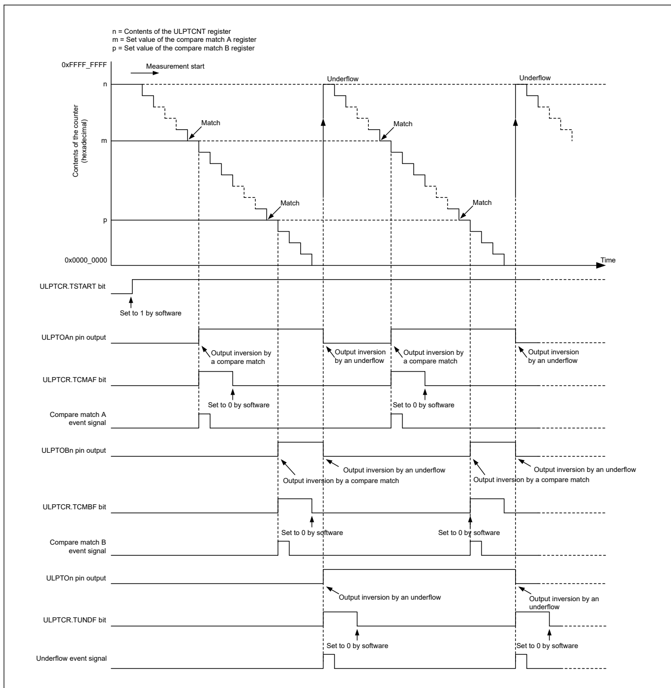
Figure 26.18 Operation example of the compare match function (both the TOPOLA and TOPOLB bits of the ULPTCMSR register are set to 0)
