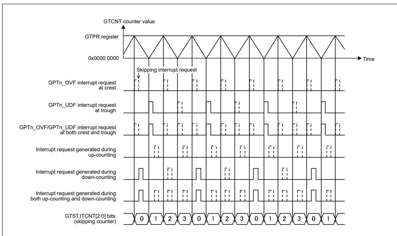
Figure 23.132 Example of Interrupt Skipping Function Operation (Triangle Waves, Counting and Skipping Both Troughs and Crests, Skipping Count: 3, Skipping Started at Up-Counting)
