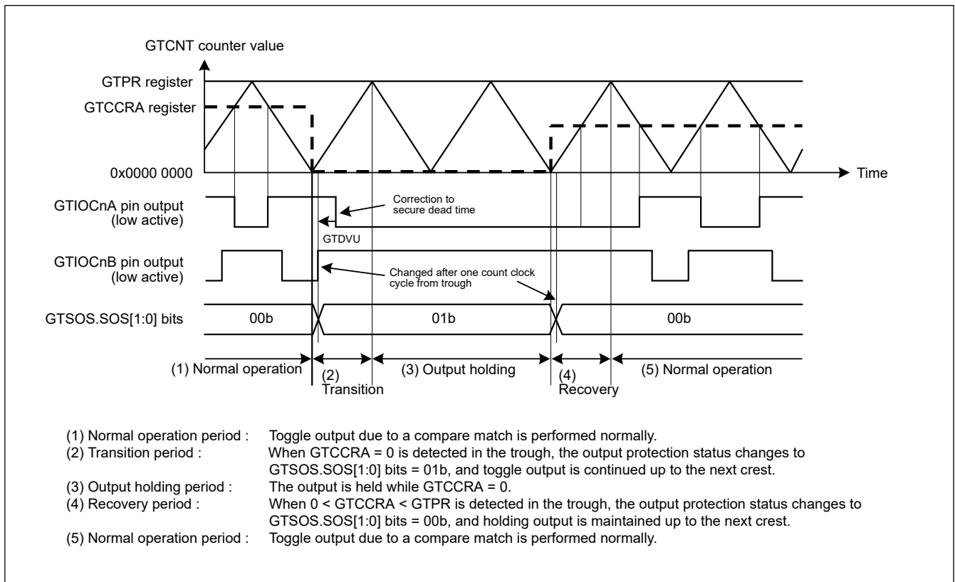
Figure 23.162 Example of Output Protection Function Operation When GTCCRA is Set to 0x0000 0000 during Buffer Transfer at Troughs (Restored to 0 < GTCCRA < GTPR during Buffer Transfer at Troughs, Active Level: Low) (n = 0 to 13)
