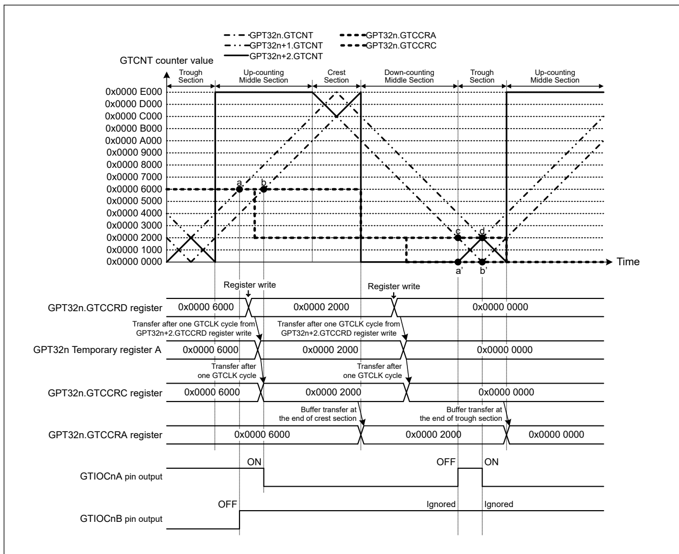
Figure 23.62 Example of Compare Match Generation Sequence Operation in Complementary PWM Mode (Complementary PWM mode 3 single buffer operation, GTIOCnA pin = Low / GTIOCnB pin = High at GTCCRA register compare match during up-counting, GTIOCnA pin = High / GTIOCnB pin = Low at GTCCRA register compare match during down-counting, the dead time value is 0x0000 2000, compare match generation order: (c, a') → (d, b')) (n = 4, 7)
