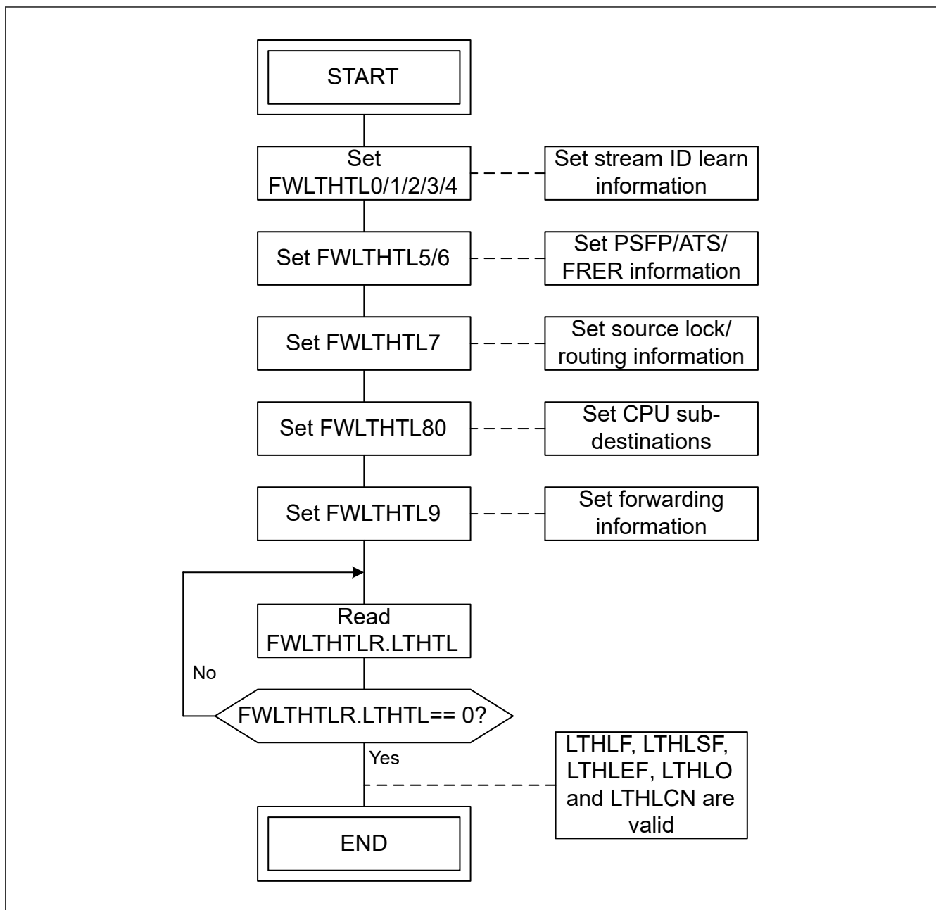
Figure 31.12 Layer 3 entry learn flow
