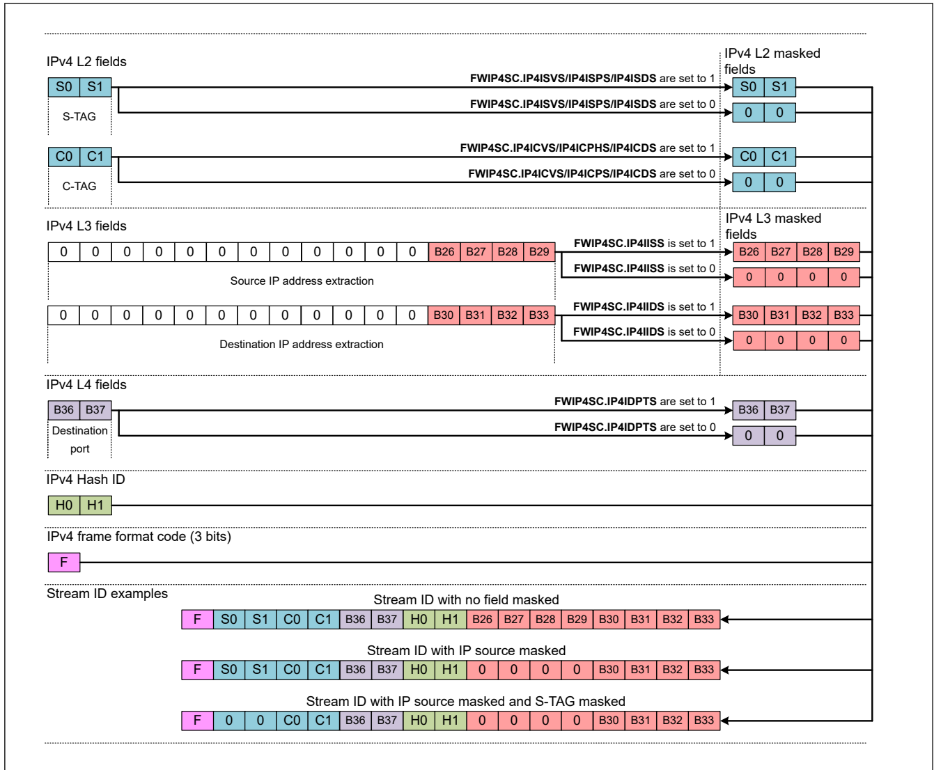
Figure 31.81 IPv4 Stream ID creation
