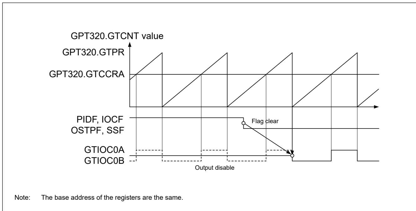
Figure 22.3 Output-disable release timing for GPT pin outputs
