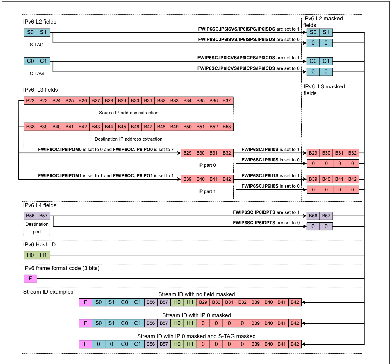
Figure 31.82 IPv6 Stream ID creation
