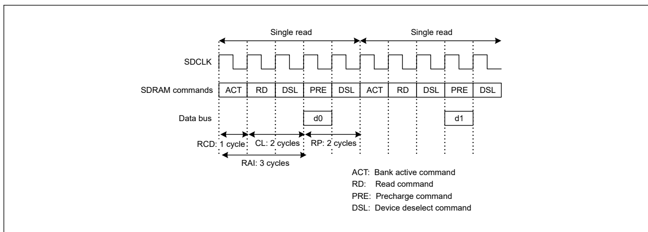
Figure 15.51 Example timing for single read (1)
