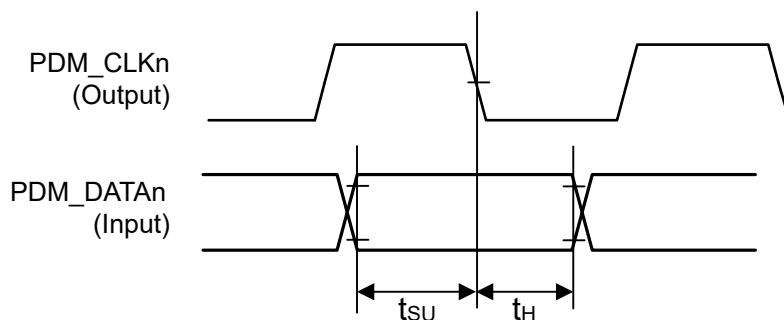
Figure 70.125 Receive Timing (Synchronized with the fall of PDM_CLKn)
