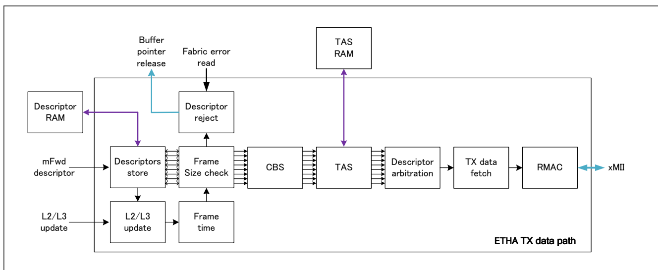
Figure 33.18 ETHA TX data path block diagram
