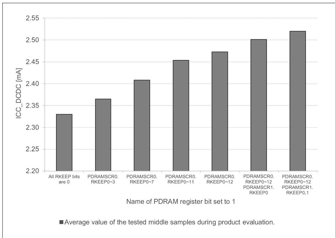
Figure 70.11 Software Standby current per SRAM state (ICC_DCDC, SS2LP_0, SVSCR_2) (reference data)
