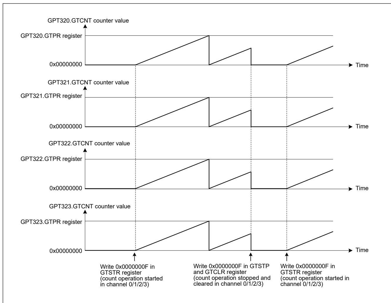
Figure 23.93 Example of a simultaneous start, stop, and clear by software with the same count cycle (GTPR register value)
