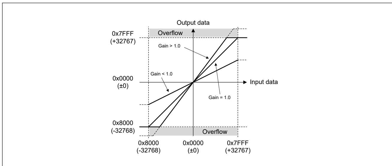
Figure 54.37 User's Gain Adjustment (16-bit data length format and Signed data format)
