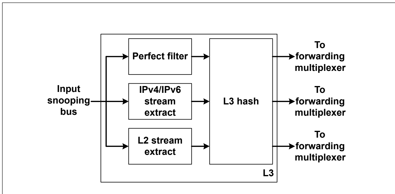
Figure 31.61 Block diagram of Layer 3 forwarding/routing/filtering
