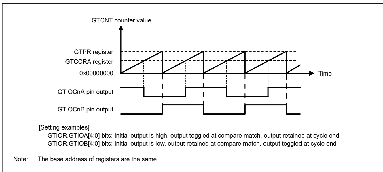
Figure 23.12 Example of toggled output operation (2)
