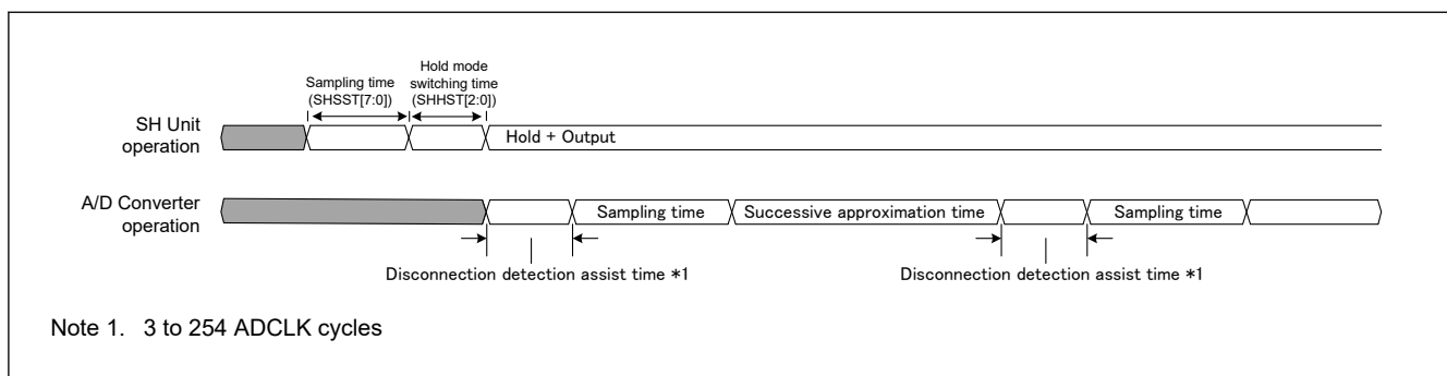
Figure 54.25 Operation of A/D conversion when the disconnection detection assist function and channel-dedicated sample-and-hold circuit are used
