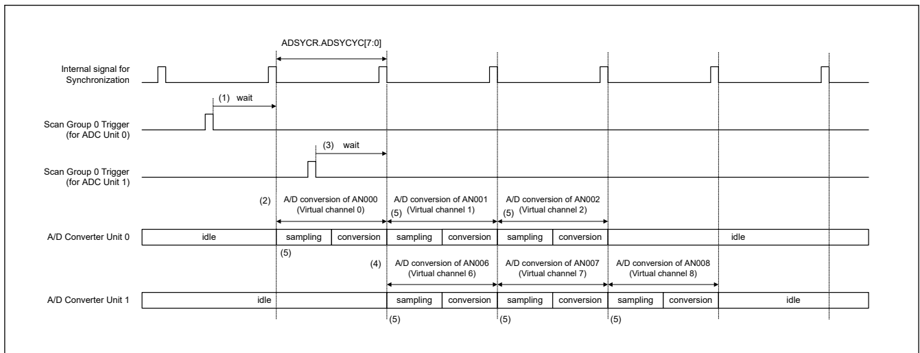
Figure 54.31 Example of synchronous operation in SAR mode – Single scan mode
