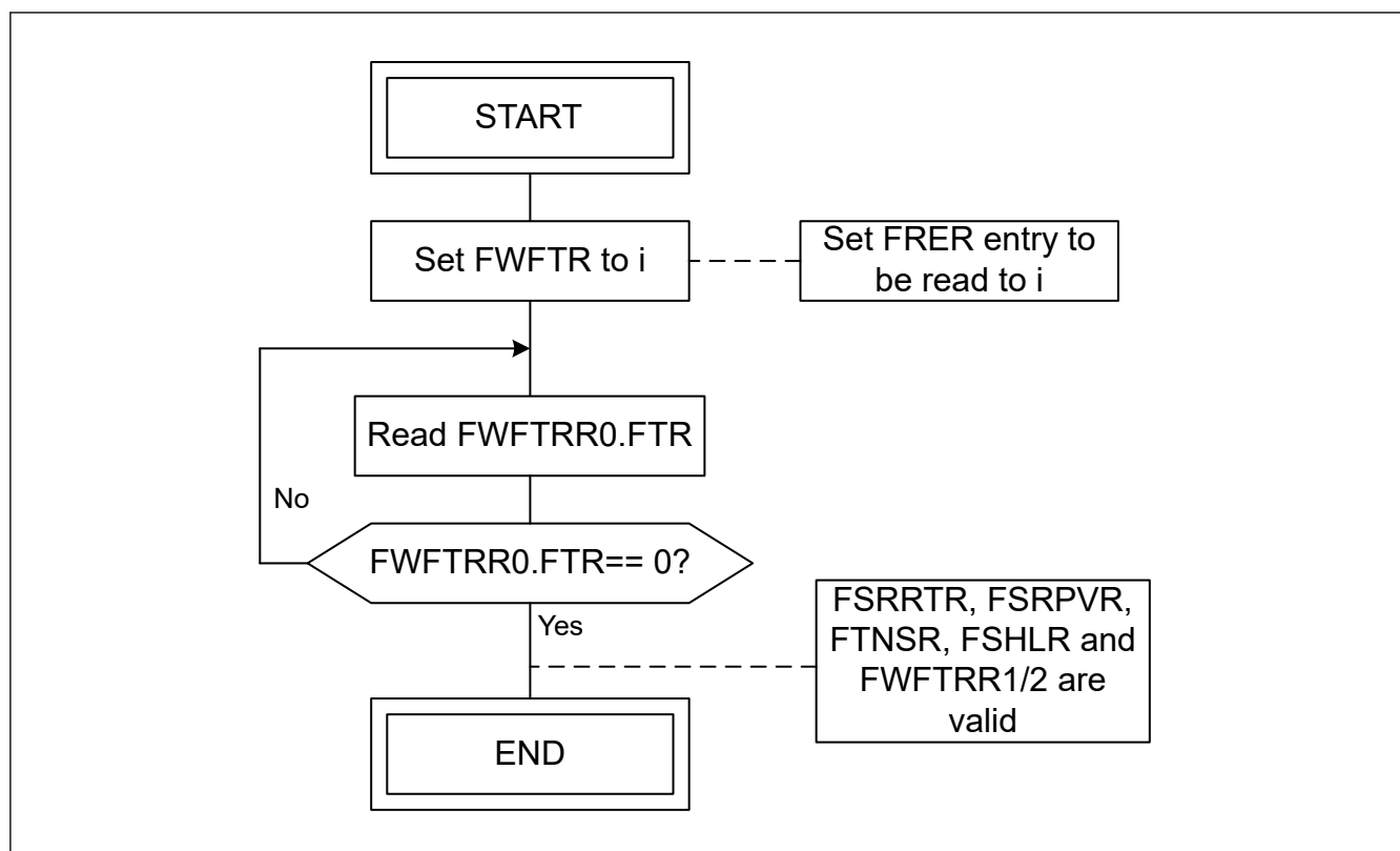
Figure 31.32 Read flow of FRER entry i
