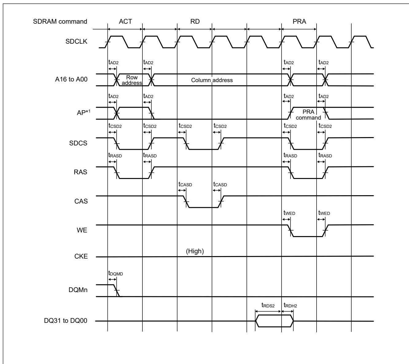
Figure 70.45 SDRAM single read timing
