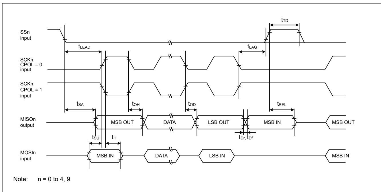
Figure 70.72 SCI simple SPI mode timing for slave when CPHA = 0
