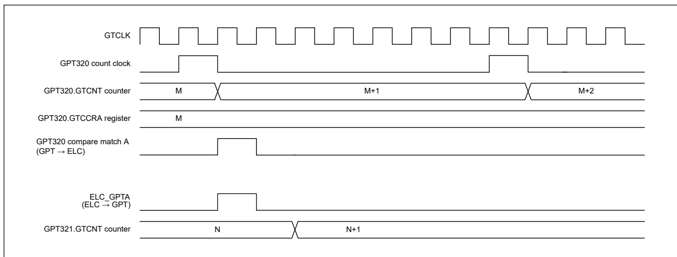
Figure 23.8 Example of Event Count Operation (Up-Counting the Number of Event Signals Input from ELC_GPTA)
