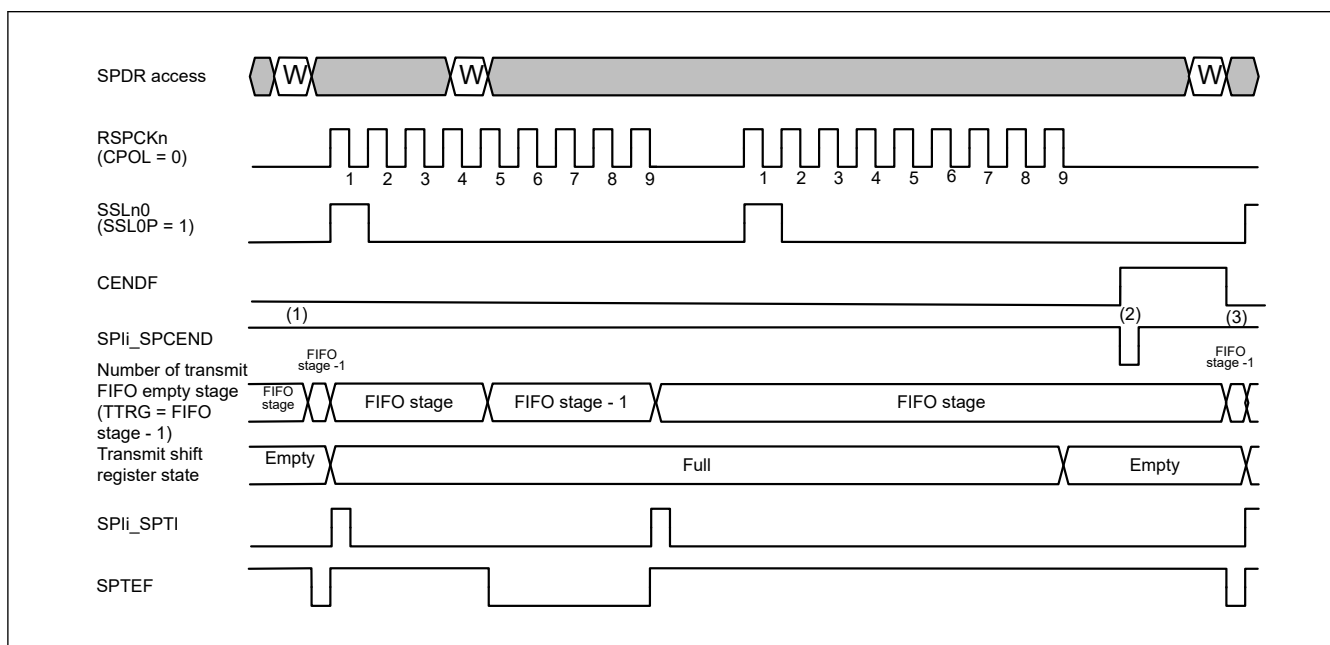
Figure 36.41 Example of Communication End Interrupt Operation (Transmit-Receive/Transmit-only Slave mode on SPI Operation / TI-SSP)
