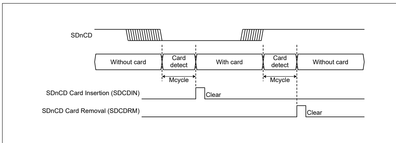
Figure 40.7 Example of card detect with SDnCD
