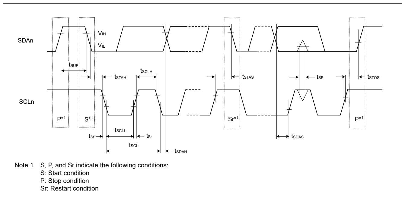
Figure 55.71 I²C bus interface input/output timing
