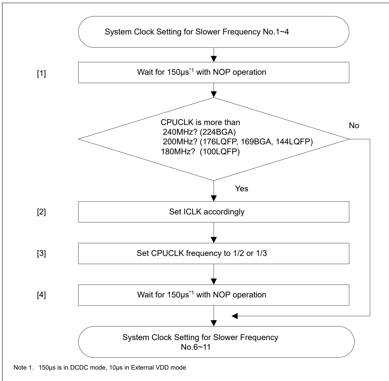
Figure 8.15 Additional flow of system clock setting when PLL is used for the system clock source and CPUCLK to be slower frequency
