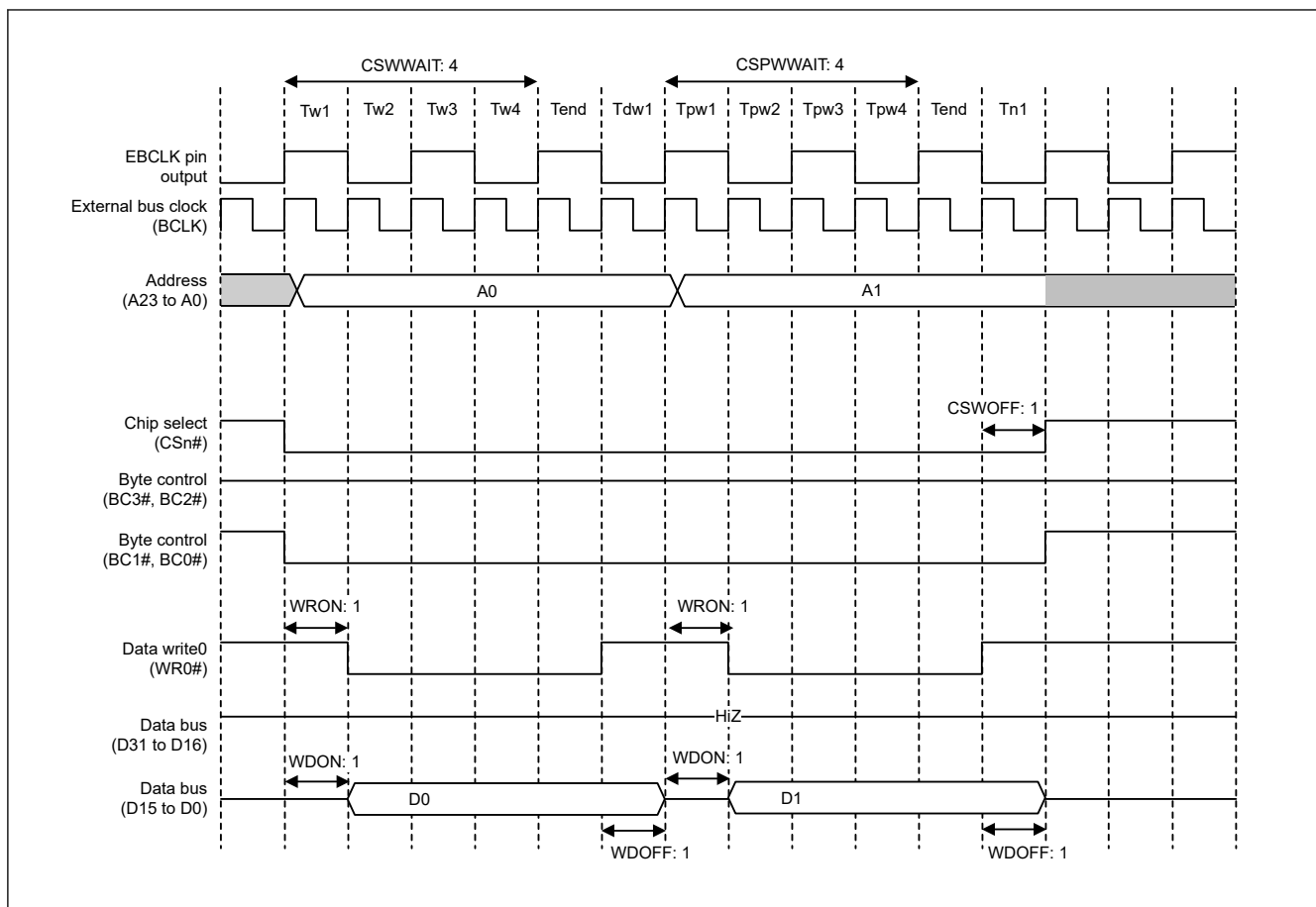
Figure 14.20 Example page write access operation when BCLK/2 is selected in the EBCLK Pin Output Select bit and two rounds of bus access are generated in response to a single transfer request, in single-write strobe mode (n = 0 to 7)
