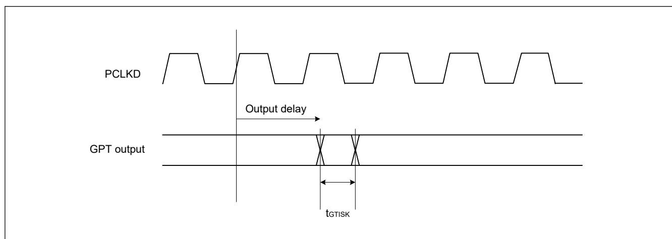
Figure 55.46 GPT output delay skew
