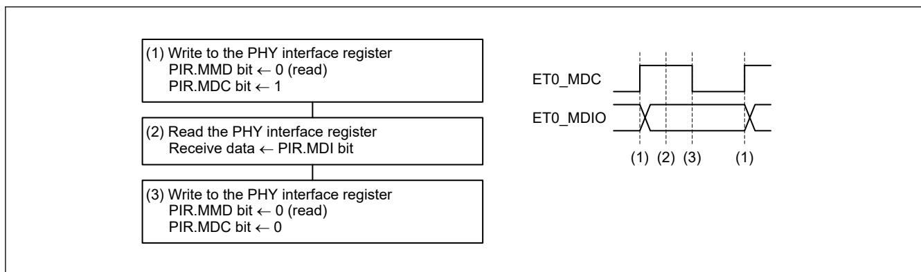
Figure 27.17 1-bit data read flow
