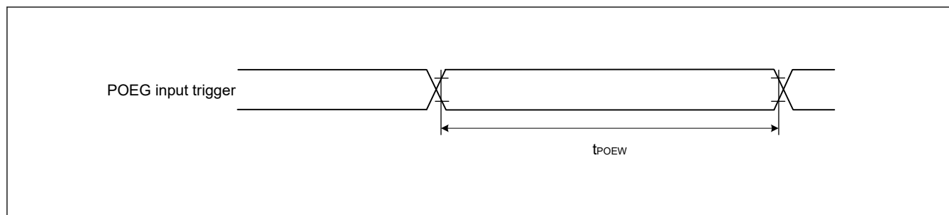
Figure 55.44 POEG input trigger timing
