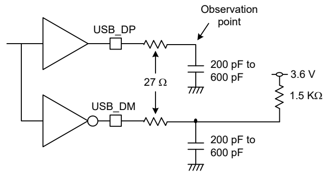
Figure 55.105 Test circuit in low-speed mode
