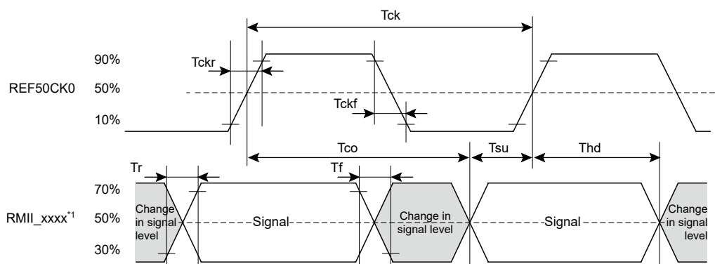
Figure 55.91 REF50CK0 and RMII signal timing
