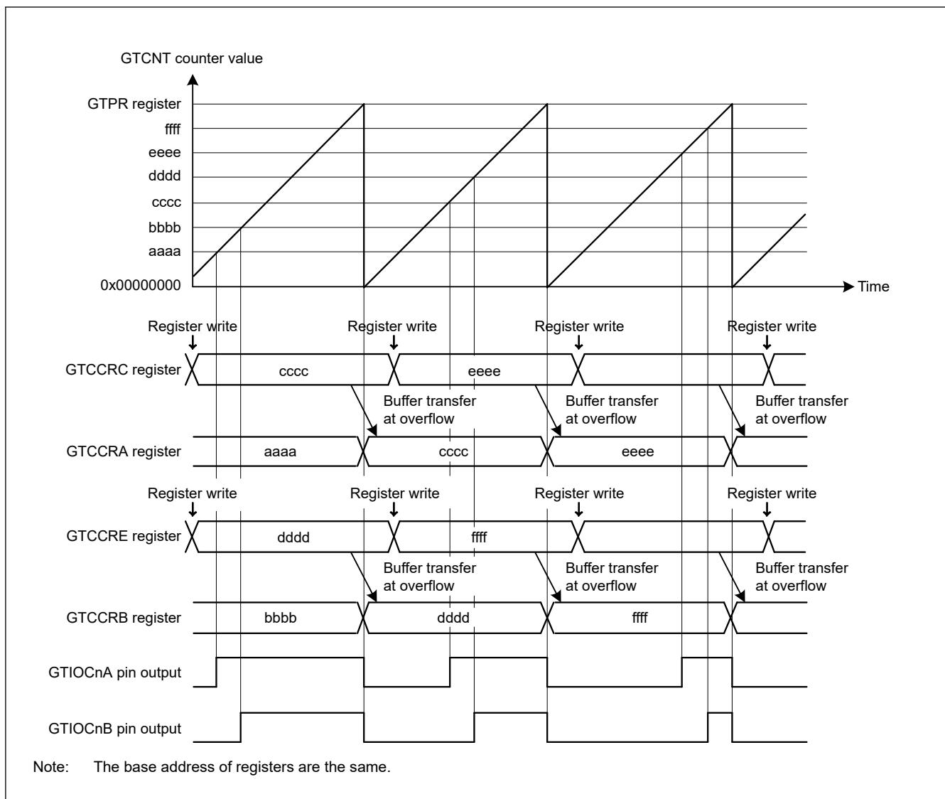
Figure 21.21 Example of saw-wave PWM mode operation with up-counting, buffer operation, high output at GTCCRA/GTCCRB compare match, and low output at cycle end
