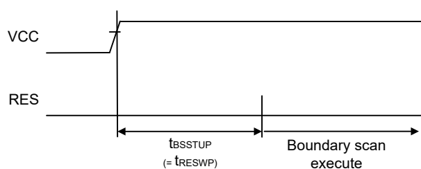
Figure 55.127 Boundary scan circuit startup timing
