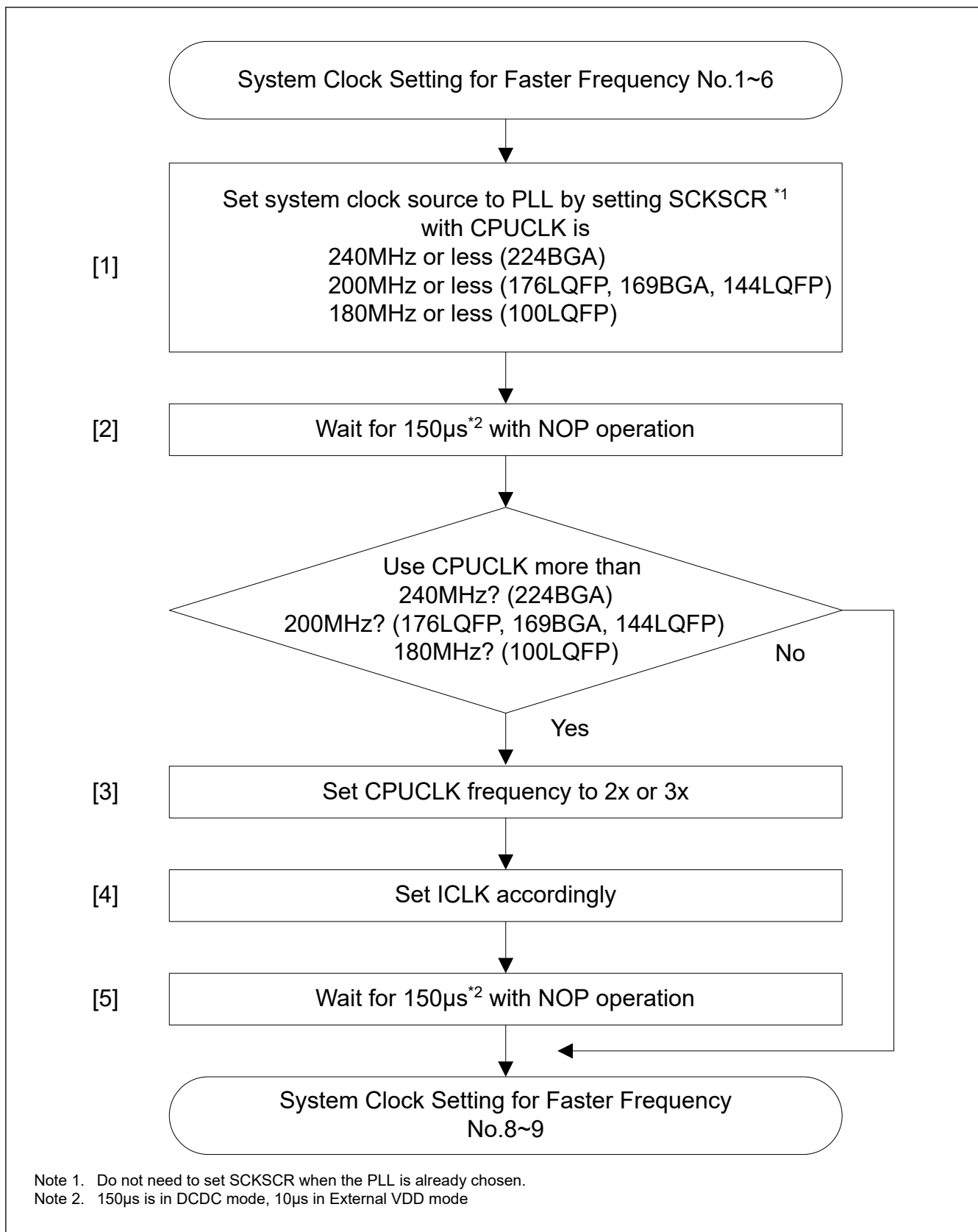
Figure 8.14 Additional flow of system clock setting when PLL is used for the system clock source and CPUCLK to be faster frequency
