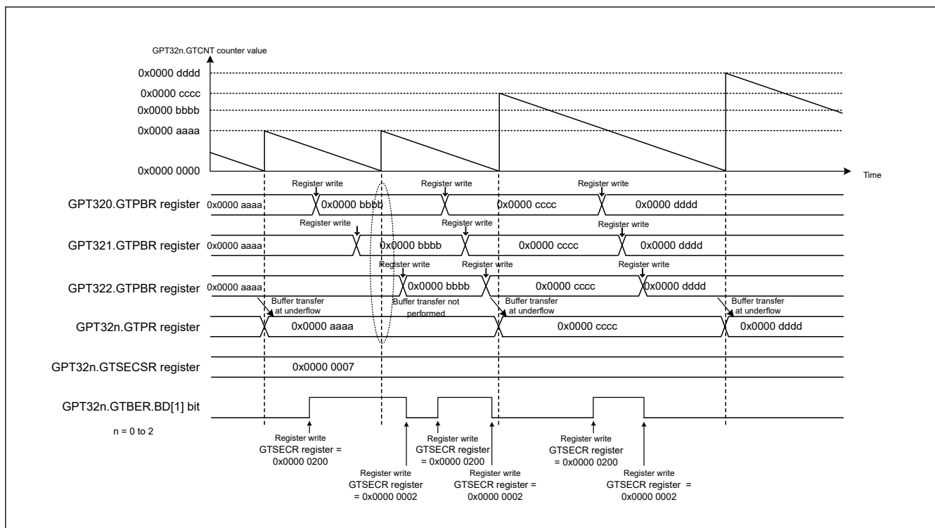
Figure 21.74 Example of Multiple Channel Operation for Disabling Buffer Operation (Saw Waves, Single Buffer Operation)
