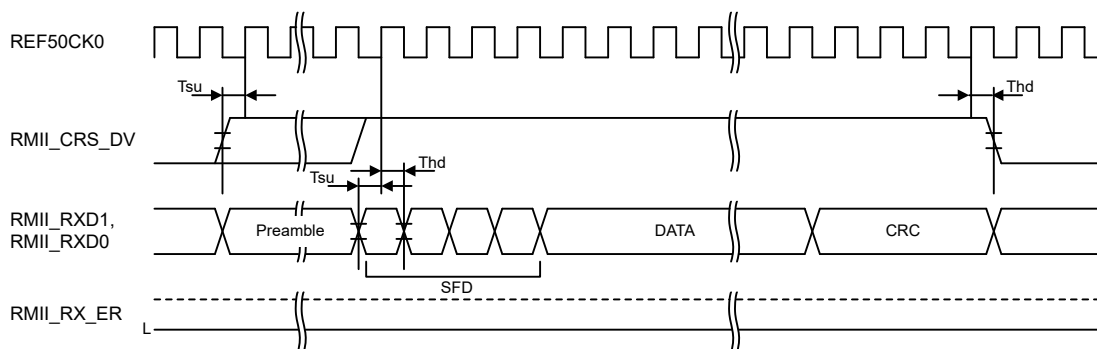
Figure 55.93 RMII reception timing in normal operation
