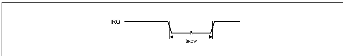
Figure 55.27 IRQ interrupt input timing
