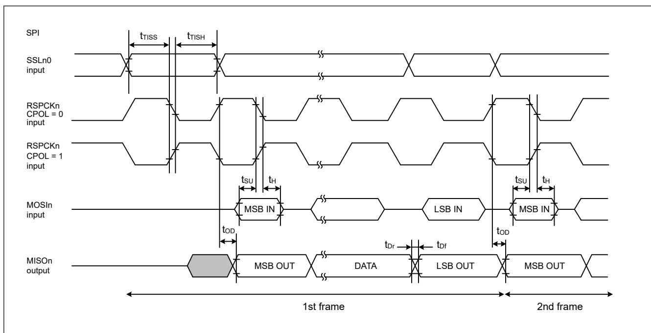
Figure 55.65 SPI timing for TI SSP slave when transmit with no delay between frames
