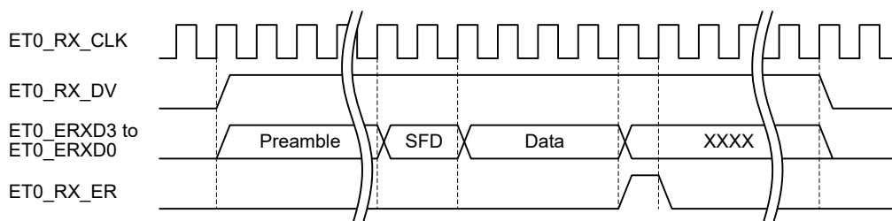
Figure 27.10 MII frame receive timing for receive error notification
