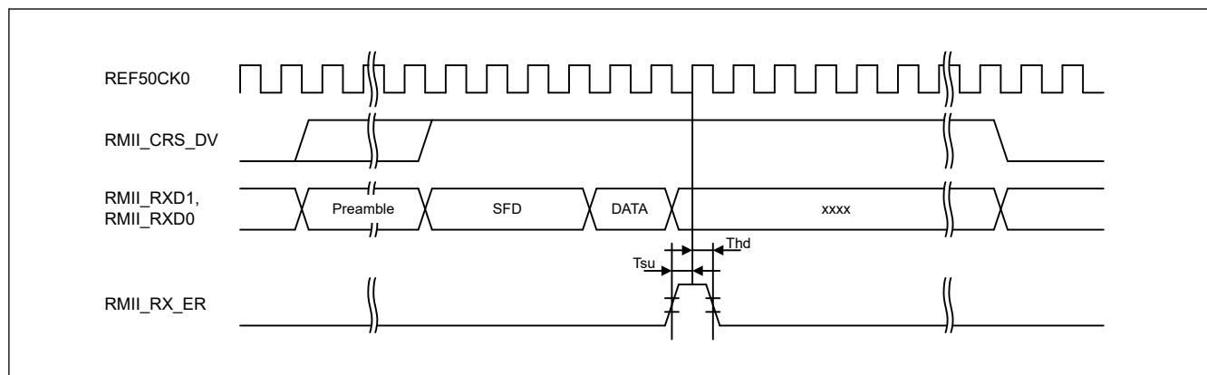
Figure 55.94 RMII reception timing when an error occurs
