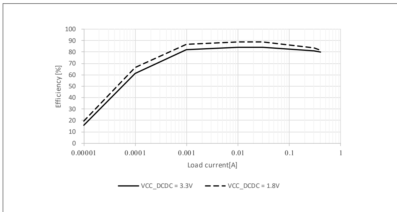
Figure 55.11 Typical DCDC efficiency (%) vs load current (A) in Low-speed mode and Software Standby mode, T_j = 25\text{ °C}
