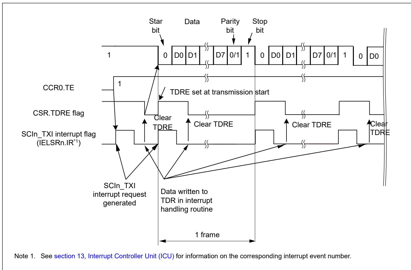
Figure 31.15 Example of Operation for Serial Transmission in Asynchronous Mode (4)(with 8-Bit Data, Parity, 1 Stop Bit, CTS Function Not Used, from the Middle of Transmission until Transmission Completion)
