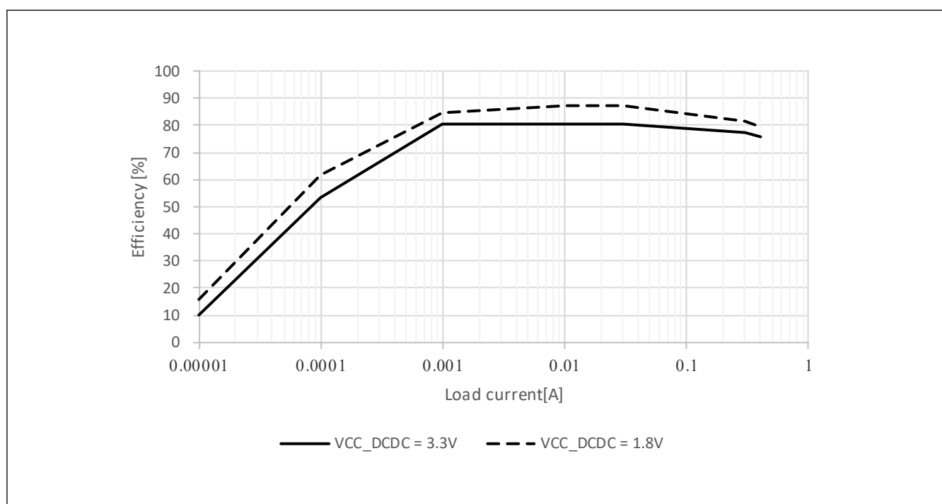
Figure 55.12 Typical DCDC efficiency (%) vs load current (A) in Low-speed mode and Software Standby mode, T_j = 125\text{ °C}
