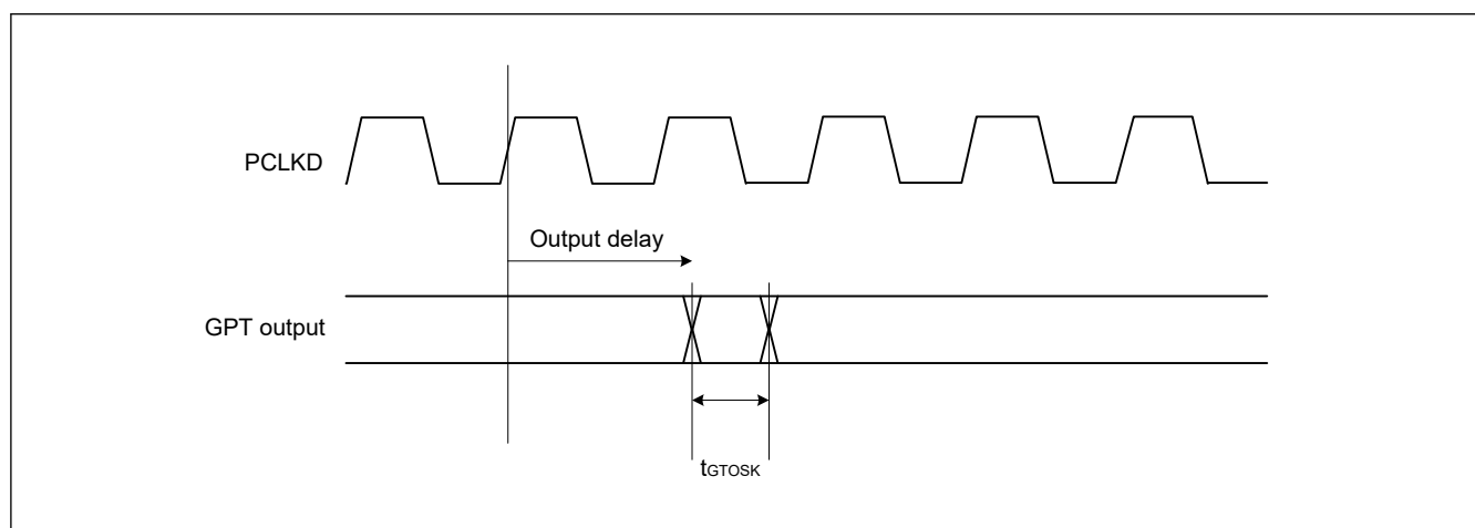
Figure 55.47 GPT output delay skew for OPS
