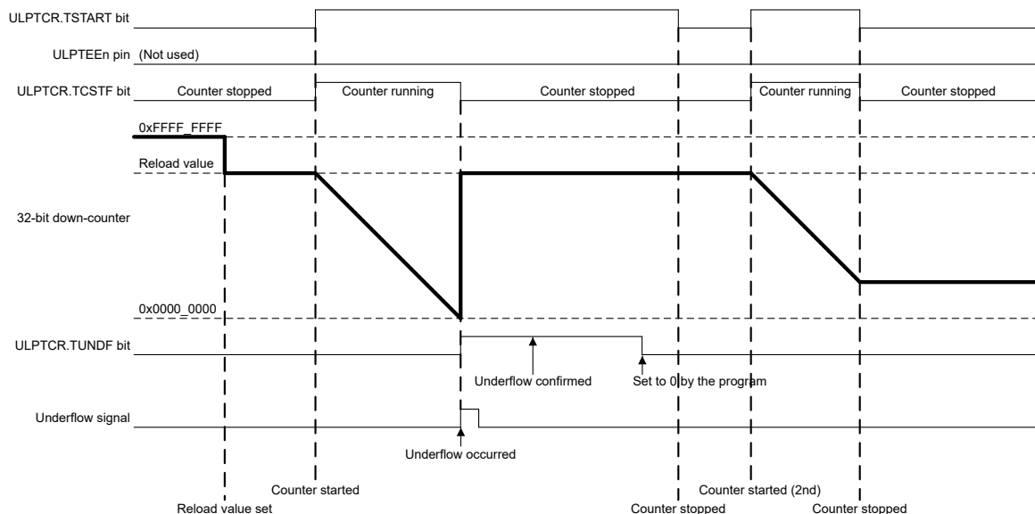
Figure 23.7 Operation example in event counter & one-shot & count enable mode (with the ULPTIOC.TIOGT0 bit set to 0)
