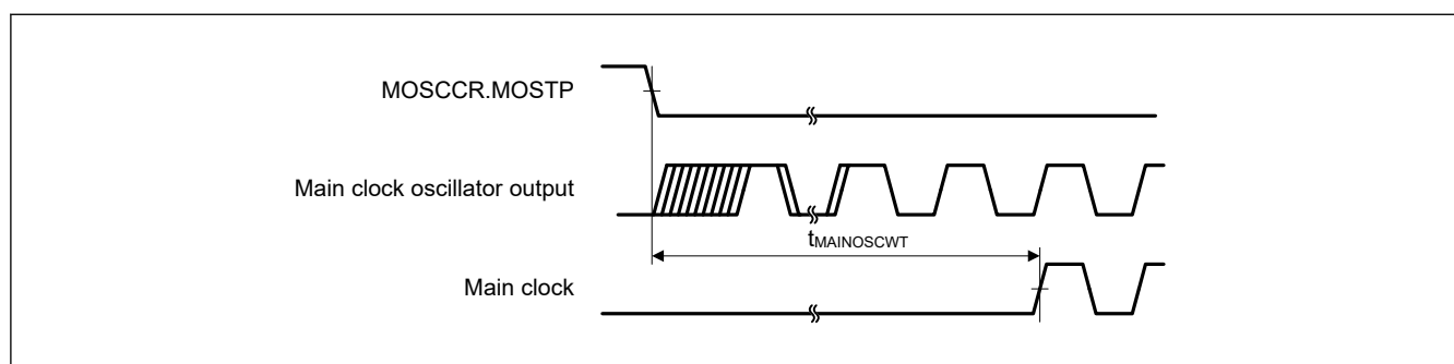
Figure 55.17 Main clock oscillation start timing
