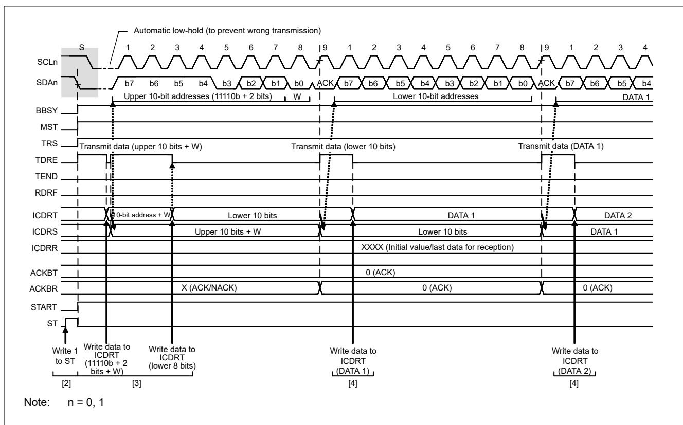
Figure 32.8 Master transmit operation timing (2) with 10-bit address format
