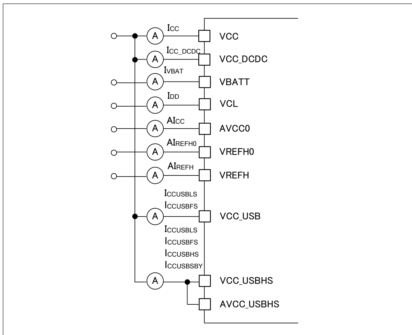
Figure 55.2 Consumption current measurement diagram
