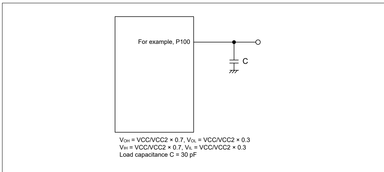
Figure 55.1 Input or output timing measurement conditions
