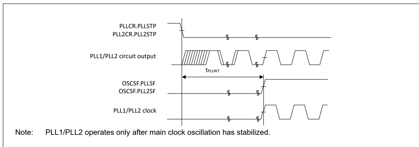
Figure 55.19 PLL1/PLL2 clock oscillation start timing
