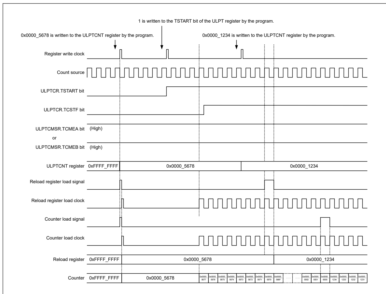
Figure 23.14 Counter and reload rewrite timing (under condition A or C)
