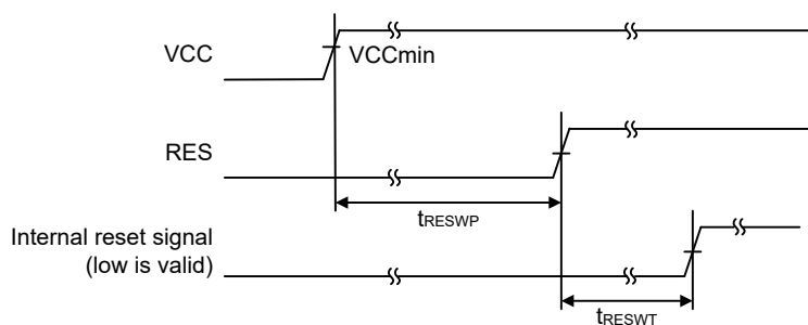
Figure 55.22 RES pin input timing under the condition that VCC exceeds V POR voltage threshold
