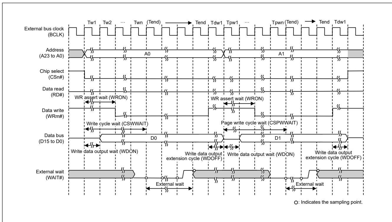
Figure 14.26 Example external wait timing for page write access to 16-bit bus space in byte strobe mode (when 1/1 BCLK is selected with the BCLK Pin Output Select bit) (n = 0 to 7, m = 0, 1)
