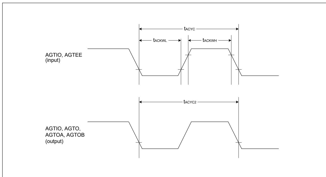
Figure 55.48 AGT input/output timing
