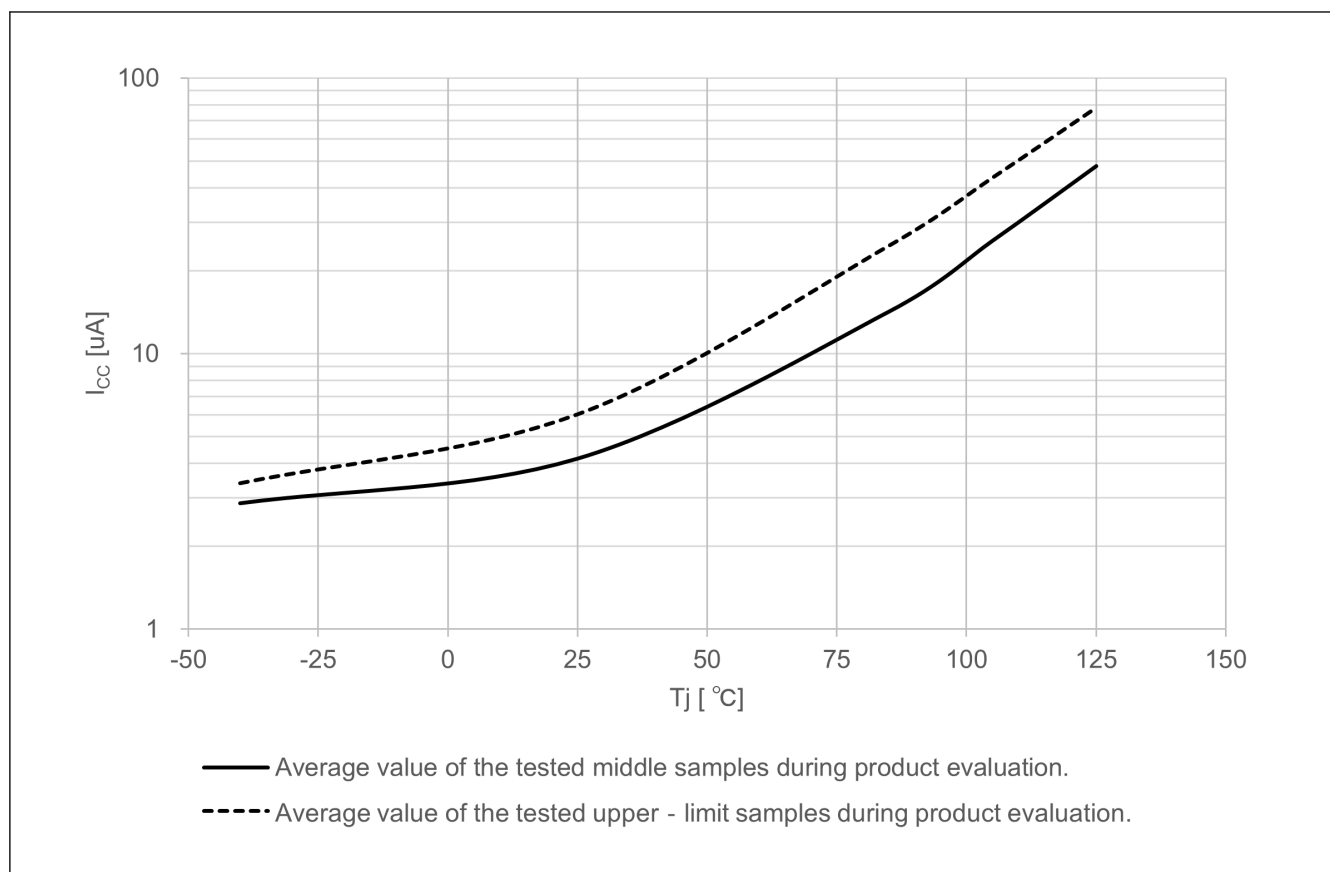
Figure 55.5 Temperature dependency in Deep Software Standby mode 1 (reference data)
