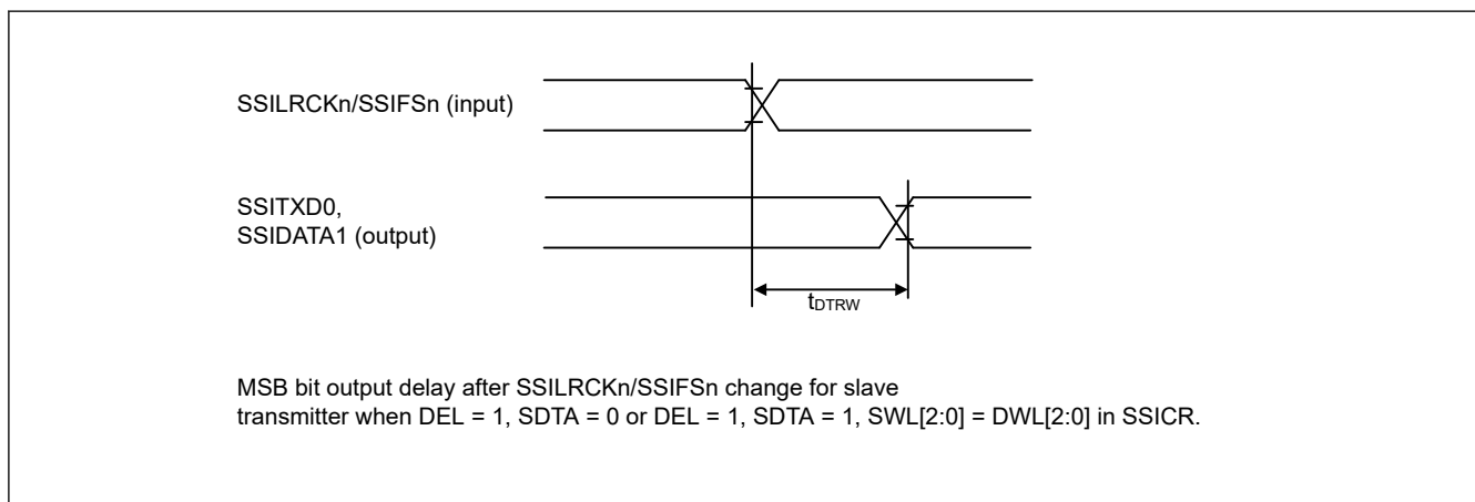
Figure 55.89 SSIE data output delay after SSILRCK0/SSIFS0 change
