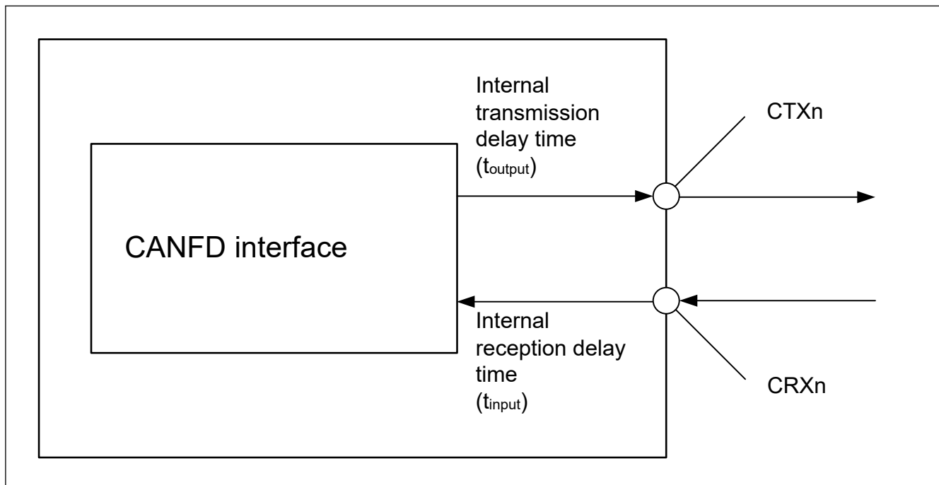
Figure 55.103 CANFD interface condition
