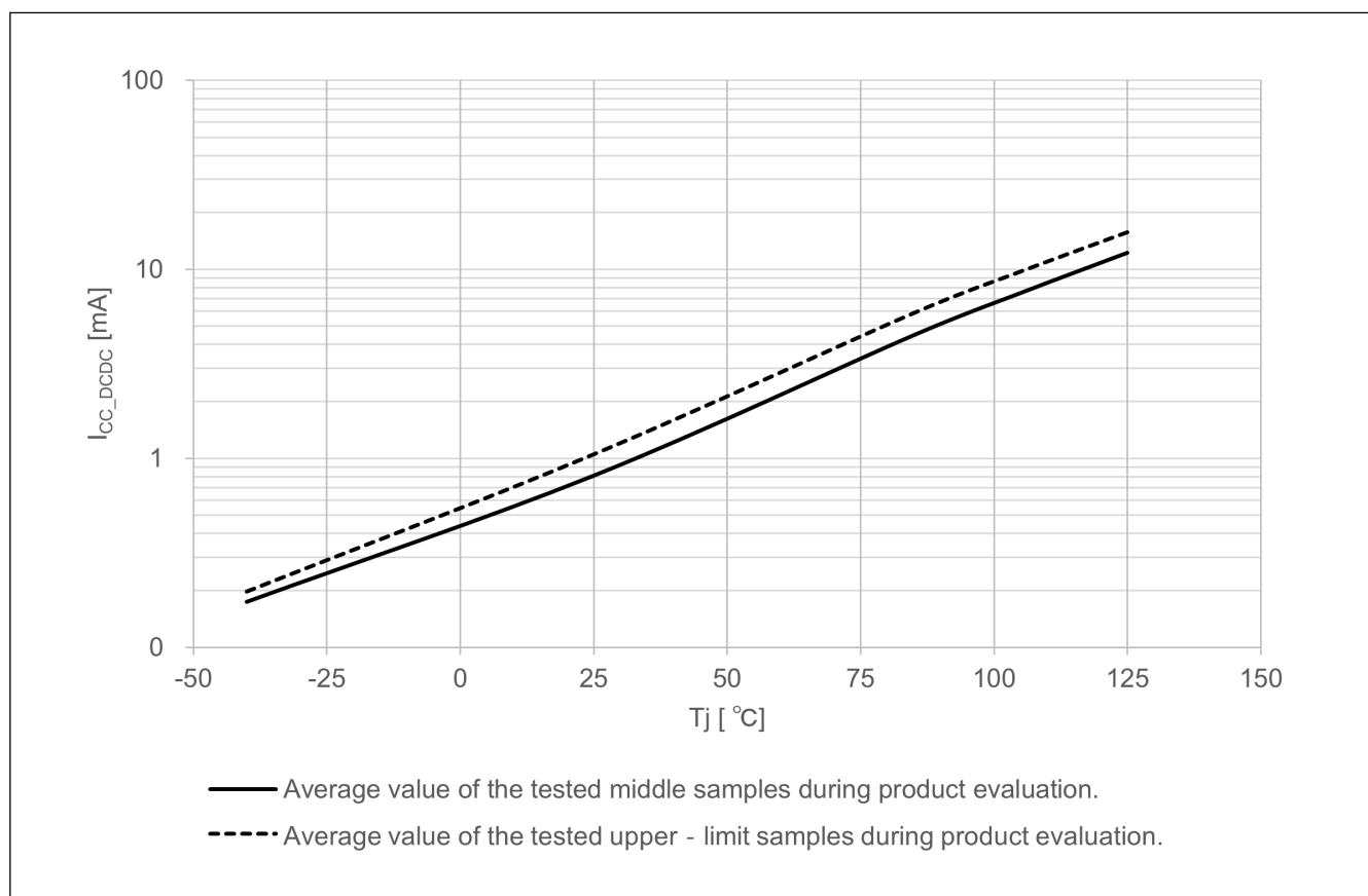
Figure 55.4 Temperature dependency in Software Standby mode ( I_{CC\_DcDc} ) (reference data)
