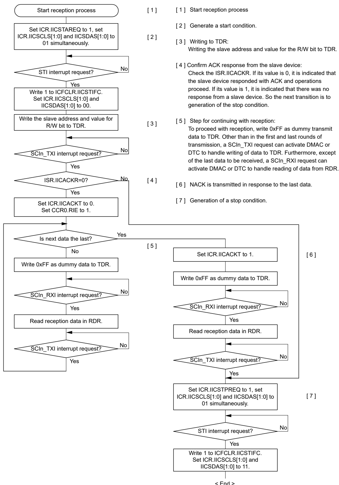
Figure 31.96 Example flow of master reception in simple IIC mode with transmission interrupts and reception interrupts (ICR.IICINTM = 1)
