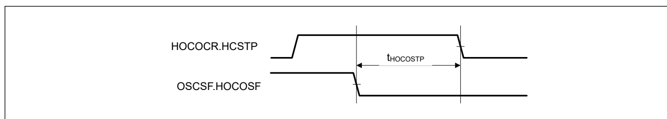
Figure 55.21 HOCO stop width time
