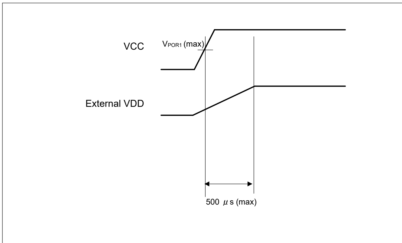
Figure 54.3 Power-up sequence of external VDD mode without using RES pin
