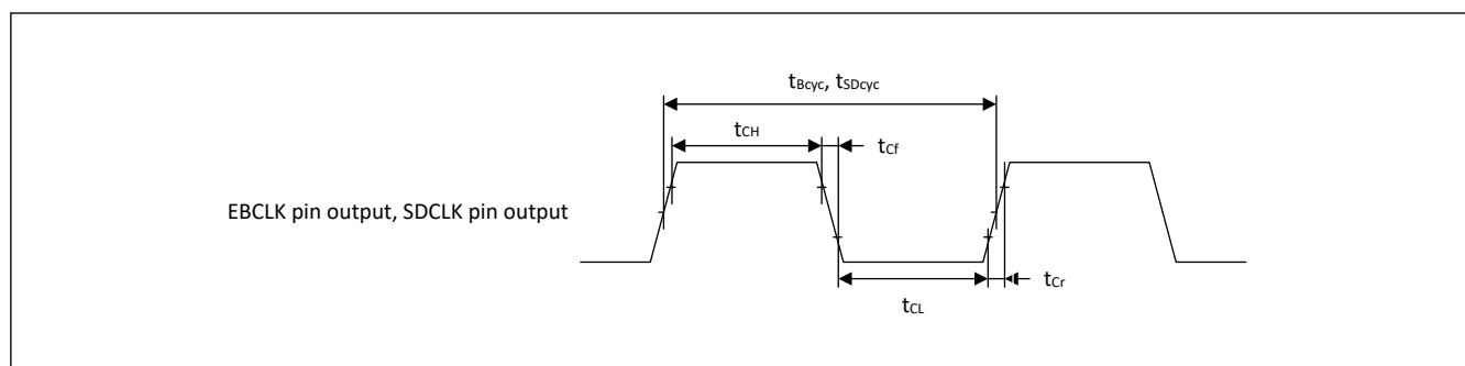
Figure 55.15 EBCLK and SDCLK output timing
