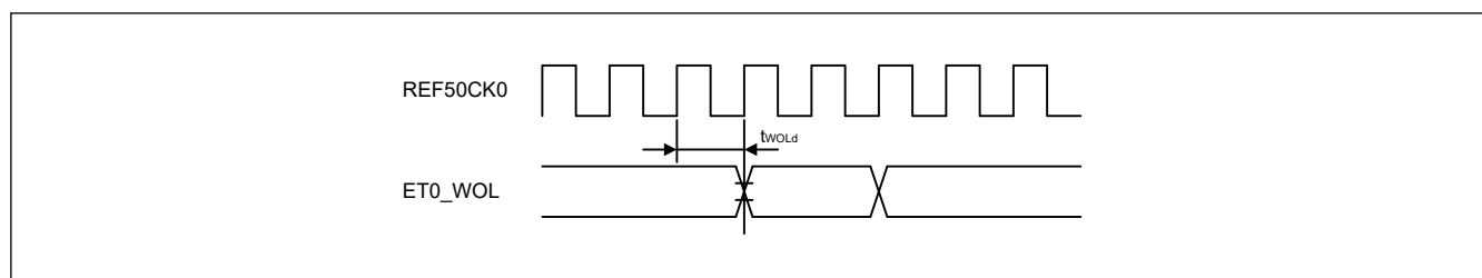
Figure 55.95 WOL output timing for RMII
