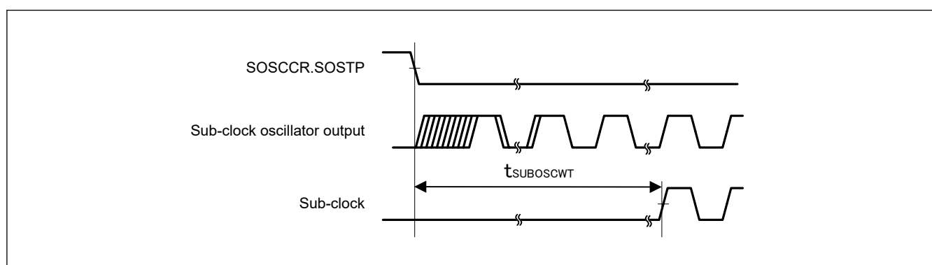
Figure 55.20 Sub-clock oscillation start timing
