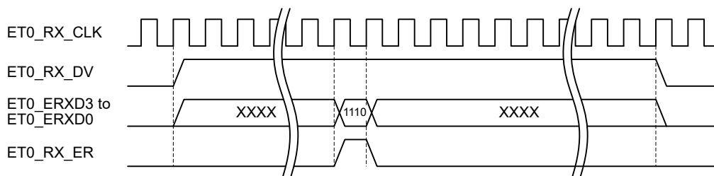
Figure 27.11 MII frame receive timing for false carrier notification
