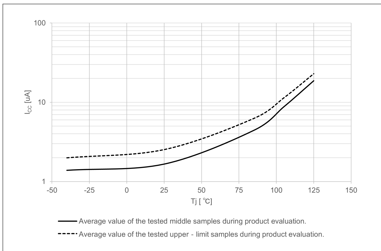
Figure 55.6 Temperature dependency in Deep Software Standby mode 2 (reference data)
