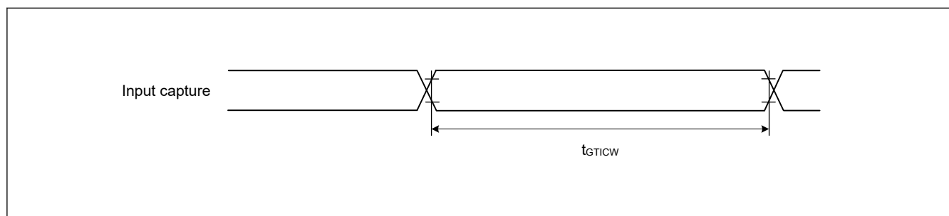
Figure 55.45 GPT input capture timing
