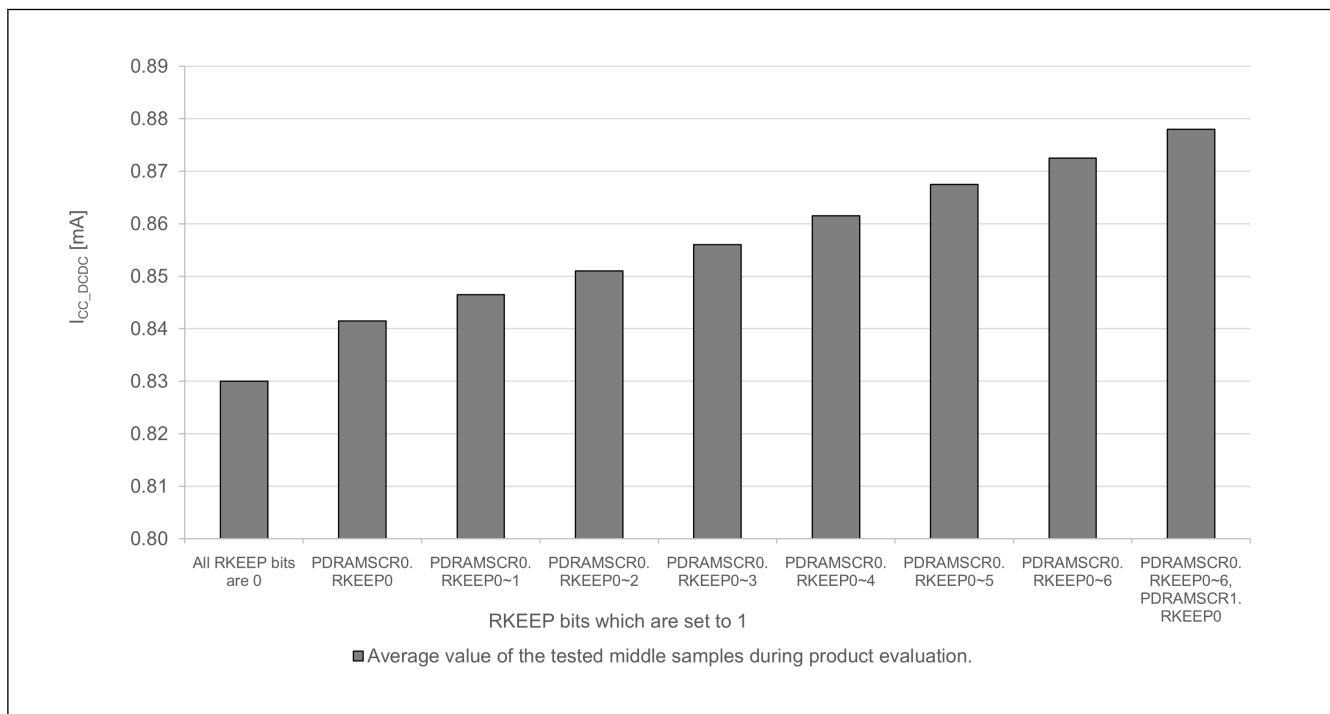
Figure 55.8 Software Standby current per SRAM state (reference data)
