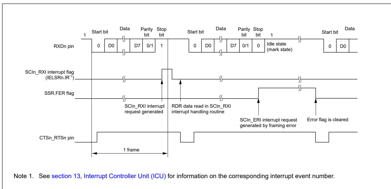
Figure 31.20 Example of SCI operation for serial reception in Asynchronous mode (2) when RTS function is used, and with 8-bit data, parity bit, and 1 stop bit
