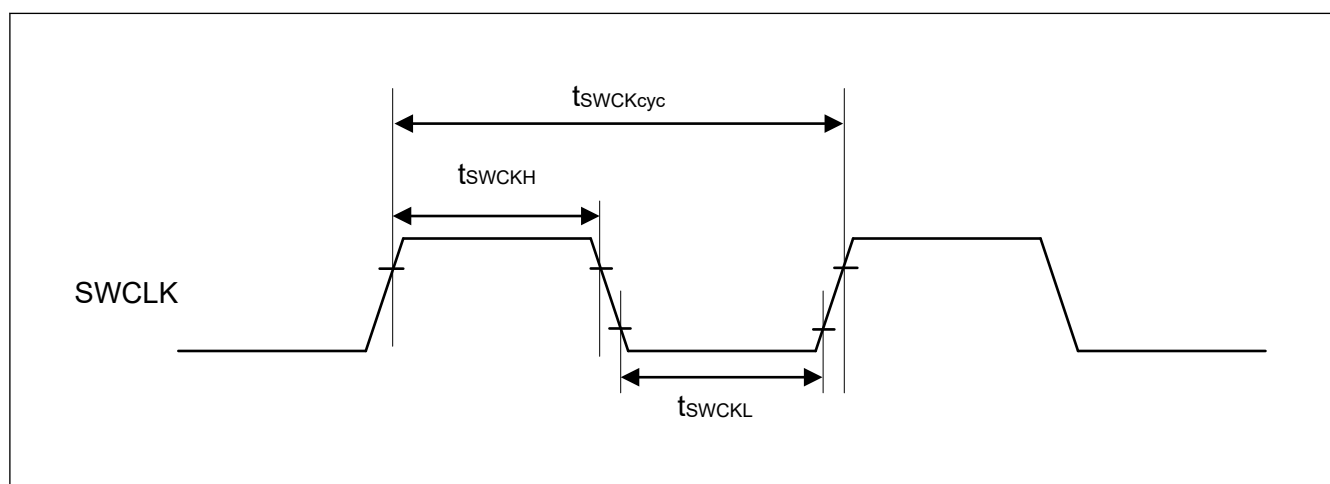
Figure 55.130 SWD SWCLK timing
