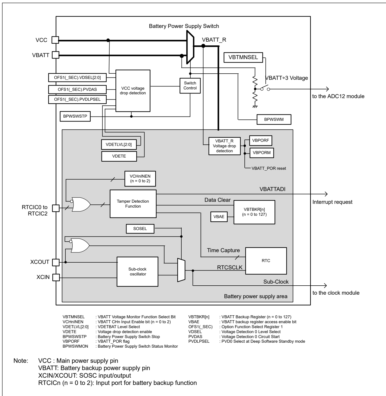
Figure 11.1 Battery Backup Function block diagram
