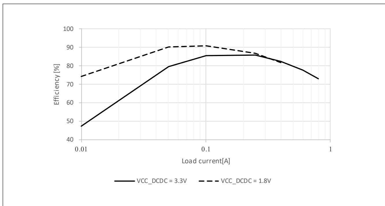
Figure 55.10 Typical DCDC efficiency (%) vs load current (A) in High-speed mode, Tj = 125 °C
