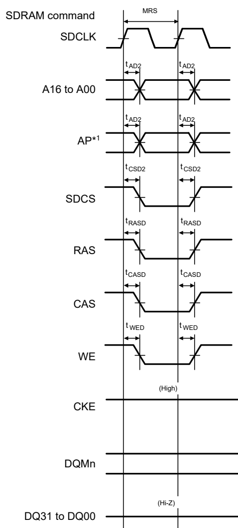
Figure 55.40 SDRAM mode register set timing
