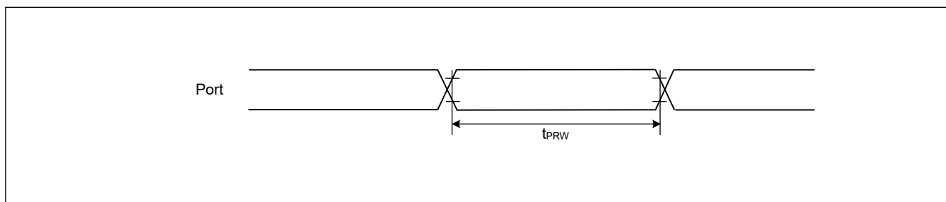
Figure 55.42 I/O ports input timing
