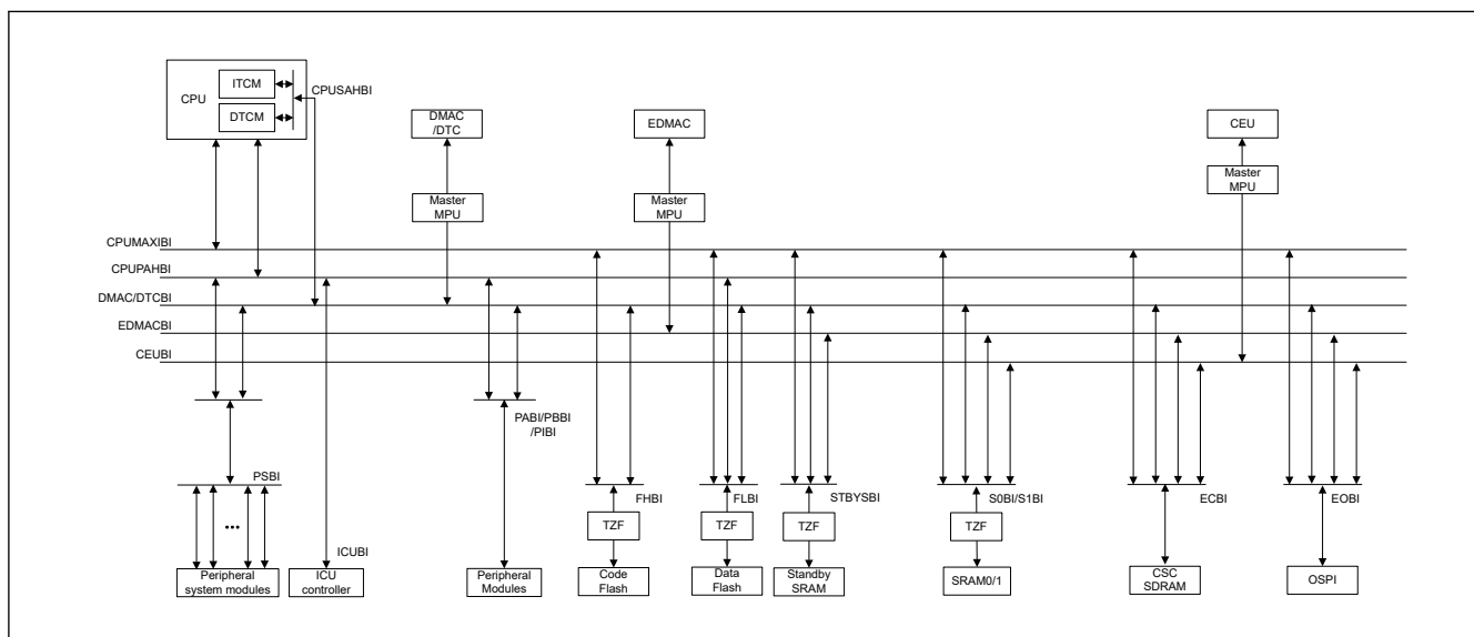
Figure 14.1 System bus connection
