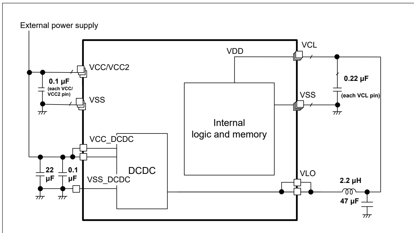
Figure 54.1 DCDC mode setting
