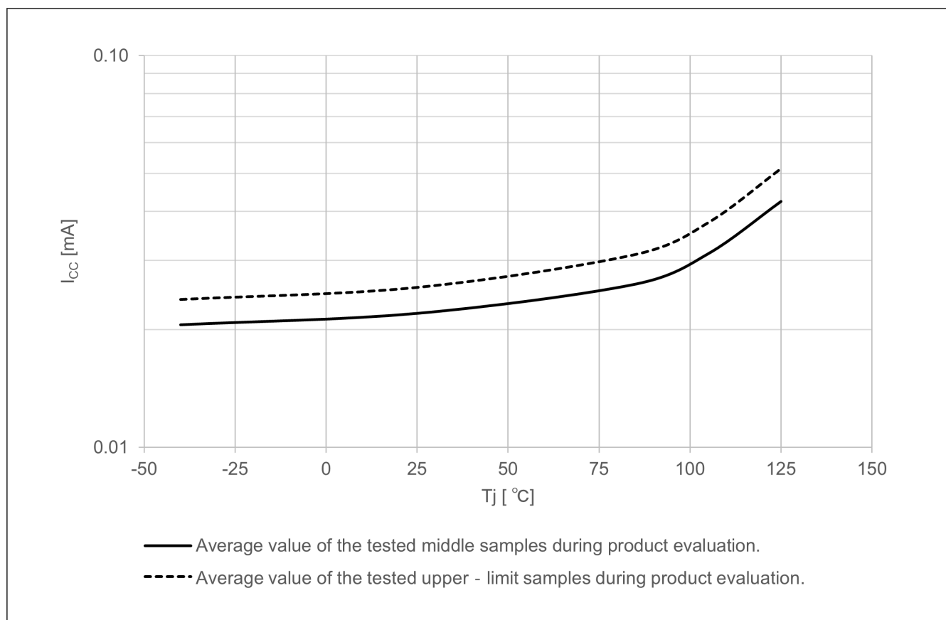
Figure 55.3 Temperature dependency in Software Standby mode ( I_{CC} ) (reference data)
