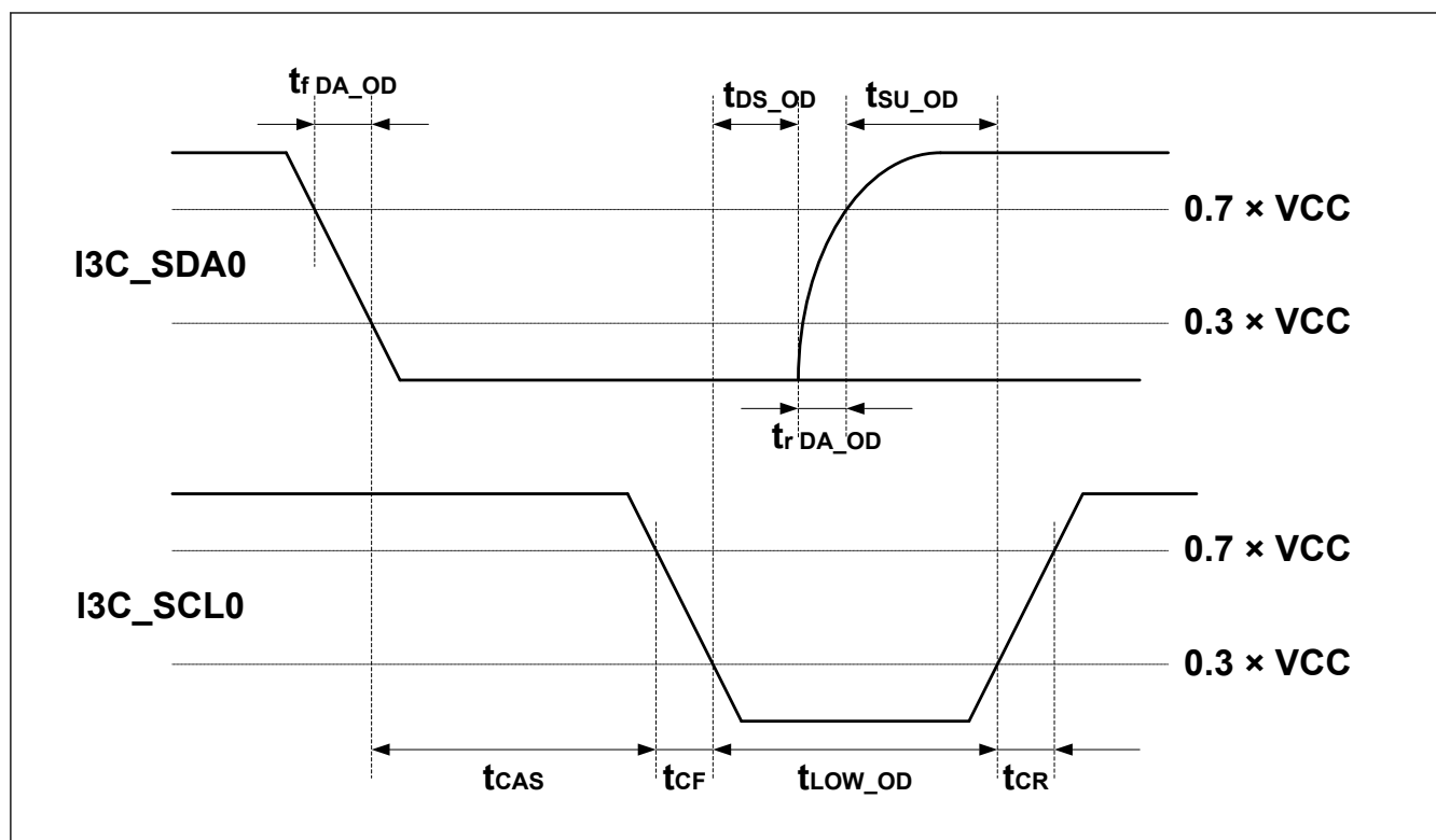
Figure 55.76 I3C START condition Timing
