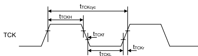
Figure 55.124 Boundary scan TCK timing
