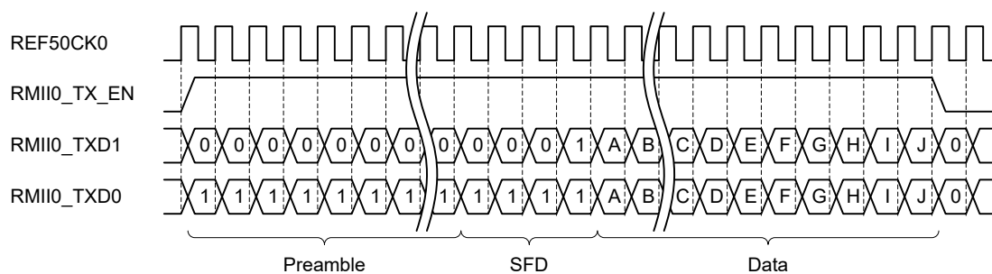
Figure 27.12 RMII frame transmit timing during normal transmission
