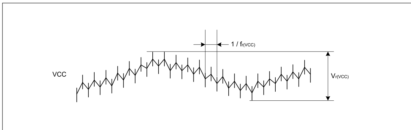
Figure 55.13 Ripple waveform
