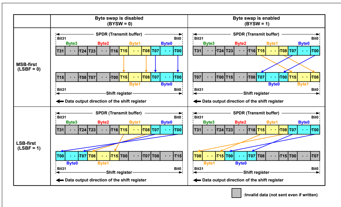
Figure 36.24 Byte swap with MSB/LSB transfer (16bit)
