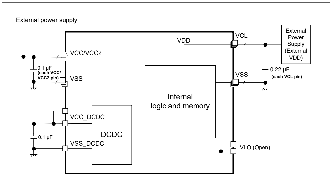
Figure 54.2 External VDD mode setting
