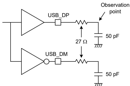
Figure 55.107 Test circuit in full-speed mode
