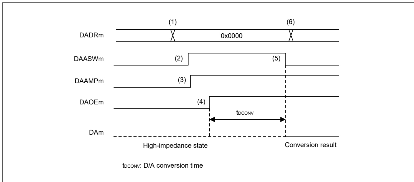
Figure 46.5 Example of the initial flow with the output amplifier in DAC12
