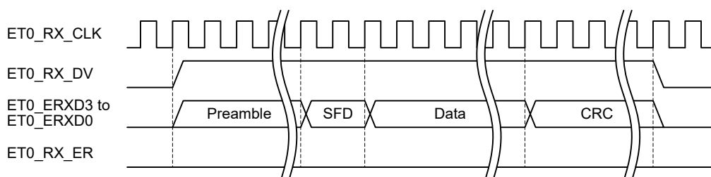
Figure 27.9 MII frame receive timing during normal reception
