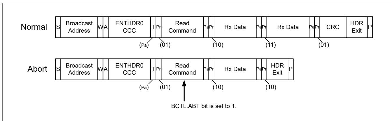
Figure 33.119 Abort operation of HDR-DDR read transfer
