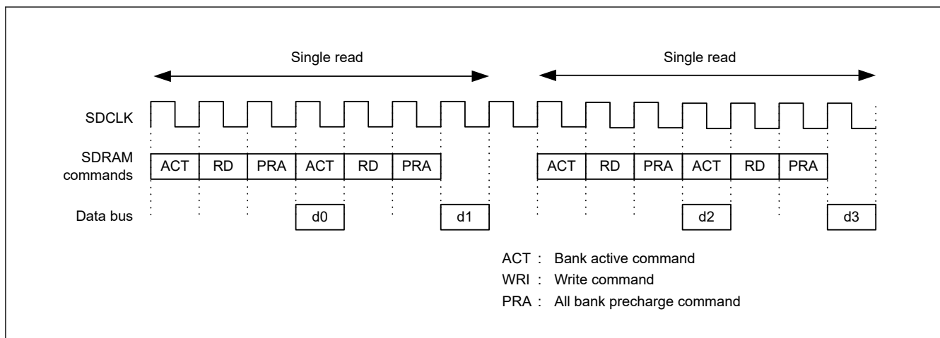
Figure 14.44 Timing Example of Single Read (Burst transfer from bus master with SDAMOD.BE = 0 and SDTR.CL[2:0] = 010b: 2 Cycles)
