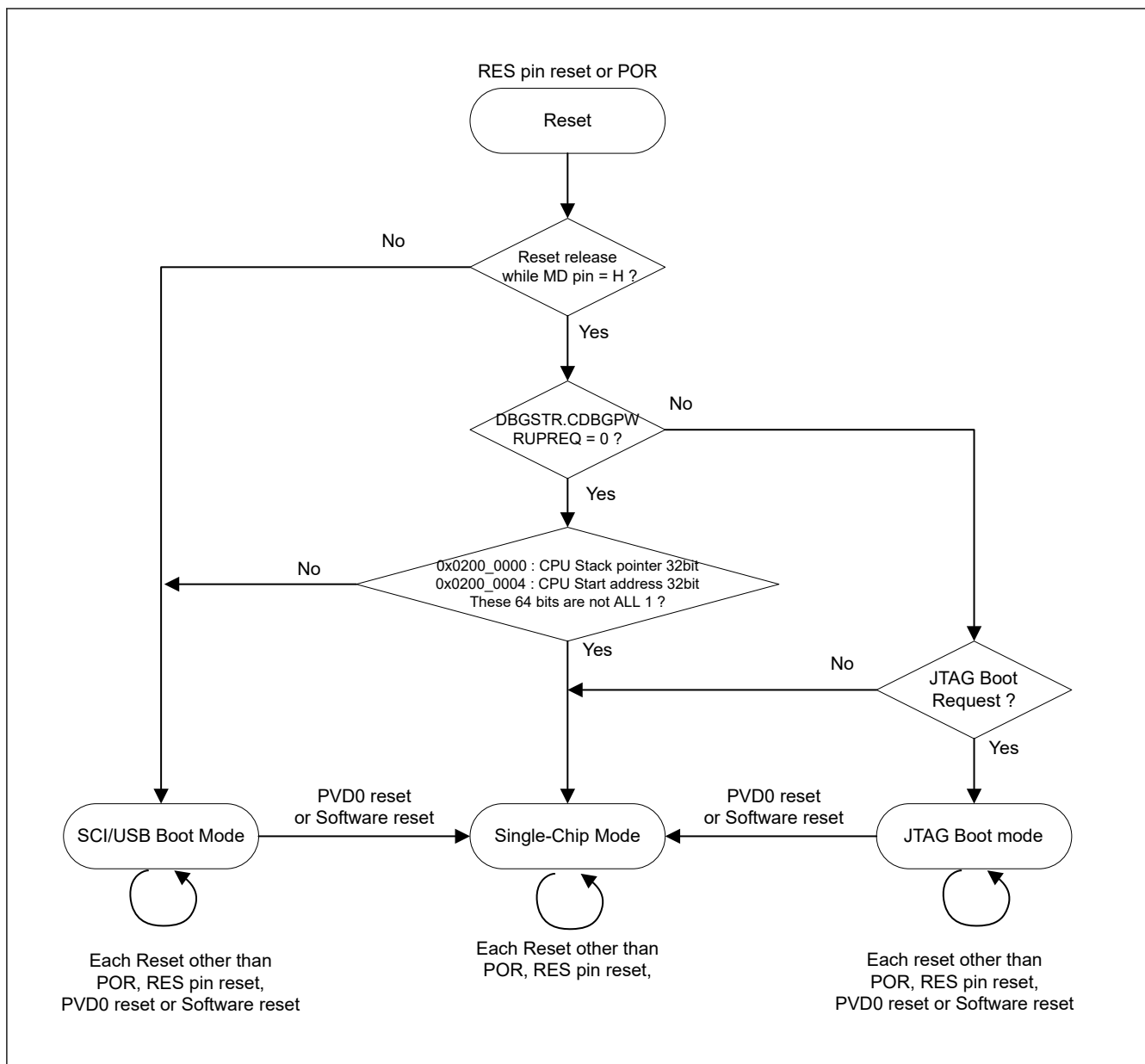
Figure 3.1 Operation modes and the relationship of mode transition
