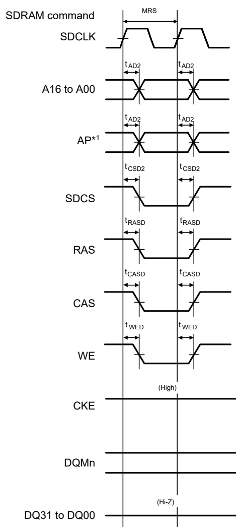
Figure 60.40 SDRAM mode register set timing
