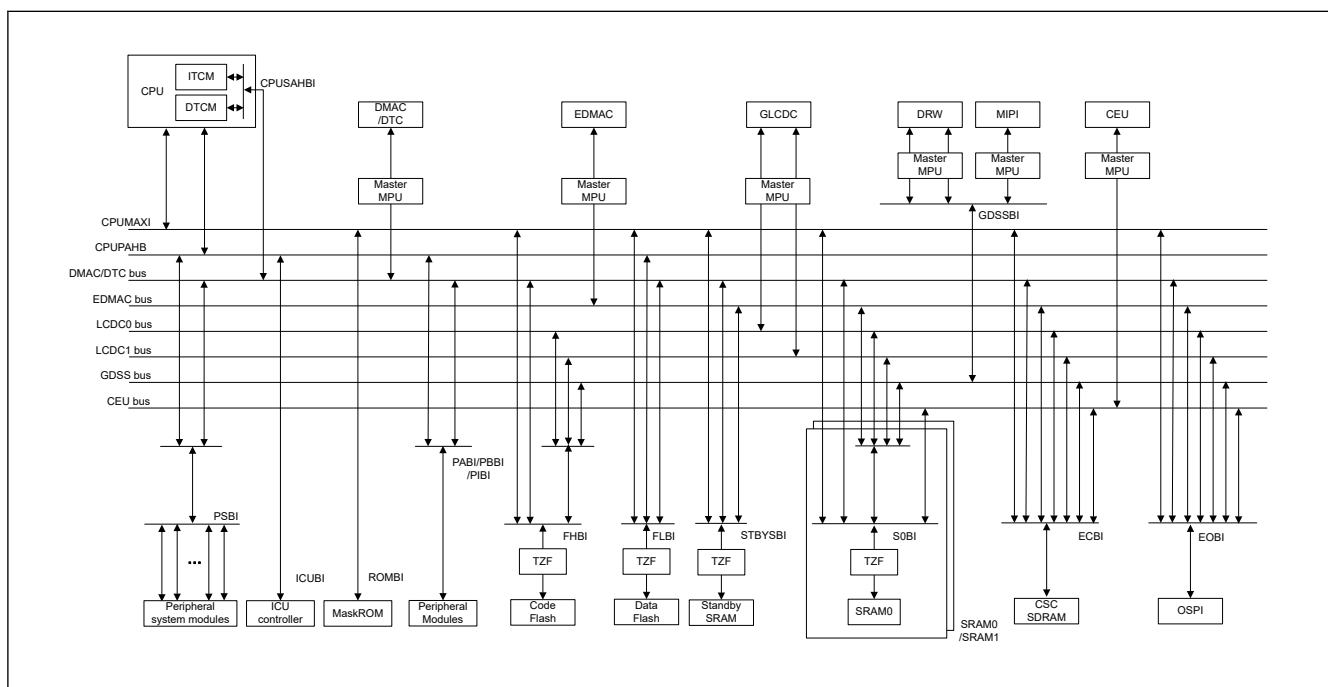
Figure 14.1 System bus connection
