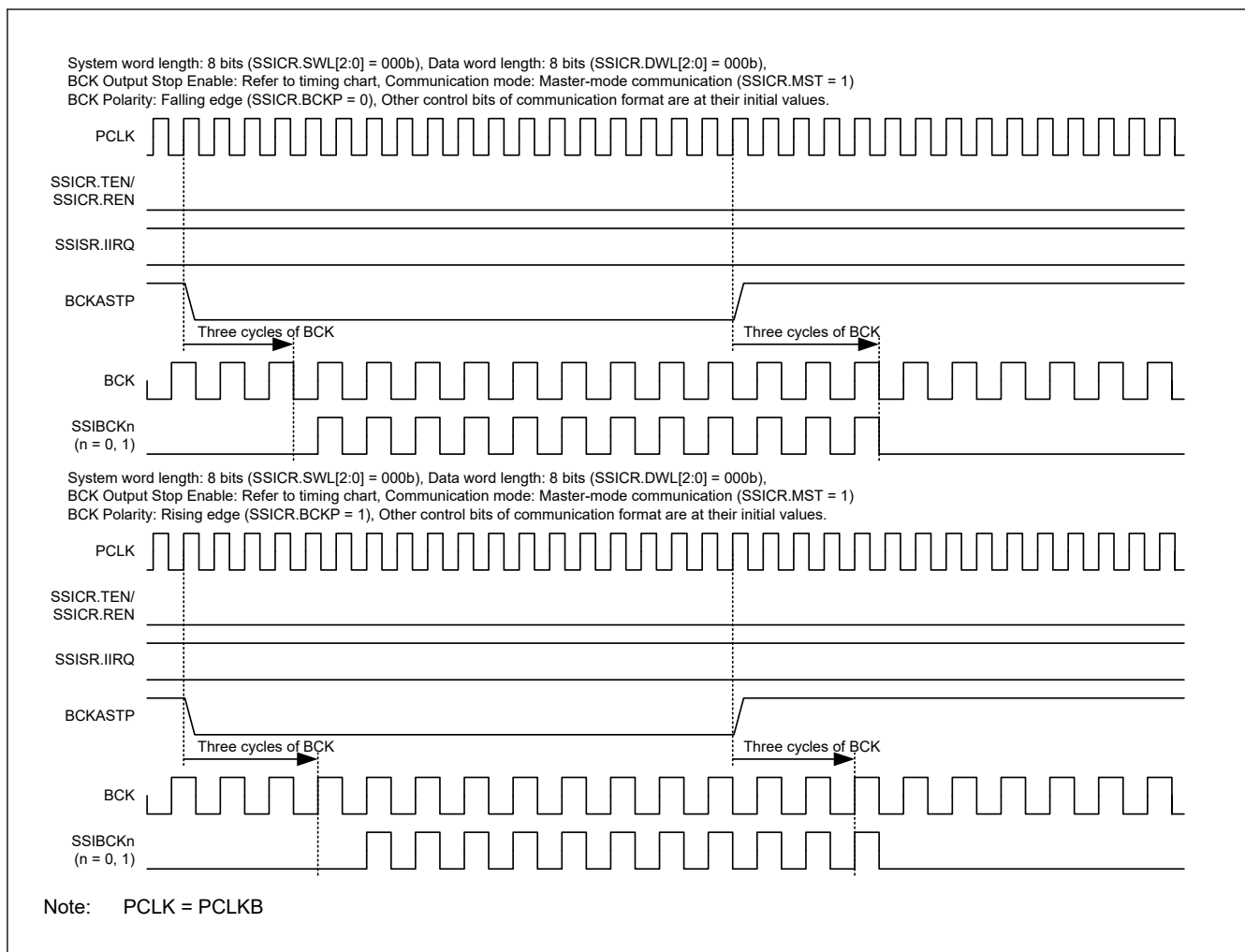
Figure 39.34 Example operation of the BCKASTP bit (idle state)
