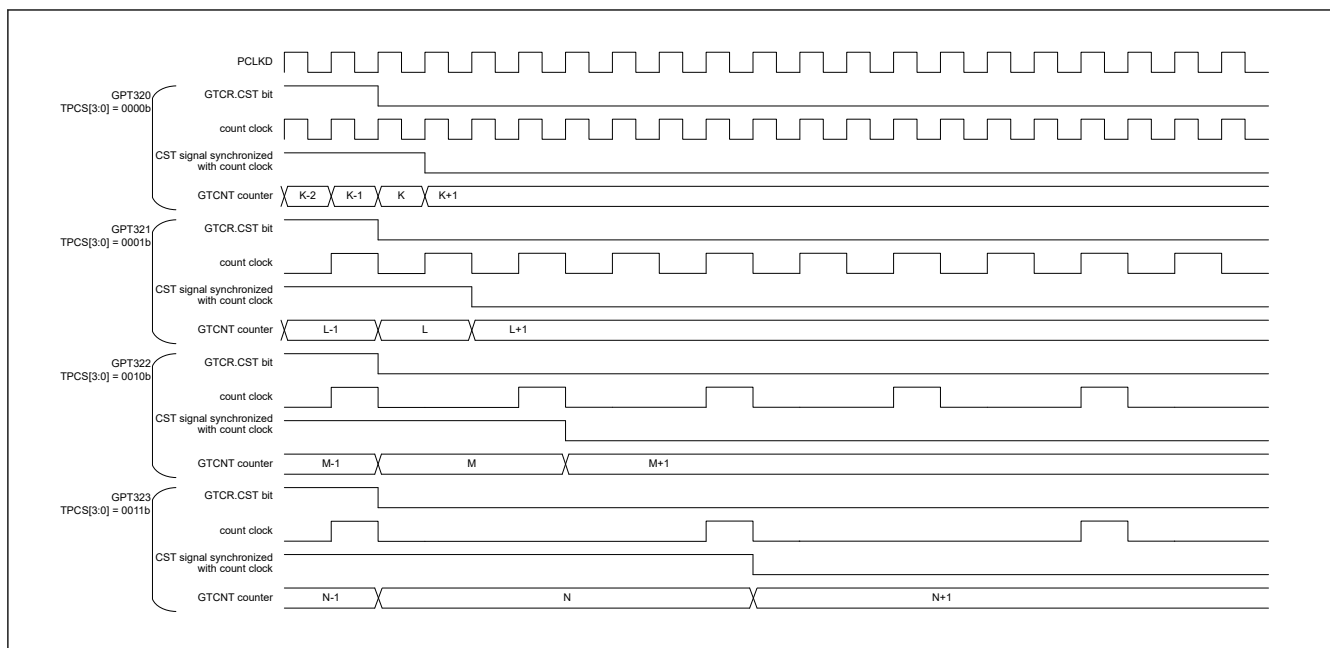
Figure 21.41 Example of Simultaneous Stop Operation by Software (with Different Count Period)
