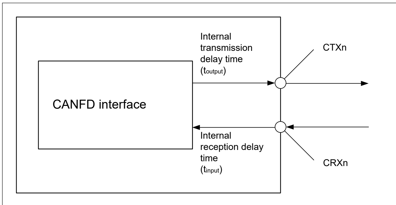
Figure 60.106 CANFD interface condition
