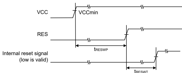
Figure 60.22 RES pin input timing under the condition that VCC exceeds V_{POR} voltage threshold
