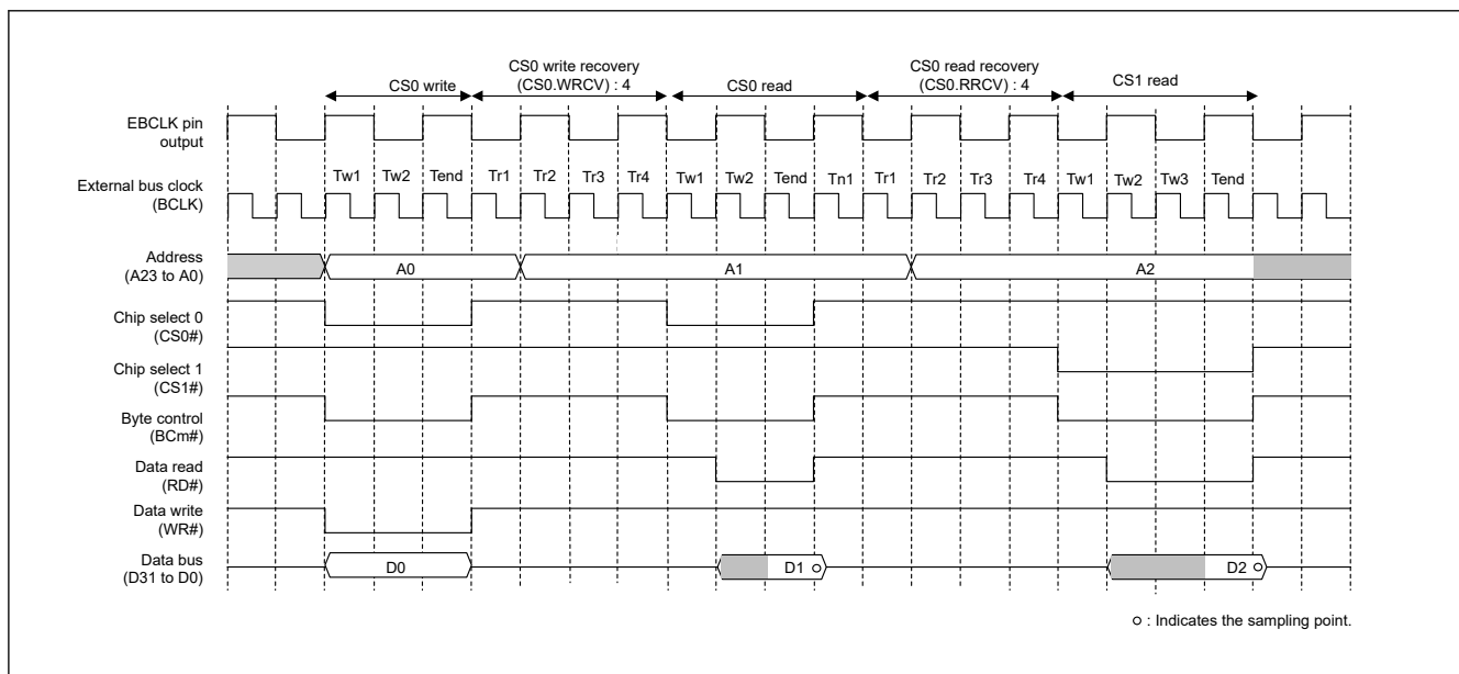
Figure 14.32 Example operation for recovery cycles when BCLK/2 is selected in the EBCLK Pin Output Select bit, with normal access through a separate bus interface ( m = 0 to 3)
