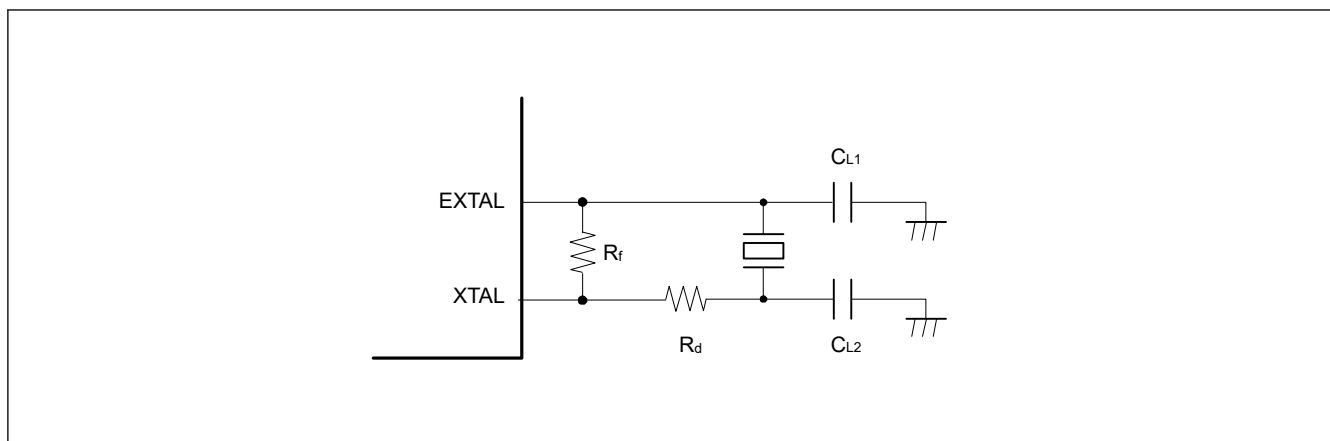
Figure 8.2 Example of a crystal resonator connection
