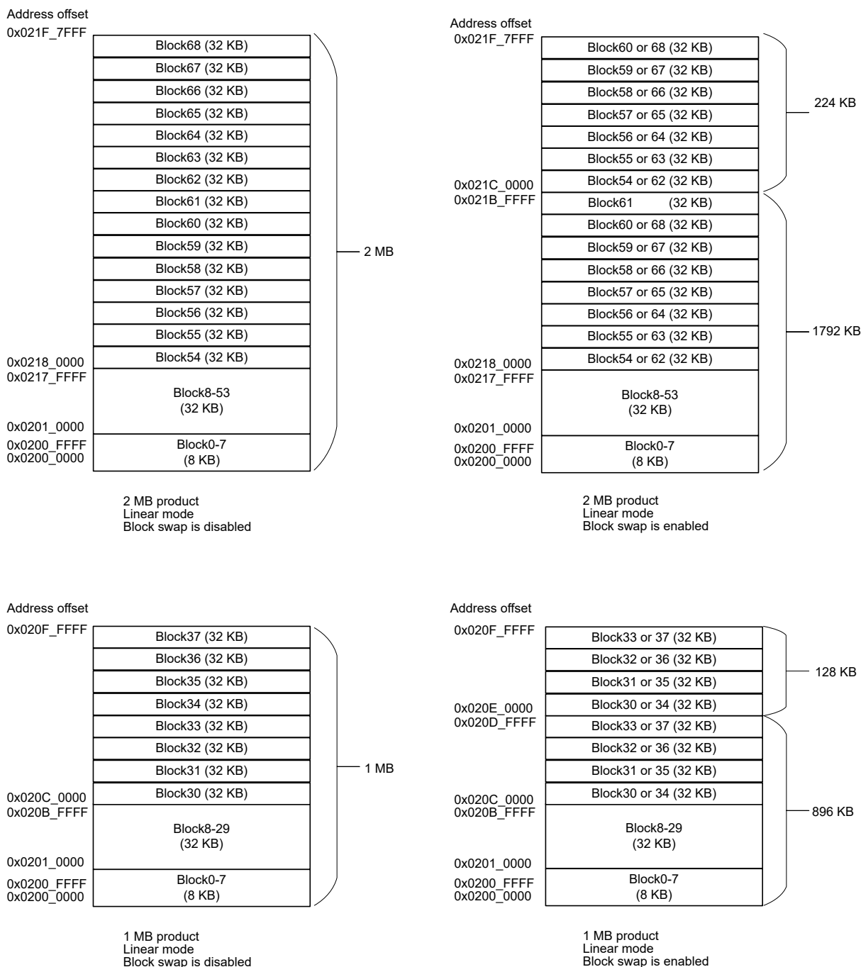
Figure 6.2 Mapping of the flash memory
