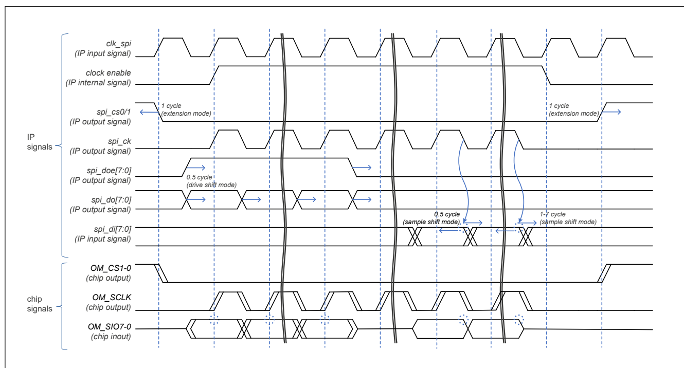
Figure 37.8 Timing control for SDR without OM_DQS
