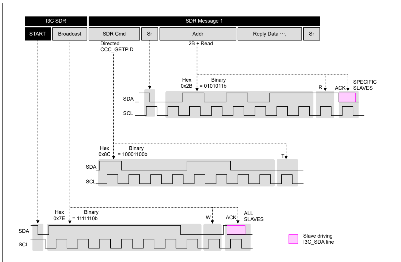
Figure 33.73 Example communication using I3C coding SDR with CCC direct addressing
