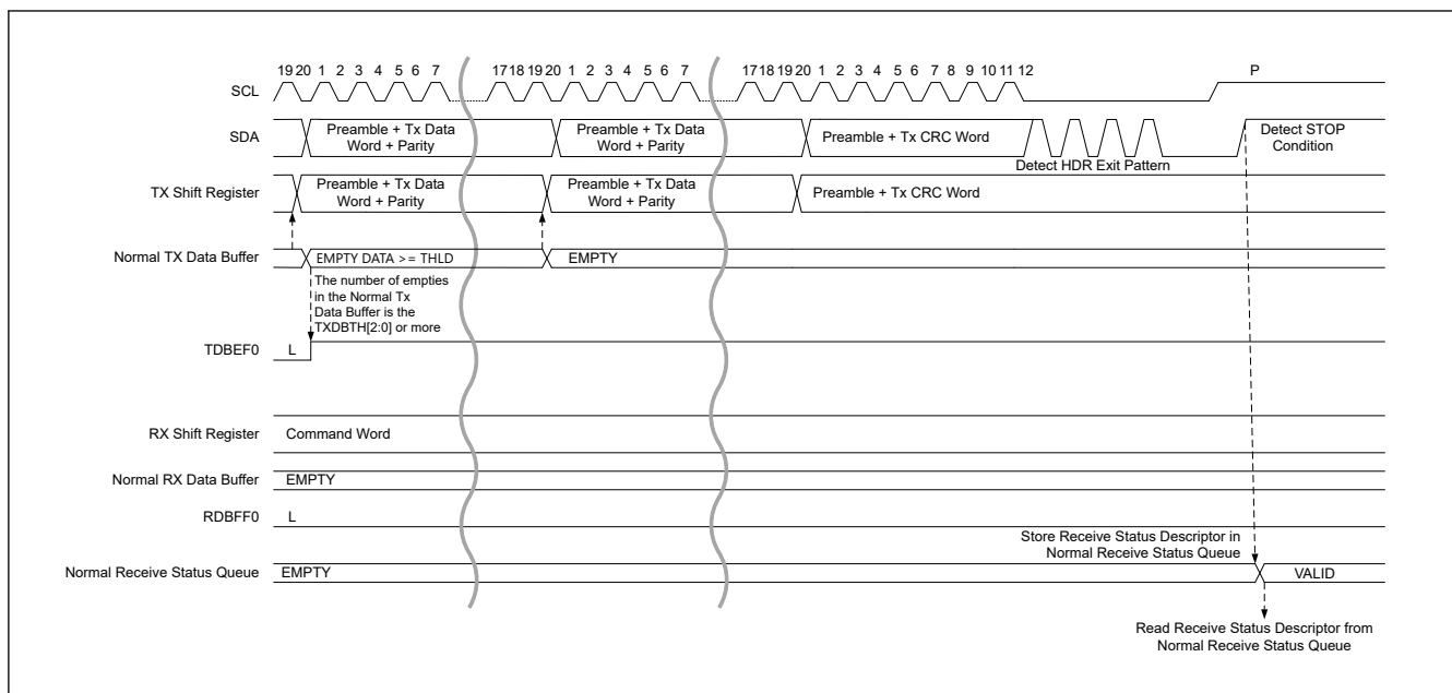
Figure 33.60 HDR data read transfer (HDR-DDR) timing (3/3)
