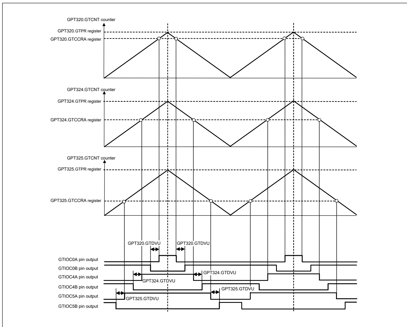
Figure 21.48 Example of 3-phase triangle-wave complementary PWM output with automatic dead time setting
