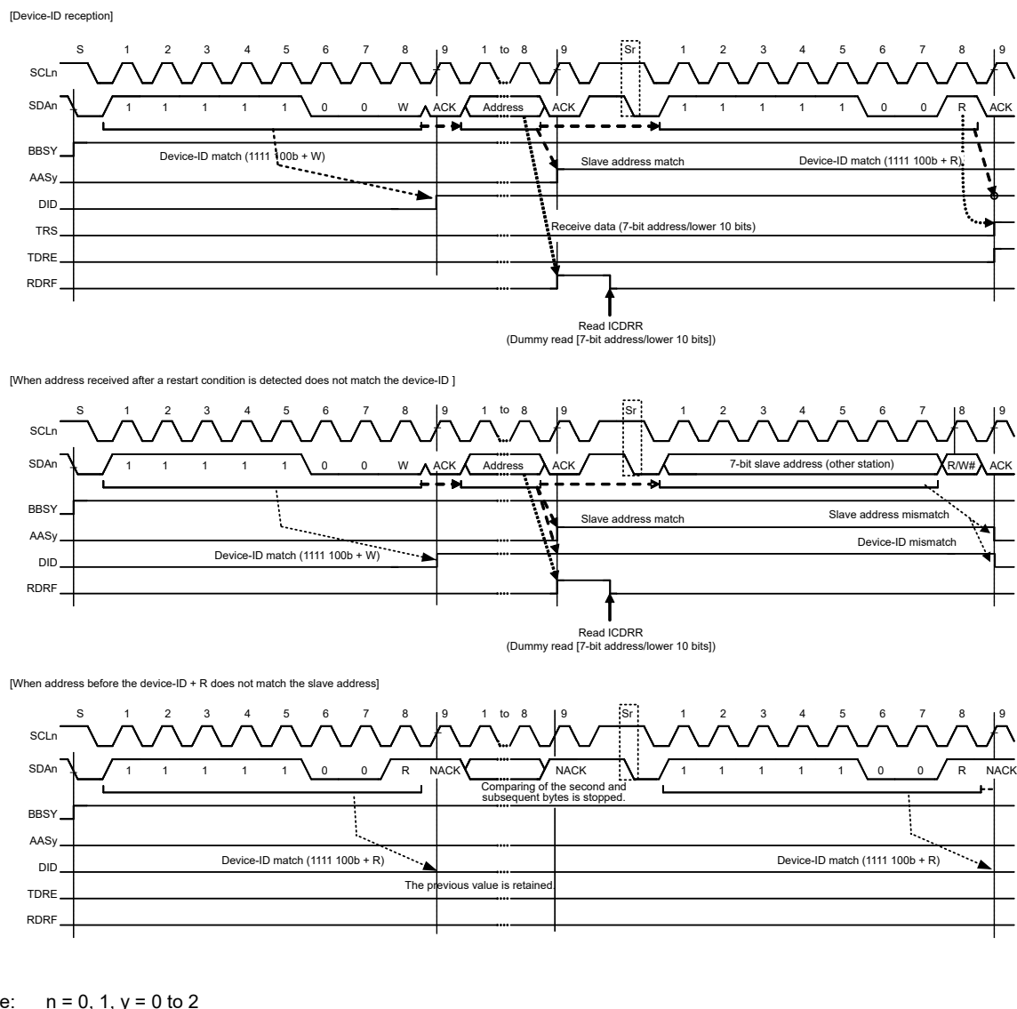
Figure 32.28 AASy and DID flag set and clear timing during reception of device ID
