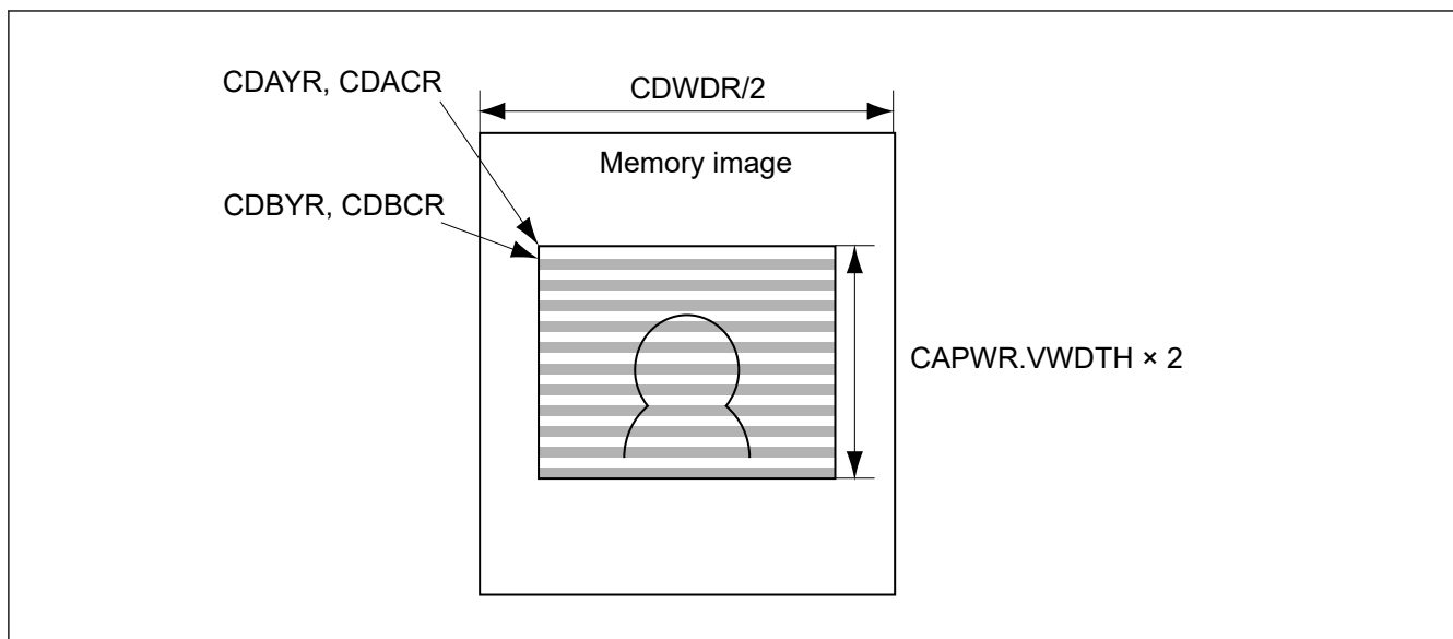
Figure 53.29 Image of storing Interlace input as frame image in memory
