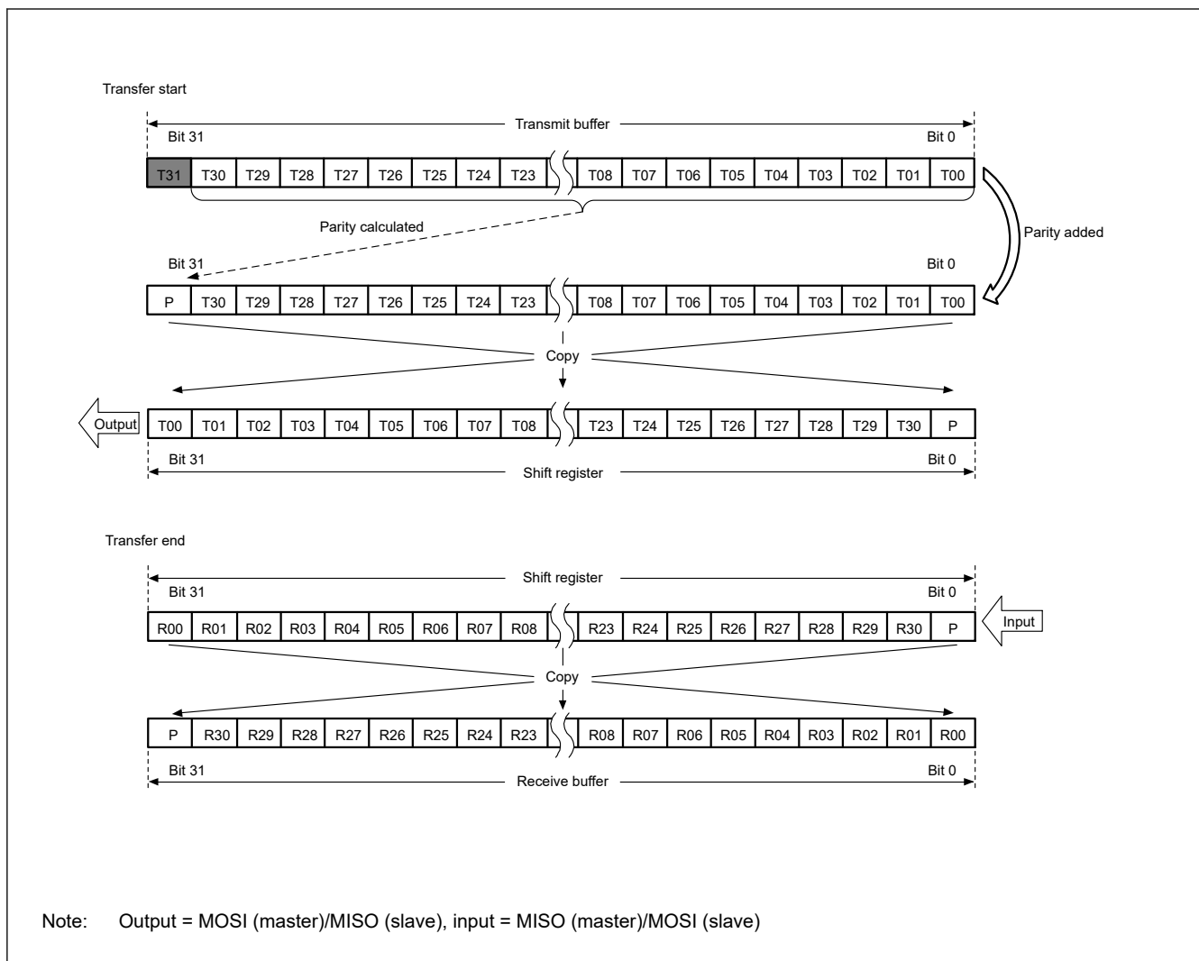
Figure 36.21 LSB-first transfer with 32-bit data and parity enabled
