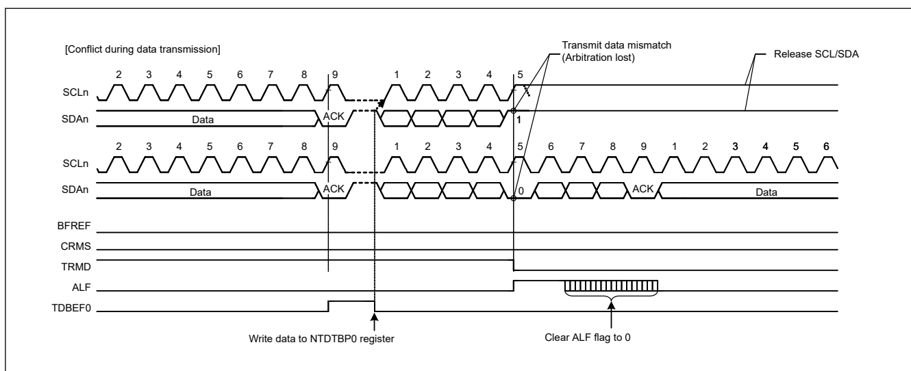
Figure 33.92 Example of slave arbitration-lost detection (SALE = 1)
