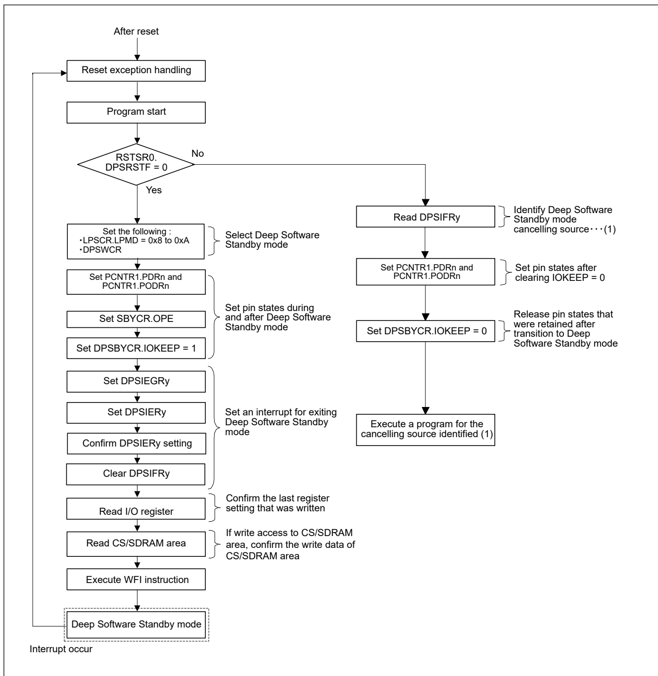
Figure 10.5 Example flow for using Deep Software Standby mode
