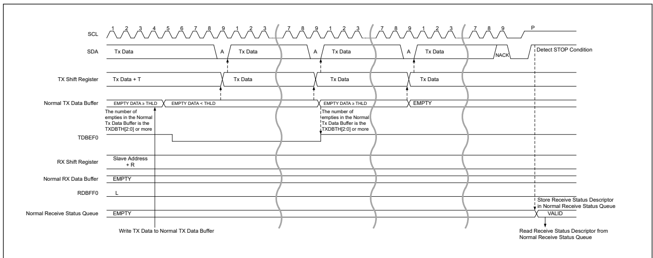
Figure 33.52 Legacy I 2 C message data read transfer timing (2/2)
