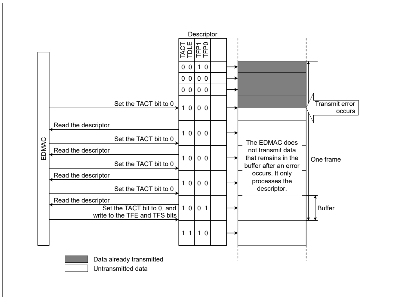
Figure 28.7 EDMAC operation after transmit error occurs
