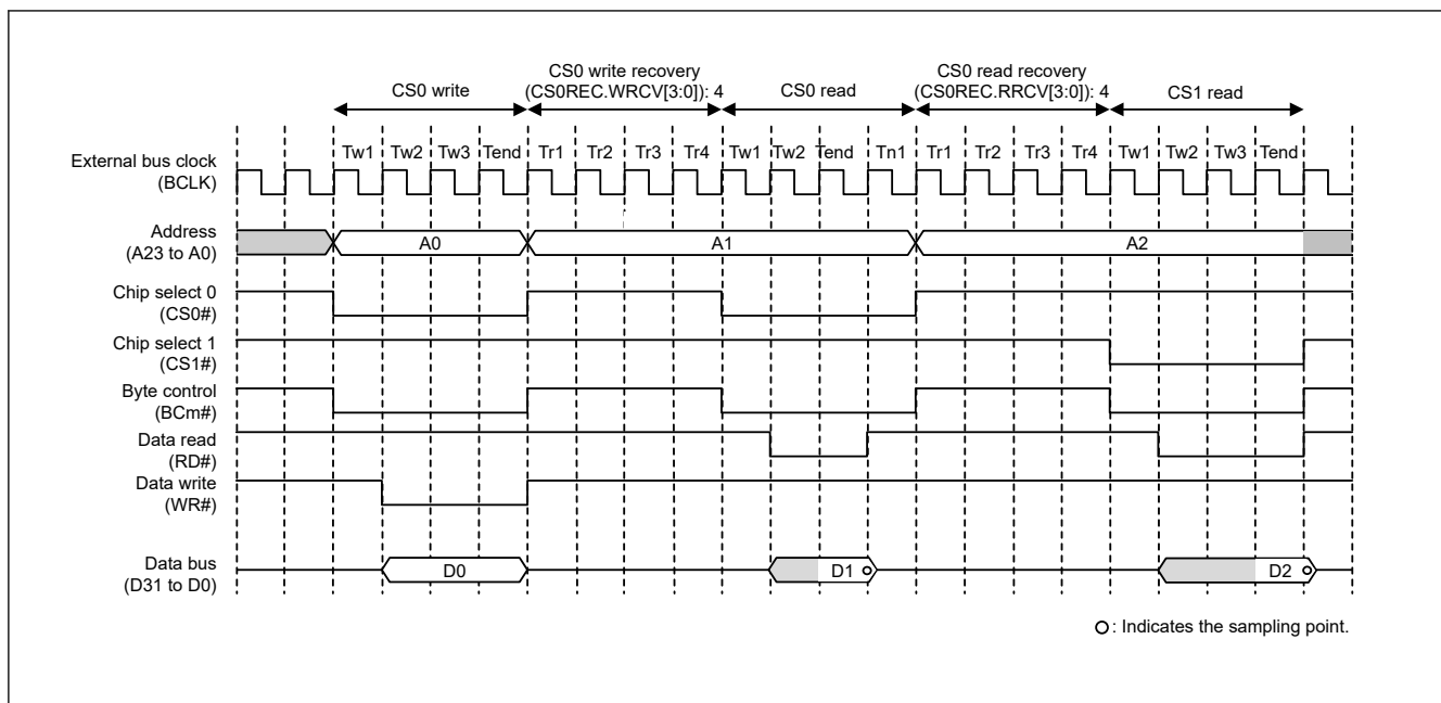
Figure 14.29 Example recovery cycle insertion with separate bus interface (m = 0 to 3)
