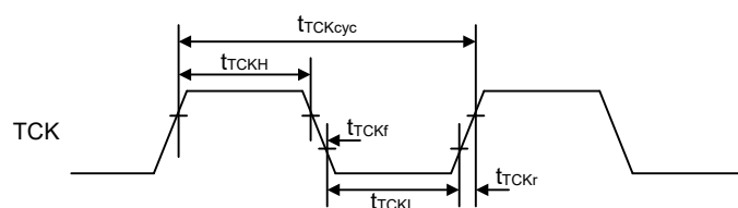
Figure 60.127 Boundary scan TCK timing
