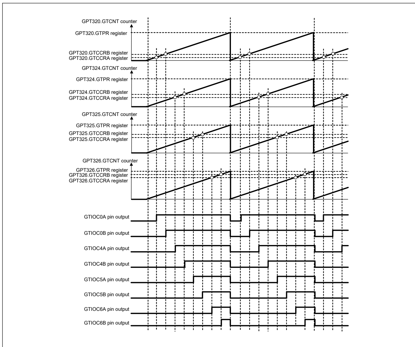
Figure 21.44 Example of synchronized PWM output
