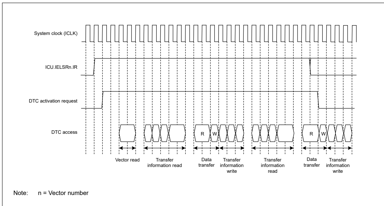
Figure 17.12 Example 3 of DTC operation timing for chain transfer
