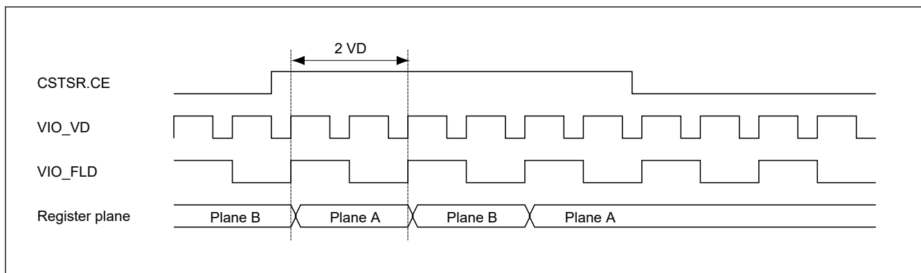
Figure 53.30 Timing for register plane switching when RVS = 0
