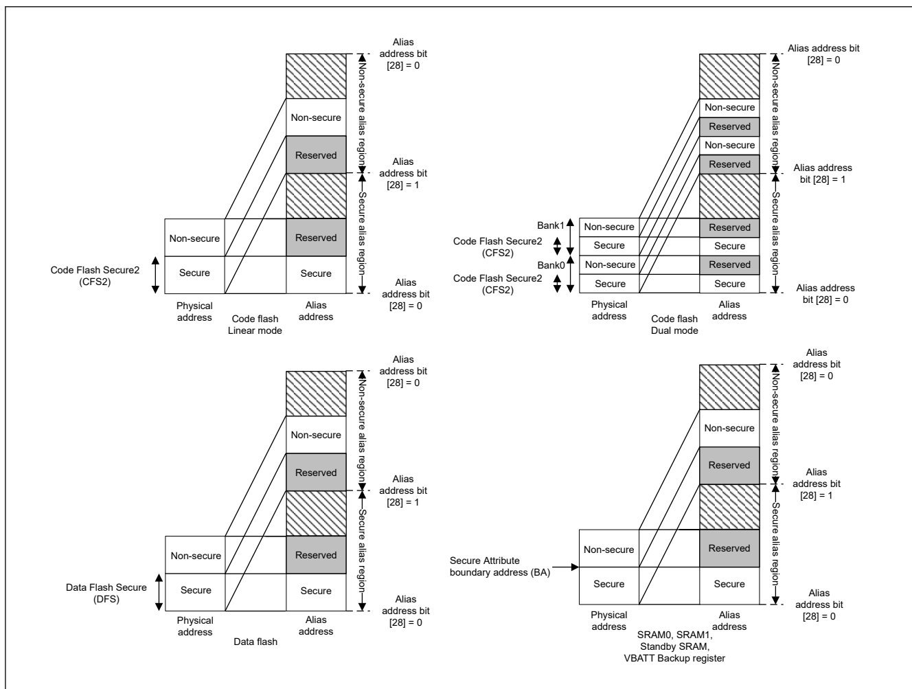
Figure 43.6 Memory mapping
