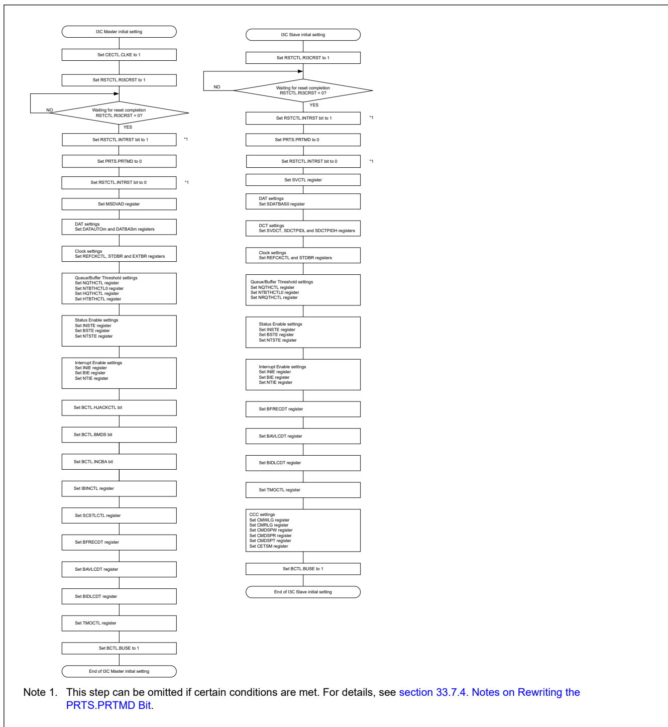
Figure 33.141 Example of each initialization flowchart for I3C master mode and slave mode
