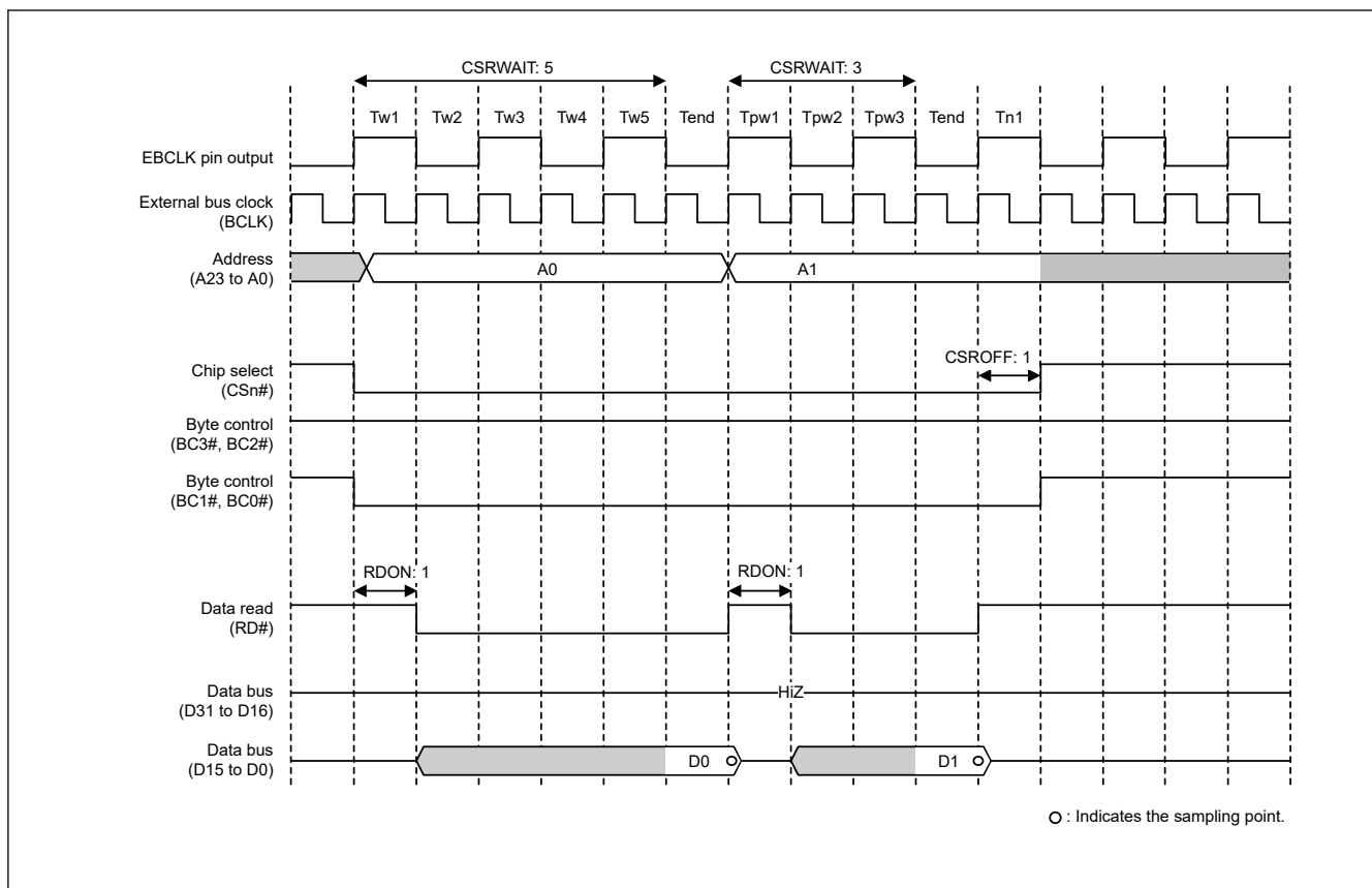
Figure 14.19 Example page read access operation when BCLK/2 is selected in the EBCLK Pin Output Select bit and two rounds of bus access are generated in response to a single transfer request ( n = 0 to 7)
