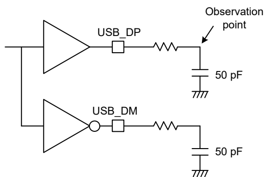
Figure 60.114 Test circuit in full-speed mode
