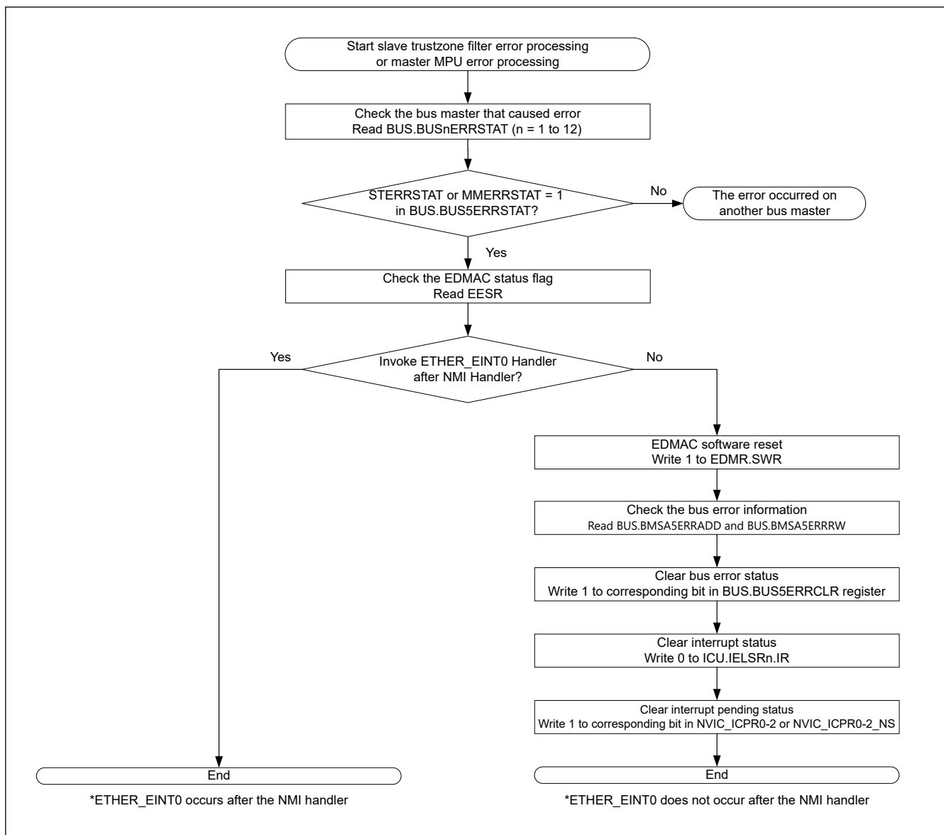
Figure 28.9 Processing for bus transfer error in NMI handler
