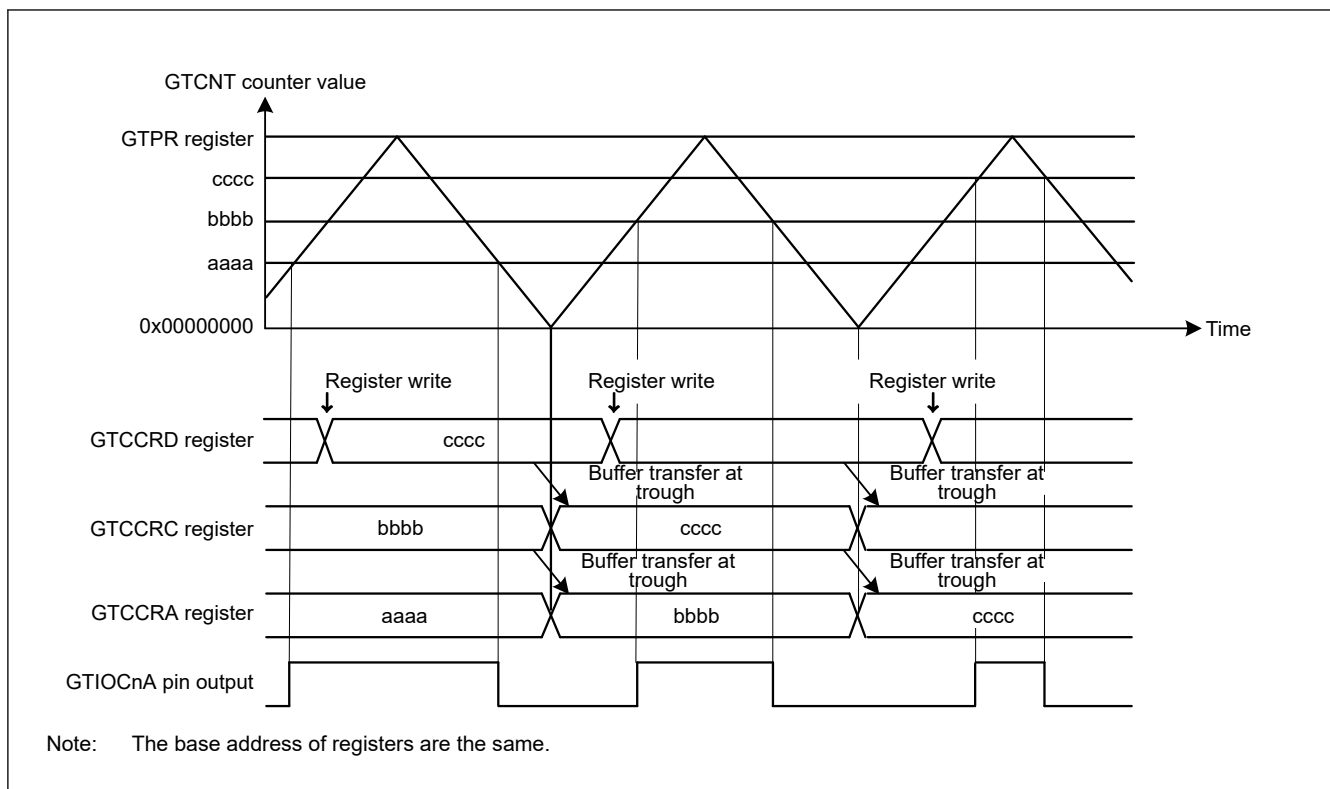
Figure 21.14 Example of GTCCRA double buffer operation with output compare, triangle waves, buffer operation at trough, output toggled at GTCCRA compare match, and output retained at cycle end
