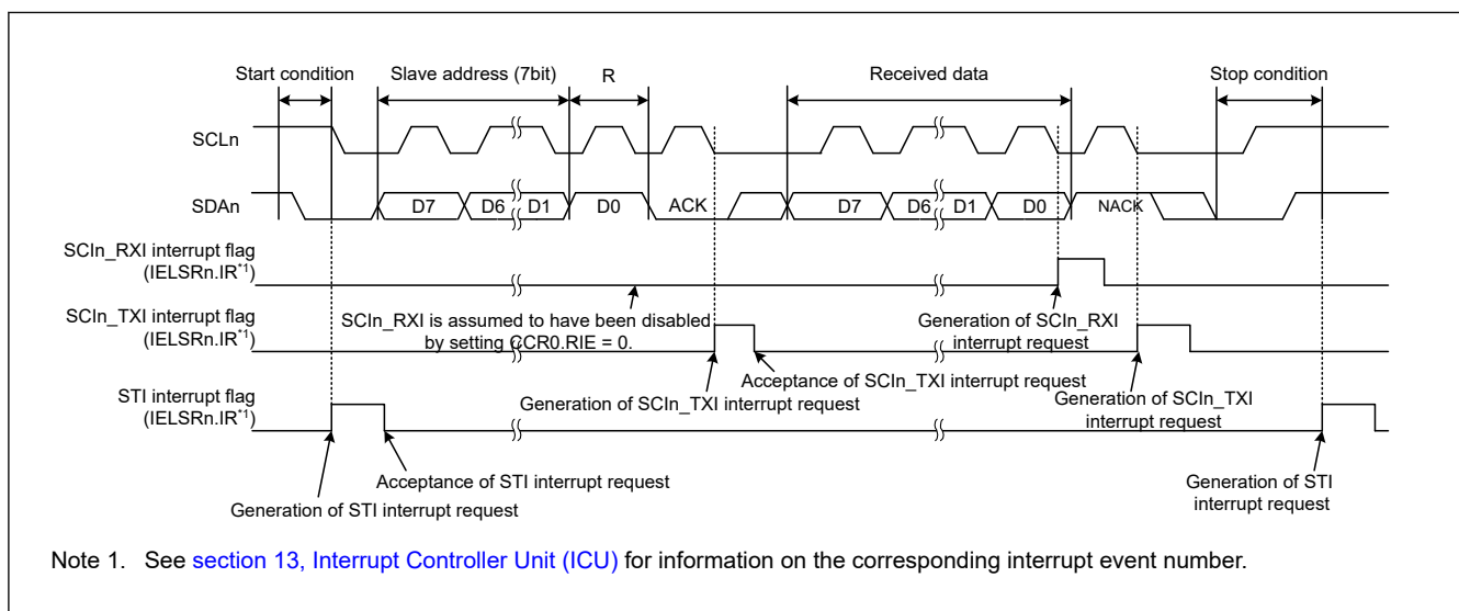
Figure 31.94 Example operations for master reception in simple IIC mode with 7-bit slave addresses, transmission interrupts, and reception interrupts (ICR.IICINTM = 1)
