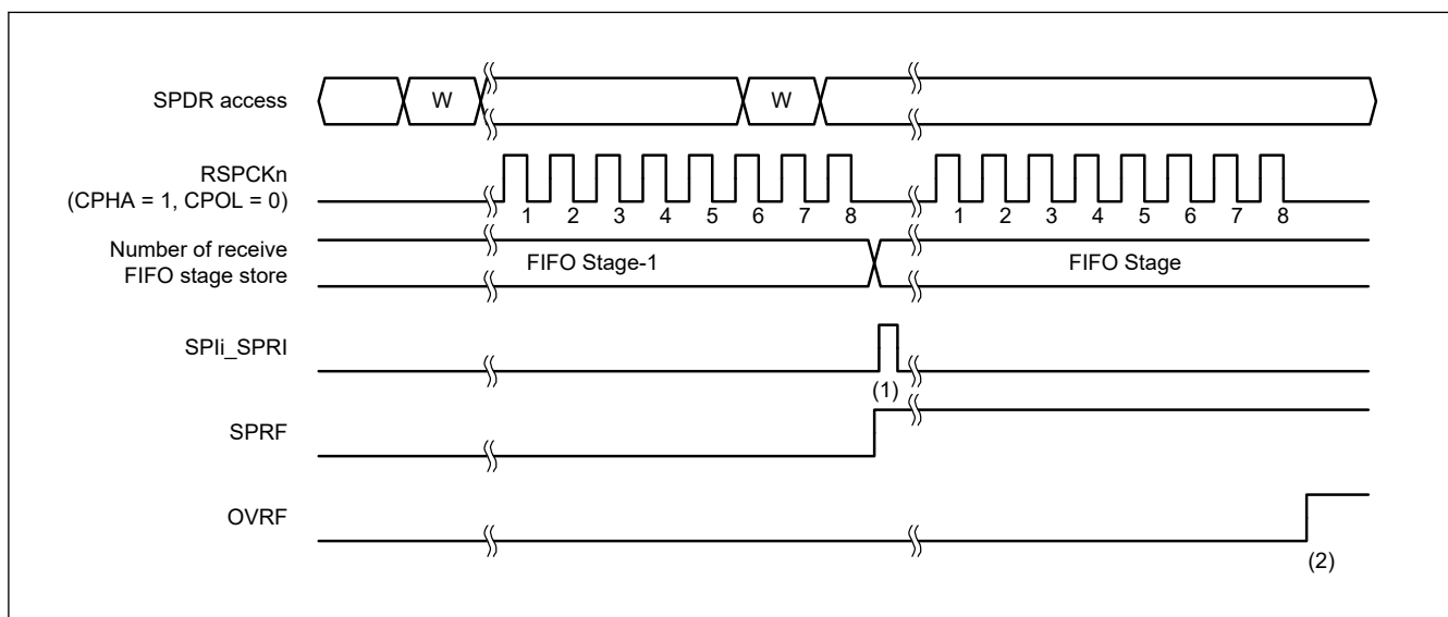
Figure 36.30 Operation example when SPCR.TXMD[1:0] = 00b
