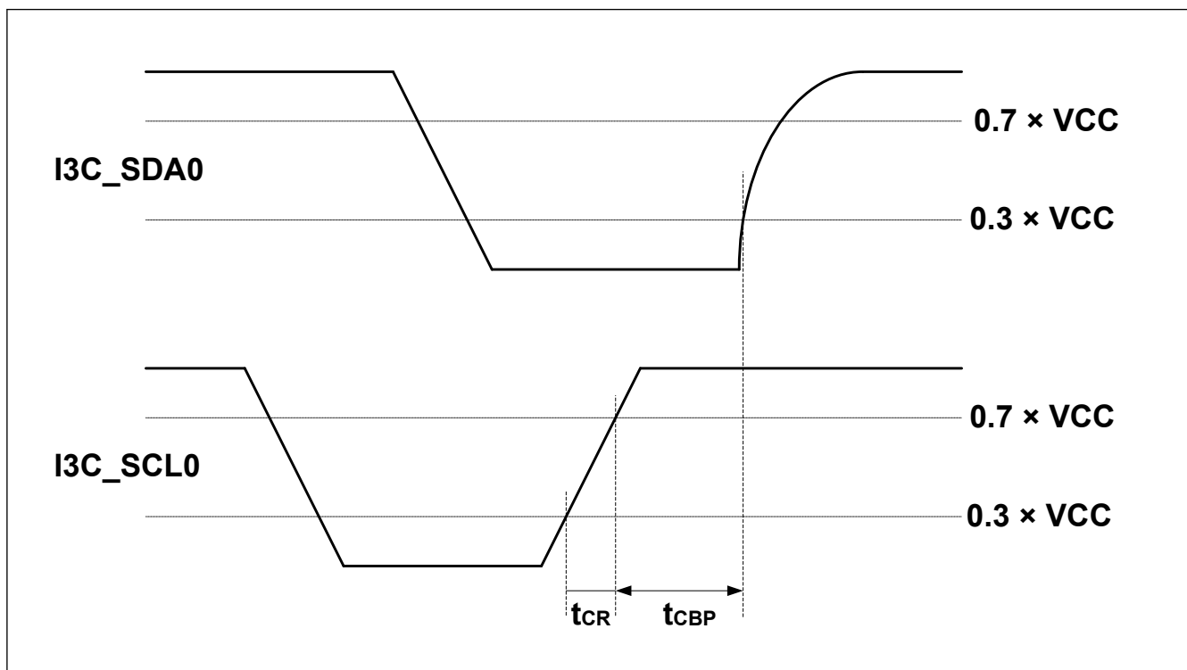
Figure 60.77 I3C STOP condition Timing
