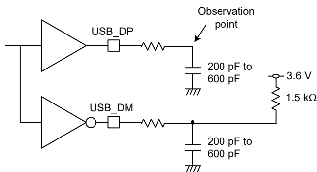
Figure 60.112 Test circuit in low-speed mode
