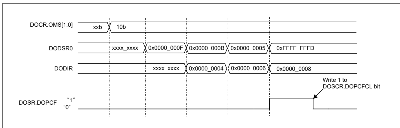
Figure 49.9 Example of Operation in Data Subtraction Mode
