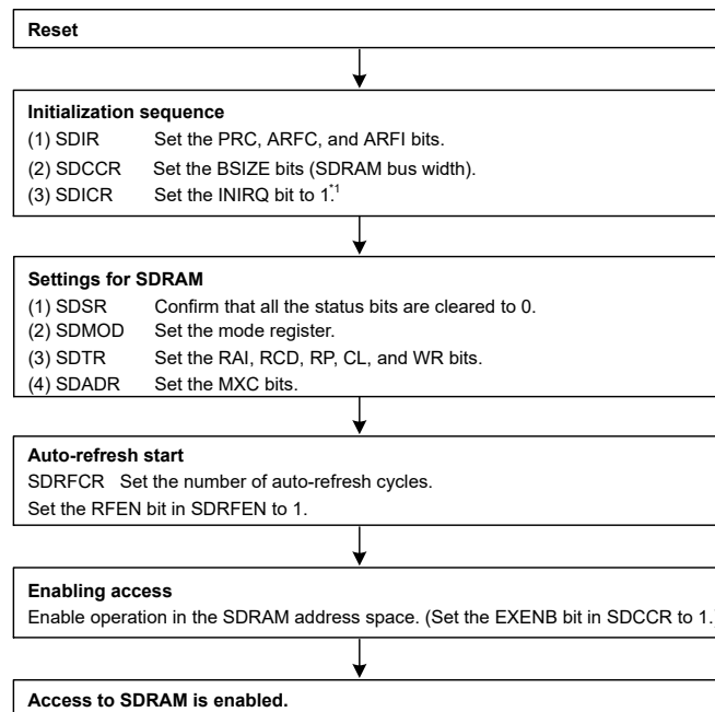
Figure 14.49 SDRAMC setting procedure
