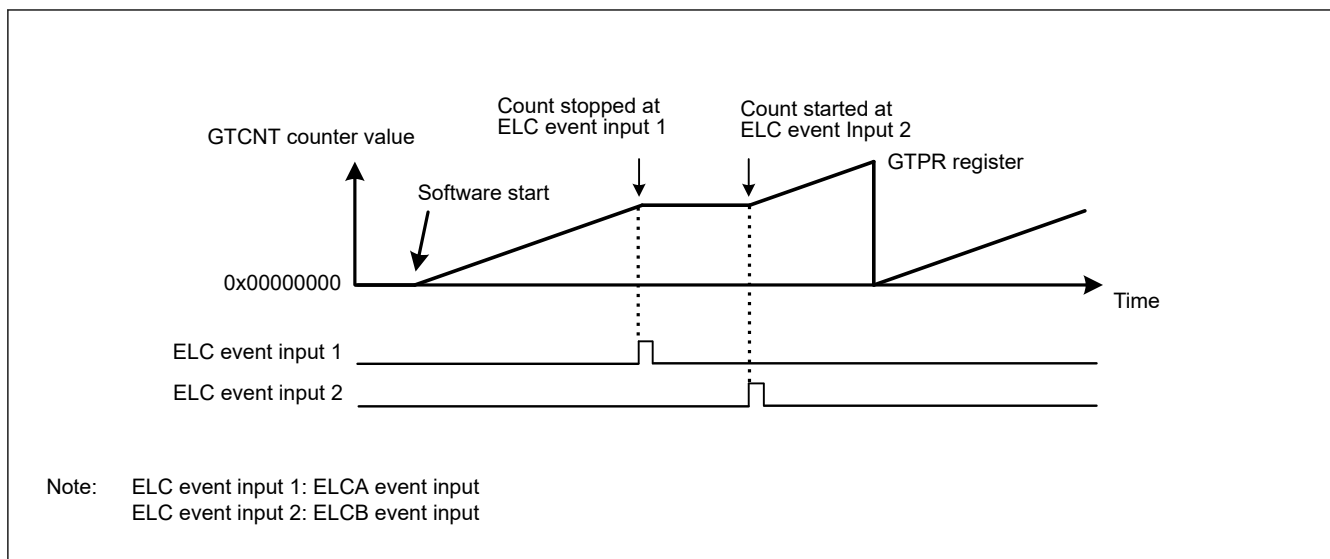
Figure 21.33 Example of count stop operation by hardware source started by software, stopped at ELCA input, and restarted at ELCB input
