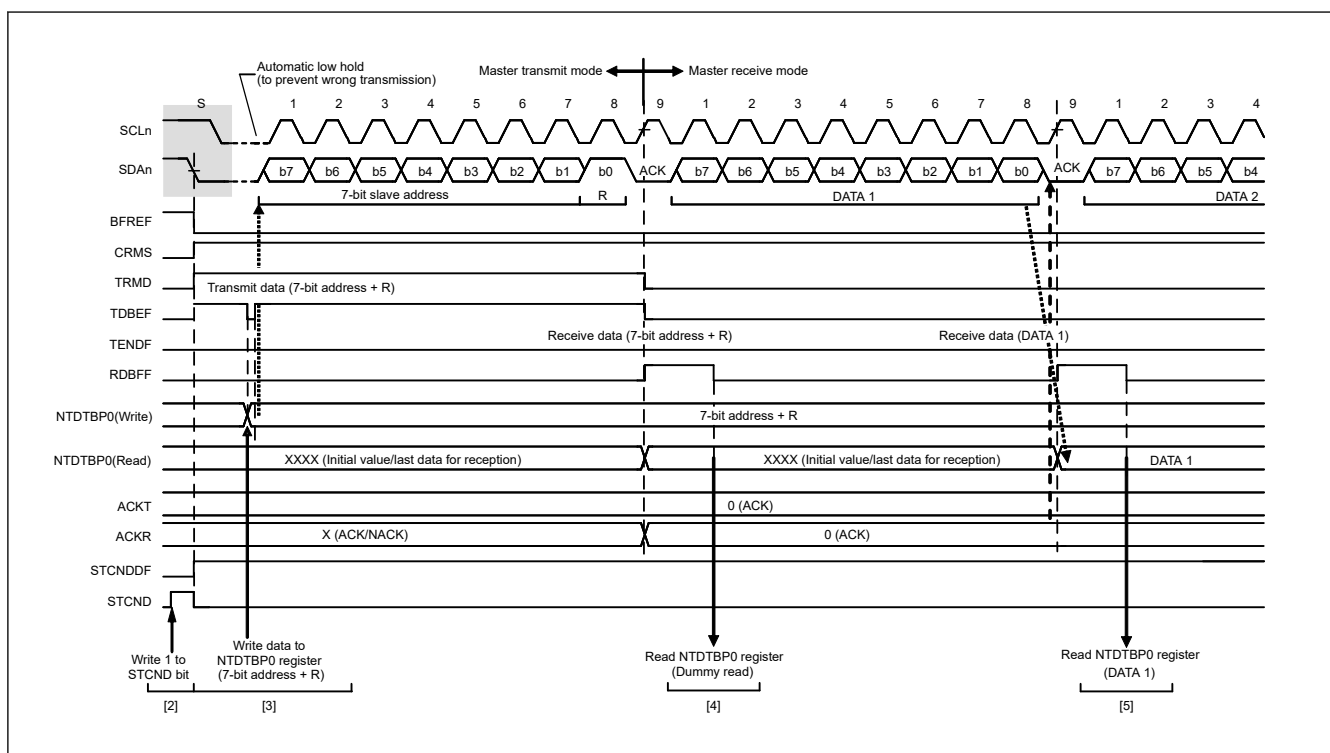
Figure 33.9 Master receive operation timing (1) (7-bit address format, when ACKTWE = 0)
