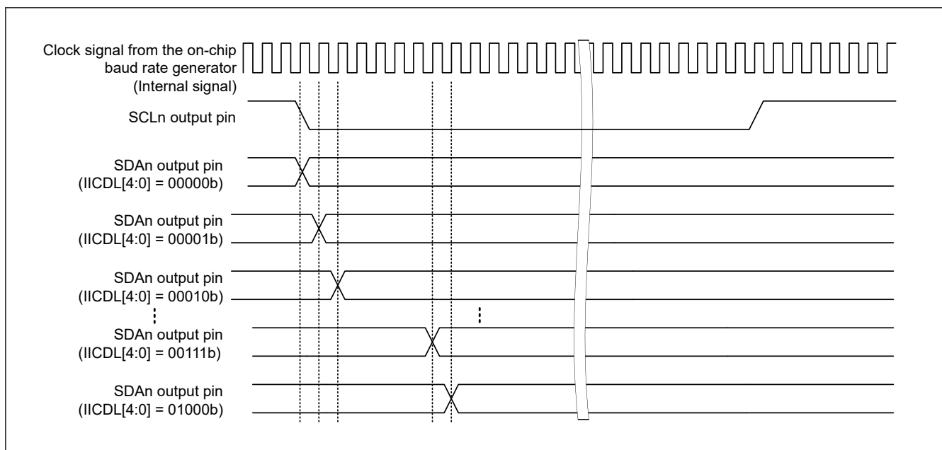
Figure 31.90 Timing of delays in SDAn output
