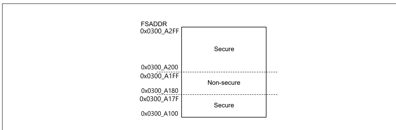
Figure 52.41 Secure and Non-secure region in option-setting memory for Secure alias
