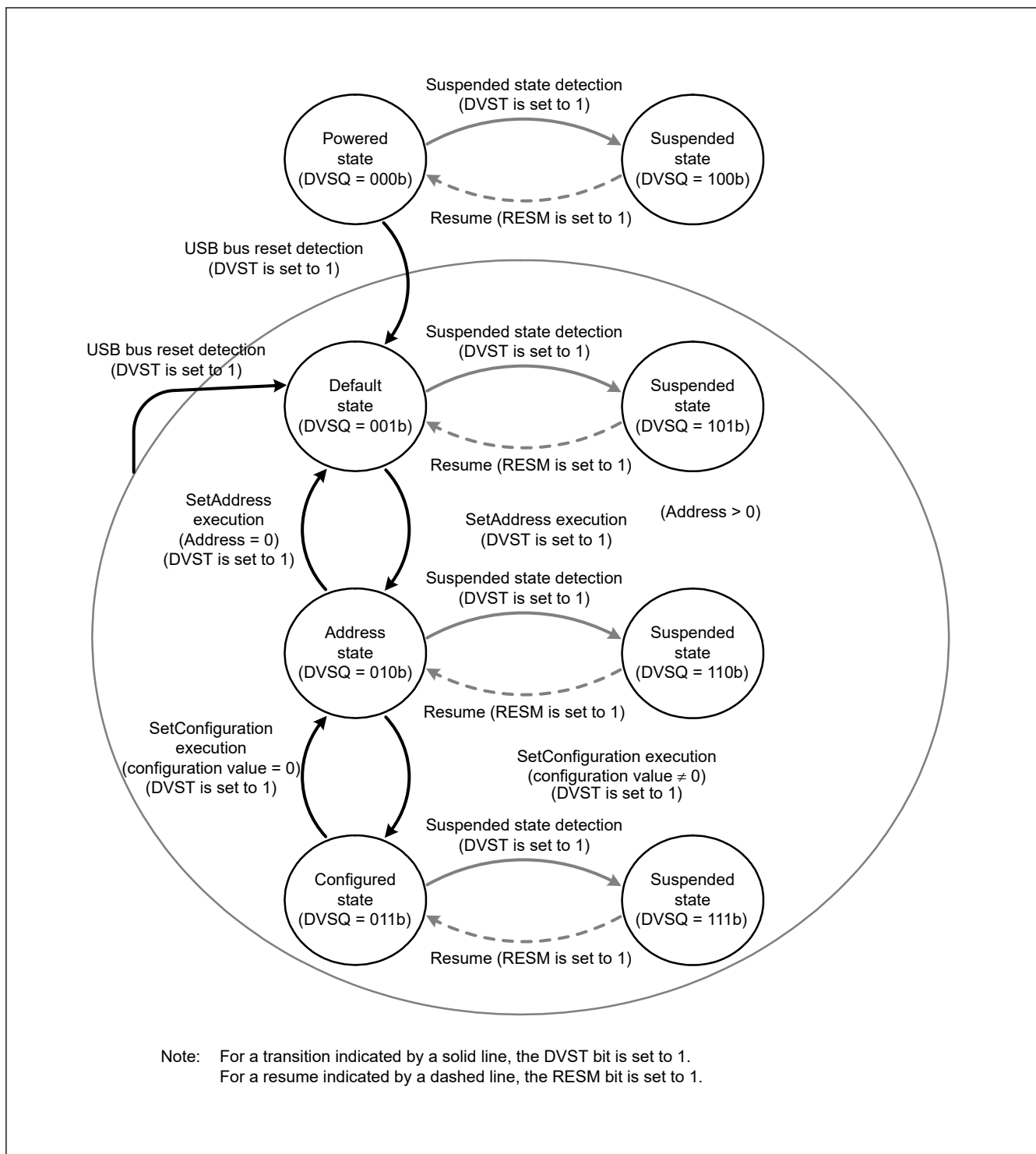
Figure 29.14 Device state transitions
