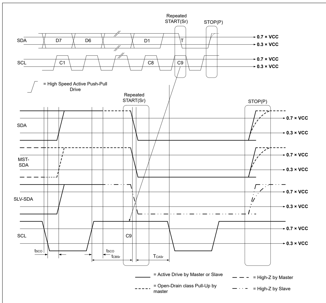
Figure 60.82 T-Bit When Master Ends Read with Repeated START and STOP
