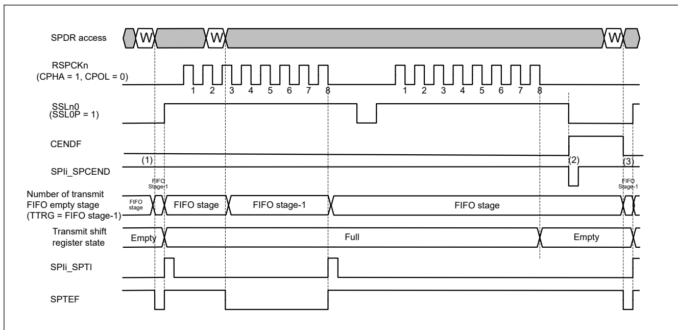
Figure 36.40 Example of Communication End Interrupt Operation (Transmit-Receive/Transmit Slave mode on SPI Operation/Motorola-SPI)
