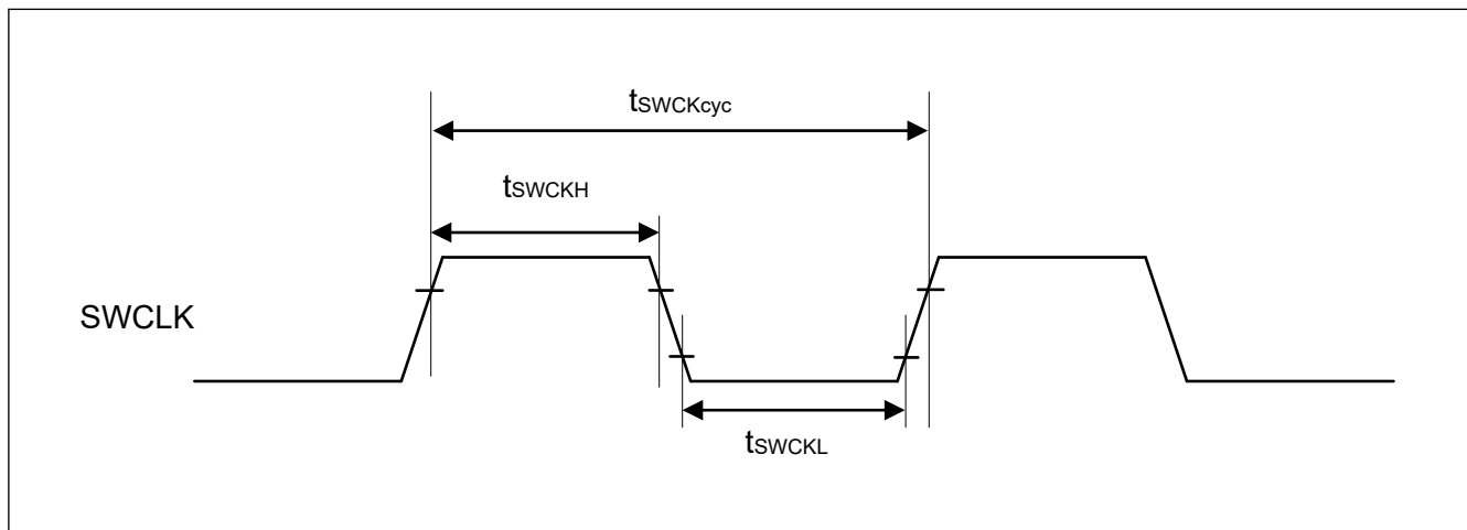
Figure 60.133 SWD SWCLK timing
