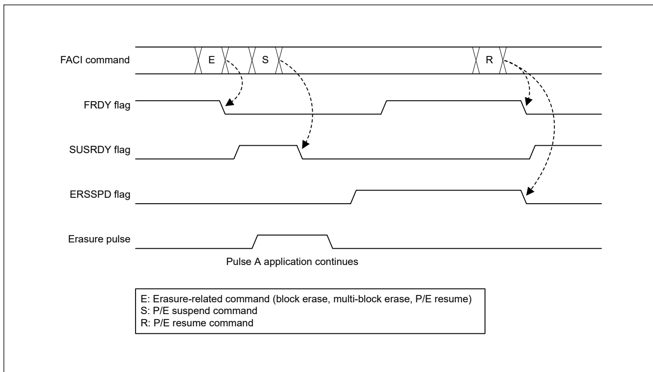
Figure 52.20 Suspension during erasure (eraser priority mode)
