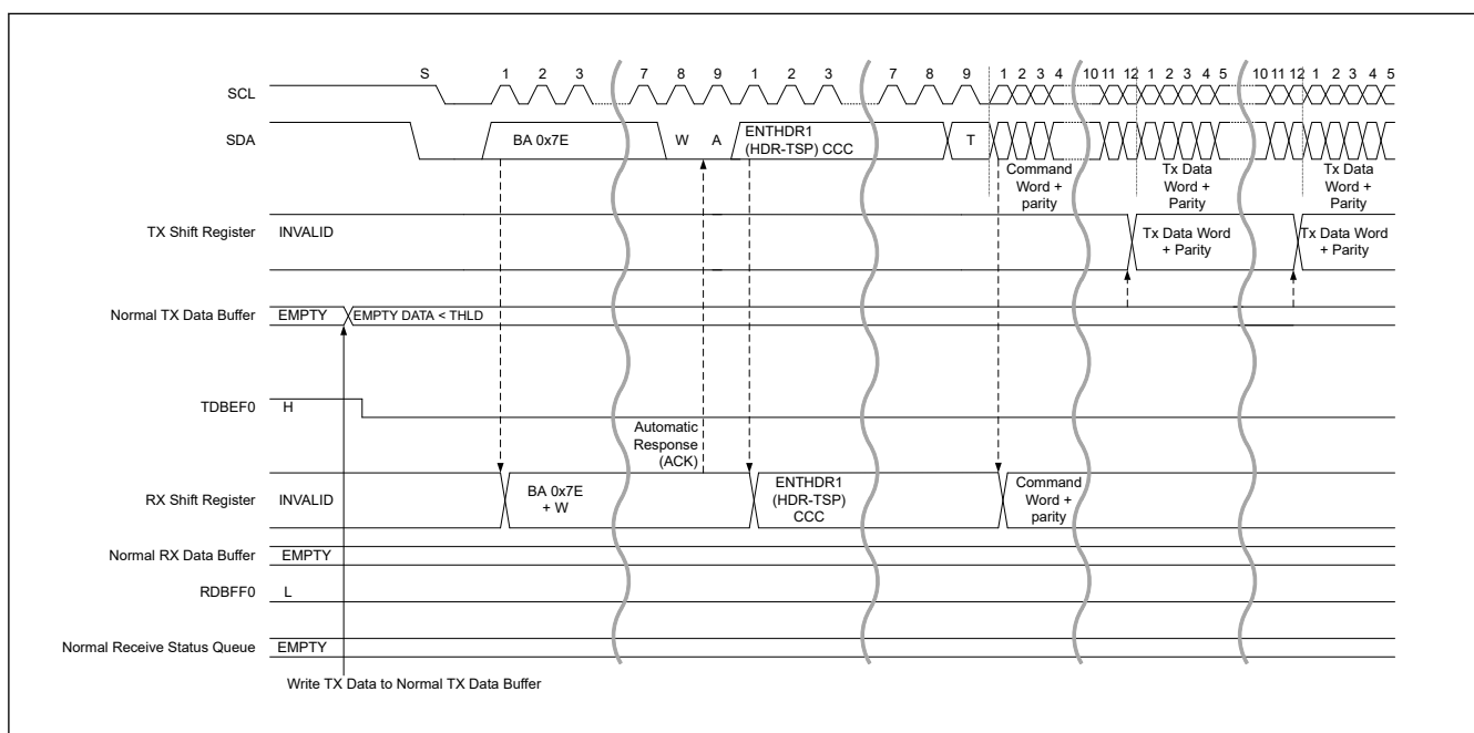
Figure 33.61 HDR data read transfer (HDR-TSP, TSL) timing (1/2)
