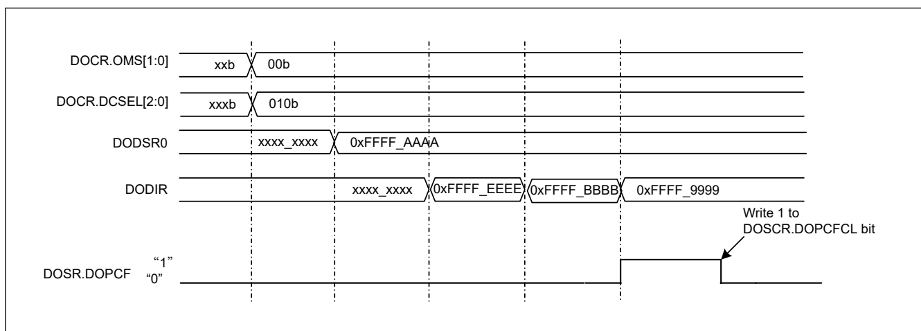
Figure 49.4 Example of Operation in Data Comparison Mode (Detection condition: Lower)
