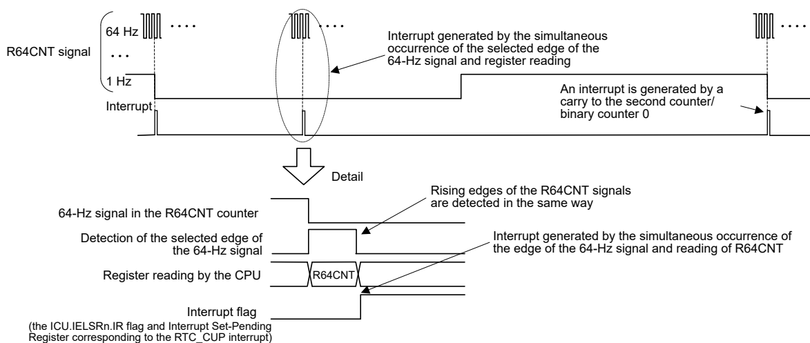
Figure 24.12 Timing for the carry interrupt (RTC_CUP)
