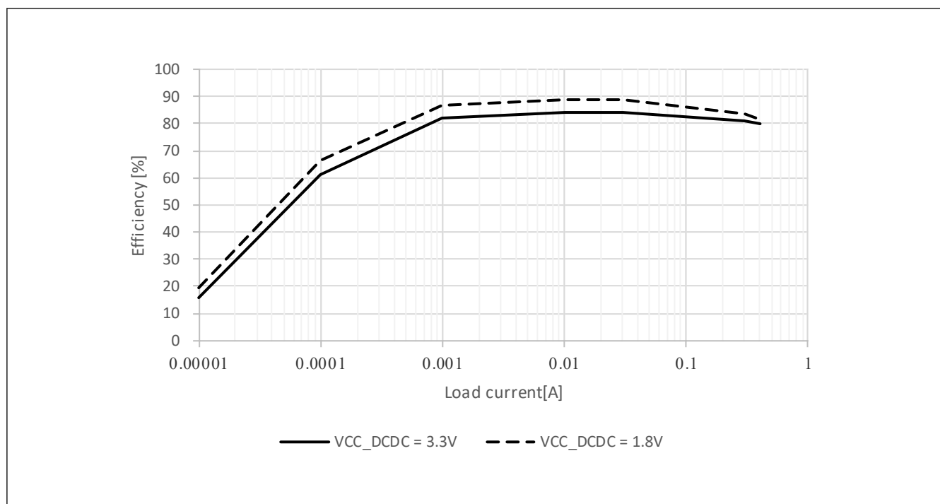
Figure 60.11 Typical DCDC efficiency (%) vs load current (A) in Low-speed mode and Software Standby mode, T_j = 25\text{ }^{\circ}\text{C}
