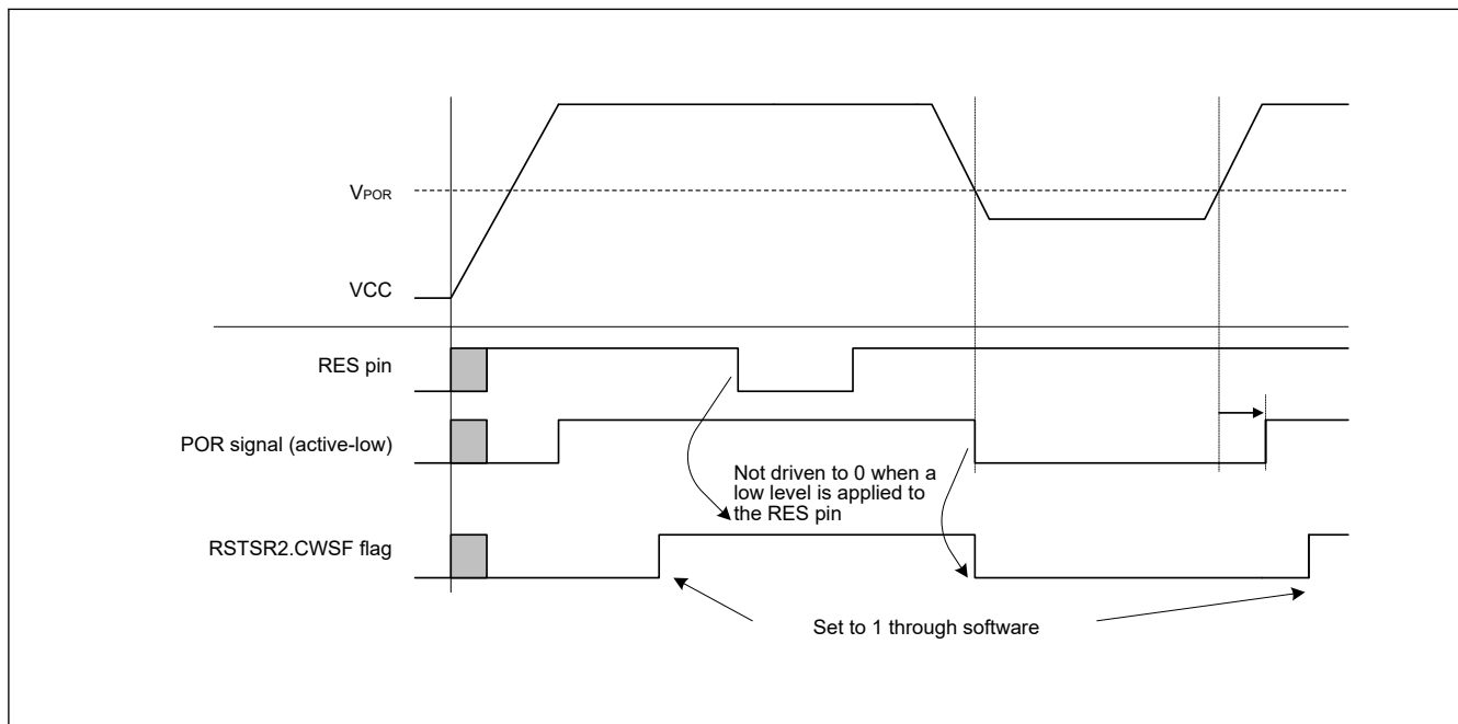
Figure 5.4 Example of cold/warm start determination operation
