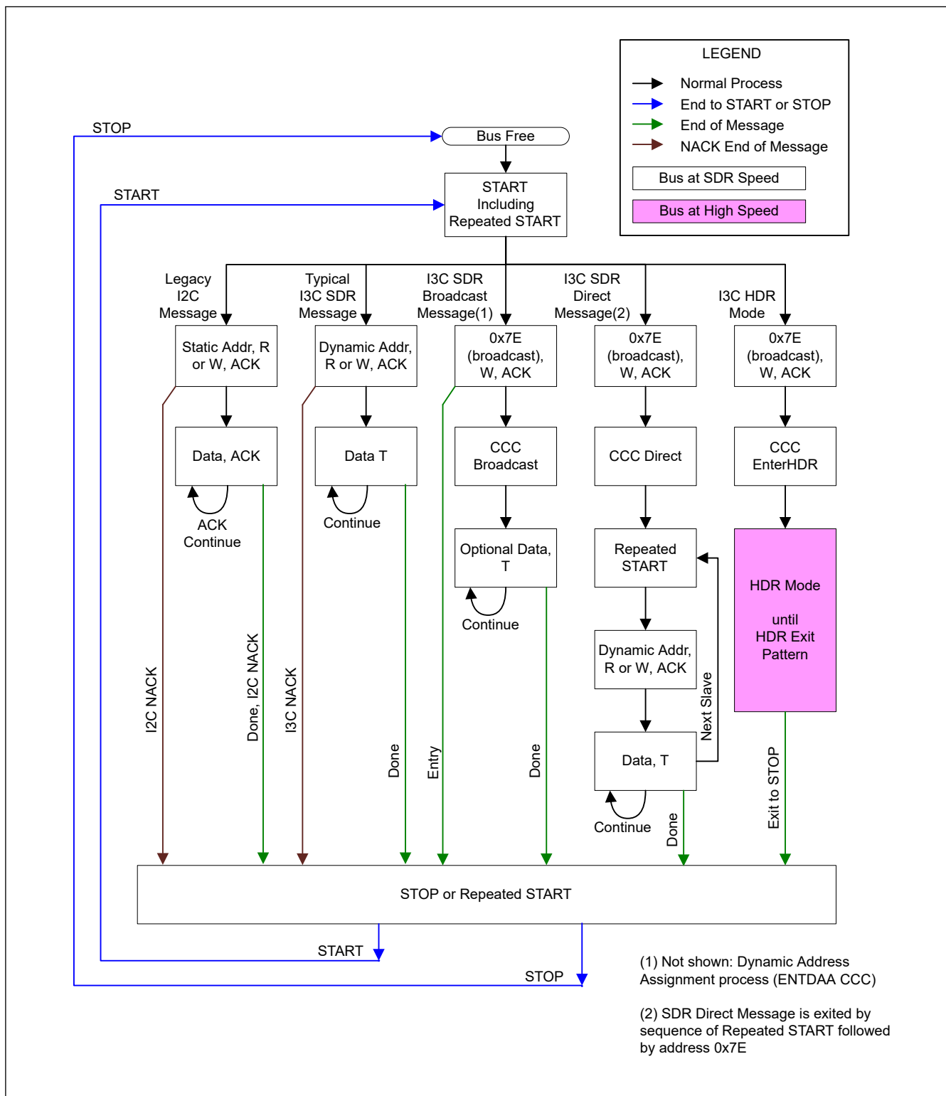
Figure 33.142 I3C communication flow
