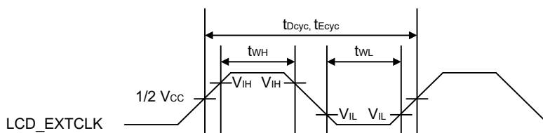
Figure 60.103 LCD_EXTCLK clock timing
