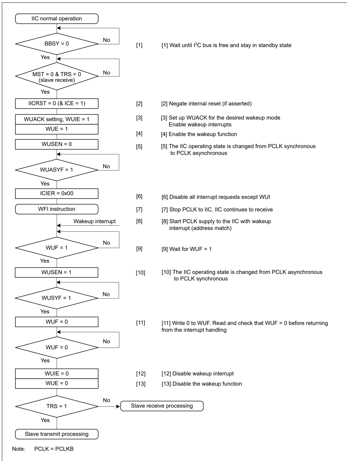
Figure 32.33 Example operation of normal wakeup mode 2 when wakeup is triggered by a wakeup interrupt on match of the slave address
