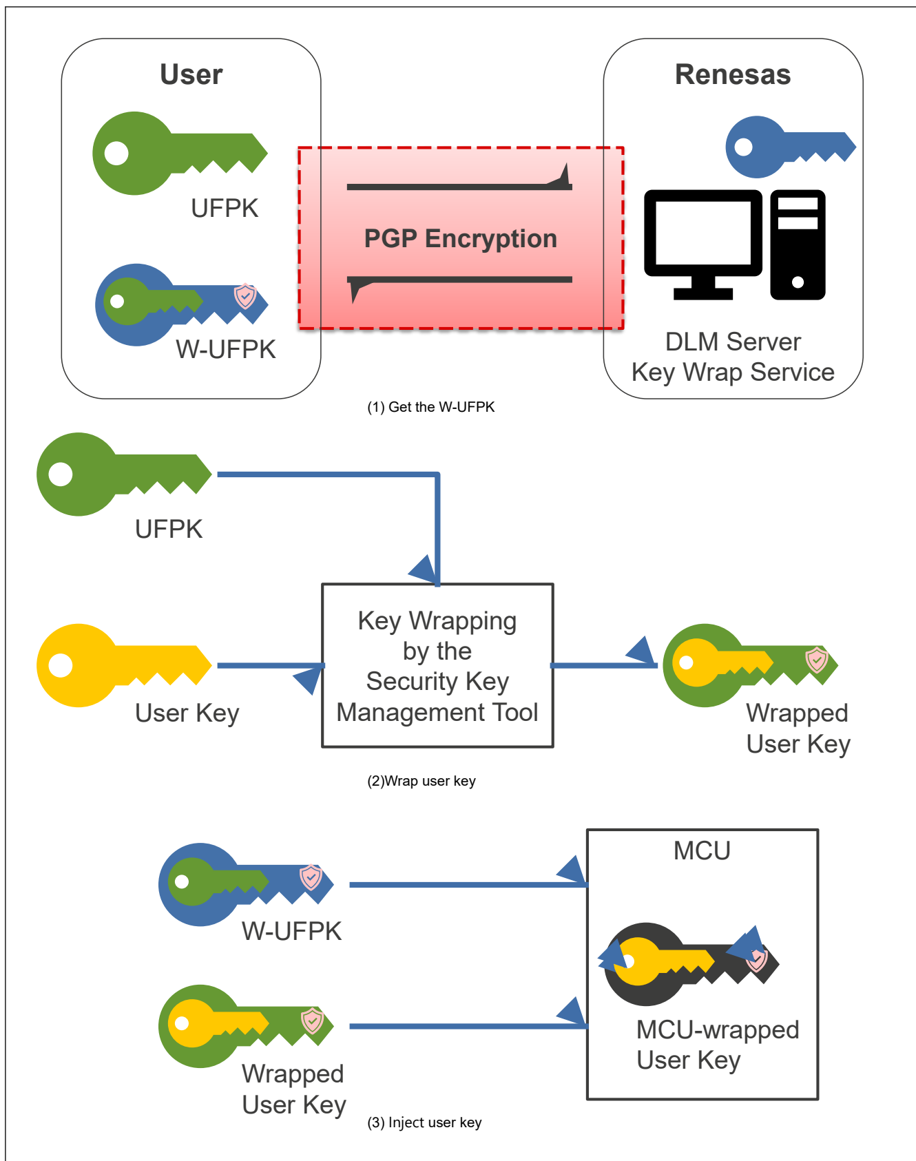
Figure 43.9 Key injection
