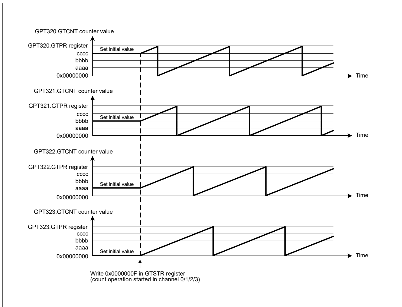
Figure 21.39 Example of software phase start with the same count cycle (GTPR register value)
