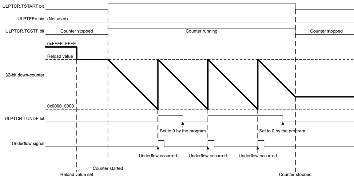
Figure 23.4 Operation example in event counter & continuous & count enable mode (with the ULPTIOC.TIOGT0 bit set to 0)
