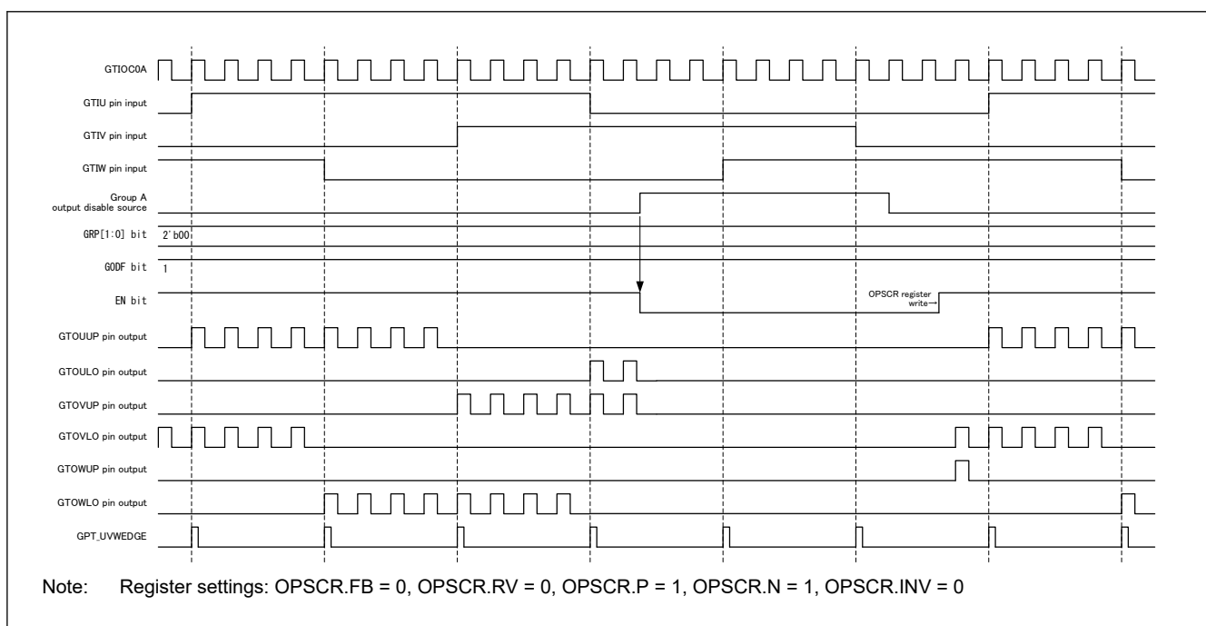
Figure 21.67 Example of group output disable control operation
