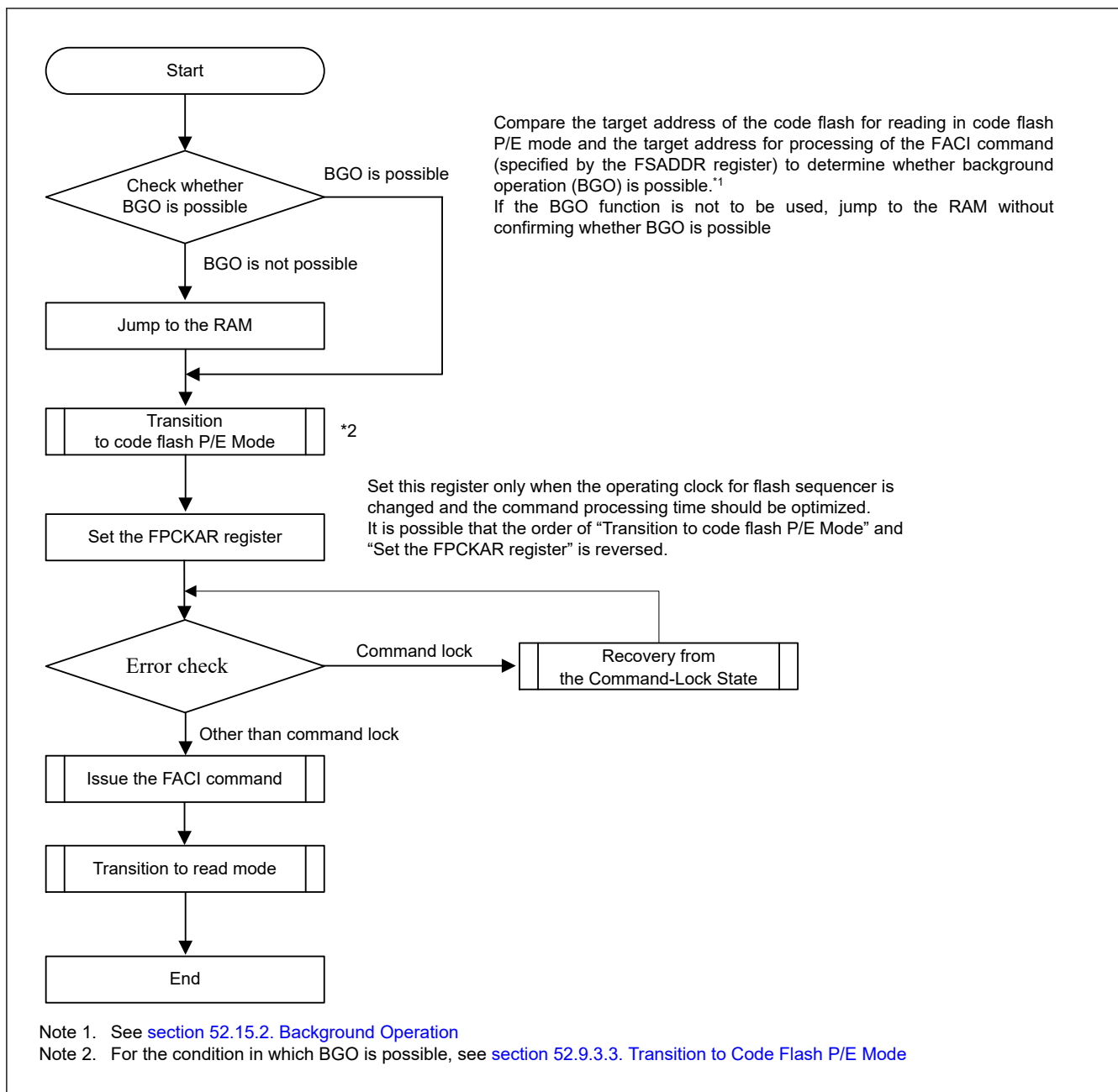
Figure 52.8 Overview of command usage in code flash P/E mode
