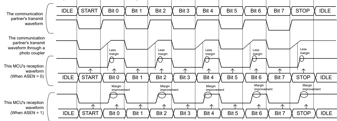
Figure 31.28 Example of improvement in reception margin by the reception sampling timing adjustment function
