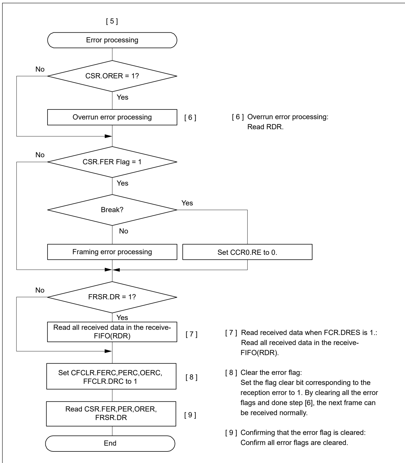
Figure 31.44 Example Flowchart of Serial Reception in Multi-Processor Mode (2) (FIFO selected)
