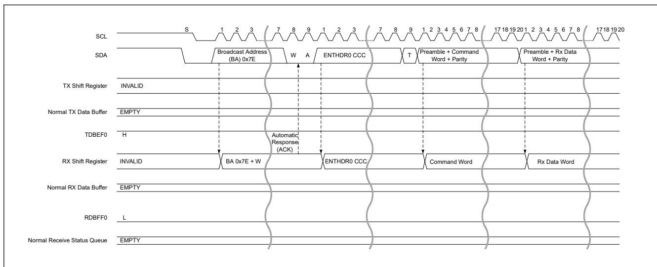
Figure 33.53 HDR data write transfer (HDR-DDR) timing (1/3)
