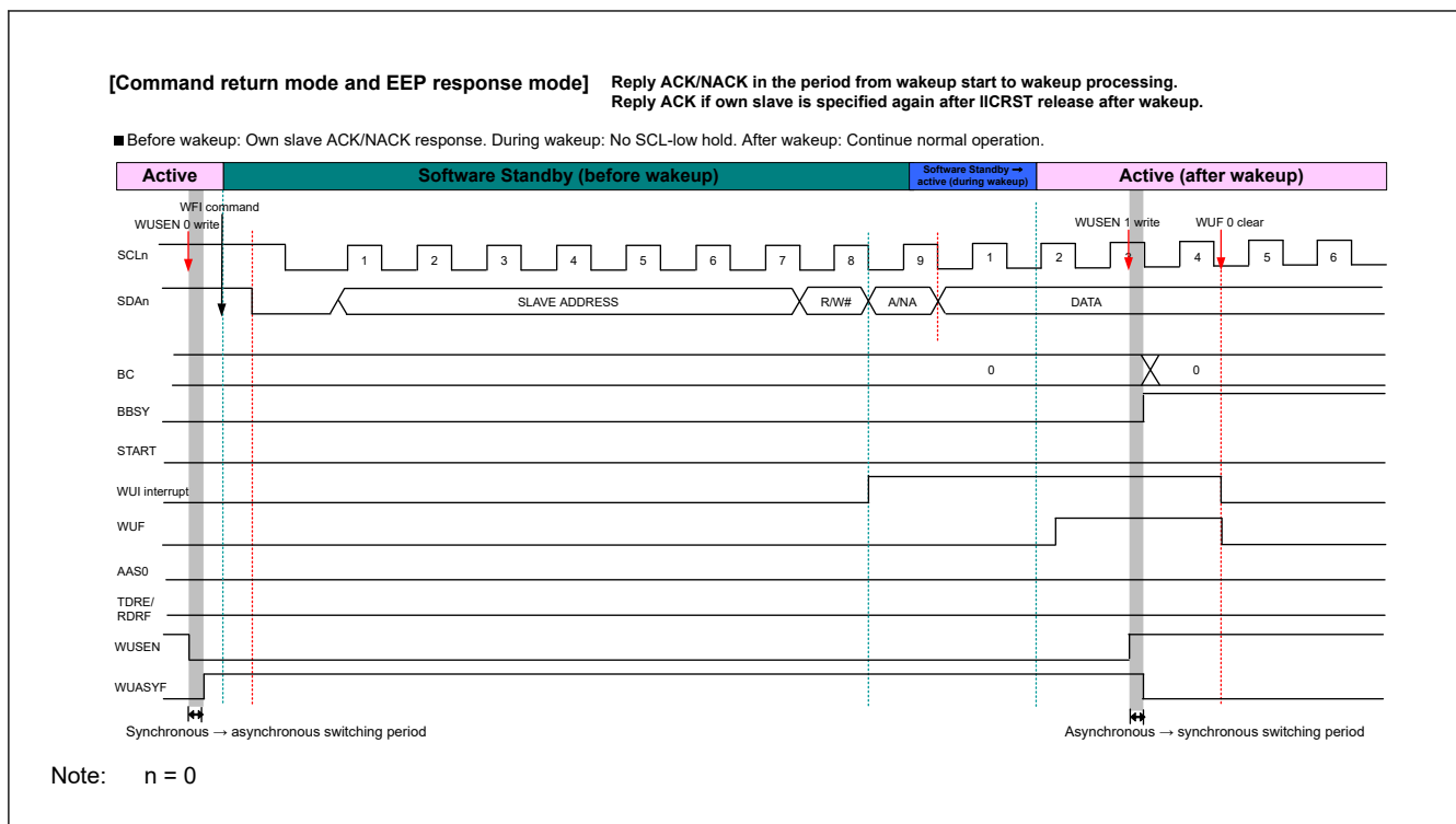
Figure 32.37 Timing of command recovery and EEP response modes
