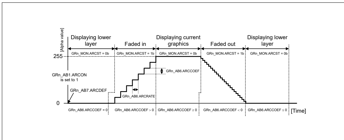
Figure 56.9 Updating of alpha blending value
