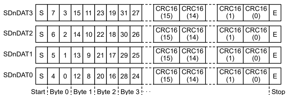
Figure 40.3 SDnDAT in 4-bit width mode
