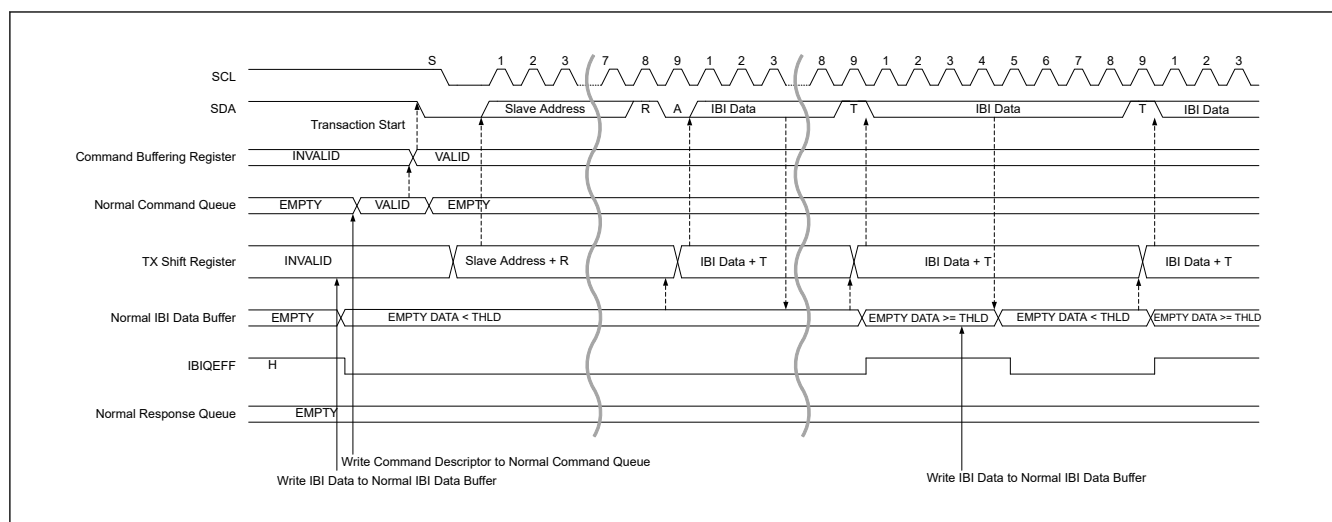
Figure 33.63 I3C slave IBI transfer timing (1/2)
