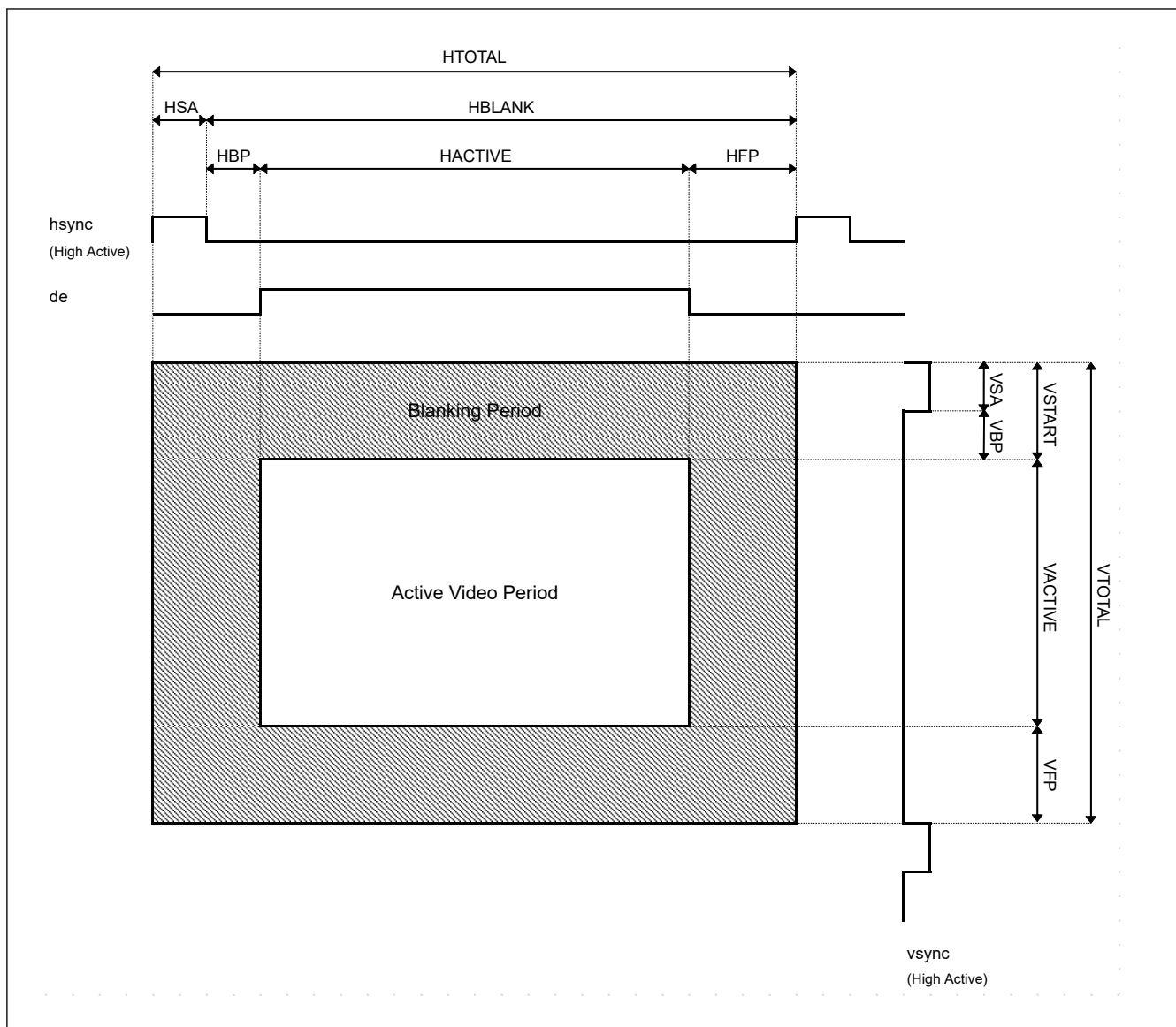
Figure 58.9 Video mode Timing
