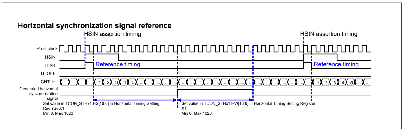
Figure 56.20 Signal generation based on input horizontal synchronization signal (HSIN)
