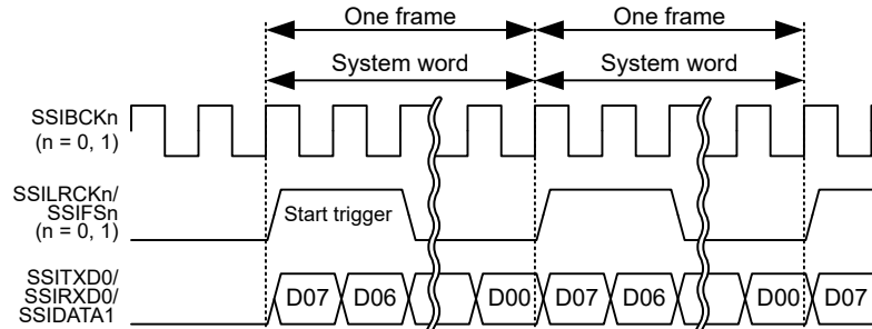
Figure 39.40 Long frame in monaural format (without padding)
