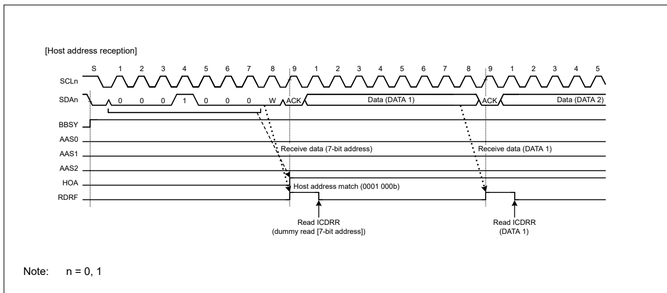
Figure 32.29 HOA flag set timing during reception of host address
