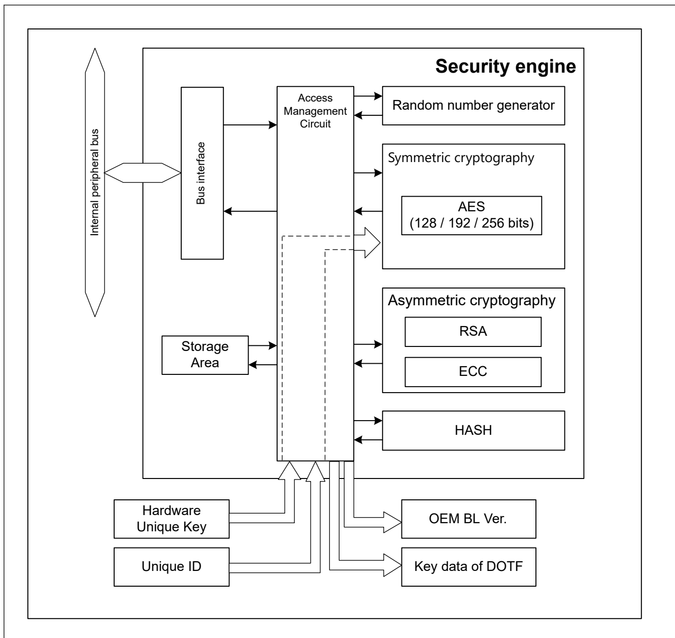
Figure 44.1 Security engine block diagram
