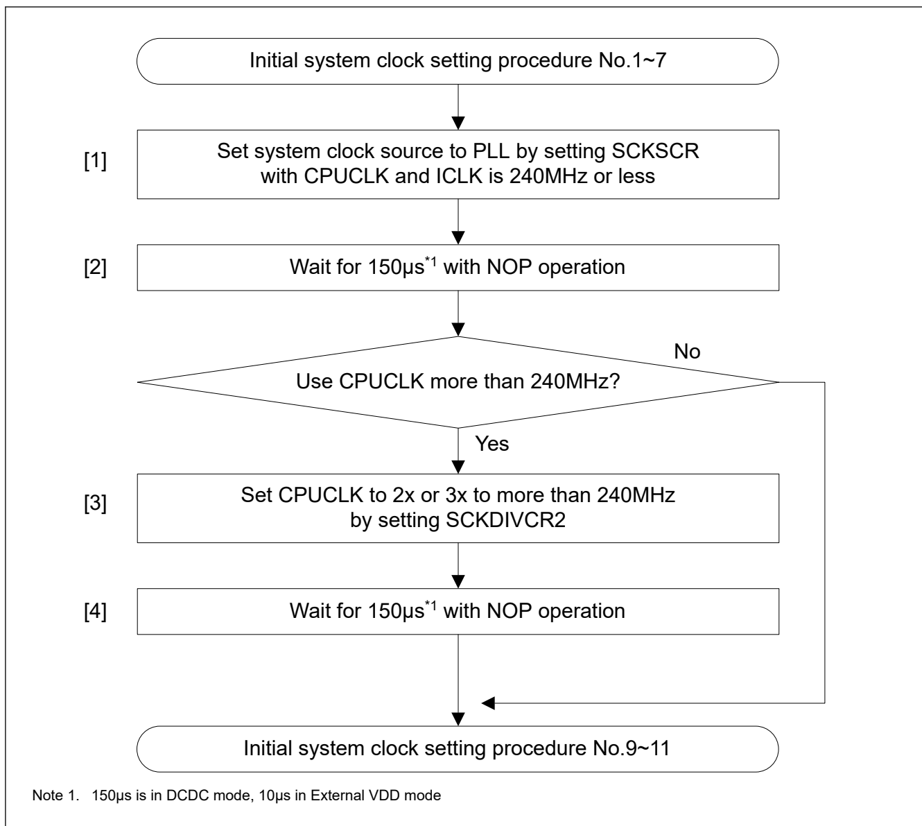
Figure 8.13 Additional flow of initial system clock setting when PLL is used for the system clock source. (assuming all module stop bit are initial value)
