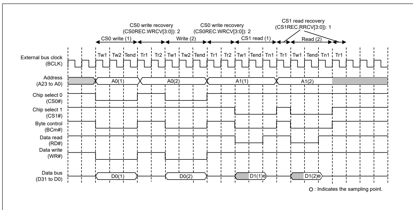
Figure 14.30 Example recovery cycle insertion when bus access is split, with separate bus interface and normal access (m = 0 to 3)
