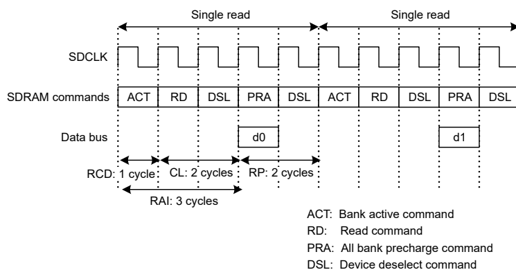
Figure 14.52 Example timing for single read (1)
