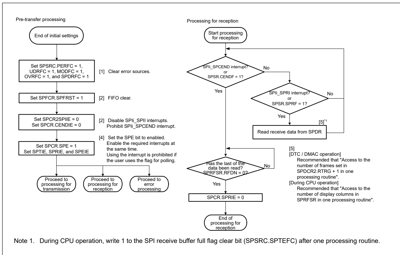
Figure 36.70 Reception flow in slave mode
