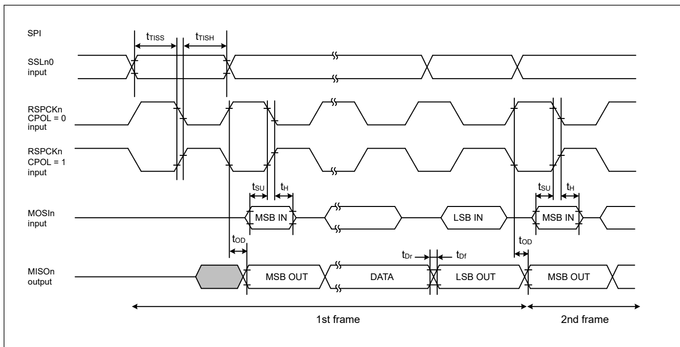
Figure 60.65 SPI timing for TI SSP slave when transmit with no delay between frames
