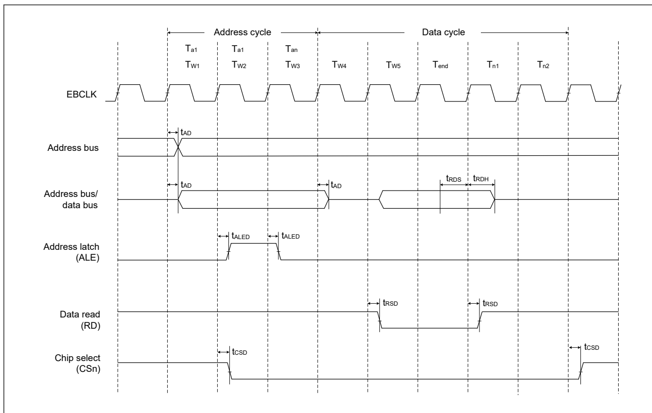
Figure 60.28 Address/data multiplexed bus read access timing
