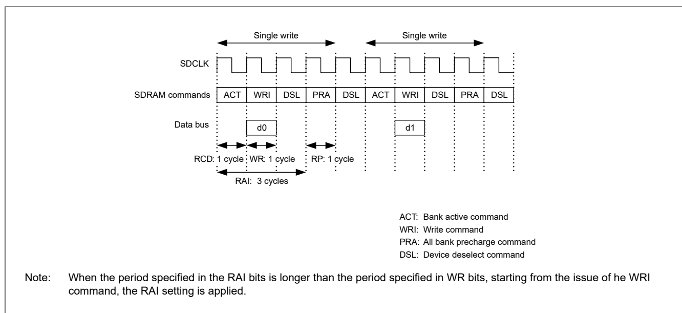
Figure 14.60 Example timing for single write (4)
