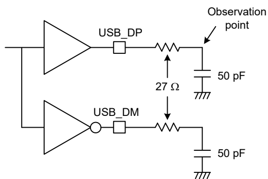
Figure 60.110 Test circuit in full-speed mode
