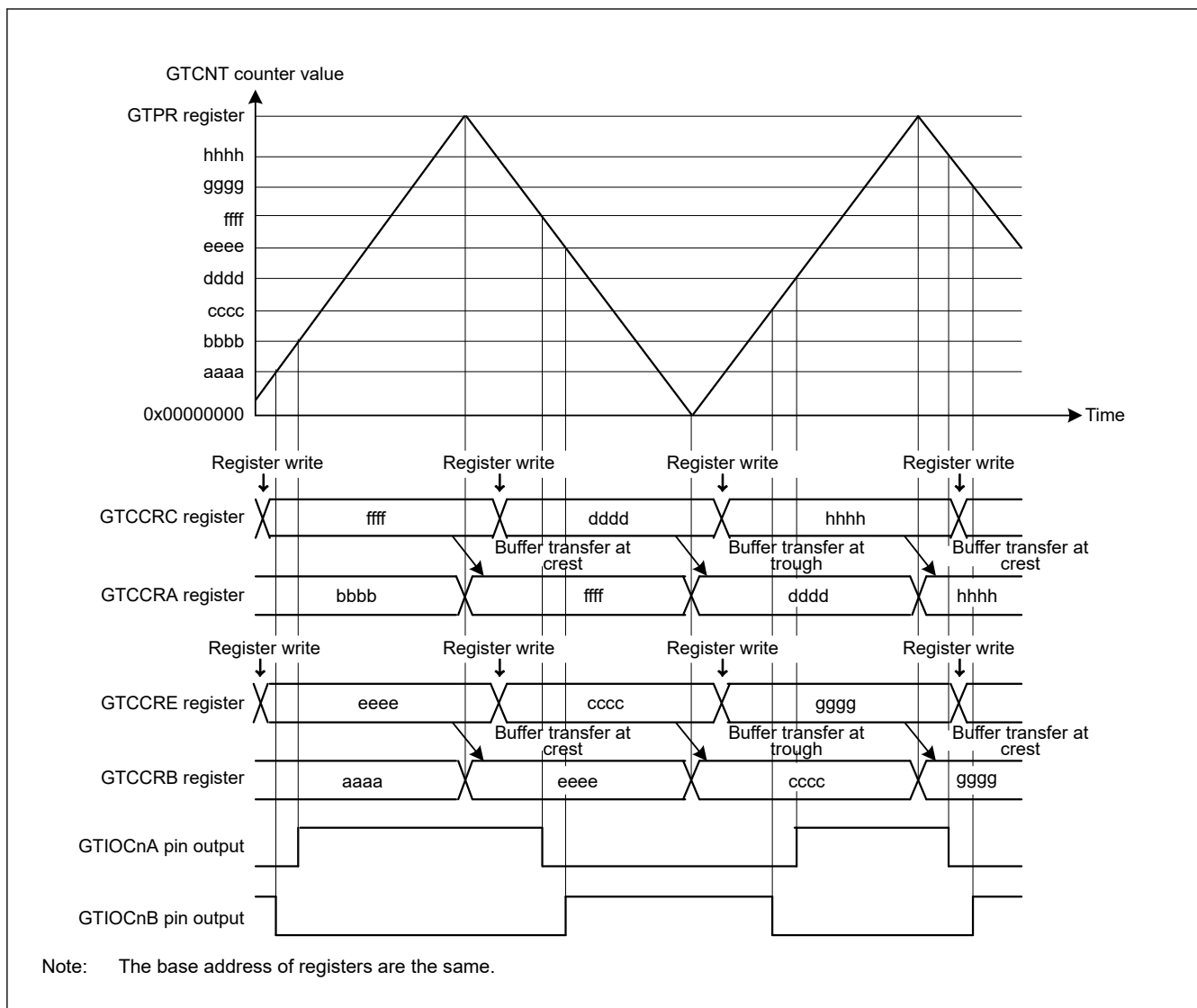
Figure 21.24 Example of triangle-wave PWM mode 2 operation with buffer operation, low output from the GTIOcNA pin and high output from the GTIOcNB pin at count start, output toggled at GTCCRA/ GTCCRB compare match, and output retained at cycle end
