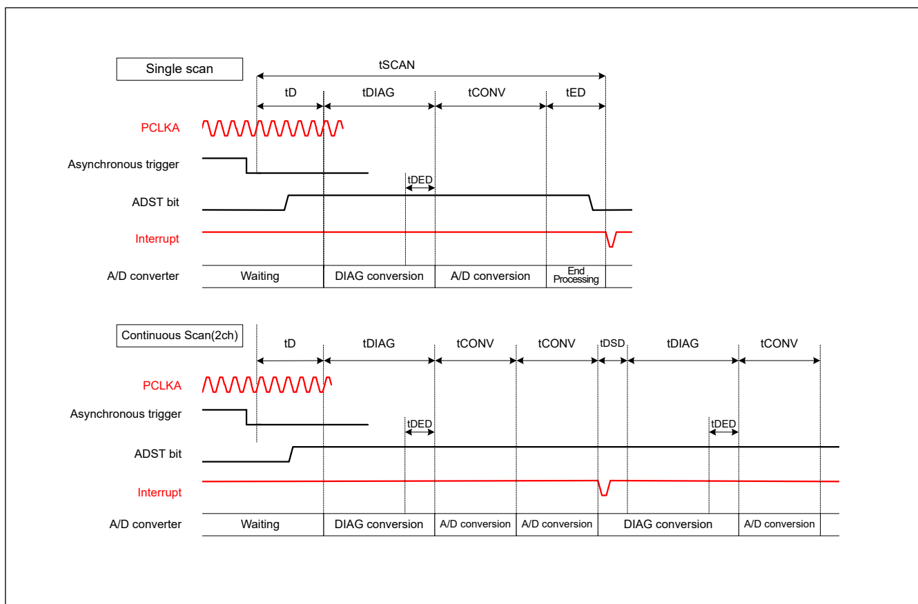
Figure 45.36 Scan conversion timing when activated by an asynchronous trigger input (ADTRGn (n = 0, 1))
