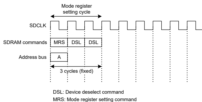
Figure 14.48 Mode register setting timing
