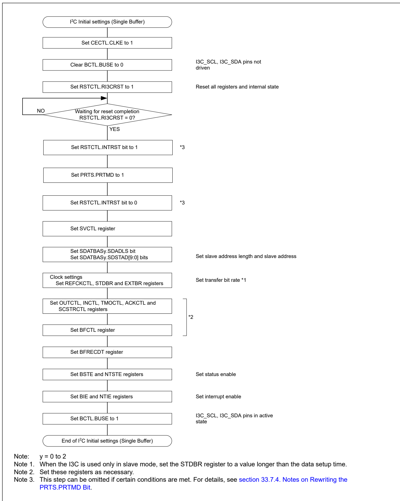
Figure 33.140 Example of I 2 C initialization flowchart (single buffer transfer)
