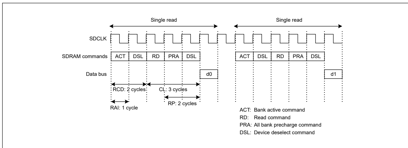
Figure 14.54 Example timing for single read (3)
