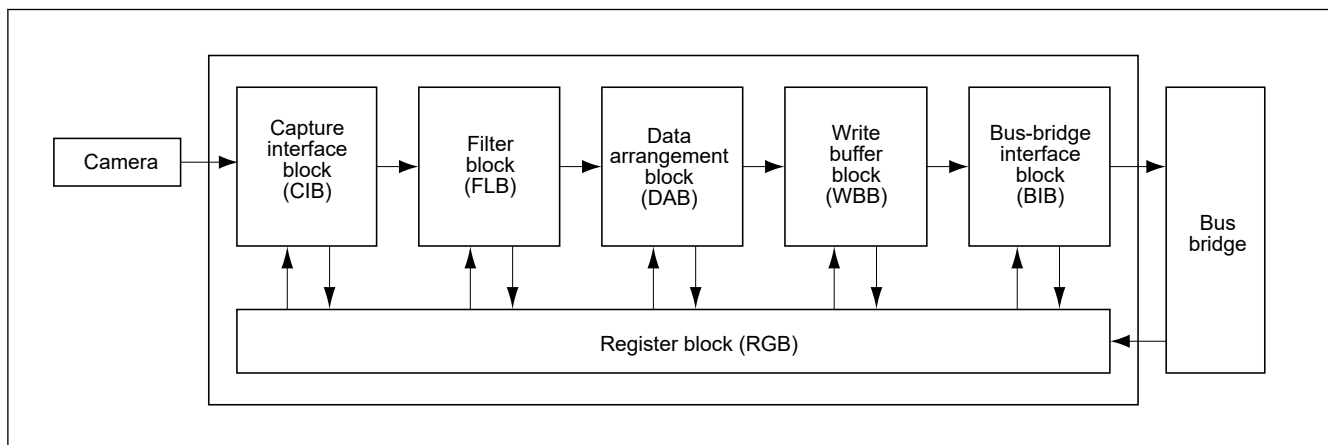
Figure 53.1 Block diagram of CEU
