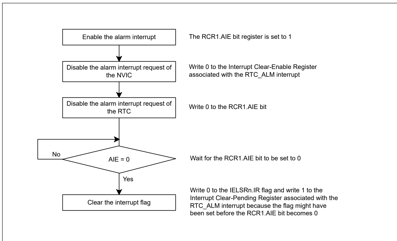
Figure 24.8 Procedure for disabling alarm interrupt request
