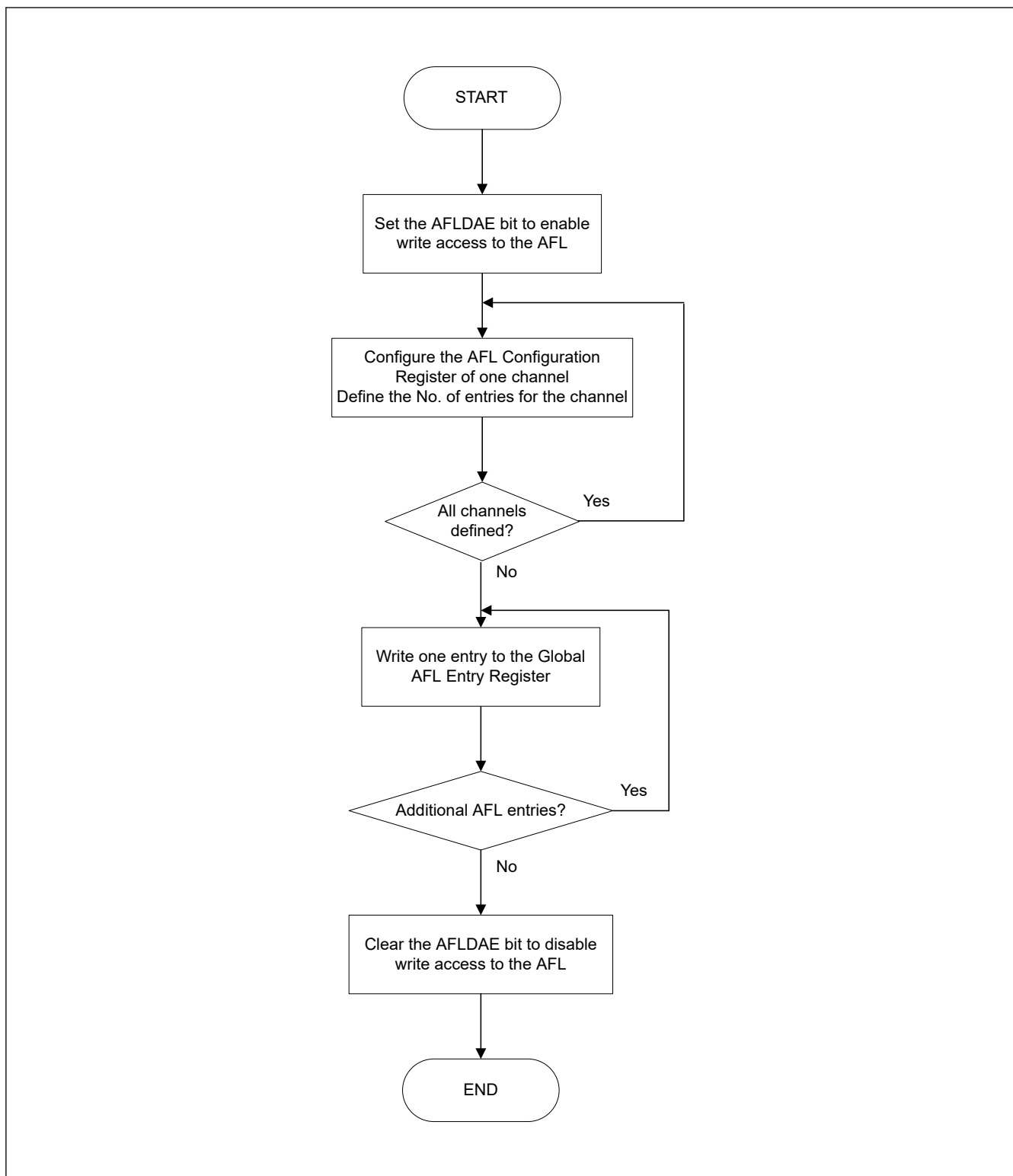
Figure 34.26 AFL configuration flow
