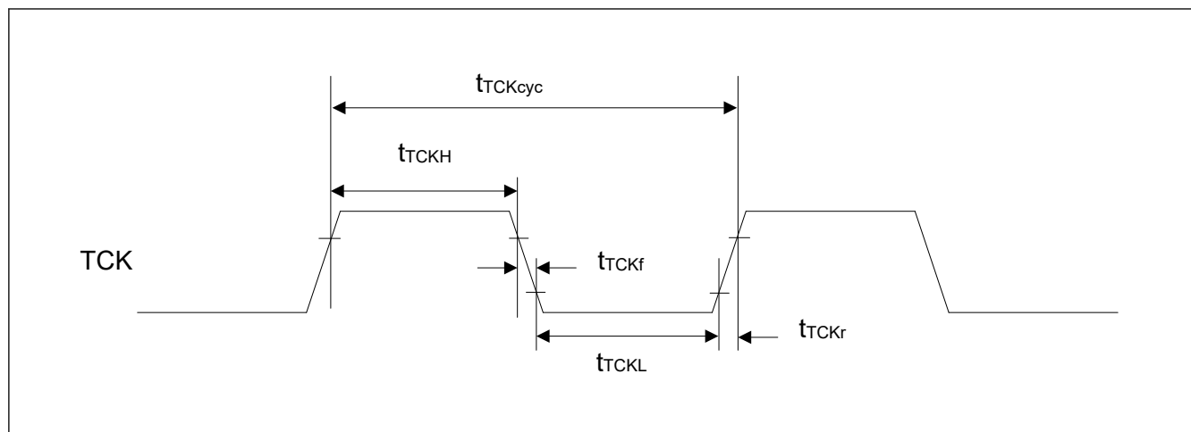
Figure 60.131 JTAG TCK timing
