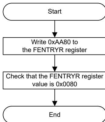
Figure 52.11 Procedure to transition to data flash P/E mode
