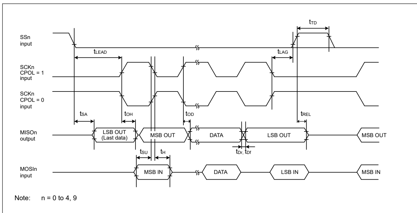
Figure 60.56 SCI simple SPI mode timing for slave when CPHA = 1
