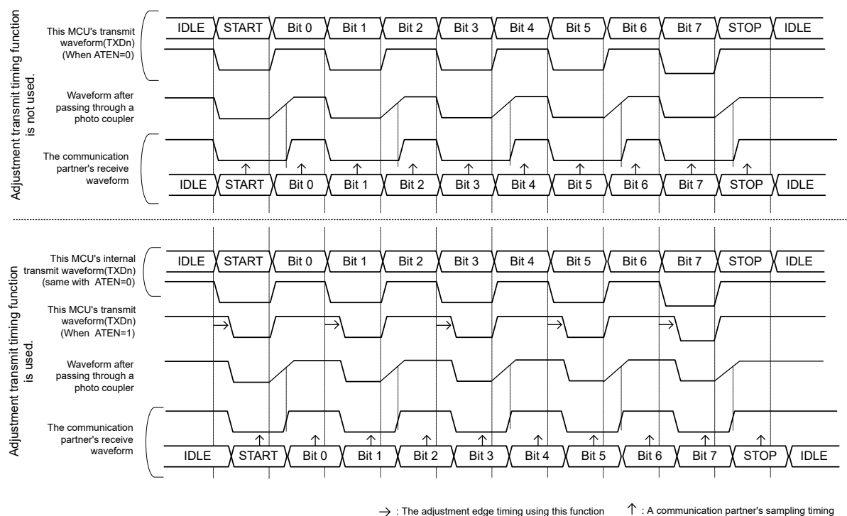
Figure 31.32 The explanation for the transmit waveform through a photo coupler
