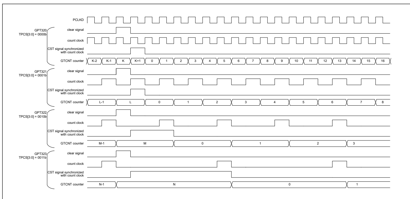
Figure 21.42 Example of Simultaneous Clearing Operation by Software (with Different Count Period)
