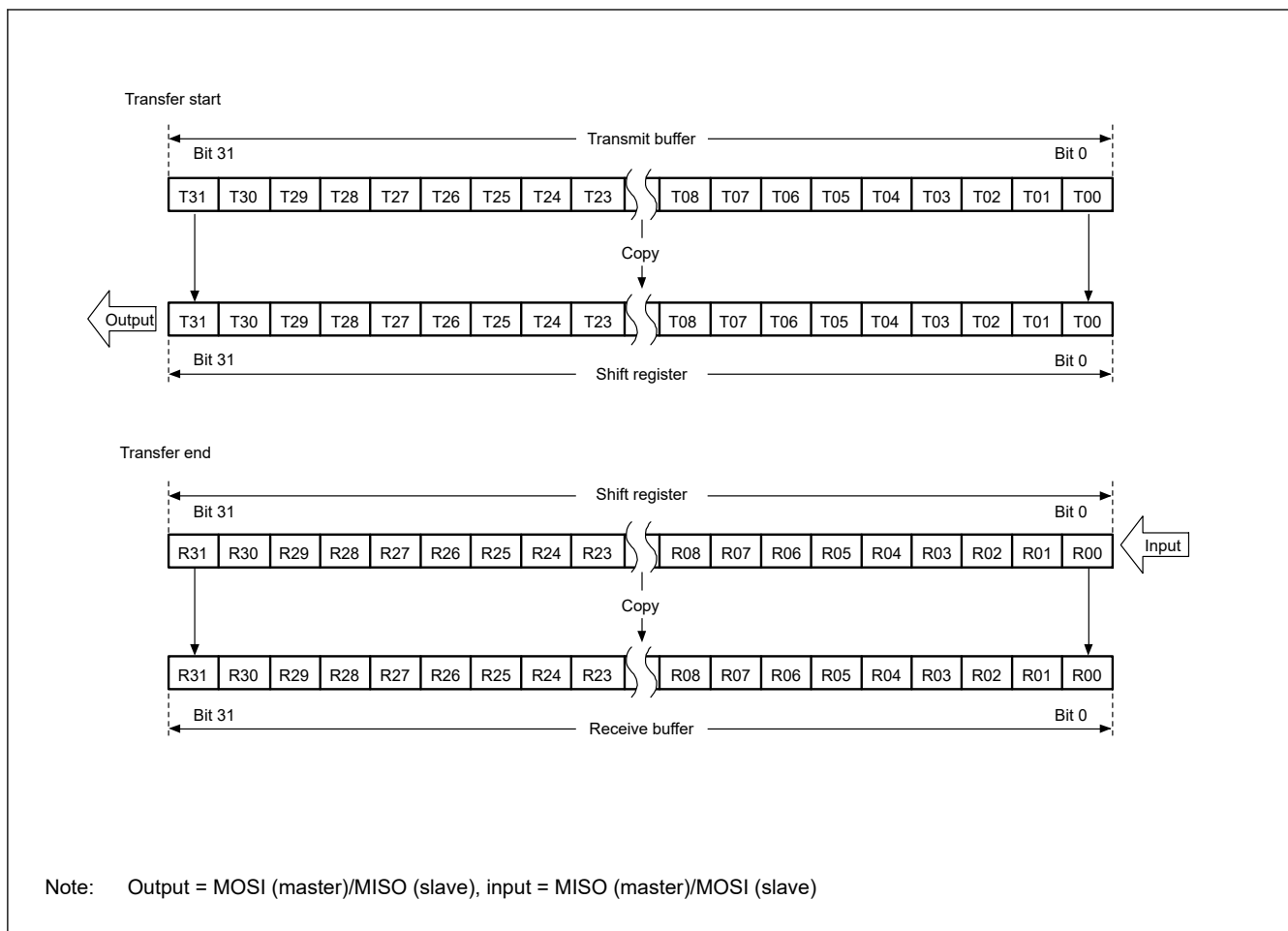
Figure 36.15 MSB-first transfer with 32-bit data and parity disabled
