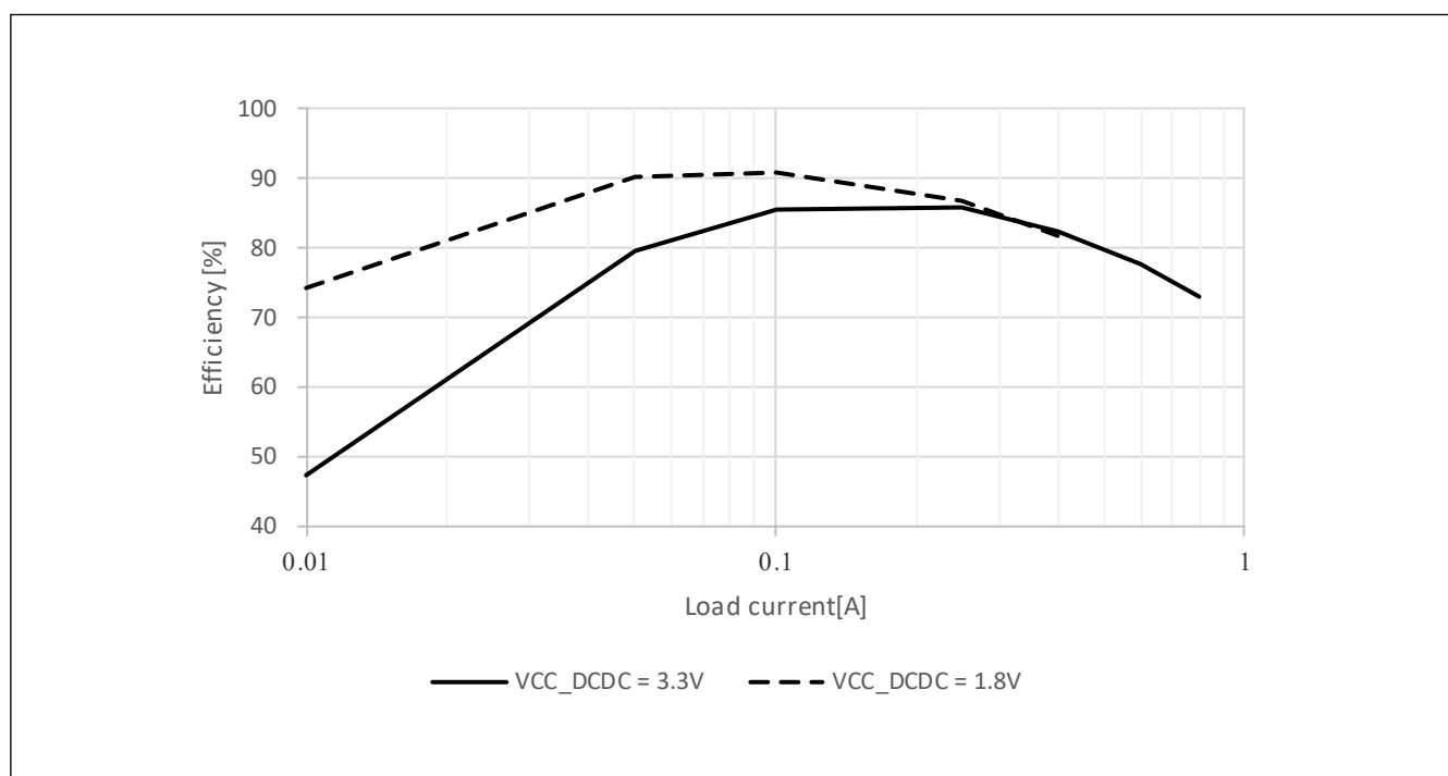
Figure 60.10 Typical DCDC efficiency (%) vs load current (A) in High-speed mode, T_j = 125\text{ }^{\circ}\text{C}
