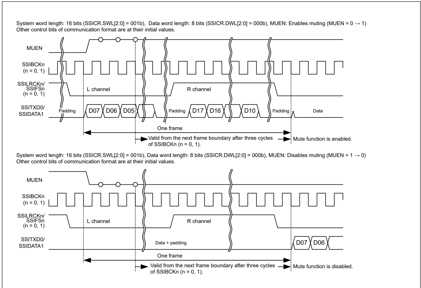
Figure 39.5 Transmit data with the mute function set
