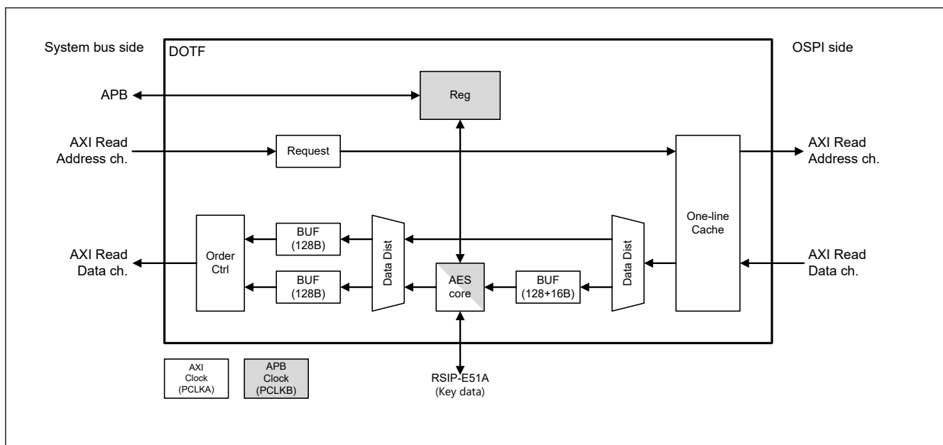
Figure 38.1 Block diagram
