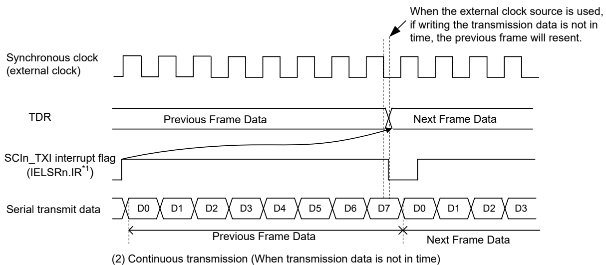
Figure 31.121 Restrictions on Use of External Clock in Clock Synchronous Transmission
