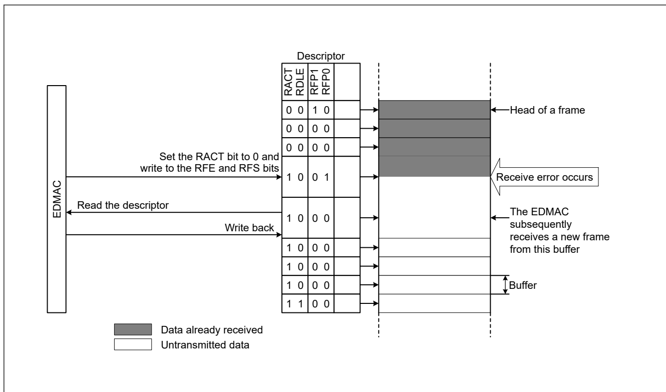
Figure 28.8 EDMAC operation after receive error occurs
