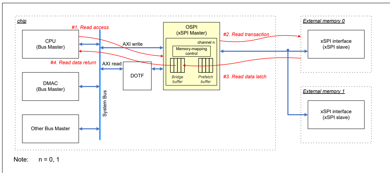
Figure 37.16 Read access for memory area
