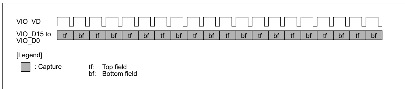
Figure 53.26 Continuous both-field capture in interlace mode (Image Immediately after Activation is Top Field (FCI[1:0] = 00b))
