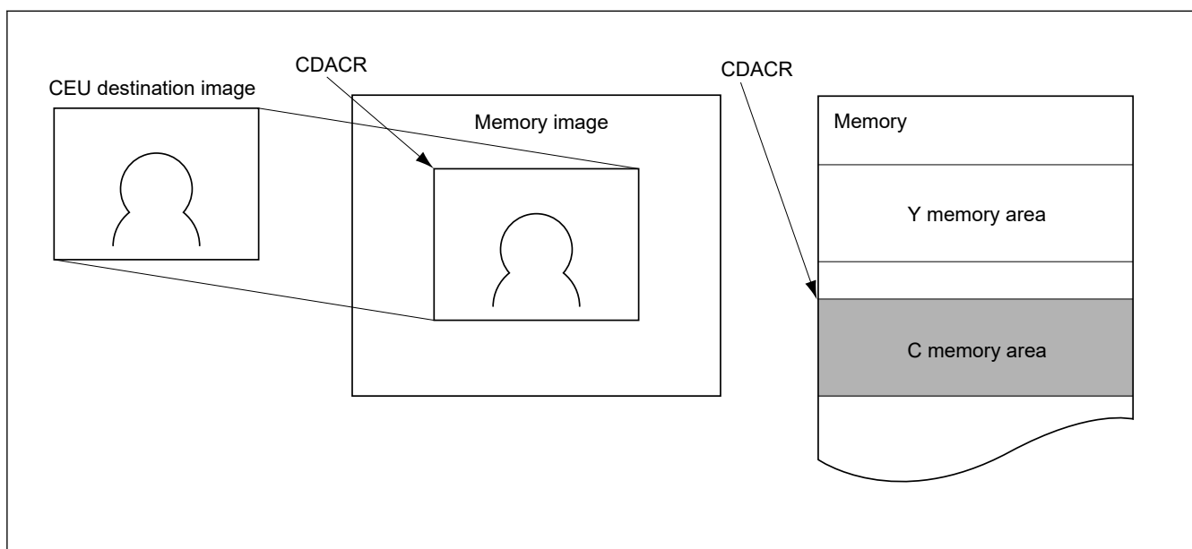
Figure 53.35 Relationship between captured image and chrominance component memory area
