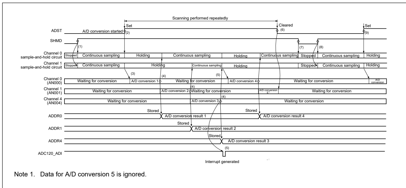
Figure 45.19 Example operation in continuous scan mode when channel-dedicated sample-and-hold circuits are used, AN000, AN001, and AN004 are selected, and continuous sampling is enabled
