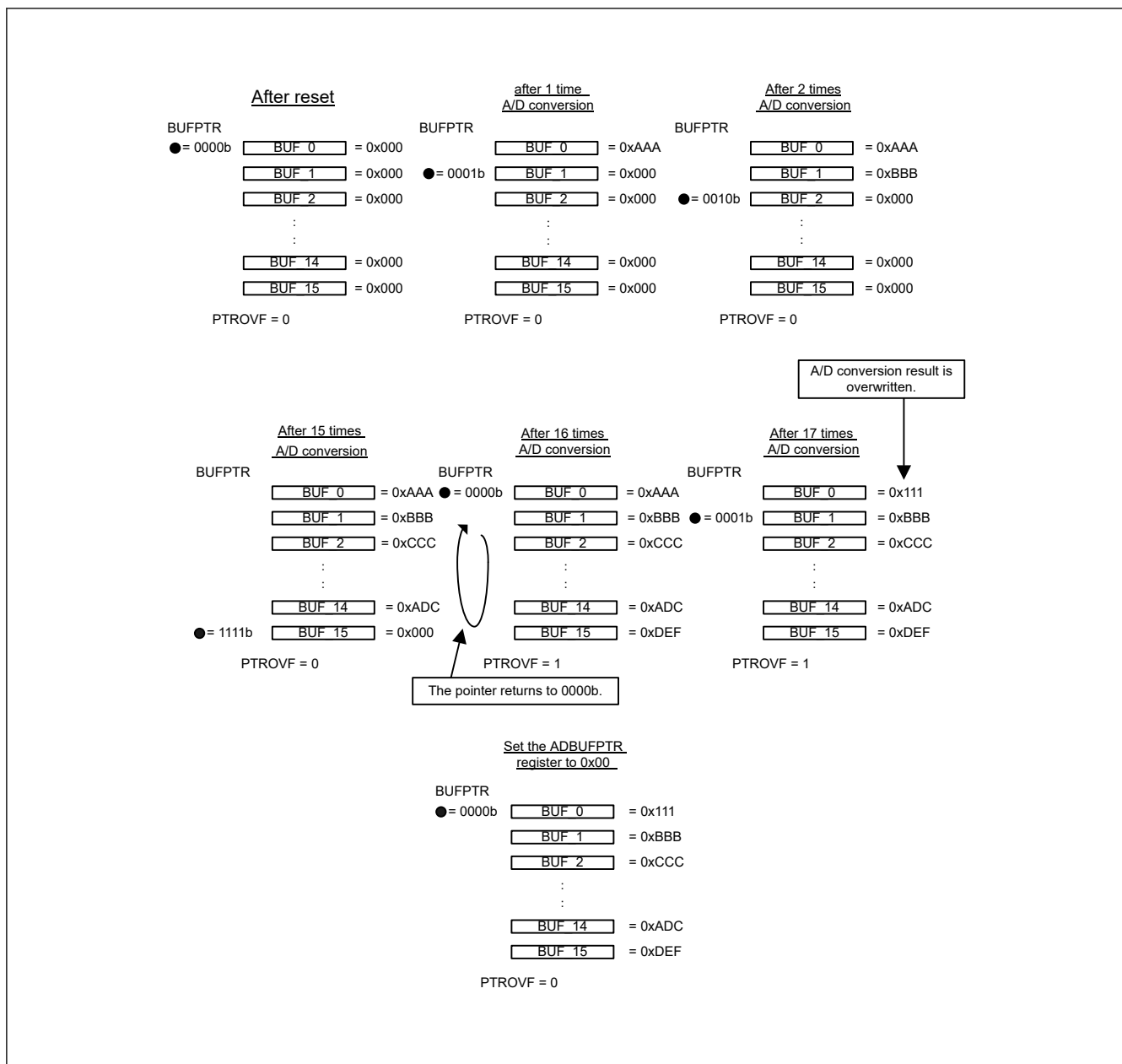
Figure 45.42 Data Buffers, Pointer, and Overflow Flag Operations
