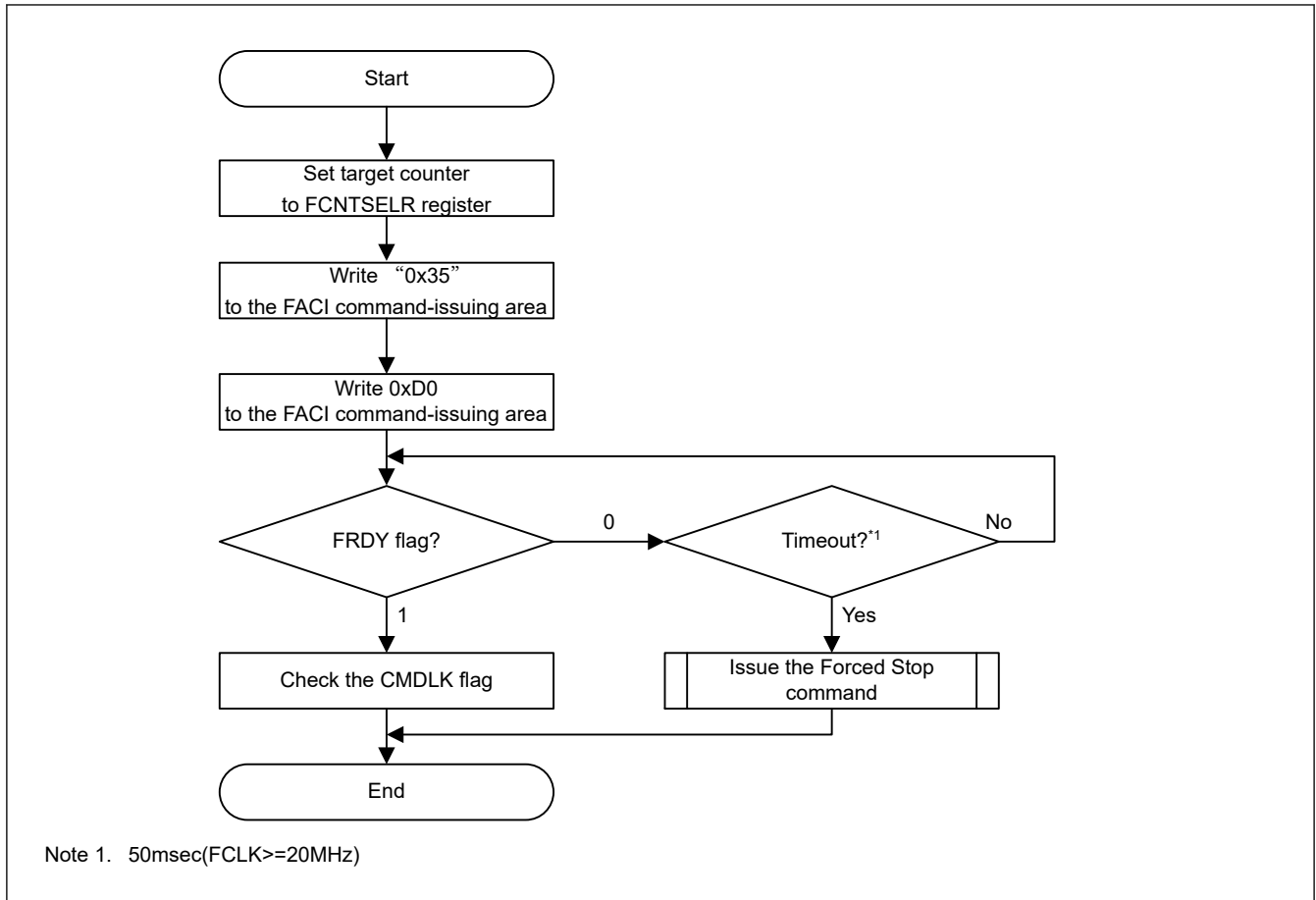
Figure 52.26 Usage of the Increment Counter Command
