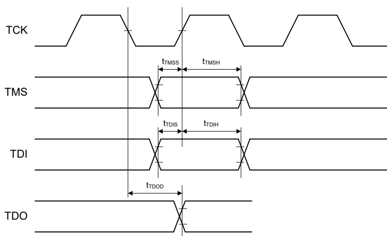
Figure 60.128 Boundary scan input/output timing (1)
