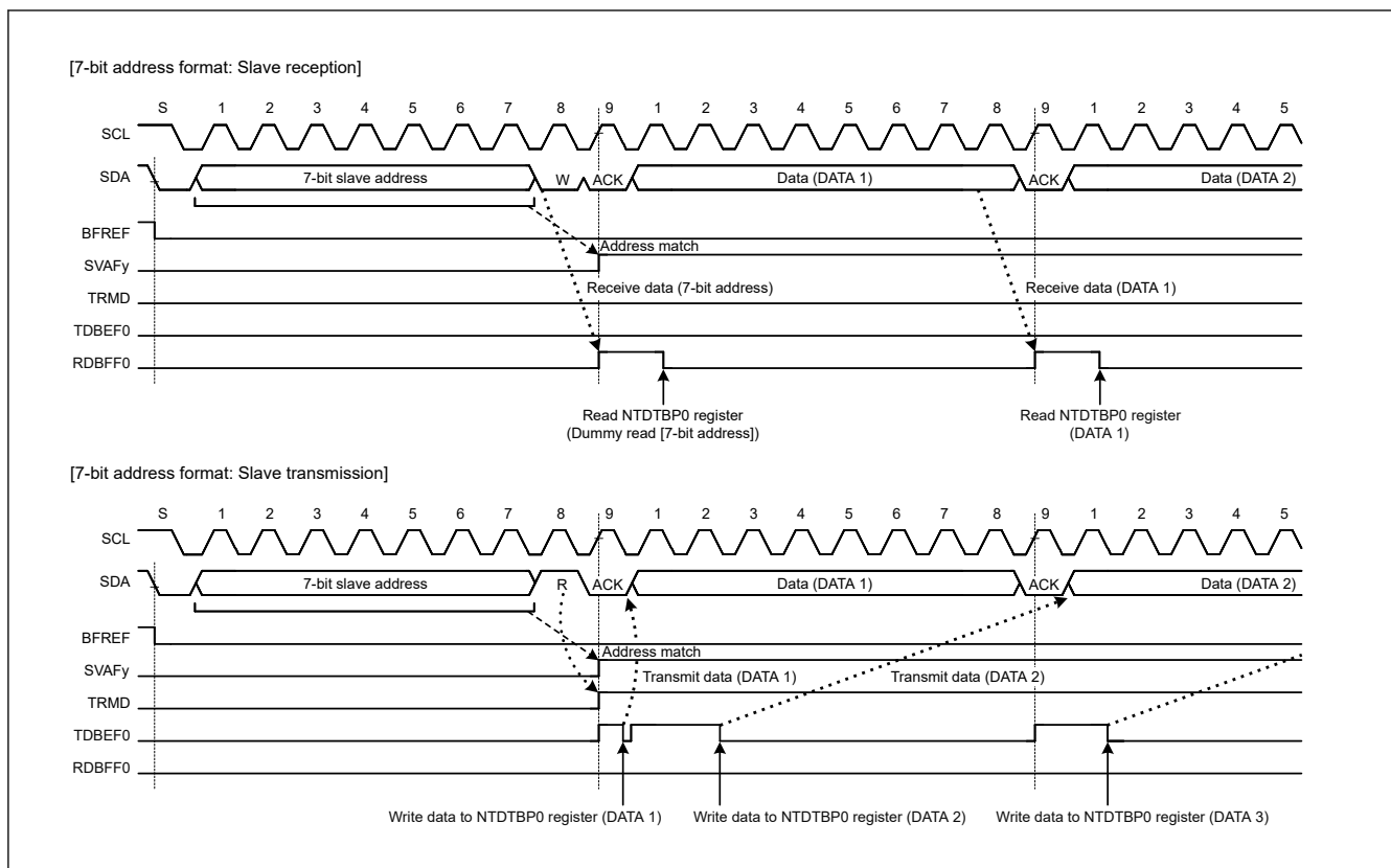
Figure 33.82 SVAfy flag set timing with 7-bit address format selected
