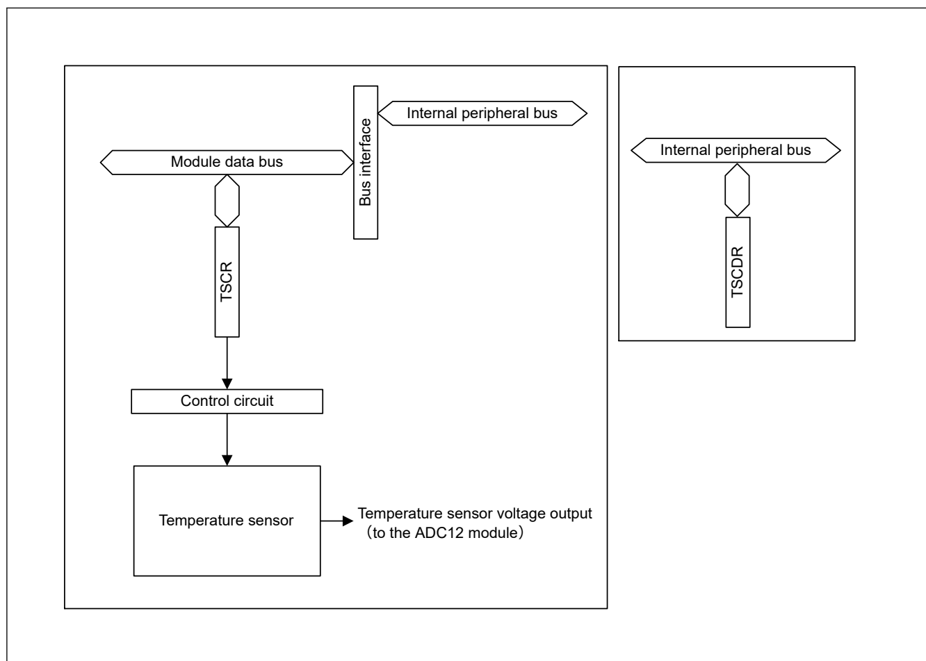
Figure 47.1 TSN block diagram
