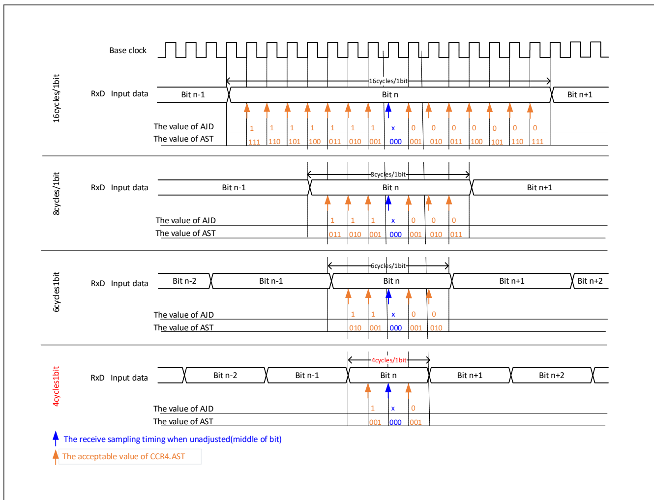
Figure 31.29 Overview of the adjustment operation for the reception sampling timing (Asynchronous mode using internal clock)
