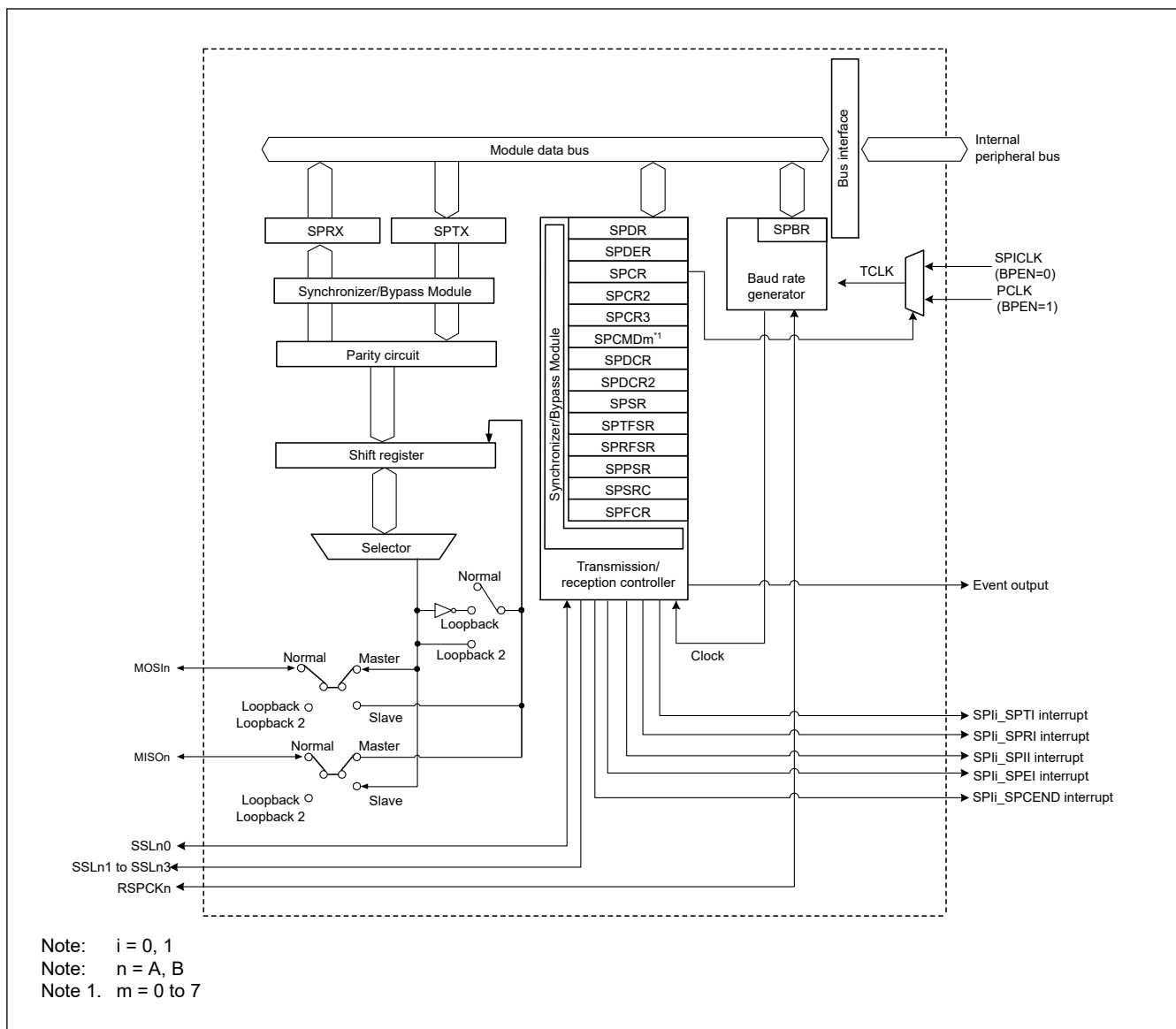
Figure 36.1 SPI block diagram
