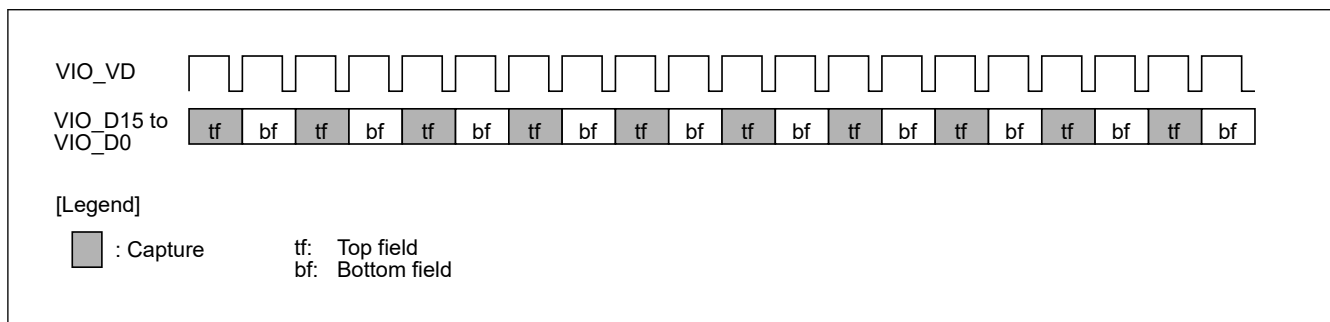
Figure 53.27 Continuous one-field capture in interlace mode (Image Immediately after Activation is Top Field (FCI[1:0] = 00b))
