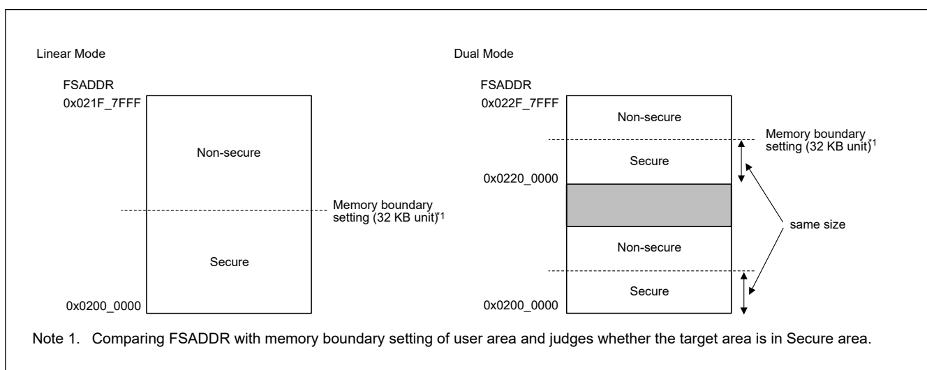
Figure 52.39 Secure and Non-secure region in user area for Secure alias
