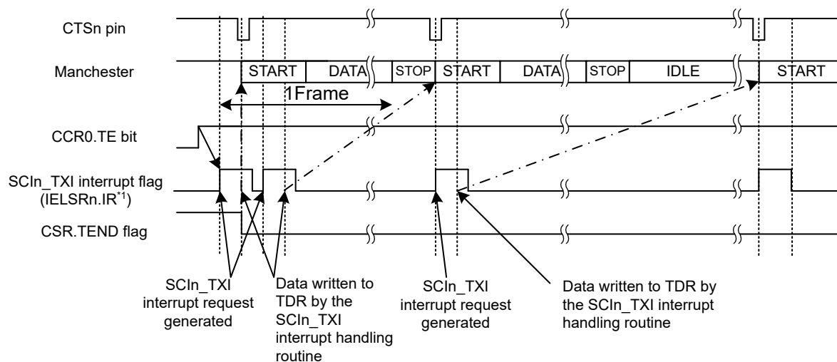
Figure 31.53 Example of Start-of-Transmission Operation for Serial Transmission in Manchester Mode (Without Preface but with the CTS Function)
