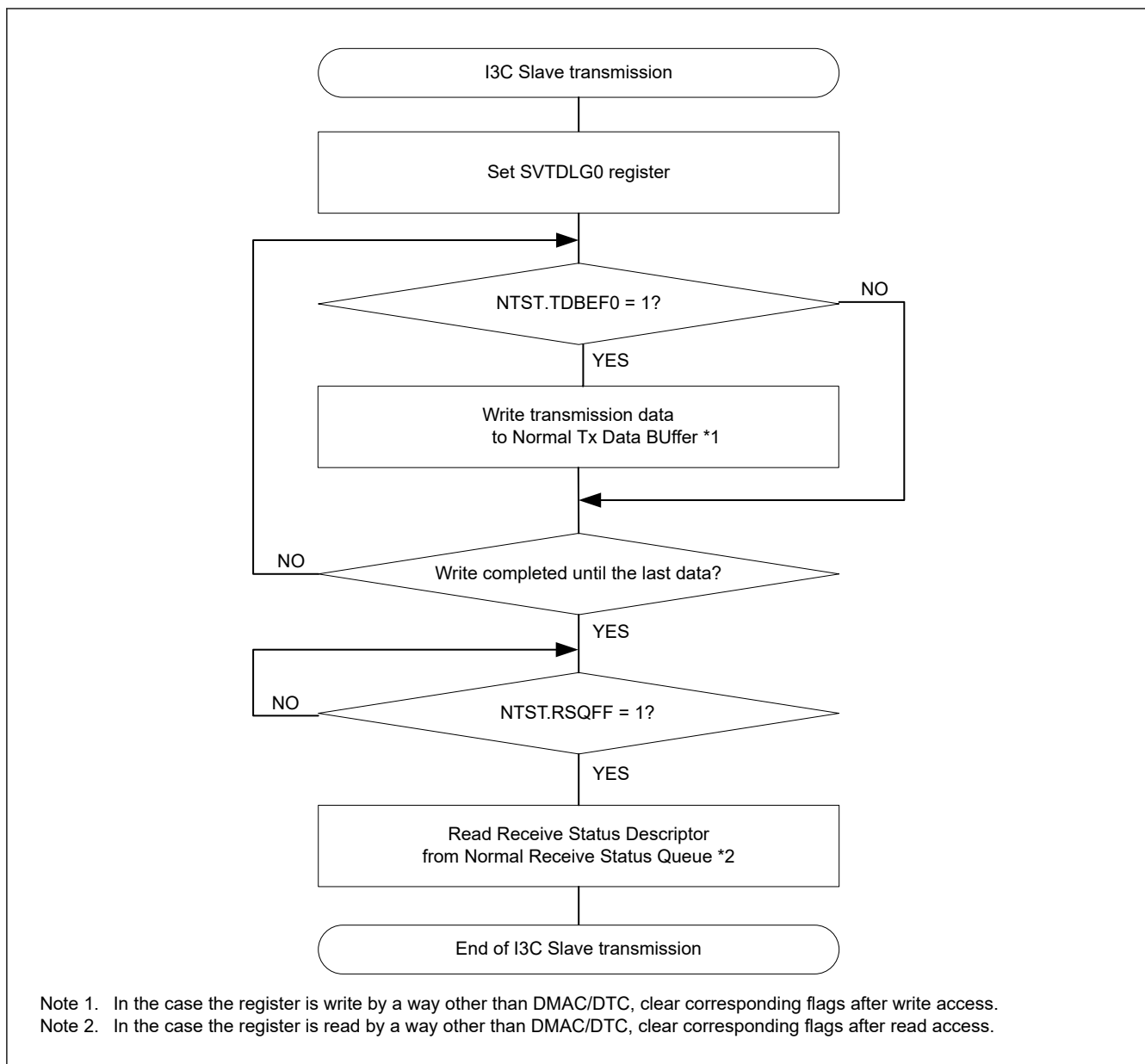
Figure 33.154 Example of I3C slave transmission flowchart (normal FIFO buffer transfer)
