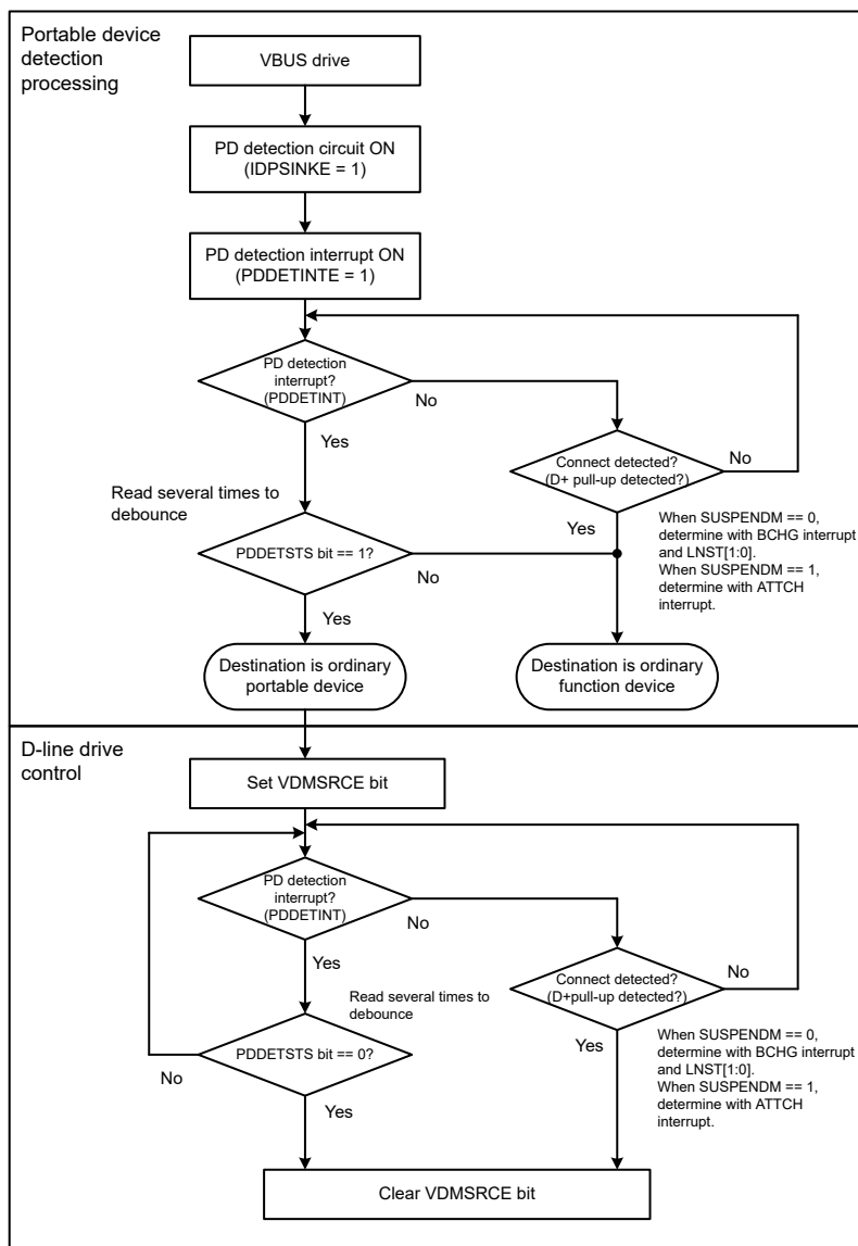
Figure 30.21 Processing flow as charging downstream port with hardware portable device detection function
