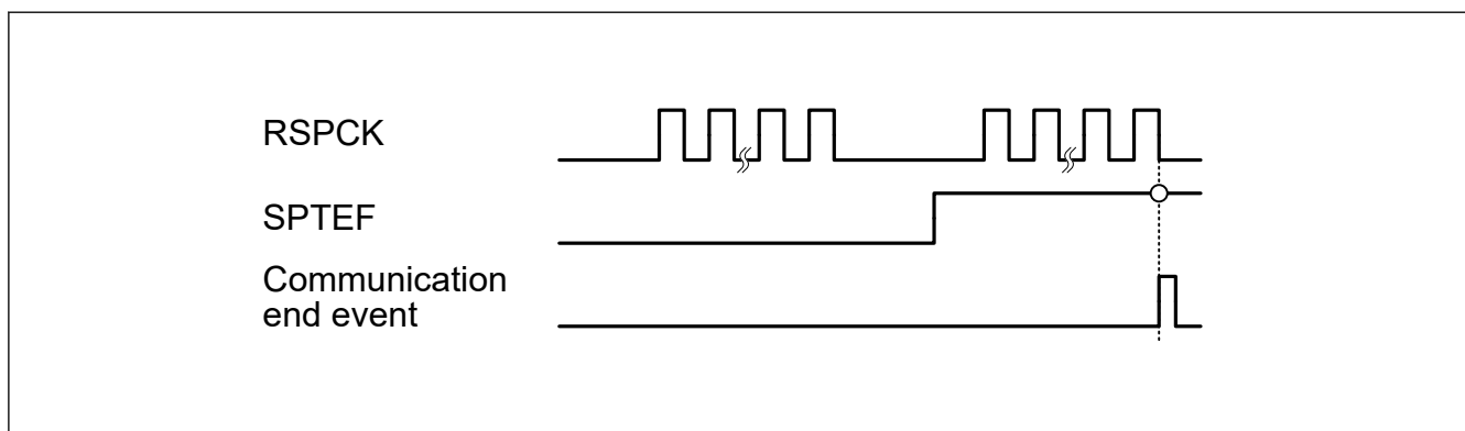
Figure 36.82 Communication End Event Output Timing (Transmit slave mode, Clock Synchronous Operation)
