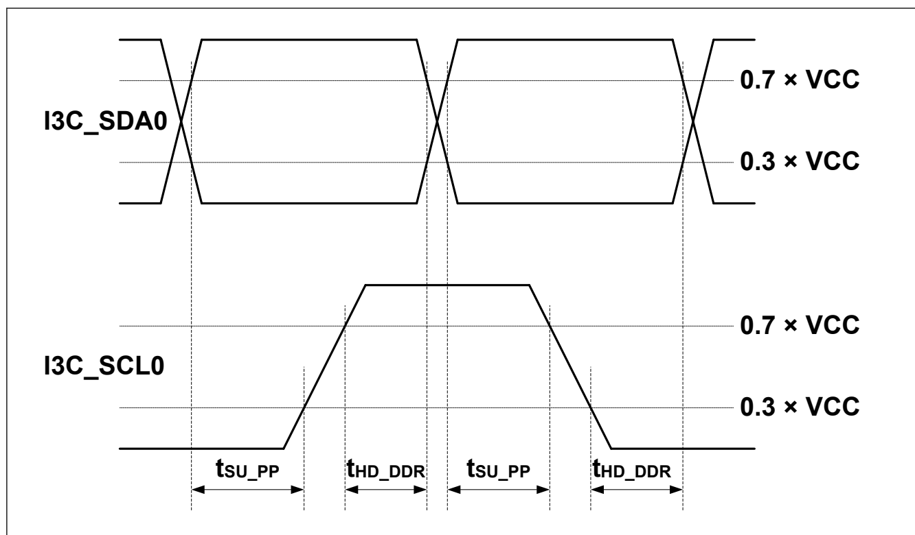
Figure 60.81 Master DDR Timing
