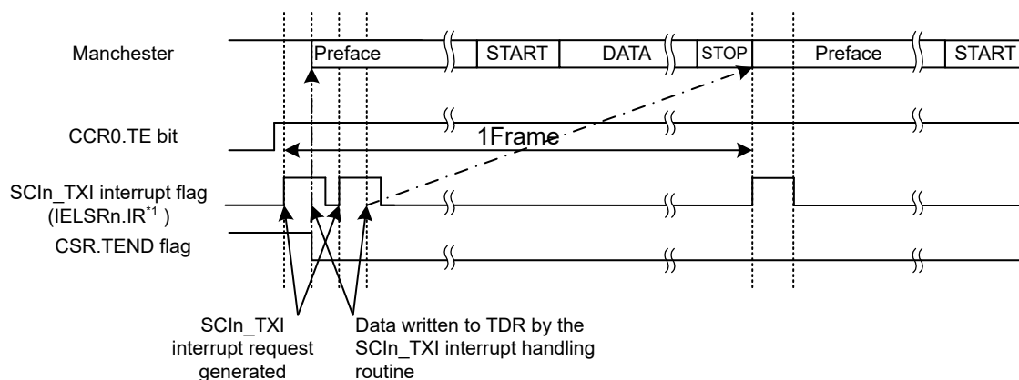
Figure 31.52 Example of Start-of-Transmission Operation for Serial Transmission in Manchester mode (with Preface but Without the CTS Function)
