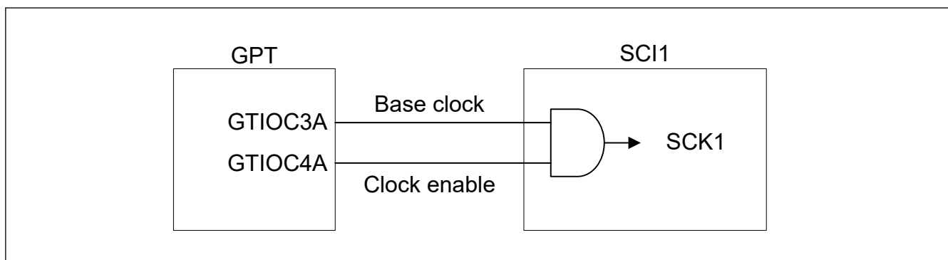
Figure 31.4 Example of GPT and SCI connection
