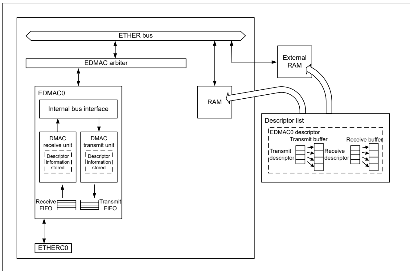
Figure 28.2 Configuration of descriptors and transmit and receive buffers in memory
