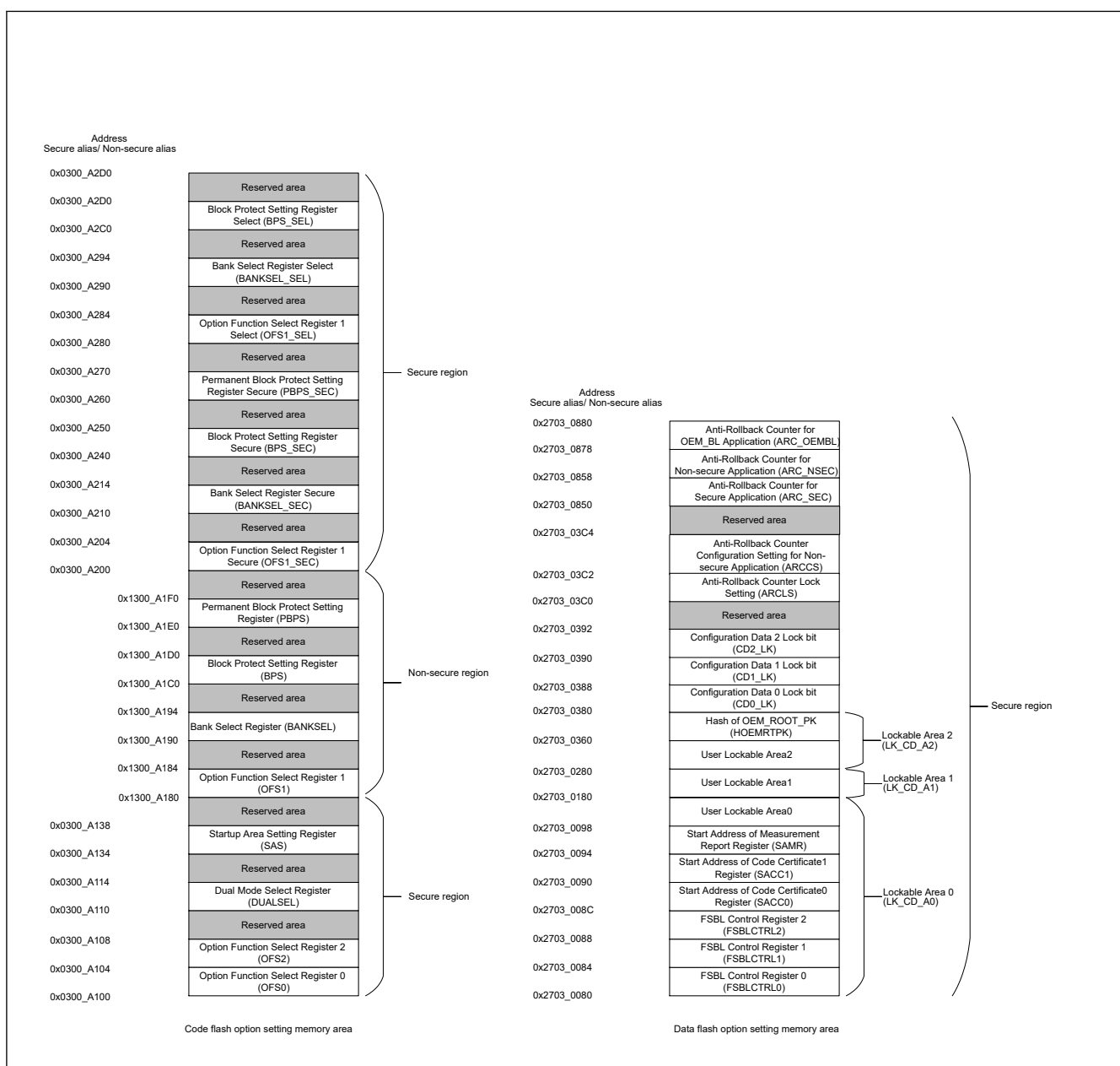
Figure 6.1 Option-setting memory area
