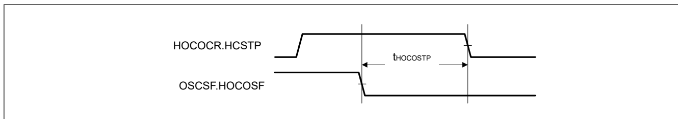
Figure 60.21 HOCO stop width time
