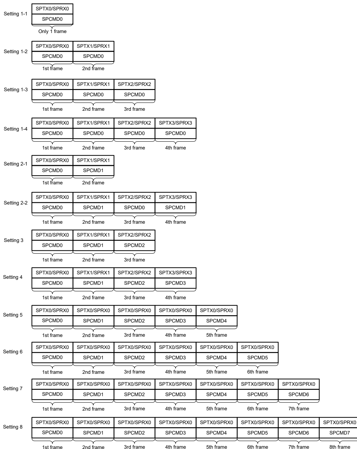
Figure 36.75 Correspondence between SPI Command Register and transmit and receive buffers in sequence operations
