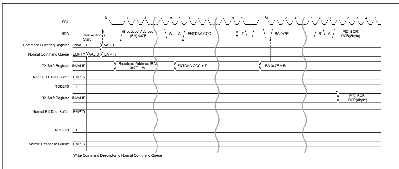
Figure 33.12 Dynamic address assign procedure (ENTDAAs CCC) timing (1/3)
