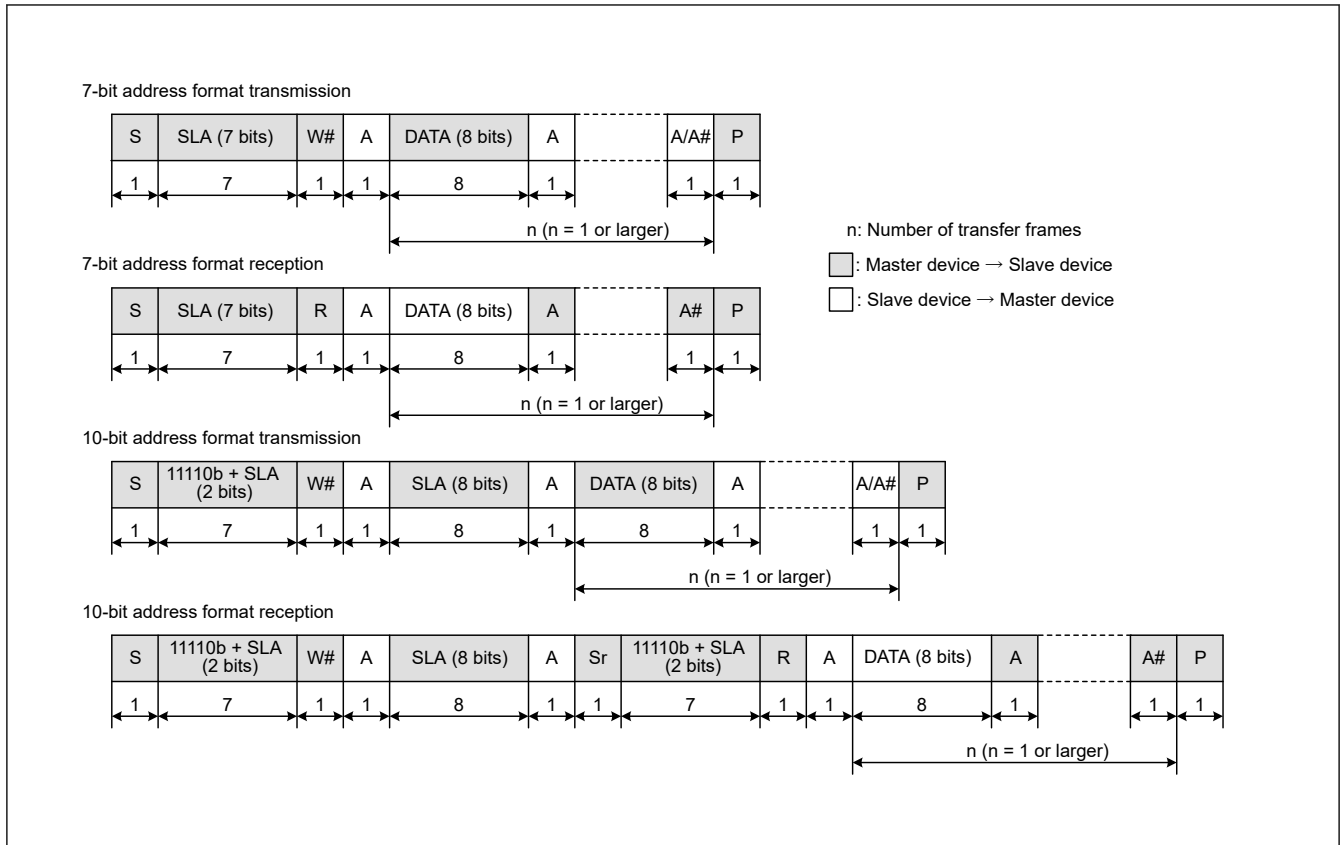
Figure 31.86 I 2 C bus format
