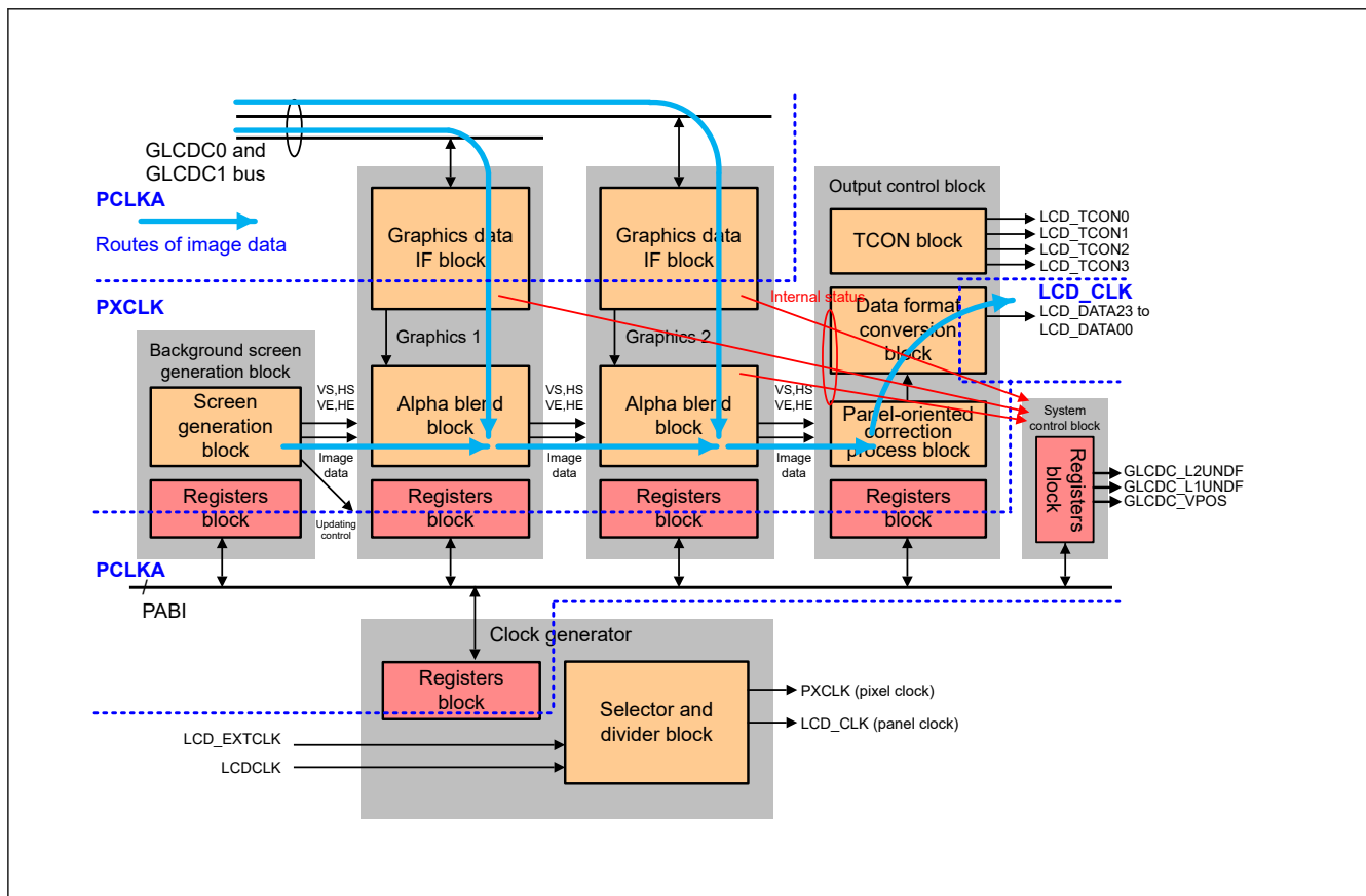
Figure 56.22 GLCDC configuration
