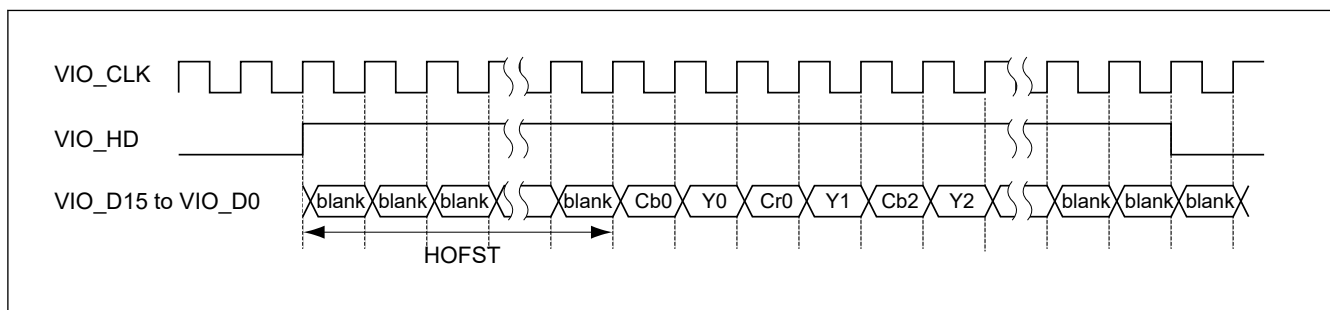
Figure 53.19 Horizontal offset
