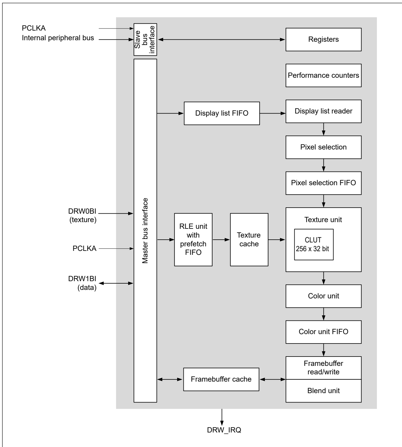
Figure 55.3 2D Drawing Engine block diagram
