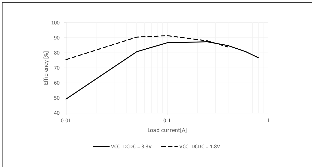
Figure 60.9 Typical DCDC efficiency (%) vs load current (A) in High-speed mode, T_j = 25\text{ }^{\circ}\text{C}
