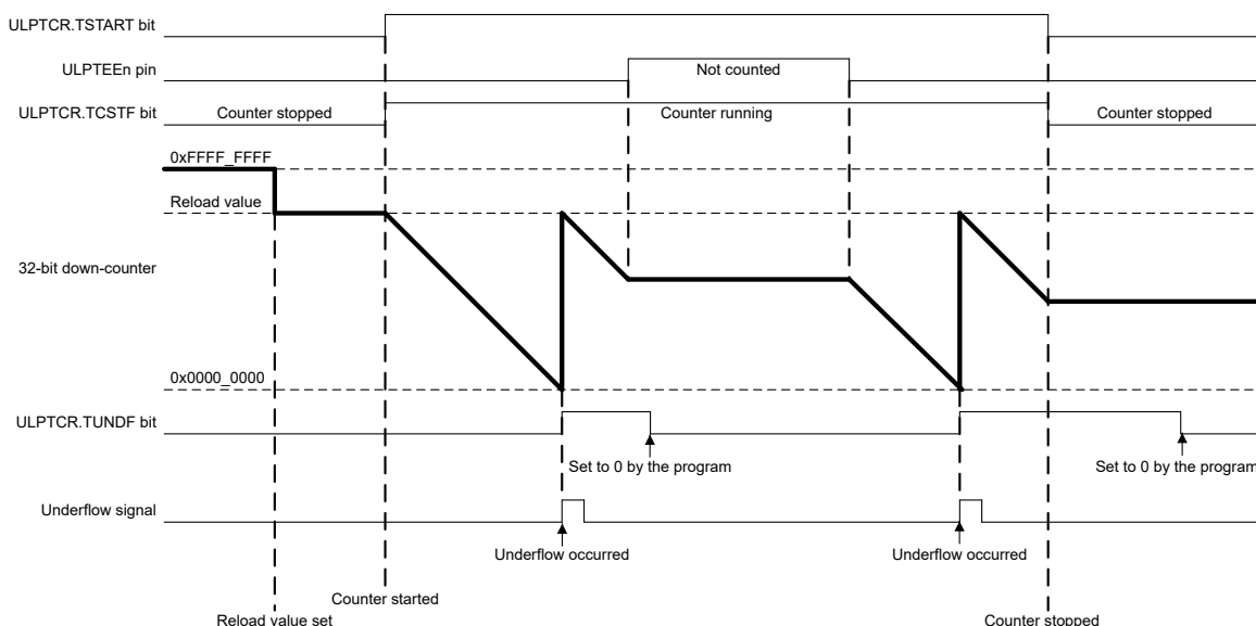
Figure 23.5 Operation example 1 in event counter & continuous & count enable mode (with the ULPTIOC.TIOGT0 bit set to 1)
