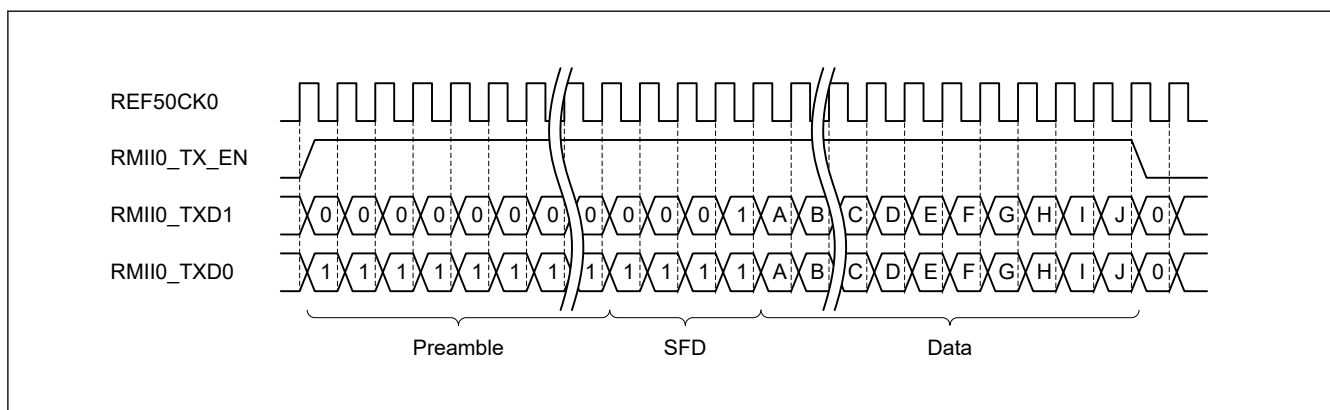
Figure 27.12 RMII frame transmit timing during normal transmission
