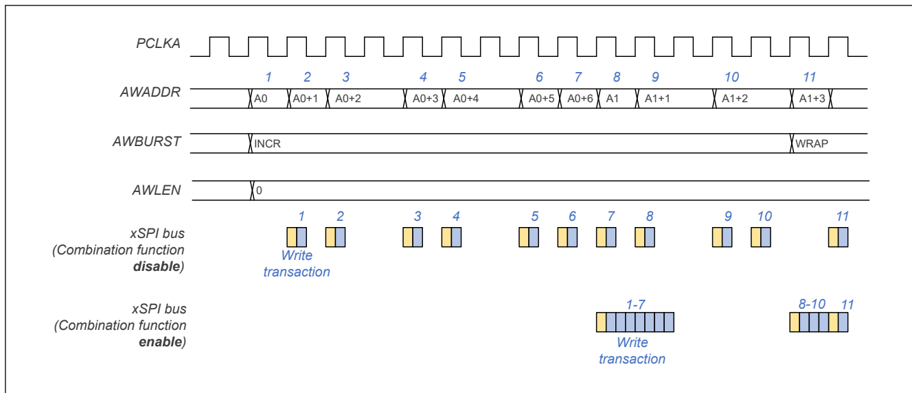
Figure 37.14 Combination function
