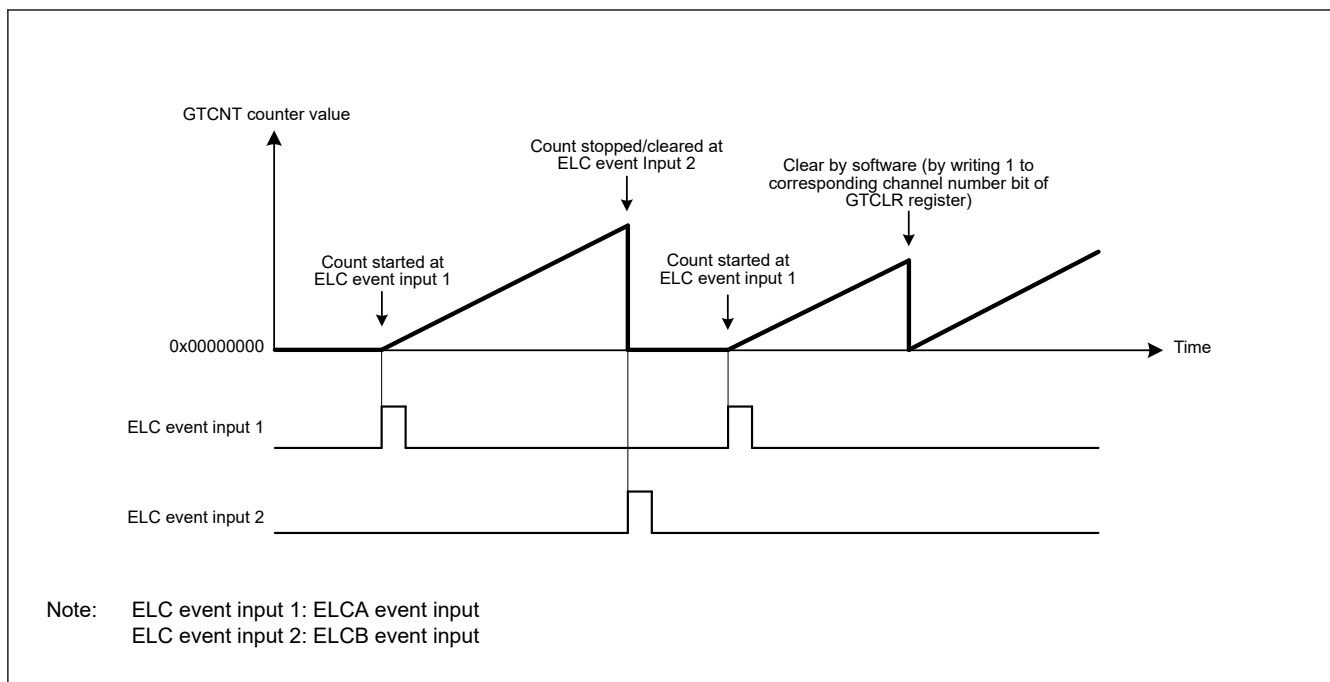
Figure 21.35 Examples of count clearing operation by hardware source in saw wave up-counting, started at ELCA input, and stopped/cleared at ELCB input
