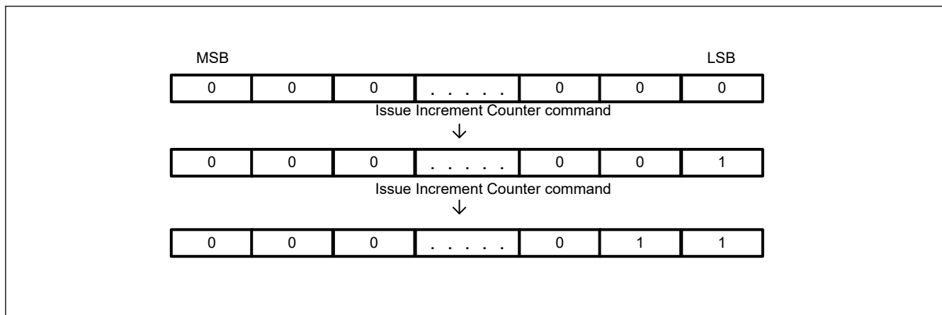
Figure 52.43 Increment image of anti-rollback counter
