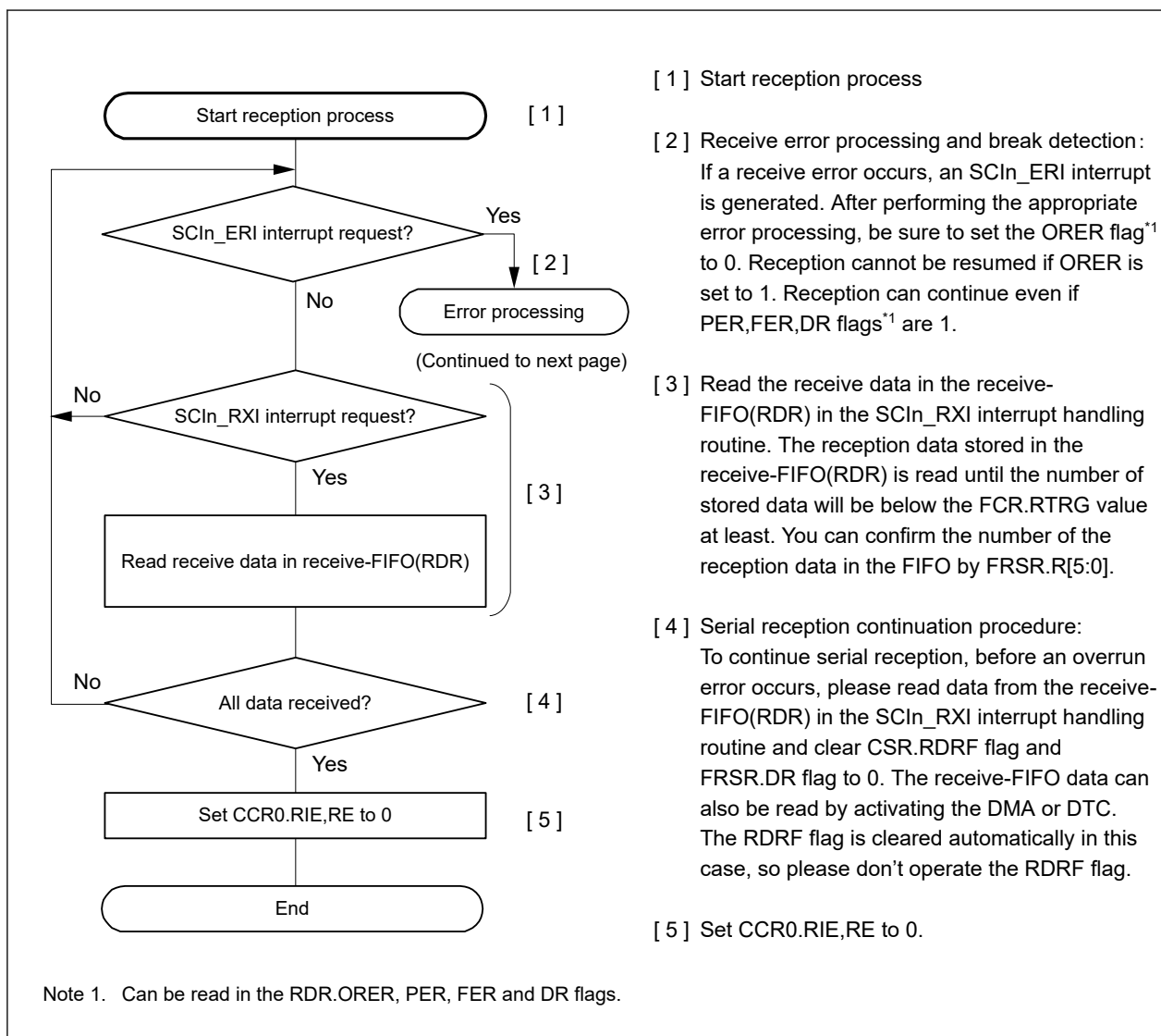
Figure 31.24 Example flow of serial reception in Asynchronous mode with FIFO selected and Address Matching Enabled (1)
