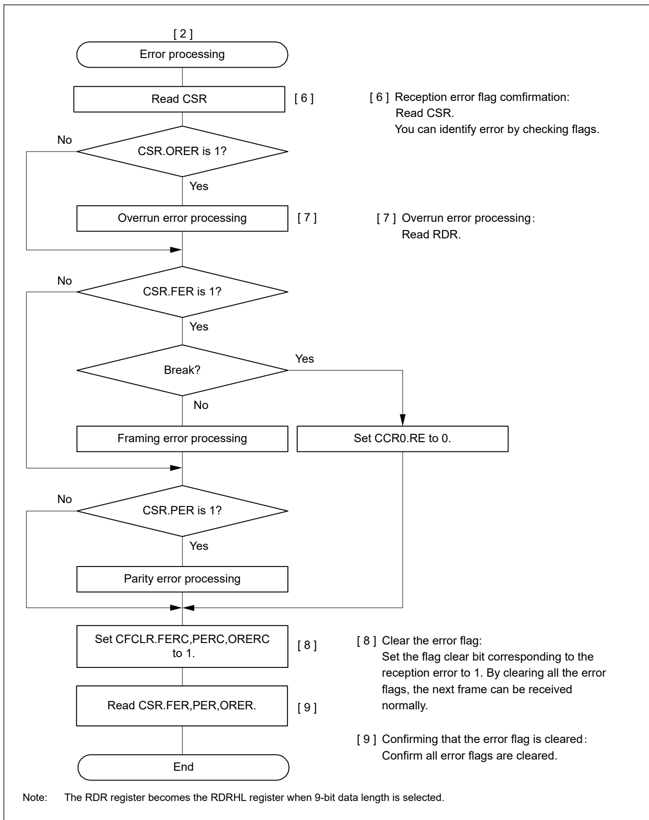
Figure 31.22 Example flow of serial reception in Asynchronous mode with non-FIFO selected and Address Matching Disabled (2)
