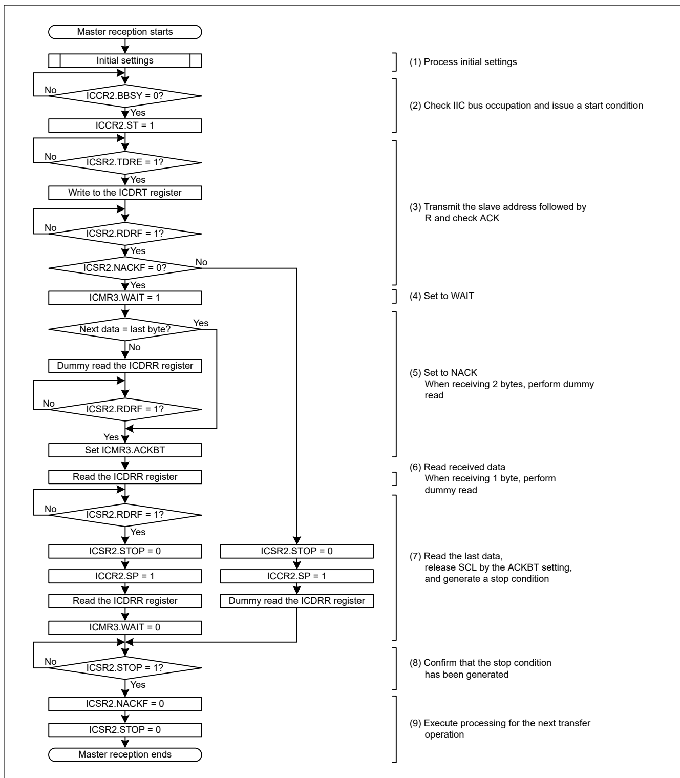
Figure 32.10 Example master reception flow with 7-bit address format of 1 byte or 2 bytes
