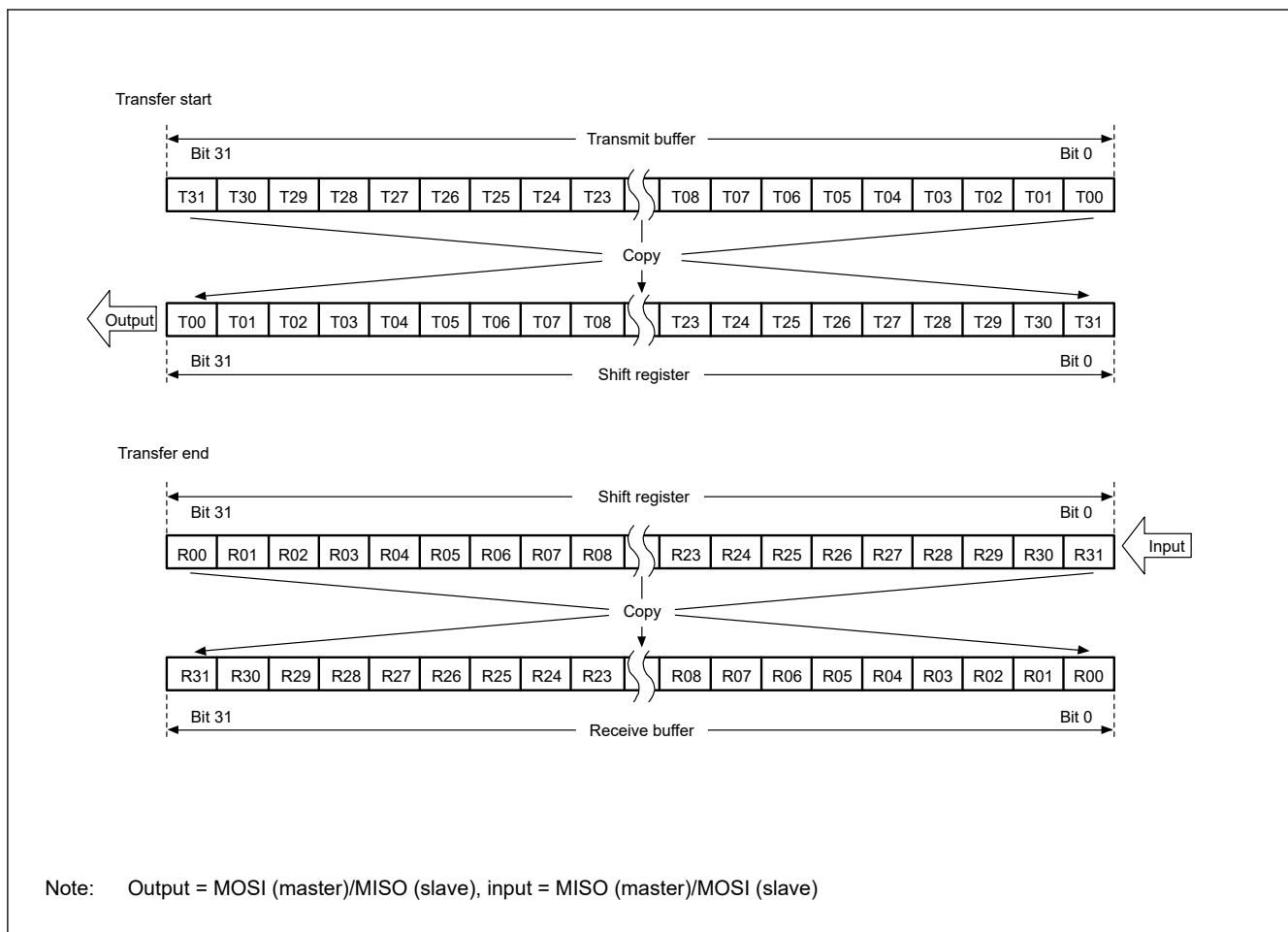
Figure 36.17 LSB-first transfer with 32-bit data and parity disabled
