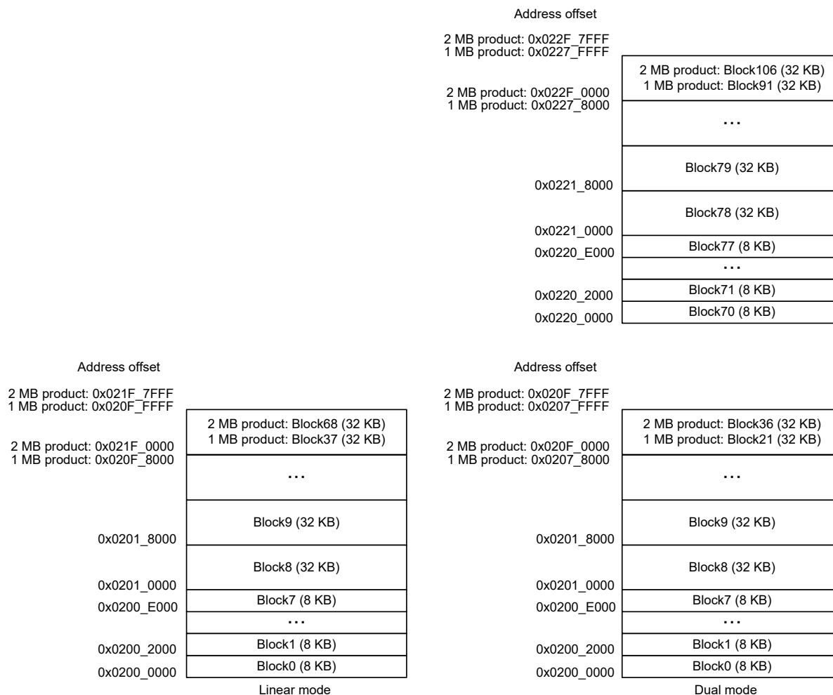
Figure 6.3 Code Flash block structure
