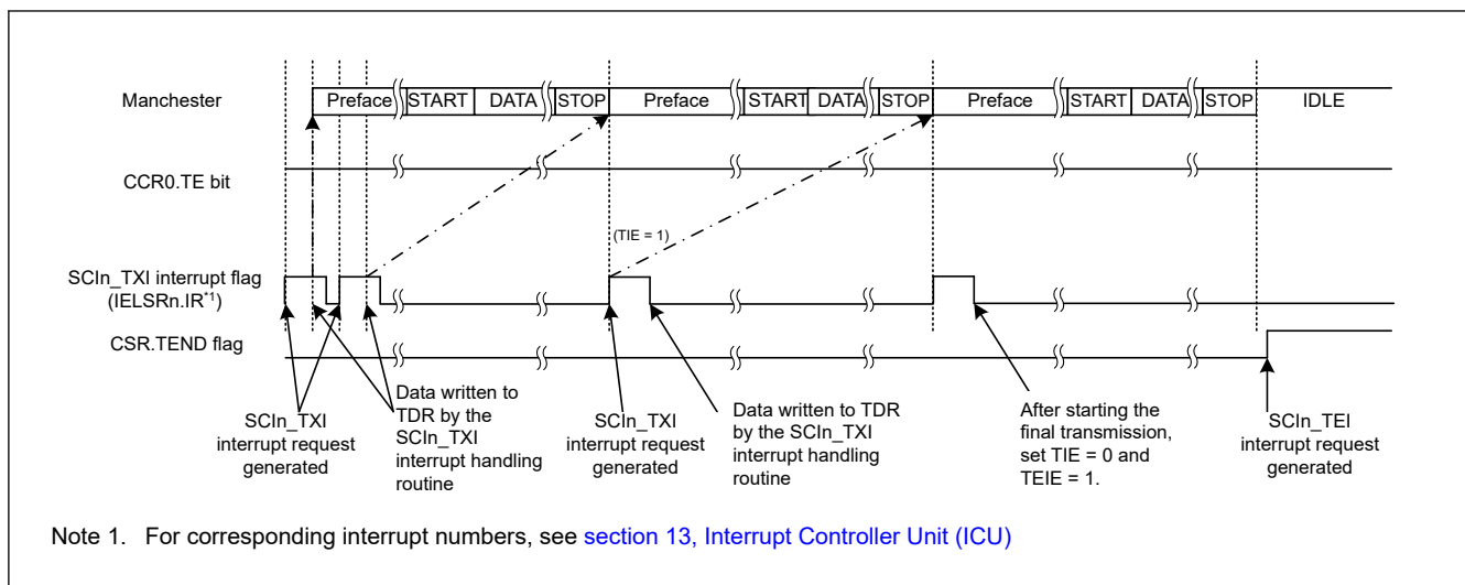
Figure 31.54 Example of End-of-Transmission Operation for Serial Transmission in Manchester Mode (with Preface but Without the CTS Function)
