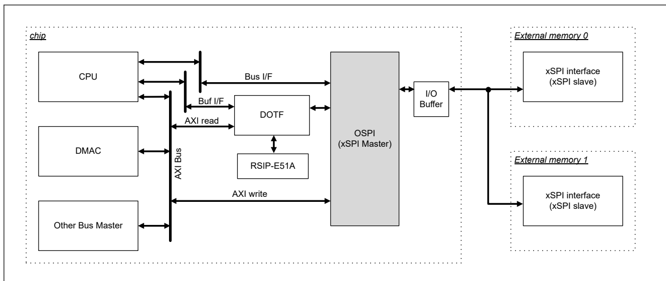
Figure 37.1 Block diagram
