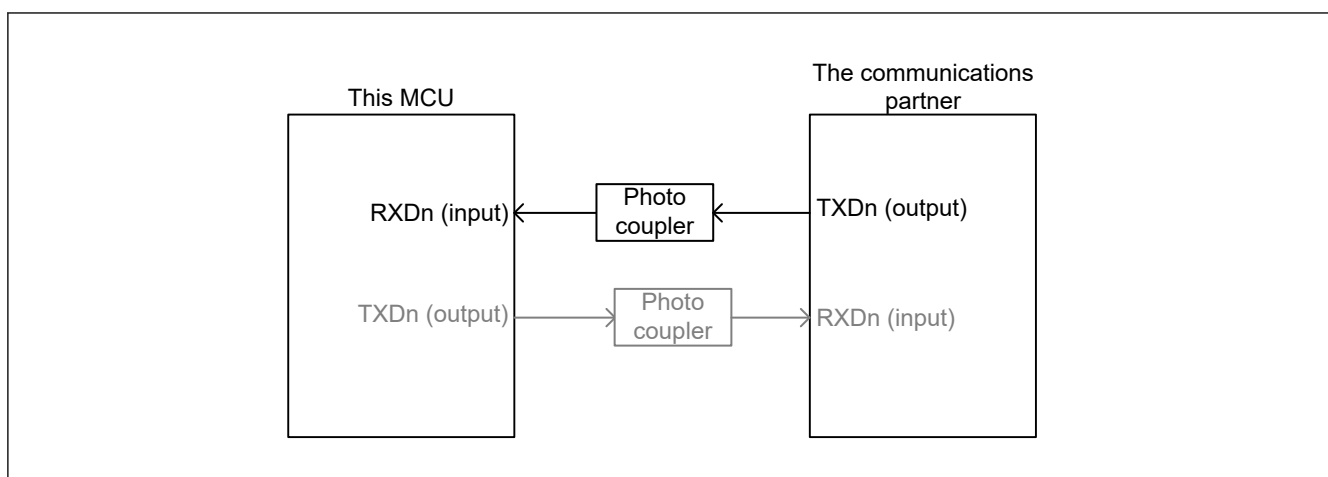
Figure 31.26 Block diagram image of the reception through a photo coupler
