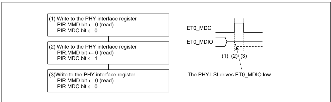
Figure 27.16 Bus release flow, with TA in read operation in Table 27.3
