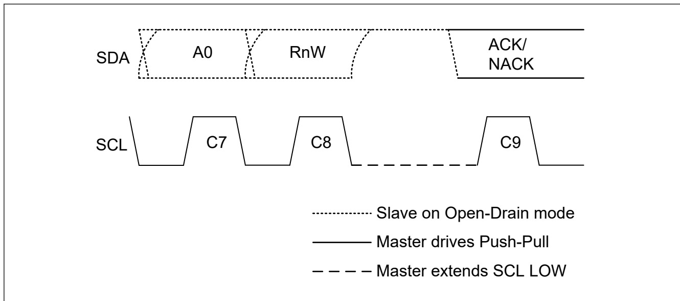
Figure 33.96 Master clock stalling in ACK phase
