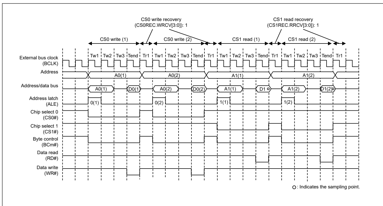
Figure 14.34 Example of recovery cycle insertion when a bus access is split with address/data multiplexed I/O interface (m = 0, 1)
