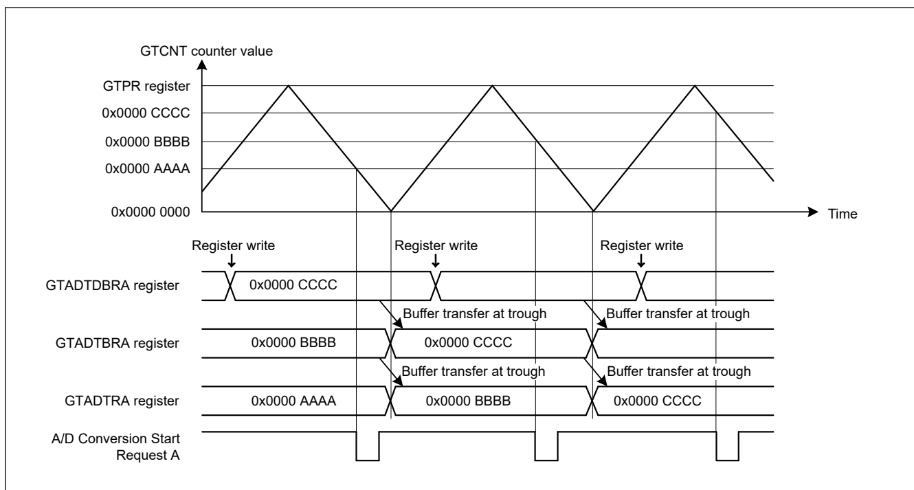
Figure 21.19 Example of double buffer operation of the GTADTRA registers (triangle waves, buffer transfer at troughs, A/D conversion start request generated by down-counting)
