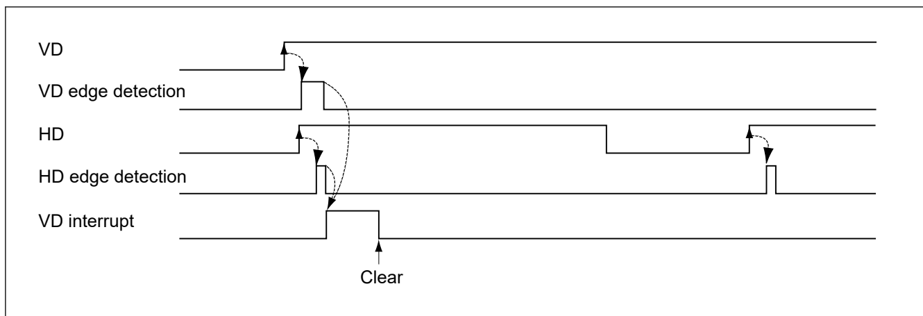
Figure 53.15 Relationship between the VIO_VD and VIO_HD signals and the VD Interrupt when VD and HD are high-active (in Image capture mode or data synchronous fetch mode)
