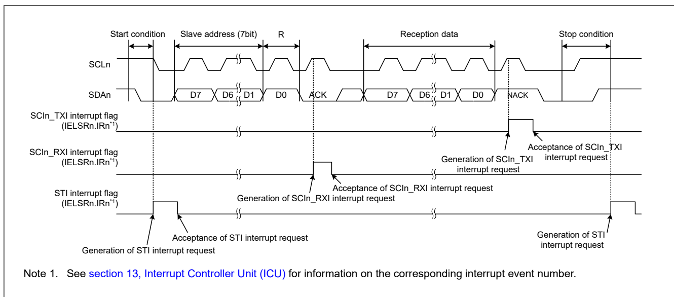
Figure 31.95 Example of Operations for Master Reception in Simple IIC Mode (7bit Slave address, ACK and NACK interrupt in use (ICR.IICINTM = 0))
