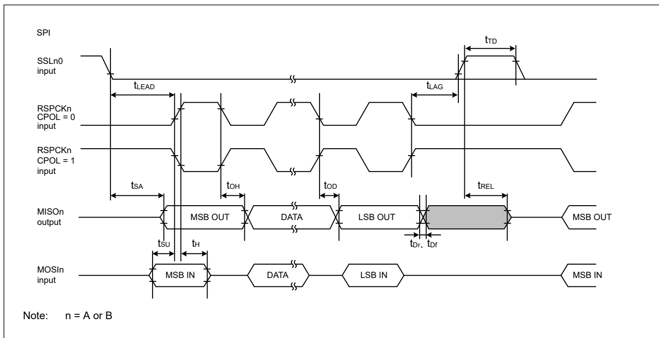
Figure 60.62 SPI timing for Motorola SPI slave when CPHA = 0
