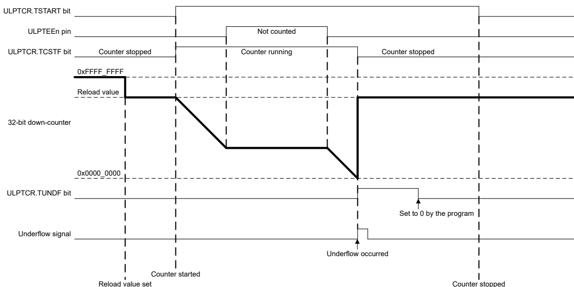
Figure 23.8 Operation example in event counter & one-shot & count enable mode (with the ULPTIOC.TIOGT0 bit set to 1)
