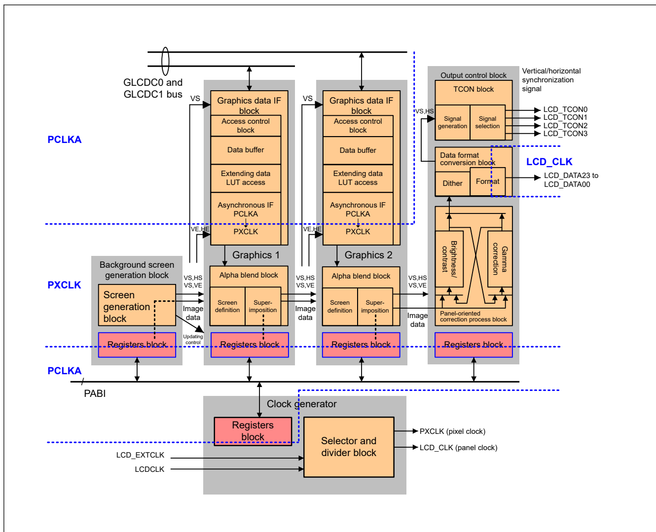
Figure 56.2 GLCDC configuration
