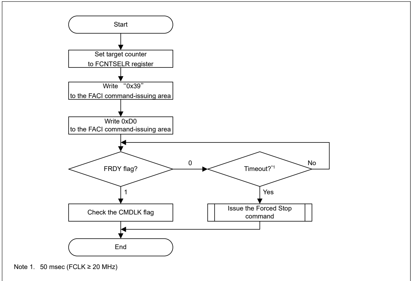
Figure 52.28 Usage of the Read Counter Command
