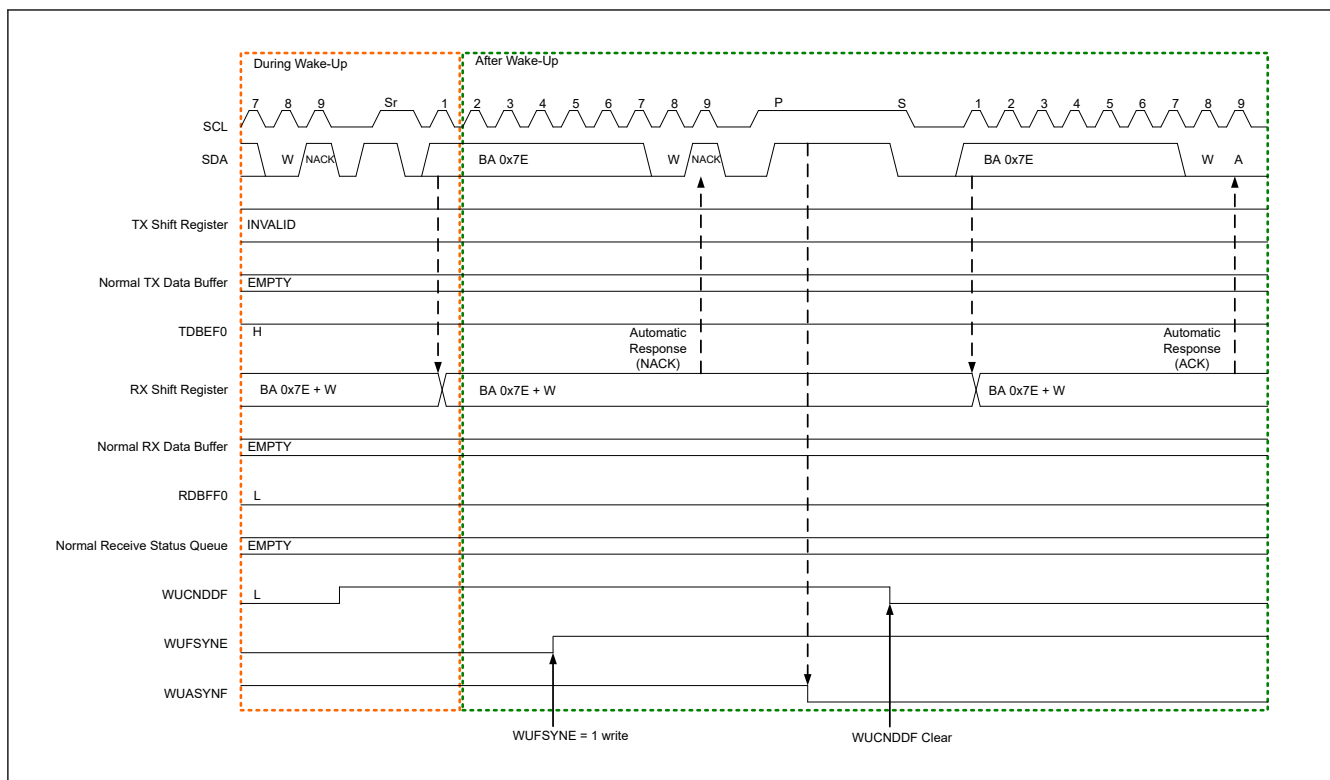
Figure 33.136 I3C slave wake-up operation (2/2)
