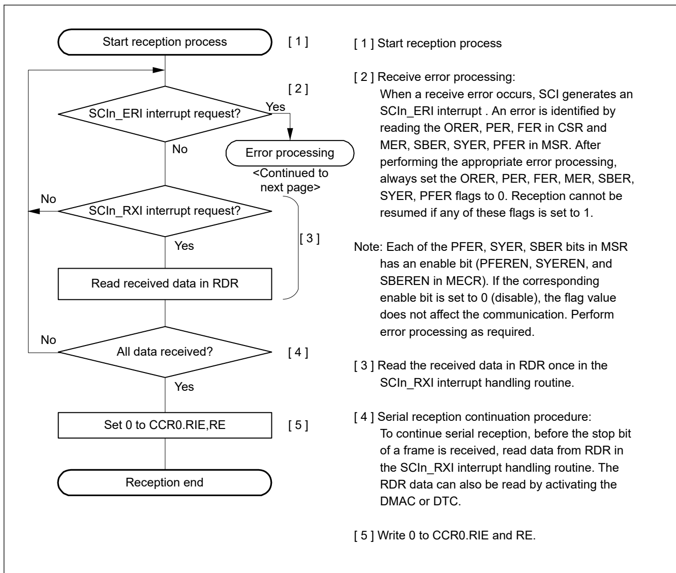
Figure 31.57 Example of Serial Data Reception Flowchart in Manchester Mode (Normal Reception)
