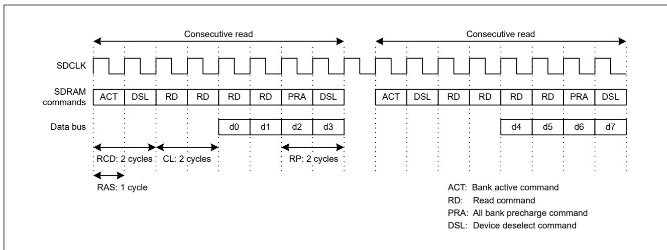
Figure 14.63 Timing example of consecutive read (2)
