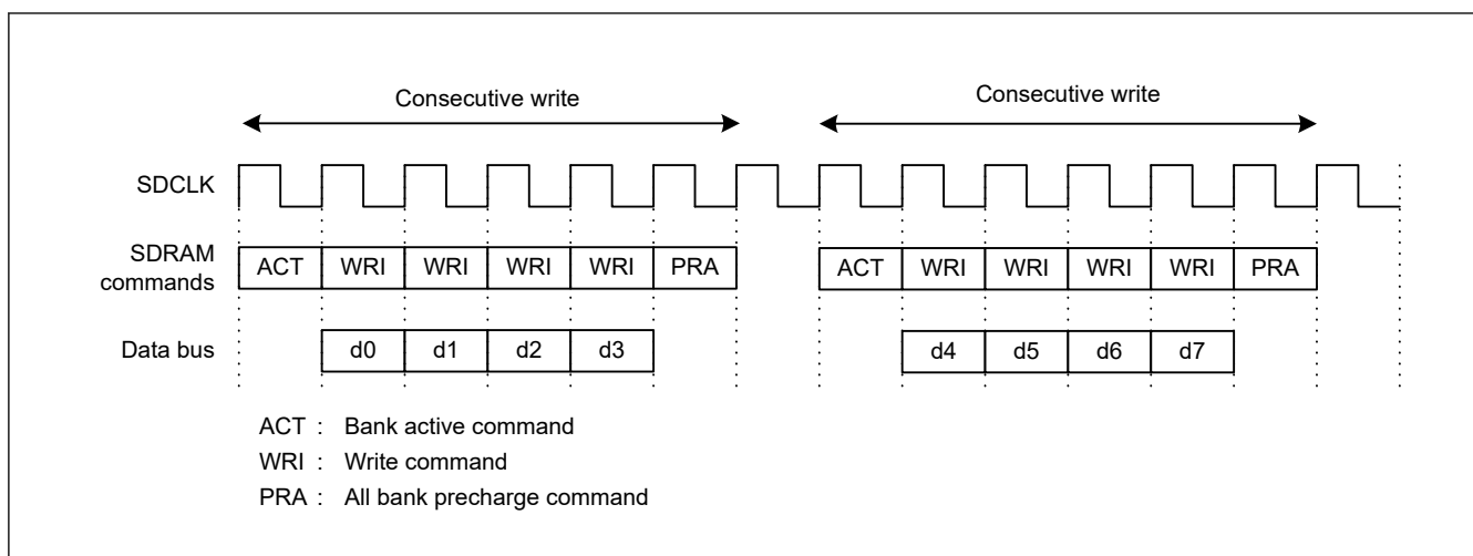
Figure 14.47 Timing Example of Consecutive Write (SDAMOD.BE = 1, when the Earliest Timing is Set)
