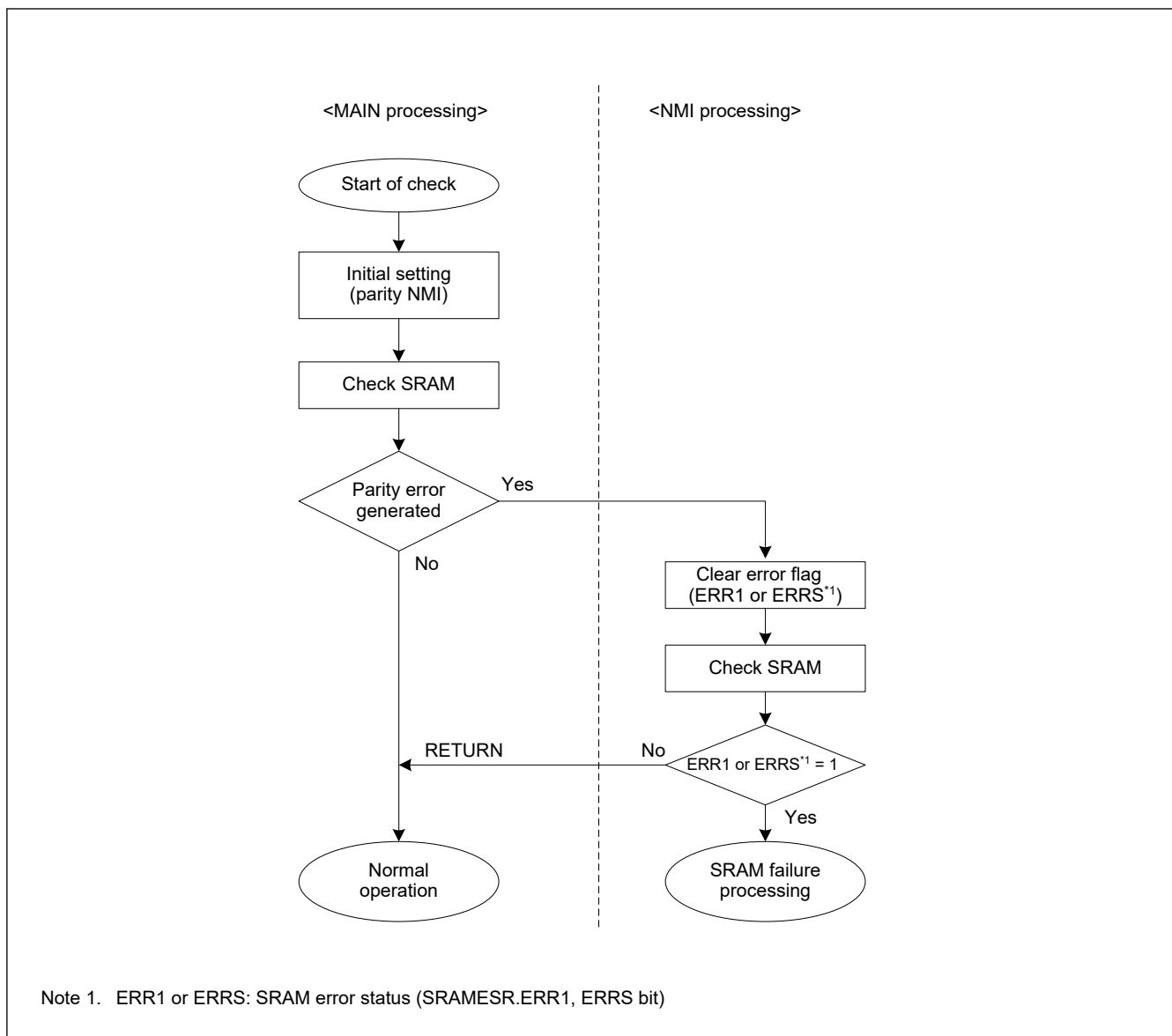
Figure 50.3 Flow of SRAM parity check when SRAM parity interrupt is enabled
