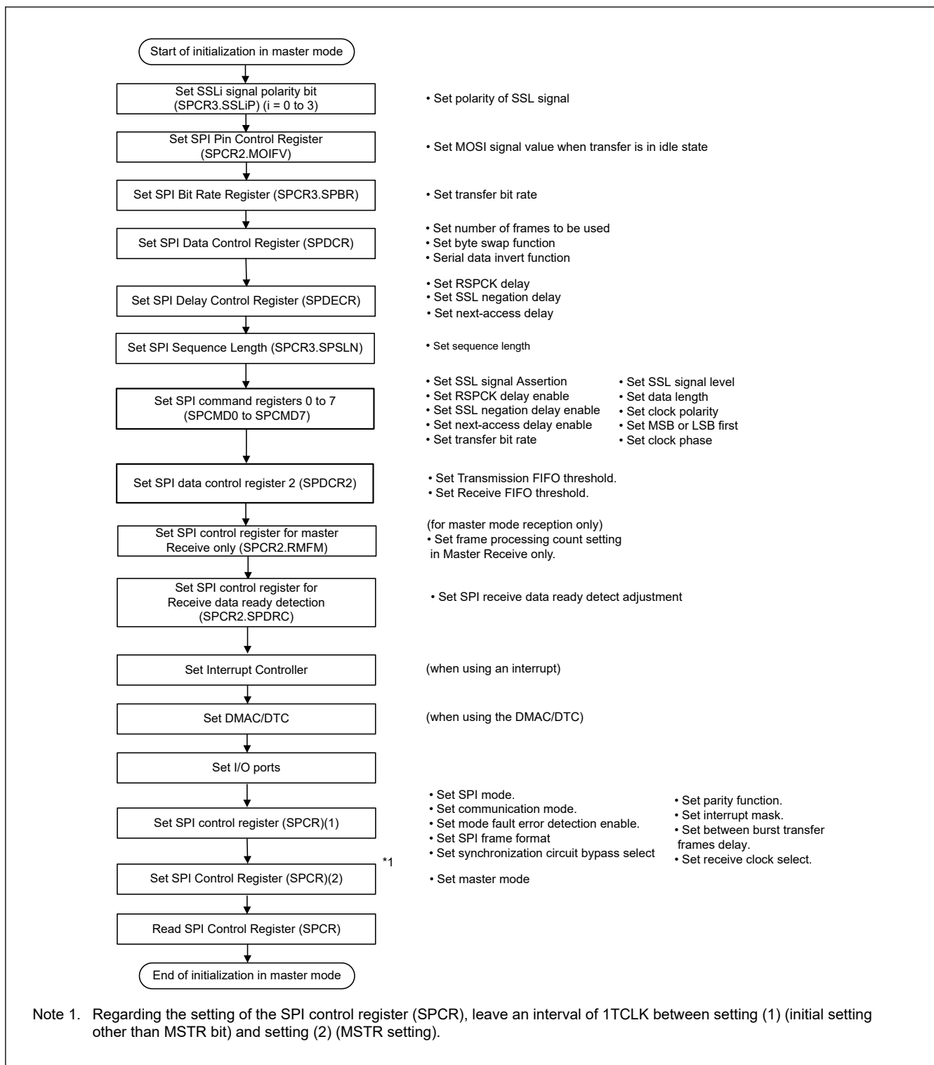
Figure 36.63 Example of initialization flow in master mode for SPI operation
