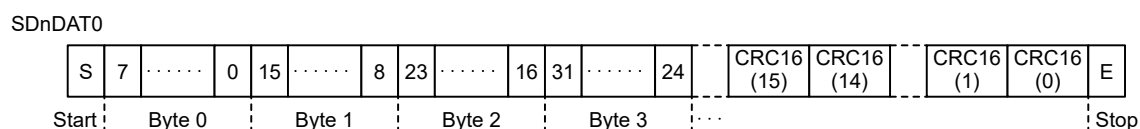
Figure 40.2 SDnDAT in 1-bit width mode
