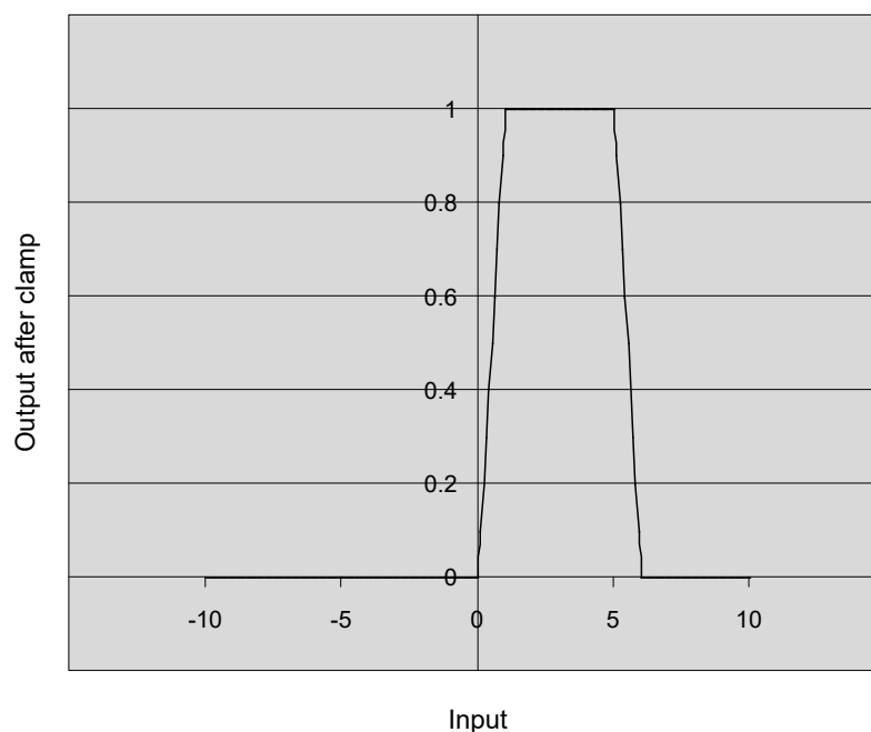
Figure 55.11 Band filter output after clamp with w = 7
