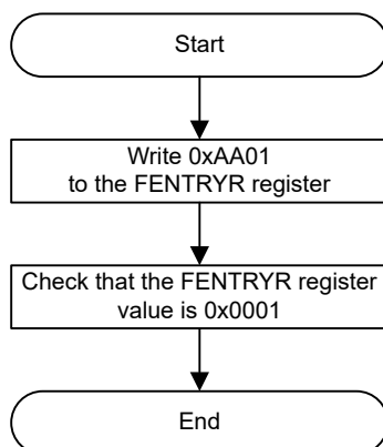
Figure 52.10 Procedure to transition to code flash P/E mode
