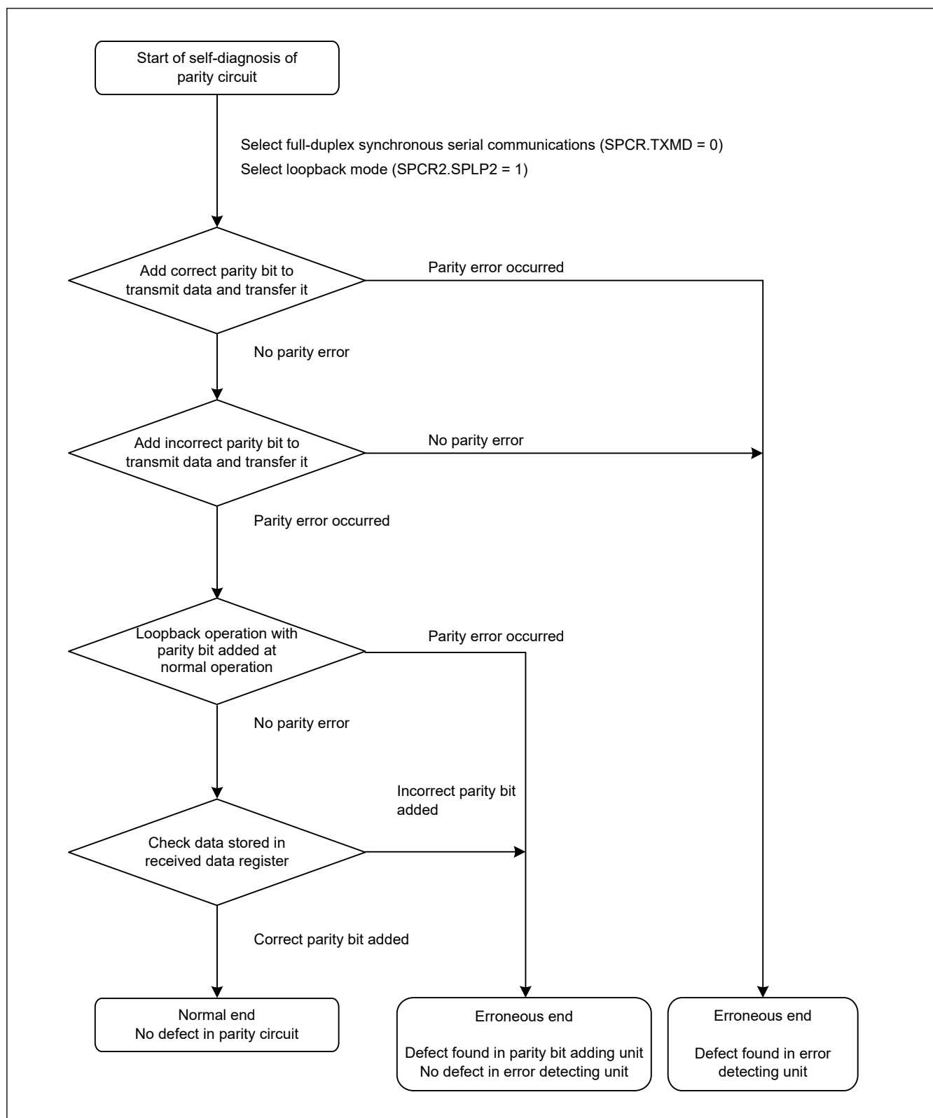
Figure 36.79 Self-diagnosis flow for parity circuit
