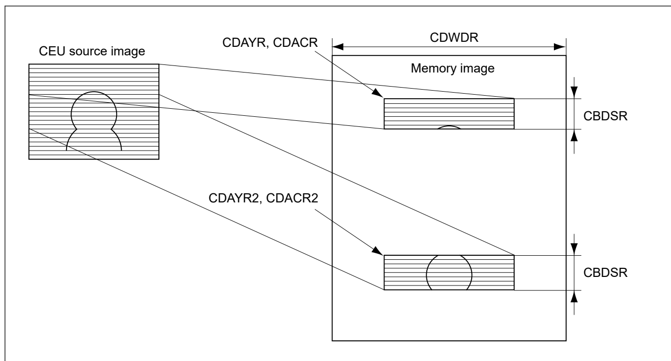
Figure 53.41 Image of bundle write to memory
