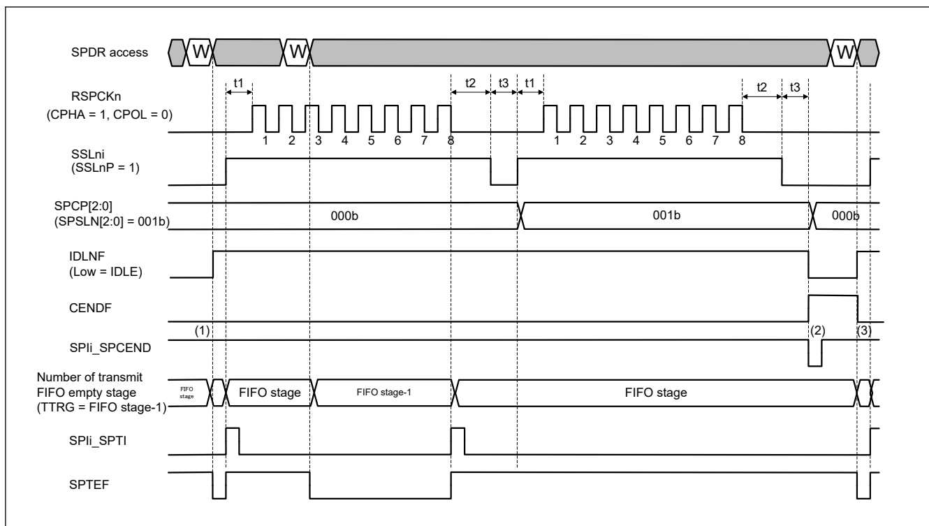
Figure 36.36 Example of Communication End Interrupt Operation (Transmit-Receive/Transmit Master mode/Motorola-SPI)
