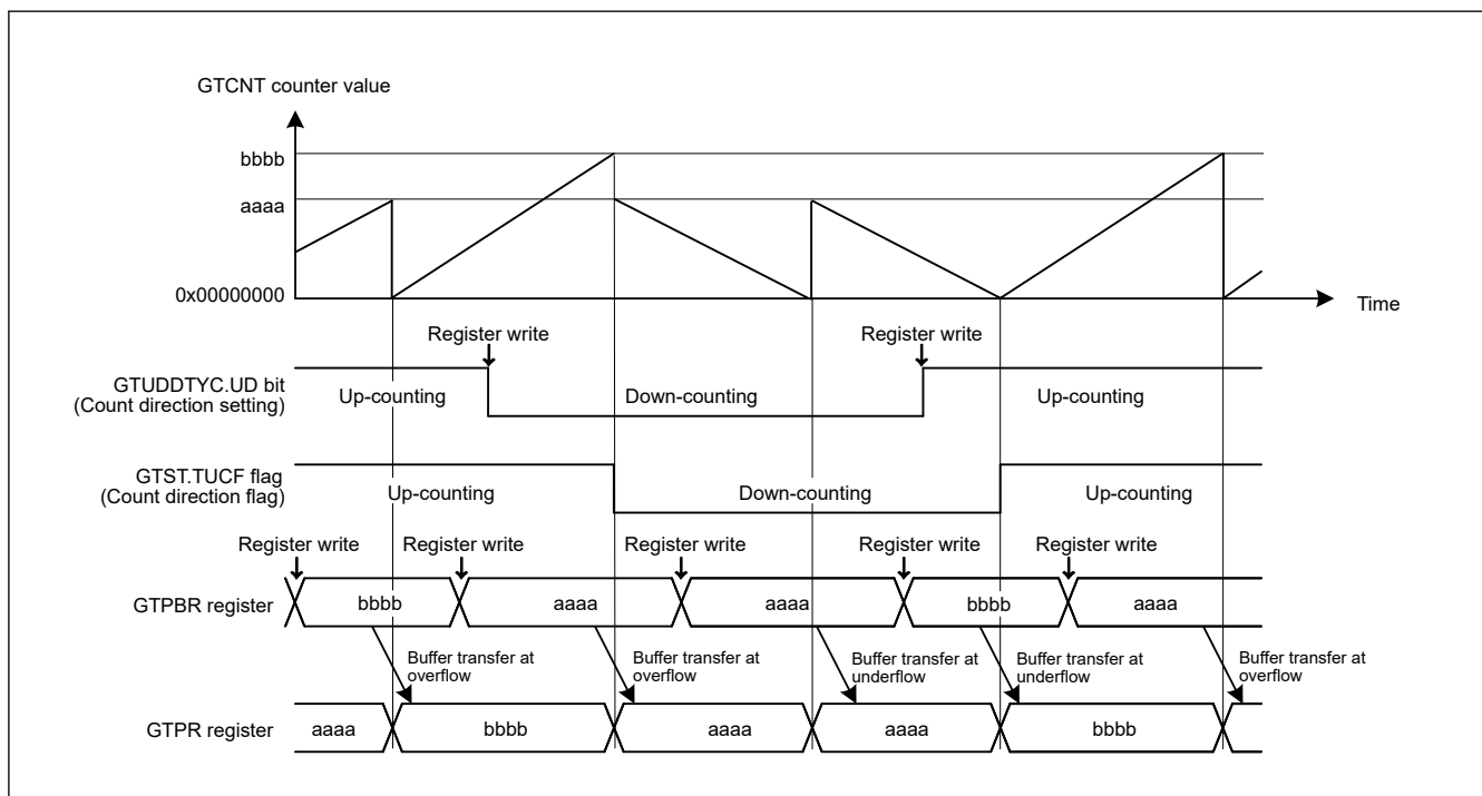
Figure 21.30 Example of a count direction changing function operation during buffer operation
