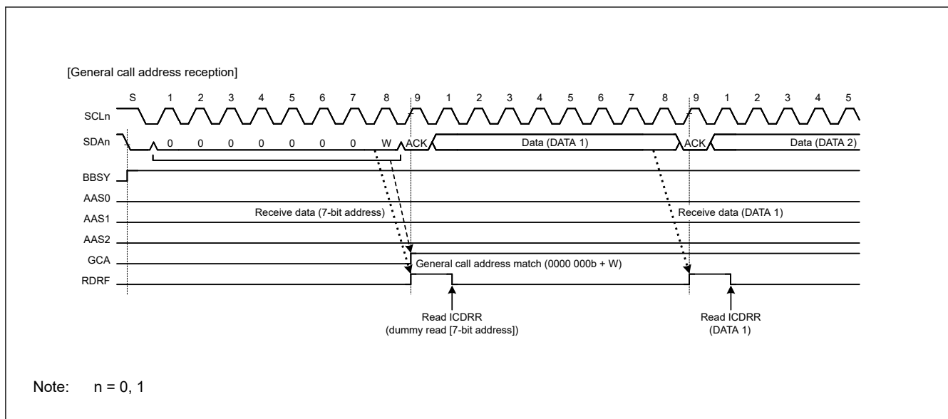
Figure 32.27 Timing of GCA flag setting during reception of general call address
