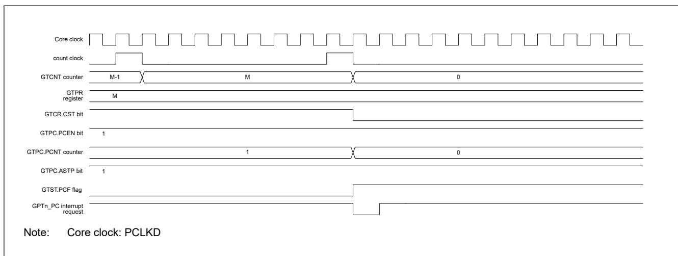
Figure 21.51 Example of the timing of operations for PWM cycle count function (saw-wave one-shot pulse mode, up-counting)
