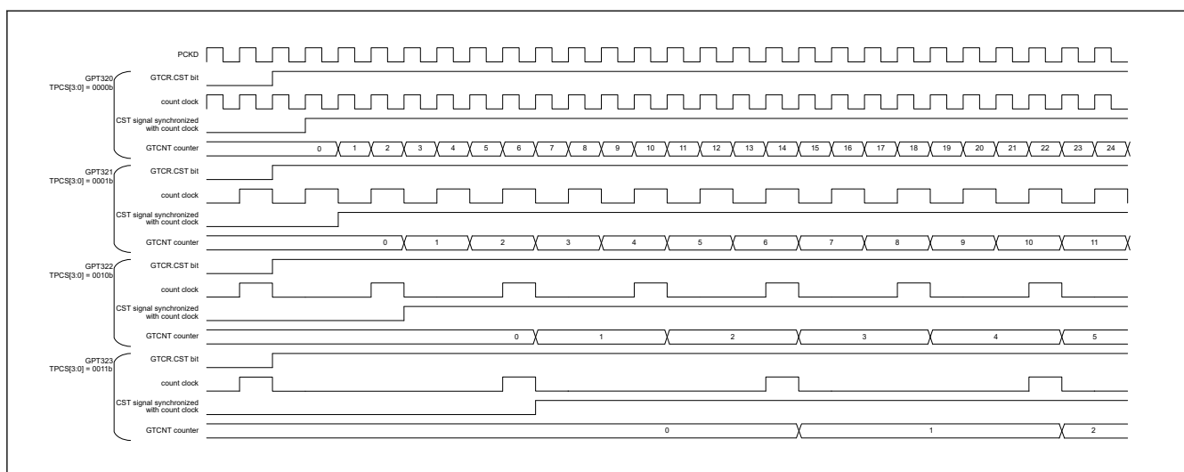
Figure 21.40 Example of Simultaneous Start Operation by Software (with Different Count Period)
