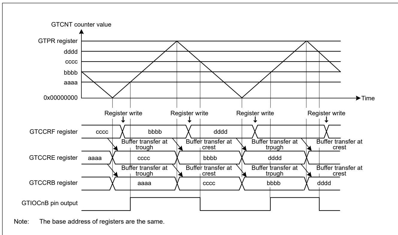
Figure 21.15 Example of GTCCRB double buffer operation with output compare, triangle waves, buffer operation at both troughs and crests, output toggled at GTCCRB compare match, and output retained at cycle end
