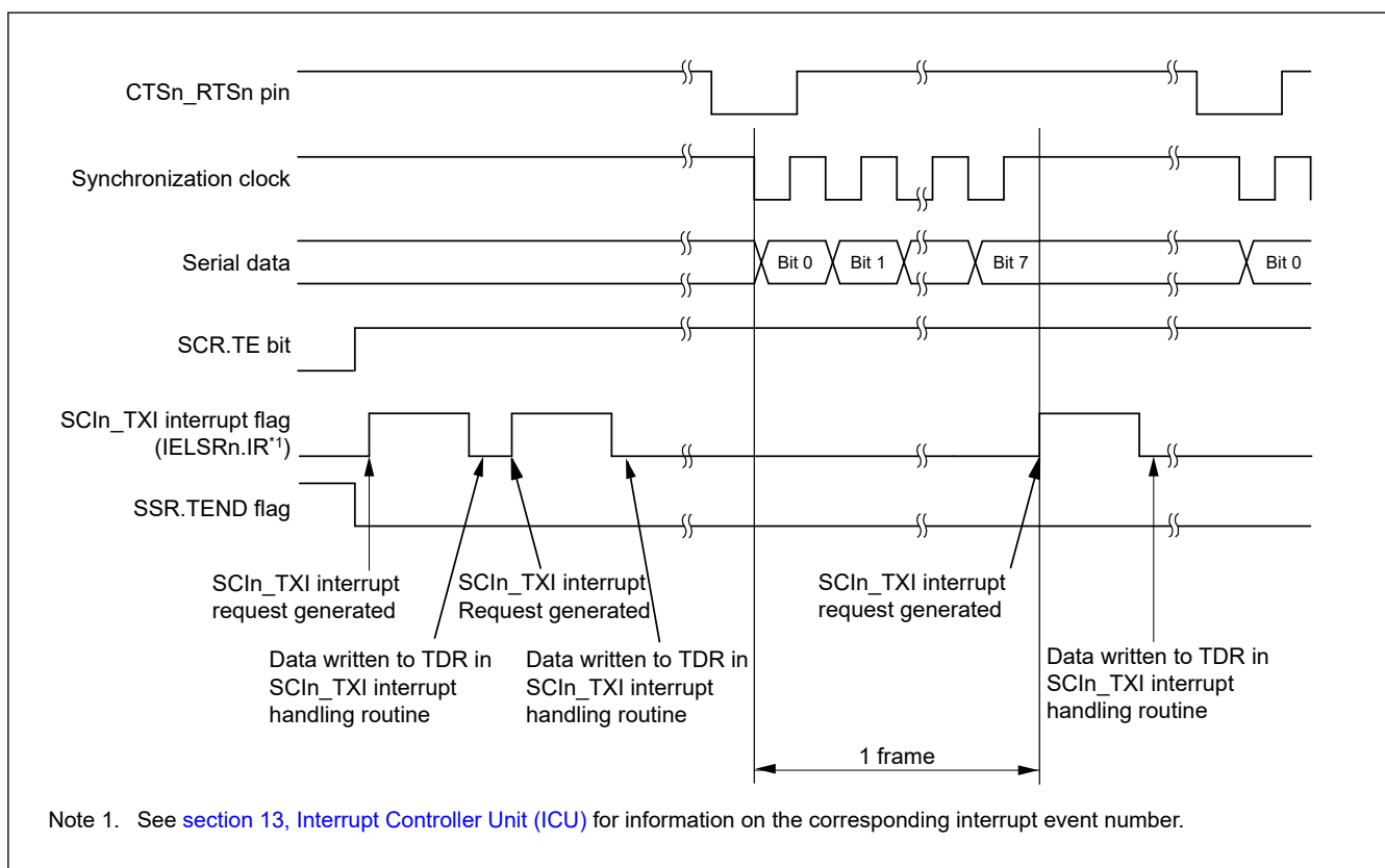
Figure 31.63 Example of serial data transmission in clock synchronous mode when the CTS function is used at the beginning of transmission
