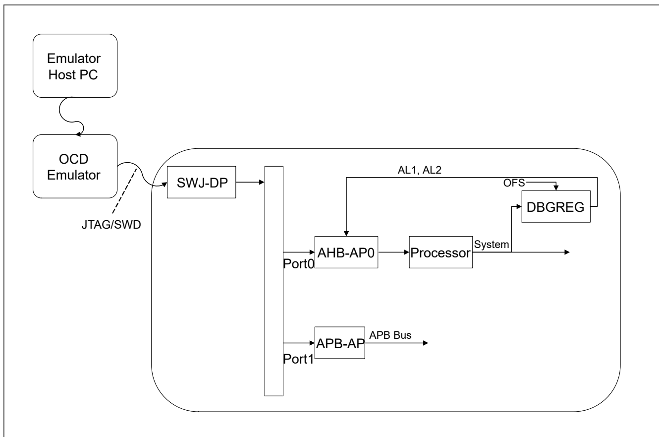
Figure 2.6 Control authentication level using software
