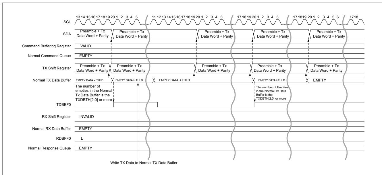
Figure 33.26 HDR data write transfer (HDR-DDR) timing (3/4)
