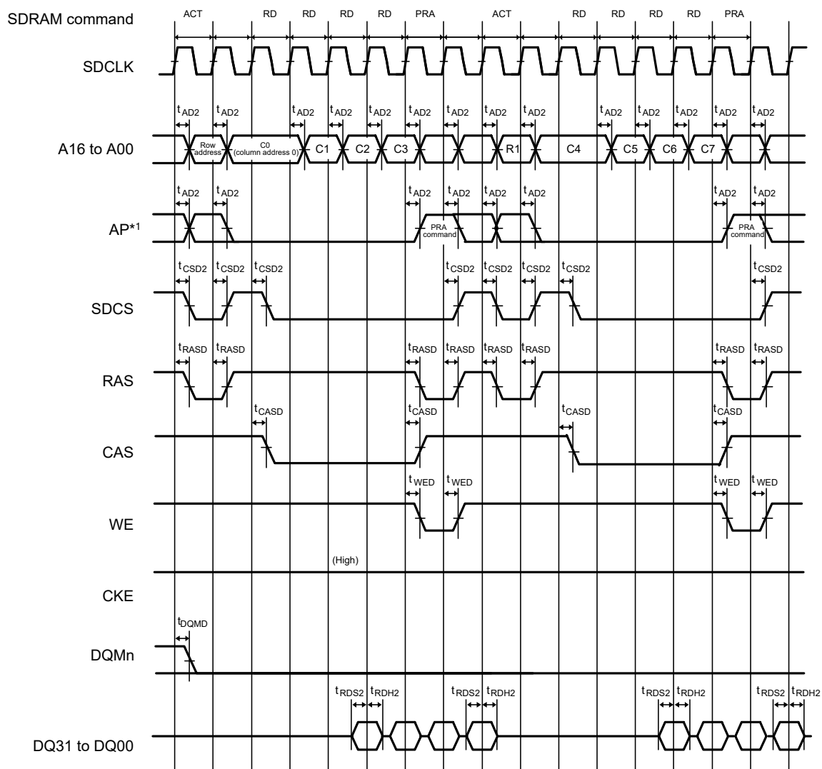
Figure 60.39 SDRAM multiple read line stride timing
