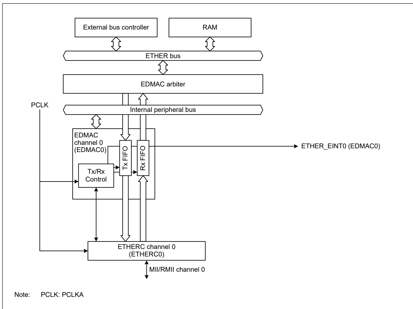
Figure 28.1 EDMAC configuration
