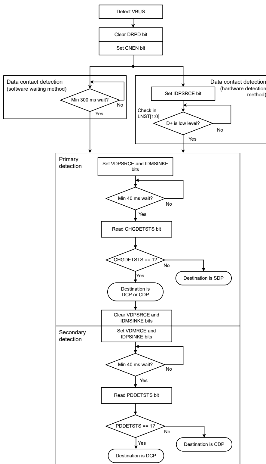
Figure 30.19 Processing flow as portable device
