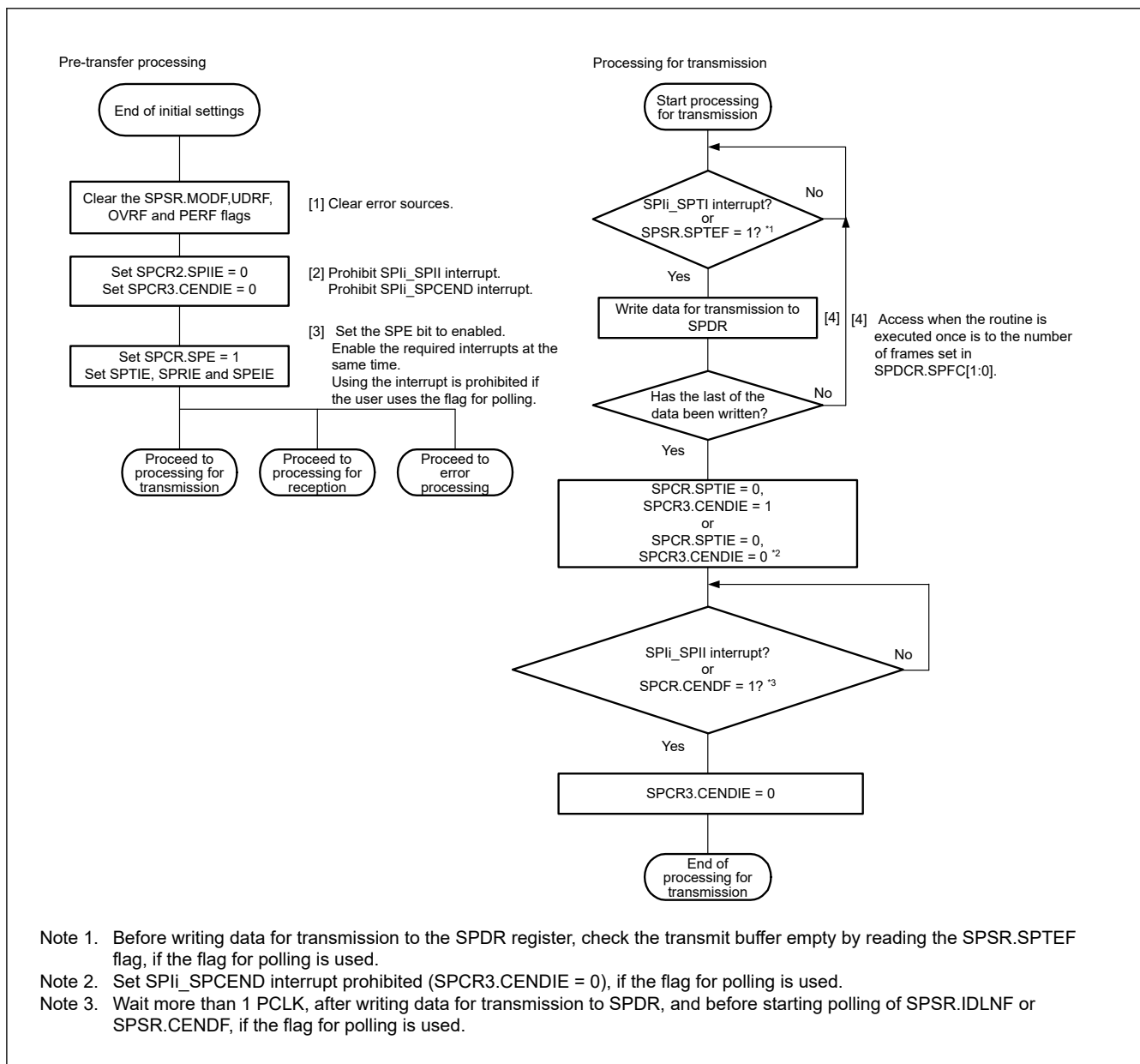
Figure 29.53 Transmission flow in slave mode
