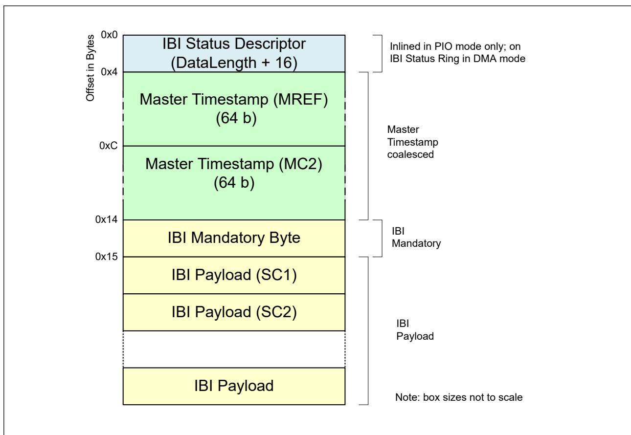
Figure 26.87 Master timestamp counters for IBI event
