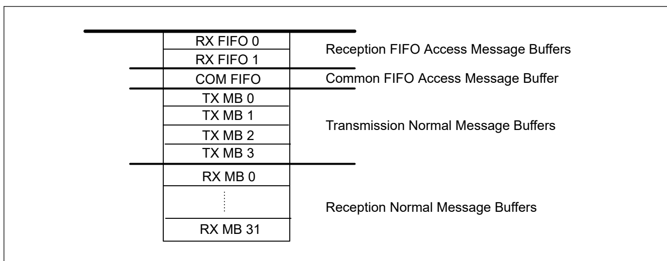
Figure 27.29 Message buffer configuration
