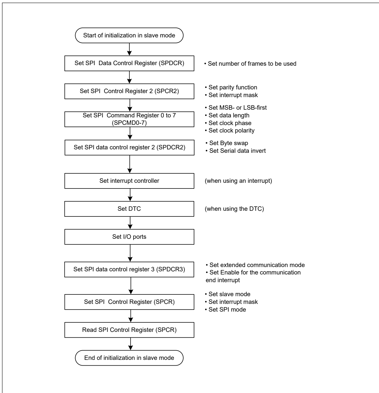
Figure 29.60 Example of initialization flow in slave mode for clock synchronous operation
