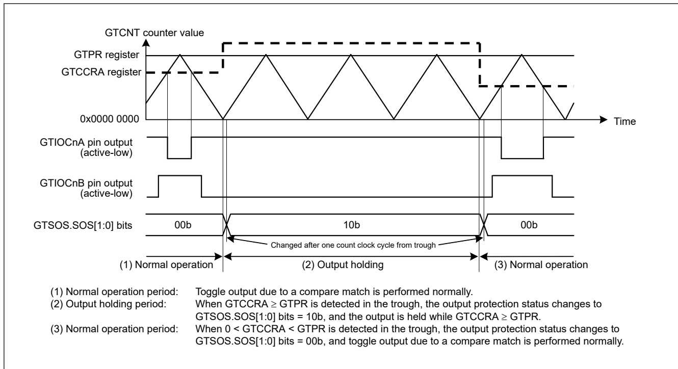
Figure 20.87 Example of output protection function operation when GTCCRA \geq GTPR is set during buffer transfer at troughs (restored to 0 < \text{GTCCRA} < \text{GTPR} during buffer transfer at troughs, active-low) (n = 0 to 5)
