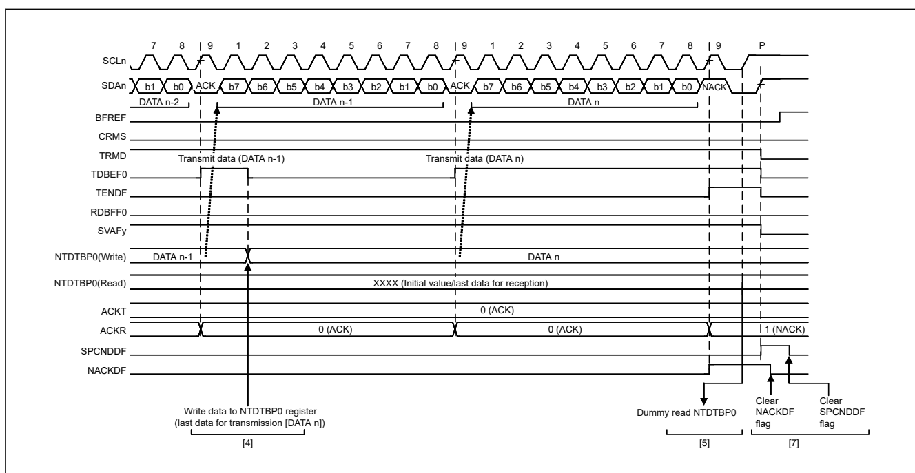
Figure 26.30 Slave transmit operation timing (2)
