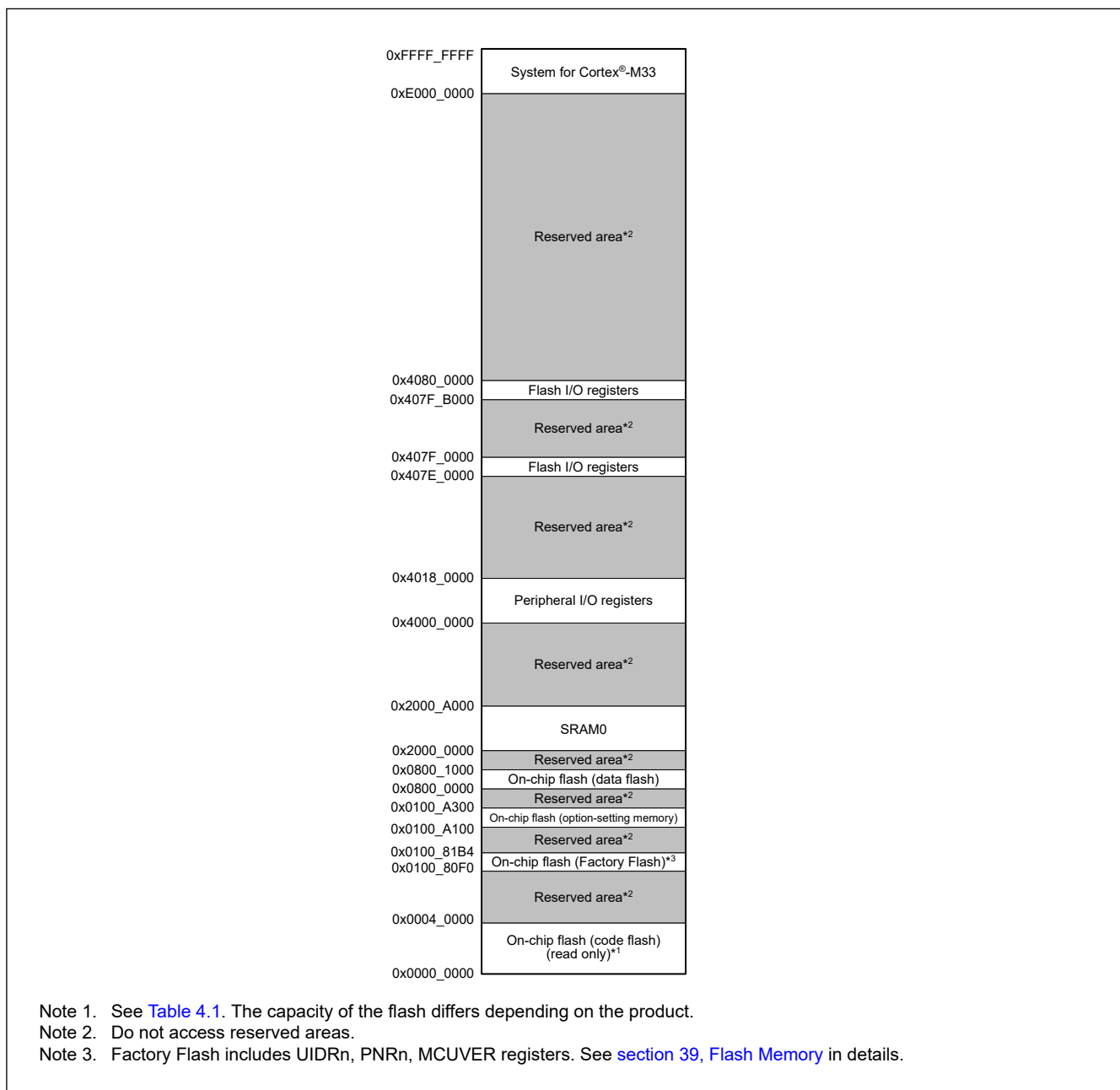
Figure 4.1 Memory map
