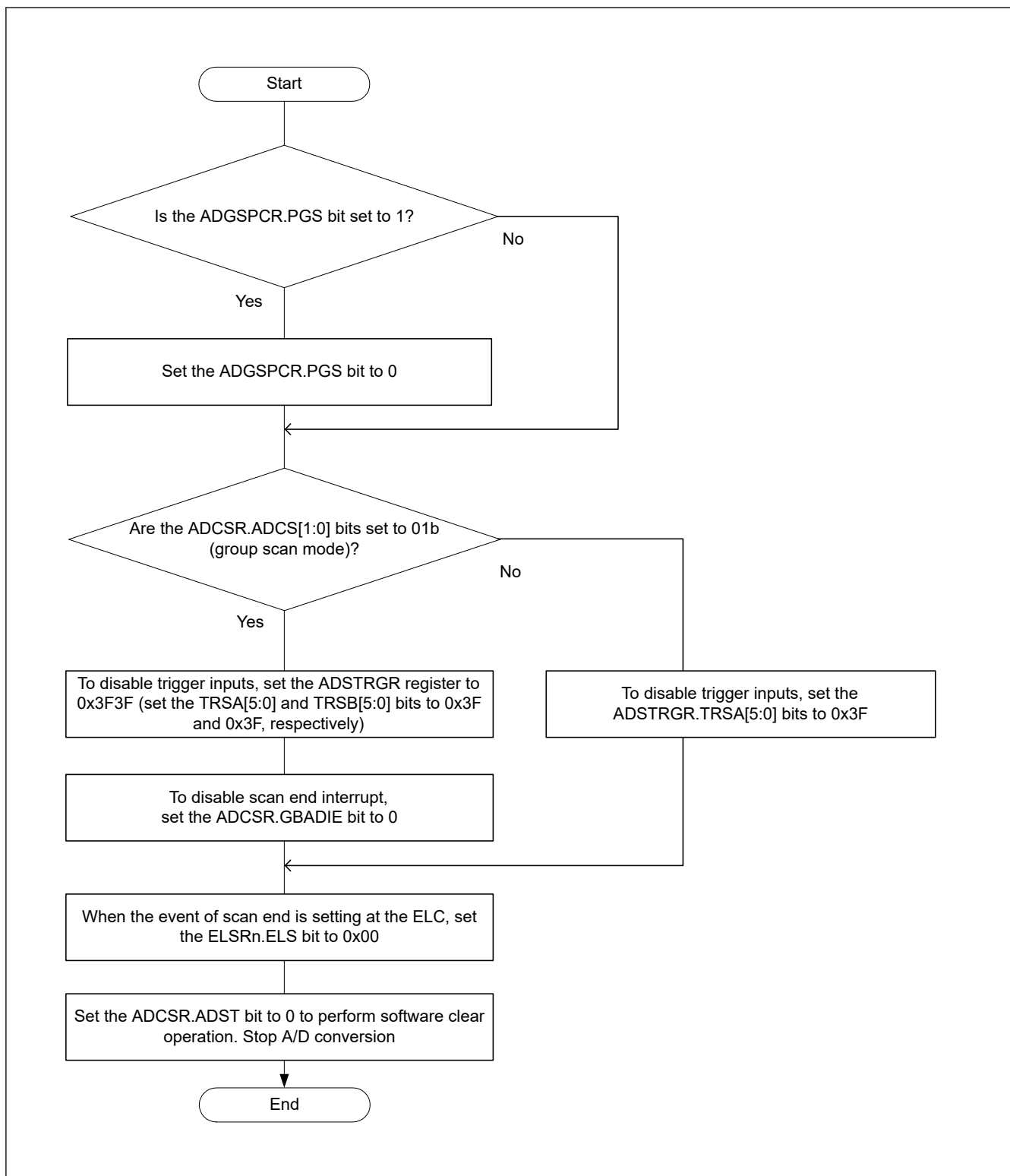
Figure 33.41 Procedure for clearing the ADCSR.ADST bit by software
