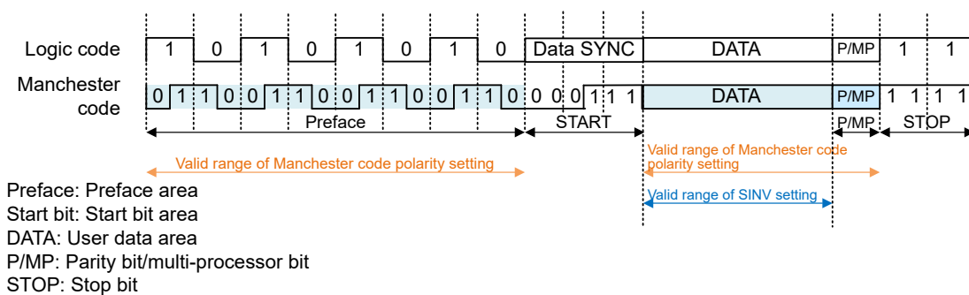
Figure 25.61 Valid Range of the Manchester Code Polarity Setting
