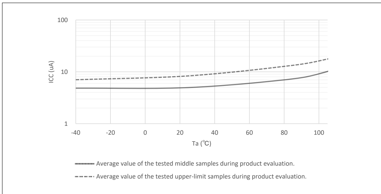
Figure 42.5 Temperature dependency in Deep Software Standby mode, DPSBYCR.DEEPCUT[1:0] = 11b (reference data)
