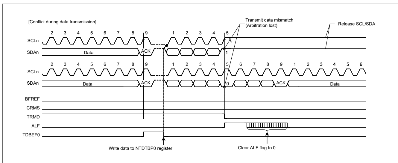
Figure 26.69 Example of slave arbitration-lost detection (SALE = 1)
