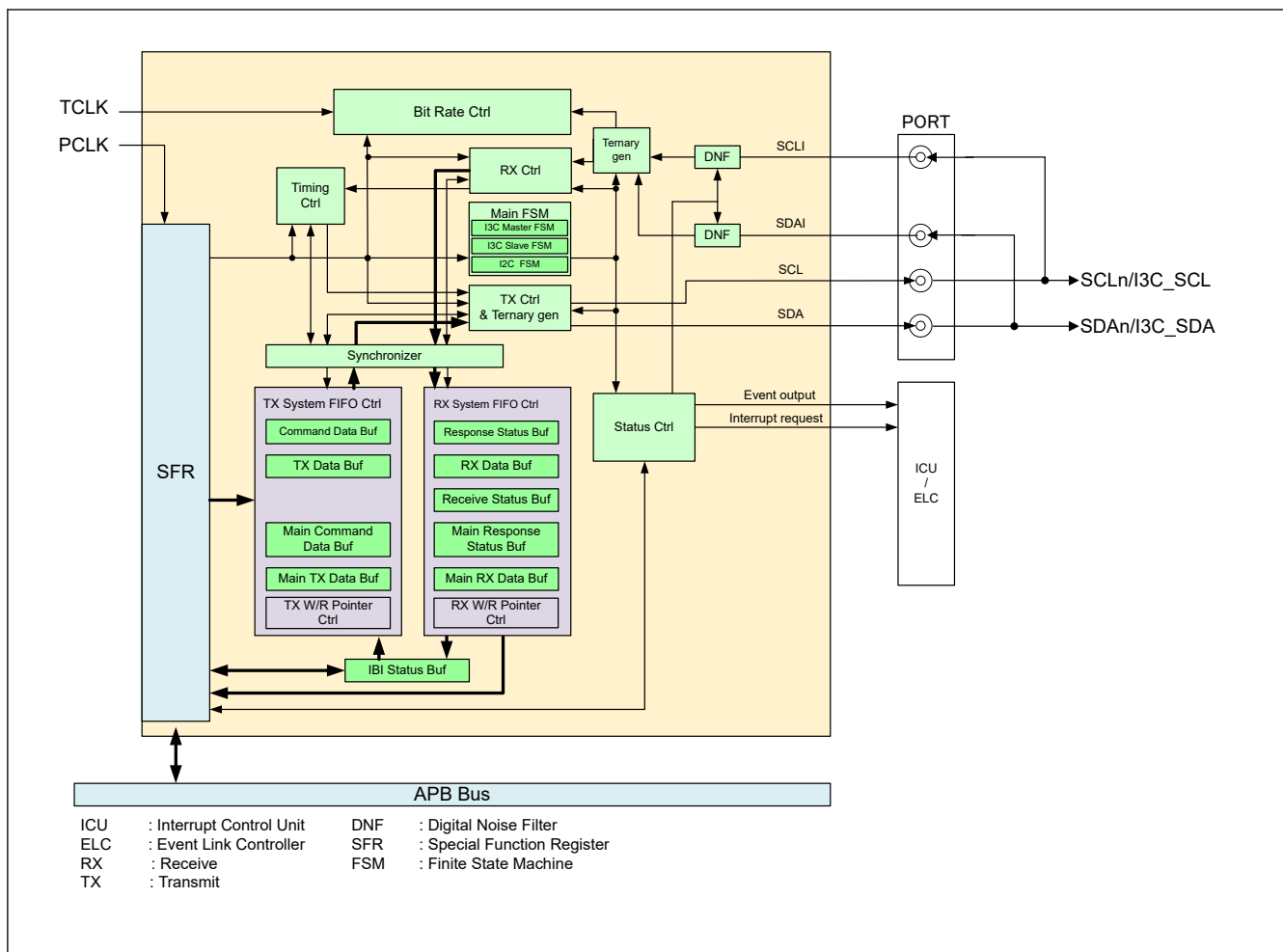
Figure 26.1 I3C block diagram
