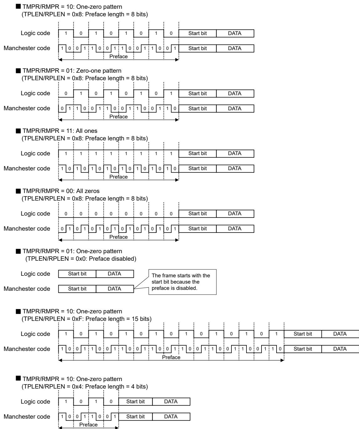
Figure 25.48 Preface Pattern Setting Example
