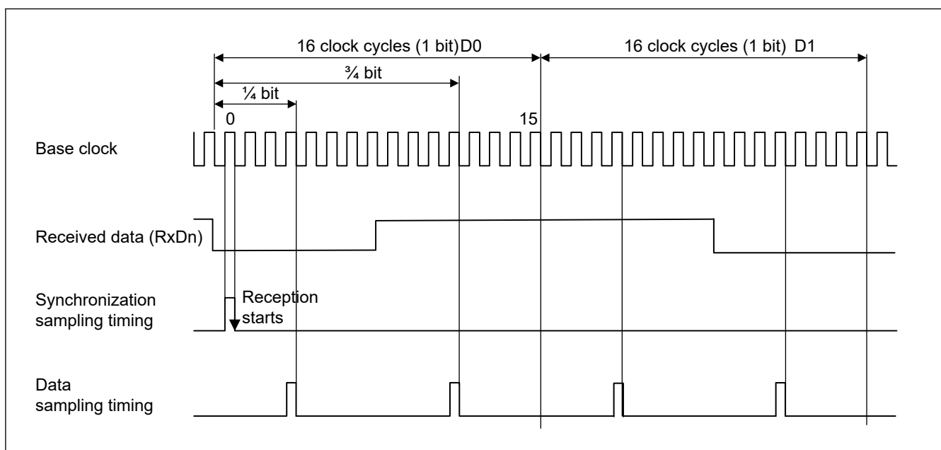
Figure 25.56 Data Reception Sampling Timing in Manchester Mode
