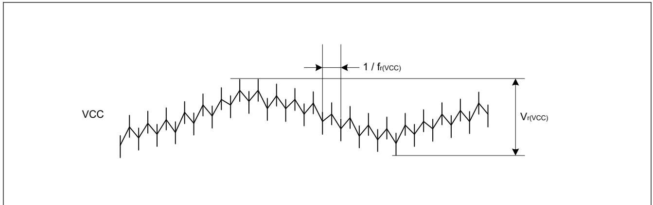
Figure 46.2 Ripple waveform
