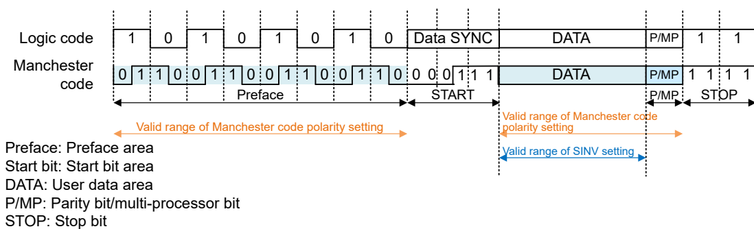
Figure 26.58 Valid Range of the Manchester Code Polarity Setting
