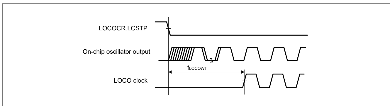
Figure 46.5 LOCO clock oscillation start timing
