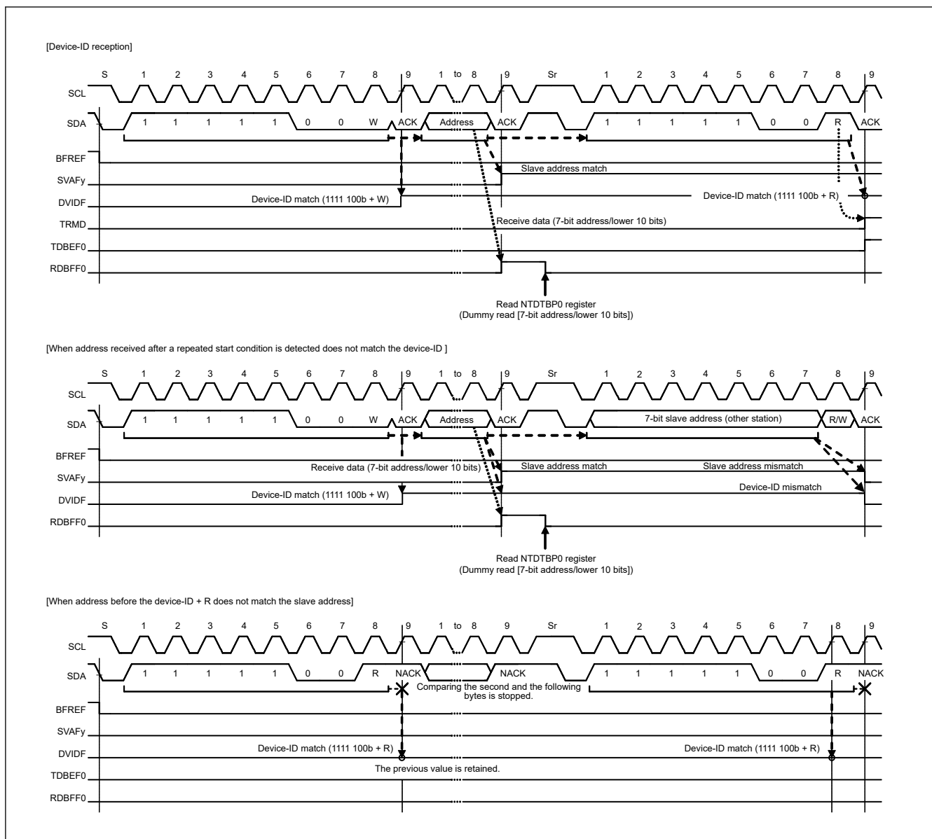
Figure 27.22 SVAy/DVIDF flag set/clear timing during reception of device-ID
