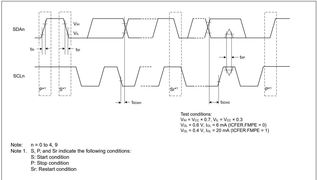
Figure 46.38 SCL simple IIC mode timing
