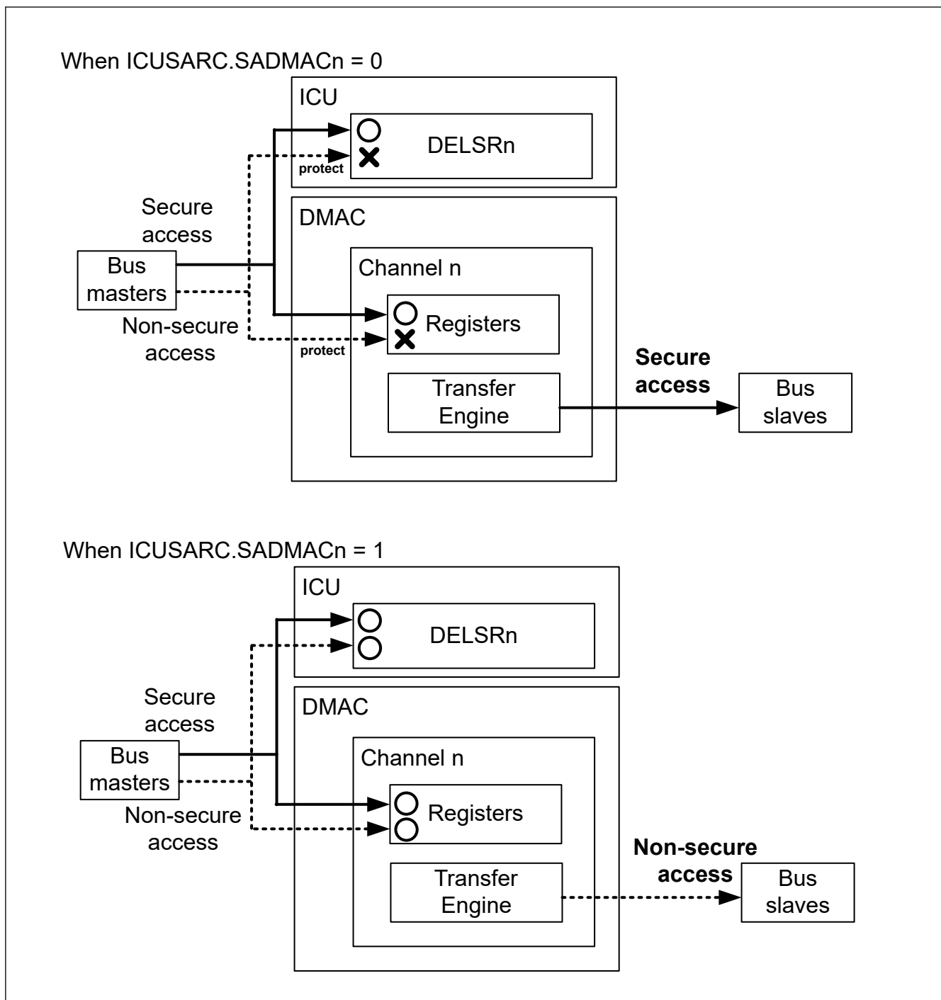
Figure 15.22 Security attribute about each DMAC channels
