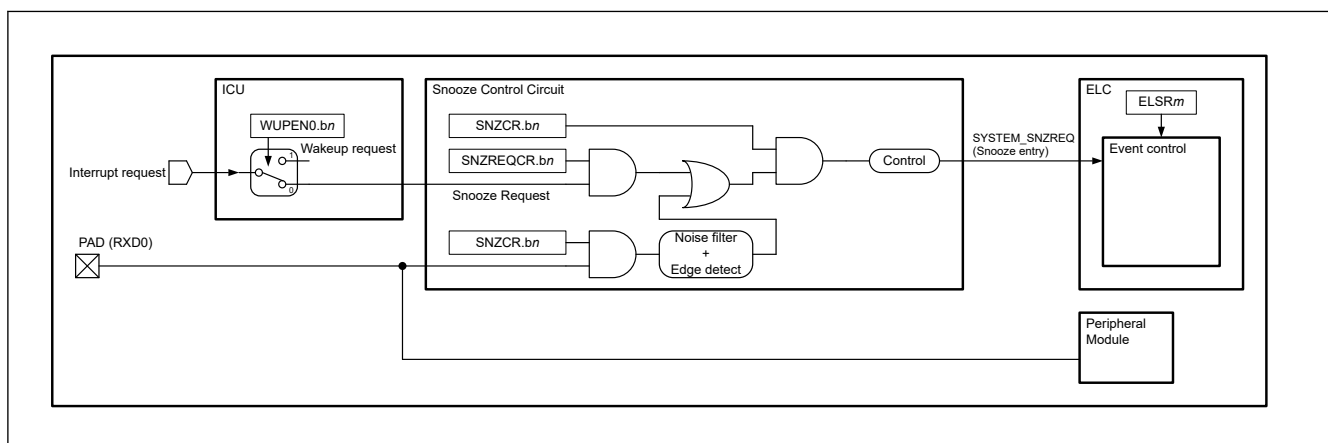
Figure 10.5 Snooze mode entry configuration
