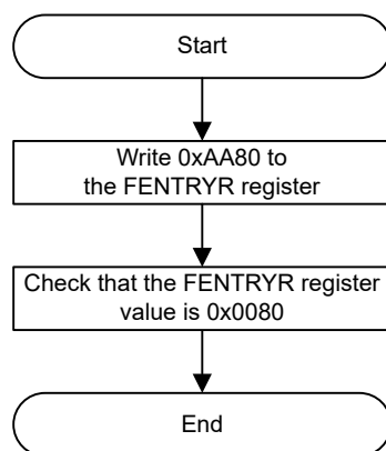
Figure 43.10 Procedure to transition to data flash P/E mode
