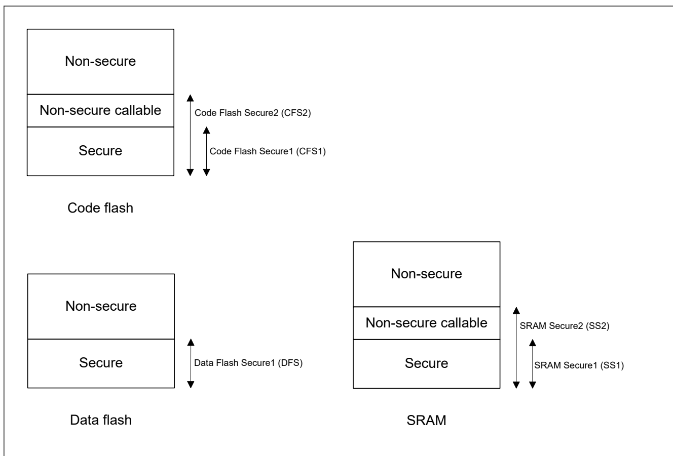
Figure 44.1 Memory mapping
