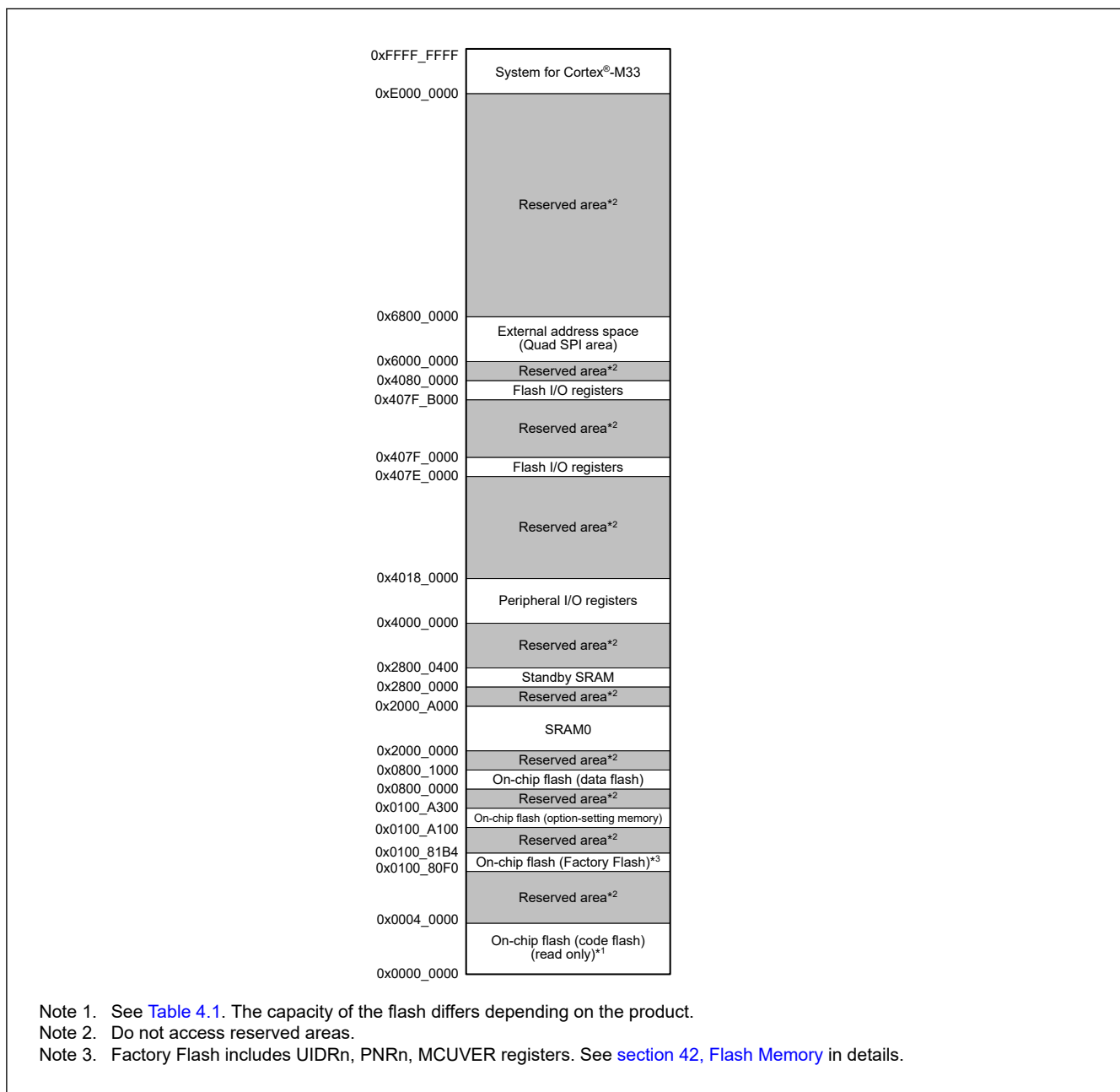
Figure 4.1 Memory map
