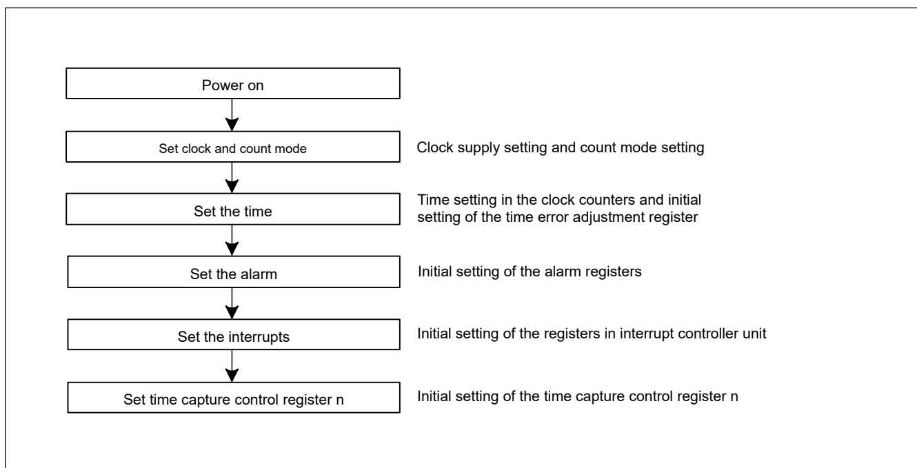
Figure 22.2 Outline of initial settings after a power on
