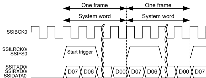
Figure 33.40 Long frame in monaural format (without padding)
