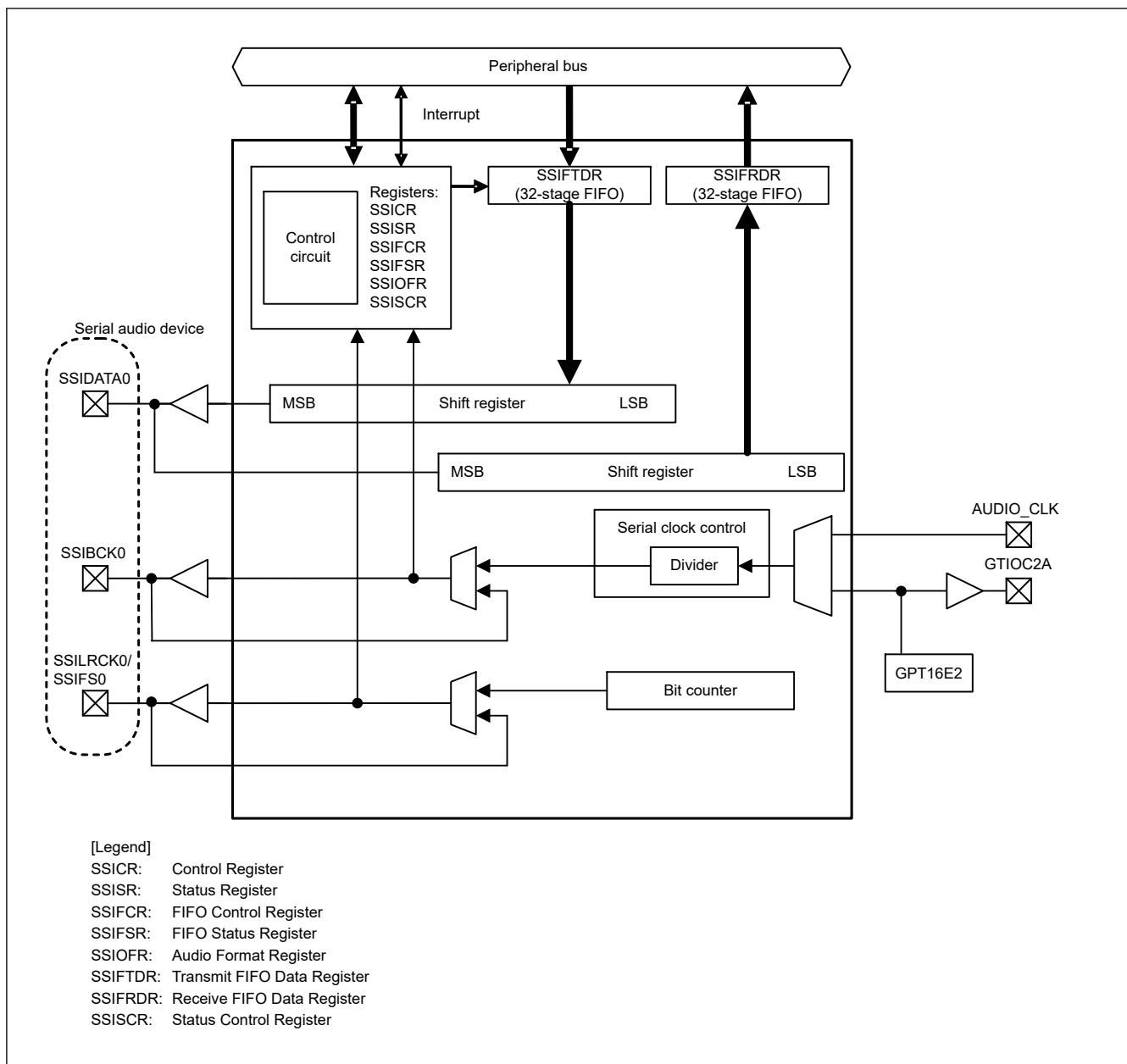
Figure 33.3 SSIE block diagram for half-duplex communication
