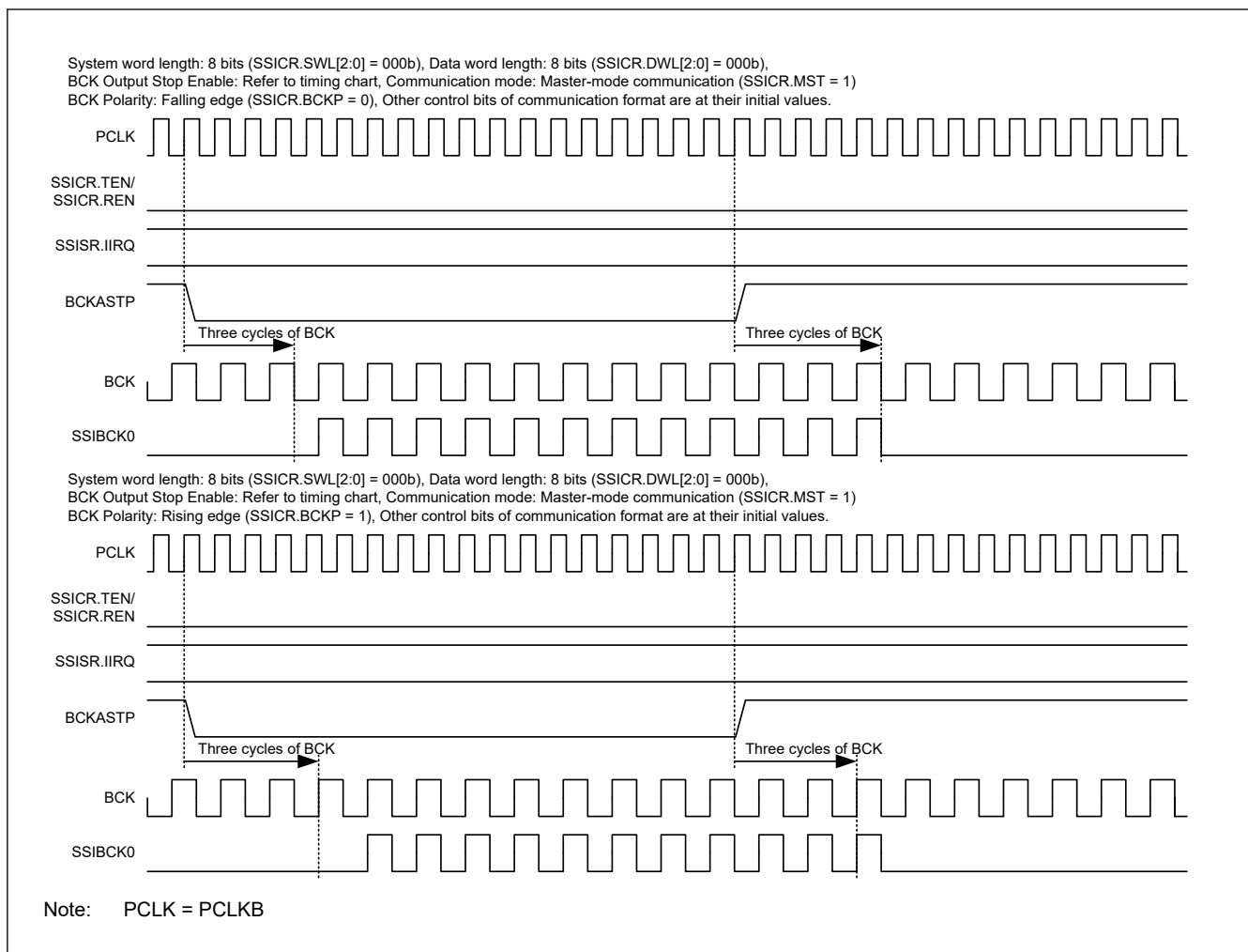
Figure 33.34 Example operation of the BCKASTP bit (idle state)
