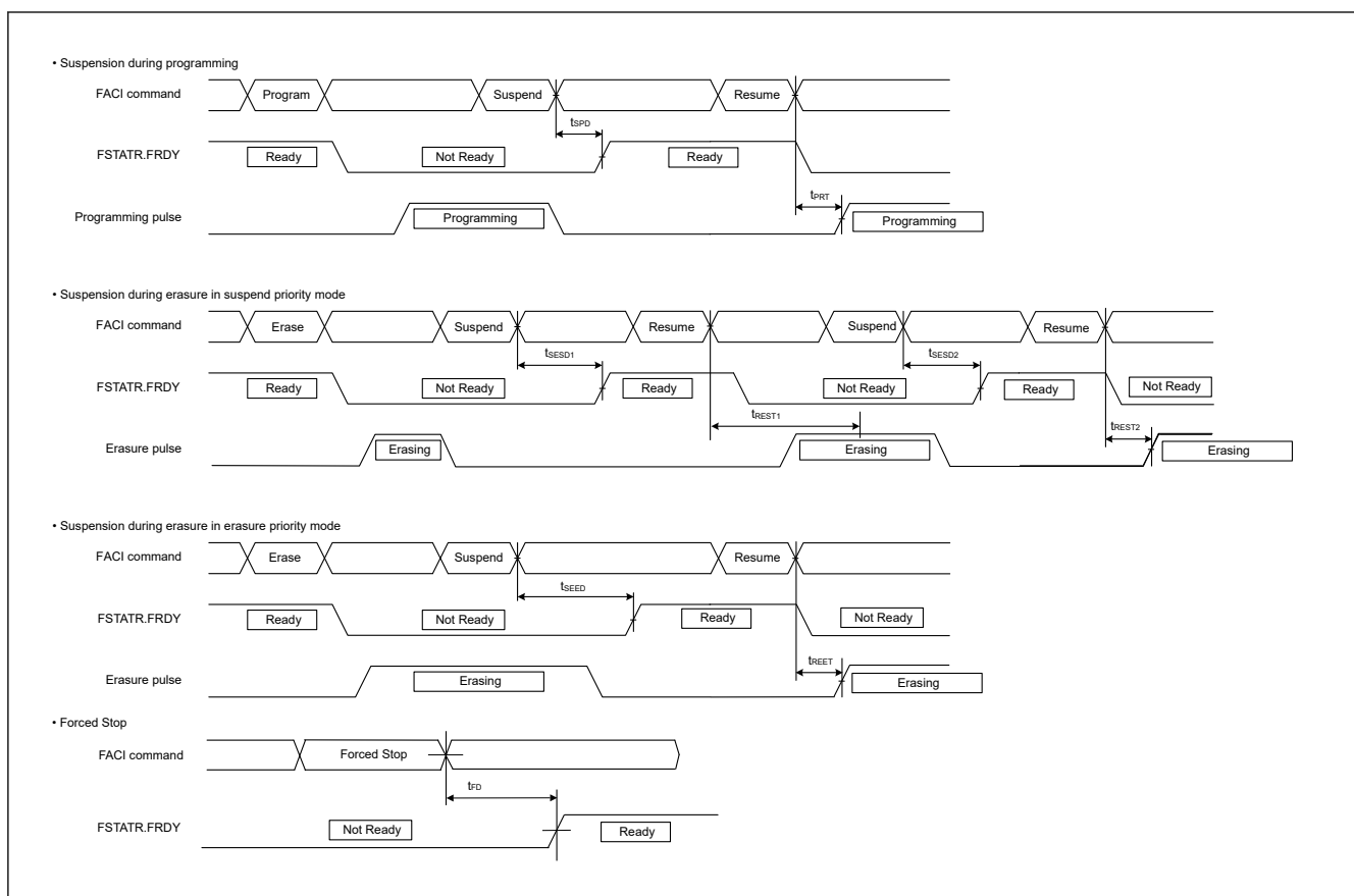
Figure 45.68 Suspension and forced stop timing for flash memory programming and erasure
