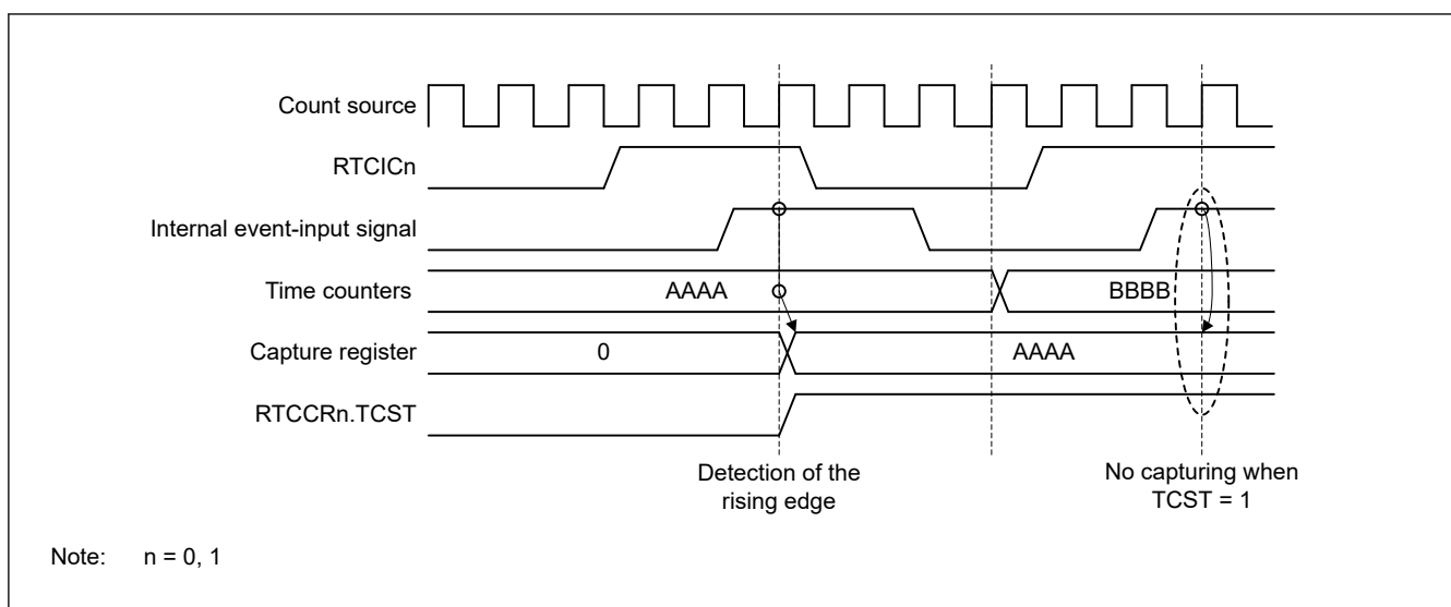
Figure 22.9 Timing of a time capture operation with the noise filter off
