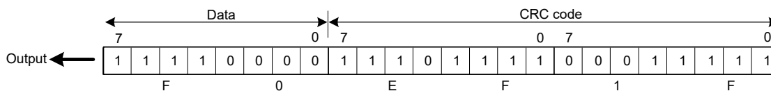
Figure 34.3 MSB-first data transmission
