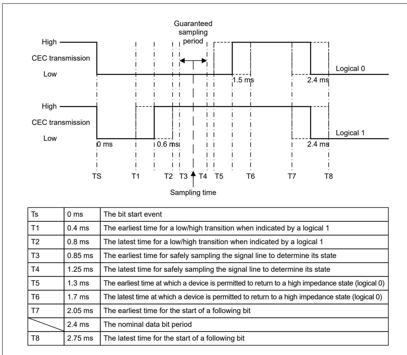
Figure 32.7 Example of data bit format
