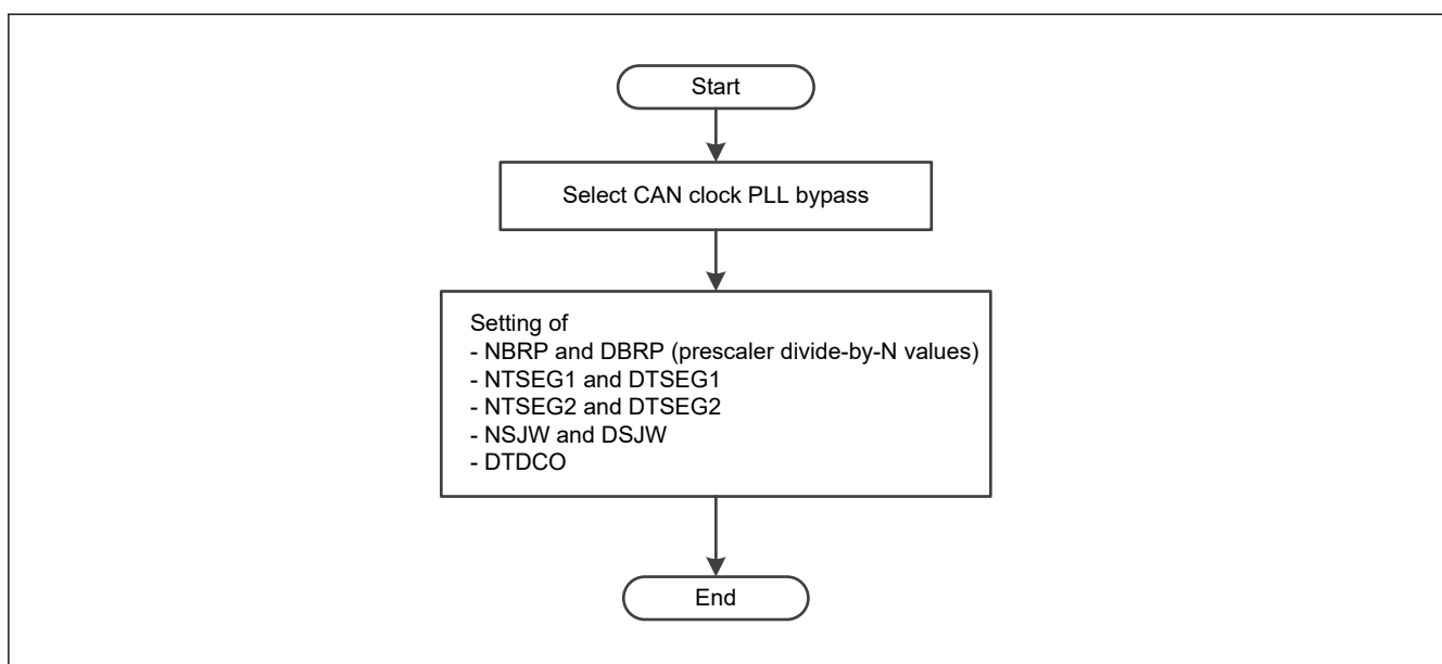
Figure 28.17 Procedure for setting the CAN bit timing and baud rate
