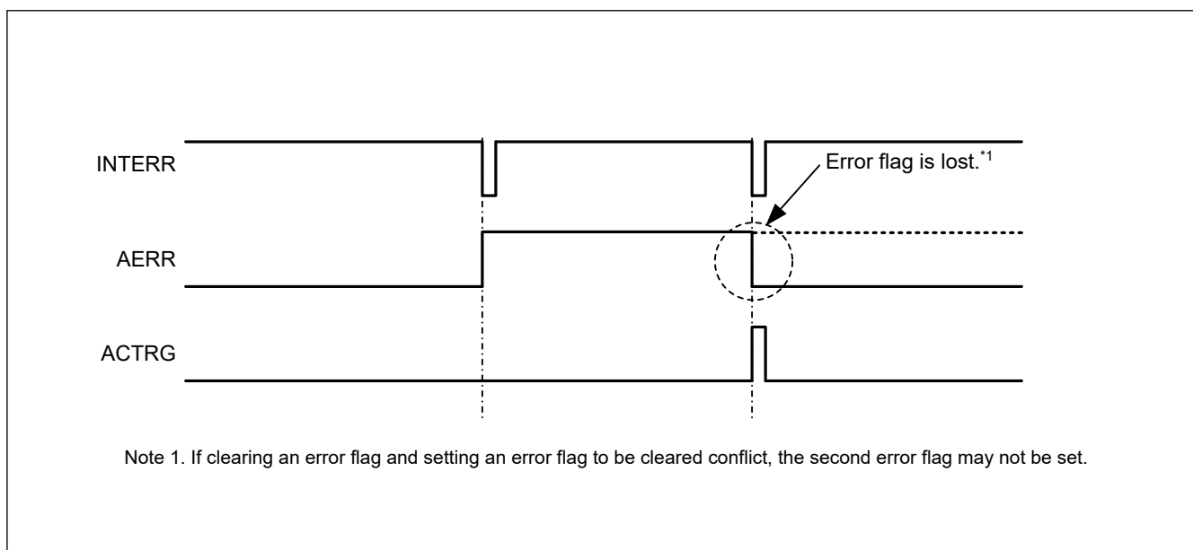
Figure 32.45 When two identical errors occurred and conflicted with the clear trigger
