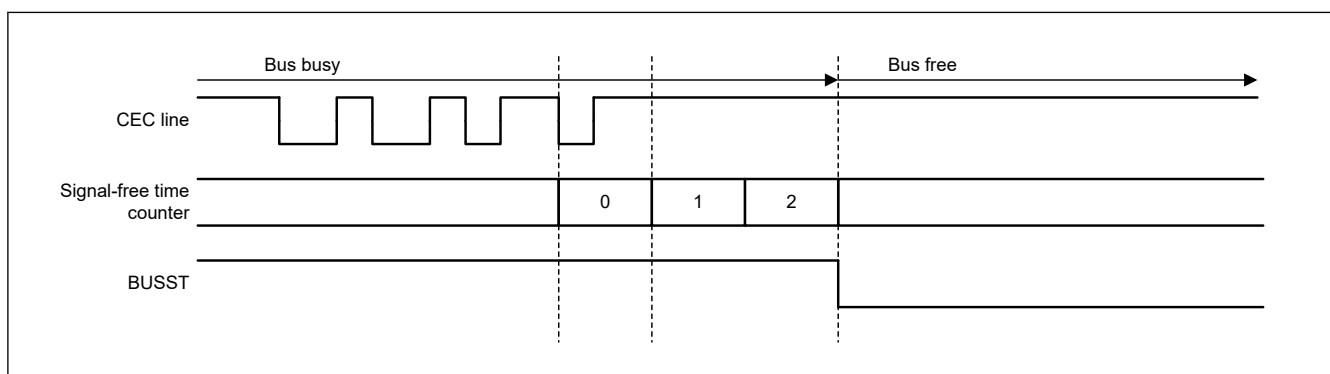
Figure 32.25 Timing when signal-free time set by CECCTL1.SFT[1:0] bits has elapsed after completion of communication
