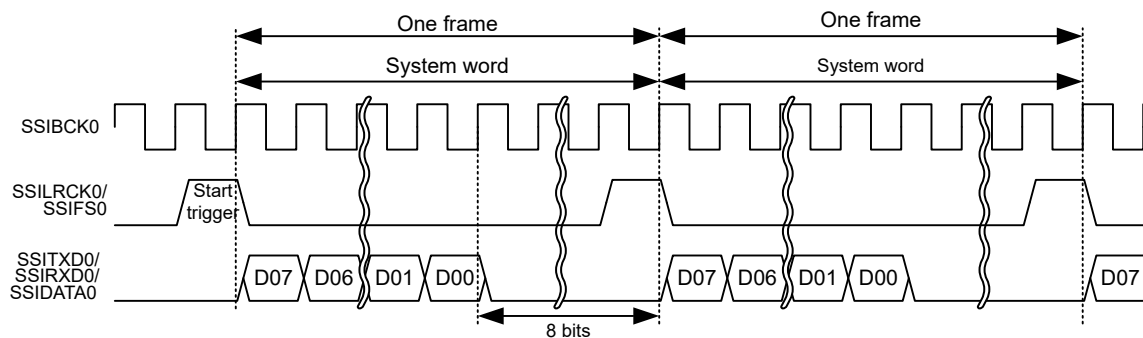
Figure 33.39 Short frame in monaural format (with padding: system word length > data word length)
