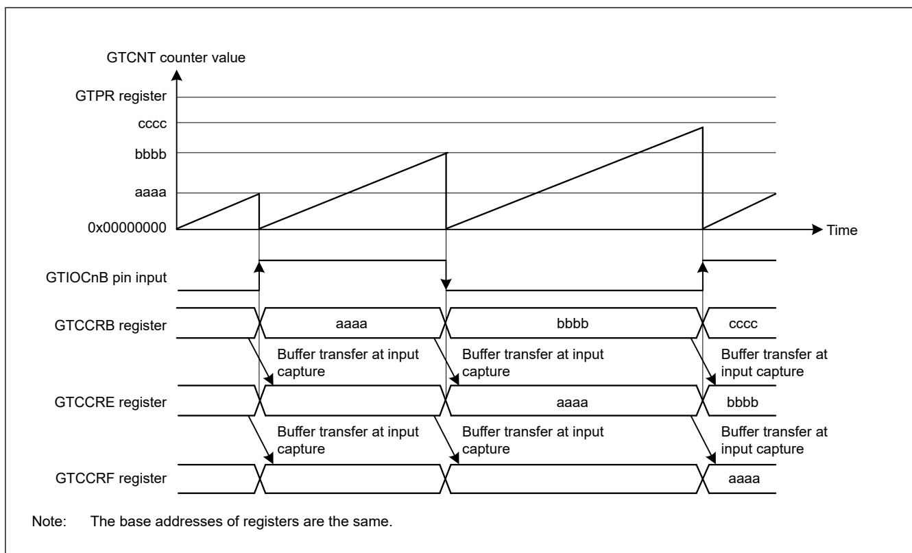
Figure 20.18 Example of GTCCRB double buffer operation with input capture at both edges of GTIOcNB input, saw waves in up-counting, and GTCNT counter cleared at both edges of GTIOcNB input
