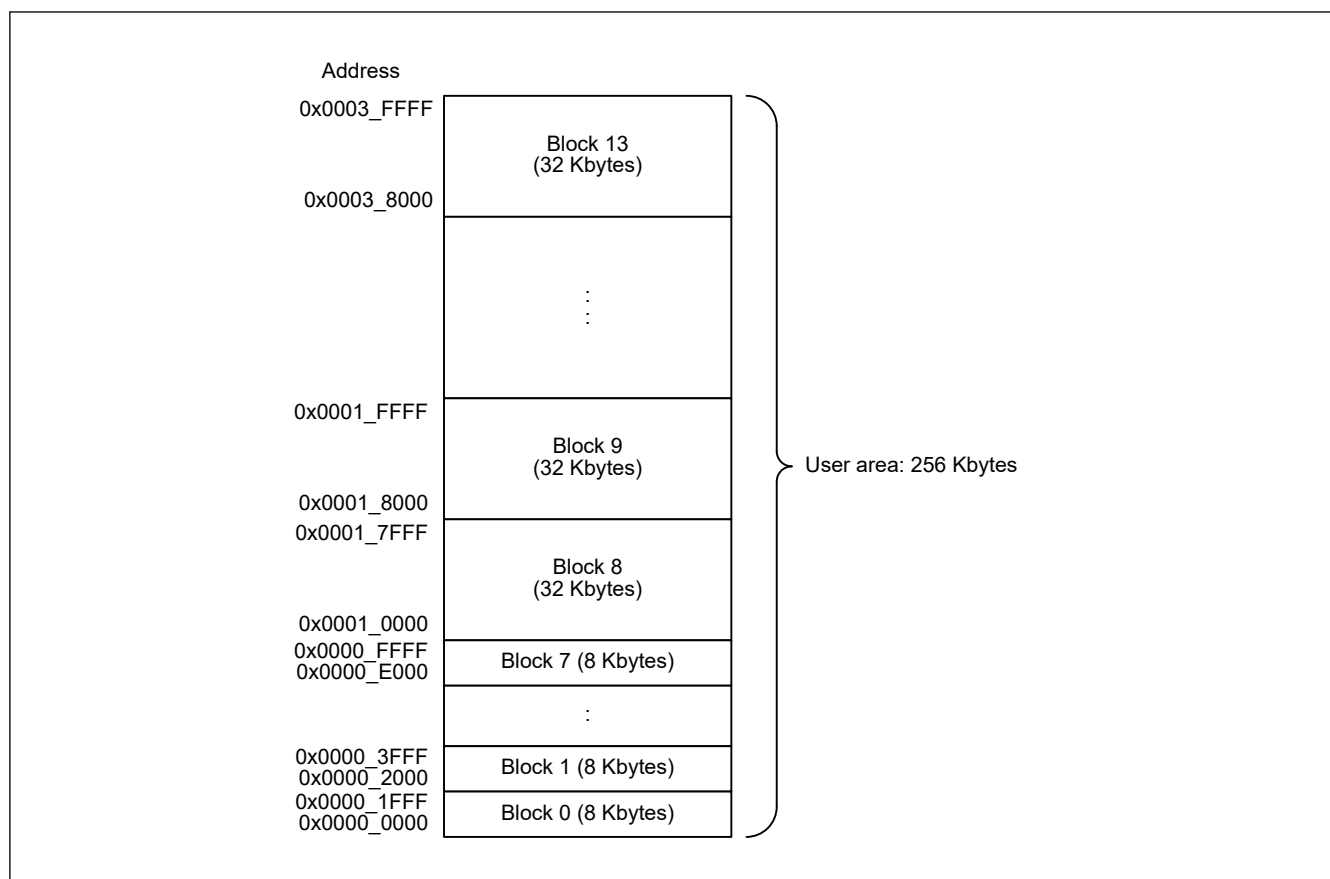
Figure 42.2 Map of the code flash memory
