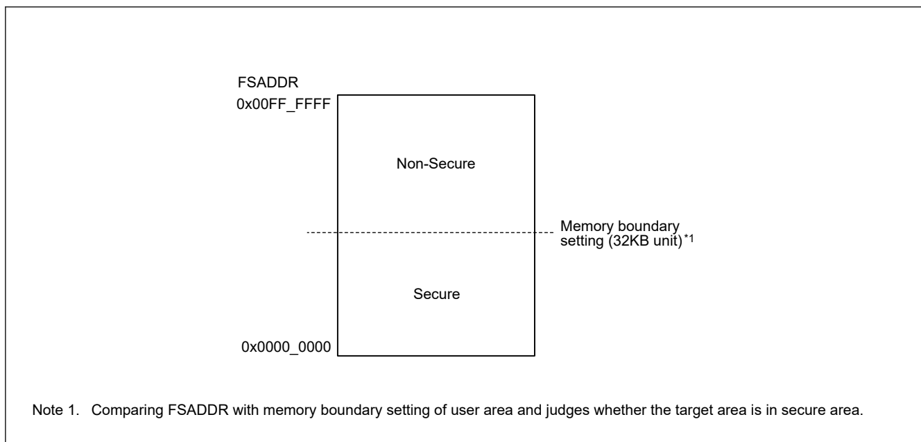
Figure 42.30 Secure/non-secure region in user area
