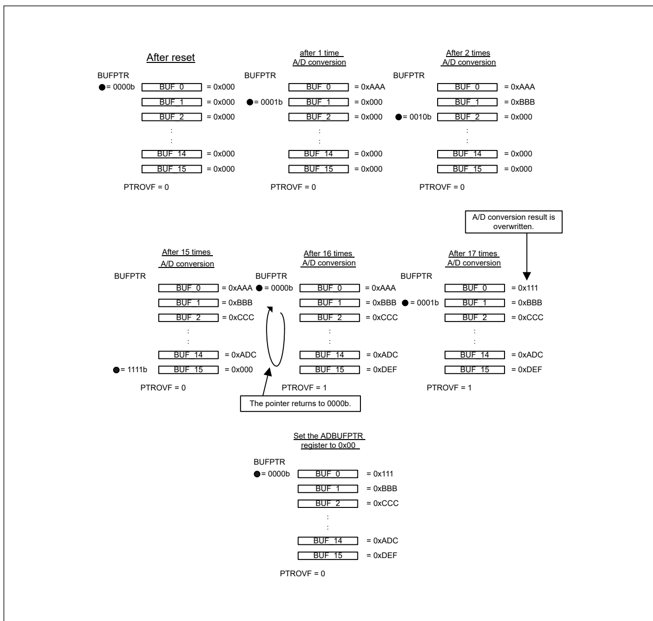
Figure 36.32 Data Buffers, Pointer, and Overflow Flag Operations
