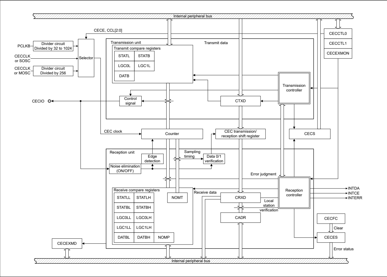
Figure 32.1 CEC block diagram
