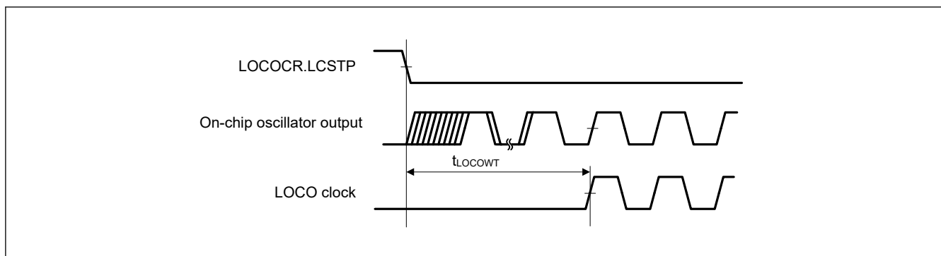
Figure 45.9 LOCO clock oscillation start timing
