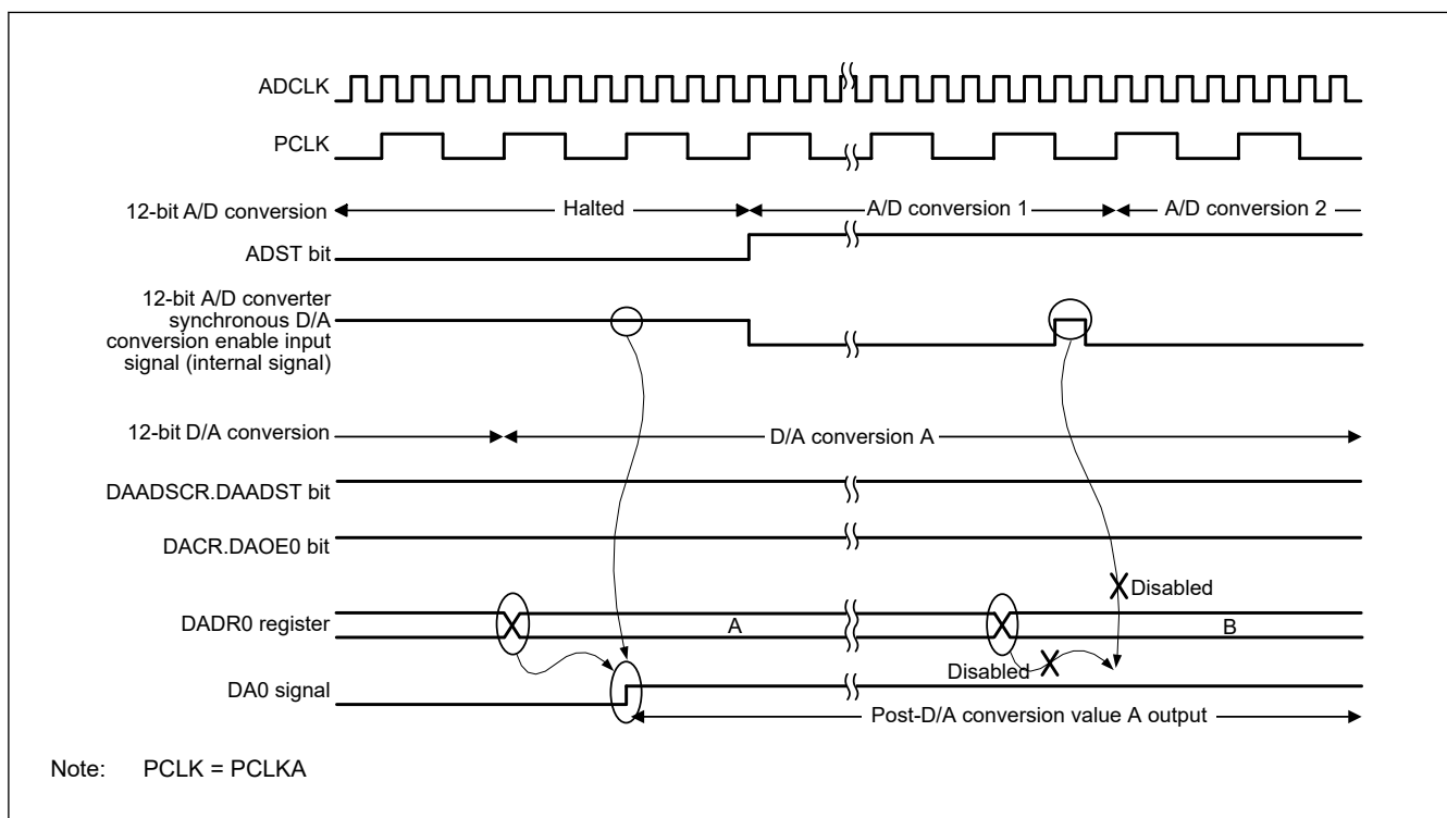
Figure 37.4 Example when the DAC12 cannot capture the synchronous D/A conversion enable input signal from the ADC12
