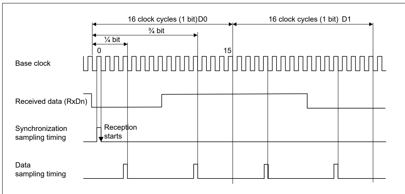
Figure 26.56 Data Reception Sampling Timing in Manchester Mode
