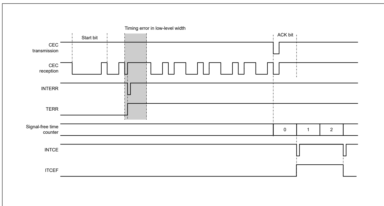
Figure 32.42 Timing error when bit width is not short during follower operation
