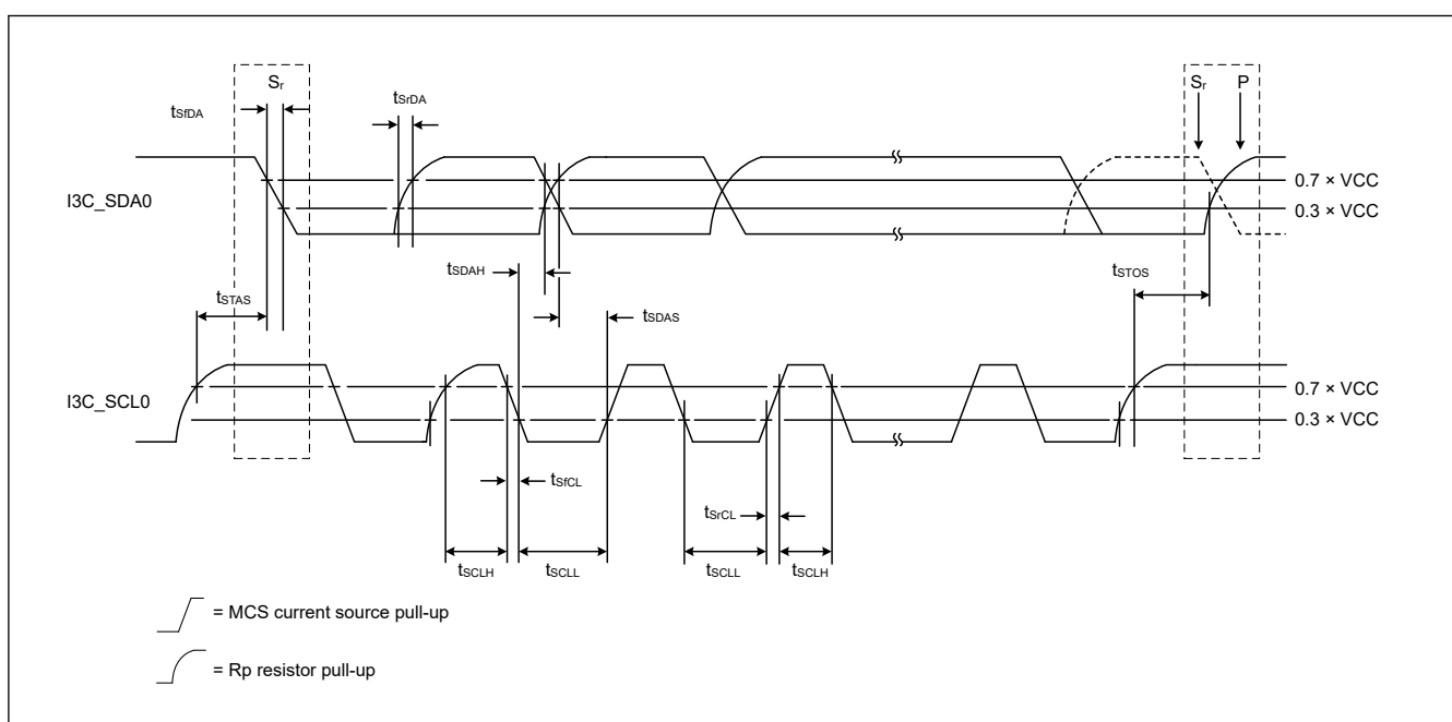
Figure 45.44 I 2 C bus interface input/output timing (Hs-mode)
