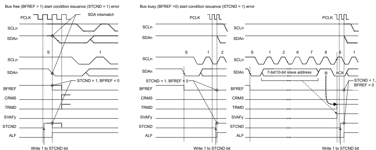
Figure 27.67 Arbitration-lost detection when a START condition is issued (MALE = 1)
