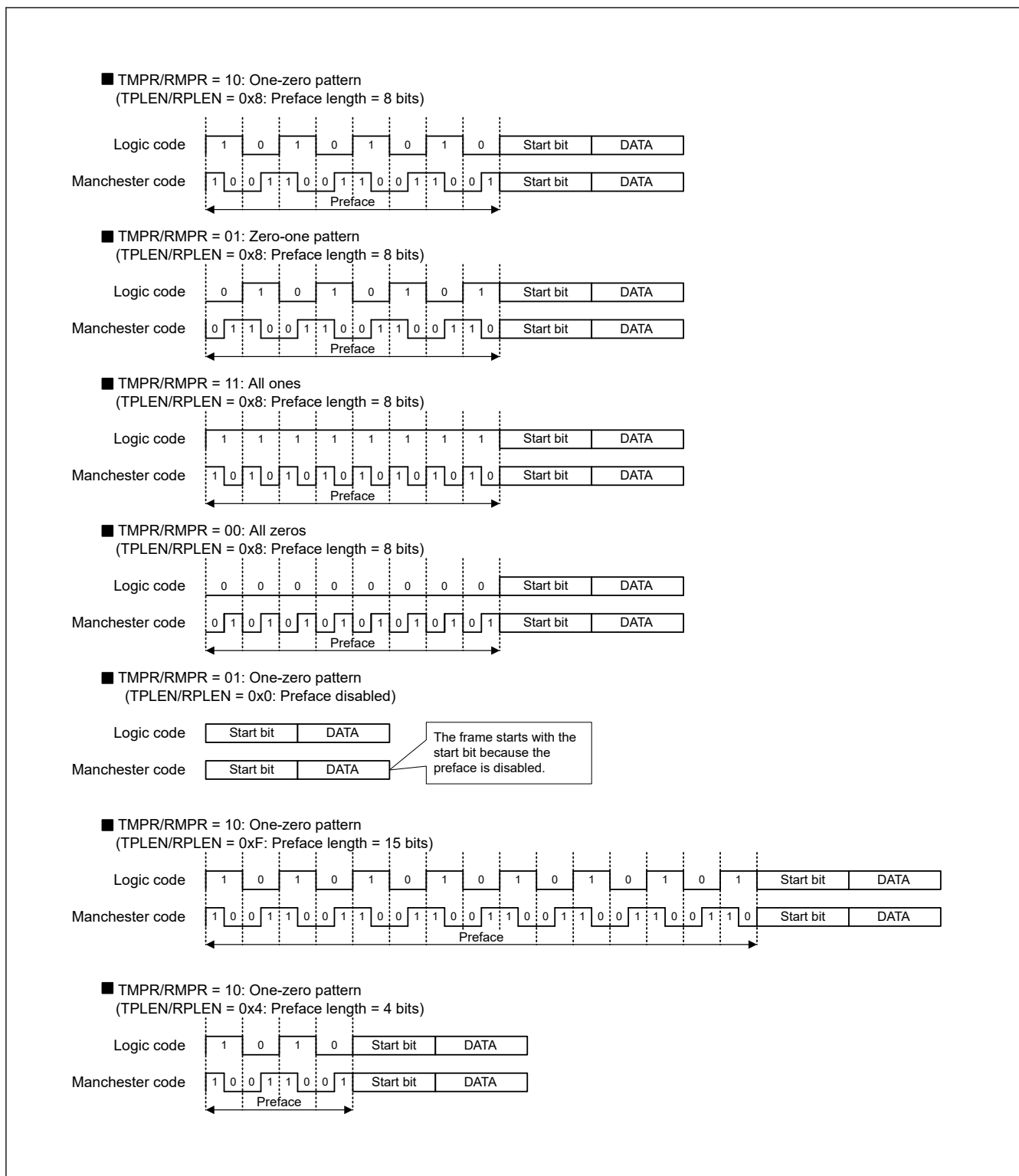
Figure 26.48 Preface Pattern Setting Example
