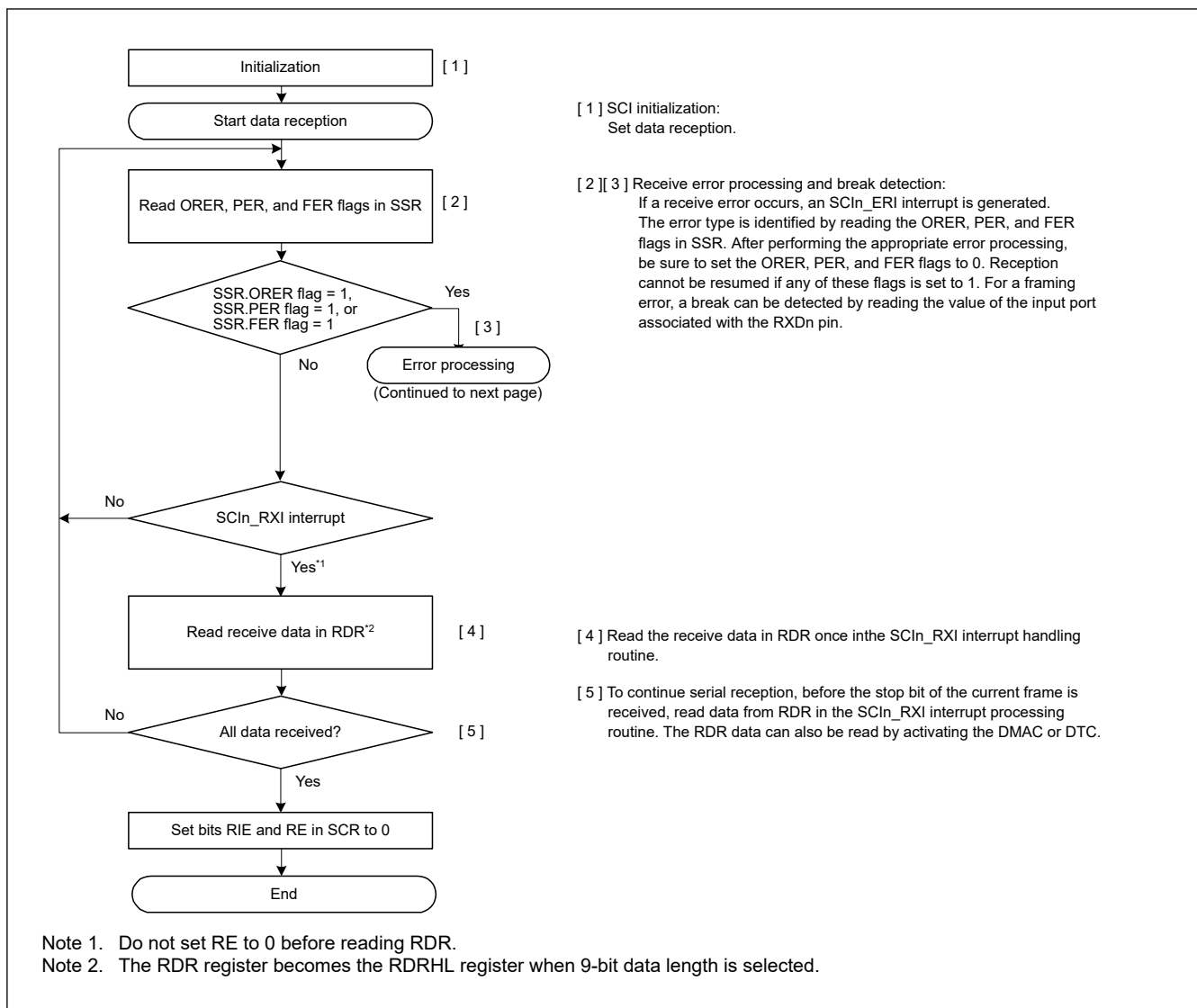
Figure 26.17 Example flow of serial reception in asynchronous mode with non-FIFO selected and Address Matching Disabled (1)
