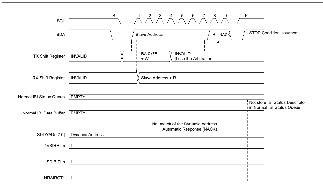
Figure 27.79 Slave interrupt request : NACK (not match the SDDYAD[7:0] of DAT) and NRSIRCTL = 0
