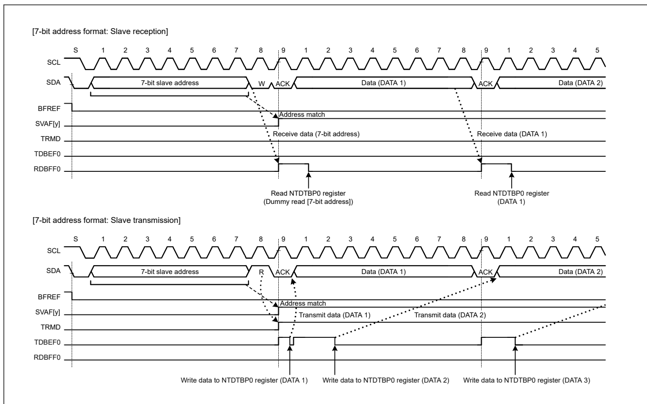
Figure 27.59 SVAF[y] flag set timing with 7-bit address format selected
