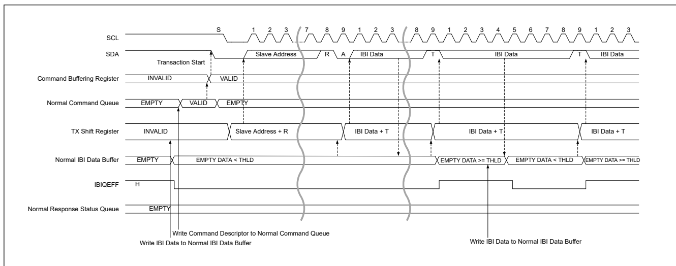
Figure 27.43 I3C slave IBI transfer timing (1/2)
