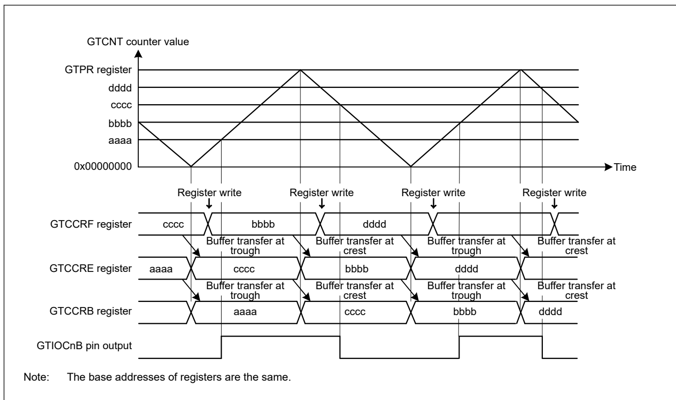
Figure 20.16 Example of GTCCRB double buffer operation with output compare, triangle waves, buffer operation at both troughs and crests, output toggled at GTCCRB compare match, and output retained at cycle end
