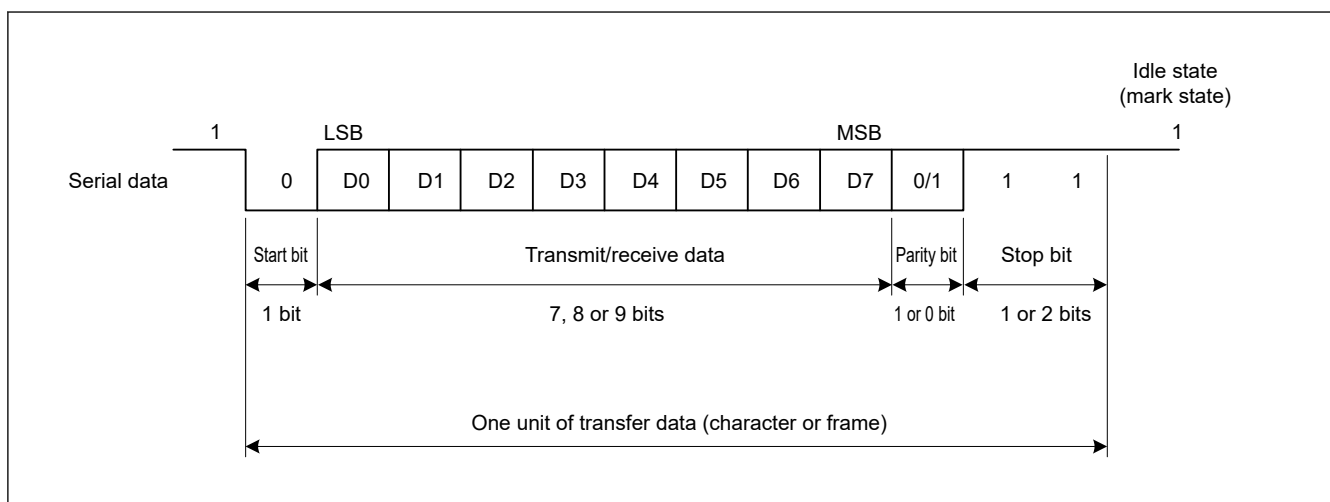
Figure 26.3 Data format in asynchronous serial communications with 8-bit data, parity bit, and 2 stop bits
