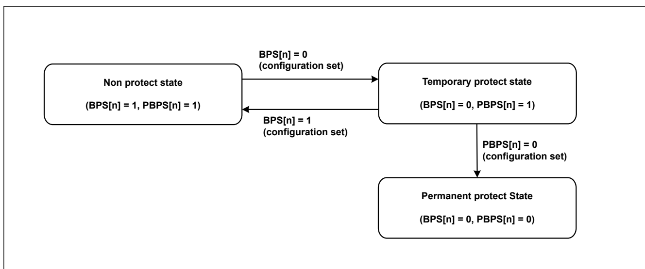
Figure 42.29 Status transition of flash sequencer by BPS[n] and PBPS[n]
