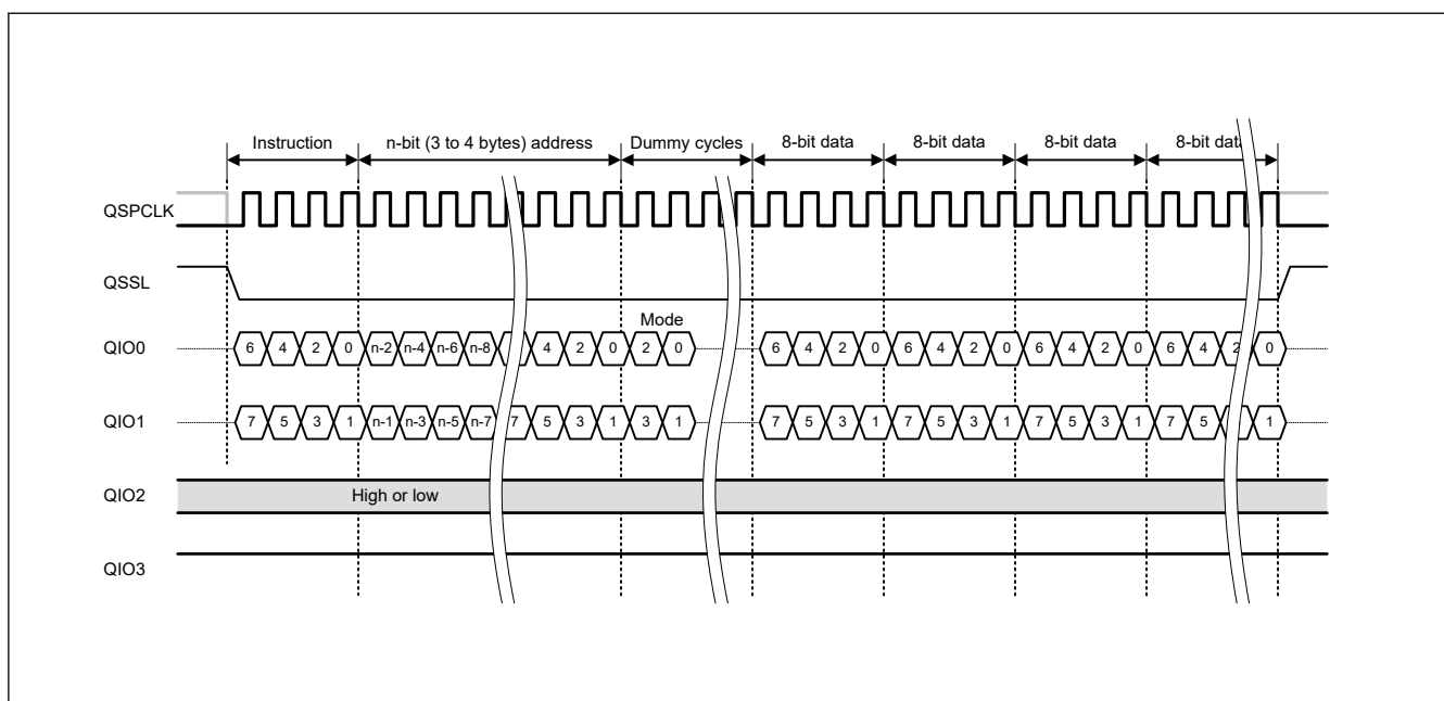
Figure 31.6 Dual SPI protocol example for Fast Read Dual I/O
