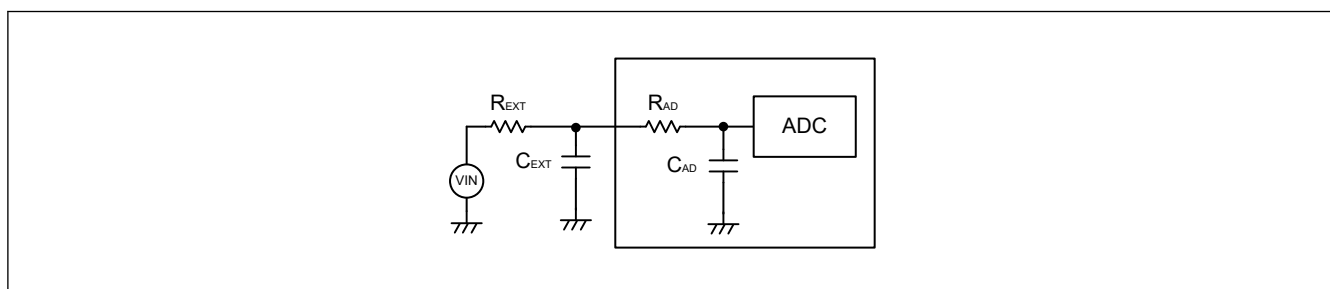
Figure 36.35 Sample and hold circuit simplified diagram
