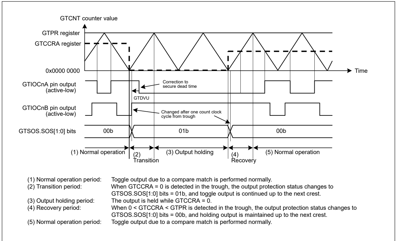
Figure 20.83 Example of output protection function operation when GTCCRA is set to 0 during buffer transfer at troughs (restored to 0 < \text{GTCCRA} < \text{GTPR} during buffer transfer at troughs, active-low) ( n = 0 to 5)
