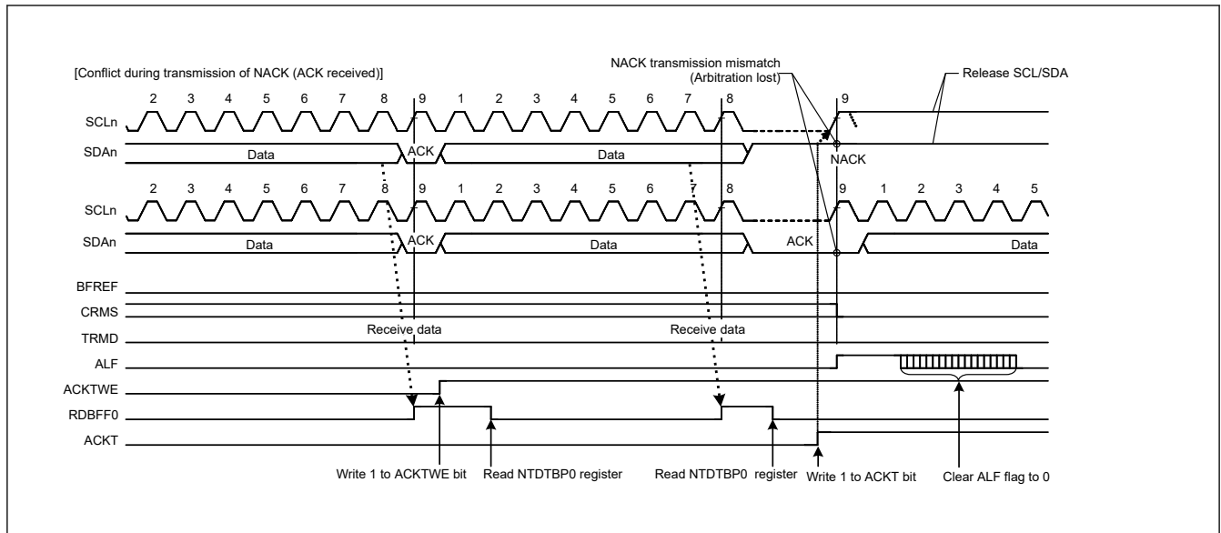
Figure 27.68 Example of arbitration-lost detection during transmission of NACK (NALE = 1)
