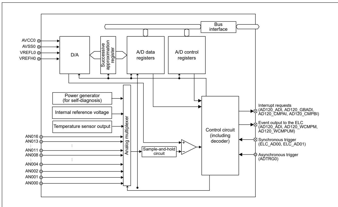
Figure 36.1 ADC12 block diagram
