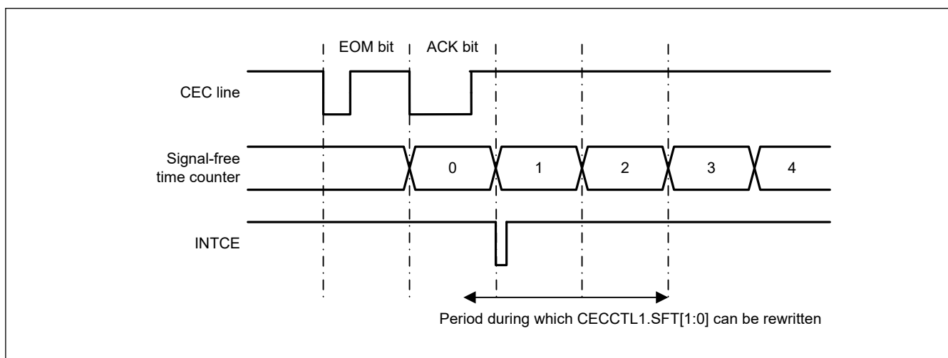
Figure 32.47 Period during which CECCTL1.SFT[1:0] can be rewritten while counting signal-free time
