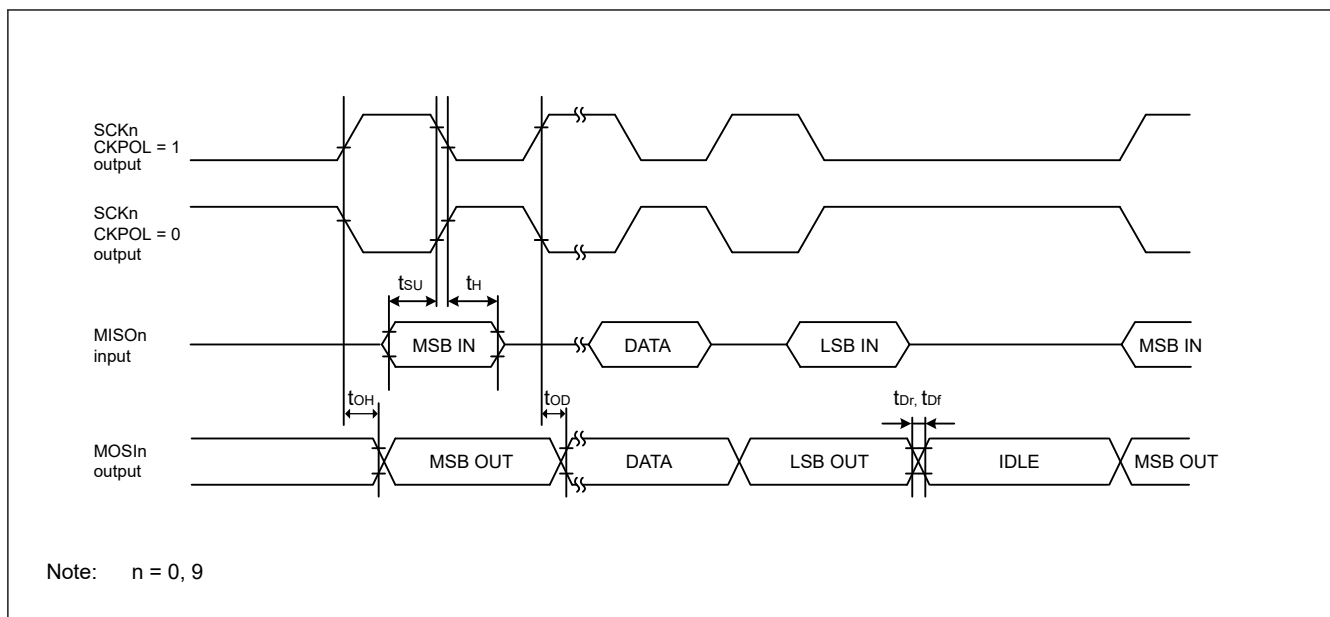
Figure 45.30 SCI simple SPI mode timing for master when CKPH = 0
