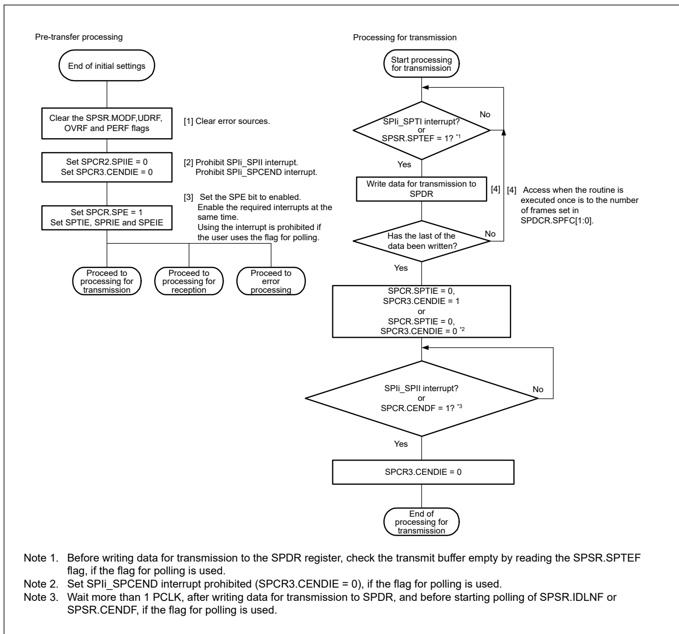
Figure 30.53 Transmission flow in slave mode
