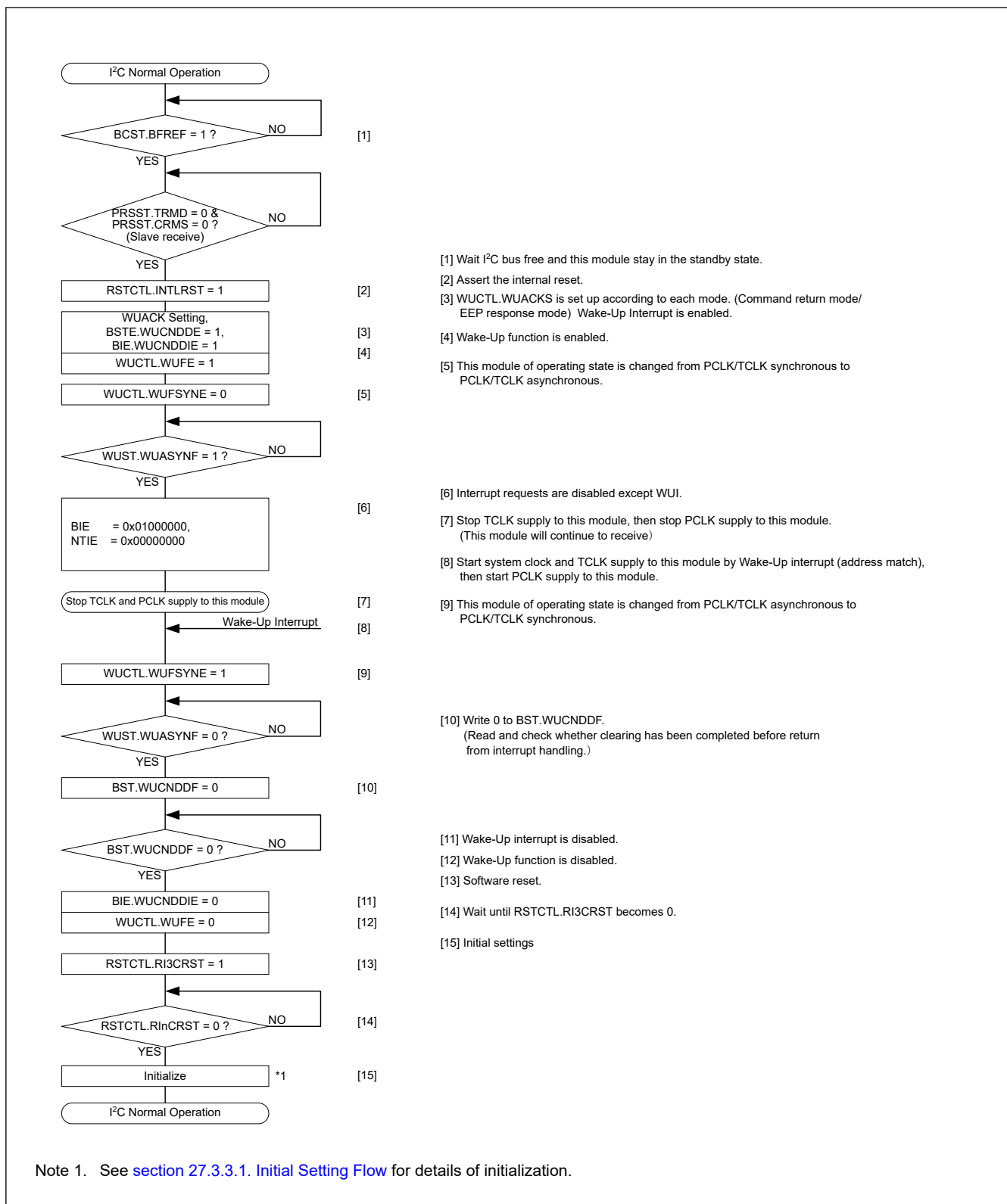
Figure 27.104 Use case of command recover mode and EEP response mode (wake-up recovery by a wake-up interrupt triggered by the match of the slave address)
