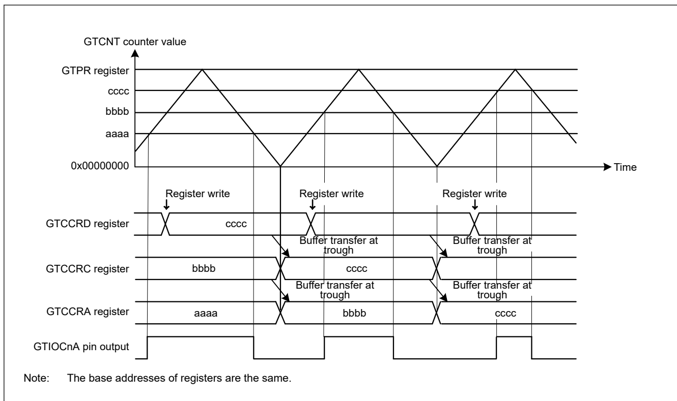
Figure 20.15 Example of GTCCRA double buffer operation with output compare, triangle waves, buffer operation at trough, output toggled at GTCCRA compare match, and output retained at cycle end
