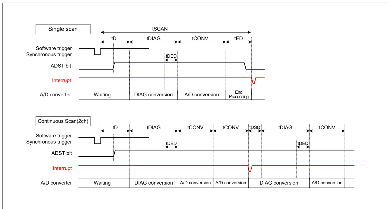
Figure 36.26 Scan conversion timing when activated by software or a synchronous trigger input (ELC)
