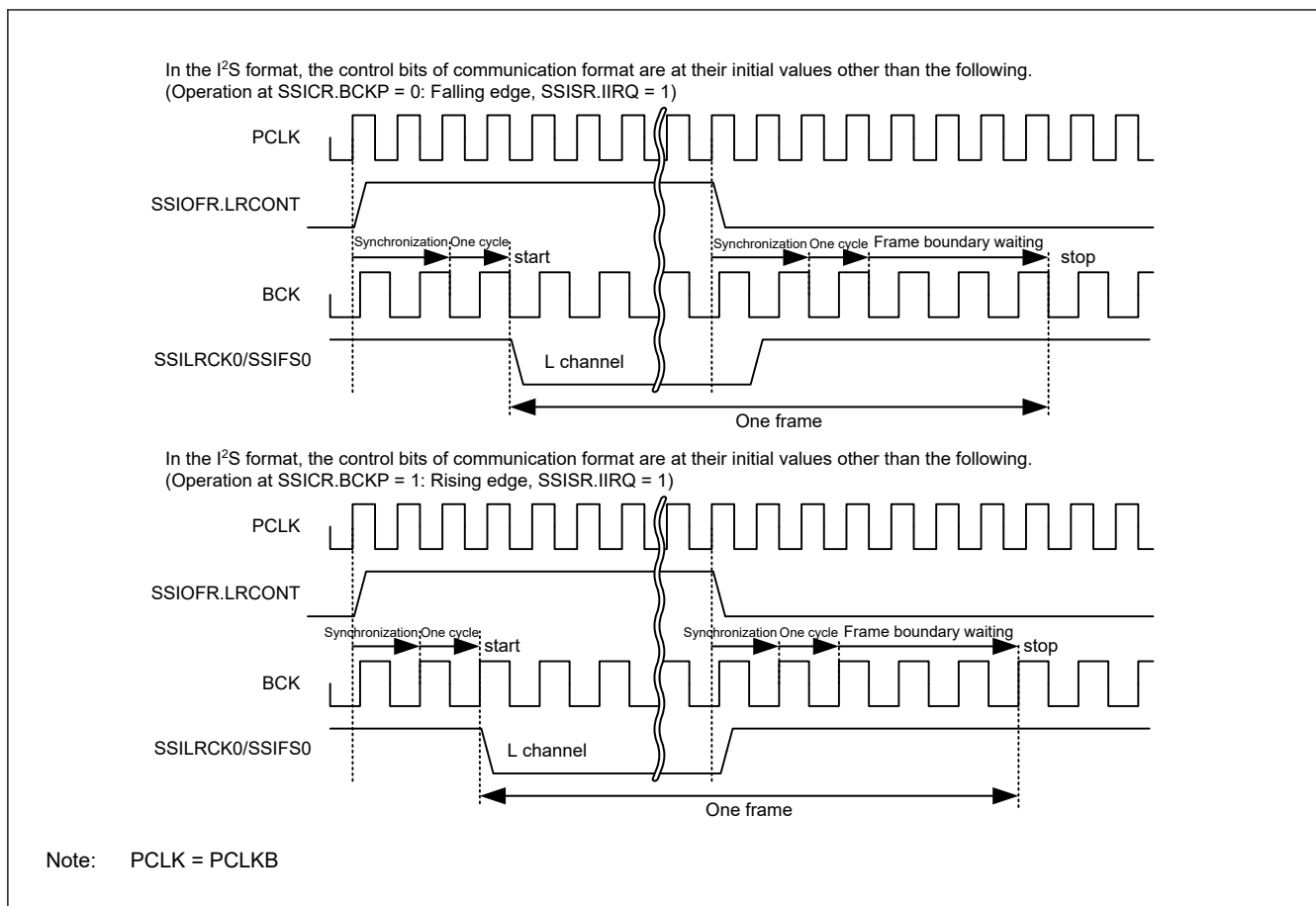
Figure 33.44 Example of disabling LR clock/frame synchronization continuation by SSIOFR.LRCONT
