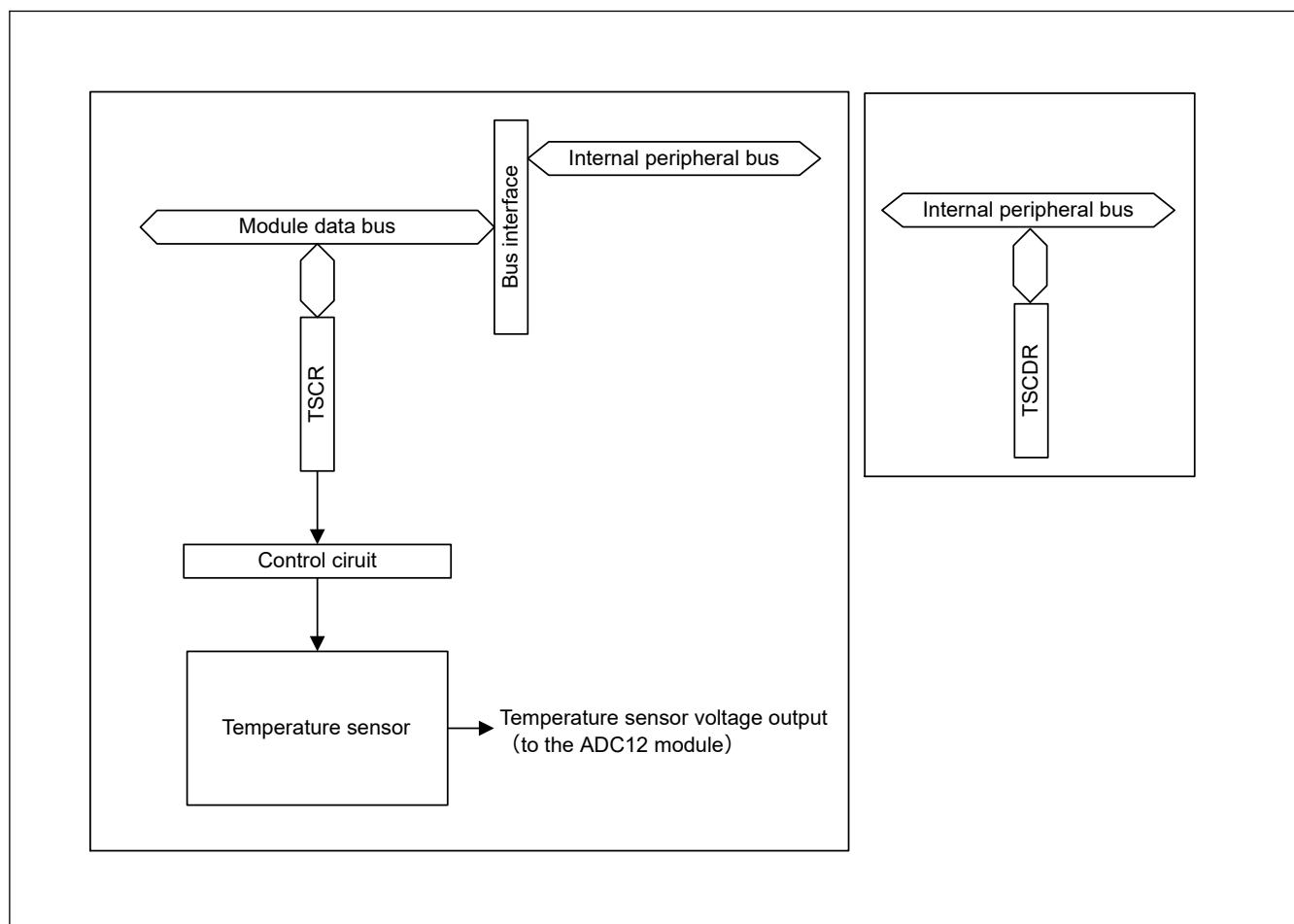
Figure 38.1 TSN block diagram
