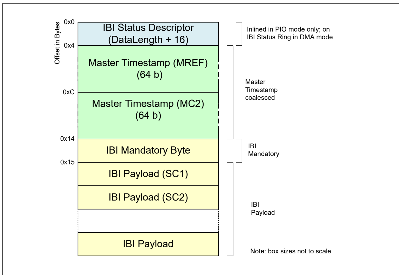
Figure 27.87 Master timestamp counters for IBI event
