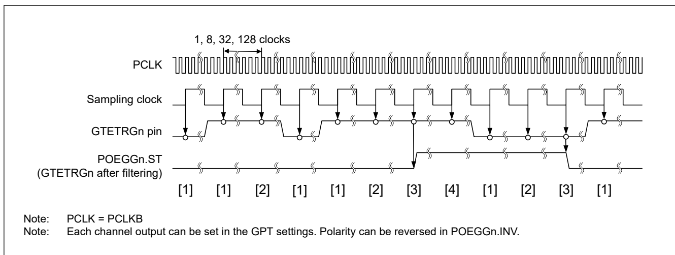
Figure 19.4 Output timing of external trigger to the GPT
