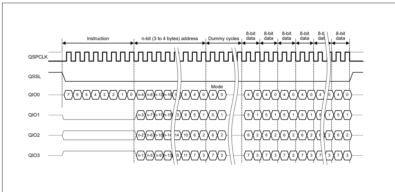
Figure 31.5 Extended SPI Protocol example for Fast Read Quad I/O
