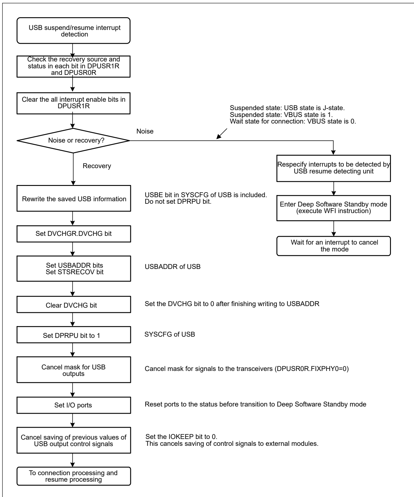
Figure 25.6 USBFS setup flow for canceling Deep Software Standby mode
