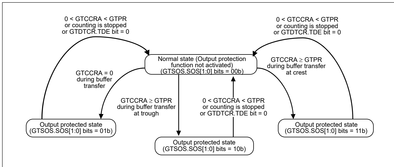
Figure 20.82 Output protection function
