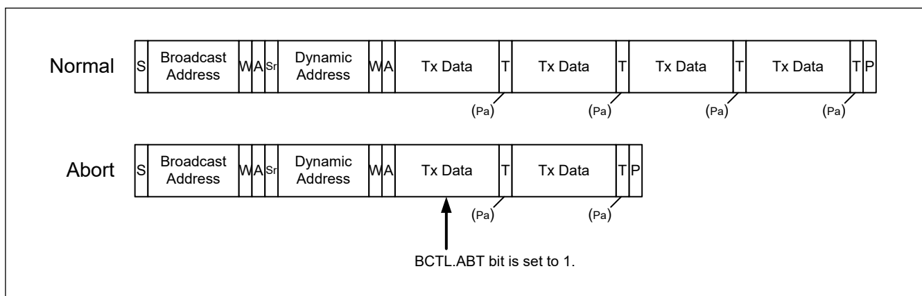
Figure 27.93 Abort operation of SDR write transfer
