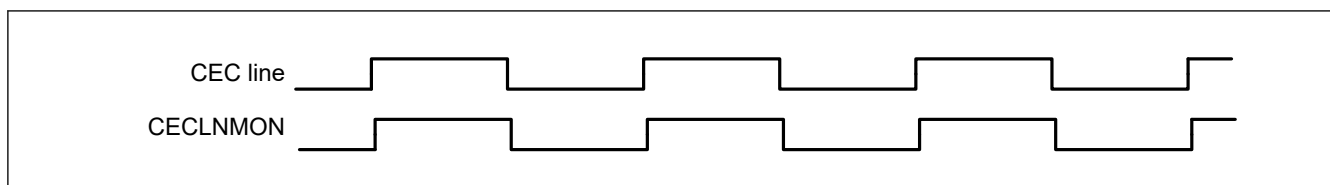
Figure 32.31 Timing of CECLNMON bit
