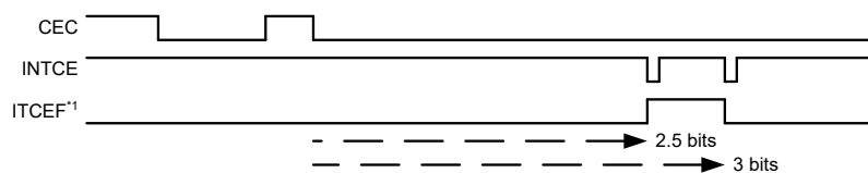
Figure 32.29 Using ITCEF to check INTCE generation source when CECCTL1.CESEL[1:0] = 00b
