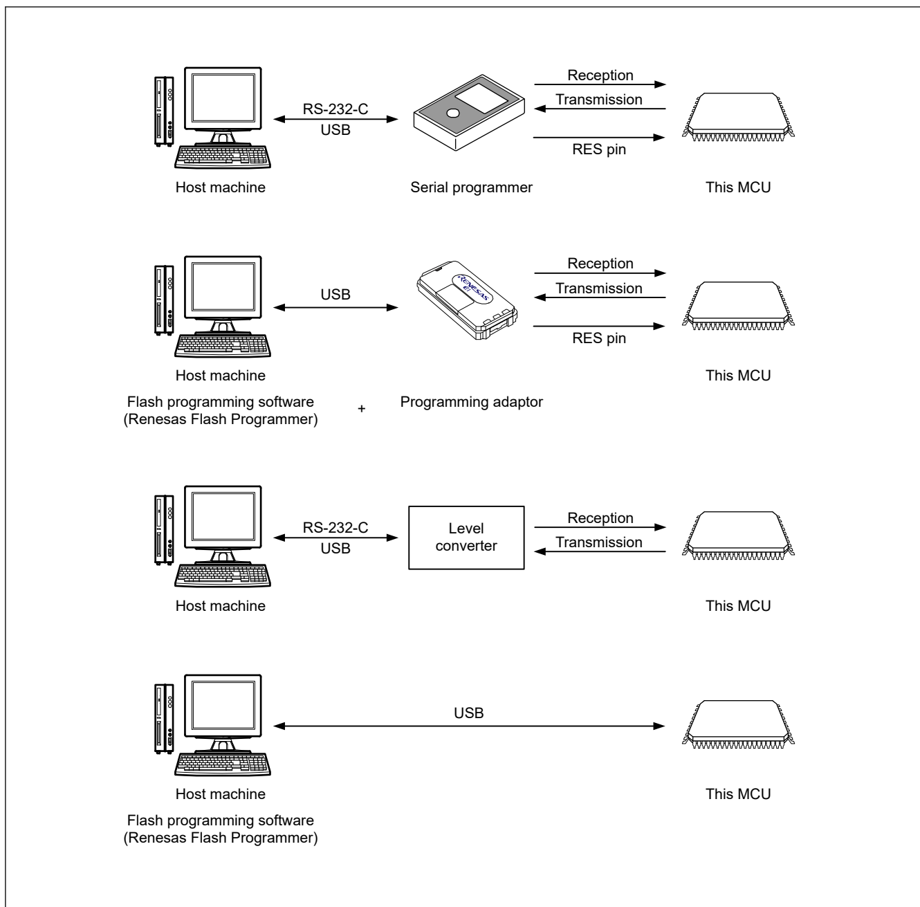
Figure 42.40 Environments for rewriting the flash memory
