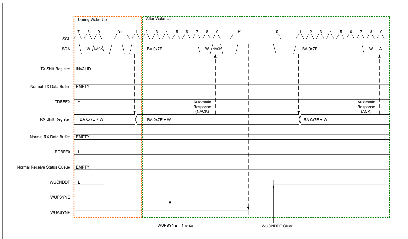
Figure 27.109 I3C slave wake-up operation (2/2)
