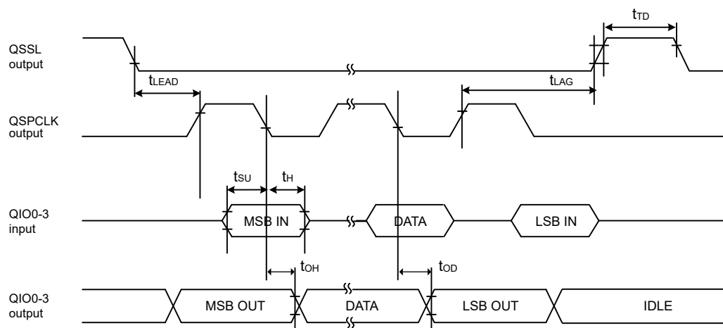
Figure 45.42 Transmit and receive timing
