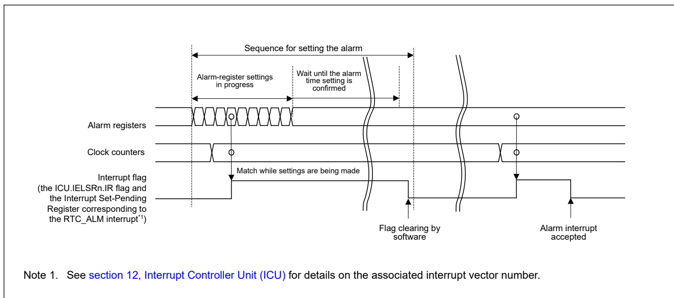
Figure 22.11 Timing for the alarm interrupt (RTC_ALM)
