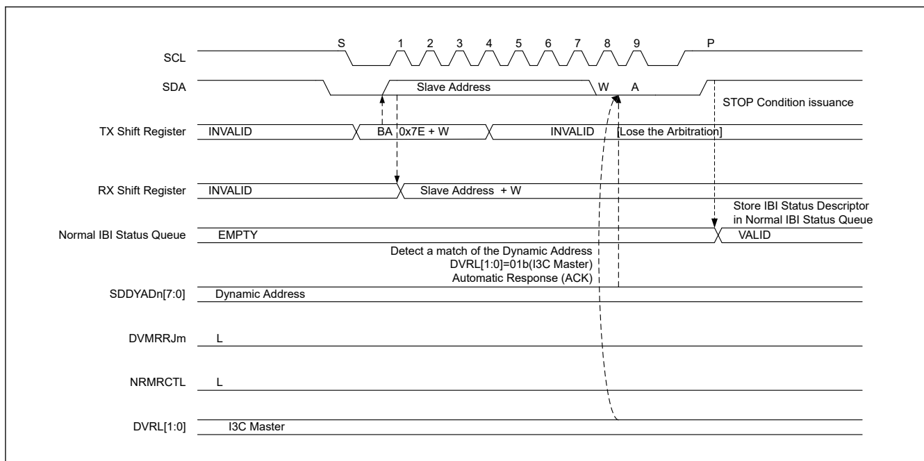
Figure 27.82 Mastership request : ACK
