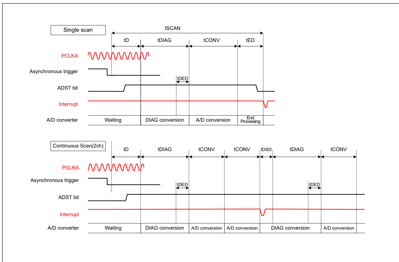
Figure 36.27 Scan conversion timing when activated by an asynchronous trigger input (ADTRG0)
