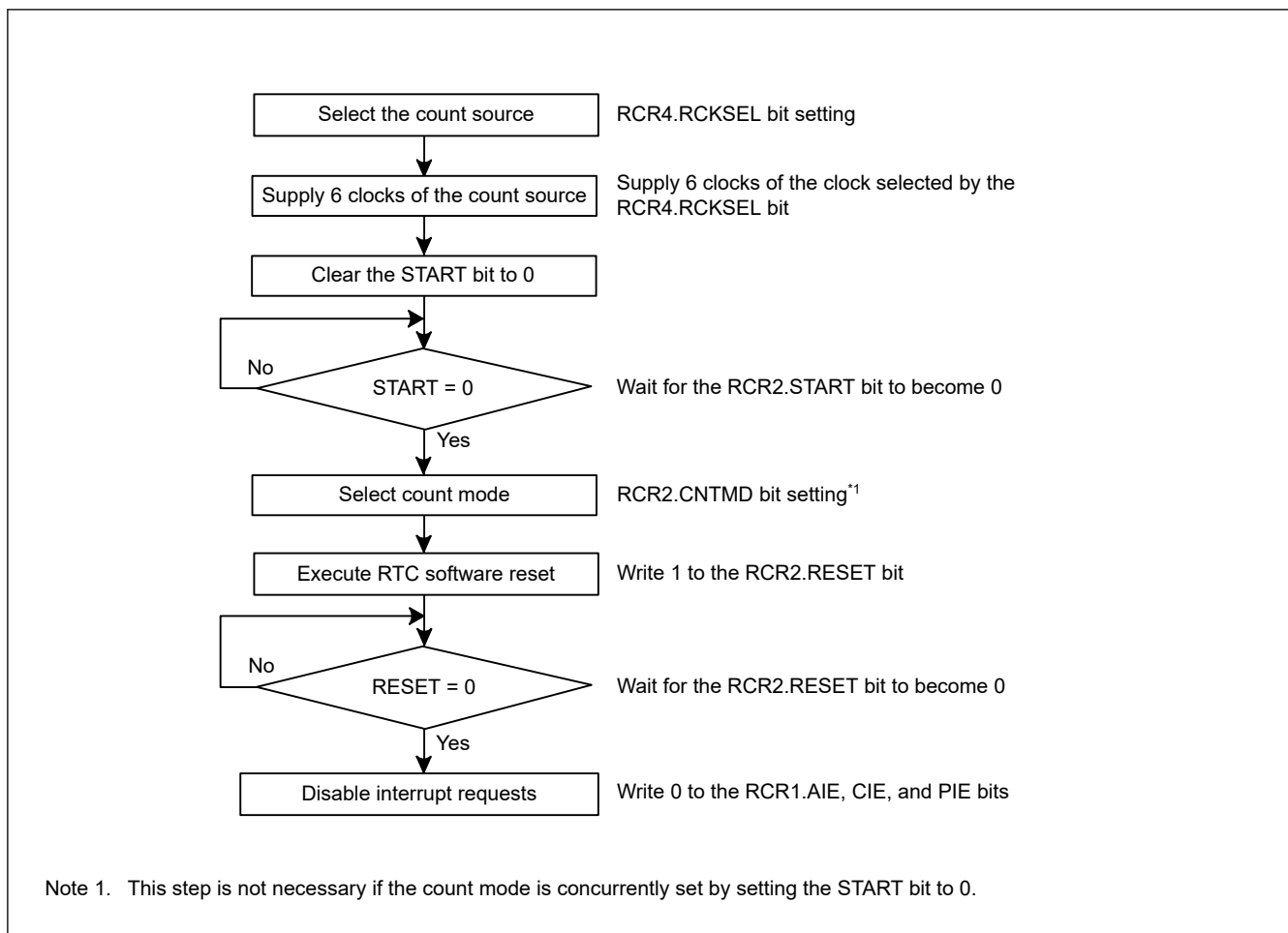
Figure 22.14 Initialization procedure
