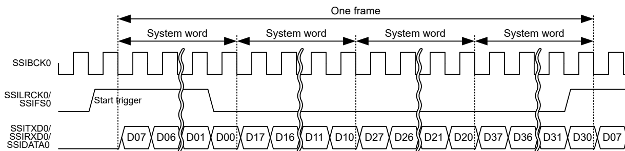
Figure 33.41 TDM format (without padding: system word length = data word length)
