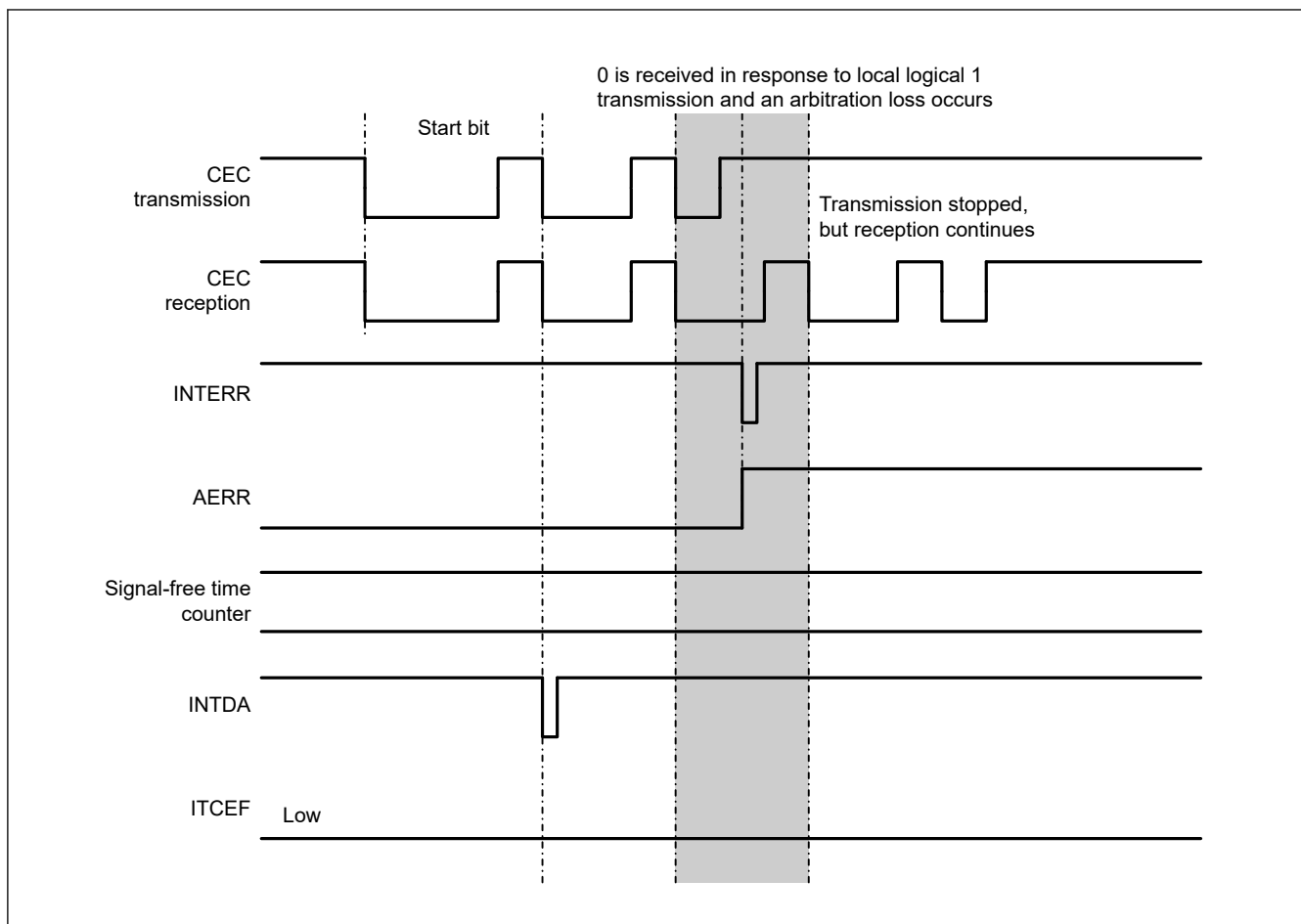
Figure 32.38 Arbitration timing
