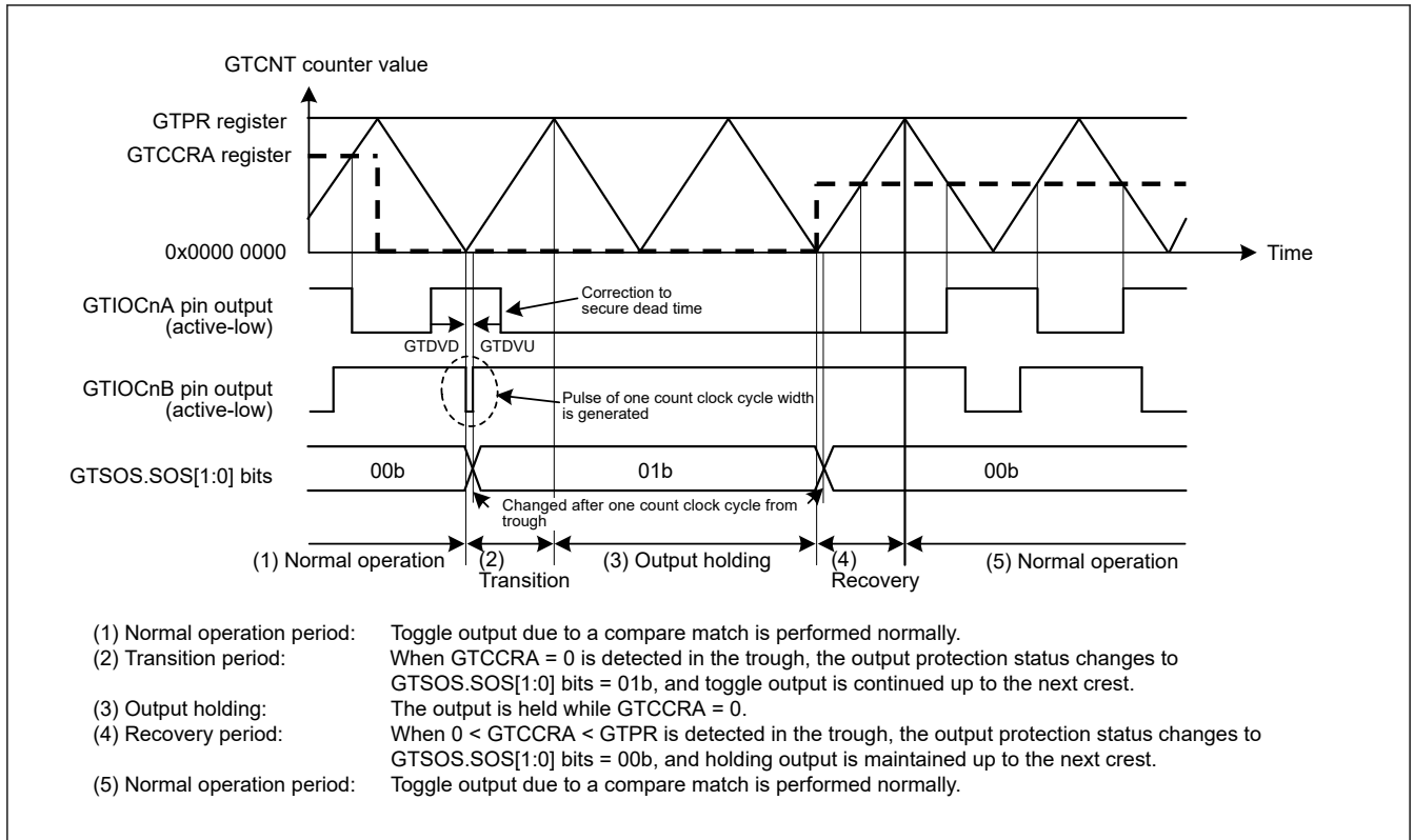
Figure 20.85 Example of output protection function operation when GTCCRA is set to 0 during buffer transfer at crests (restored to 0 < \text{GTCCRA} < \text{GTPR} during buffer transfer at troughs, active-low) ( n = 0 to 5)
