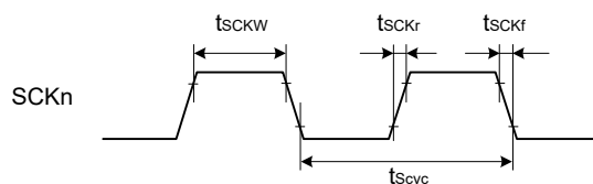
Figure 45.26 SCK clock input/output timing
