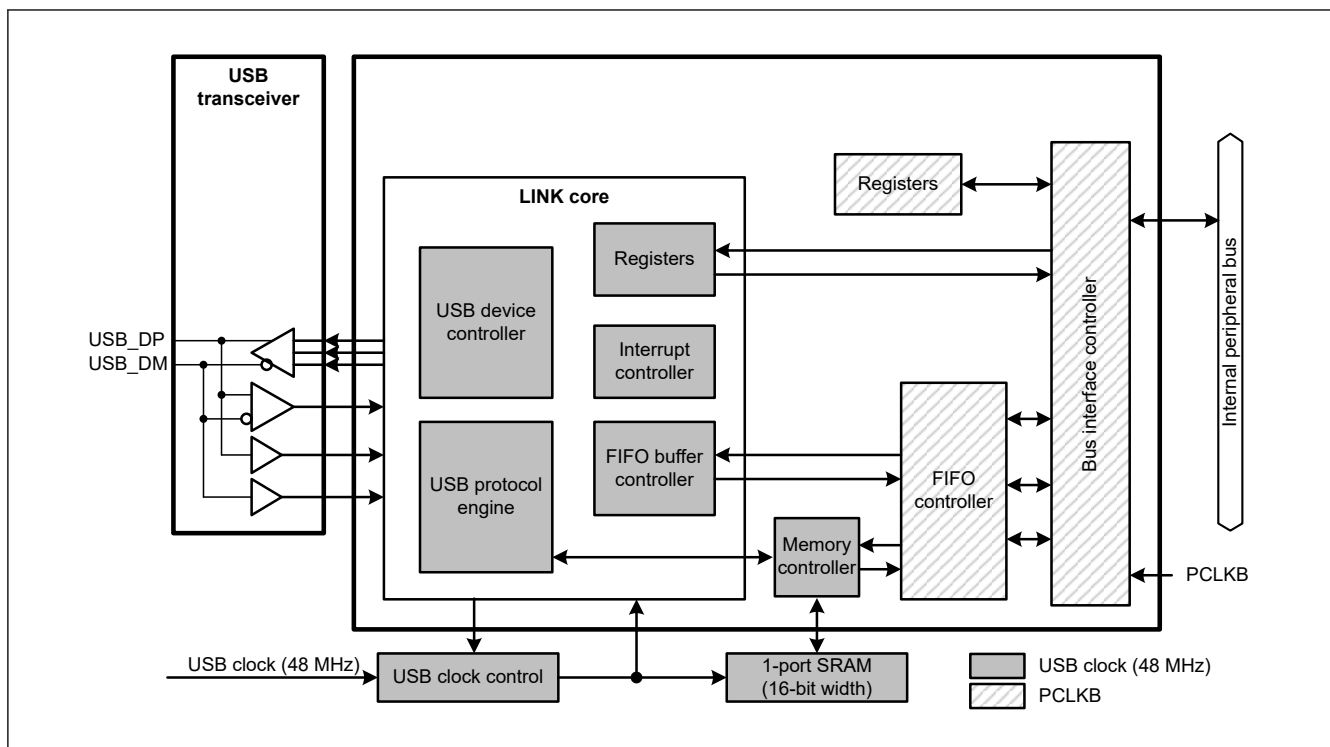
Figure 25.1 USBFS block diagram
