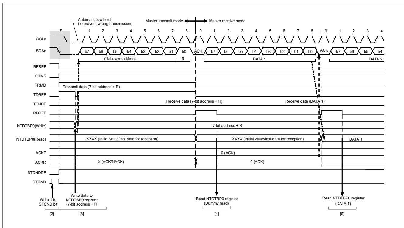
Figure 27.9 Master receive operation timing (1) (7-bit address format, when ACKTWE = 0 )
