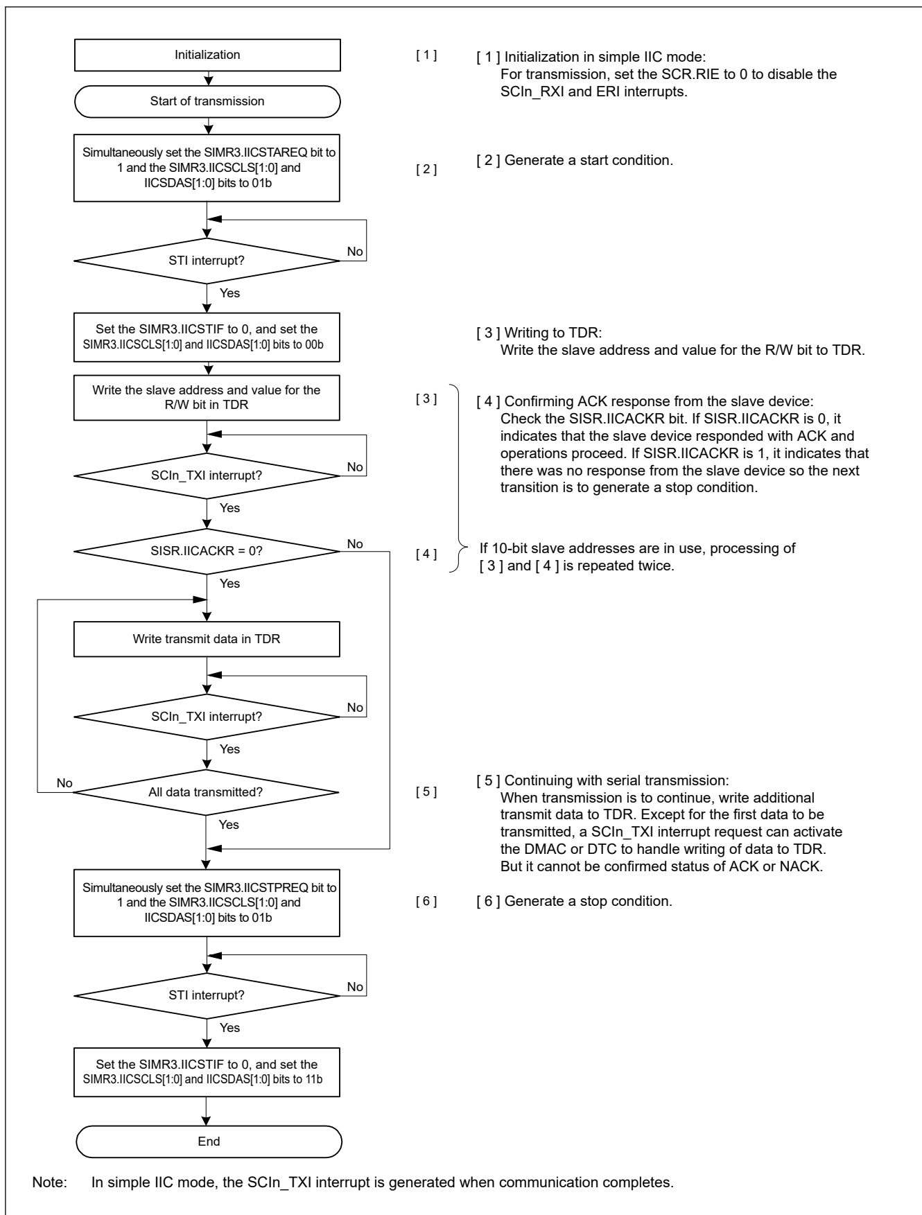
Figure 26.92 Example flow of master transmission in simple IIC mode with transmission interrupts and reception interrupts
