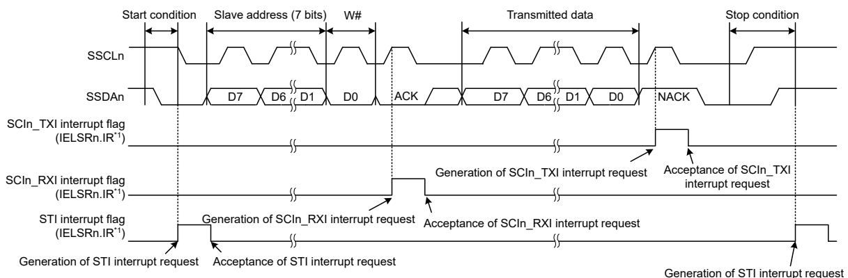
Figure 26.91 Example 2 of operations for master transmission in simple IIC mode with 7-bit slave addresses, ACK interrupts, and NACK interrupts
