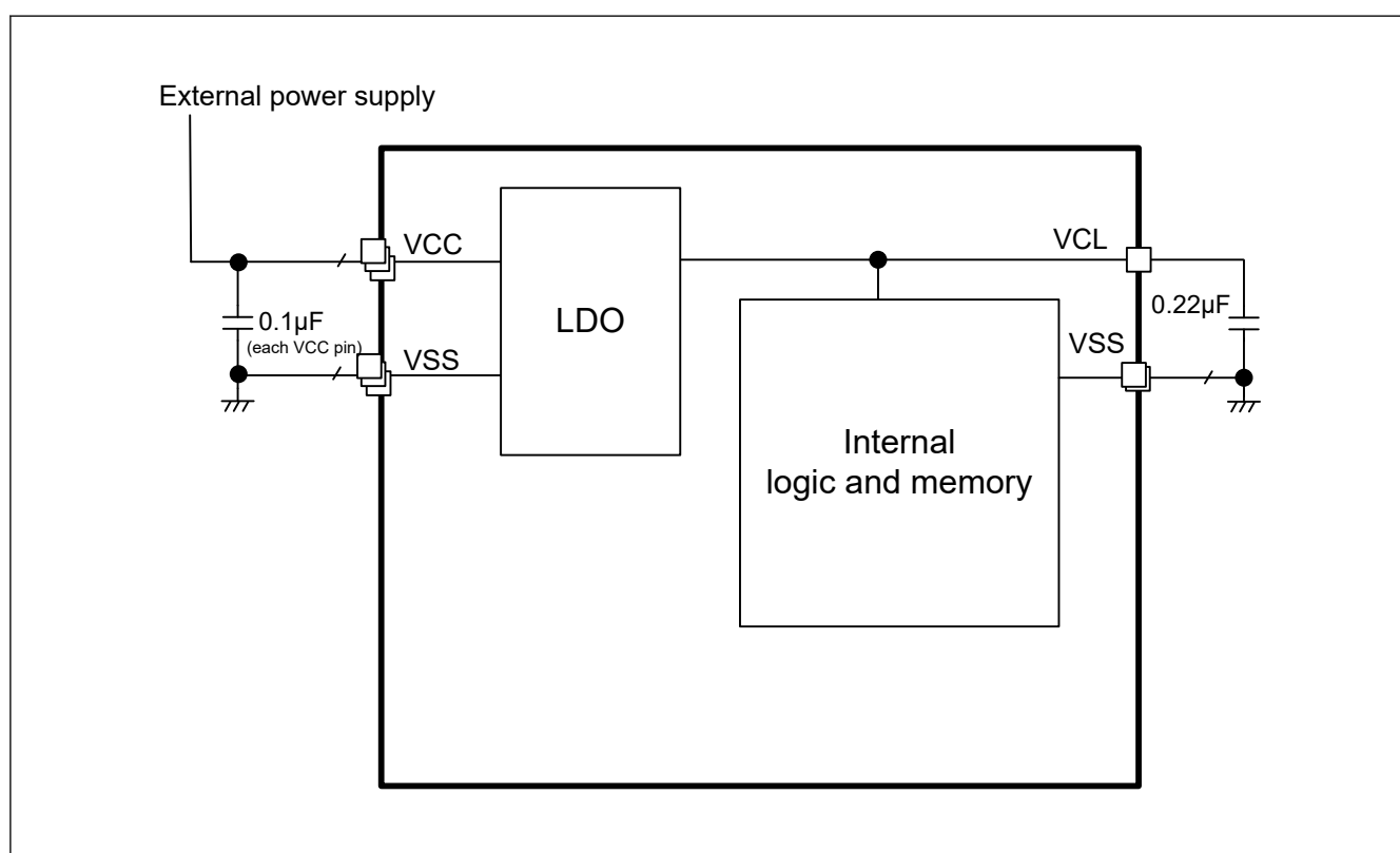
Figure 43.1 LDO mode settings
