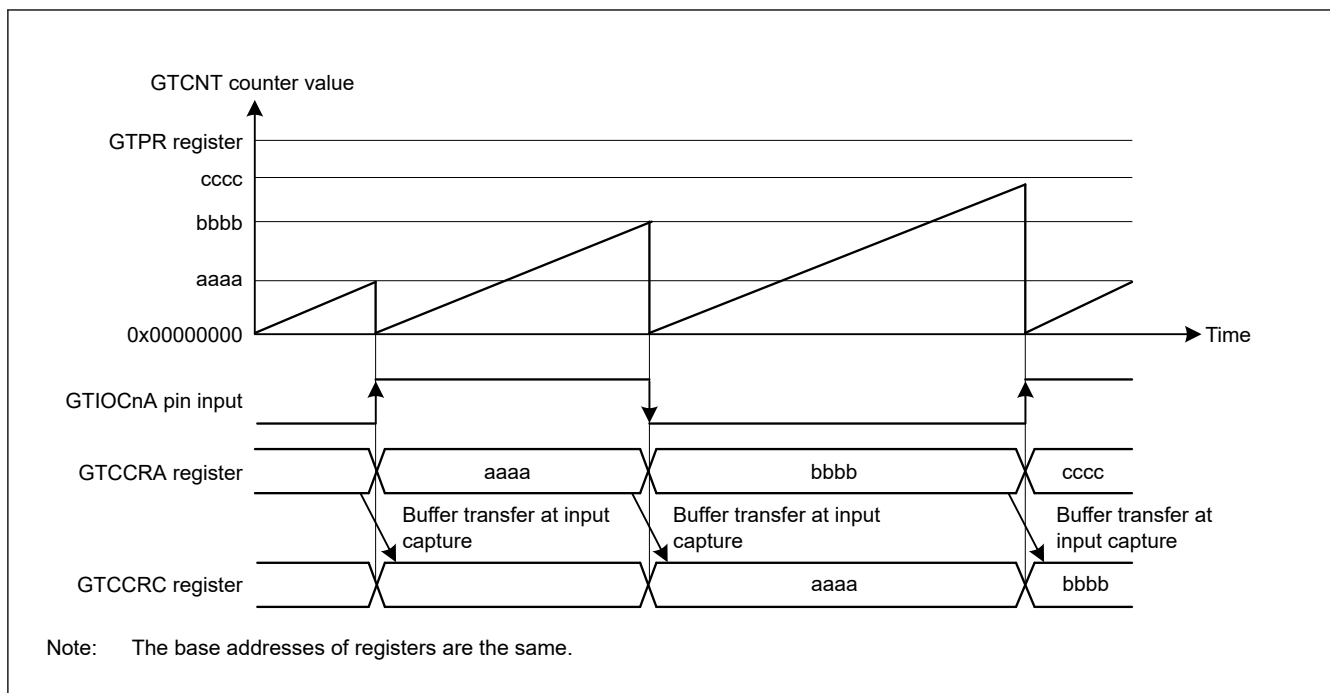
Figure 20.17 Example of GTCRA buffer operation with input capture at both edges of GTIOcNA input, saw waves in up-counting, and GTCNT counter cleared at both edges of GTIOcNA input
