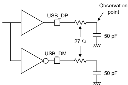
Figure 45.61 Test circuit in full-speed mode
