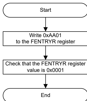
Figure 42.9 Procedure to transition to code flash P/E mode
