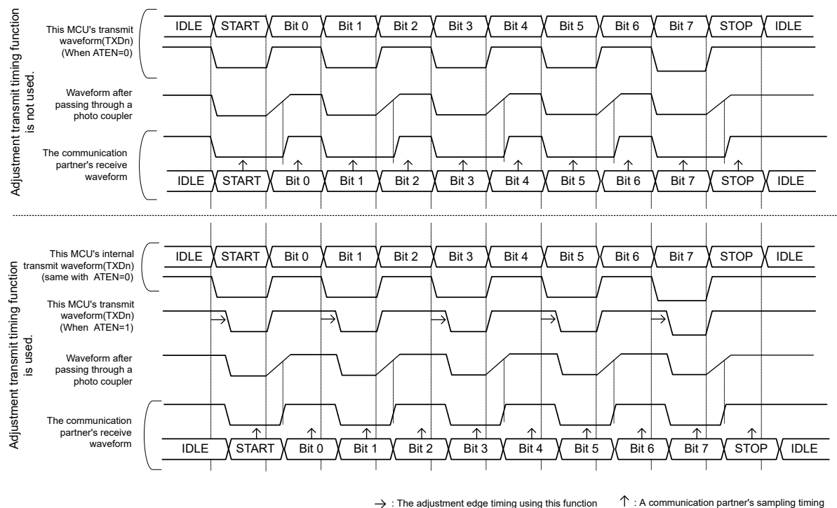
Figure 26.34 The explanation for the transmit waveform through a photo coupler
