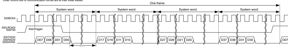
Figure 33.42 TDM format (with padding: system word length > data word length)
