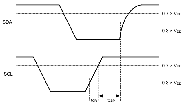
Figure 45.48 I3C STOP condition timing
