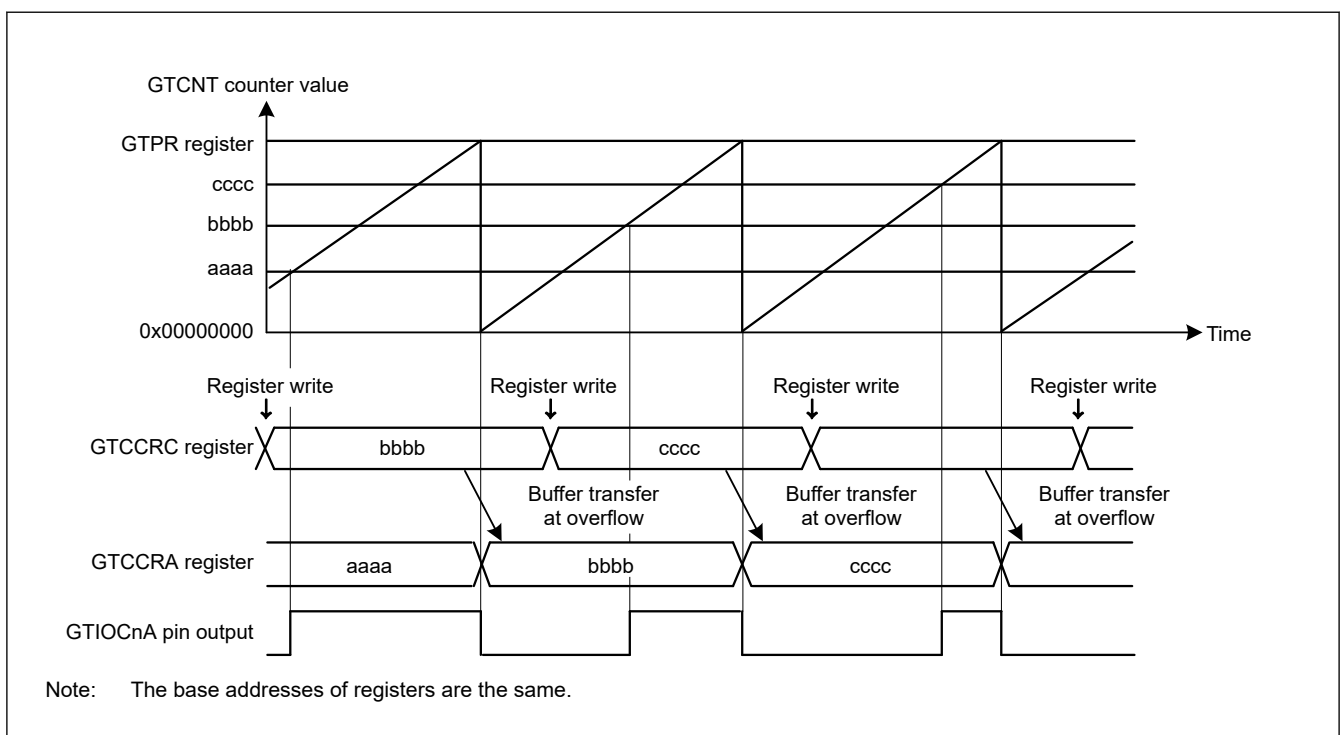
Figure 20.14 Example of GTCCRA buffer operation with output compare, saw waves in up-counting, high output at GTCCRA compare match, and low output at cycle end
