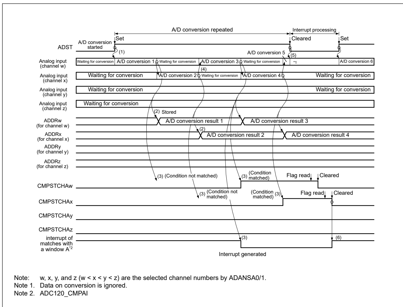
Figure 36.23 Example of compare function operation, when the analog inputs (channel w to z) are compared
