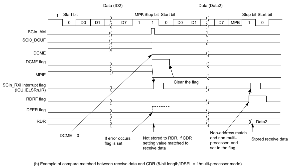
Figure 26.7 Example of address match (2) multi-processor mode
