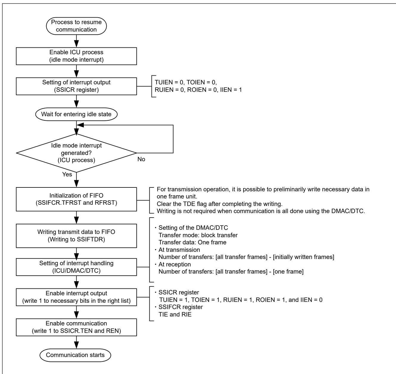
Figure 33.58 Procedure to resume communication (CPU operation procedure)
